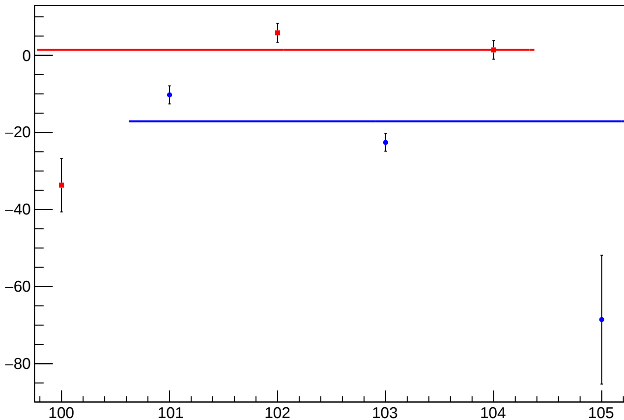
diff_bpm0i02aX_mean vs slug
