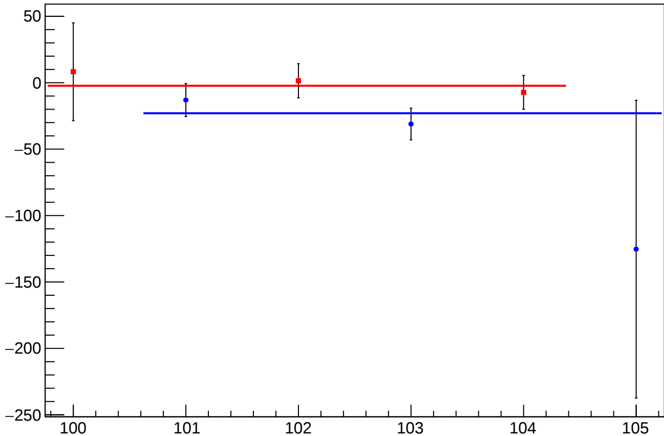
diff_bpm0l02X_mean vs slug
