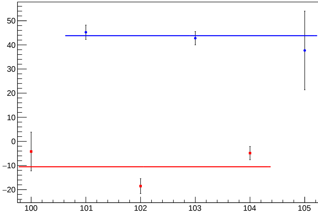
diff_bpm0i01X_mean vs slug
