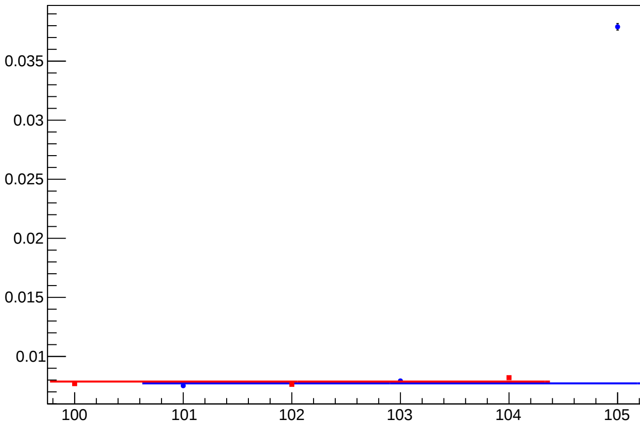
yield_bpm0i02X_rms vs slug
