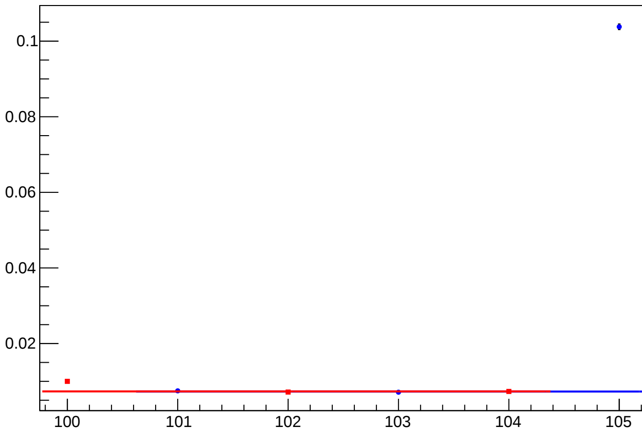
yield_bpm0i02aY_rms vs slug
