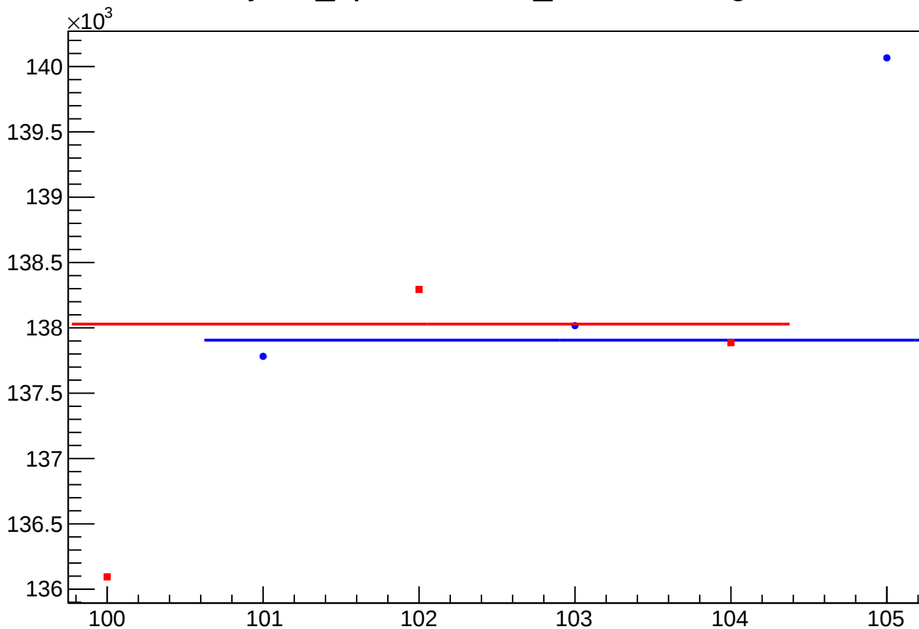
yield_bpm0i02aWS_mean vs slug
