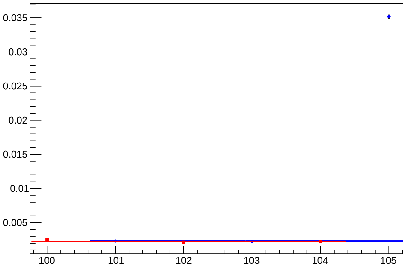
yield_bpm0i01aY_rms vs slug
