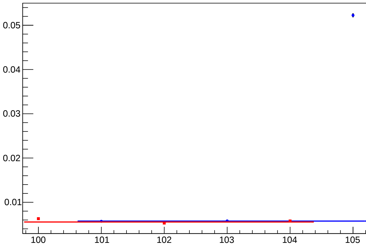
yield_bpm0i01aX_rms vs slug
