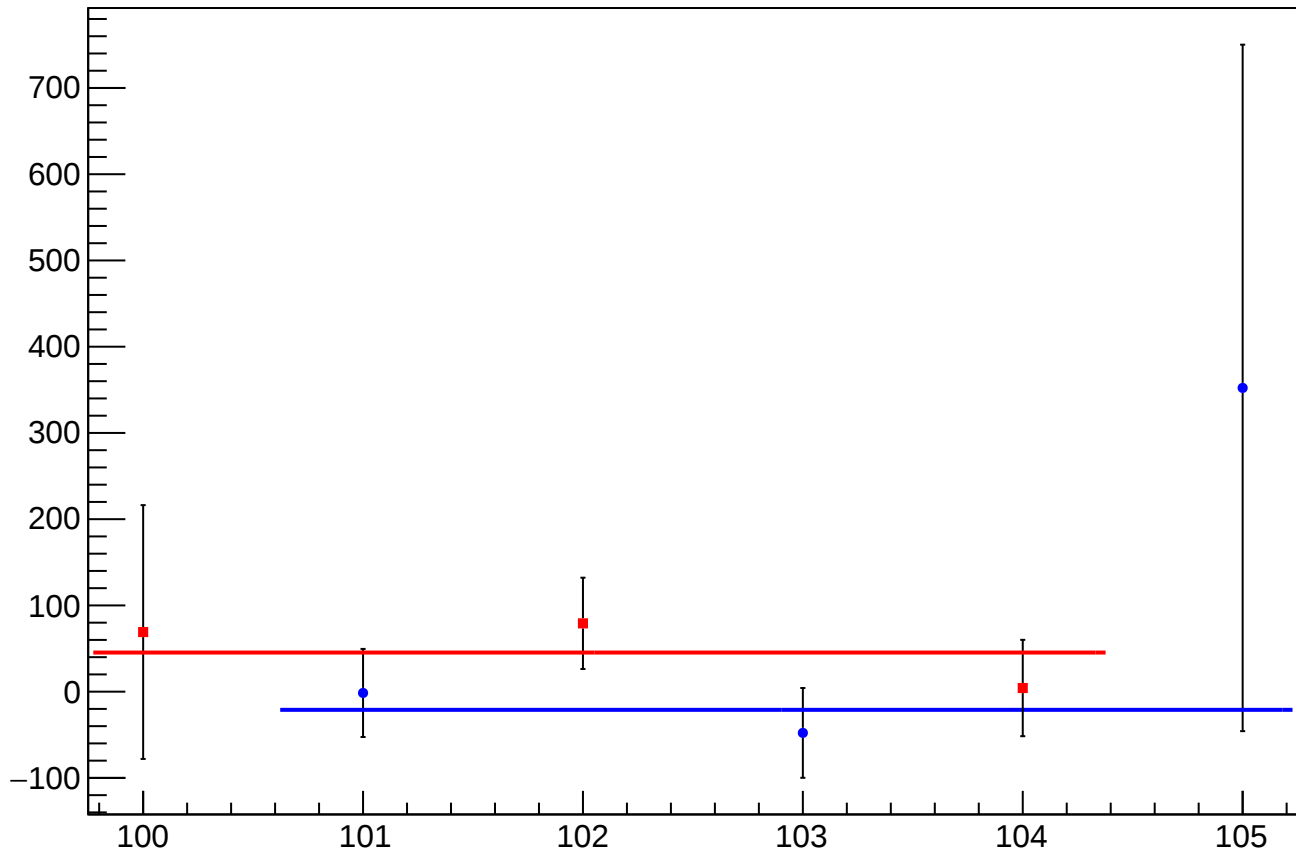
diff_bpm1p03aX_mean vs slug
