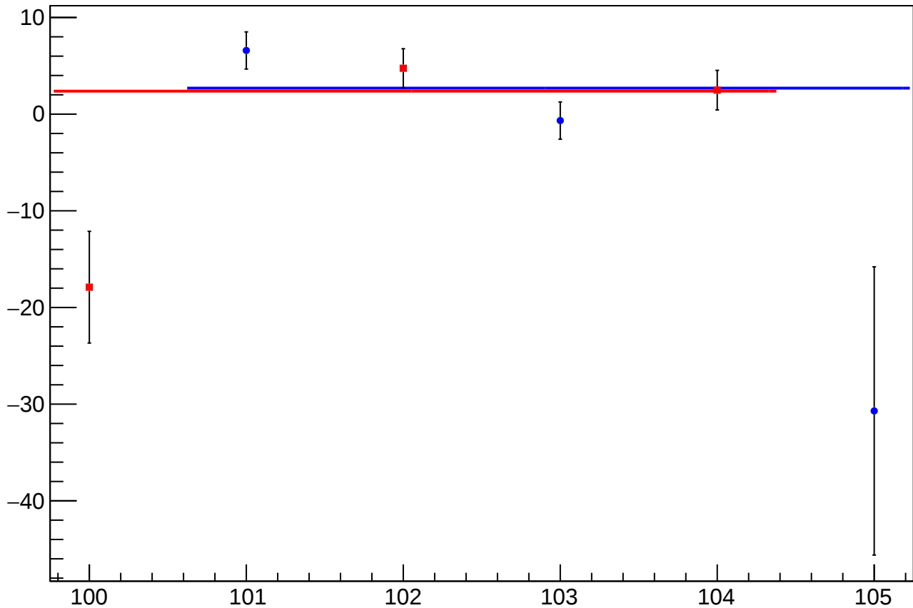
diff_bpm0i02X_mean vs slug
