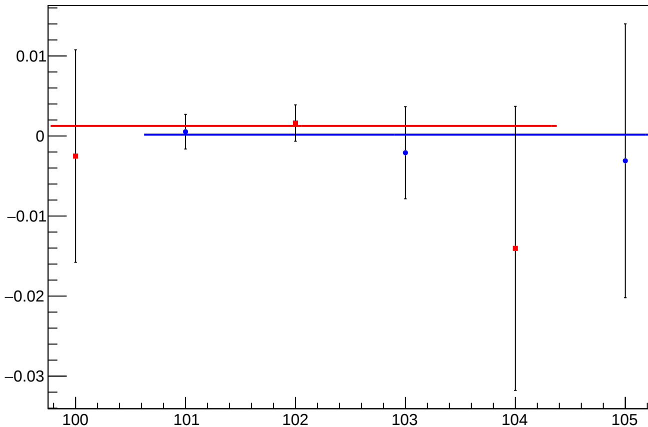
diff_cav4dY_mean vs slug
