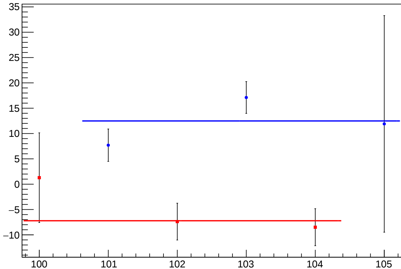
diff_bpm0i07X_mean vs slug
