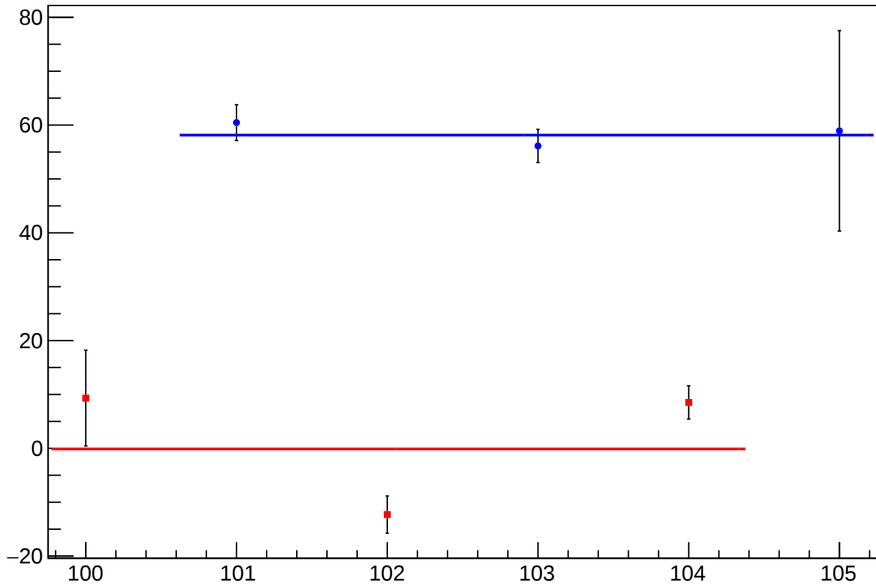
diff_bpm1i06X_mean vs slug
