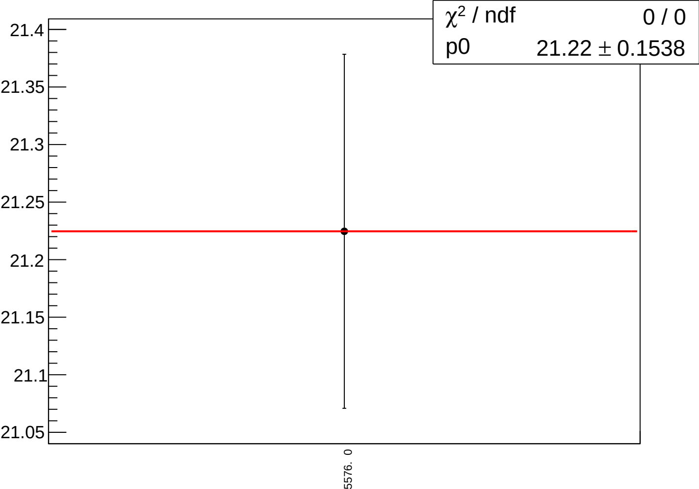
asym_bcm_an_us_ds3_avg_bcm_dg_us_agg_dd_rms vs run
