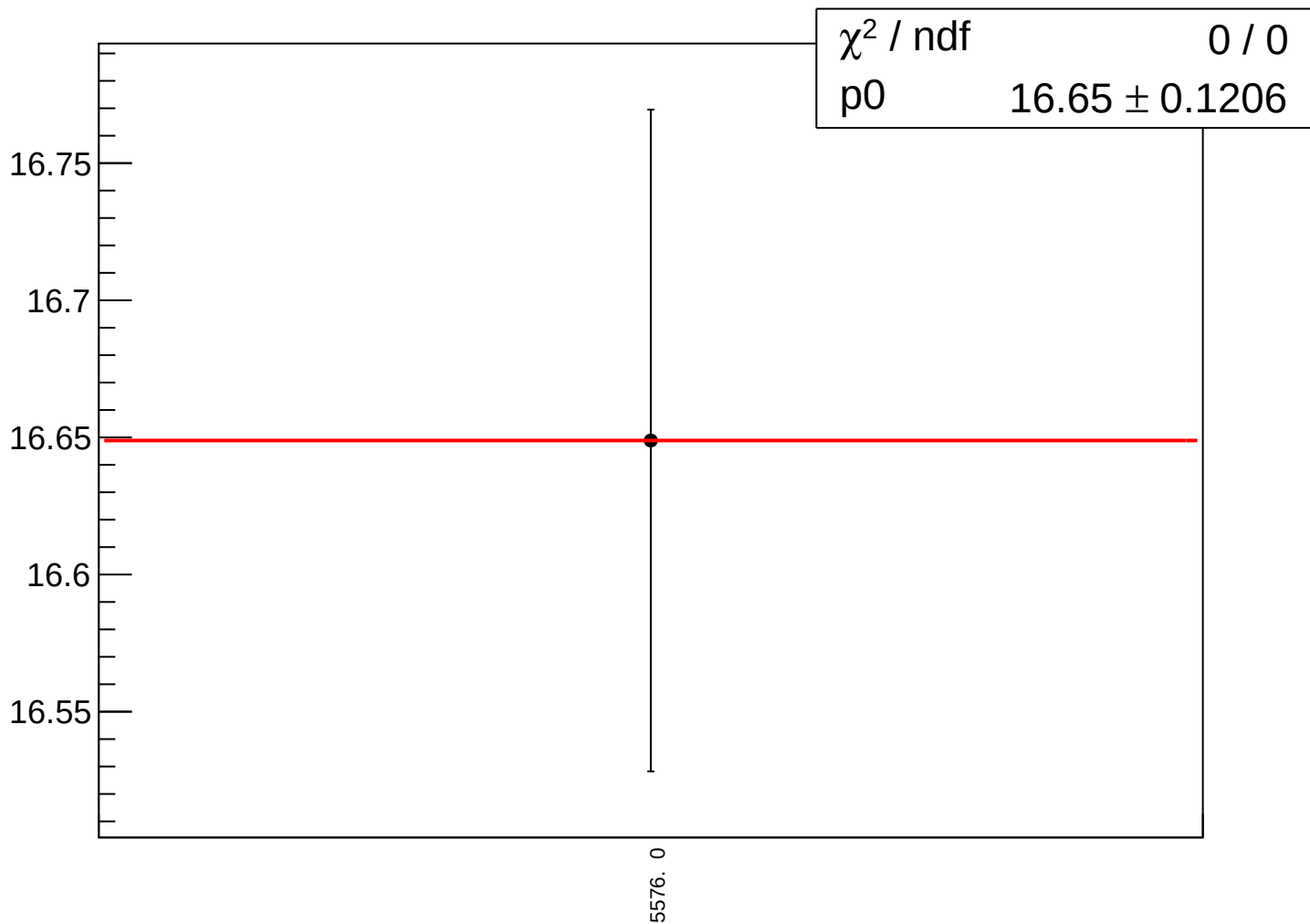
asym_bcm_dg_ds_bcm_an_ds_agg_dd_rms vs run
