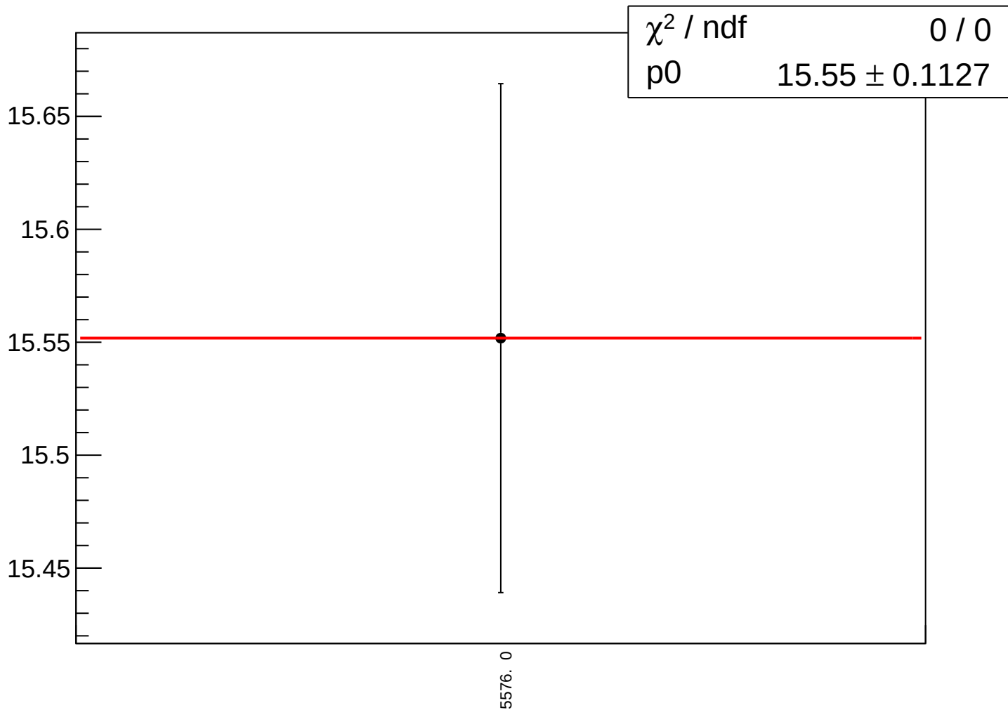
asym_bcm_an_avg_bcm_dg_ds_agg_dd_rms vs run
