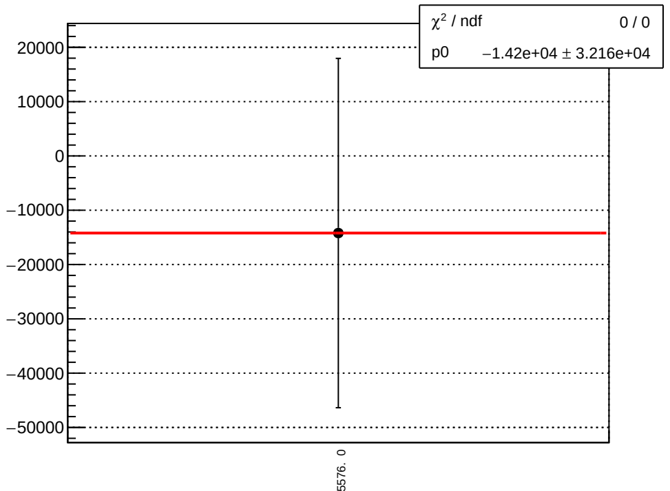
asym_bcm_cav4cQ_bcm_dg_us_agg_dd_mean vs run
