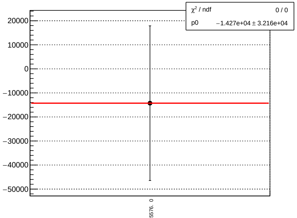
asym_bcm_cav4cQ_bcm_an_ds_agg_dd_mean vs run
