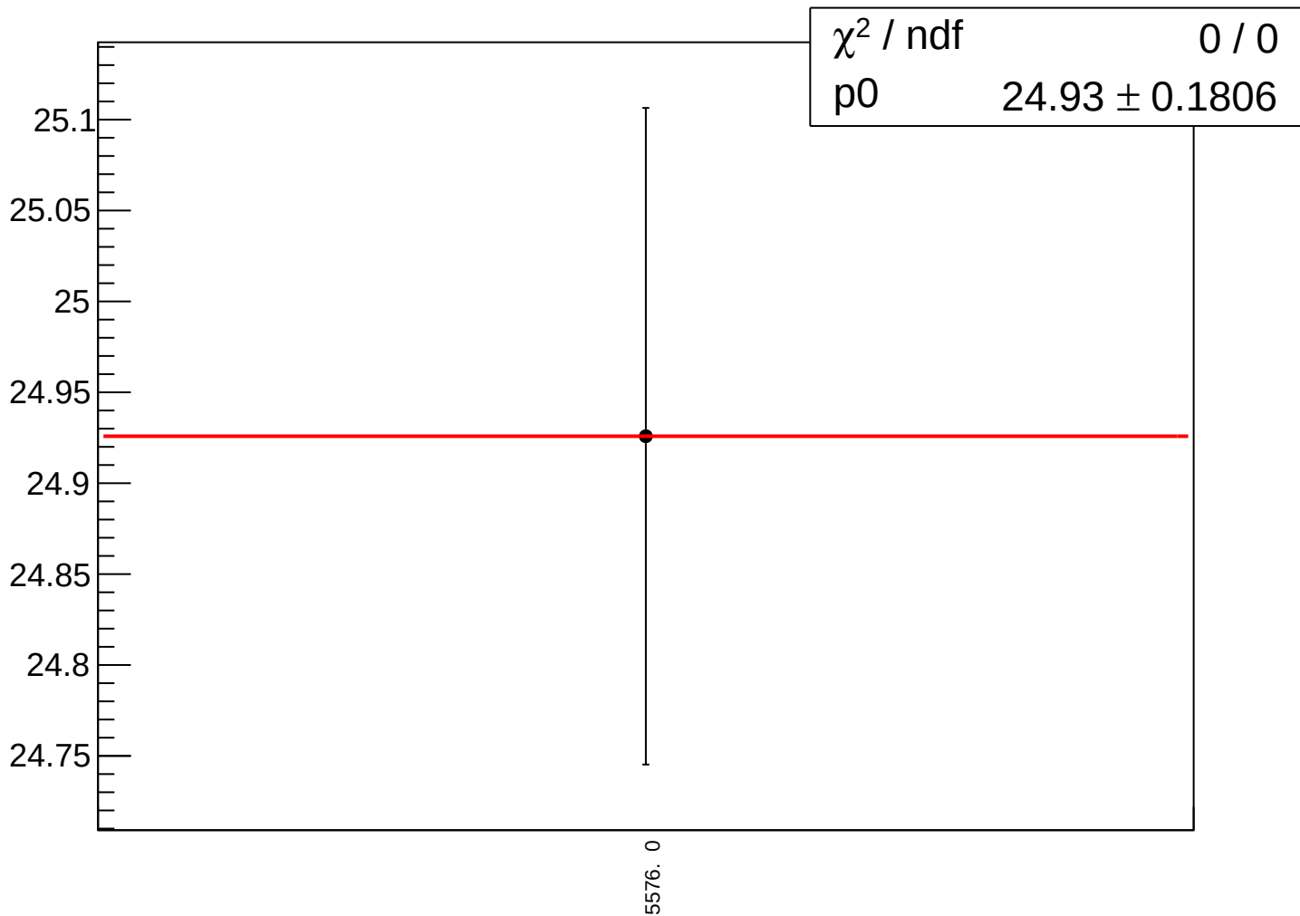
asym_bcm_dg_us_bcm_dg_ds_agg_dd_rms vs run
