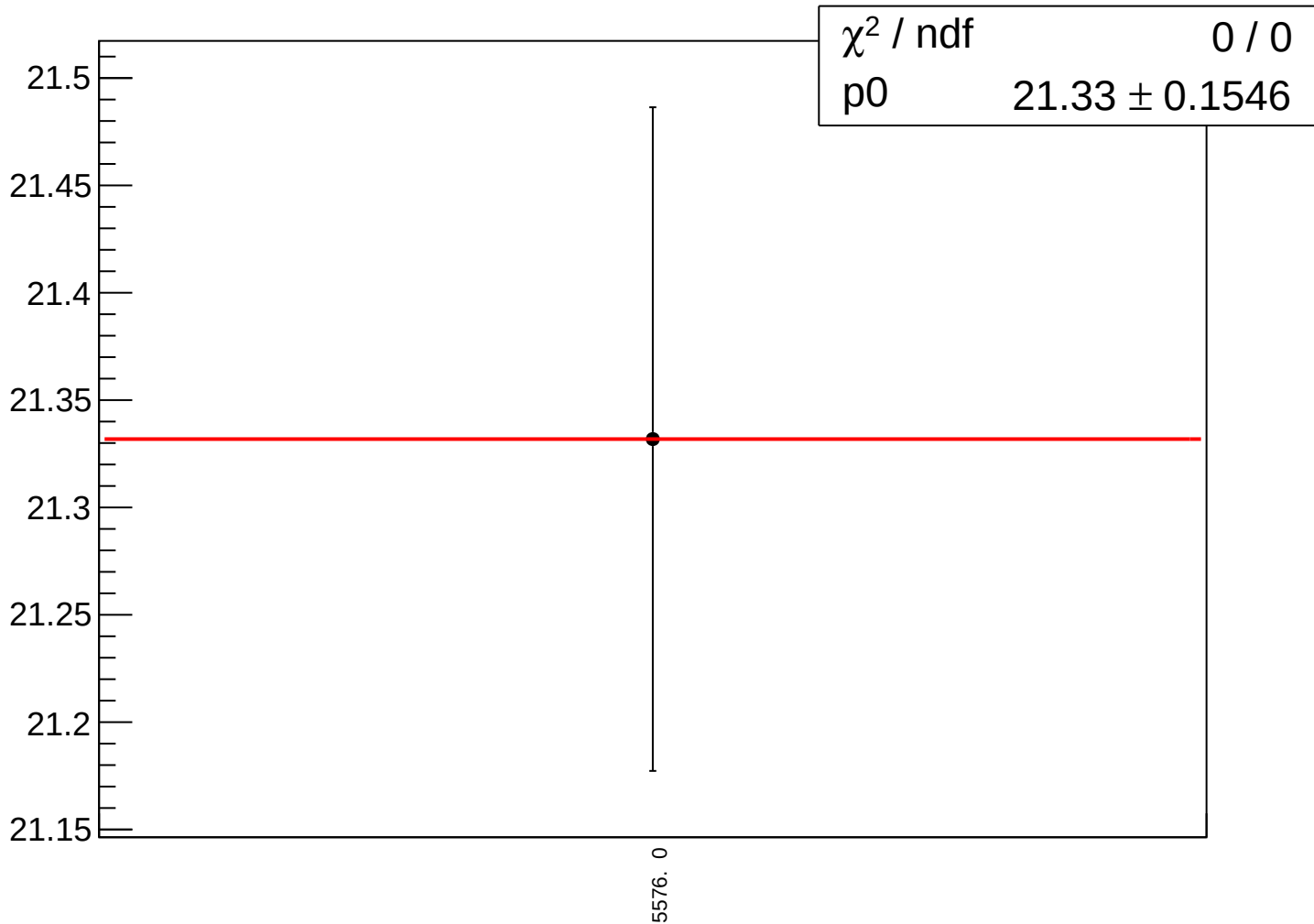
asym_bcm_an_avg_bcm_dg_us_agg_dd_rms vs run
