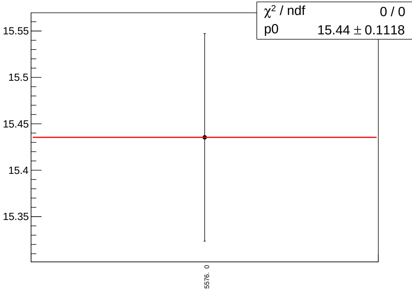
asym_bcm_an_us_ds3_avg_bcm_dg_ds_agg_dd_rms vs run
