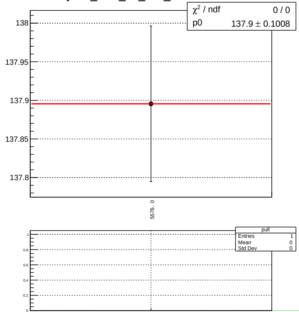
yield_bcm_an_ds3_mean vs run
