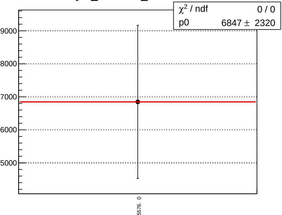
asym_bcm0l02_mean vs run
