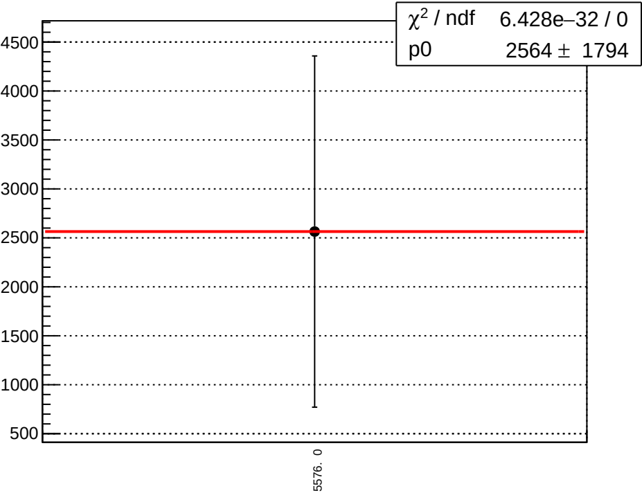
asym_bpm0i02WS_mean vs run
