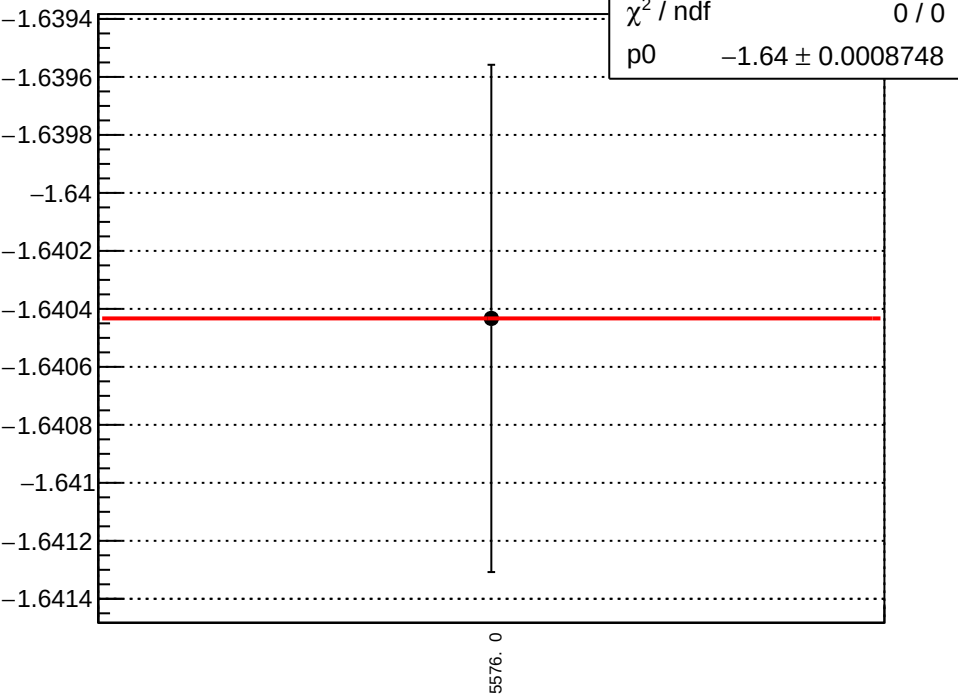
yield_bpm0i05Y_mean vs run
