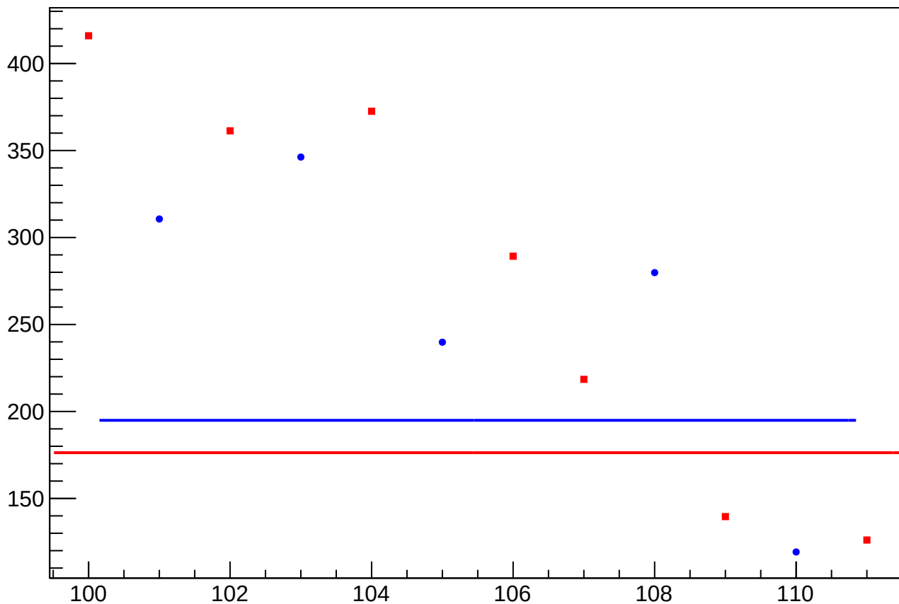
asym_bpm0l04WS_rms vs slug
