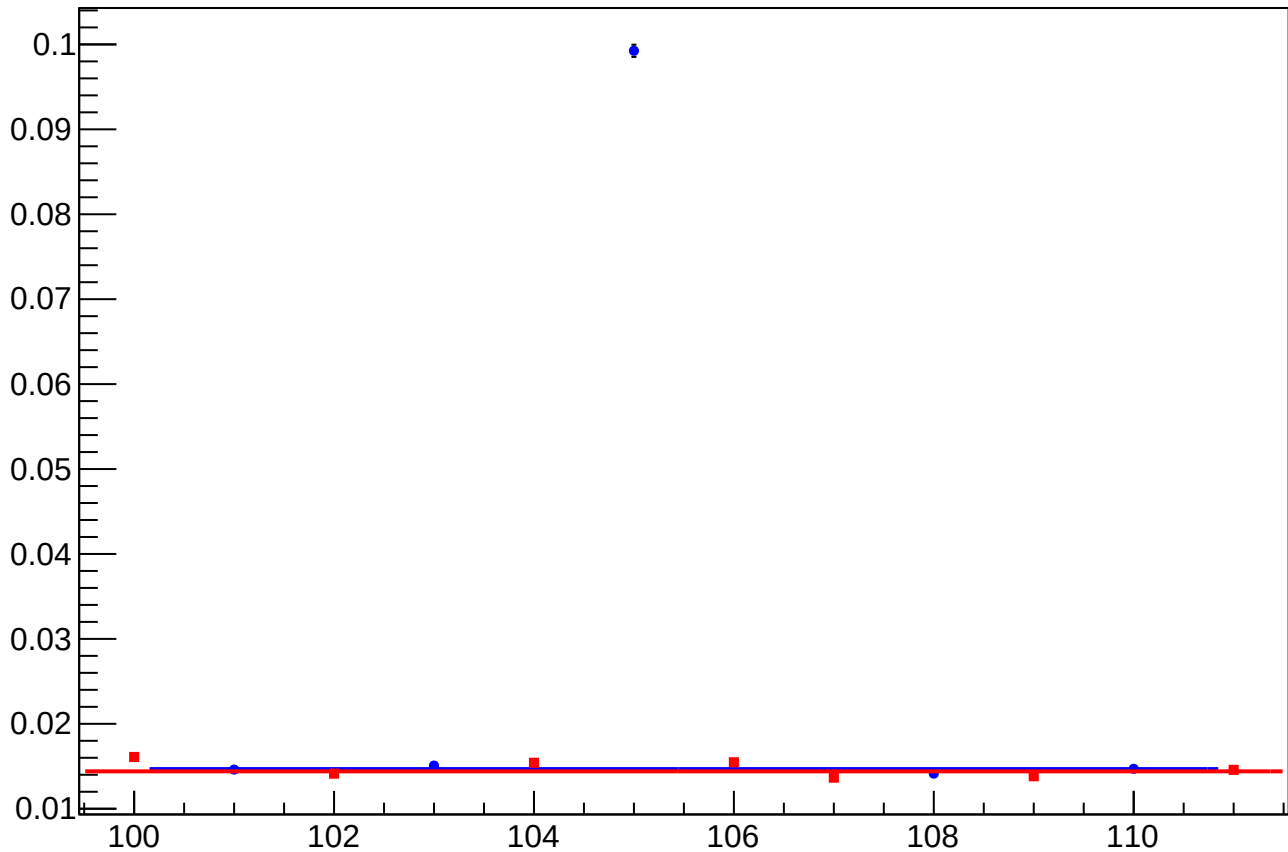
yield_bpm1i06X_rms vs slug
