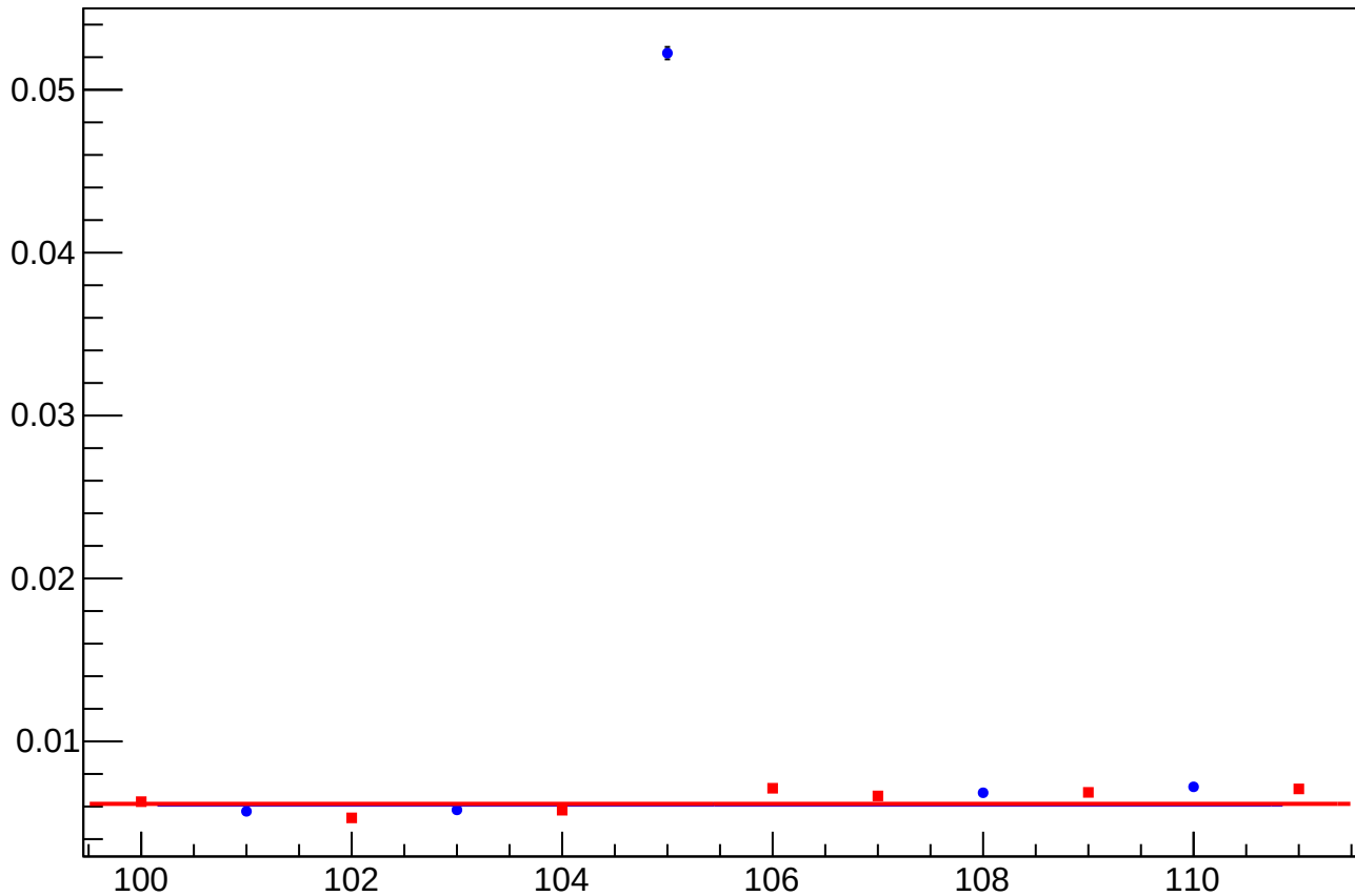
yield_bpm0i01aX_rms vs slug
