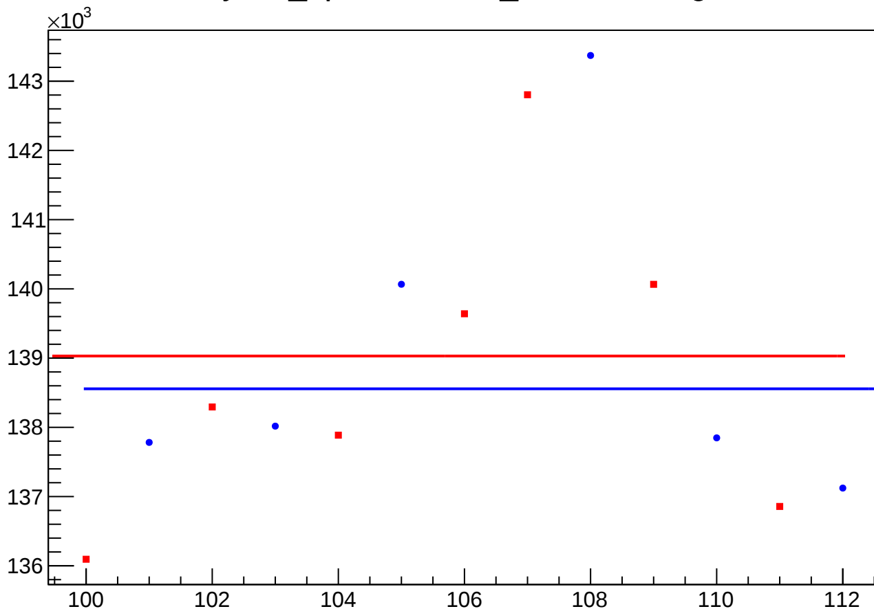
yield_bpm0i02aWS_mean vs slug
