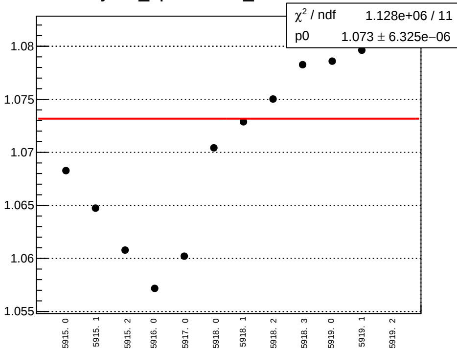
yield_bpm0i01aY_mean vs run
