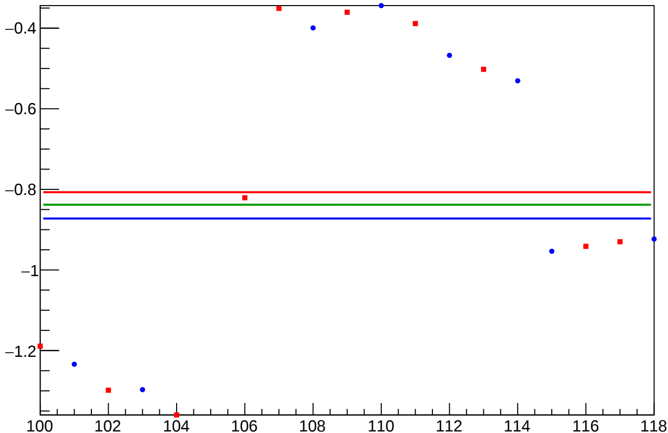
yield_bpm0i01X_mean vs Slug, Sign Corrected
