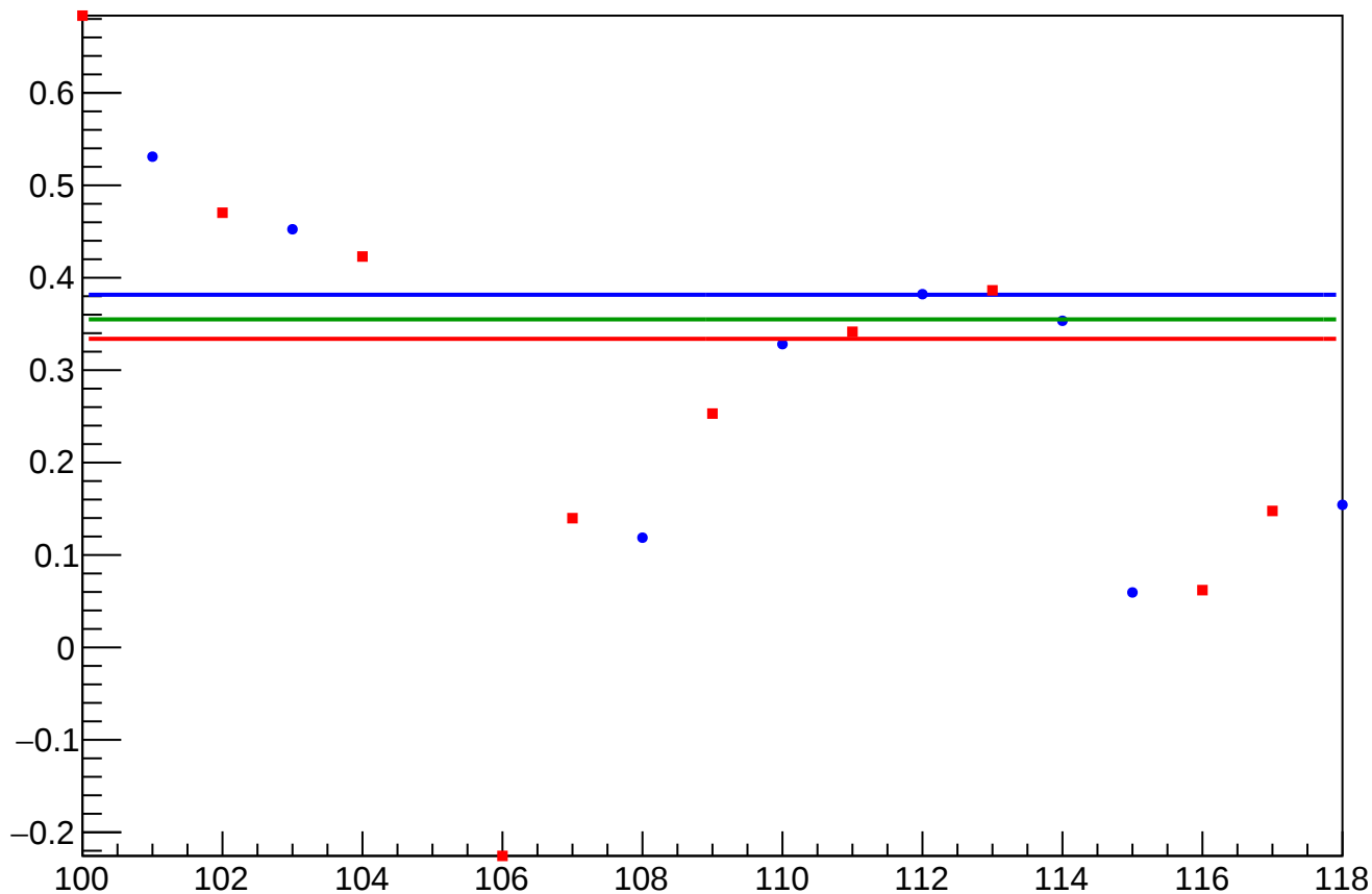
yield_bpm0i07Y_mean vs Slug, Sign Corrected
