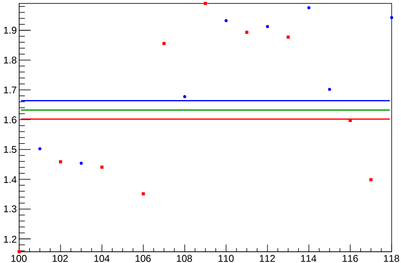
yield_bpm0r05Y_mean vs Slug, Sign Corrected
