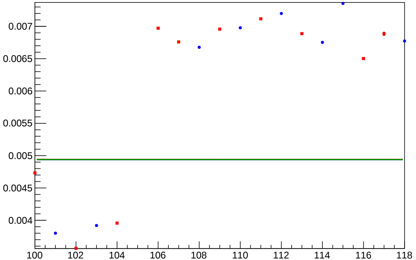
yield_bpm1i06Y_rms vs Slug, Sign Corrected
