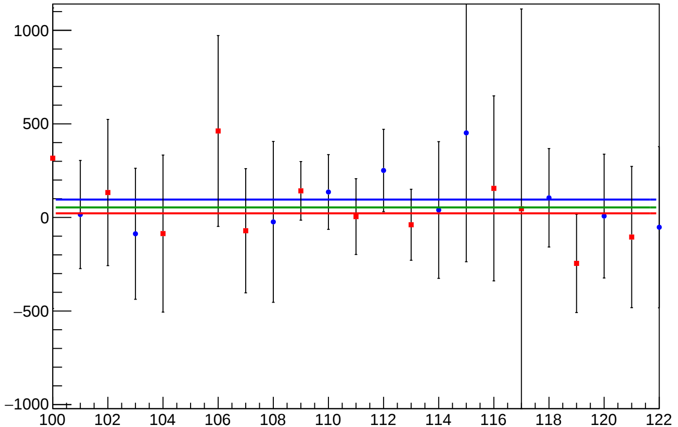
asym_bcm_dg_ds_bcm_an_us_agg_avg_mean vs Slug, Sign Corrected
