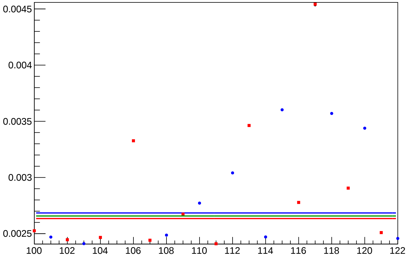
yield_bpm0l06Y_rms vs Slug, Sign Corrected
