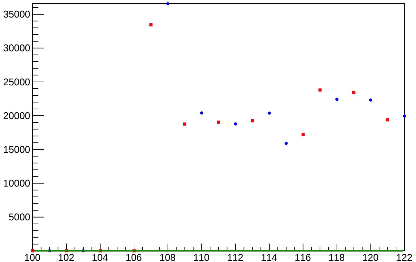
diff_cav4bX_rms vs Slug, Sign Corrected
