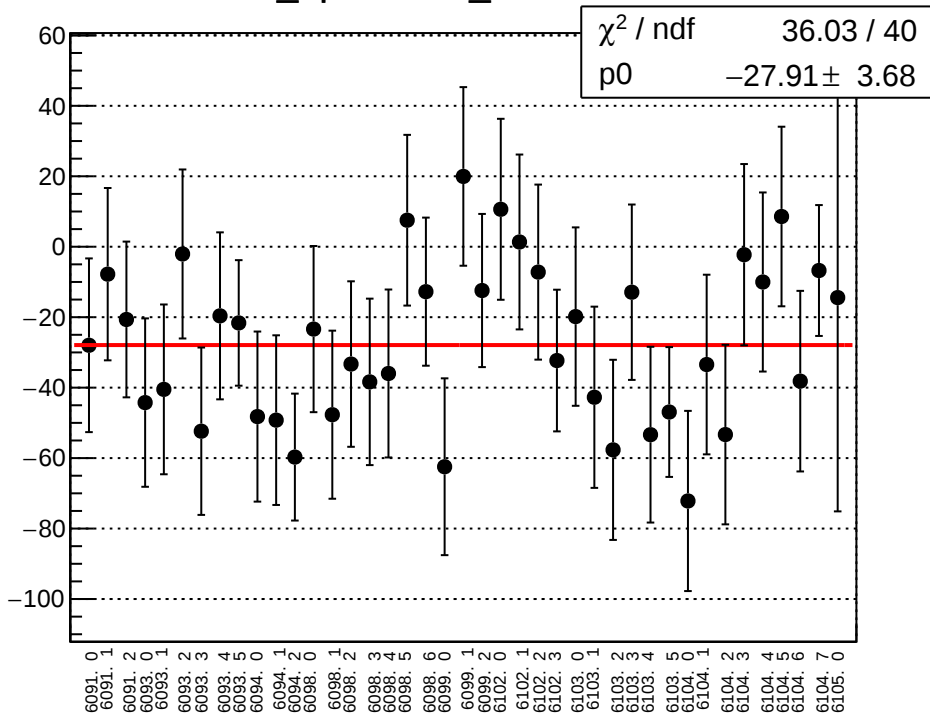
diff_bpm0105Y_mean vs run
