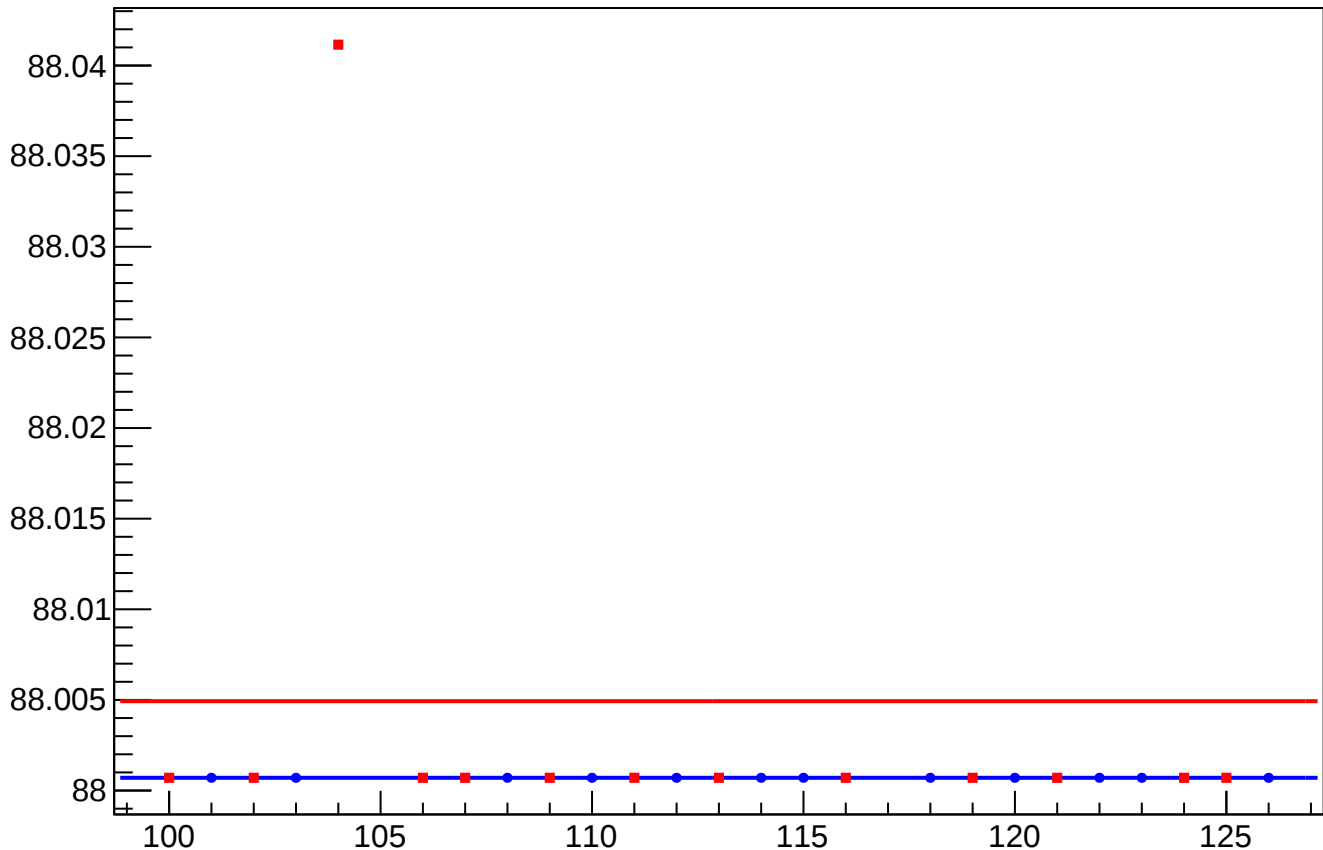
epics_VWienAngles_mean vs Slug, Sign Corrected
