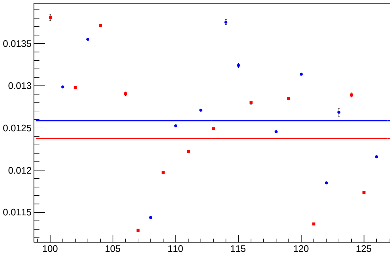
yield_bpm0i02aX_rms vs Slug, Sign Corrected
