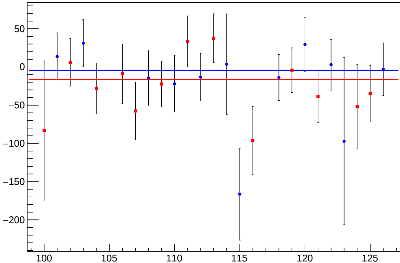
asym_bcm_an_us_ds3_avg_bcm_dg_us_agg_dd_mean vs Slug, Sign Corrected
