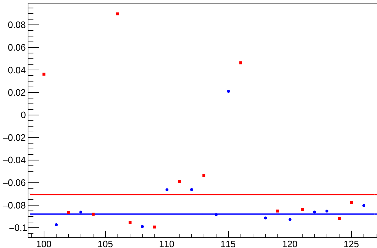
yield_bpm0l09Y_mean vs Slug, Sign Corrected
