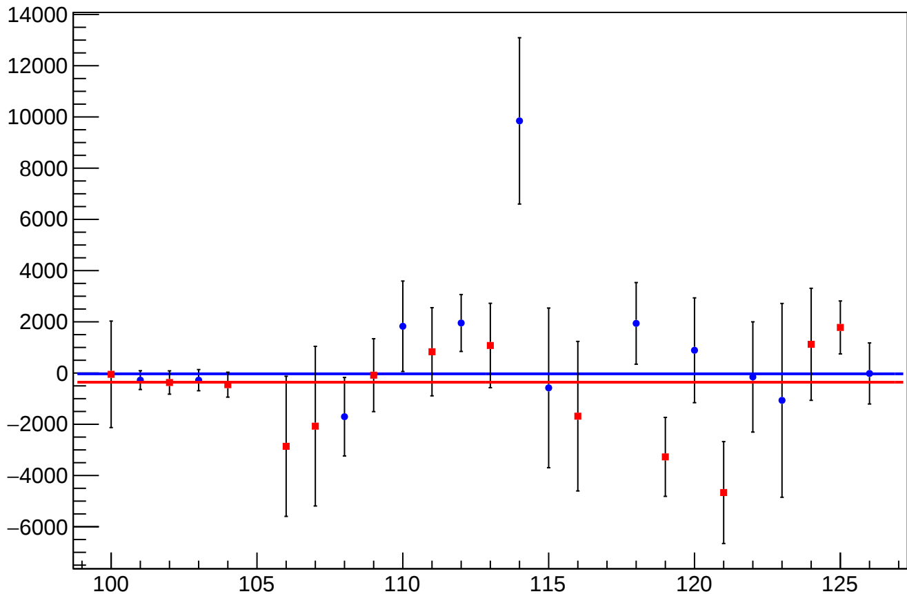
asym_bpm0l03WS_mean vs Slug, Sign Corrected
