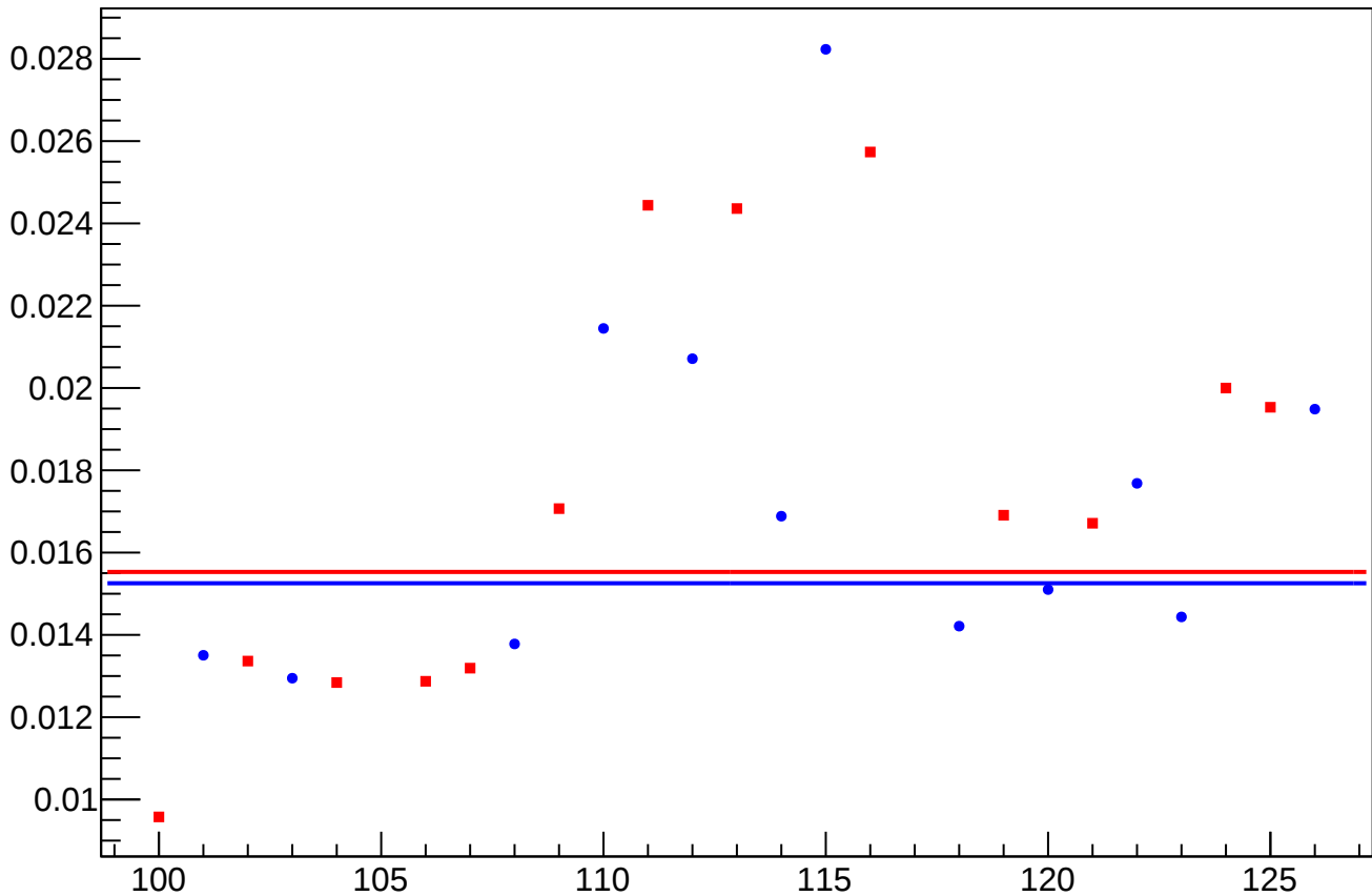
yield_bpm0r05Y_rms vs Slug, Sign Corrected
