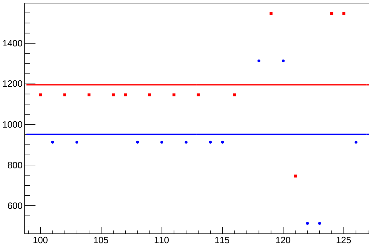
epics_RTPAPOSUCNTs_mean vs Slug, Sign Corrected
