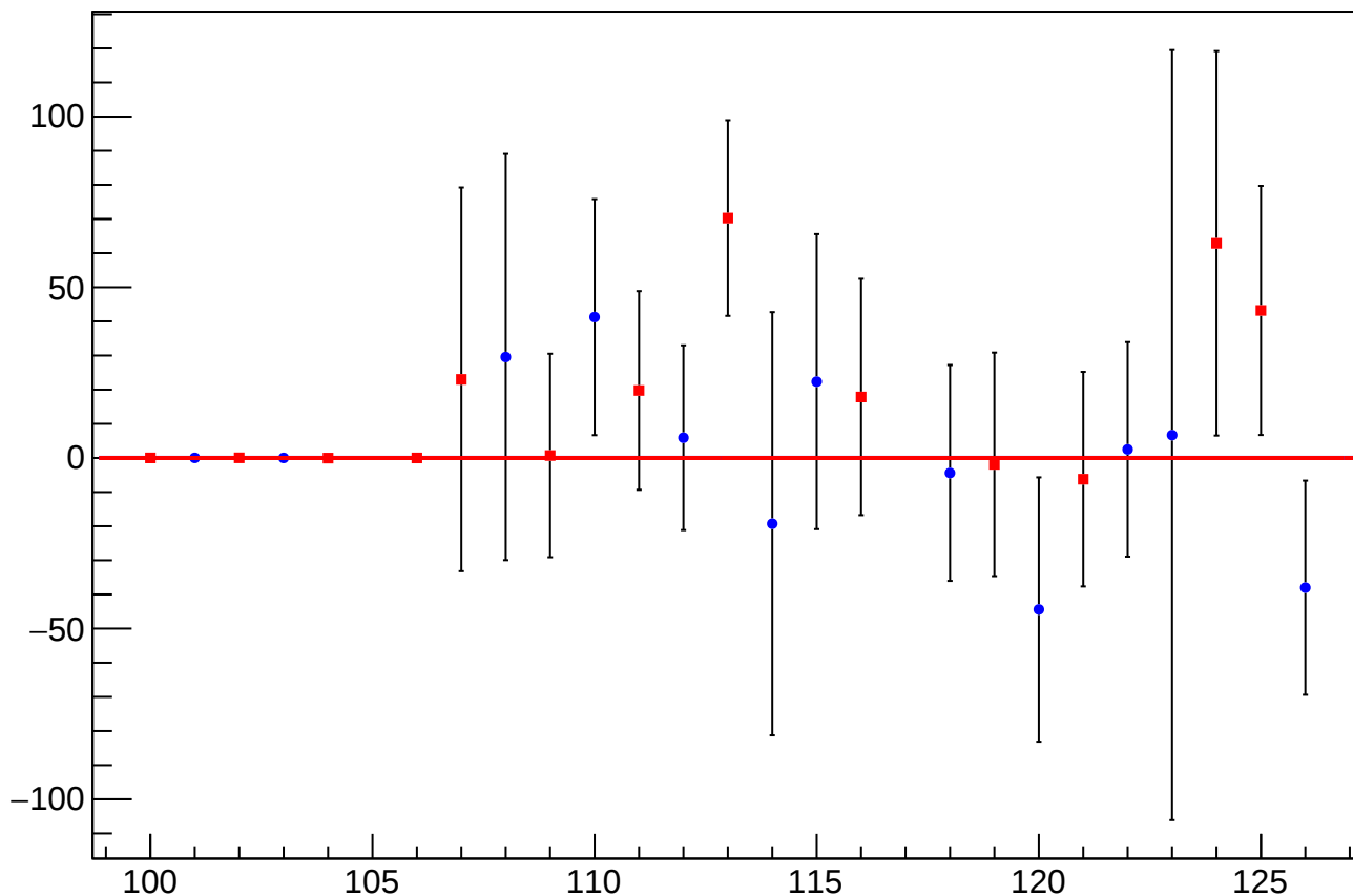
diff_cav4bX_mean vs Slug, Sign Corrected
