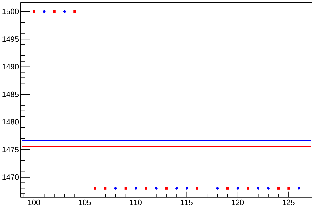
epics_psub_pl_poss_mean vs Slug, Sign Corrected
