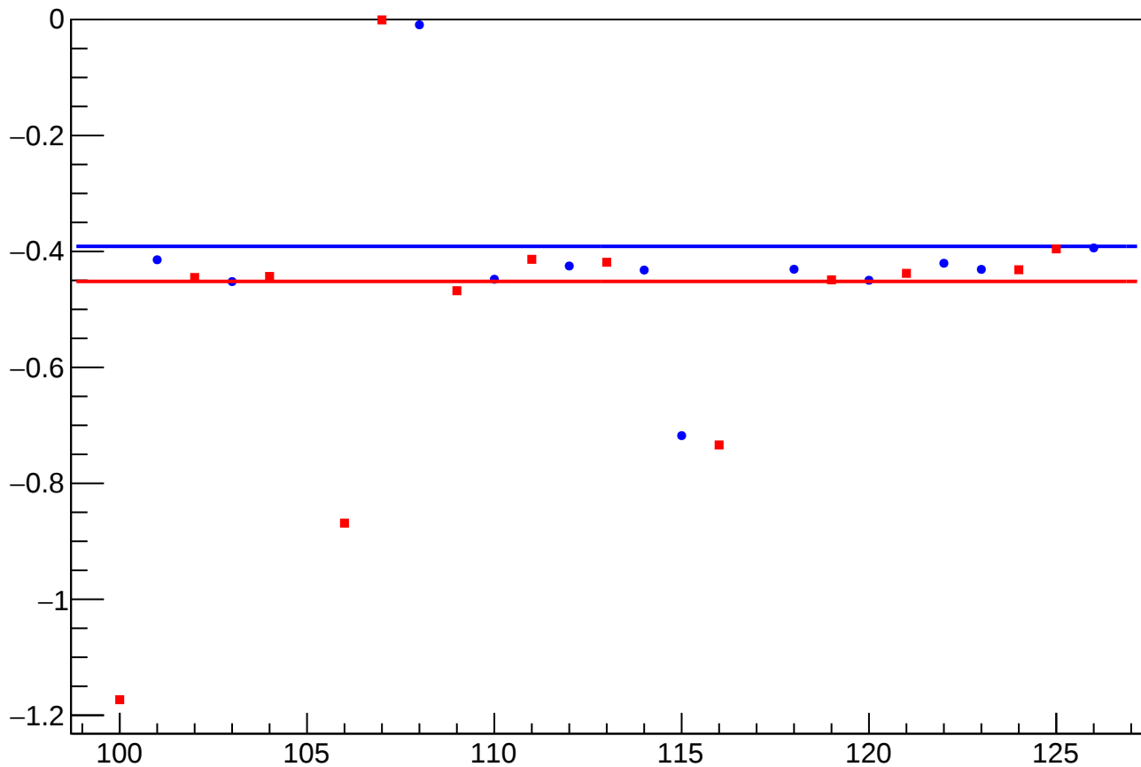
yield_bpm0l07X_mean vs Slug, Sign Corrected
