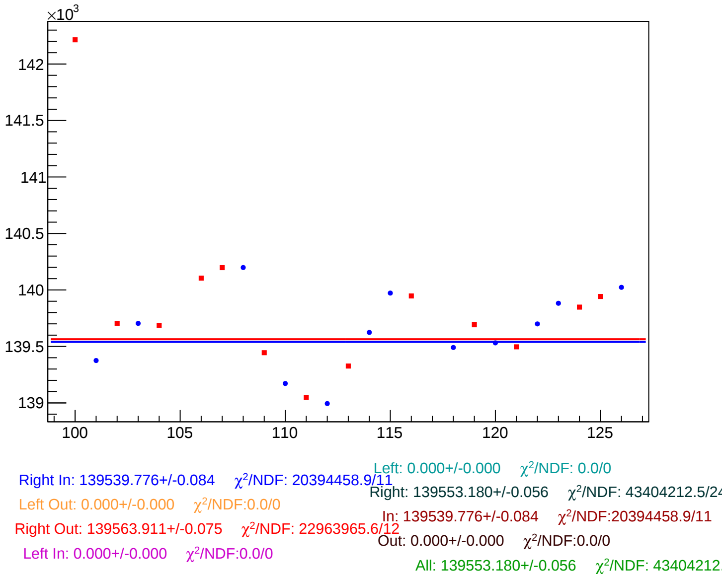
yield_bpm0l09WS_mean vs Slug, Sign Corrected
