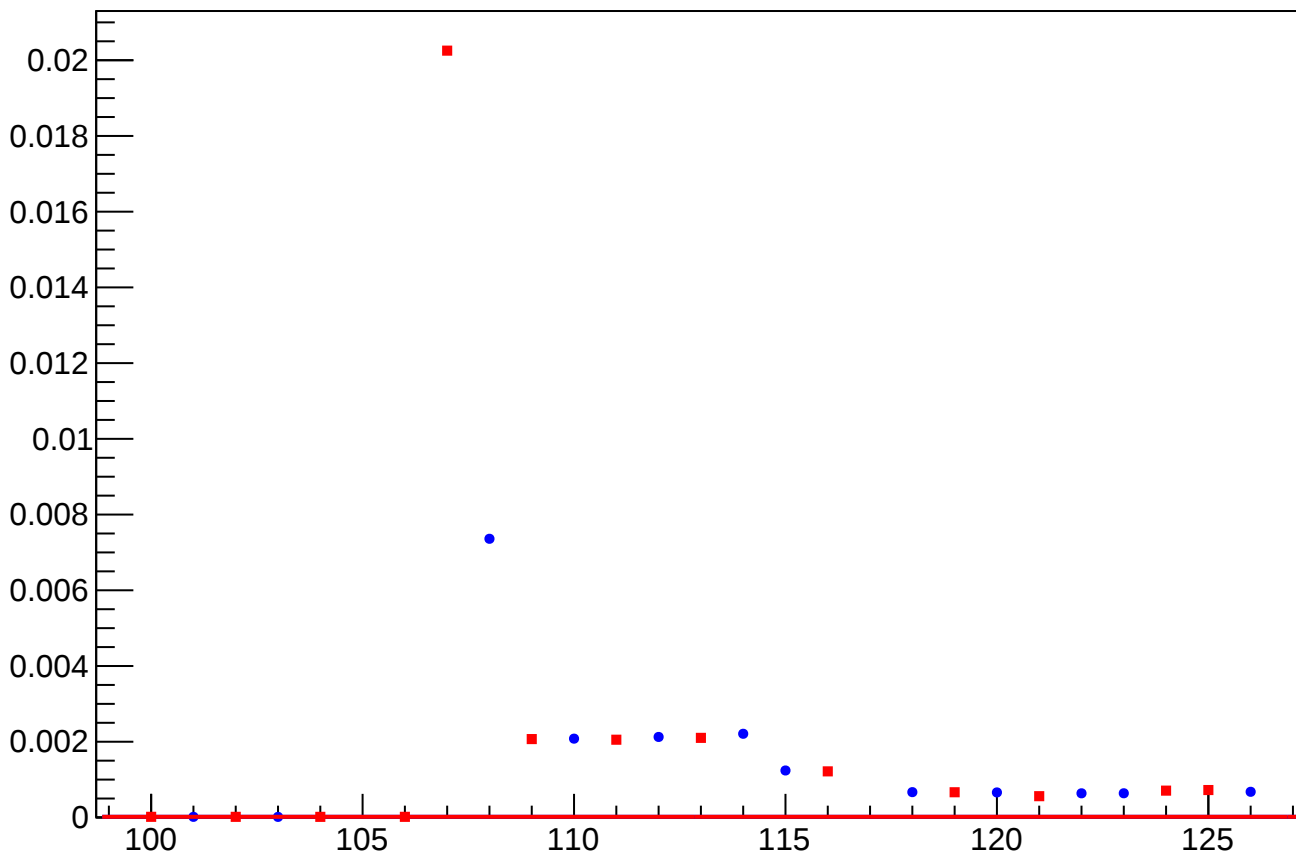
yield_cav4dY_rms vs Slug, Sign Corrected
