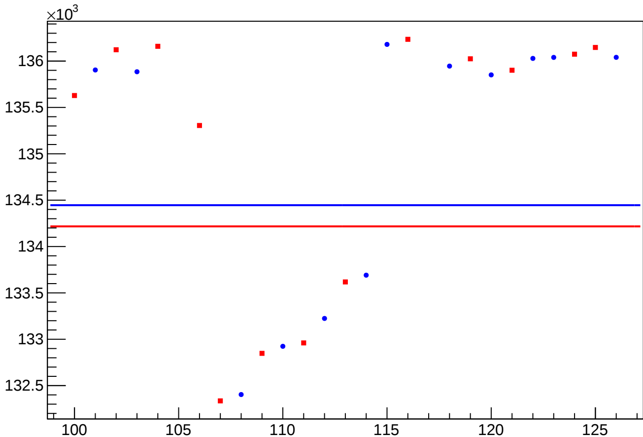
yield_bpm1i04WS_mean vs Slug, Sign Corrected
