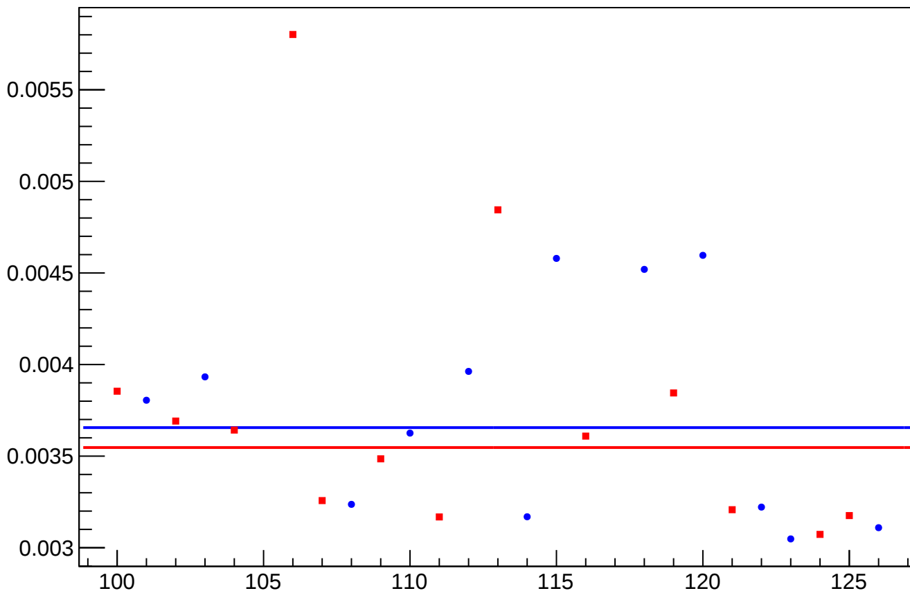
yield_bpm0l04Y_rms vs Slug, Sign Corrected
