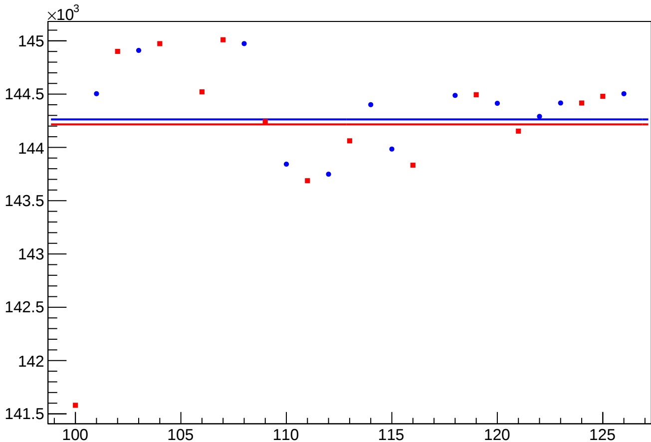
yield_bpm0l08WS_mean vs Slug, Sign Corrected
