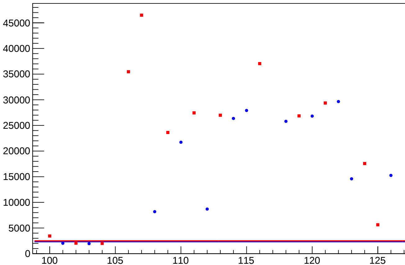
diff_bpm0l03Y_rms vs Slug, Sign Corrected
