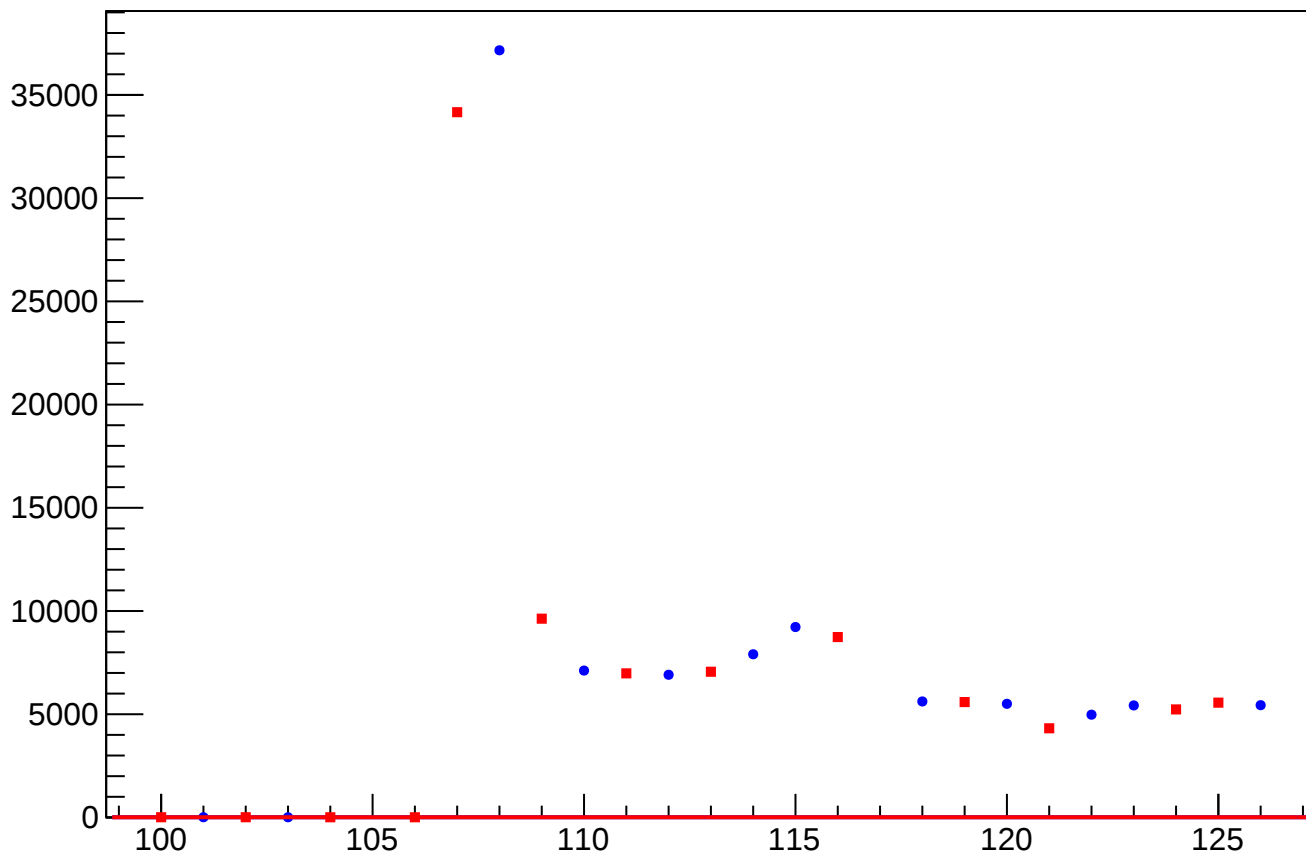
diff_cav4bY_rms vs Slug, Sign Corrected
