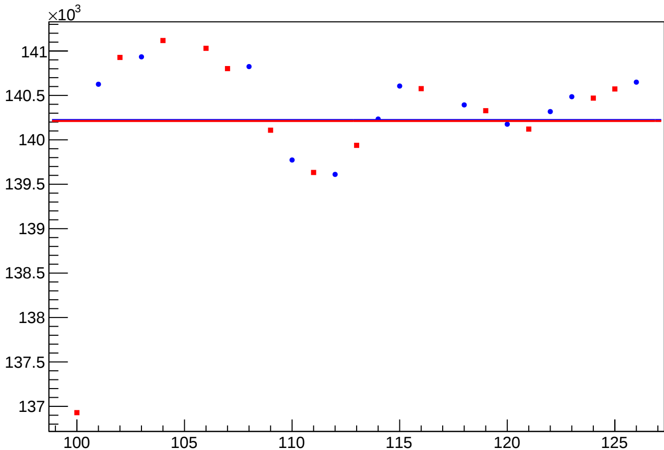
yield_bpm0l10WS_mean vs Slug, Sign Corrected
