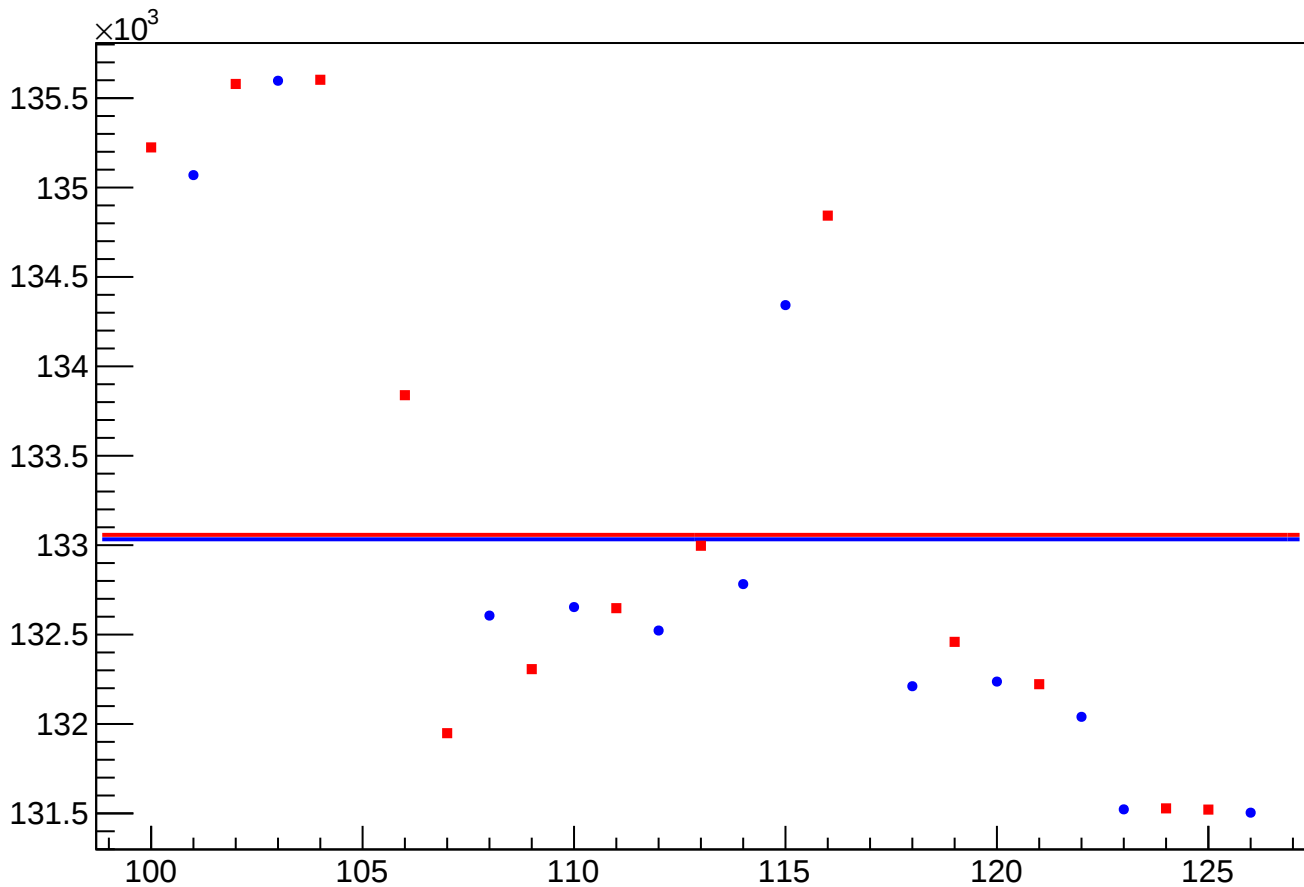
yield_bpm0r05WS_mean vs Slug, Sign Corrected
