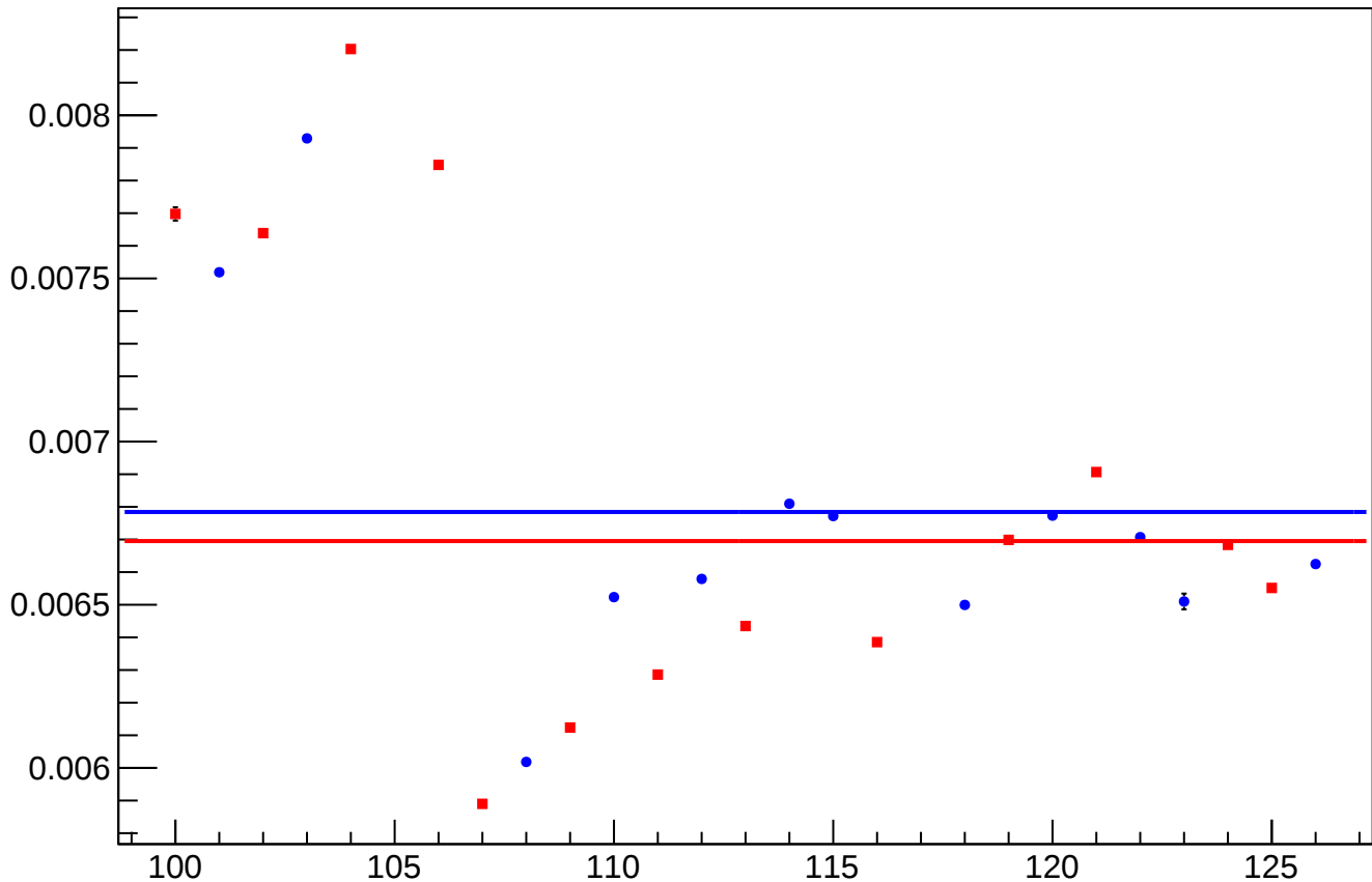
yield_bpm0i02X_rms vs Slug, Sign Corrected
