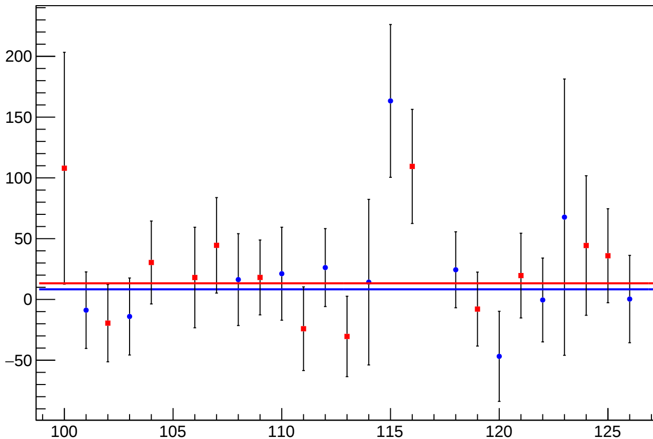
asym_bcm_dg_us_bcm_an_us_agg_dd_mean vs Slug, Sign Corrected
