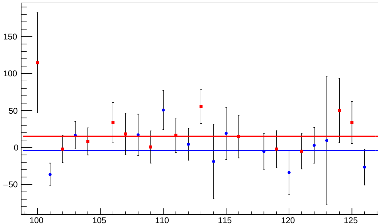
diff_bpm4aX_mean vs Slug, Sign Corrected
