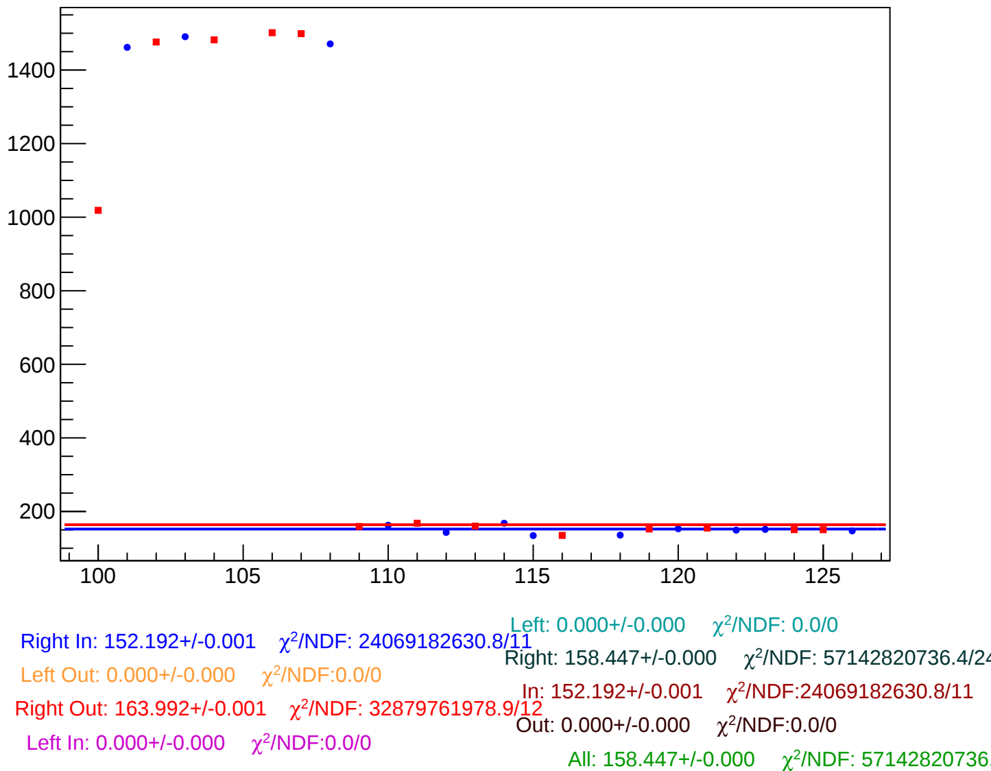
yield_bcm0l02_mean vs Slug, Sign Corrected
