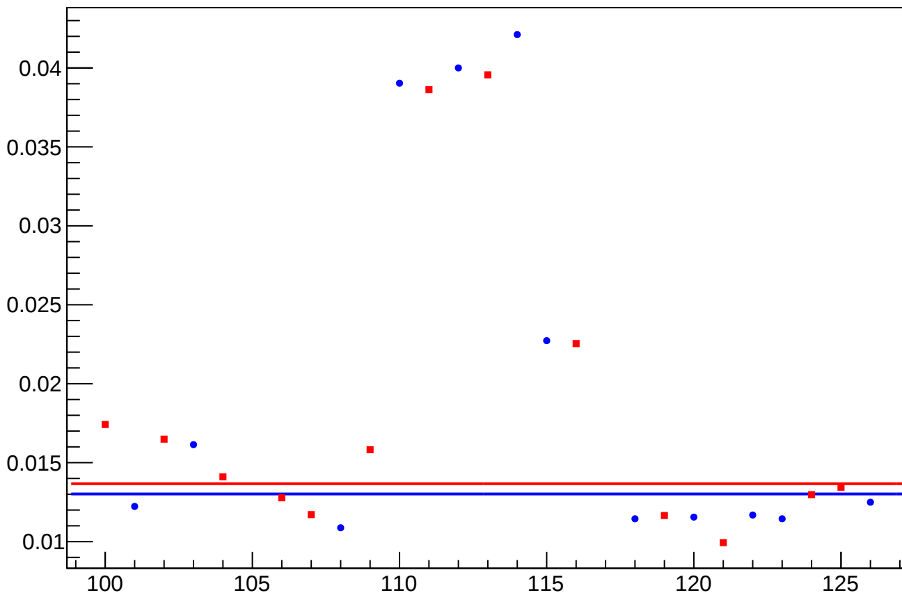
yield_bpm4ecY_rms vs Slug, Sign Corrected
