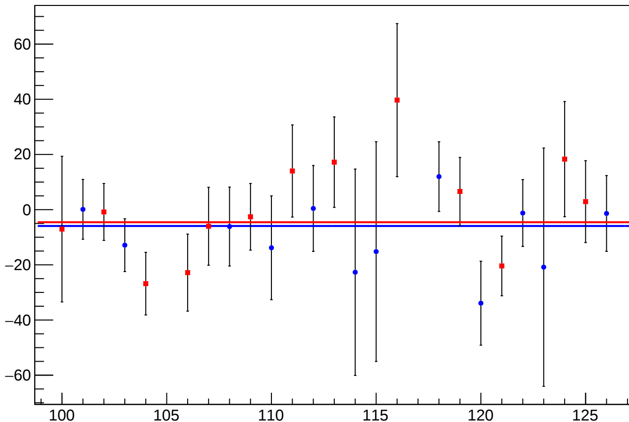
diff_bpm4acY_mean vs Slug, Sign Corrected
