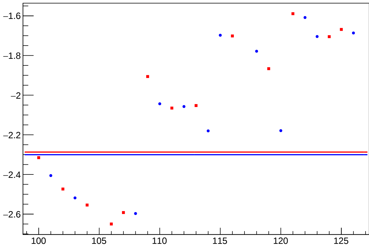
yield_bpm0i05X_mean vs Slug, Sign Corrected
