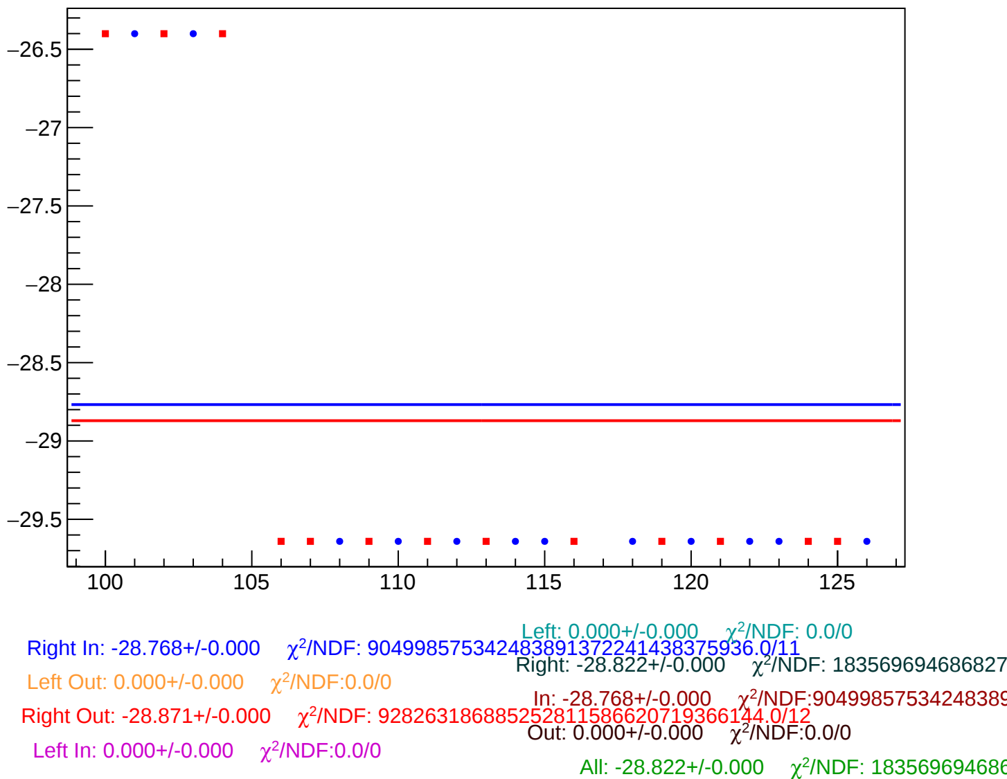
epics_HWienAngles_mean vs Slug, Sign Corrected
