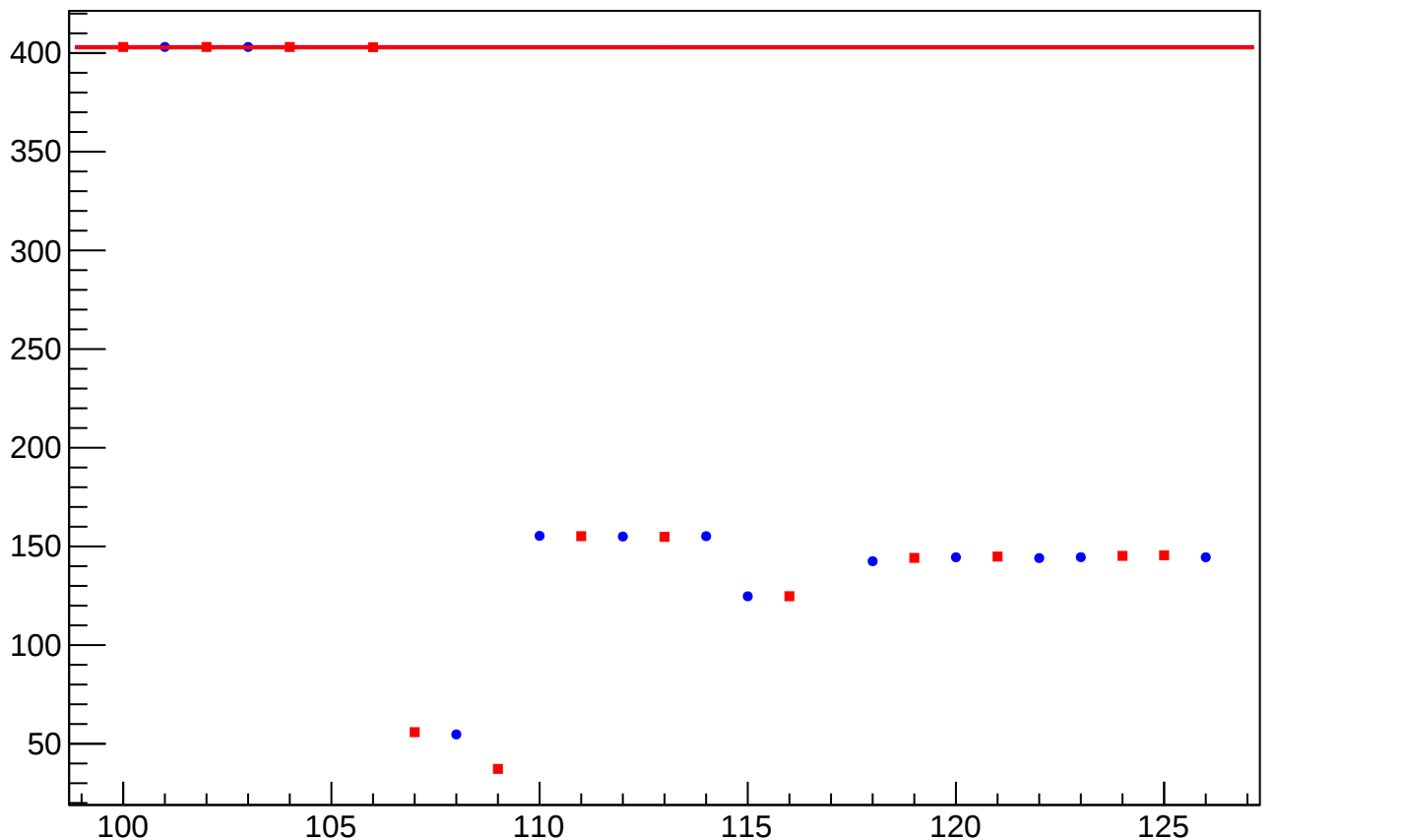
yield_cav4bQ_mean vs Slug, Sign Corrected
