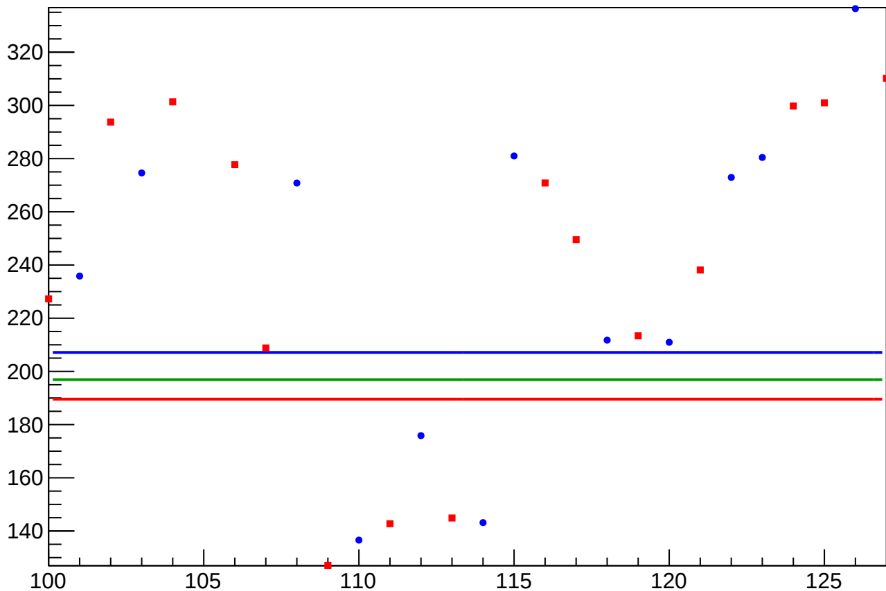
asym_bcm0l02_rms vs Slug, Sign Corrected
