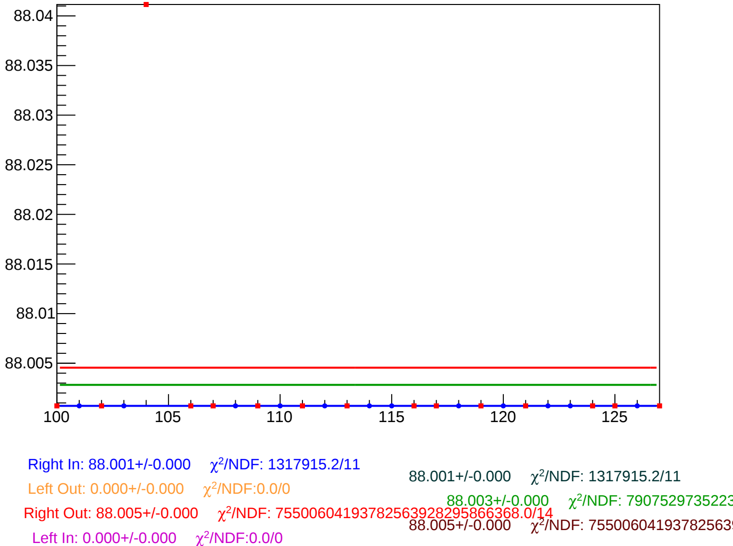
epics_VWienAngles_mean vs Slug, Sign Corrected
