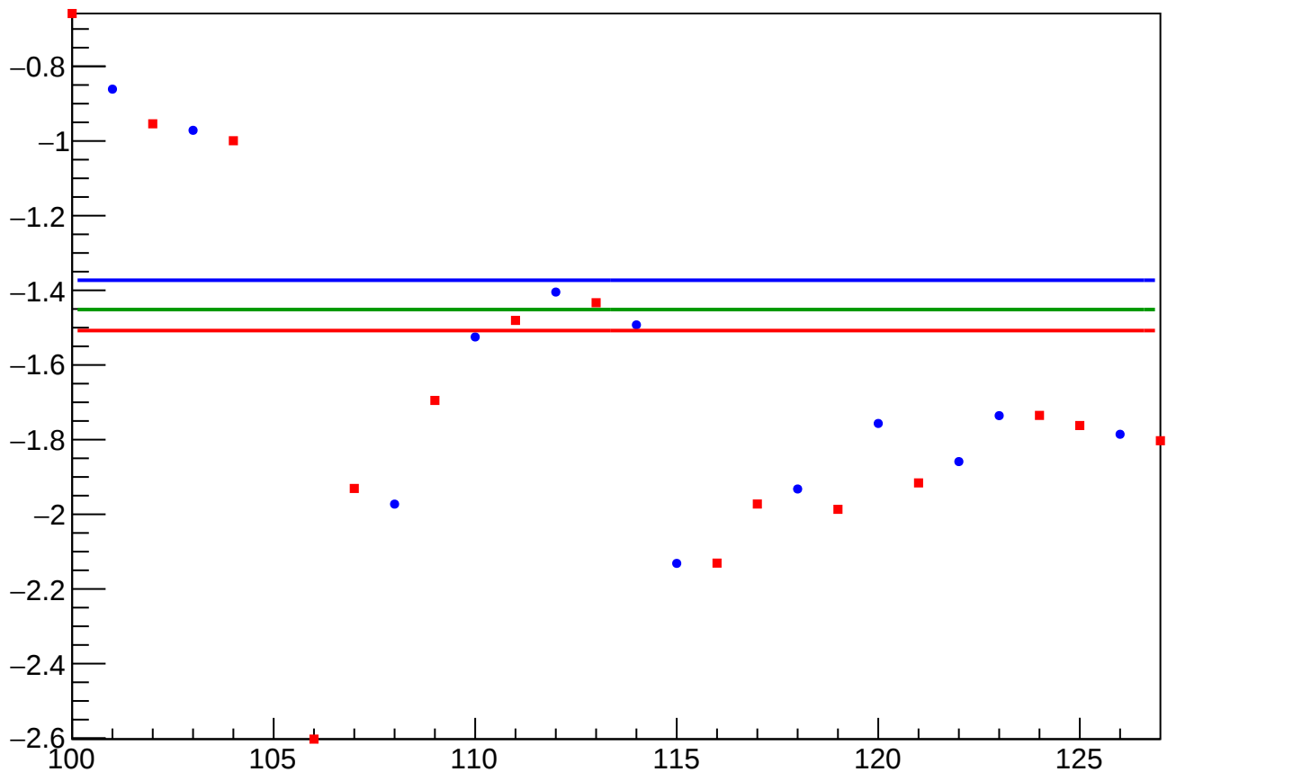
yield_bpm0i05Y_mean vs Slug, Sign Corrected
