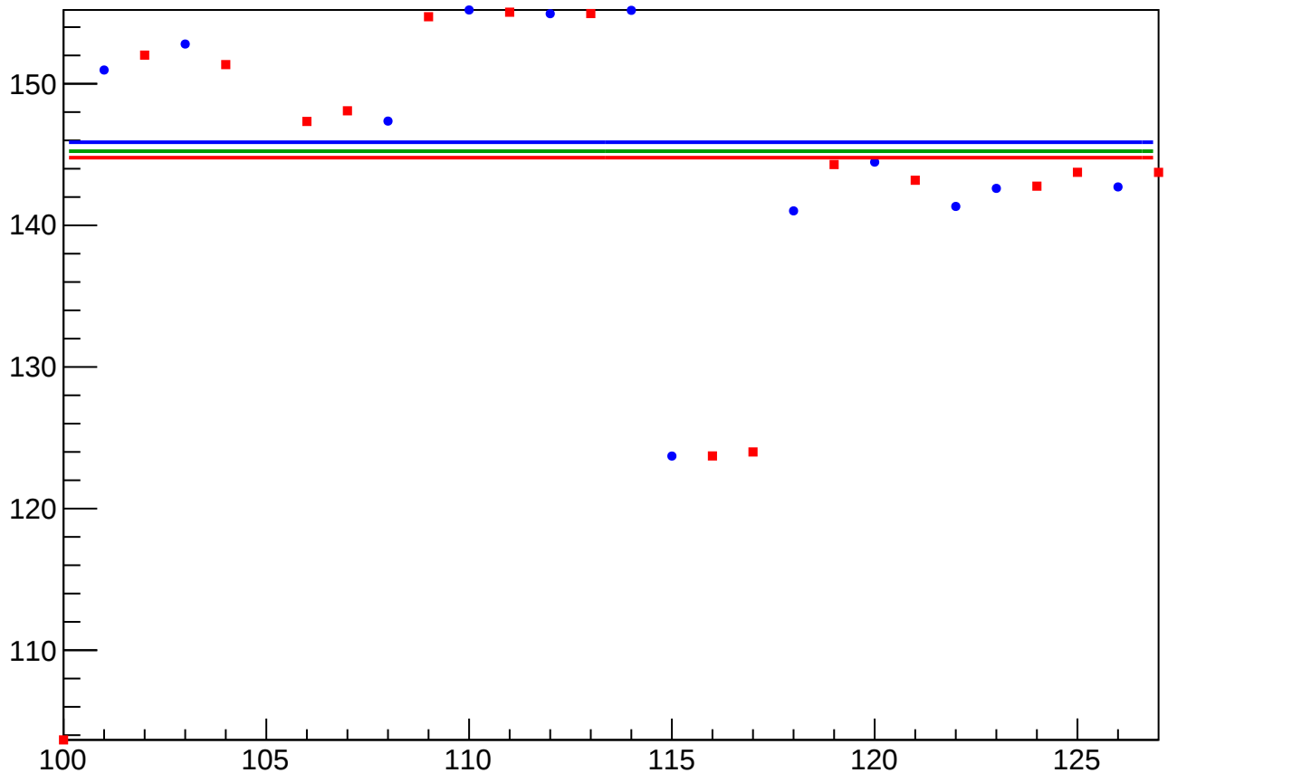
yield_bcm_an_ds_mean vs Slug, Sign Corrected
