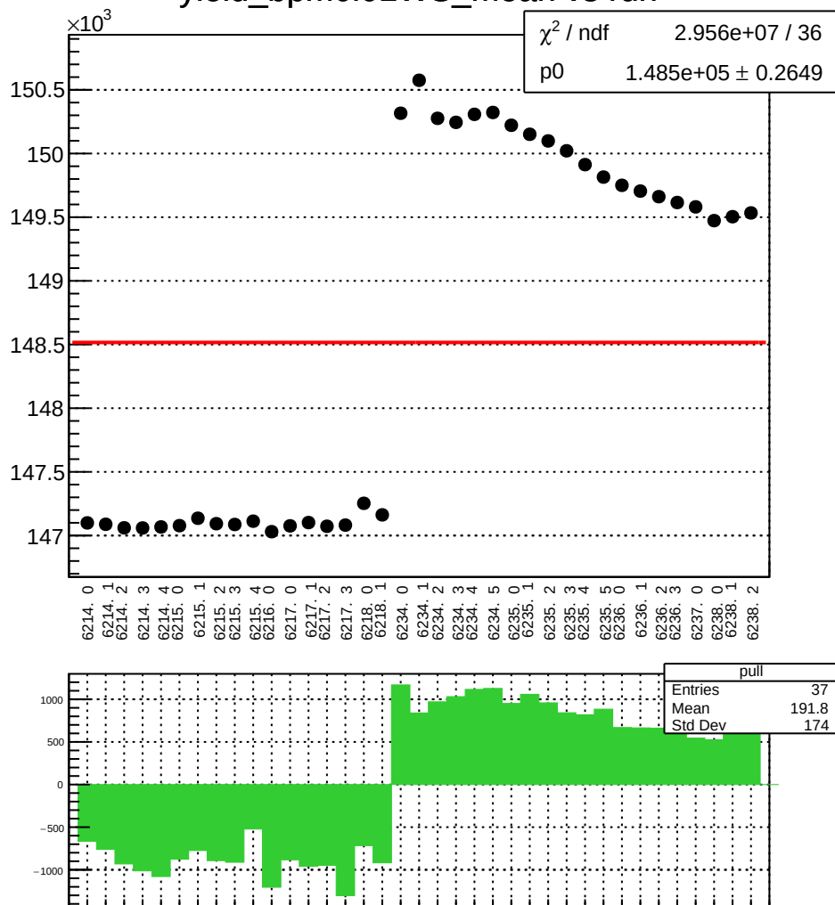
yield_bpm0i01WS_mean vs run
