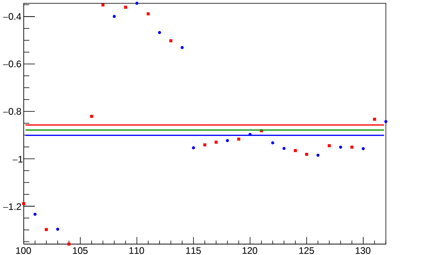
yield_bpm0i01X_mean vs Slug, Sign Corrected
