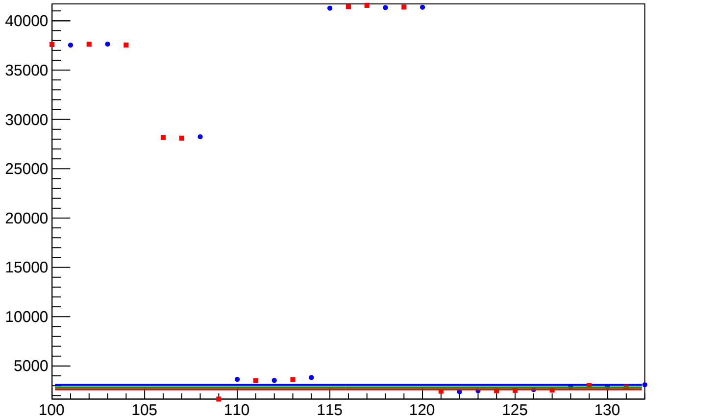
diff_bpm1p02bY_rms vs Slug, Sign Corrected
