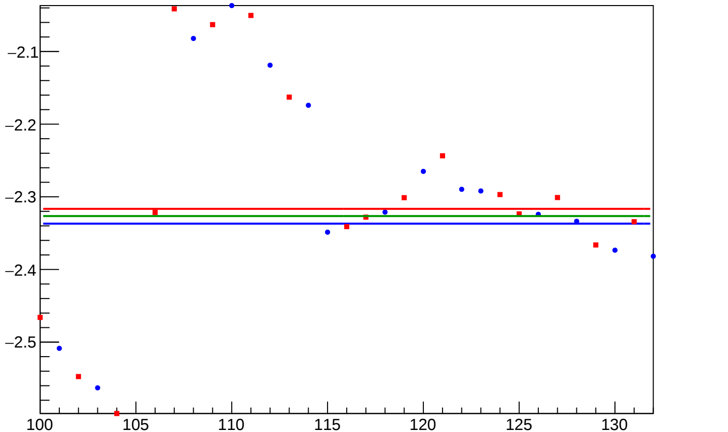
yield_bpm0i01aX_mean vs Slug, Sign Corrected
