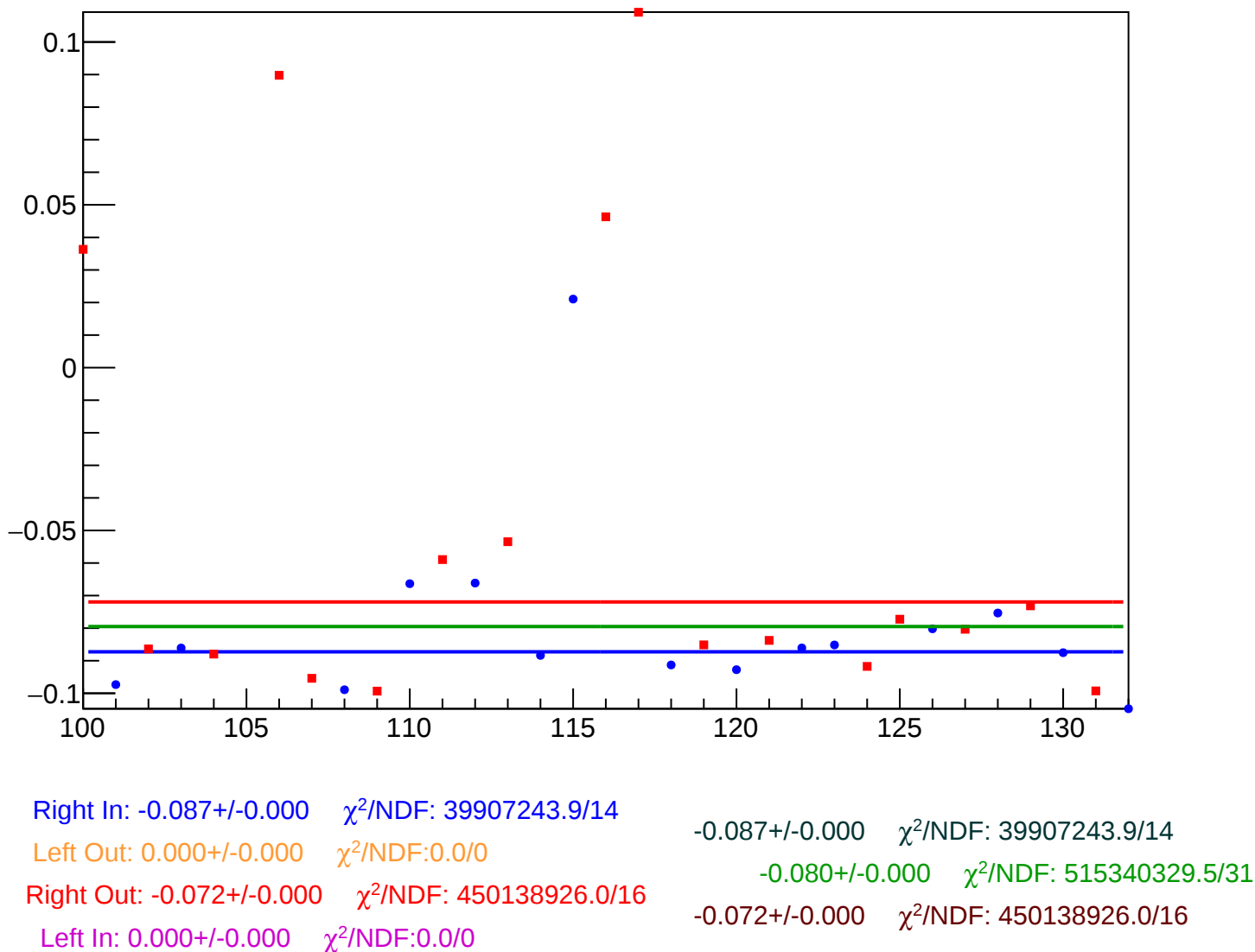
yield_bpm0l09Y_mean vs Slug, Sign Corrected
