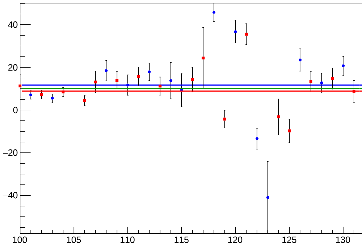
diff_bpm0r03Y_mean vs Slug, Sign Corrected
