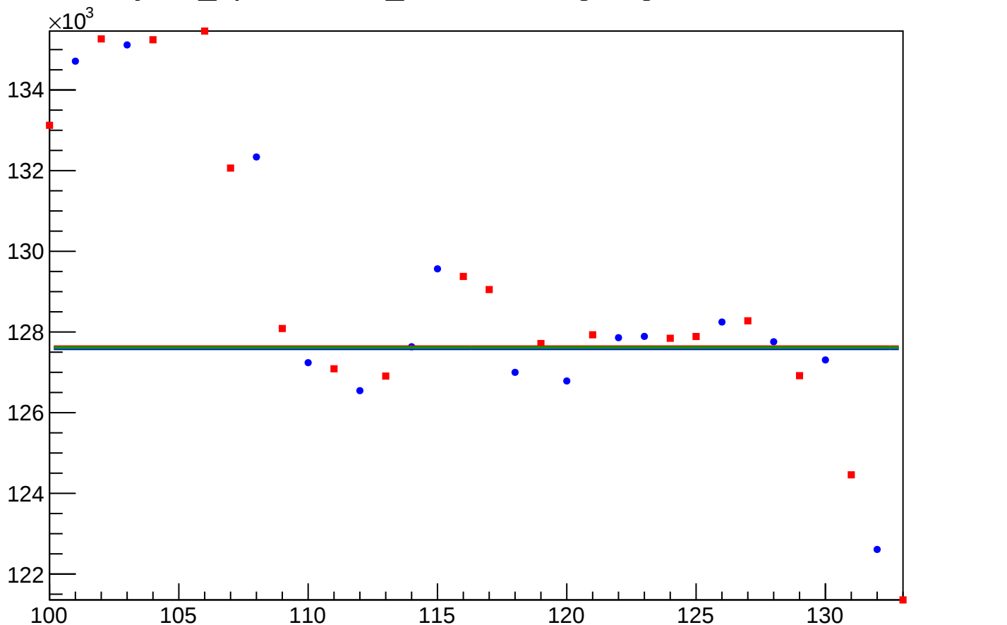
yield_bpm0l05WS_mean vs Slug, Sign Corrected
