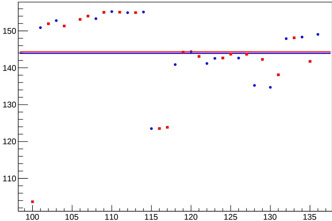
yield_bcm_an_us_mean vs Slug, Sign Corrected
