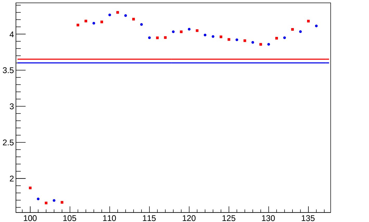
yield_bpm1i04Y_mean vs Slug, Sign Corrected
