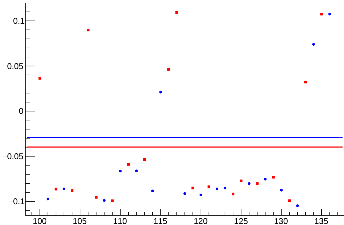
yield_bpm0l09Y_mean vs Slug, Sign Corrected
