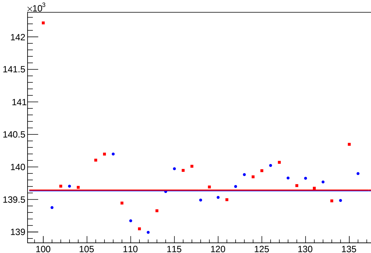
yield_bpm0l09WS_mean vs Slug, Sign Corrected
