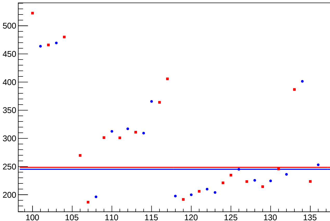
yield_bpm0r03WS_rms vs Slug, Sign Corrected
