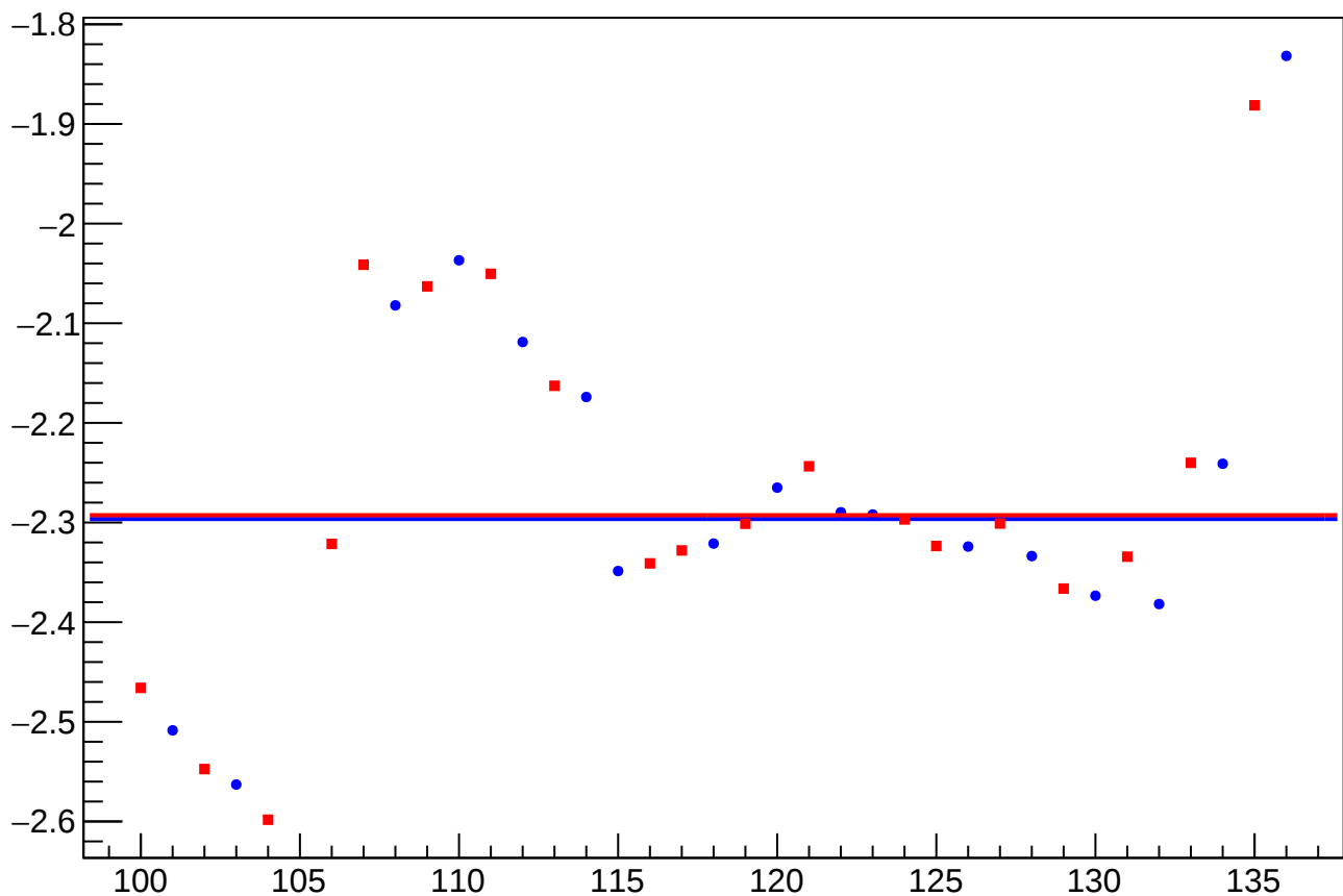
yield_bpm0i01aX_mean vs Slug, Sign Corrected
