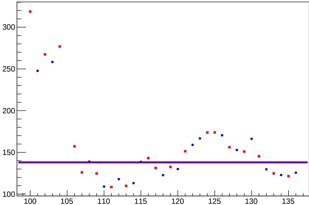
asym_bpm0i01WS_rms vs Slug, Sign Corrected
