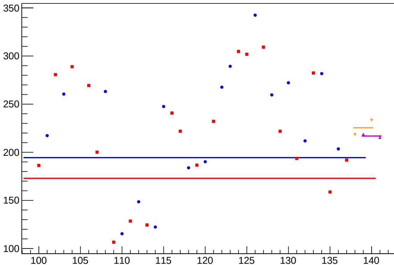
asym_bcm_ds_bcm_an_ds_agg_avg_rms vs Slug, Sign Corrected
