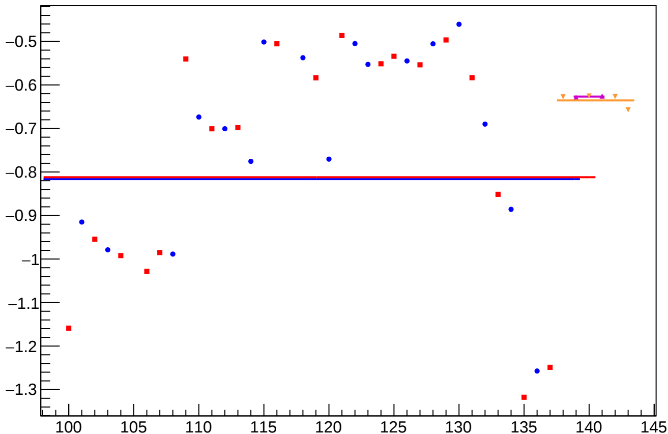
yield_bpm0i07X_mean vs Slug, Sign Corrected
