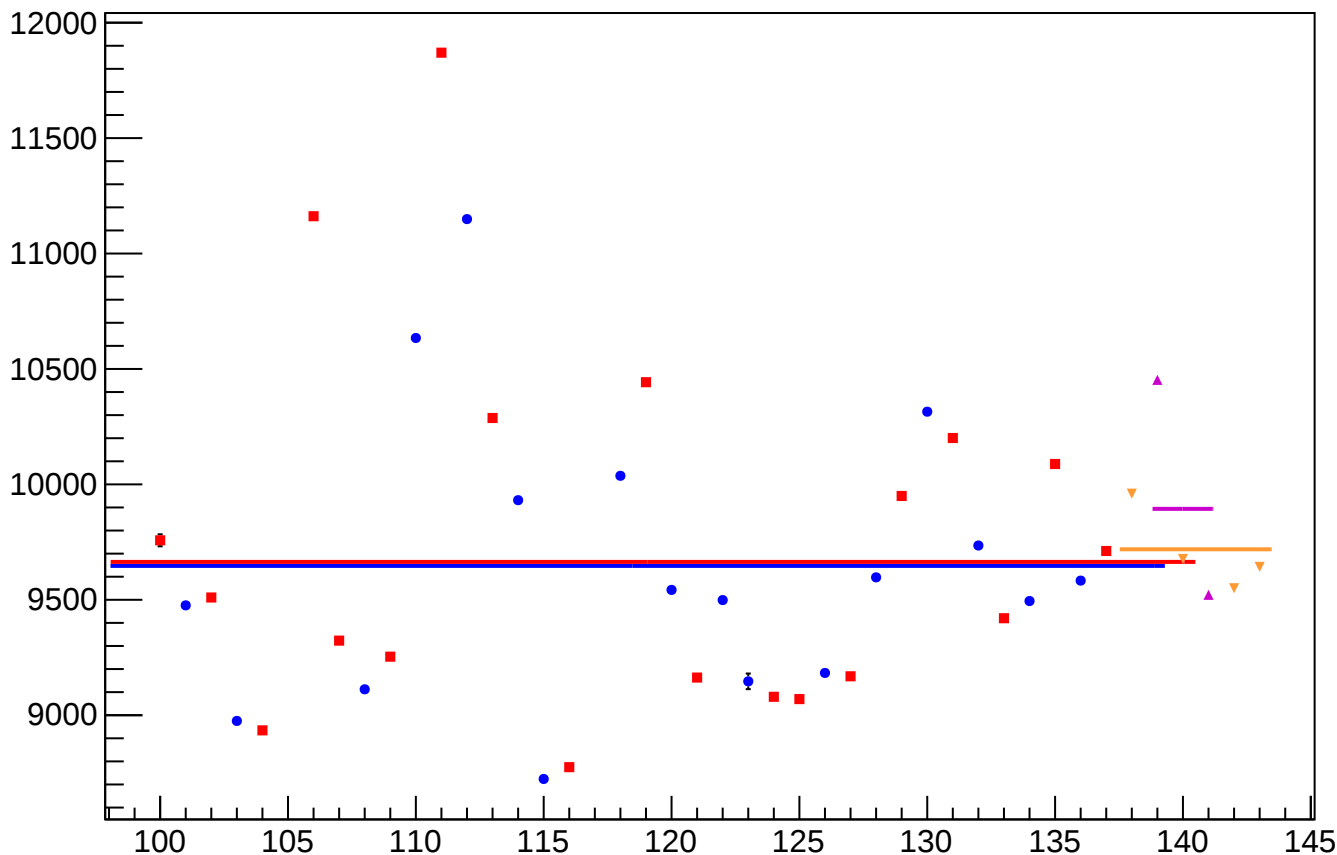
diff_bpm0l02X_rms vs Slug, Sign Corrected
