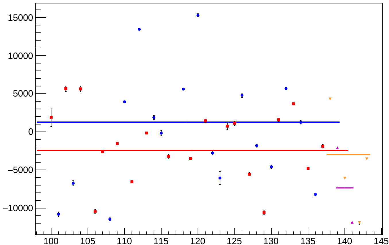
asym_bpm0i01aWS_mean vs Slug, Sign Corrected
