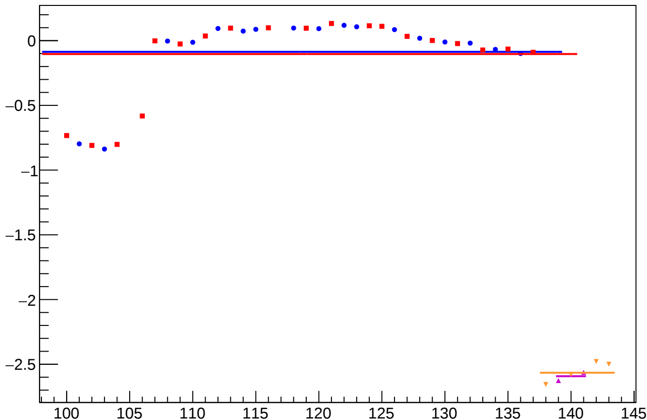
yield_bpm1i02X_mean vs Slug, Sign Corrected
