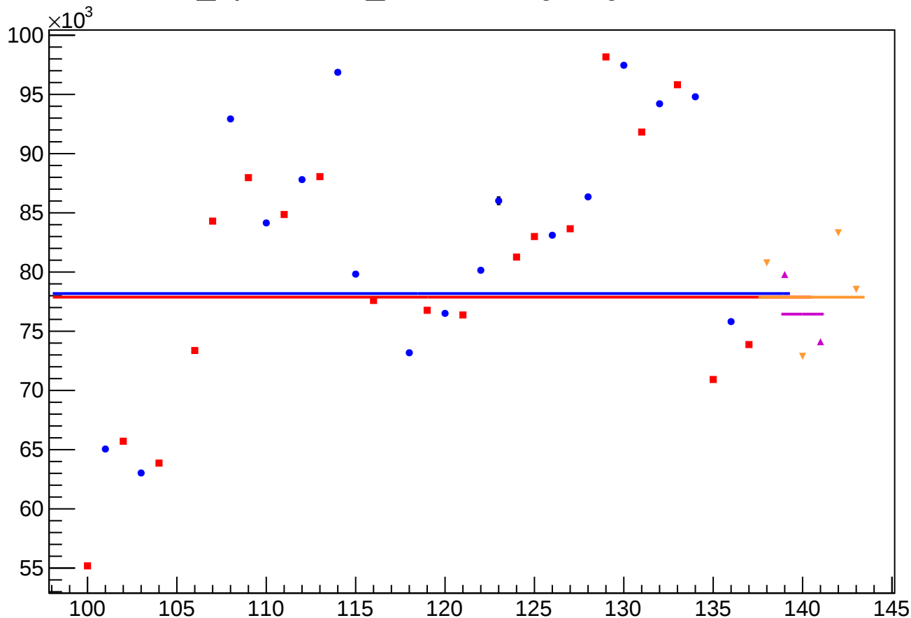
diff_bpm0r05X_rms vs Slug, Sign Corrected
