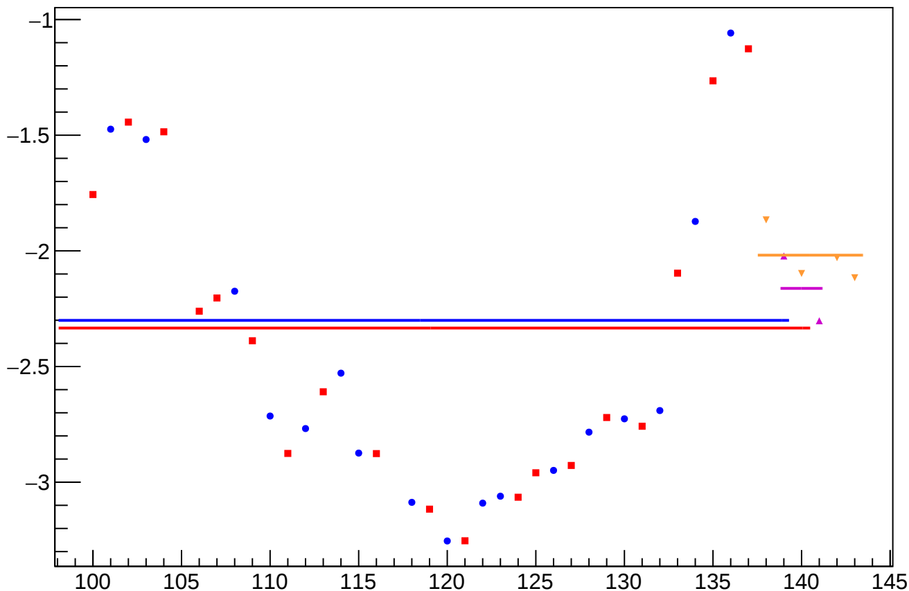
yield_bpm2i02Y_mean vs Slug, Sign Corrected
