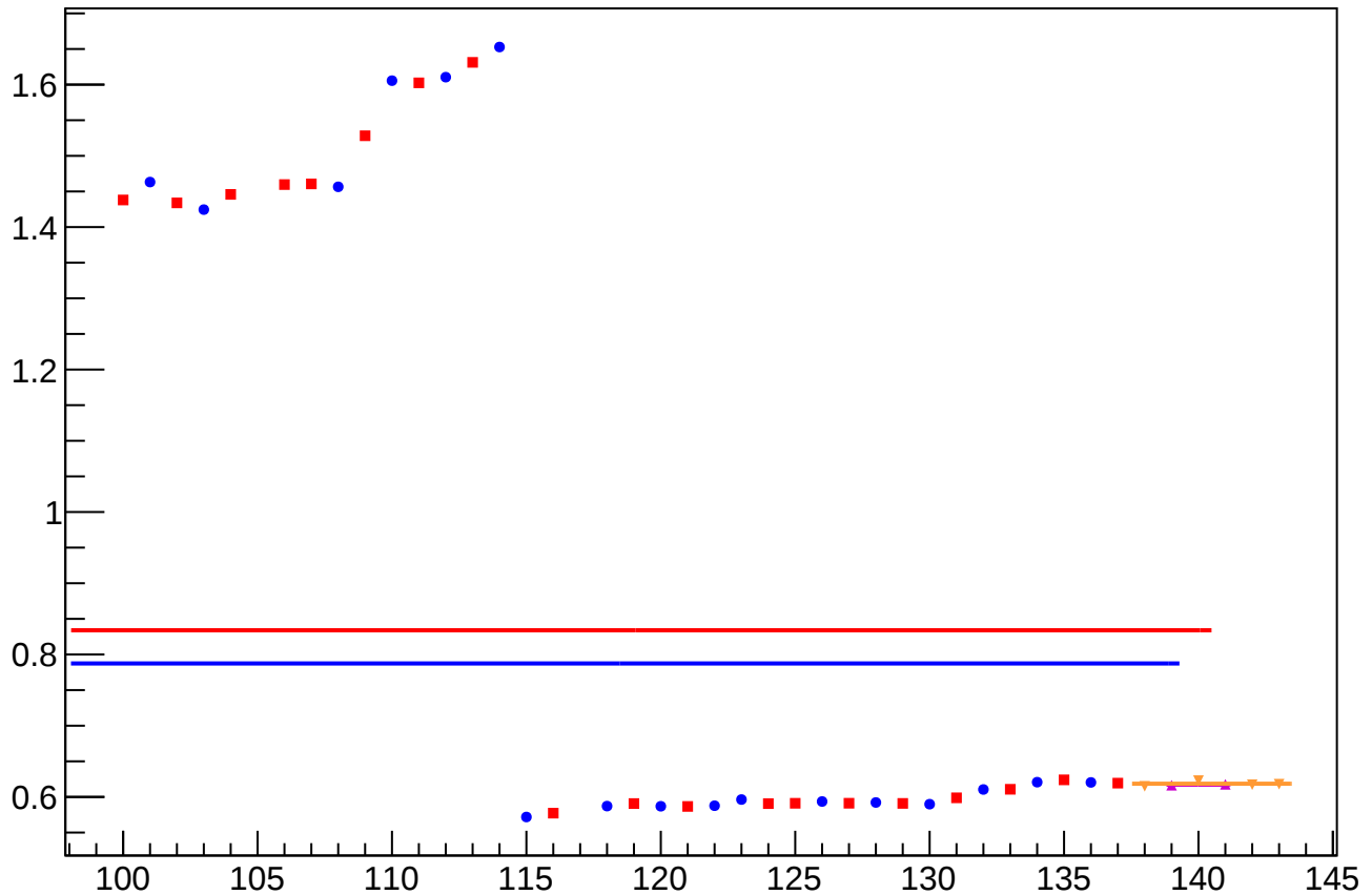
yield_bpm4aY_mean vs Slug, Sign Corrected
