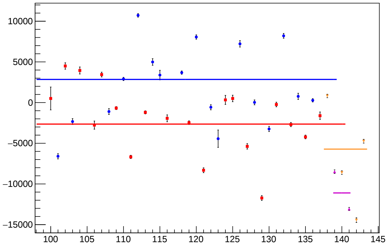
asym_bpm0i02aWS_mean vs Slug, Sign Corrected
