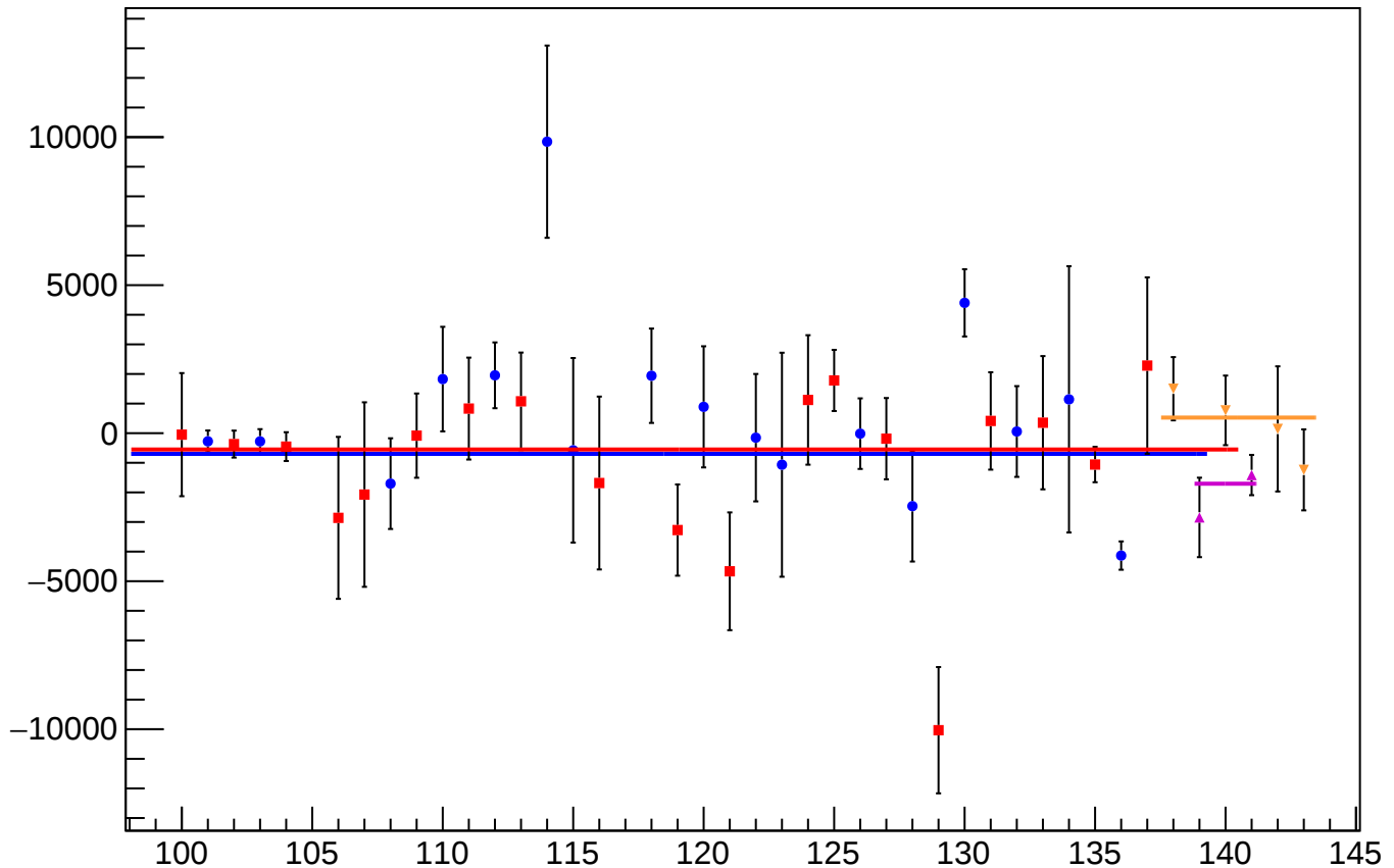
asym_bpm0l03WS_mean vs Slug, Sign Corrected
