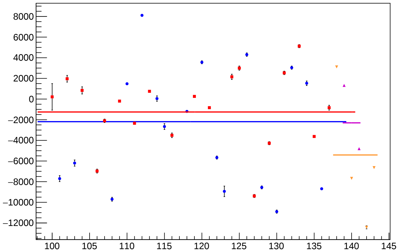
asym_bpm1i04WS_mean vs Slug, Sign Corrected
