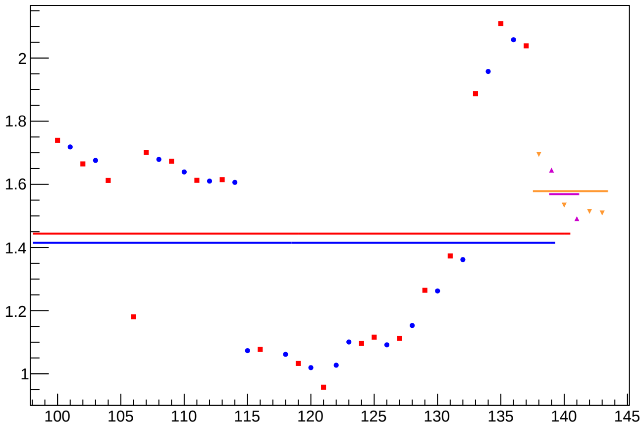
yield_bpm0i01aY_mean vs Slug, Sign Corrected
