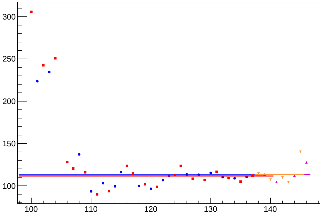
asym_bpm2i02WS_rms vs Slug, Sign Corrected
