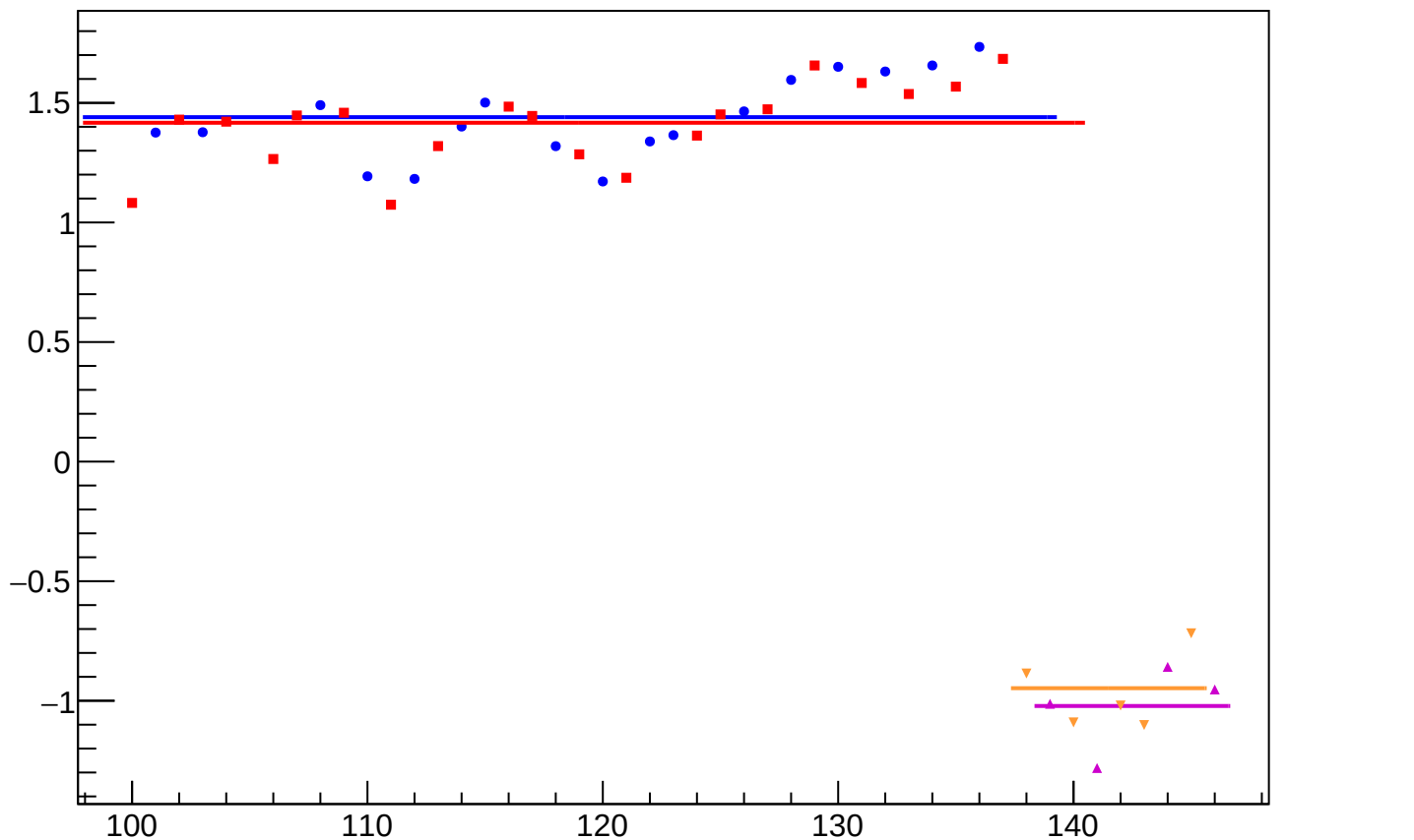
yield_bpm1i02Y_mean vs Slug, Sign Corrected
