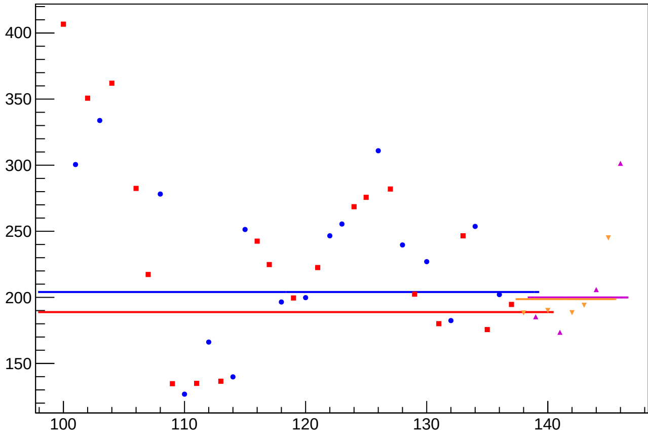
asym_bpm0l06WS_rms vs Slug, Sign Corrected
