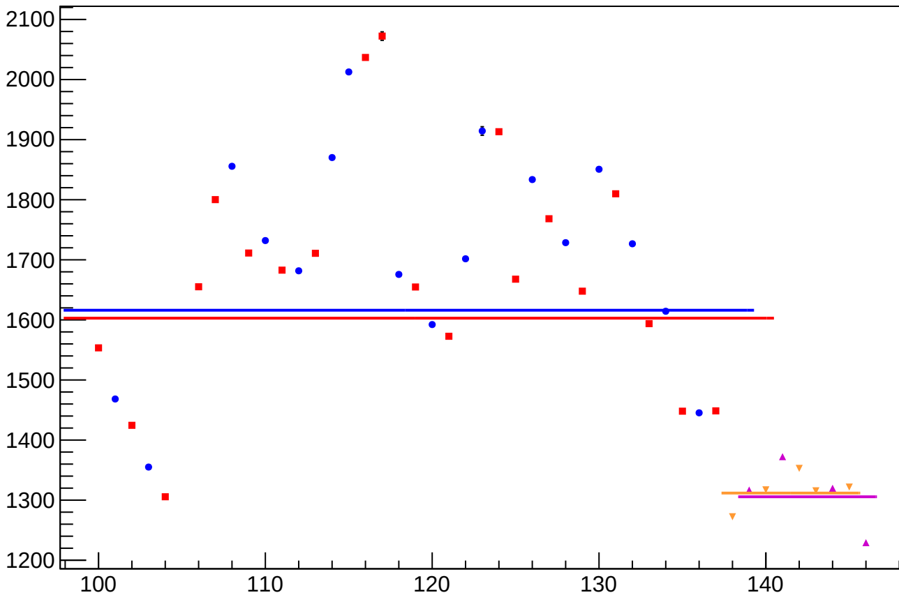
diff_bpm0i02aY_rms vs Slug, Sign Corrected
