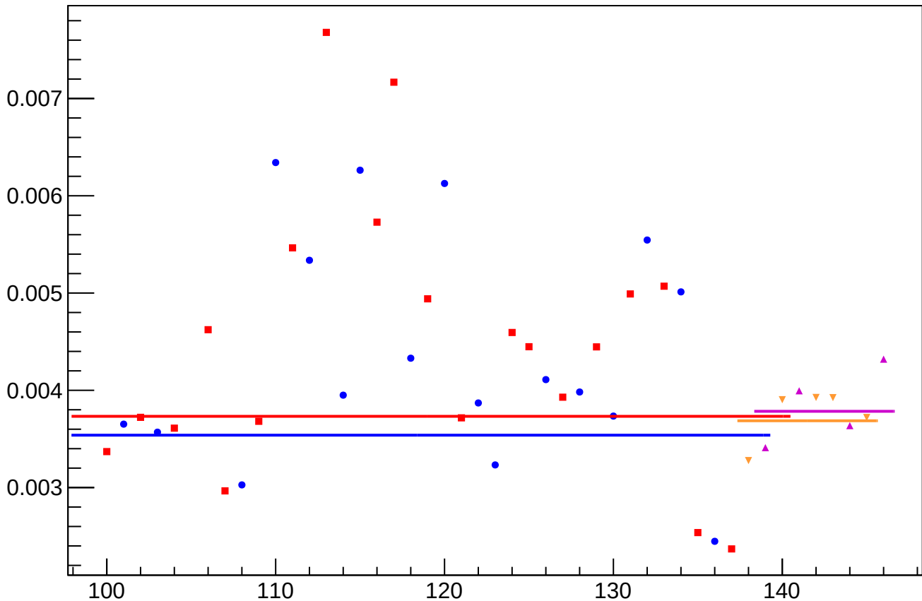
yield_bpm0l10Y_rms vs Slug, Sign Corrected
