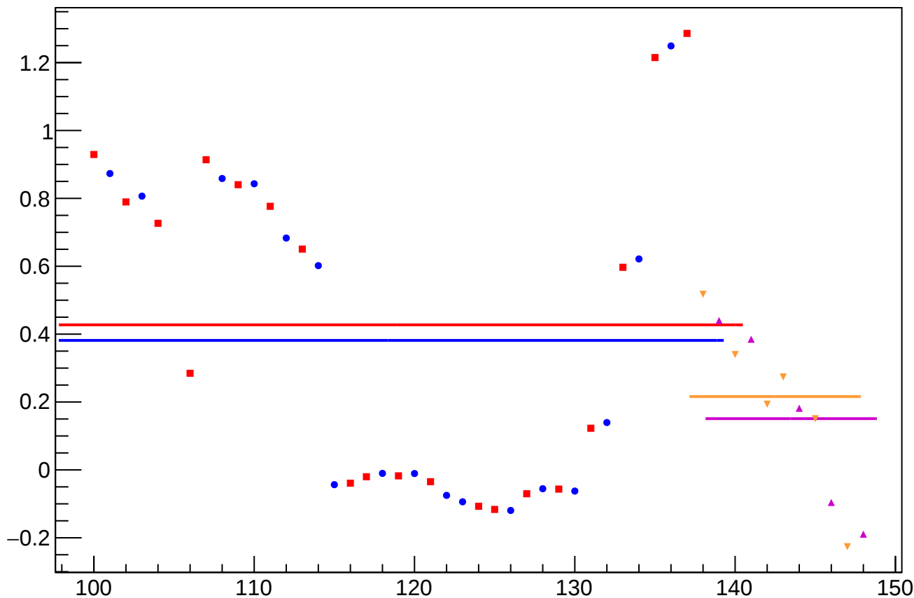
yield_bpm1i06X_mean vs Slug, Sign Corrected
