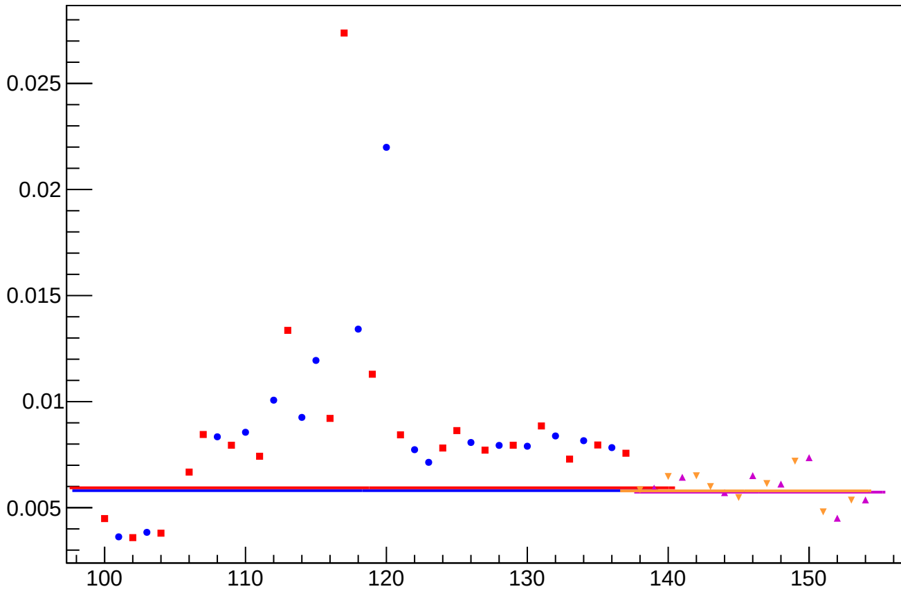
yield_bpm0105Y_rms vs Slug, Sign Corrected
