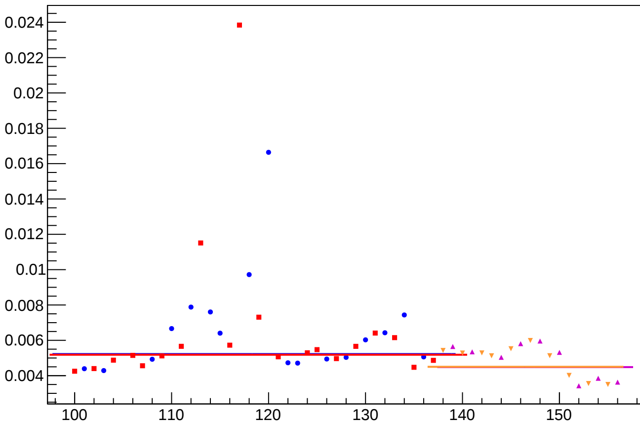
yield_bpm0i07X_rms vs Slug, Sign Corrected
