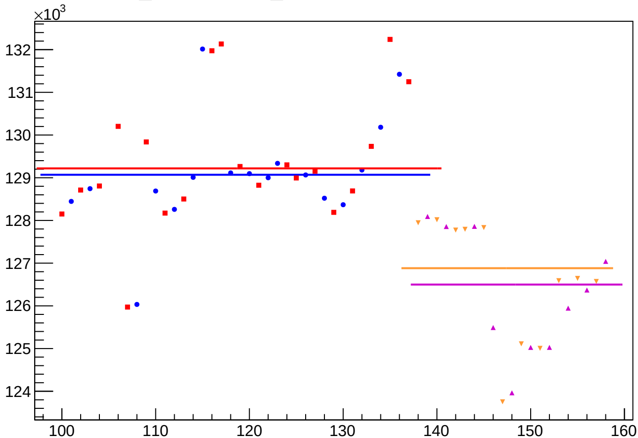
yield_bpm0l06WS_mean vs Slug, Sign Corrected
