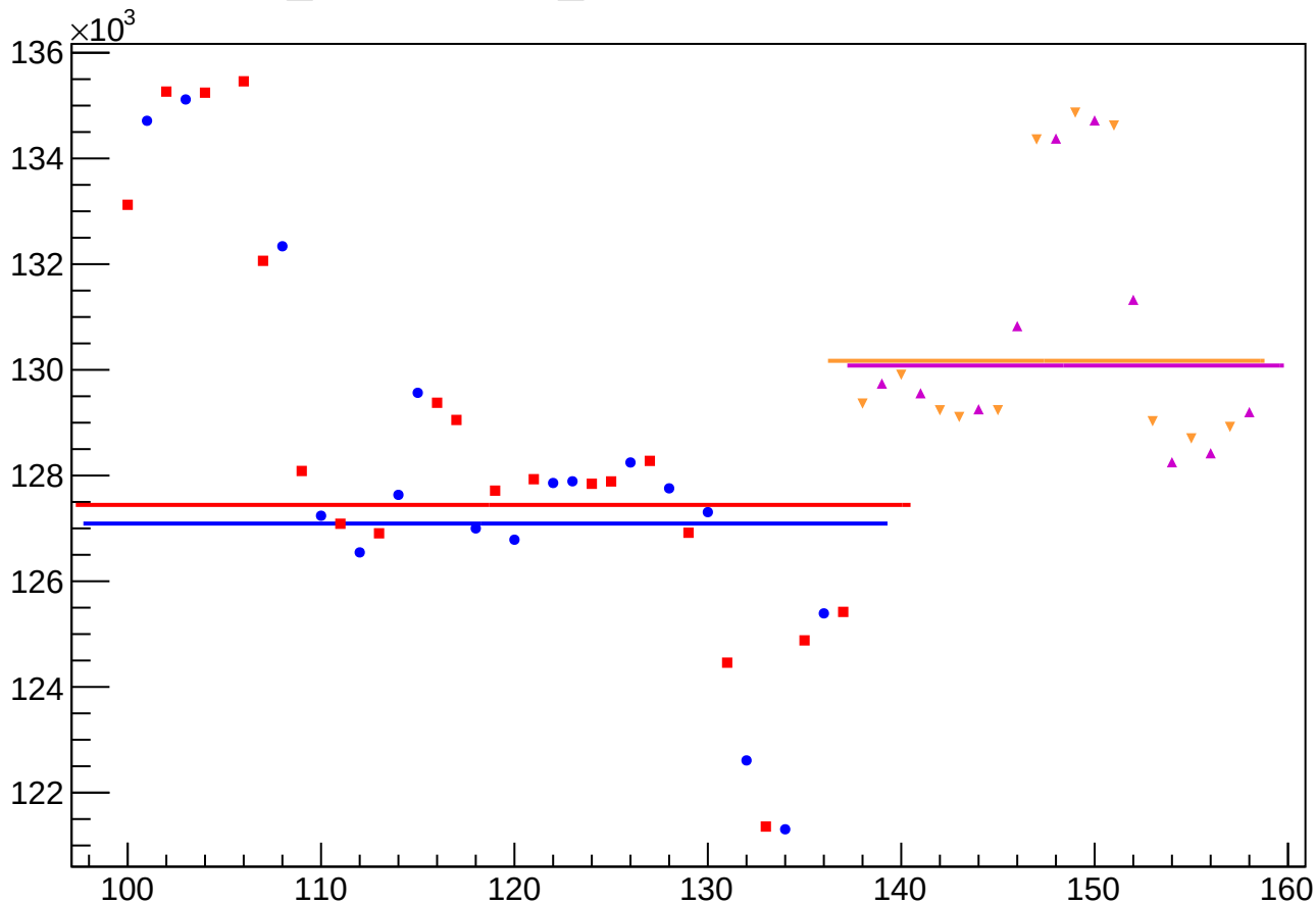
yield_bpm0l05WS_mean vs Slug, Sign Corrected
