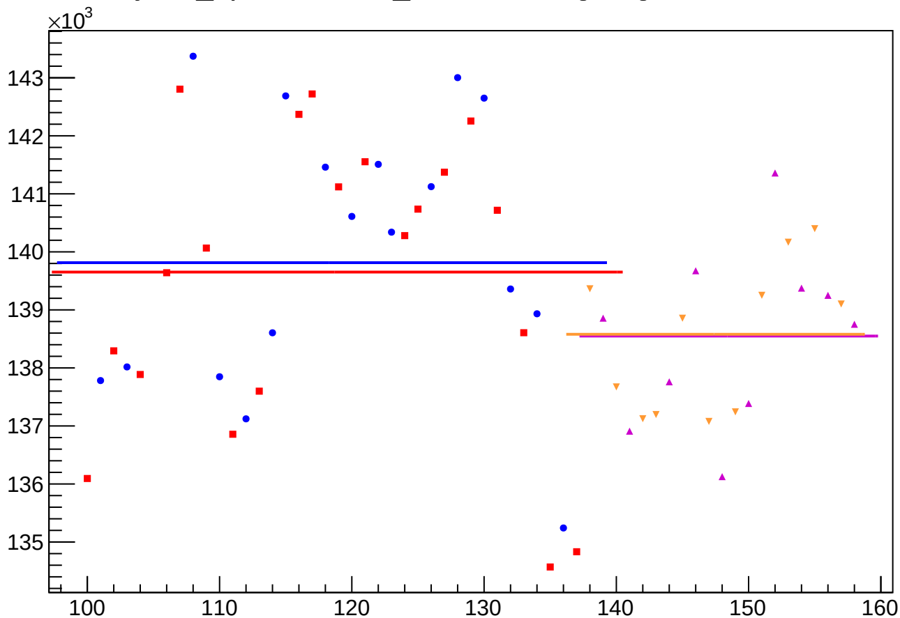
yield_bpm0i02aWS_mean vs Slug, Sign Corrected
