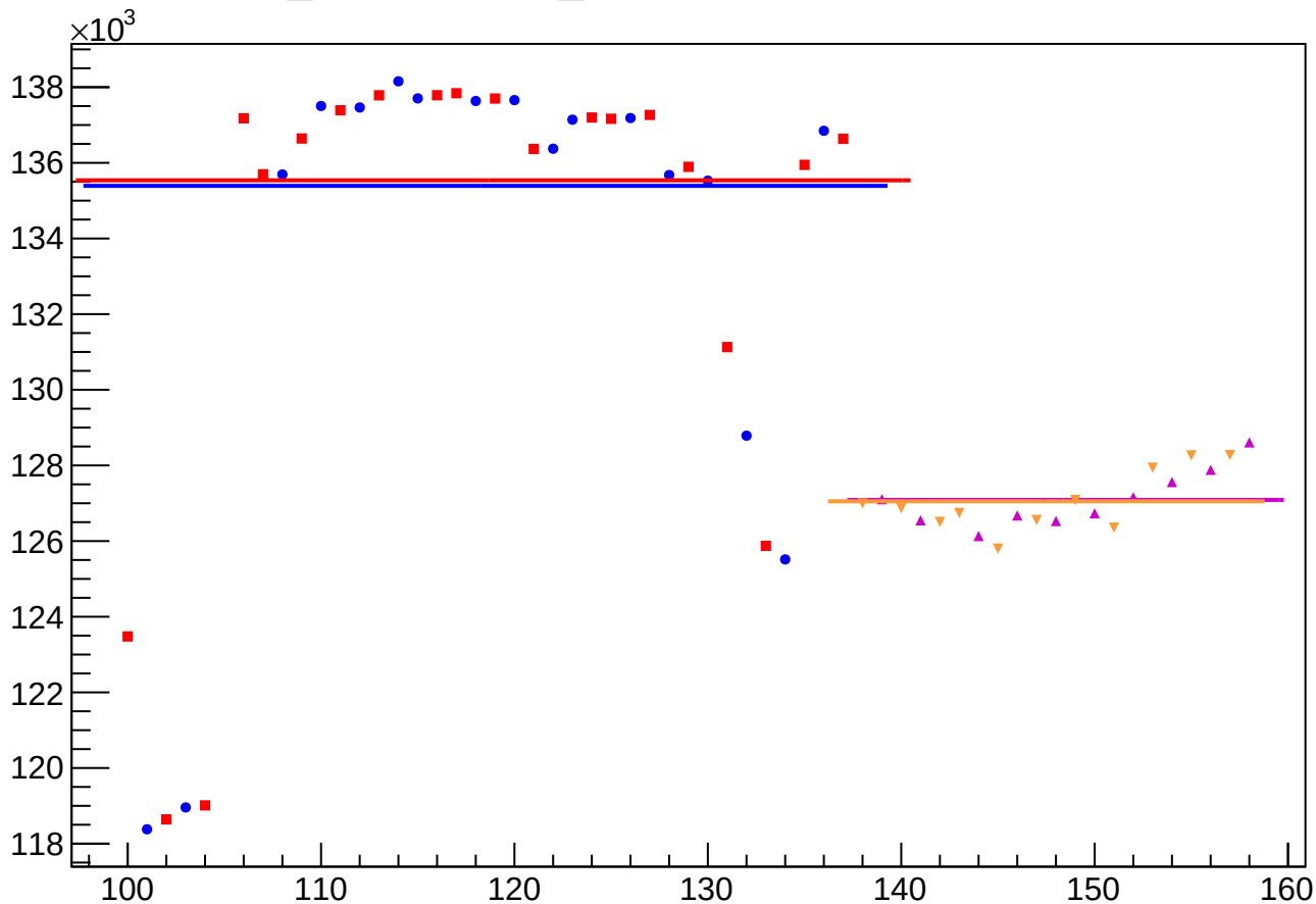
yield_bpm0l04WS_mean vs Slug, Sign Corrected
