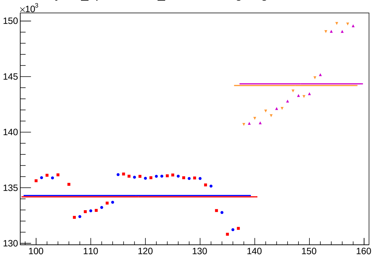
yield_bpm1i04WS_mean vs Slug, Sign Corrected
