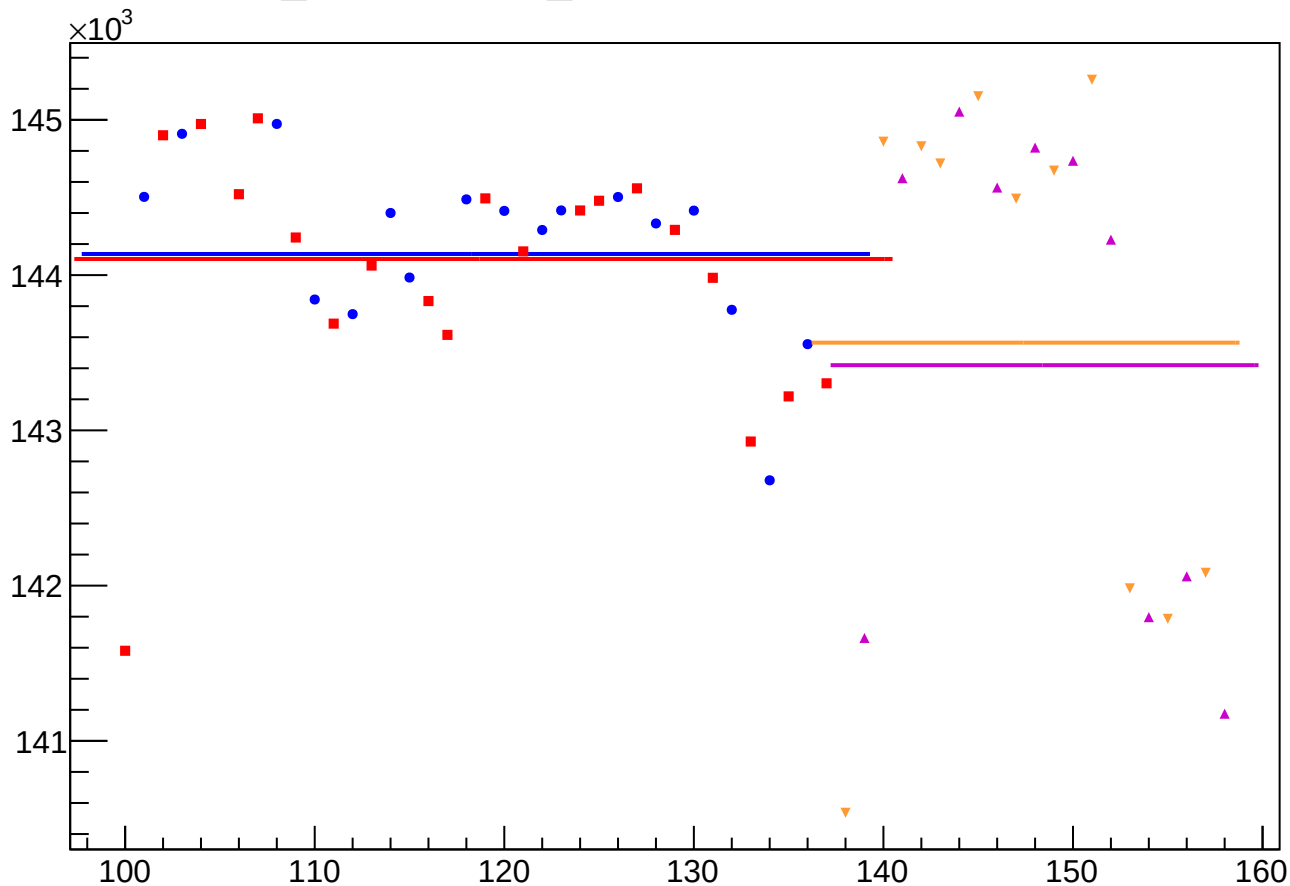
yield_bpm0l08WS_mean vs Slug, Sign Corrected
