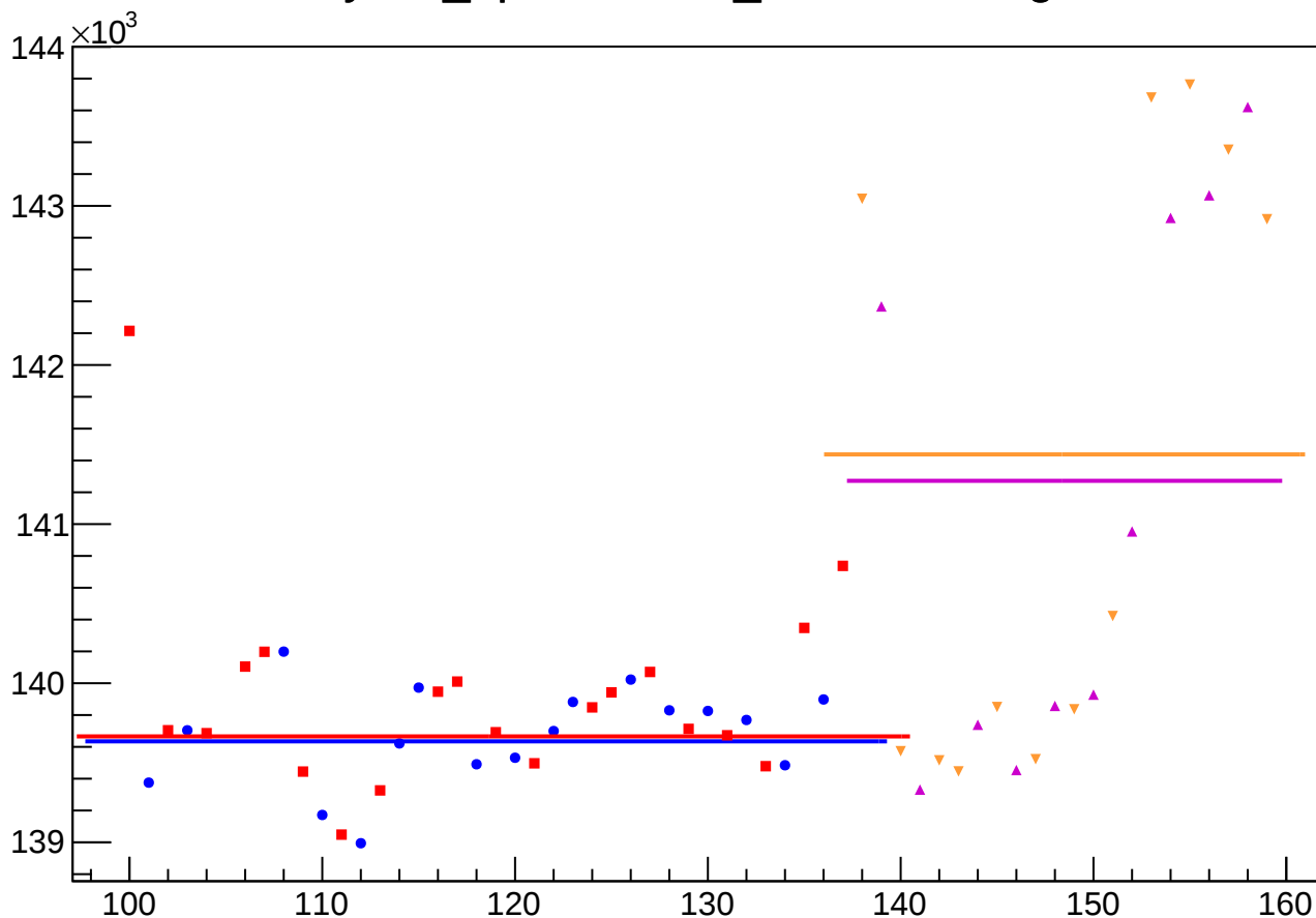
yield_bpm0l09WS_mean vs Slug
