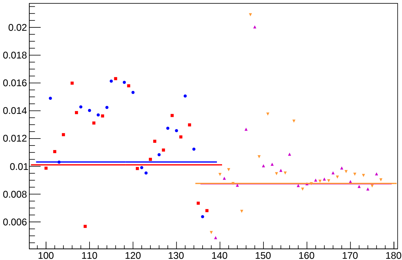
yield_bpm12Y_rms vs Slug, Sign Corrected
