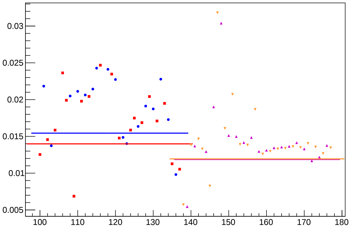
yield_bpm11Y_rms vs Slug, Sign Corrected
