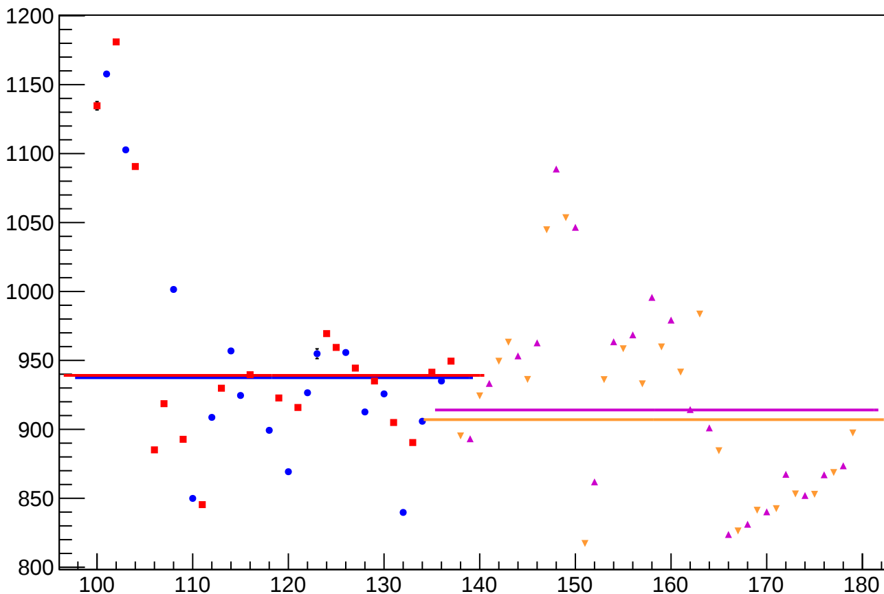
diff_bpm1i02X_rms vs Slug, Sign Corrected
