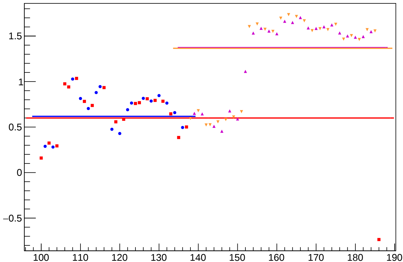
yield_bpm0l02Y_mean vs Slug, Sign Corrected
