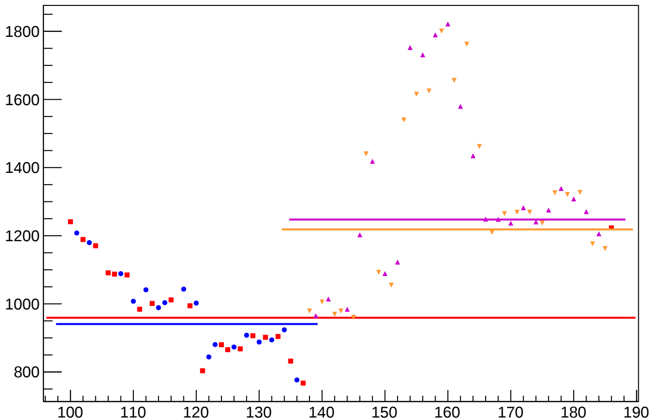
diff_bpm0l10Y_rms vs Slug, Sign Corrected
