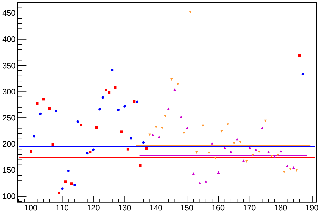
asym_bcm_an_ds_rms vs Slug, Sign Corrected
