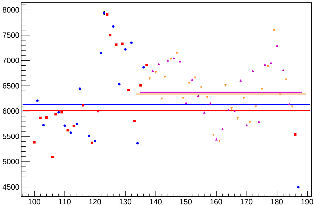
diff_bpm0l05X_rms vs Slug, Sign Corrected
