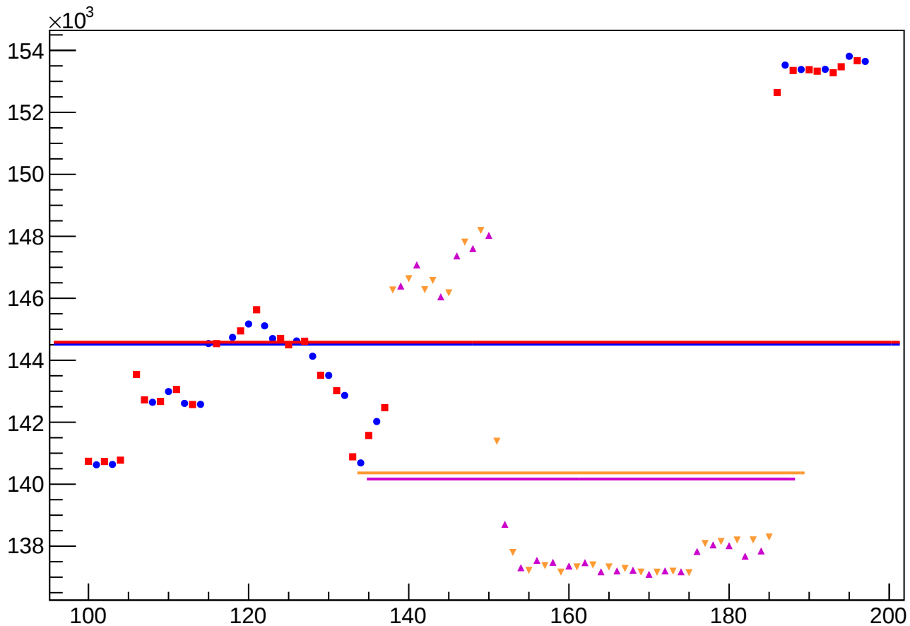
yield_bpm0i01aWS_mean vs Slug, Sign Corrected
