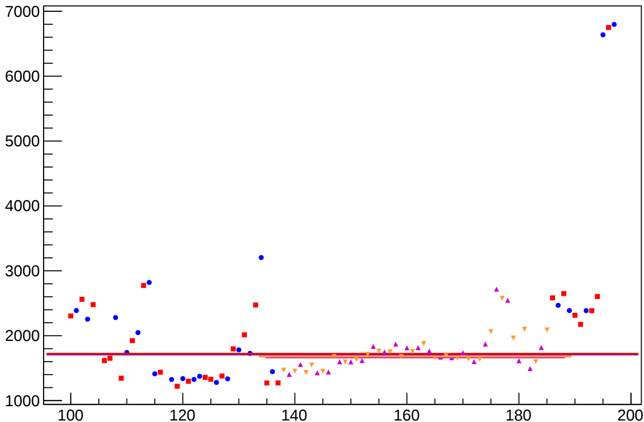
diff_bpm0i07X_rms vs Slug, Sign Corrected
