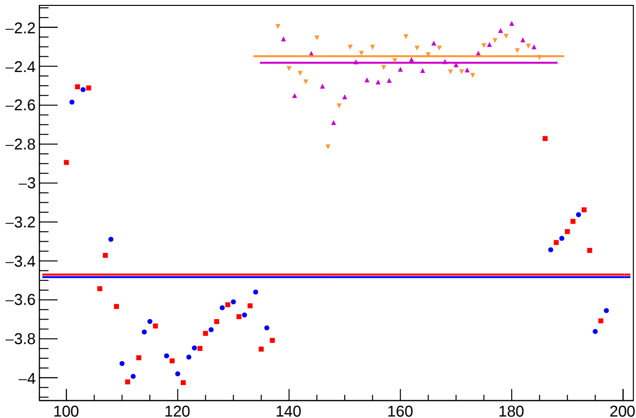
yield_bpm0i02Y_mean vs Slug, Sign Corrected
