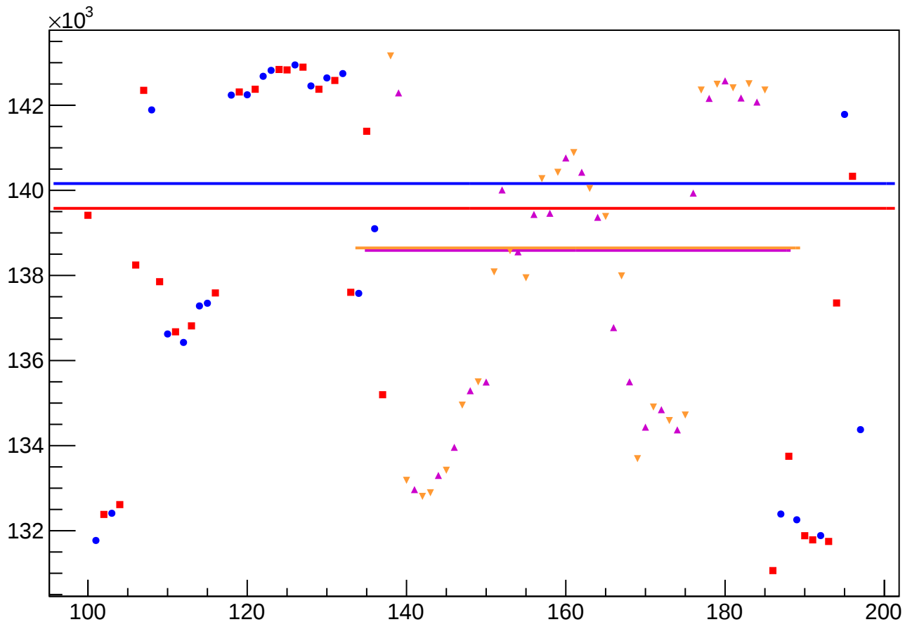
yield_bpm0r03WS_mean vs Slug, Sign Corrected
