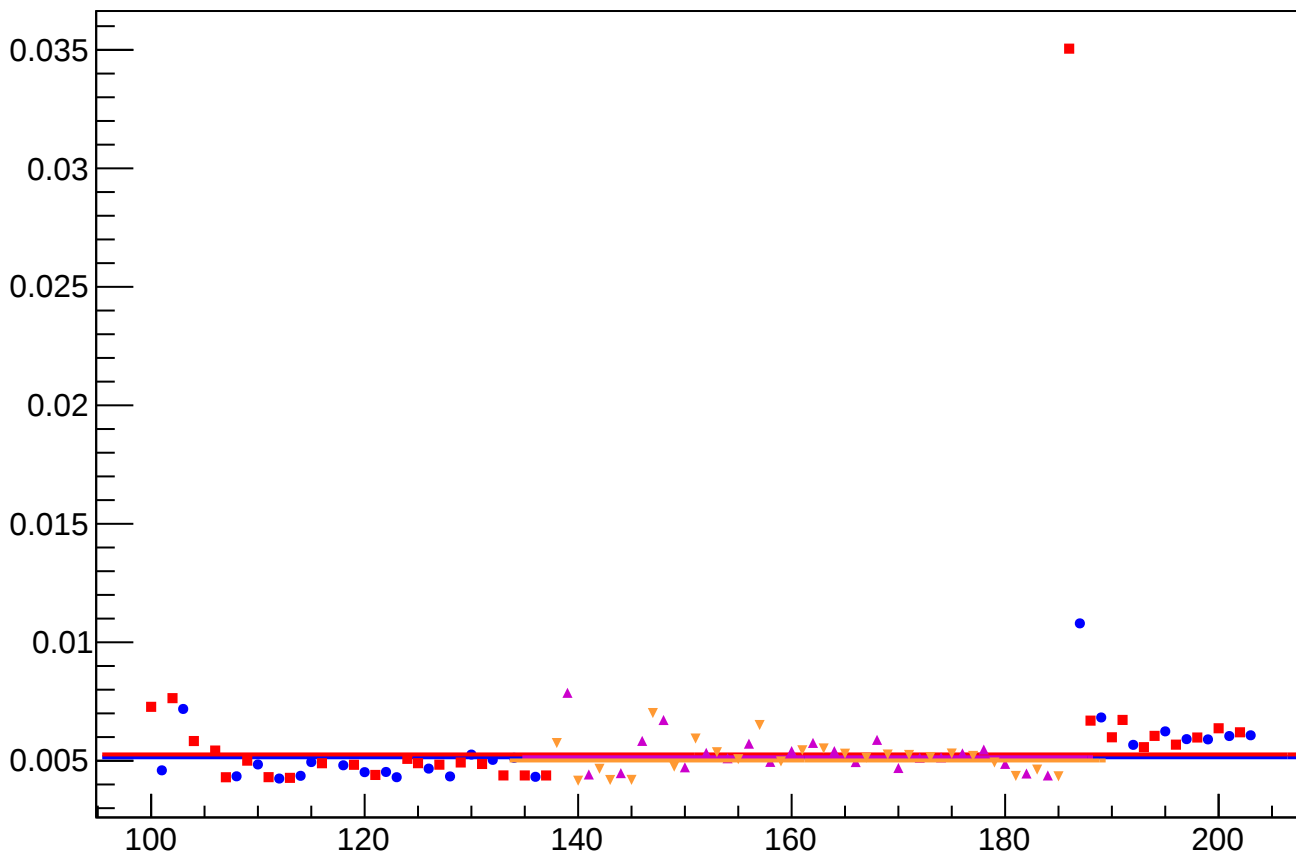
yield_bpm16Y_rms vs Slug, Sign Corrected
