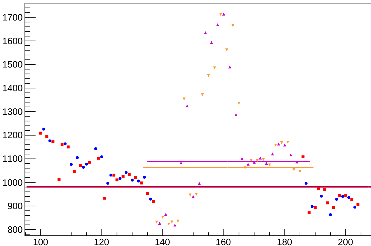
diff_bpm0l07Y_rms vs Slug, Sign Corrected
