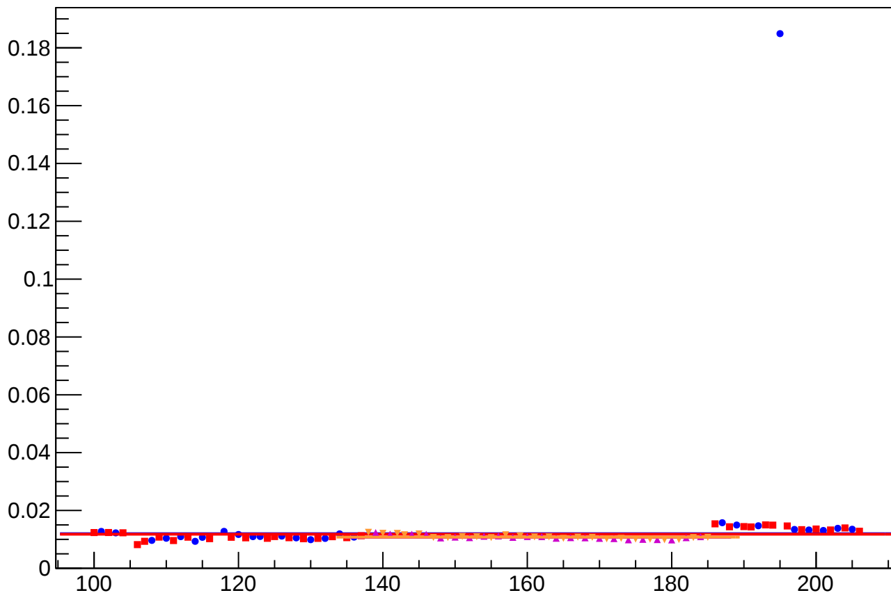
yield_bpm0l09X_rms vs Slug, Sign Corrected
