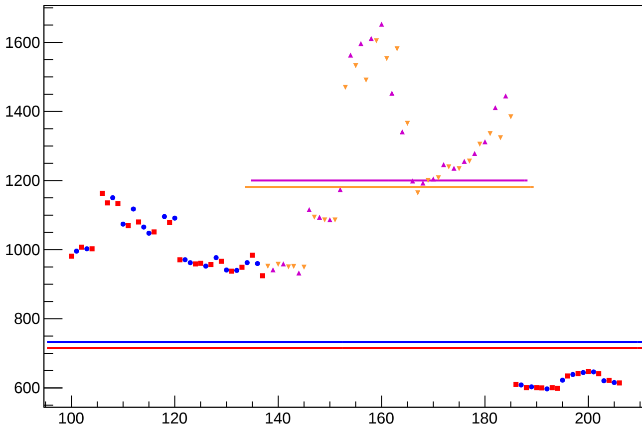
diff_bpm2i02Y_rms vs Slug, Sign Corrected
