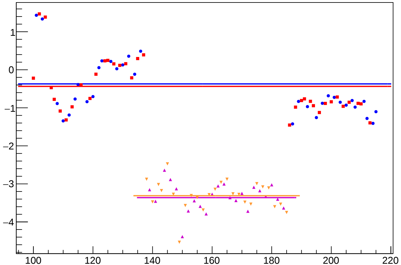
yield_bpm0l02X_mean vs Slug, Sign Corrected
