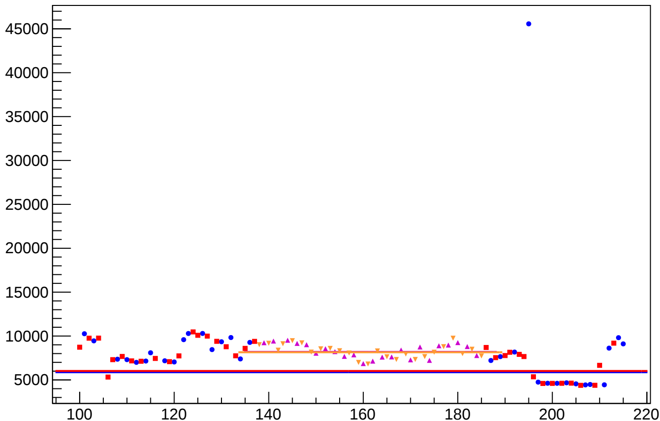
diff_bpm0l09X_rms vs Slug, Sign Corrected
