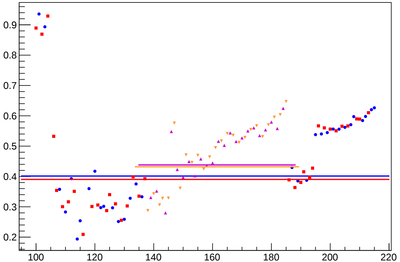
yield_bcm_an_ds3_rms vs Slug, Sign Corrected
