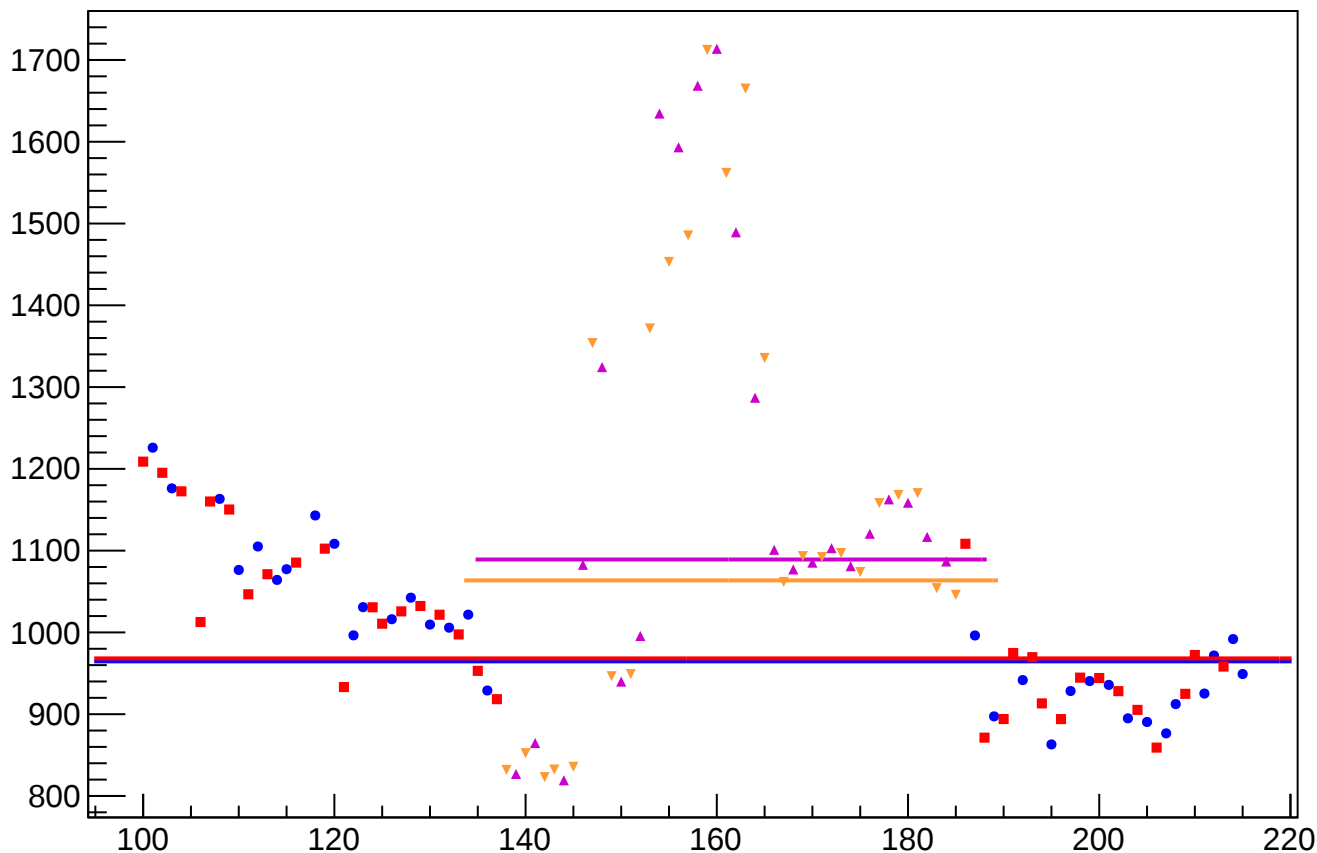
diff_bpm0l07Y_rms vs Slug, Sign Corrected
