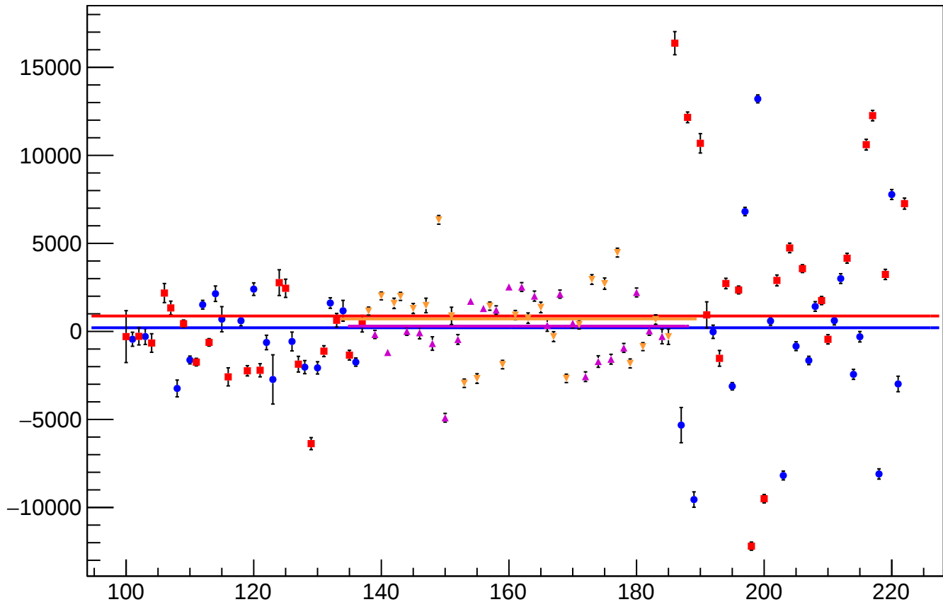
asym_bpm0l05WS_mean vs Slug, Sign Corrected
