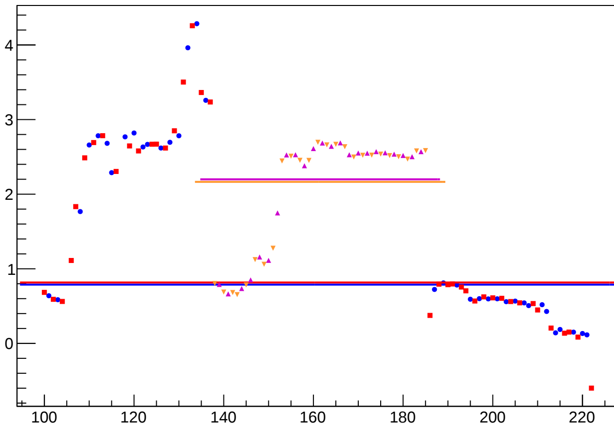
yield_bpm0l05Y_mean vs Slug, Sign Corrected
