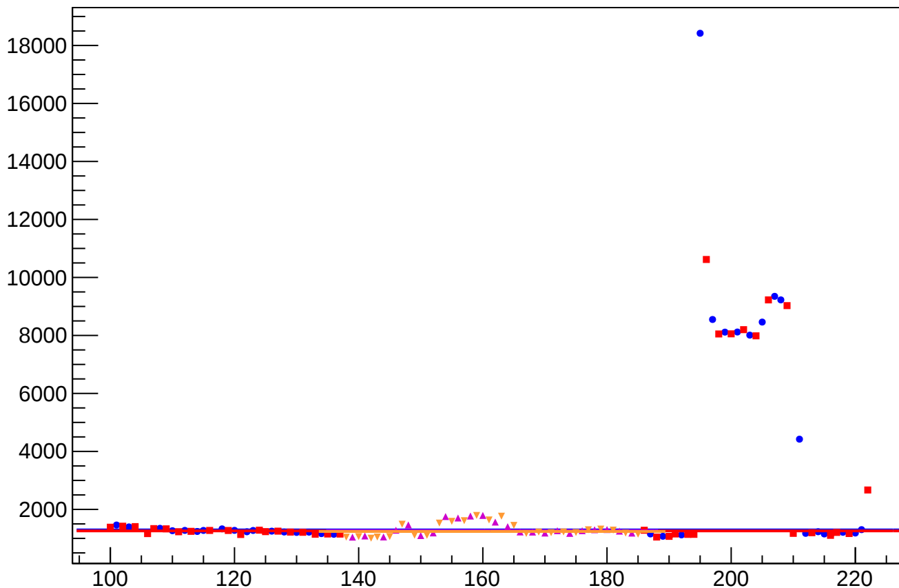
diff_bpm0l08Y_rms vs Slug, Sign Corrected
