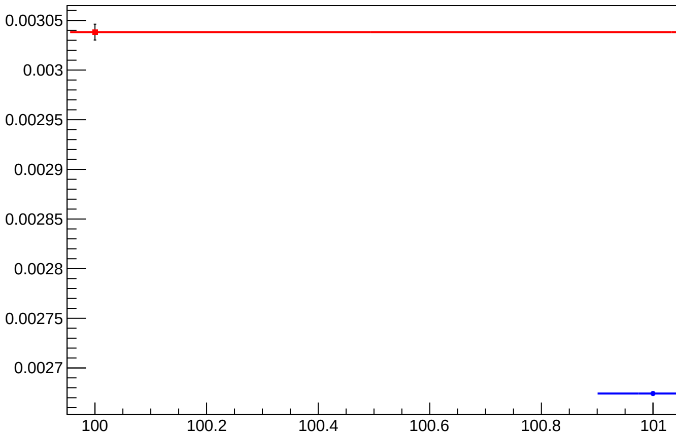
asym_us_avg_at1lr_avg_avg_eigen_dit_vs_dit_diff_rms vs Slug, Sign Corrected
