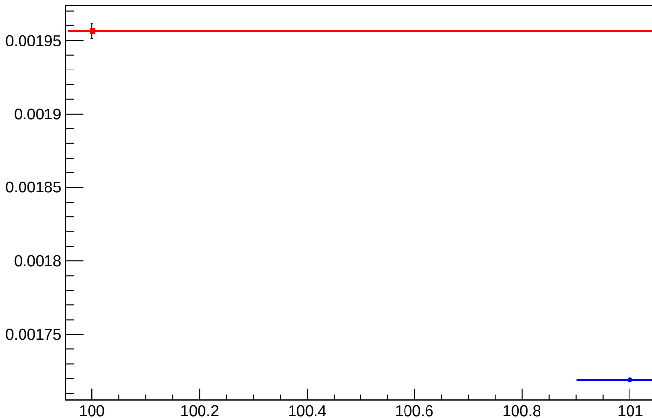
asym_at1_avg_eigen_dit_vs_dit_diff_rms vs Slug, Sign Corrected
