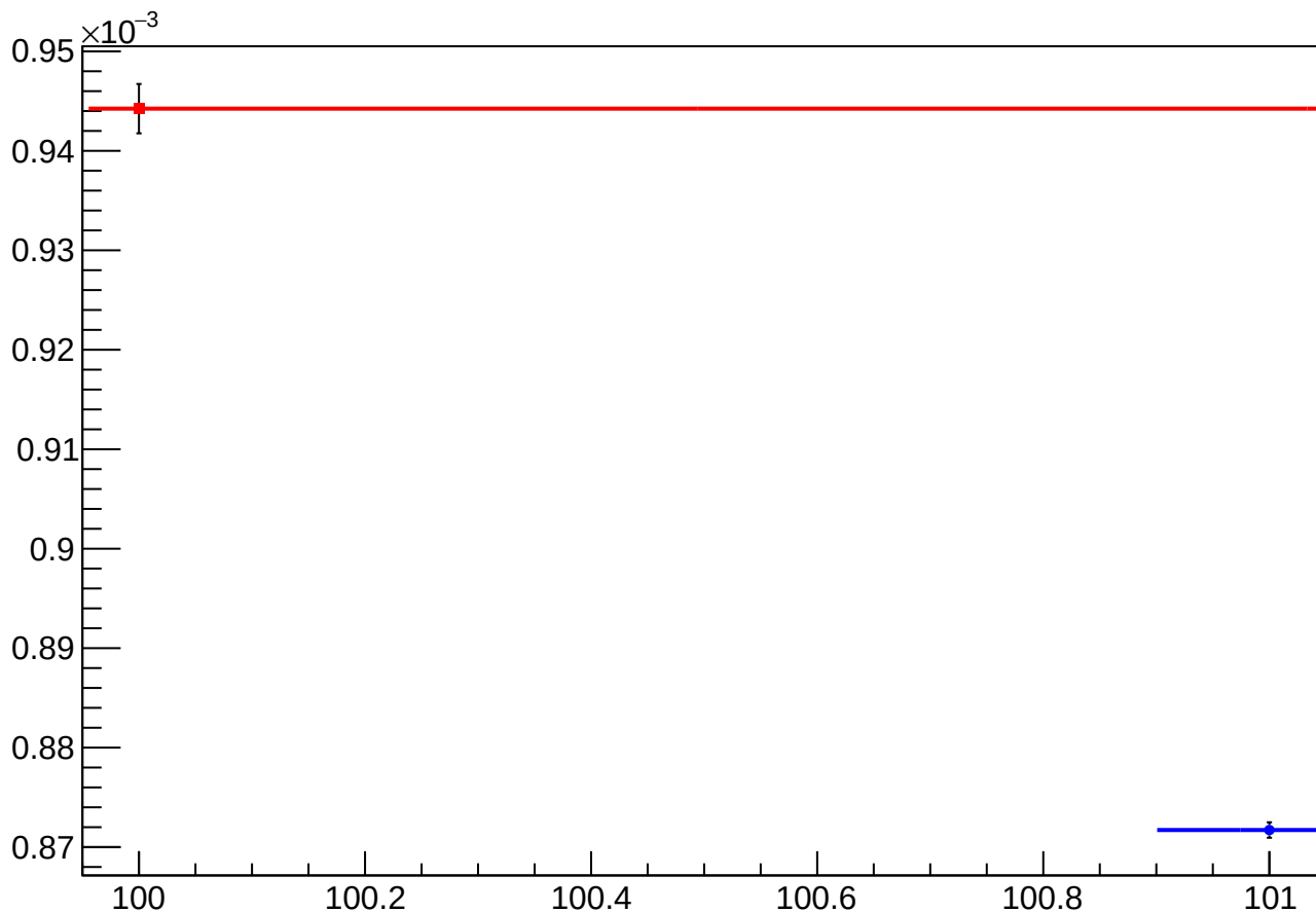
asym_us_avg_at1lr_avg_dd_eigen_dit_vs_dit_diff_rms vs Slug, Sign Corrected
