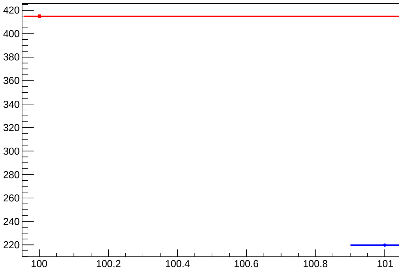
asym_atl_avg_atr_avg_avg_eigen_dit_vs_eigen_cor_diff_rms vs Slug, Sign Corrected
