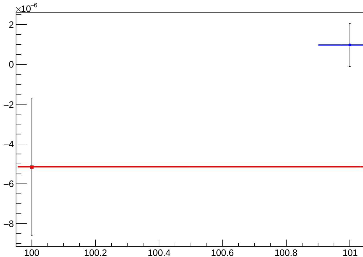
asym_us_dd_eigen_dit_vs_dit_diff_mean vs Slug, Sign Corrected
