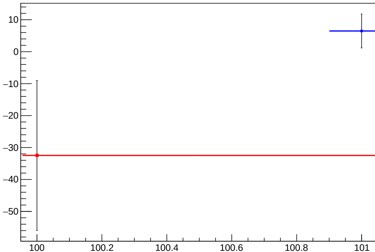
reg_asym_us_dd_at2lr_dd_avg_diff_bpm1X_slope vs Slug, Sign Corrected
