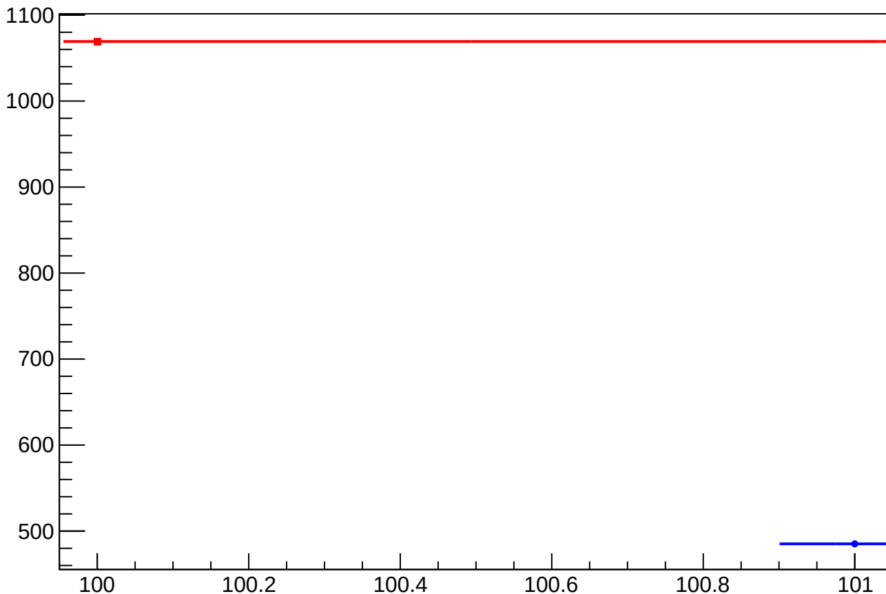
asym_atr2_eigen_dit_vs_cor_diff_rms vs Slug, Sign Corrected
