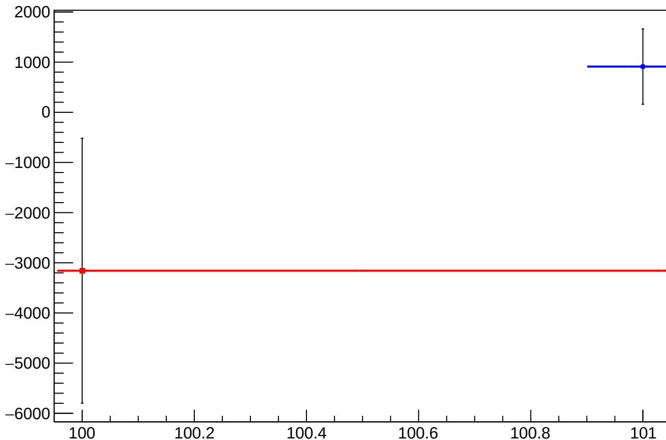
asym_sam_37_26_dd_eigen_cor_correction_mean vs Slug, Sign Corrected
