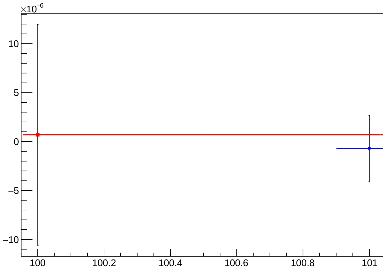
asym_us_avg_at1lr_avg_avg_eigen_dit_vs_dit_diff_mean vs Slug, Sign Corrected
