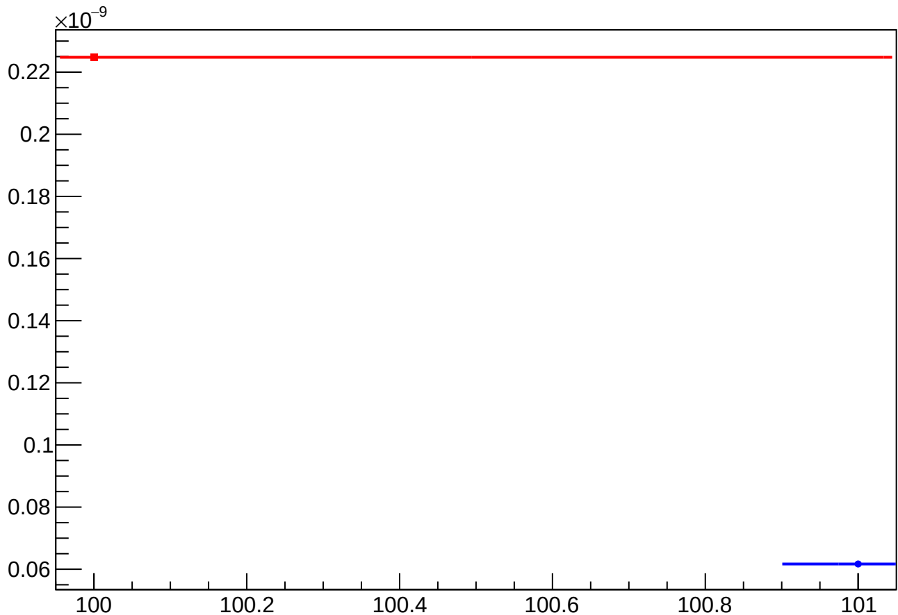
asym_sam_26_dd_eigen_cor_vs_cor_diff_rms vs Slug, Sign Corrected
