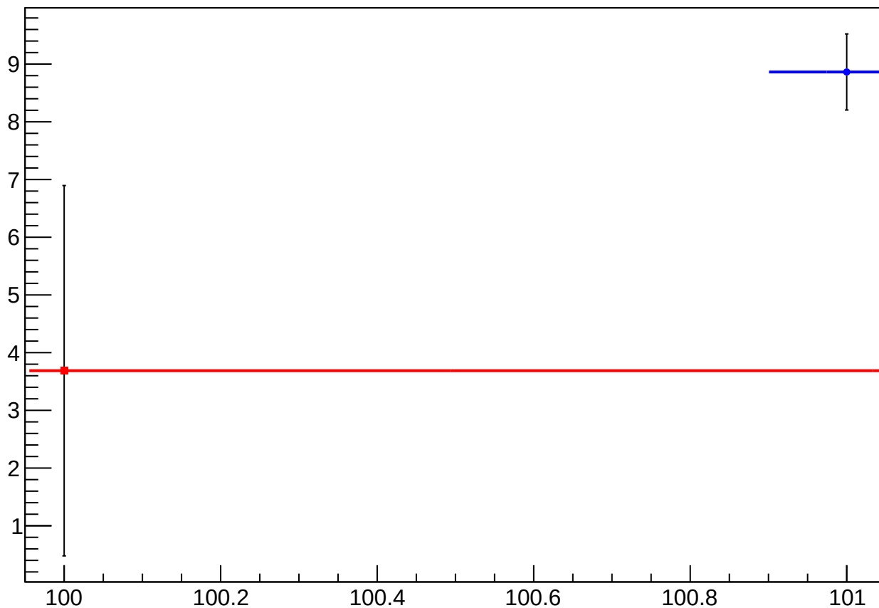
reg_asym_sam_1357_2468_dd_diff_bpm4eY_slope vs Slug, Sign Corrected
