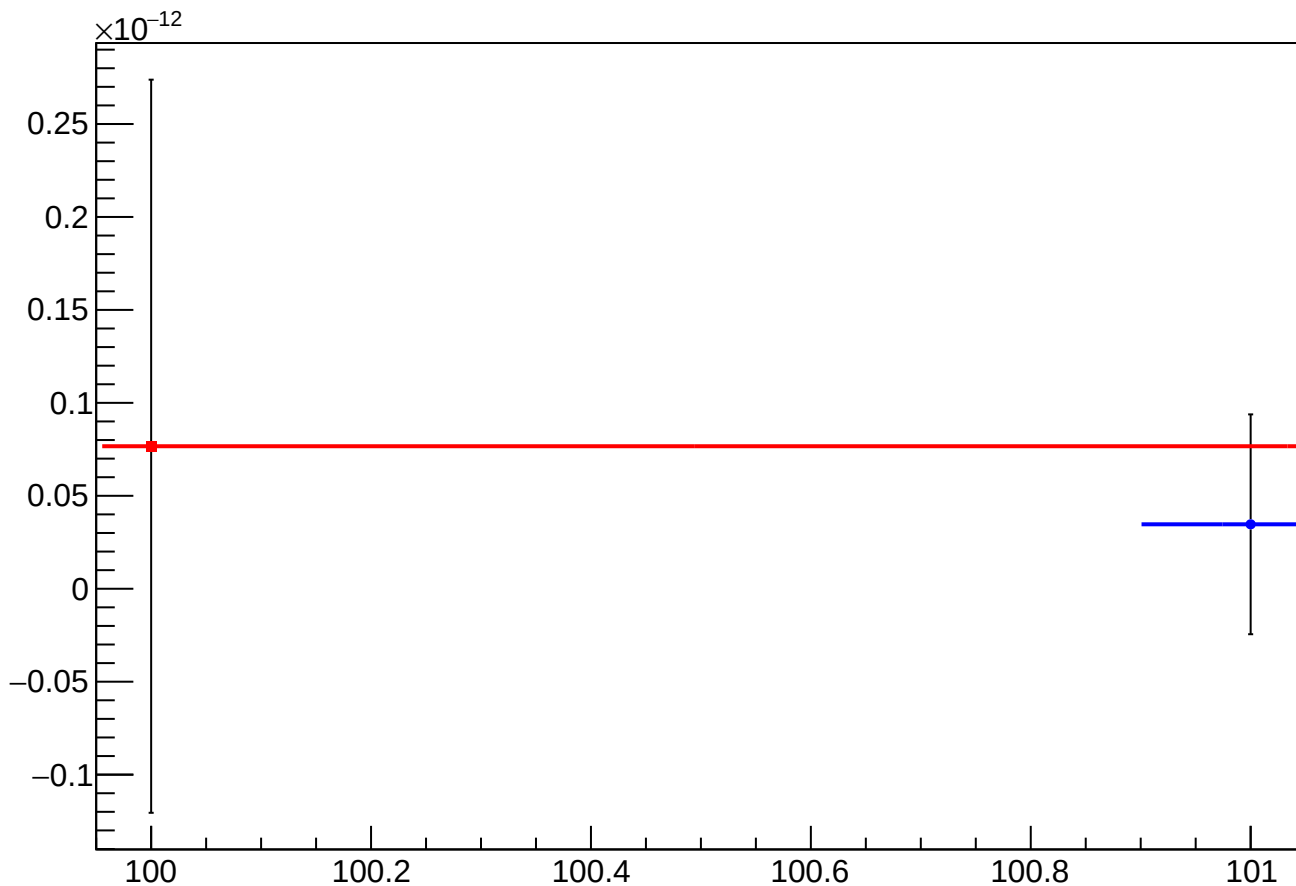
asym_us_dd_at1lr_dd_dd_eigen_cor_vs_cor_diff_mean vs Slug, Sign Corrected
