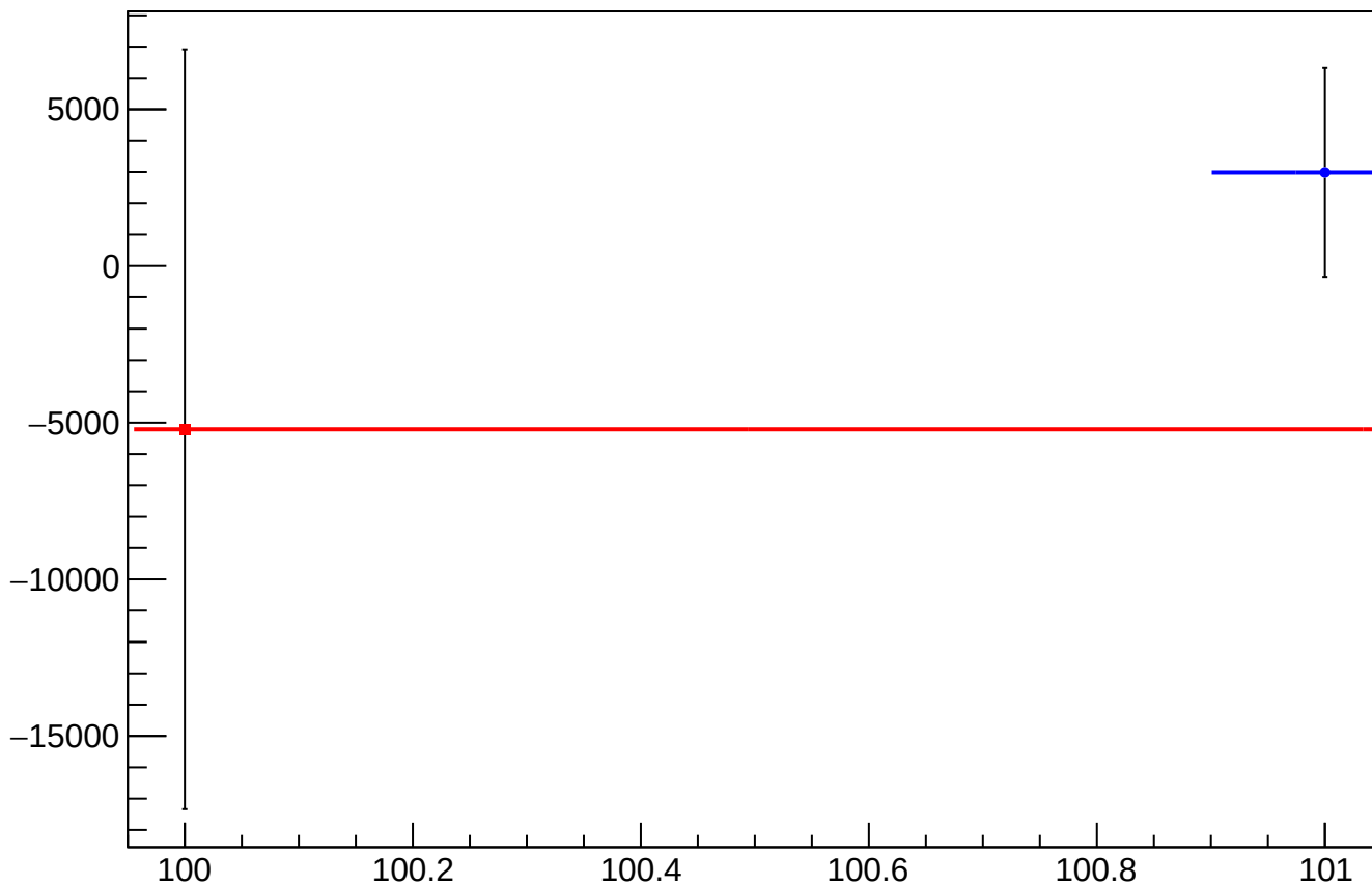
reg_asym_atl1_mean vs Slug, Sign Corrected
