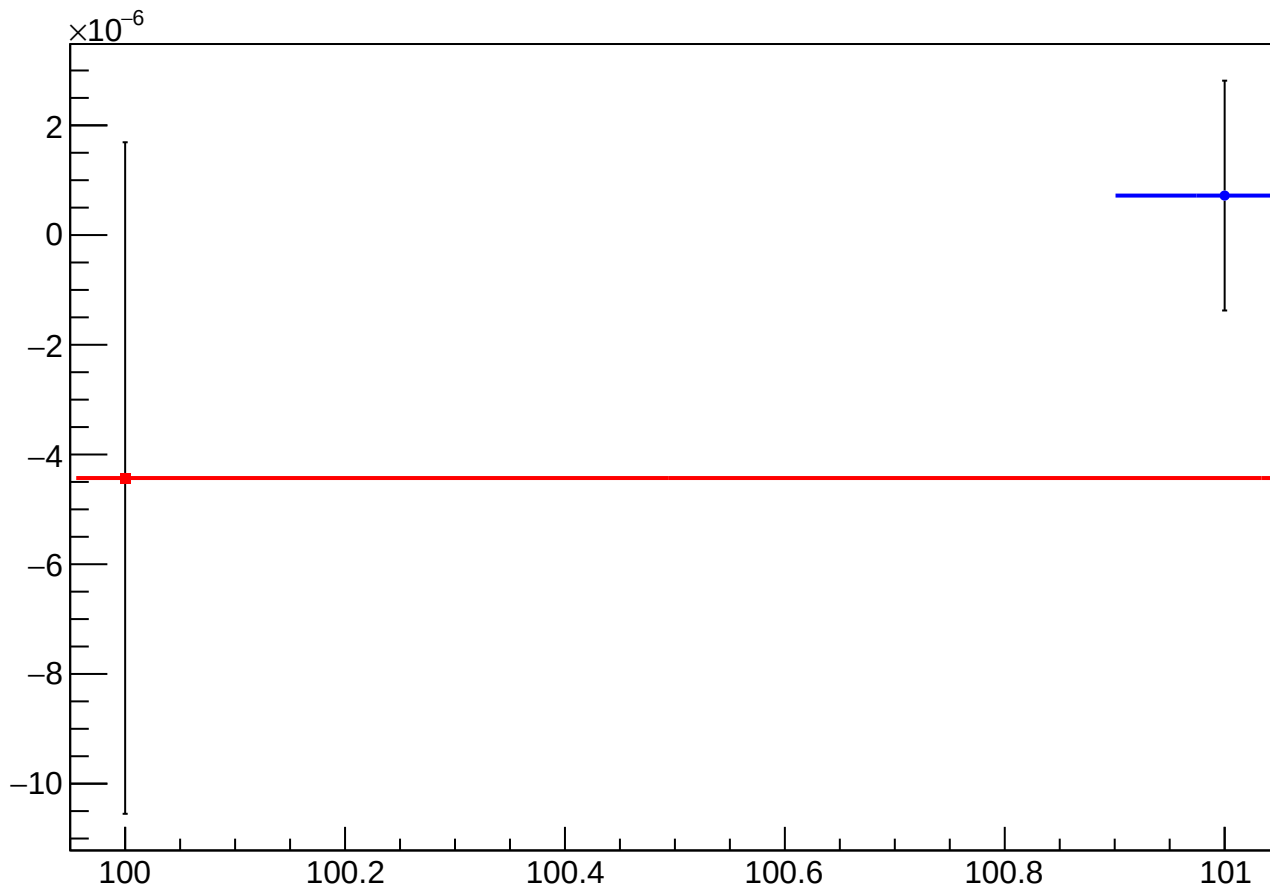
asym_usl_eigen_dit_vs_dit_diff_mean vs Slug, Sign Corrected
