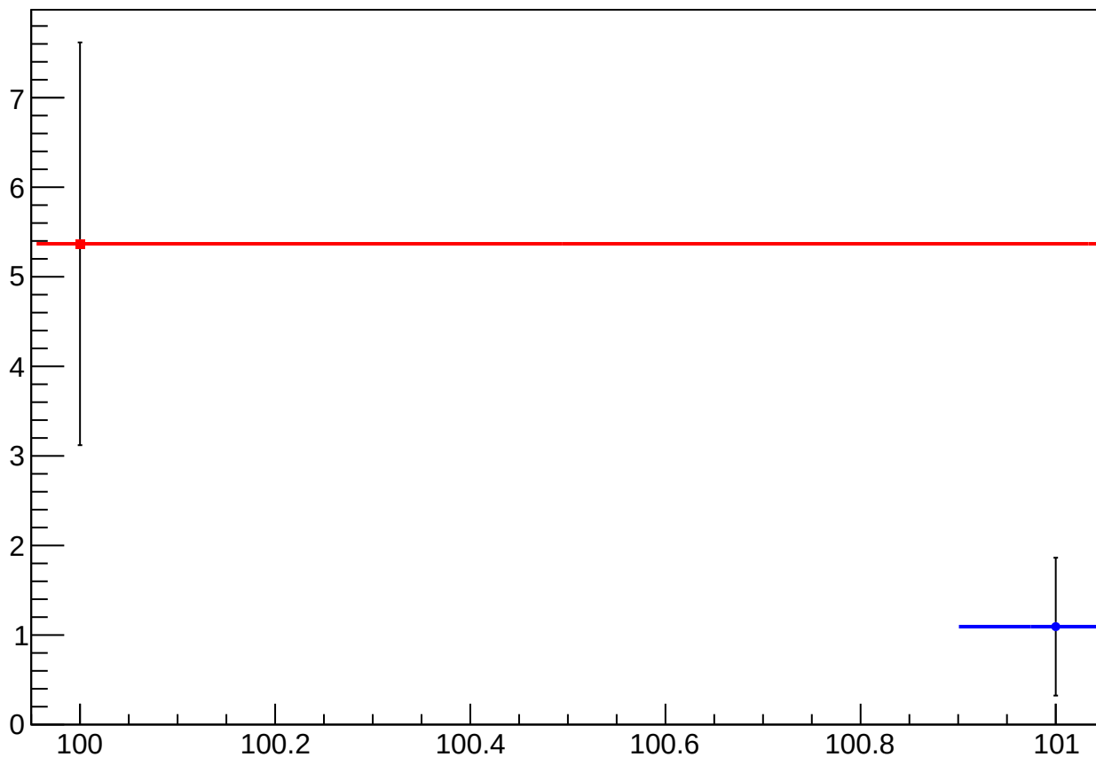
reg_asym_sam5_diff_bpm1X_slope vs Slug, Sign Corrected
