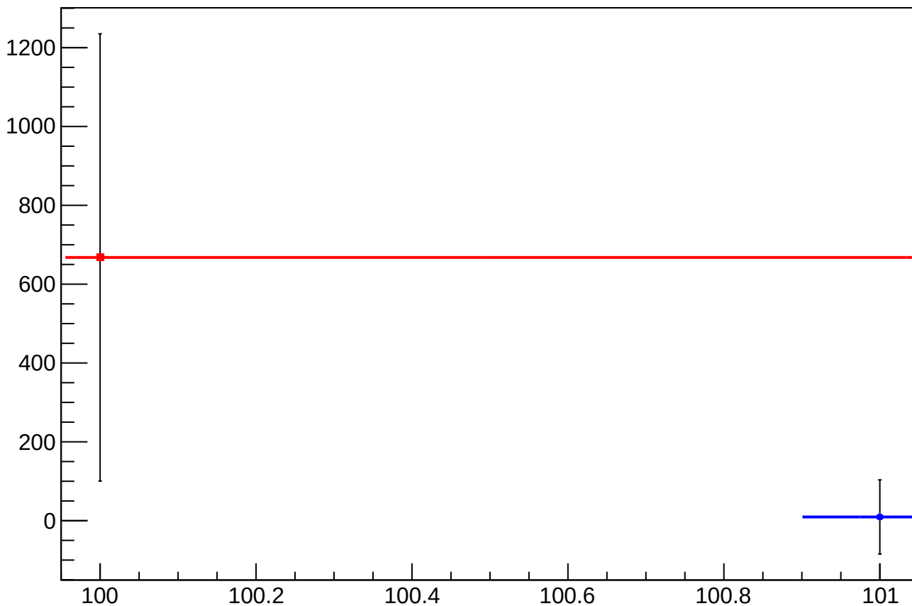
dit_asym_sam_1548_avg_mean vs Slug, Sign Corrected
