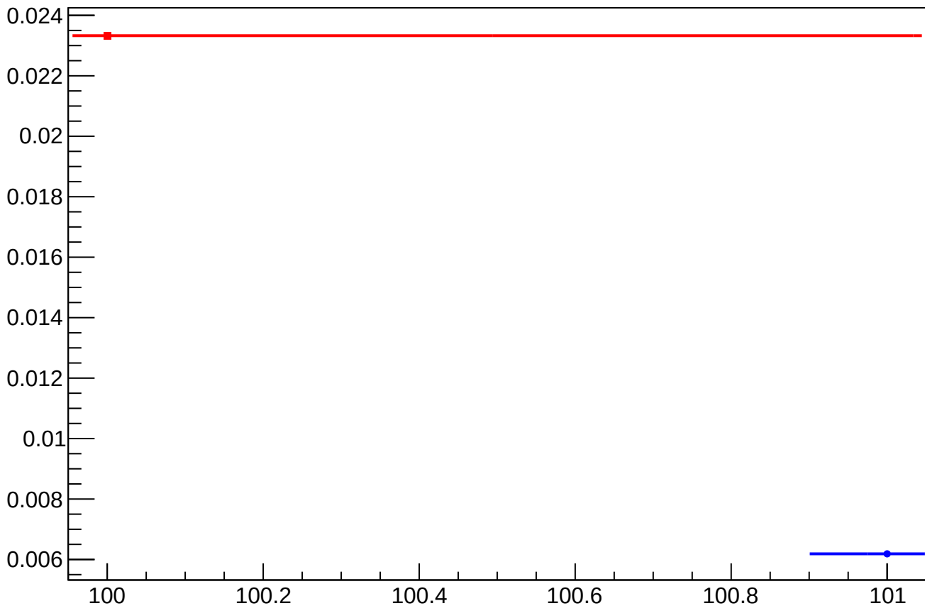
asym_at2_dd_eigen_dit_vs_dit_diff_rms vs Slug, Sign Corrected
