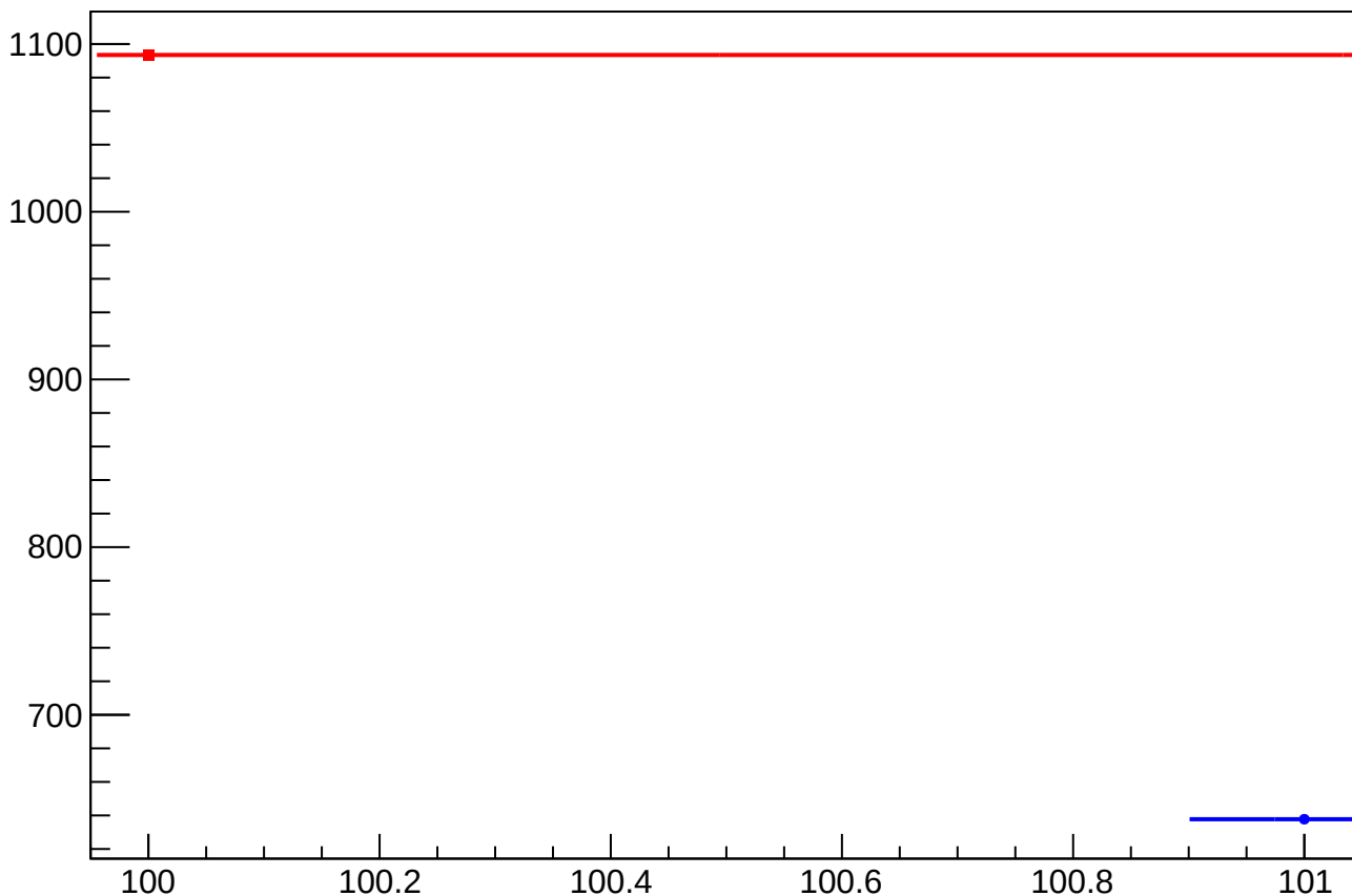
asym_at1_avg_eigen_cor_correction_rms vs Slug, Sign Corrected
