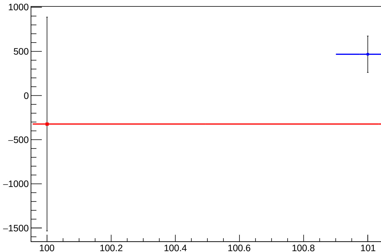
eigen_dit_asym_sam_3726_avg_mean vs Slug, Sign Corrected
