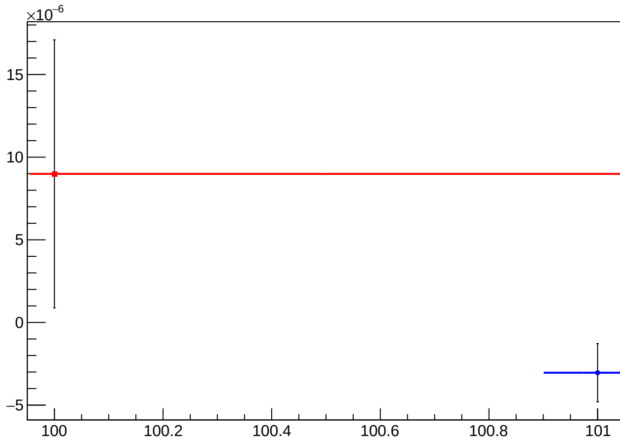
asym_usl_atl1_avg_eigen_dit_vs_dit_diff_mean vs Slug, Sign Corrected
