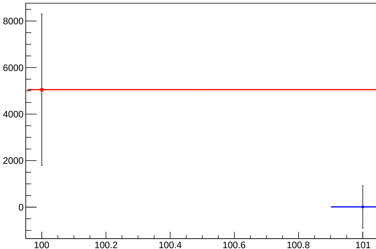
eigen_dit_asym_us_dd_mean vs Slug, Sign Corrected
