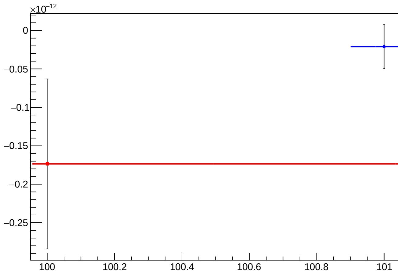
asym_usl_atl1_dd_eigen_cor_vs_cor_diff_mean vs Slug, Sign Corrected
