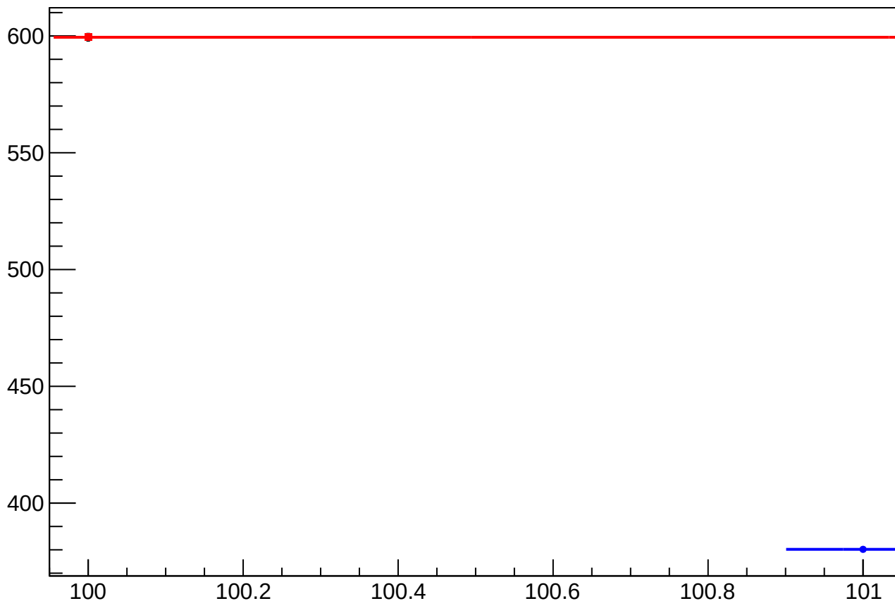
asym_usl_atl1_avg_eigen_dit_correction_rms vs Slug, Sign Corrected
