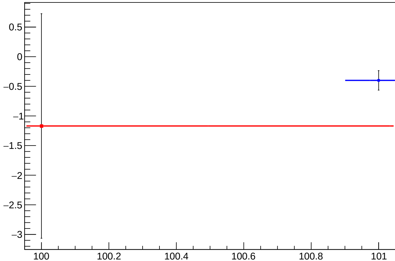
asym_us_avg_at1lr_avg_avg_eigen_dit_vs_cor_diff_mean vs Slug, Sign Corrected
