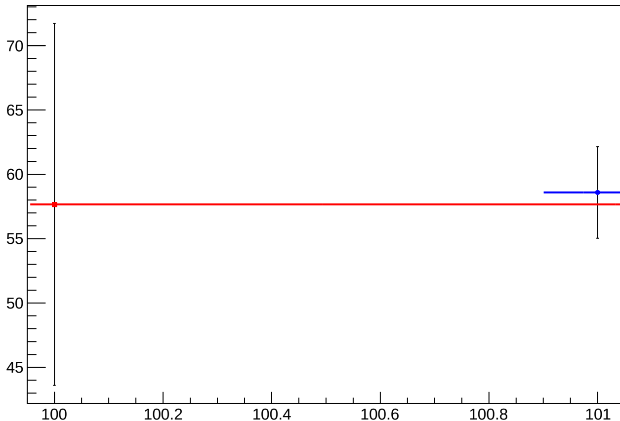
reg_asym_us_dd_atlr_dd_dd_diff_bpm4eX_slope vs Slug, Sign Corrected
