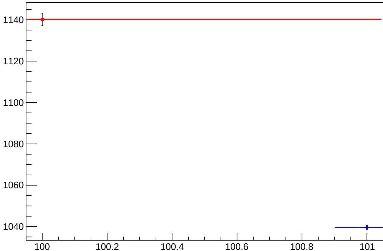
diff_bpm_4aY_4acY_dd_rms vs Slug, Sign Corrected
