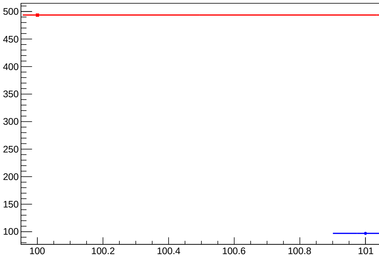
asym_us_avg_at1lr_avg_dd_eigen_dit_vs_cor_diff_rms vs Slug, Sign Corrected
