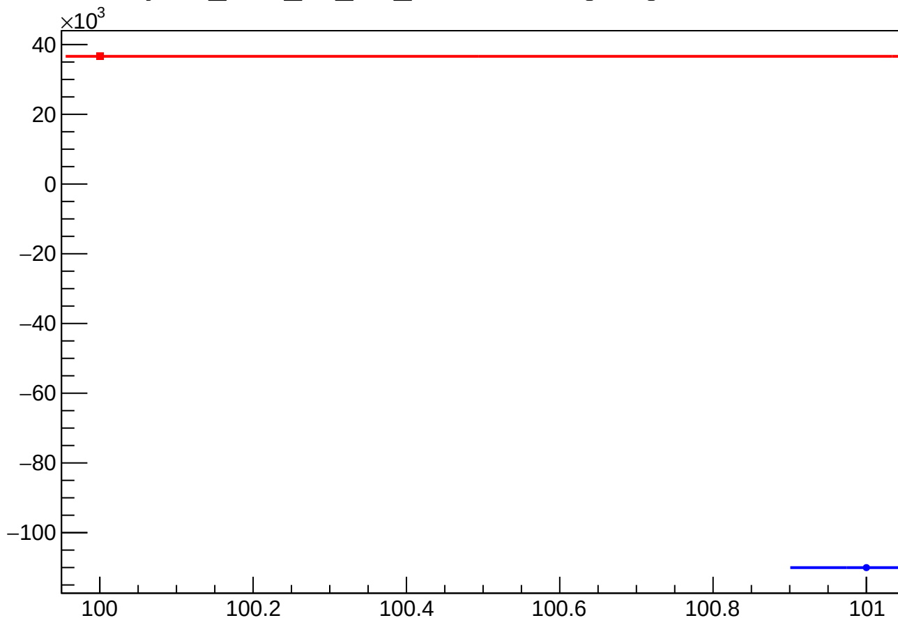
yield_bcm_an_diff_mean vs Slug, Sign Corrected
