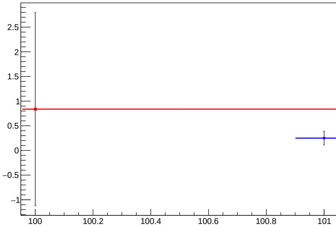
asym_us_avg_at1lr_avg_dd_dit_vs_eigen_cor_diff_mean vs Slug, Sign Corrected
