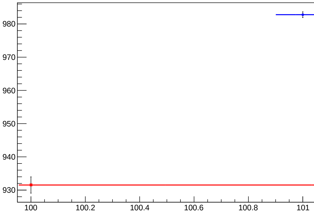
asym_usl_atl1_dd_dit_correction_rms vs Slug, Sign Corrected
