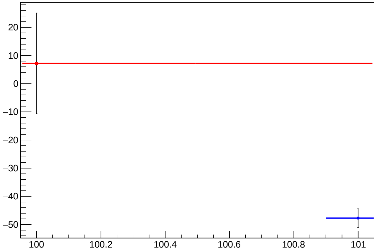
reg_asym_sam_26_dd_diff_bpm4eY_slope vs Slug, Sign Corrected
