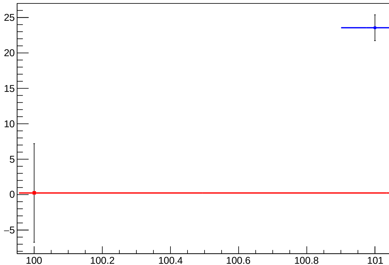
reg_asym_usl_atl1_dd_diff_bpm4eX_slope vs Slug, Sign Corrected
