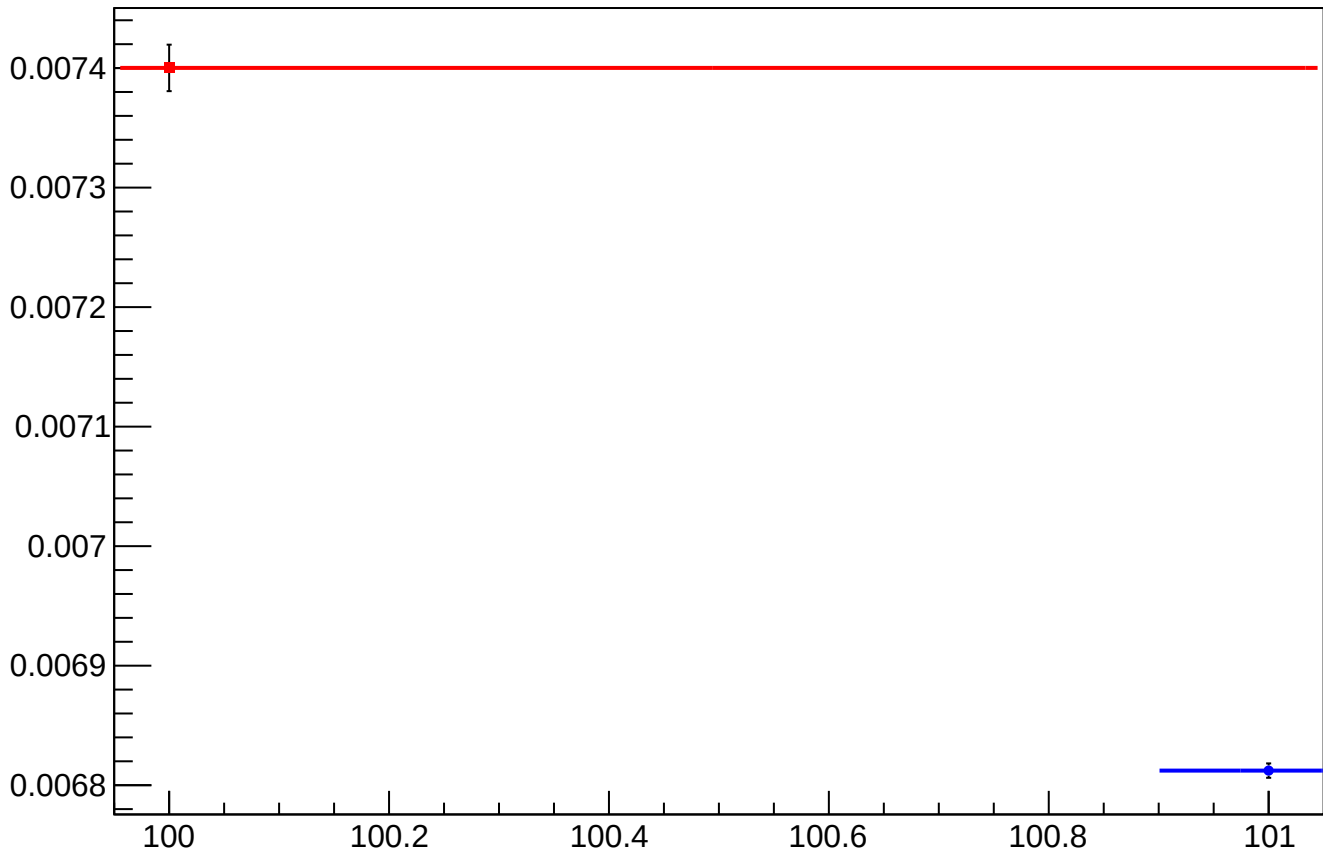
asym_usl_atl2_dd_eigen_dit_vs_dit_diff_rms vs Slug, Sign Corrected
