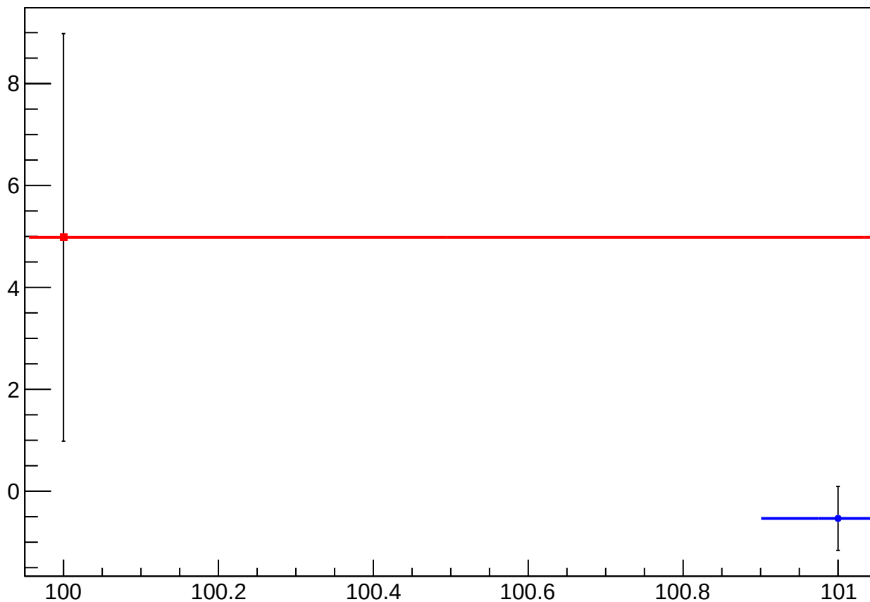
asym_atr2_eigen_dit_vs_eigen_cor_diff_mean vs Slug, Sign Corrected
