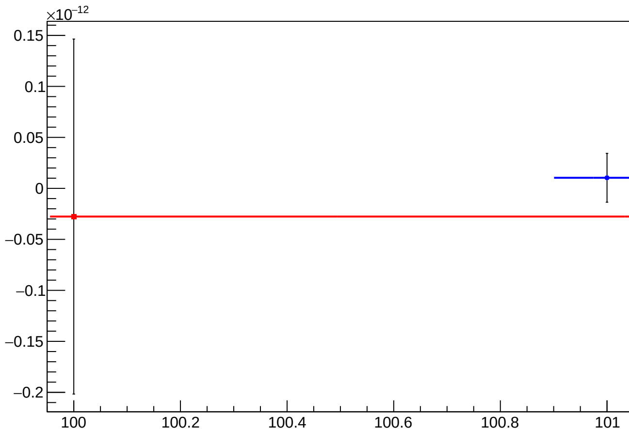
asym_usl_eigen_cor_vs_cor_diff_mean vs Slug, Sign Corrected
