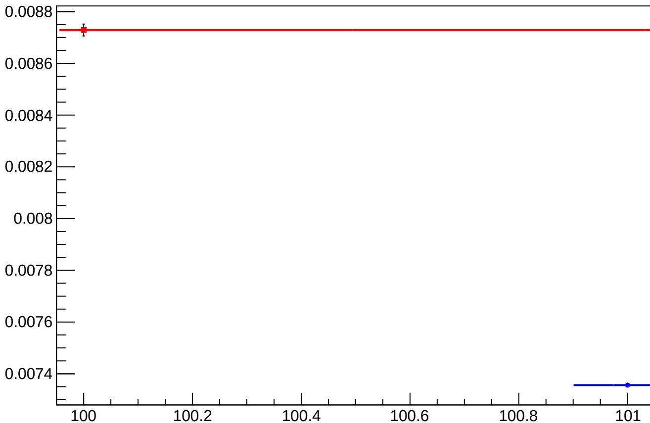
asym_sam2_eigen_dit_vs_dit_diff_rms vs Slug, Sign Corrected
