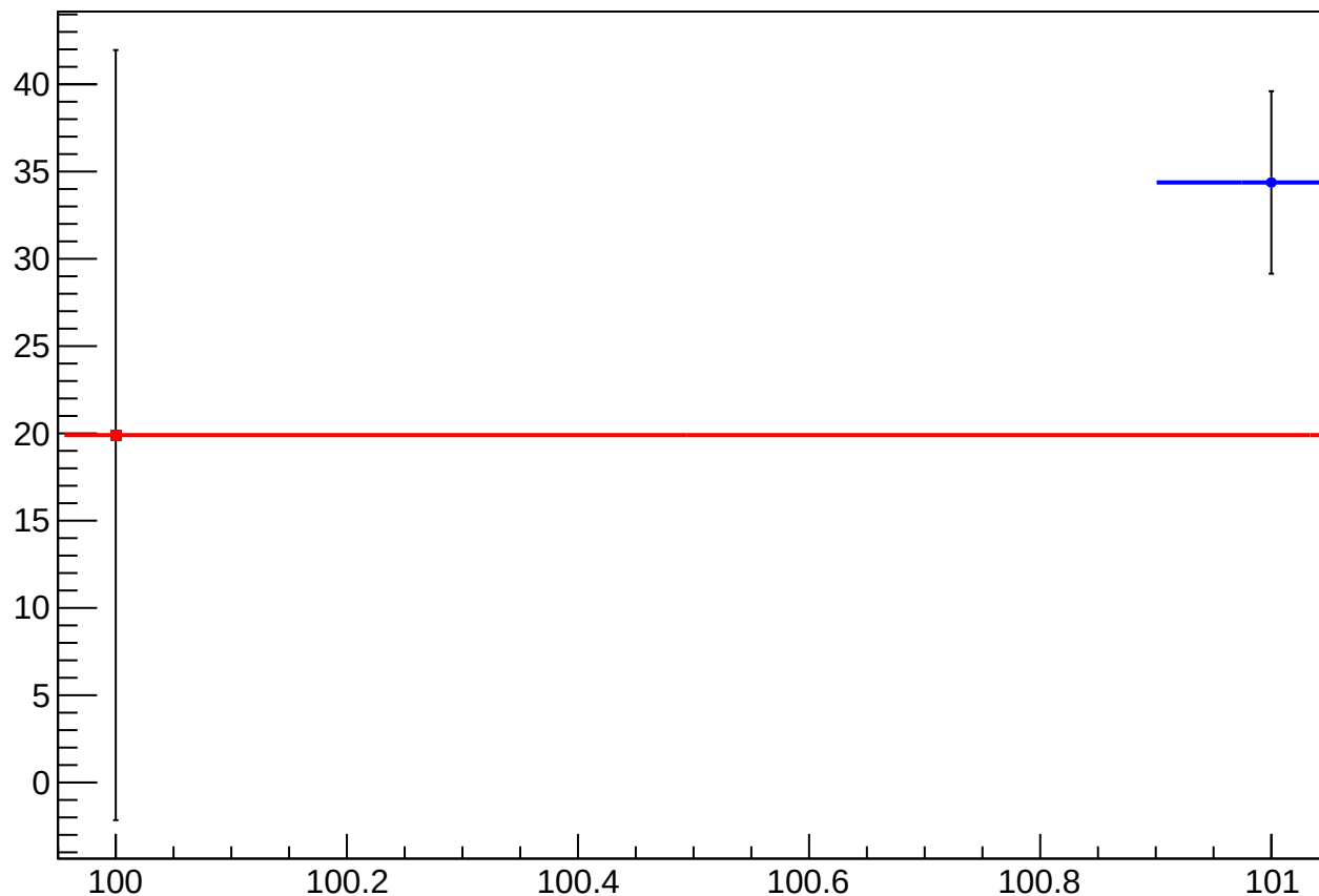
reg_asym_us_dd_atlr_dd_avg_diff_bpm1X_slope vs Slug, Sign Corrected
