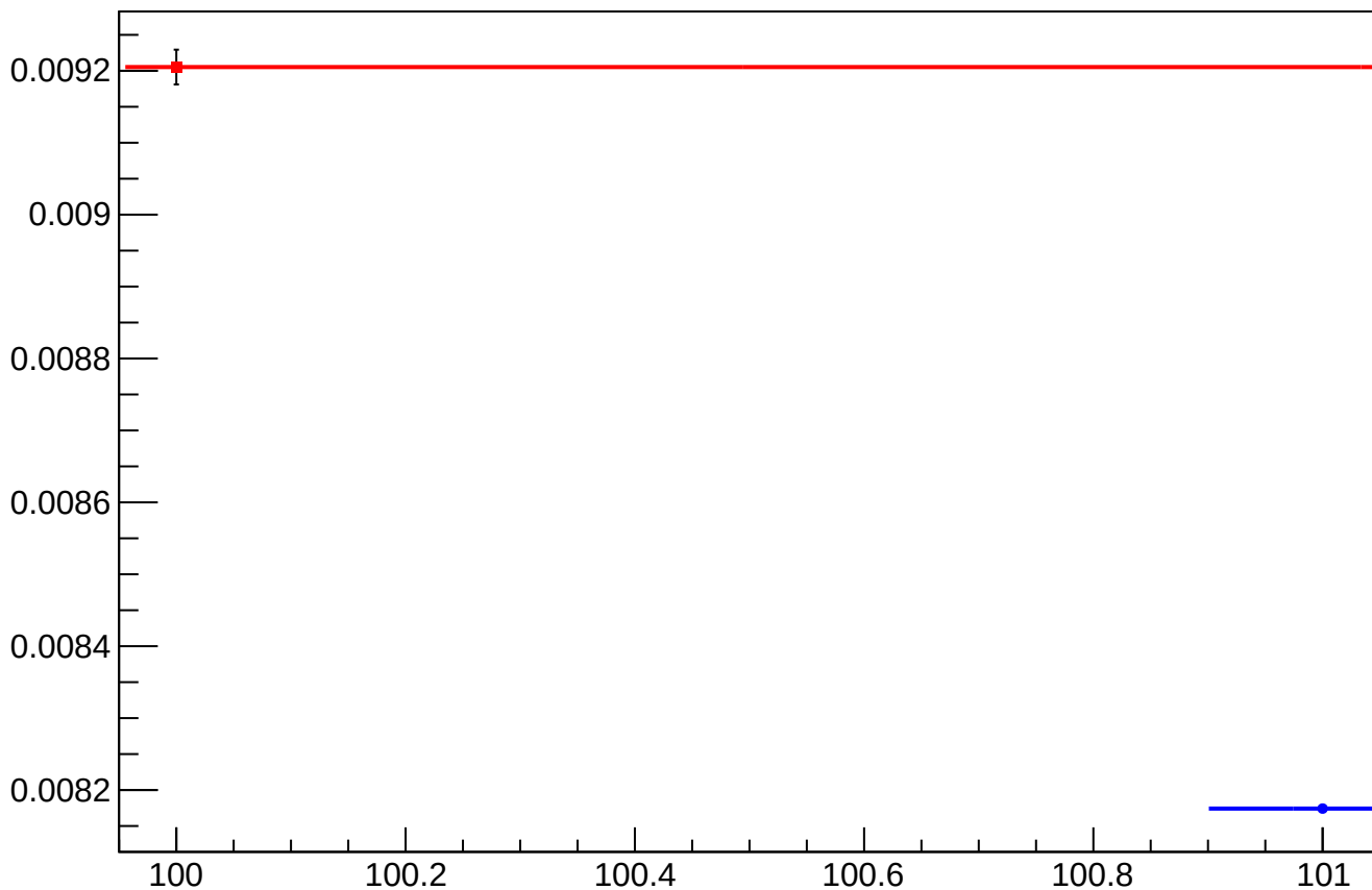
asym_atl_avg_eigen_dit_vs_dit_diff_rms vs Slug, Sign Corrected
