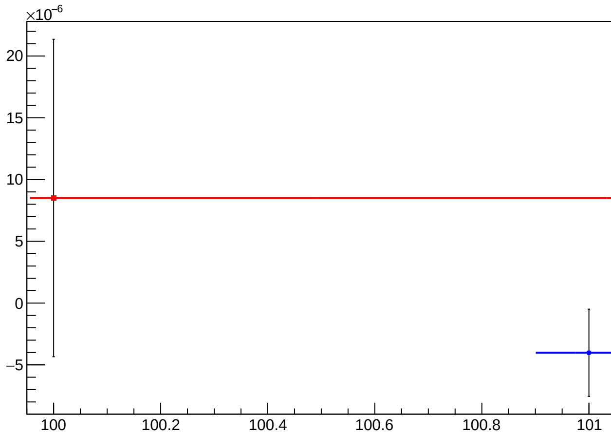
asym_sam_26_avg_eigen_dit_vs_dit_diff_mean vs Slug, Sign Corrected
