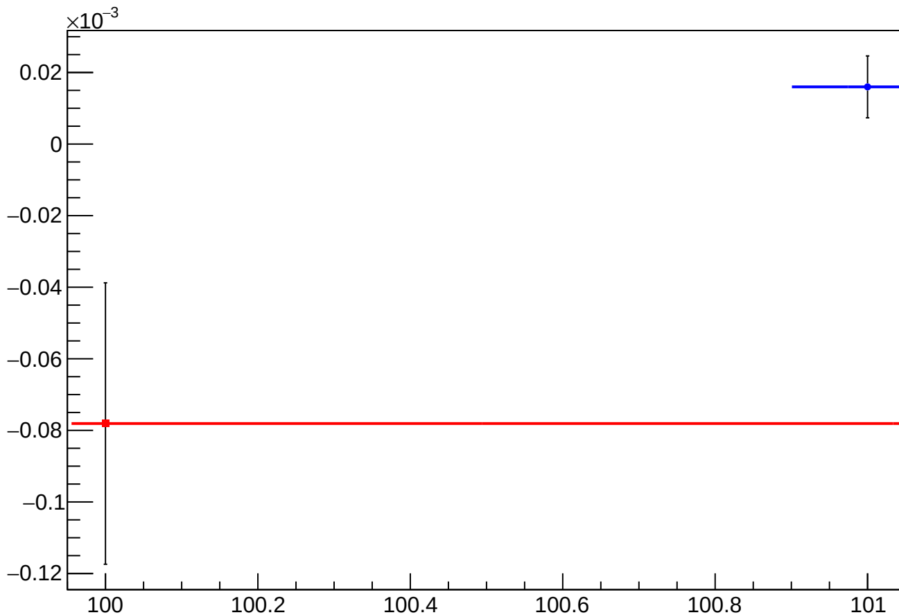
asym_sam3_eigen_dit_vs_dit_diff_mean vs Slug, Sign Corrected
