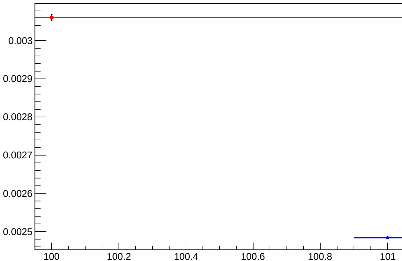
asym_sam_3726_avg_eigen_dit_vs_dit_diff_rms vs Slug, Sign Corrected
