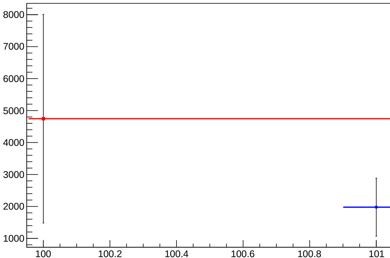
eigen_dit_asym_us_avg_mean vs Slug, Sign Corrected
