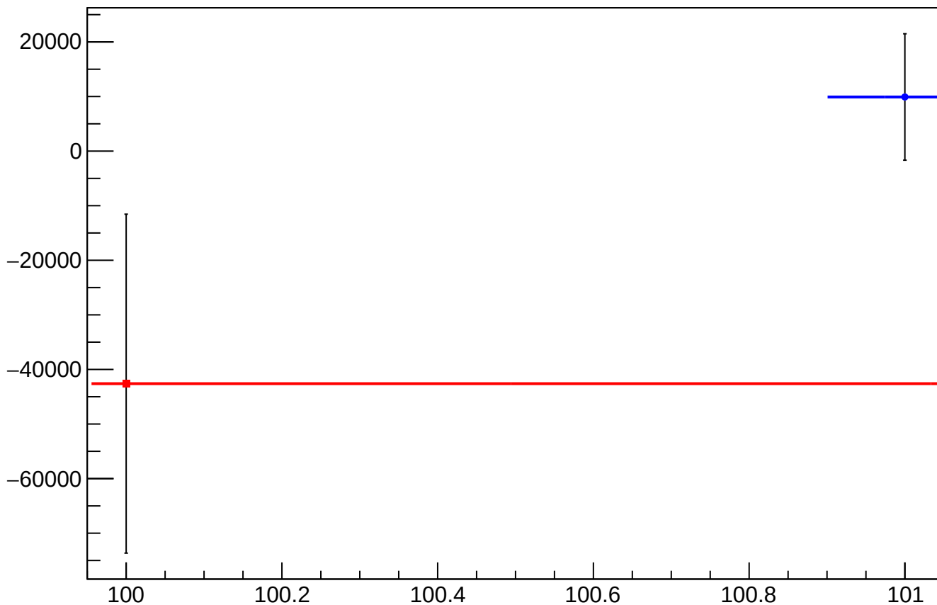
asym_atl2_mean vs Slug, Sign Corrected
