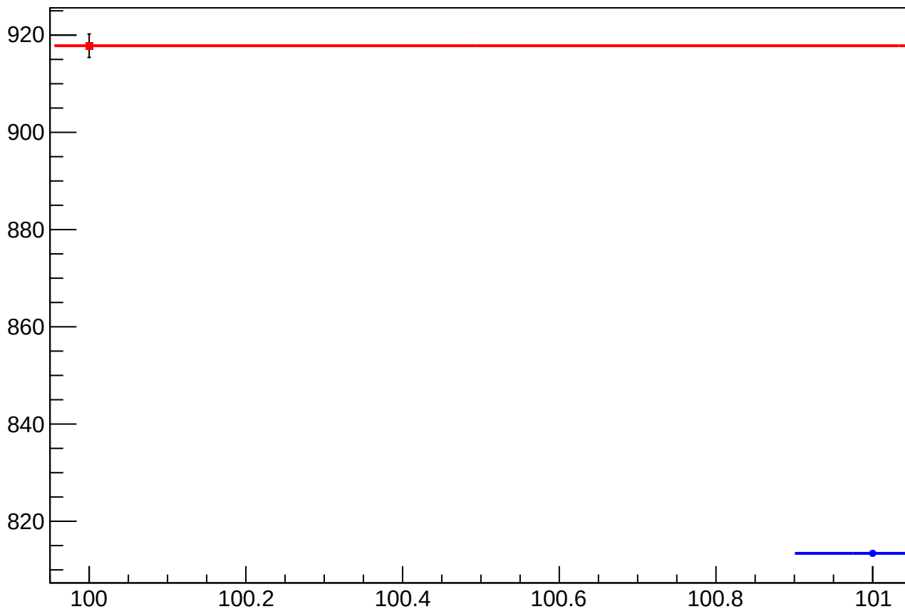
asym_us_avg_eigen_dit_correction_rms vs Slug, Sign Corrected
