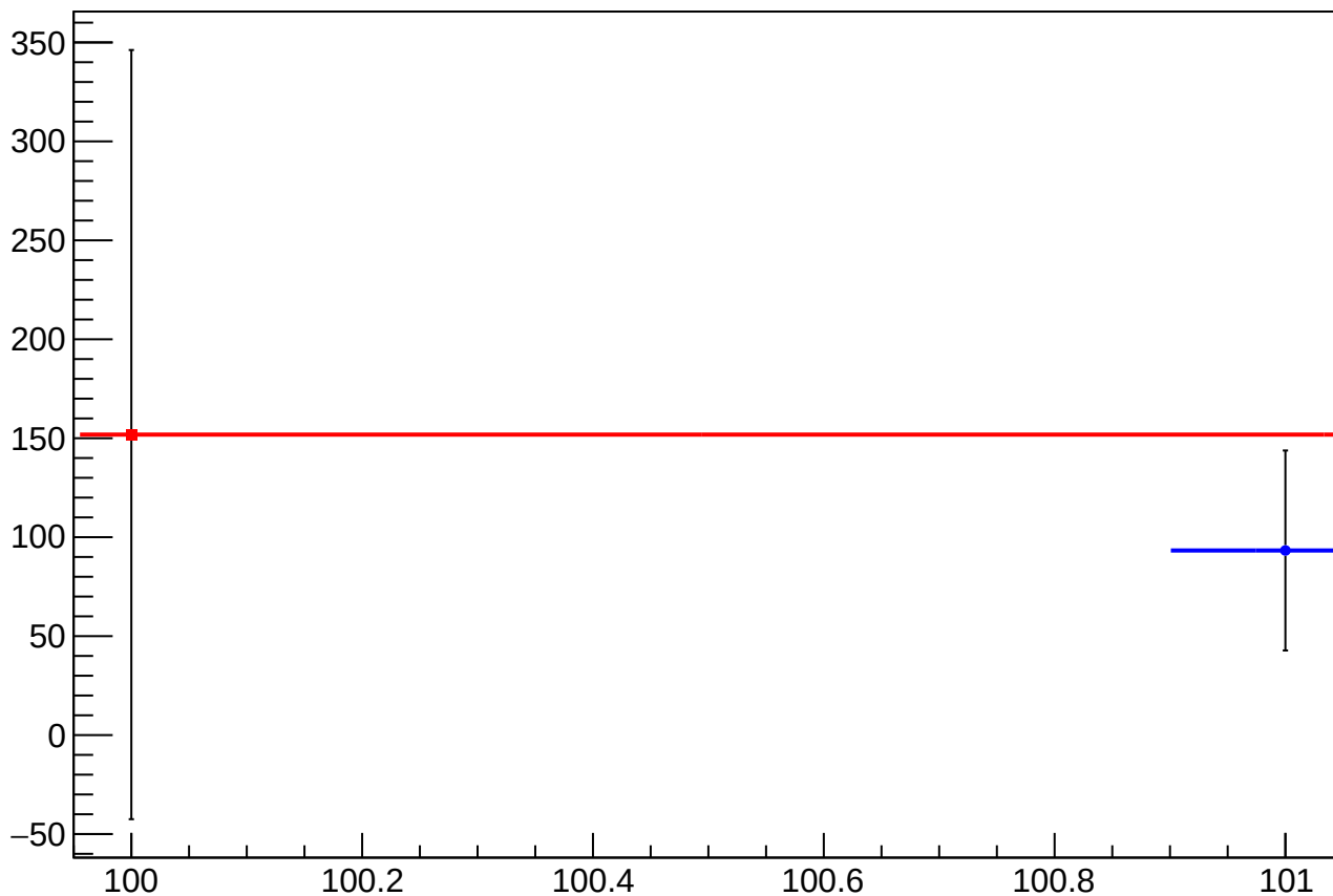
eigen_cor_asym_sam_15_avg_mean vs Slug, Sign Corrected
