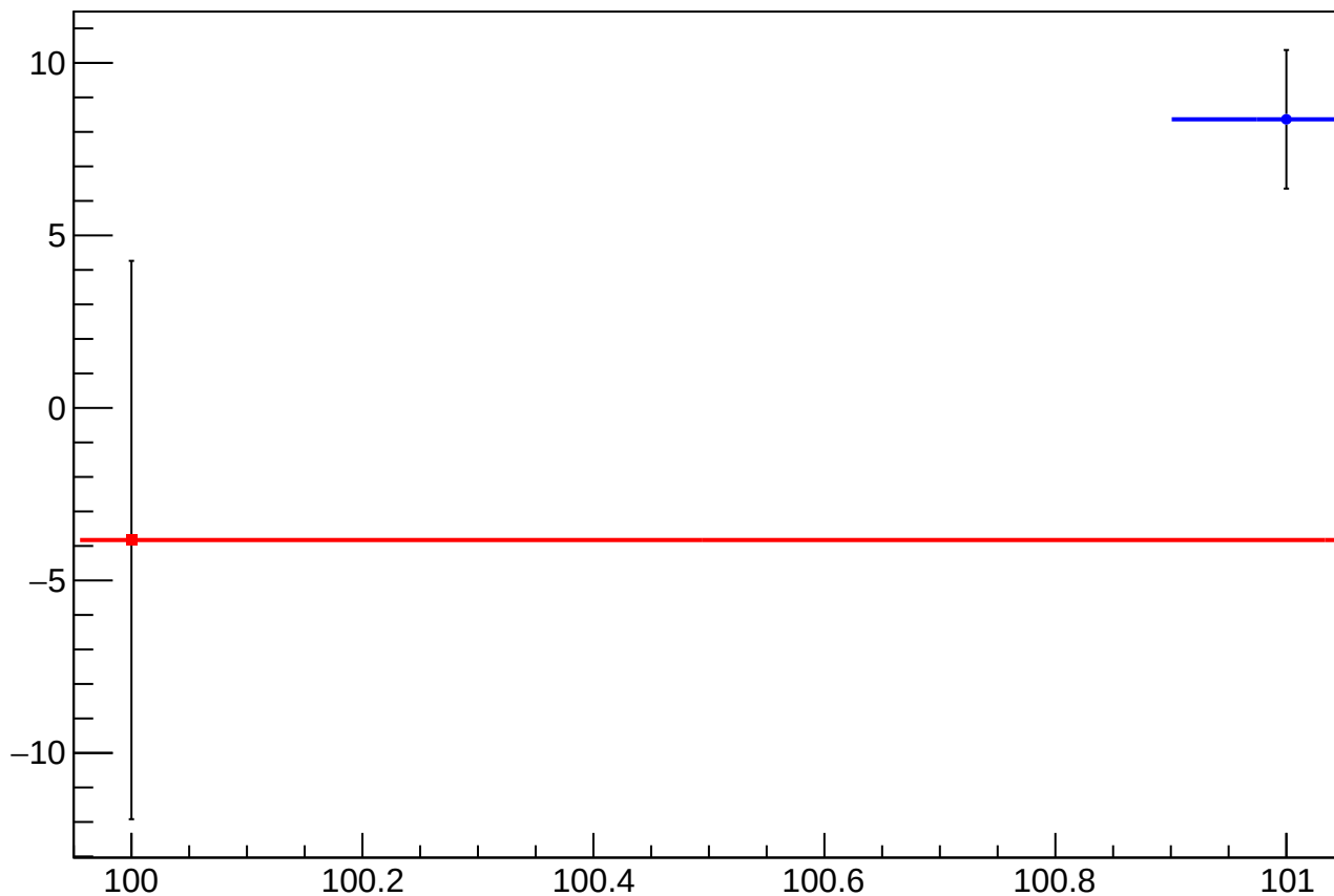
reg_asym_usl_atl1_avg_diff_bpm1X_slope vs Slug, Sign Corrected
