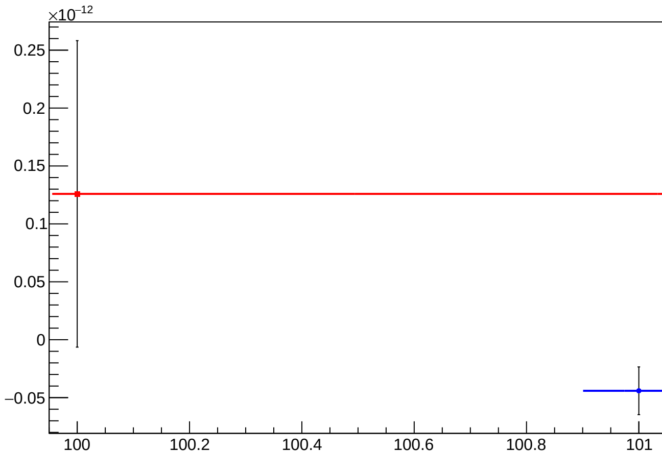
asym_sam_15_48_dd_eigen_cor_vs_cor_diff_mean vs Slug, Sign Corrected
