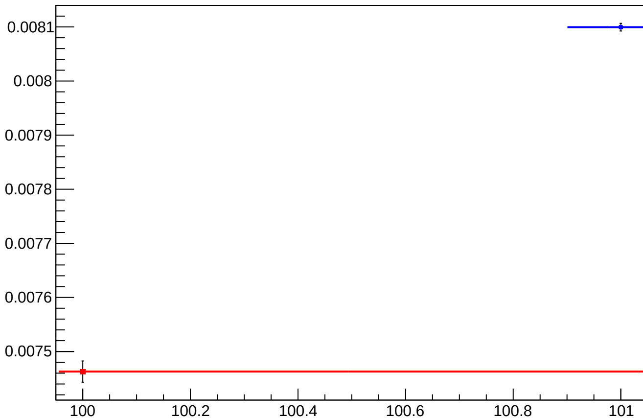
asym_atl_dd_eigen_dit_vs_dit_diff_rms vs Slug, Sign Corrected
