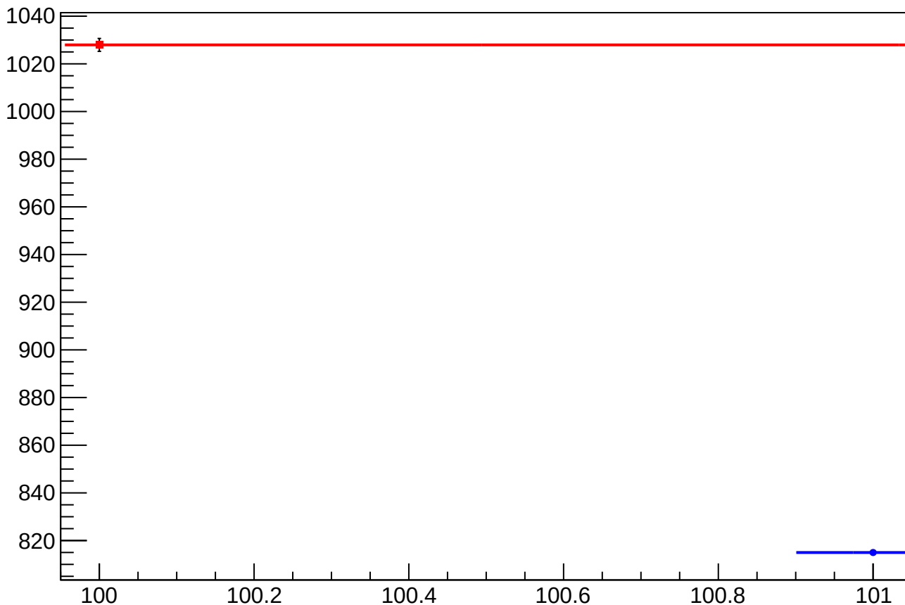
asym_sam_26_48_dd_eigen_dit_correction_rms vs Slug, Sign Corrected
