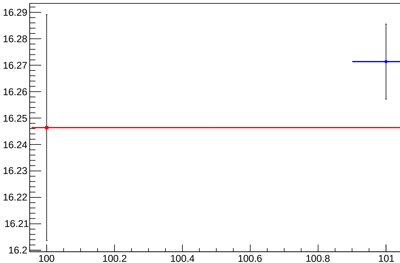
asym_bcm_an_us_ds3_avg_bcm_dg_ds_agg_dd_rms vs Slug, Sign Corrected
