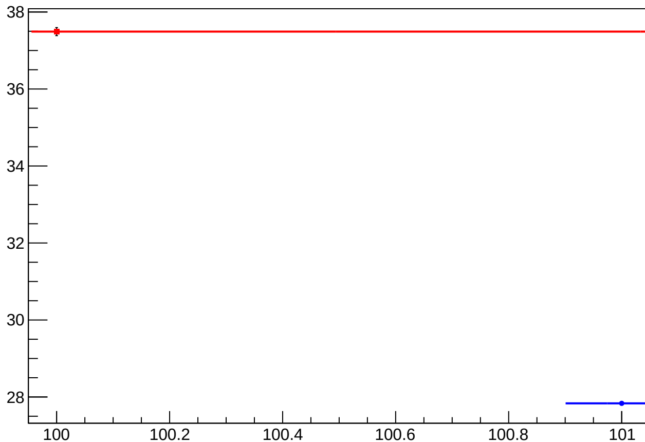
asym_us_dd_dit_vs_eigen_cor_diff_rms vs Slug, Sign Corrected
