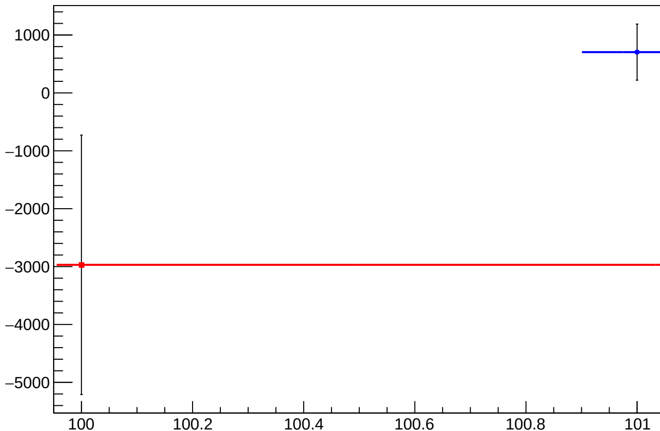
asym_us_avg_at1lr_avg_dd_eigen_dit_correction_mean vs Slug, Sign Corrected
