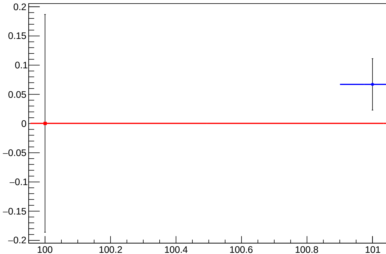
asym_sam_37_dd_eigen_dit_vs_cor_diff_mean vs Slug, Sign Corrected
