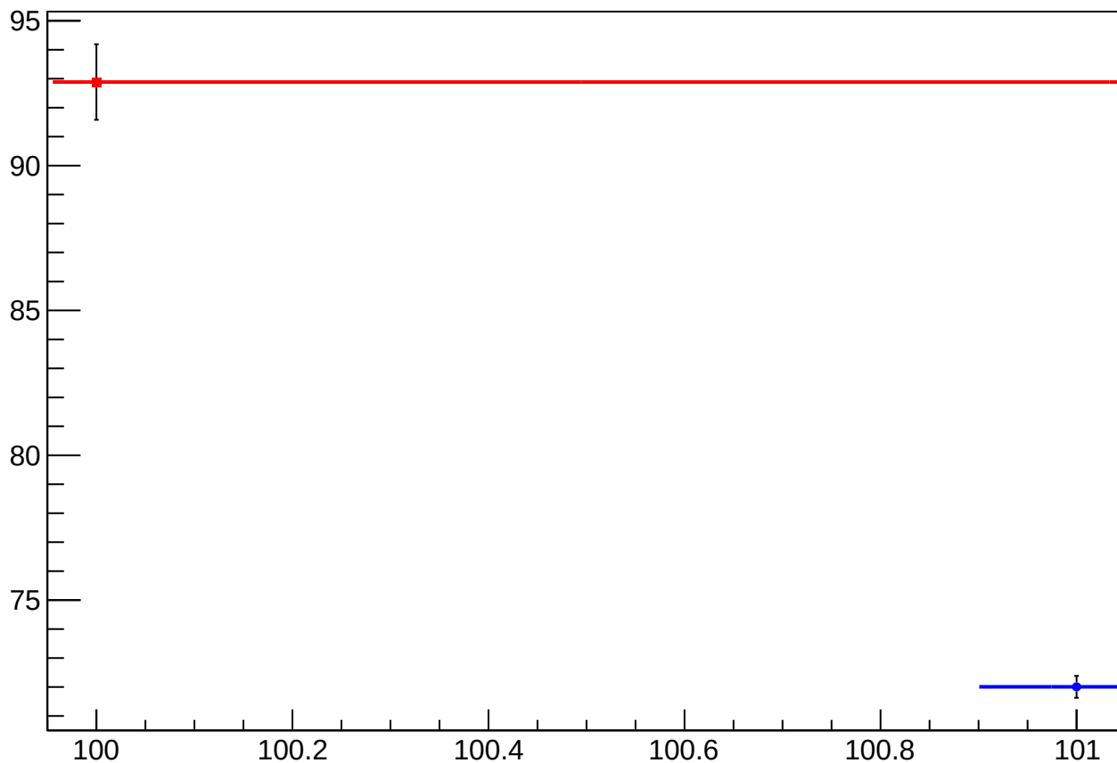
reg_asym_us_dd_at1lr_dd_avg_diff_bpm12X_slope vs Slug, Sign Corrected
