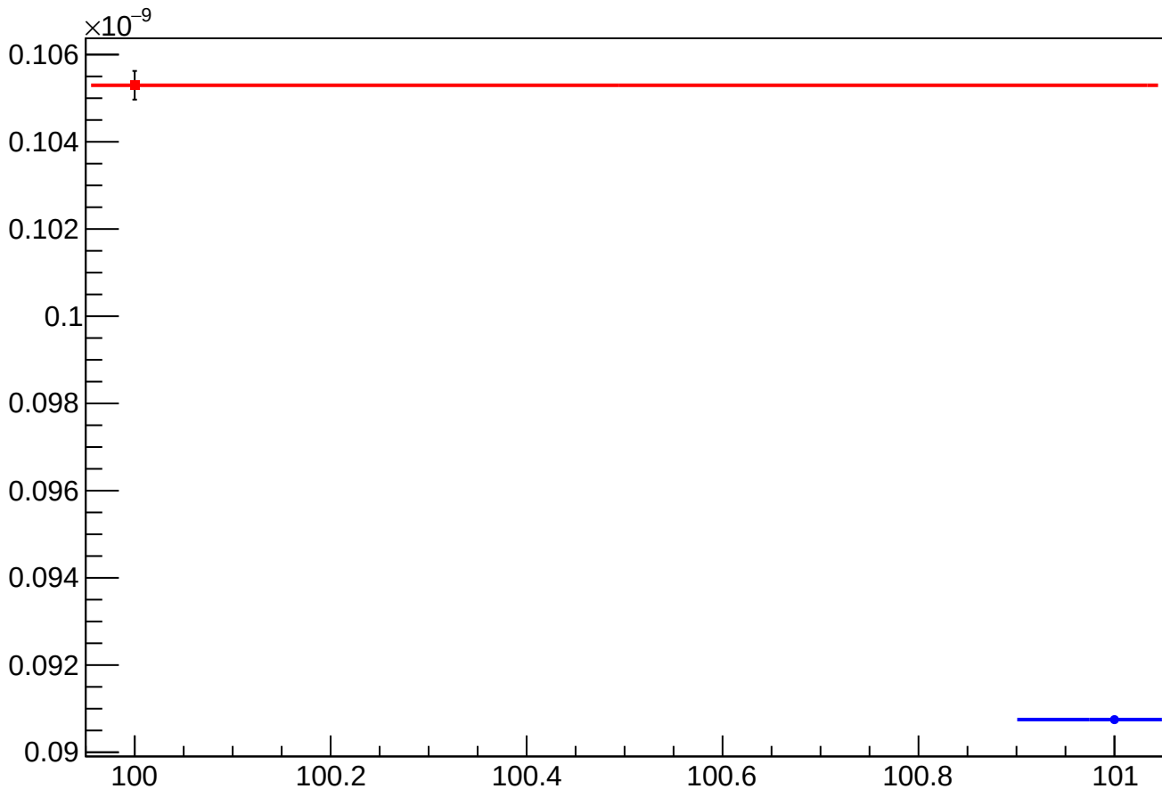
asym_atl_avg_atr_avg_avg_eigen_cor_vs_cor_diff_rms vs Slug, Sign Corrected
