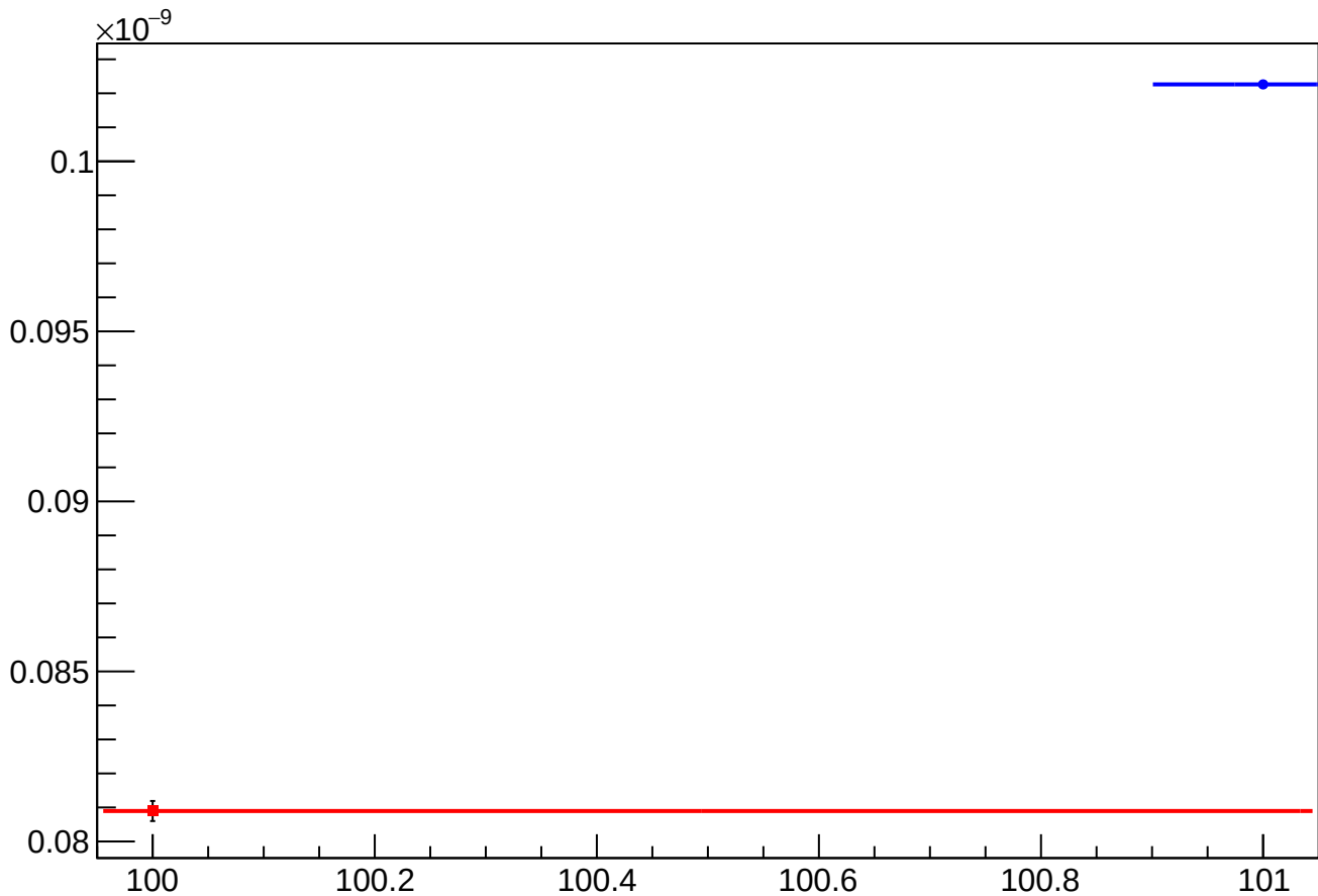
asym_atl1r2_dd_atl2r1_dd_dd_reg_vs_cor_diff_rms vs Slug, Sign Corrected
