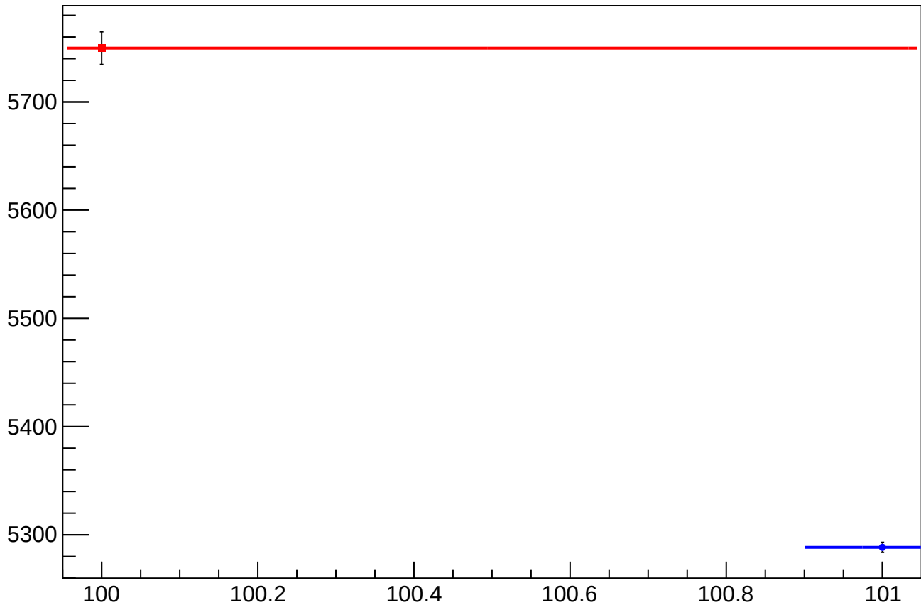
asym_atl1r2_dd_eigen_dit_correction_rms vs Slug, Sign Corrected
