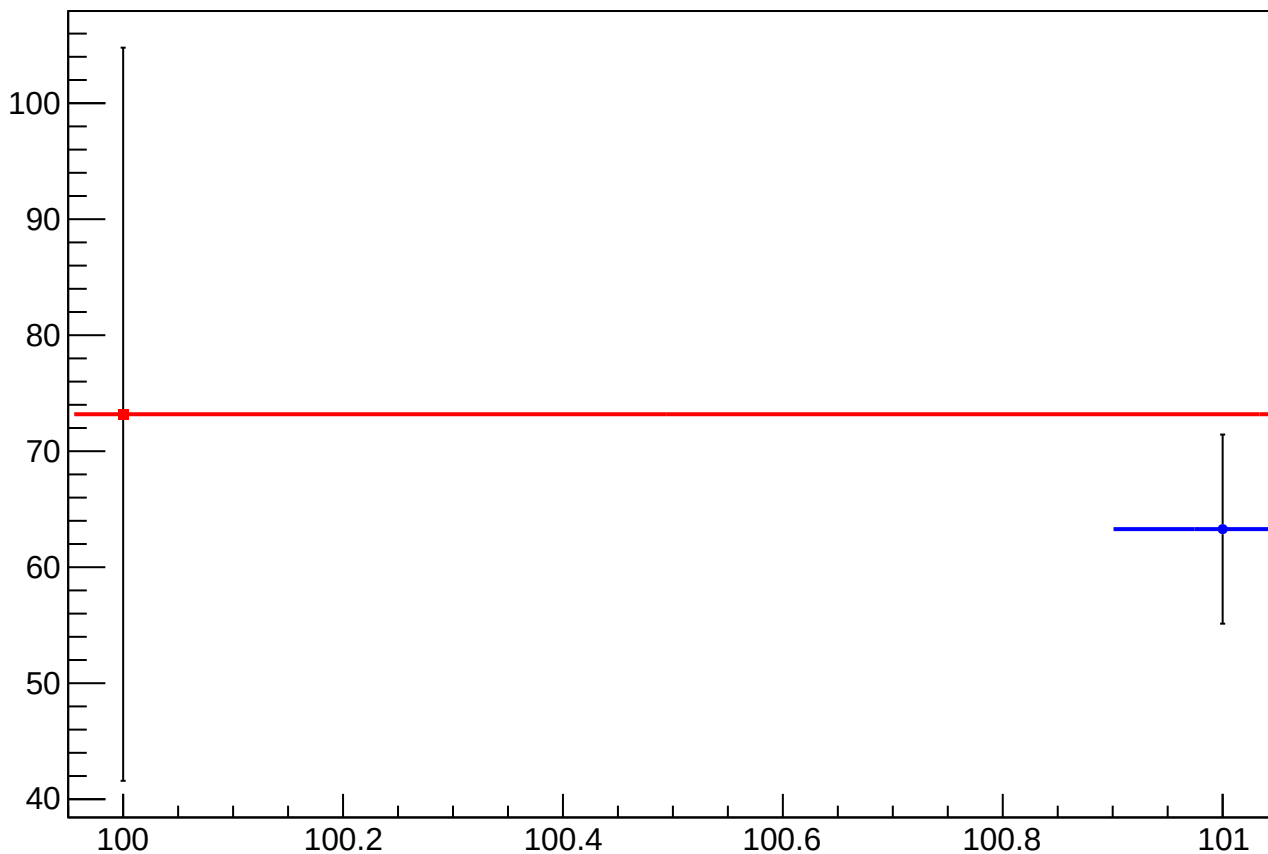
reg_asym_us_dd_at1lr_dd_avg_diff_bpm1X_slope vs Slug, Sign Corrected
