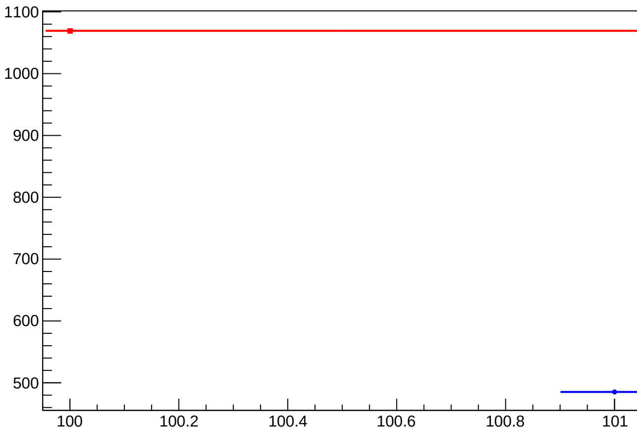
asym_atr2_dit_vs_cor_diff_rms vs Slug, Sign Corrected
