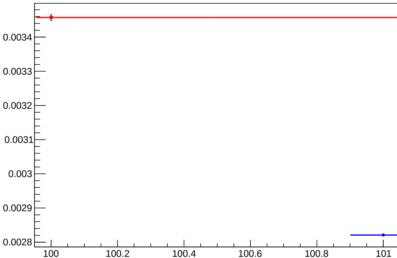
asym_sam_26_avg_eigen_dit_vs_dit_diff_rms vs Slug, Sign Corrected
