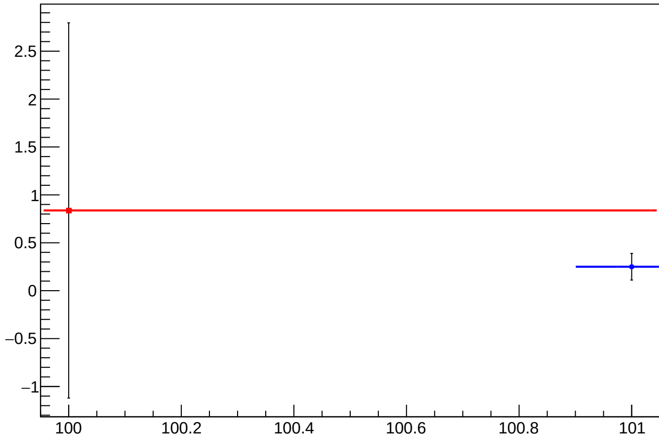
asym_us_avg_at1lr_avg_dd_eigen_dit_vs_eigen_cor_diff_mean vs Slug, Sign Corrected
