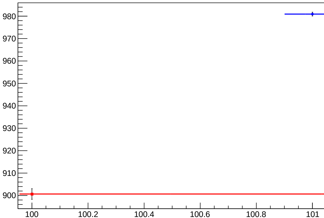
asym_usl_atl1_dd_cor_correction_rms vs Slug, Sign Corrected
