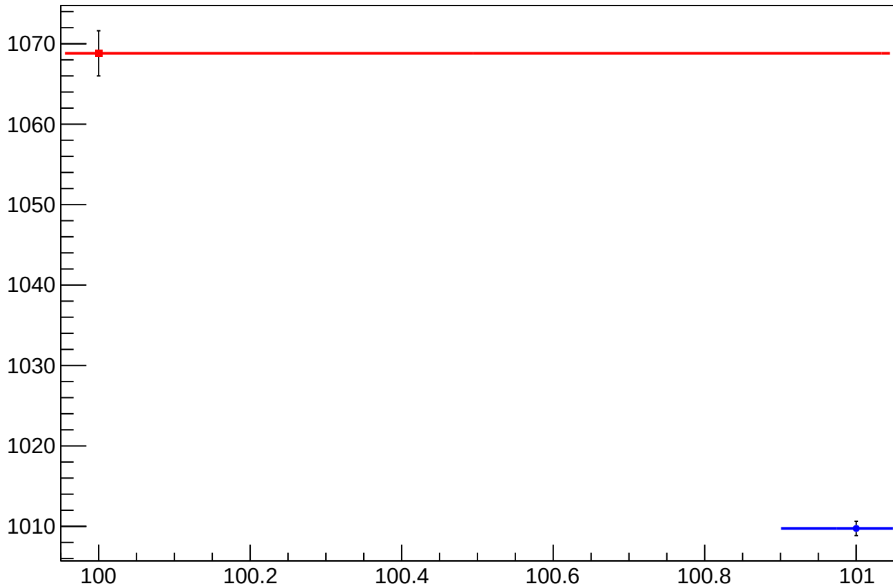
diff_bpm_4eY_4ecY_dd_rms vs Slug, Sign Corrected
