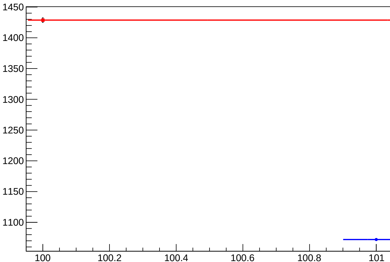
asym_at1_dd_at2_dd_avg_reg_correction_rms vs Slug, Sign Corrected
