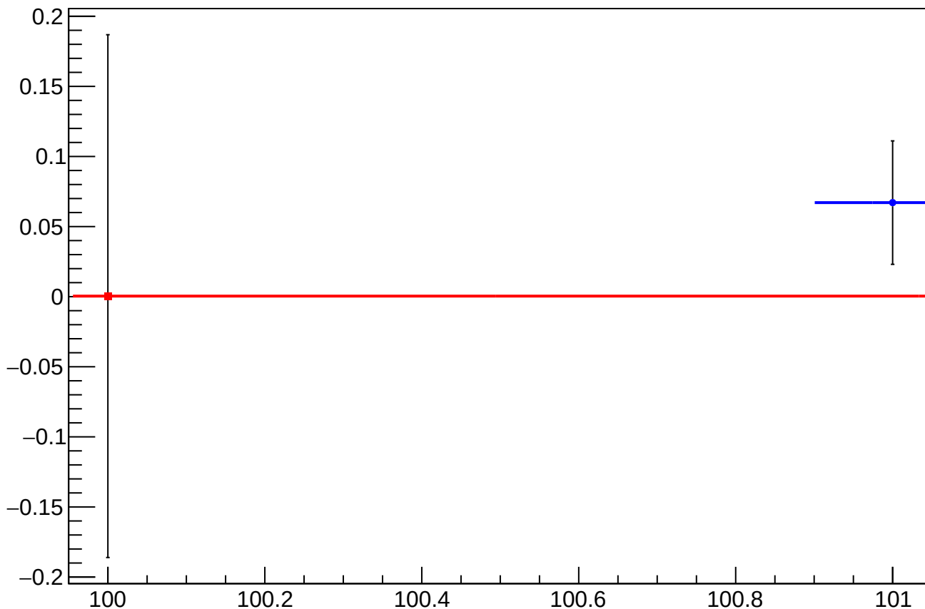
asym_sam_37_dd_dit_vs_cor_diff_mean vs Slug, Sign Corrected
