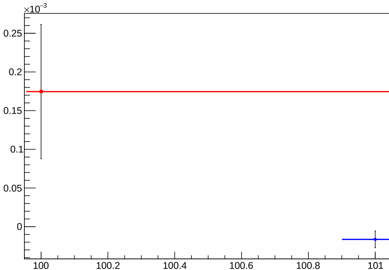
asym_at2_dd_eigen_dit_vs_dit_diff_mean vs Slug, Sign Corrected
