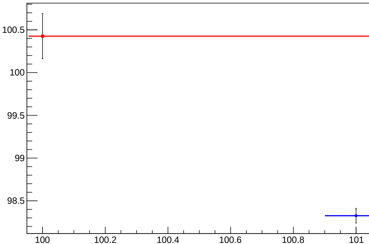
eigen_cor_asym_sam_15_dd_rms vs Slug, Sign Corrected
