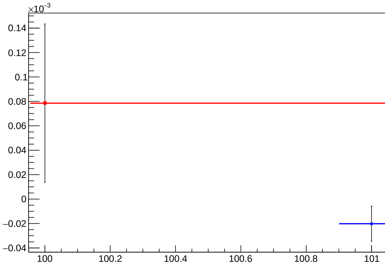
asym_us_avg_atlr_avg_avg_eigen_dit_vs_dit_diff_mean vs Slug, Sign Corrected
