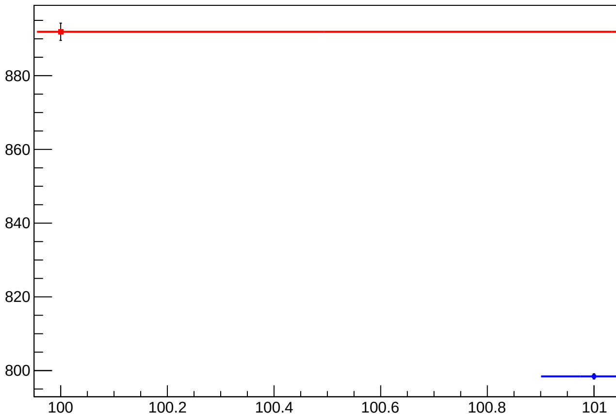
asym_us_avg_reg_correction_rms vs Slug, Sign Corrected
