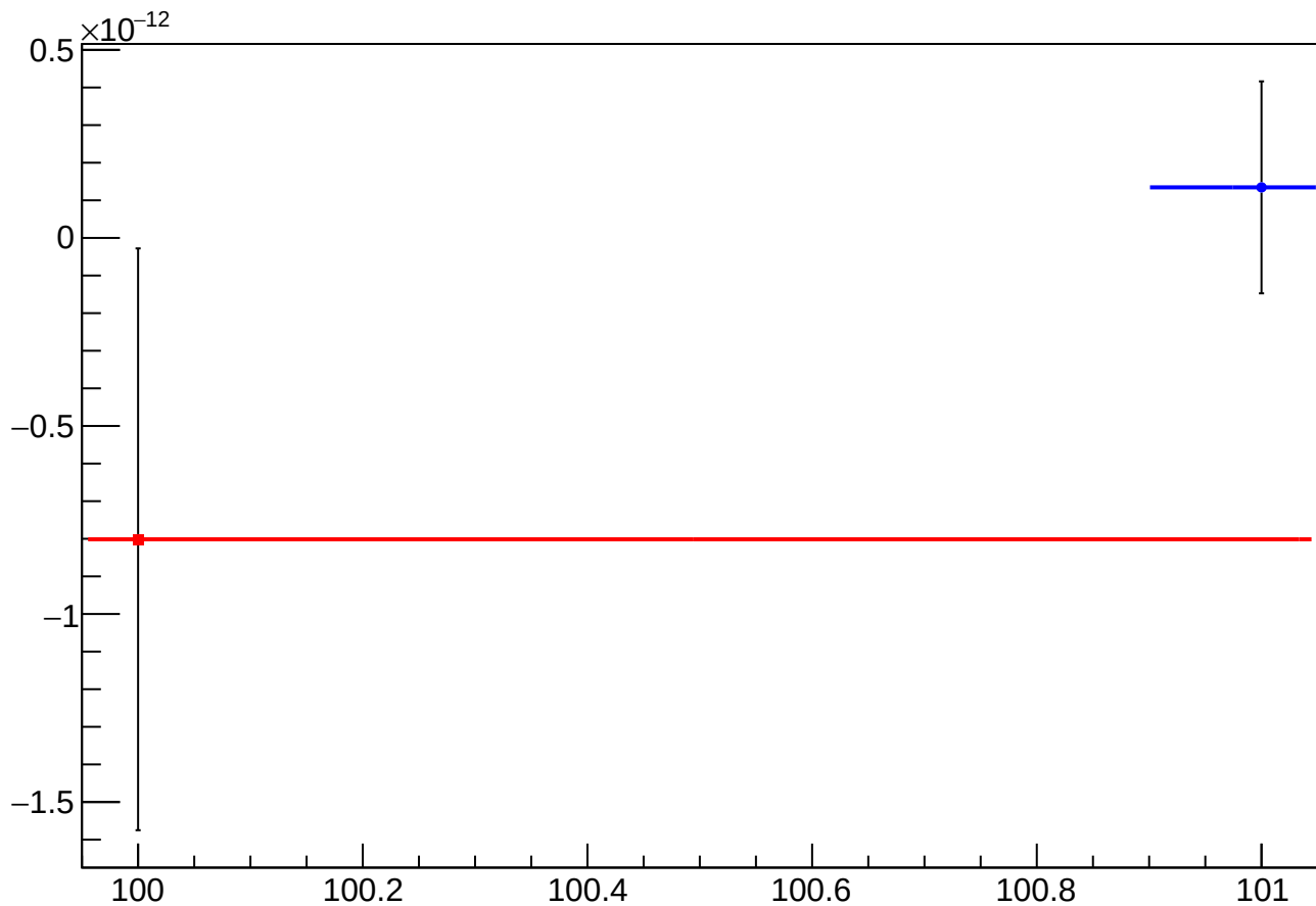
asym_at2_avg_eigen_cor_vs_cor_diff_mean vs Slug, Sign Corrected
