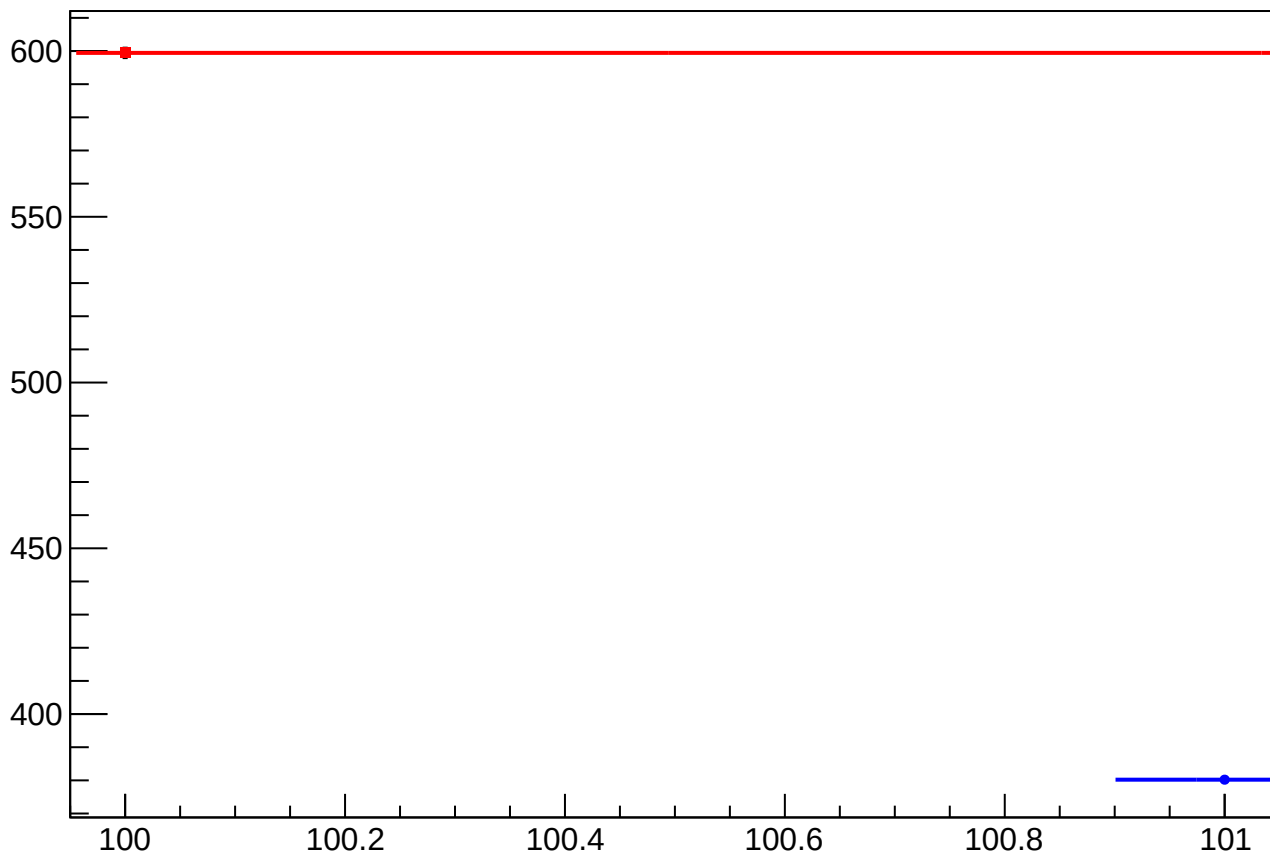
asym_usl_atl1_avg_dit_correction_rms vs Slug, Sign Corrected
