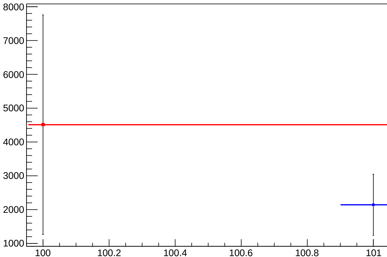
overload_cor_asym_us_avg_mean vs Slug, Sign Corrected
