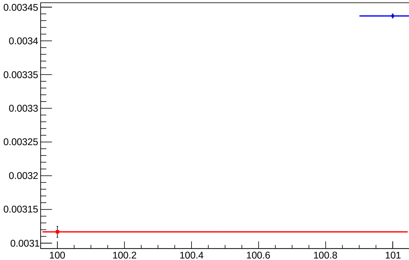
asym_atr1_eigen_dit_vs_dit_diff_rms vs Slug, Sign Corrected
