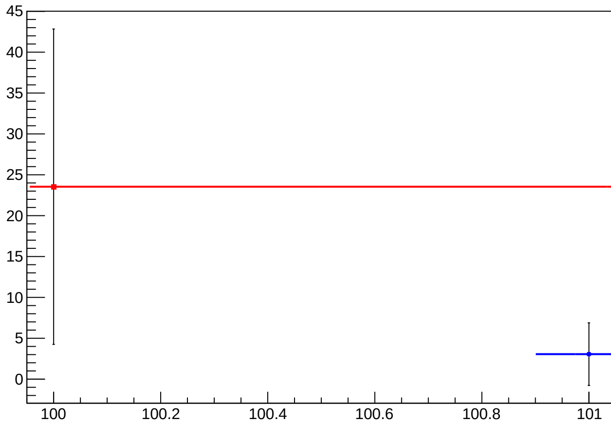
reg_asym_atl_avg_atr_avg_dd_diff_bpm4aY_slope vs Slug, Sign Corrected
