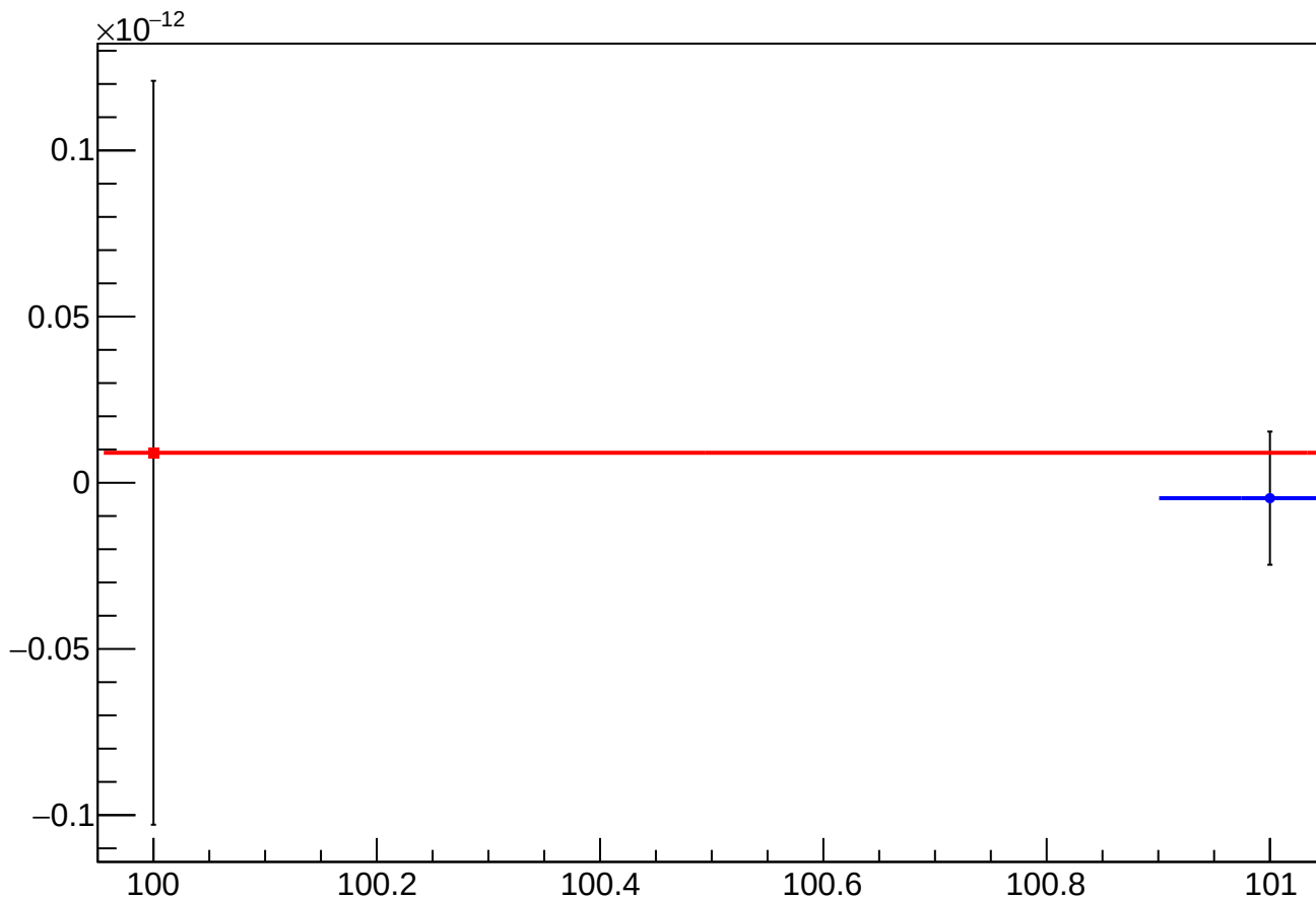
asym_usl_atl1_avg_eigen_cor_vs_cor_diff_mean vs Slug, Sign Corrected
