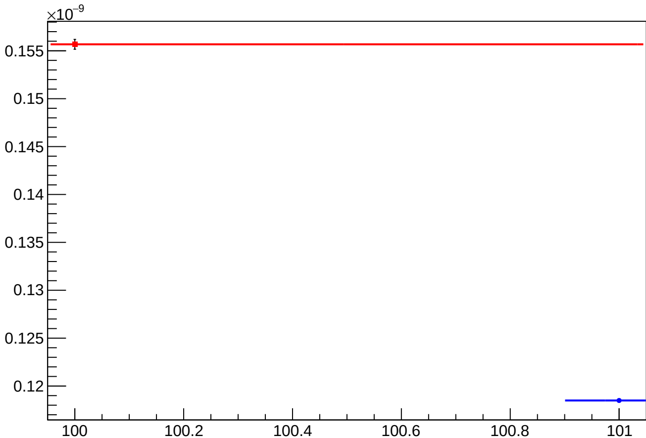
asym_usl_atl2_avg_reg_vs_cor_diff_rms vs Slug, Sign Corrected
