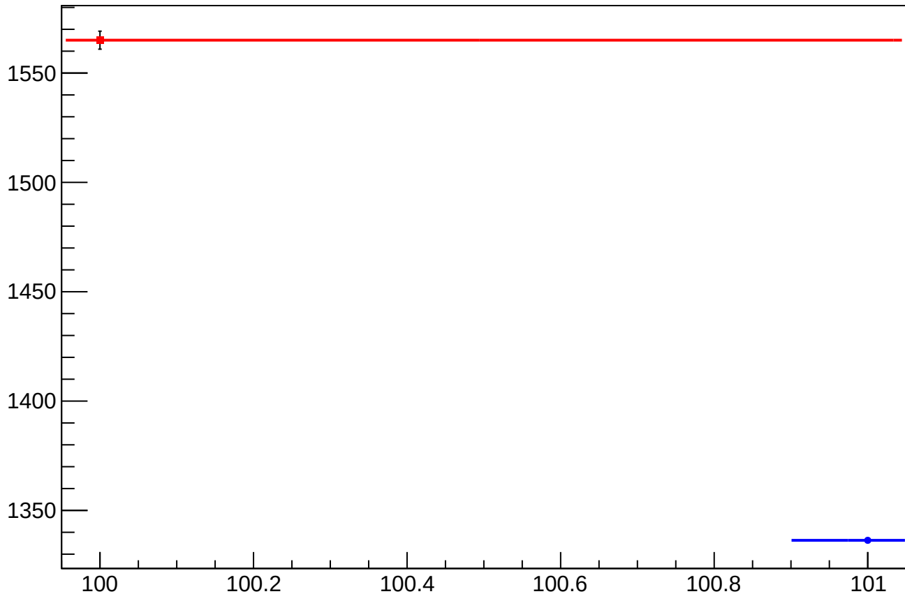
dit_asym_usl_atl2_dd_rms vs Slug, Sign Corrected
