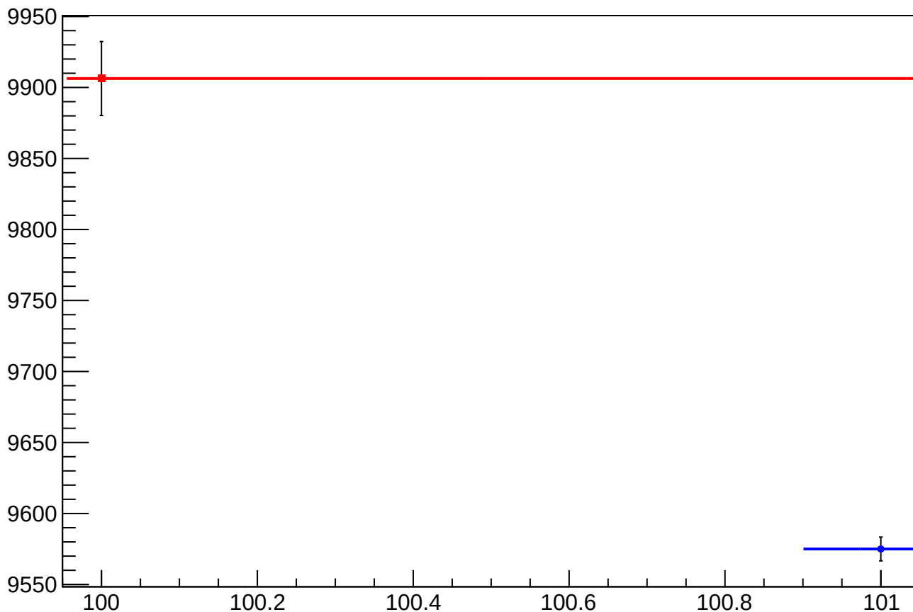
asym_atr2_reg_correction_rms vs Slug, Sign Corrected
