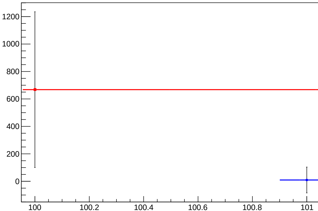
eigen_dit_asym_sam_1548_avg_mean vs Slug, Sign Corrected
