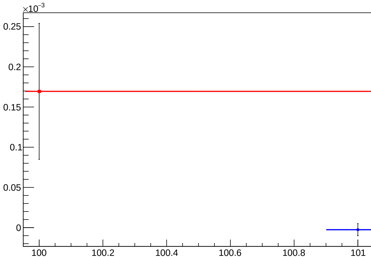
asym_us_dd_at2lr_dd_dd_eigen_dit_vs_dit_diff_mean vs Slug, Sign Corrected
