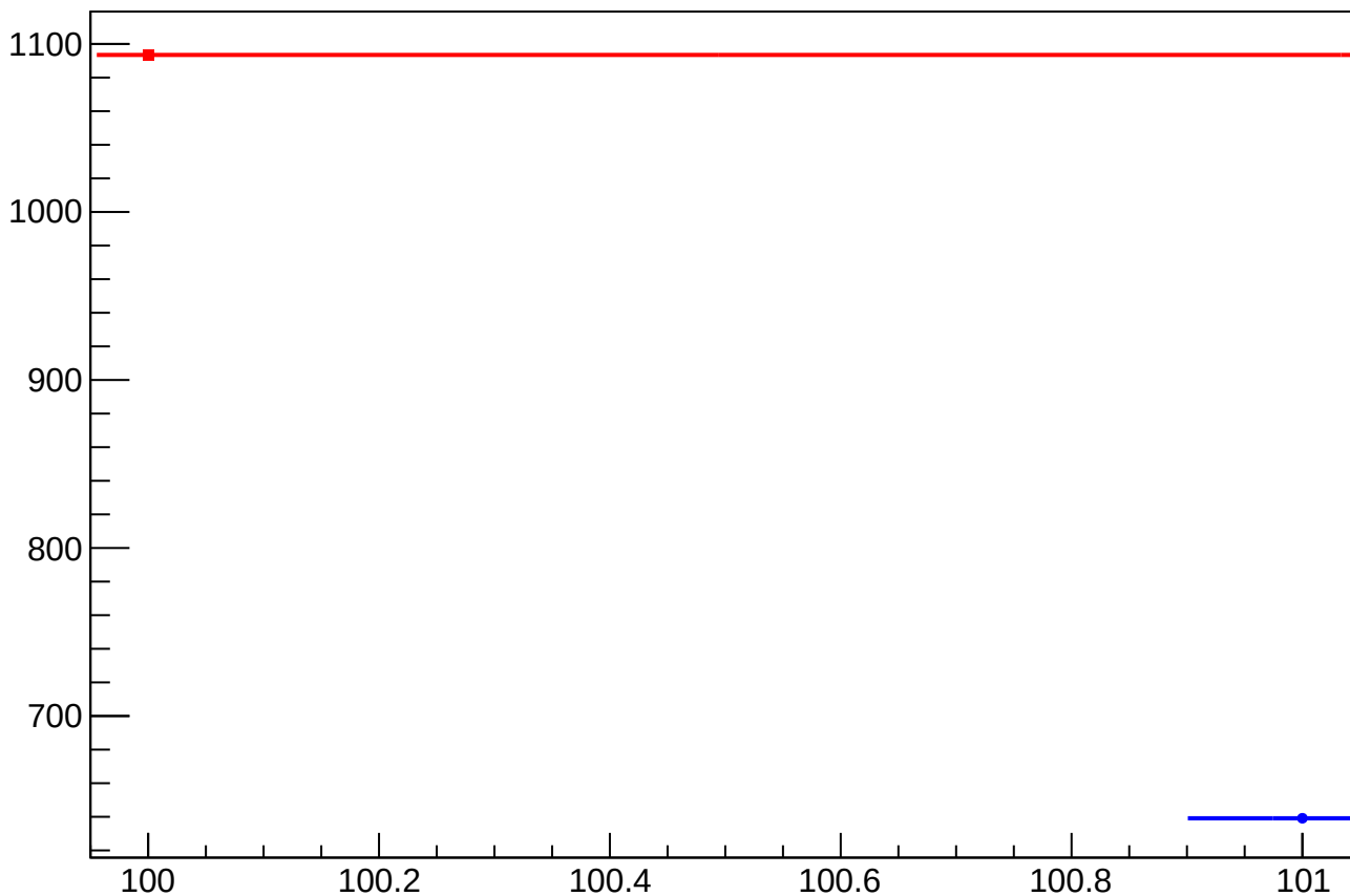
asym_at1_avg_reg_correction_rms vs Slug, Sign Corrected
