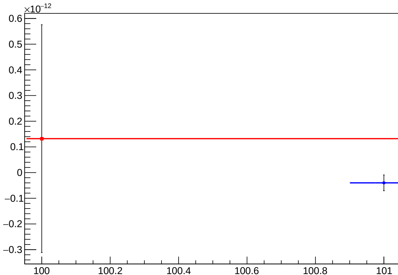
asym_sam_48_avg_eigen_cor_vs_cor_diff_mean vs Slug, Sign Corrected
