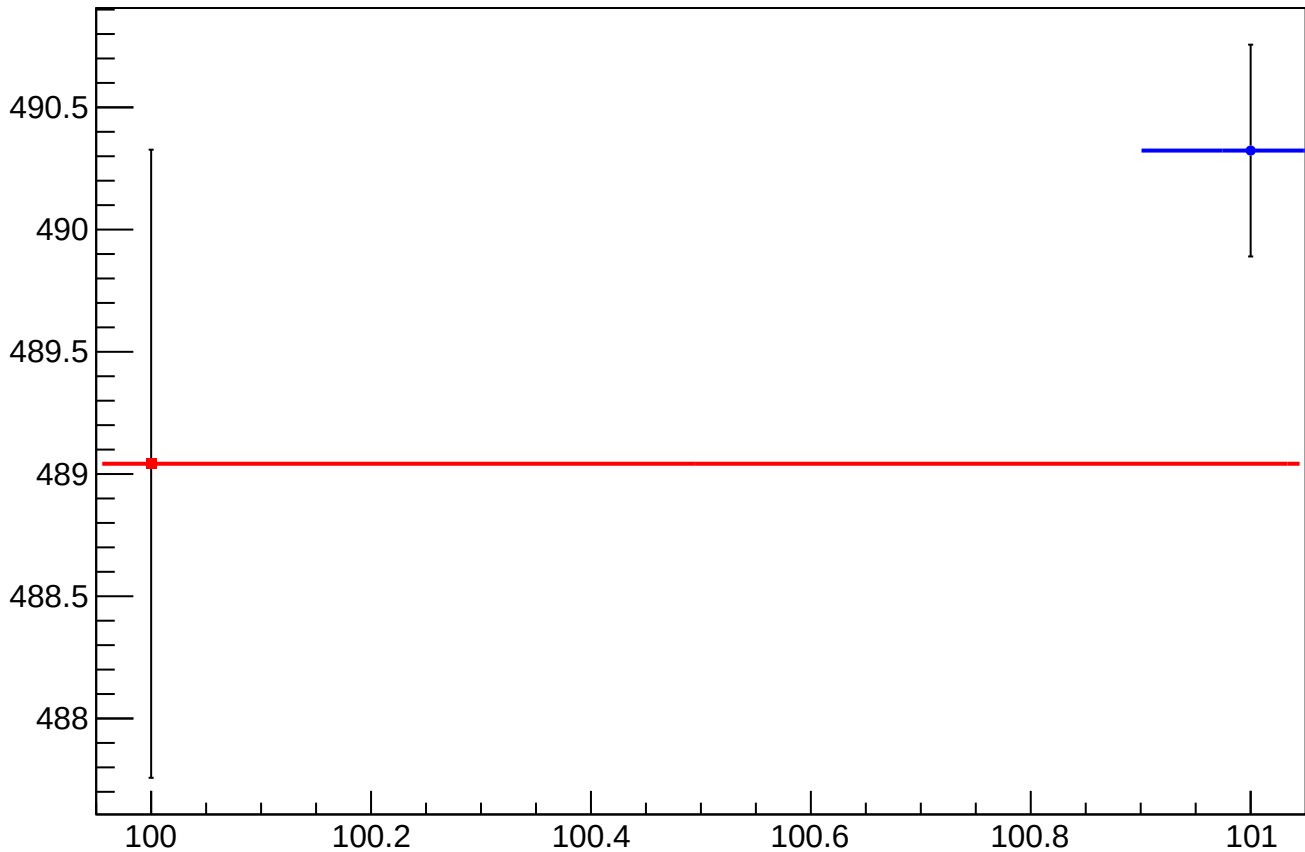
diff_bpm_4aX_4ecX_dd_rms vs Slug, Sign Corrected
