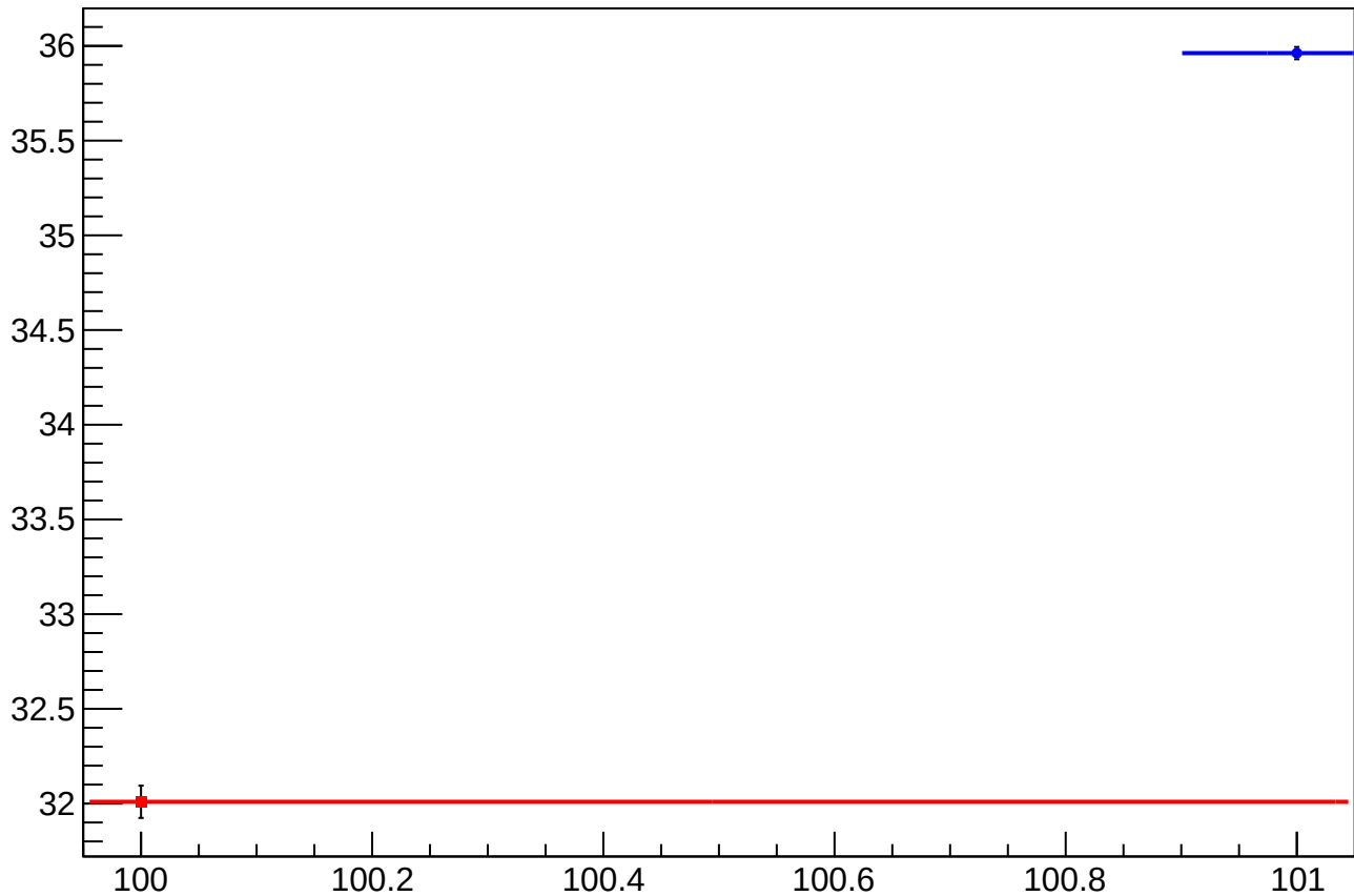
asym_sam_13_57_dd_dit_vs_eigen_cor_diff_rms vs Slug, Sign Corrected
