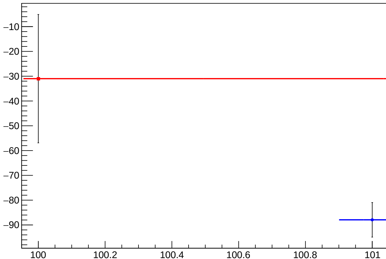
reg_asym_usr_atr2_dd_diff_bpm4eY_slope vs Slug, Sign Corrected
