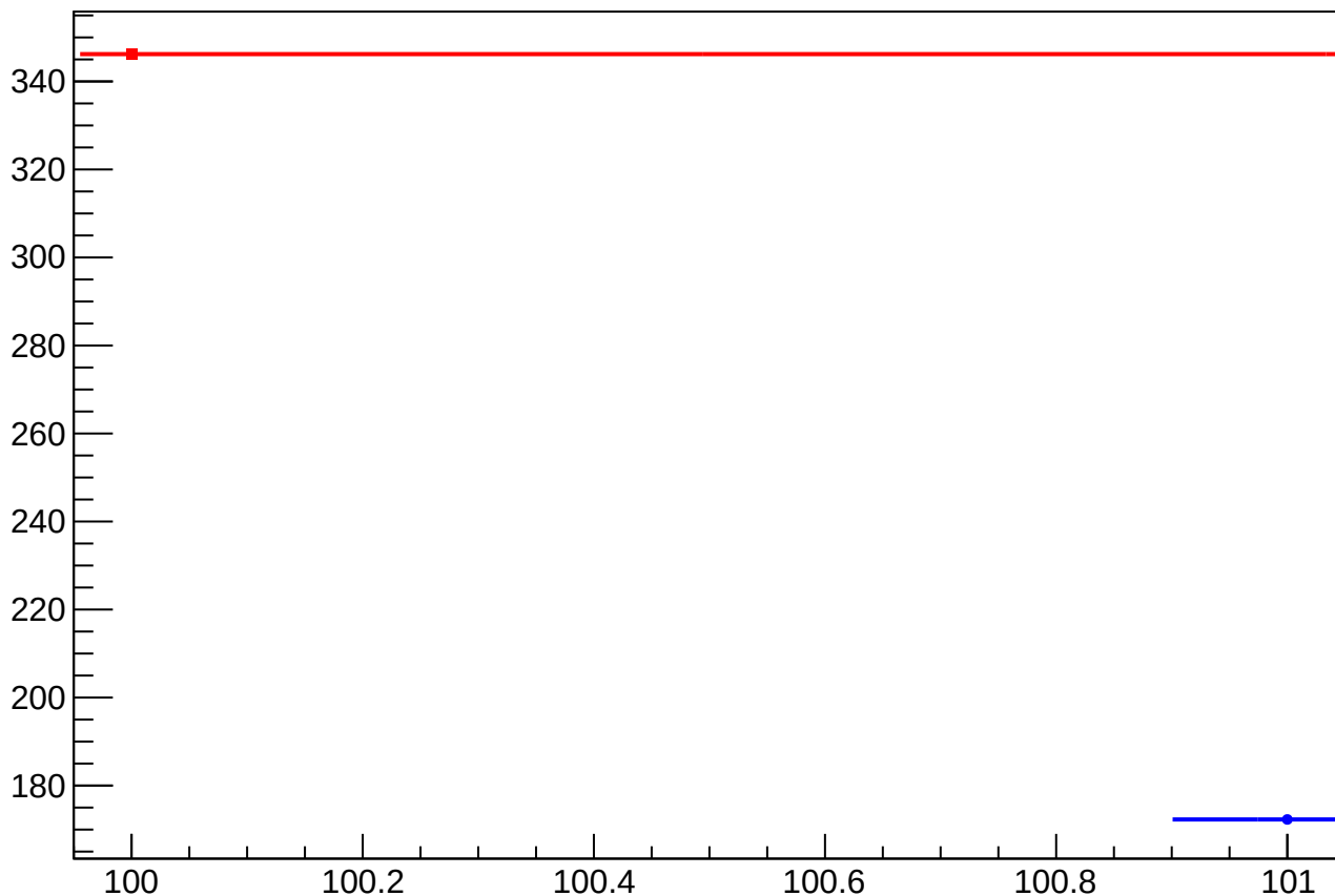
asym_us_avg_atlr_avg_dd_eigen_dit_vs_cor_diff_rms vs Slug, Sign Corrected
