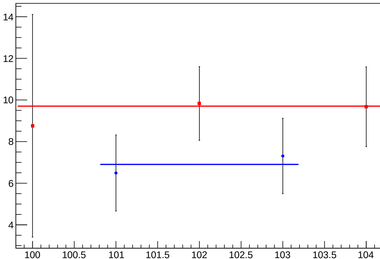
diff_bpm0l04Y_mean vs Slug, Sign Corrected
