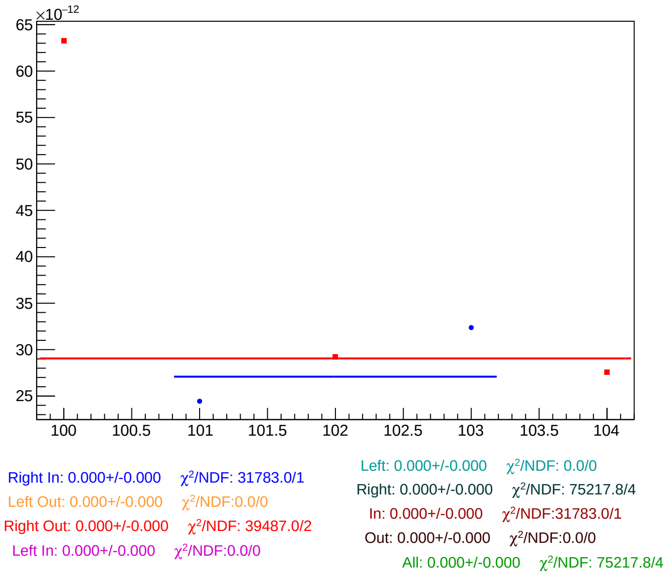
asym_sam_15_26_dd_eigen_cor_vs_cor_diff_rms vs Slug, Sign Corrected
