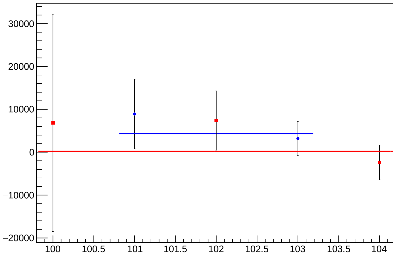
asym_us_atlr_avg_avg_mean vs Slug, Sign Corrected
