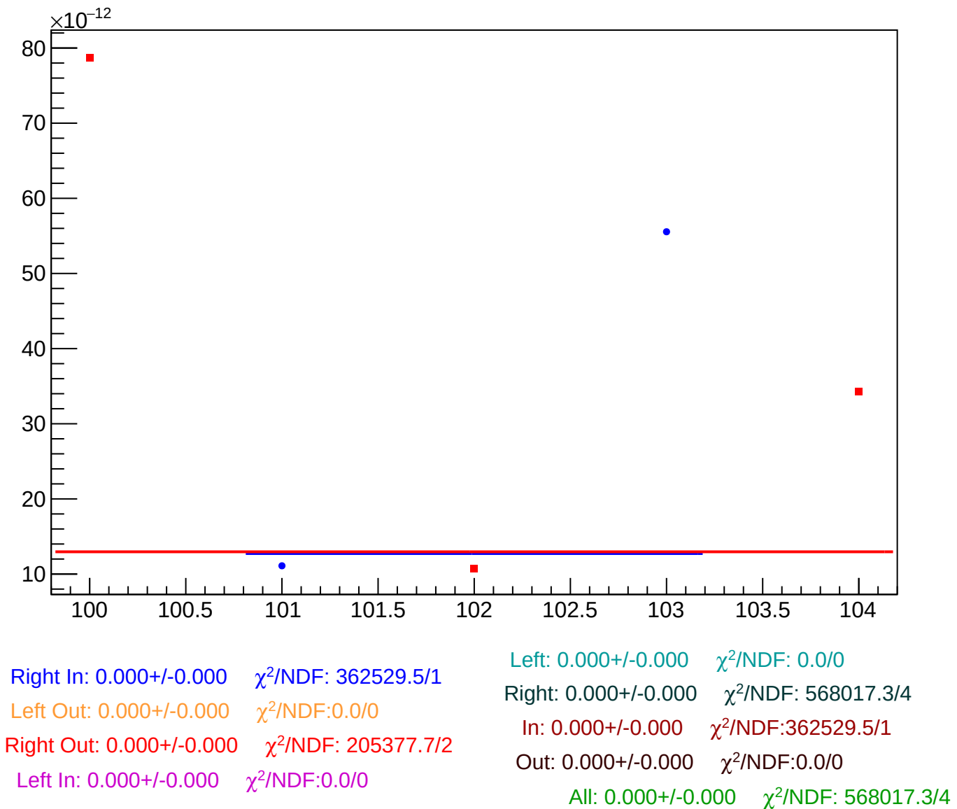
asym_usl_atl1_avg_reg_vs_cor_diff_rms vs Slug, Sign Corrected
