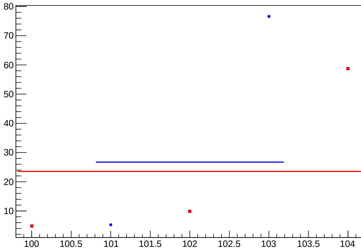
reg_asym_usl_atl1_avg_diff_bpm12X_slope vs Slug, Sign Corrected
