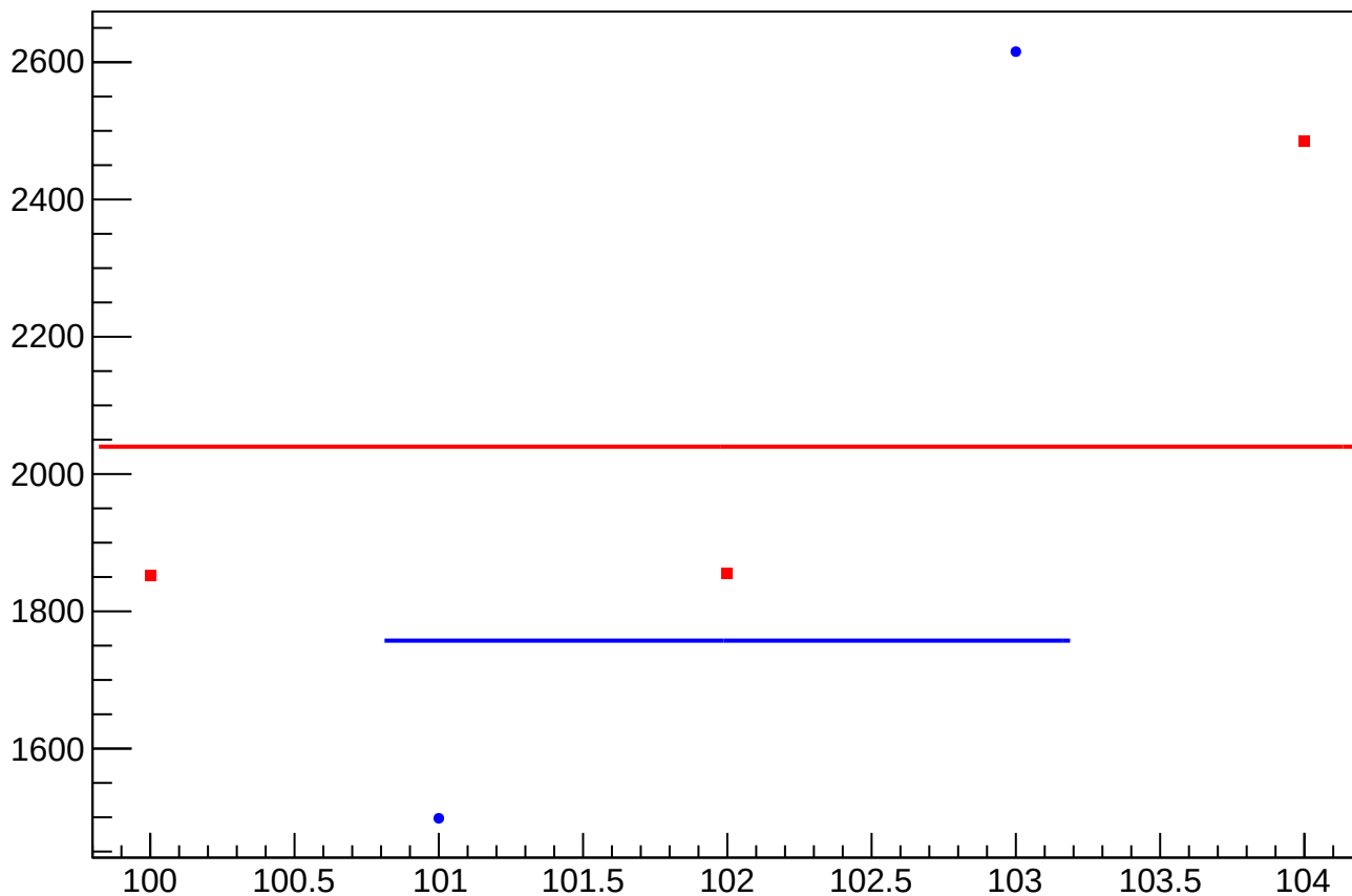
asym_usl_atl1_avg_rms vs Slug, Sign Corrected
