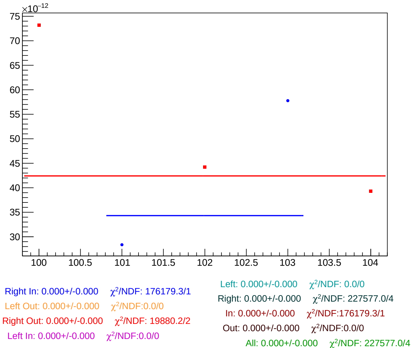
asym_sam_26_48_dd_reg_vs_cor_diff_rms vs Slug, Sign Corrected
