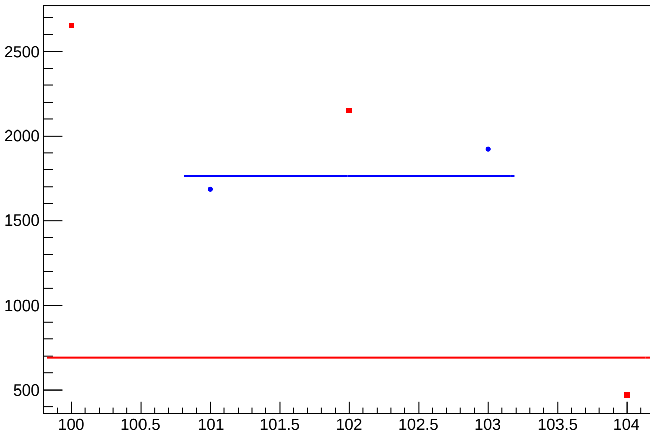
asym_us_dd_at1lr_dd_avg_cor_correction_rms vs Slug, Sign Corrected
