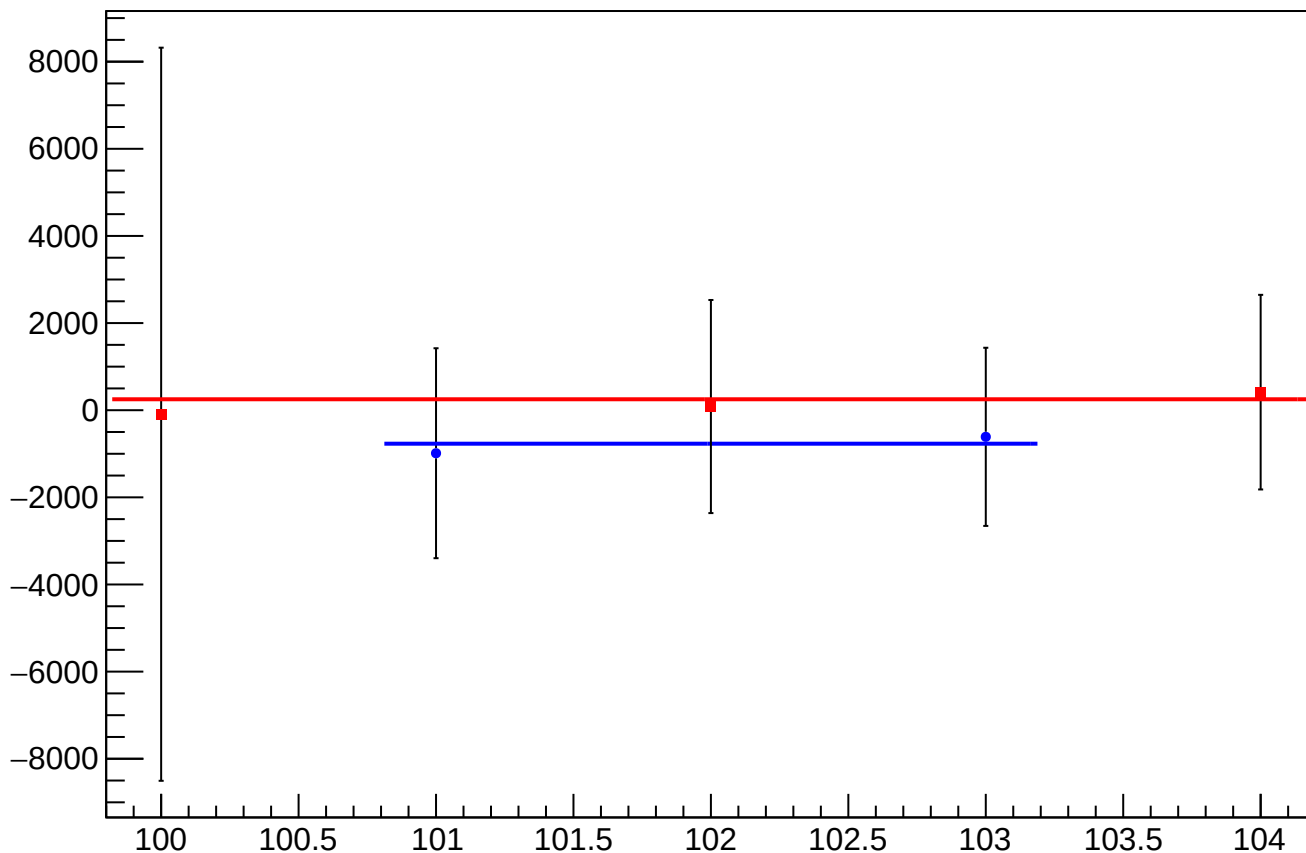
cor_asym_atl_dd_mean vs Slug, Sign Corrected
