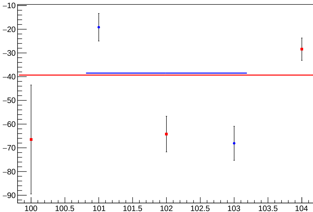
reg_asym_atl1r2_dd_atl2r1_dd_diff_bpm4aY_slope vs Slug, Sign Corrected
