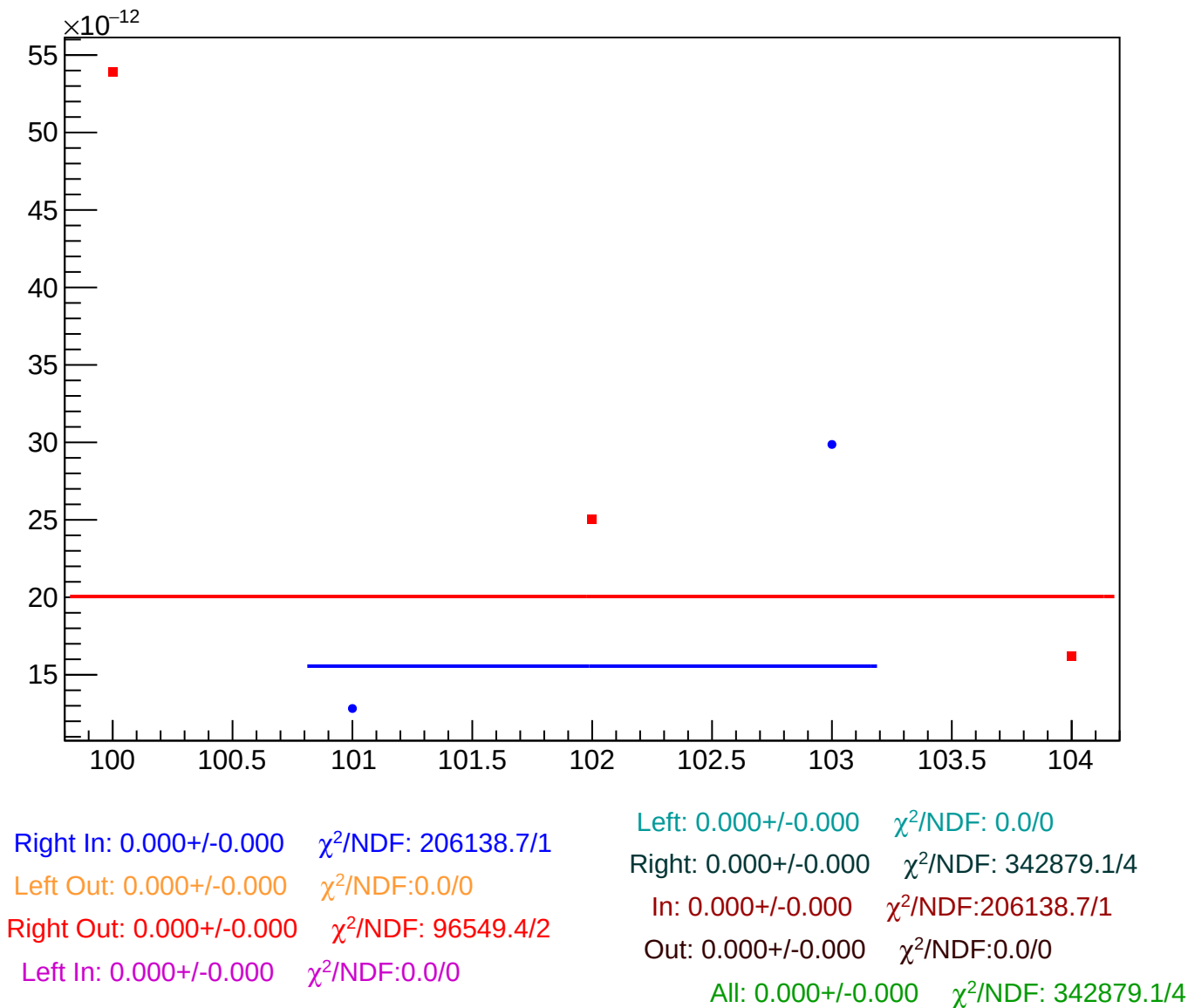
asym_us_dd_eigen_cor_vs_cor_diff_rms vs Slug, Sign Corrected
