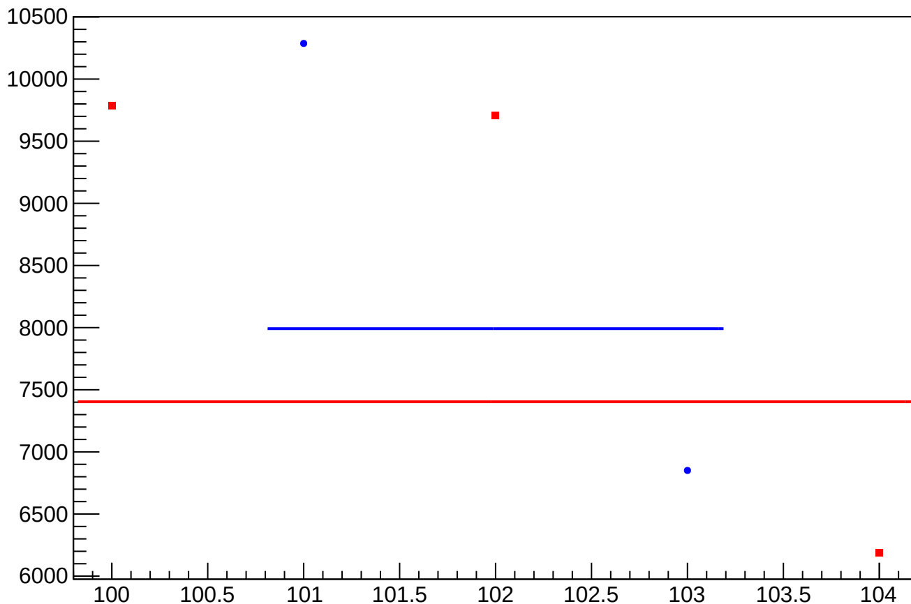
asym_us_avg_at2lr_avg_avg_rms vs Slug, Sign Corrected
