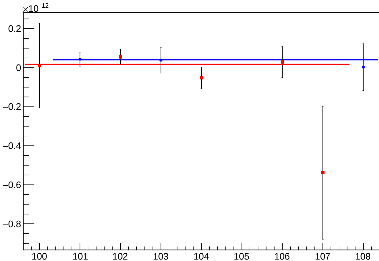
asym_us_avg_at1lr_avg_avg_eigen_cor_vs_cor_diff_mean vs Slug, Sign Corrected
