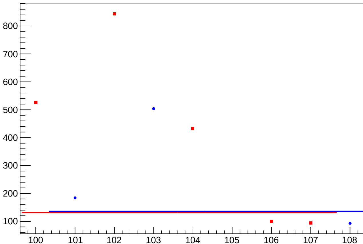
asym_atl_dd_eigen_dit_vs_cor_diff_rms vs Slug, Sign Corrected
