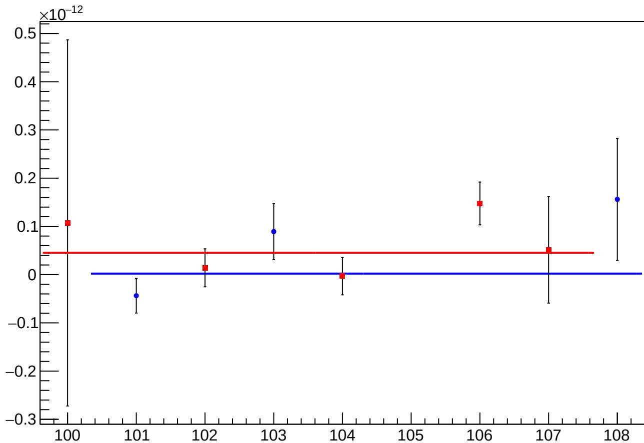
asym_sam_3748_avg_eigen_cor_vs_cor_diff_mean vs Slug, Sign Corrected
