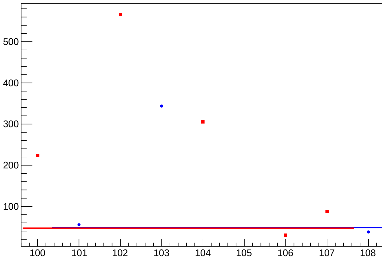
asym_at1_dd_at2_dd_avg_dit_vs_eigen_cor_diff_rms vs Slug, Sign Corrected
