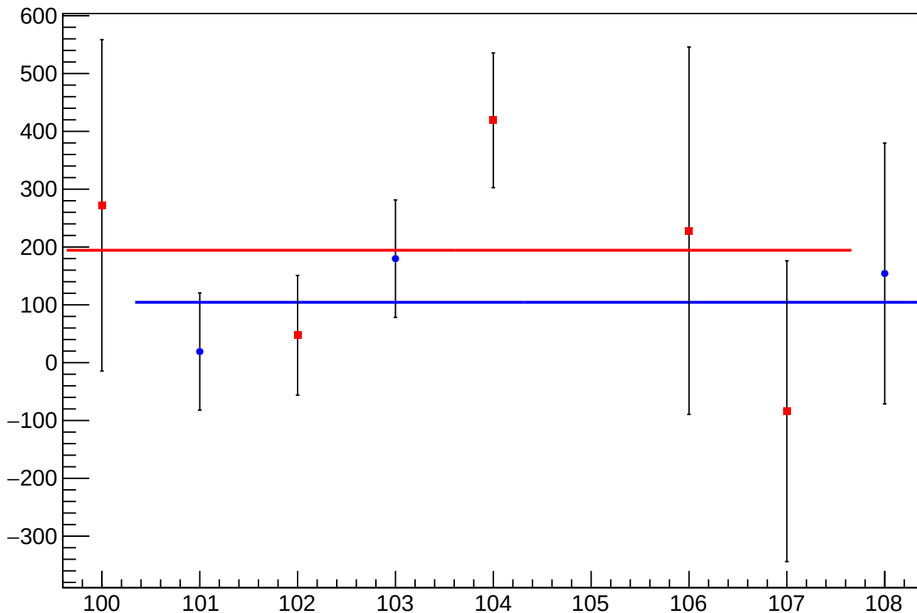
asym_sam_15_avg_mean vs Slug, Sign Corrected
