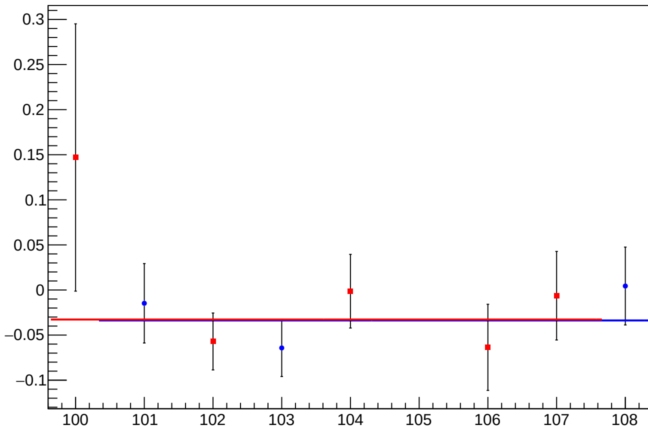
asym_us_dd_overload_cor_vs_eigen_cor_diff_mean vs Slug, Sign Corrected
