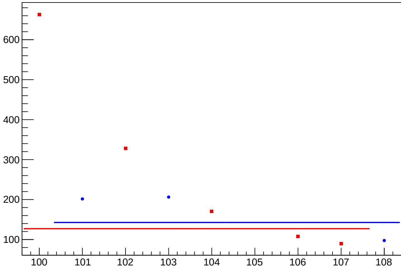
asym_atl_dd_atr_dd_avg_dit_vs_cor_diff_rms vs Slug, Sign Corrected
