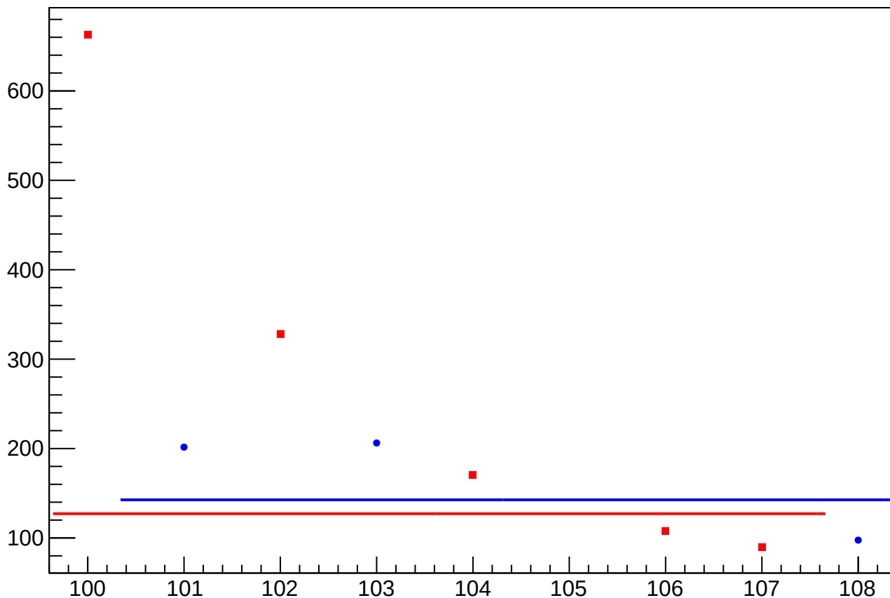
asym_at1_avg_at2_avg_dd_eigen_dit_vs_cor_diff_rms vs Slug, Sign Corrected
