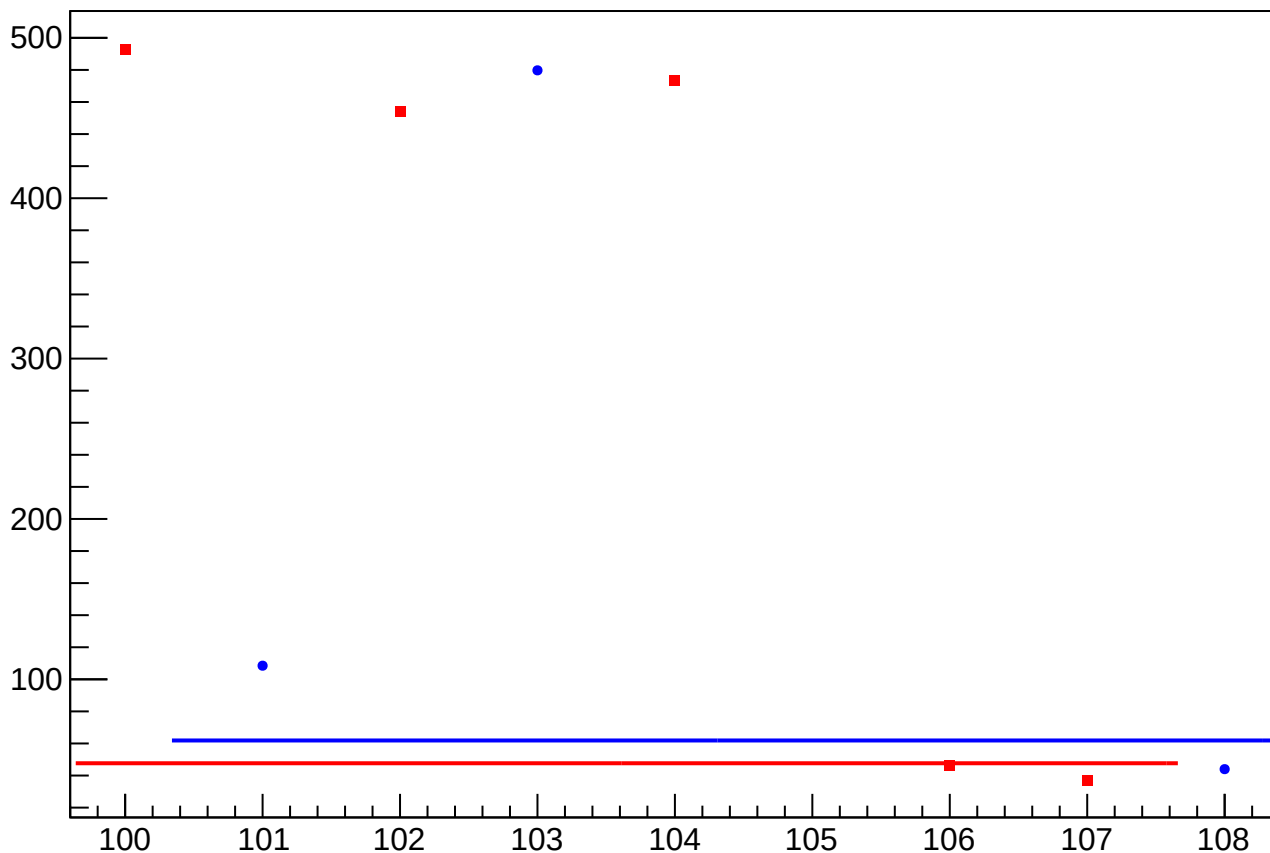
asym_usr_atr1_dd_dit_vs_cor_diff_rms vs Slug, Sign Corrected
