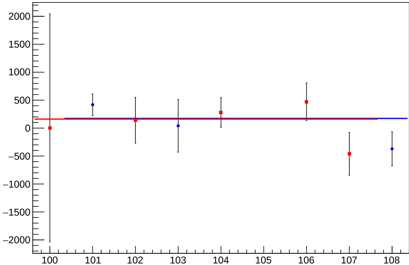
eigen_cor_asym_sam3_mean vs Slug, Sign Corrected
