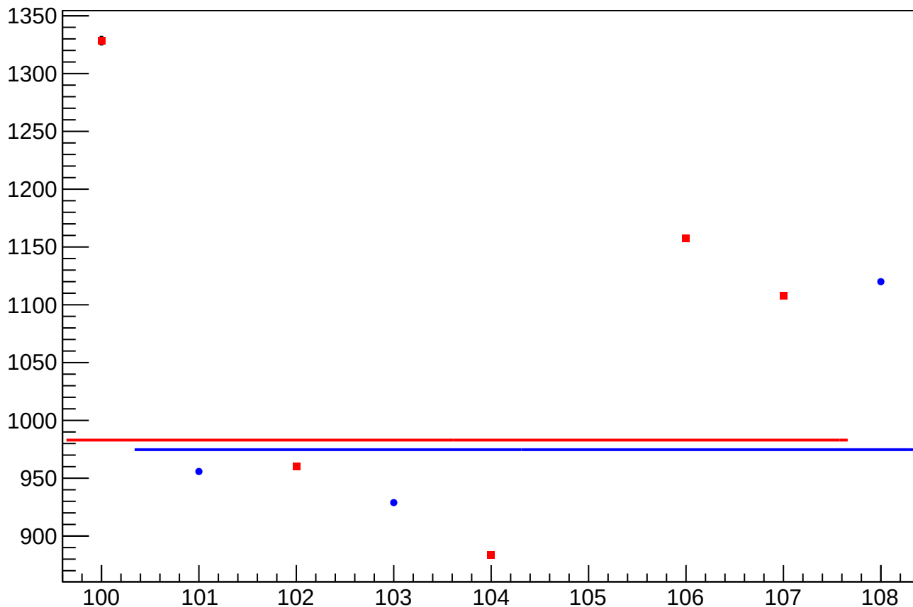
asym_usr_atr1_dd_reg_correction_rms vs Slug, Sign Corrected
