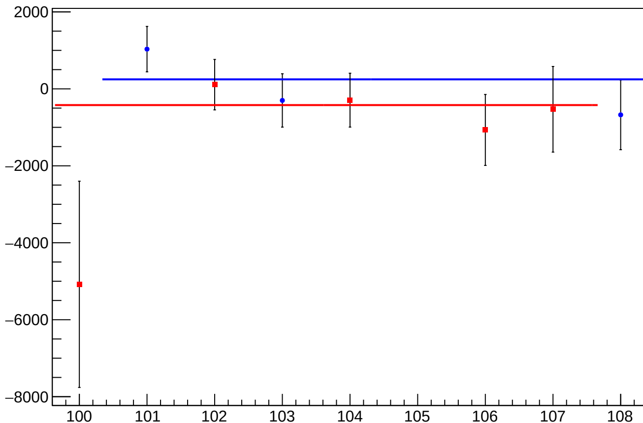
asym_sam_1357_2468_dd_dit_correction_mean vs Slug, Sign Corrected
