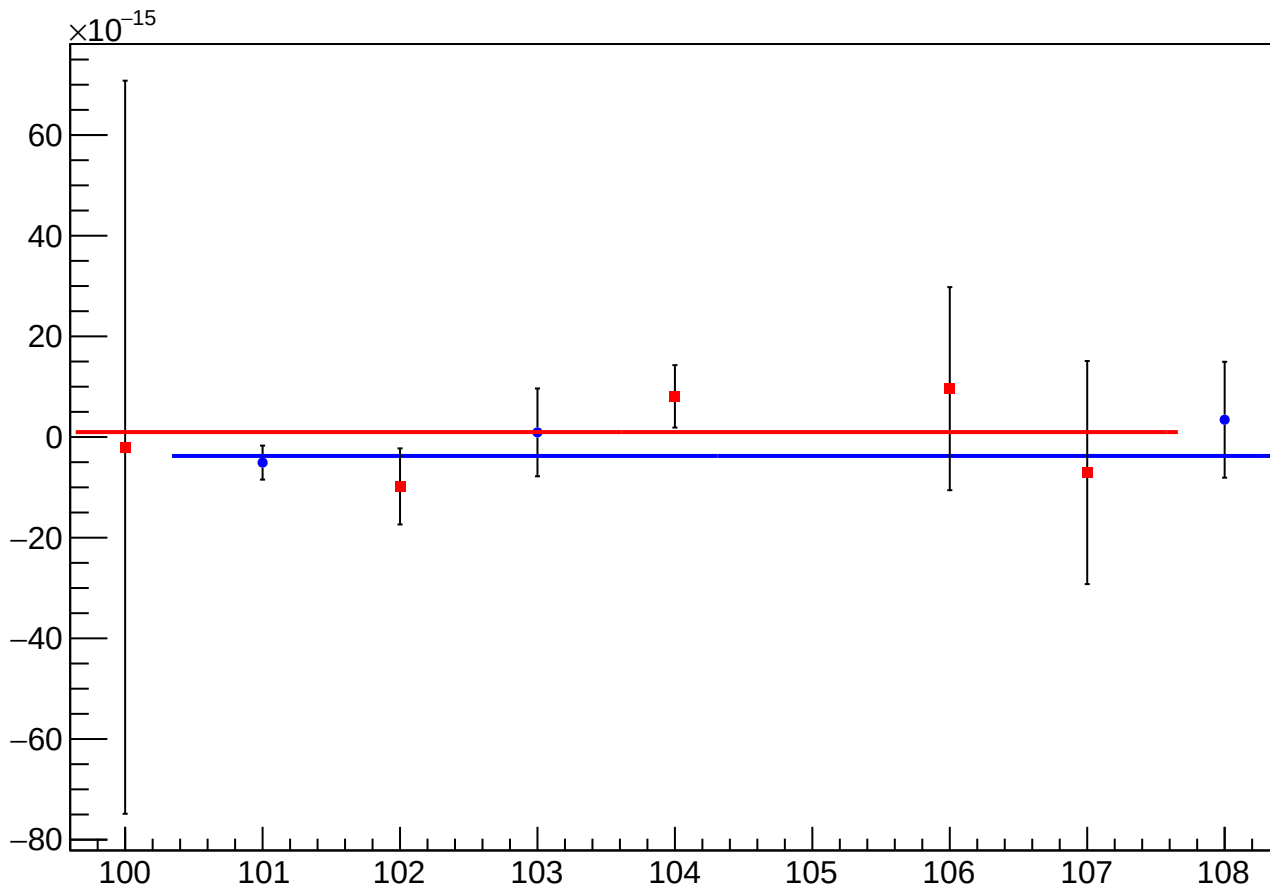
asym_sam_15_avg_reg_vs_cor_diff_mean vs Slug, Sign Corrected
