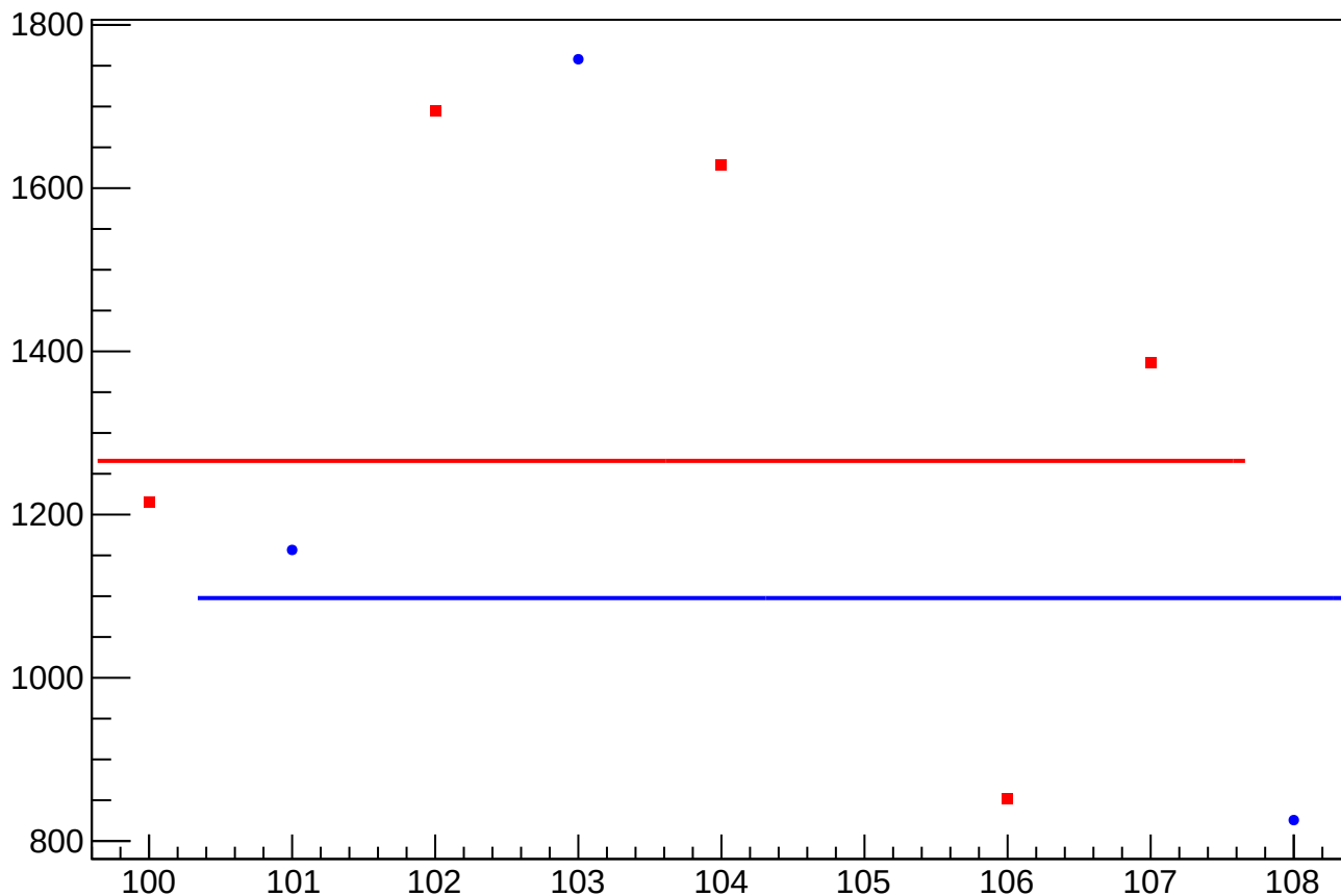
asym_us_dd_atlr_dd_dd_eigen_dit_correction_rms vs Slug, Sign Corrected
