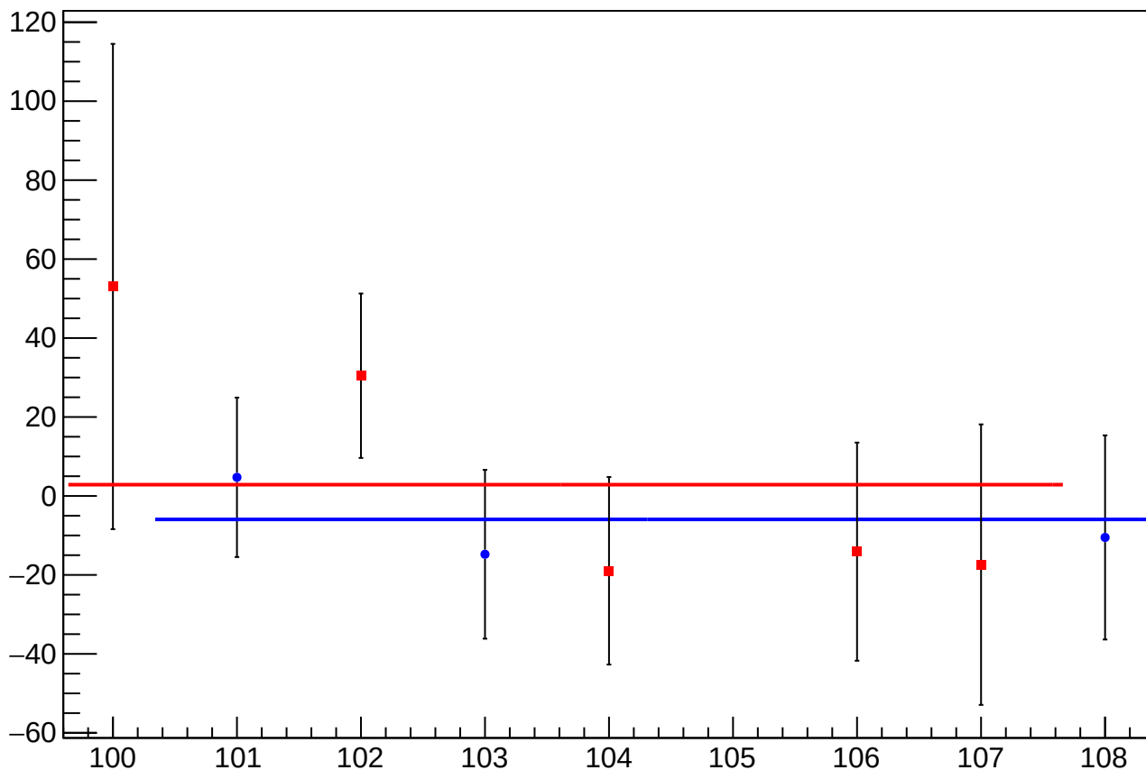
asym_bcm_an_avg_bcm_dg_ds_agg_dd_mean vs Slug, Sign Corrected
