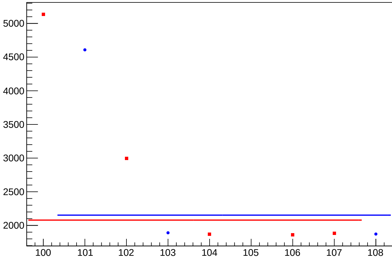
eigen_cor_asym_atr2_rms vs Slug, Sign Corrected
