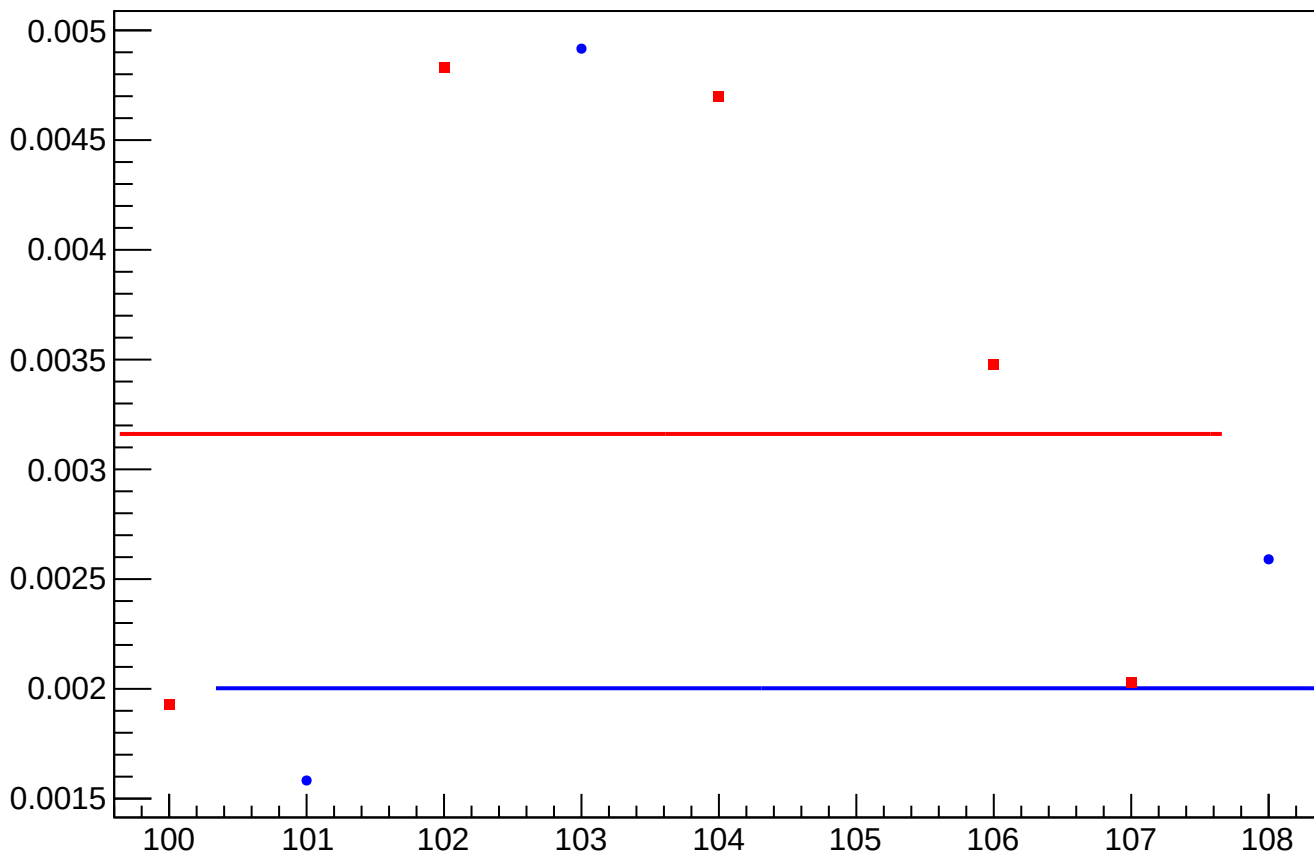
asym_sam_15_26_dd_eigen_dit_vs_dit_diff_rms vs Slug, Sign Corrected
