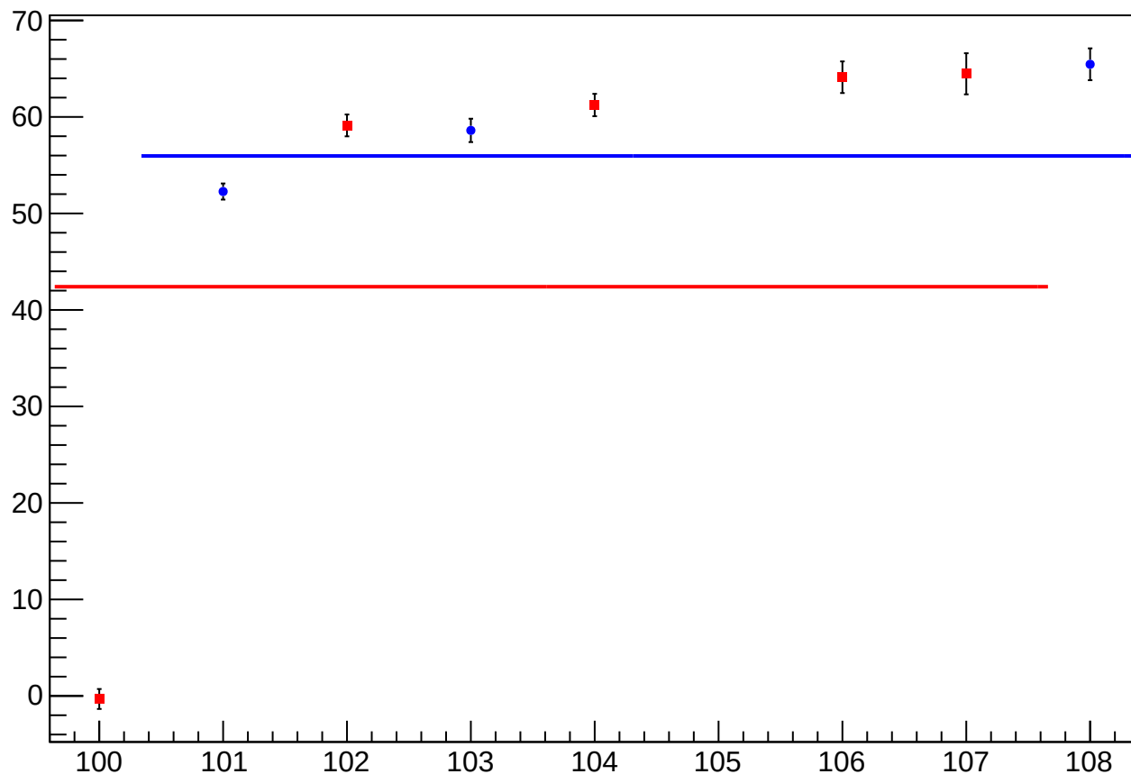
reg_asym_right_dd_diff_bpm4eX_slope vs Slug, Sign Corrected
