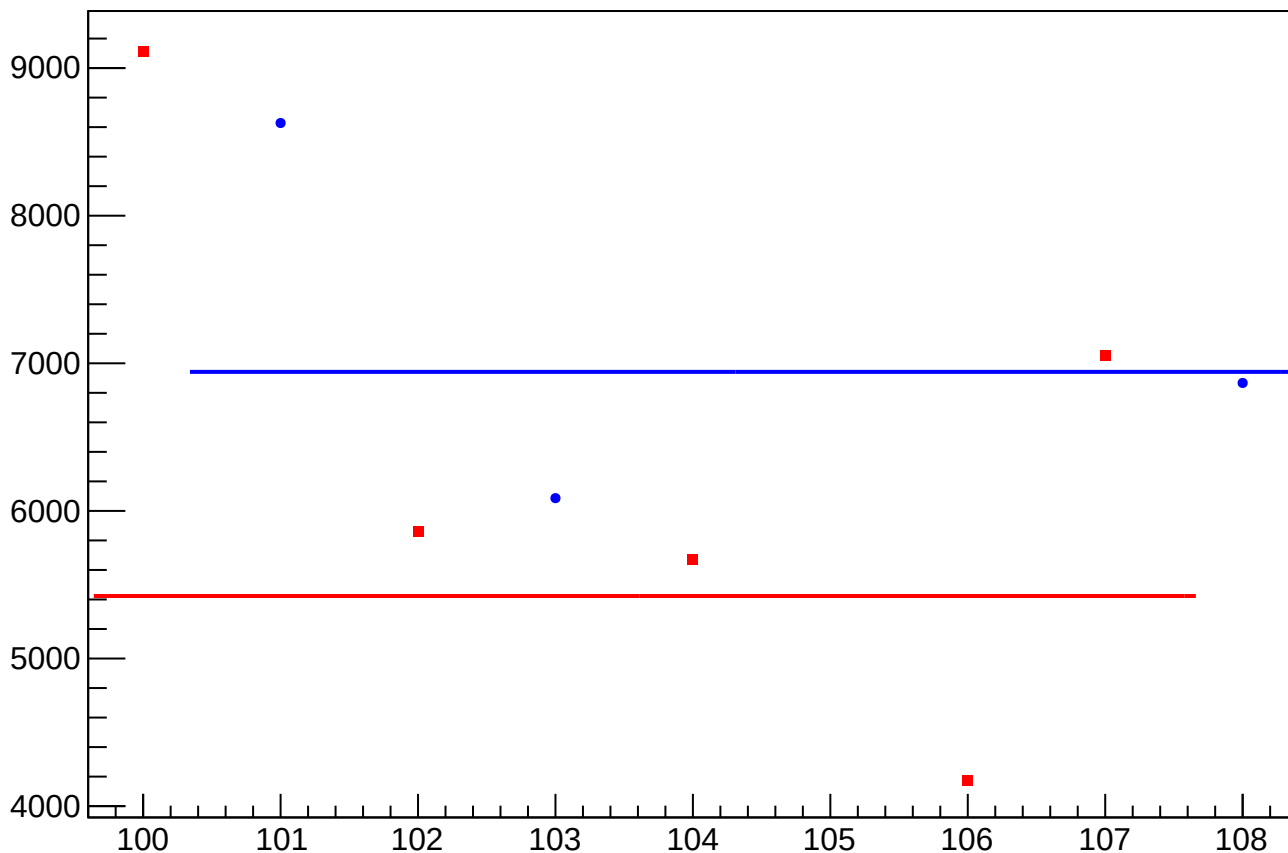
asym_at2_avg_dit_correction_rms vs Slug, Sign Corrected
