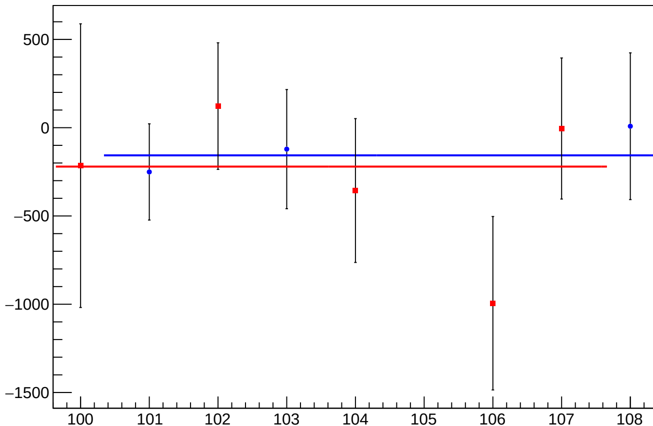
asym_bcm_dg_ds_an_us_avg_mean vs Slug, Sign Corrected
