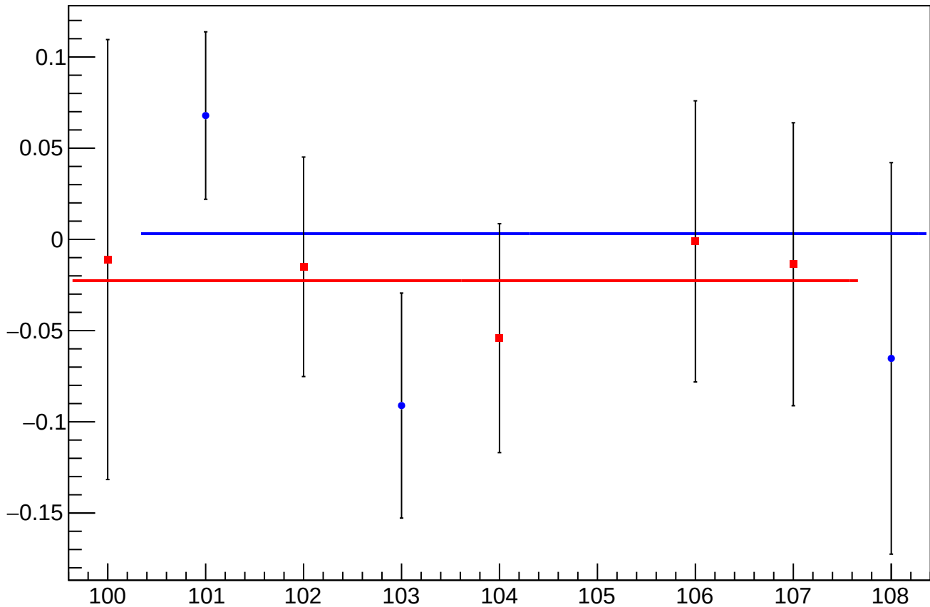
asym_sam_13_57_dd_dit_vs_eigen_cor_diff_mean vs Slug, Sign Corrected
