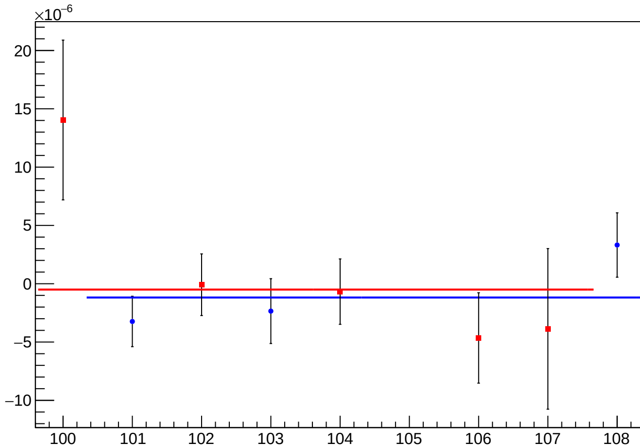
asym_usr_atr1_dd_eigen_dit_vs_dit_diff_mean vs Slug, Sign Corrected
