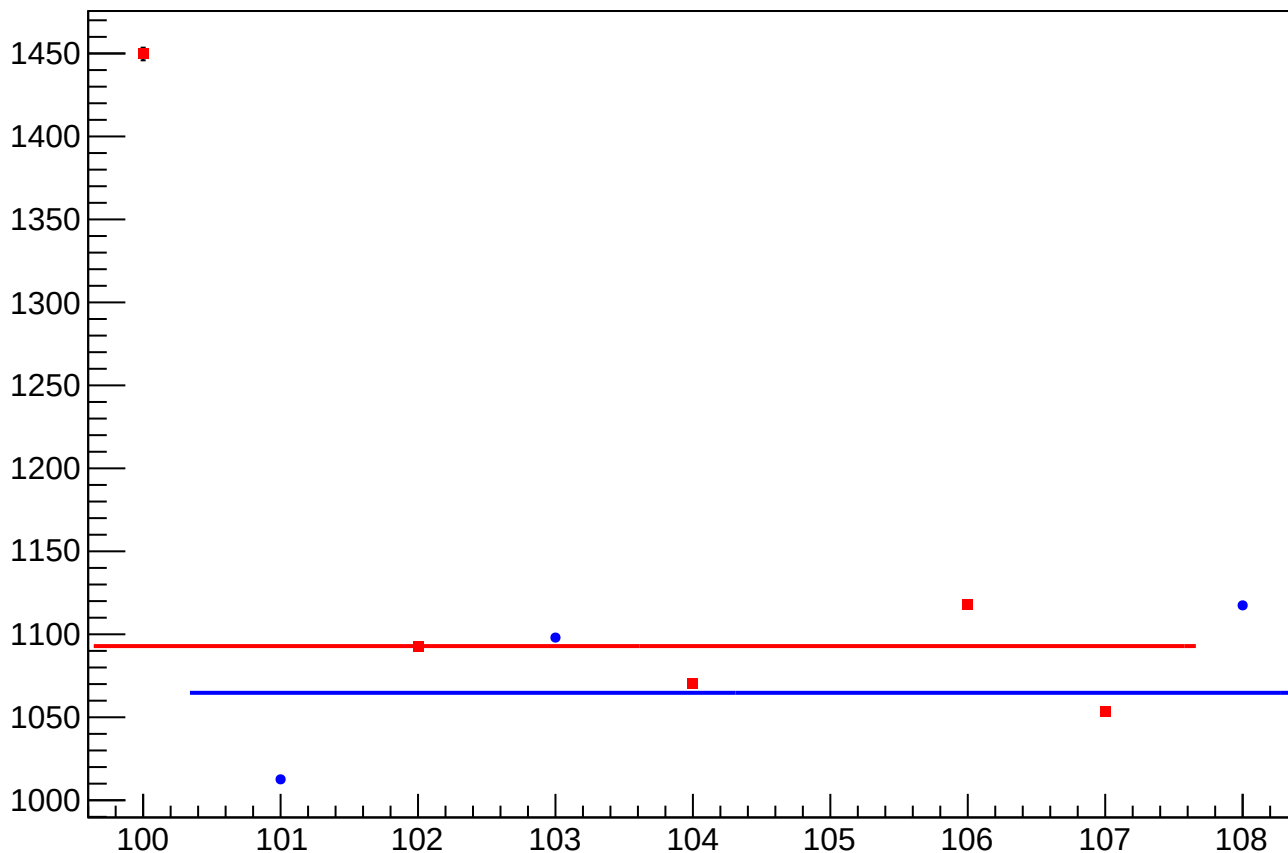
asym_sam_15_26_dd_reg_correction_rms vs Slug, Sign Corrected
