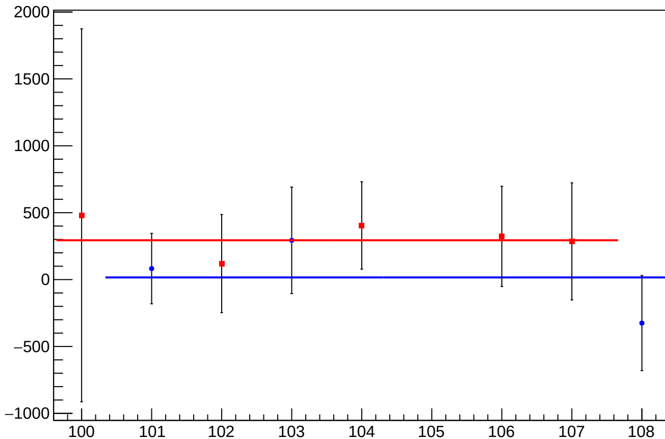
eigen_cor_asym_sam4_mean vs Slug, Sign Corrected
