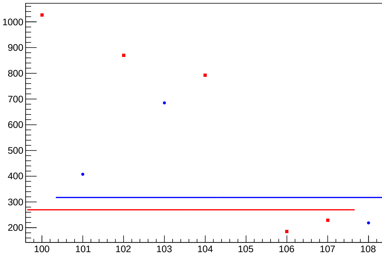
asym_at2_avg_eigen_dit_vs_cor_diff_rms vs Slug, Sign Corrected
