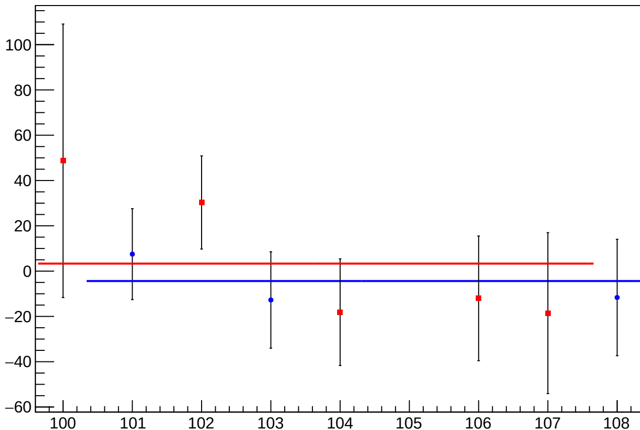
asym_bcm_an_us_ds3_avg_bcm_dg_ds_agg_dd_mean vs Slug, Sign Corrected
