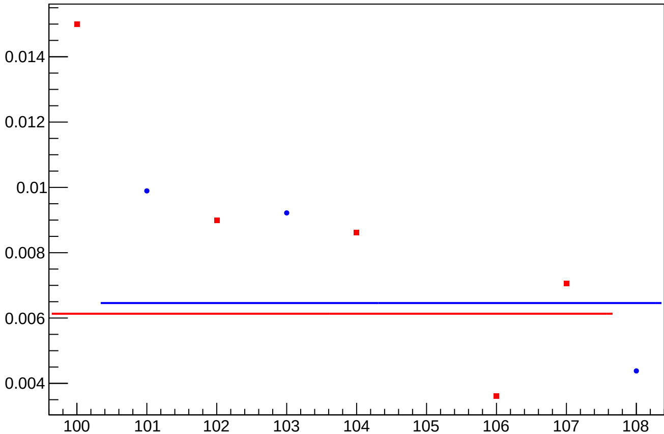
asym_atl1r2_dd_atl2r1_dd_dd_eigen_dit_vs_dit_diff_rms vs Slug, Sign Corrected
