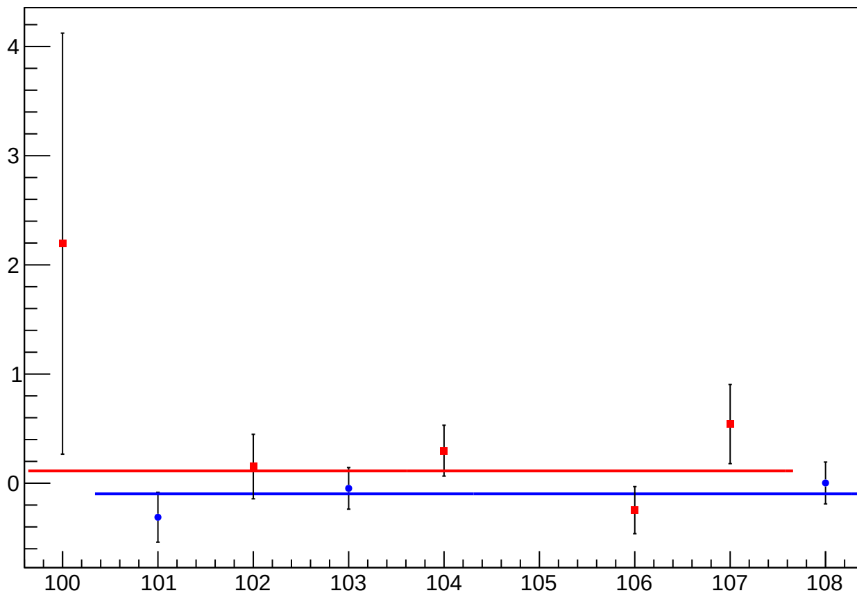
asym_usl_atl2_avg_dit_vs_eigen_cor_diff_mean vs Slug, Sign Corrected
