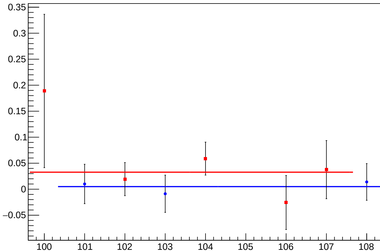
asym_us_dd_dit_vs_cor_diff_mean vs Slug, Sign Corrected
