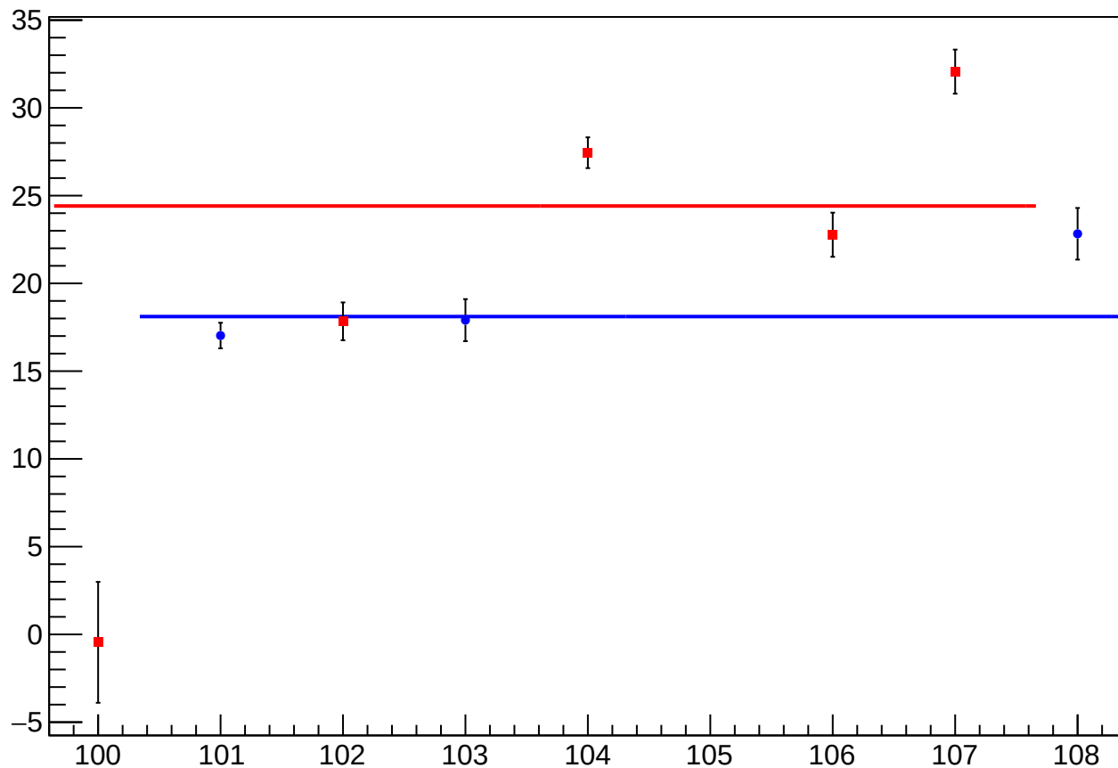
reg_asym_sam_1548_avg_diff_bpm4eY_slope vs Slug, Sign Corrected
