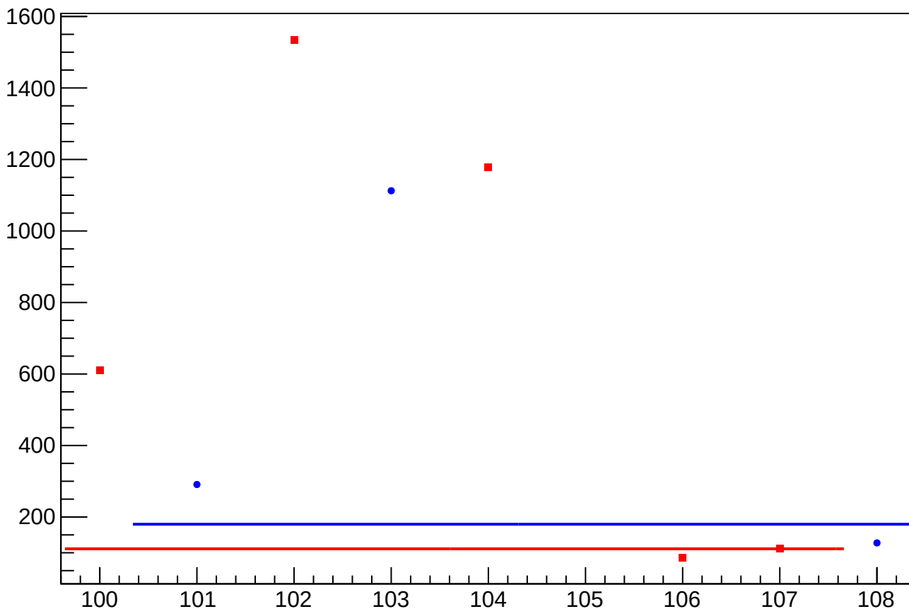
asym_atr_avg_eigen_dit_vs_cor_diff_rms vs Slug, Sign Corrected
