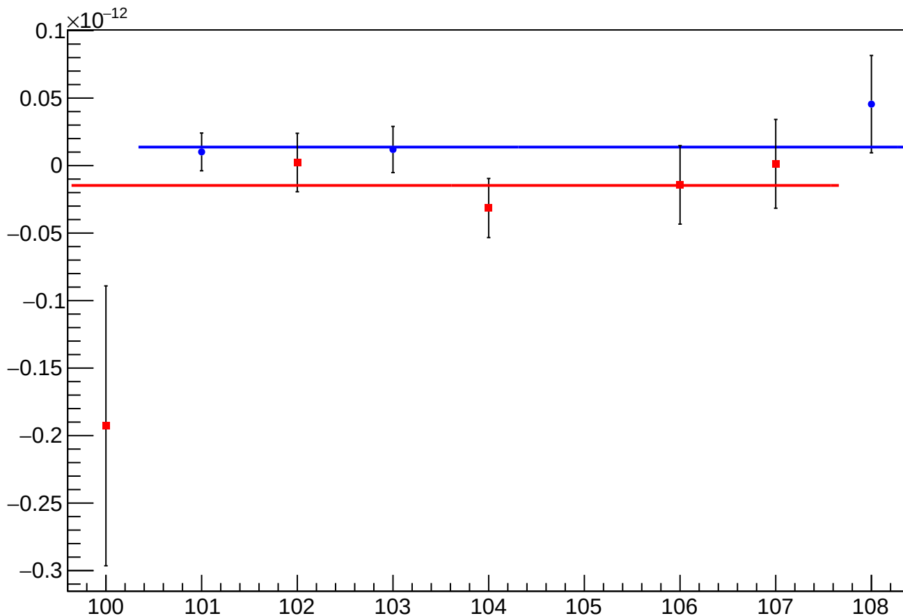
asym_sam_15_dd_eigen_cor_vs_cor_diff_mean vs Slug, Sign Corrected
