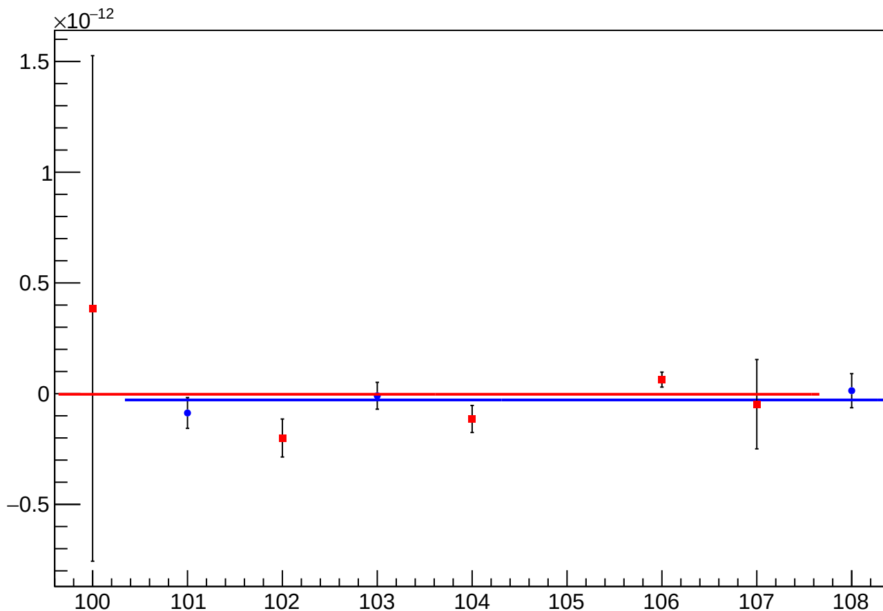
asym_atl_avg_atr_avg_dd_reg_vs_cor_diff_mean vs Slug, Sign Corrected
