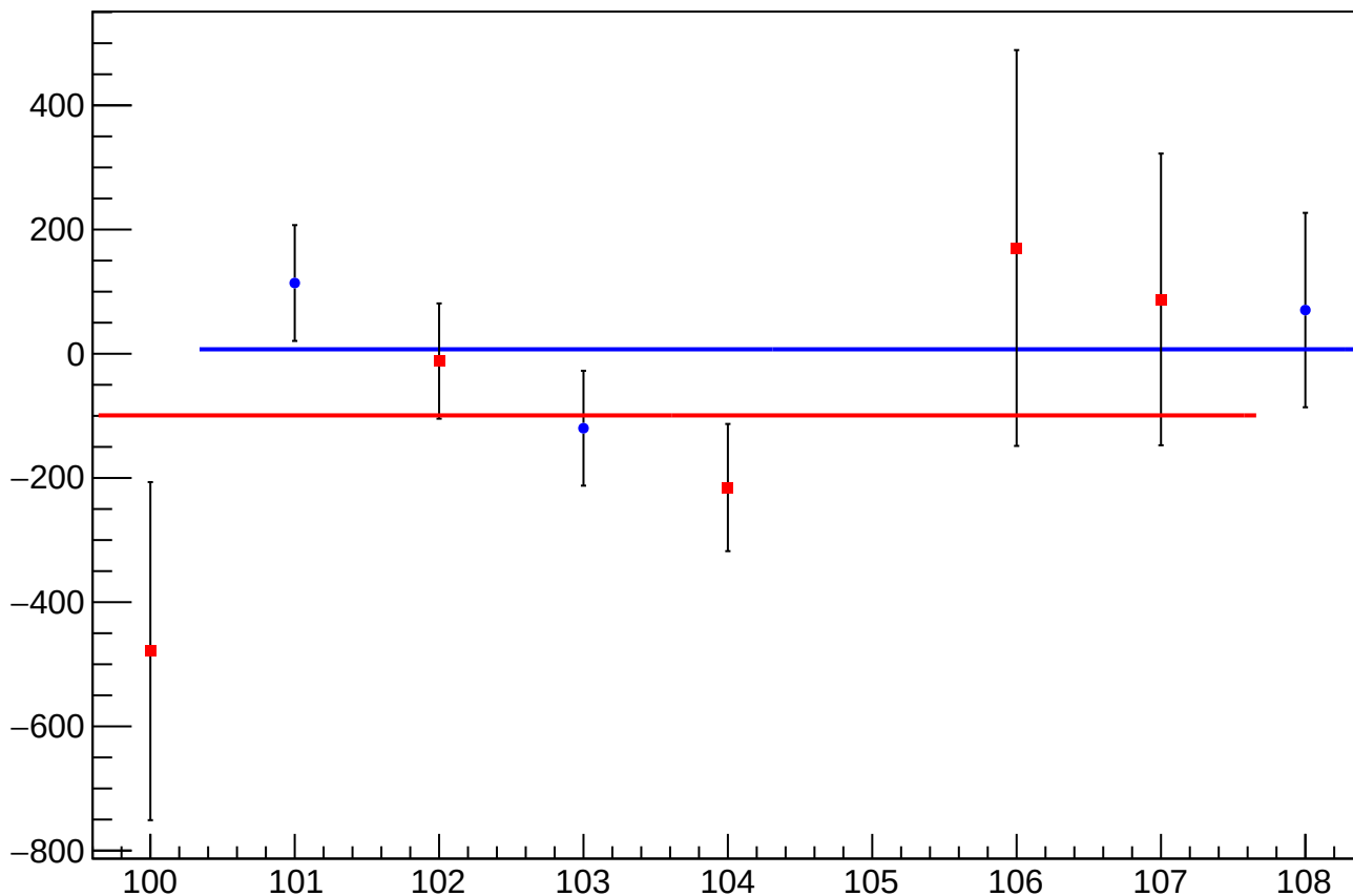
asym_sam_15_avg_dit_correction_mean vs Slug, Sign Corrected
