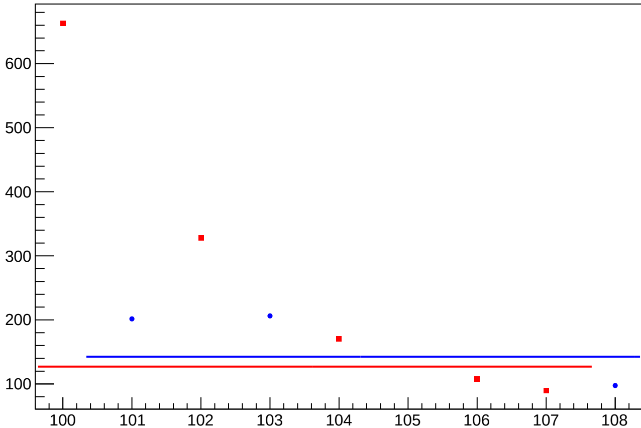
asym_atl_dd_atr_dd_avg_eigen_dit_vs_eigen_cor_diff_rms vs Slug, Sign Corrected
