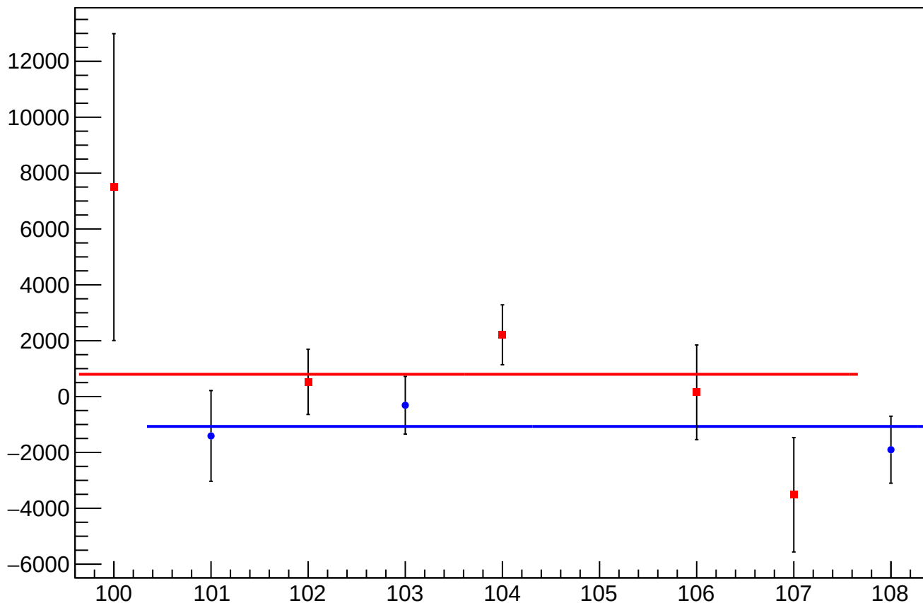
eigen_cor_asym_usl_atl2_dd_mean vs Slug, Sign Corrected
