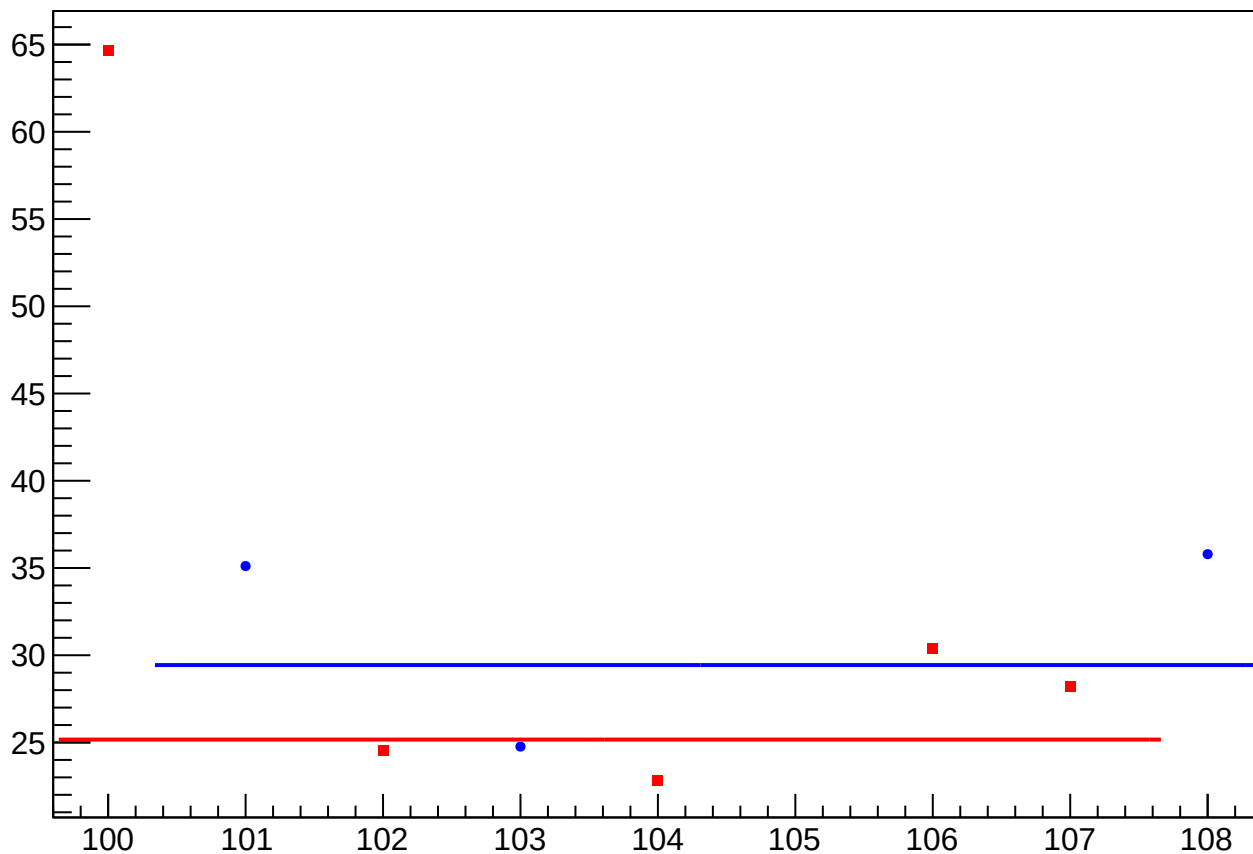
asym_sam_1548_avg_eigen_dit_vs_cor_diff_rms vs Slug, Sign Corrected
