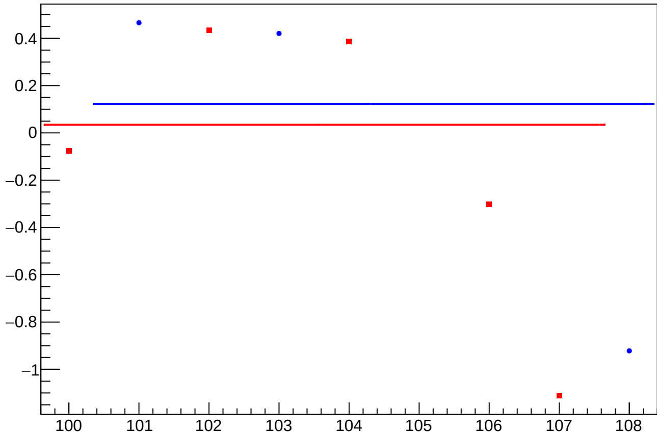
yield_bpm0r05X_mean vs Slug, Sign Corrected
