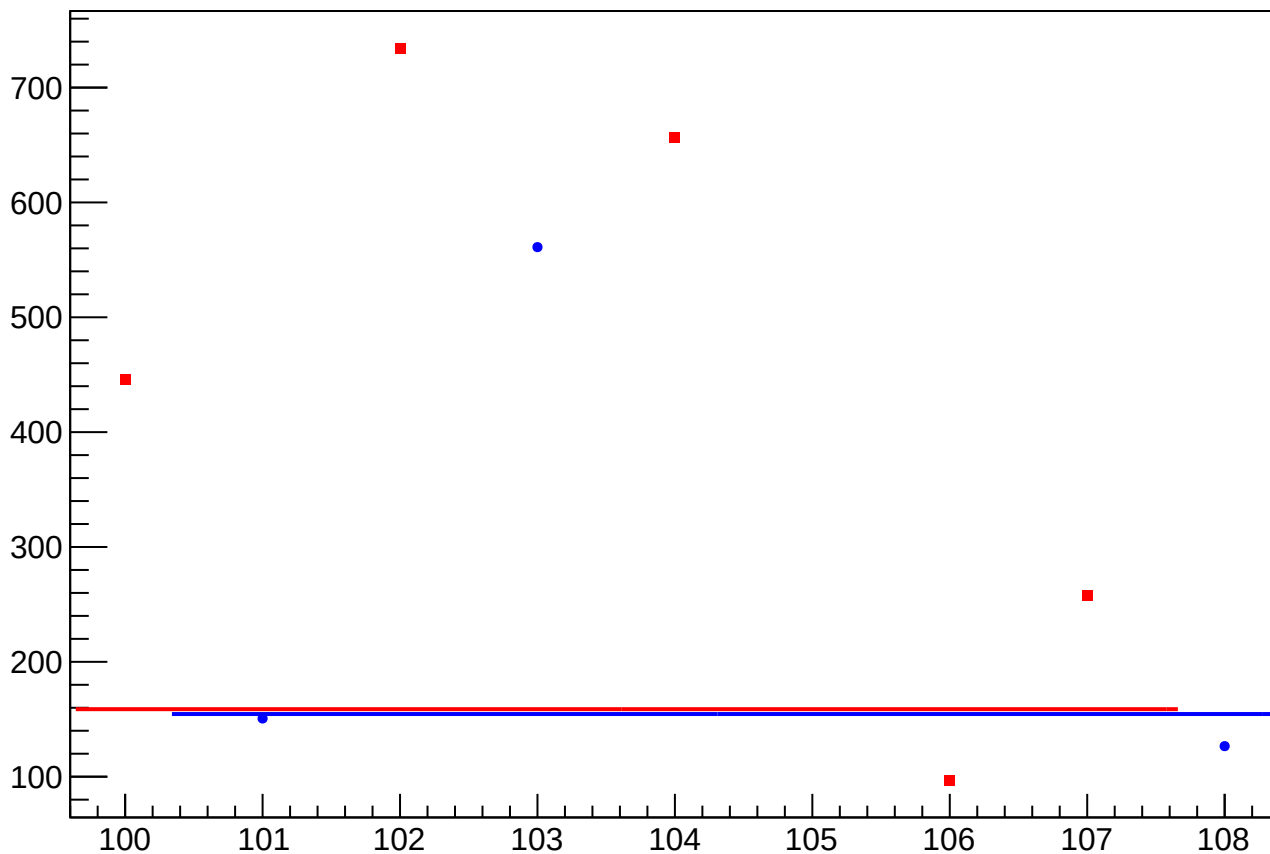
asym_atl_avg_eigen_dit_vs_eigen_cor_diff_rms vs Slug, Sign Corrected
