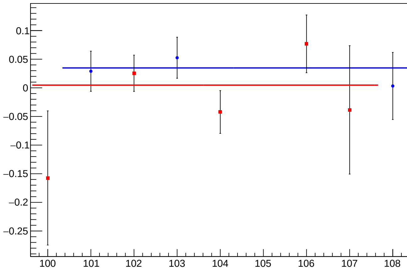
asym_us_avg_overload_cor_vs_cor_diff_mean vs Slug, Sign Corrected
