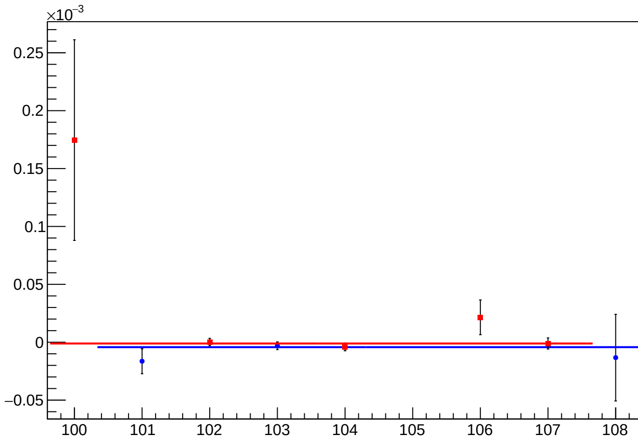
asym_at2_dd_eigen_dit_vs_dit_diff_mean vs Slug, Sign Corrected
