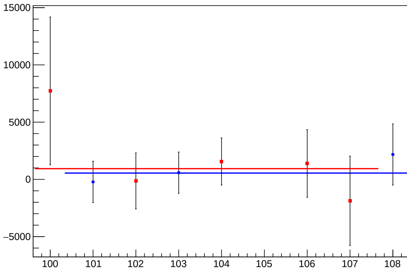
eigen_dit_asym_usl_atl1_dd_mean vs Slug, Sign Corrected
