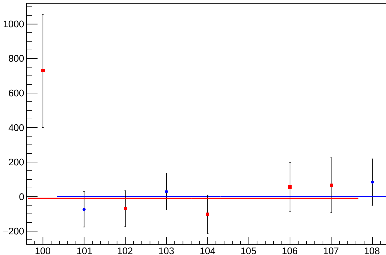
eigen_cor_asym_sam5_mean vs Slug, Sign Corrected
