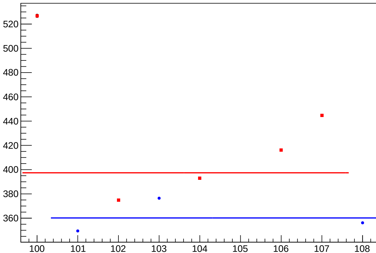
asym_sam6_cor_correction_rms vs Slug, Sign Corrected
