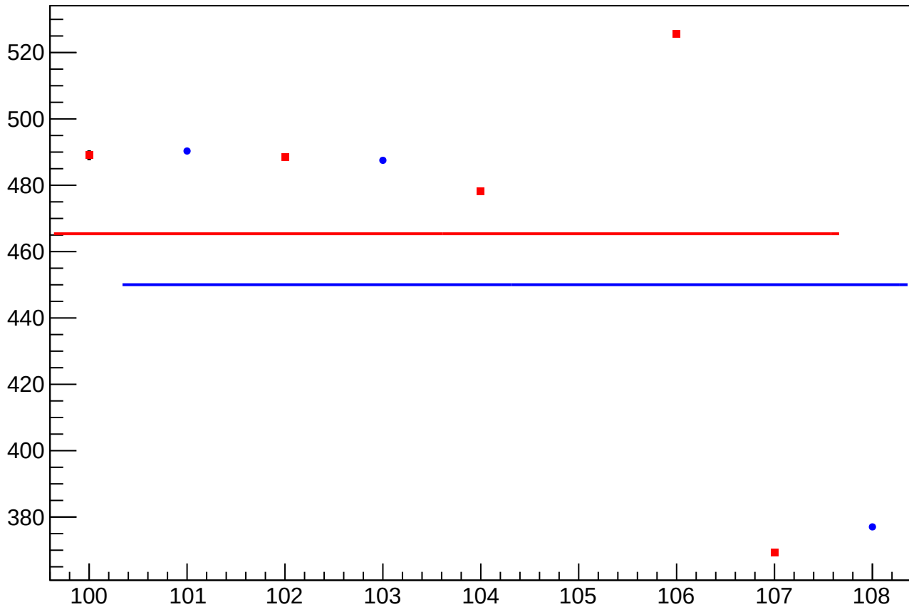
diff_bpm_4aX_4ecX_dd_rms vs Slug, Sign Corrected
