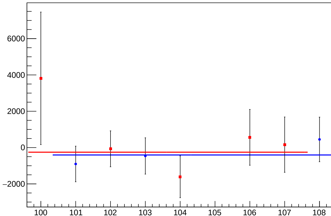
asym_sam_26_48_dd_reg_correction_mean vs Slug, Sign Corrected
