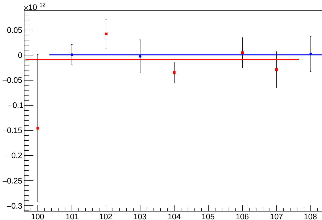
asym_sam_13_57_dd_eigen_cor_vs_cor_diff_mean vs Slug, Sign Corrected
