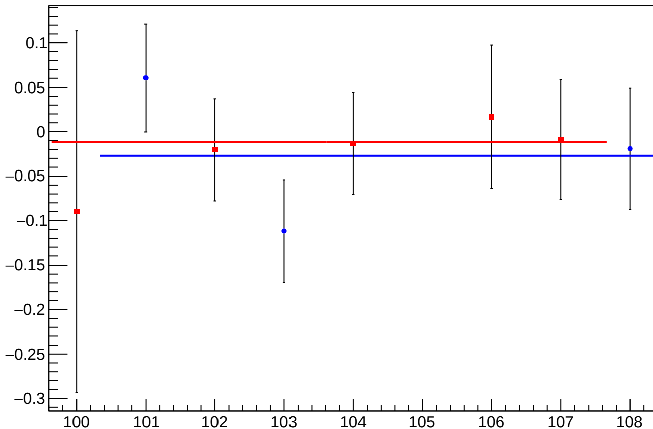
asym_sam_15_dd_eigen_dit_vs_cor_diff_mean vs Slug, Sign Corrected
