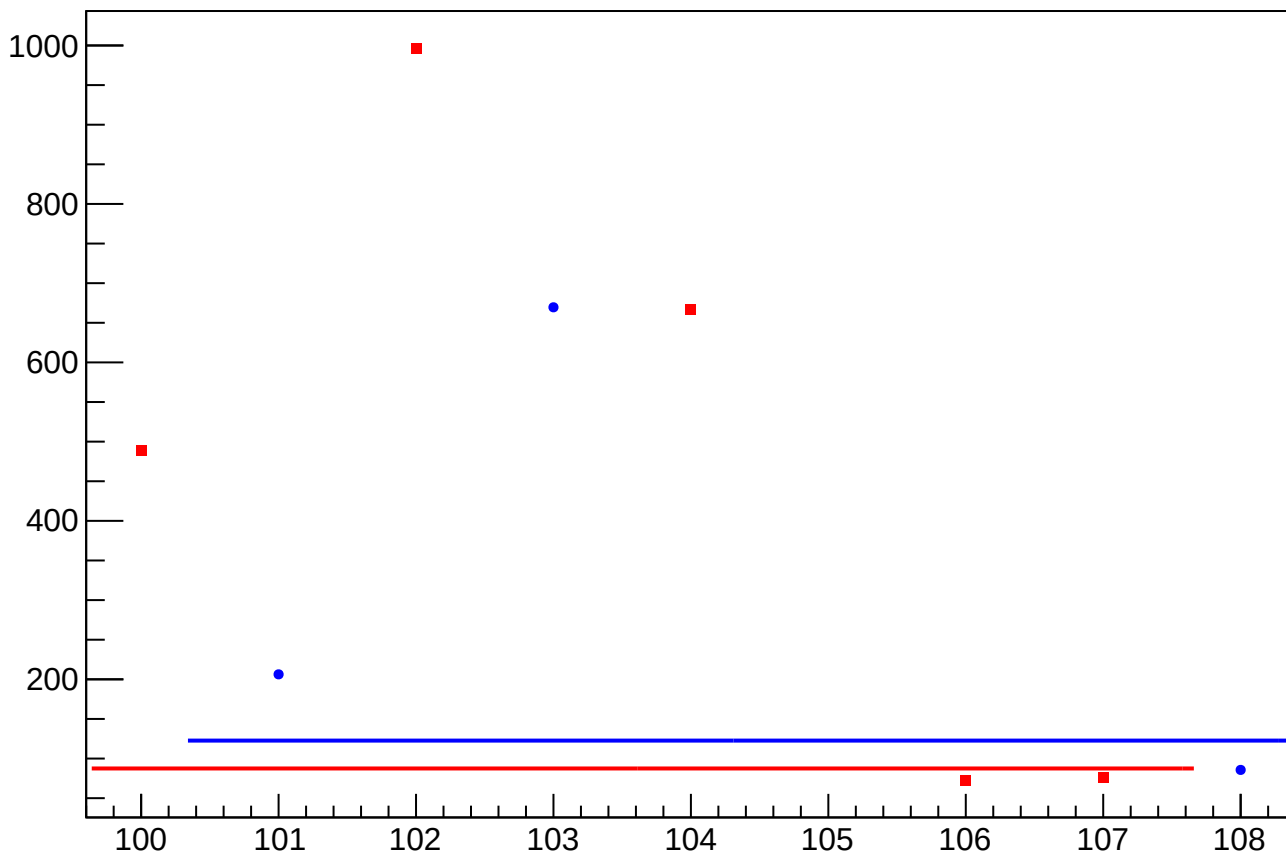
asym_usr_atr2_dd_dit_vs_cor_diff_rms vs Slug, Sign Corrected
