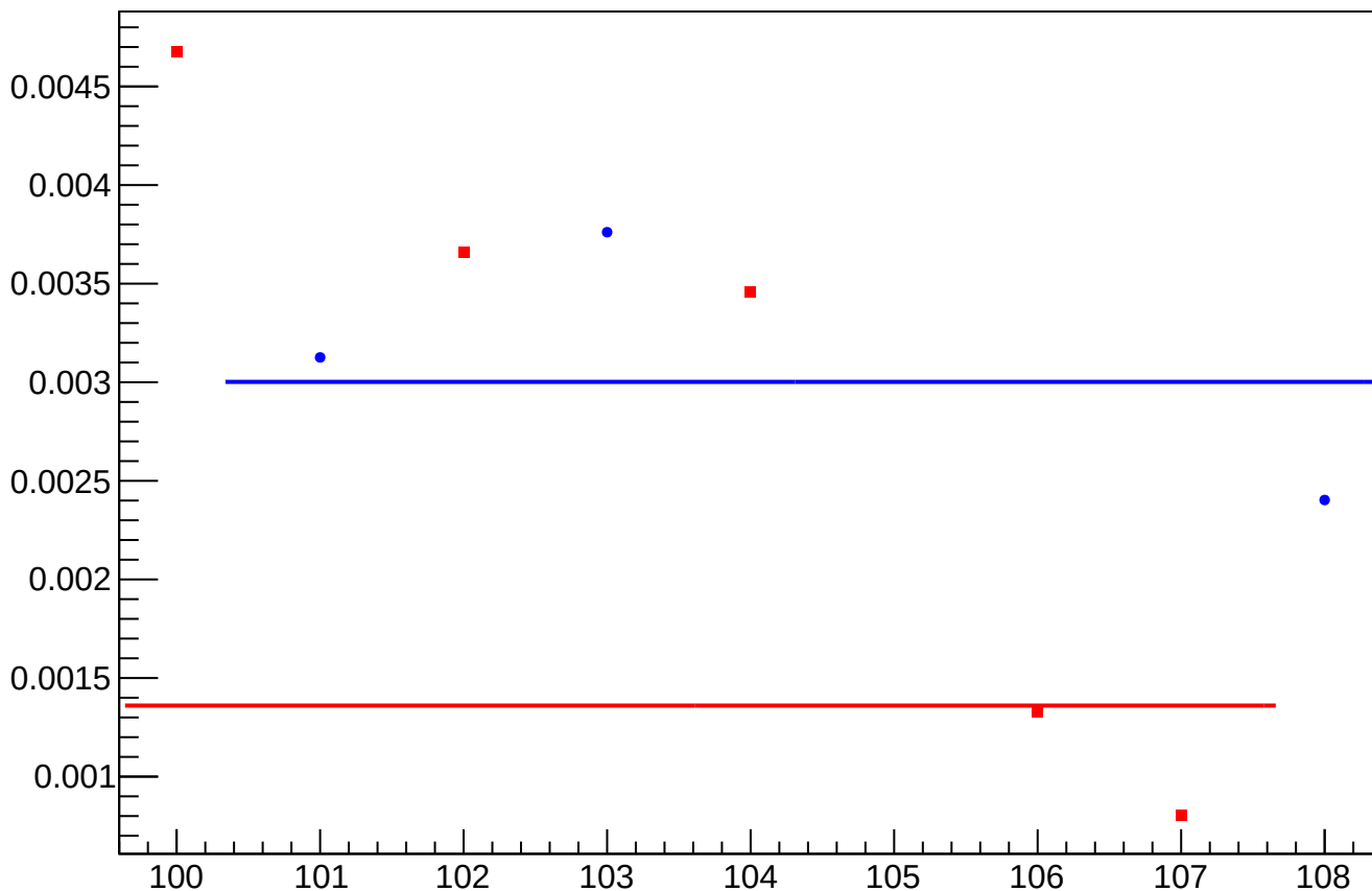
asym_sam_37_dd_eigen_dit_vs_dit_diff_rms vs Slug, Sign Corrected
