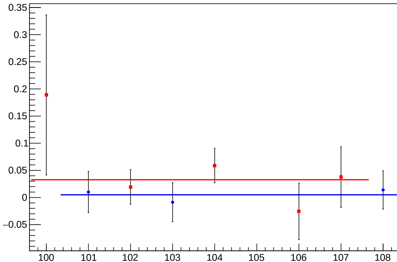
asym_us_dd_eigen_dit_vs_eigen_cor_diff_mean vs Slug, Sign Corrected
