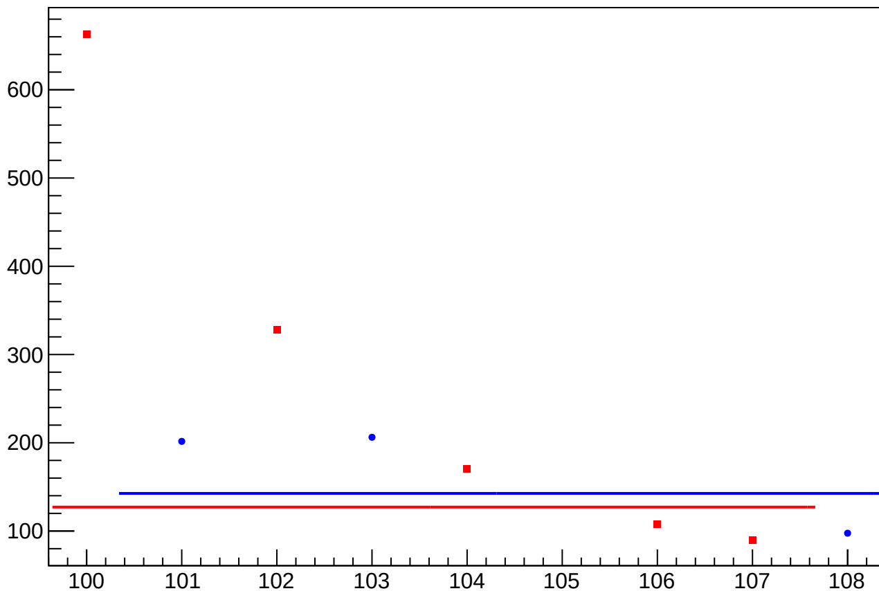
asym_atl1r2_dd_atl2r1_dd_dd_dit_vs_cor_diff_rms vs Slug, Sign Corrected
