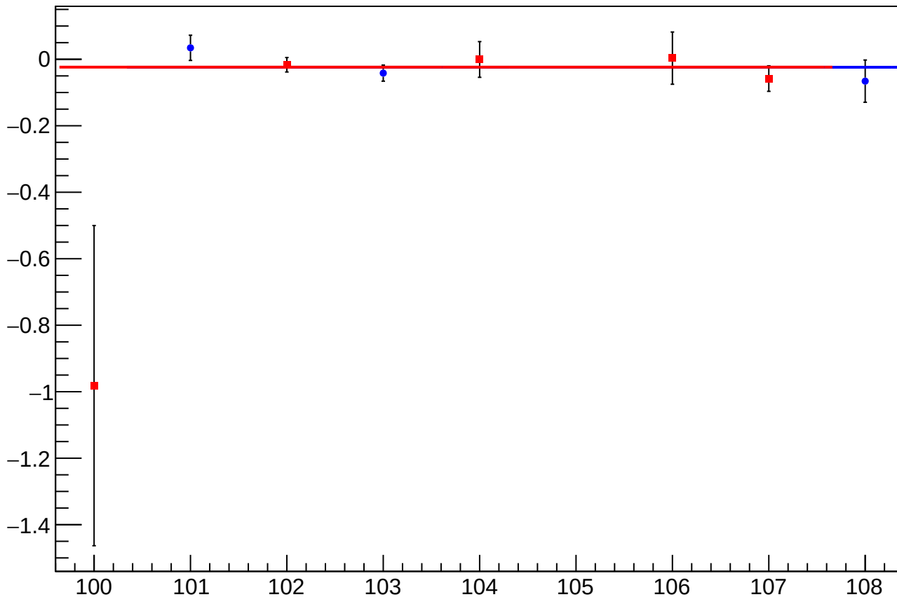
asym_sam_1357_avg_eigen_dit_vs_eigen_cor_diff_mean vs Slug, Sign Corrected
