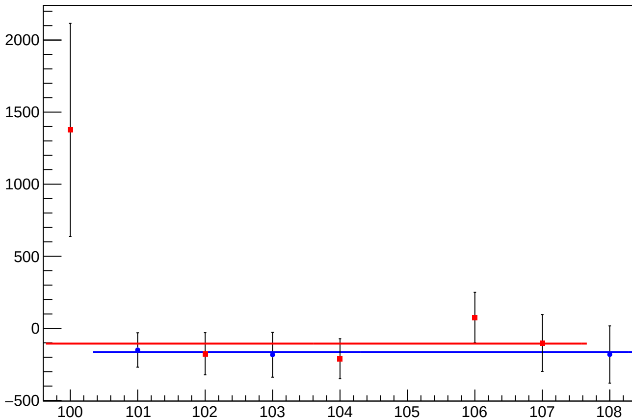
eigen_dit_asym_sam6_mean vs Slug, Sign Corrected
