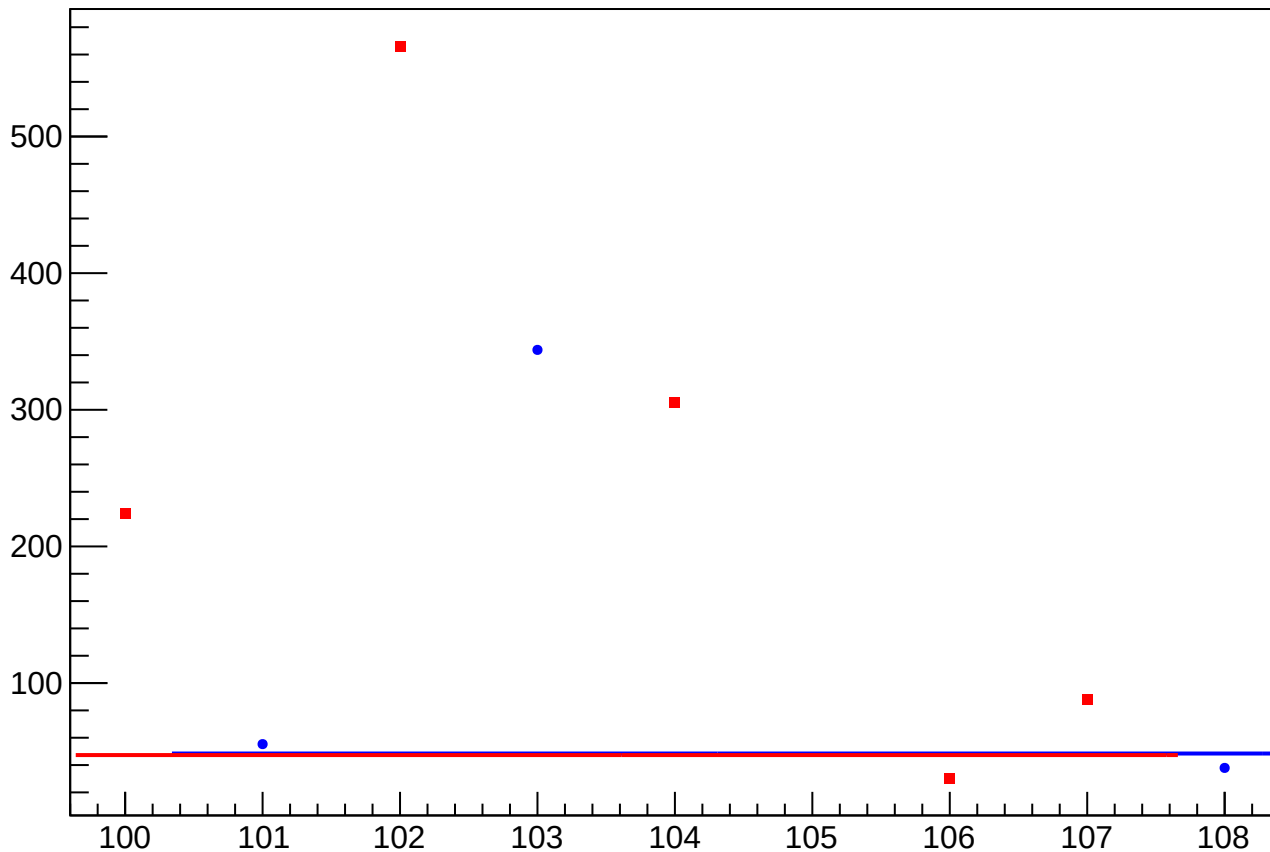
asym_atl_dd_atr_dd_dd_dit_vs_eigen_cor_diff_rms vs Slug, Sign Corrected
