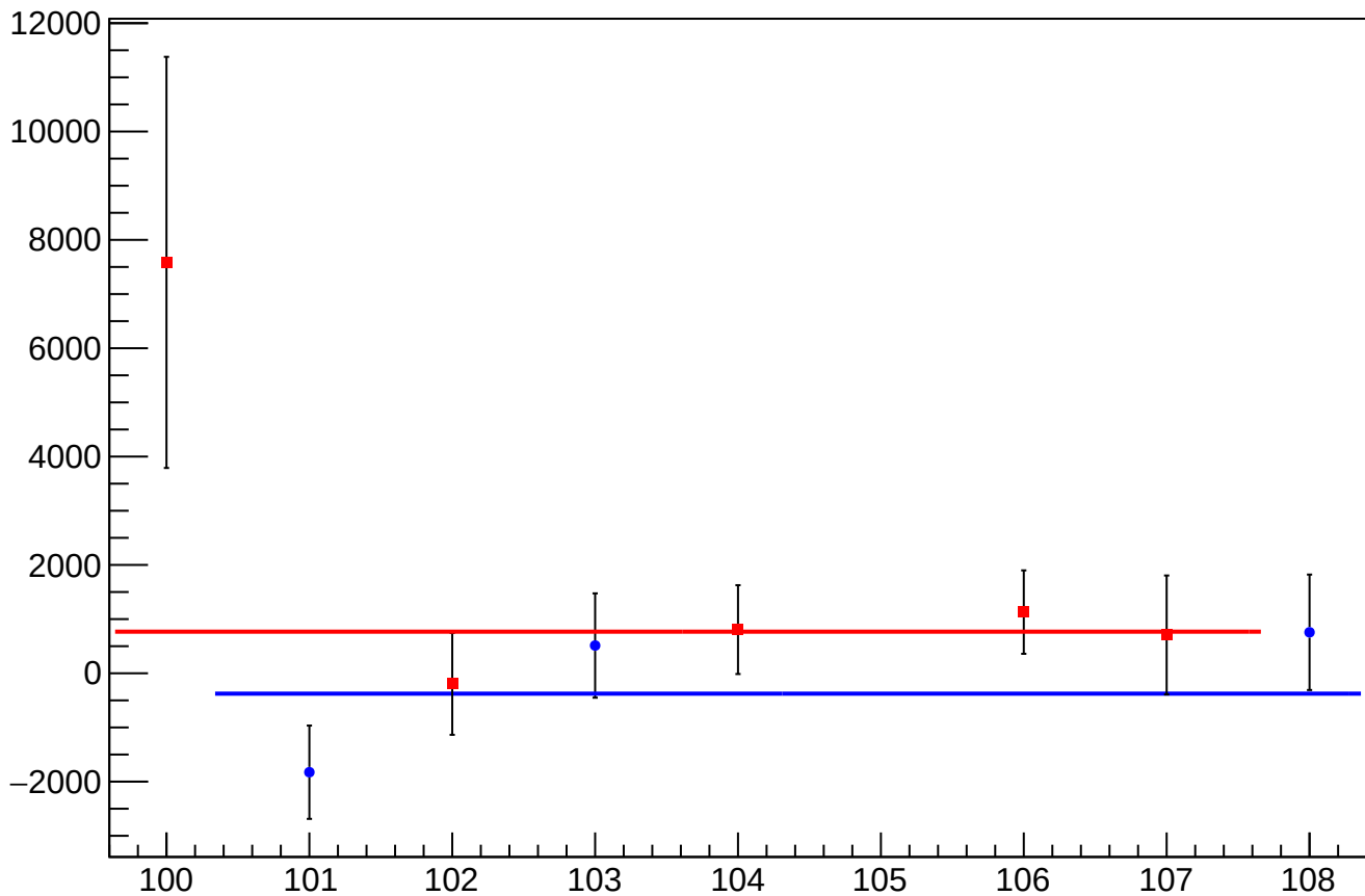
asym_sam_37_dd_reg_correction_mean vs Slug, Sign Corrected
