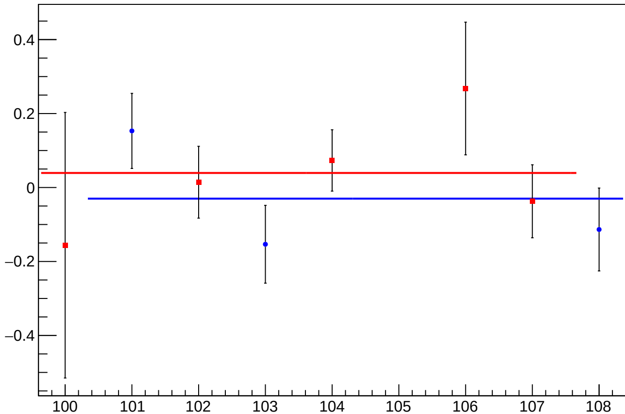
asym_sam_1526_avg_dit_vs_cor_diff_mean vs Slug, Sign Corrected
