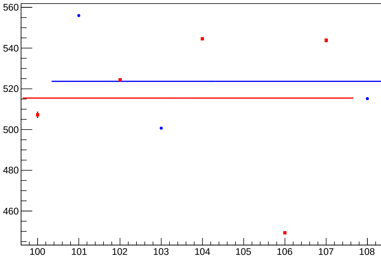
asym_sam5_reg_correction_rms vs Slug, Sign Corrected
