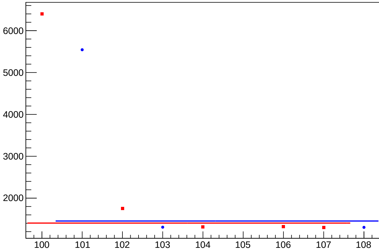
reg_asym_usr_atr1_dd_rms vs Slug, Sign Corrected
