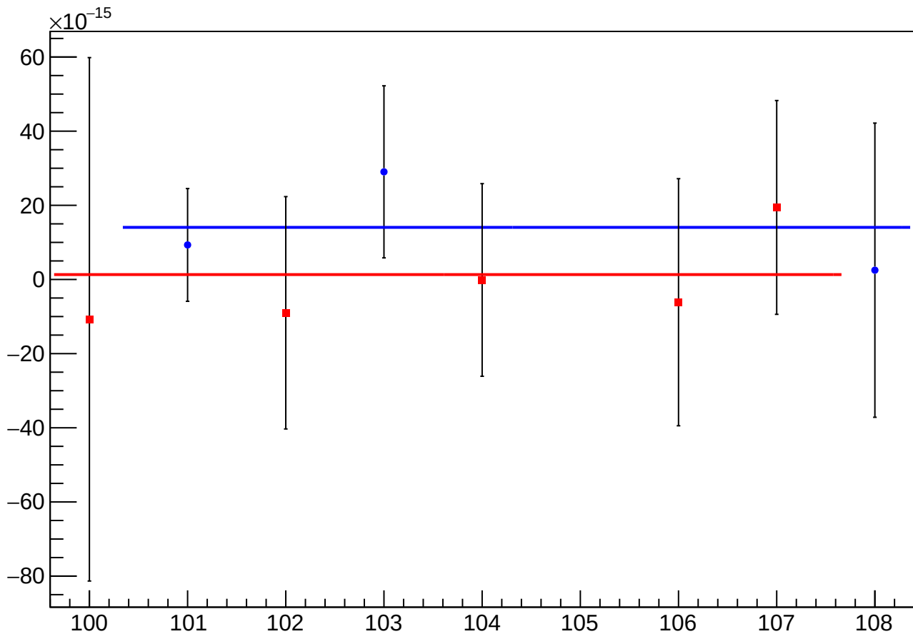
asym_sam1_eigen_cor_vs_cor_diff_mean vs Slug, Sign Corrected
