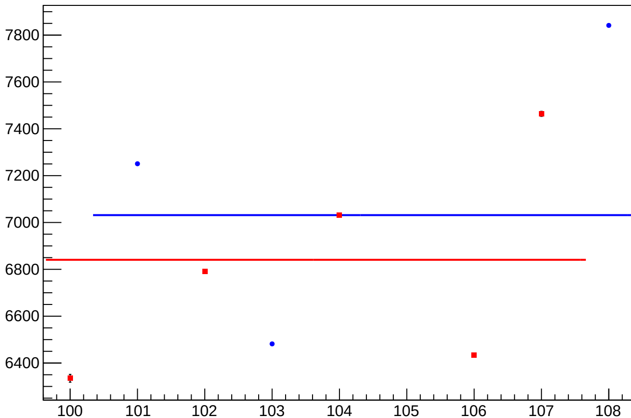
diff_bpm_4aY_4ecY_avg_rms vs Slug, Sign Corrected
