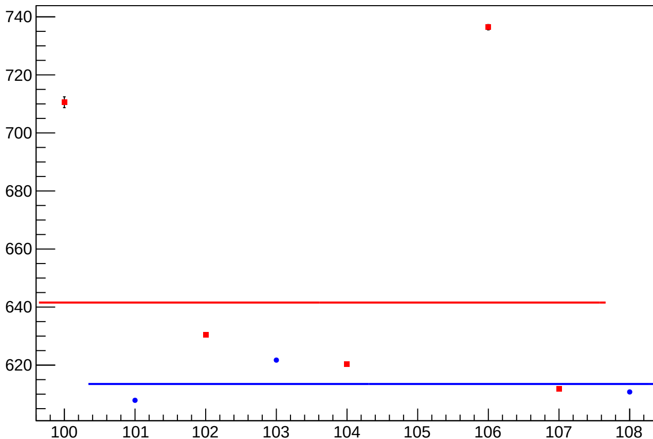
asym_sam_37_26_dd_reg_correction_rms vs Slug, Sign Corrected
