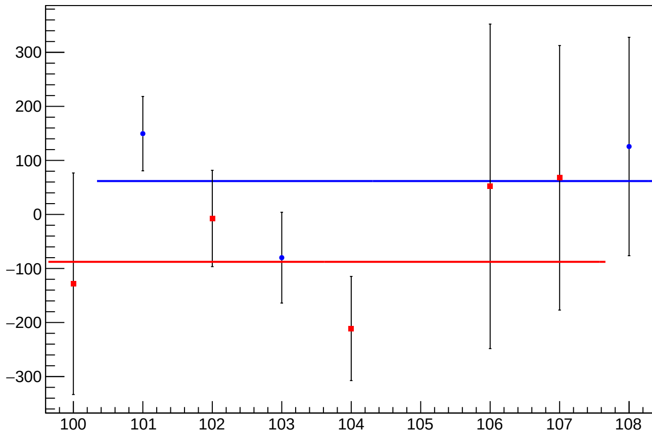
asym_sam_15_avg_reg_correction_mean vs Slug, Sign Corrected
