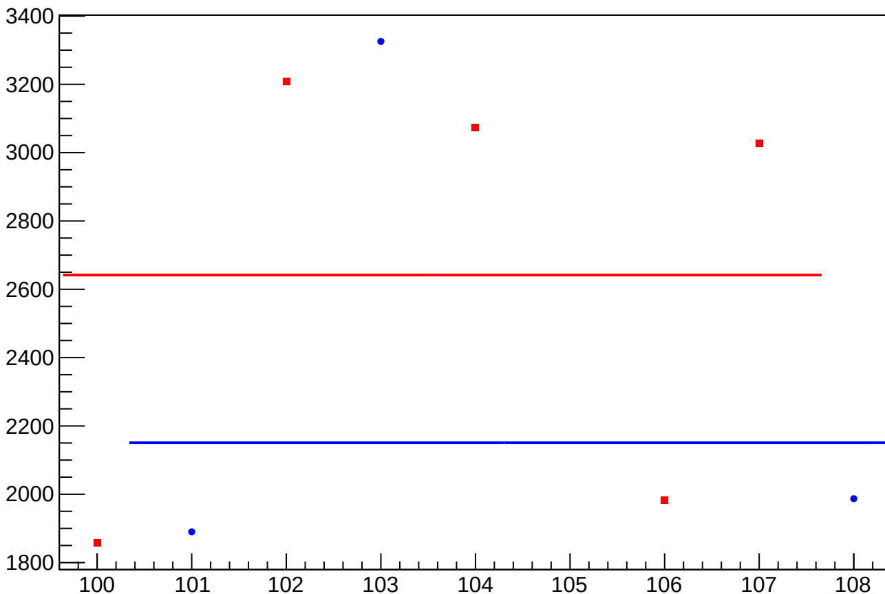
asym_us_dd_at1lr_dd_dd_eigen_dit_correction_rms vs Slug, Sign Corrected
