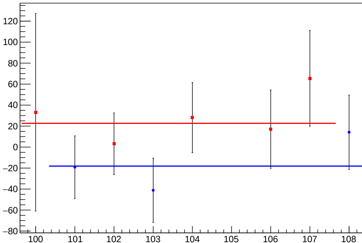
asym_bcm_dg_us_an_ds_dd_mean vs Slug, Sign Corrected
