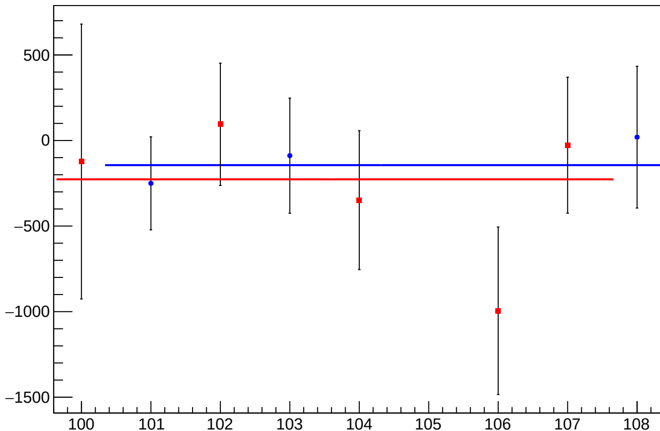
asym_bcm_dg_ds_an_ds_avg_mean vs Slug, Sign Corrected
