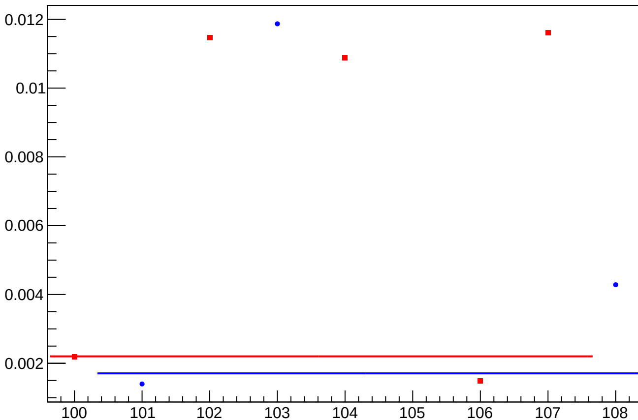
asym_usl_atl1_avg_eigen_dit_vs_dit_diff_rms vs Slug, Sign Corrected
