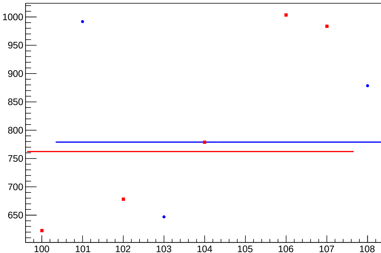
diff_bpm_4aY_4eY_dd_rms vs Slug, Sign Corrected
