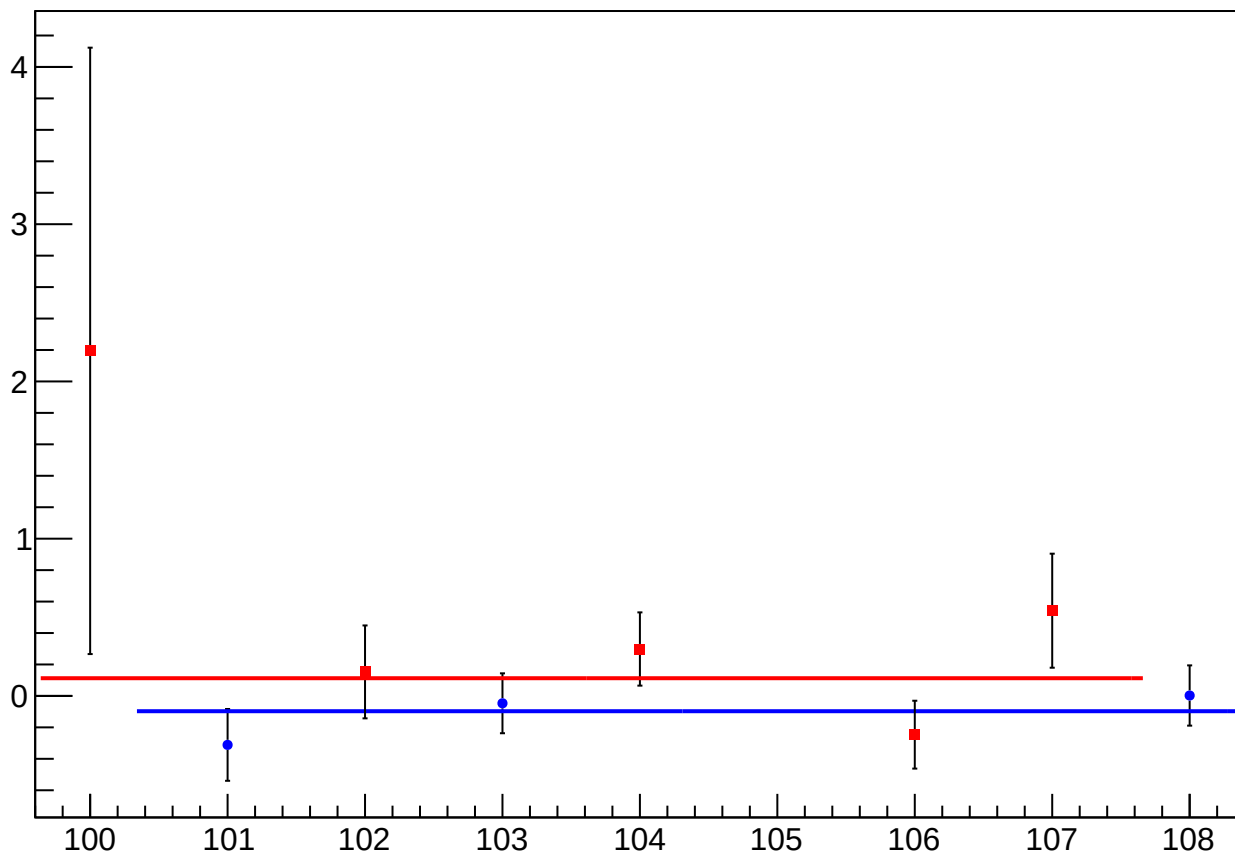
asym_usl_atl2_avg_eigen_dit_vs_eigen_cor_diff_mean vs Slug, Sign Corrected
