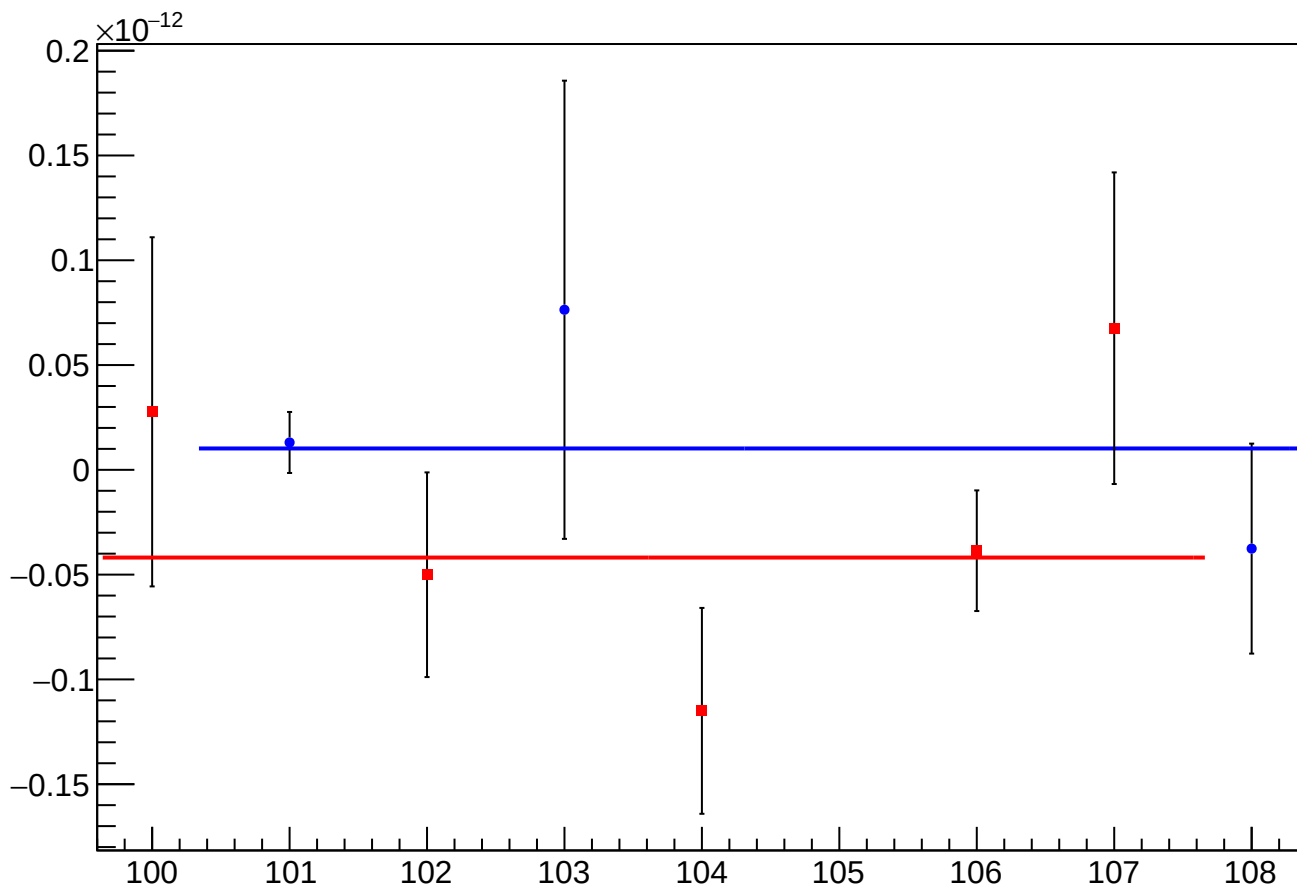
asym_us_avg_at1lr_avg_dd_eigen_cor_vs_cor_diff_mean vs Slug, Sign Corrected
