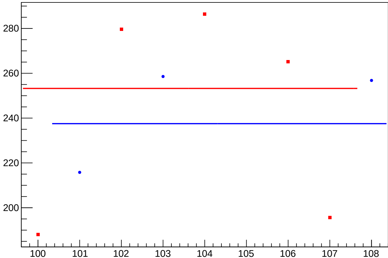
asym_bcm_target_rms vs Slug, Sign Corrected
