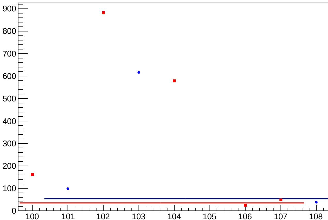
asym_at2_dd_dit_vs_eigen_cor_diff_rms vs Slug, Sign Corrected
