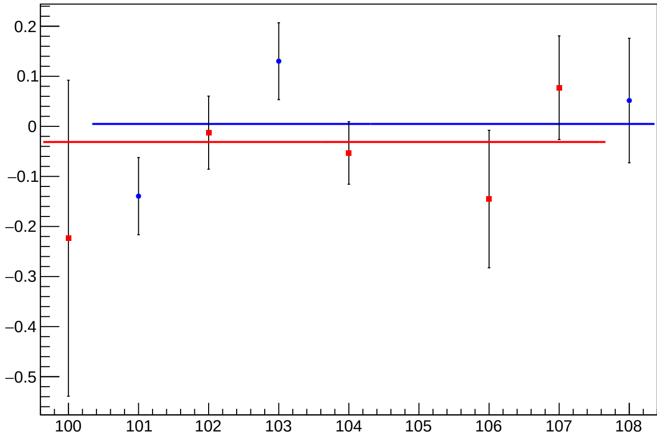
asym_sam_15_26_dd_dit_vs_cor_diff_mean vs Slug, Sign Corrected
