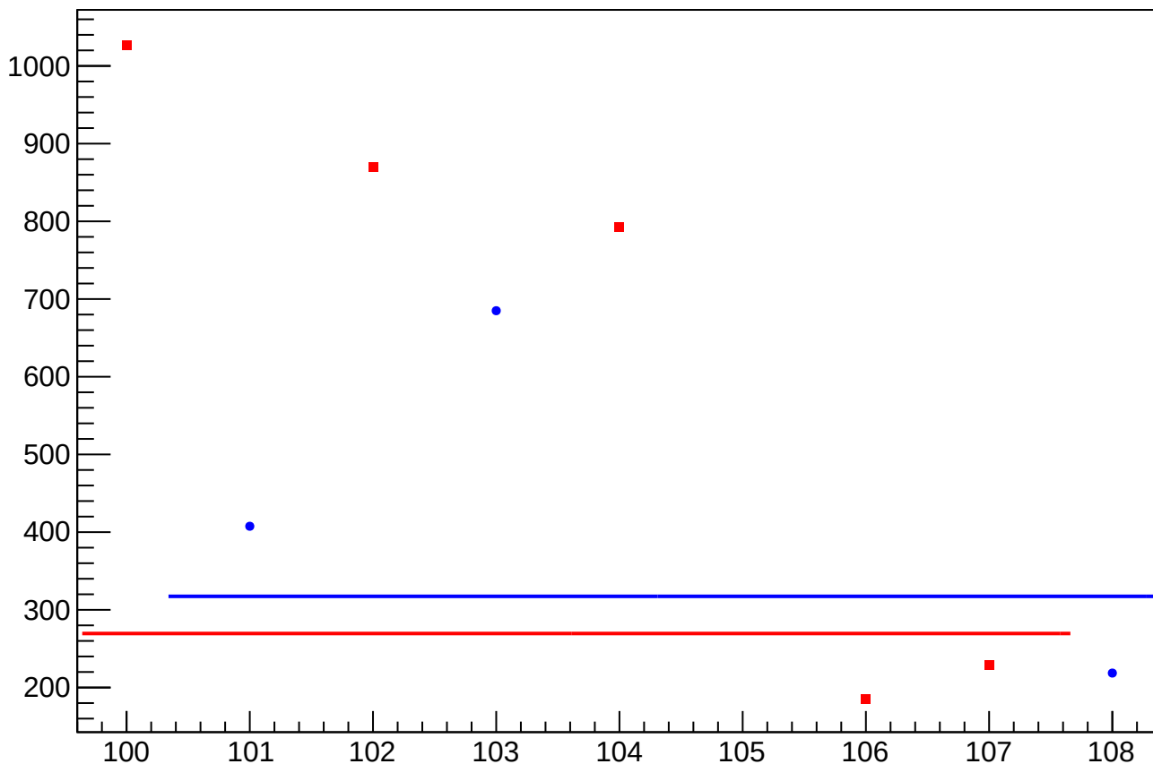
asym_at2_avg_dit_vs_eigen_cor_diff_rms vs Slug, Sign Corrected
