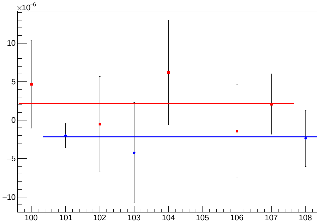
asym_sam_1526_avg_eigen_dit_vs_dit_diff_mean vs Slug, Sign Corrected
