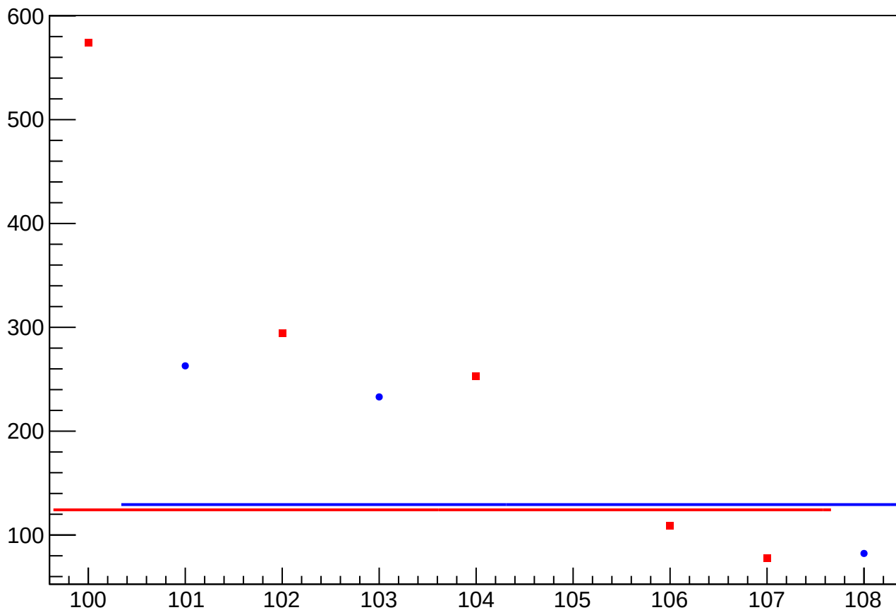
asym_atl1r2_dd_eigen_dit_vs_cor_diff_rms vs Slug, Sign Corrected
