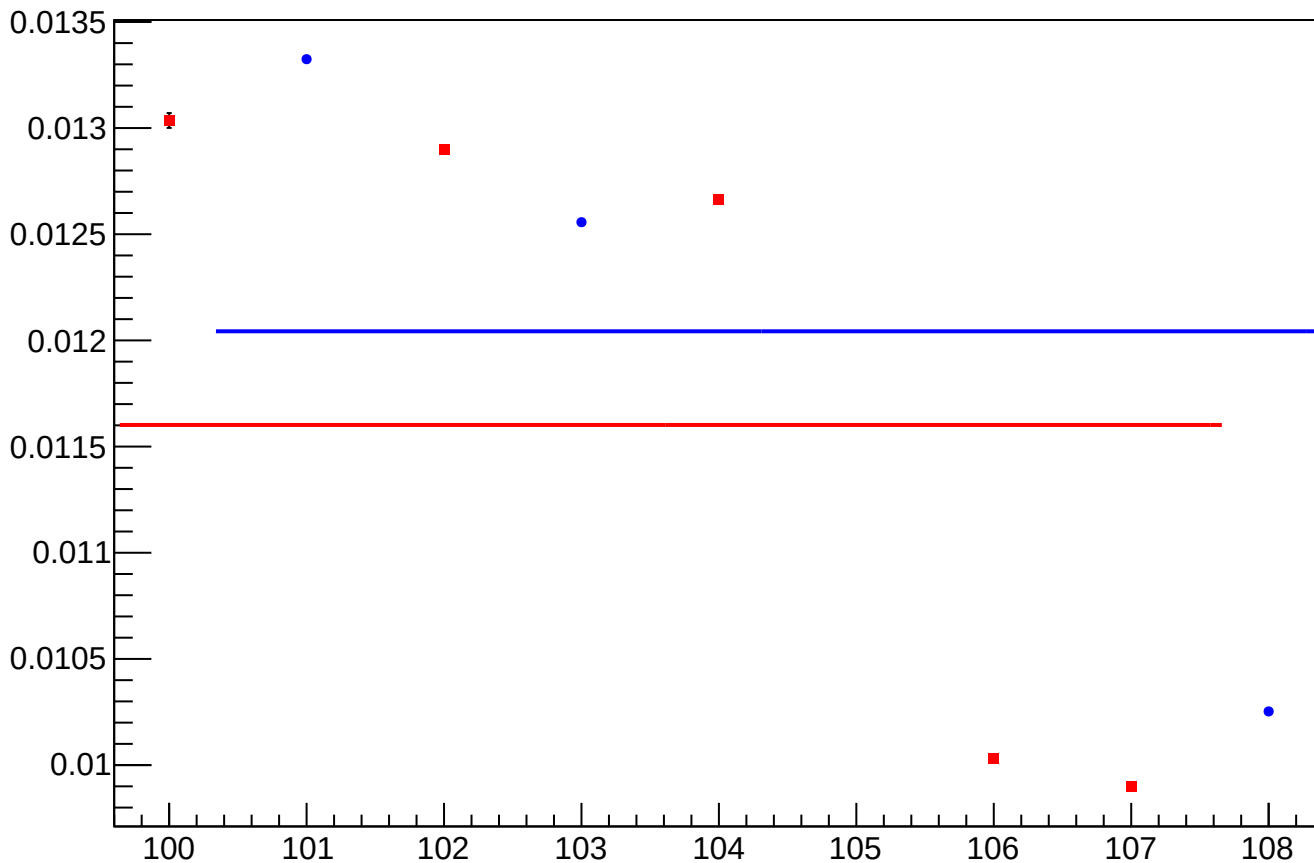
yield_bpm0l07X_rms vs Slug, Sign Corrected
