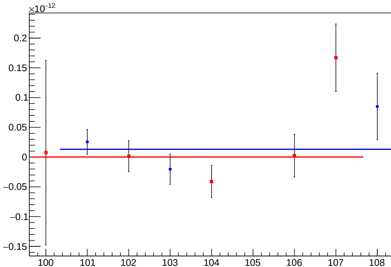
asym_sam8_reg_vs_cor_diff_mean vs Slug, Sign Corrected
