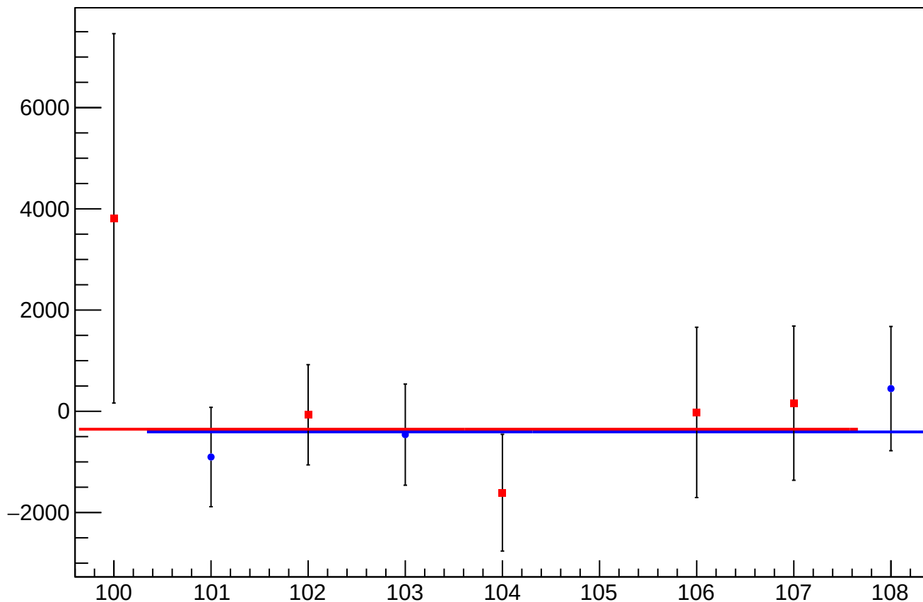
asym_sam_26_48_dd_cor_correction_mean vs Slug, Sign Corrected
