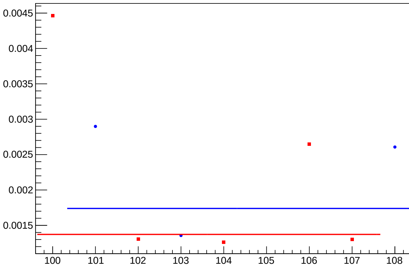
asym_sam_48_avg_eigen_dit_vs_dit_diff_rms vs Slug, Sign Corrected
