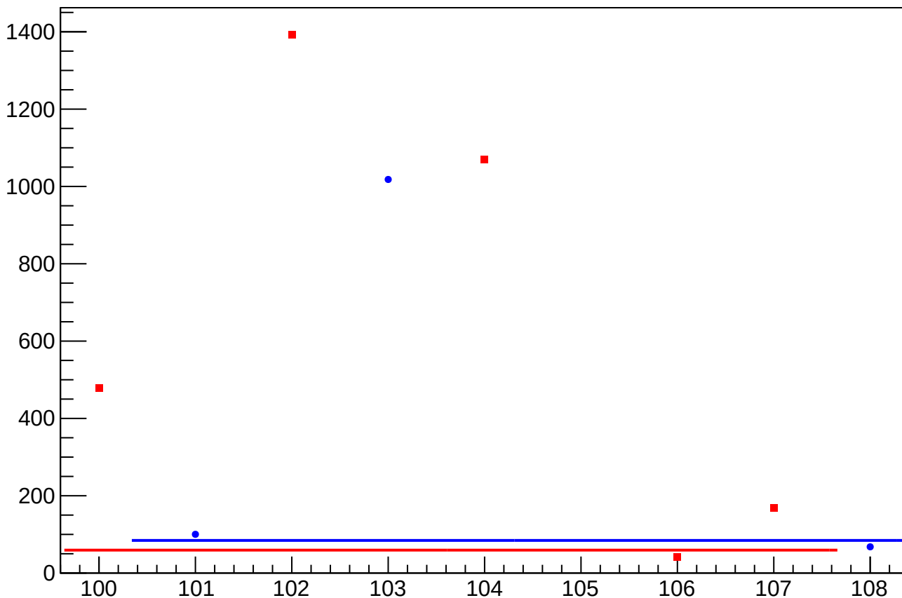
asym_at1_avg_eigen_dit_vs_eigen_cor_diff_rms vs Slug, Sign Corrected
