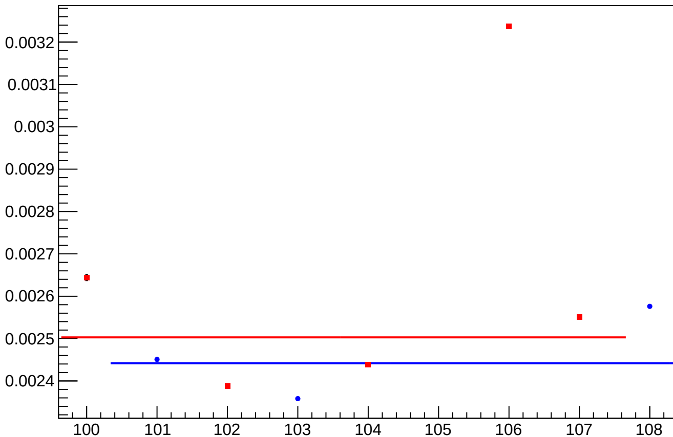
yield_bpm0l07Y_rms vs Slug, Sign Corrected
