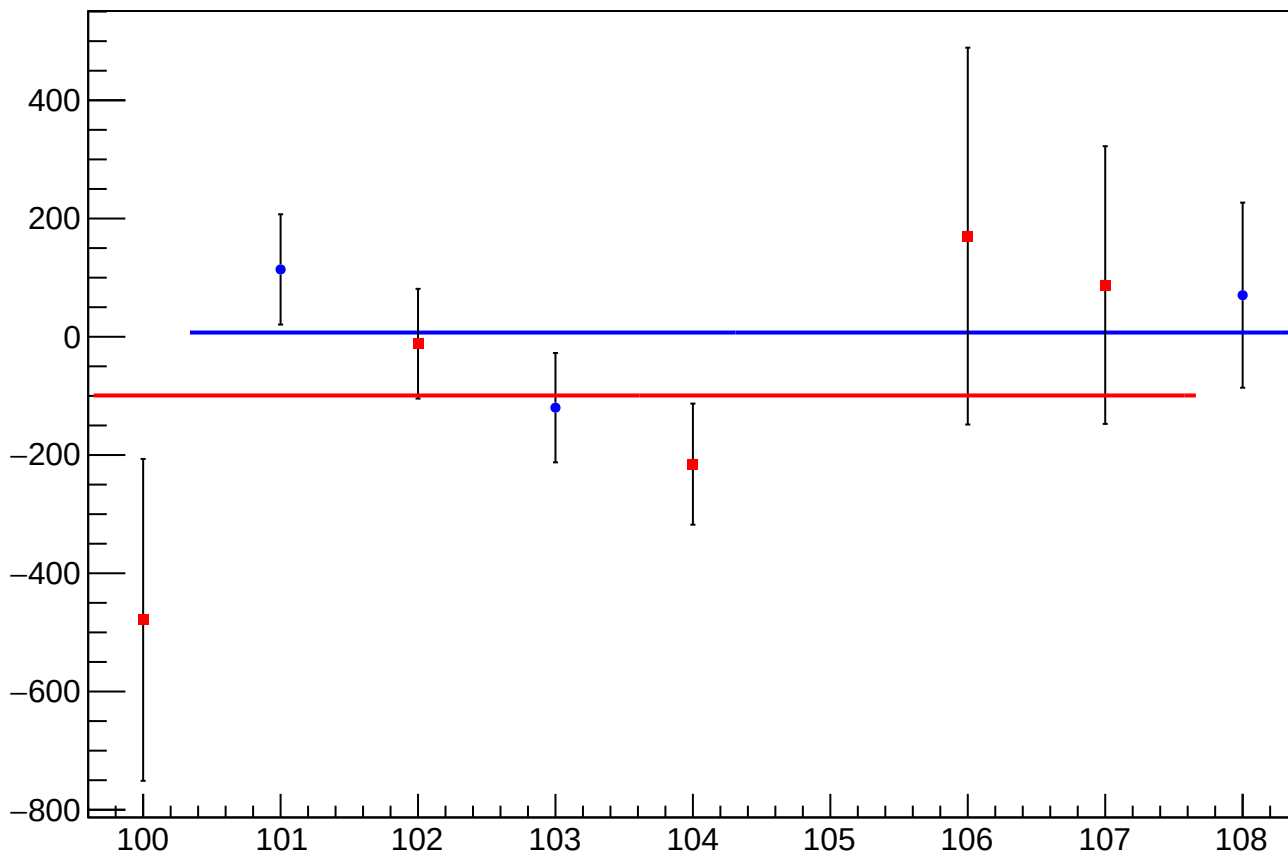
asym_sam_15_avg_eigen_dit_correction_mean vs Slug, Sign Corrected
