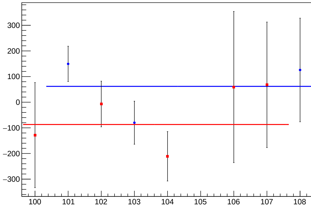
asym_sam_15_avg_eigen_cor_correction_mean vs Slug, Sign Corrected
