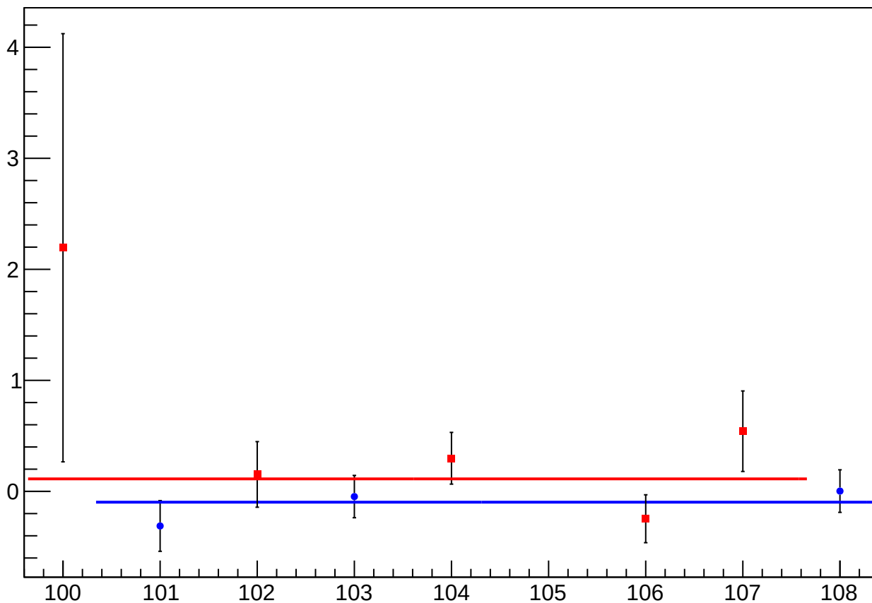
asym_usl_atl2_avg_dit_vs_cor_diff_mean vs Slug, Sign Corrected
