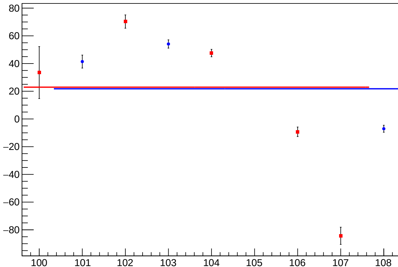
reg_asym_atl1r2_dd_atl2r1_dd_avg_diff_bpm1X_slope vs Slug, Sign Corrected
