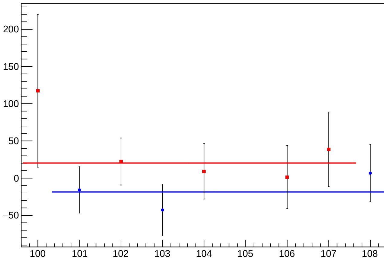
asym_bcm_dg_us_dg_ds_dd_mean vs Slug, Sign Corrected
