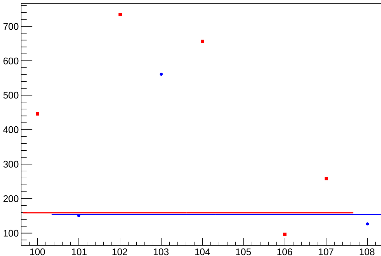
asym_atl_avg_eigen_dit_vs_cor_diff_rms vs Slug, Sign Corrected
