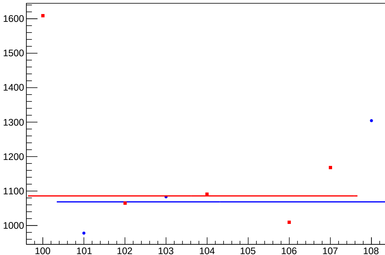
asym_sam_37_avg_eigen_cor_correction_rms vs Slug, Sign Corrected
