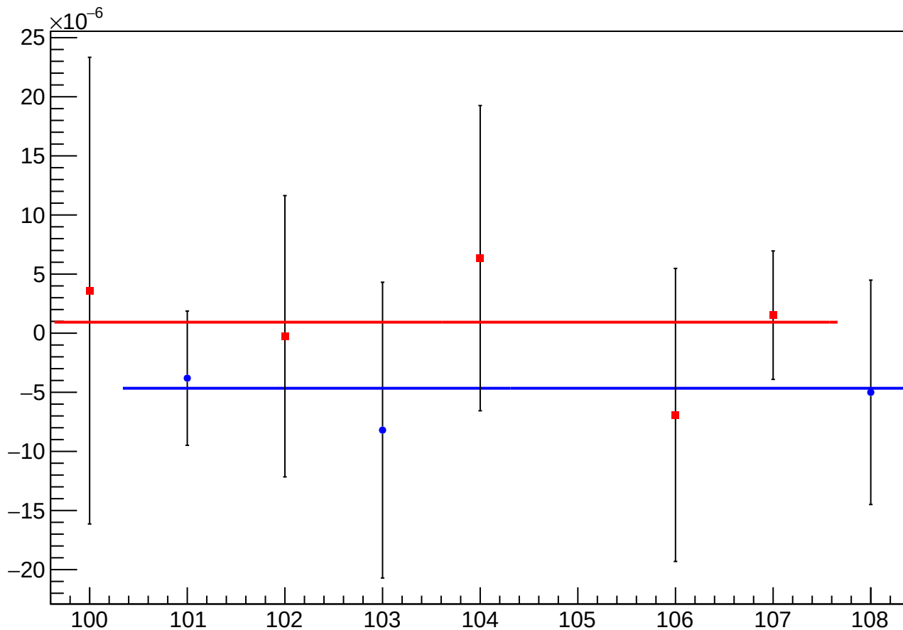
asym_sam_26_dd_eigen_dit_vs_dit_diff_mean vs Slug, Sign Corrected
