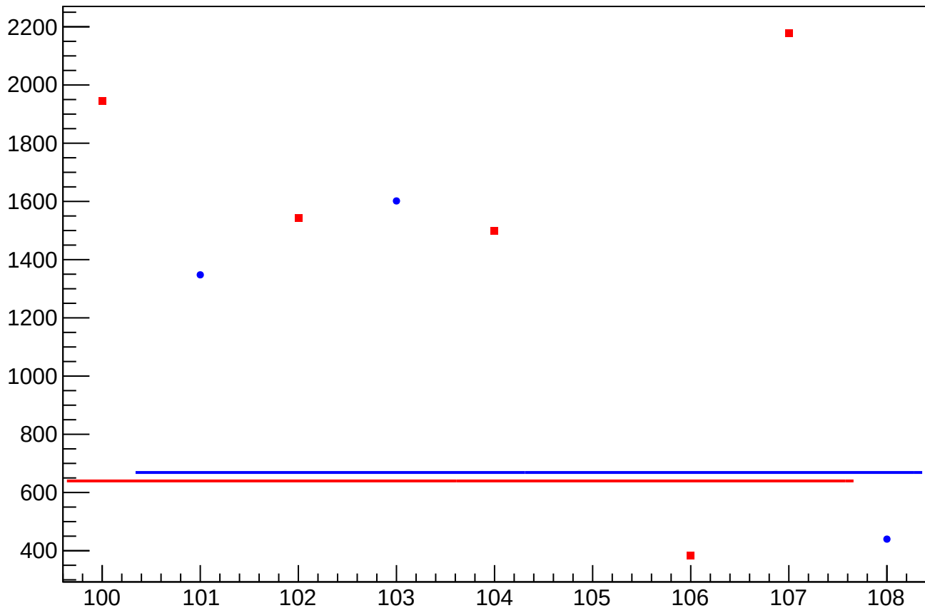
asym_atl_avg_atr_avg_dd_eigen_dit_correction_rms vs Slug, Sign Corrected
