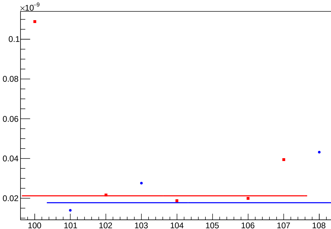
asym_sam7_reg_vs_cor_diff_rms vs Slug, Sign Corrected
