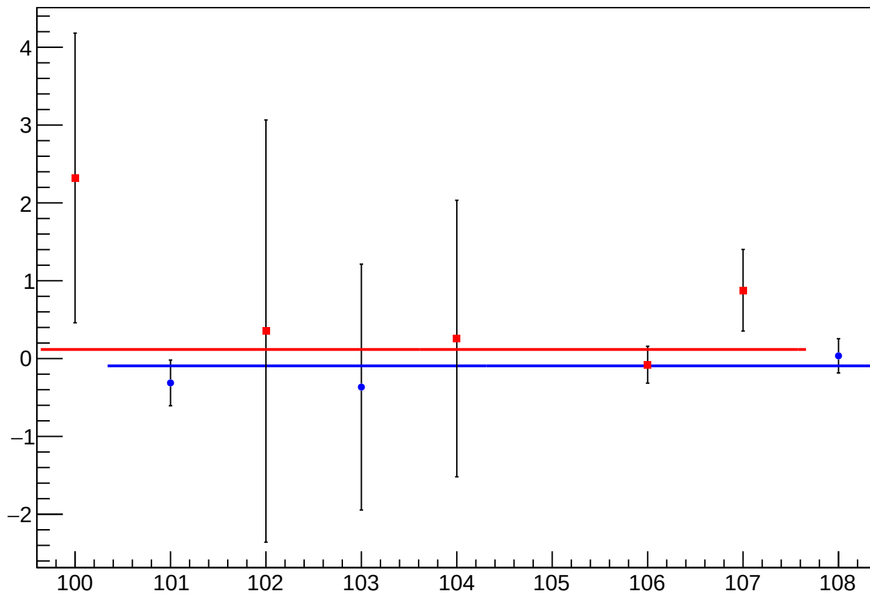
asym_atl1r2_avg_eigen_dit_vs_cor_diff_mean vs Slug, Sign Corrected
