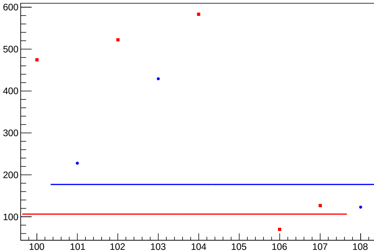
asym_atr1l2_avg_eigen_dit_vs_eigen_cor_diff_rms vs Slug, Sign Corrected
