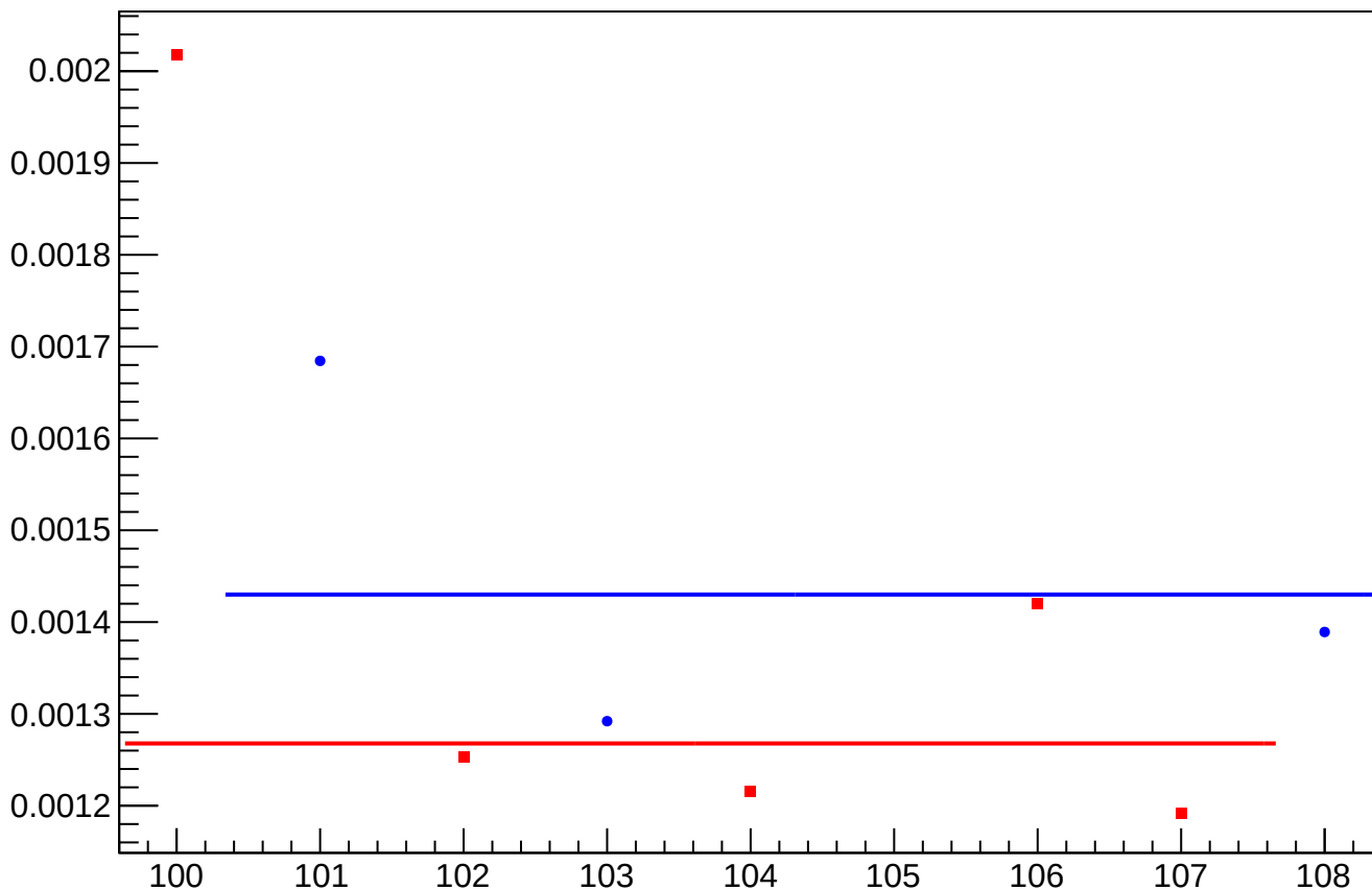
asym_sam5_eigen_dit_vs_dit_diff_rms vs Slug, Sign Corrected
