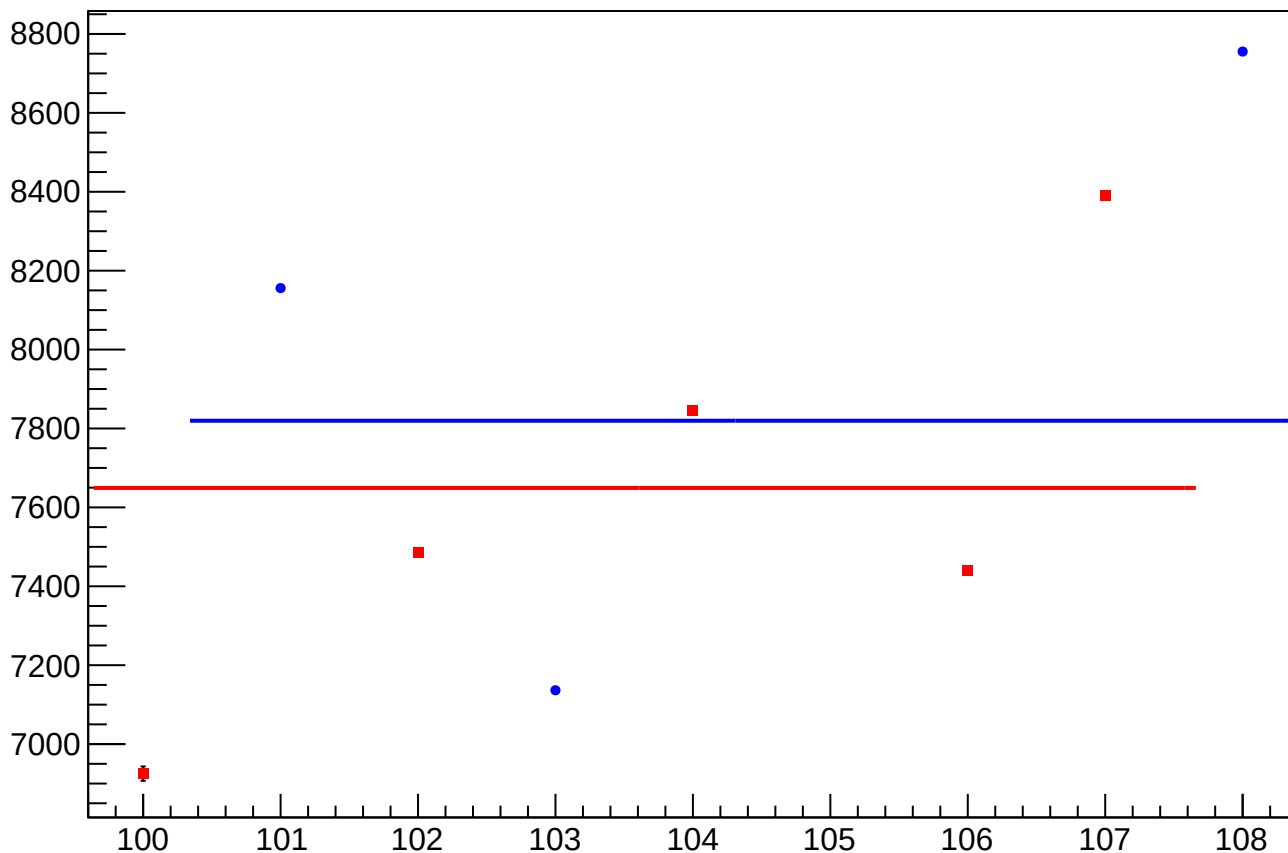
diff_bpm_4aY_4acY_avg_rms vs Slug, Sign Corrected
