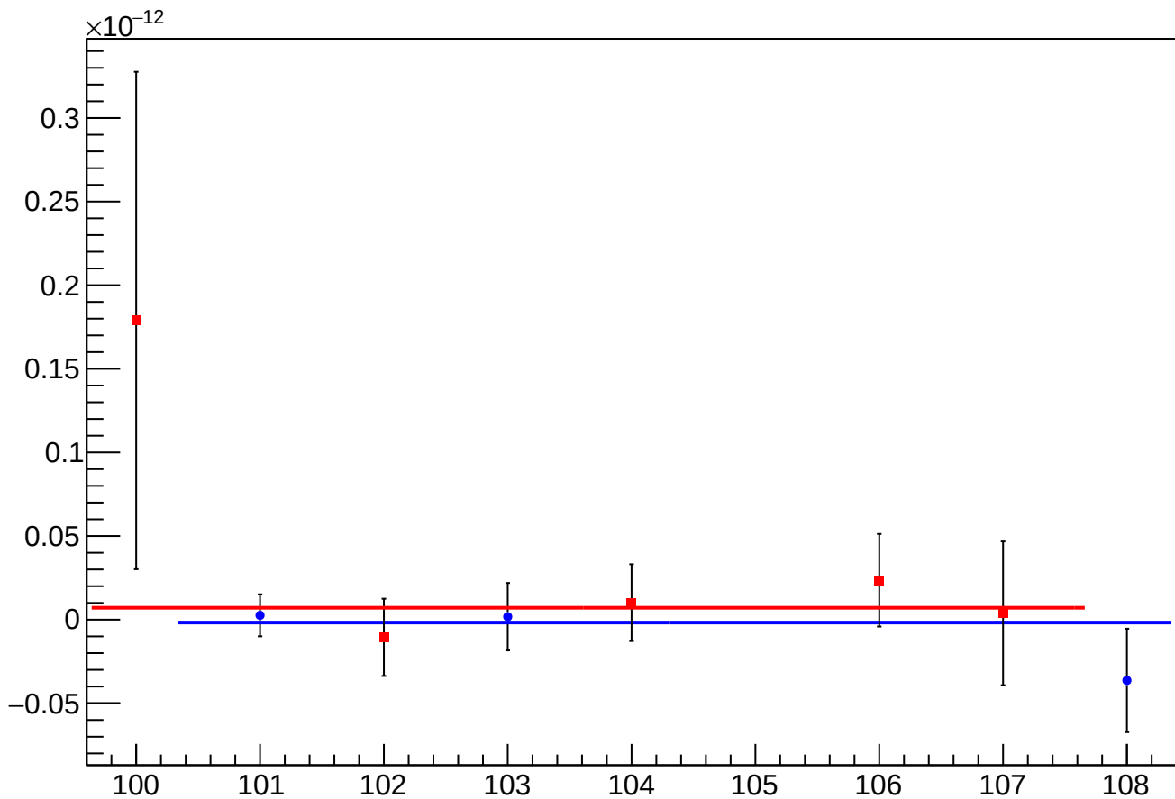
asym_sam6_eigen_cor_vs_cor_diff_mean vs Slug, Sign Corrected
