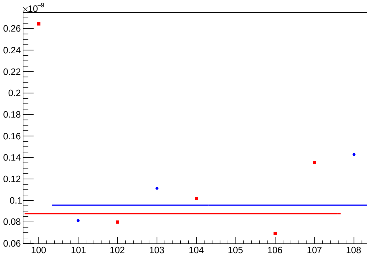
asym_sam4_reg_vs_cor_diff_rms vs Slug, Sign Corrected
