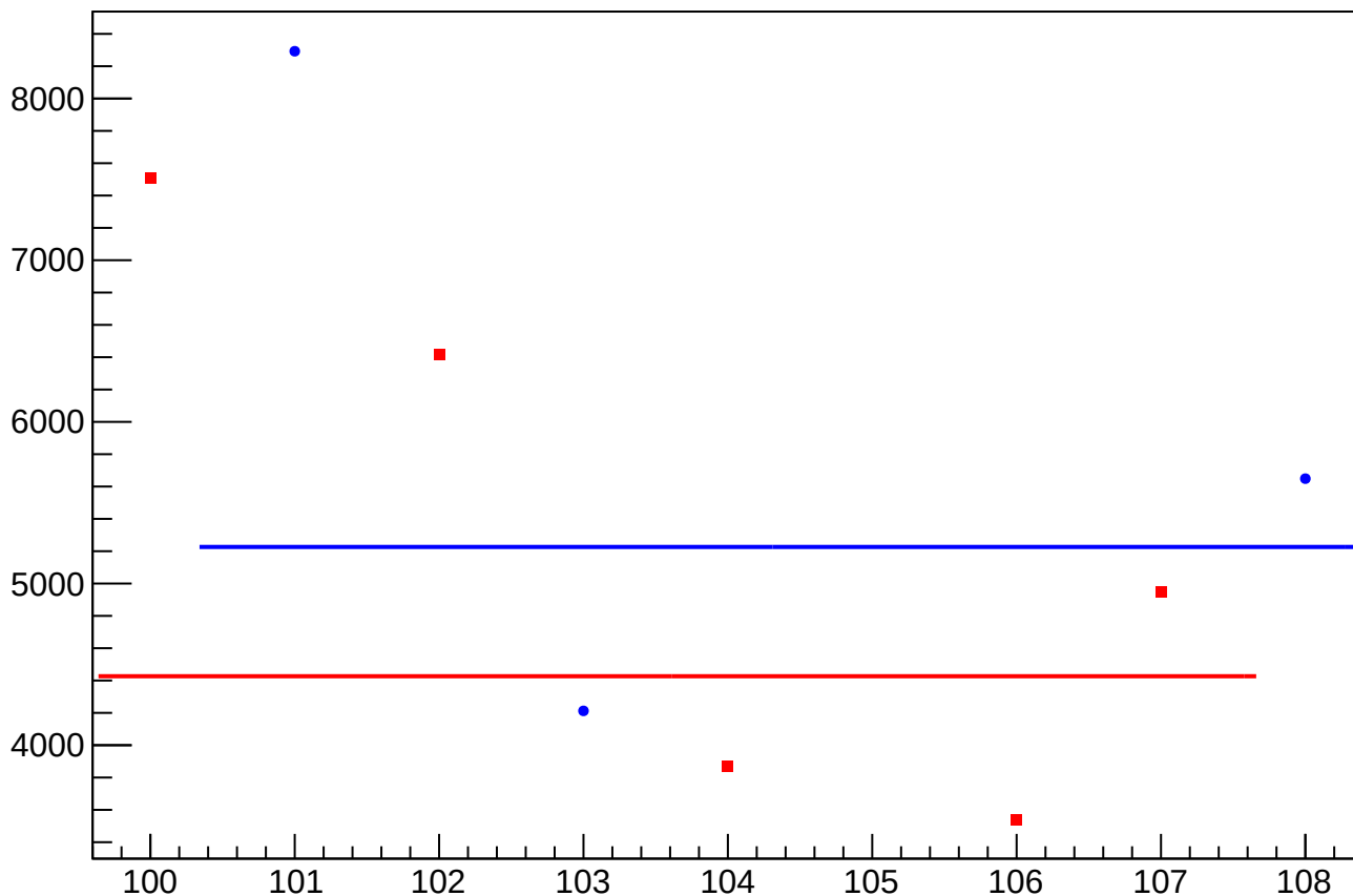
asym_us_avg_at2lr_avg_dd_cor_correction_rms vs Slug, Sign Corrected
