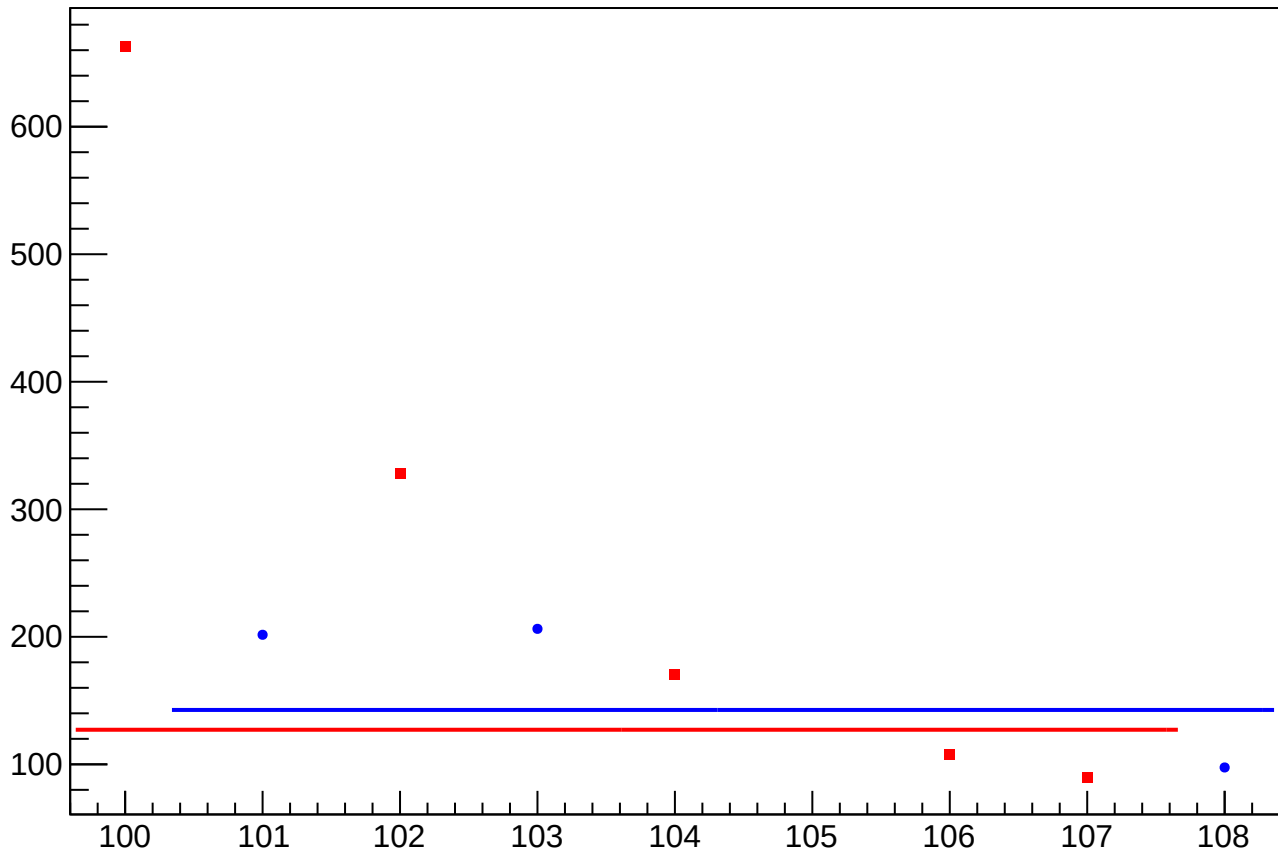
asym_atl_dd_atr_dd_avg_dit_vs_eigen_cor_diff_rms vs Slug, Sign Corrected
