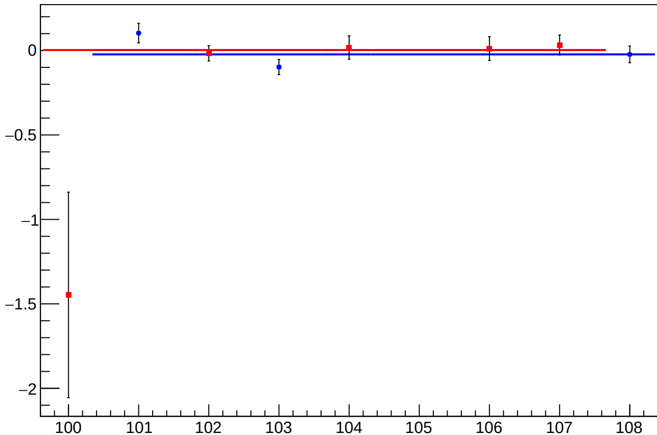
asym_sam_37_48_dd_dit_vs_cor_diff_mean vs Slug, Sign Corrected
