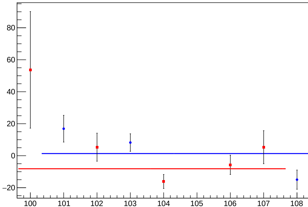
reg_asym_us_avg_at1lr_avg_avg_diff_bpm4eY_slope vs Slug, Sign Corrected
