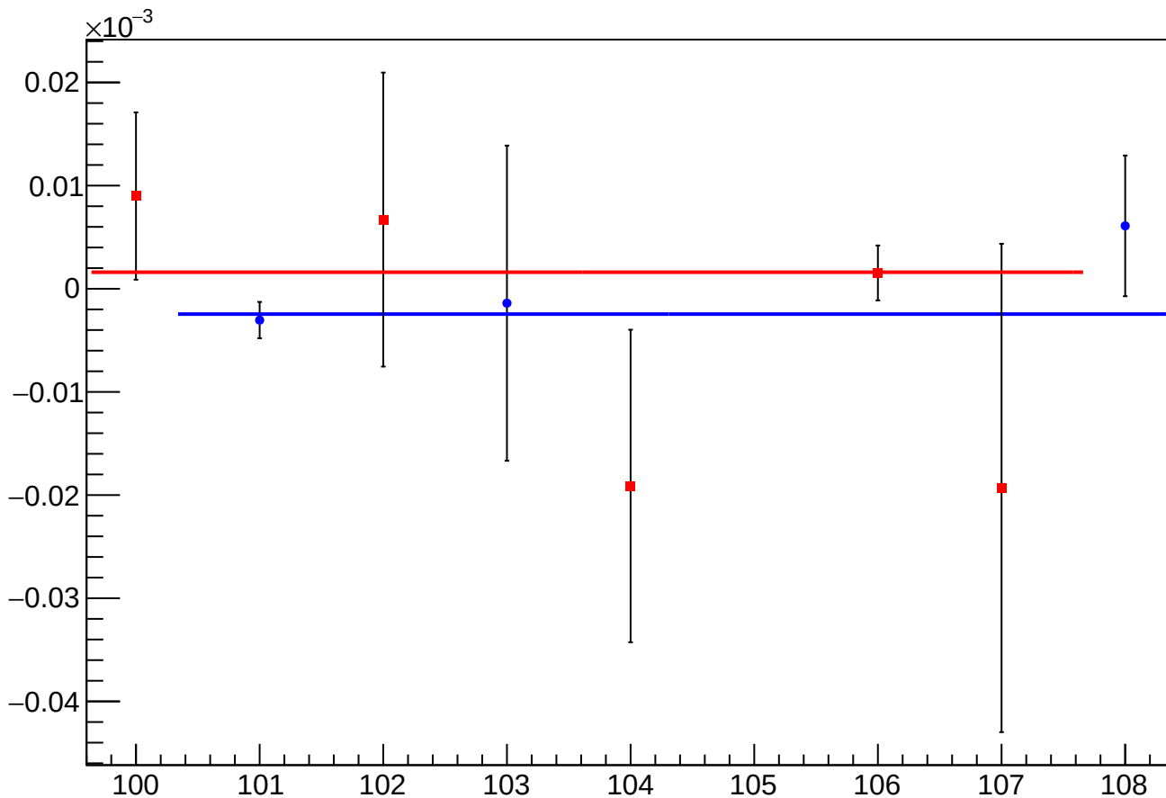
asym_usl_atl1_avg_eigen_dit_vs_dit_diff_mean vs Slug, Sign Corrected
