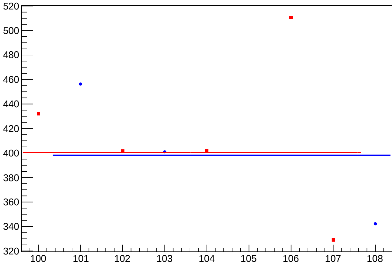
diff_bpm_4aX_4eX_dd_rms vs Slug, Sign Corrected
