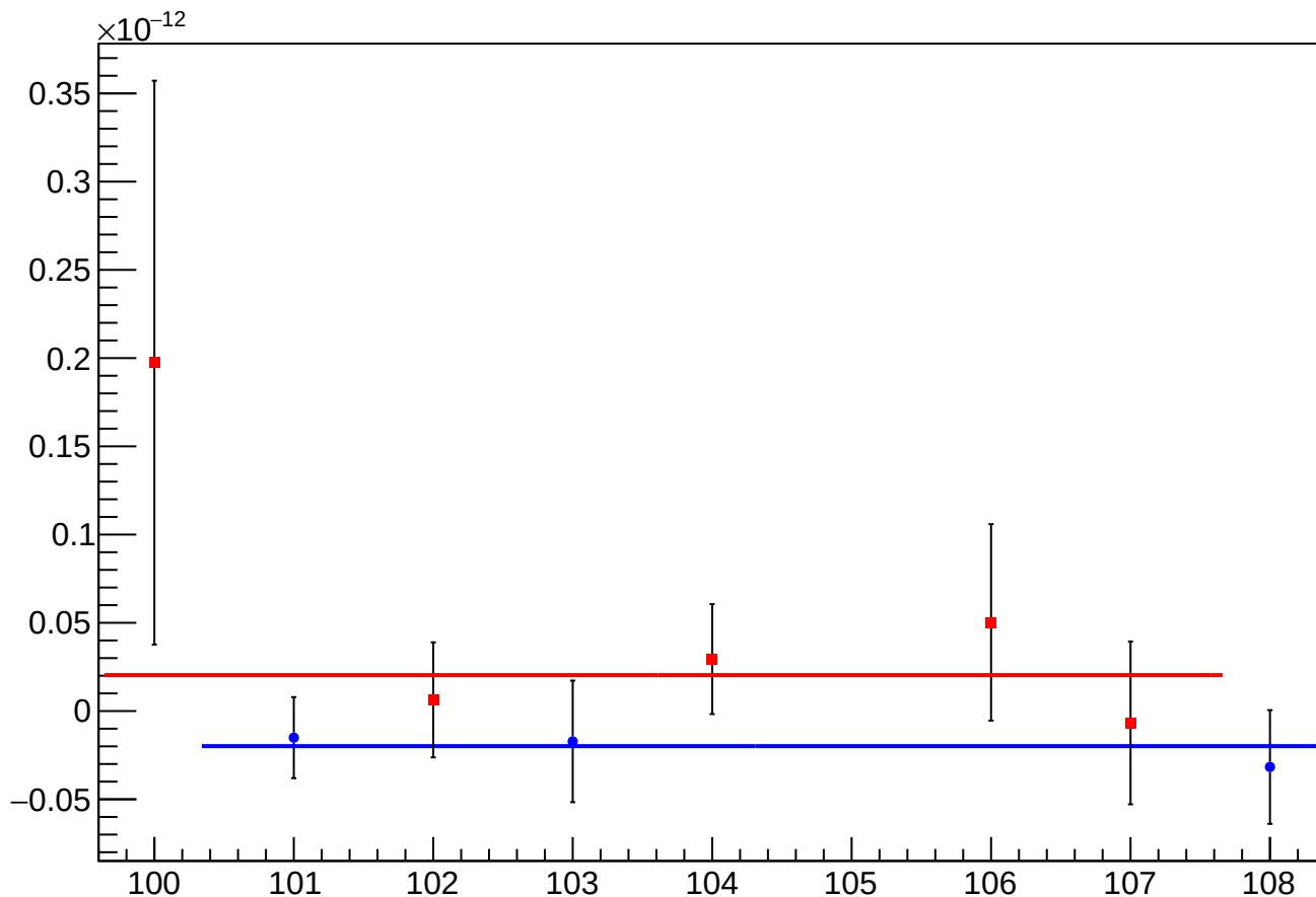
asym_sam_37_26_dd_eigen_cor_vs_cor_diff_mean vs Slug, Sign Corrected
