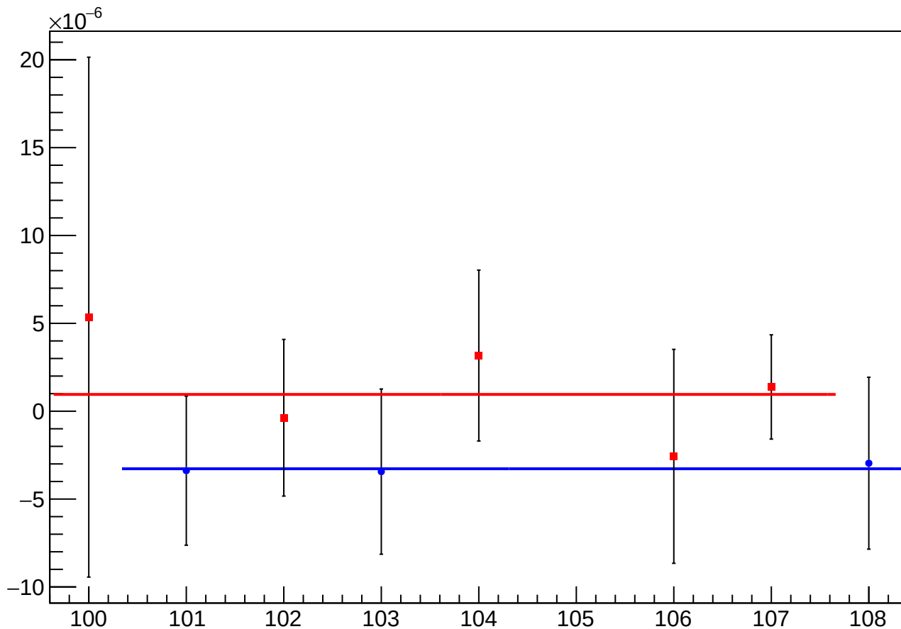
asym_sam_24_68_dd_eigen_dit_vs_dit_diff_mean vs Slug, Sign Corrected
