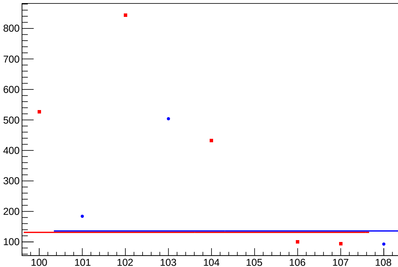
asym_atl_dd_eigen_dit_vs_eigen_cor_diff_rms vs Slug, Sign Corrected
