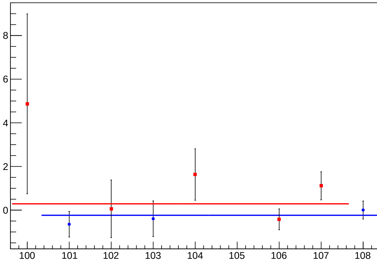
asym_us_avg_at2lr_avg_avg_eigen_dit_vs_eigen_cor_diff_mean vs Slug, Sign Corrected
