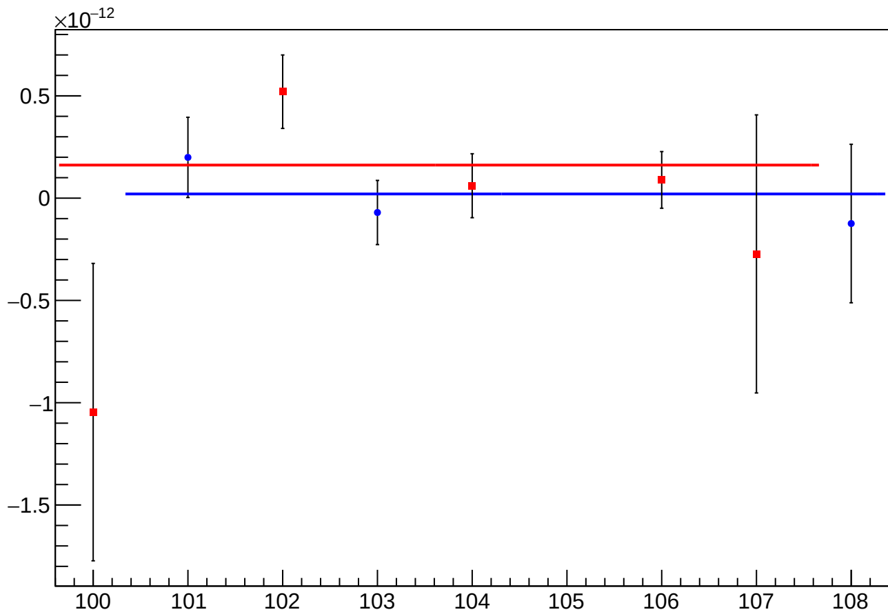
asym_usl_atl2_avg_reg_vs_cor_diff_mean vs Slug, Sign Corrected
