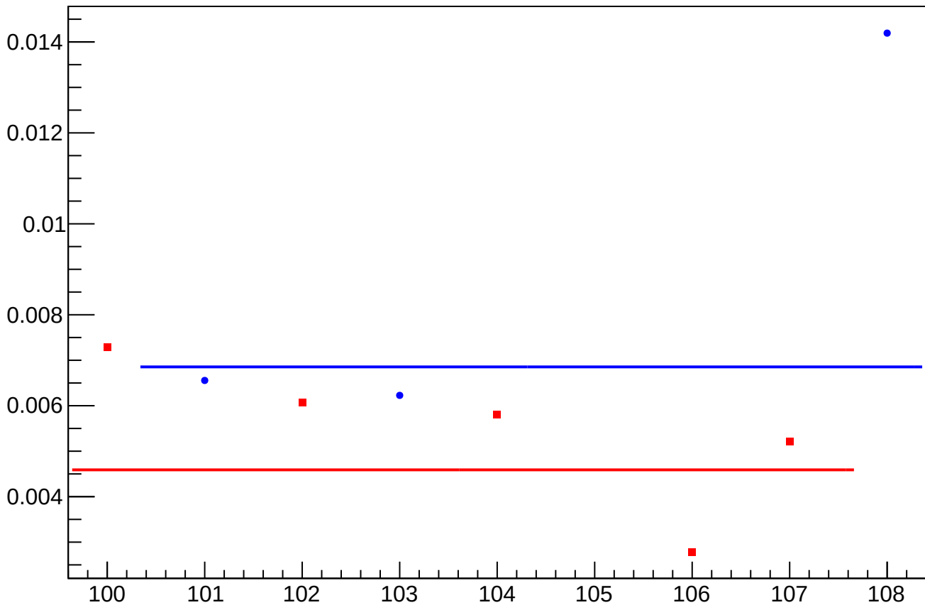
asym_atr1l2_dd_eigen_dit_vs_dit_diff_rms vs Slug, Sign Corrected
