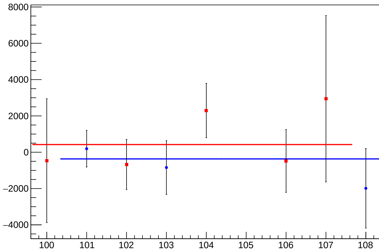
asym_us_avg_dit_correction_mean vs Slug, Sign Corrected
