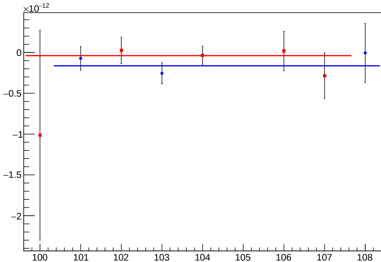
asym_usr_atr2_avg_eigen_cor_vs_cor_diff_mean vs Slug, Sign Corrected
