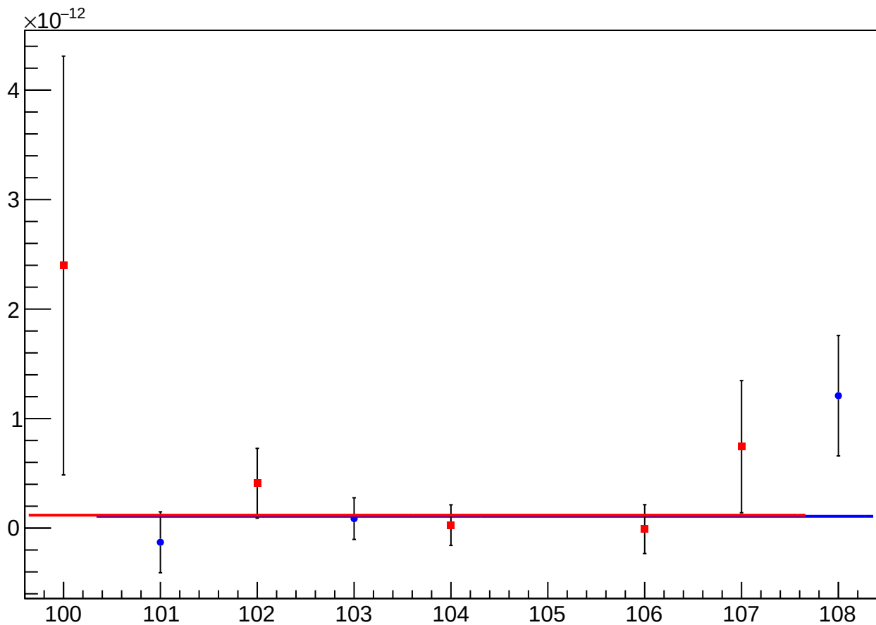
asym_us_avg_at2lr_avg_dd_reg_vs_cor_diff_mean vs Slug, Sign Corrected
