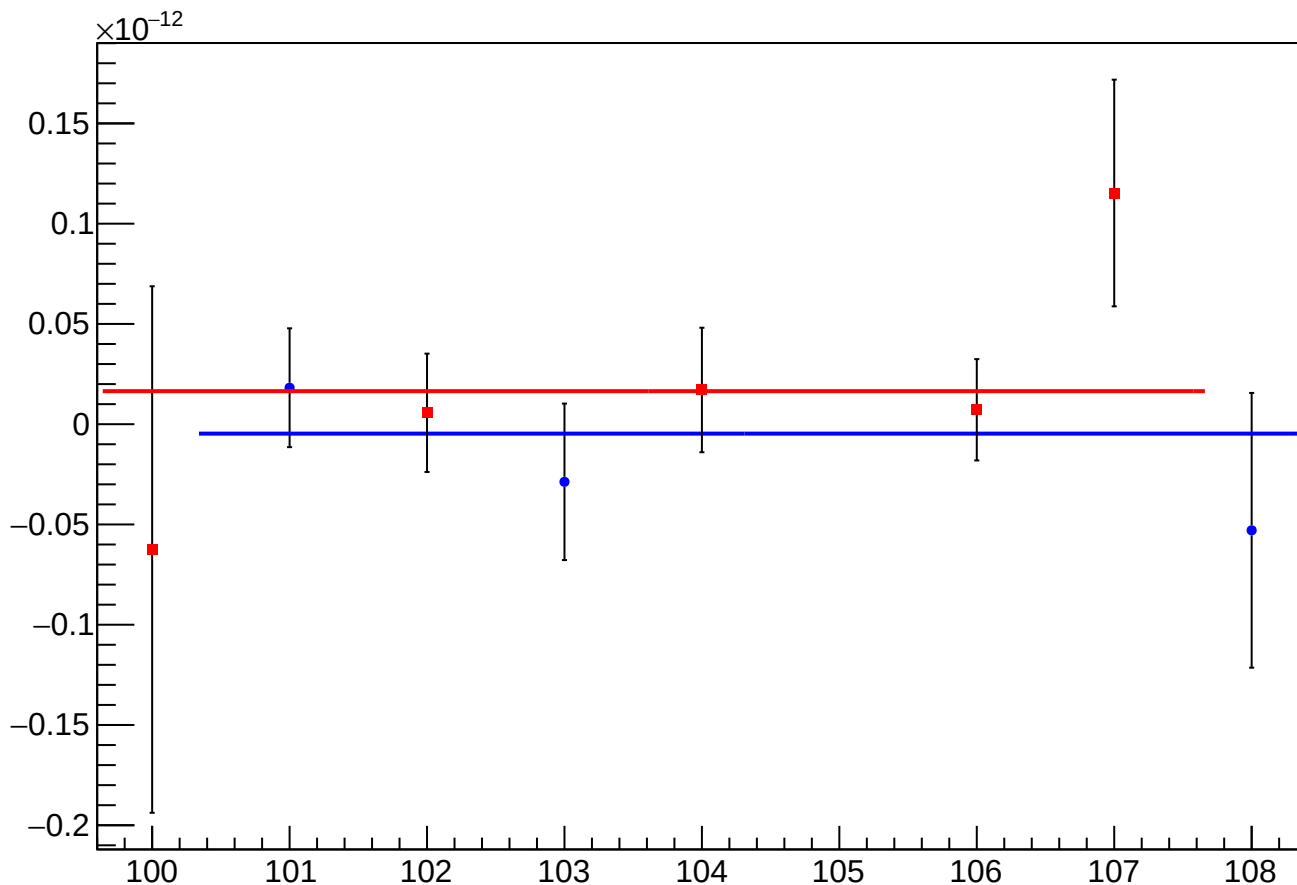
asym_sam5_reg_vs_cor_diff_mean vs Slug, Sign Corrected
