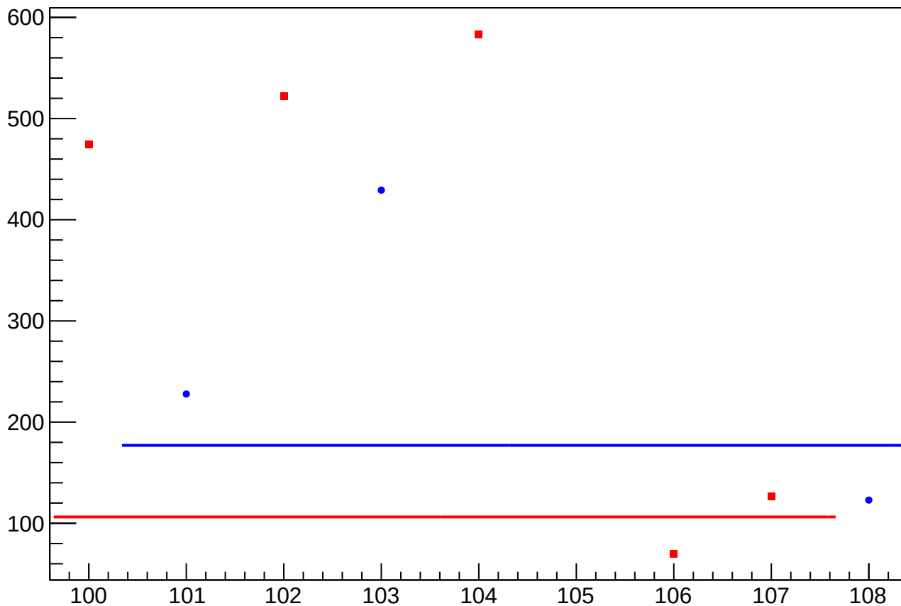
asym_atr1l2_avg_dit_vs_cor_diff_rms vs Slug, Sign Corrected
