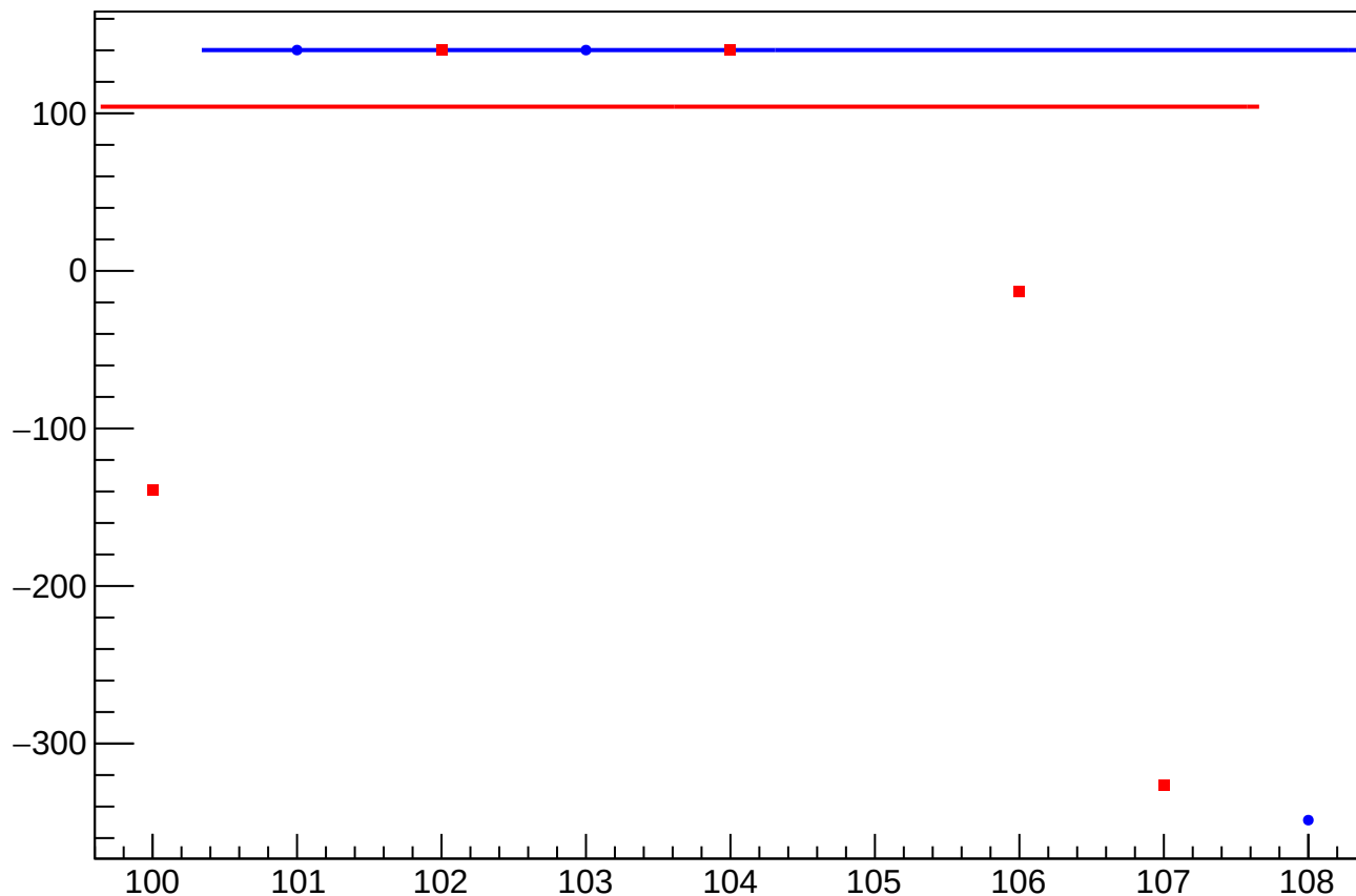
yield_cav4bY_mean vs Slug, Sign Corrected
