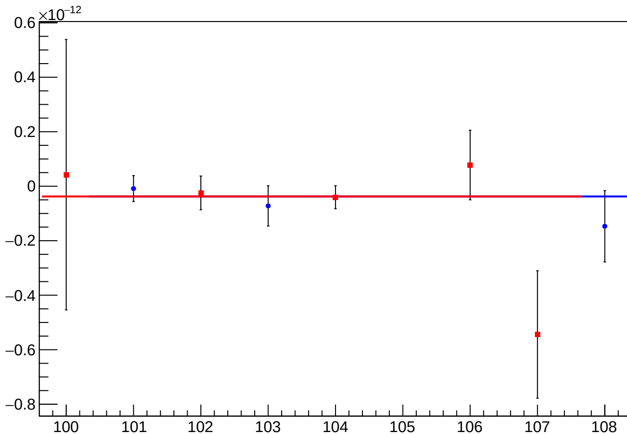
asym_usr_atr1_dd_reg_vs_slug_corr_diff_mean vs Slug, Sign Corrected
