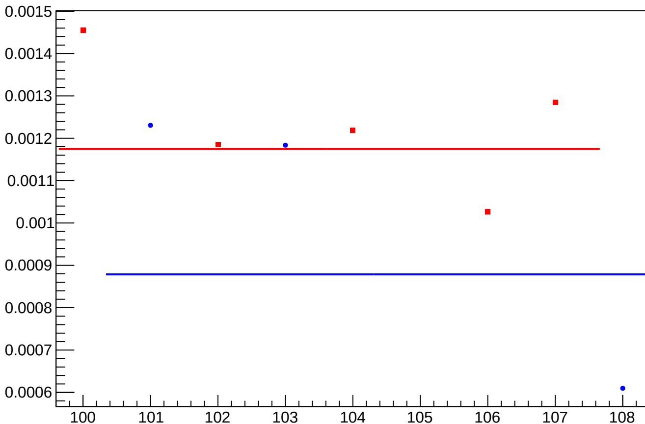
asym_sam1_eigen_dit_vs_dit_diff_rms vs Slug, Sign Corrected
