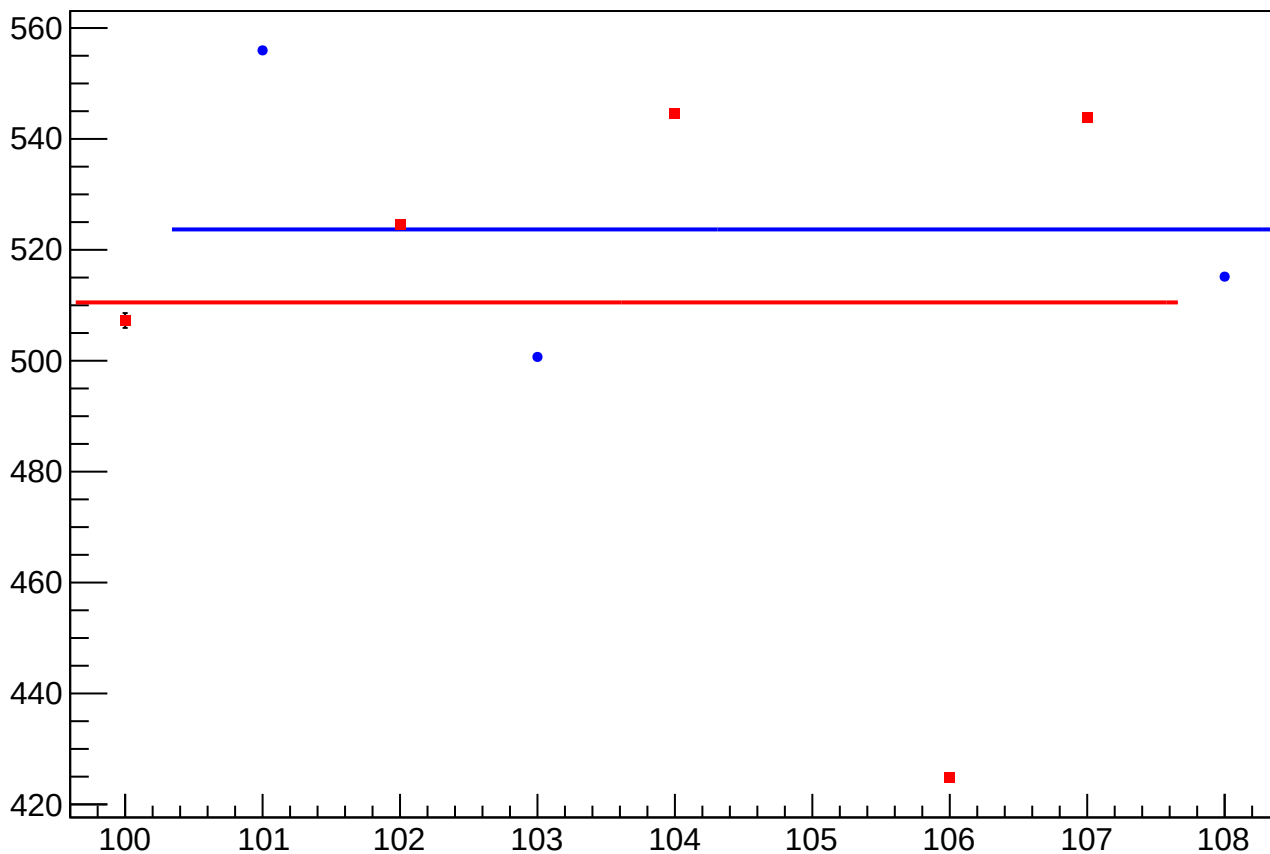
asym_sam5_eigen_cor_correction_rms vs Slug, Sign Corrected
