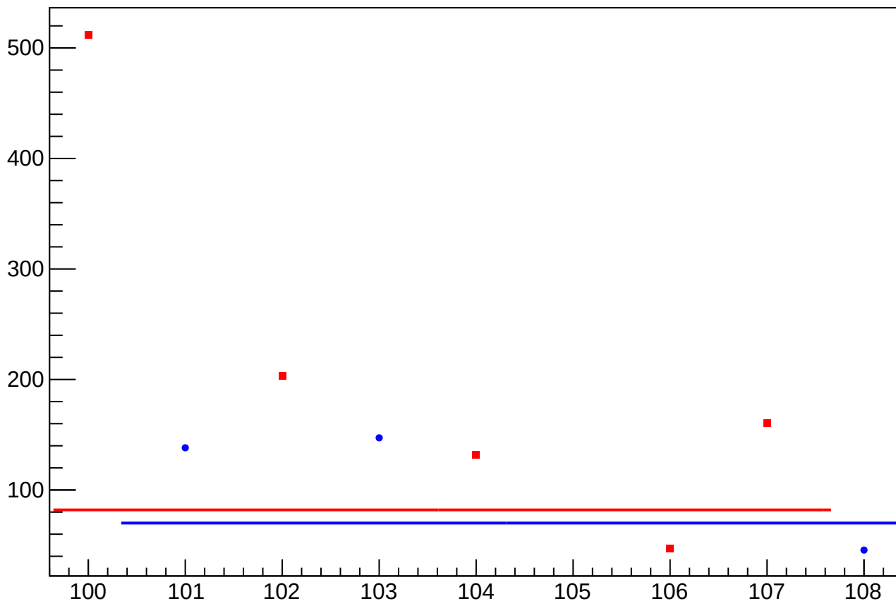
asym_at1_dd_eigen_dit_vs_eigen_cor_diff_rms vs Slug, Sign Corrected
