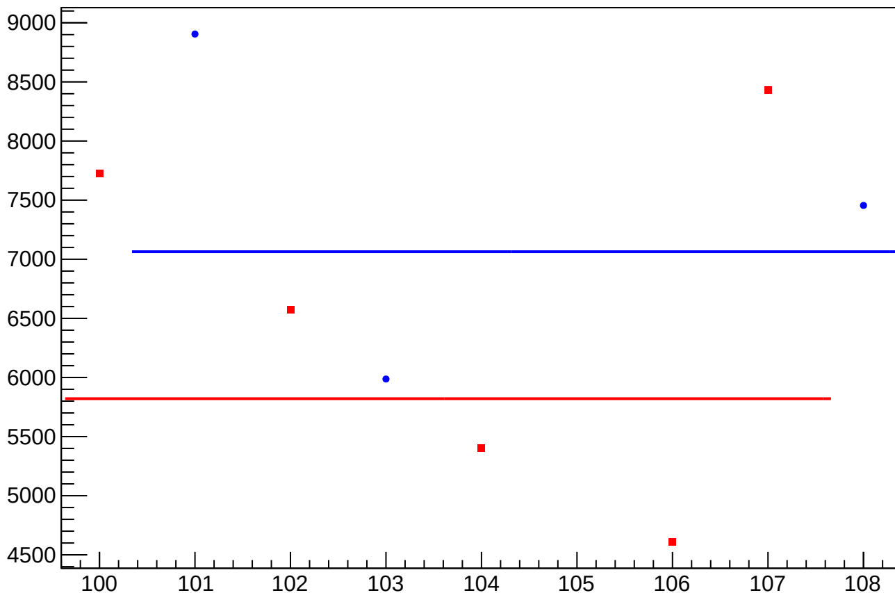
asym_atl2_reg_correction_rms vs Slug, Sign Corrected
