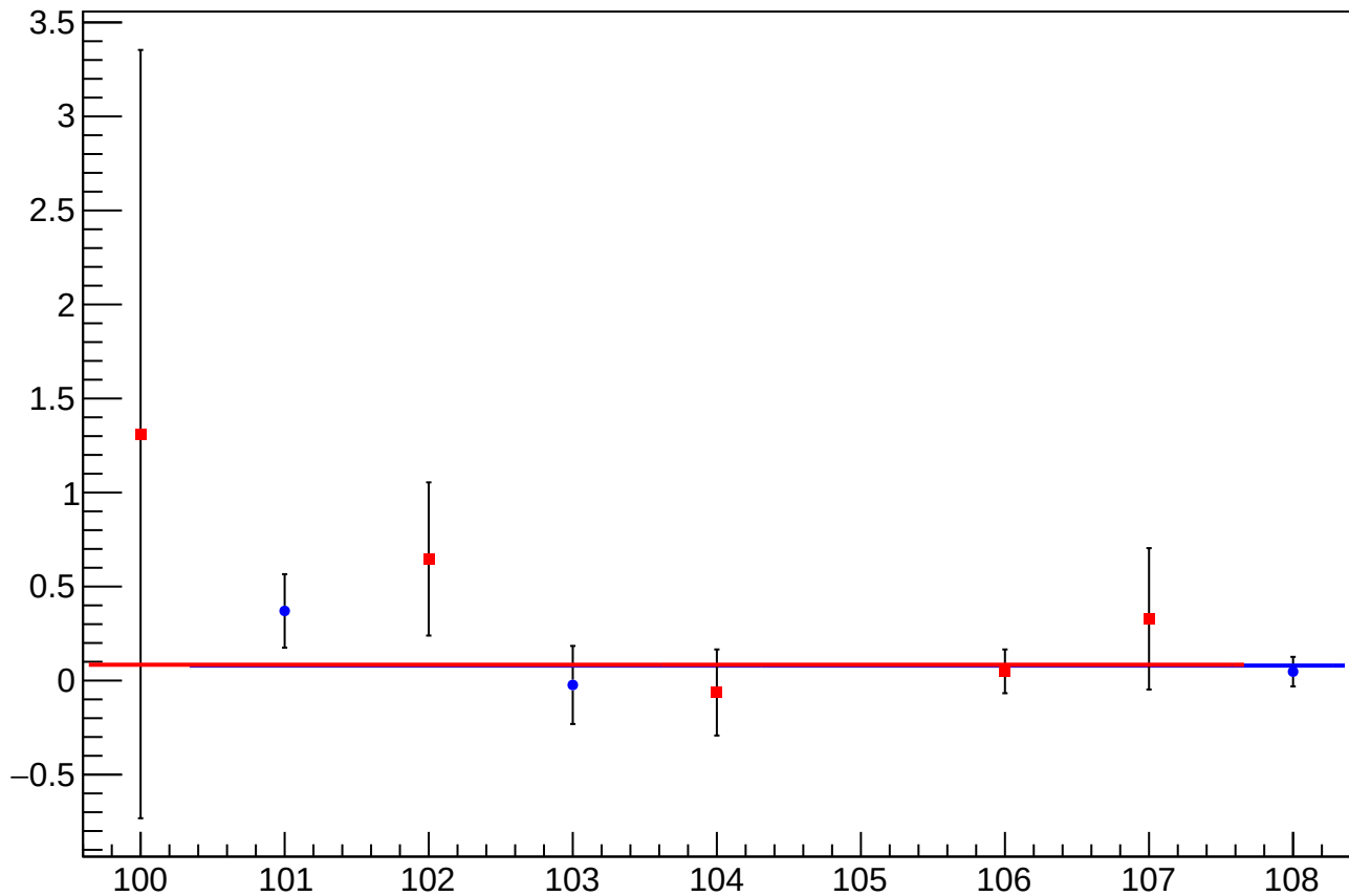
asym_us_dd_at1lr_dd_avg_dit_vs_cor_diff_mean vs Slug, Sign Corrected
