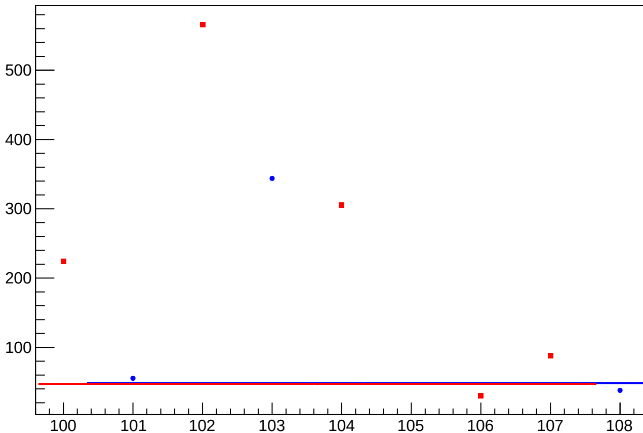
asym_at1_dd_at2_dd_avg_dit_vs_slug_Sign_Corrected
