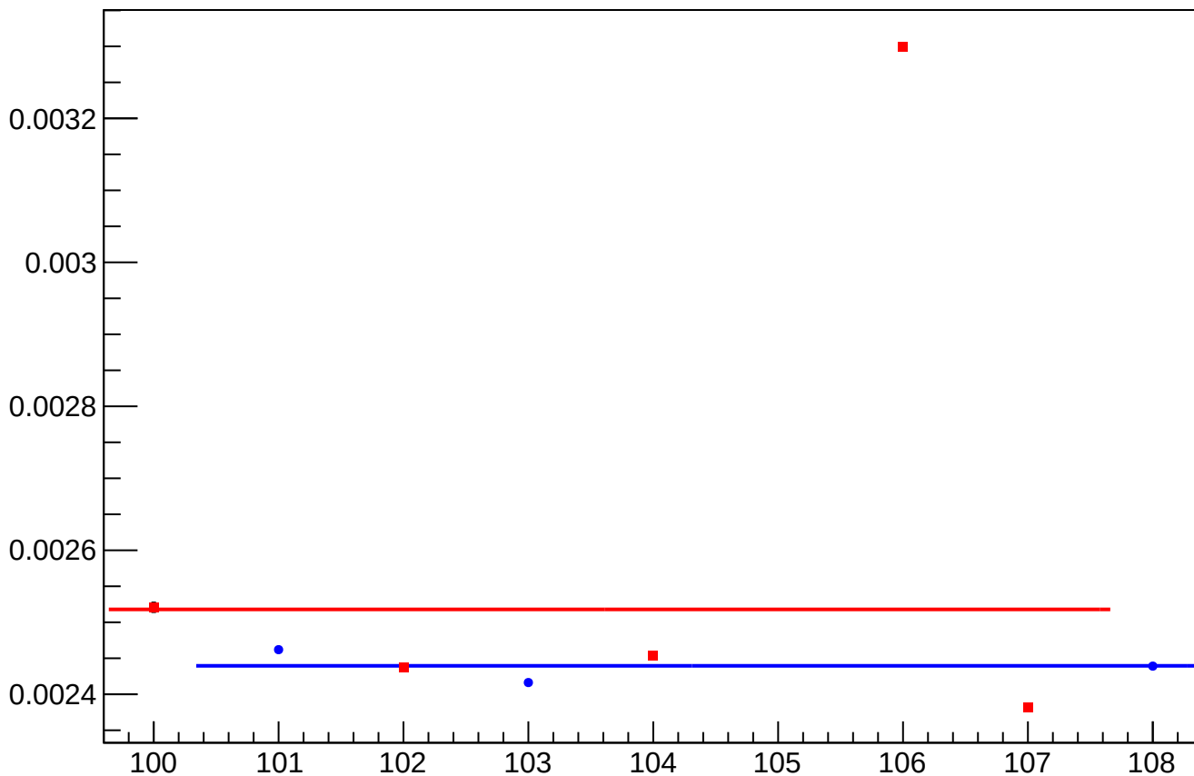
yield_bpm0l06Y_rms vs Slug, Sign Corrected
