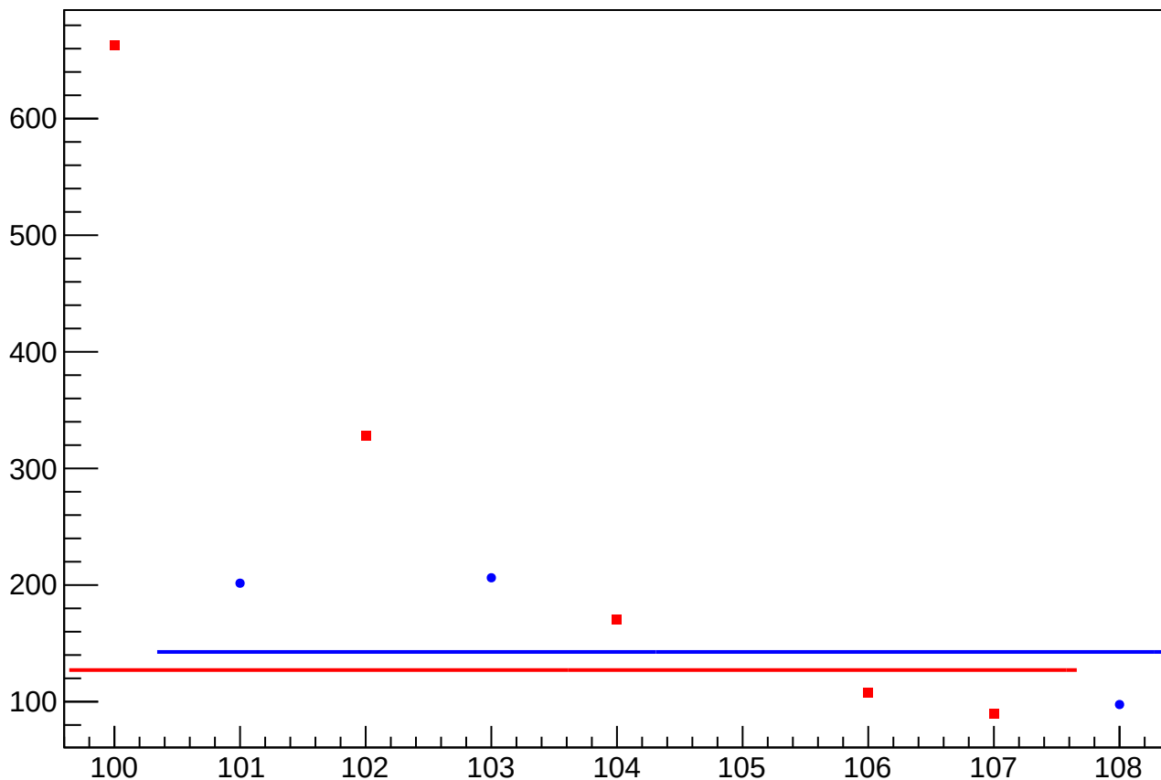
asym_at1_avg_at2_avg_dd_dit_vs_cor_diff_rms vs Slug, Sign Corrected
