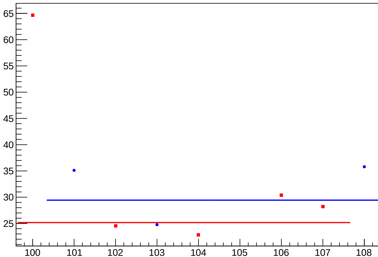
asym_sam_1548_avg_dit_vs_eigen_cor_diff_rms vs Slug, Sign Corrected
