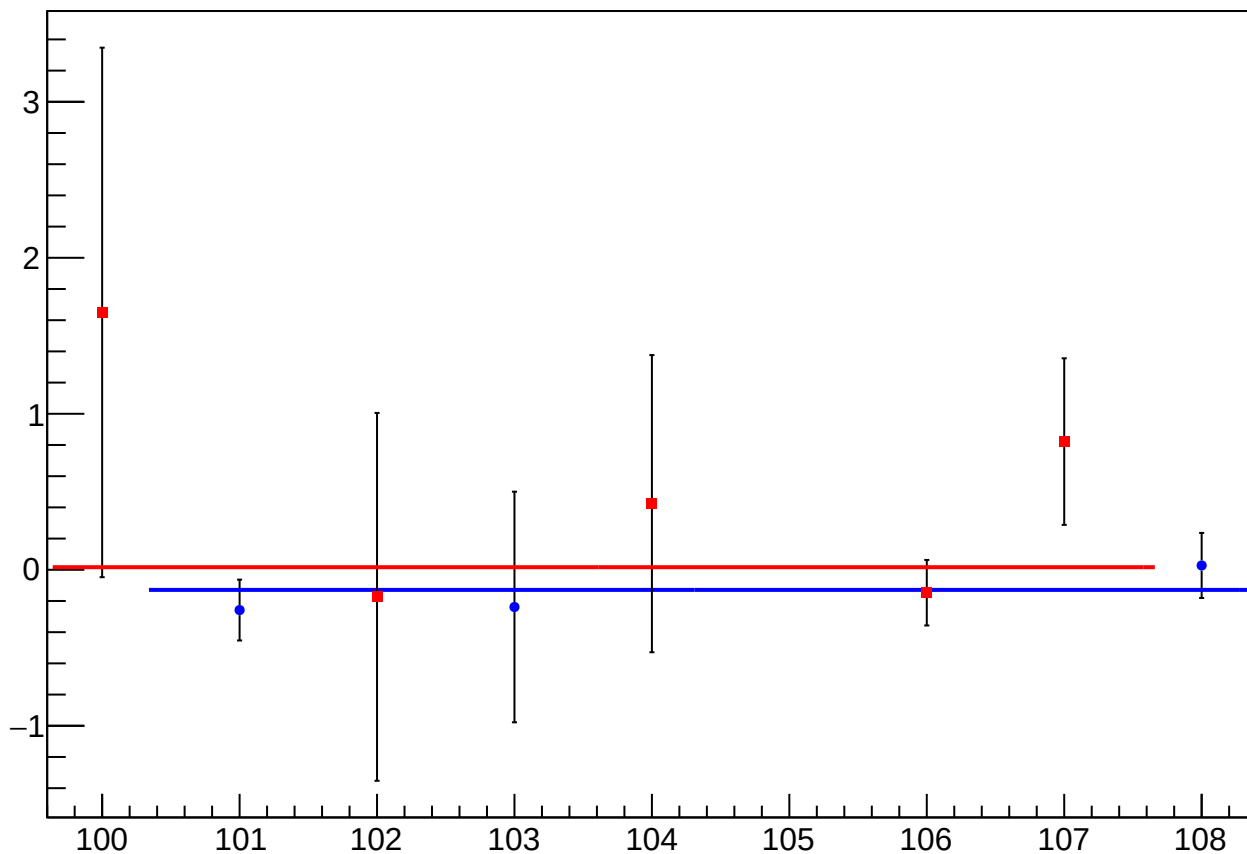
asym_atl_avg_dit_vs_cor_diff_mean vs Slug, Sign Corrected
