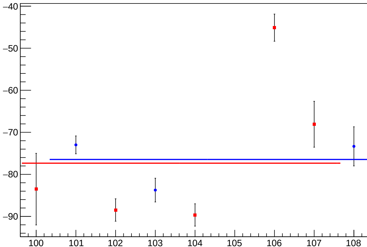
reg_asym_sam4_diff_bpm4eX_slope vs Slug, Sign Corrected
