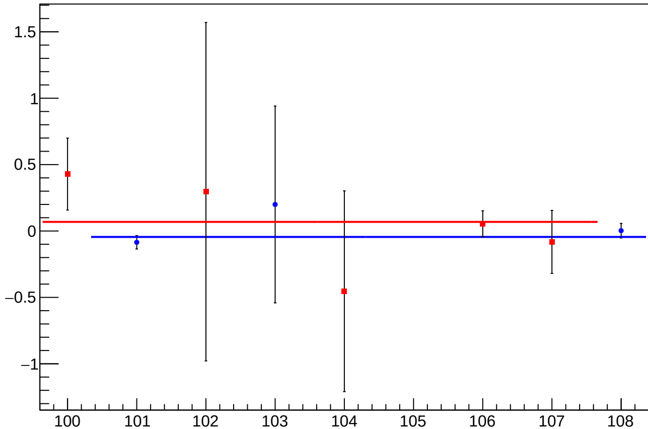
asym_usl_atl1_dd_dit_vs_eigen_cor_diff_mean vs Slug, Sign Corrected
