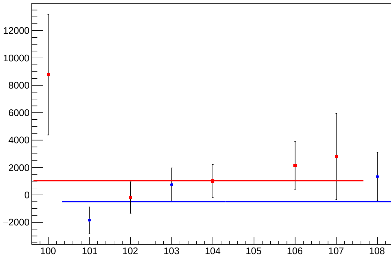
asym_us_dd_eigen_dit_correction_mean vs Slug, Sign Corrected
