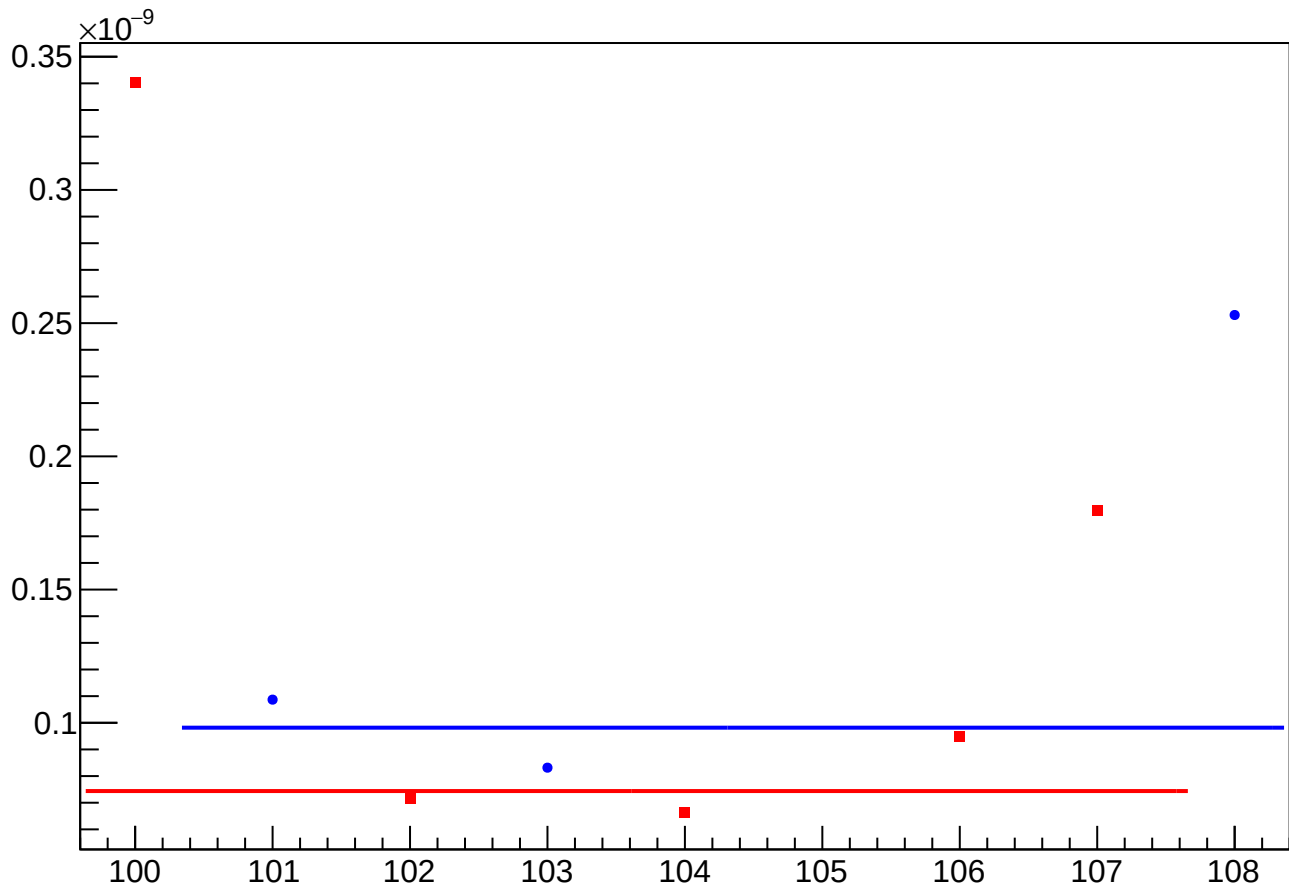
asym_us_avg_atlr_avg_avg_reg_vs_cor_diff_rms vs Slug, Sign Corrected
