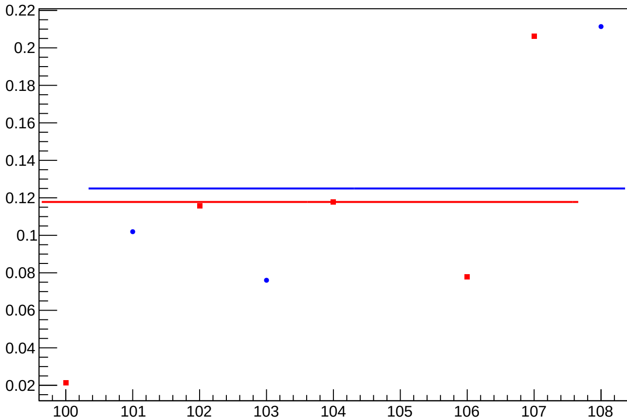
yield_bpm2i01X_mean vs Slug, Sign Corrected
