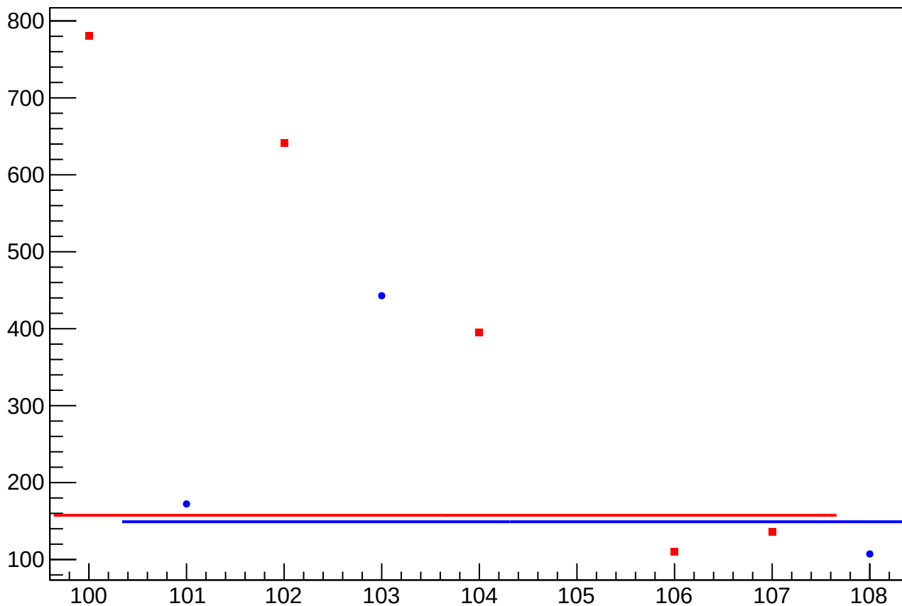
asym_atr1l2_dd_eigen_dit_vs_cor_diff_rms vs Slug, Sign Corrected
