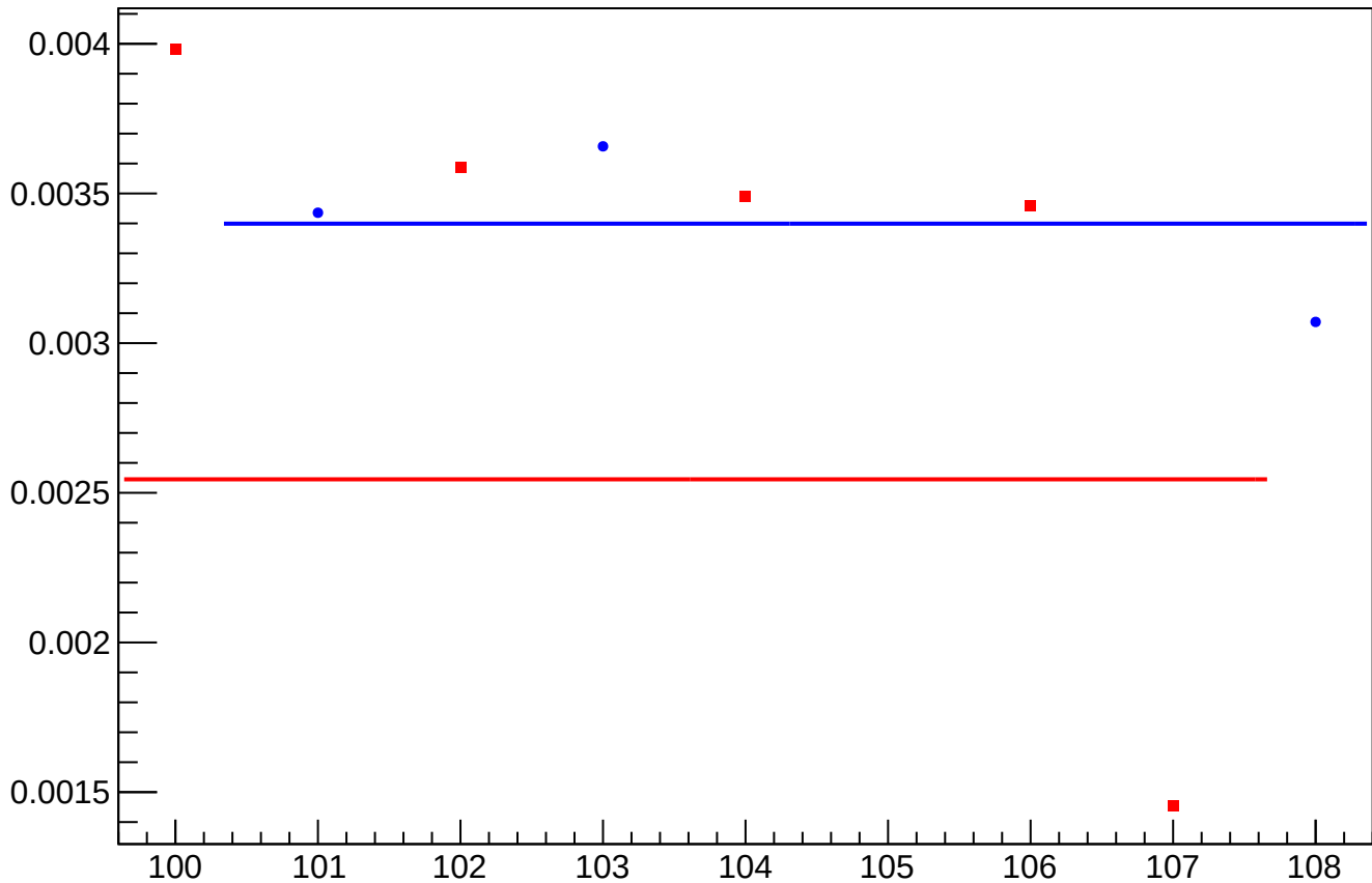
asym_sam_24_68_dd_eigen_dit_vs_dit_diff_rms vs Slug, Sign Corrected
