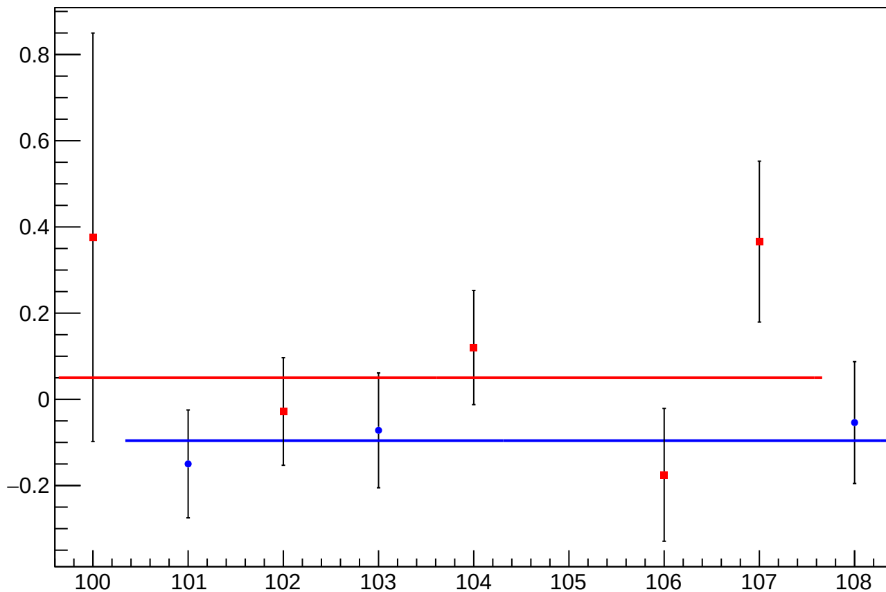
asym_usr_eigen_dit_vs_overload_cor_diff_mean vs Slug, Sign Corrected
