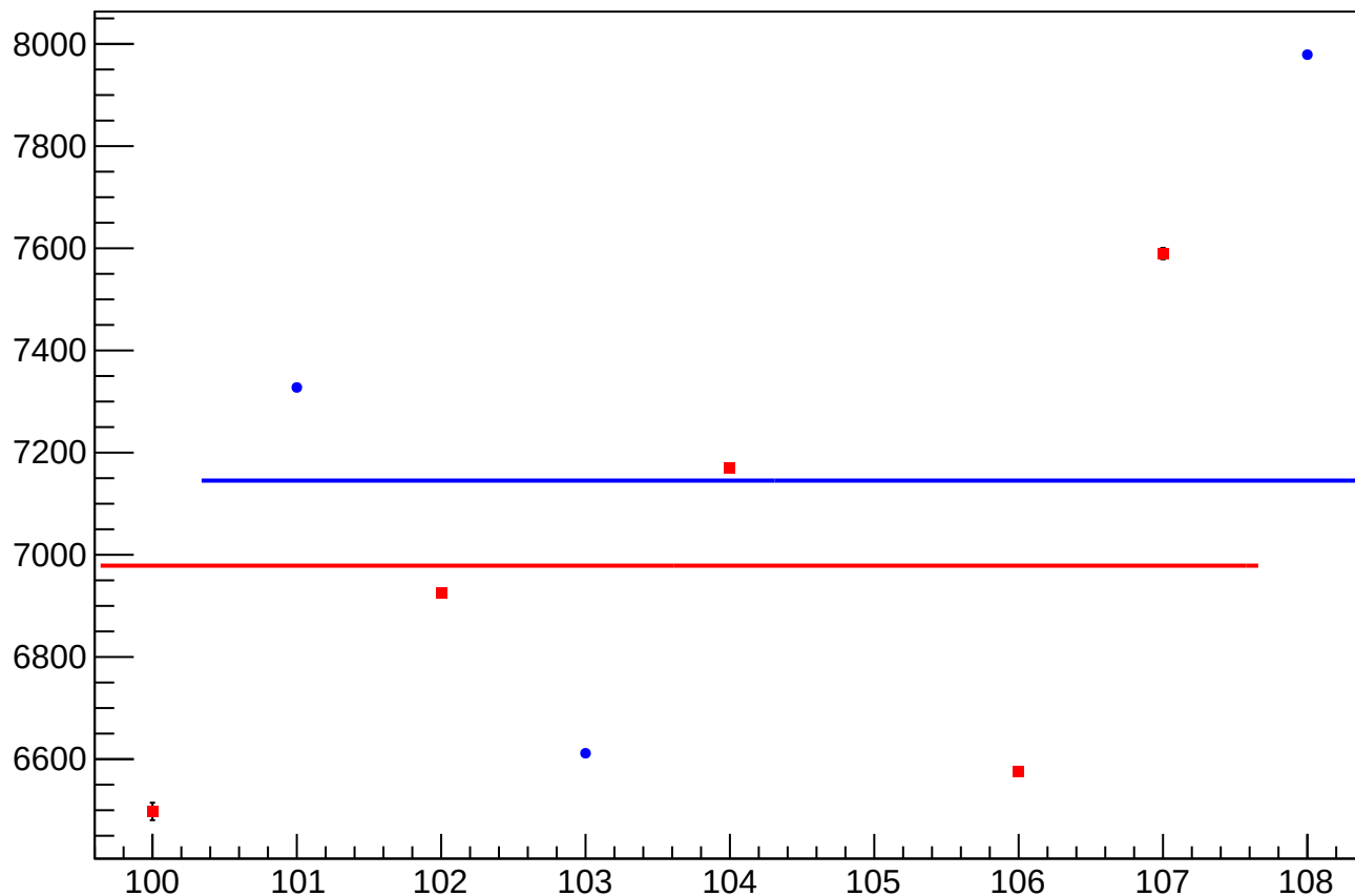
diff_bpm_4aY_4eY_avg_rms vs Slug, Sign Corrected
