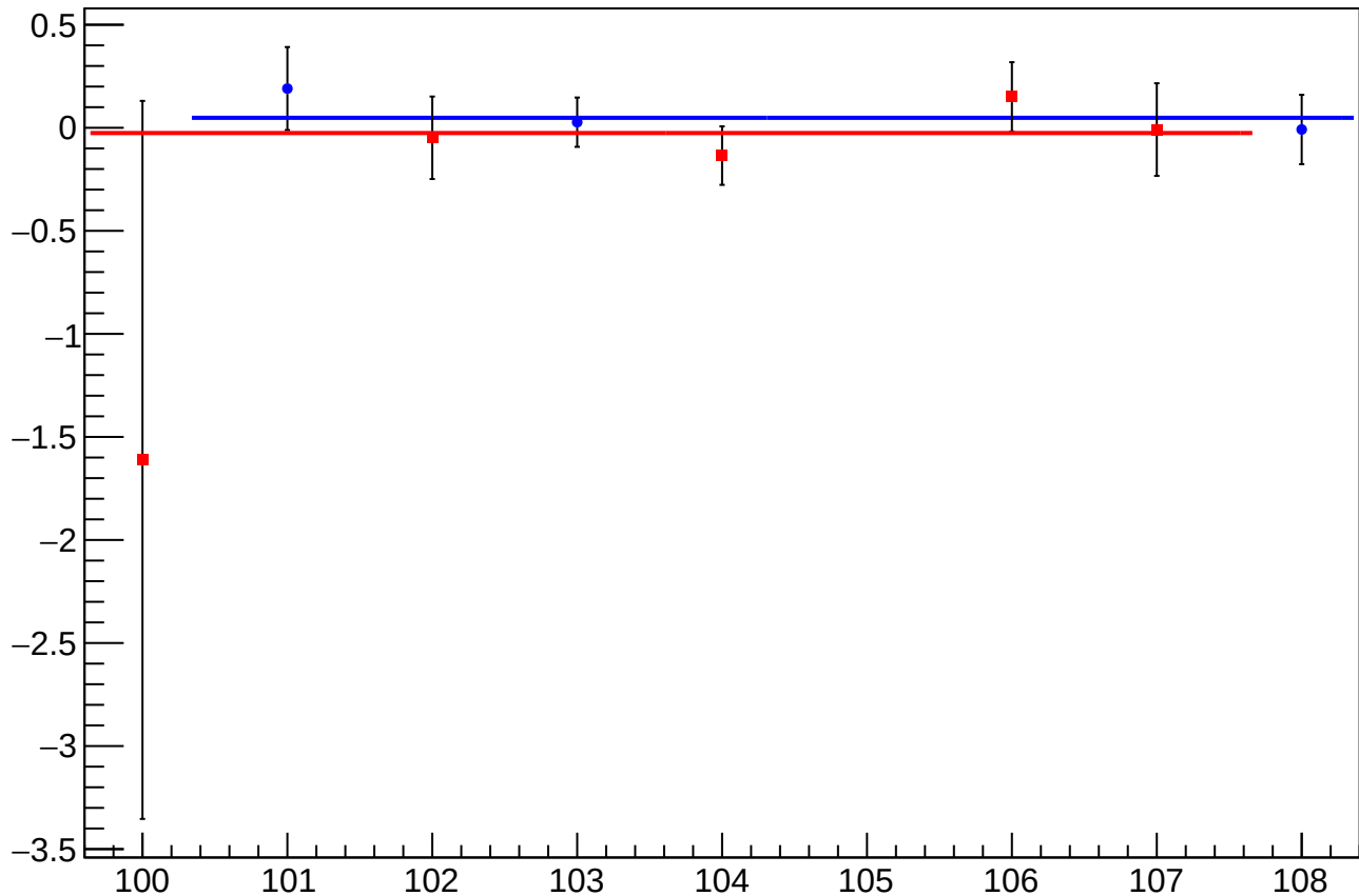
asym_usl_atl2_dd_dit_vs_eigen_cor_diff_mean vs Slug, Sign Corrected
