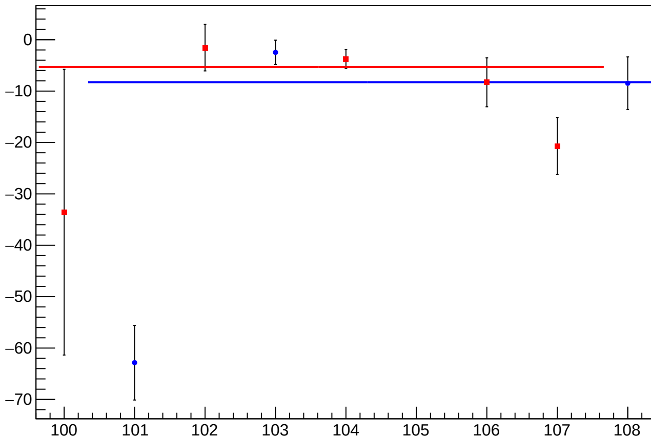
reg_asym_us_avg_atlr_avg_dd_diff_bpm4eY_slope vs Slug, Sign Corrected
