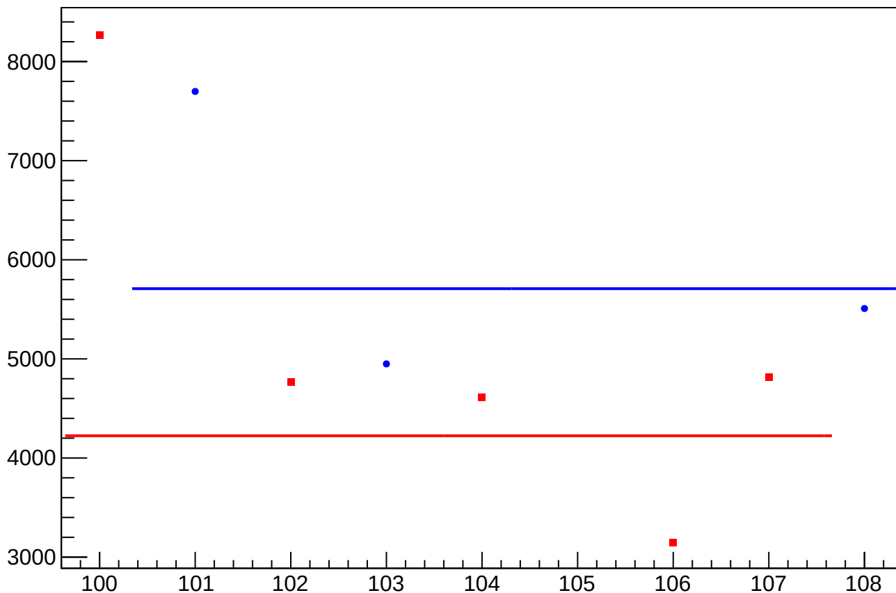
asym_us_avg_at2lr_avg_dd_eigen_dit_correction_rms vs Slug, Sign Corrected
