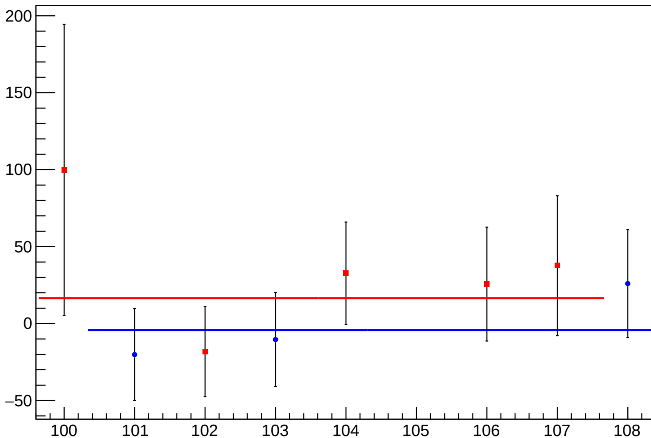
asym_bcm_dg_us_an_us_dd_mean vs Slug, Sign Corrected
