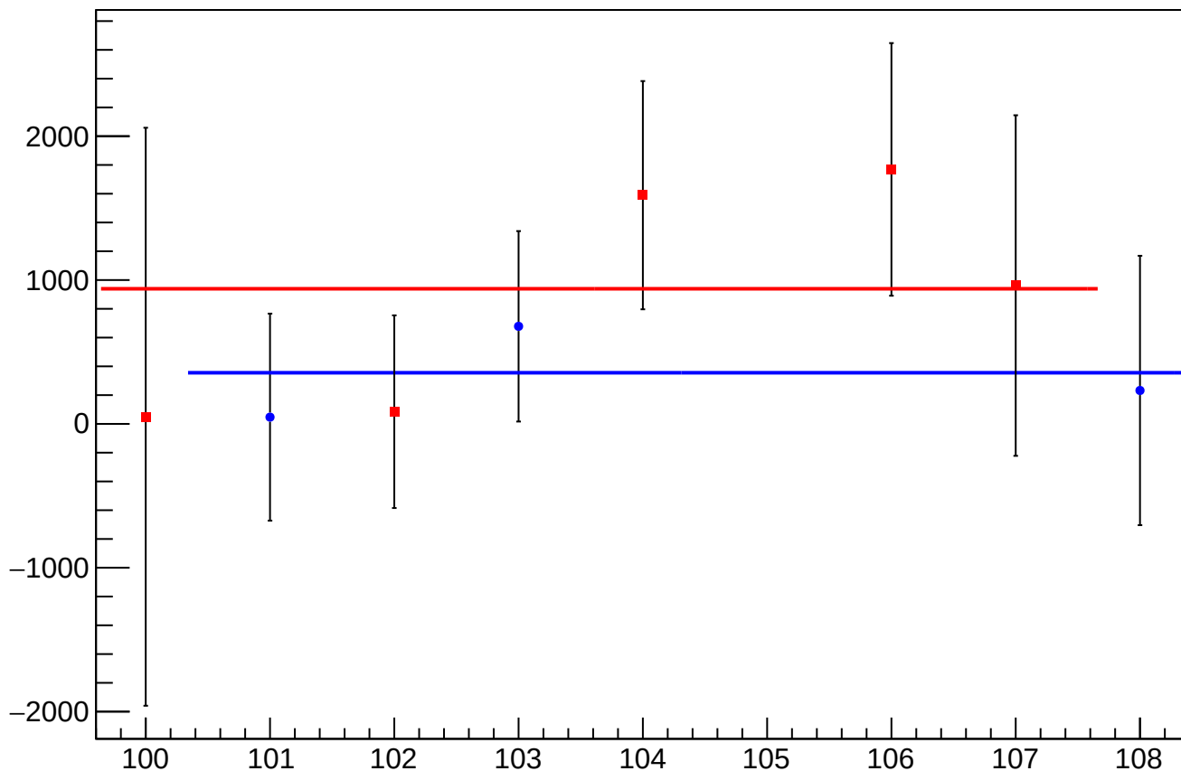
asym_sam5_eigen_dit_correction_mean vs Slug, Sign Corrected
