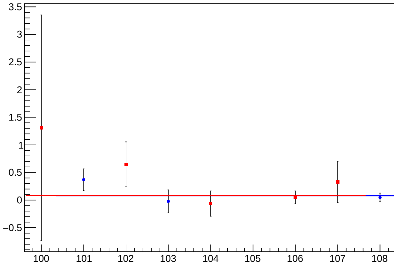
asym_us_dd_at1lr_dd_avg_dit_vs_eigen_cor_diff_mean vs Slug, Sign Corrected
