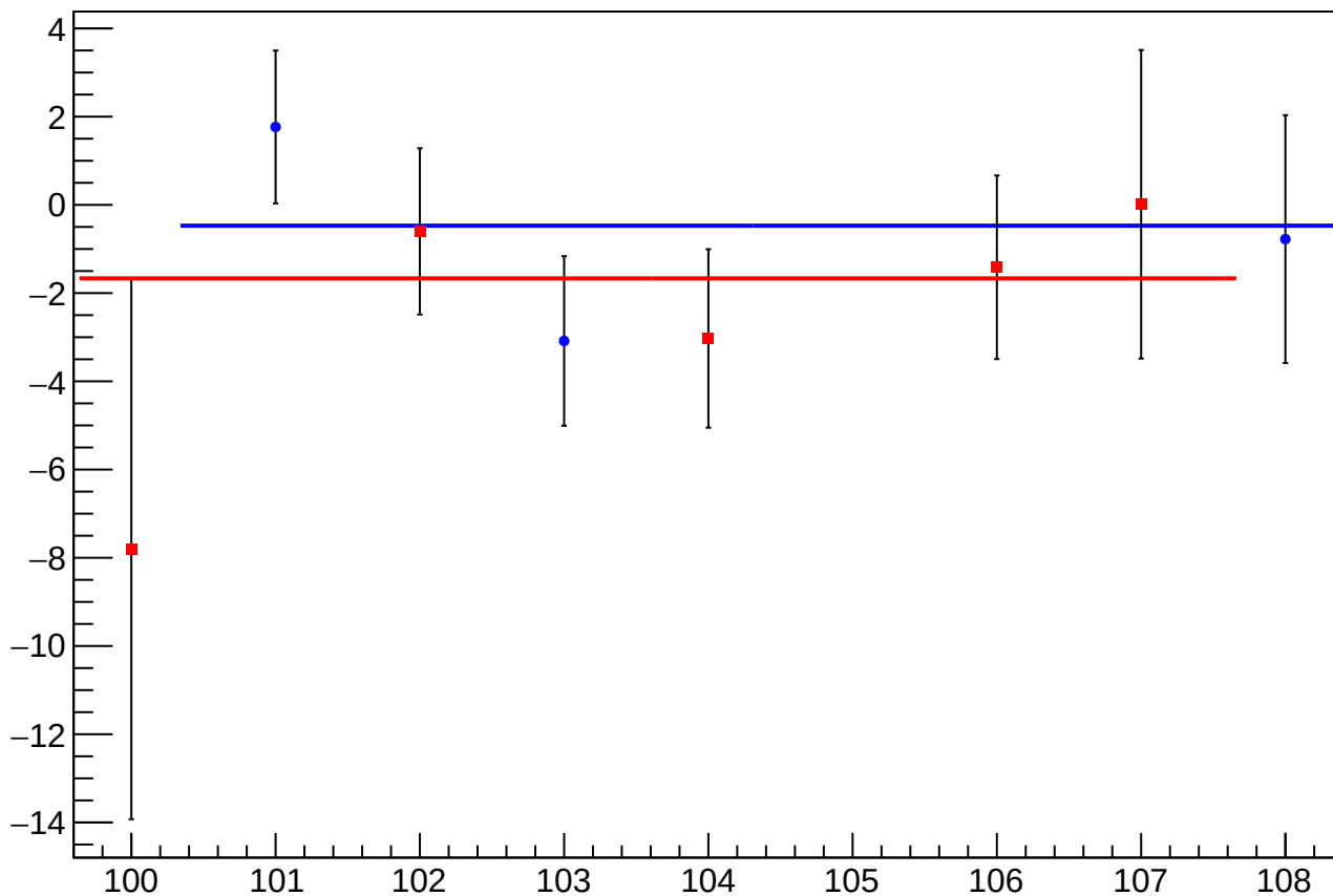
diff_bpm4aediY_mean vs Slug, Sign Corrected
