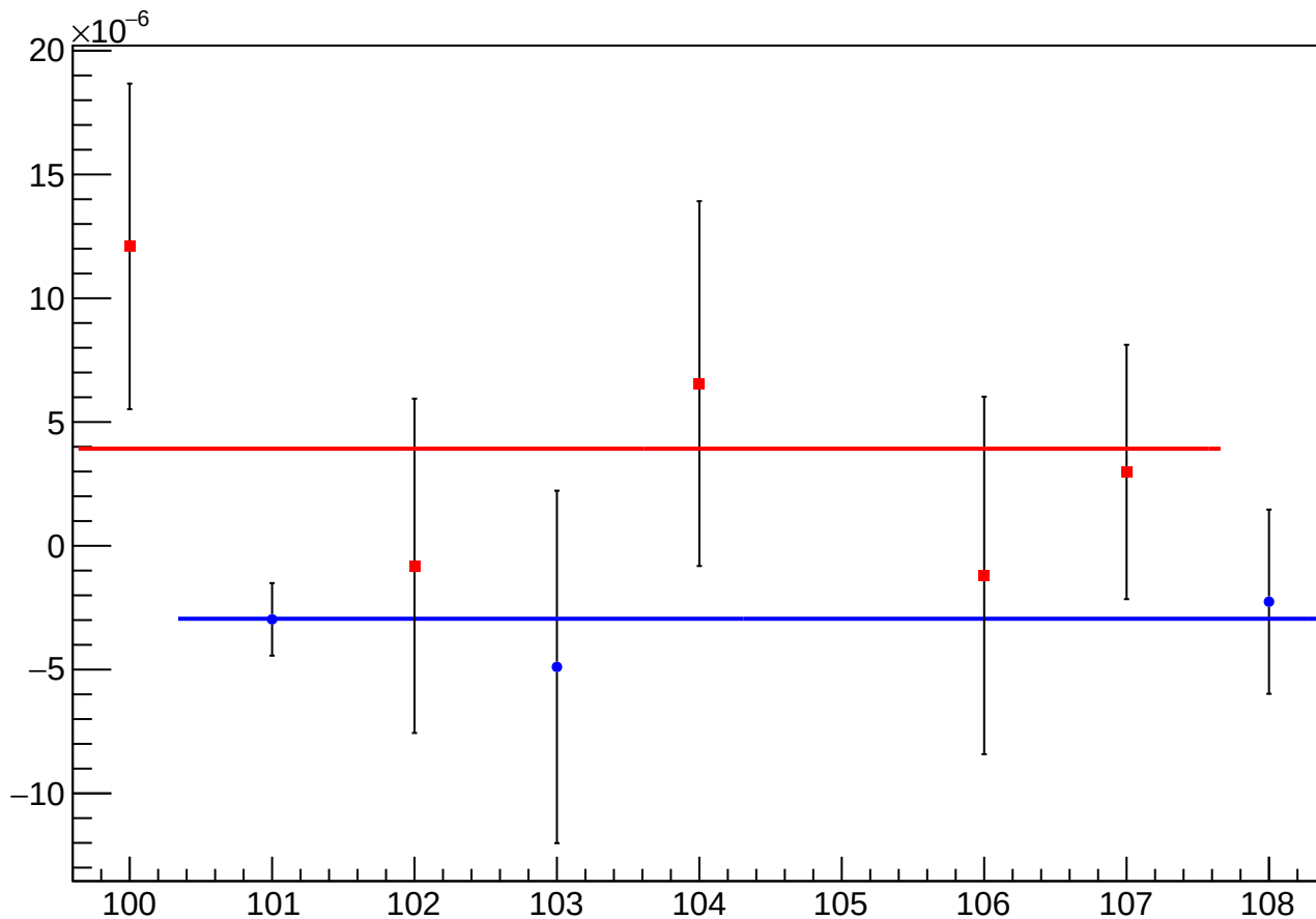
asym_sam_26_48_dd_eigen_dit_vs_dit_diff_mean vs Slug, Sign Corrected
