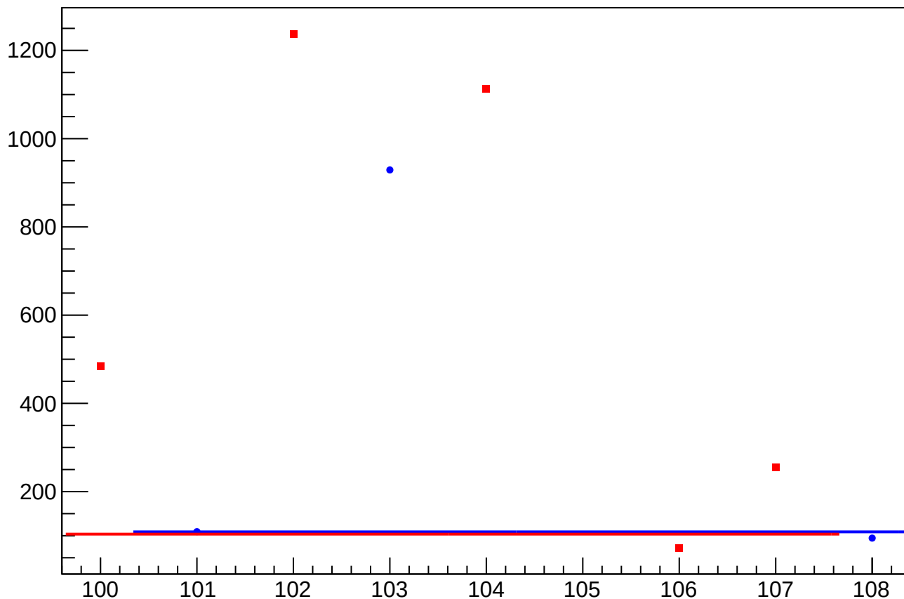
asym_us_avg_at1lr_avg_avg_eigen_dit_vs_eigen_cor_diff_rms vs Slug, Sign Corrected
