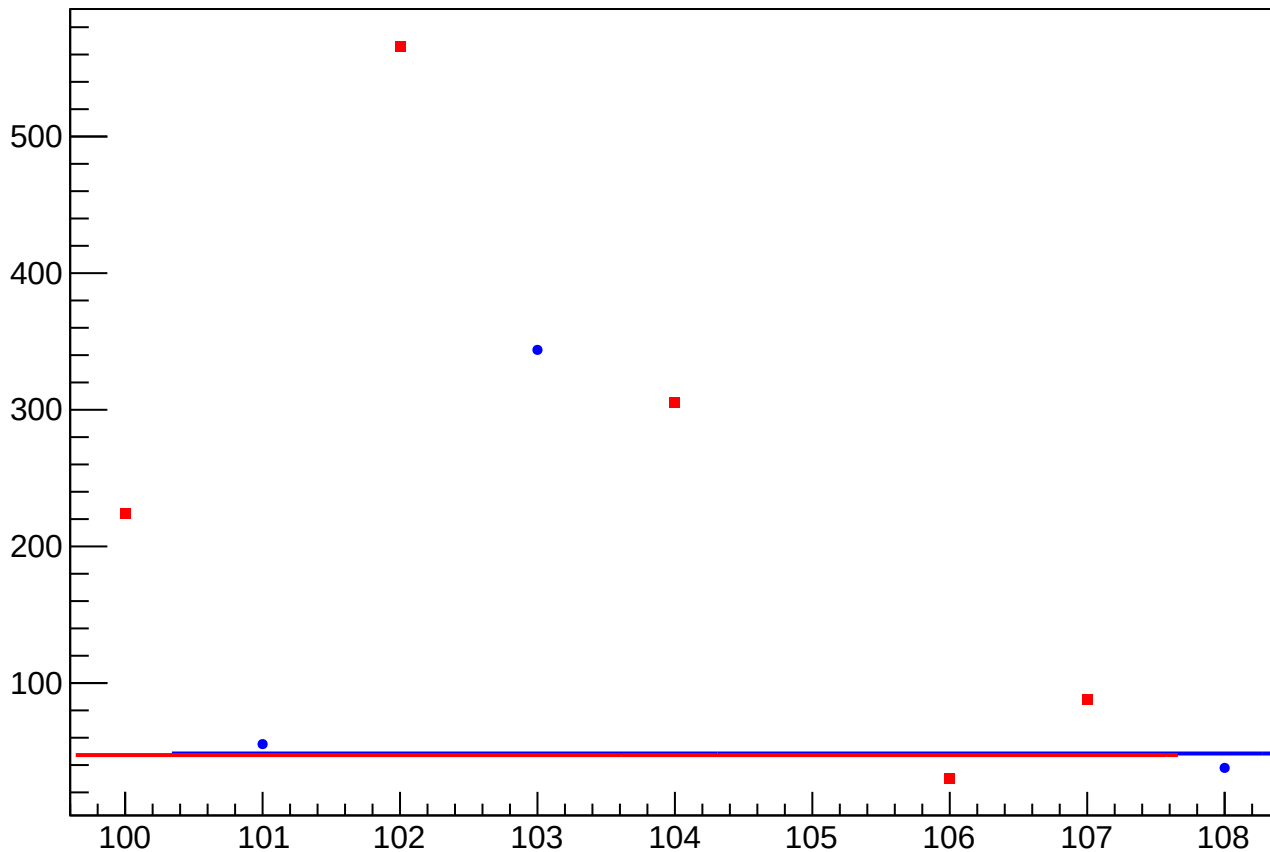
asym_at1_dd_at2_dd_avg_eigen_dit_vs_cor_diff_rms vs Slug, Sign Corrected
