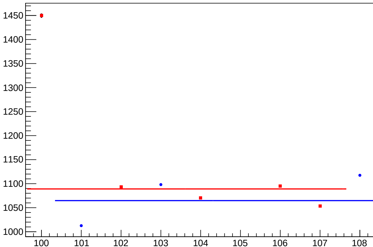
asym_sam_15_26_dd_cor_correction_rms vs Slug, Sign Corrected
