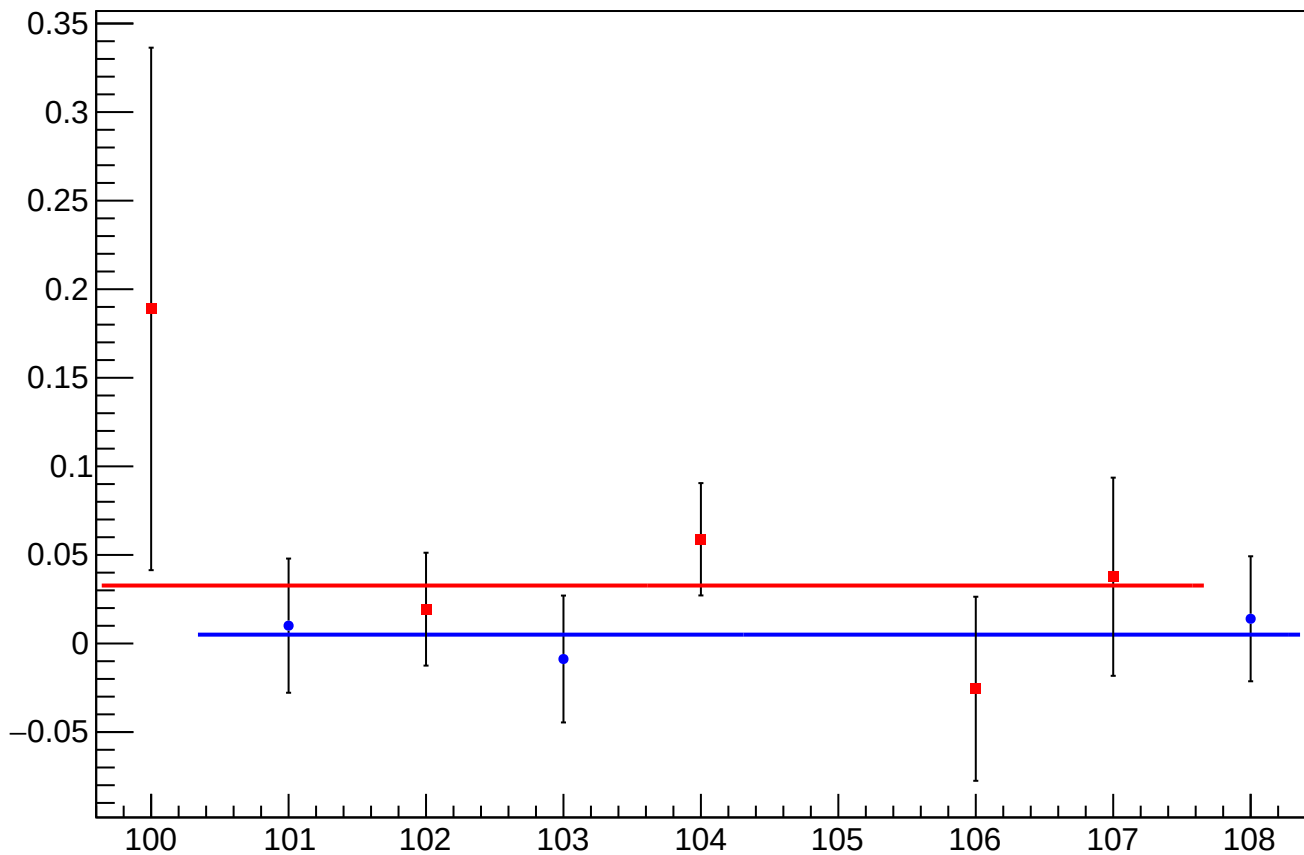
asym_us_dd_eigen_dit_vs_slug, Sign Corrected
