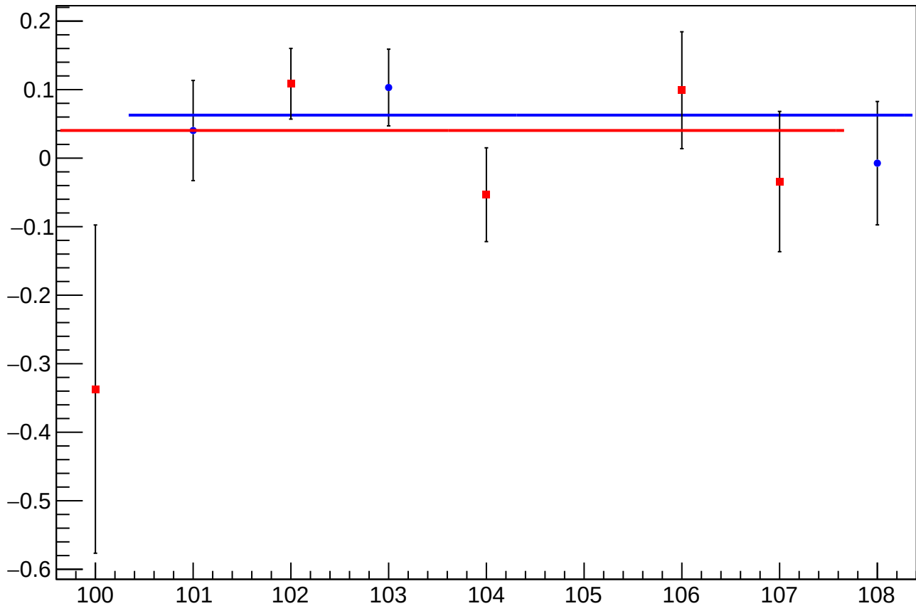
asym_usr_overload_cor_vs_eigen_cor_diff_mean vs Slug, Sign Corrected
