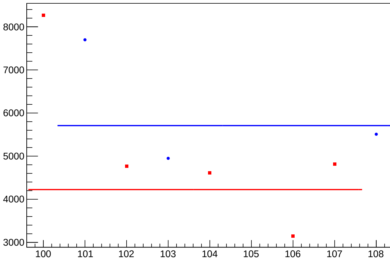
asym_us_avg_at2lr_avg_dd_dit_correction_rms vs Slug, Sign Corrected
