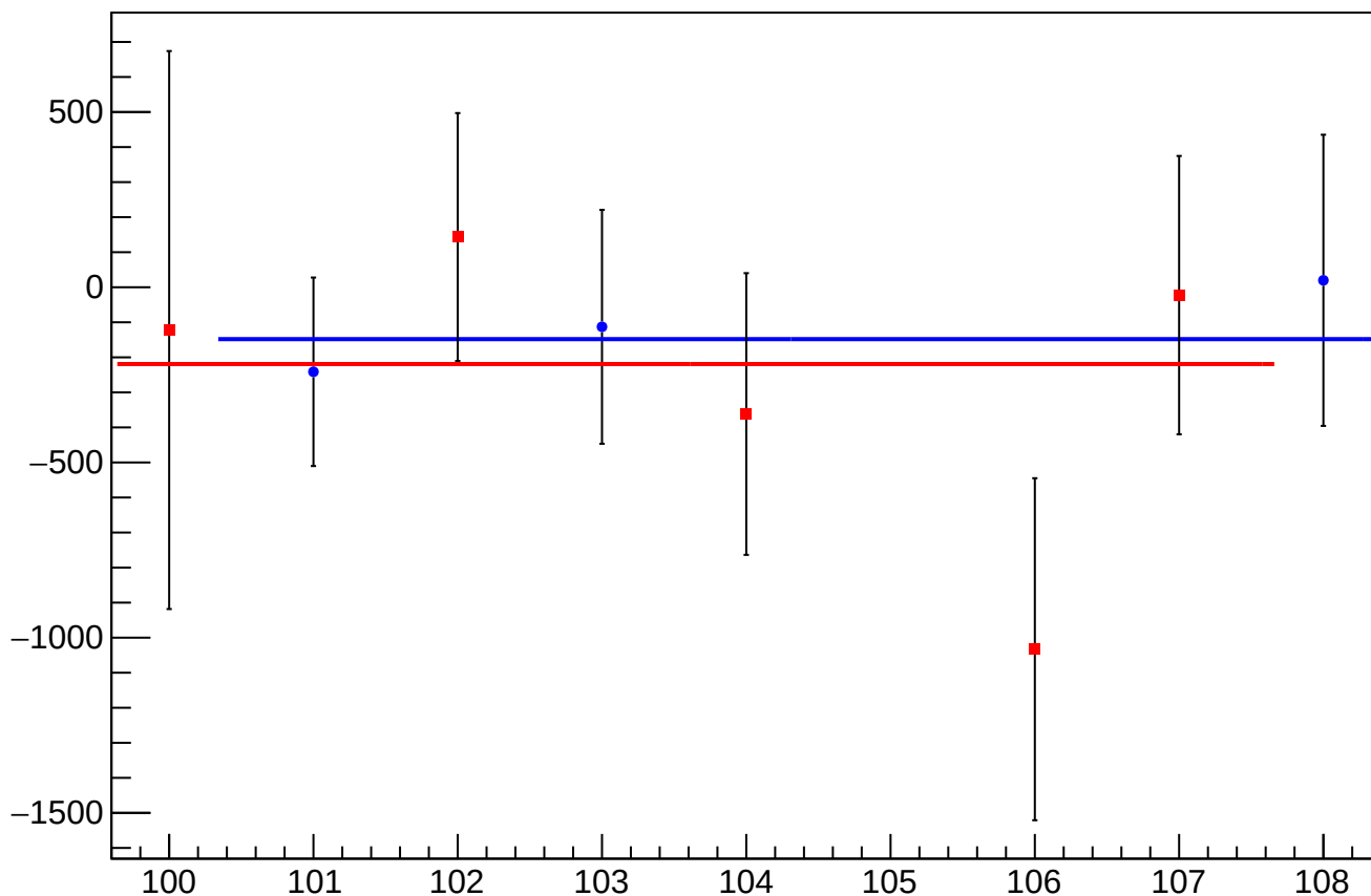
asym_bcm_an_us_an_ds_avg_mean vs Slug, Sign Corrected
