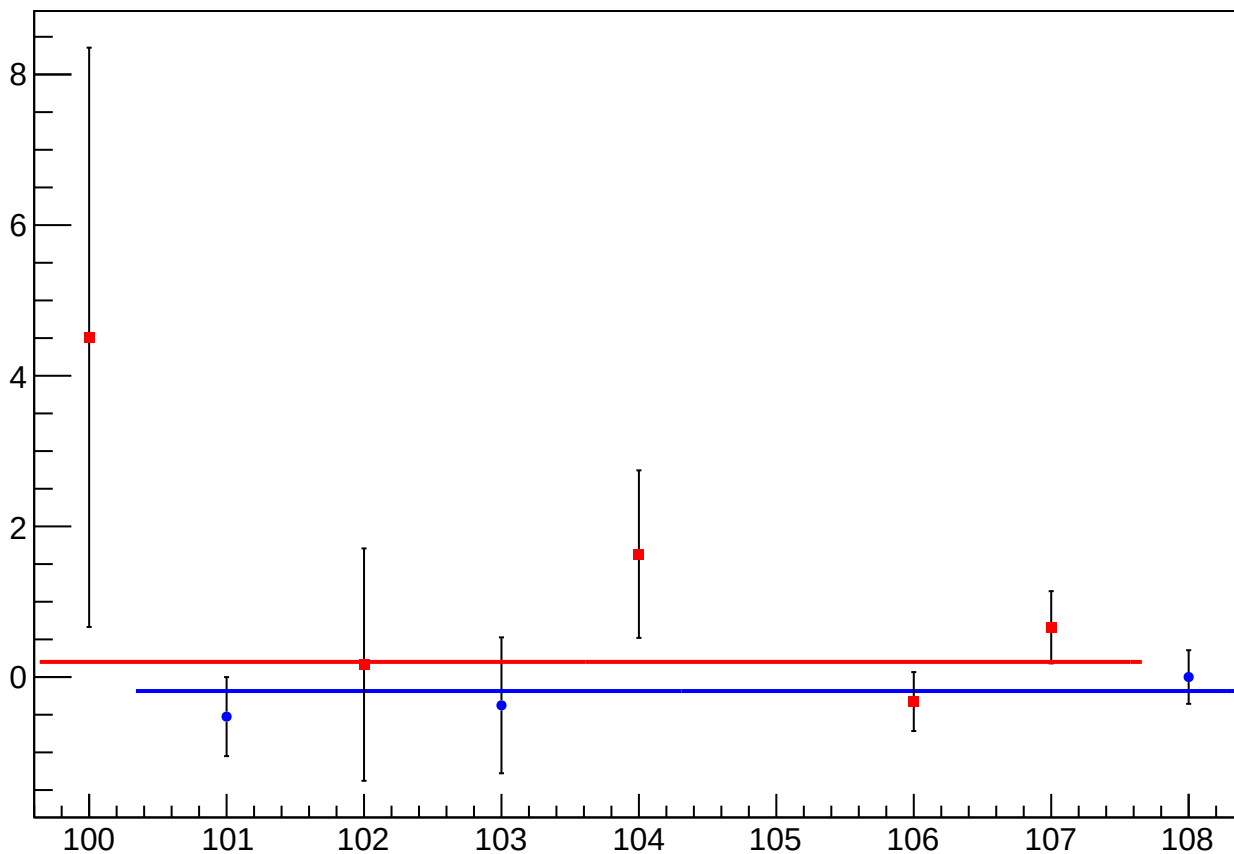
asym_at2_avg_dit_vs_eigen_cor_diff_mean vs Slug, Sign Corrected
