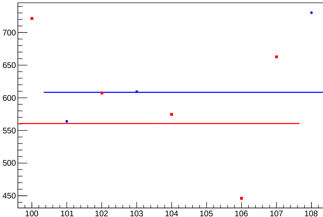
asym_sam_15_48_dd_dit_correction_rms vs Slug, Sign Corrected
