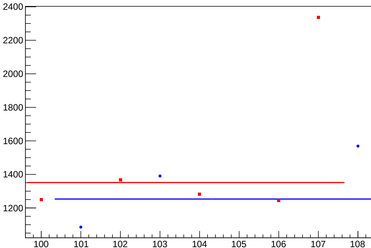
asym_us_agg_avg_rms vs Slug, Sign Corrected
