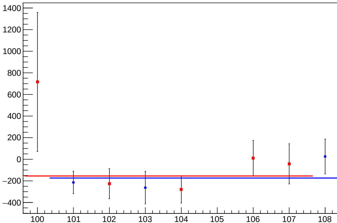
eigen_cor_asym_sam6_mean vs Slug, Sign Corrected
