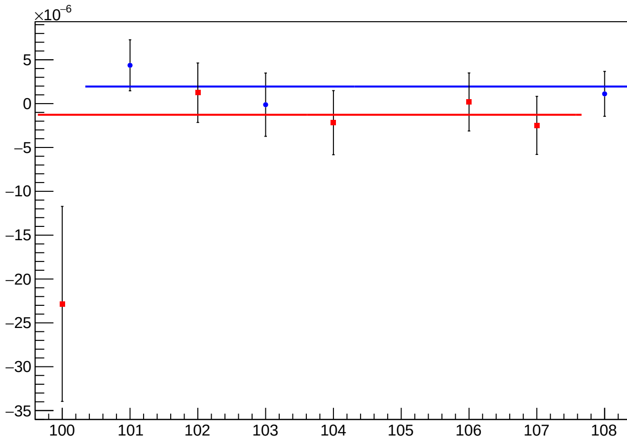
asym_sam8_eigen_dit_vs_dit_diff_mean vs Slug, Sign Corrected
