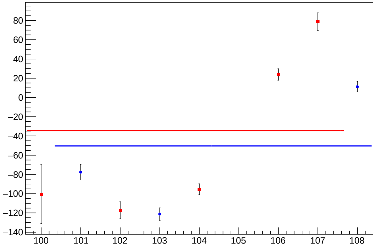
reg_asym_us_dd_at1lr_dd_dd_diff_bpm1X_slope vs Slug, Sign Corrected
