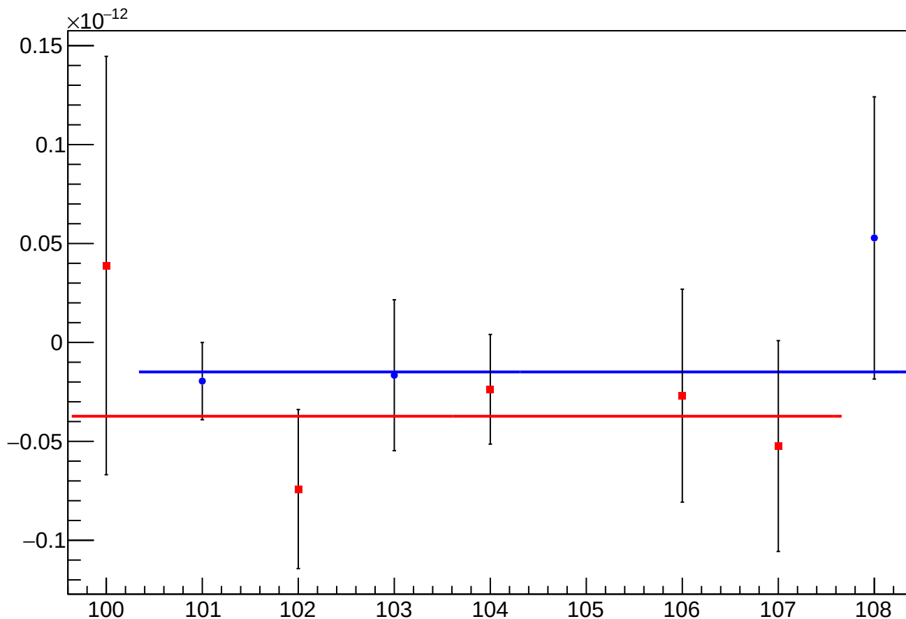
asym_sam_15_dd_reg_vs_cor_diff_mean vs Slug, Sign Corrected
