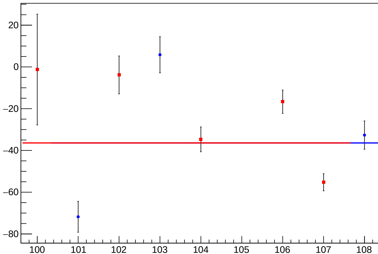
reg_asym_at1_avg_at2_avg_dd_diff_bpm4eY_slope vs Slug, Sign Corrected
