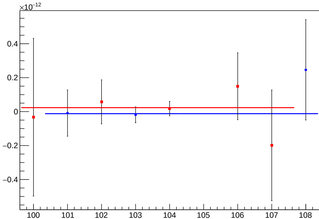
asym_atl_avg_atr_avg_avg_eigen_cor_vs_cor_diff_mean vs Slug, Sign Corrected
