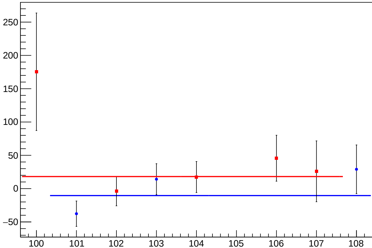
diff_bpmtargetsumX_mean vs Slug, Sign Corrected
