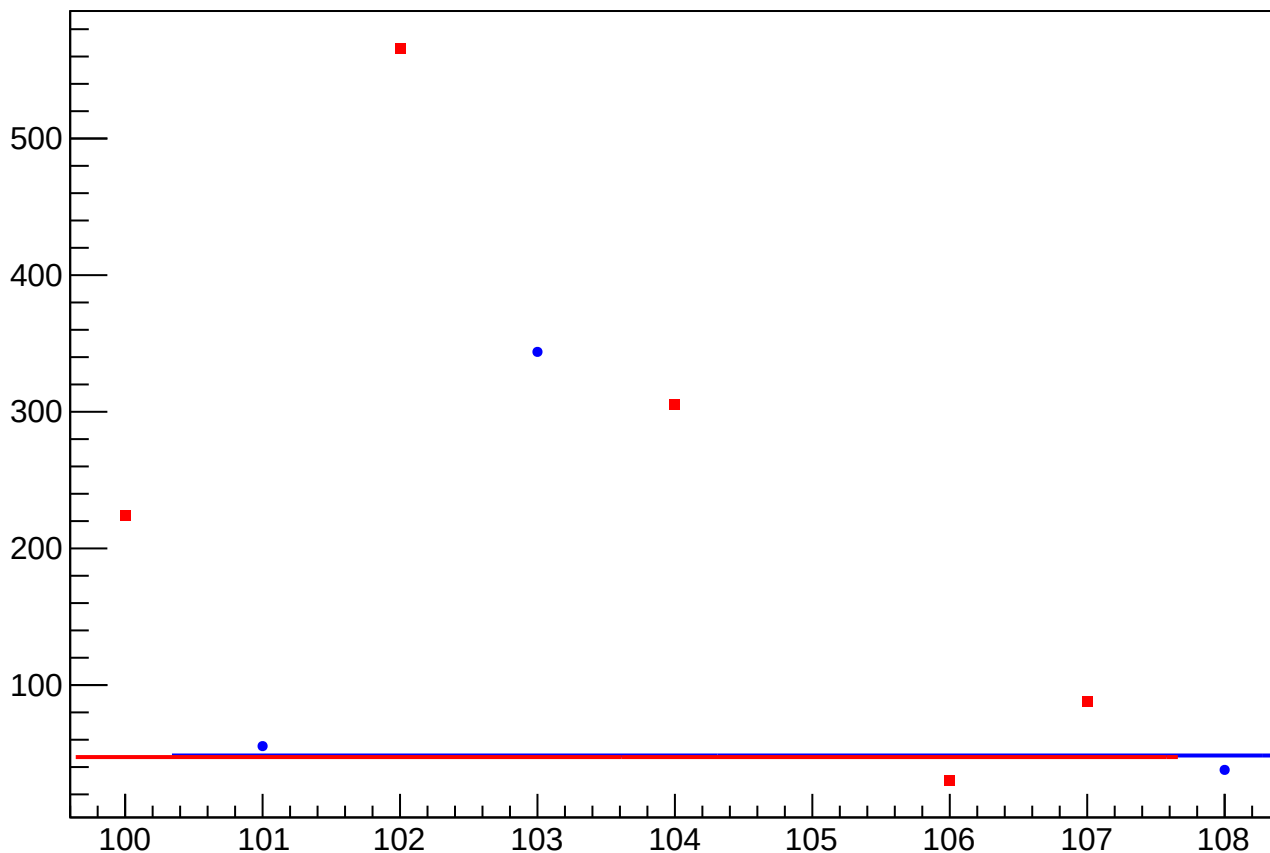
asym_atl_dd_atr_dd_dd_eigen_dit_vs_eigen_cor_diff_rms vs Slug, Sign Corrected
