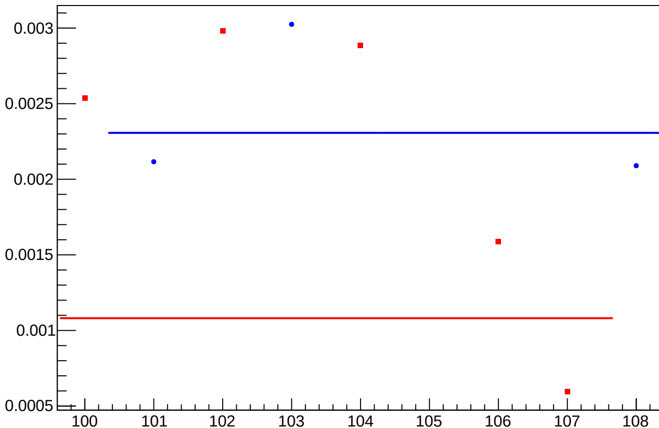
asym_sam_12345678_avg_eigen_dit_vs_dit_diff_rms vs Slug, Sign Corrected
