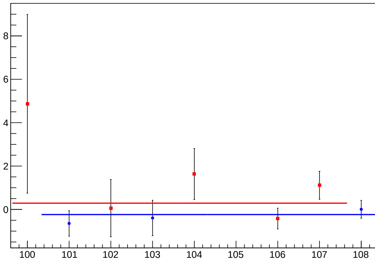
asym_us_avg_at2lr_avg_avg_dit_vs_cor_diff_mean vs Slug, Sign Corrected
