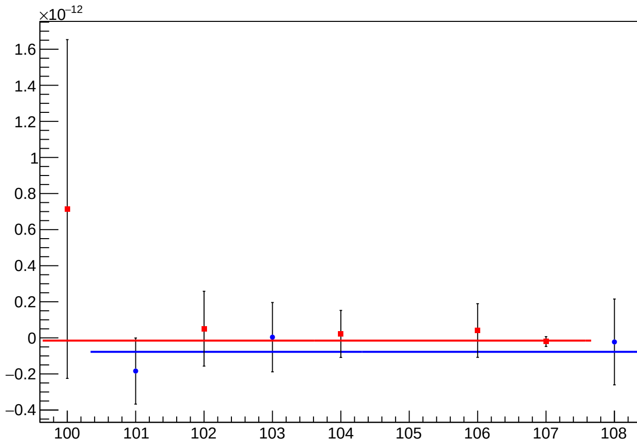
asym_atl1r2_dd_eigen_cor_vs_slug_sign_corrected
