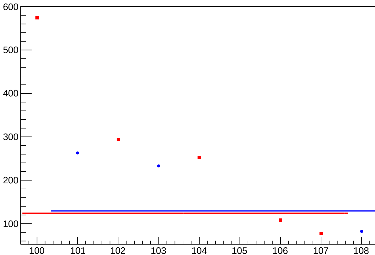
asym_atl1r2_dd_dit_vs_eigen_cor_diff_rms vs Slug, Sign Corrected
