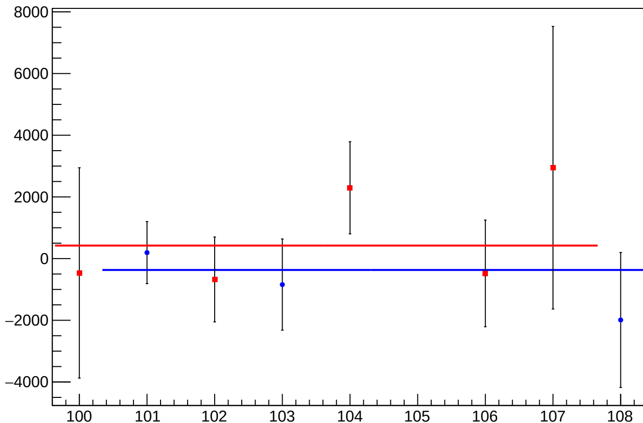
asym_us_avg_eigen_dit_correction_mean vs Slug, Sign Corrected
