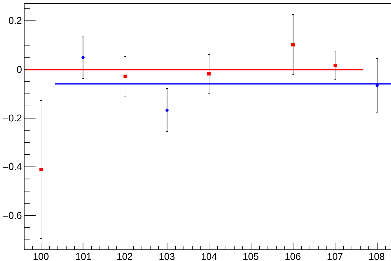
asym_sam1_dif_vs_cor_diff_mean vs Slug, Sign Corrected
