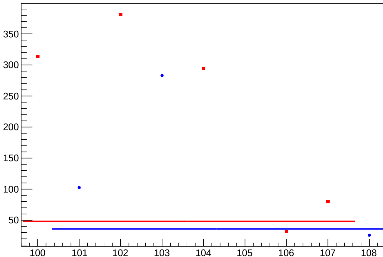
asym_atl_avg_atr_avg_dd_eigen_dit_vs_cor_diff_rms vs Slug, Sign Corrected
