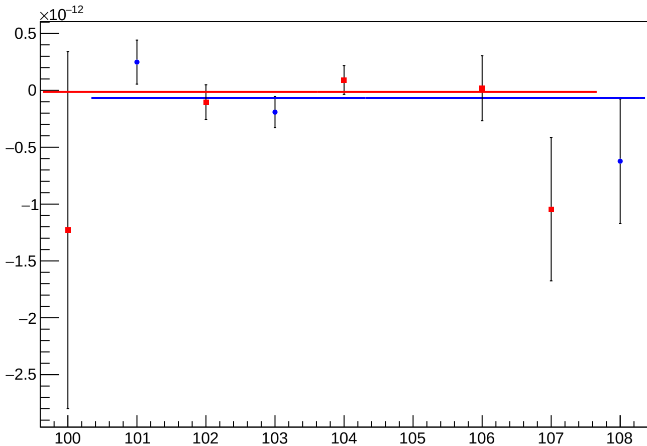
asym_us_avg_atlr_avg_avg_reg_vs_cor_diff_mean vs Slug, Sign Corrected
