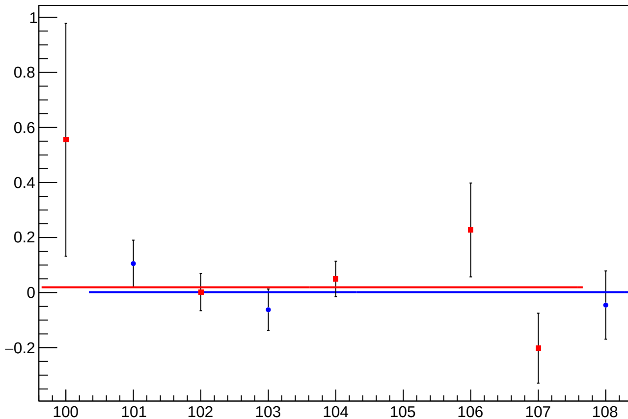
asym_sam_2468_avg_eigen_dit_vs_eigen_cor_diff_mean vs Slug, Sign Corrected
