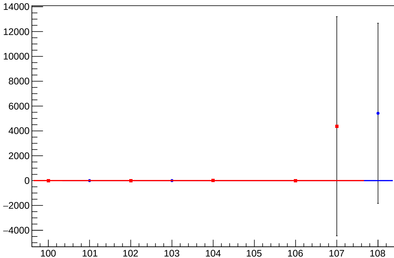
asym_cav4bQ_mean vs Slug, Sign Corrected
