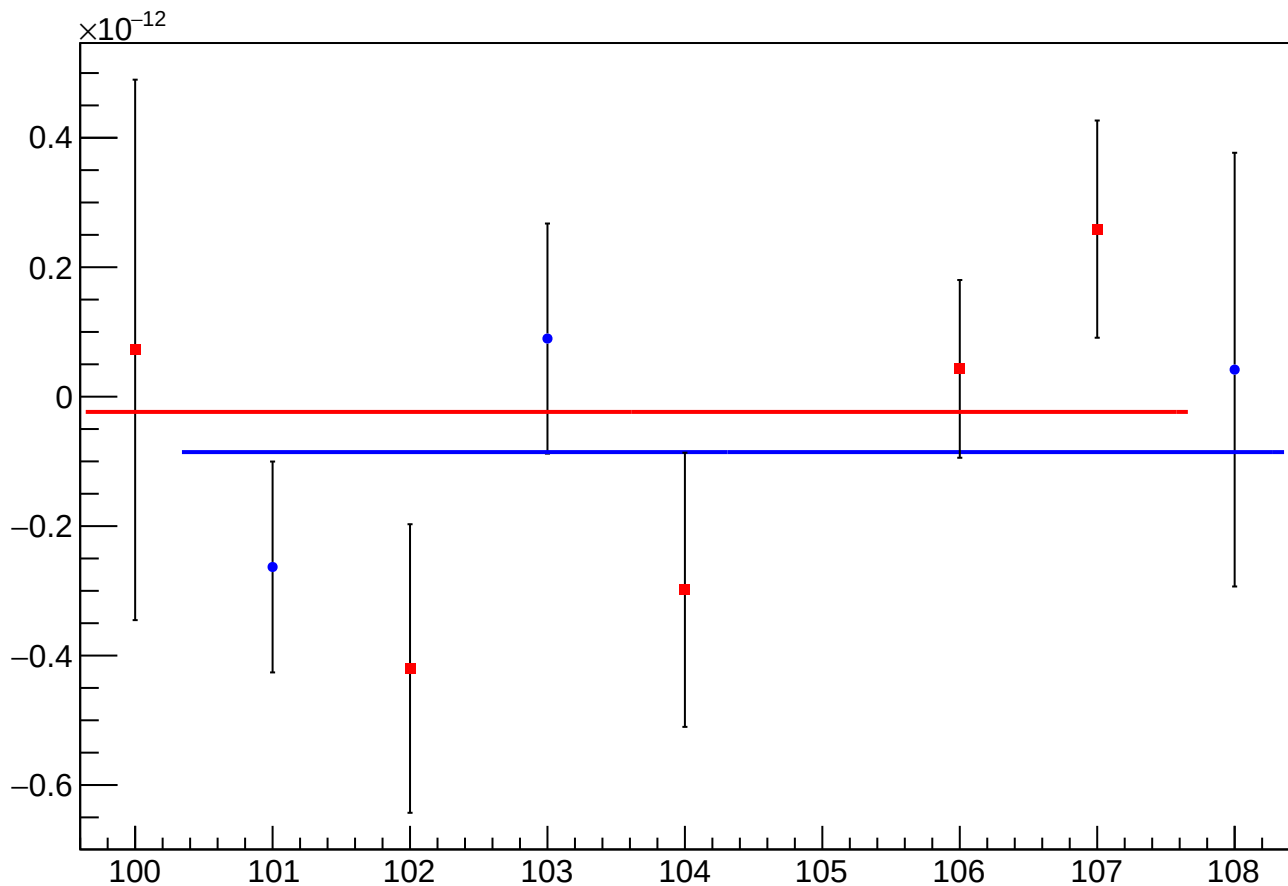
asym_atl1r2_dd_atl2r1_dd_dd_reg_vs_cor_diff_mean vs Slug, Sign Corrected
