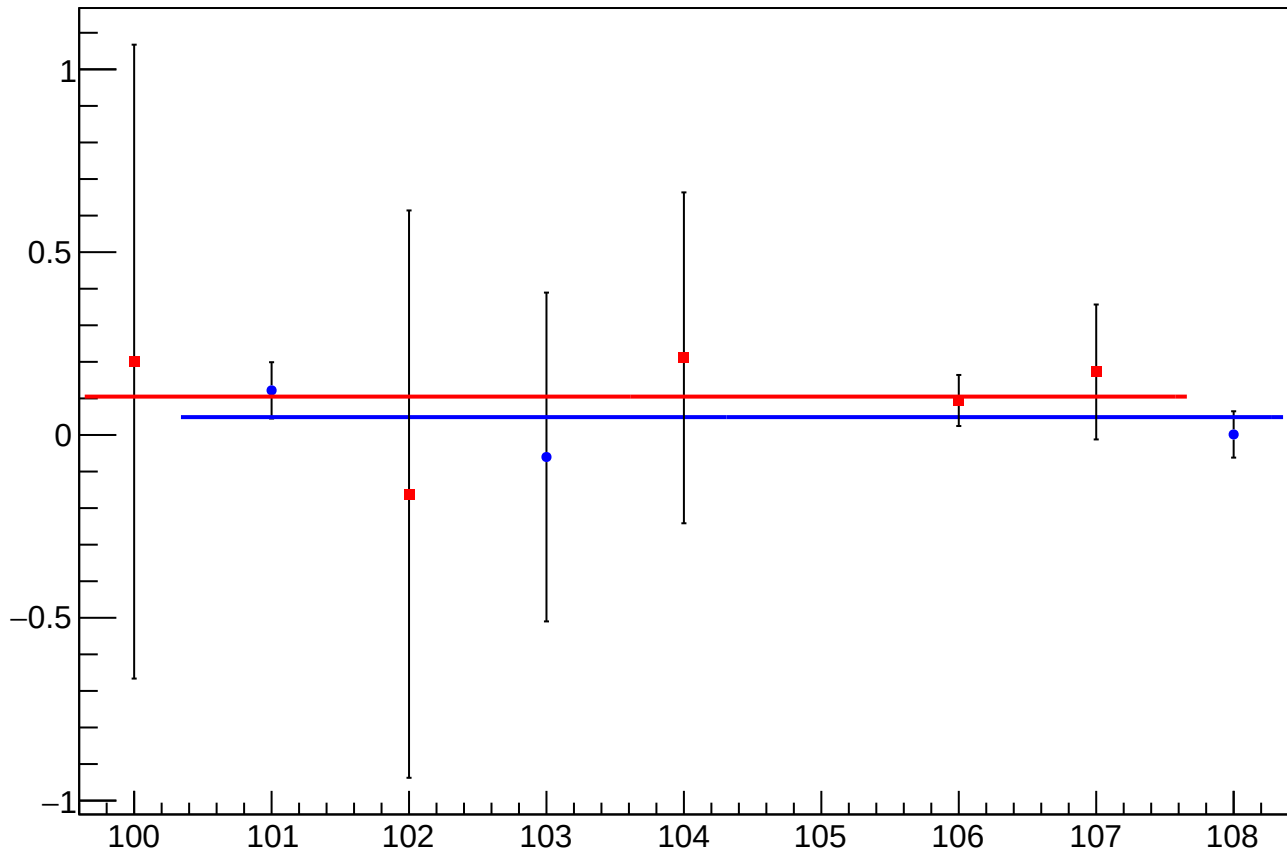
asym_atl_dd_atr_dd_dd_dit_vs_Slug, Sign Corrected
