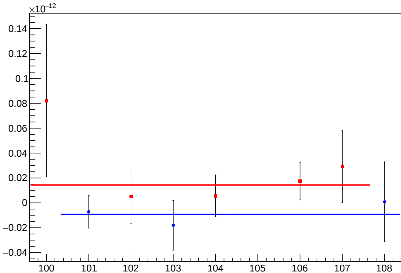
asym_sam5_eigen_cor_vs_cor_diff_mean vs Slug, Sign Corrected
