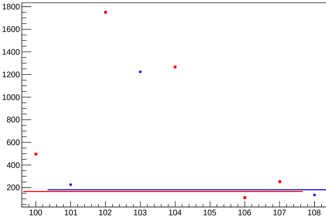
asym_atl1r2_avg_dit_vs_eigen_cor_diff_rms vs Slug, Sign Corrected
