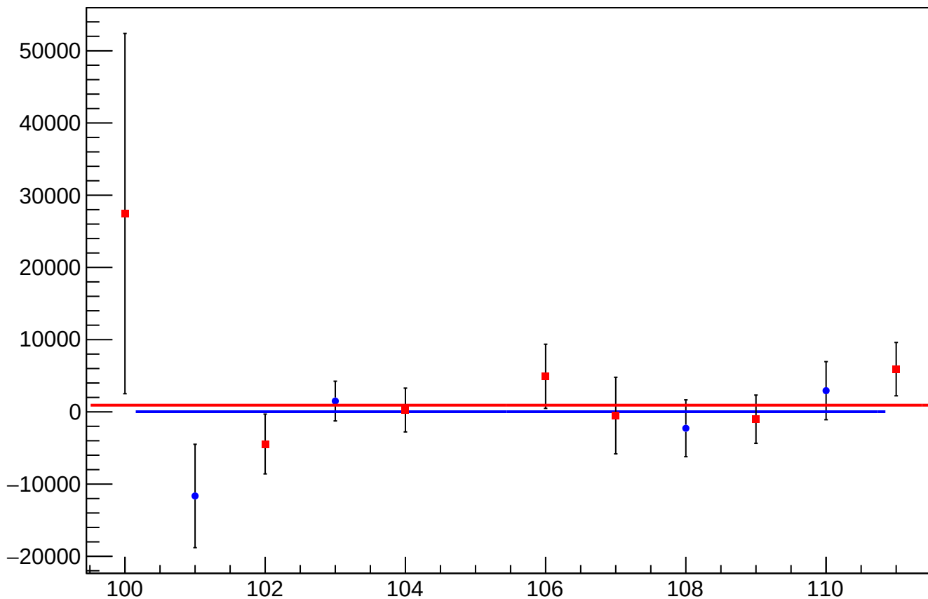
cor_asym_us_dd_at1lr_dd_avg_mean vs Slug
