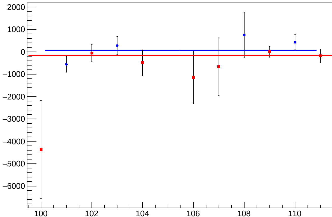
asym_sam7_cor_correction_mean vs Slug
