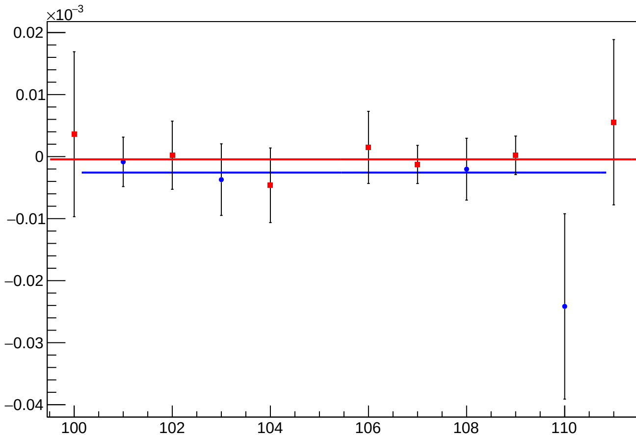
asym_sam_2468_avg_eigen_dit_vs_dit_diff_mean vs Slug
