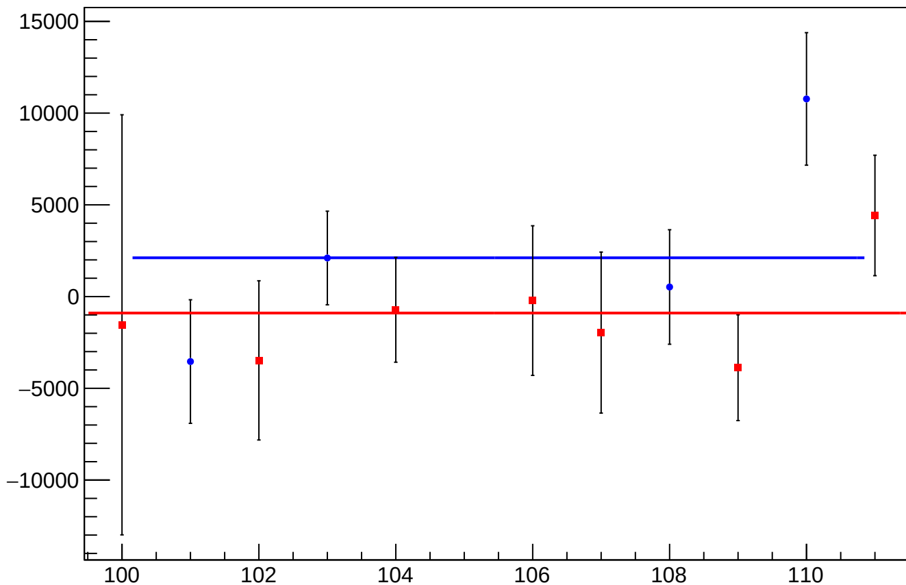
dit_asym_atl1r2_avg_mean vs Slug
