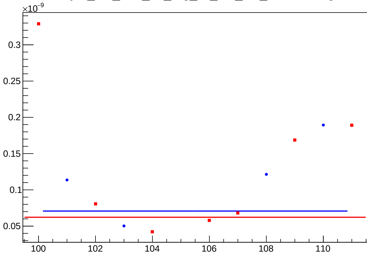
asym_usr_atr2_dd_reg_vs_cor_diff_rms vs Slug
