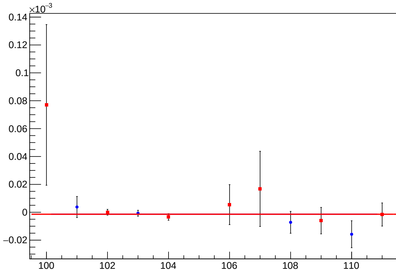
asym_us_avg_atlr_avg_dd_eigen_dit_vs_dit_diff_mean vs Slug
