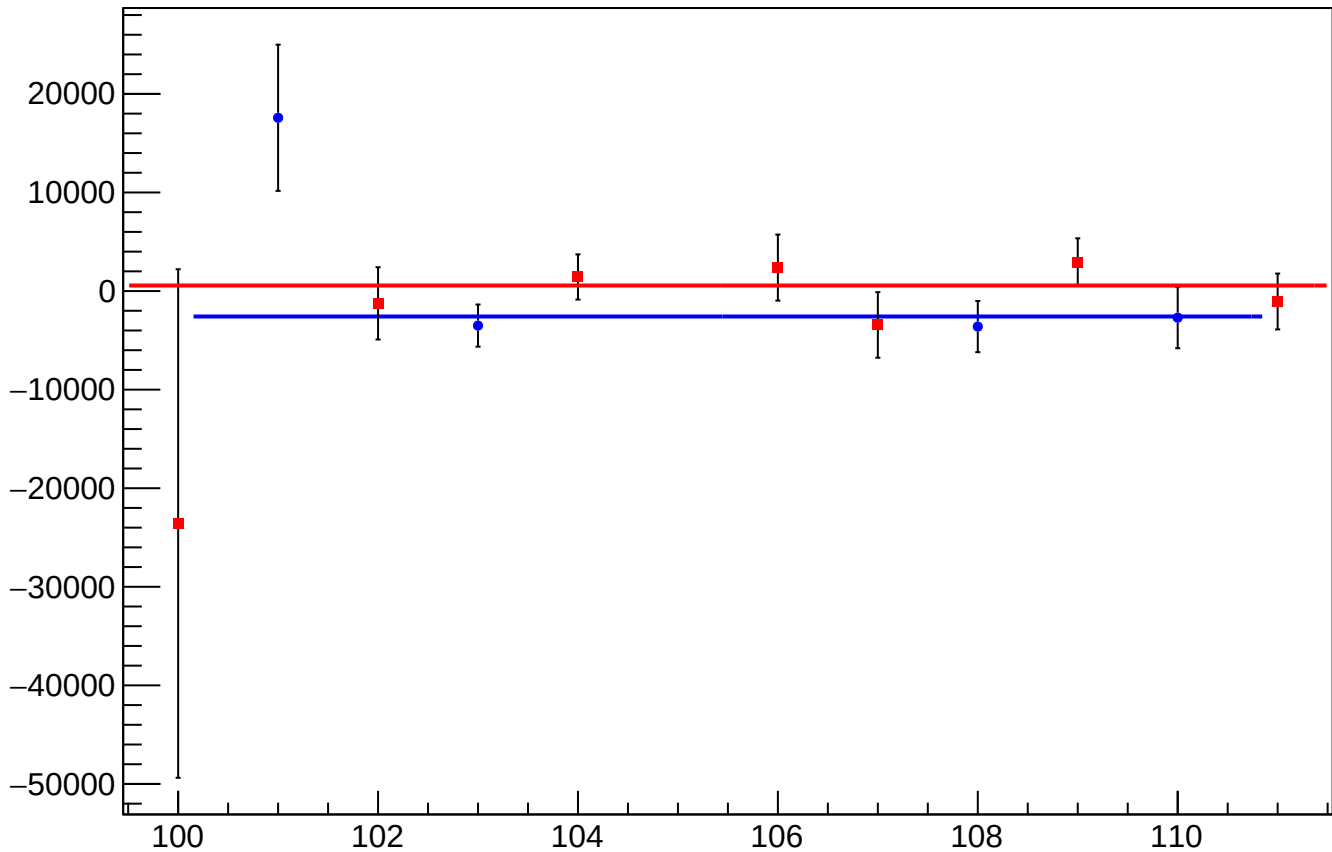
eigen_dit_asym_atr_dd_mean vs Slug
