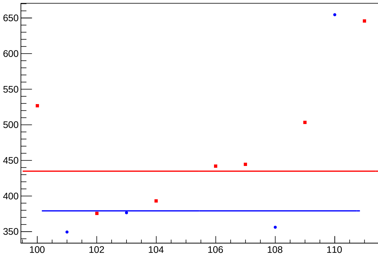
asym_sam6_reg_correction_rms vs Slug
