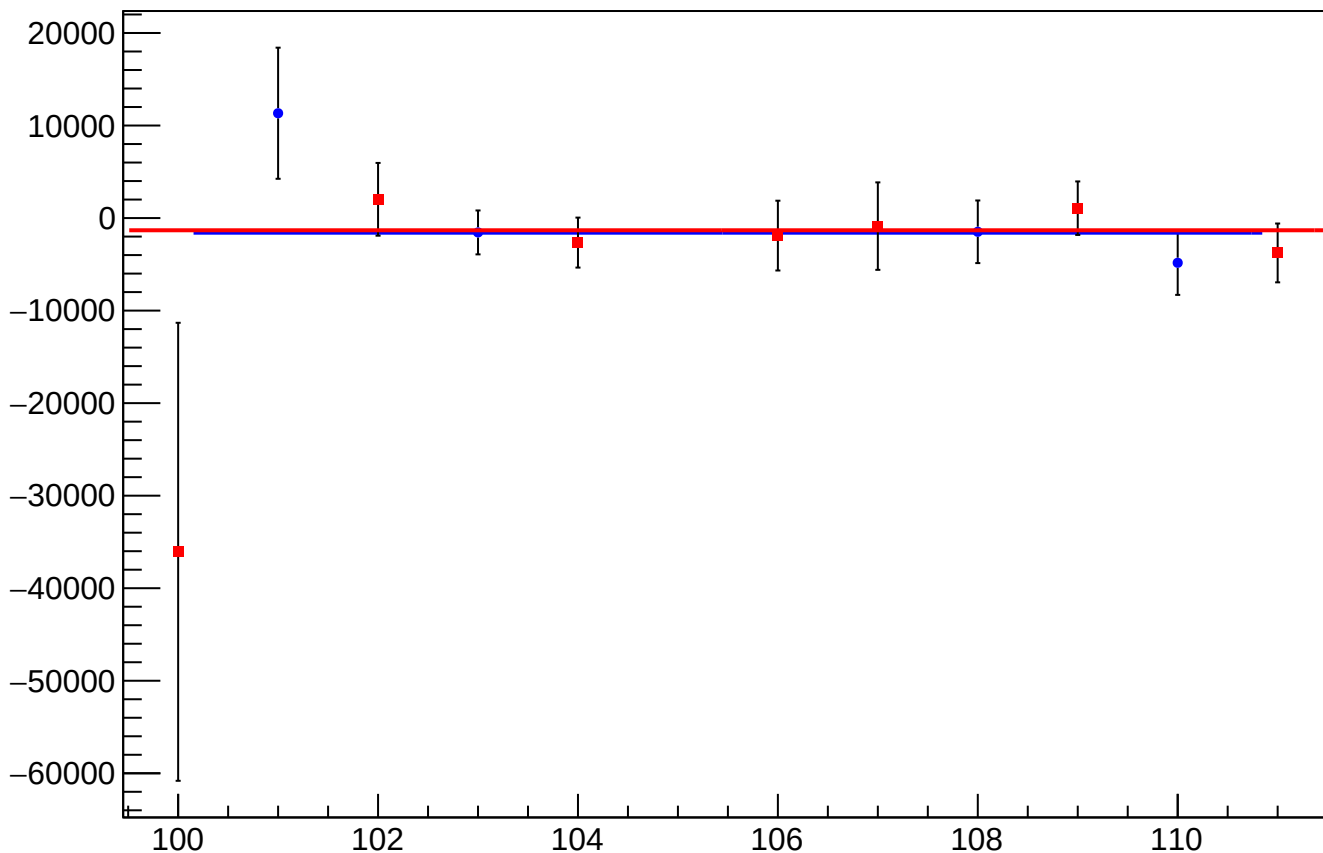
dit_asym_us_dd_at1lr_dd_dd_mean vs Slug
