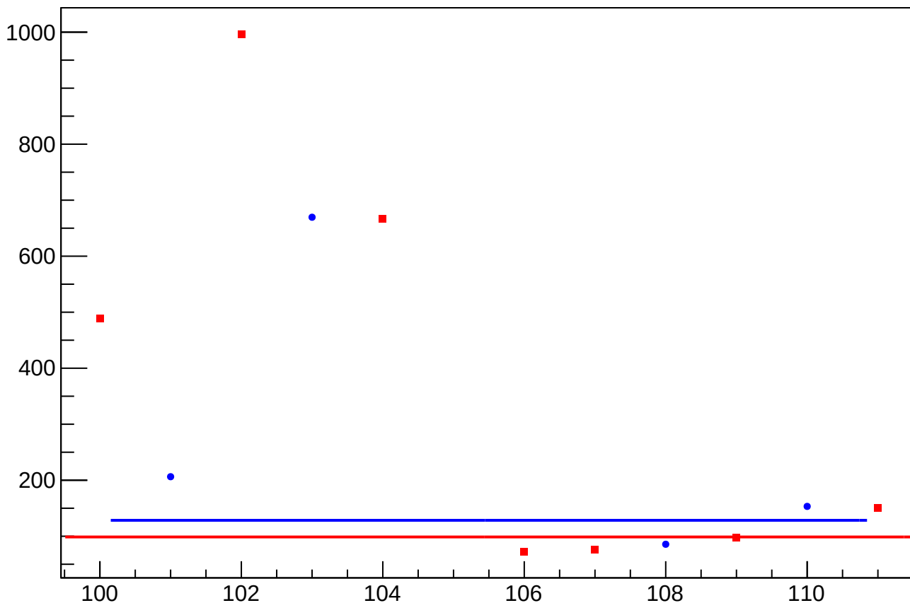
asym_usr_atr2_dd_dit_vs_cor_diff_rms vs Slug
