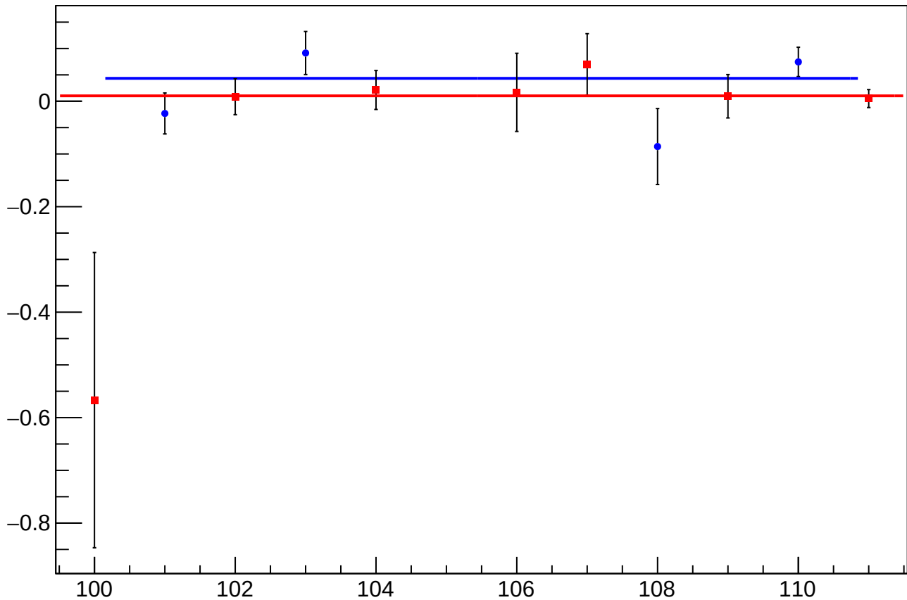
asym_sam8_dit_vs_cor_diff_mean vs Slug
