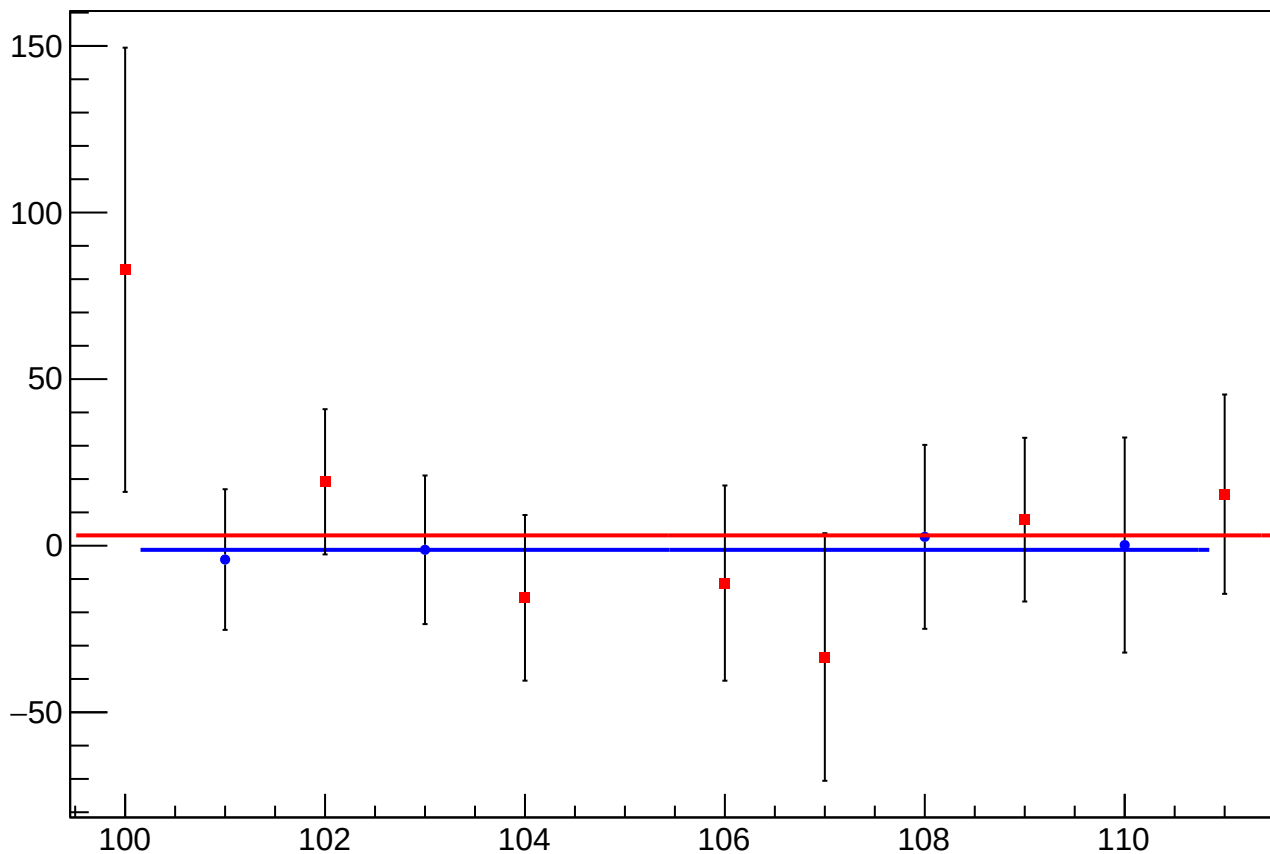
asym_bcm_dg_ds_an_ds_dd_mean vs Slug
