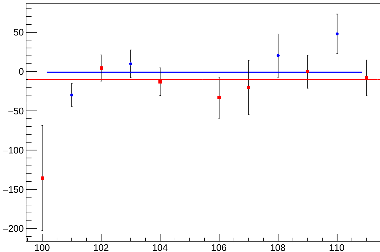
diff_bpm_4aX_4acX_avg_mean vs Slug
