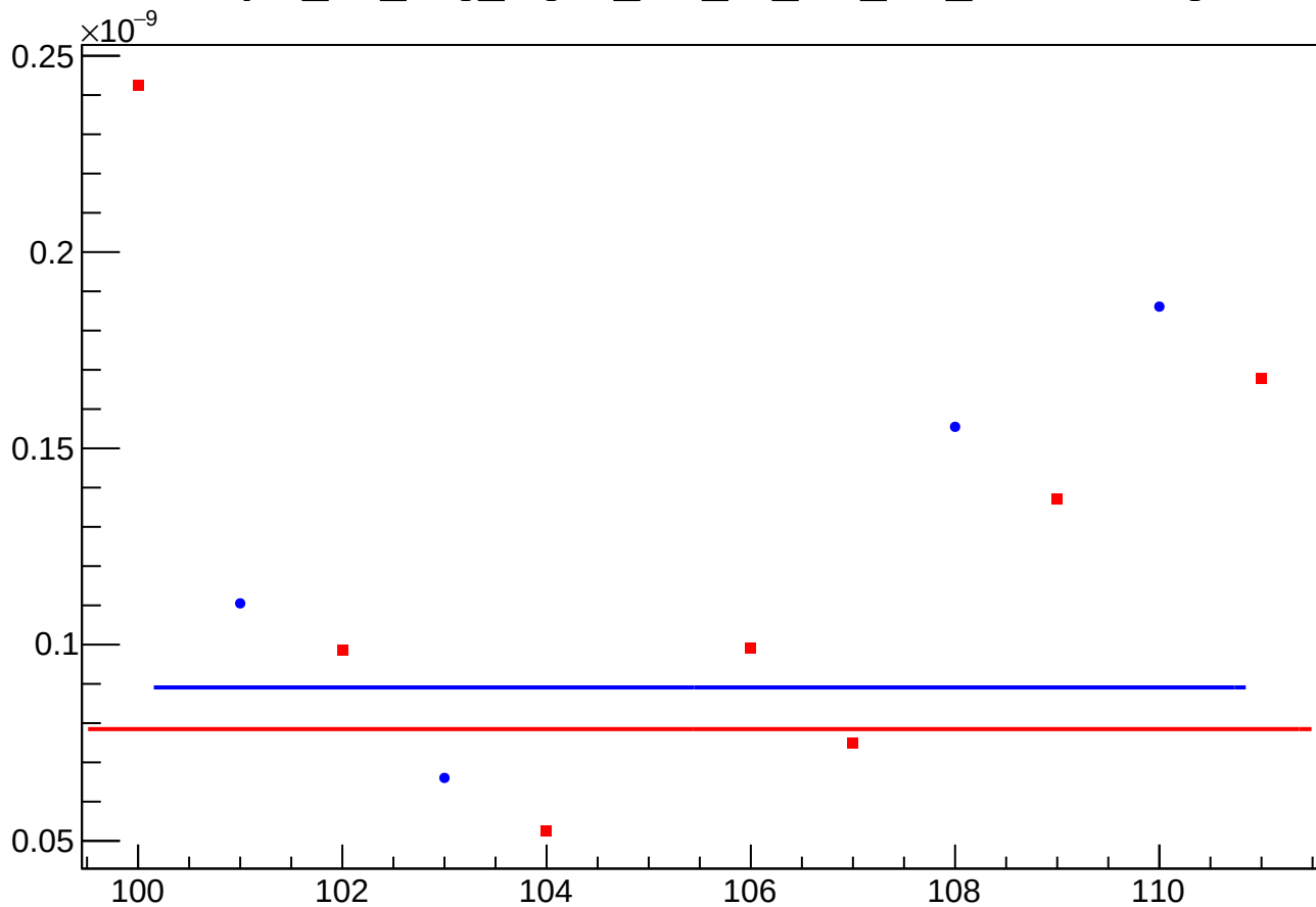
asym_atr_avg_eigen_cor_vs_cor_diff_rms vs Slug
