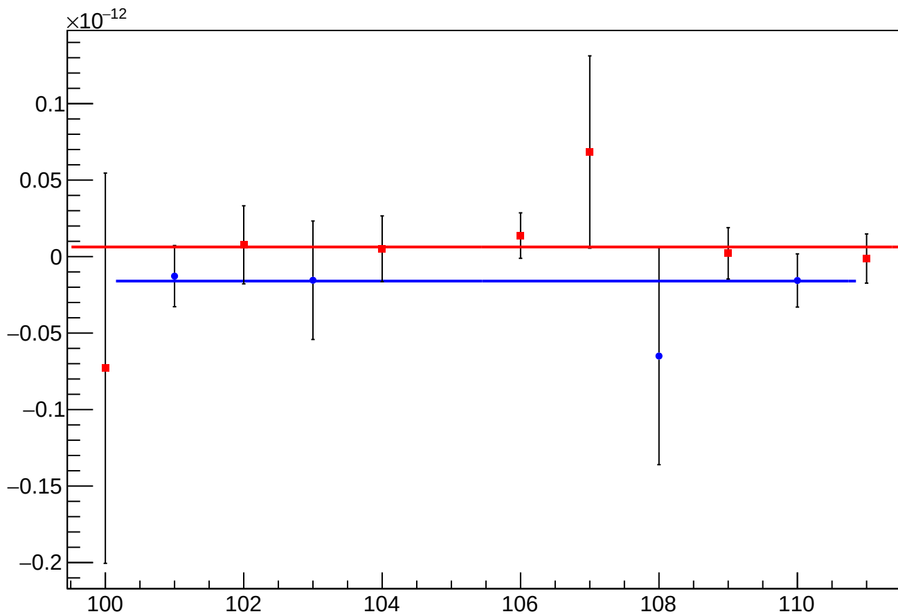
asym_sam_15_37_dd_eigen_cor_vs_cor_diff_mean vs Slug
