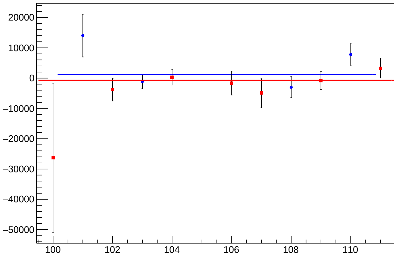
eigen_cor_asym_at1_avg_mean vs Slug
