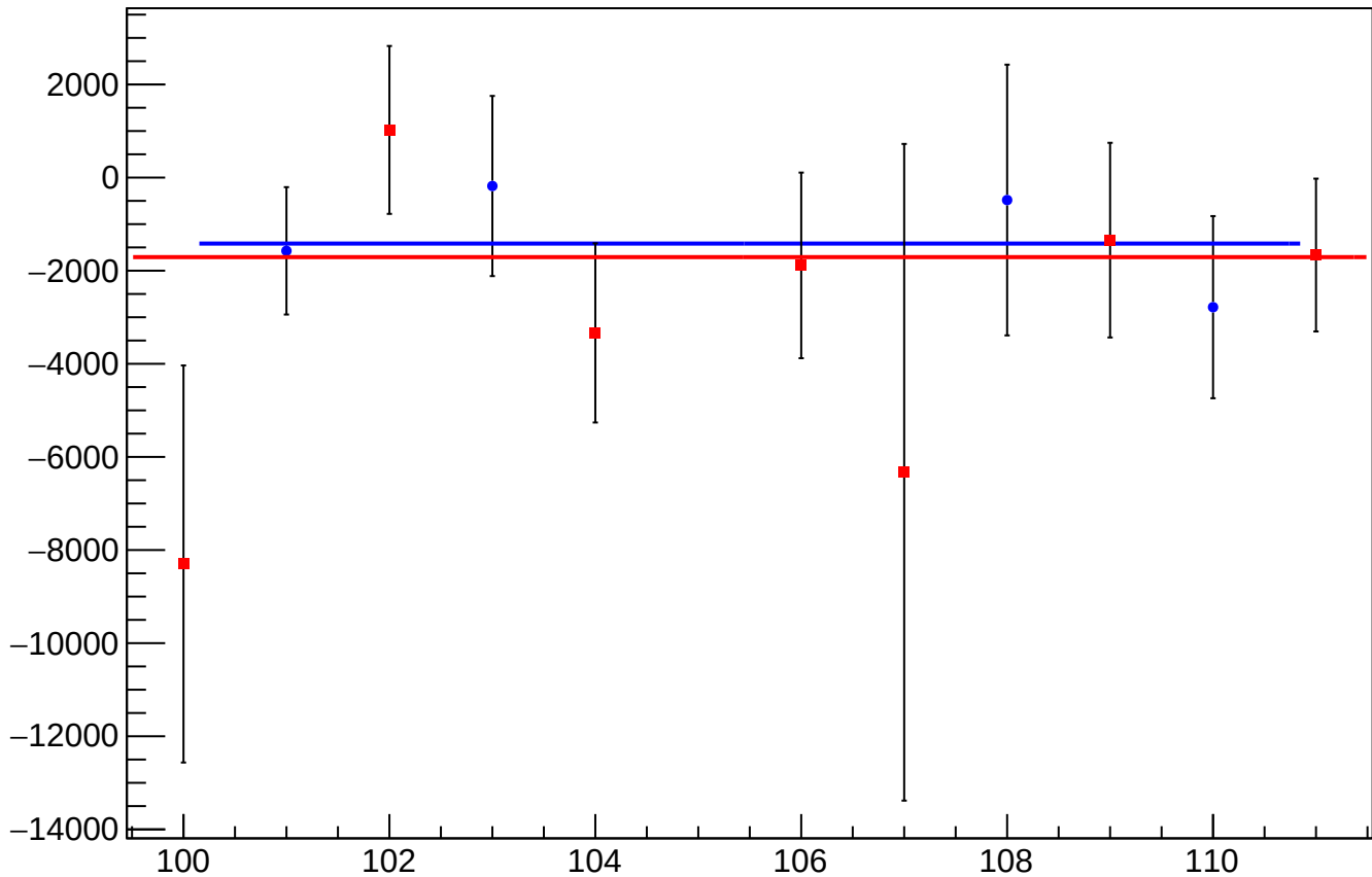
asym_usl_dit_correction_mean vs Slug
