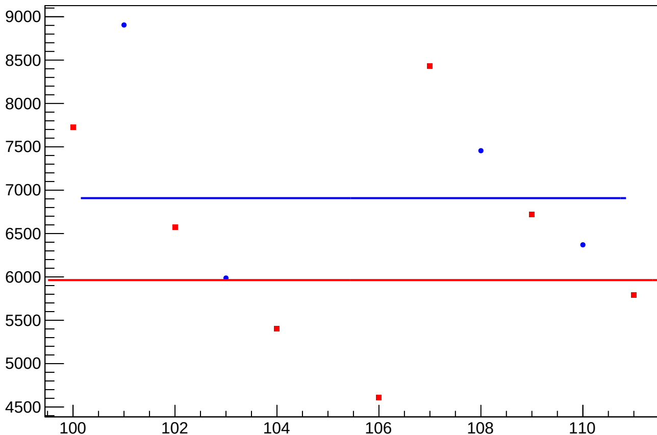
asym_atl2_reg_correction_rms vs Slug
