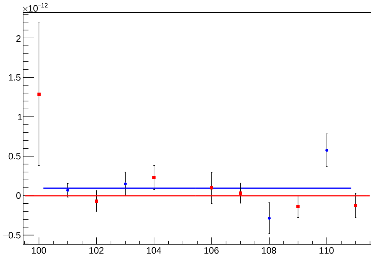
asym_sam_26_dd_eigen_cor_vs_cor_diff_mean vs Slug
