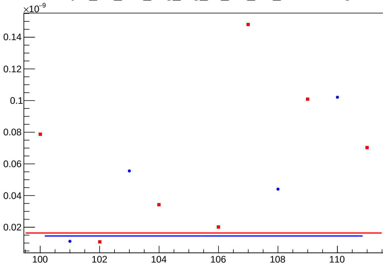
asym_usl_atl1_avg_reg_vs_cor_diff_rms vs Slug
