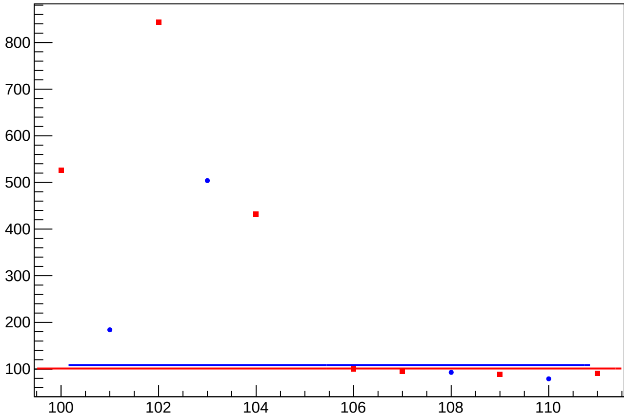
asym_atl_dd_dit_vs_cor_diff_rms vs Slug
