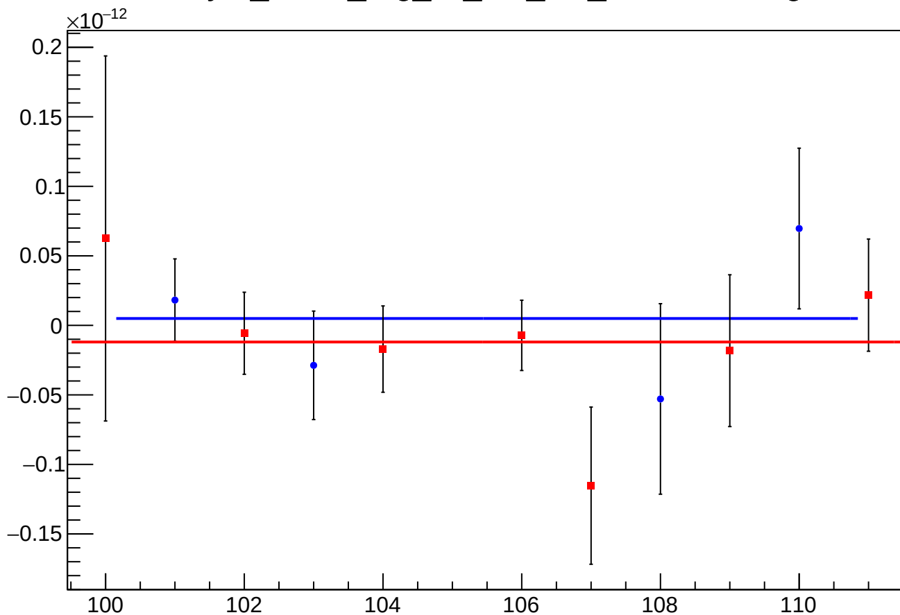
asym_sam5_reg_vs_cor_diff_mean vs Slug
