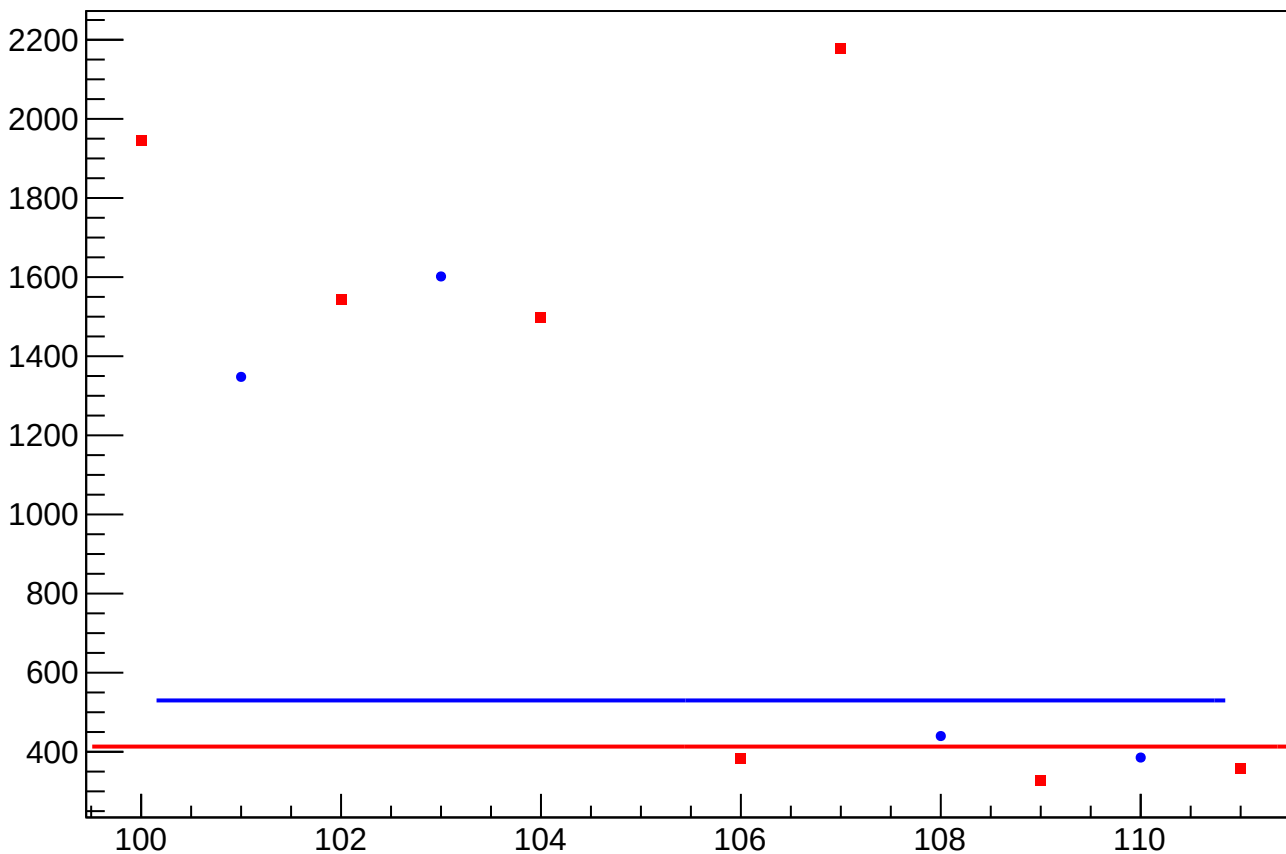
asym_atl_avg_atr_avg_dd_eigen_dit_correction_rms vs Slug
