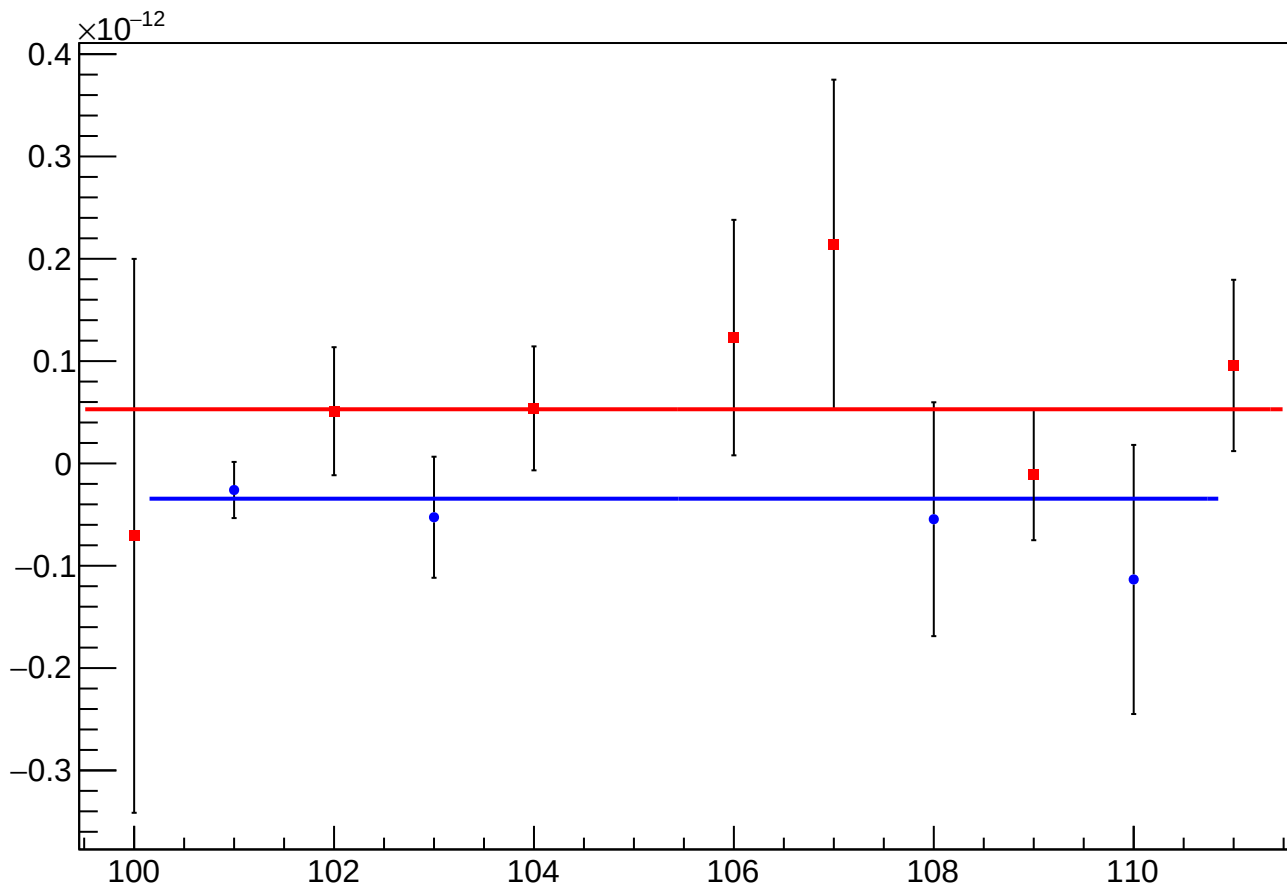
asym_at1_dd_at2_dd_avg_eigen_cor_vs_cor_diff_mean vs Slug
