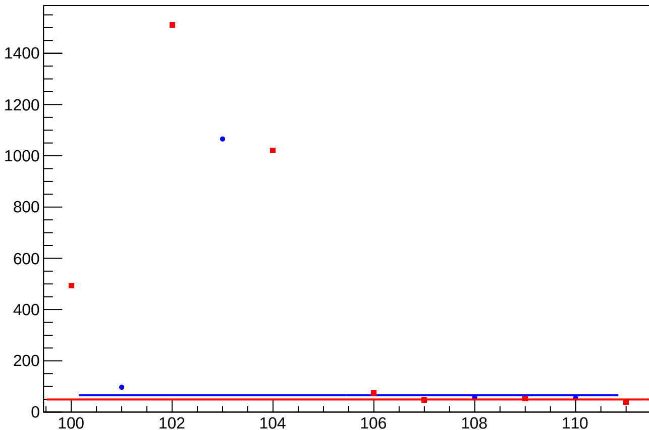
asym_us_avg_at1lr_avg_dd_eigen_dit_vs_eigen_cor_diff_rms vs Slug
