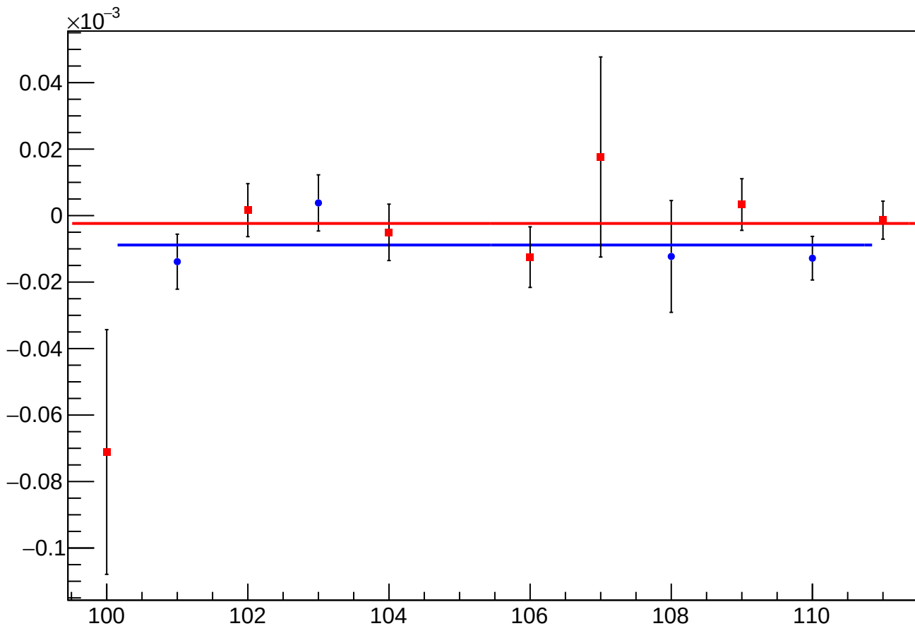
asym_us_dd_atlr_dd_dd_eigen_dit_vs_dit_diff_mean vs Slug
