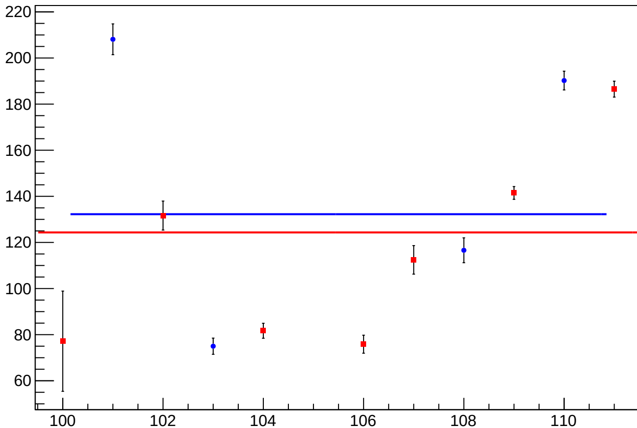
reg_asym_usr_atr2_dd_diff_bpm1X_slope vs Slug
