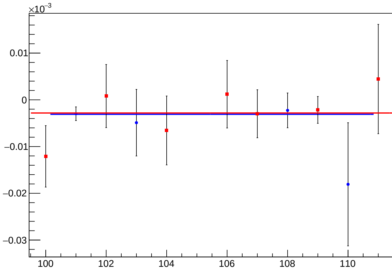
asym_sam_26_48_dd_eigen_dit_vs_dit_diff_mean vs Slug
