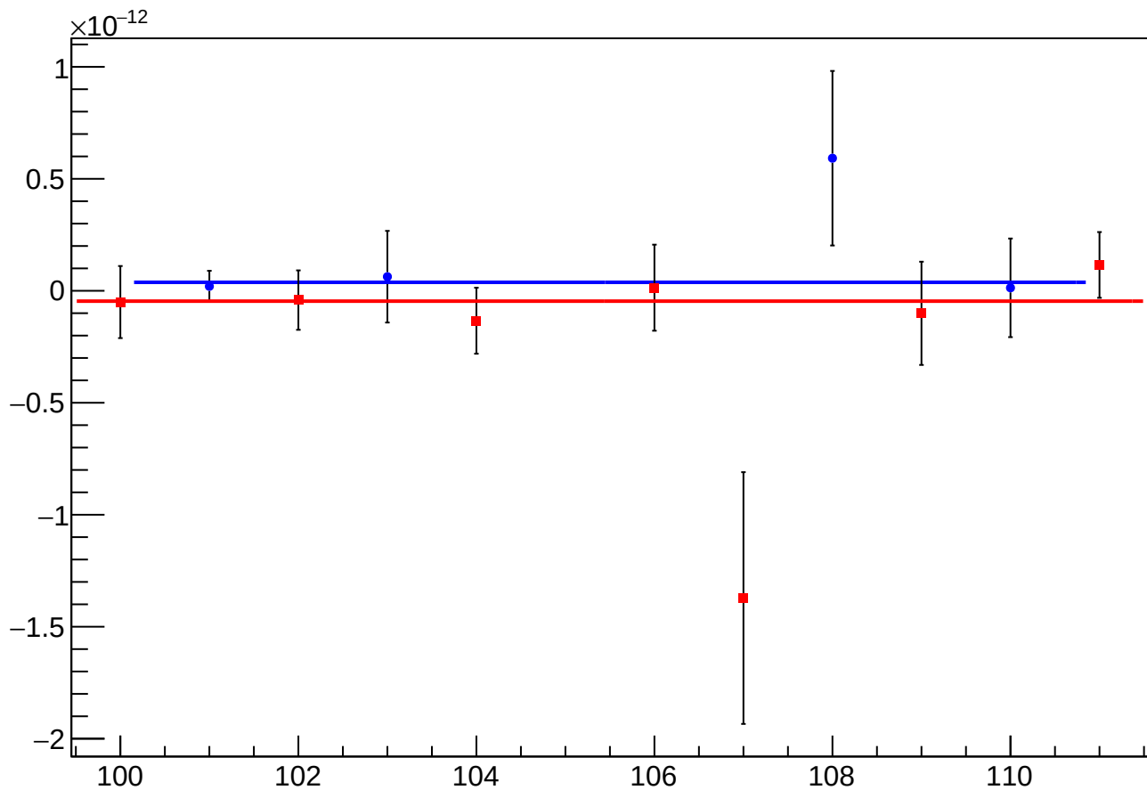
asym_us_dd_at1lr_dd_dd_reg_vs_cor_diff_mean vs Slug
