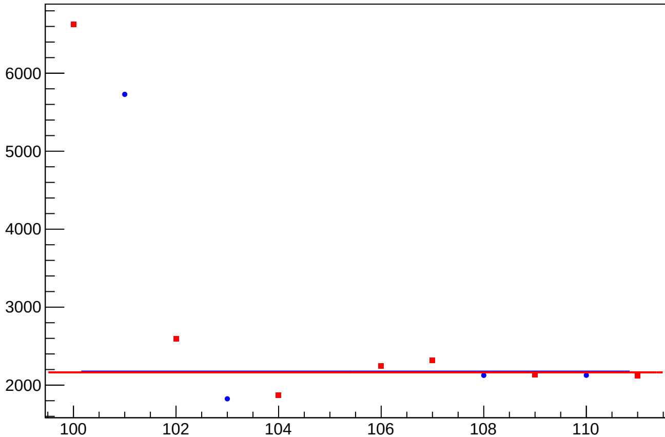
cor_asym_us_dd_at1lr_dd_dd_rms vs Slug
