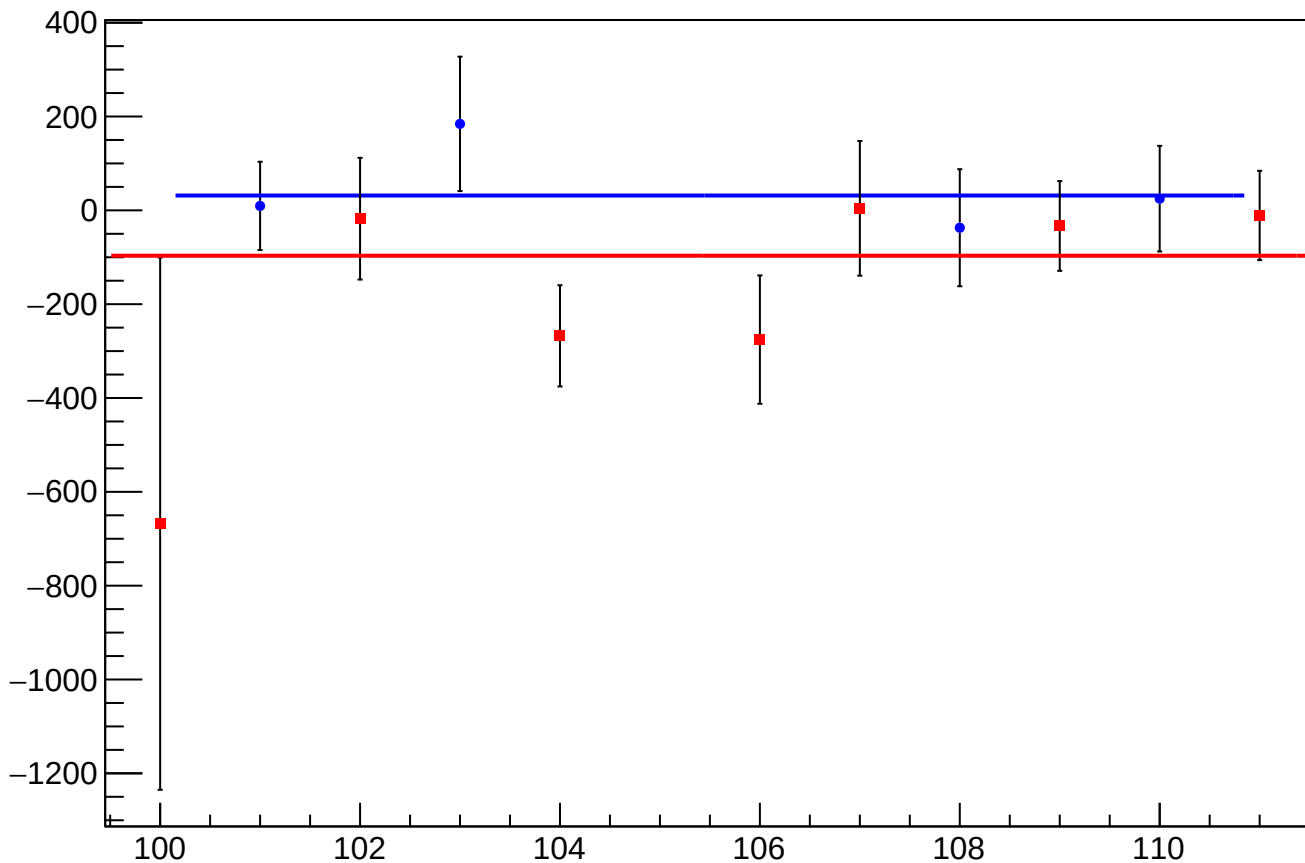
eigen_dit_asym_sam_1548_avg_mean vs Slug
