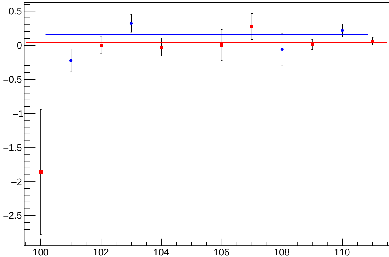
asym_sam4_dit_vs_cor_diff_mean vs Slug
