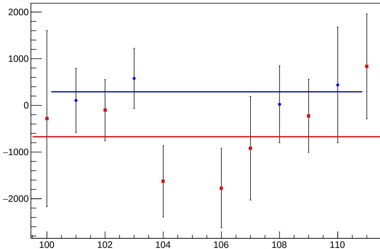
asym_sam5_reg_correction_mean vs Slug
