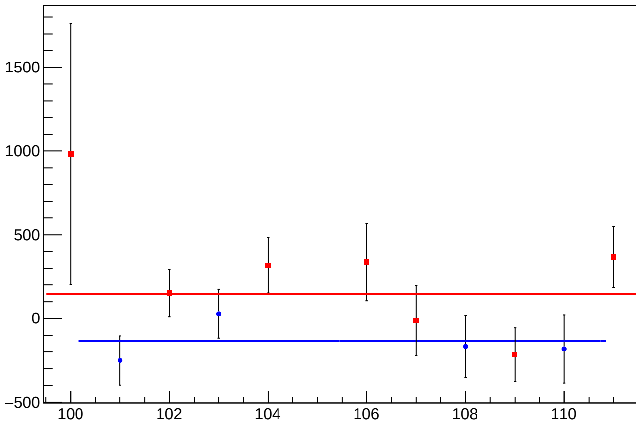
dit_asym_sam_37_26_dd_mean vs Slug
