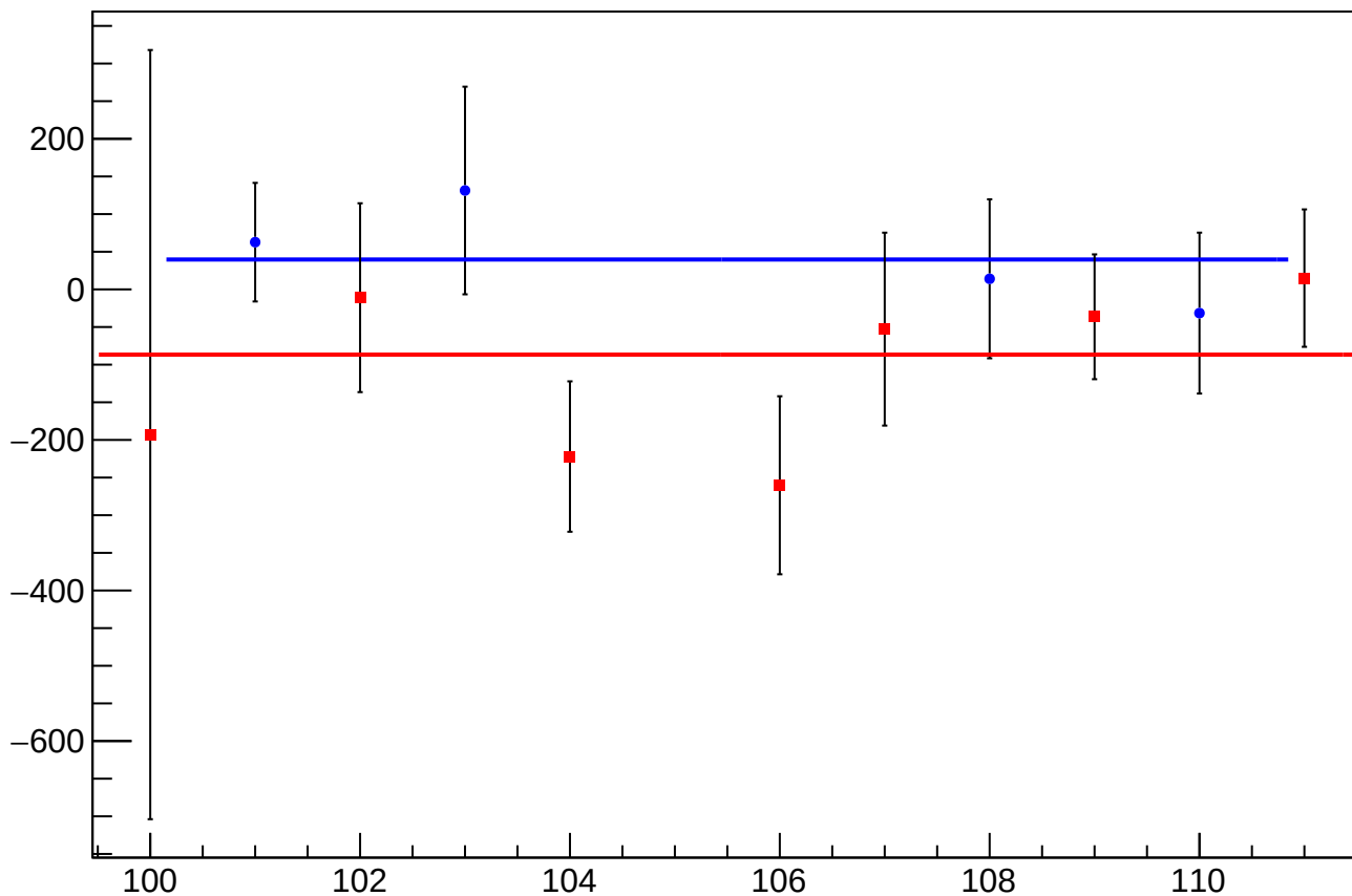
eigen_cor_asym_sam_1548_avg_mean vs Slug
