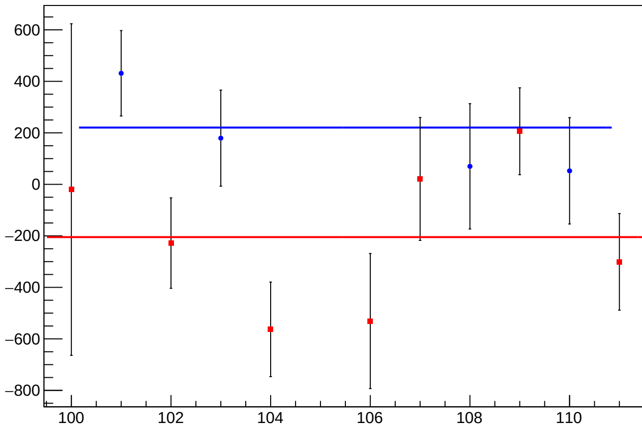
eigen_dit_asym_sam_24_68_dd_mean vs Slug
