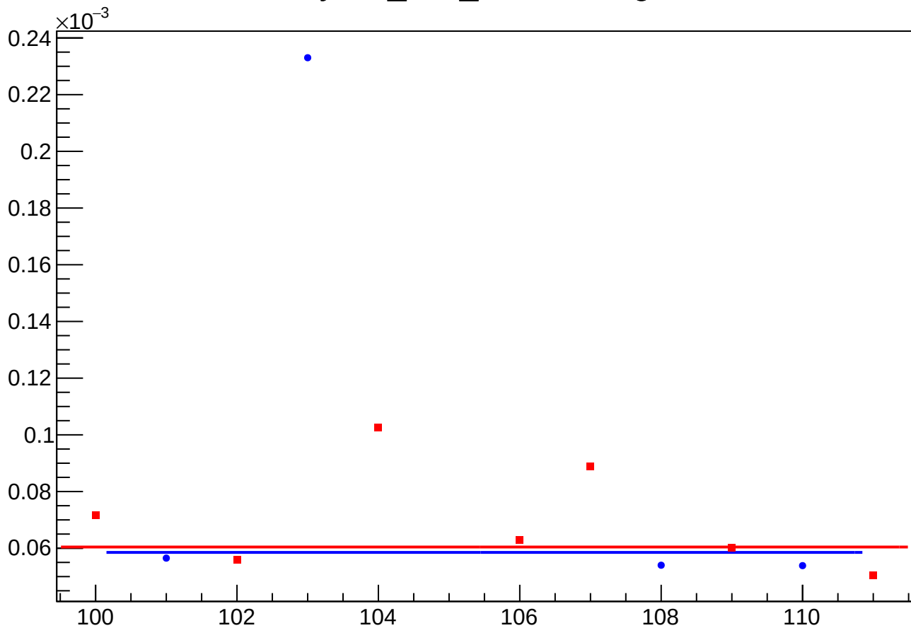
yield_atl1_rms vs Slug
