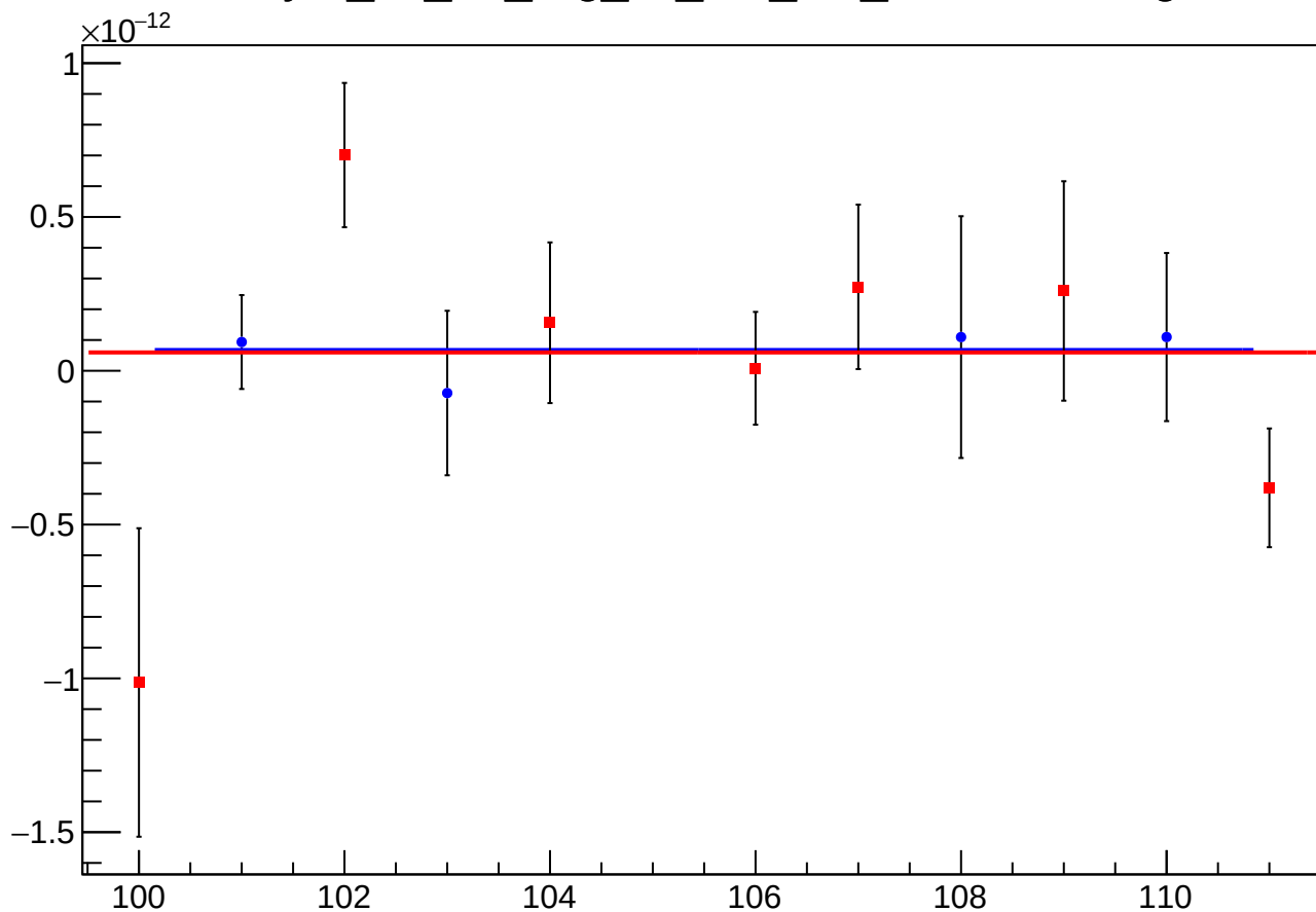
asym_atl_dd_reg_vs_cor_diff_mean vs Slug
