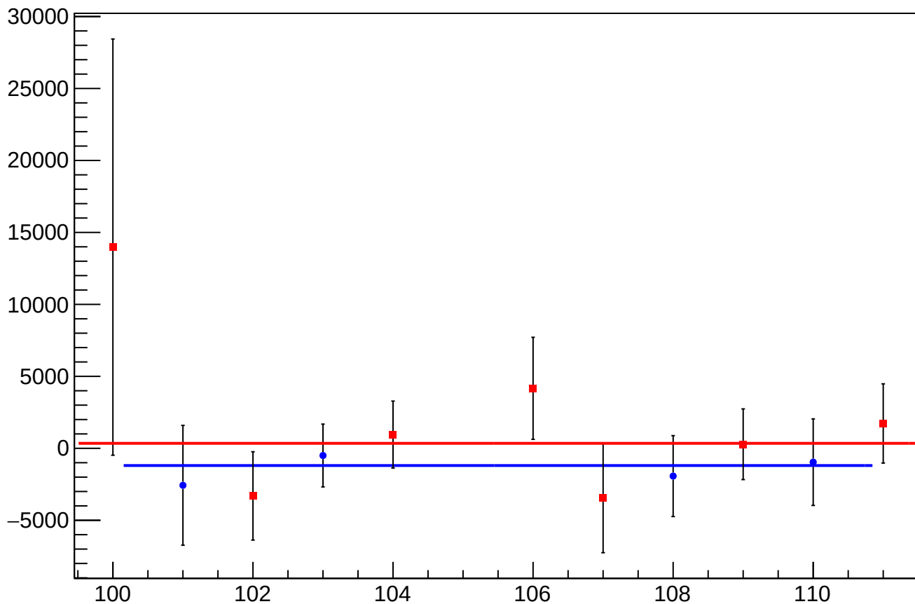
reg_asym_us_dd_atlr_dd_avg_mean vs Slug
