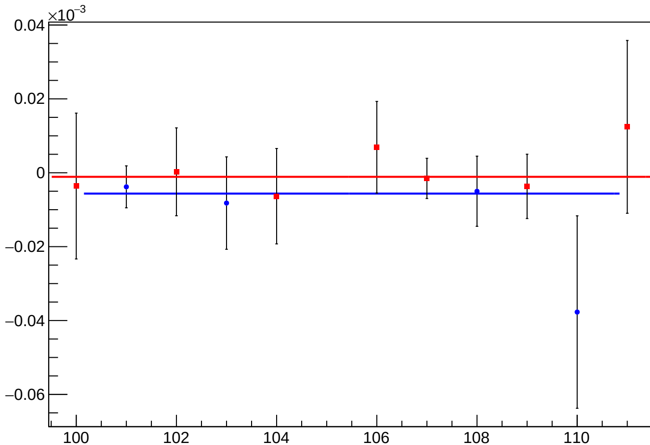
asym_sam_26_dd_eigen_dit_vs_dit_diff_mean vs Slug
