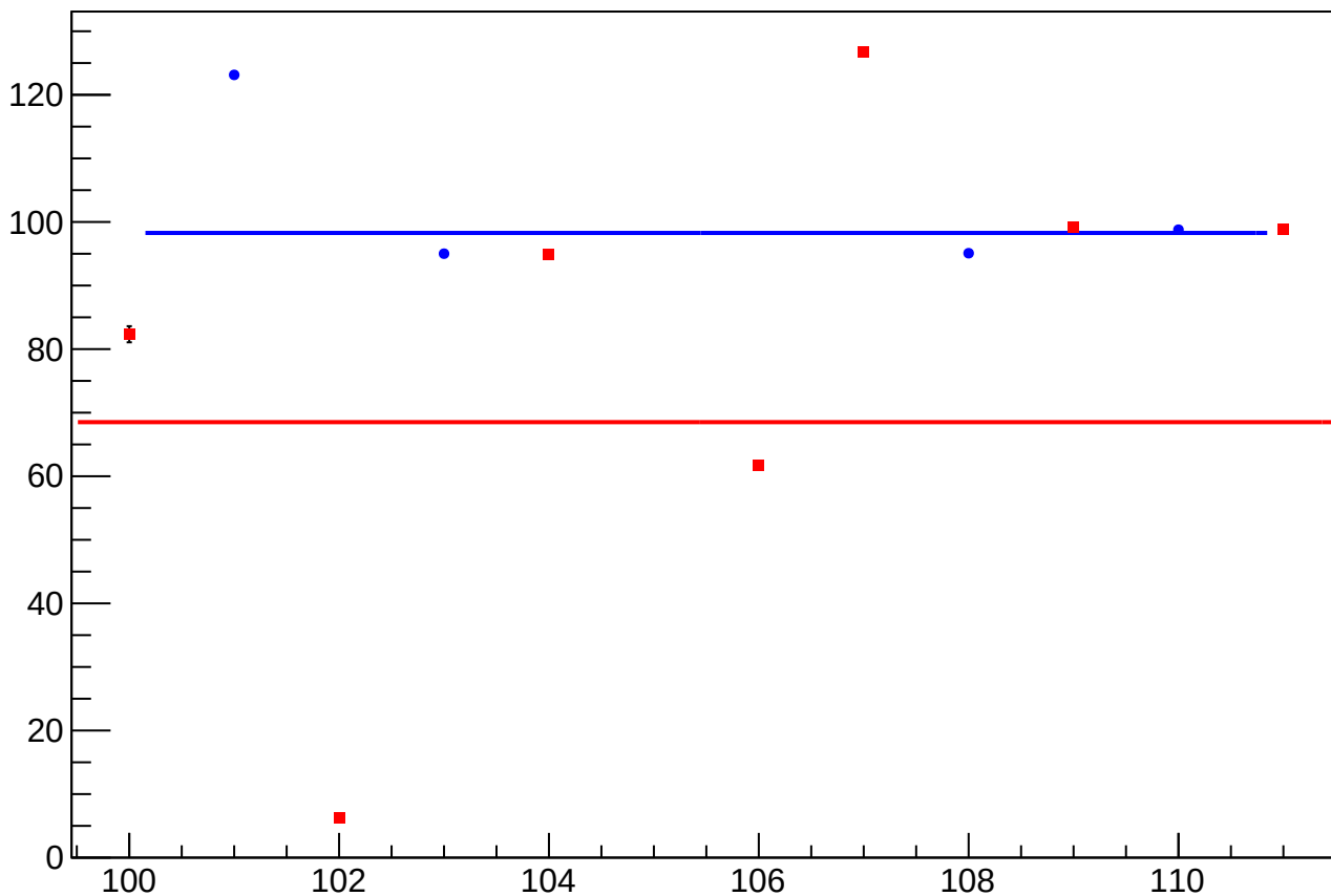
reg_asym_atr1l2_dd_diff_bpm12X_slope vs Slug
