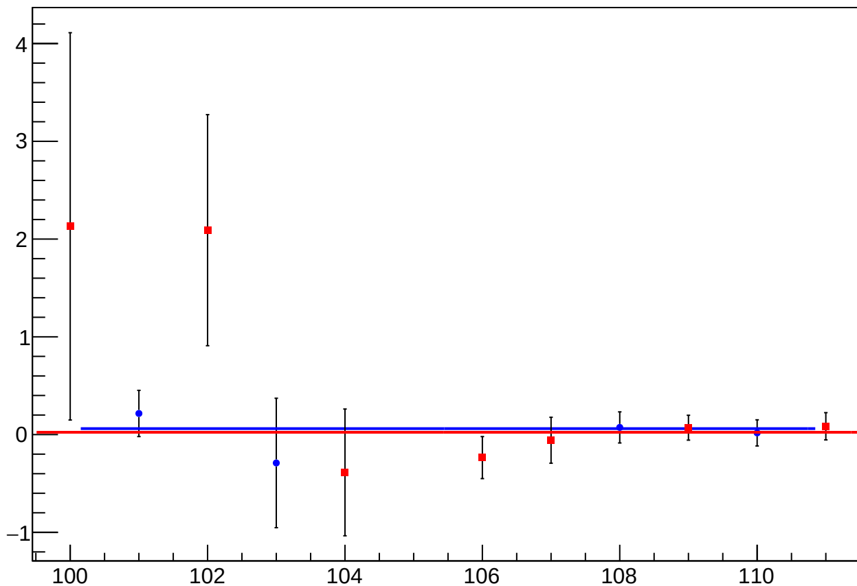
asym_atl_dd_dit_vs_cor_diff_mean vs Slug
