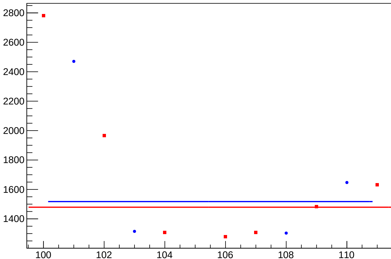
eigen_cor_asym_usr_atr2_avg_rms vs Slug
