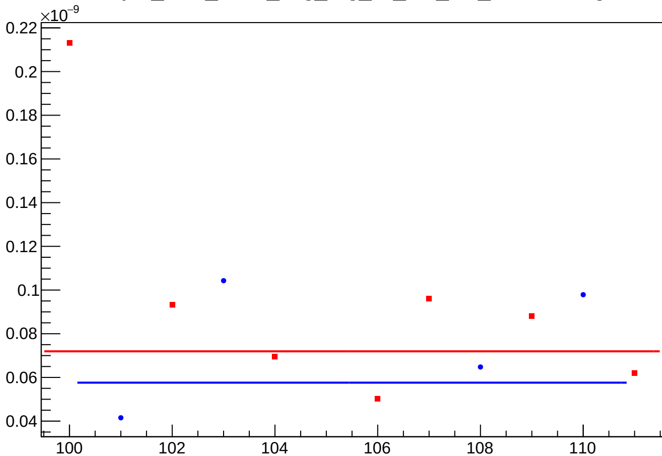
asym_sam_3726_avg_reg_vs_cor_diff_rms vs Slug
