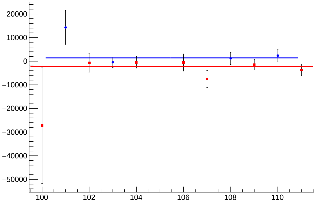
eigen_dit_asym_atr1l2_avg_mean vs Slug
