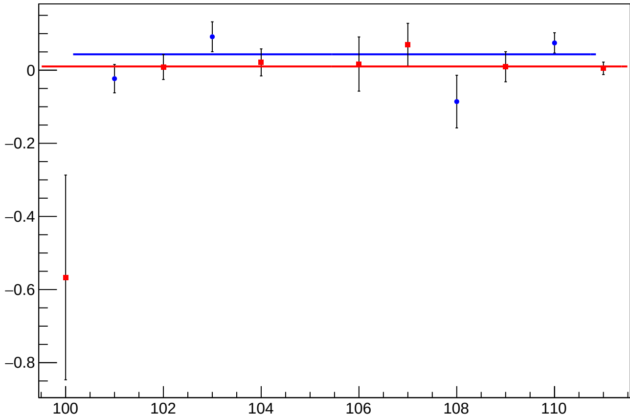
asym_sam8_eigen_dit_vs_eigen_cor_diff_mean vs Slug
