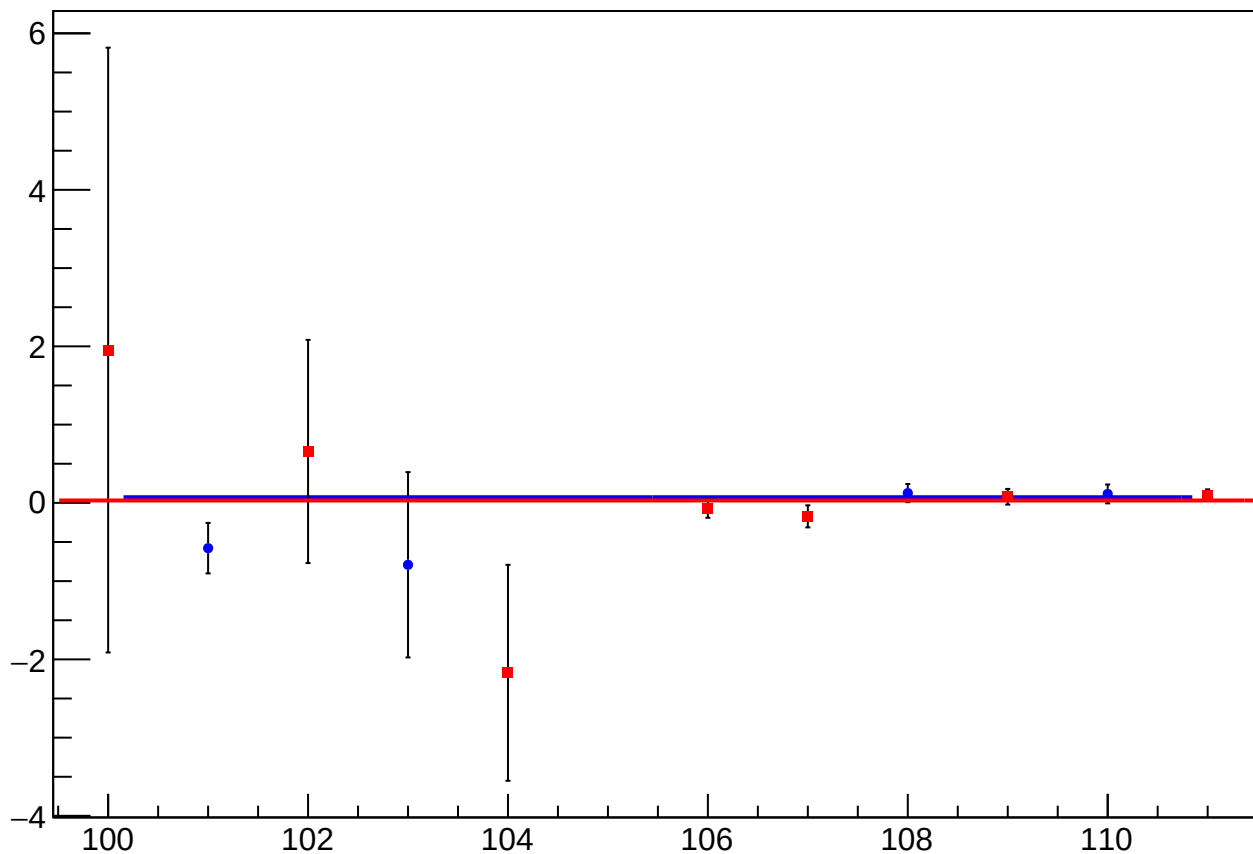
asym_atr1_eigen_dit_vs_cor_diff_mean vs Slug
