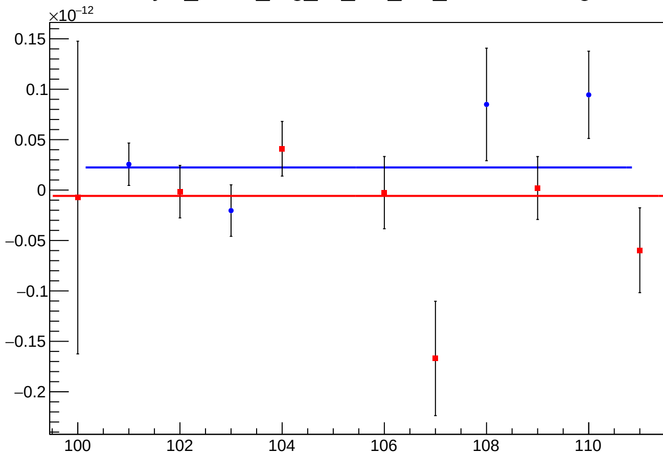
asym_sam8_reg_vs_cor_diff_mean vs Slug
