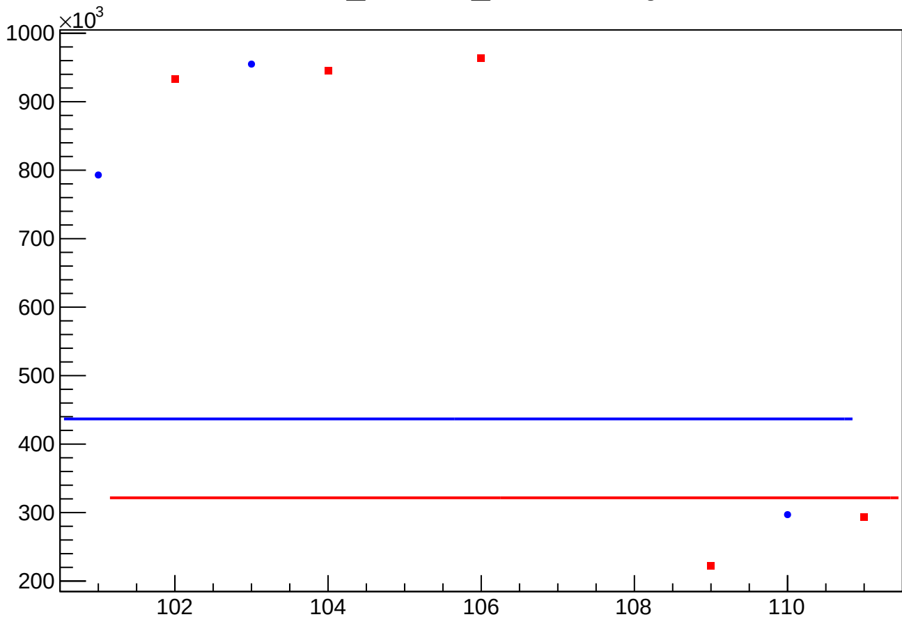
diff_cav4cY_rms vs Slug
