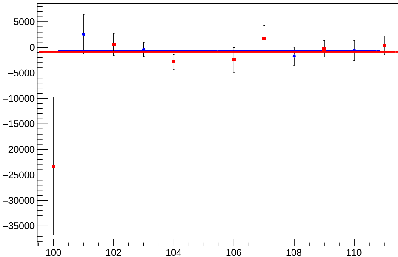
cor_asym_us_dd_atlr_dd_dd_mean vs Slug
