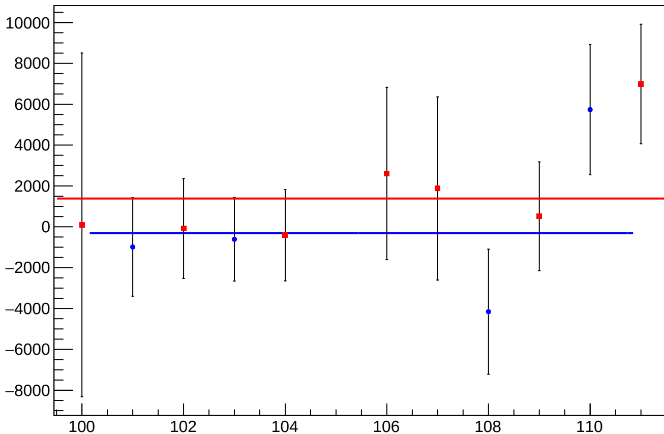
eigen_cor_asym_atl_dd_mean vs Slug
