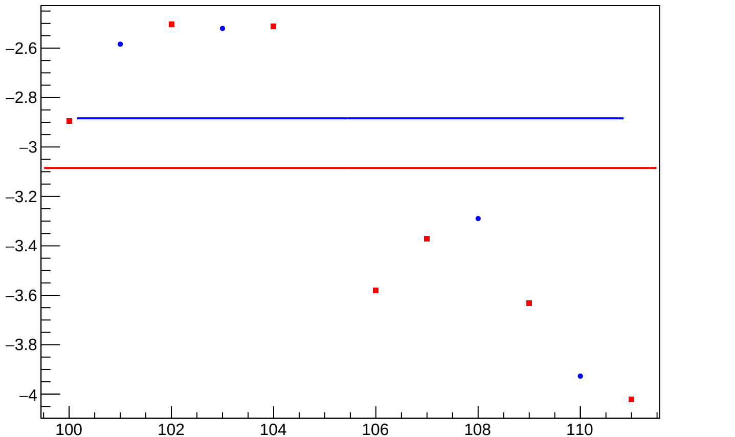
yield_bpm0i02Y_mean vs Slug
