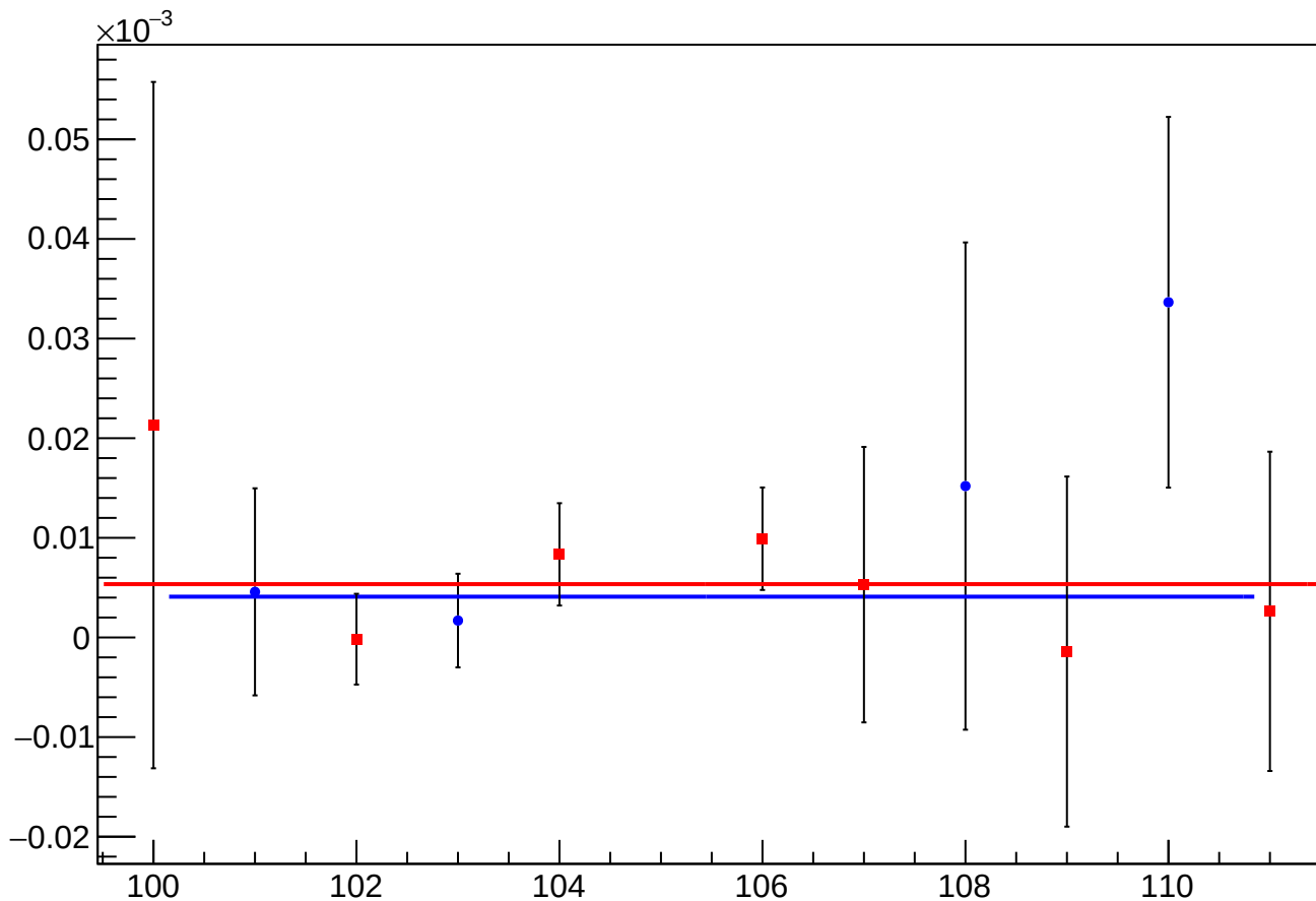
asym_atr1l2_avg_eigen_dit_vs_dit_diff_mean vs Slug
