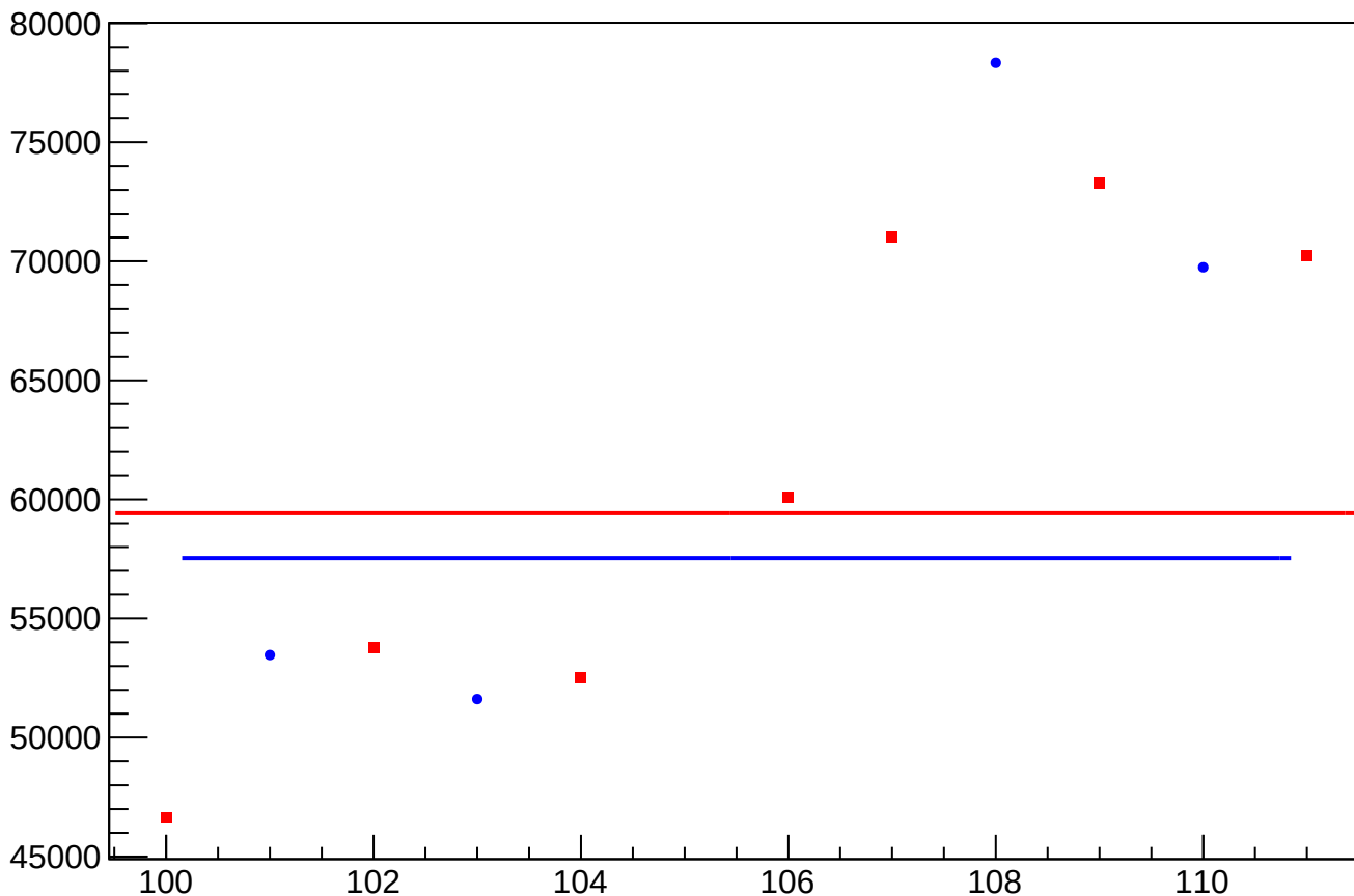
diff_bpm0r03X_rms vs Slug
