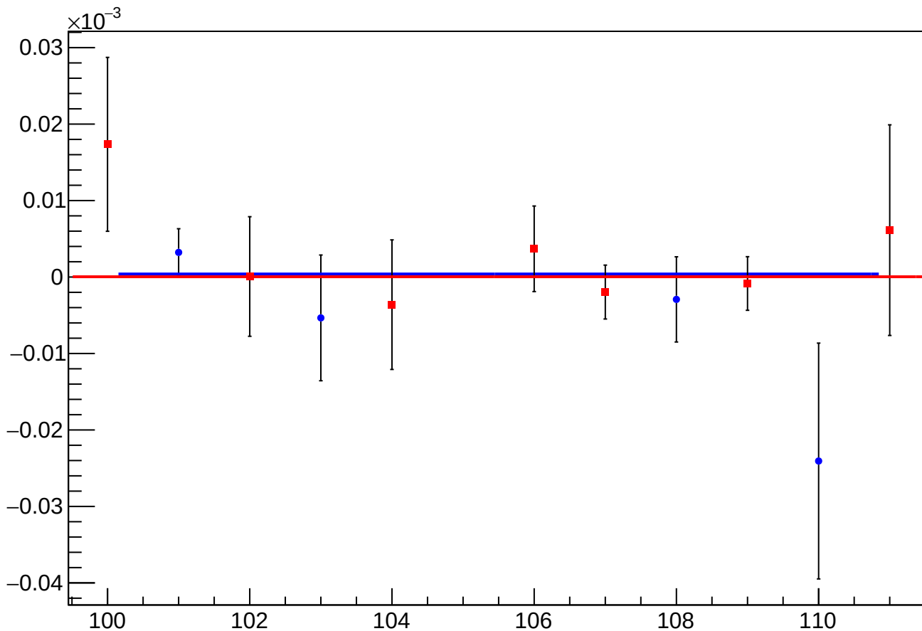
asym_sam_3726_avg_eigen_dit_vs_dit_diff_mean vs Slug
