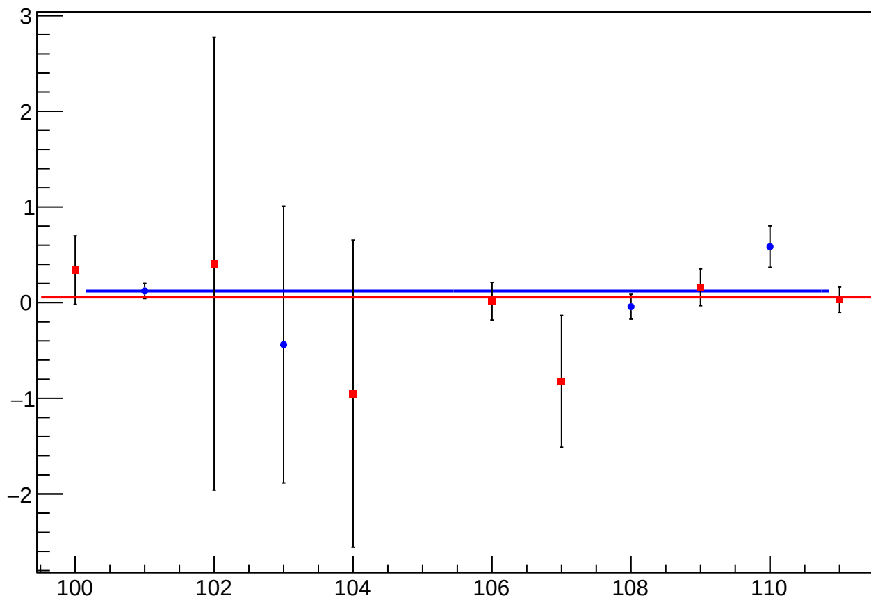
asym_atl1_dit_vs_cor_diff_mean vs Slug
