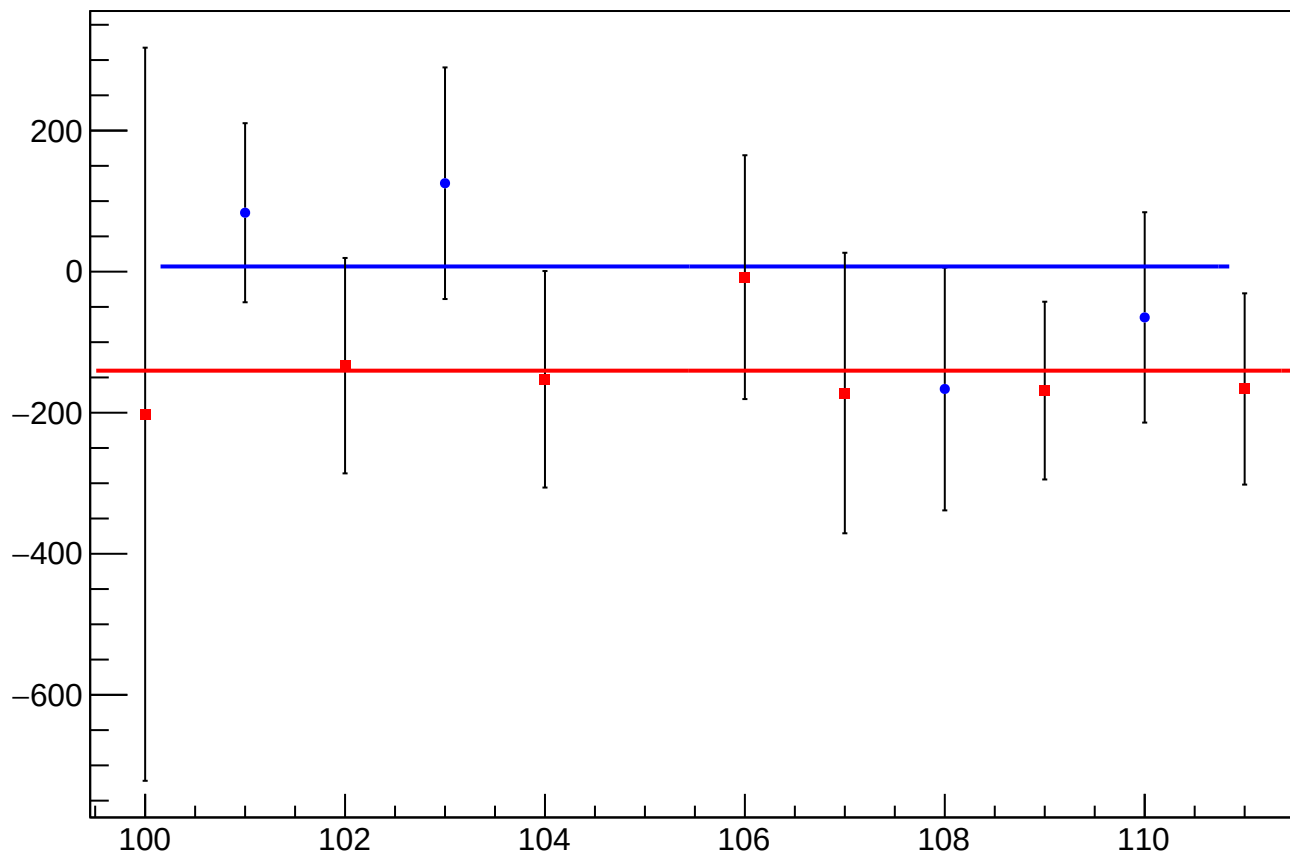
eigen_cor_asym_sam_48_dd_mean vs Slug
