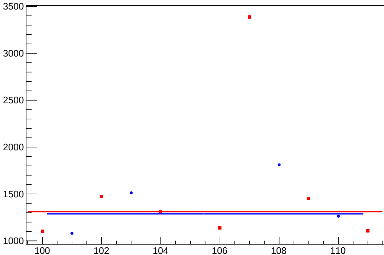
asym_usl_reg_correction_rms vs Slug
