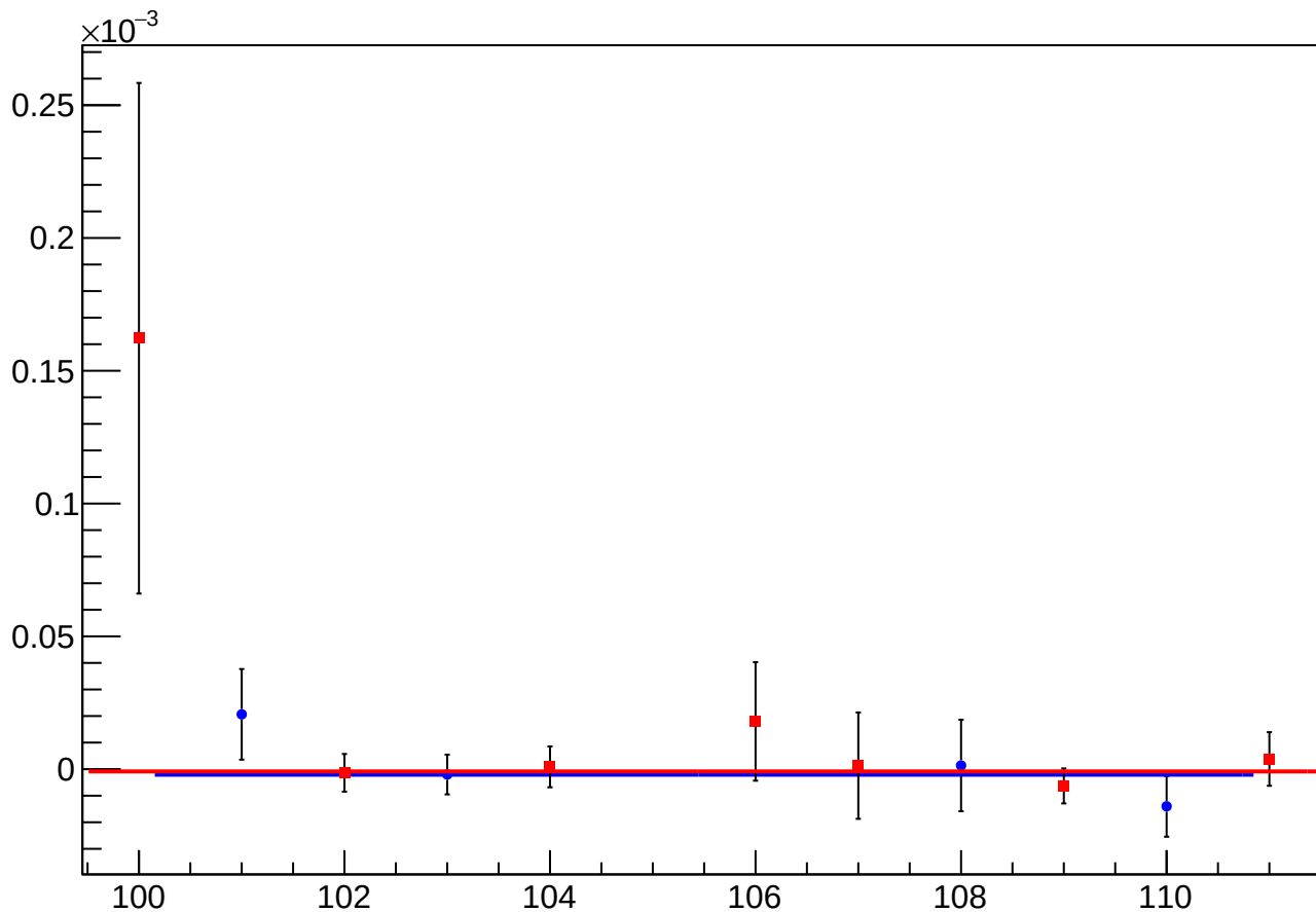
asym_usr_atr2_dd_eigen_dit_vs_dit_diff_mean vs Slug
