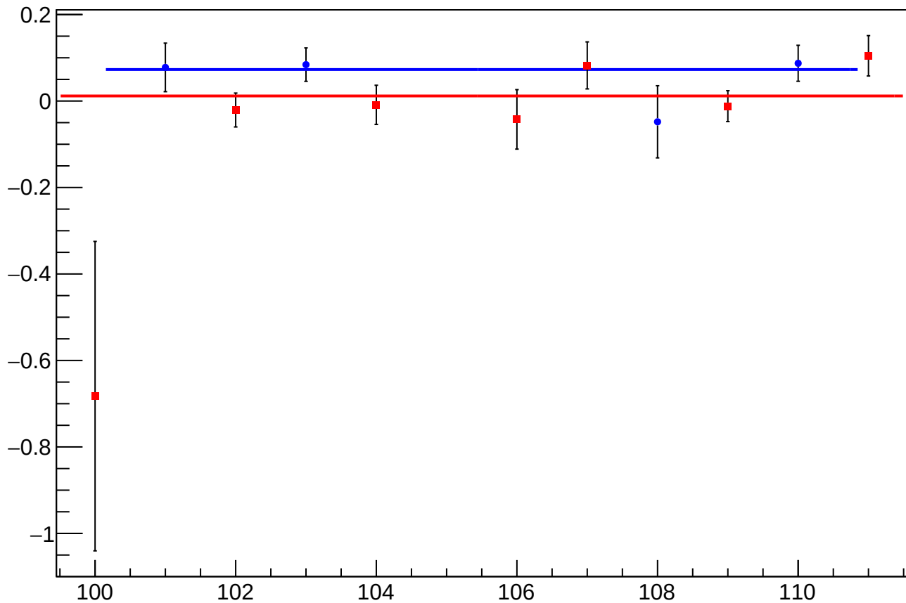
asym_sam6_dit_vs_cor_diff_mean vs Slug
