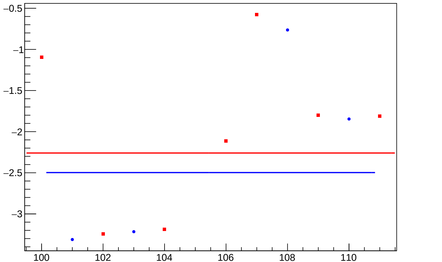
yield_bpm0r03X_mean vs Slug
