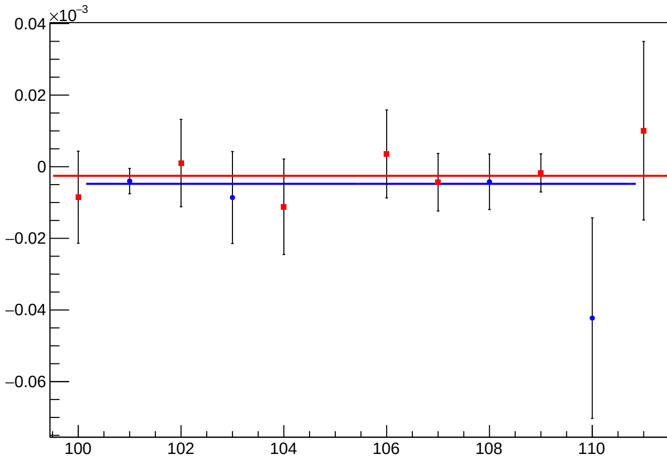
asym_sam_26_avg_eigen_dit_vs_dit_diff_mean vs Slug
