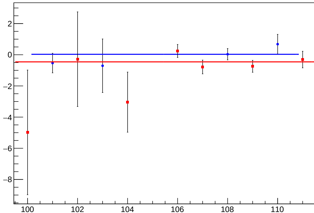
asym_atr2_dit_vs_eigen_cor_diff_mean vs Slug
