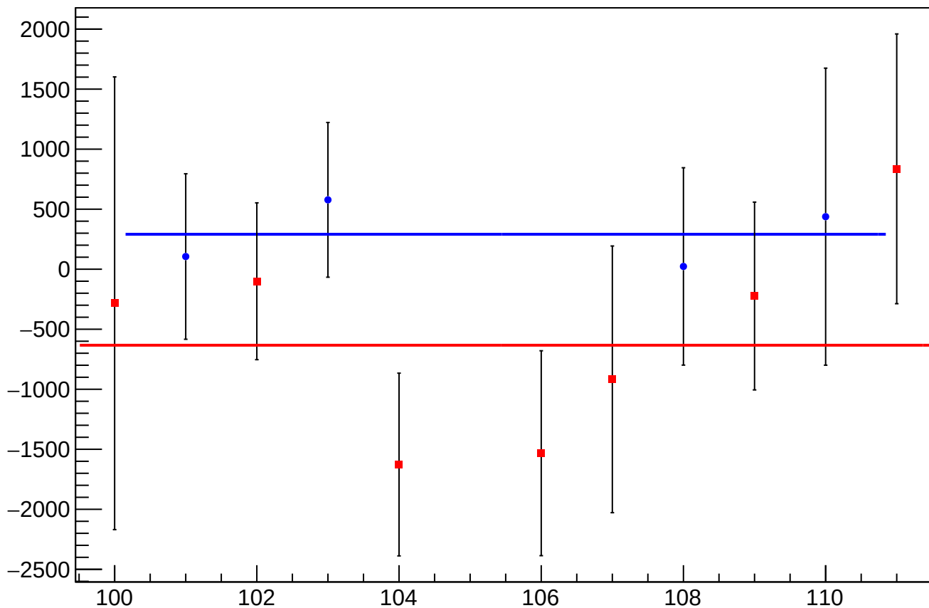
asym_sam5_cor_correction_mean vs Slug
