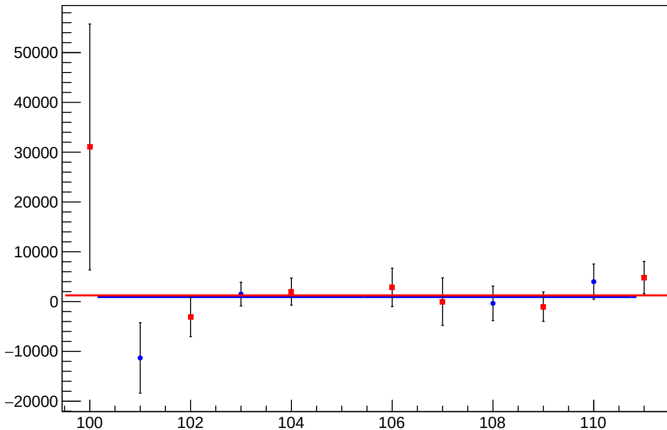
eigen_dit_asym_at1_dd_mean vs Slug
