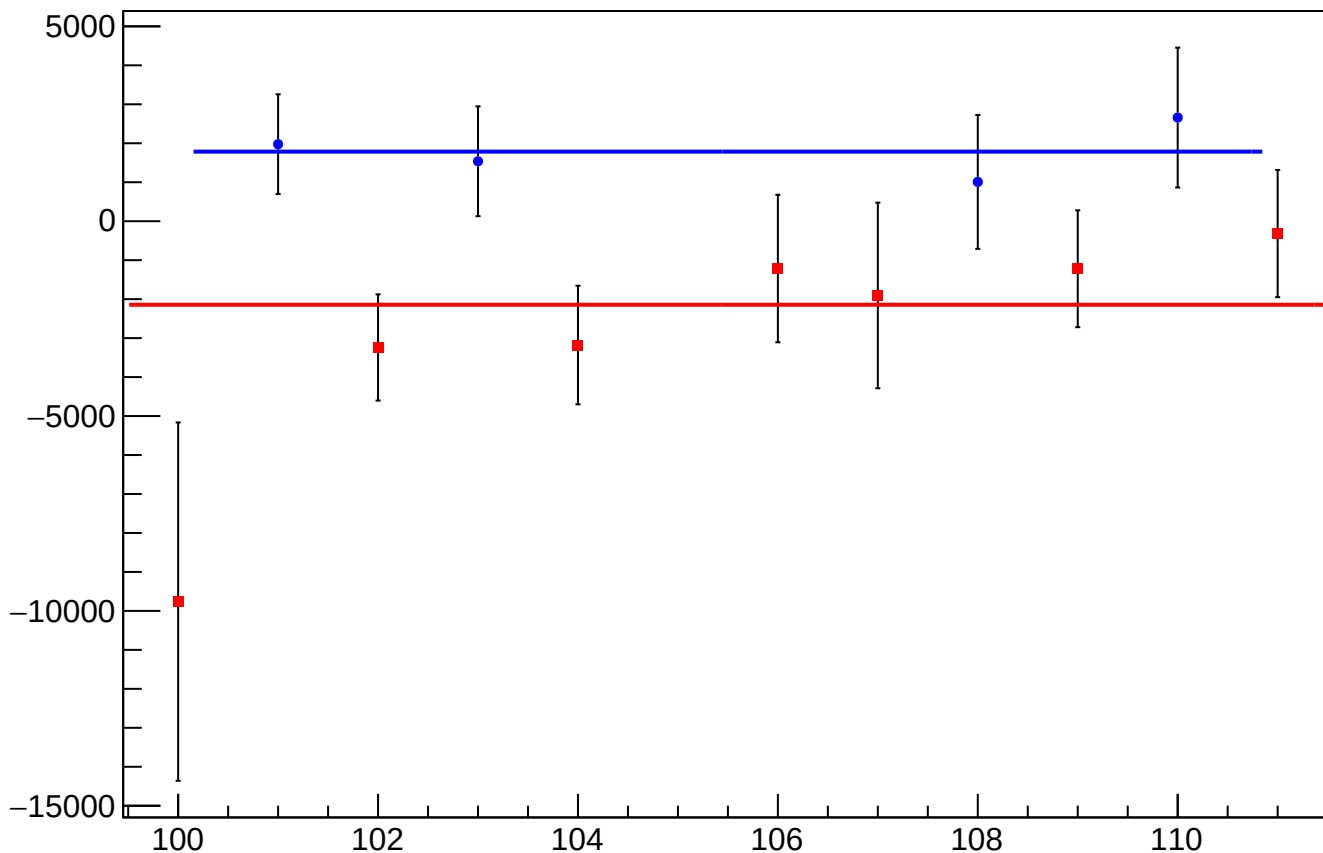
eigen_dit_asym_usl_mean vs Slug
