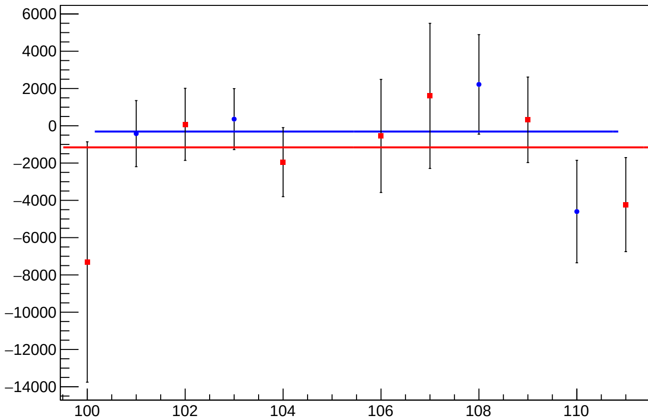
eigen_cor_asym_usl_atl1_dd_mean vs Slug
