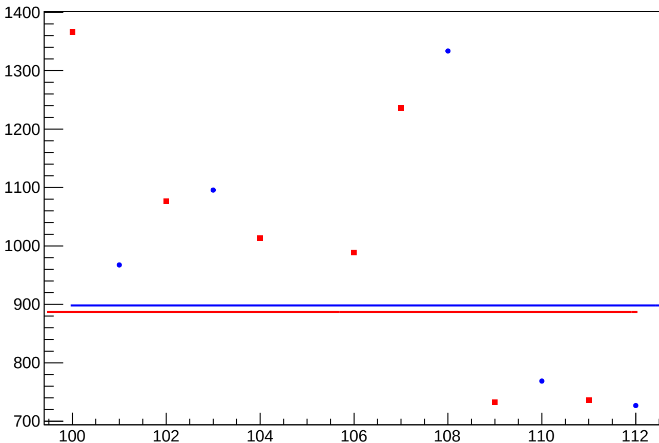
asym_sam_3748_avg_dit_correction_rms vs Slug, Sign Corrected
