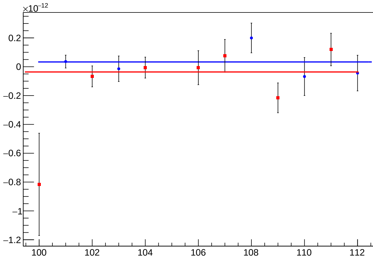
asym_sam_26_48_dd_reg_vs_cor_diff_mean vs Slug, Sign Corrected
