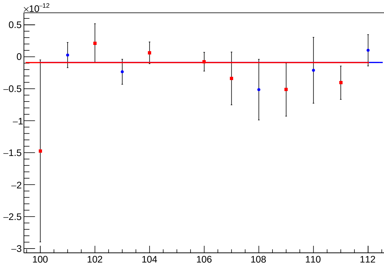
asym_atr1l2_avg_reg_vs_cor_diff_mean vs Slug, Sign Corrected
