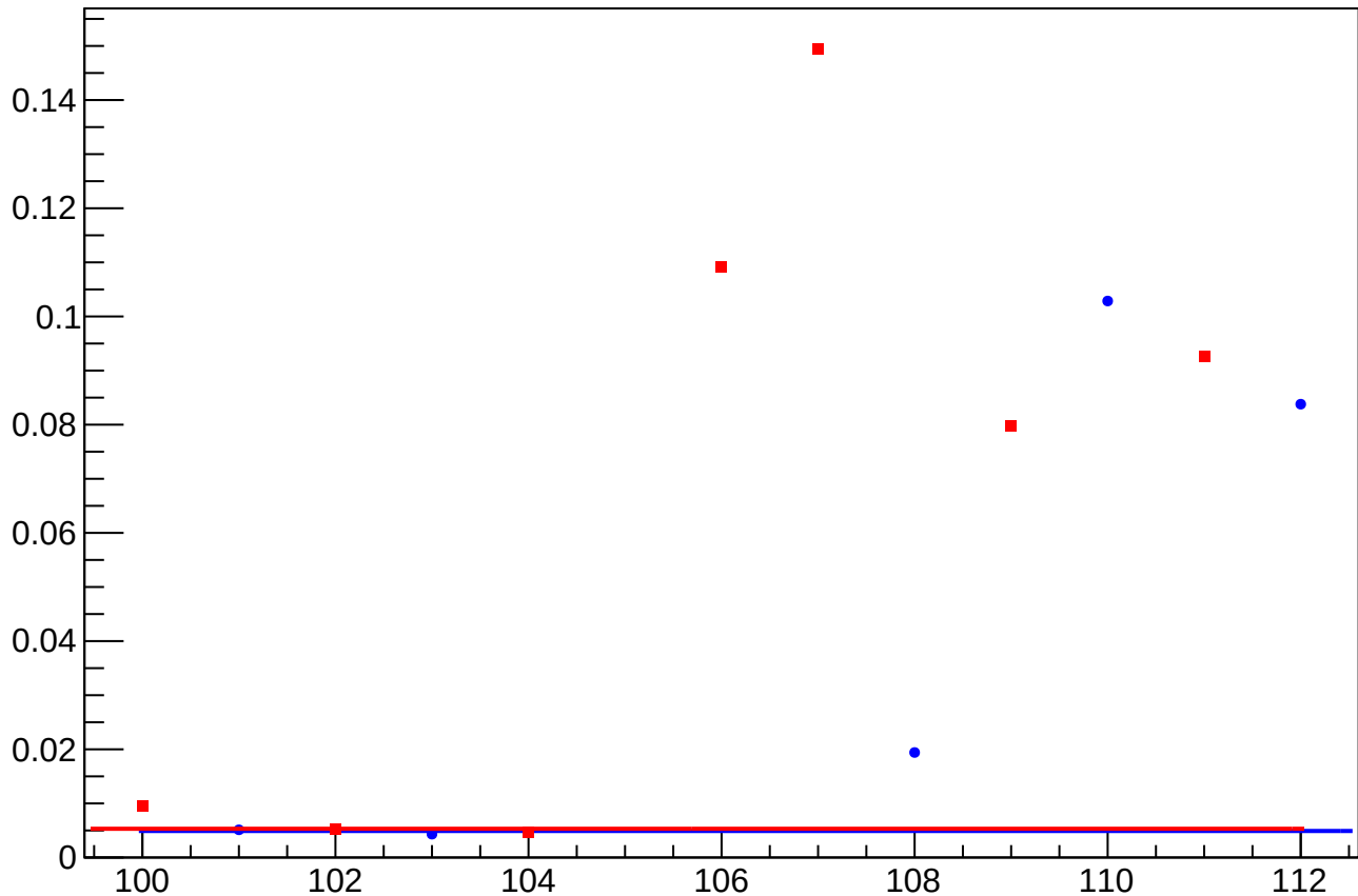
yield_bpm0l03X_rms vs Slug, Sign Corrected
