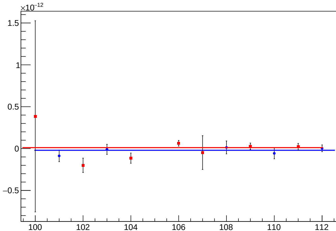
asym_atl1r2_dd_atl2r1_dd_avg_reg_vs_cor_diff_mean vs Slug, Sign Corrected
