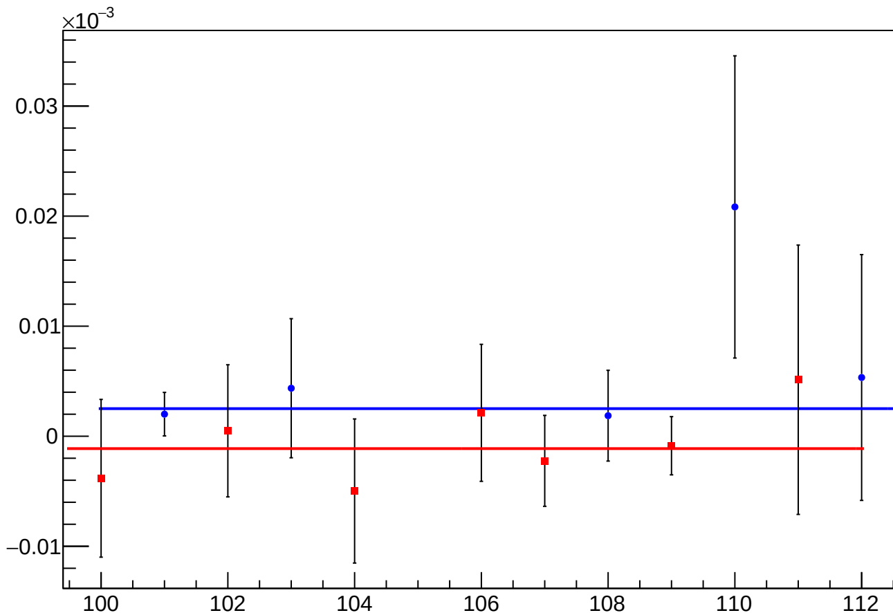
asym_sam_15_26_dd_eigen_dit_vs_dit_diff_mean vs Slug, Sign Corrected
