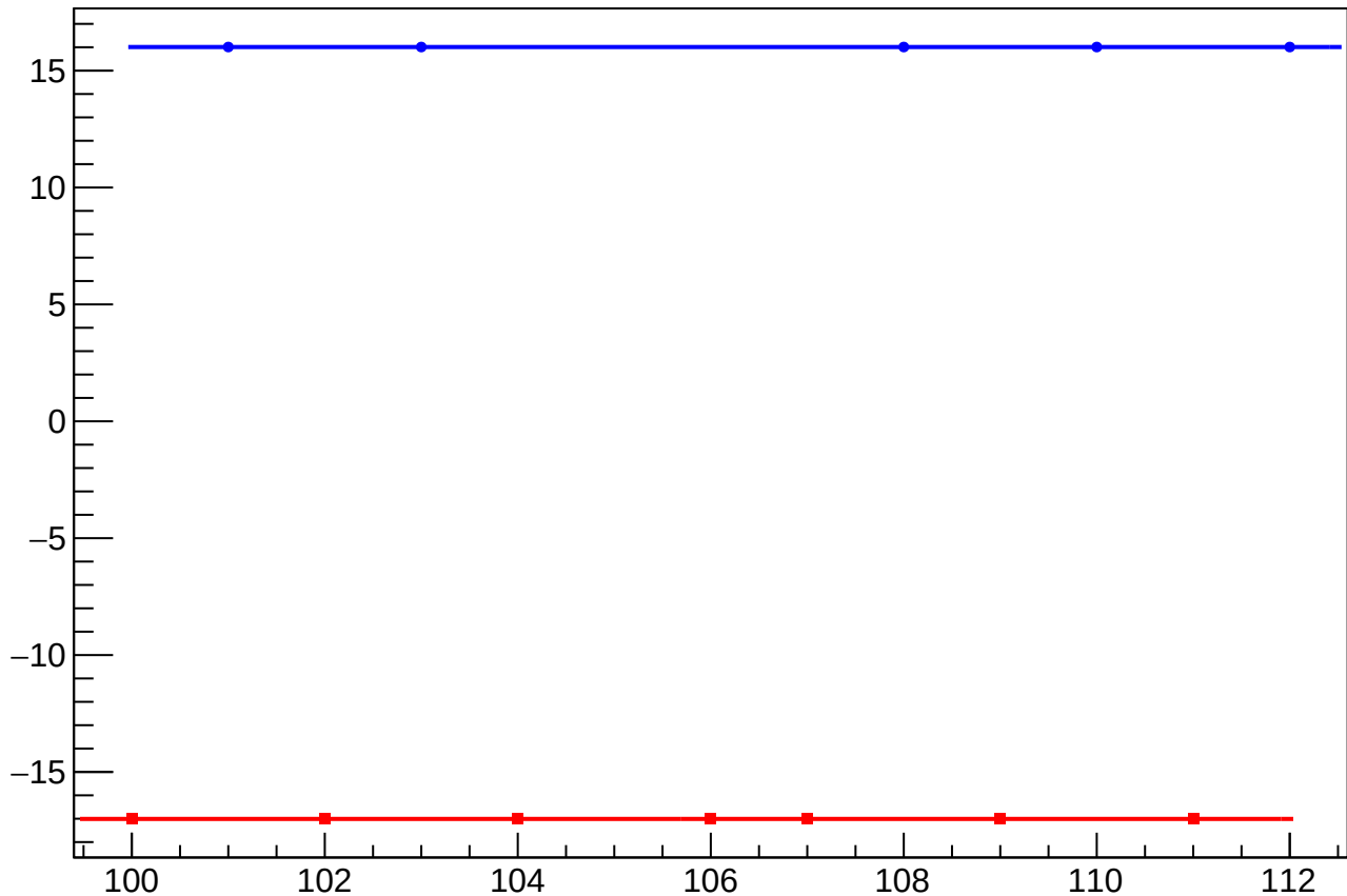
IGL1I00DI24_24M_mean vs Slug, Sign Corrected
