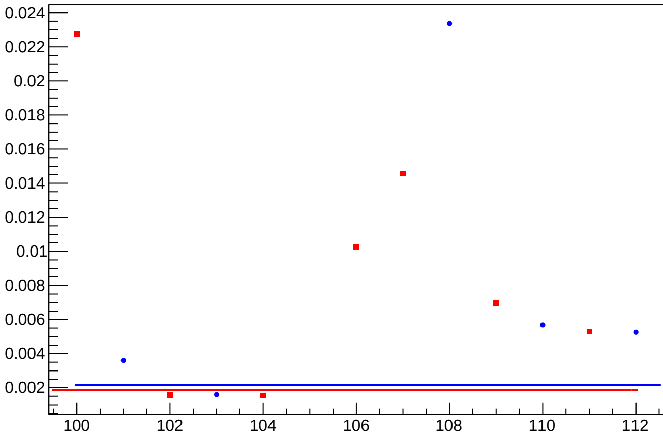
asym_us_dd_at2lr_dd_dd_eigen_dit_vs_dit_diff_rms vs Slug, Sign Corrected
