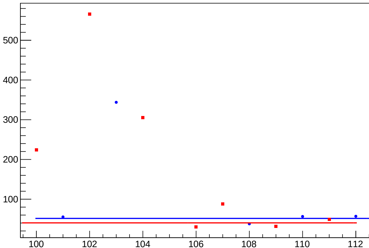
asym_at1_dd_at2_dd_avg_dit_vs_cor_diff_rms vs Slug, Sign Corrected
