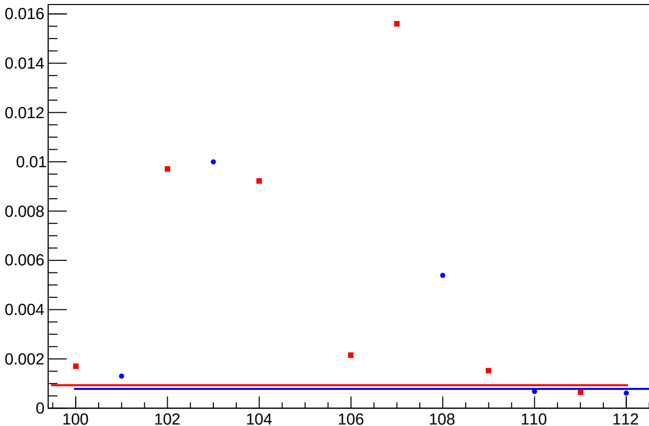
asym_usl_atl1_dd_eigen_dit_vs_dit_diff_rms vs Slug, Sign Corrected
