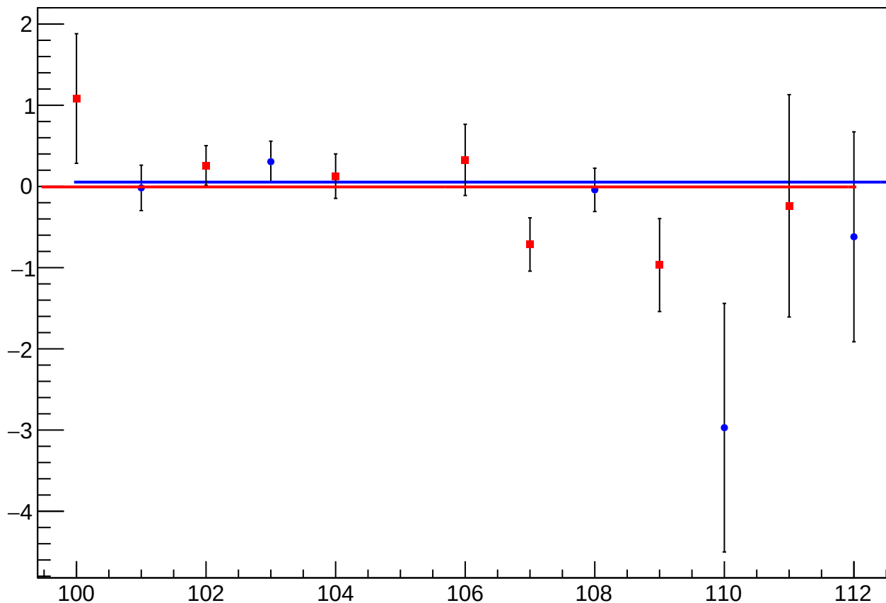
diff_targ_thetaX_mean vs Slug, Sign Corrected
