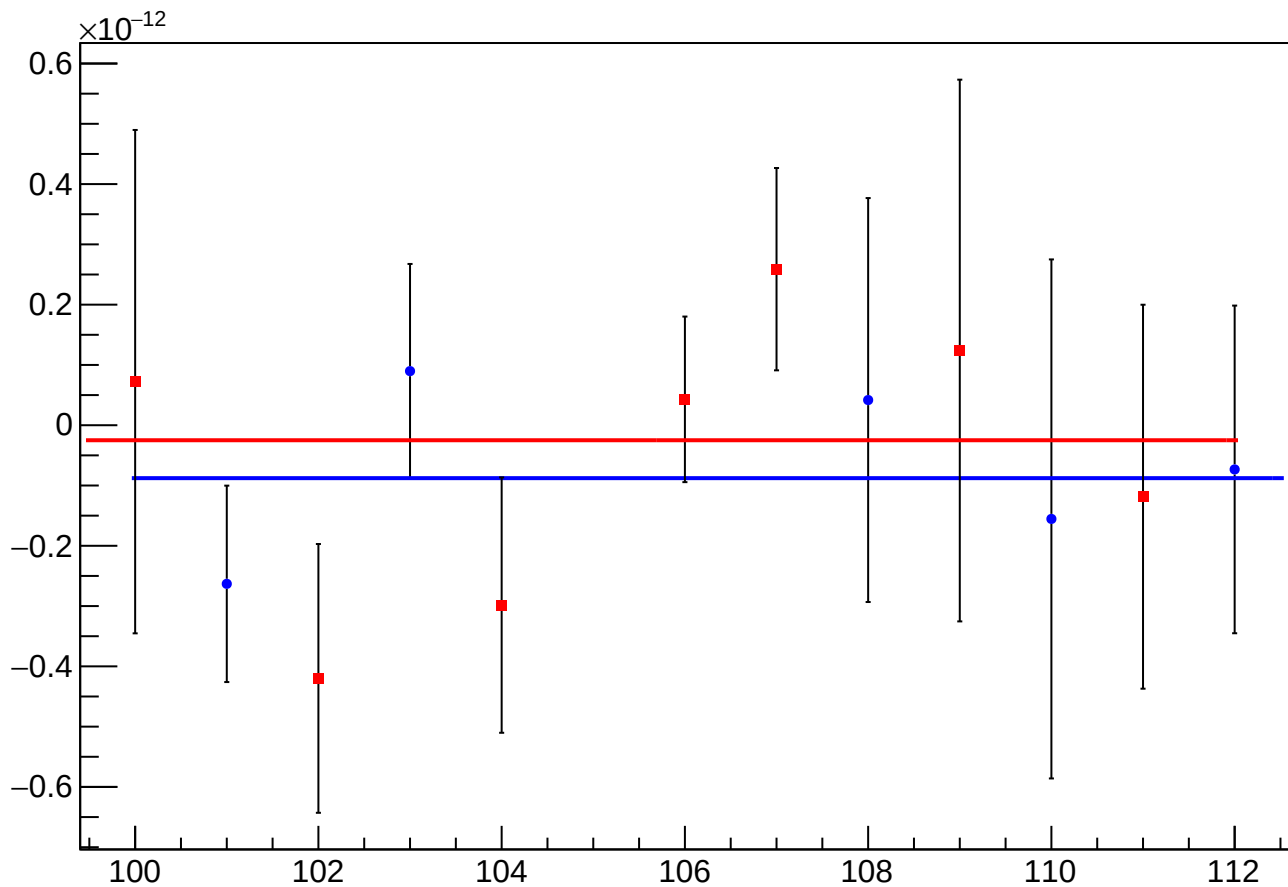
asym_atl_dd_atr_dd_avg_reg_vs_cor_diff_mean vs Slug, Sign Corrected
