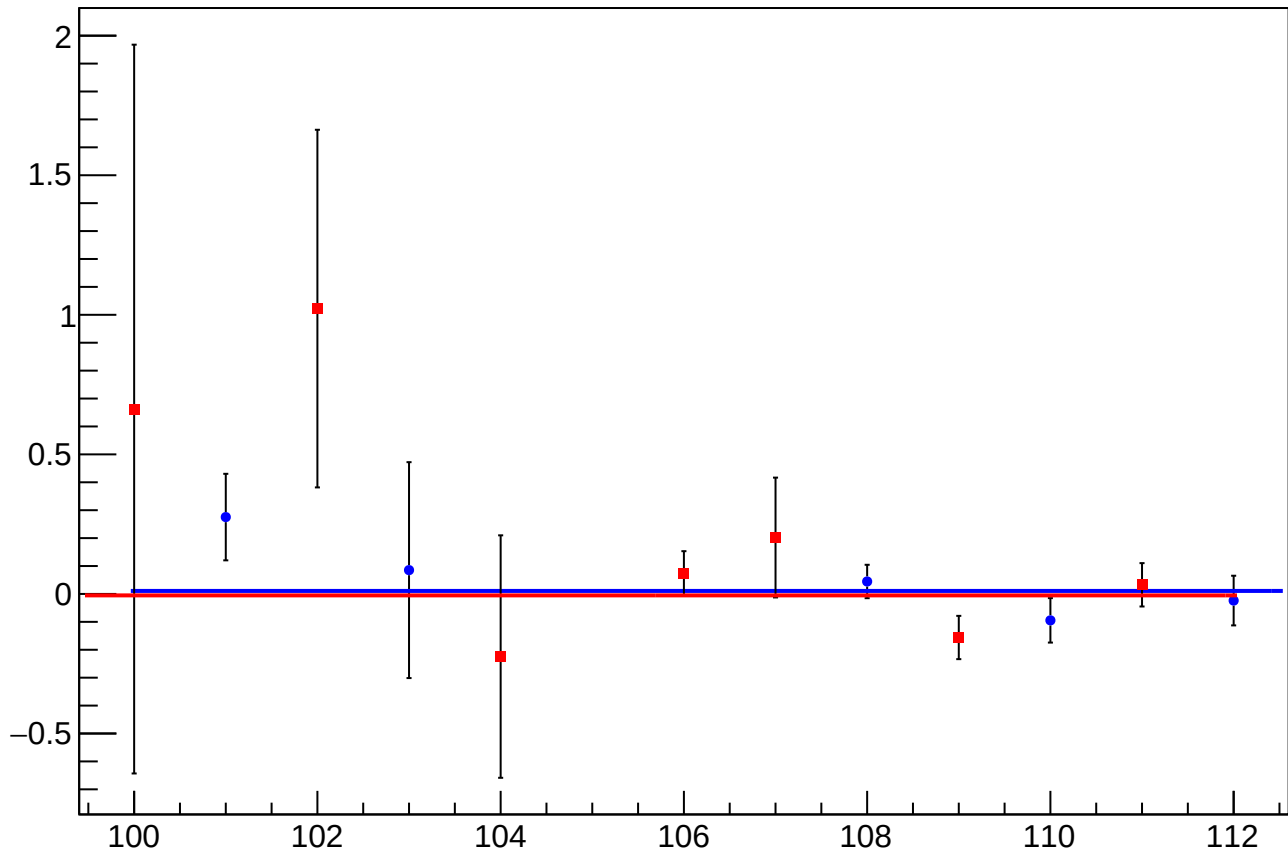
asym_us_dd_atlr_dd_avg_eigen_dit_vs_eigen_cor_diff_mean vs Slug, Sign Corrected
