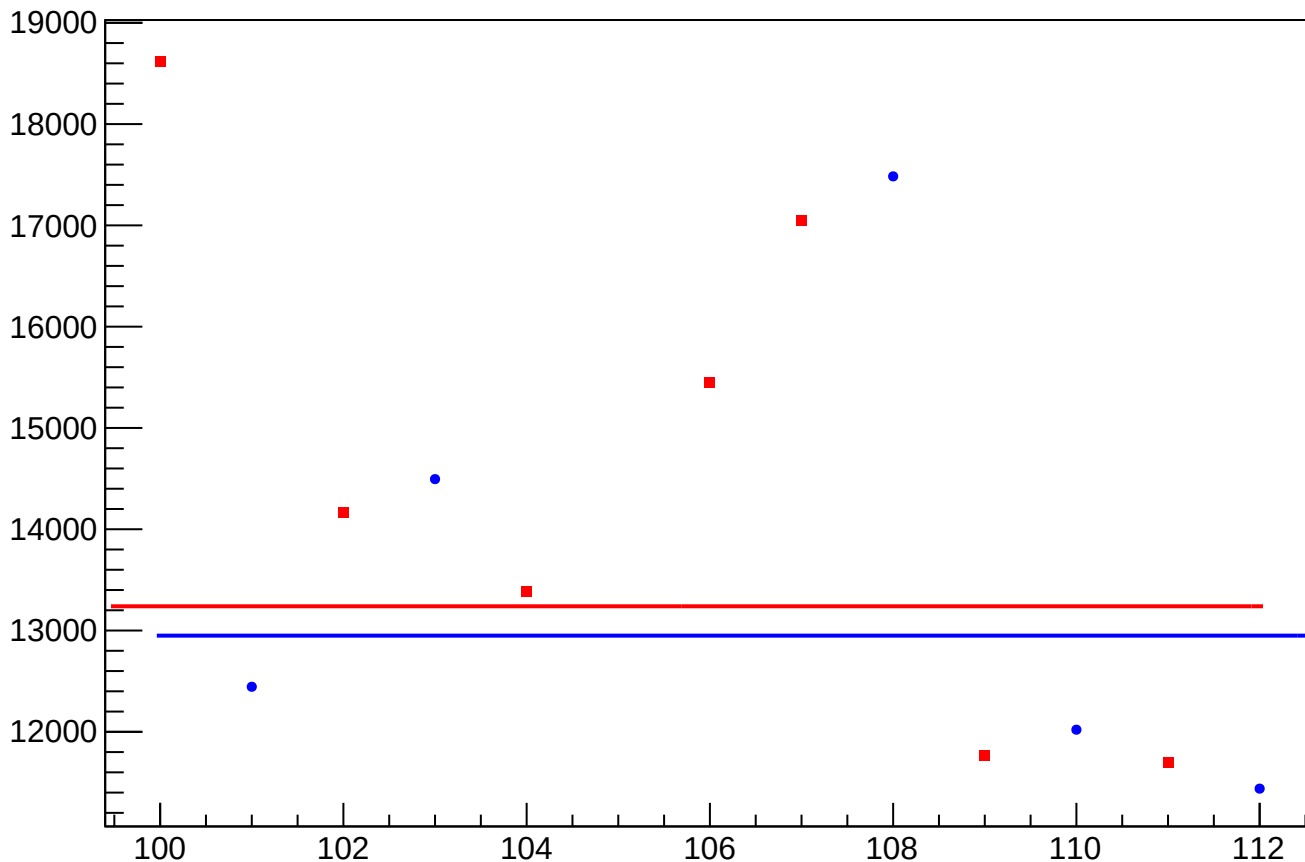
diff_bpm_4eX_4ecX_avg_rms vs Slug, Sign Corrected
