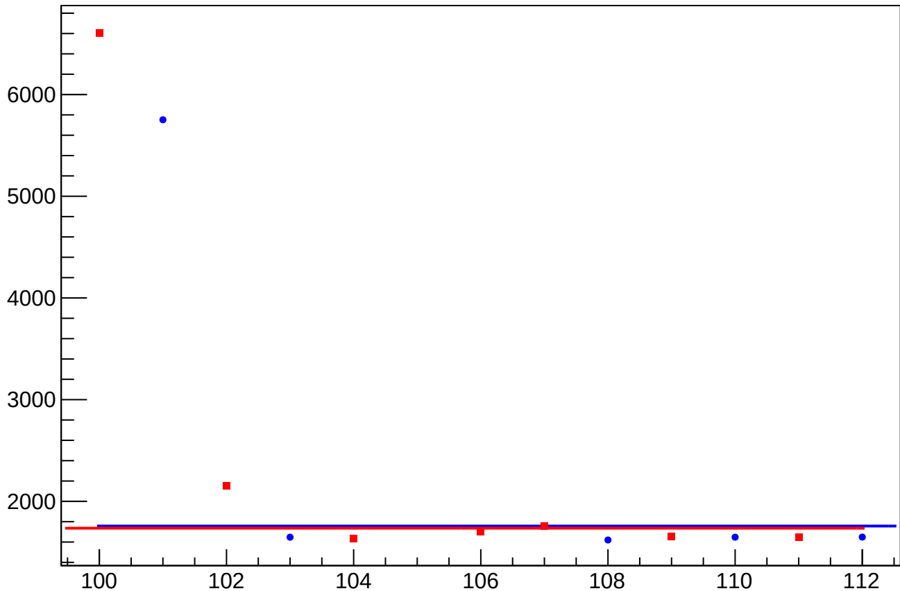
cor_asym_atr1l2_avg_rms vs Slug, Sign Corrected
