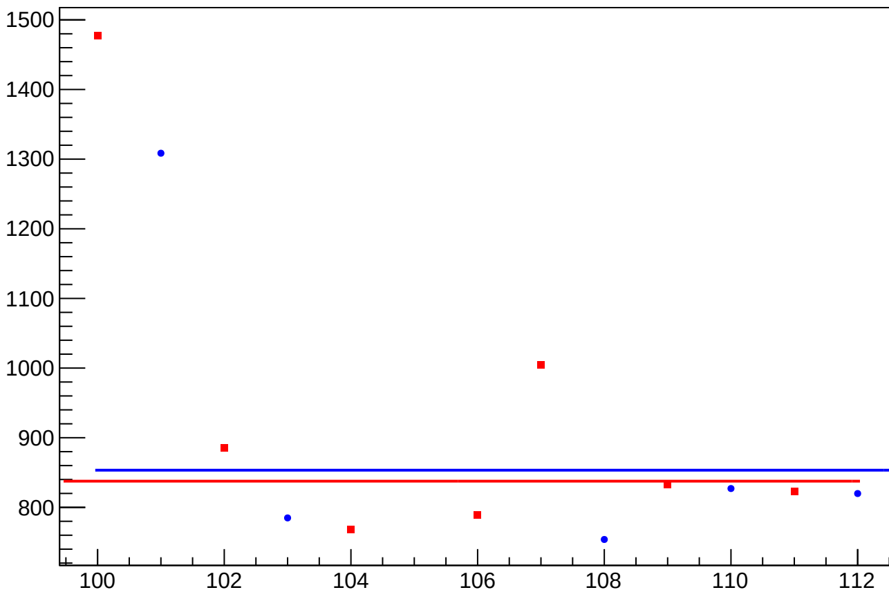
cor_asym_usl_atl2_dd_rms vs Slug, Sign Corrected
