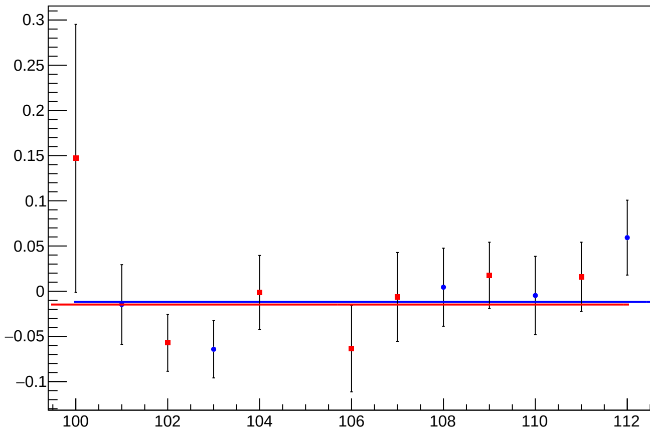
asym_us_dd_overload_cor_vs_slug_diff_mean vs Slug, Sign Corrected
