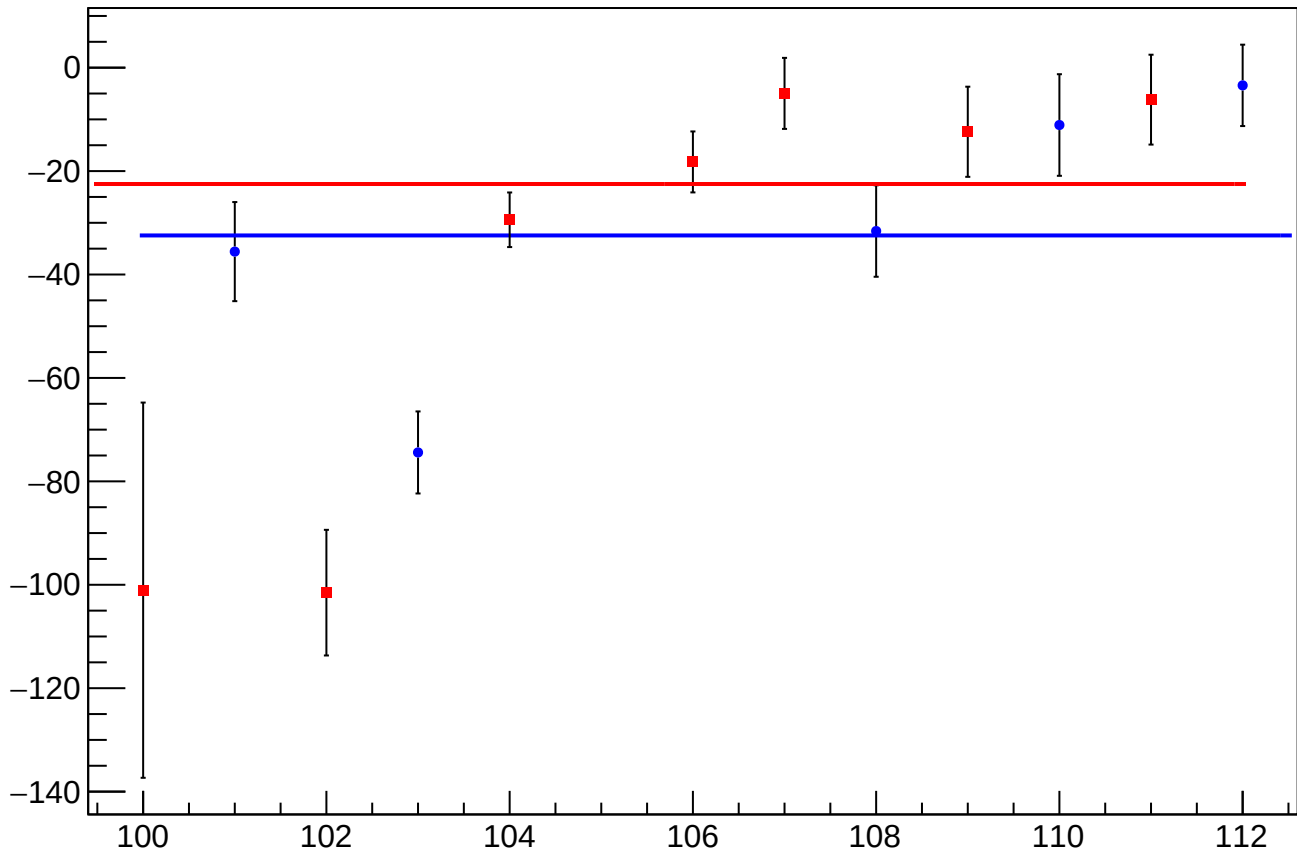
reg_asym_us_avg_at2lr_avg_dd_diff_bpm4aY_slope vs Slug, Sign Corrected
