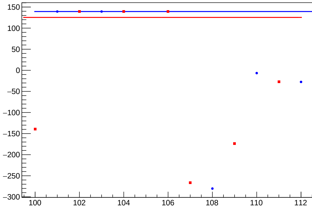
yield_cav4bX_mean vs Slug, Sign Corrected
