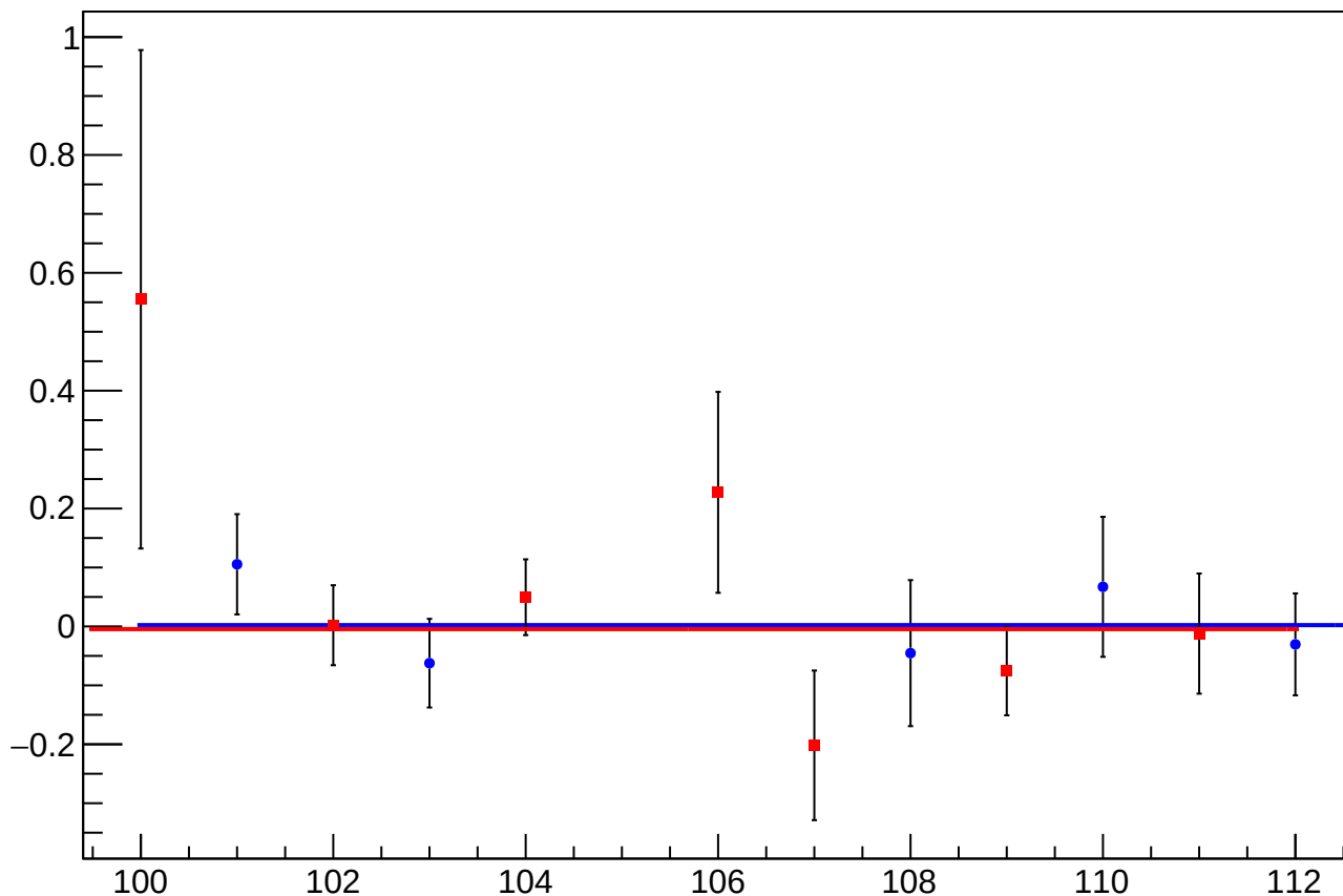
asym_sam_2468_avg_eigen_dit_vs_slug, Sign Corrected
