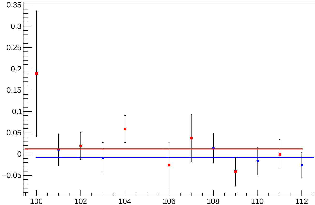
asym_us_dd_eigen_dit_vs_eigen_cor_diff_mean vs Slug, Sign Corrected
