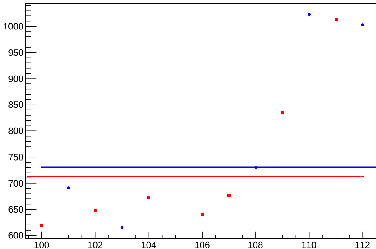
asym_sam1_eigen_cor_correction_rms vs Slug, Sign Corrected
