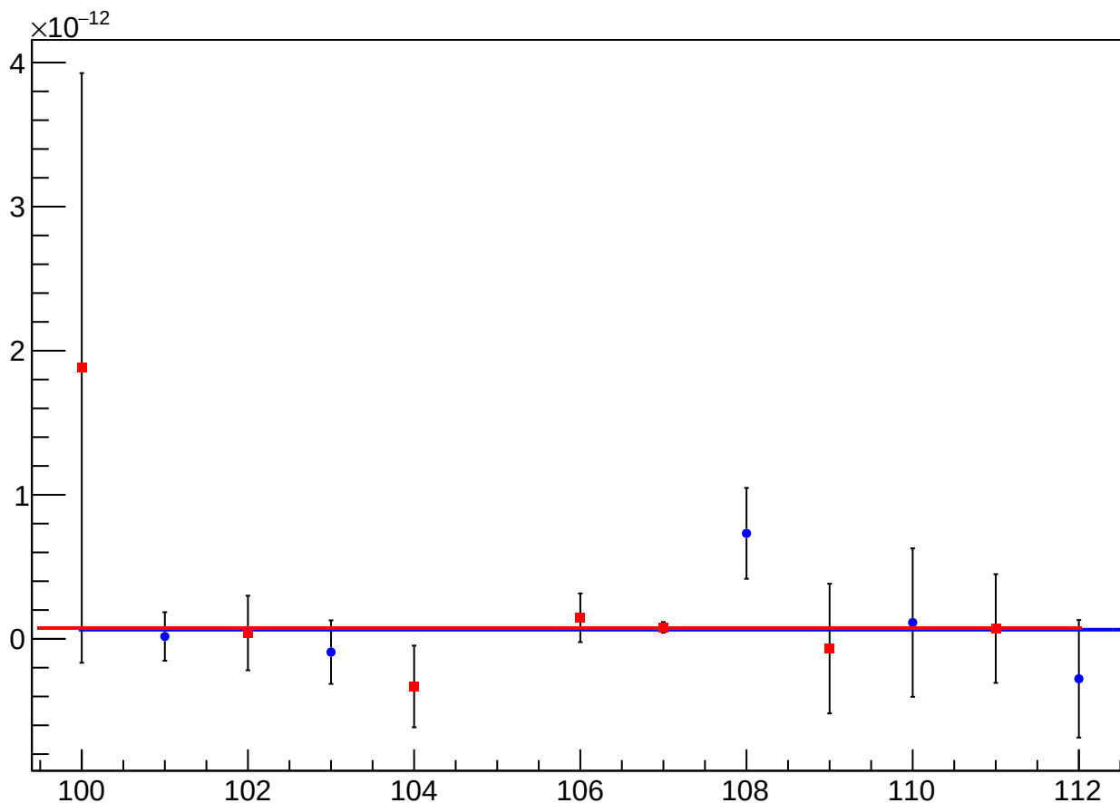
asym_atl1r2_dd_reg_vs_cor_diff_mean vs Slug, Sign Corrected
