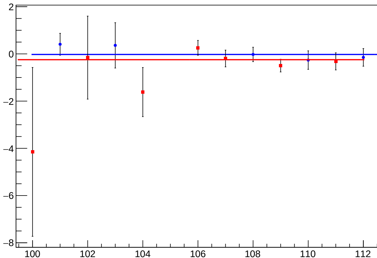
asym_us_avg_at2lr_avg_dd_dit_vs_cor_diff_mean vs Slug, Sign Corrected
