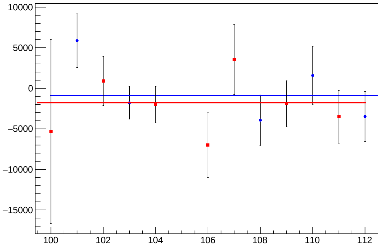
cor_asym_atl1r2_dd_mean vs Slug, Sign Corrected
