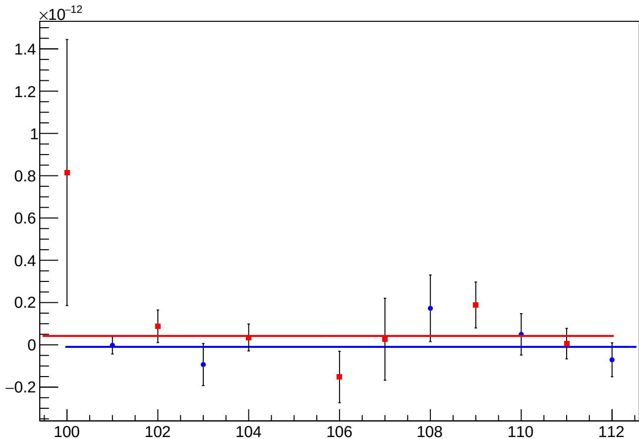
asym_sam_3726_avg_eigen_cor_vs_cor_diff_mean vs Slug, Sign Corrected
