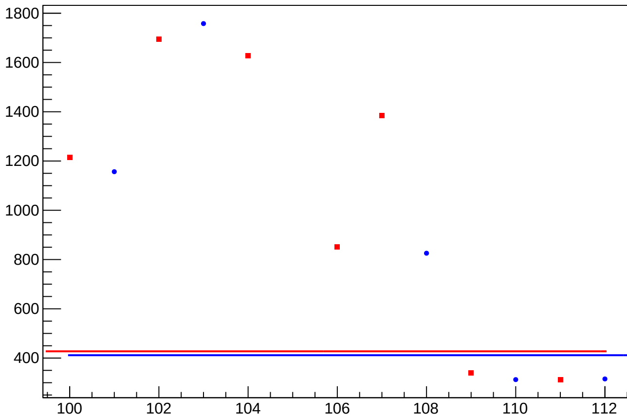
asym_us_dd_atlr_dd_dd_dit_correction_rms vs Slug, Sign Corrected
