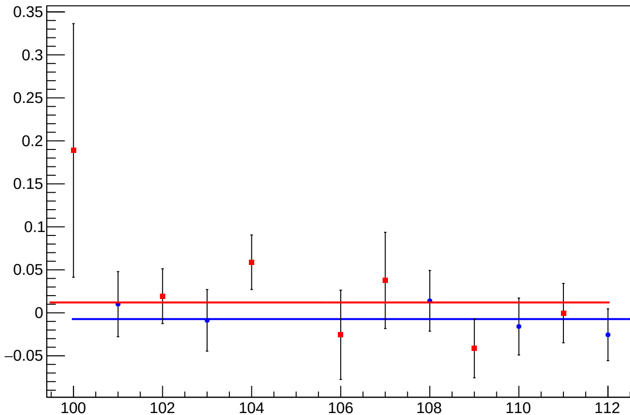
asym_us_dd_eigen_dit_vs_slug, Sign Corrected
