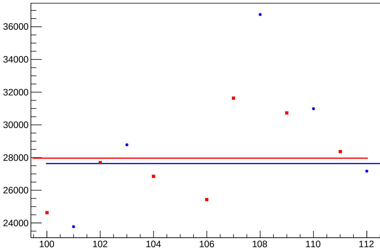
diff_bpmE_rms vs Slug, Sign Corrected
