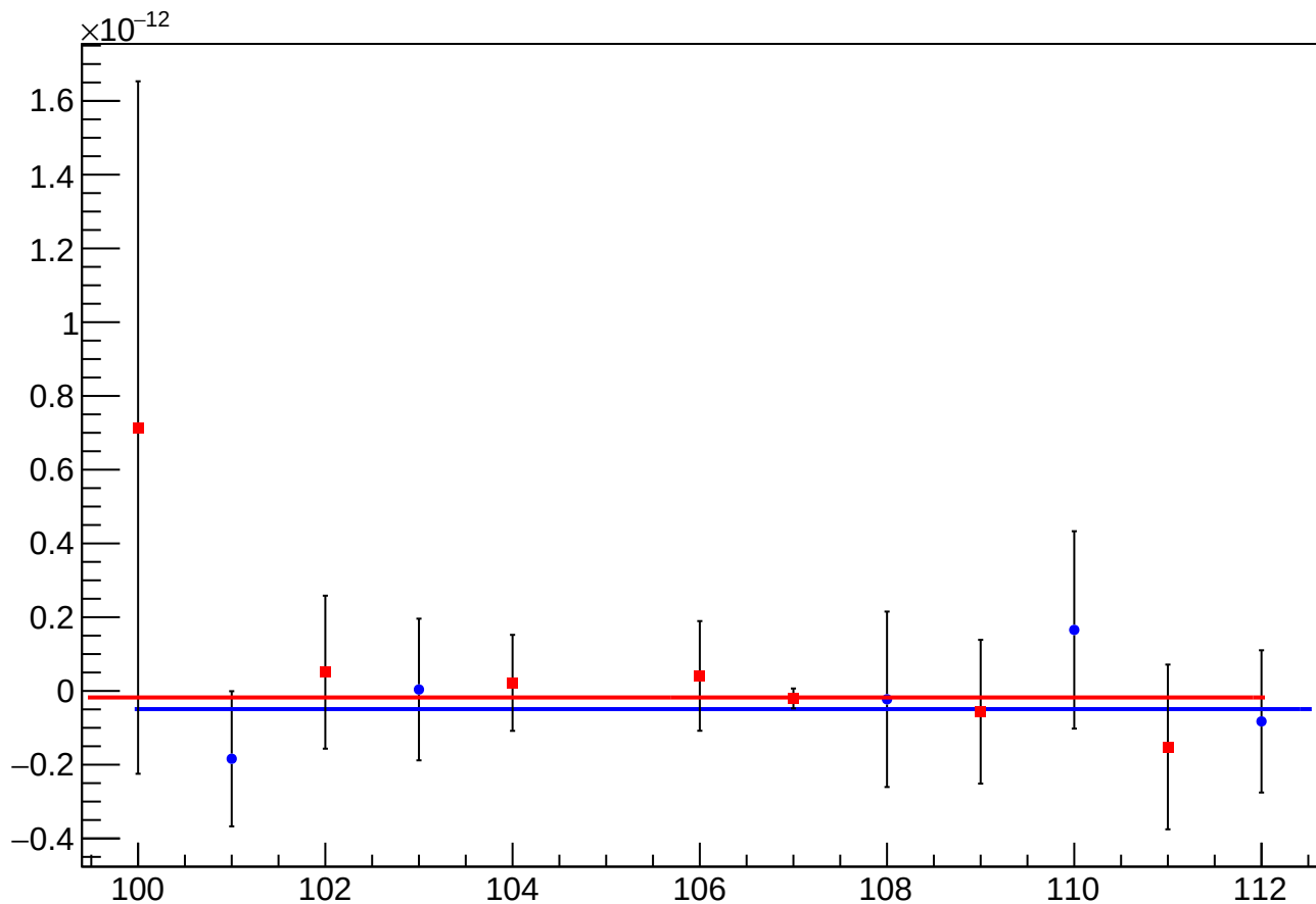
asym_atl1r2_dd_eigen_cor_vs_slug_sign_corrected
