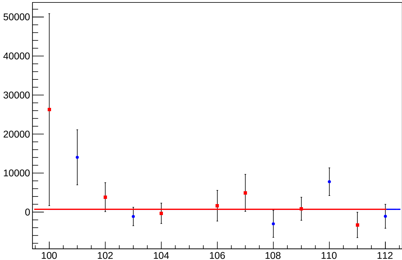
cor_asym_at1_avg_mean vs Slug, Sign Corrected
