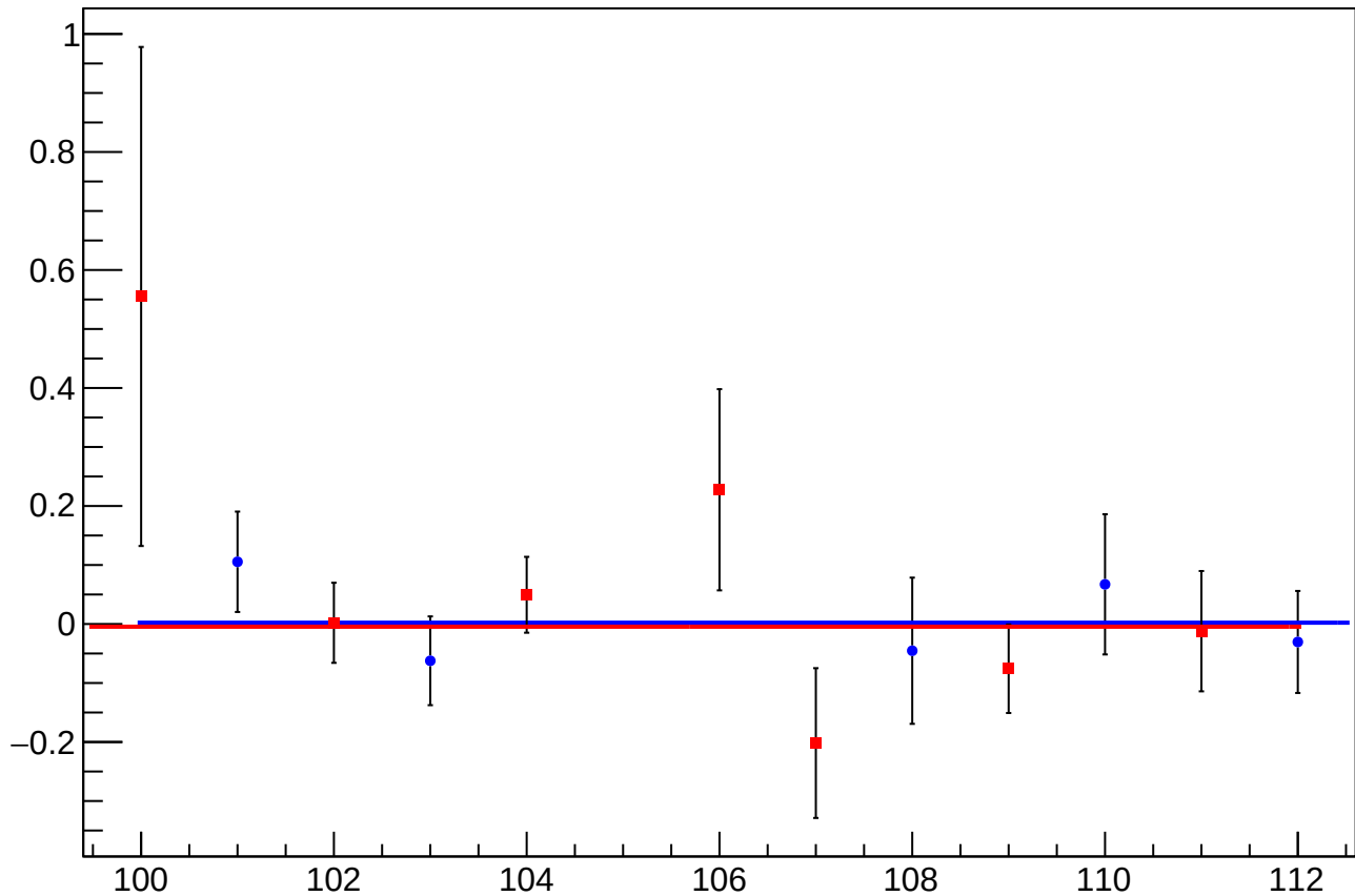
asym_sam_2468_avg_dit_vs_cor_diff_mean vs Slug, Sign Corrected
