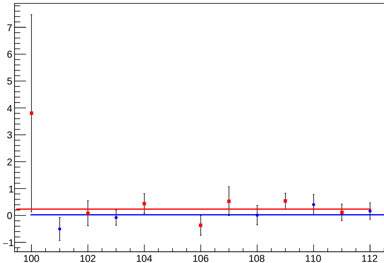
asym_atl2_dit_vs_eigen_cor_diff_mean vs Slug, Sign Corrected
