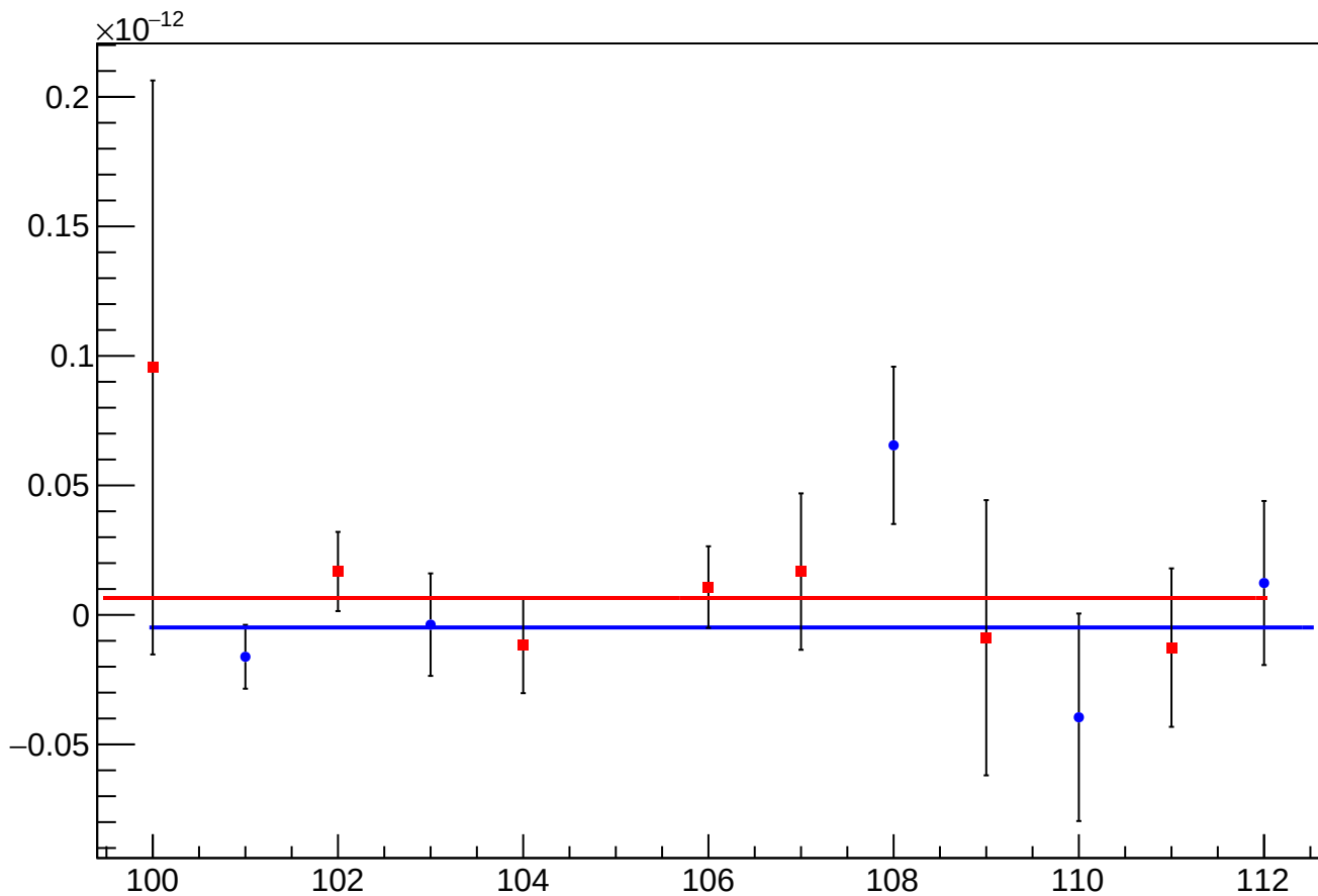
asym_sam_37_48_dd_reg_vs_cor_diff_mean vs Slug, Sign Corrected
