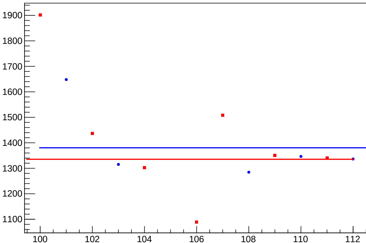
eigen_cor_asym_usl_atl2_avg_rms vs Slug, Sign Corrected
