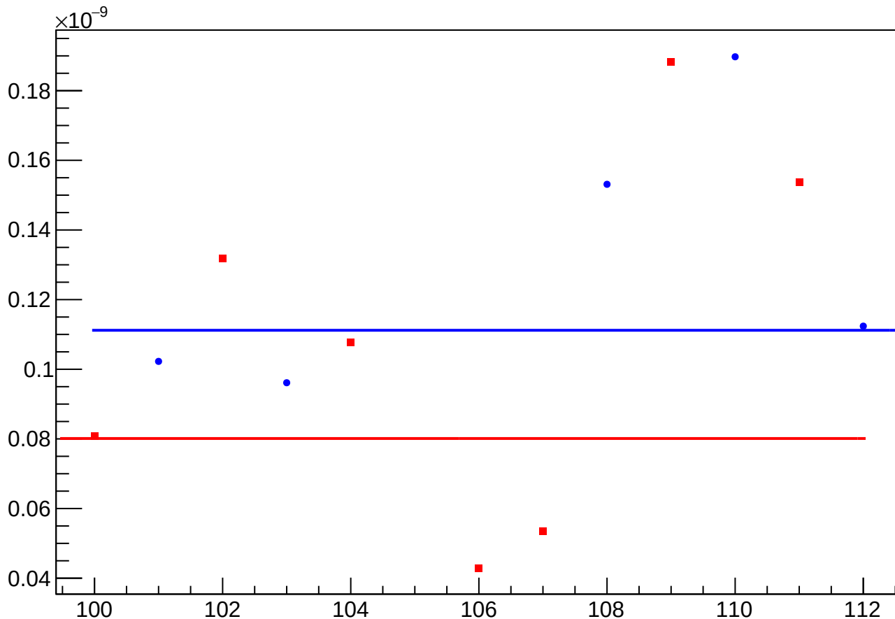
asym_atl1r2_dd_atl2r1_dd_dd_reg_vs_slug_Sign_Corrected
