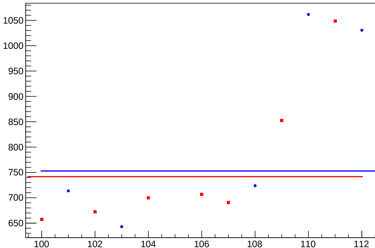
asym_sam1_eigen_dit_correction_rms vs Slug, Sign Corrected
