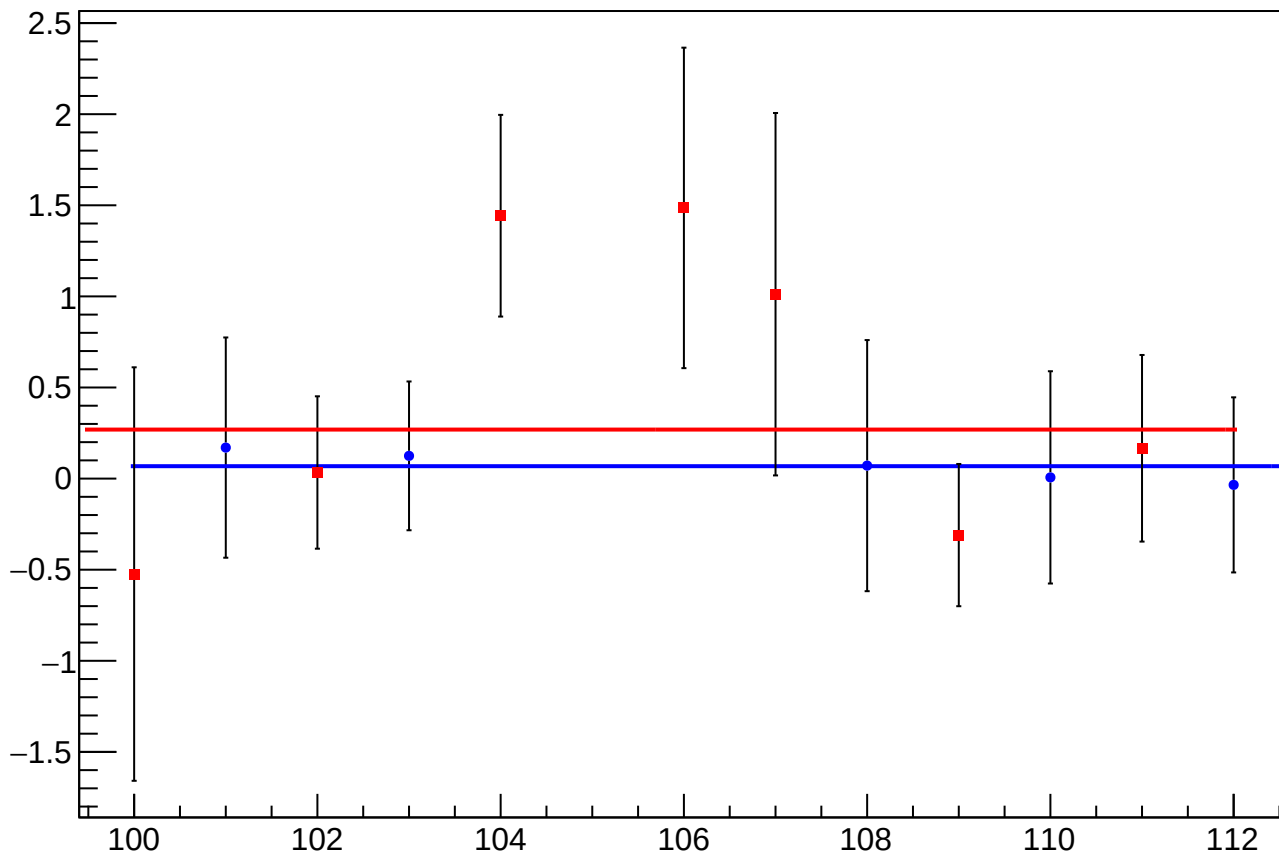
diff_targ_thetaY_mean vs Slug, Sign Corrected
