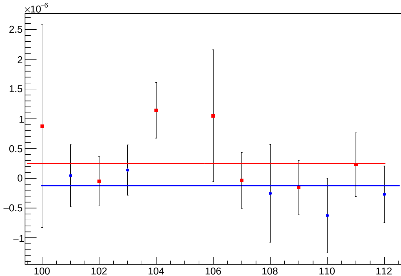
asym_sam_15_avg_eigen_dit_vs_dit_diff_mean vs Slug, Sign Corrected
