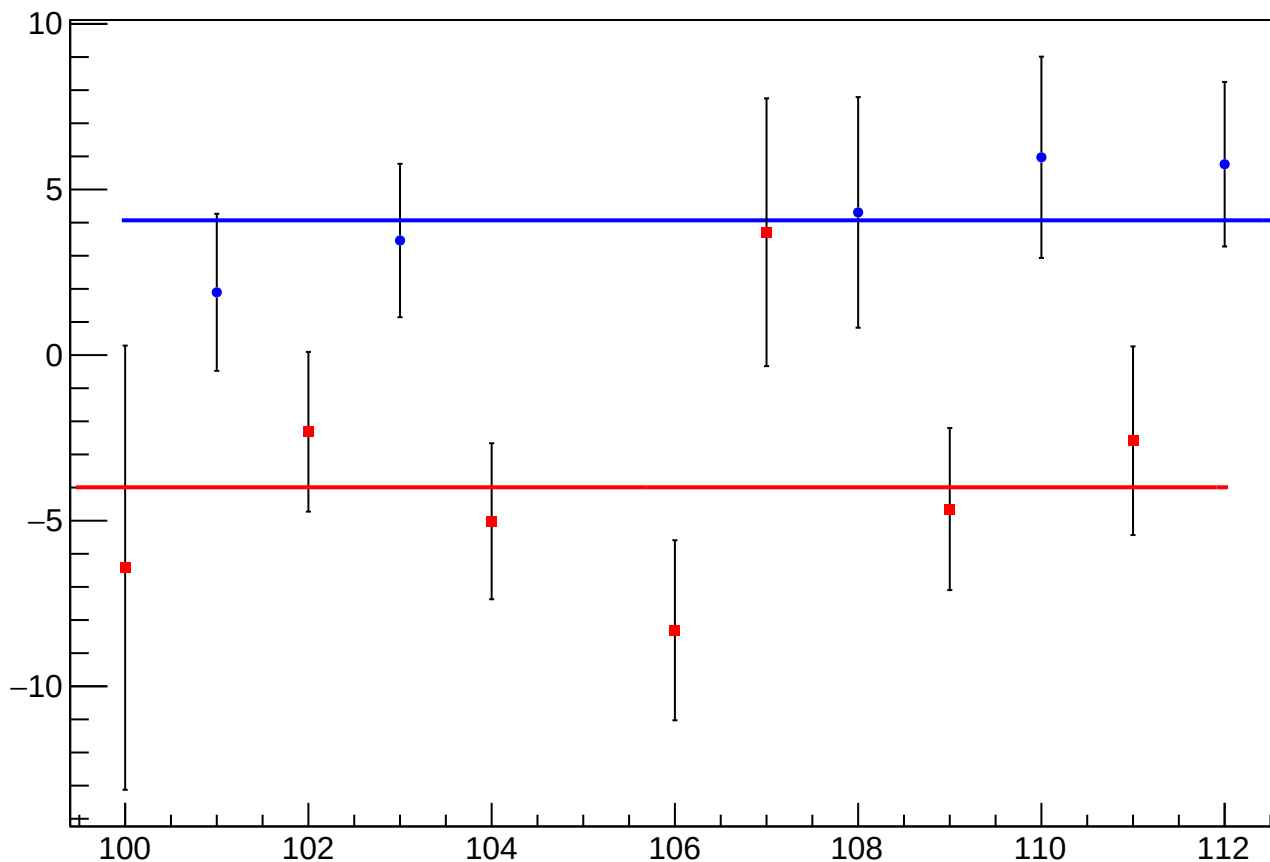
diff_bpm0i01aY_mean vs Slug, Sign Corrected
