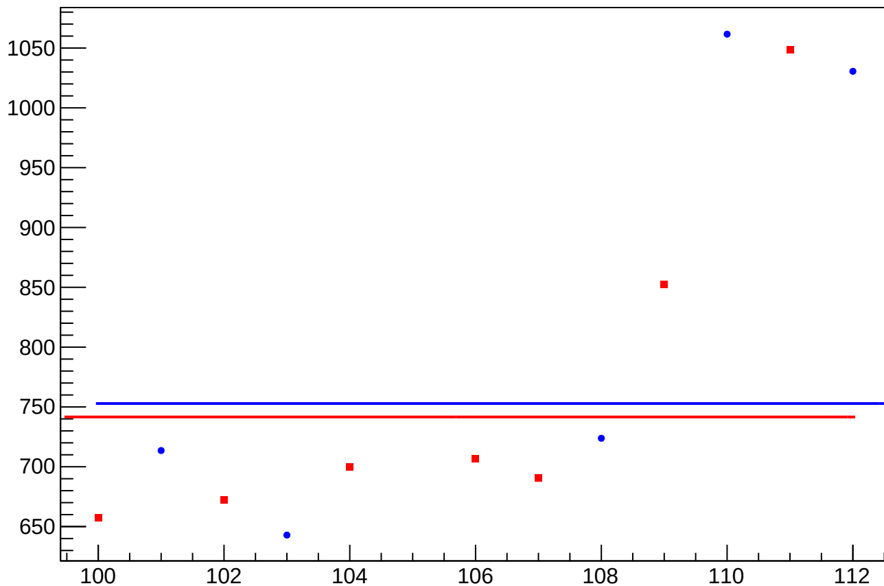
asym_sam1_dit_correction_rms vs Slug, Sign Corrected
