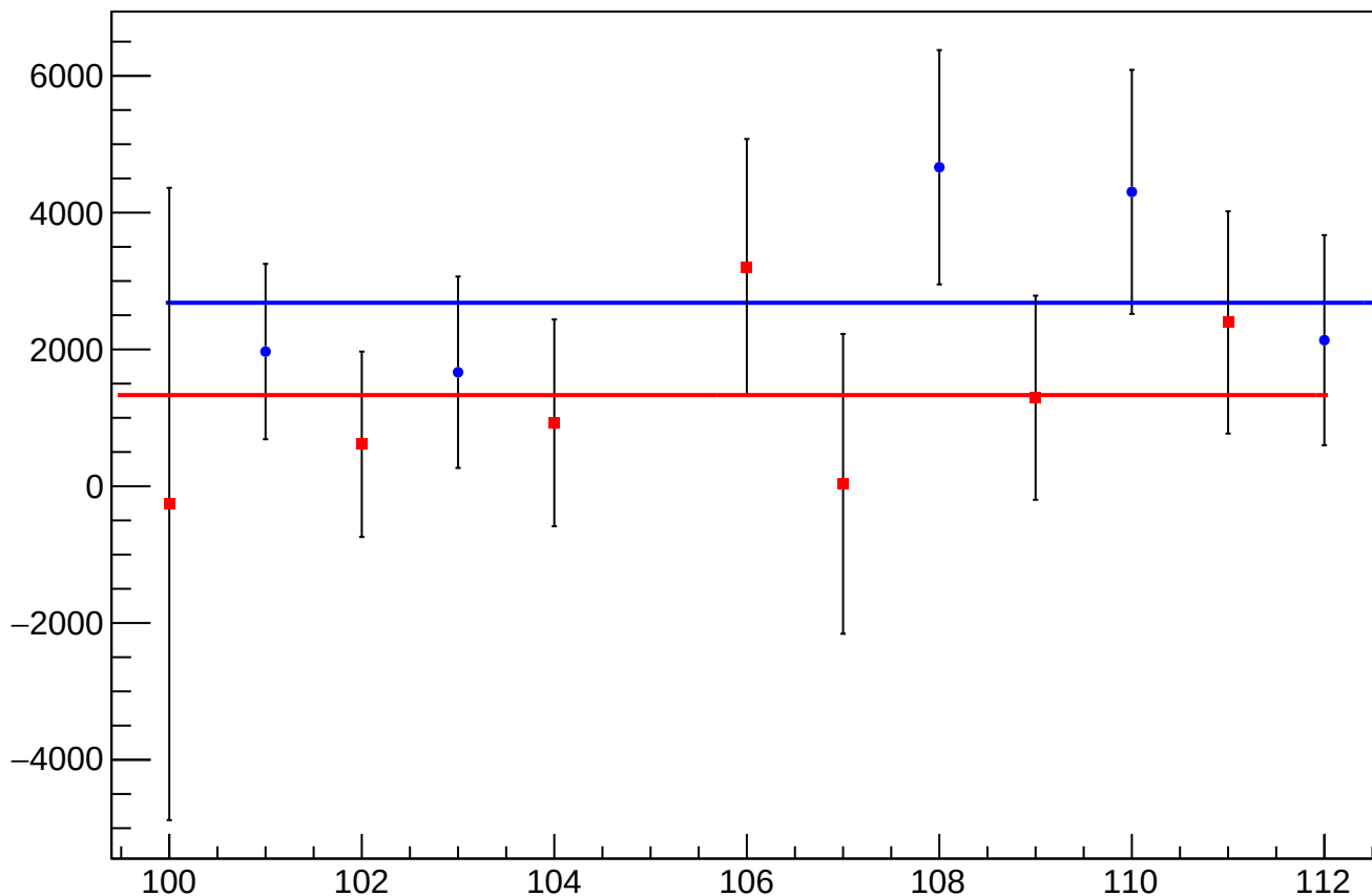
eigen_dit_asym_usr_mean vs Slug, Sign Corrected
