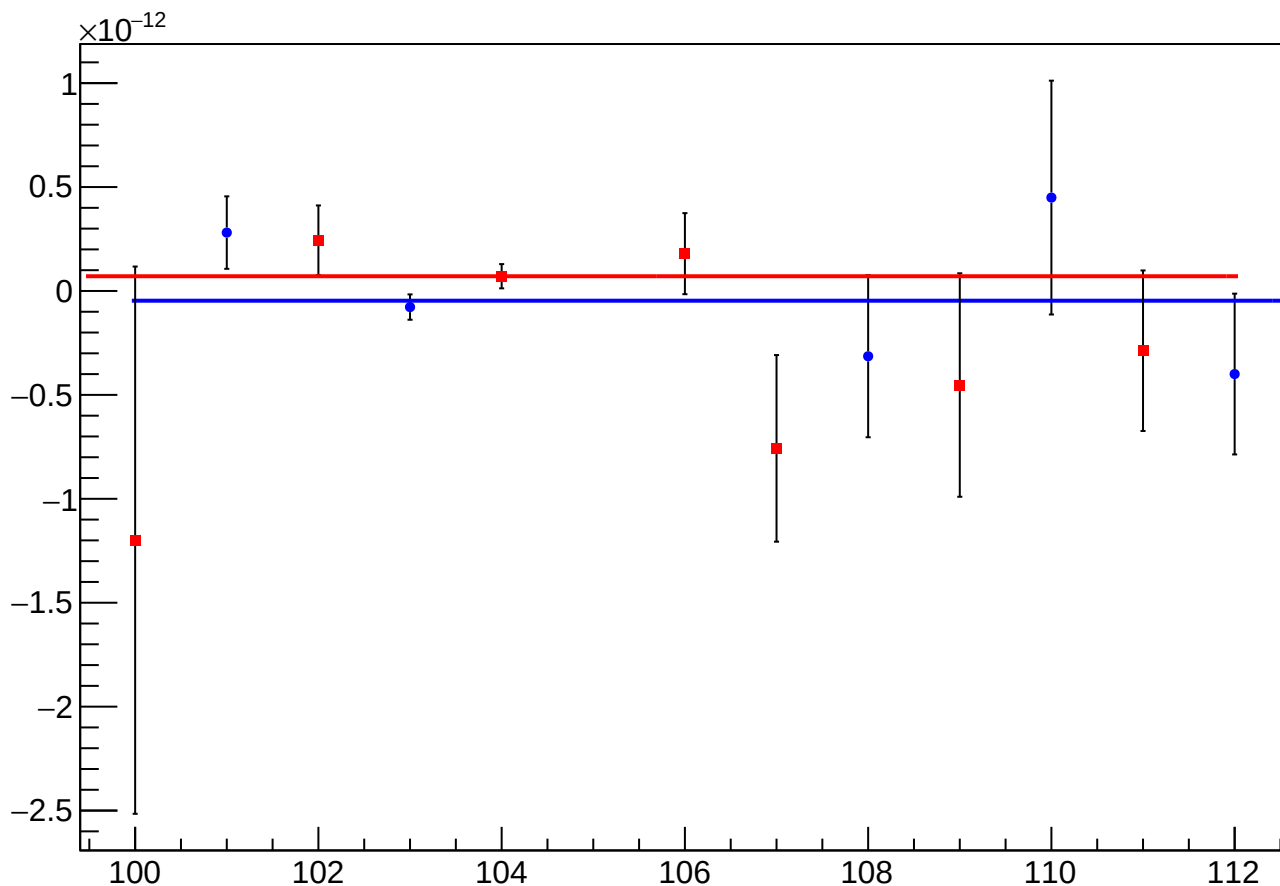
asym_atl_avg_atr_avg_avg_reg_vs_slug_sign_corrected
