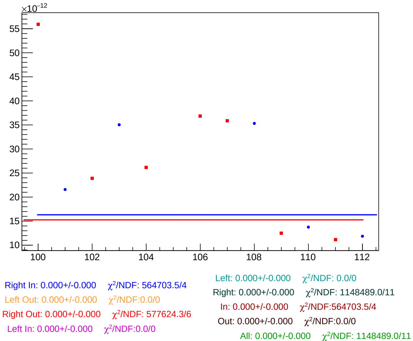
asym_us_dd_atlr_dd_dd_eigen_cor_vs_cor_diff_rms vs Slug, Sign Corrected
