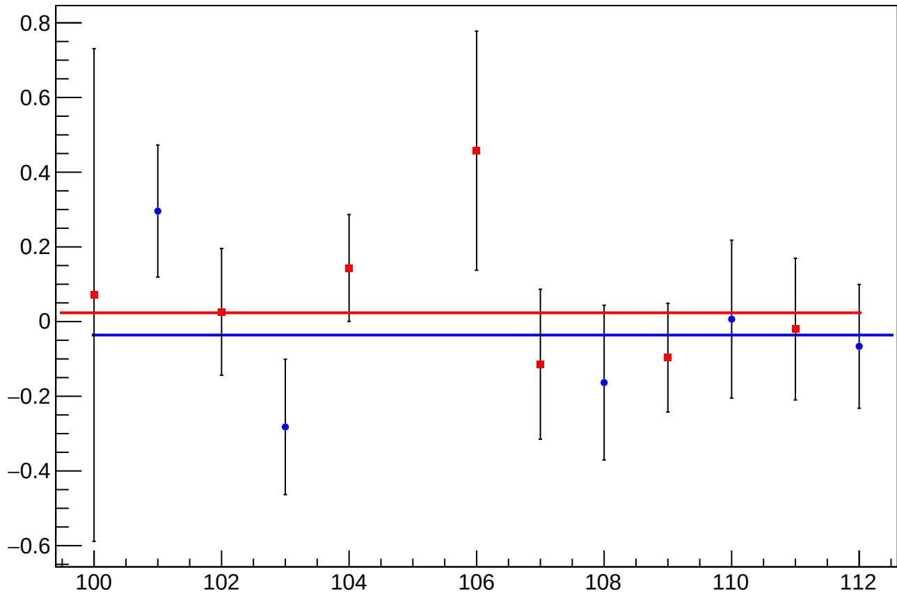
asym_sam_26_avg_eigen_dit_vs_cor_diff_mean vs Slug, Sign Corrected
