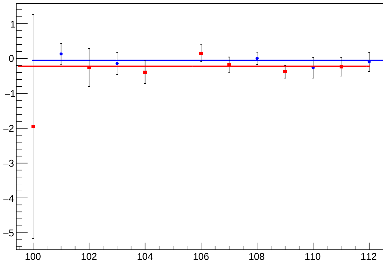
asym_atr_dd_eigen_dit_vs_cor_diff_mean vs Slug, Sign Corrected
