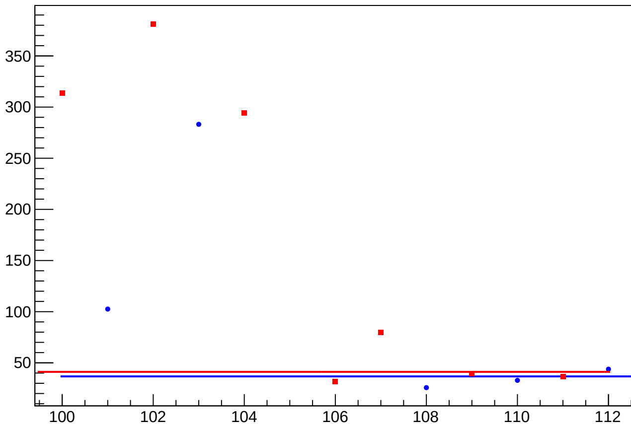
asym_atl1r2_dd_atl2r1_dd_avg_dit_vs_slug, Sign Corrected
