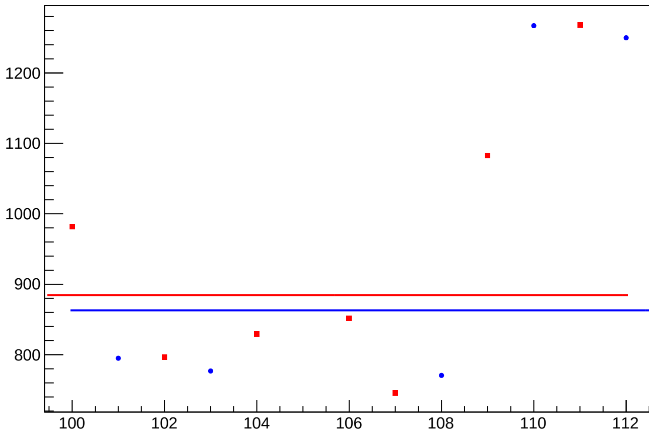
asym_sam_26_48_dd_cor_correction_rms vs Slug, Sign Corrected
