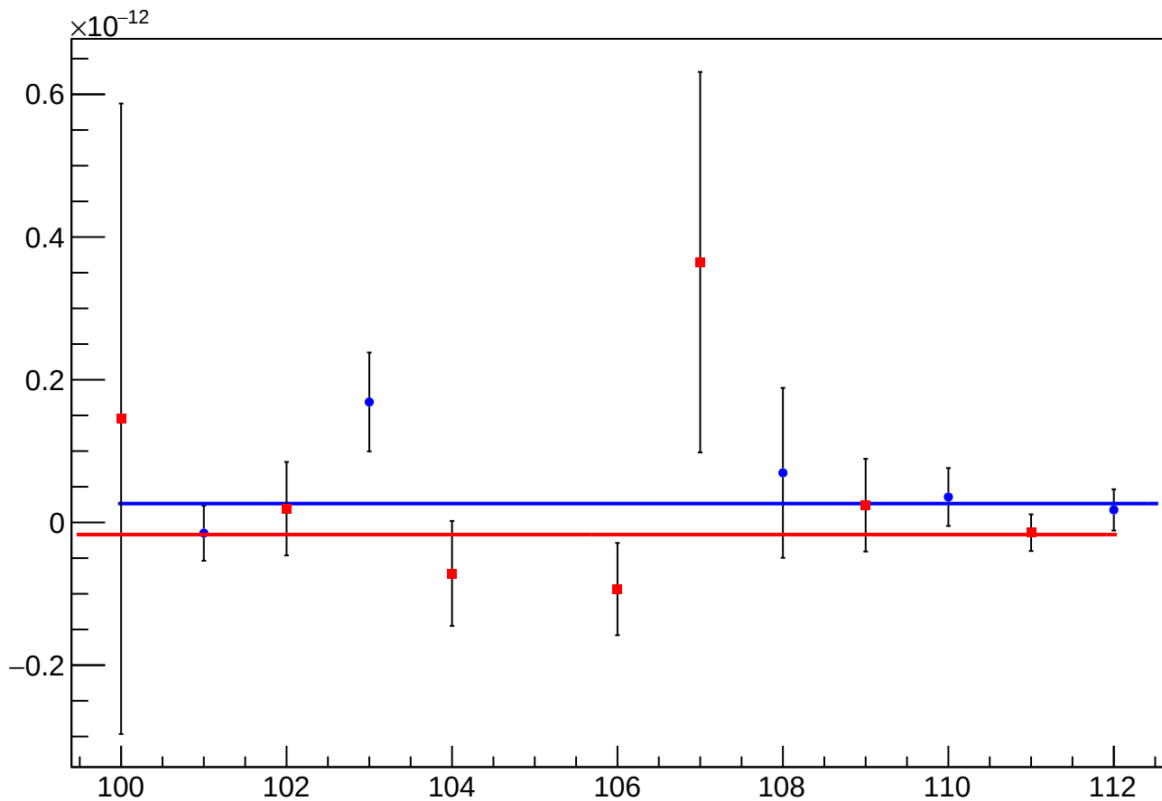
asym_us_dd_atlr_dd_dd_reg_vs_cor_diff_mean vs Slug, Sign Corrected
