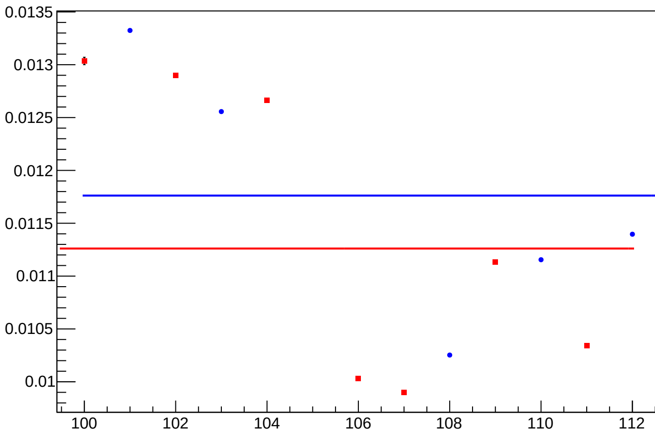
yield_bpm0l07X_rms vs Slug, Sign Corrected
