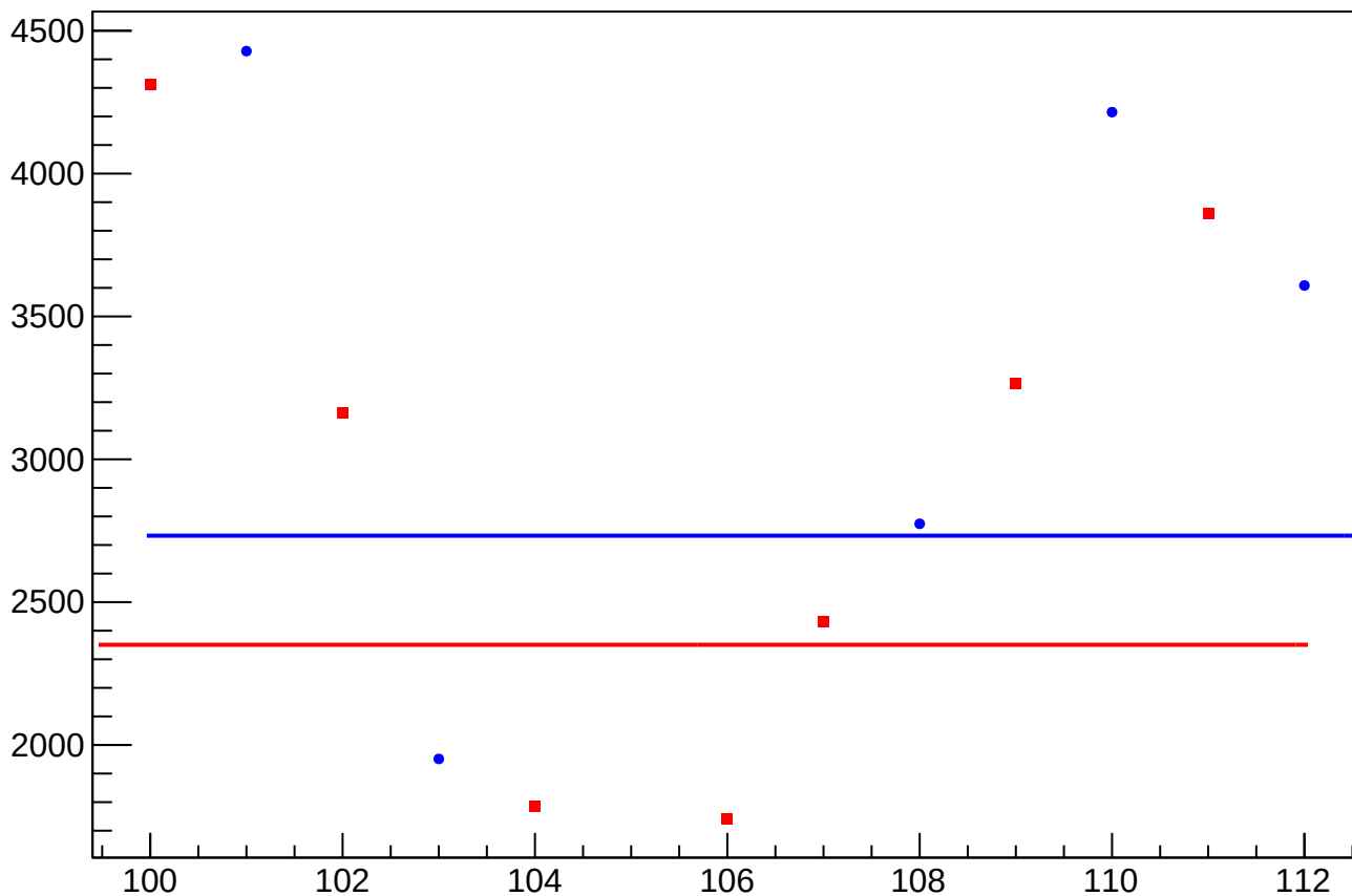
asym_usr_atr2_dd_correction_rms vs Slug, Sign Corrected
