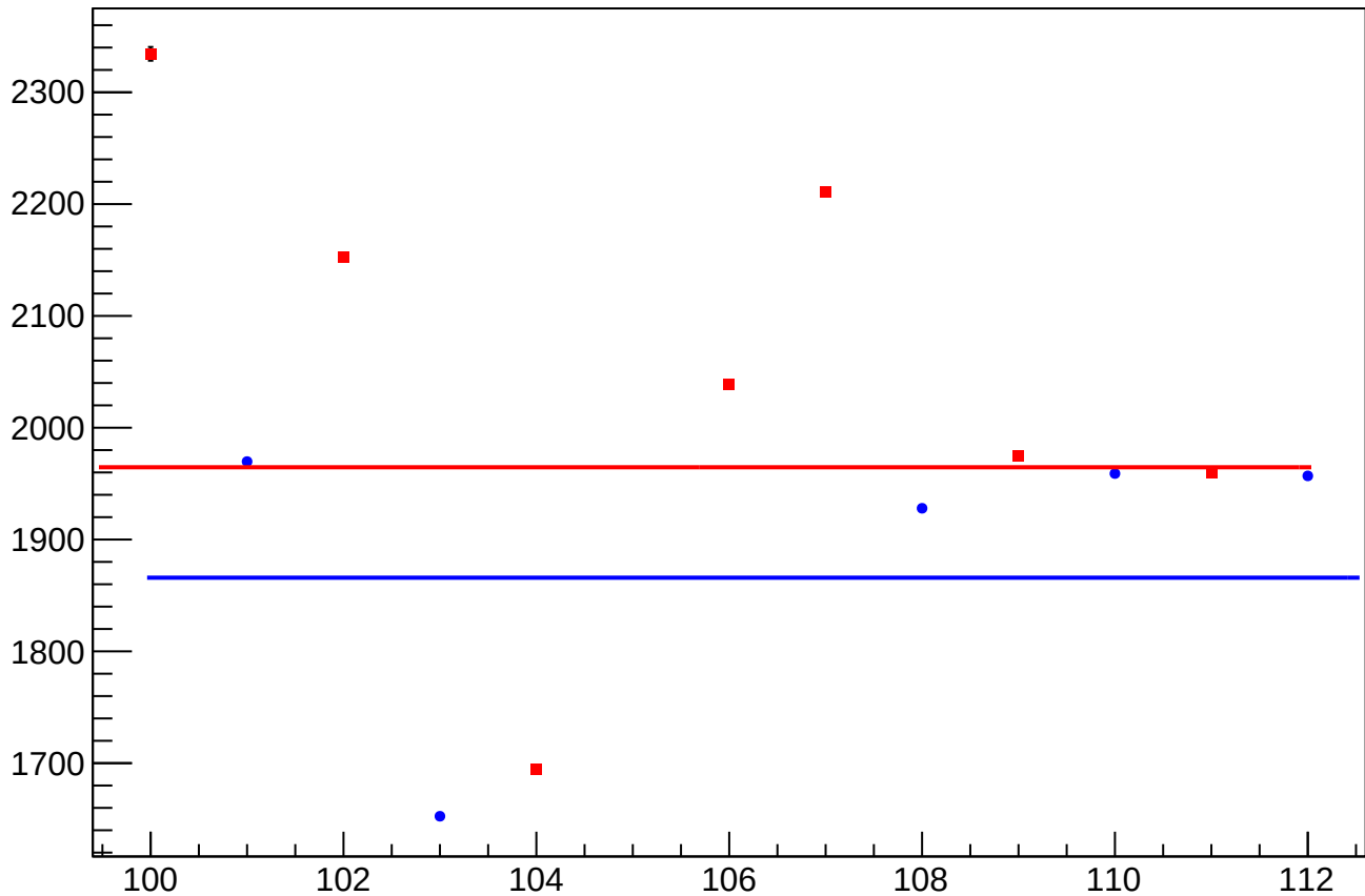
eigen_dit_asym_atl_dd_rms vs Slug, Sign Corrected
