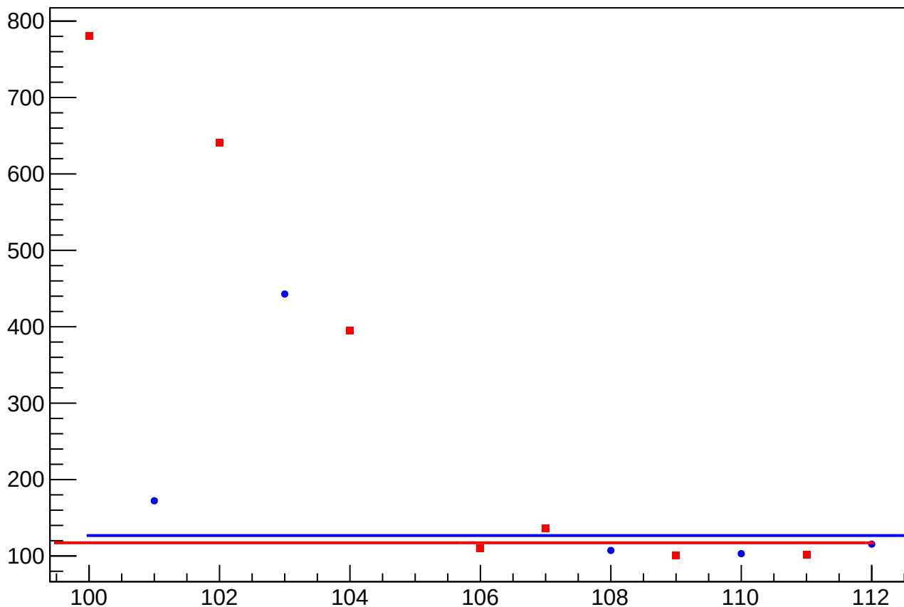
asym_atr12_dd_dit_vs_eigen_cor_diff_rms vs Slug, Sign Corrected
