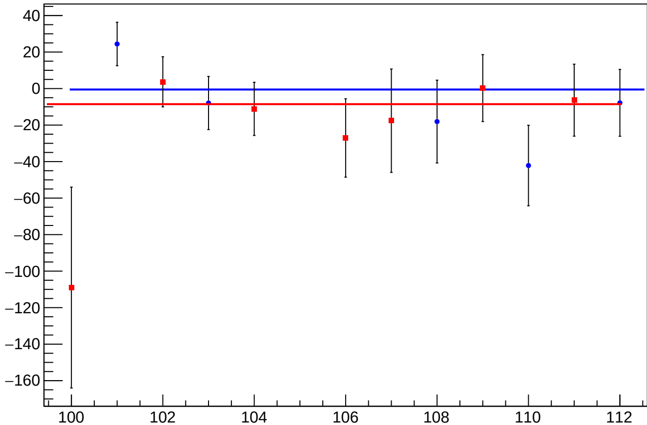
diff_bpm4aediffX_mean vs Slug, Sign Corrected
