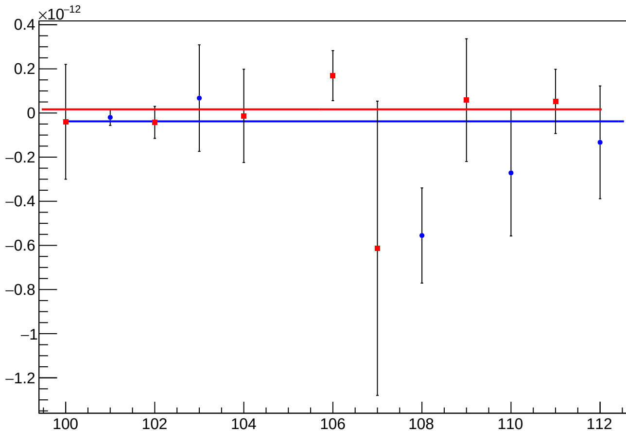
asym_atl1_reg_vs_cor_diff_mean vs Slug, Sign Corrected
