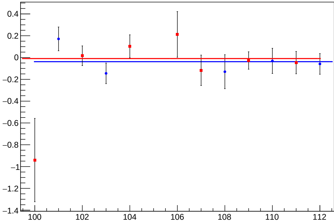
asym_sam_3726_avg_dit_vs_cor_diff_mean vs Slug, Sign Corrected
