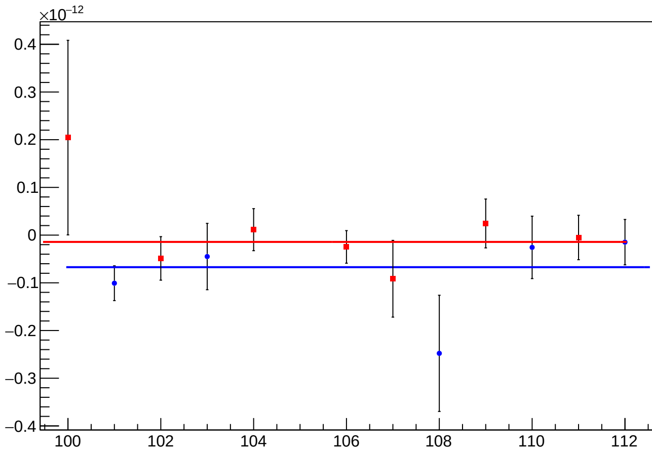
asym_sam_15_48_dd_reg_vs_cor_diff_mean vs Slug, Sign Corrected
