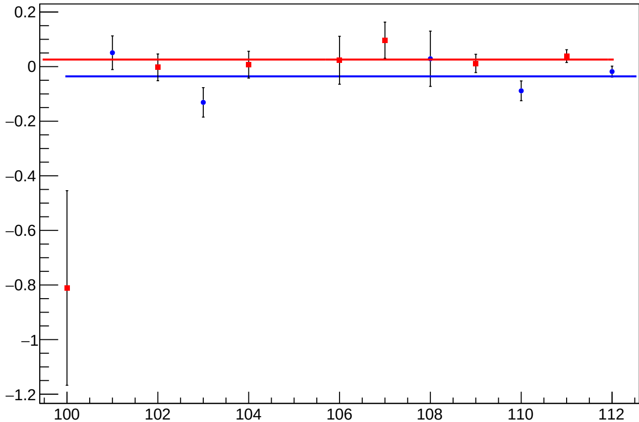
asym_sam_15_48_dd_dit_vs_cor_diff_mean vs Slug, Sign Corrected
