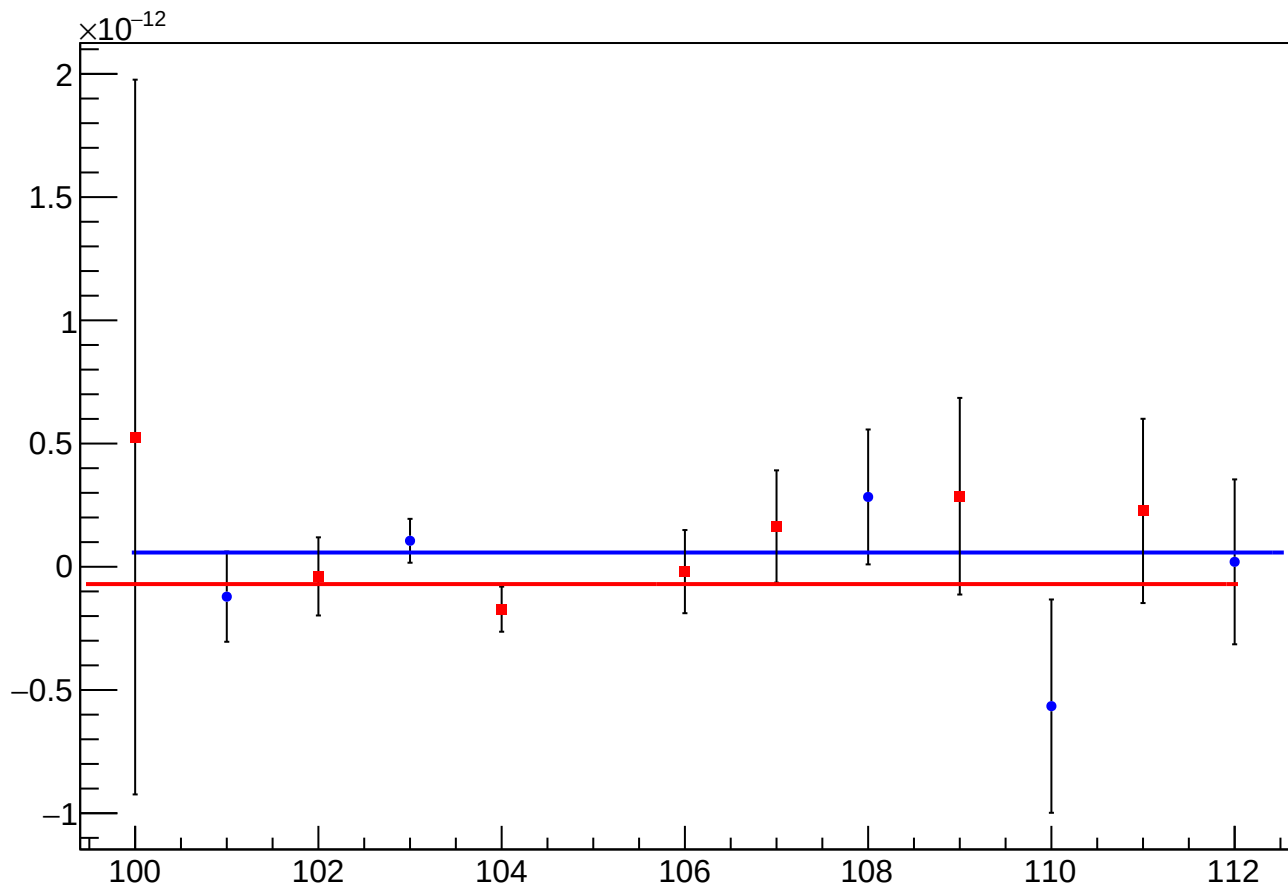
asym_usr_atr2_dd_reg_vs_slug, Sign Corrected
