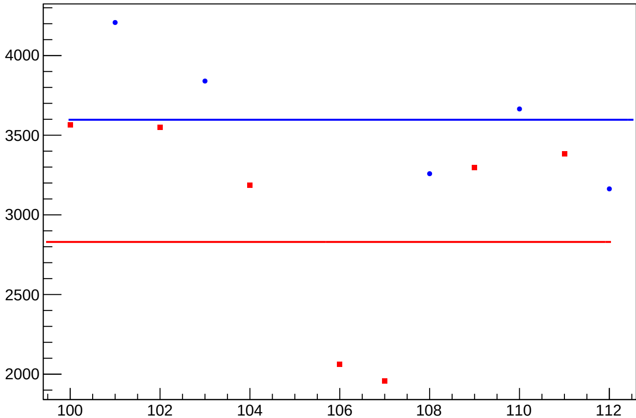
asym_atl1r2_dd_atl2r1_dd_dd_eigen_cor_correction_rms vs Slug, Sign Corrected
