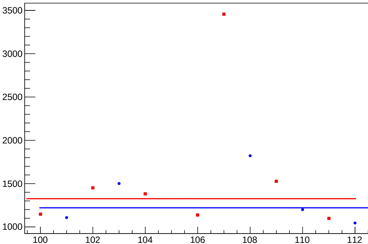
asym_usl_dit_correction_rms vs Slug, Sign Corrected
