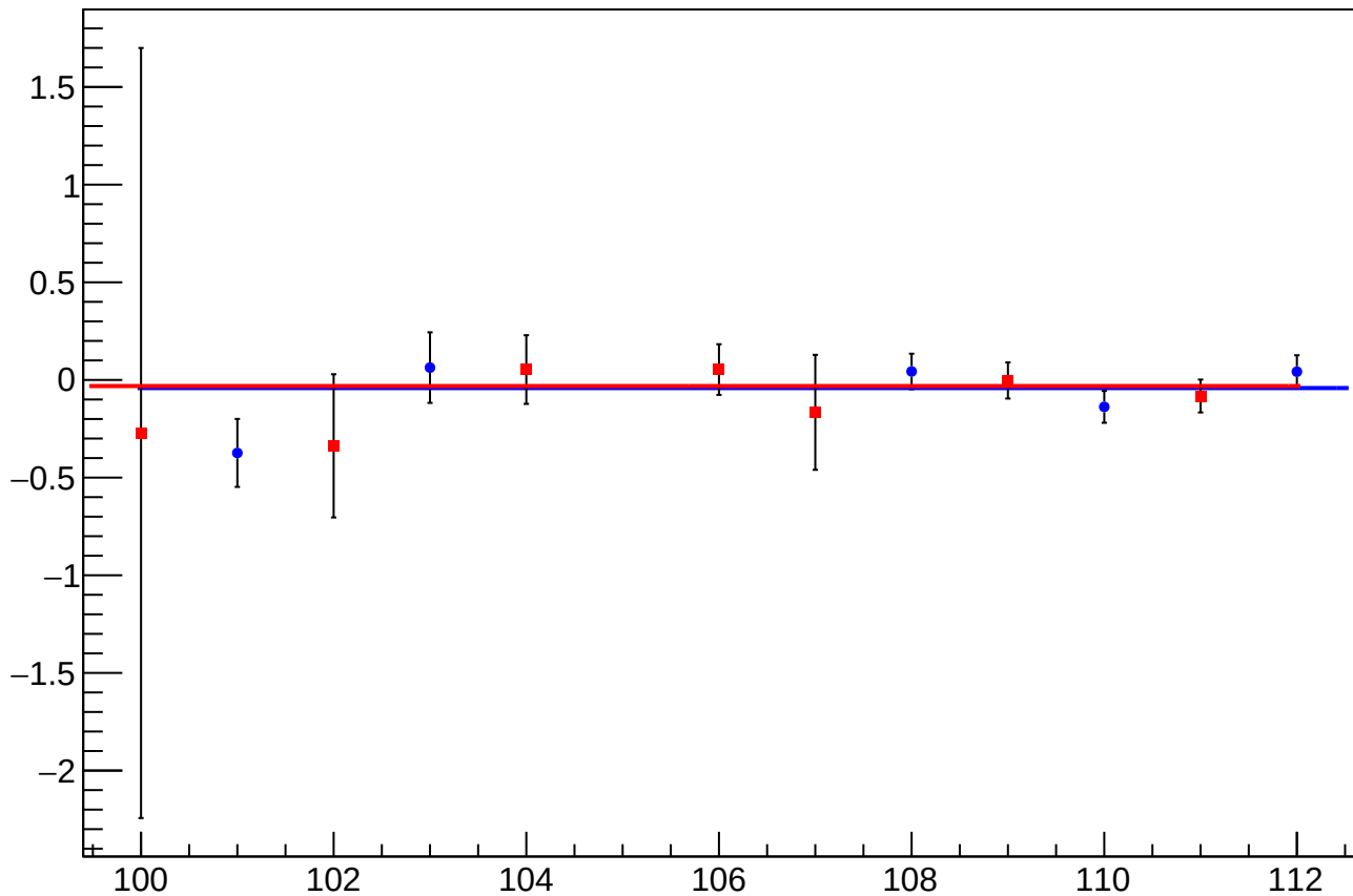
asym_us_dd_at1lr_dd_dd_dit_vs_cor_diff_mean vs Slug, Sign Corrected
