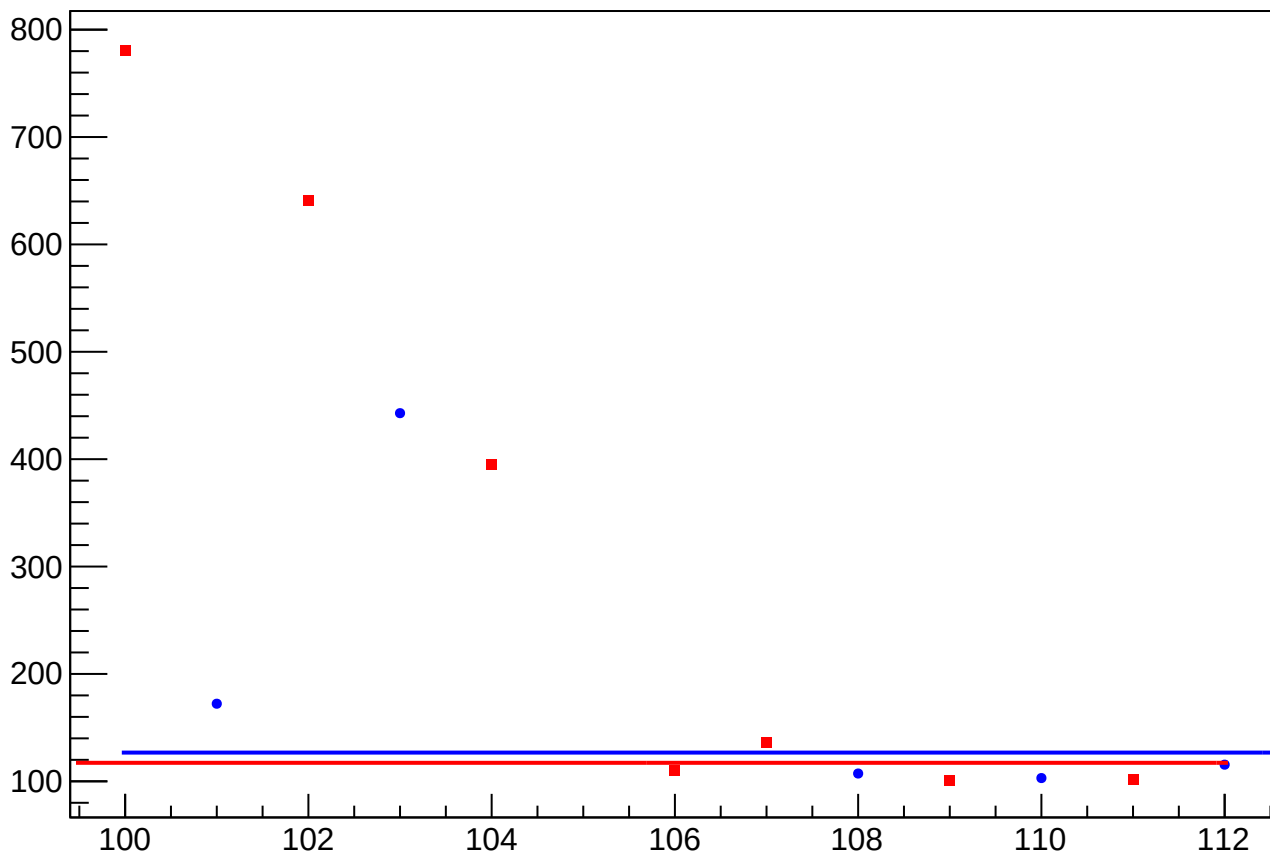
asym_atr12_dd_eigen_dit_vs_cor_diff_rms vs Slug, Sign Corrected
