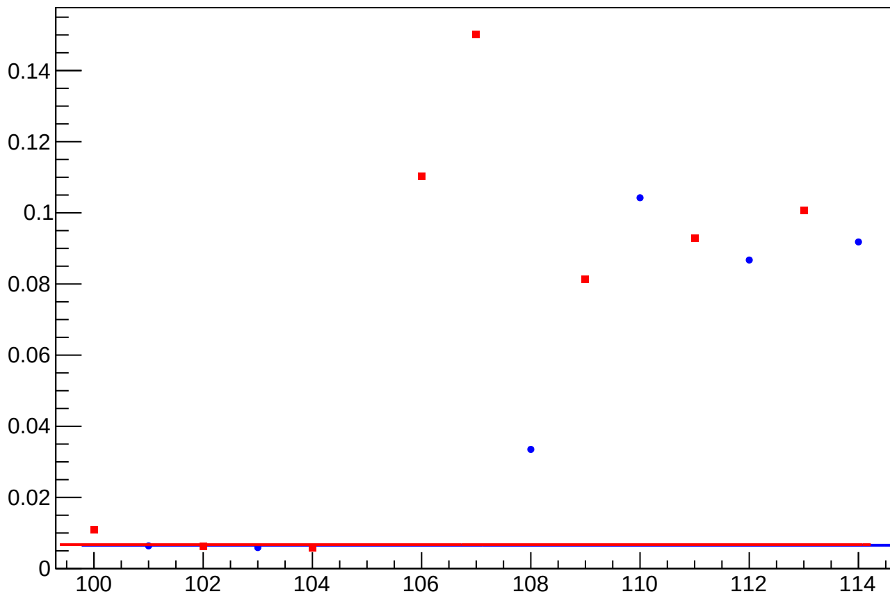
yield_bpm0l03Y_rms vs Slug, Sign Corrected
