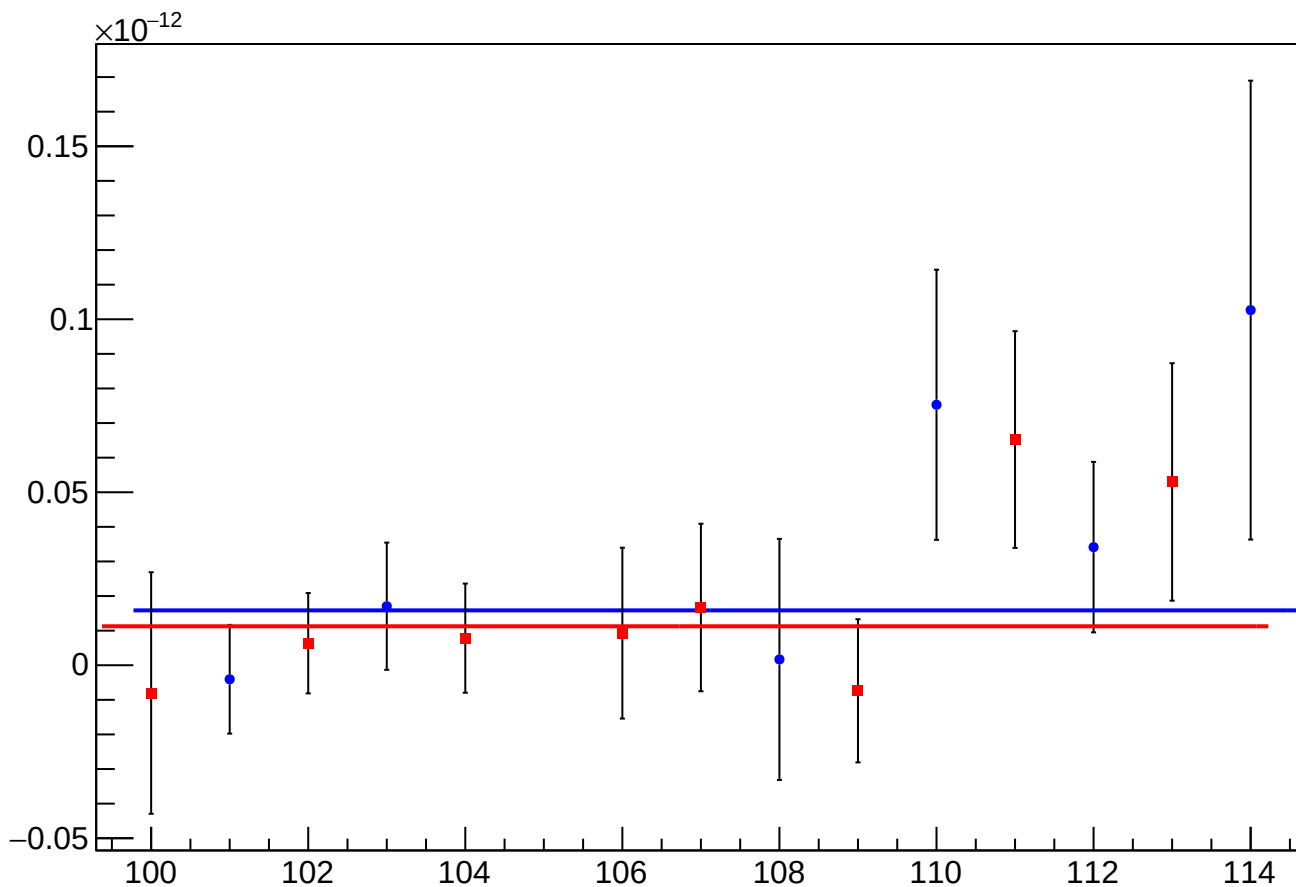
asym_sam8_eigen_cor_vs_cor_diff_mean vs Slug, Sign Corrected
