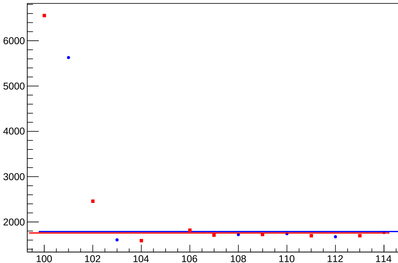
asym_usr_atr1_dd_rms vs Slug, Sign Corrected
