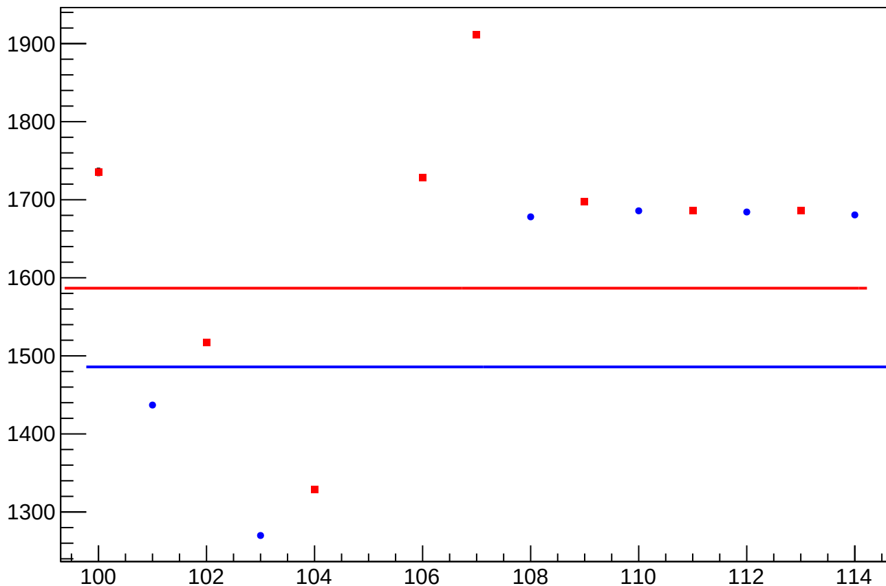
cor_asym_usl_atl1_dd_rms vs Slug, Sign Corrected
