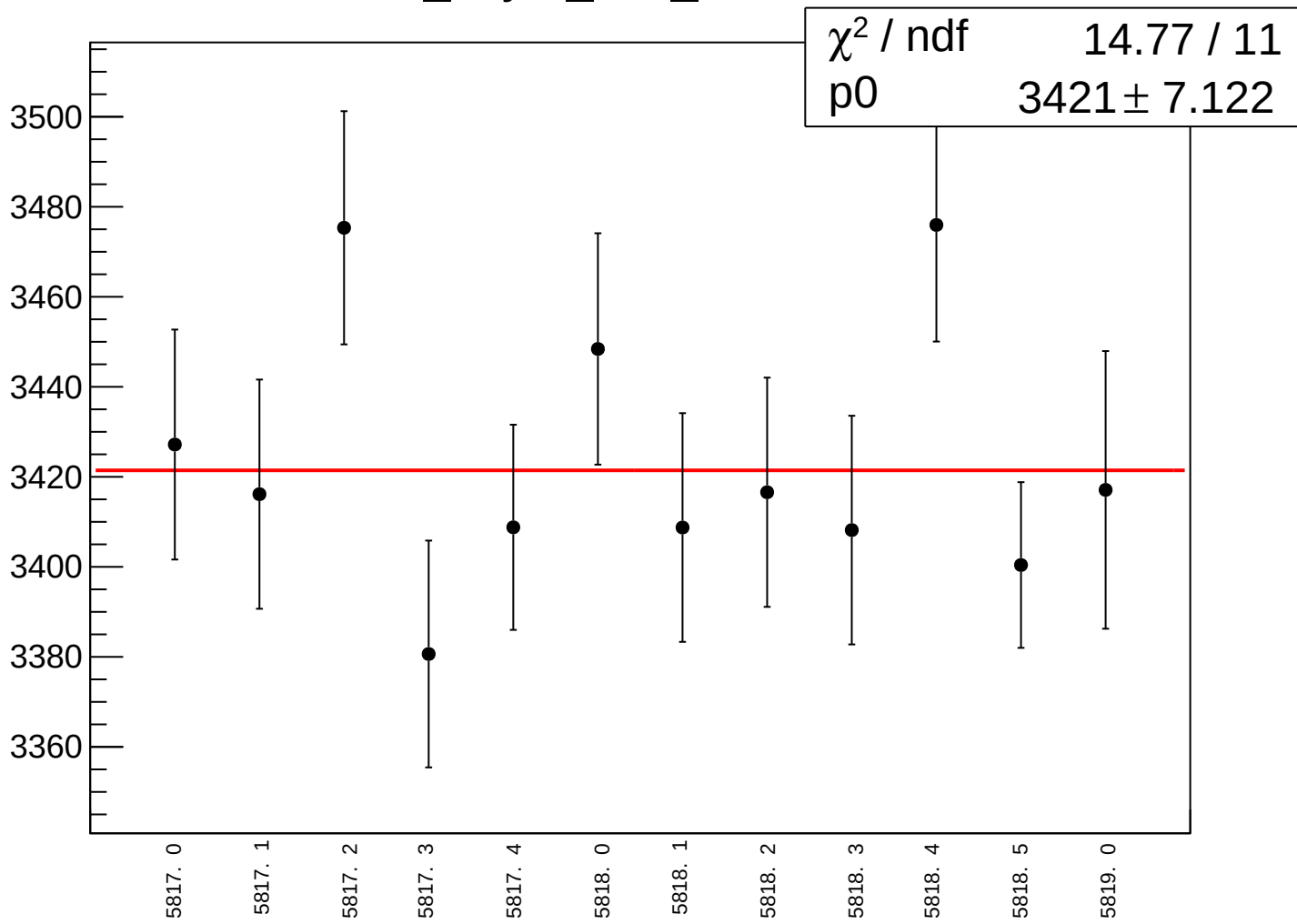
cor_asym_atl1_rms vs run
