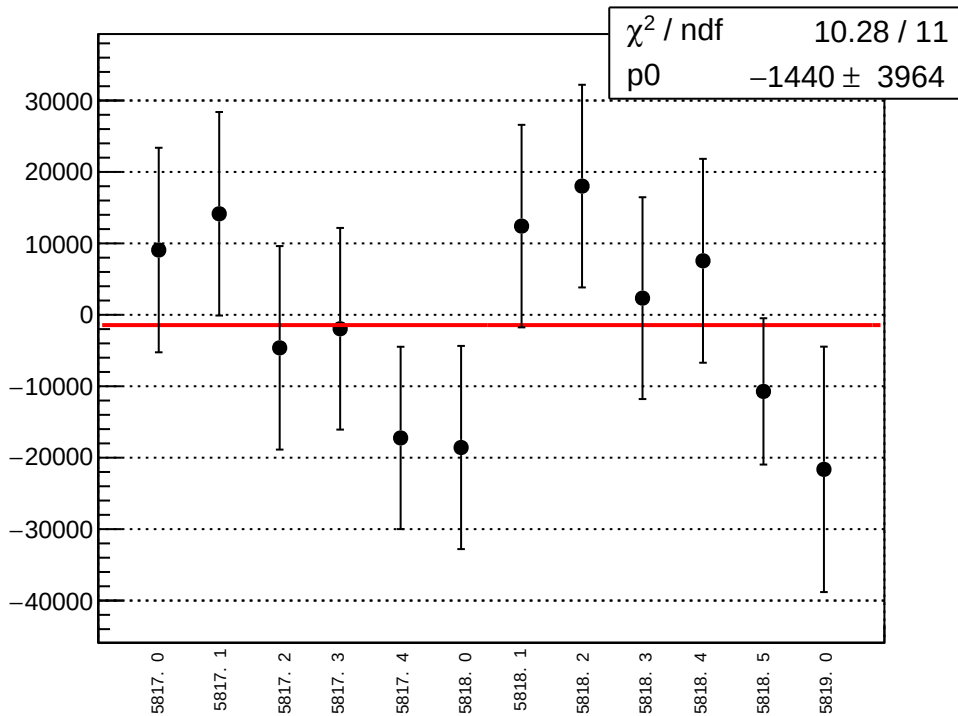
eigen_cor_asym_atl_dd_atr_dd_mean vs run
