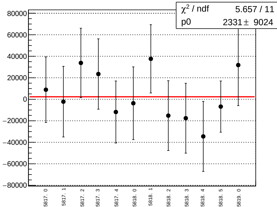
asym_atr1l2_avg_eigen_dit_correction_mean vs run
