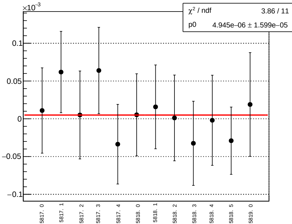
asym_us_dd_at2lr_dd_dd_eigen_dit_vs_dit_diff_mean vs run
