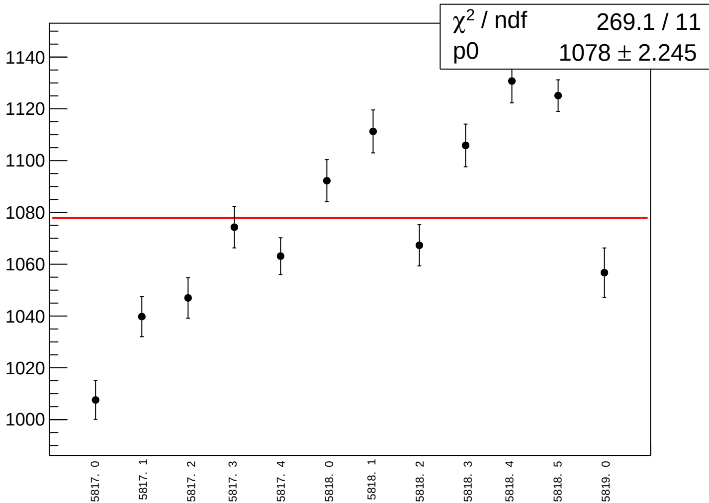
asym_sam_37_26_dd_dit_correction_rms vs run
