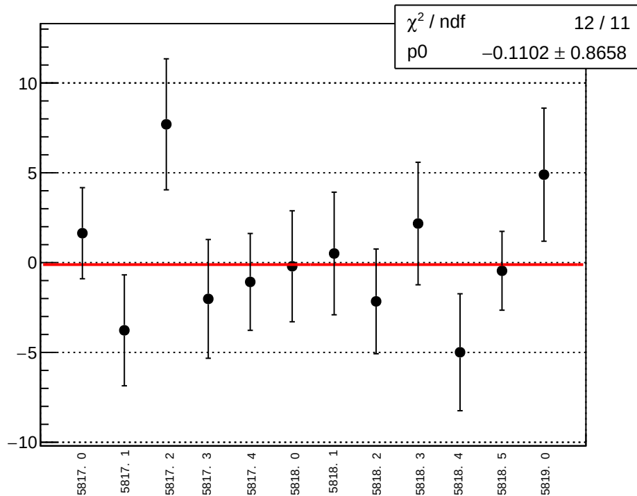
asym_atr_avg_dif_vs_eigen_cor_diff_mean vs run
