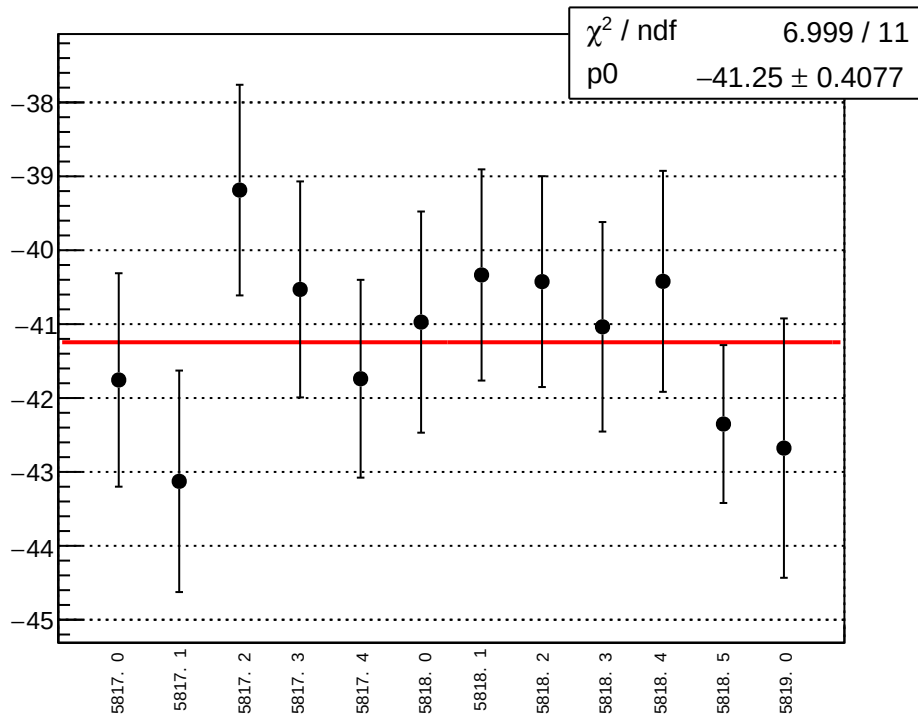
reg_asym_us_dd_at2lr_dd_diff_bpm12X_slope vs run
