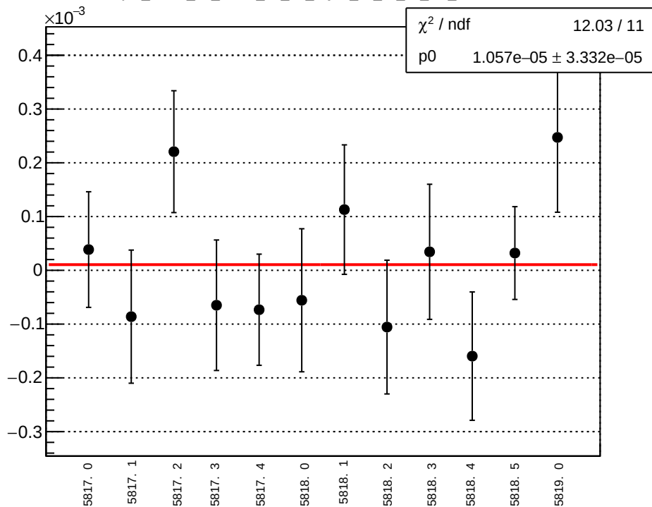
asym_atl1r2_dd_atl2r1_dd_eigen_dit_vs_dit_diff_mean vs run
