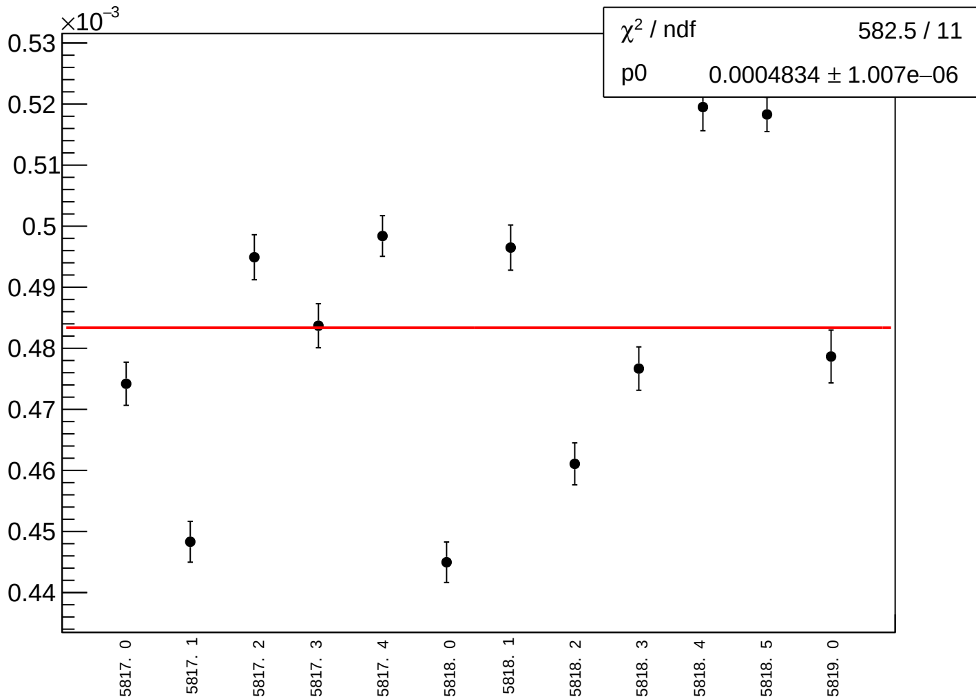
asym_sam_37_48_dd_eigen_dit_vs_dit_diff_rms vs run
