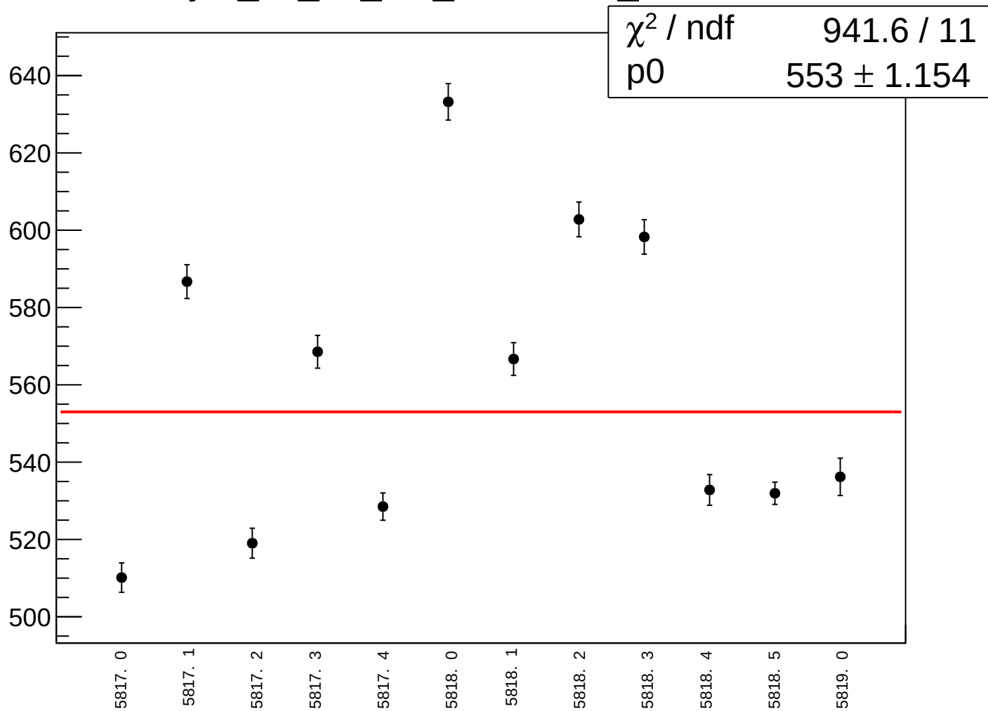
asym_us_dd_cor_correction_rms vs run
