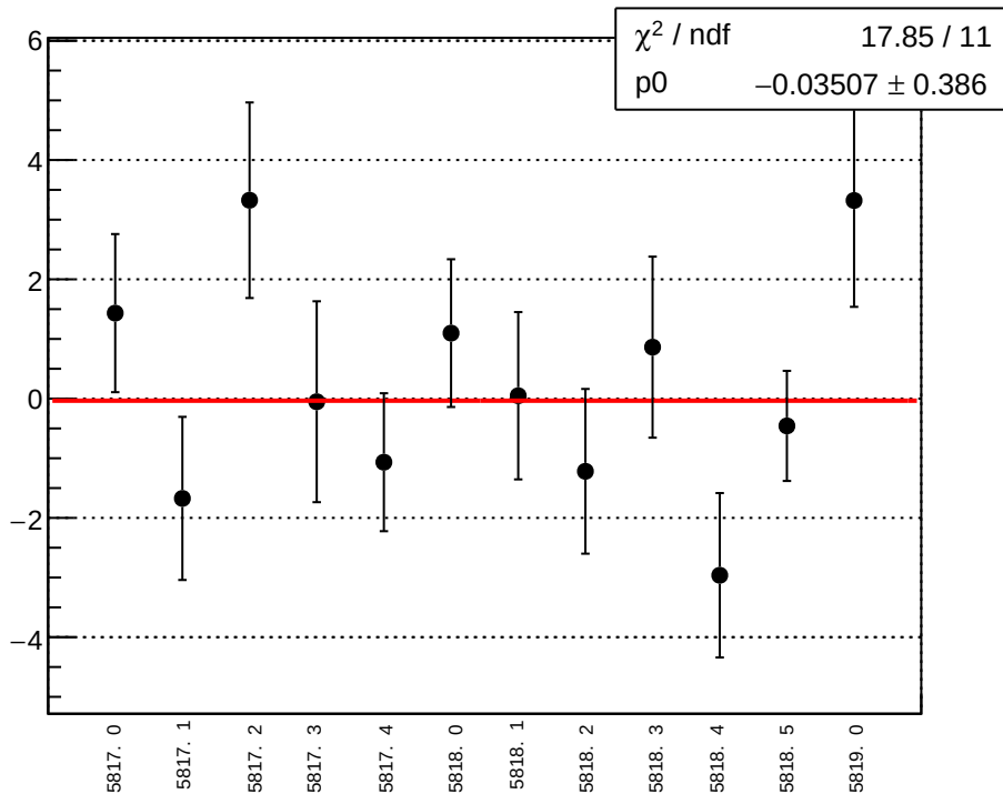
asym_us_avg_dit_vs_overload_cor_diff_mean vs un
