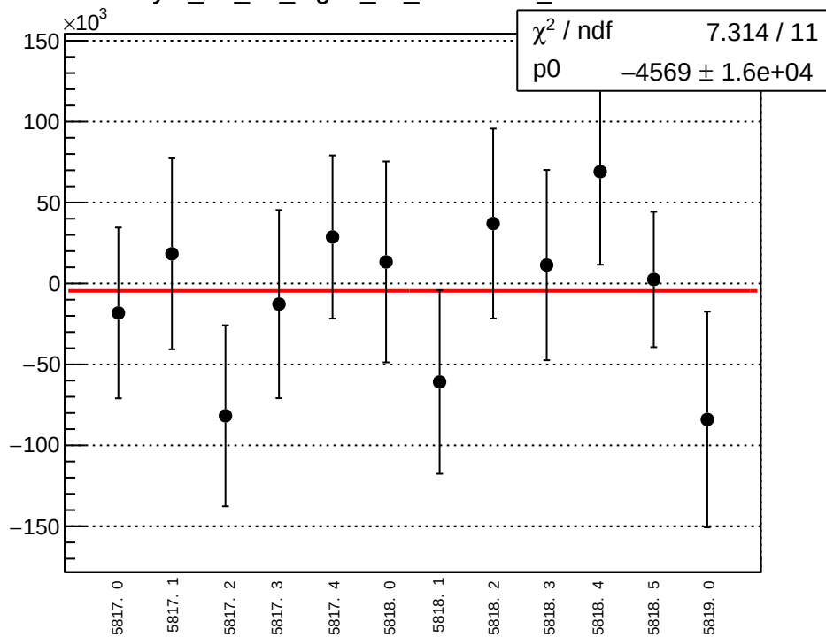
asym_atr_dd_eigen_dit_correction_mean vs run
