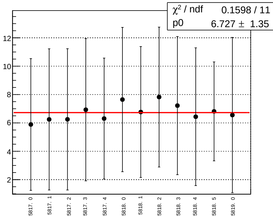
reg_asym_sam_3748_avg_diff_bpm1X_slope vs un
