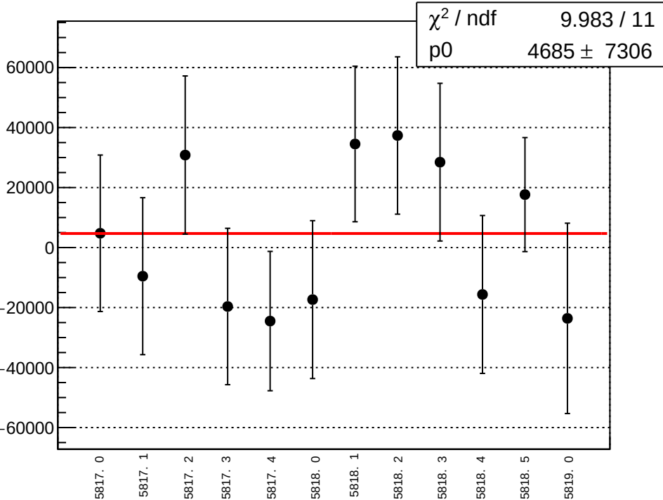
eigen dit asym us avg at1lr avg avg mean vs run
