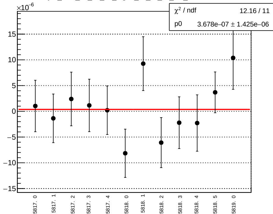
asym_sam_37_48_dd_eigen_dit_vs_dit_diff_mean vs run
