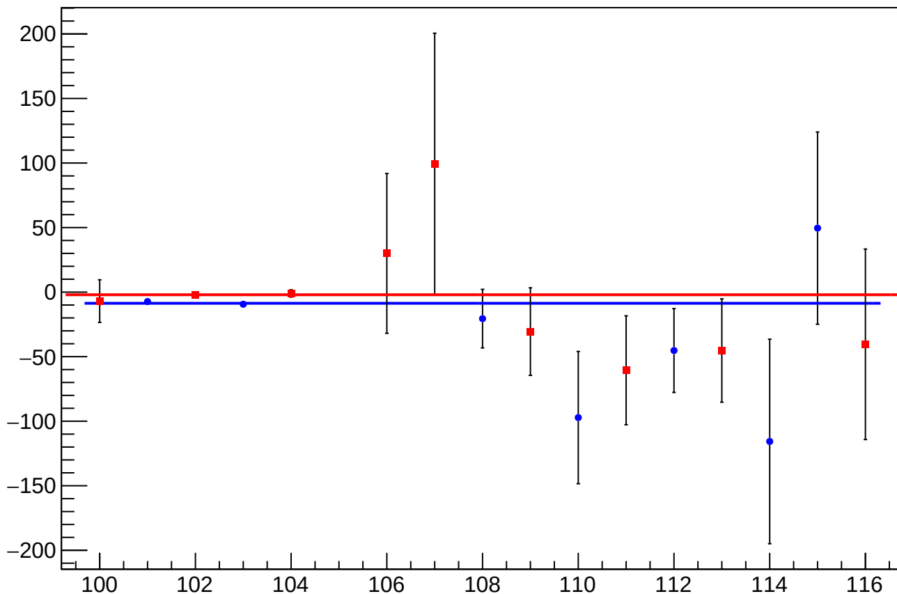
diff_bpm0l03Y_mean vs Slug, Sign Corrected
