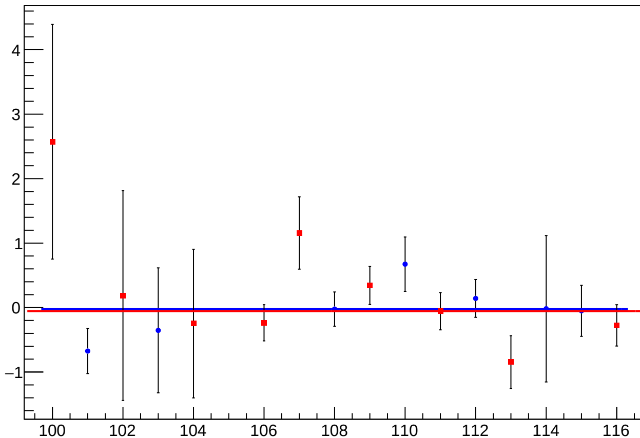
asym_us_avg_atlr_avg_avg_eigen_dit_vs_cor_diff_mean vs Slug, Sign Corrected
