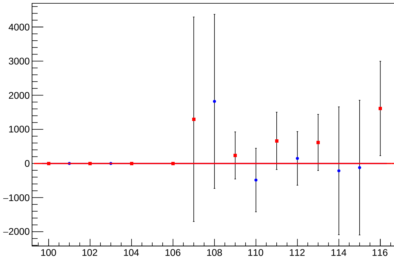
diff_cav4bY_mean vs Slug, Sign Corrected
