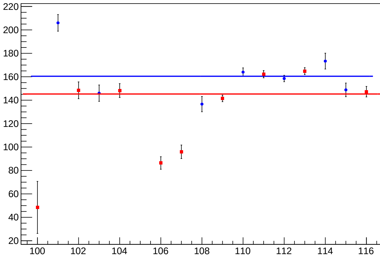
reg_asym_atl1r2_dd_atl2r1_dd_diff_bpm1X_slope vs Slug, Sign Corrected
