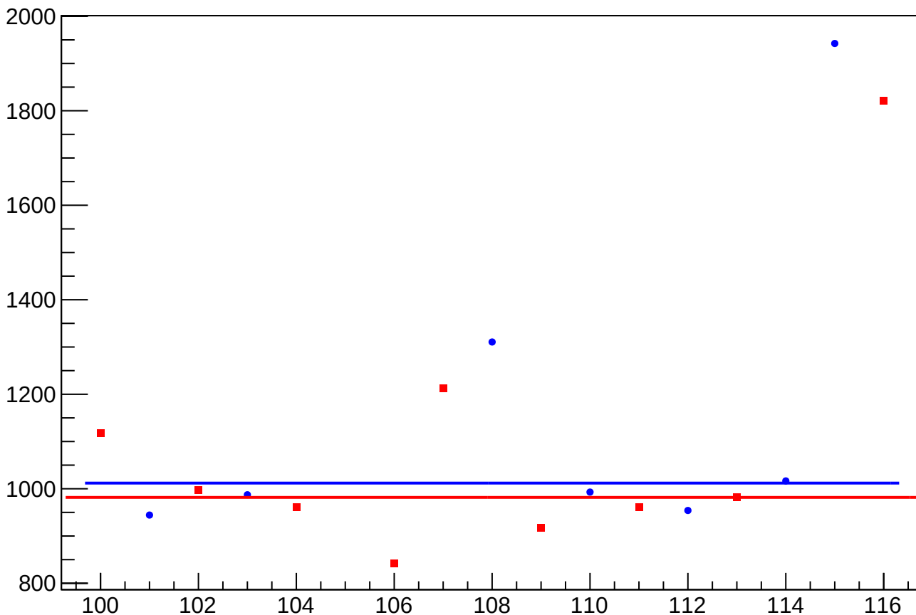
asym_sam_48_dd_dit_correction_rms vs Slug, Sign Corrected
