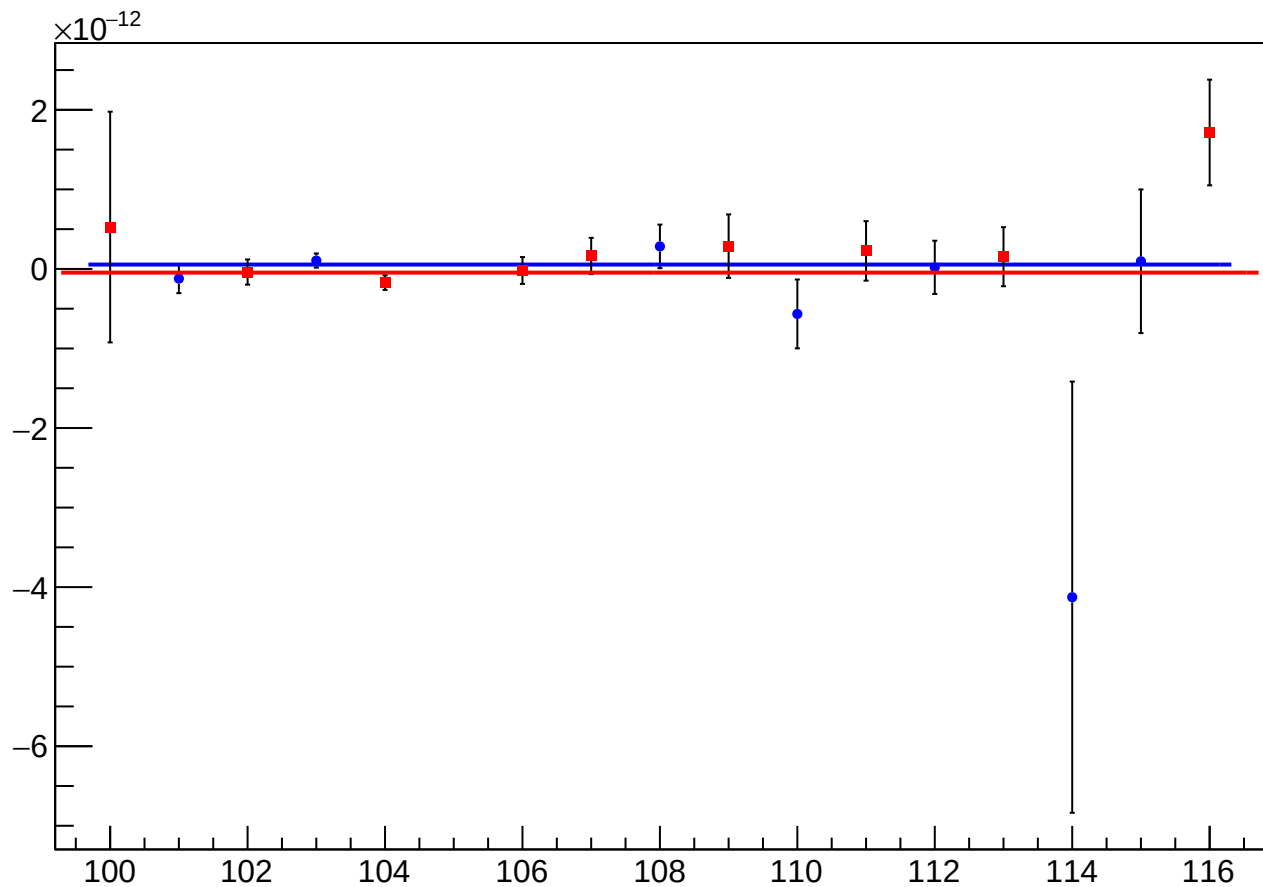
asym_usr_atr2_dd_reg_vs_slug_sign_corrected
