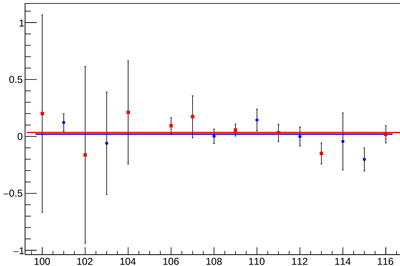
asym_atl_dd_atr_dd_dd_dit_vs_Slug_Sign_Corrected
