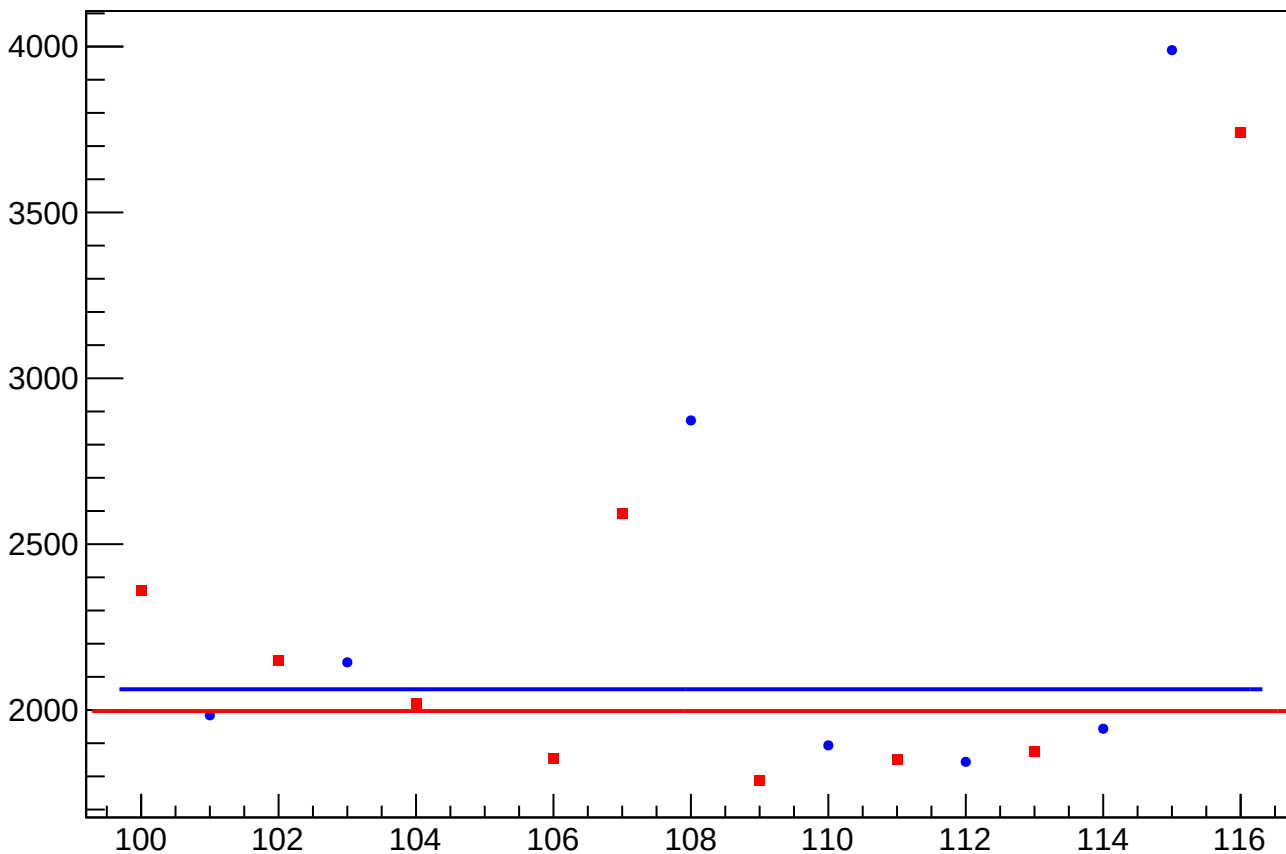
asym_sam4_reg_correction_rms vs Slug, Sign Corrected
