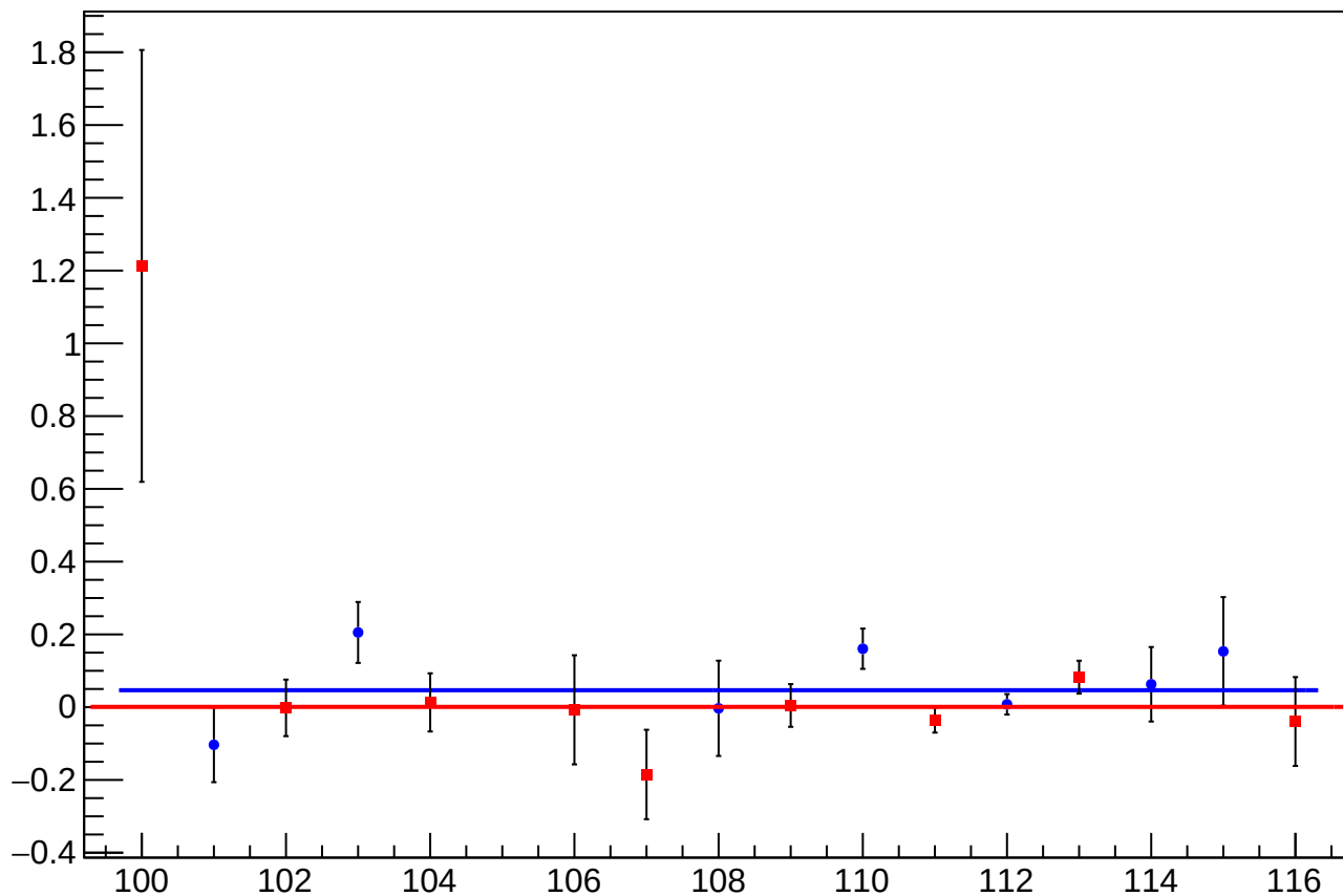
asym_sam_48_avg_dit_vs_slug_Sign_Corrected
