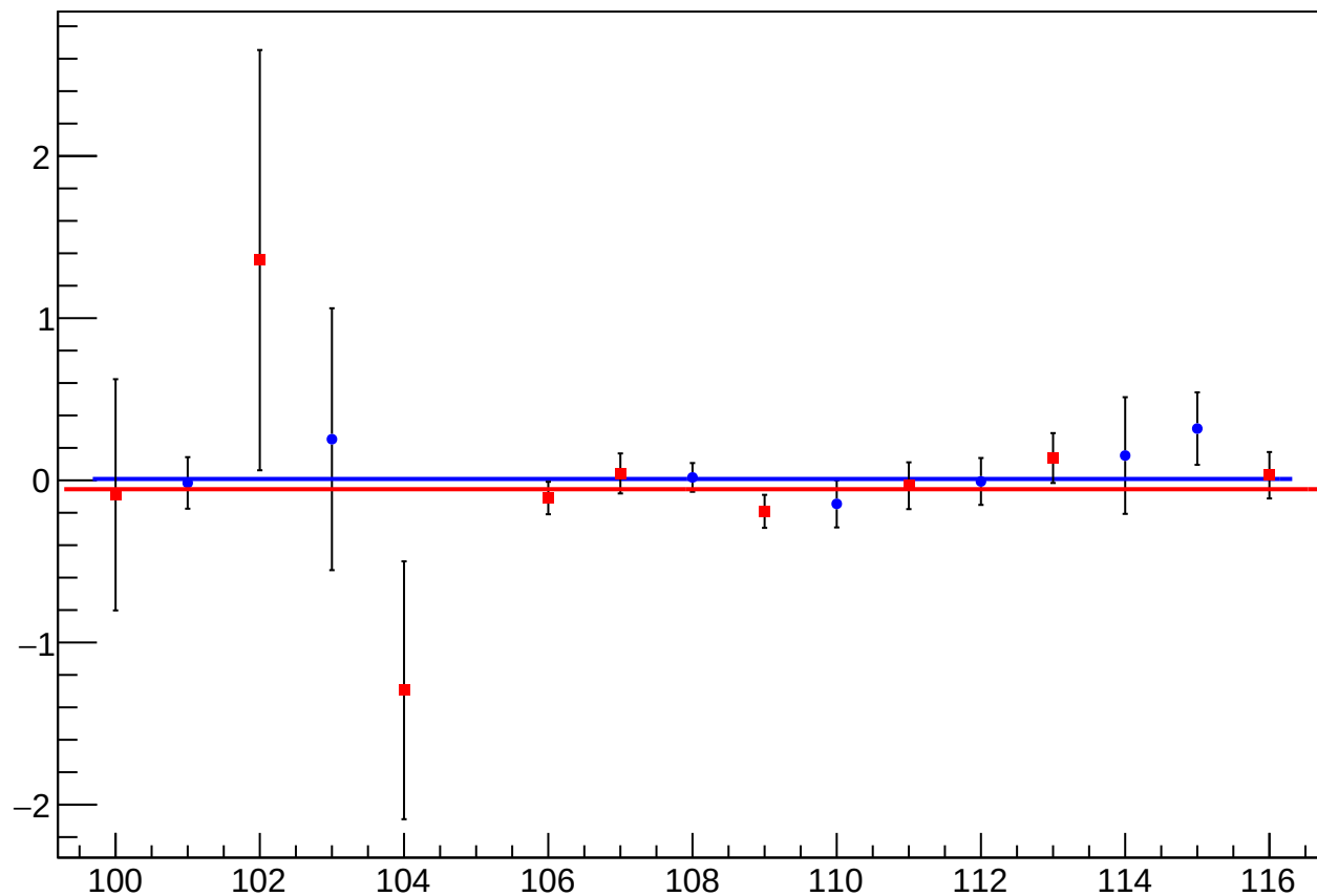
asym_us_dd_at2lr_dd_avg_eigen_dit_vs_slug_Sign_Corrected
