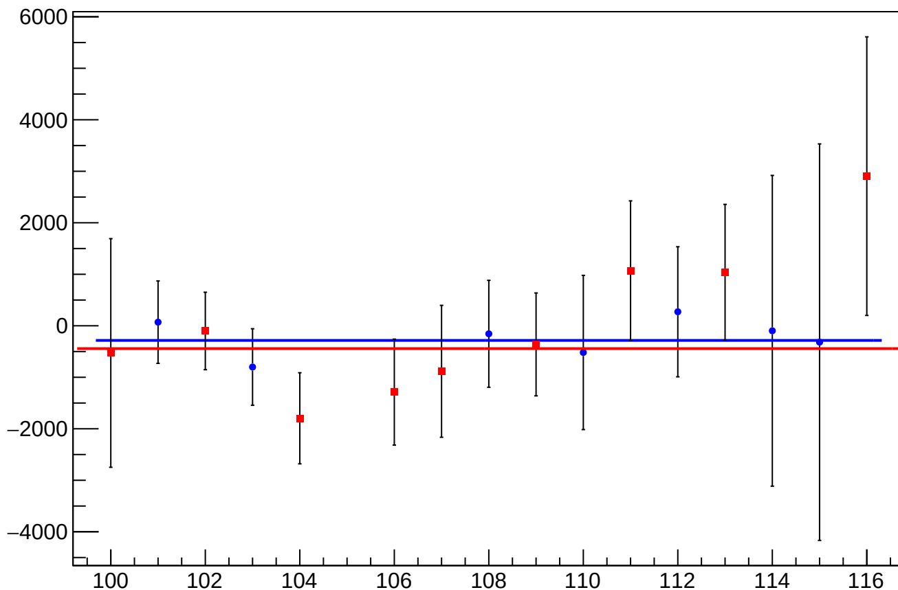
asym_sam_15_dd_dit_correction_mean vs Slug, Sign Corrected
