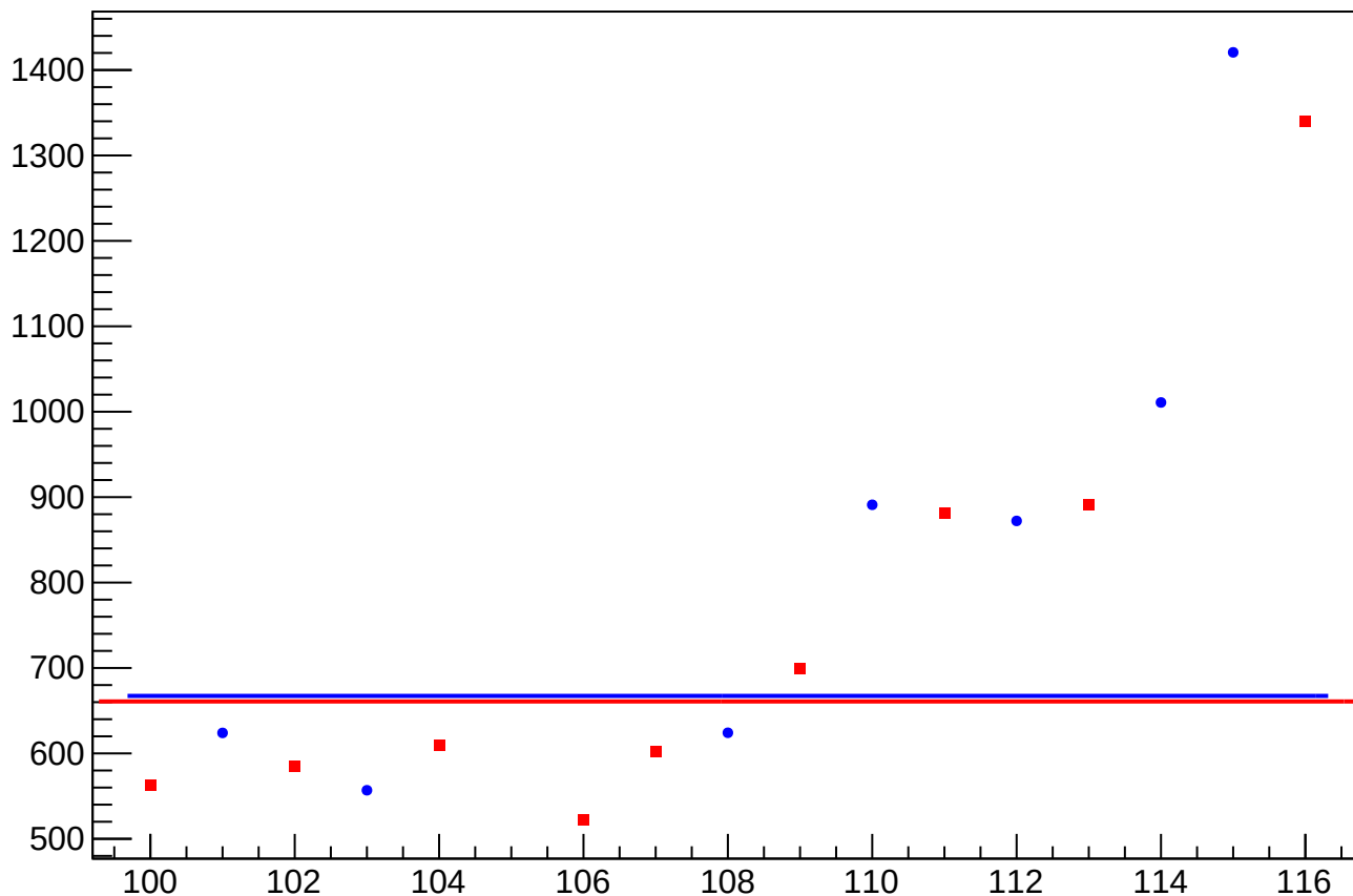
asym_sam_15_dd_eigen_cor_correction_rms vs Slug, Sign Corrected
