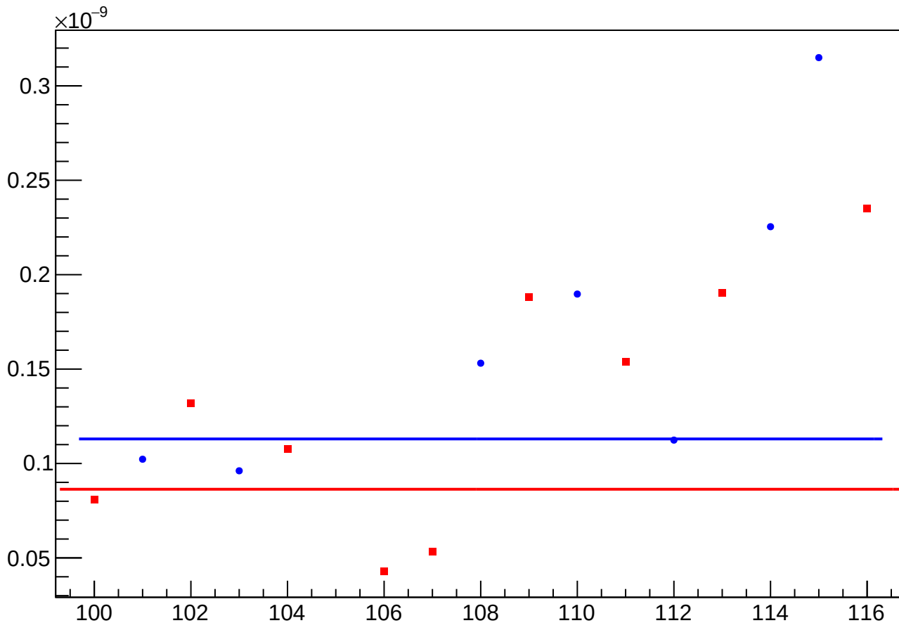
asym_atl1r2_dd_atl2r1_dd_dd_reg_vs_slug, Sign Corrected
