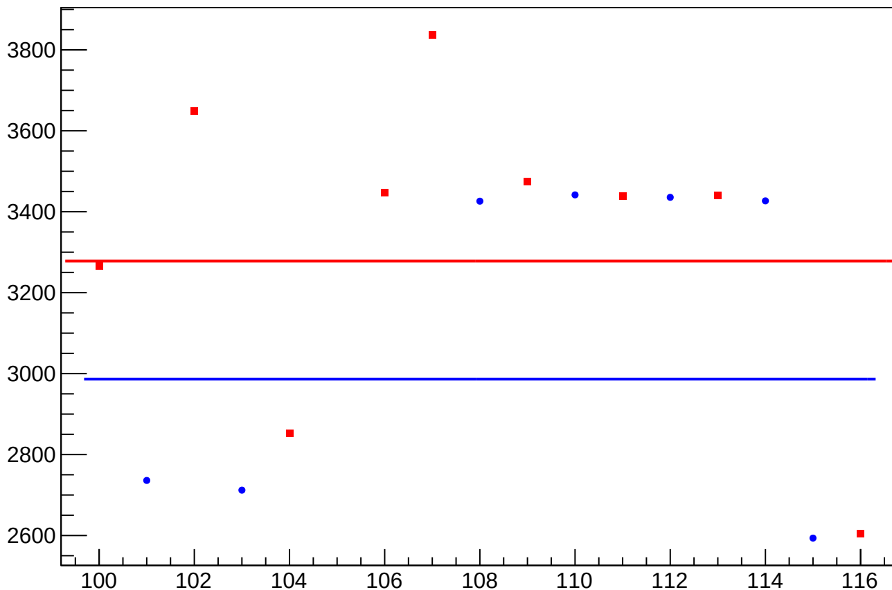
eigen_dit_asym_atl1_rms vs Slug, Sign Corrected
