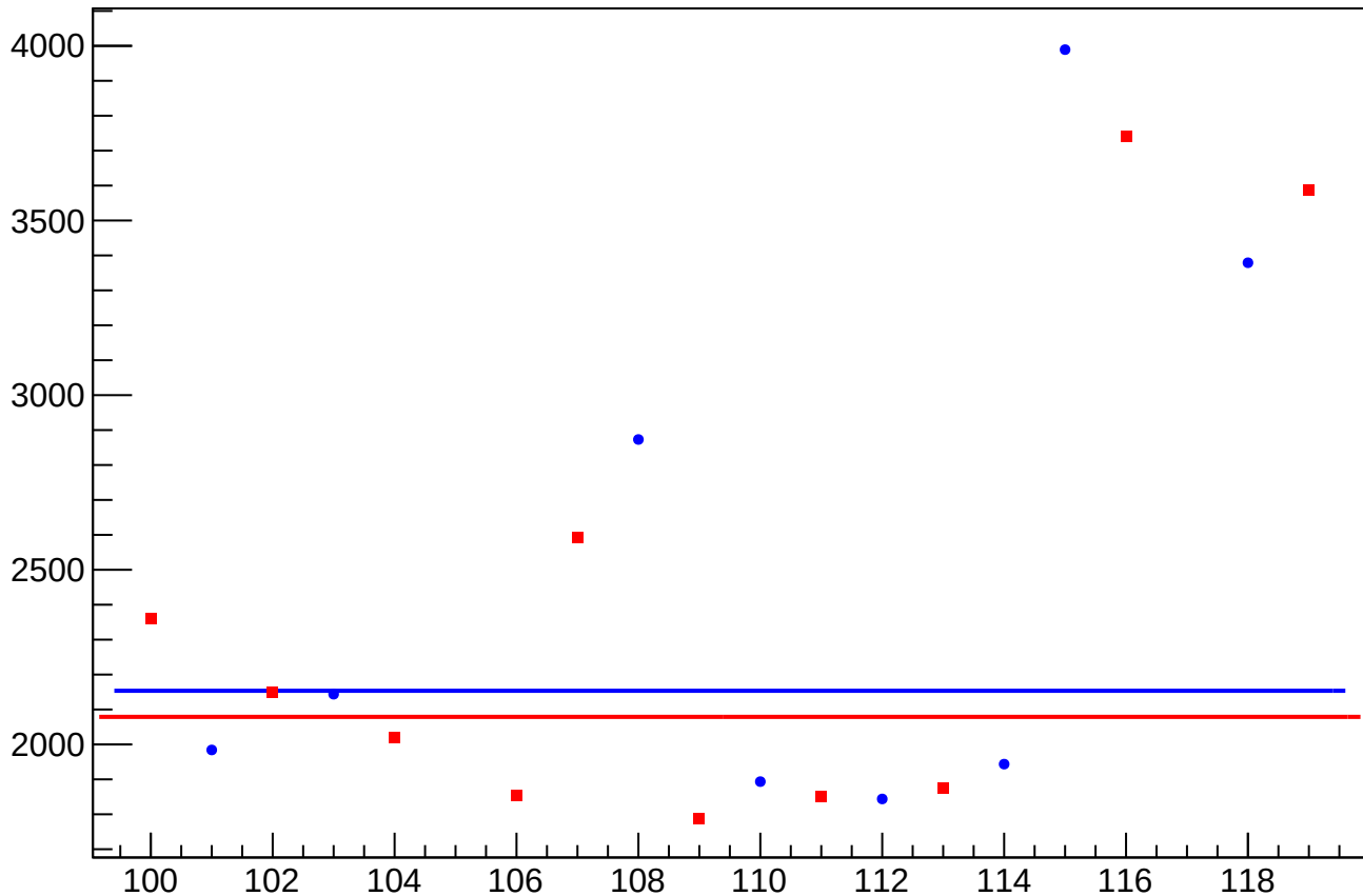
asym_sam4_reg_correction_rms vs Slug
