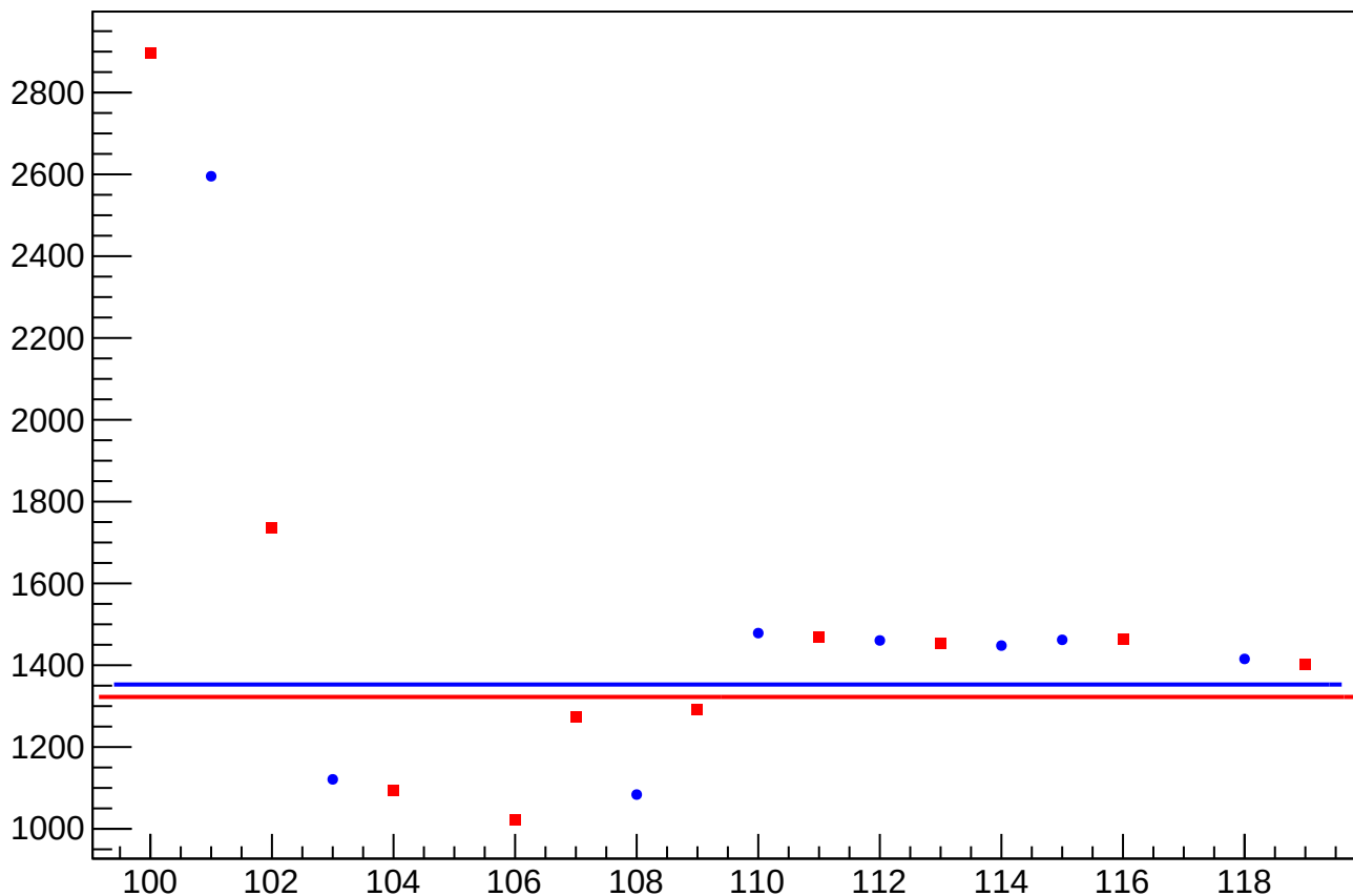
reg_asym_us_dd_at2lr_dd_dd_rms vs Slug
