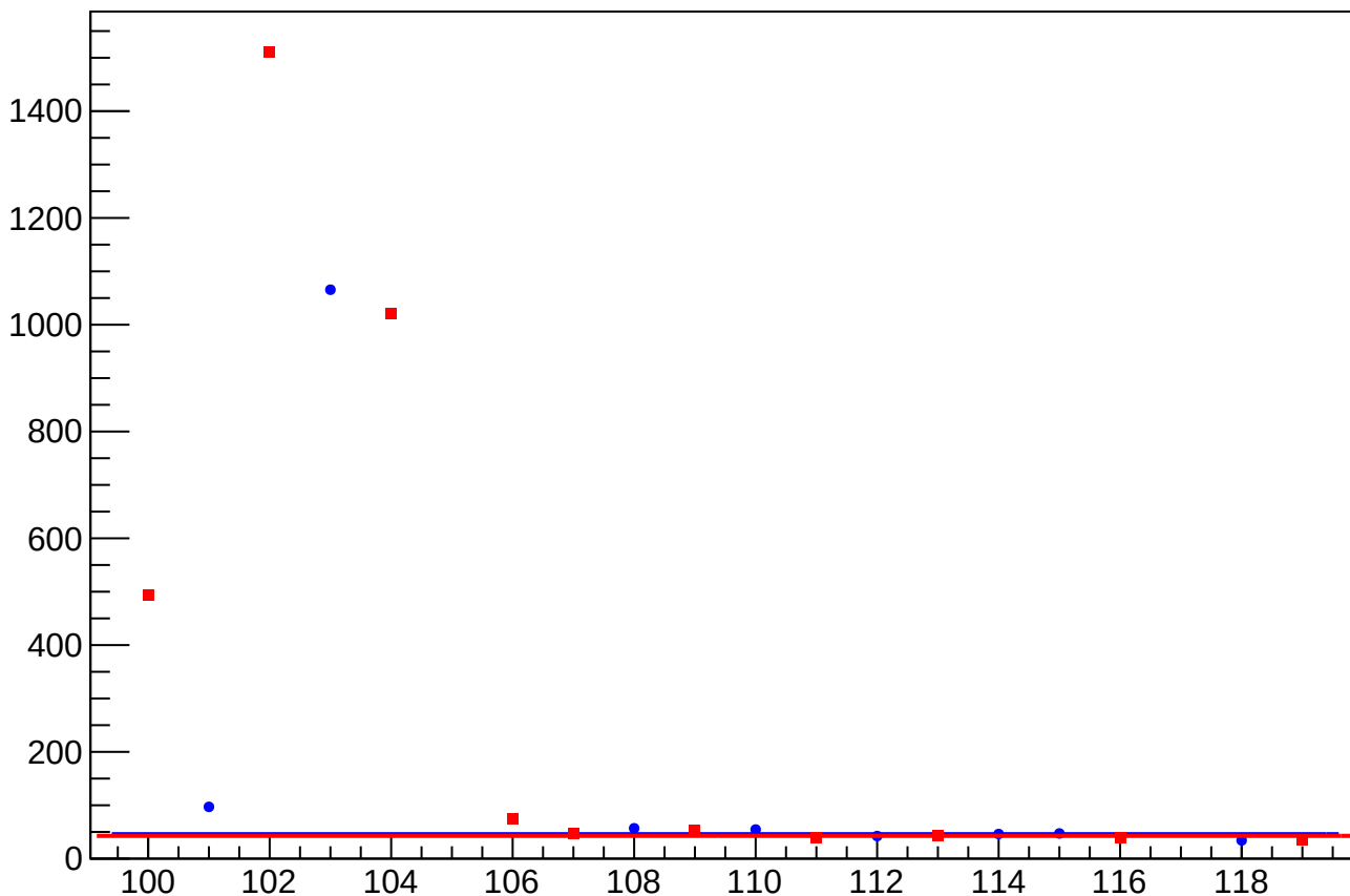
asym_us_avg_at1lr_avg_dd_dit_vs_cor_diff_rms vs Slug
