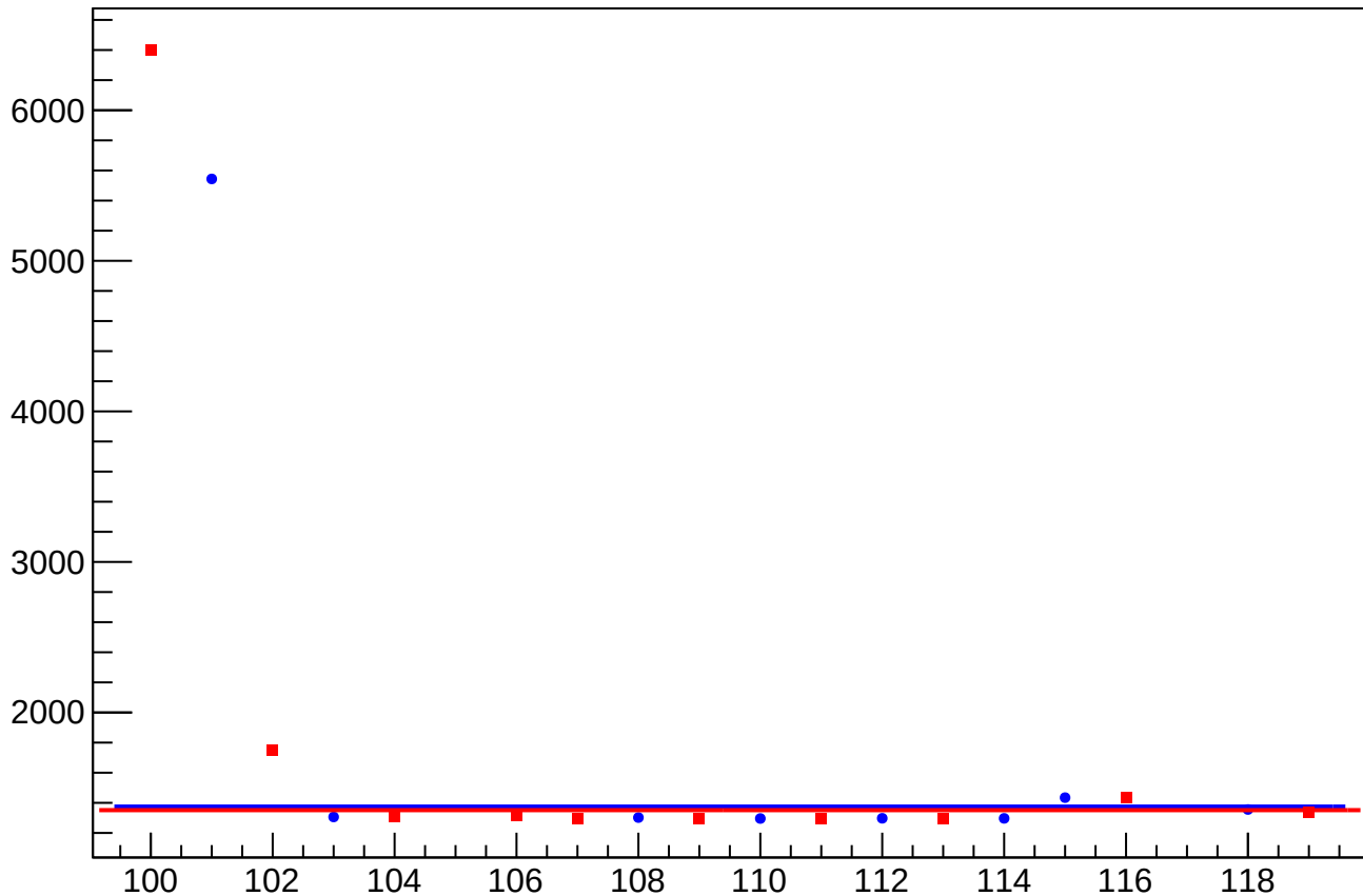
reg_asym_usr_atr1_dd_rms vs Slug
