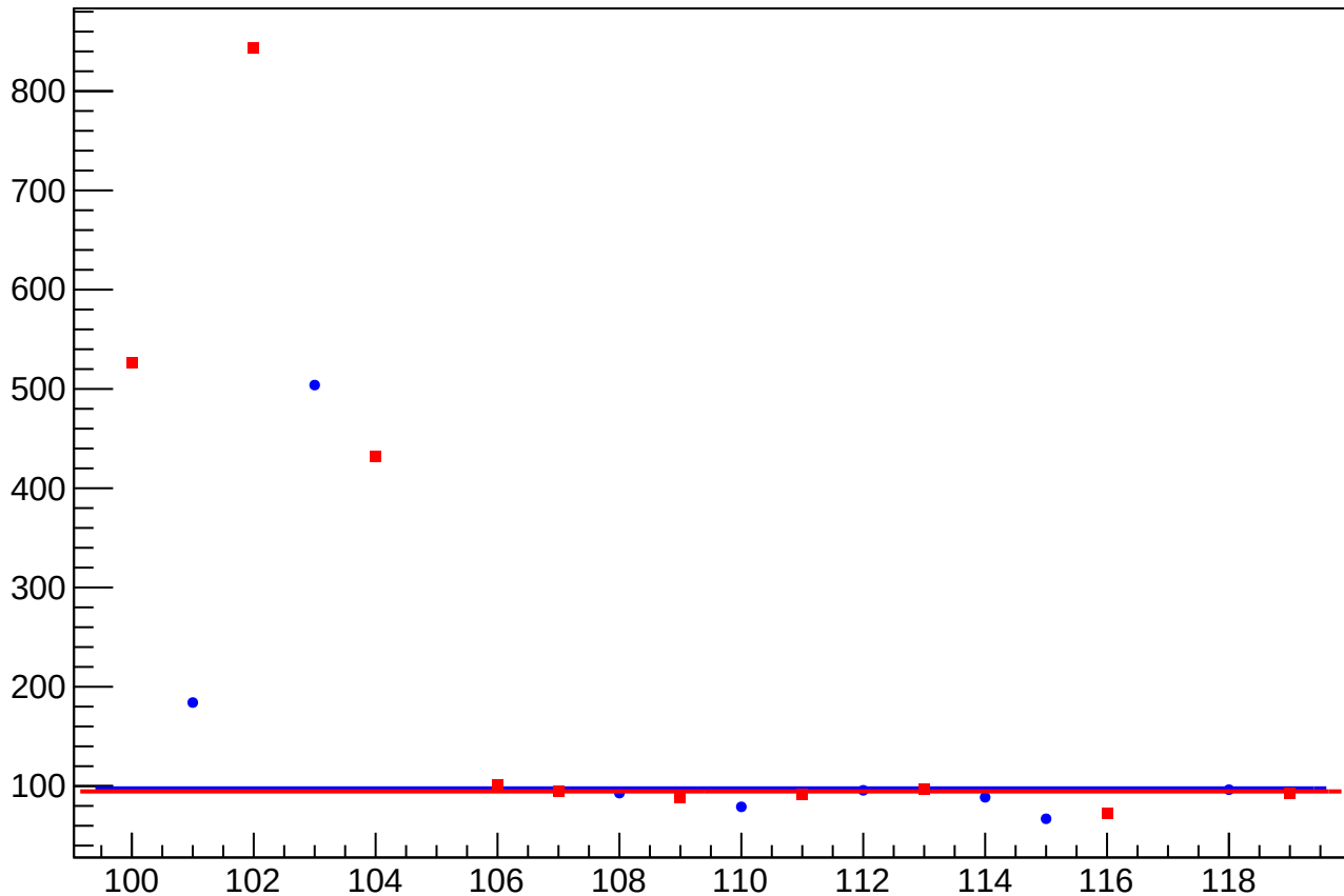
asym_atl_dd_eigen_dit_vs_cor_diff_rms vs Slug
