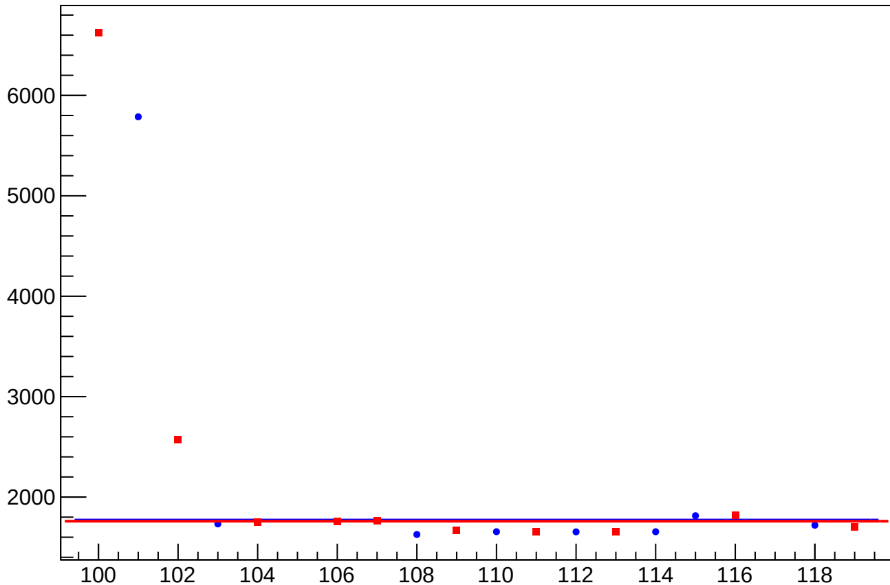
dit_asym_atr1l2_avg_rms vs Slug
