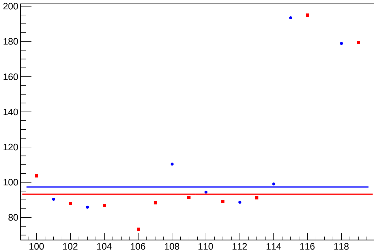
eigen_dit_asym_sam5_rms vs Slug
