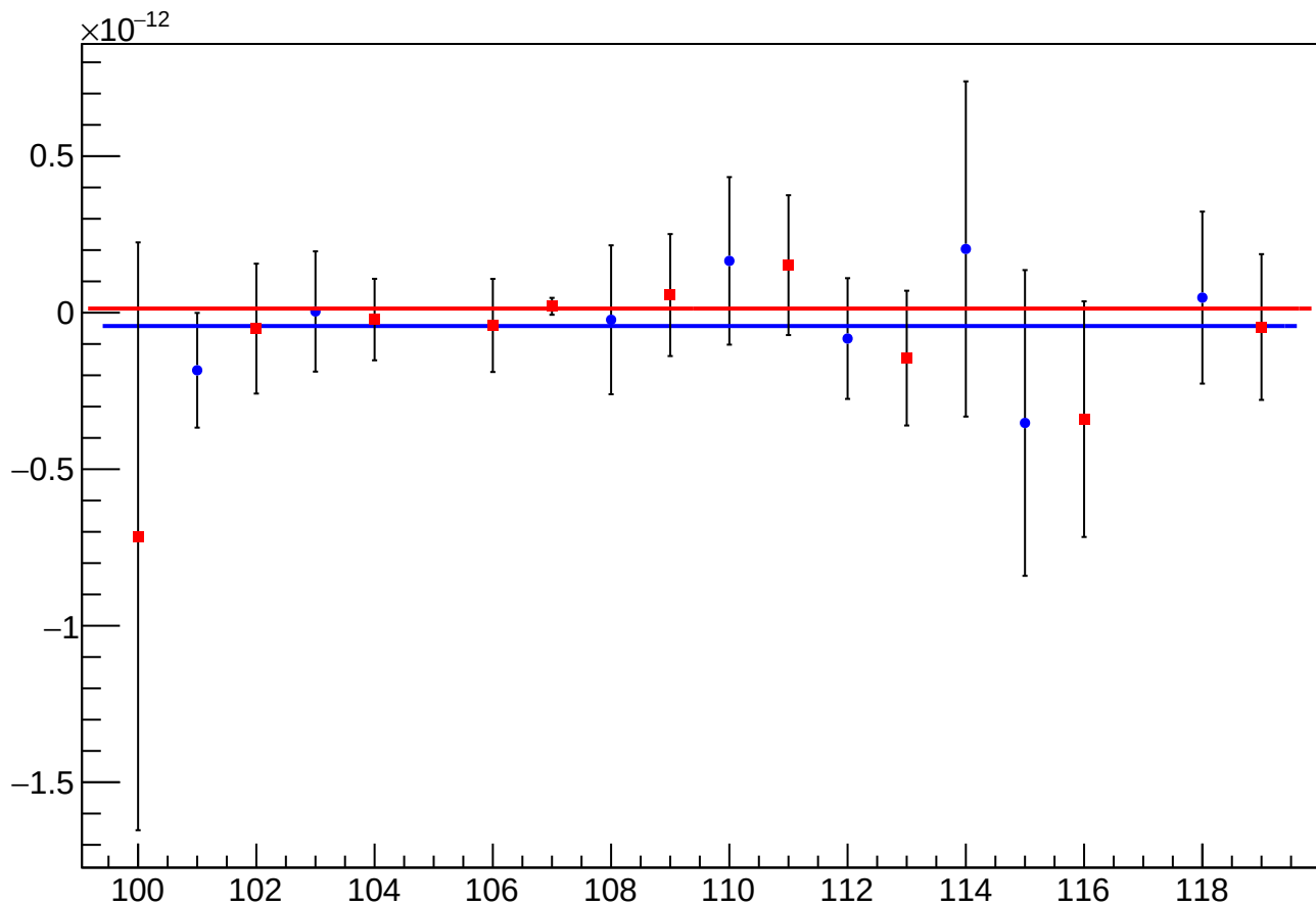
asym_atl1r2_dd_eigen_cor_vs_cor_diff_mean vs Slug
