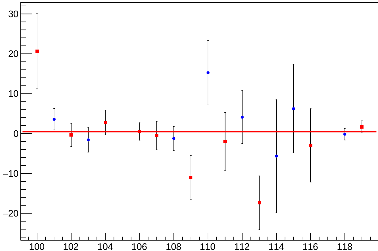
diff_bpmtargetdiffX_mean vs Slug
