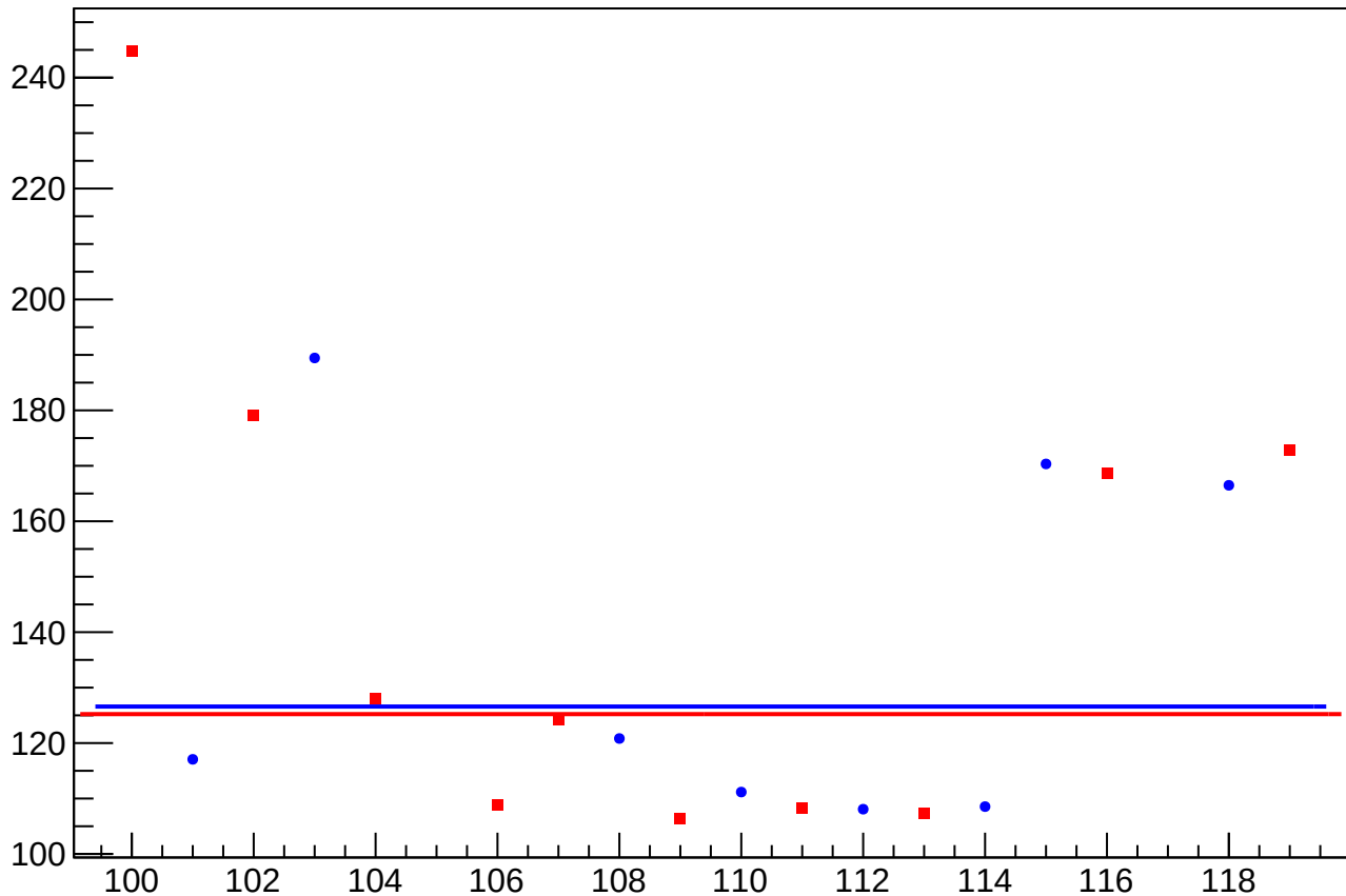
cor_asym_sam_48_avg_rms vs Slug
