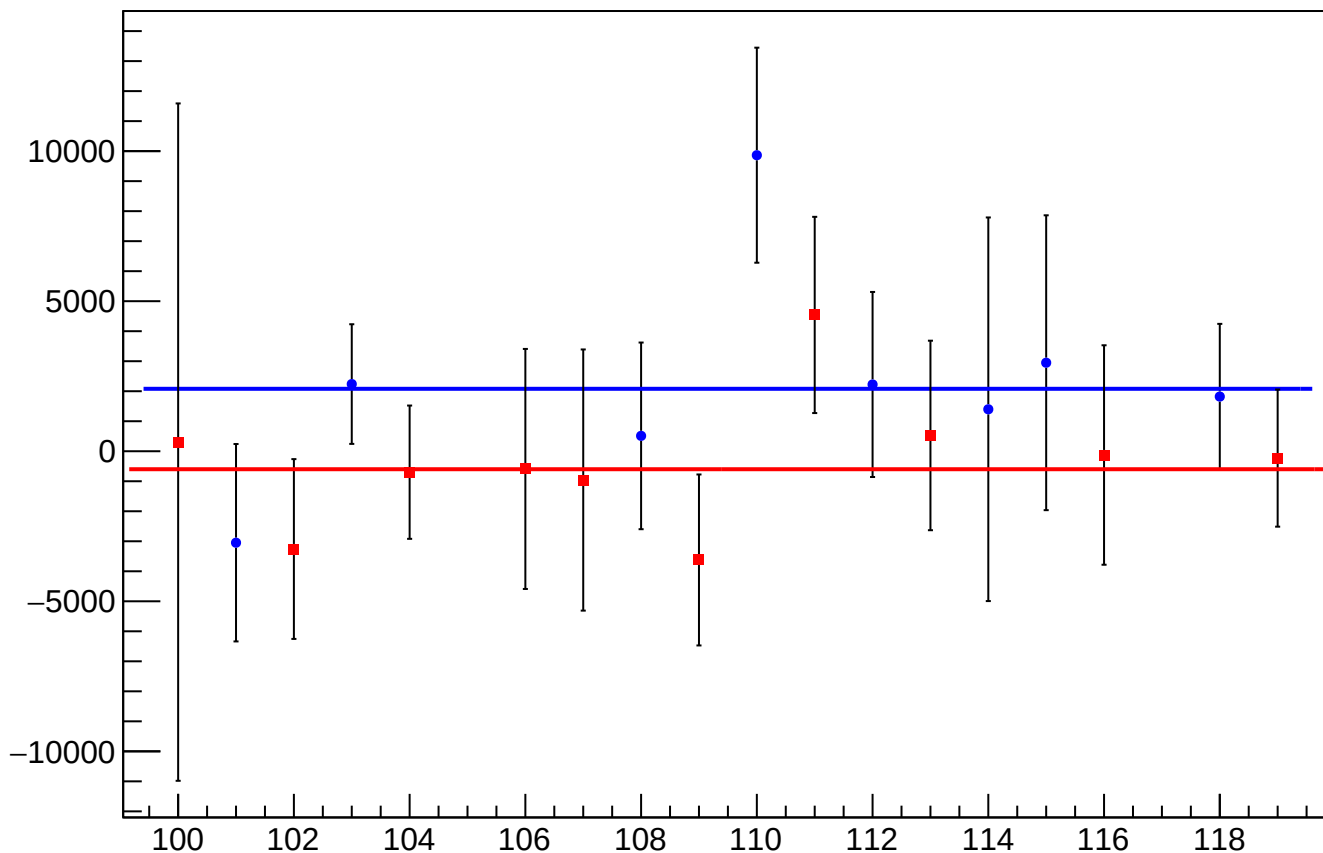
cor_asym_atl1r2_avg_mean vs Slug
