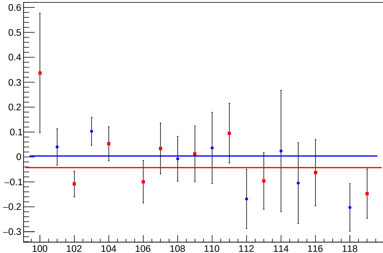
asym_usr_overload_cor_vs_cor_diff_mean vs Slug
