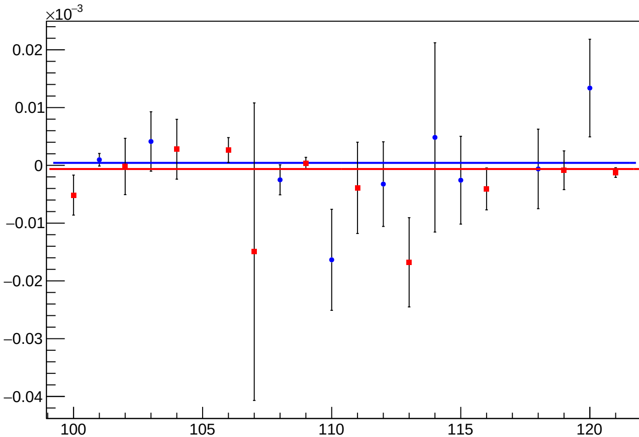
asym us dd eigen dit vs dit diff mean vs Slug, Sign Corrected
