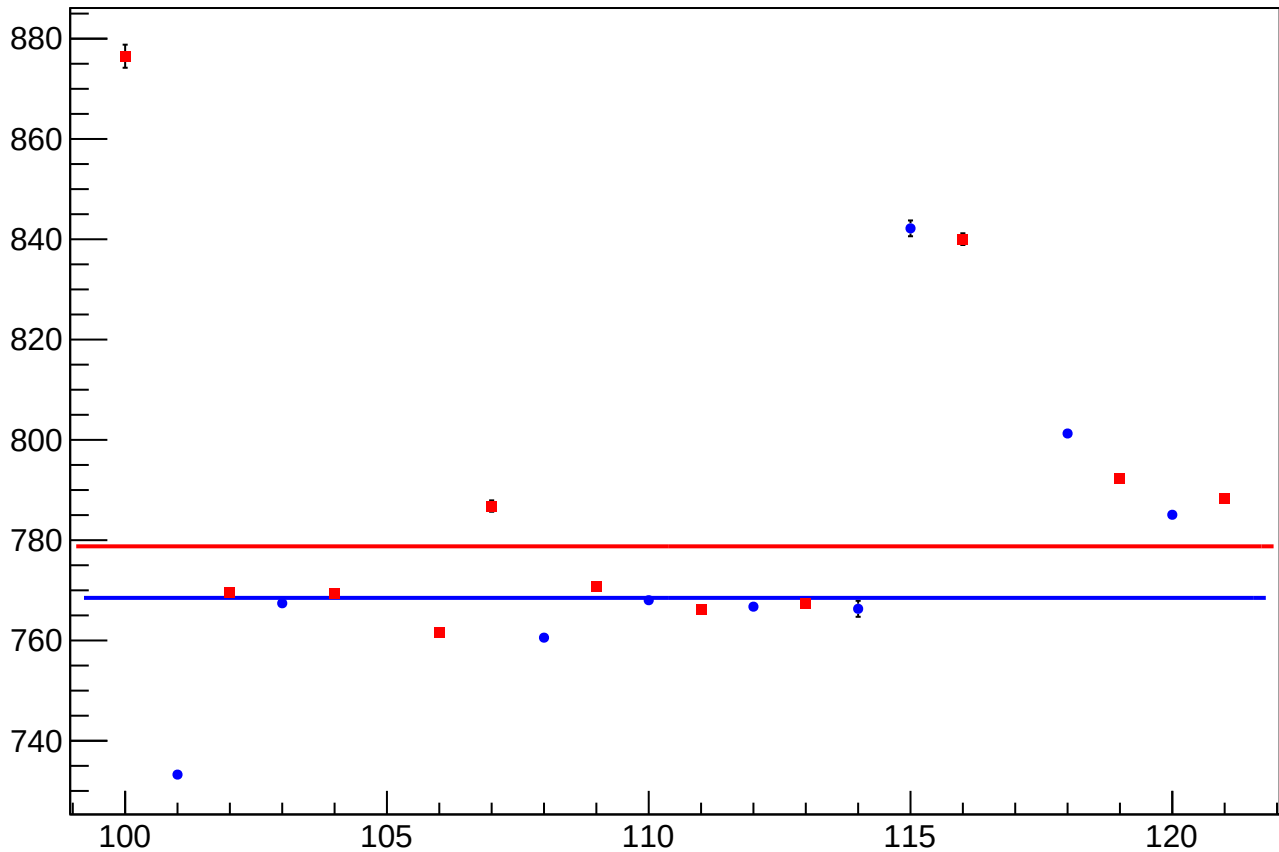
eigen_dit_asym_us_dd_rms vs Slug, Sign Corrected
