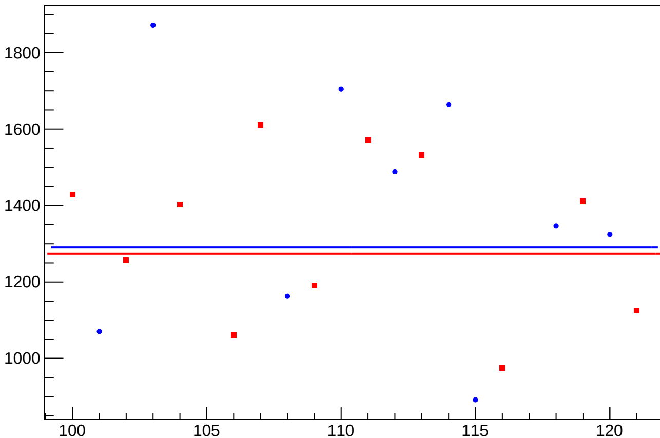
asym_at1_dd_at2_dd_avg_cor_correction_rms vs Slug, Sign Corrected
