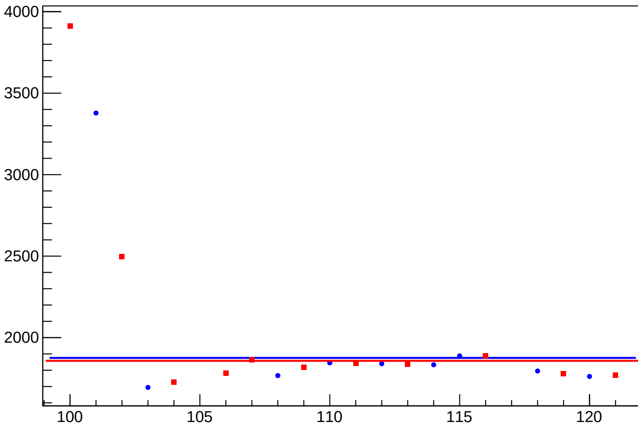
eigen_dit_asym_us_dd_atlr_dd_avg_rms vs Slug, Sign Corrected
