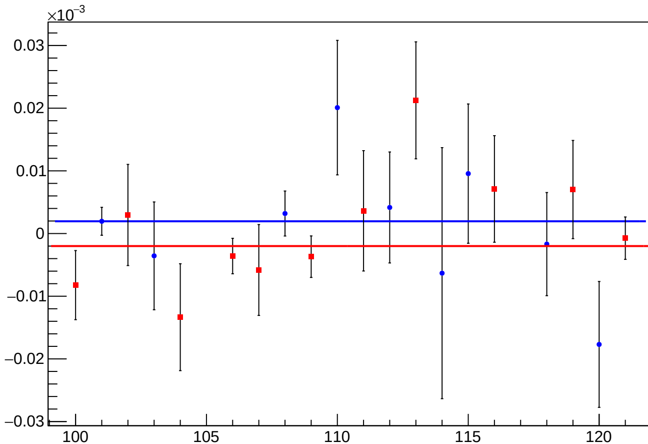
asym_usr_atr1_avg_eigen_dit_vs_dit_diff_mean vs Slug, Sign Corrected
