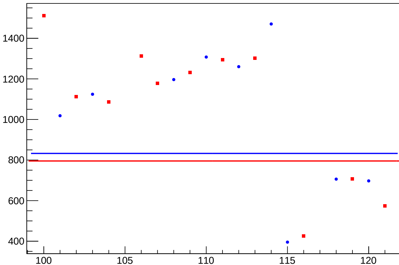
asym_sam_1526_avg_dit_correction_rms vs Slug, Sign Corrected
