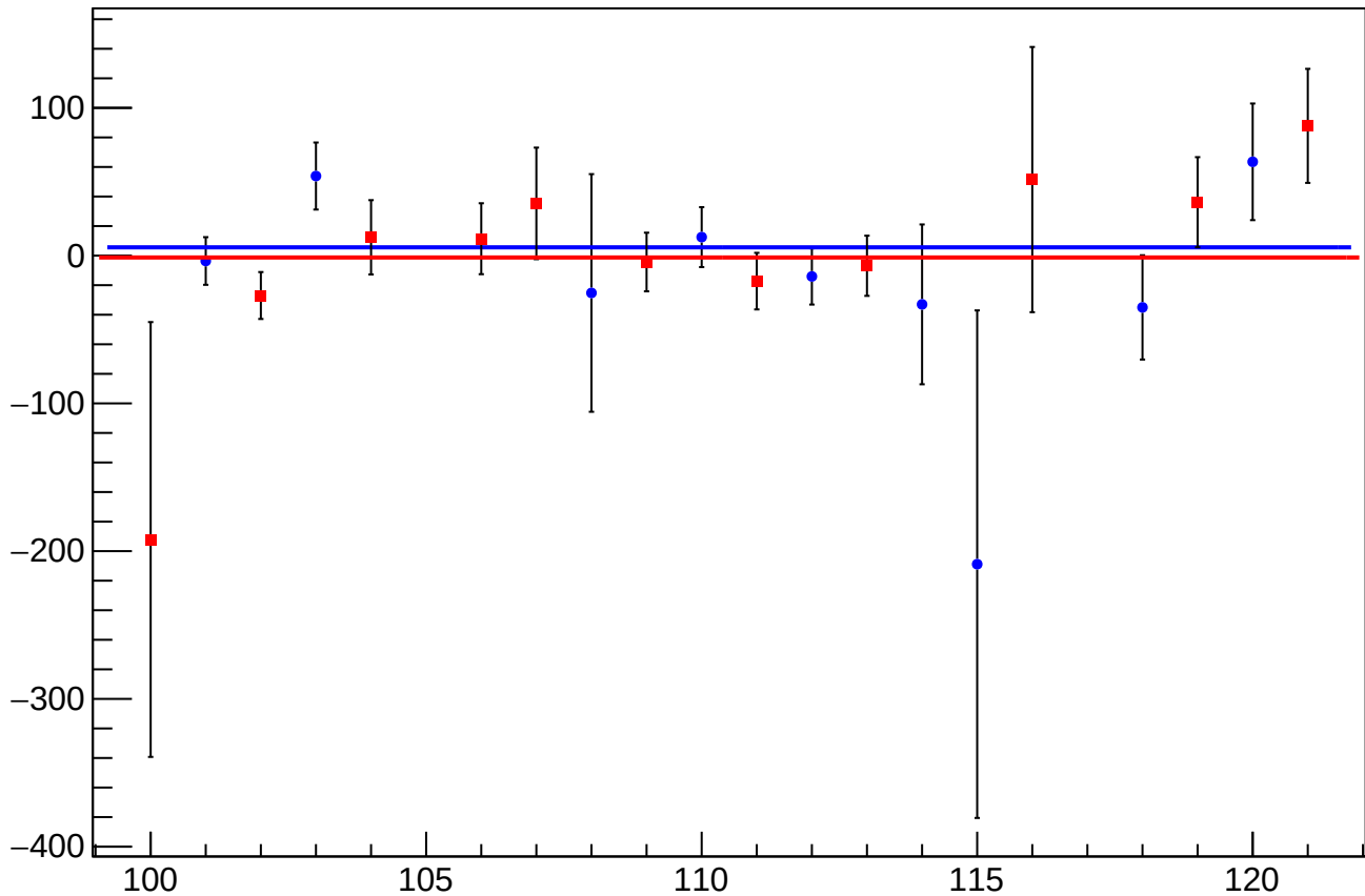
asym_bcm_an_diff_mean vs Slug, Sign Corrected
