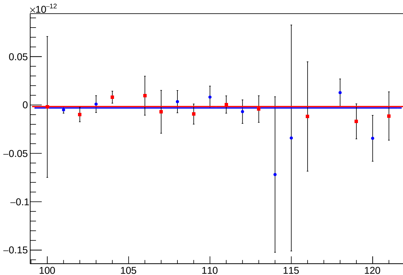
asym_sam_15_avg_reg_vs_cor_diff_mean vs Slug, Sign Corrected
