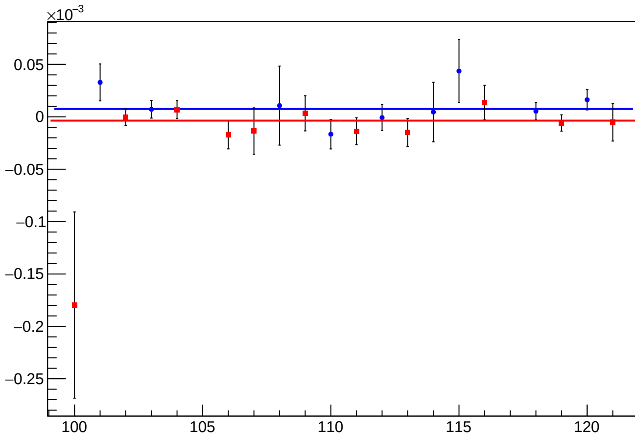
asym_us_dd_at2lr_dd_avg_eigen_dit_vs_dit_diff_mean vs Slug, Sign Corrected
