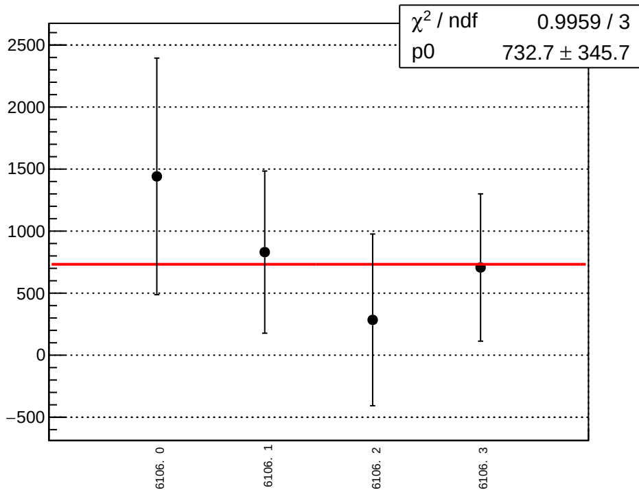
eigen_cor_asym_sam_12345678_avg_mean vs run
