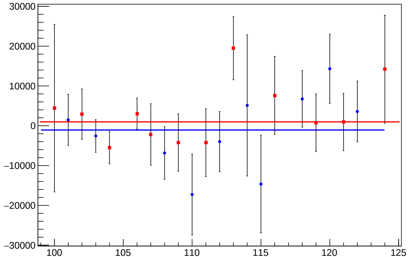
asym_usr_atr2_avg_reg_correction_mean vs Slug
