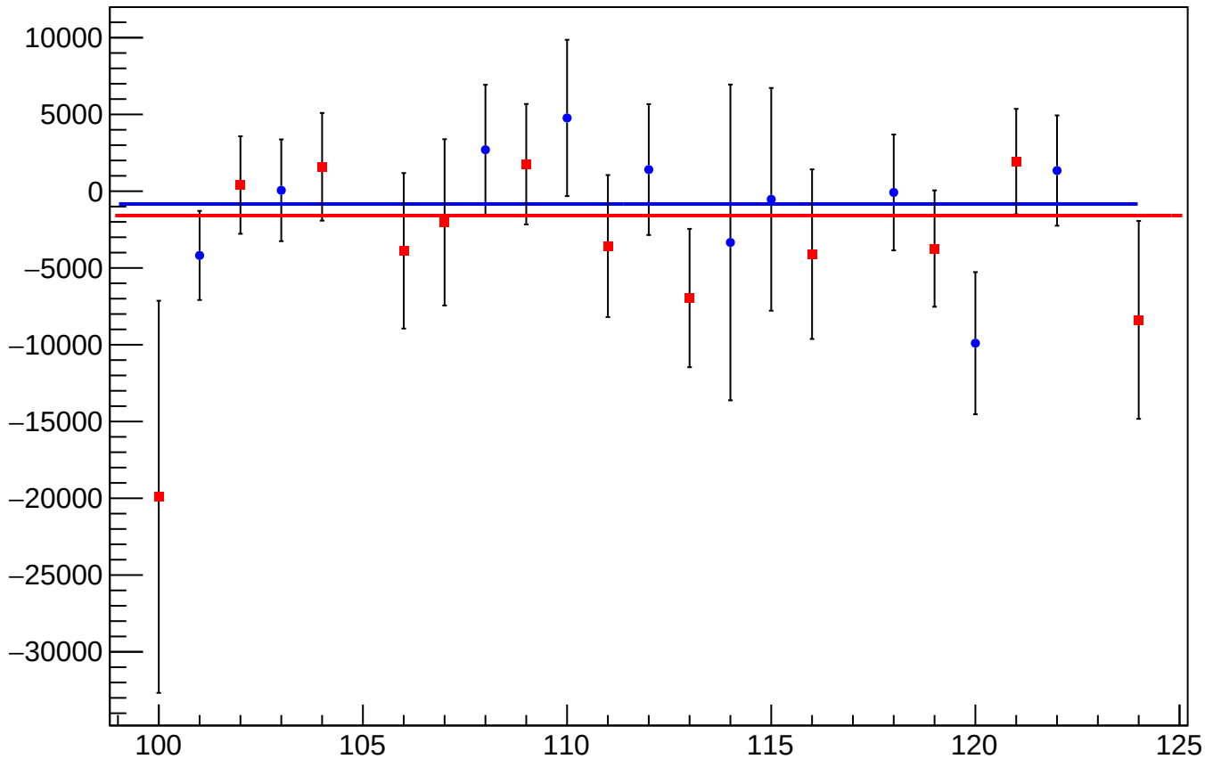
asym_sam_26_dd_dit_correction_mean vs Slug
