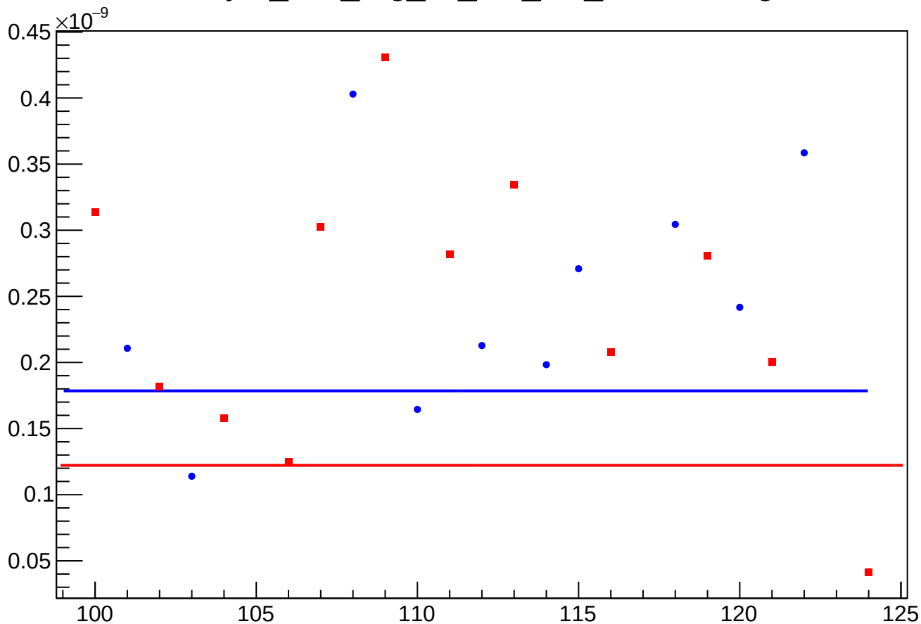
asym_atl2_reg_vs_cor_diff_rms vs Slug
