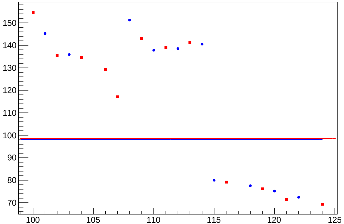
eigen_dit_asym_sam1_rms vs Slug
