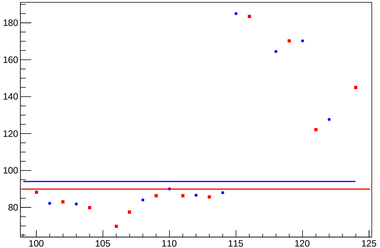
eigen_cor_asym_sam5_rms vs Slug
