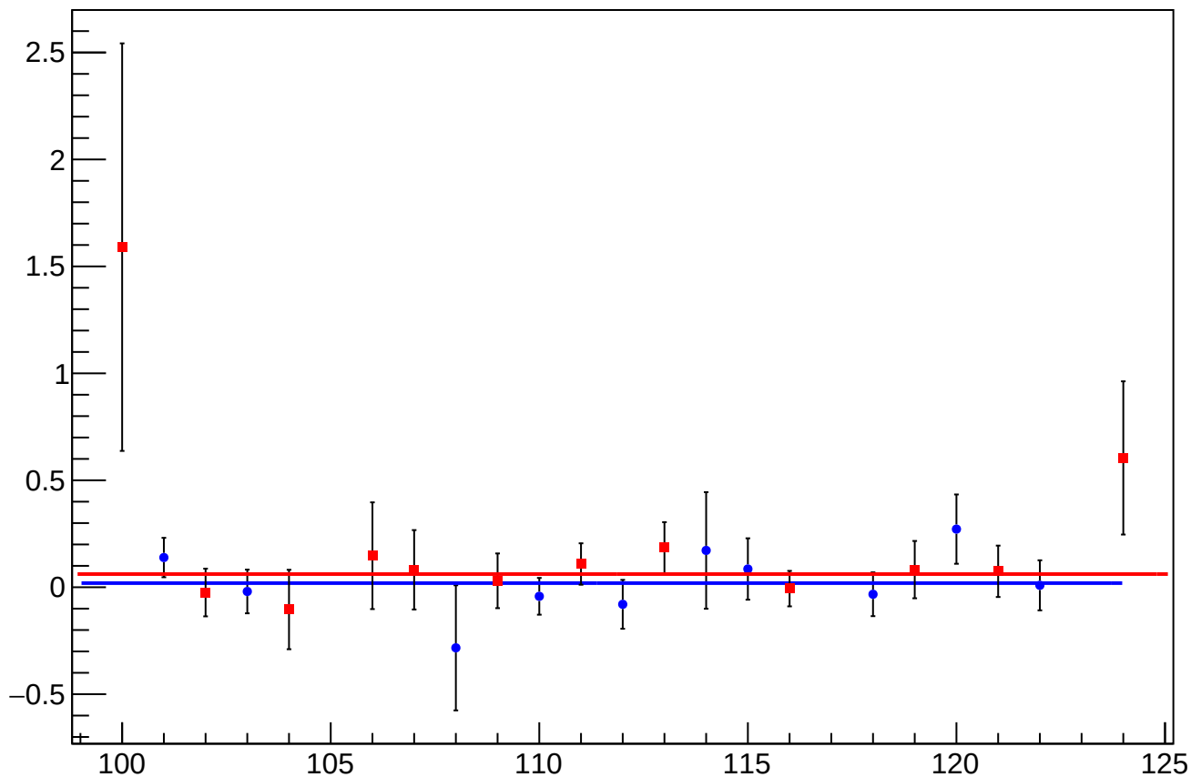
asym_sam3_dit_vs_cor_diff_mean vs Slug
