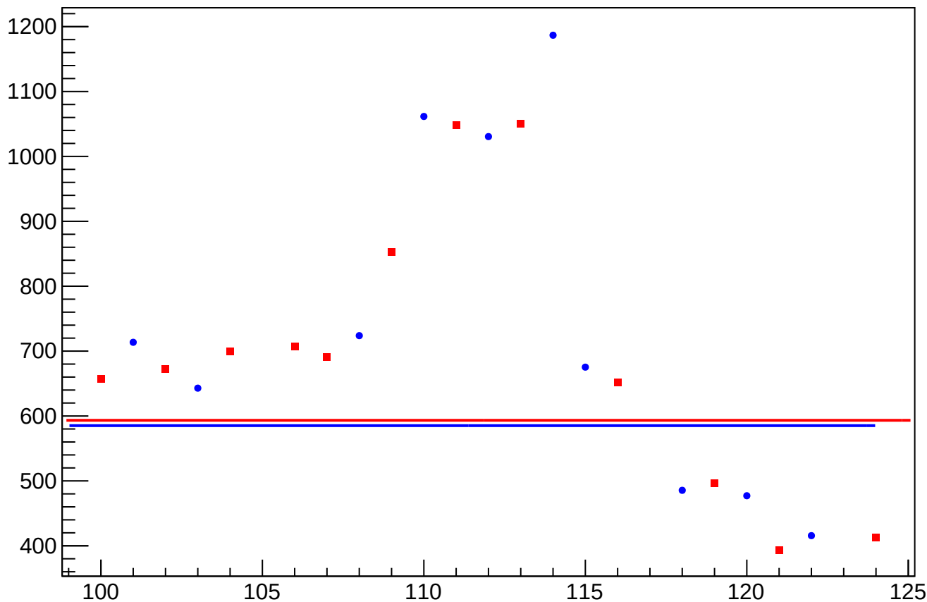
asym_sam1_dit_correction_rms vs Slug
