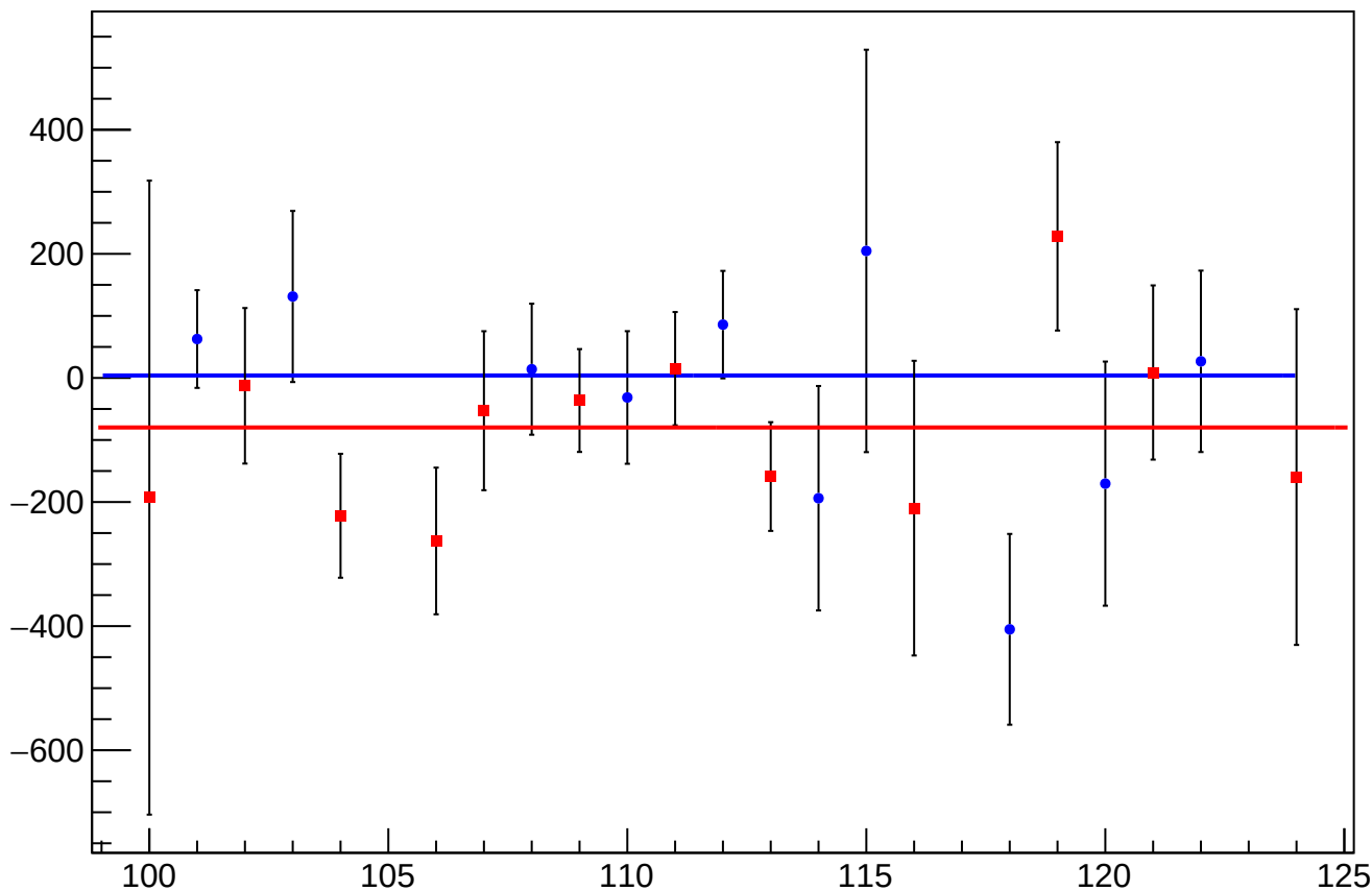
reg_asym_sam_1548_avg_mean vs Slug
