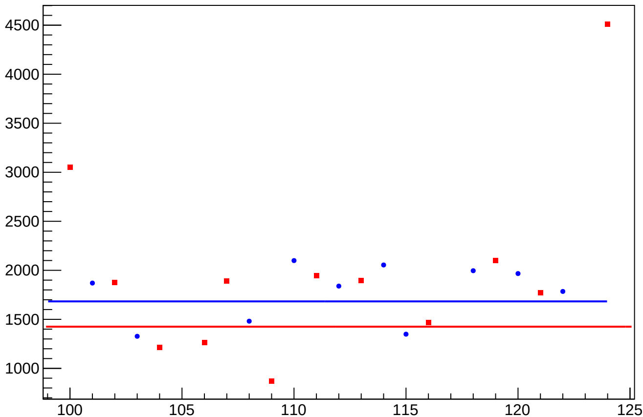
asym_at2_dd_cor_correction_rms vs Slug
