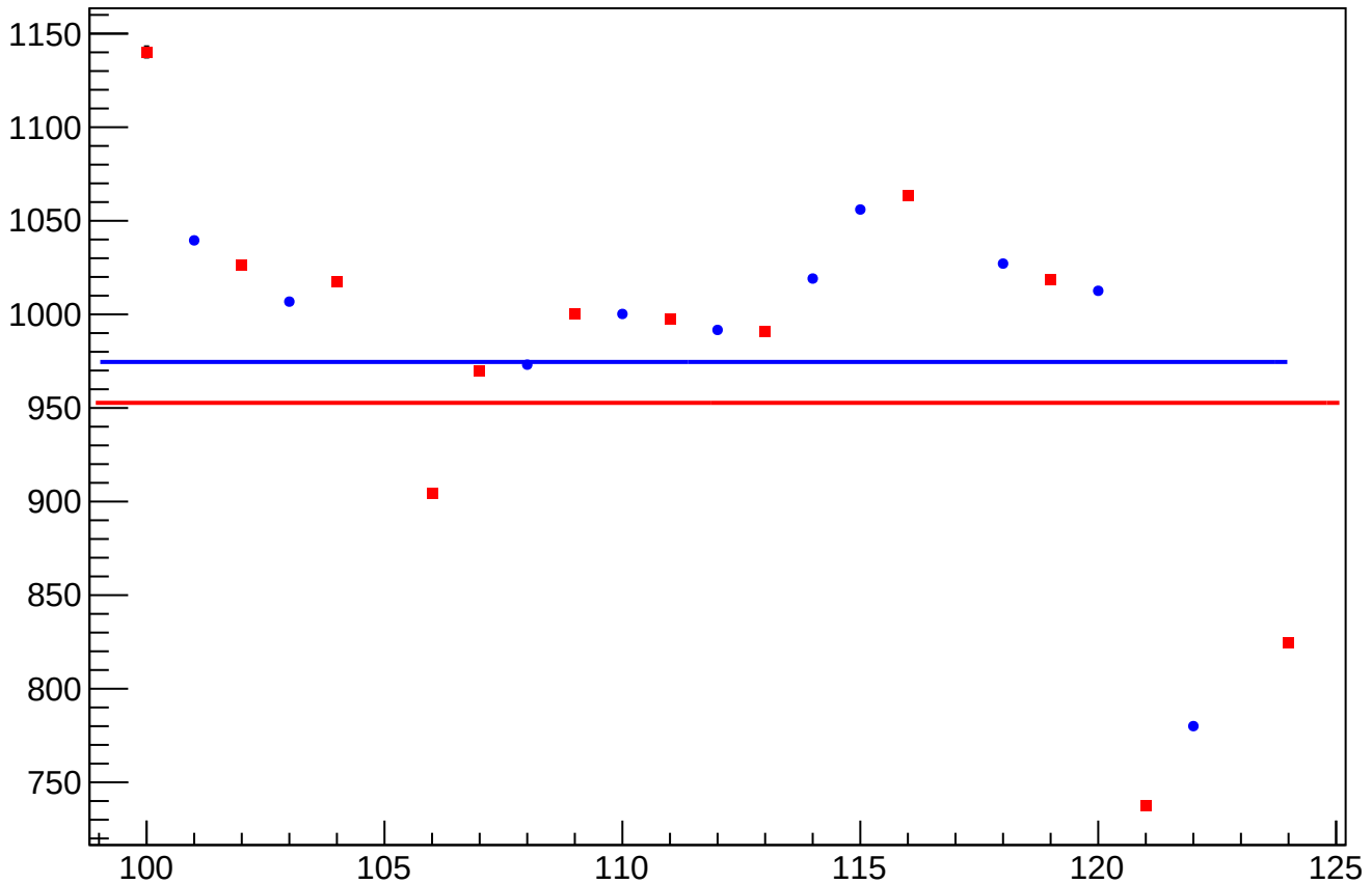
diff_bpm_4aY_4acY_dd_rms vs Slug
