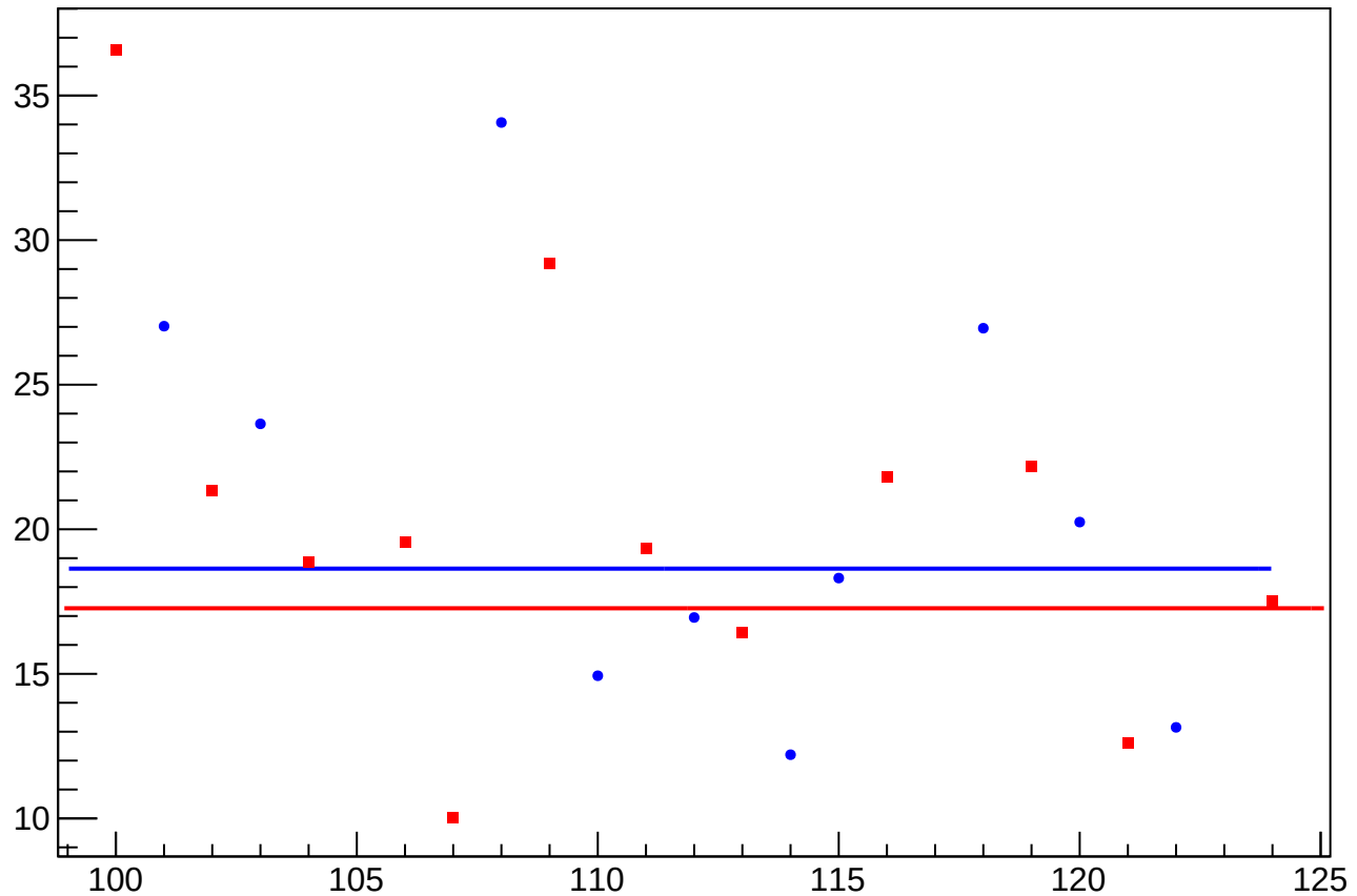
asym_sam_15_avg_dit_vs_cor_diff_rms vs Slug
