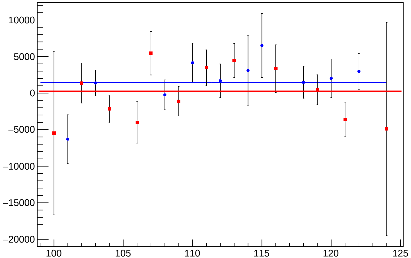
reg_asym_at2_dd_mean vs Slug
