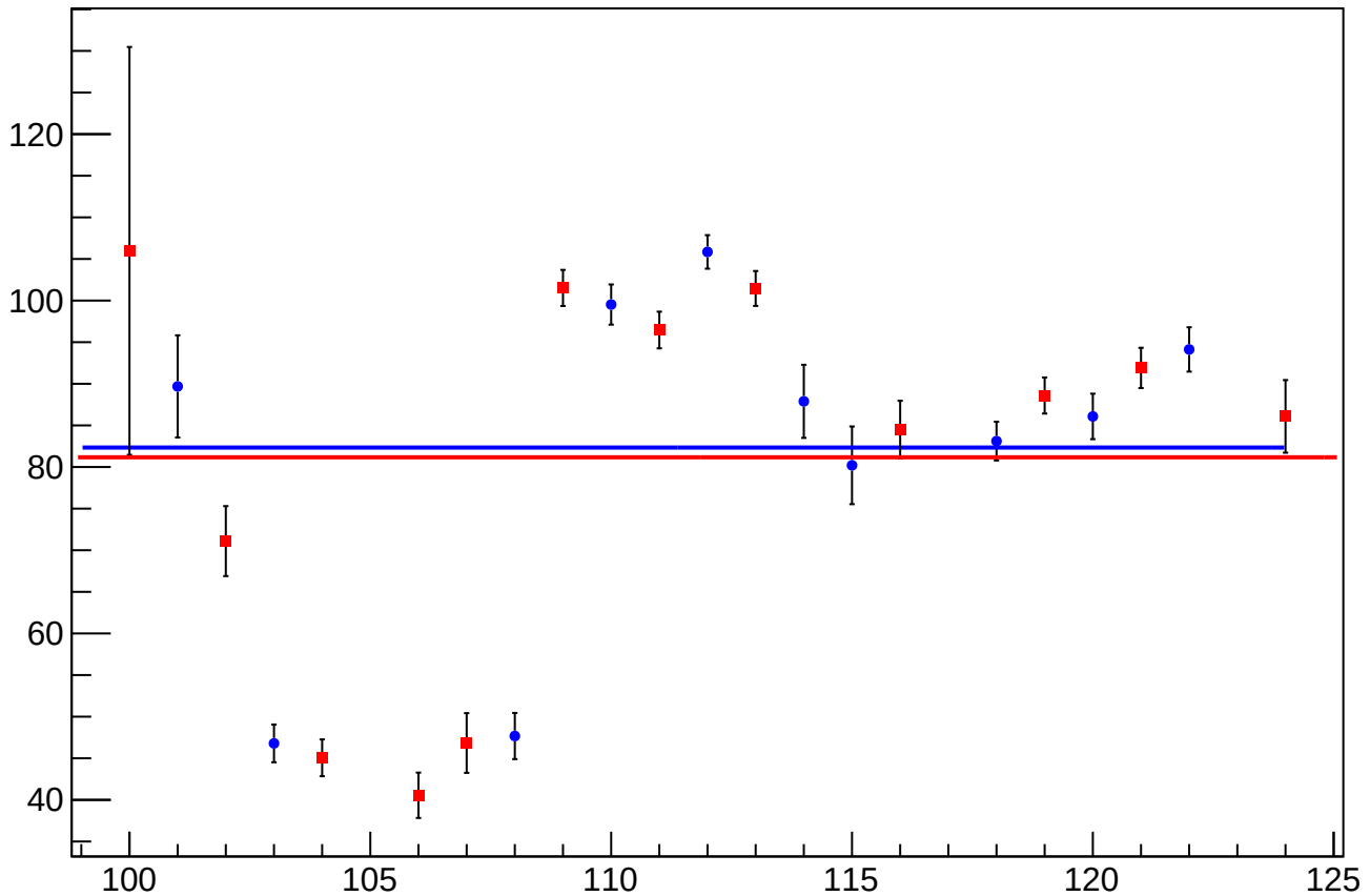
reg_asym_usr_atr1_avg_diff_bpm4eX_slope vs Slug
