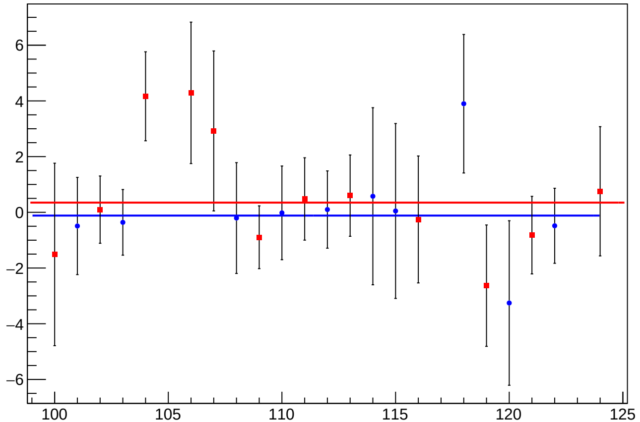
diff_bpmtargetdiffY_mean vs Slug
