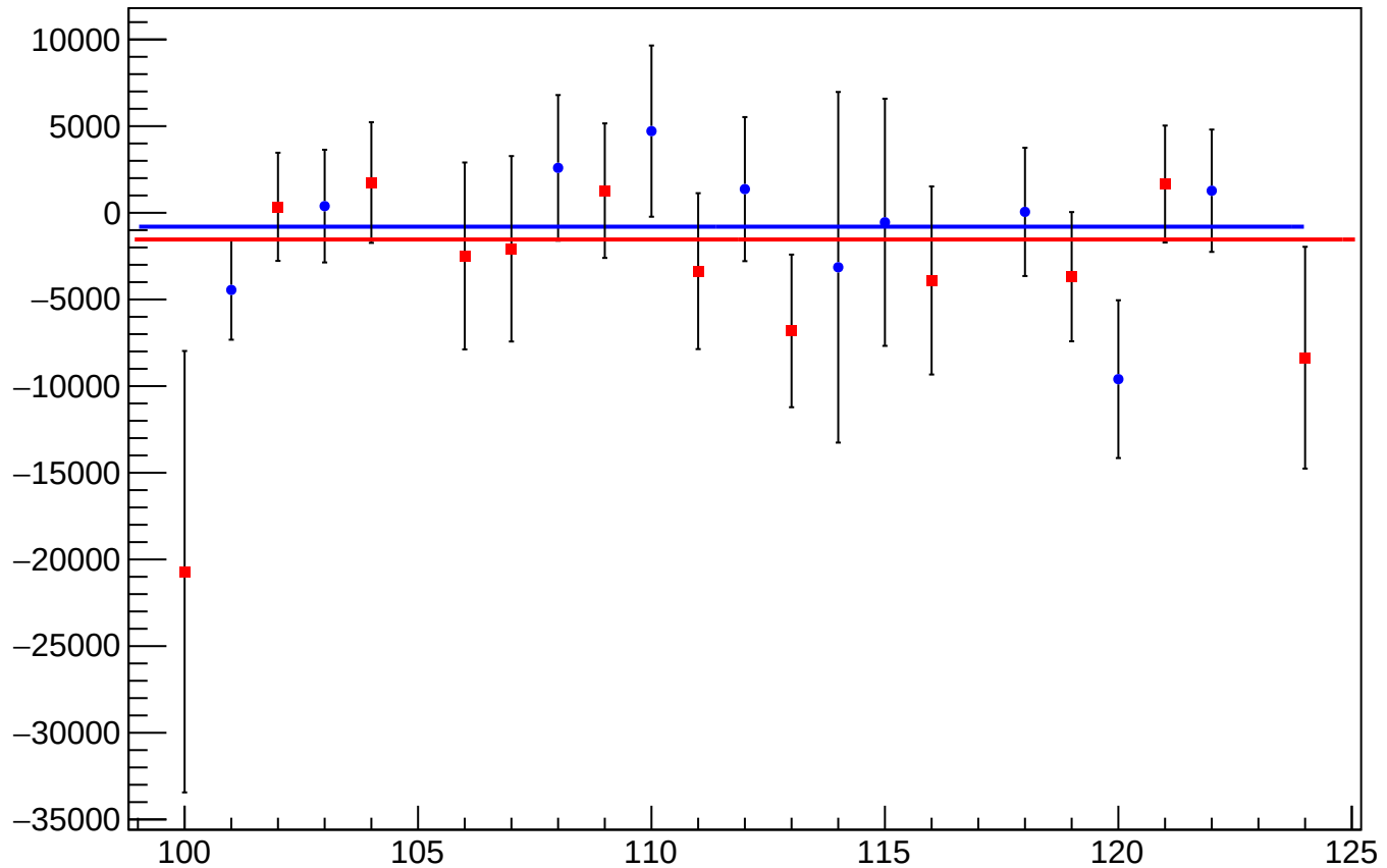
asym_sam_26_dd_cor_correction_mean vs Slug
