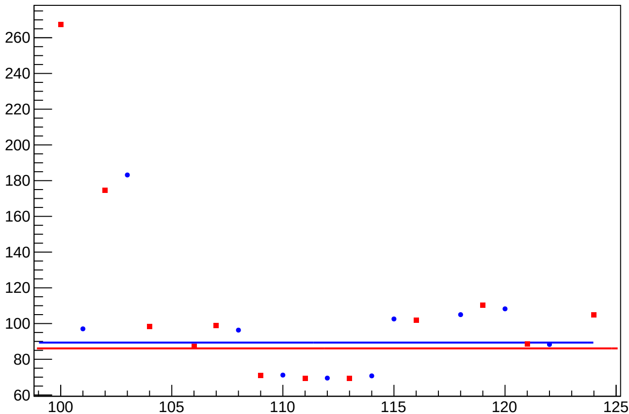
eigen_cor_asym_sam_3748_avg_rms vs Slug
