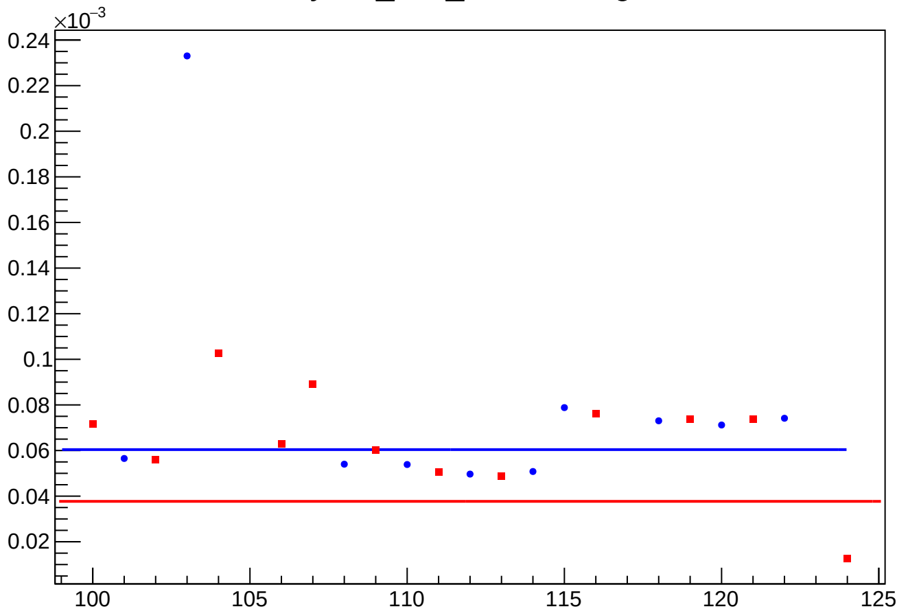
yield_atl1_rms vs Slug
