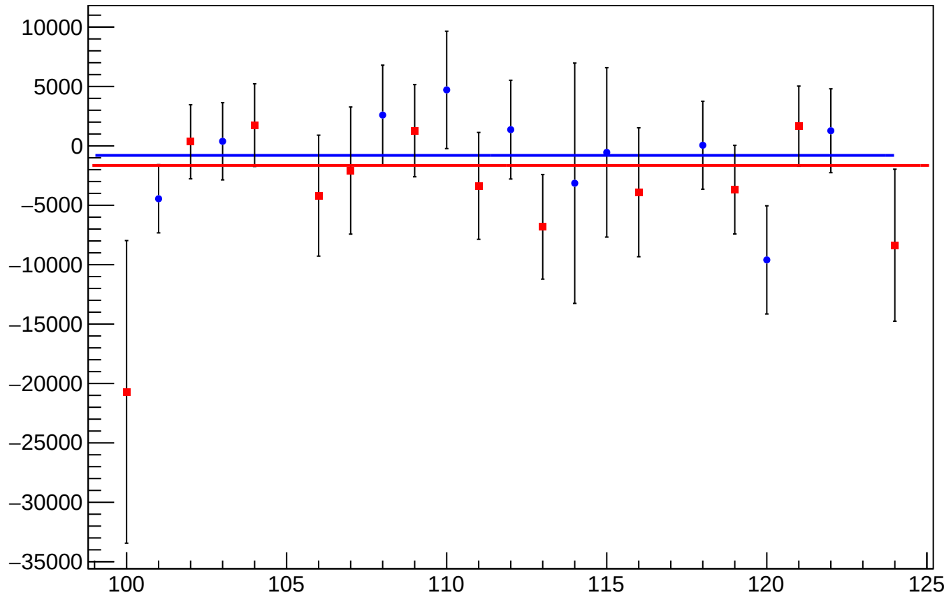
asym_sam_26_dd_reg_correction_mean vs Slug
