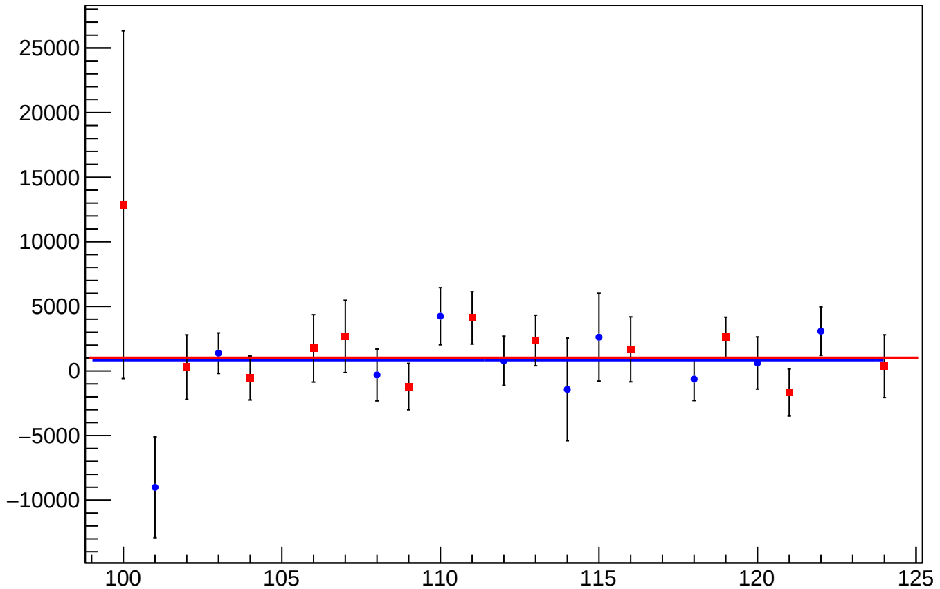
dit_asym_at1_dd_at2_dd_avg_mean vs Slug
