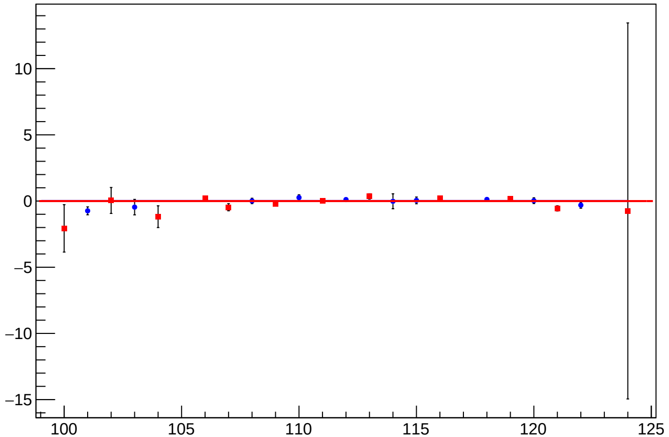
asym_atr1l2_avg_dit_vs_cor_diff_mean vs Slug
