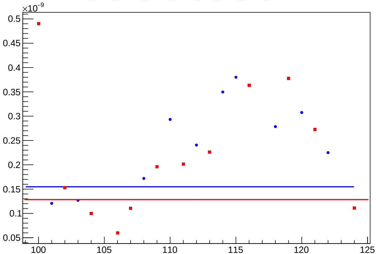
asym_usr_atr2_avg_reg_vs_cor_diff_rms vs Slug
