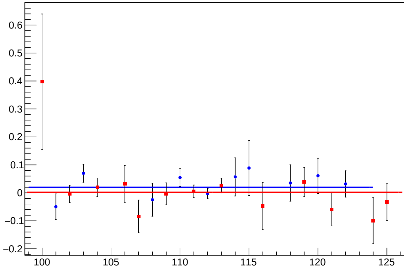
asym_sam_1548_avg_dit_vs_cor_diff_mean vs Slug, Sign Corrected
