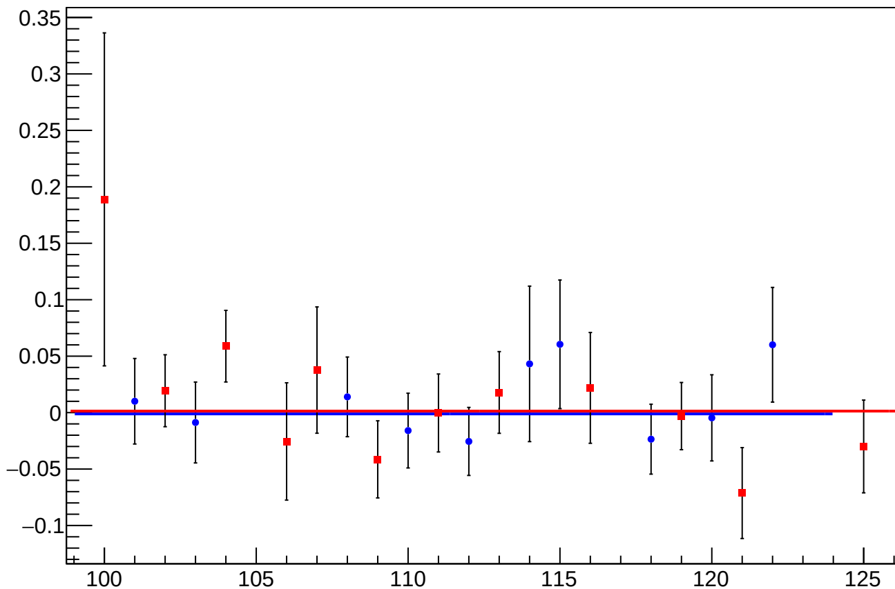
asym_us_dd_eigen_dit_vs_cor_diff_mean vs Slug, Sign Corrected
