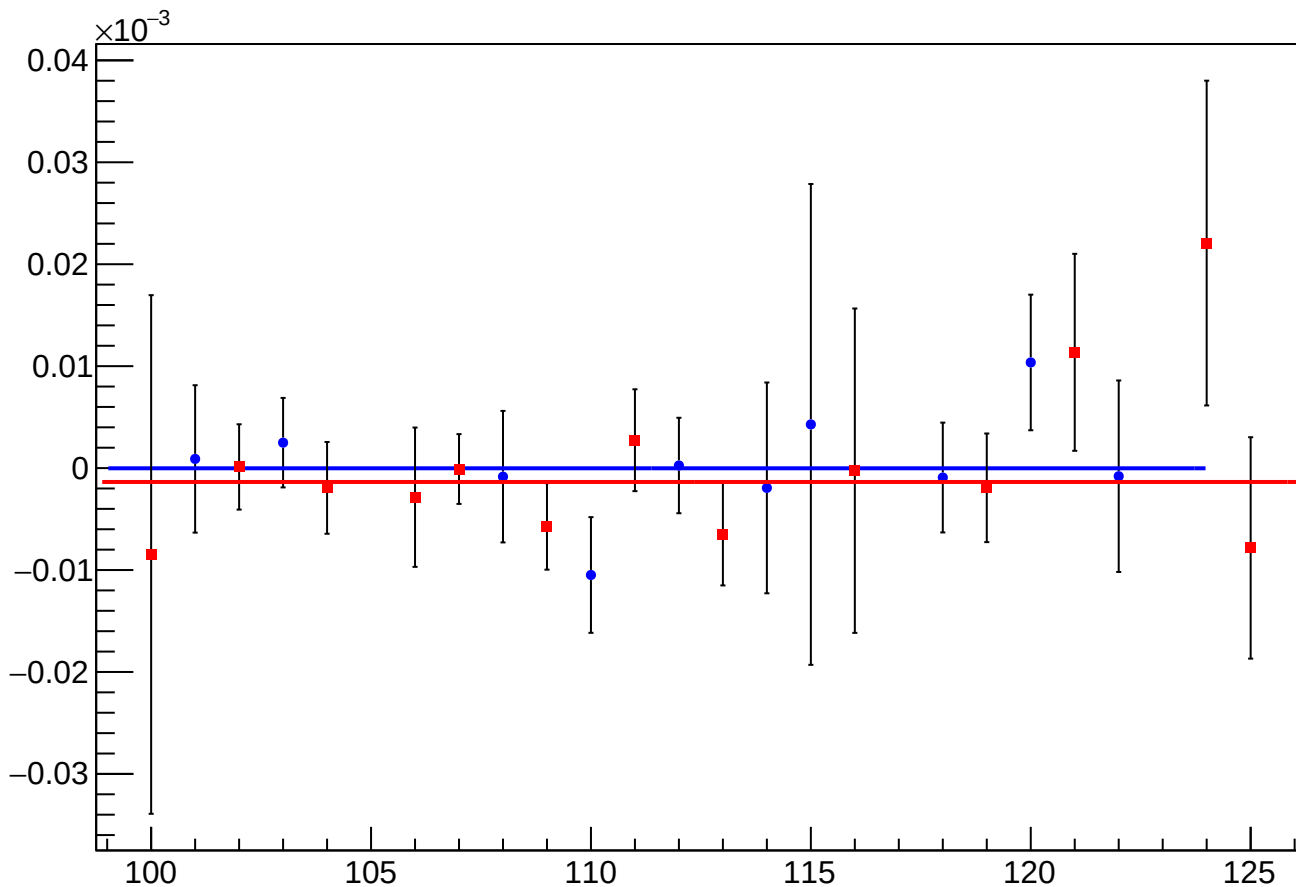
asym_sam4_eigen_dit_vs_dit_diff_mean vs Slug, Sign Corrected
