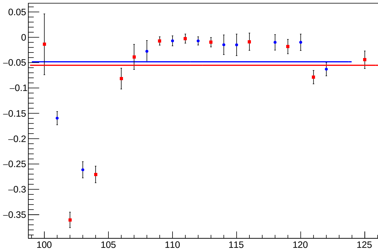
reg_asym_bcm_an_us_an_ds_dd_diff_bpm1X_slope vs Slug, Sign Corrected
