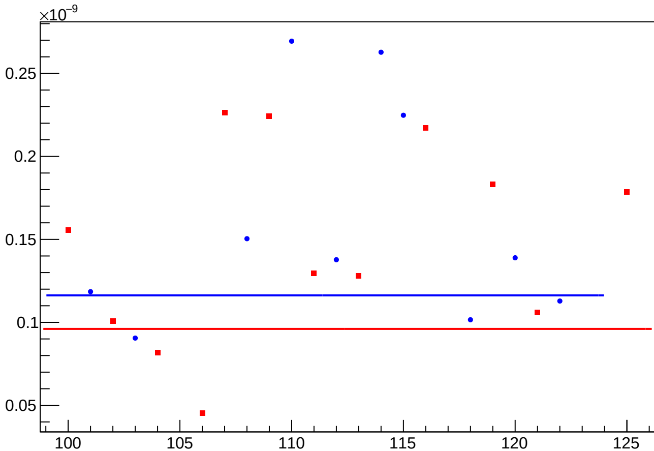
asym_usl_atl2_avg_reg_vs_cor_diff_rms vs Slug, Sign Corrected
