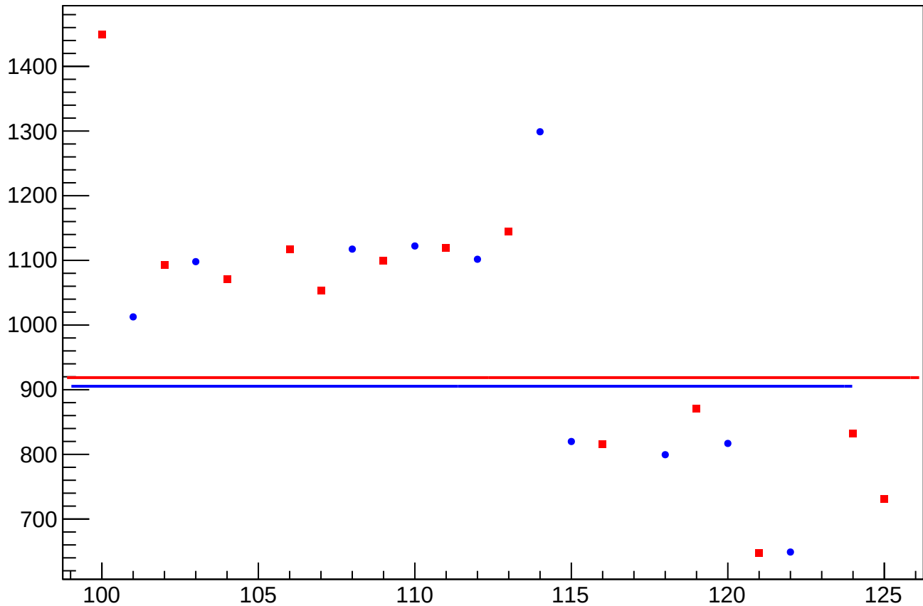
asym_sam_15_26_dd_reg_correction_rms vs Slug, Sign Corrected
