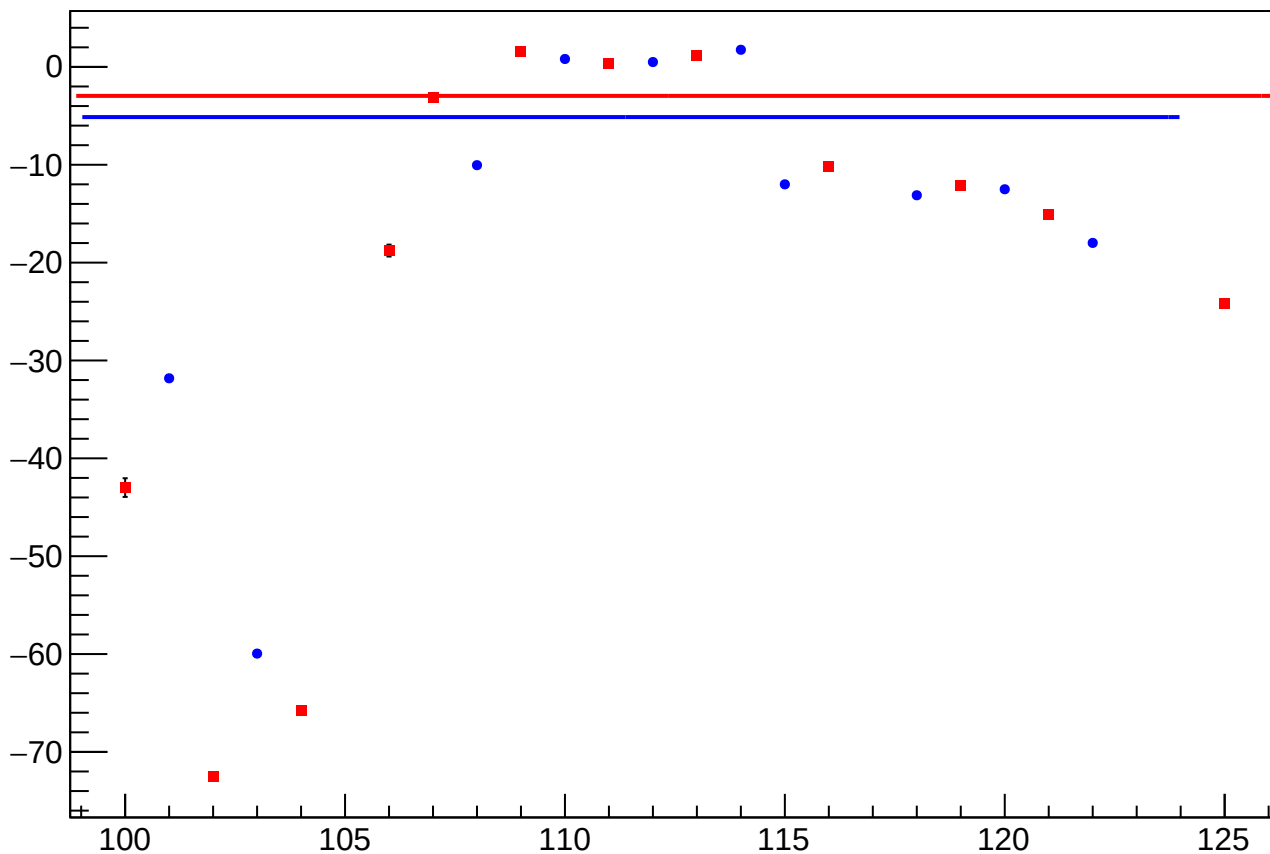
reg_asym_bcm_an_us_ds_avg_diff_bpm1X_slope vs Slug, Sign Corrected
