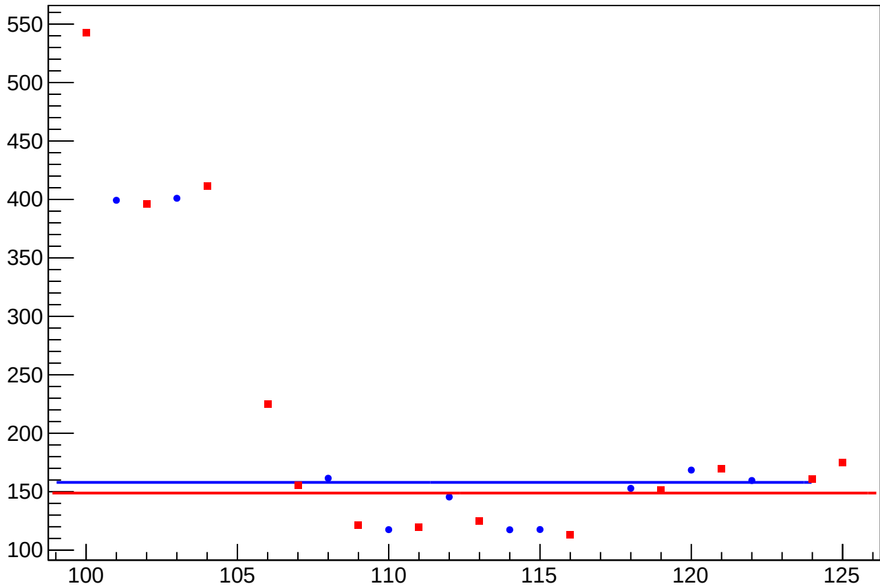
yield_bpm0l07WS_rms vs Slug, Sign Corrected
