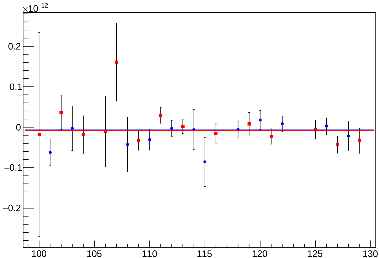
asym_us_dd_atlr_dd_dd_eigen_cor_vs_cor_diff_mean vs Slug, Sign Corrected
