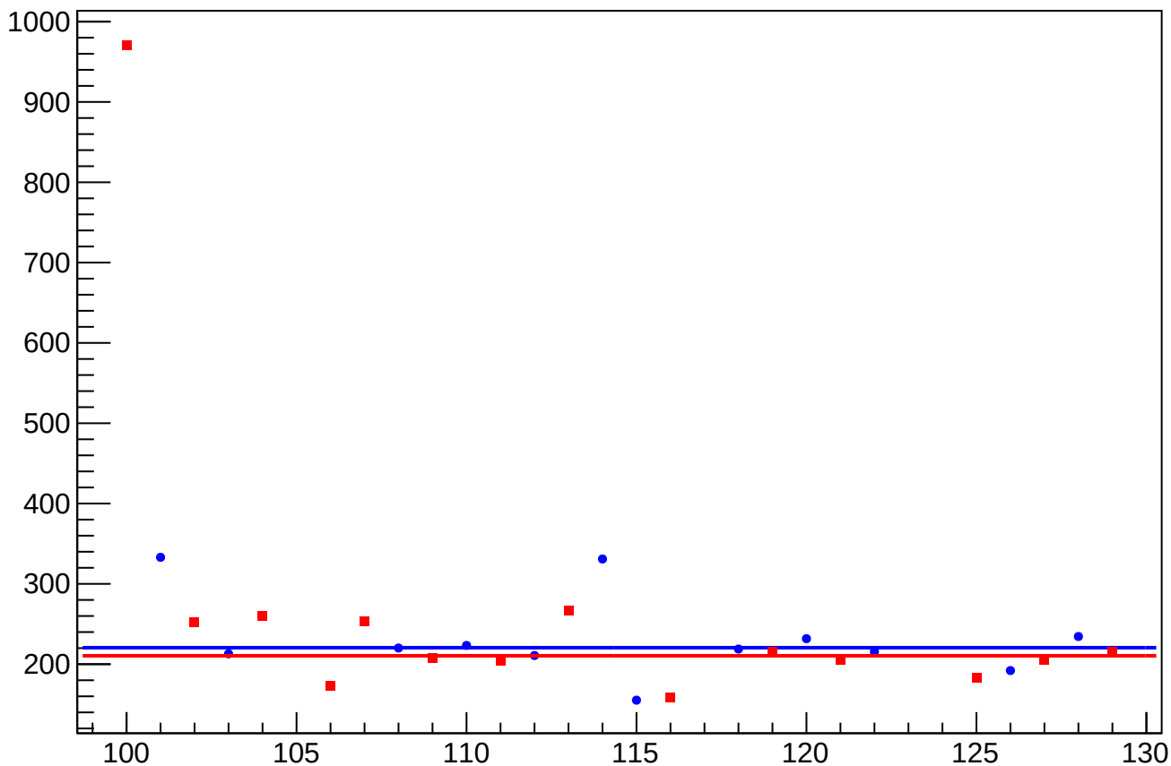
asym_atl2_eigen_dit_vs_eigen_cor_diff_rms vs Slug, Sign Corrected
