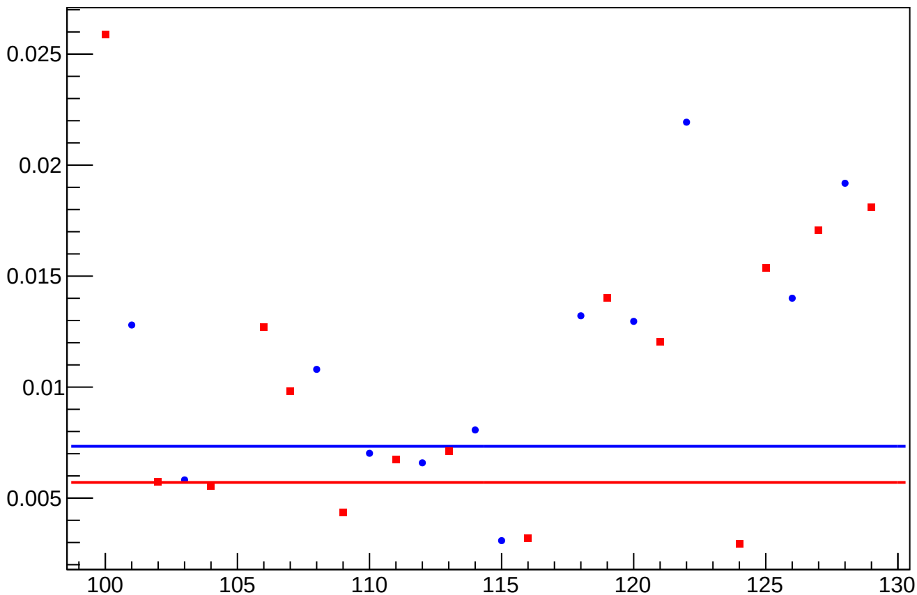
asym_usr_atr2_dd_eigen_dit_vs_dit_diff_rms vs Slug, Sign Corrected
