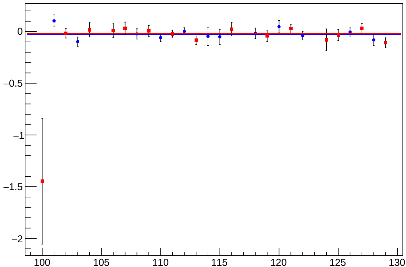
asym_sam_37_48_dd_eigen_dit_vs_eigen_cor_diff_mean vs Slug, Sign Corrected
