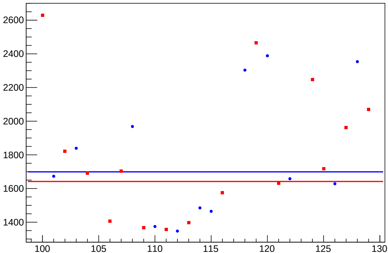
asym_sam3_cor_correction_rms vs Slug, Sign Corrected
