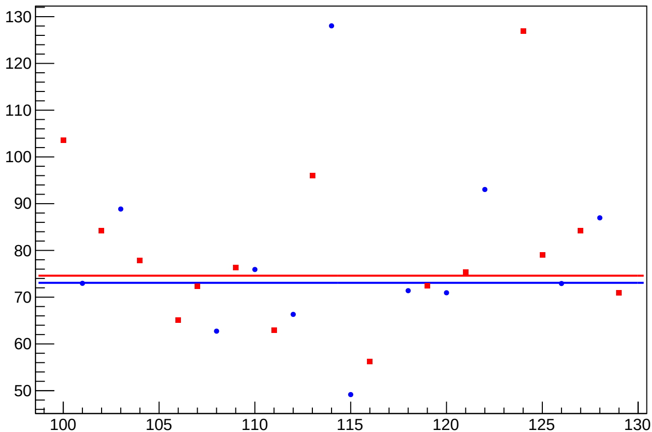
asym_usr_dit_vs_eigen_cor_diff_rms vs Slug, Sign Corrected
