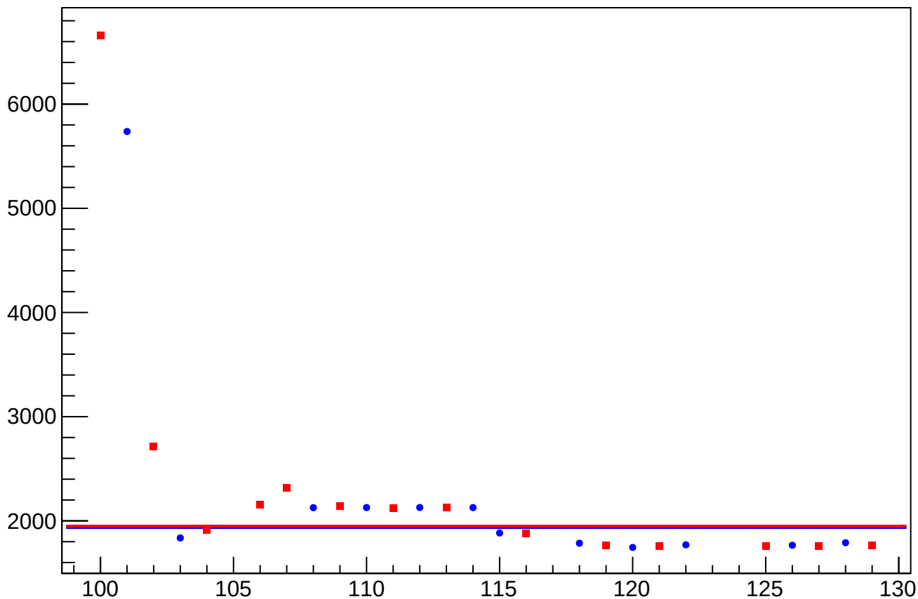
eigen_dit_asym_us_dd_at1lr_dd_dd_rms vs Slug, Sign Corrected
