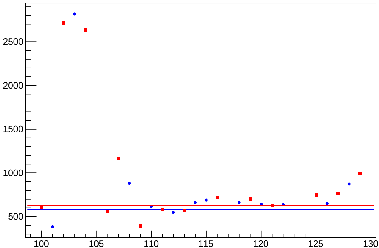
asym_us_avg_at1lr_avg_dd_dit_correction_rms vs Slug, Sign Corrected
