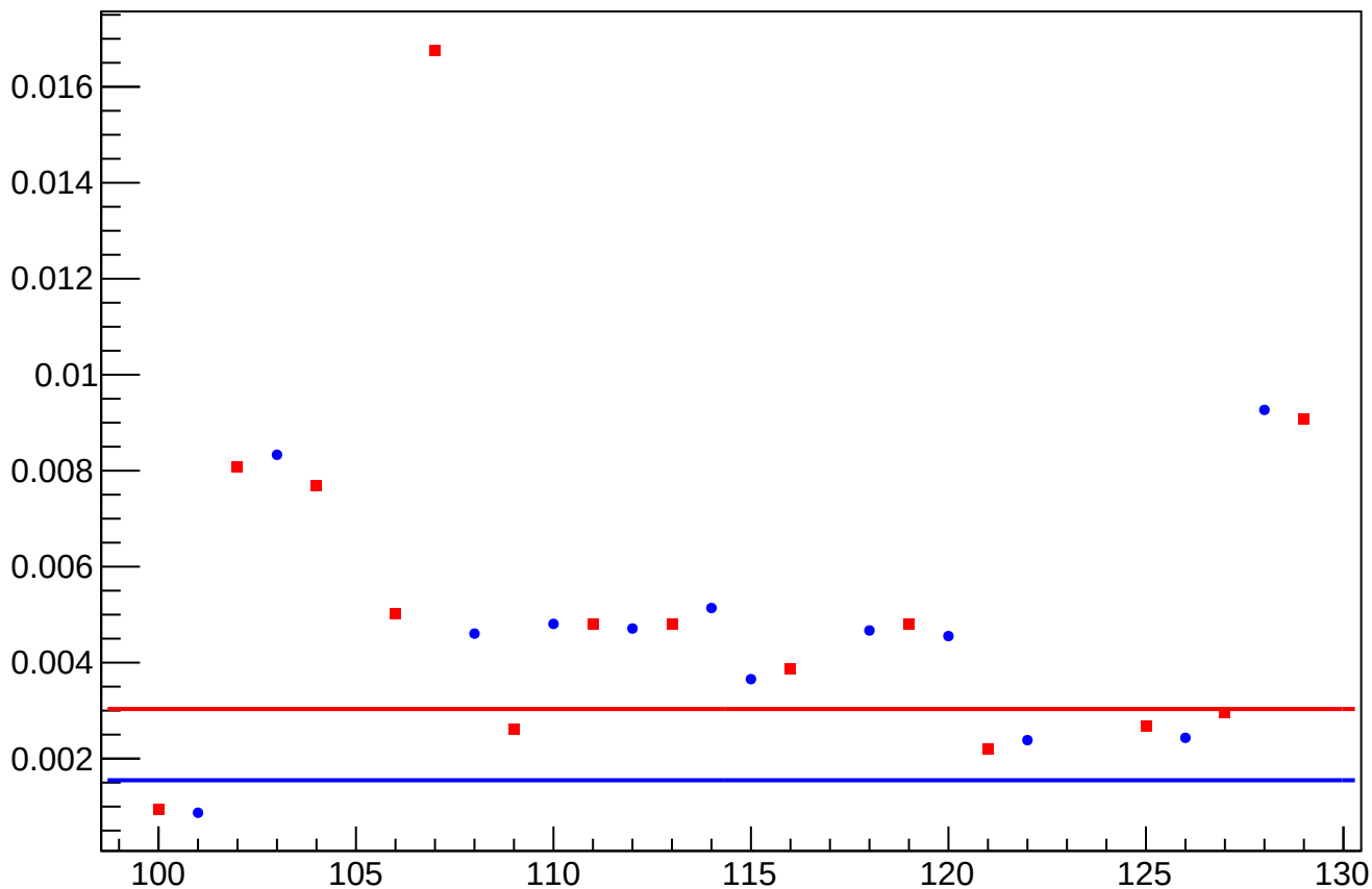
asym_us_avg_at1lr_avg_dd_eigen_dit_vs_dit_diff_rms vs Slug, Sign Corrected
