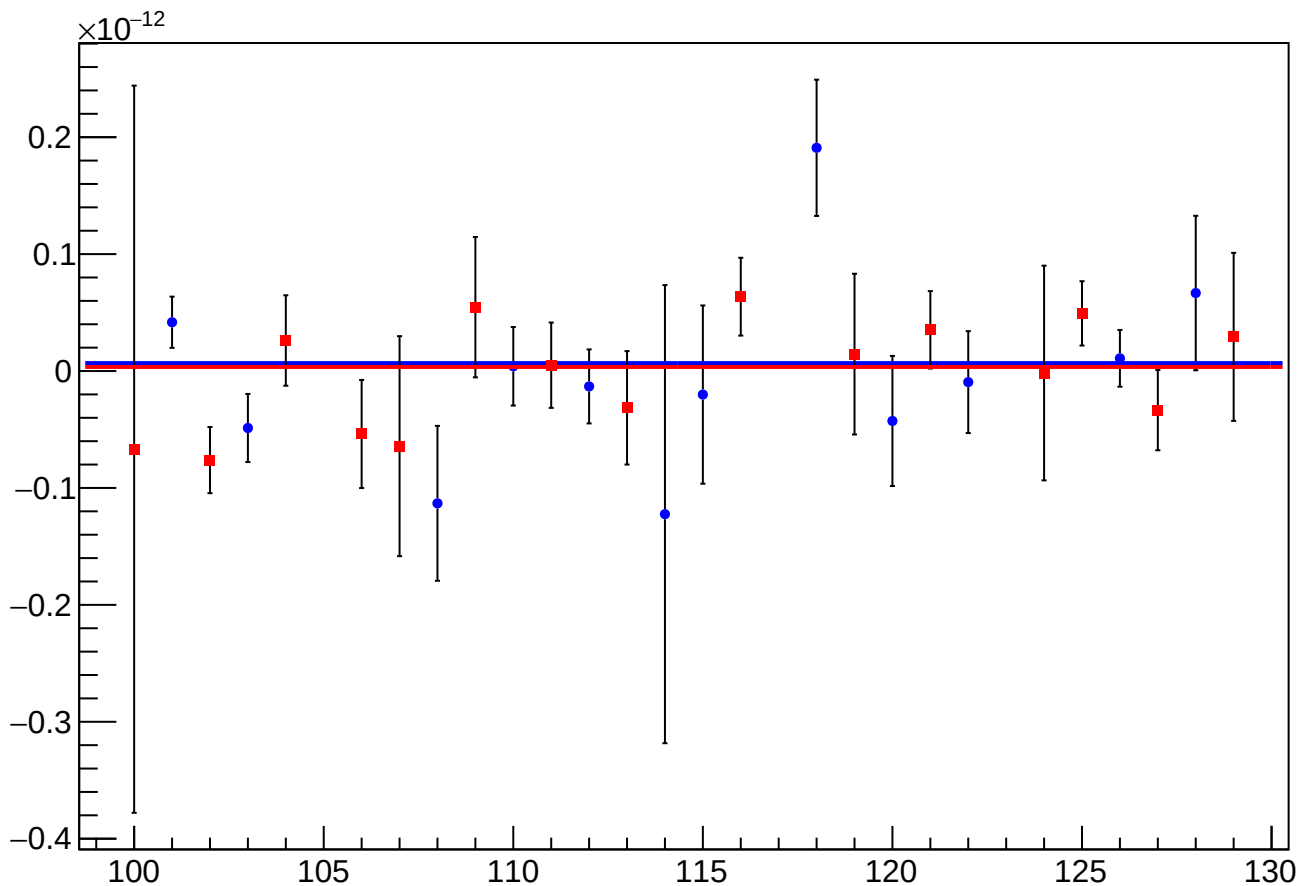
asym_sam_1357_2468_dd_reg_vs_cor_diff_mean vs Slug, Sign Corrected
