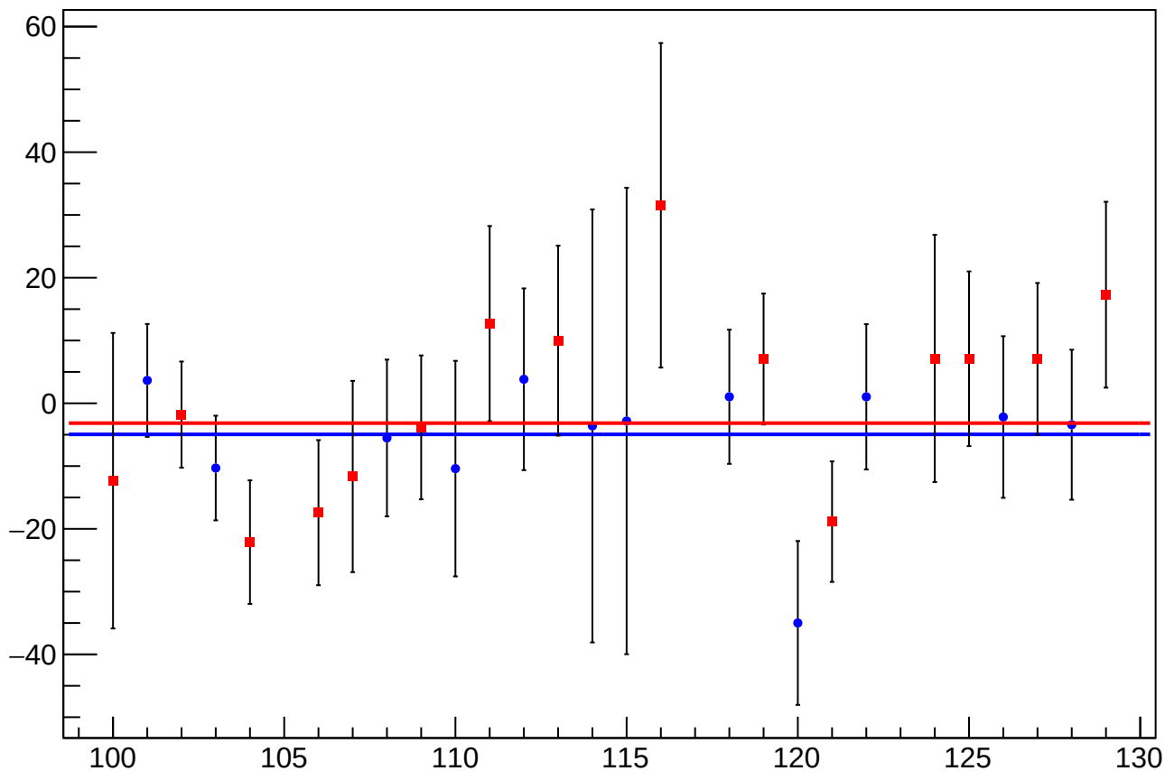
diff_bpm_4aY_4ecY_avg_mean vs Slug, Sign Corrected
