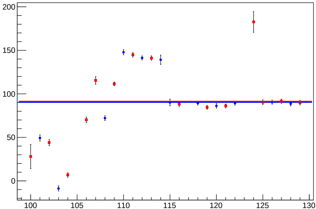
reg_asym_at1_dd_at2_dd_avg_diff_bpm4eX_slope vs Slug, Sign Corrected
