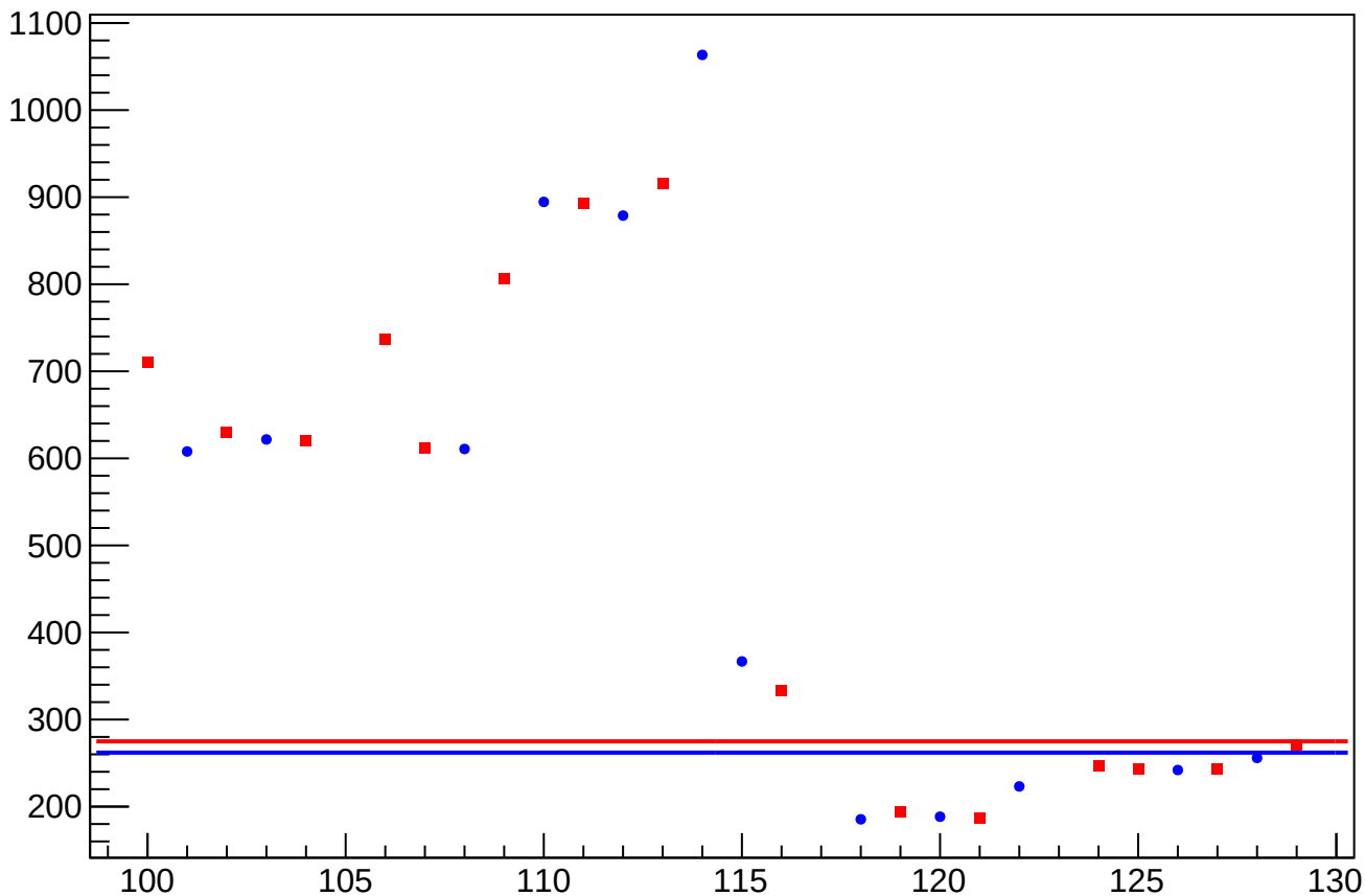
asym_sam_37_26_dd_reg_correction_rms vs Slug, Sign Corrected
