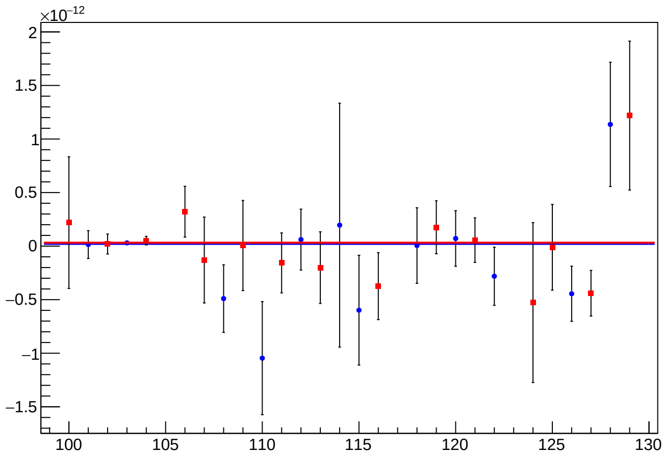
asym_atl1r2_avg_eigen_cor_vs_cor_diff_mean vs Slug, Sign Corrected
