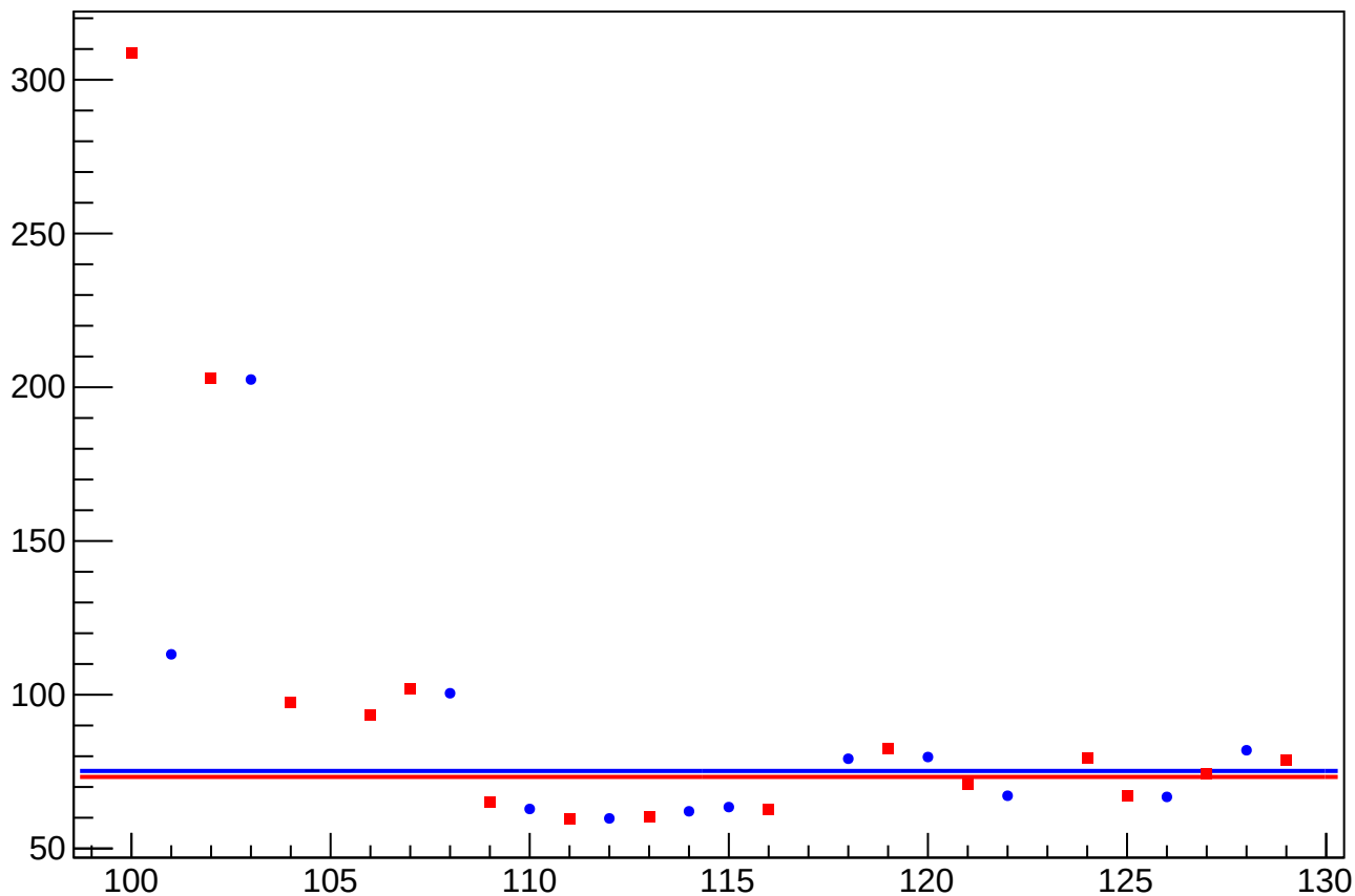
cor_asym_sam_37_avg_rms vs Slug, Sign Corrected
