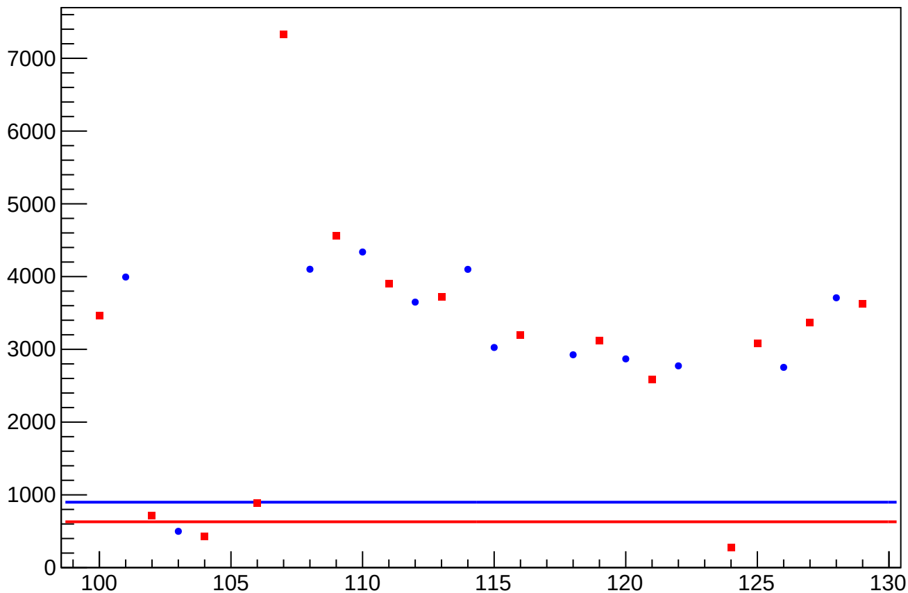
asym_atl_avg_reg_correction_rms vs Slug, Sign Corrected
