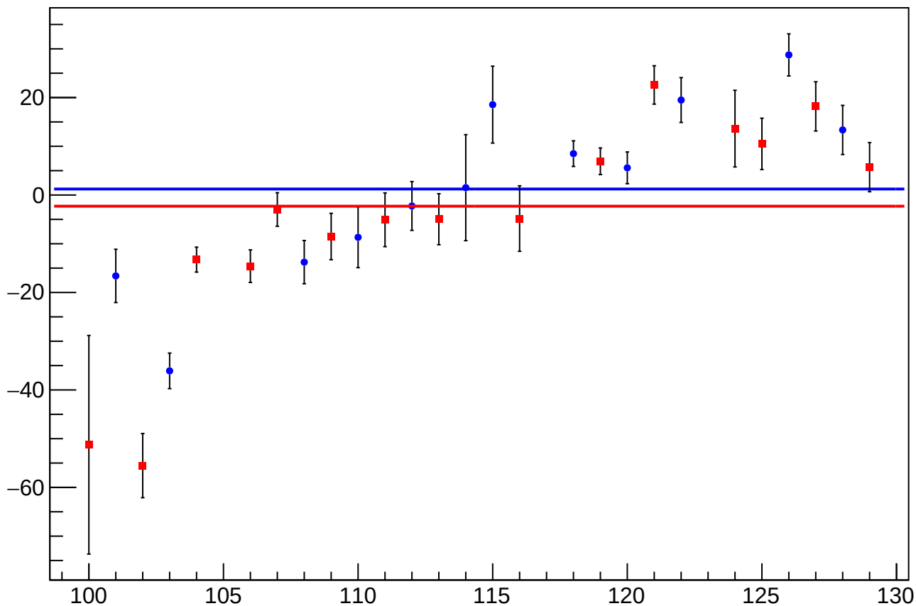
reg_asym_usr_atr2_dd_diff_bpm4aY_slope vs Slug, Sign Corrected
