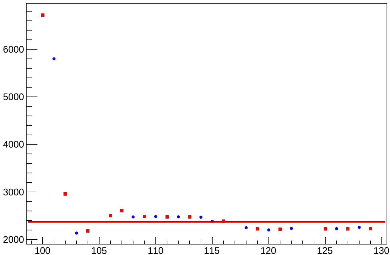
eigen_cor_asym_us_avg_at1lr_avg_avg_rms vs Slug, Sign Corrected
