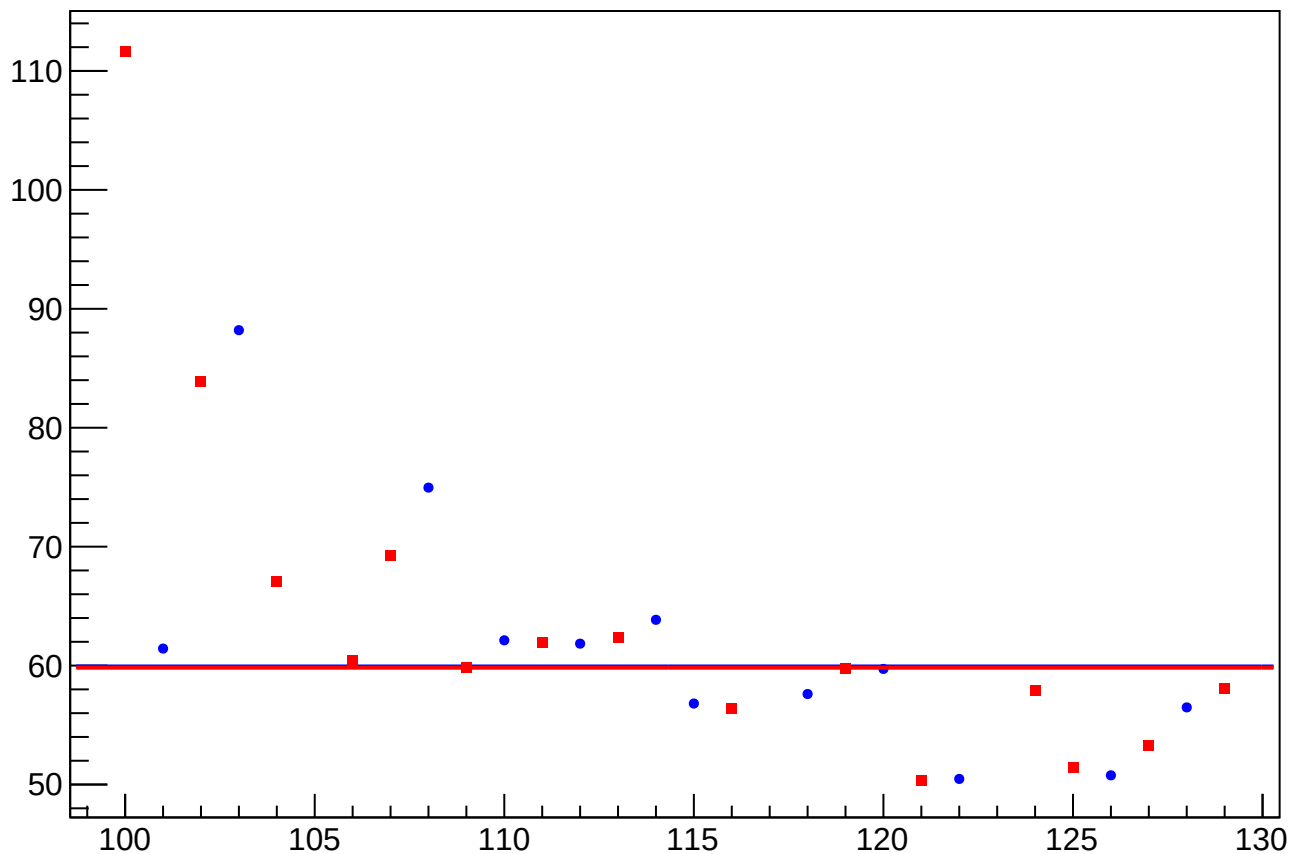
eigen_cor_asym_sam_15_48_dd_rms vs Slug, Sign Corrected
