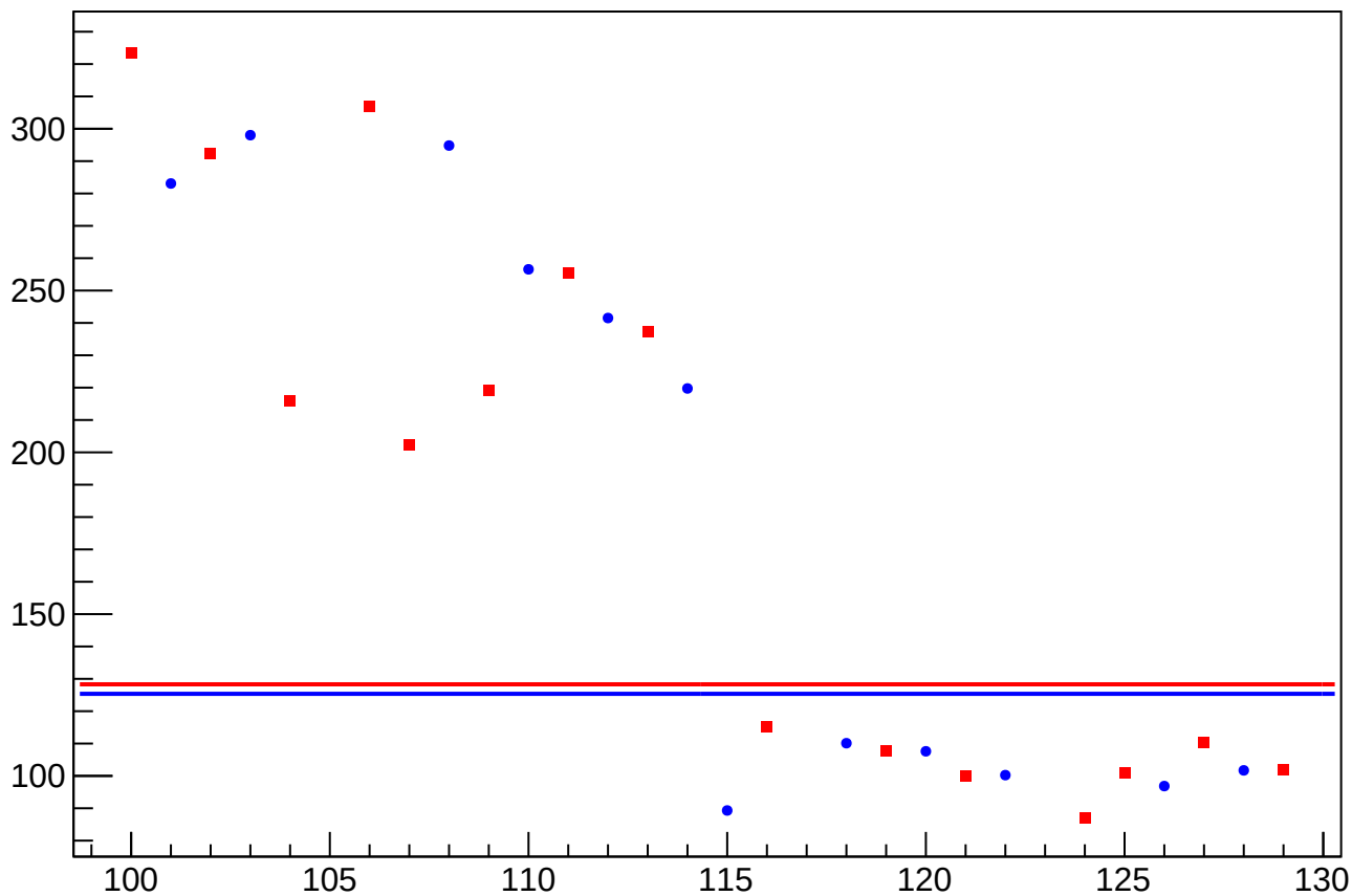
asym_sam2_dit_vs_eigen_cor_diff_rms vs Slug, Sign Corrected
