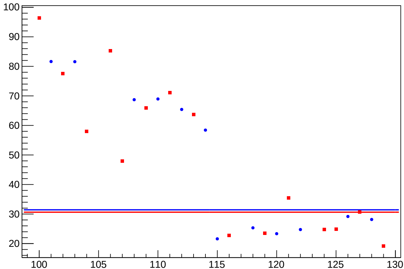
asym_sam_1526_avg_dit_vs_eigen_cor_diff_rms vs Slug, Sign Corrected
