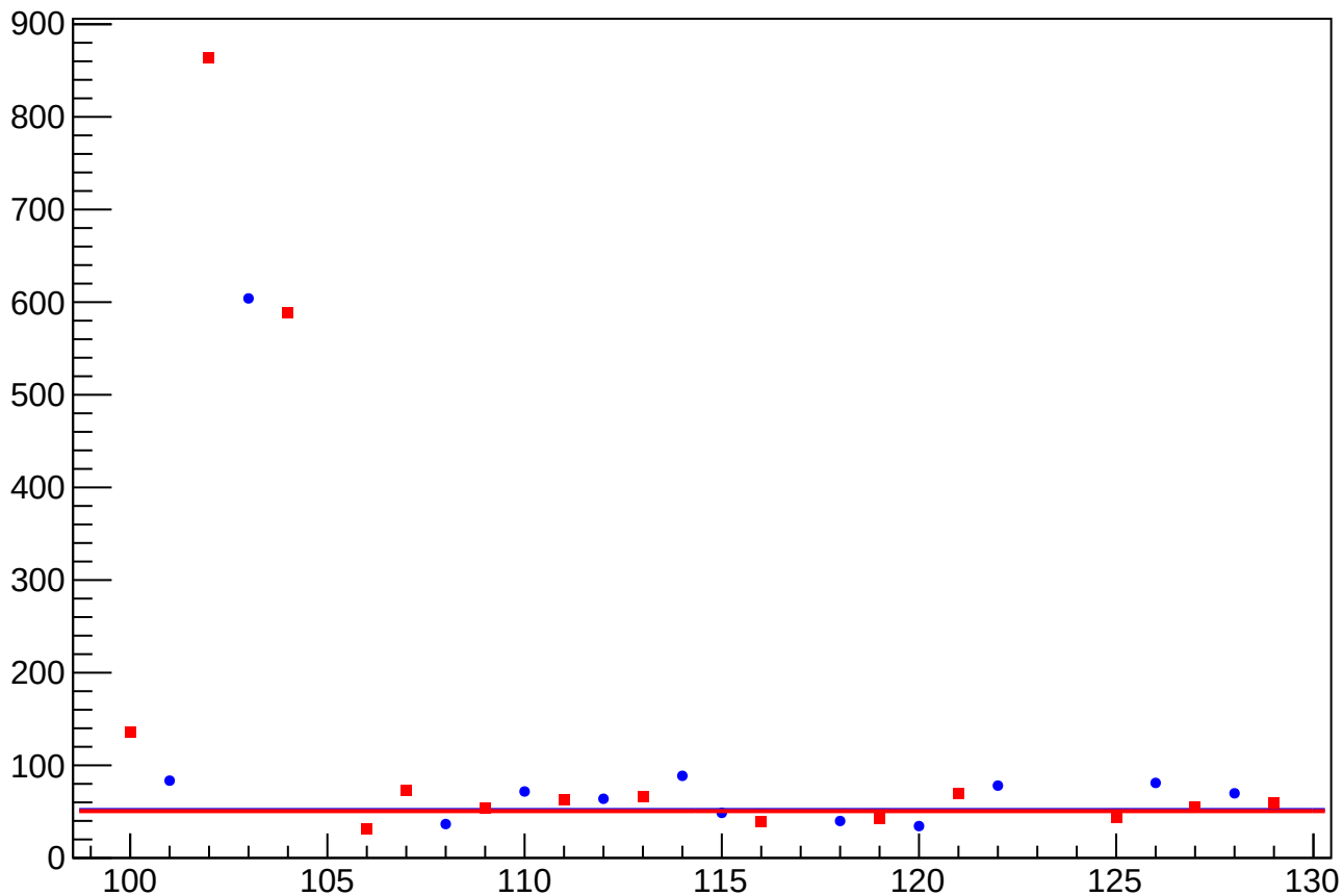
asym_us_dd_at2lr_dd_dd_dit_vs_cor_diff_rms vs Slug, Sign Corrected
