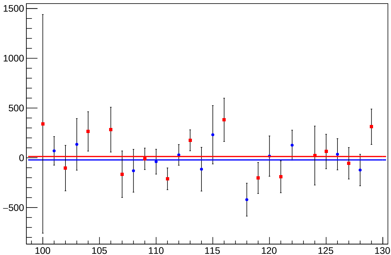
eigen_dit_asym_sam_3748_avg_mean vs Slug, Sign Corrected
