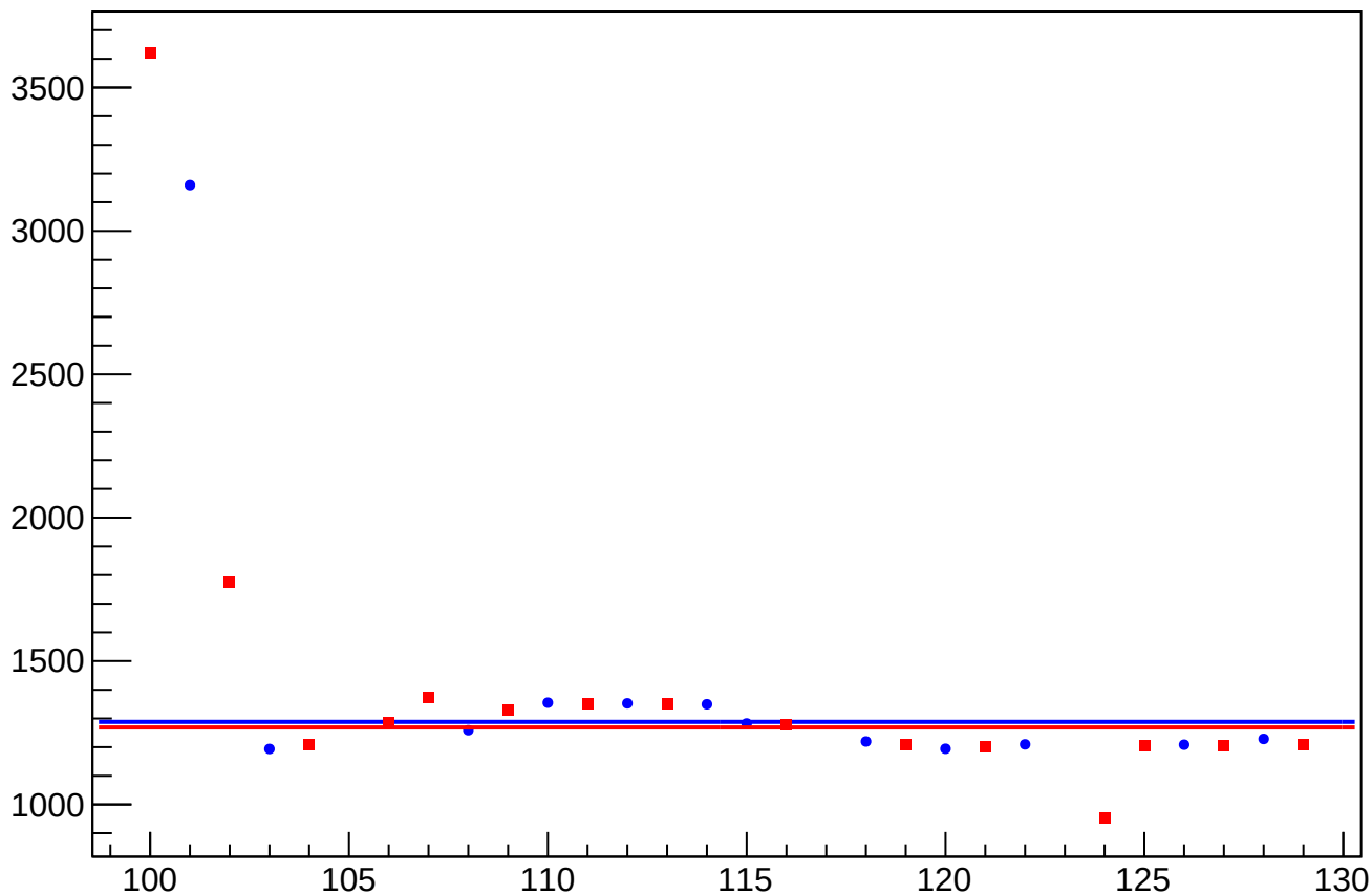
eigen_dit_asym_at1_dd_at2_dd_avg_rms vs Slug, Sign Corrected
