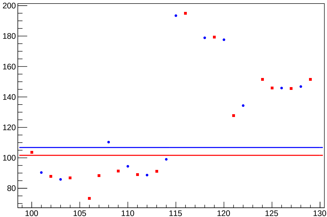
eigen_dit_asym_sam5_rms vs Slug, Sign Corrected
