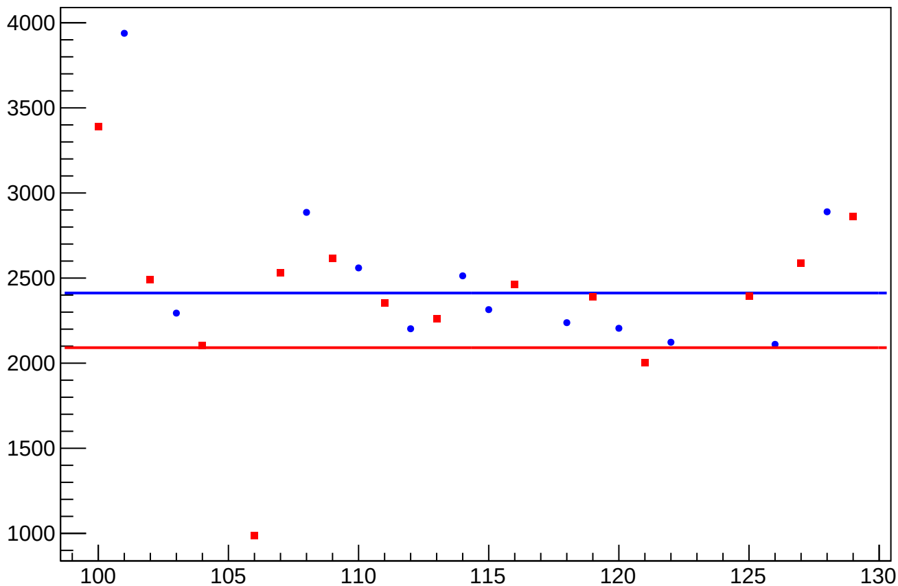
asym_usl_atl2_dd_reg_correction_rms vs Slug, Sign Corrected
