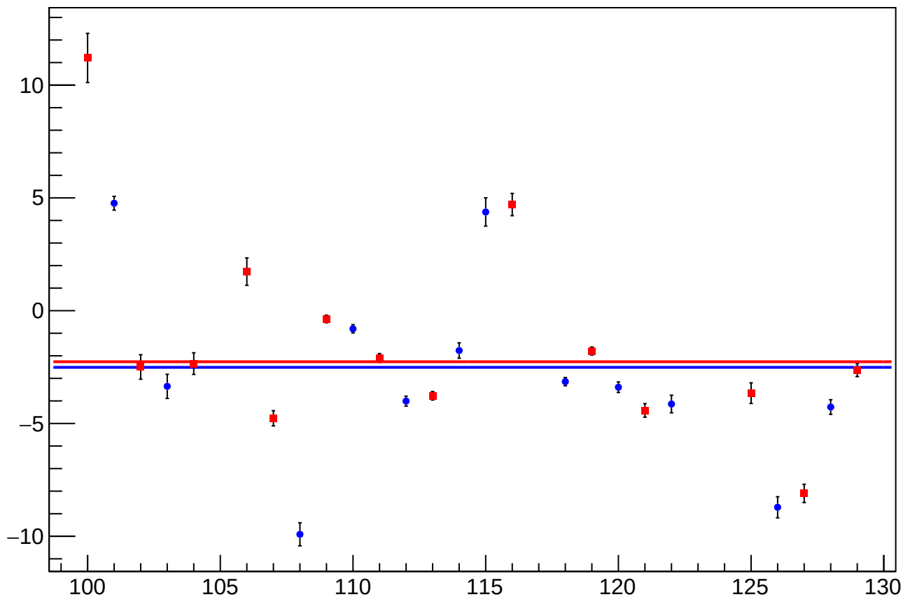
reg_asym_bcm_an_us_an_ds_avg_diff_bpm4eY_slope vs Slug, Sign Corrected
