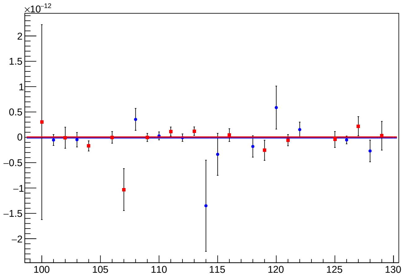
asym_us_dd_atlr_dd_avg_reg_vs_cor_diff_mean vs Slug, Sign Corrected
