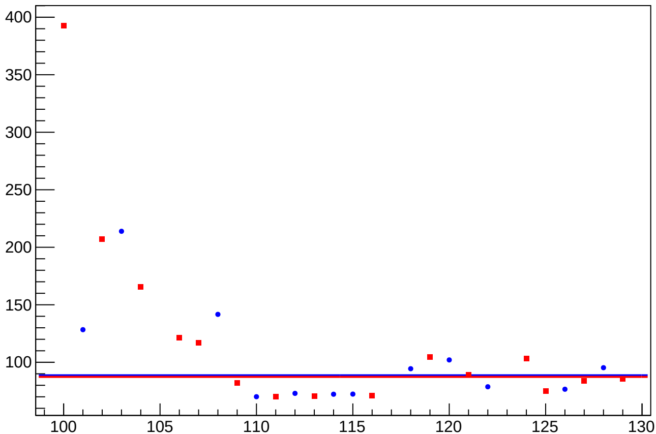
eigen_dit_asym_sam_37_avg_rms vs Slug, Sign Corrected
