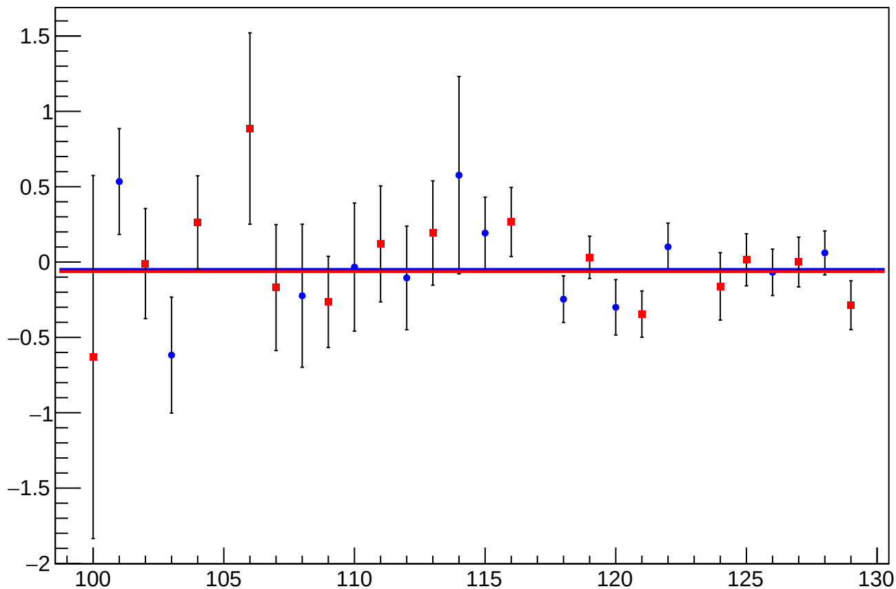
asym_sam2_dit_vs_eigen_cor_diff_mean vs Slug, Sign Corrected
