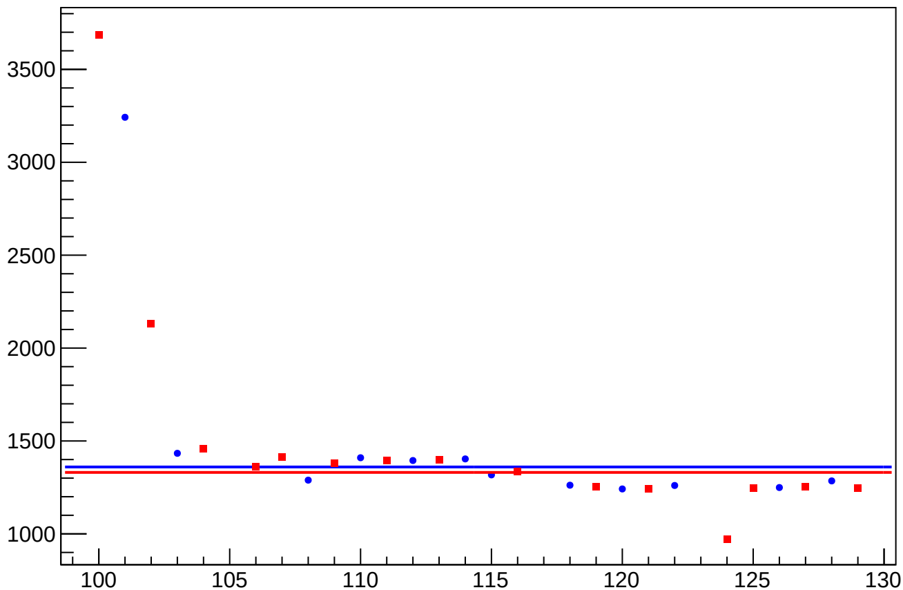
eigen_dit_asym_atl_avg_atr_avg_avg_rms vs Slug, Sign Corrected
