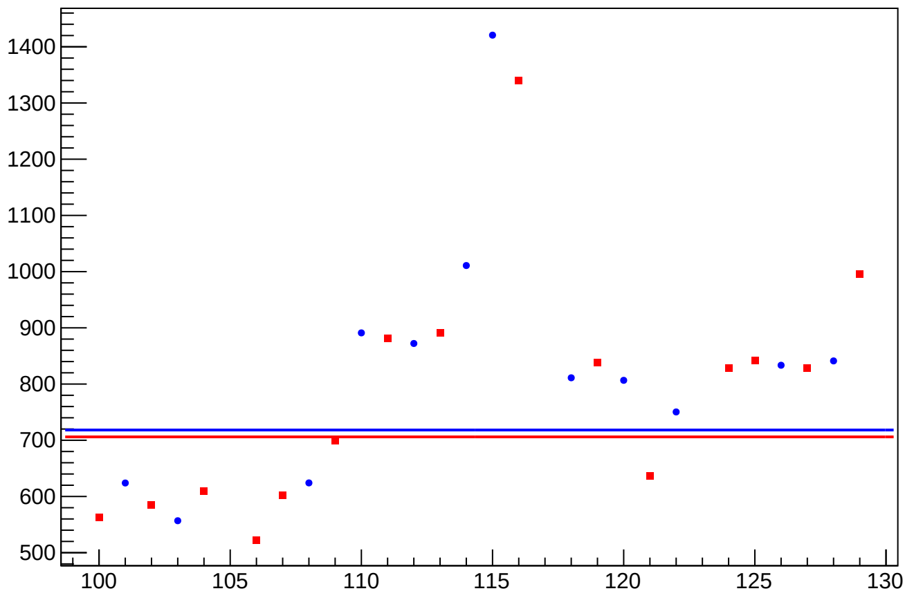
asym_sam_15_dd_cor_correction_rms vs Slug, Sign Corrected
