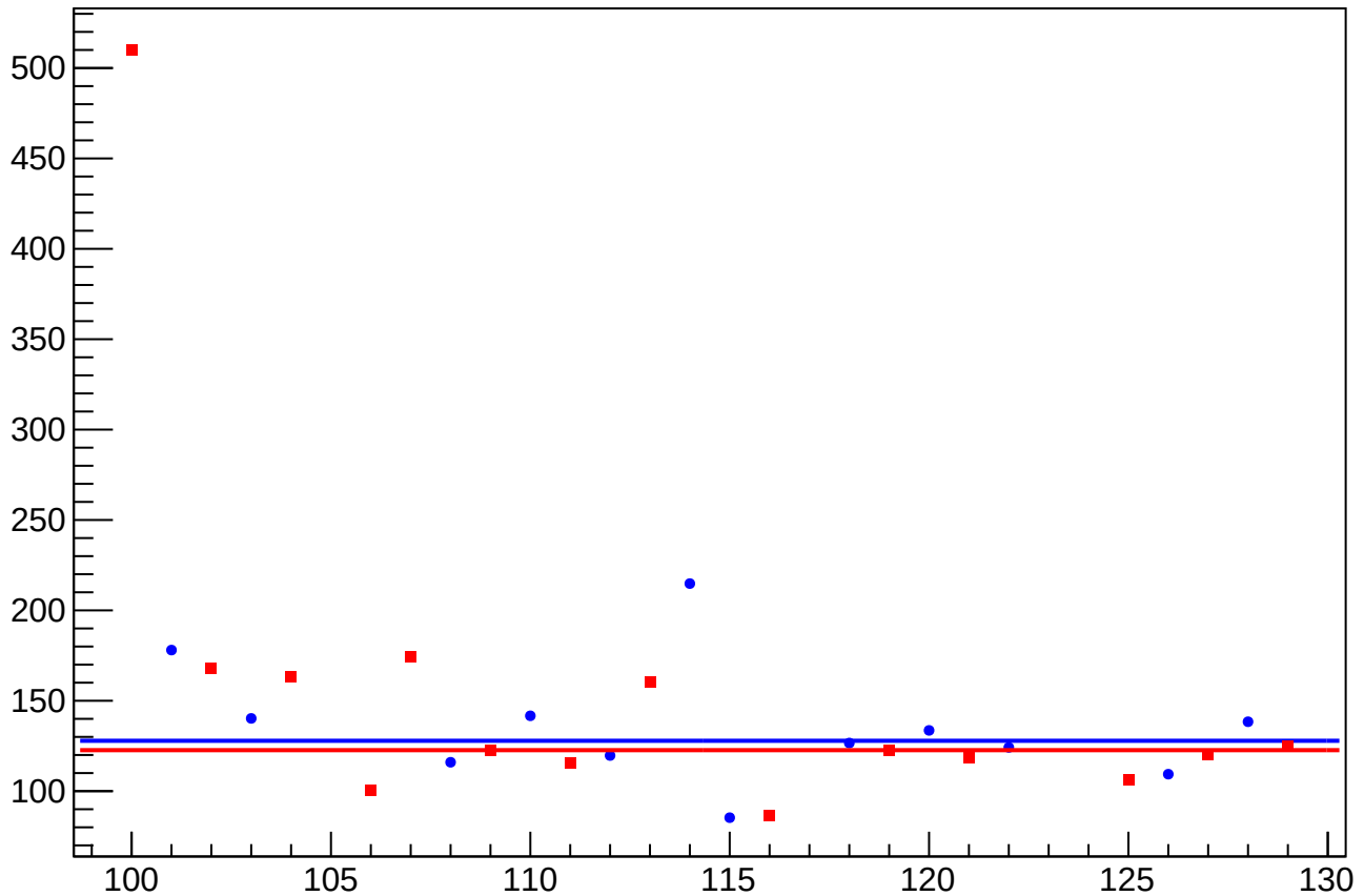
asym_usl_atl2_avg_eigen_dit_vs_cor_diff_rms vs Slug, Sign Corrected
