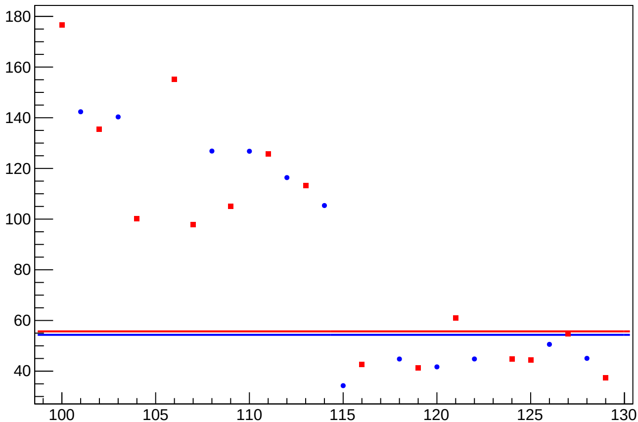
asym_sam_26_avg_eigen_dit_vs_eigen_cor_diff_rms vs Slug, Sign Corrected
