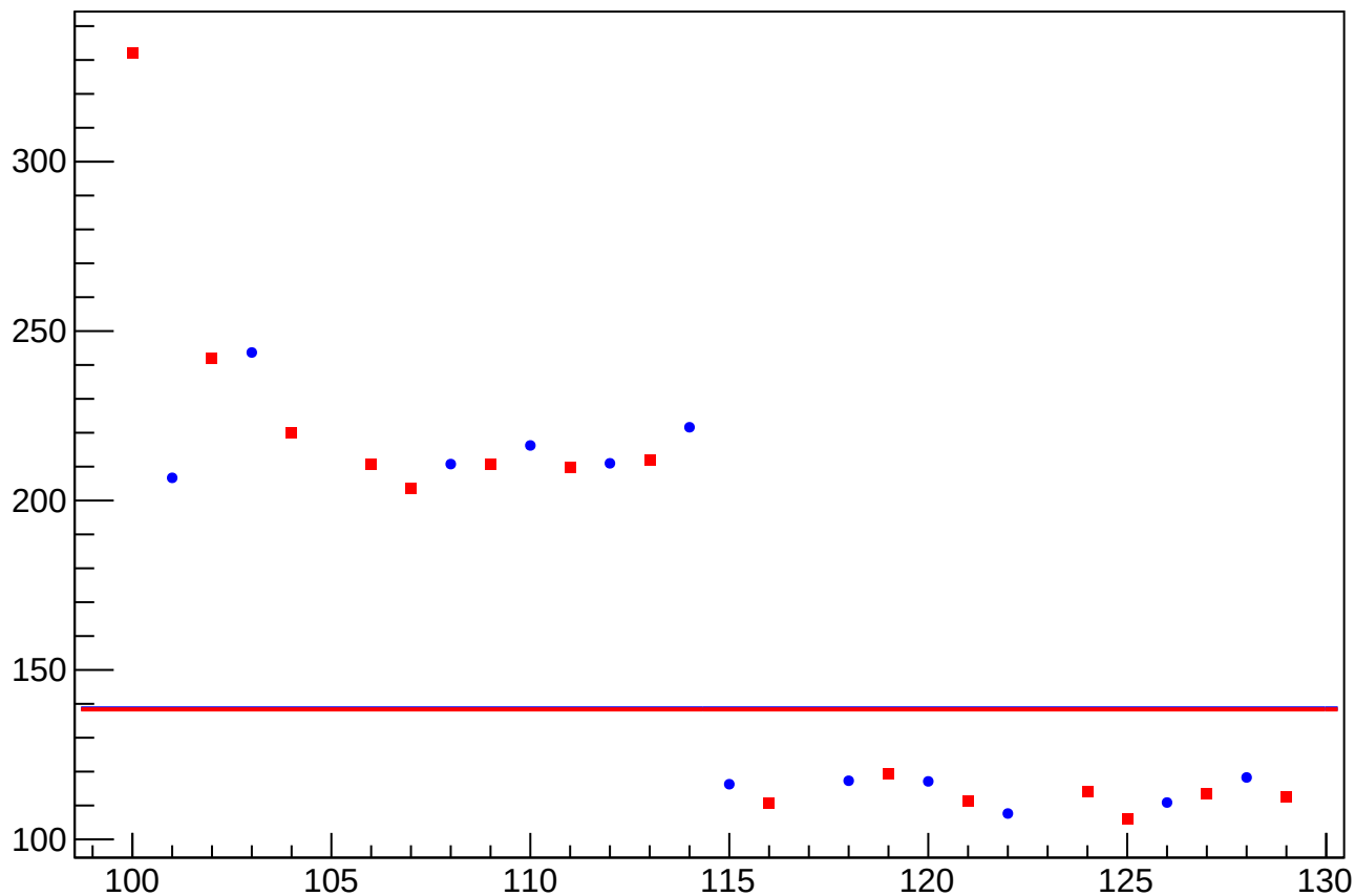
cor_asym_sam_26_avg_rms vs Slug, Sign Corrected
