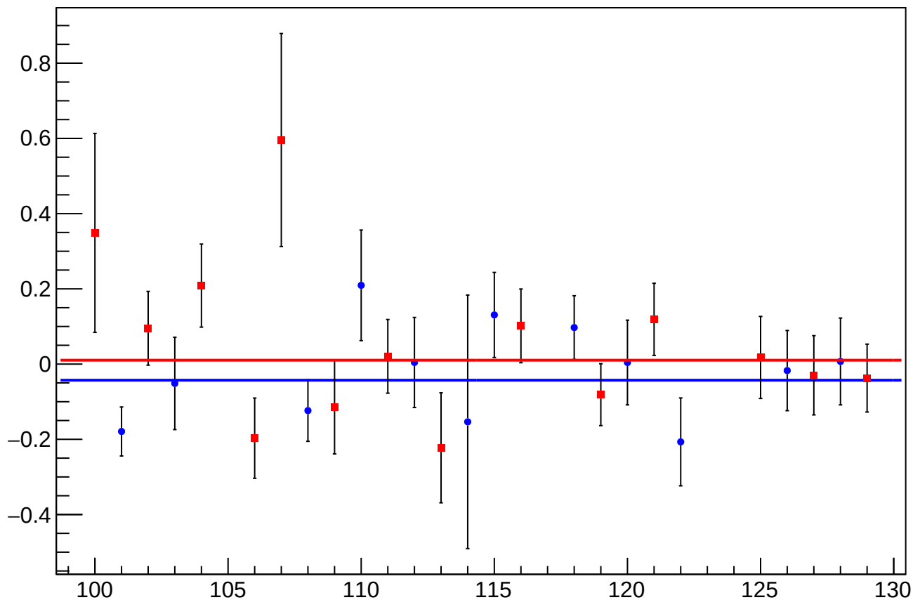
asym_usl_eigen_dit_vs_overload_cor_diff_mean vs Slug, Sign Corrected
