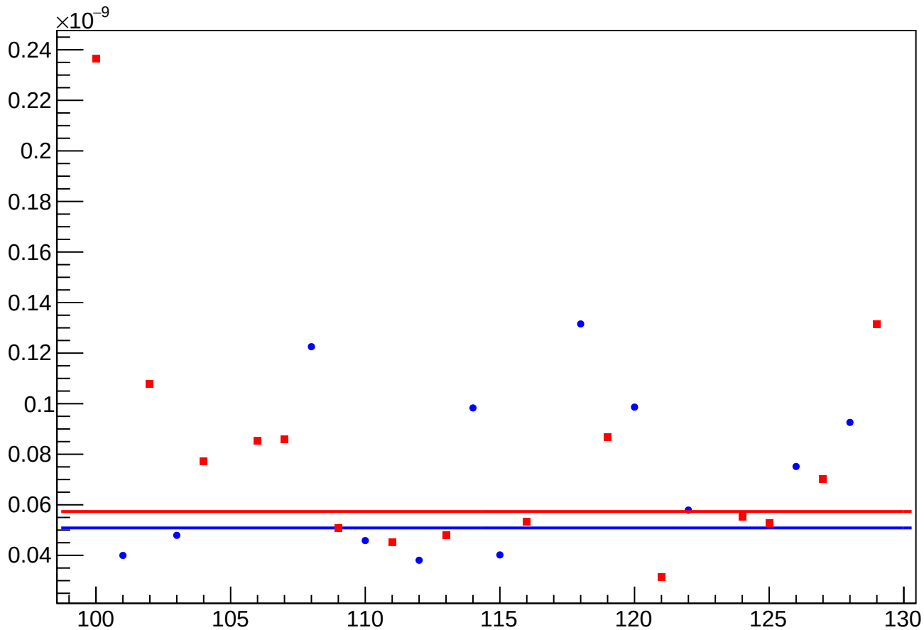
asym_sam3_reg_vs_cor_diff_rms vs Slug, Sign Corrected
