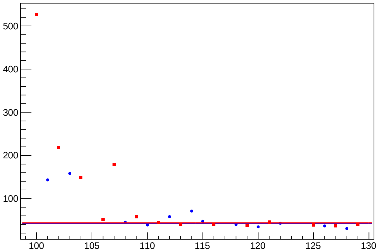
asym_us_dd_at1lr_dd_avg_dit_vs_cor_diff_rms vs Slug, Sign Corrected
