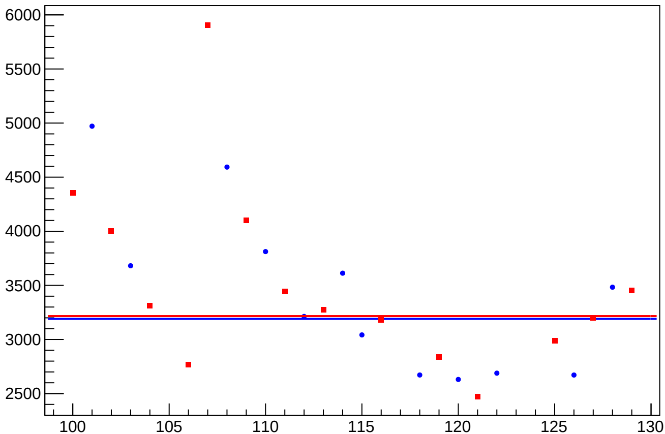
asym_usl_atl2_avg_cor_correction_rms vs Slug, Sign Corrected
