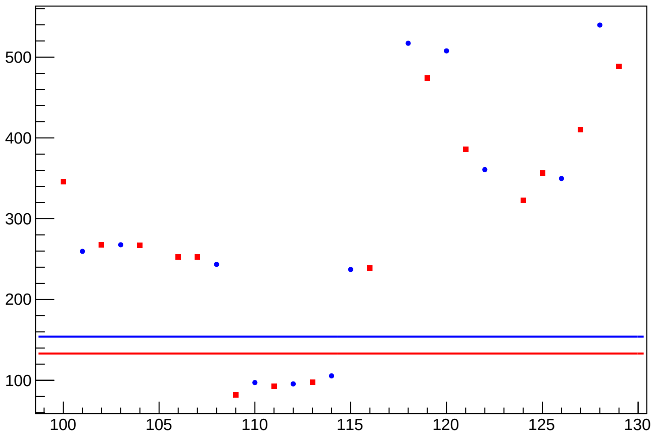
asym_sam8_eigen_dit_correction_rms vs Slug, Sign Corrected
