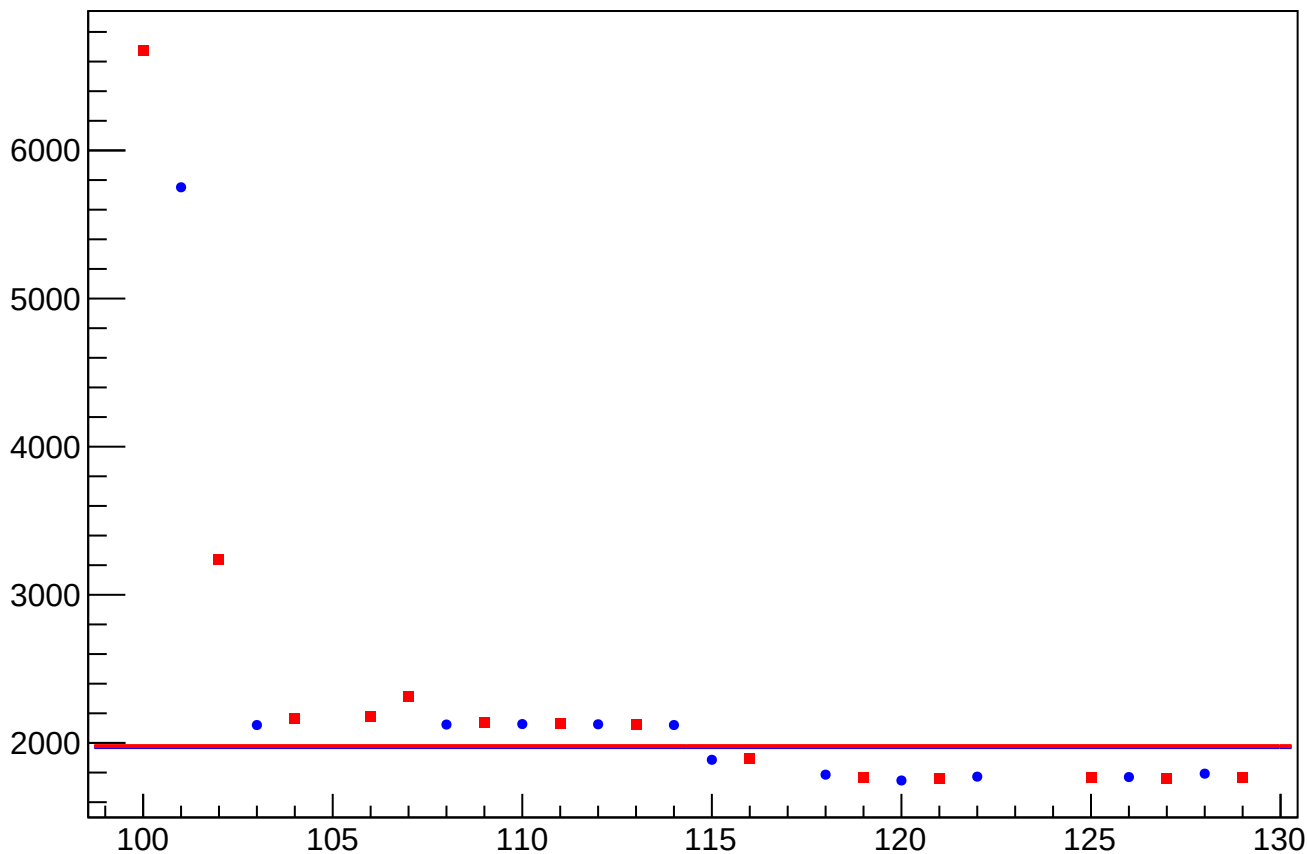
eigen_dit_asym_us_avg_at1lr_avg_dd_rms vs Slug, Sign Corrected
