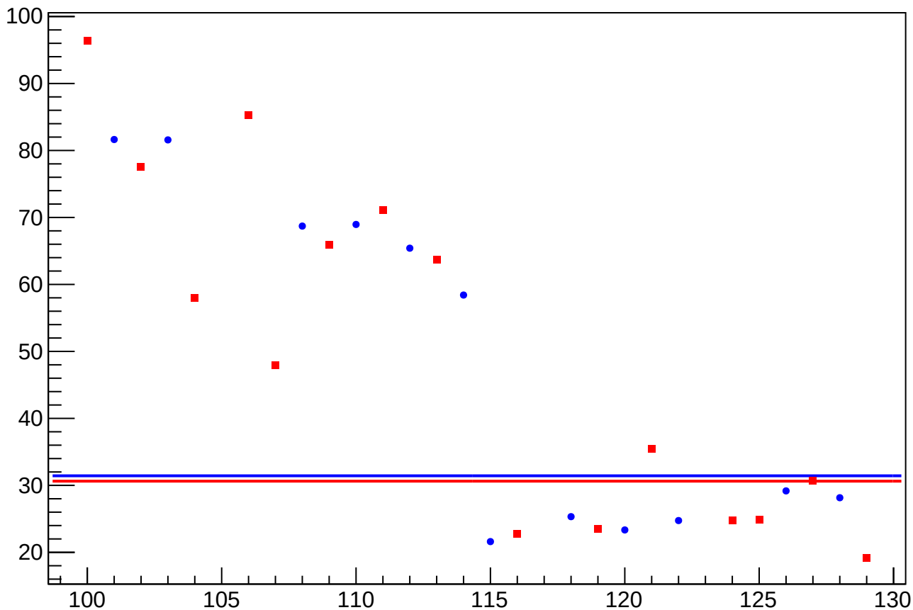
asym_sam_1526_avg_dit_vs_cor_diff_rms vs Slug, Sign Corrected
