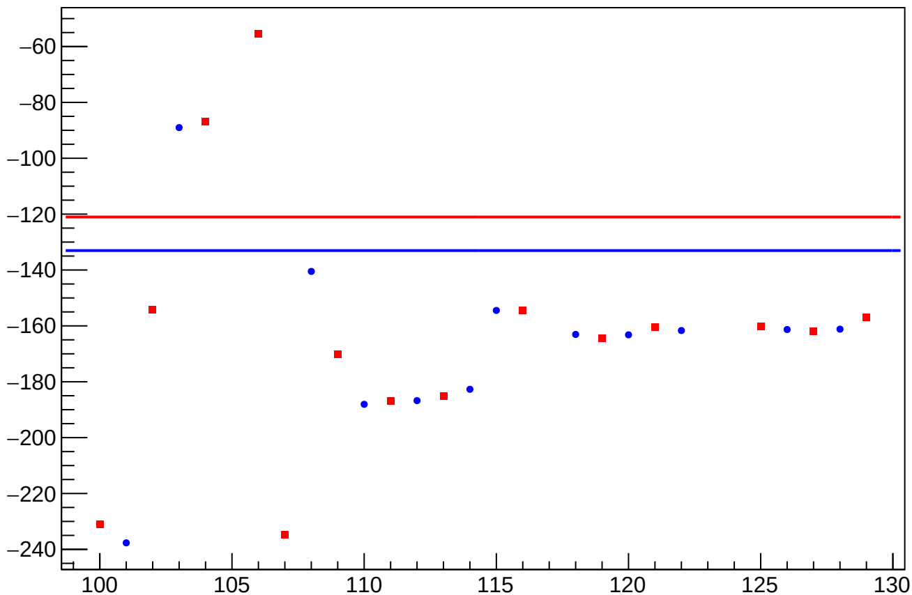
reg_asym_us_avg_atlr_avg_avg_diff_bpm12X_slope vs Slug, Sign Corrected
