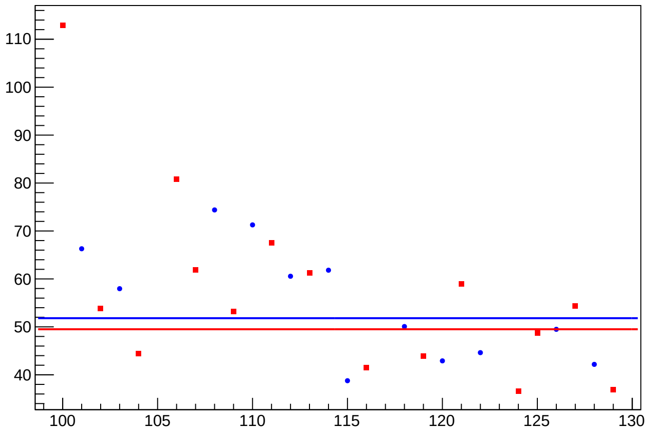
asym_sam_2468_avg_dit_vs_eigen_cor_diff_rms vs Slug, Sign Corrected
