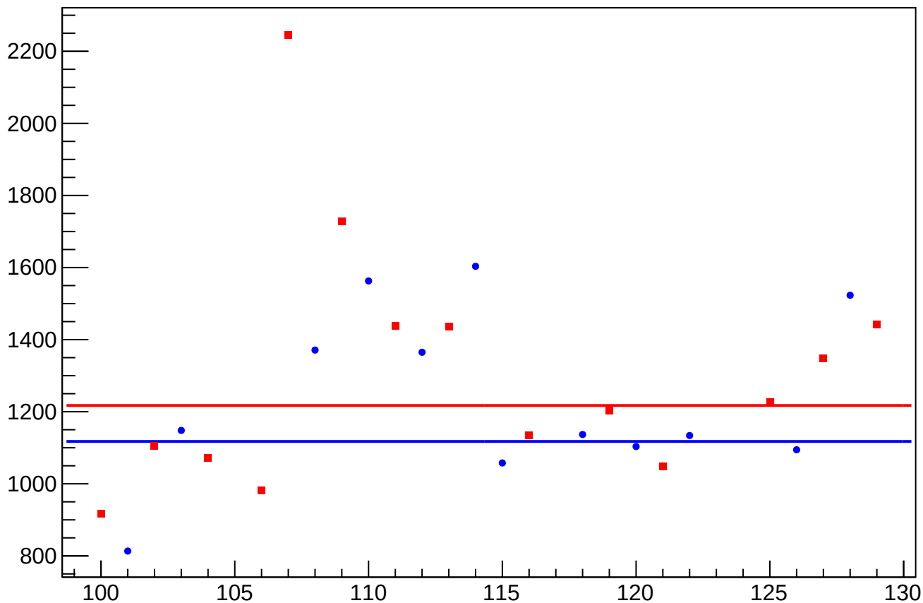
asym_us_avg_dit_correction_rms vs Slug, Sign Corrected
