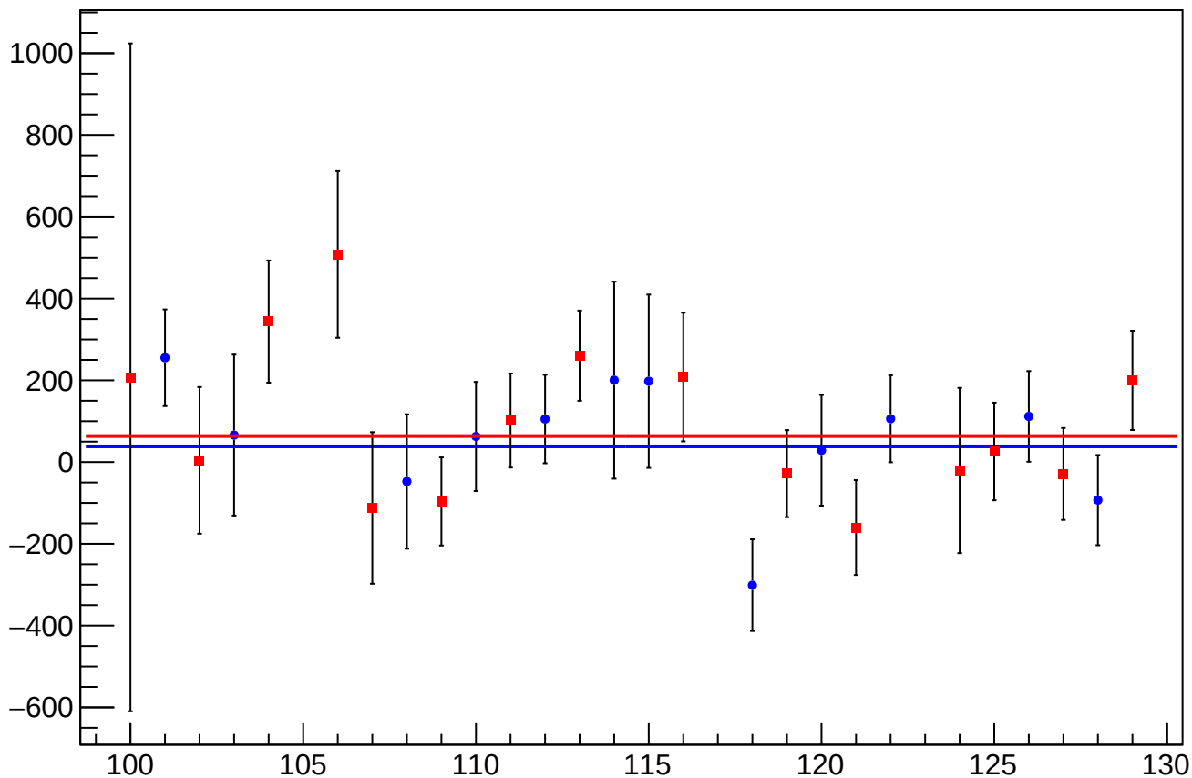
eigen_dit_asym_sam_12345678_avg_mean vs Slug, Sign Corrected
