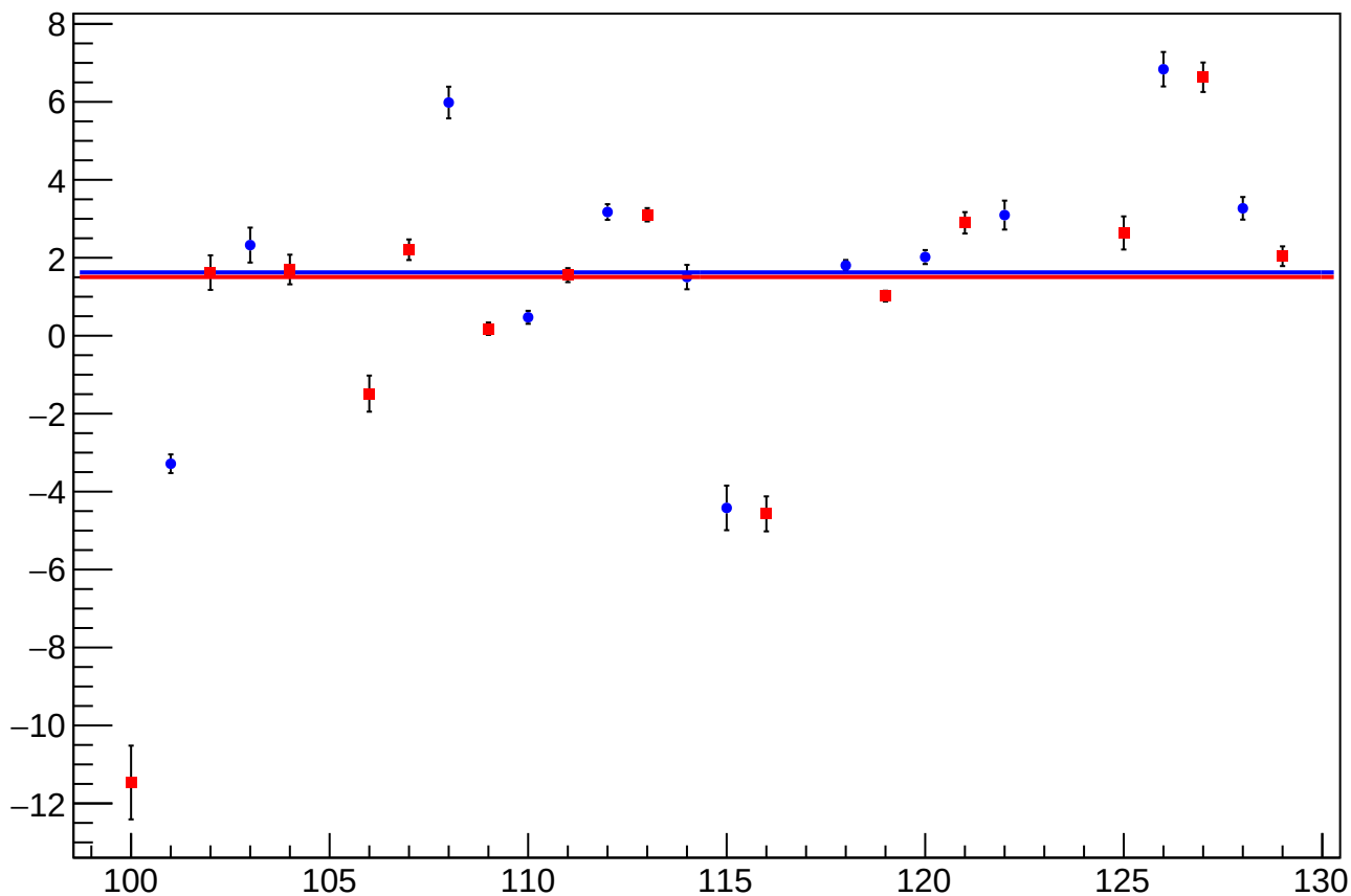
reg_asym_bcm_an_us_an_ds_avg_diff_bpm4aY_slope vs Slug, Sign Corrected
