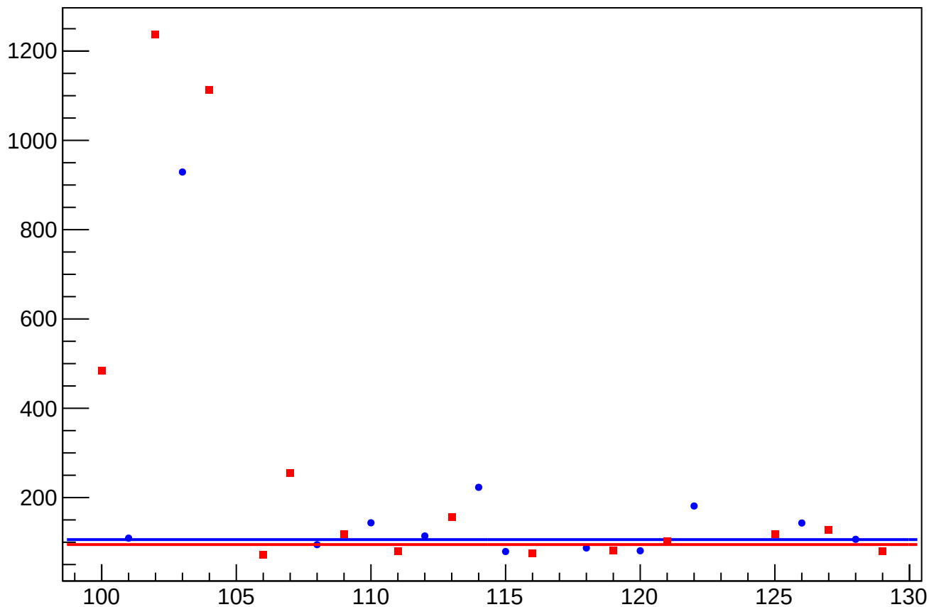
asym_us_avg_at1lr_avg_avg_eigen_dit_vs_cor_diff_rms vs Slug, Sign Corrected
