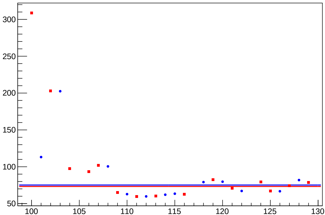
eigen_cor_asym_sam_37_avg_rms vs Slug, Sign Corrected
