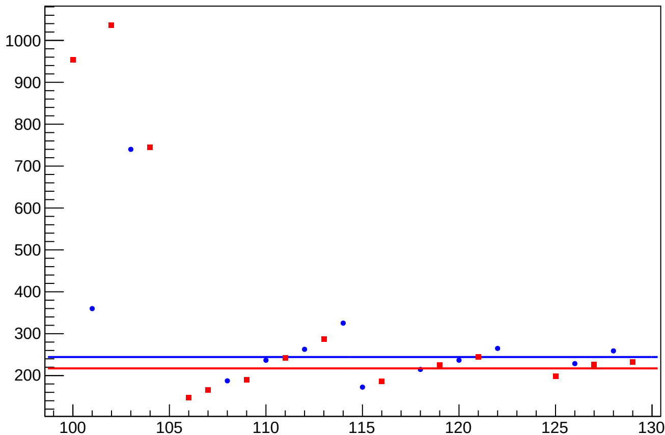
asym_us_avg_at2lr_avg_dd_eigen_dit_vs_eigen_cor_diff_rms vs Slug, Sign Corrected
