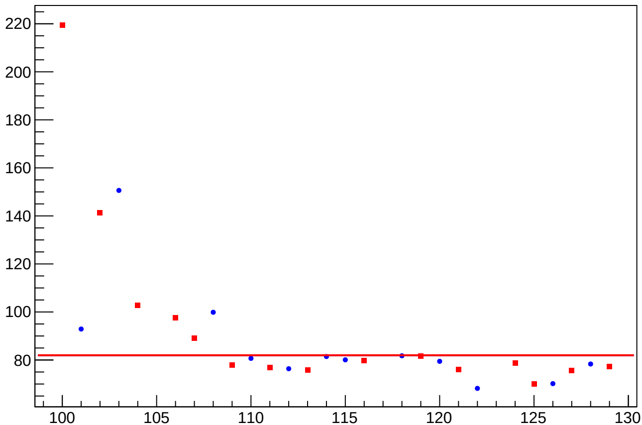
eigen_dit_asym_sam_12345678_avg_rms vs Slug, Sign Corrected
