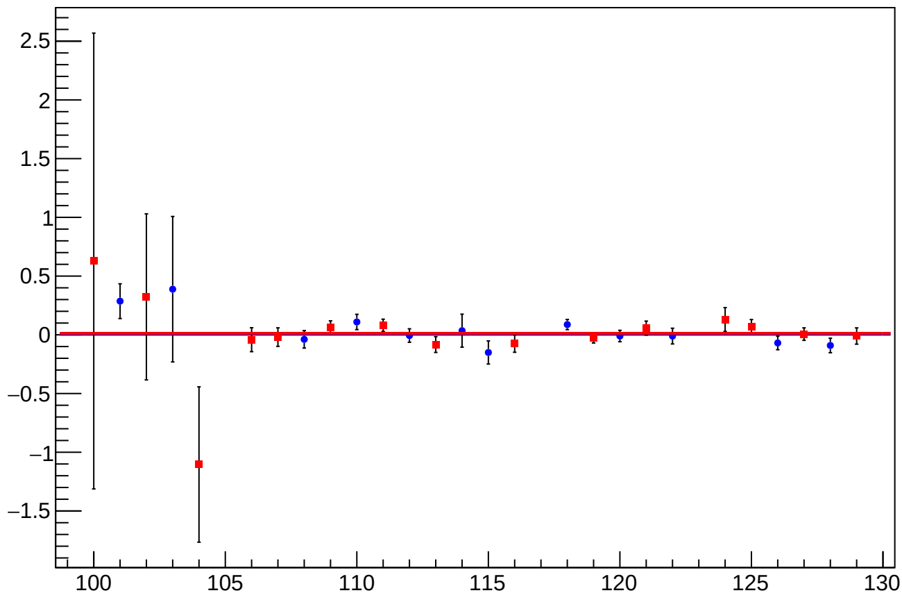
asym_usr_atr1_dd_eigen_dit_vs_eigen_cor_diff_mean vs Slug, Sign Corrected
