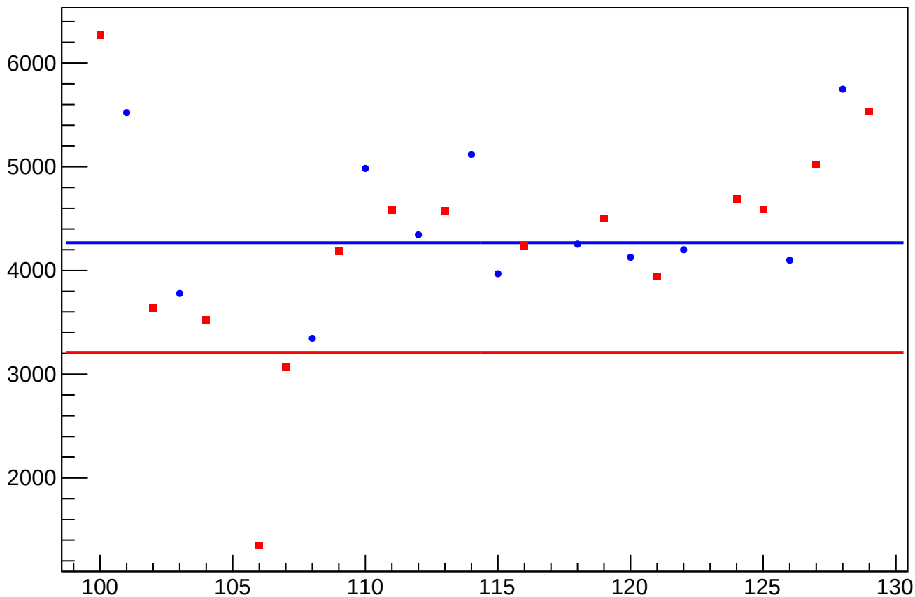
asym_atr_avg_dit_correction_rms vs Slug, Sign Corrected
