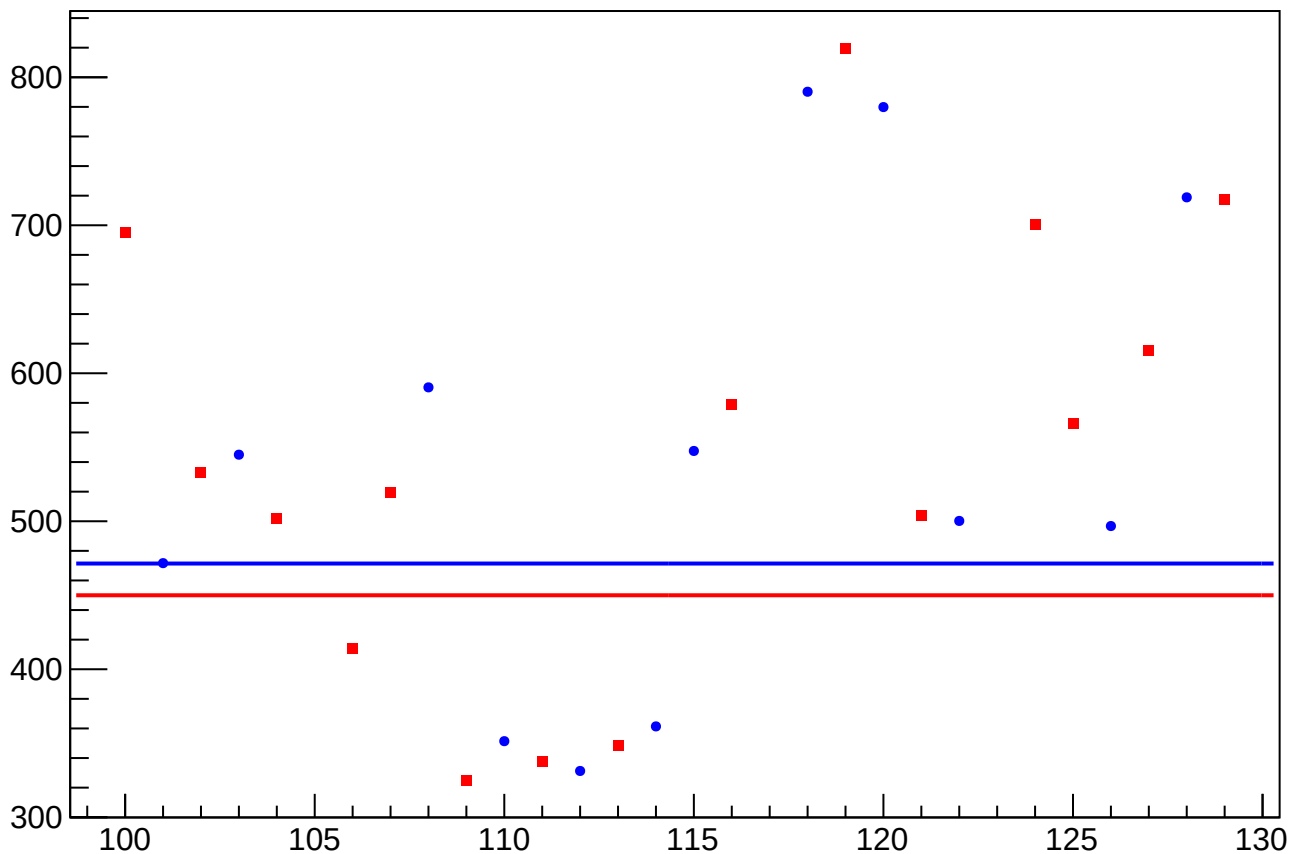
asym_sam_15_37_dd_dit_correction_rms vs Slug, Sign Corrected
