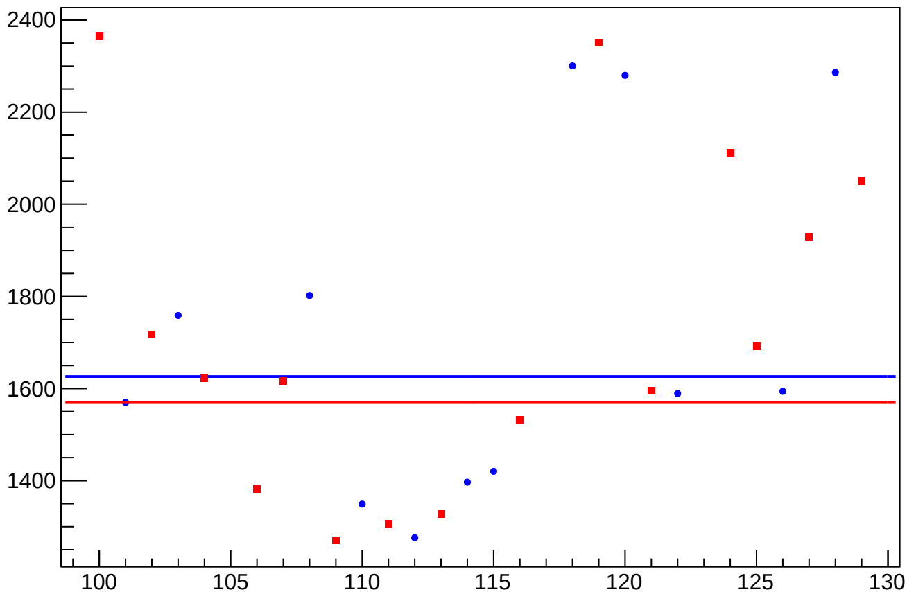
asym_sam3_dit_correction_rms vs Slug, Sign Corrected
