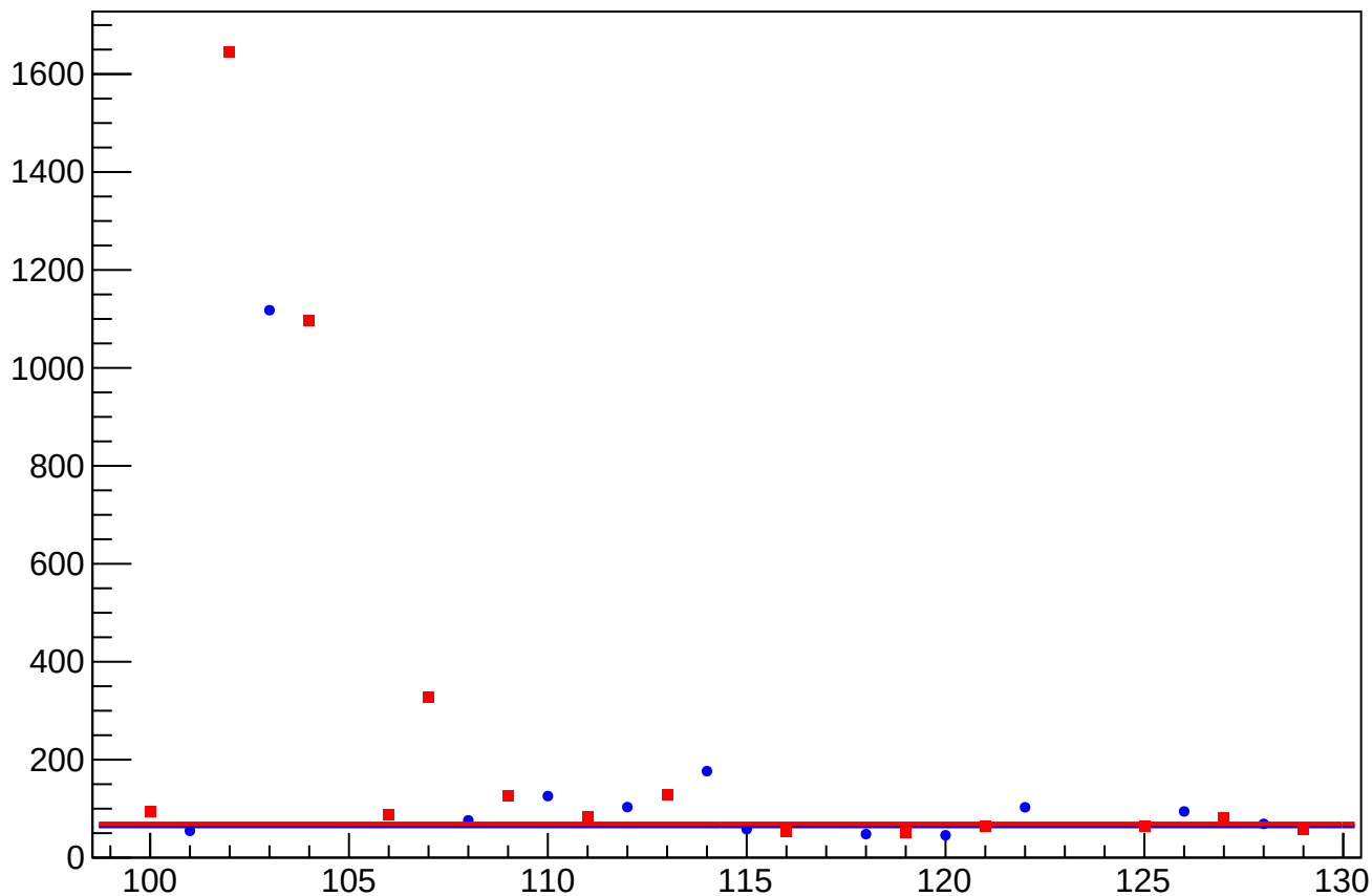
asym_atl1_eigen_dit_vs_eigen_cor_diff_rms vs Slug, Sign Corrected
