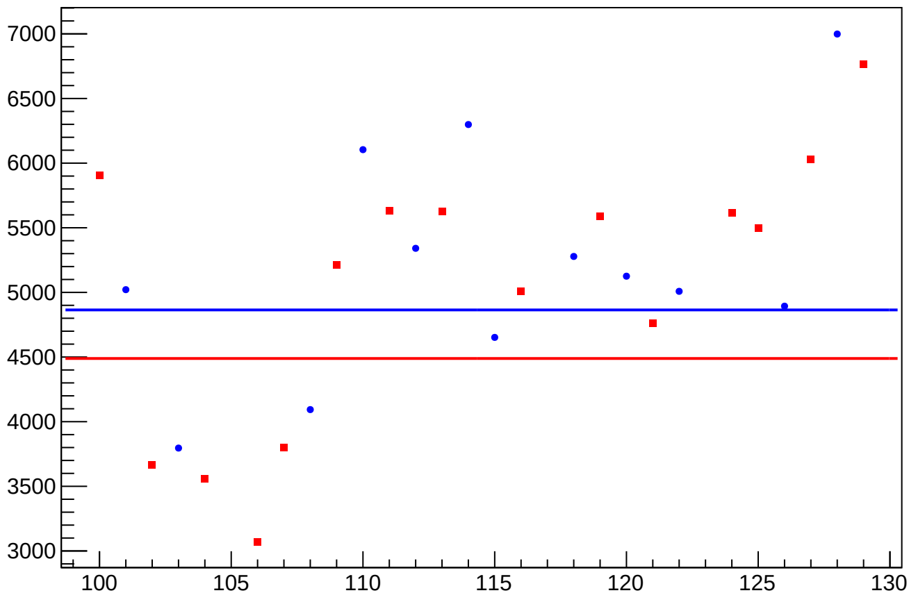
asym_usr_atr2_avg_dit_correction_rms vs Slug, Sign Corrected
