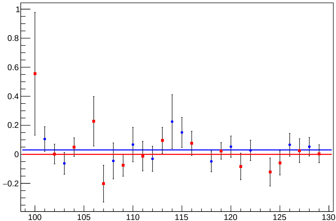
asym_sam_2468_avg_eigen_dit_vs_cor_diff_mean vs Slug, Sign Corrected
