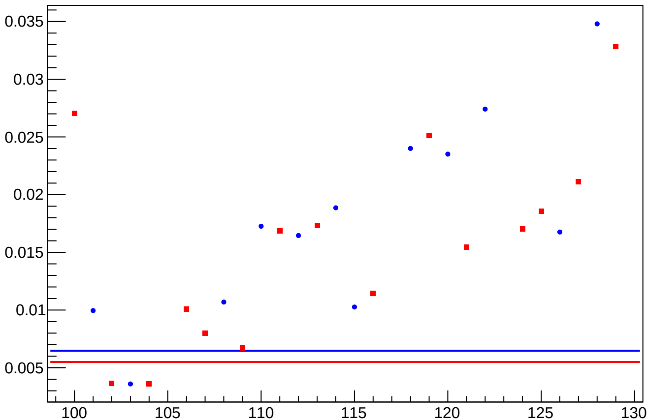
asym_usr_atr2_avg_eigen_dit_vs_dit_diff_rms vs Slug, Sign Corrected
