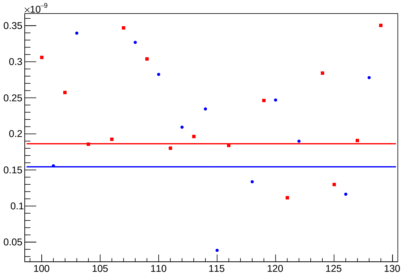
asym_sam2_reg_vs_cor_diff_rms vs Slug, Sign Corrected
