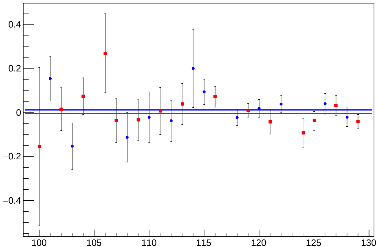
asym_sam_1526_avg_dit_vs_eigen_cor_diff_mean vs Slug, Sign Corrected
