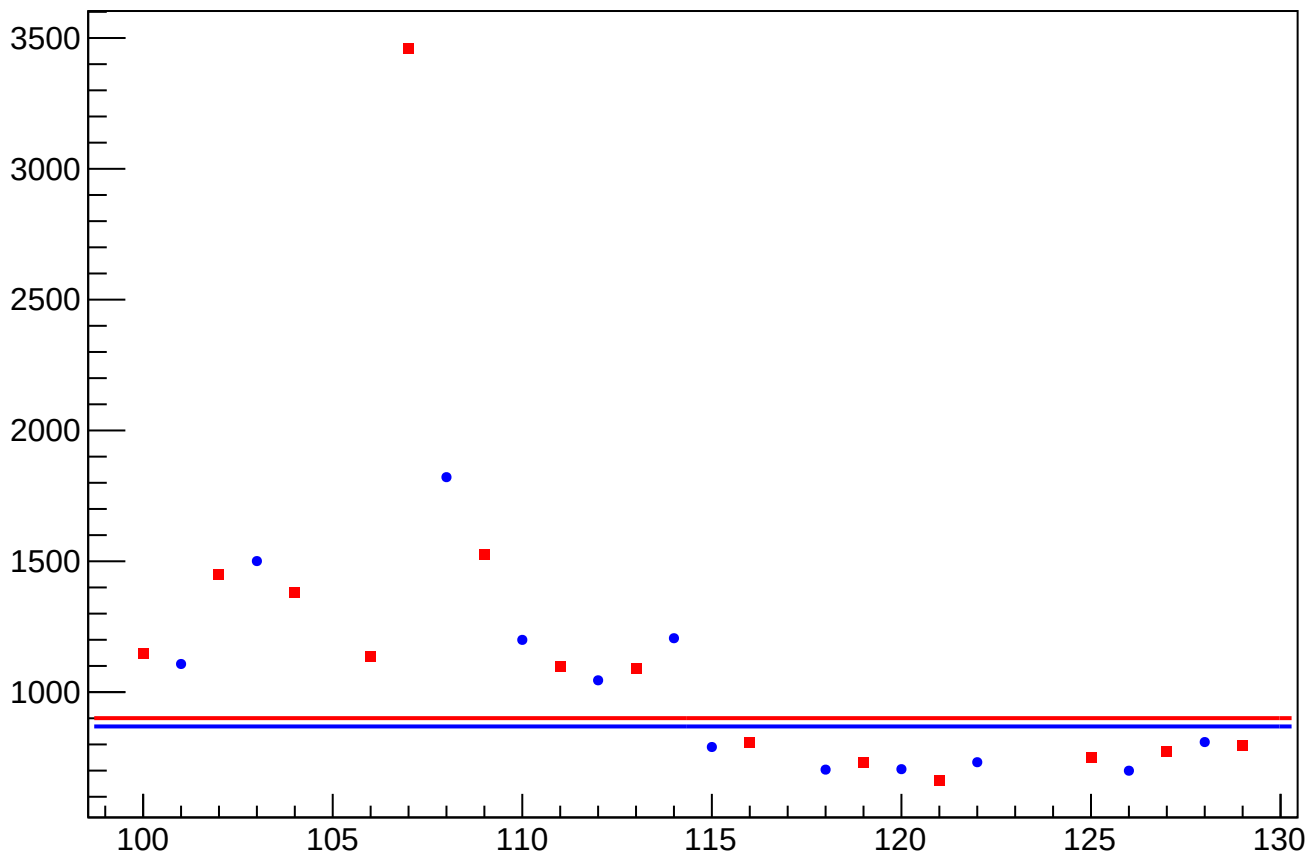
asym_usl_dit_correction_rms vs Slug, Sign Corrected
