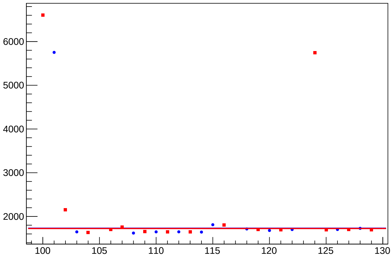
eigen_cor_asym_atr1l2_avg_rms vs Slug, Sign Corrected
