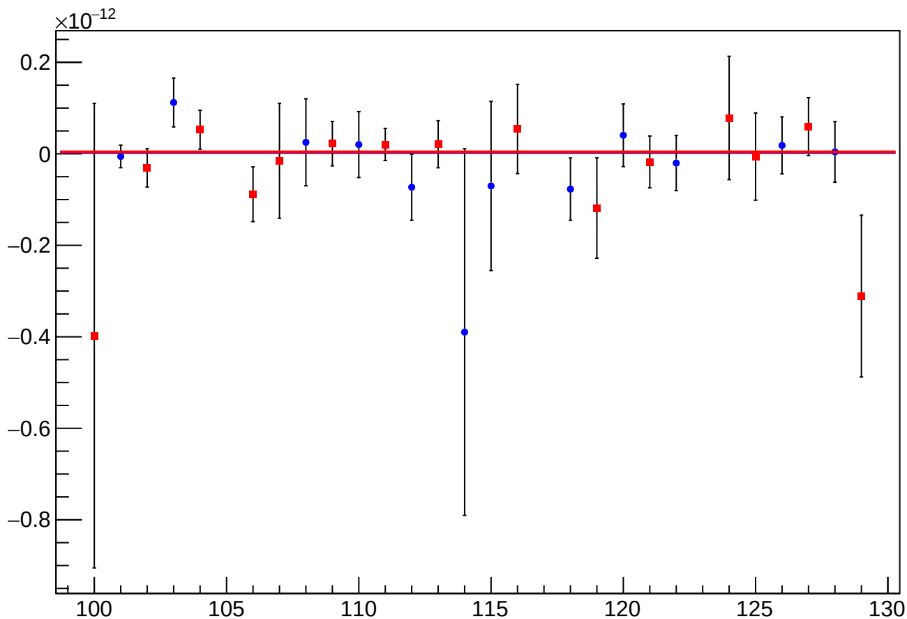
asym_sam7_reg_vs_cor_diff_mean vs Slug, Sign Corrected
