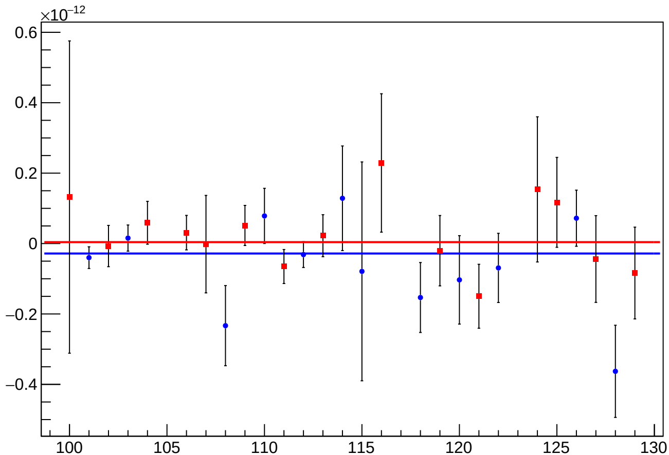
asym_sam_48_avg_eigen_cor_vs_cor_diff_mean vs Slug, Sign Corrected
