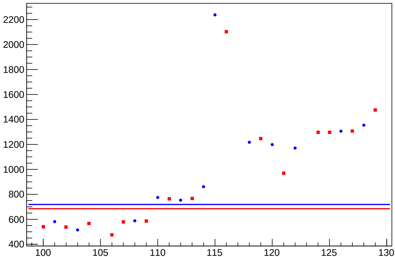
asym_sam5_eigen_dit_correction_rms vs Slug, Sign Corrected
