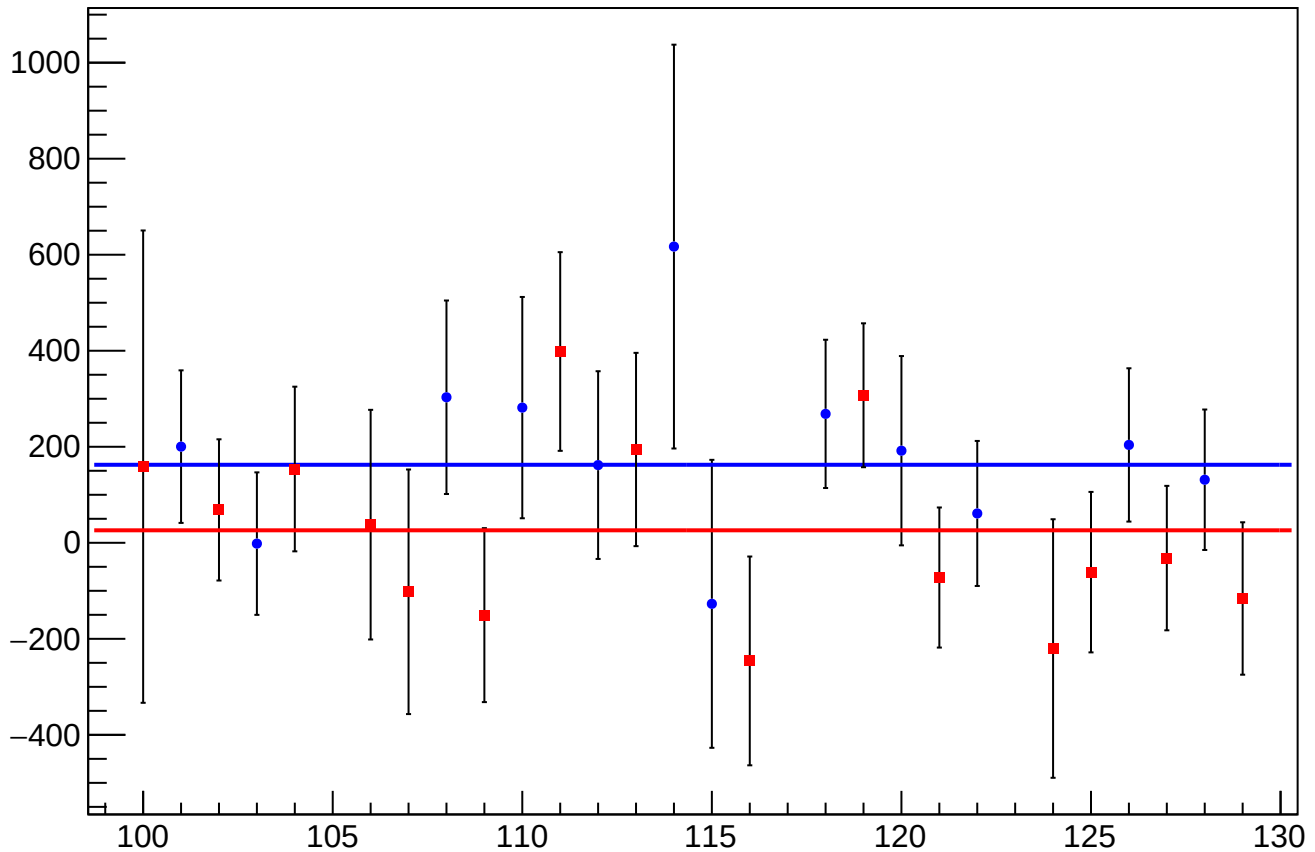
eigen_cor_asym_sam_26_48_dd_mean vs Slug, Sign Corrected
