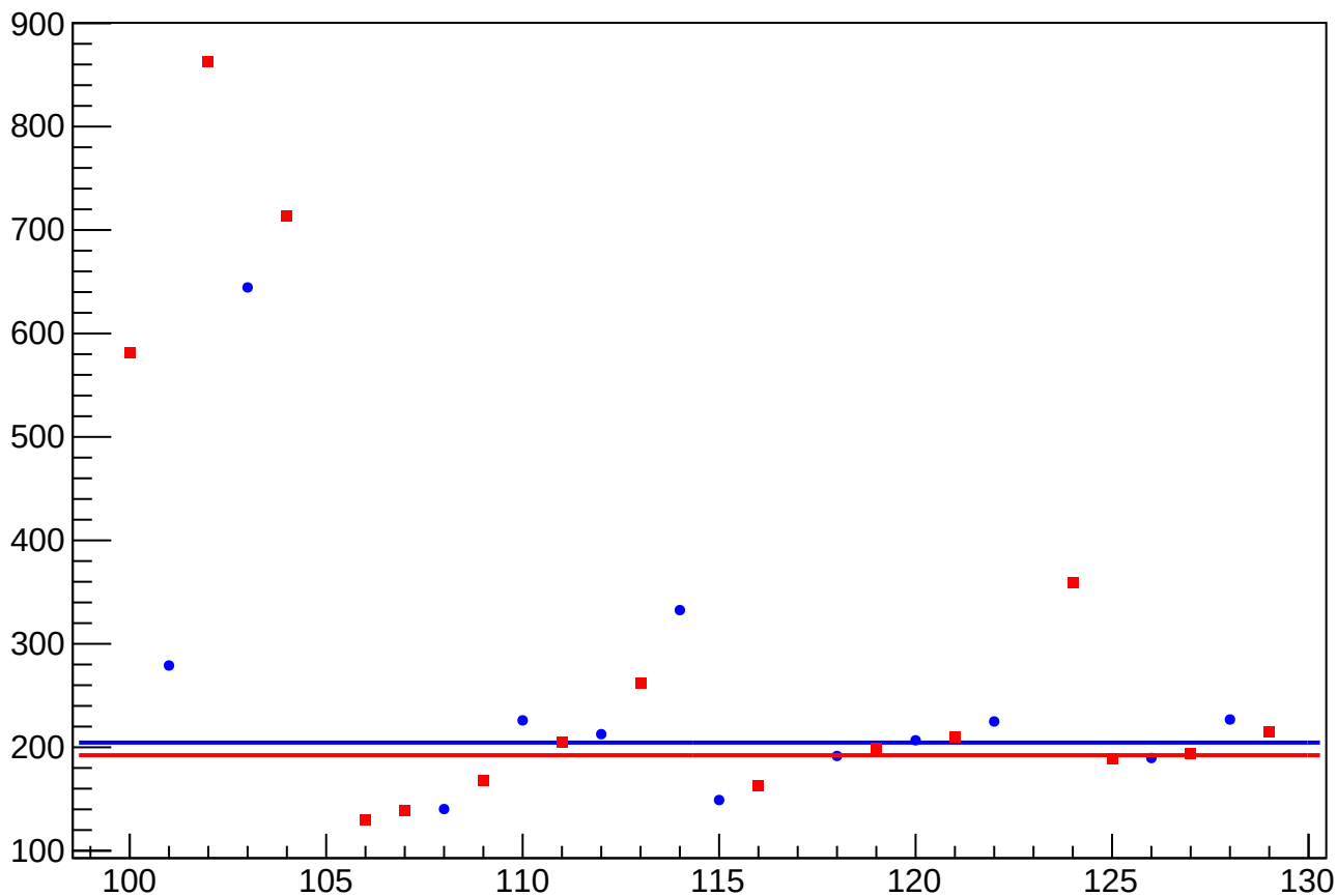
asym_usr_atr2_avg_dit_vs_cor_diff_rms vs Slug, Sign Corrected
