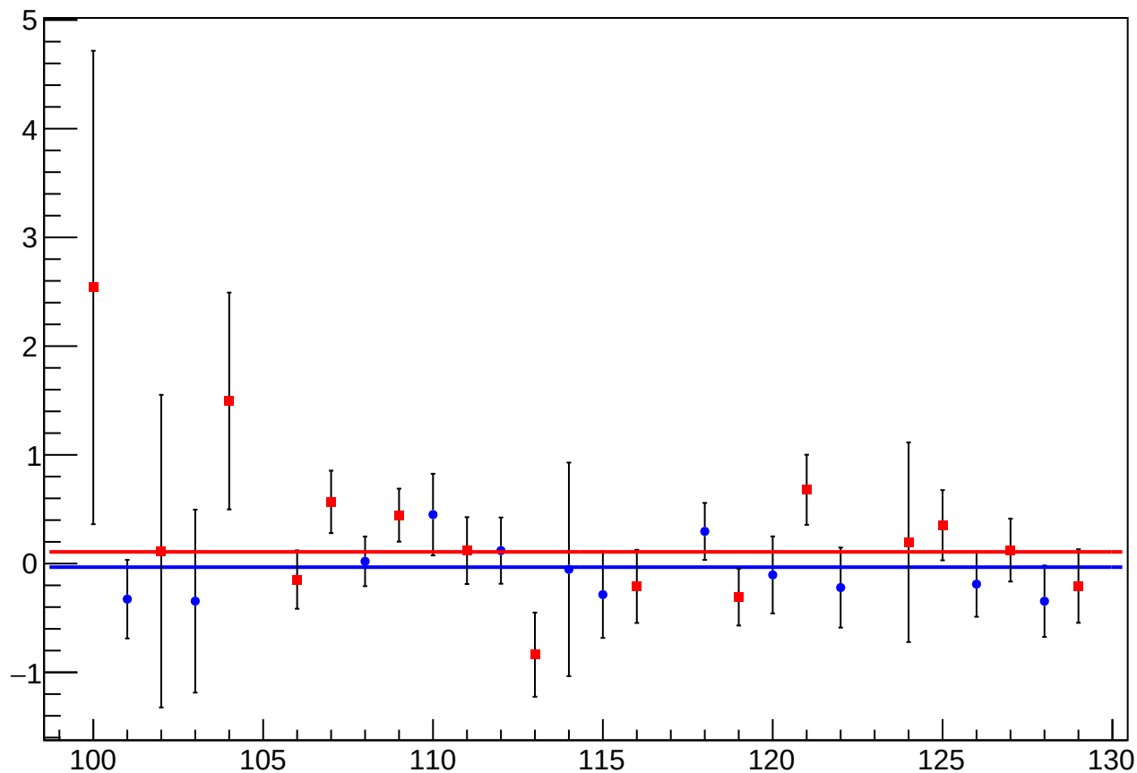
asym_usr_atr2_avg_dit_vs_eigen_cor_diff_mean vs Slug, Sign Corrected
