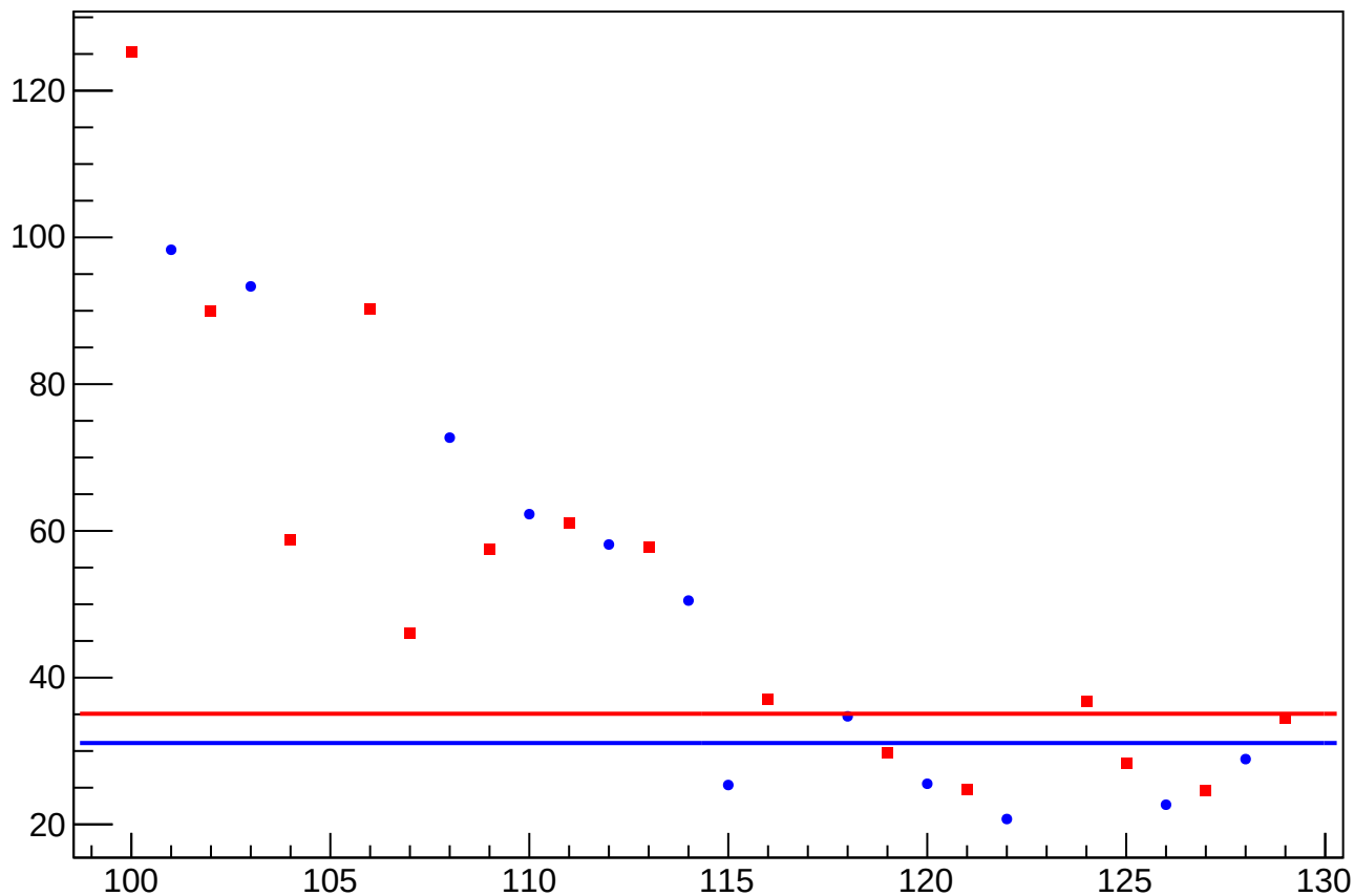
asym_sam_26_48_dd_eigen_dit_vs_eigen_cor_diff_rms vs Slug, Sign Corrected
