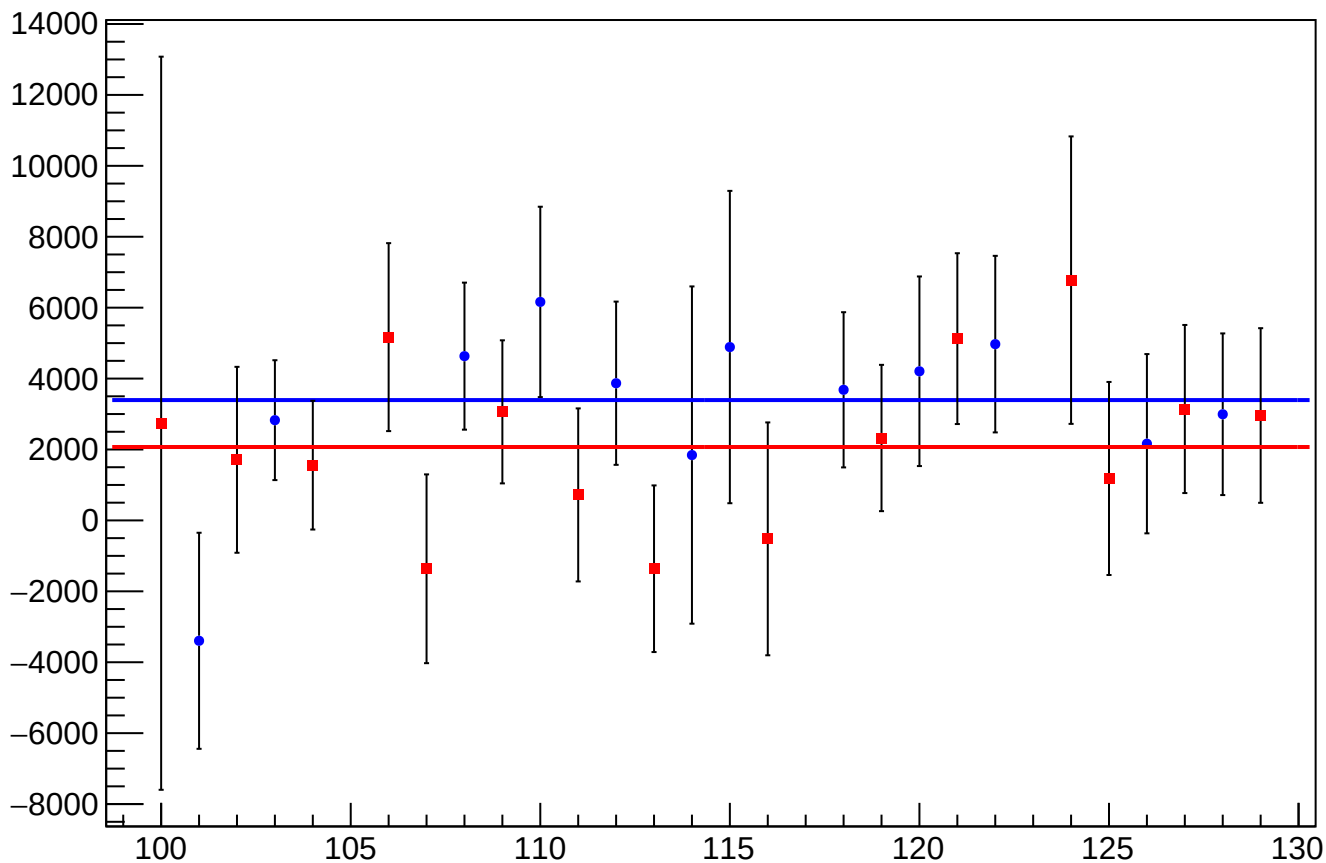
reg_asym_usr_atr2_avg_mean vs Slug, Sign Corrected
