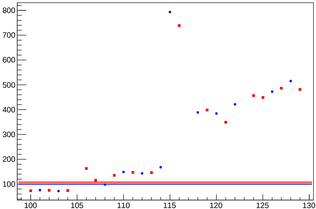
asym_sam_15_avg_dit_correction_rms vs Slug, Sign Corrected
