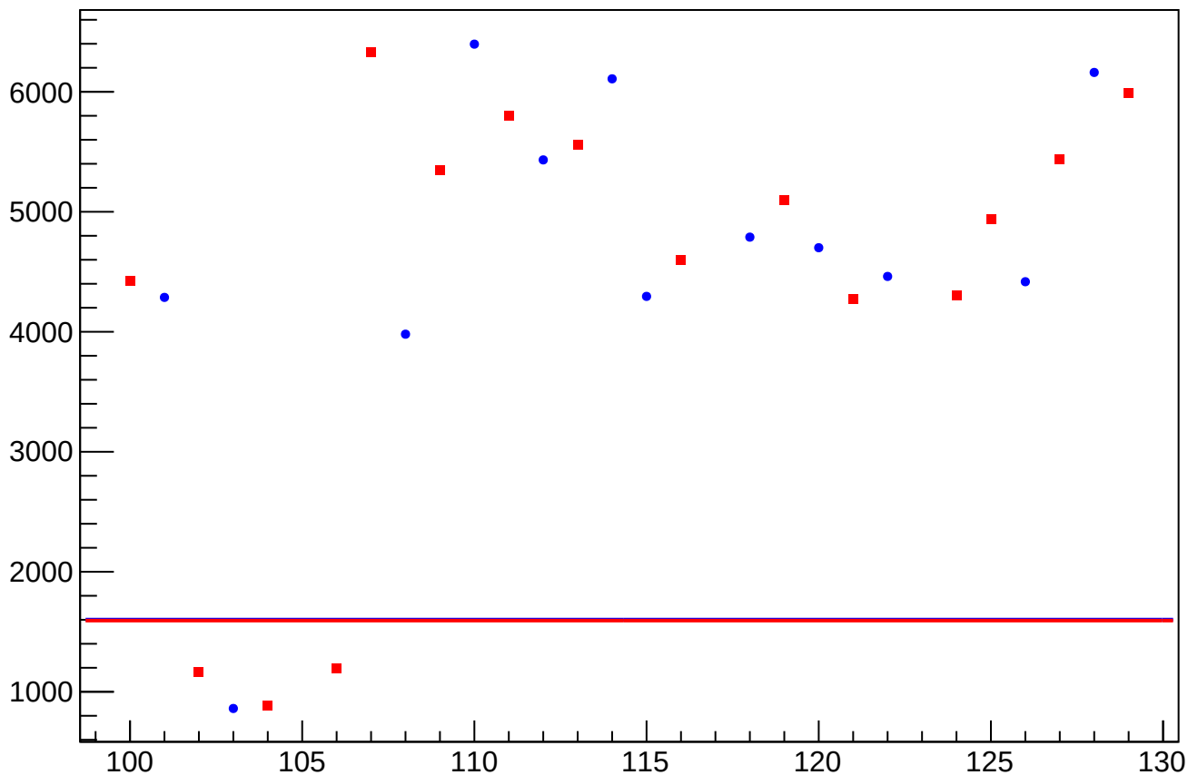
asym_atl1r2_avg_reg_correction_rms vs Slug, Sign Corrected
