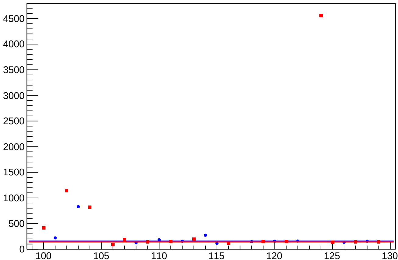
asym_atl_avg_atr_avg_avg_eigen_dit_vs_eigen_cor_diff_rms vs Slug, Sign Corrected
