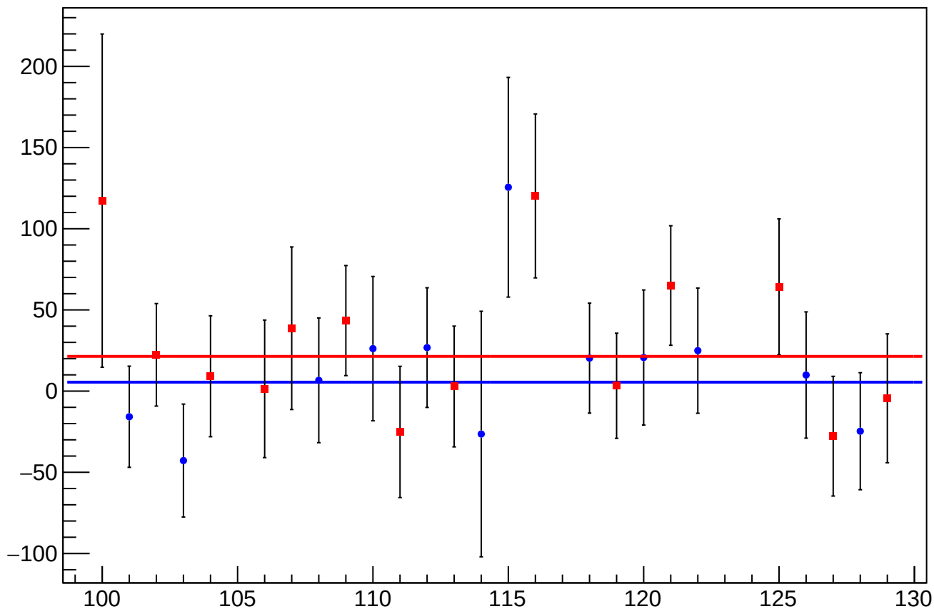
asym_bcm_dg_us_dg_ds_dd_mean vs Slug, Sign Corrected
