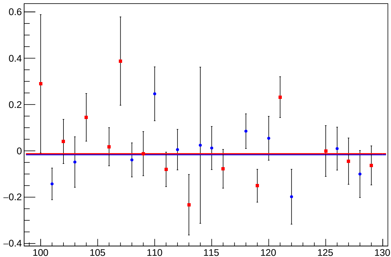
asym_us_avg_dit_vs_cor_diff_mean vs Slug, Sign Corrected
