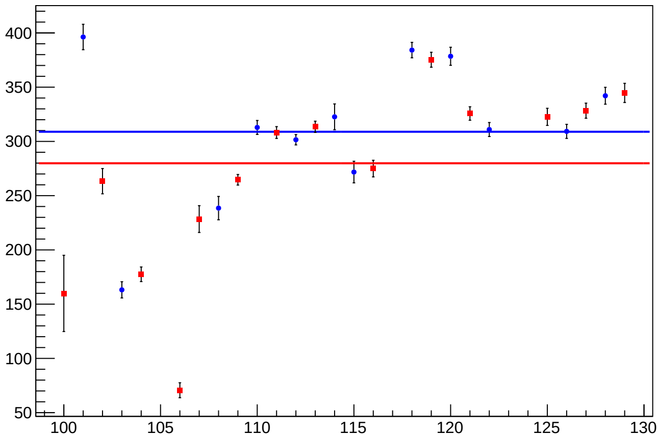
reg_asym_us_avg_at2lr_avg_dd_diff_bpm1X_slope vs Slug, Sign Corrected
