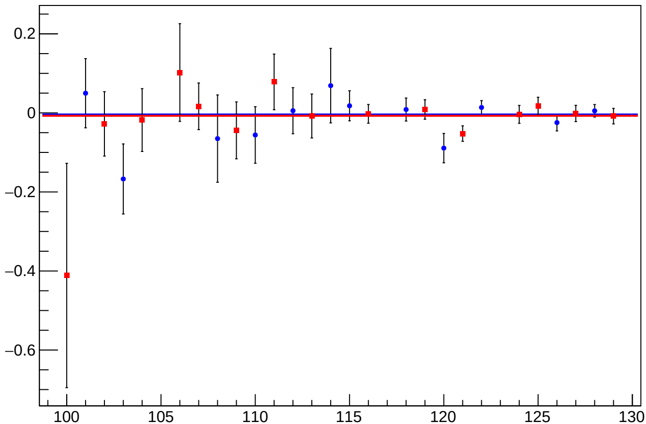
asym_sam1_dit_vs_cor_diff_mean vs Slug, Sign Corrected
