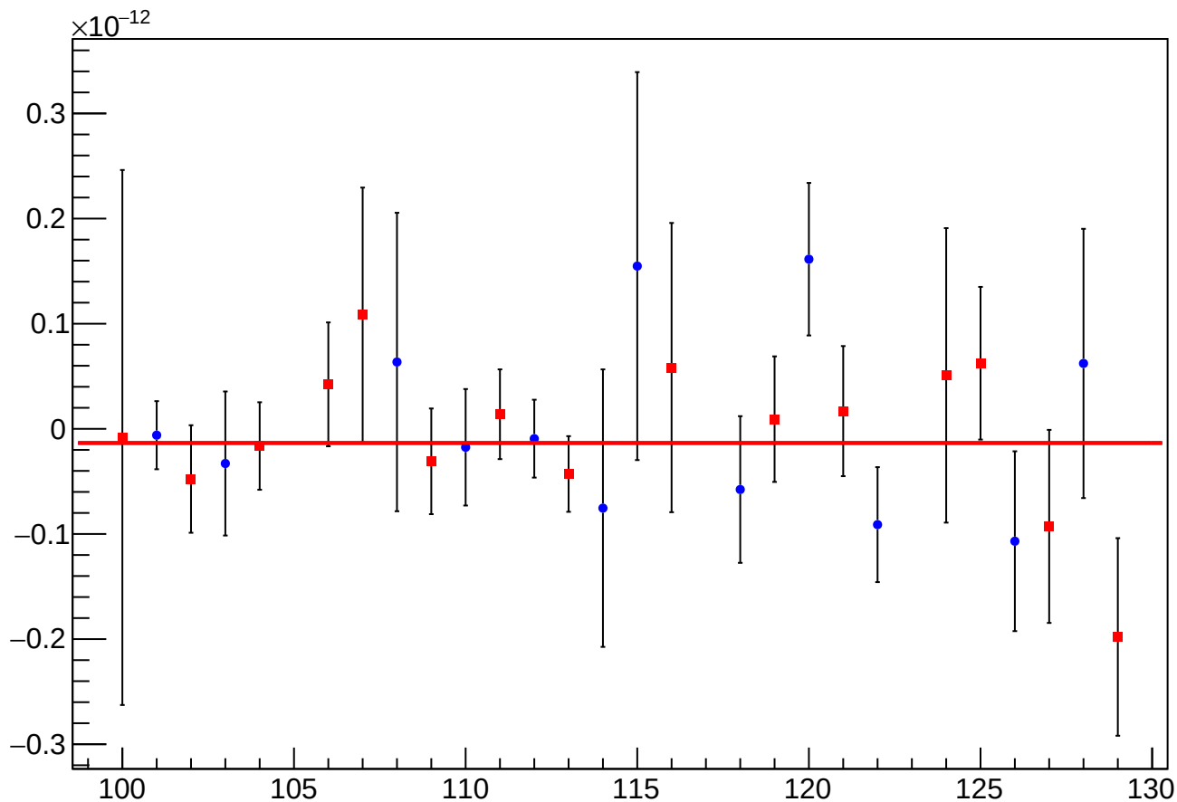
asym_sam_48_dd_eigen_cor_vs_cor_diff_mean vs Slug, Sign Corrected
