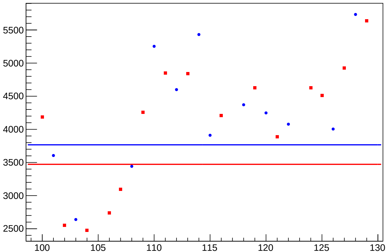
asym_atr_dd_eigen_dit_correction_rms vs Slug, Sign Corrected
