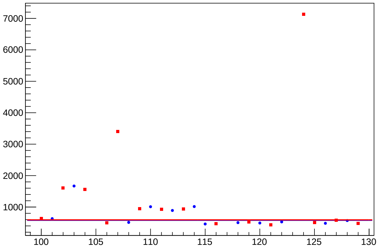
asym_at1_avg_dit_correction_rms vs Slug, Sign Corrected
