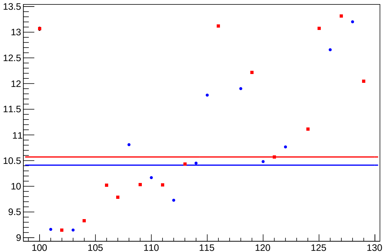
asym_bcm_an_us_an_ds3_dd_rms vs Slug, Sign Corrected
