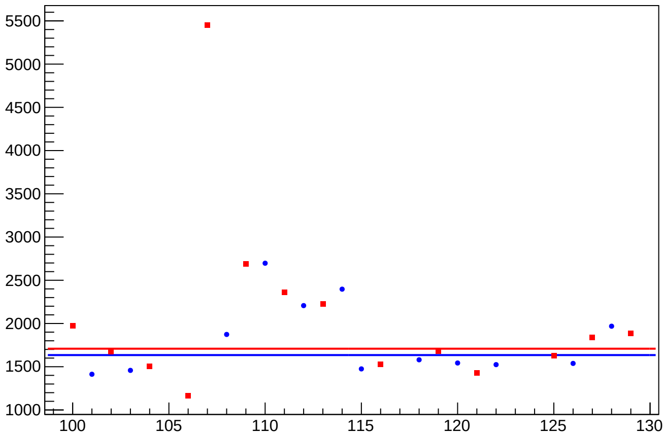
asym_us_avg_at1lr_avg_avg_cor_correction_rms vs Slug, Sign Corrected
