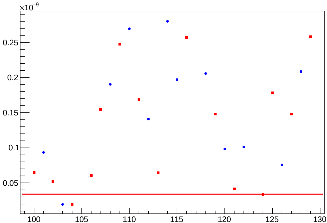
asym_atl_avg_reg_vs_cor_diff_rms vs Slug, Sign Corrected
