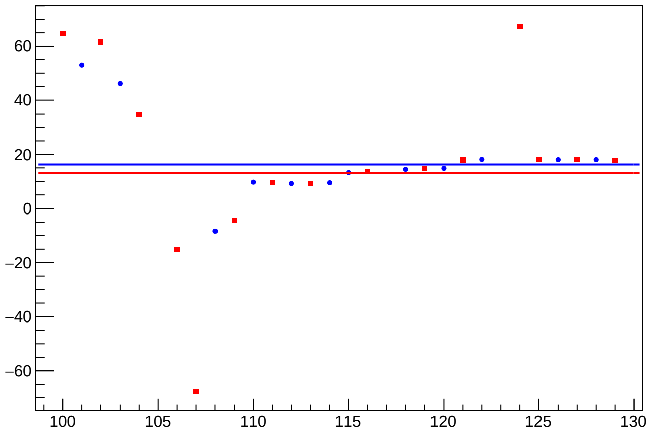
reg_asym_atl1r2_dd_atl2r1_dd_avg_diff_bpm12X_slope vs Slug, Sign Corrected
