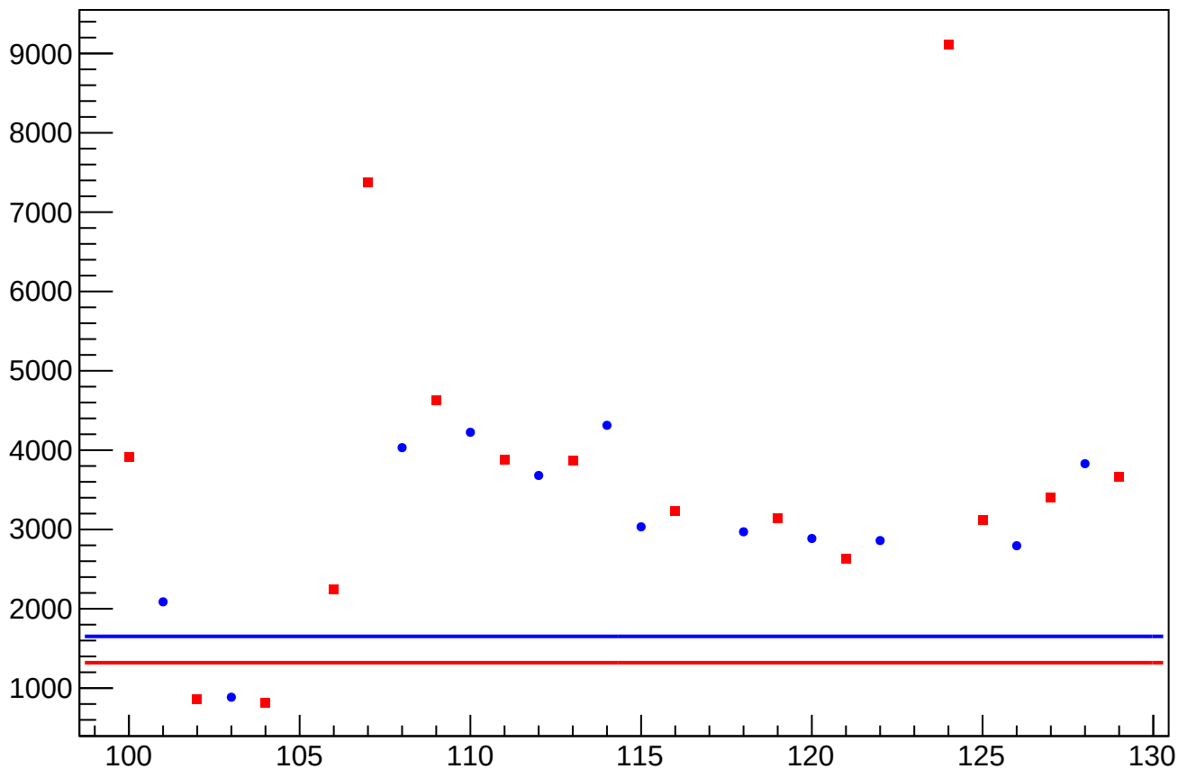
asym_atl_avg_eigen_dit_correction_rms vs Slug, Sign Corrected
