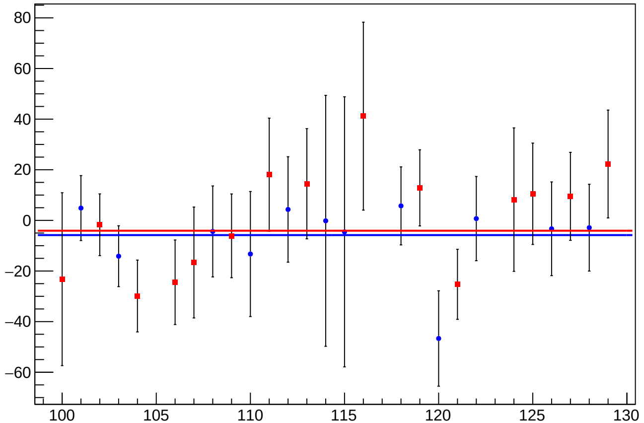
diff_bpmtargetsumY_mean vs Slug, Sign Corrected
