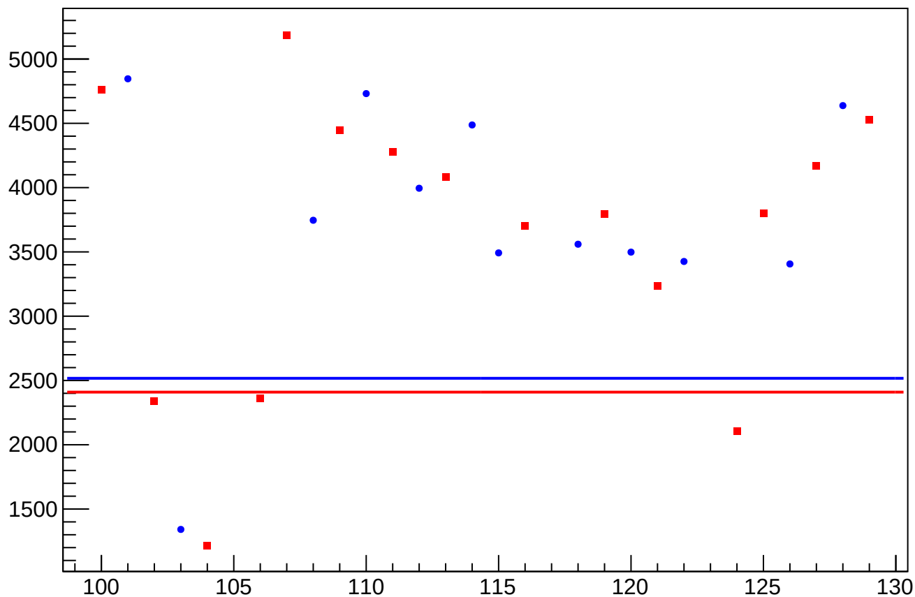
asym_atl_avg_atr_avg_avg_eigen_cor_correction_rms vs Slug, Sign Corrected
