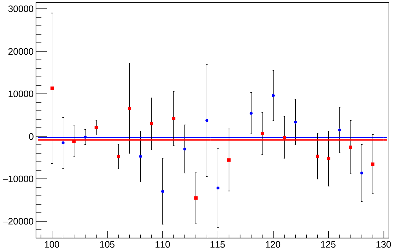
asym_atl_avg_atr_avg_avg_reg_correction_mean vs Slug, Sign Corrected
