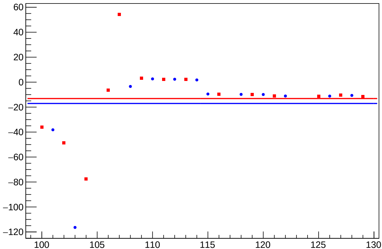
reg_asym_usl_atl1_dd_diff_bpm12X_slope vs Slug, Sign Corrected
