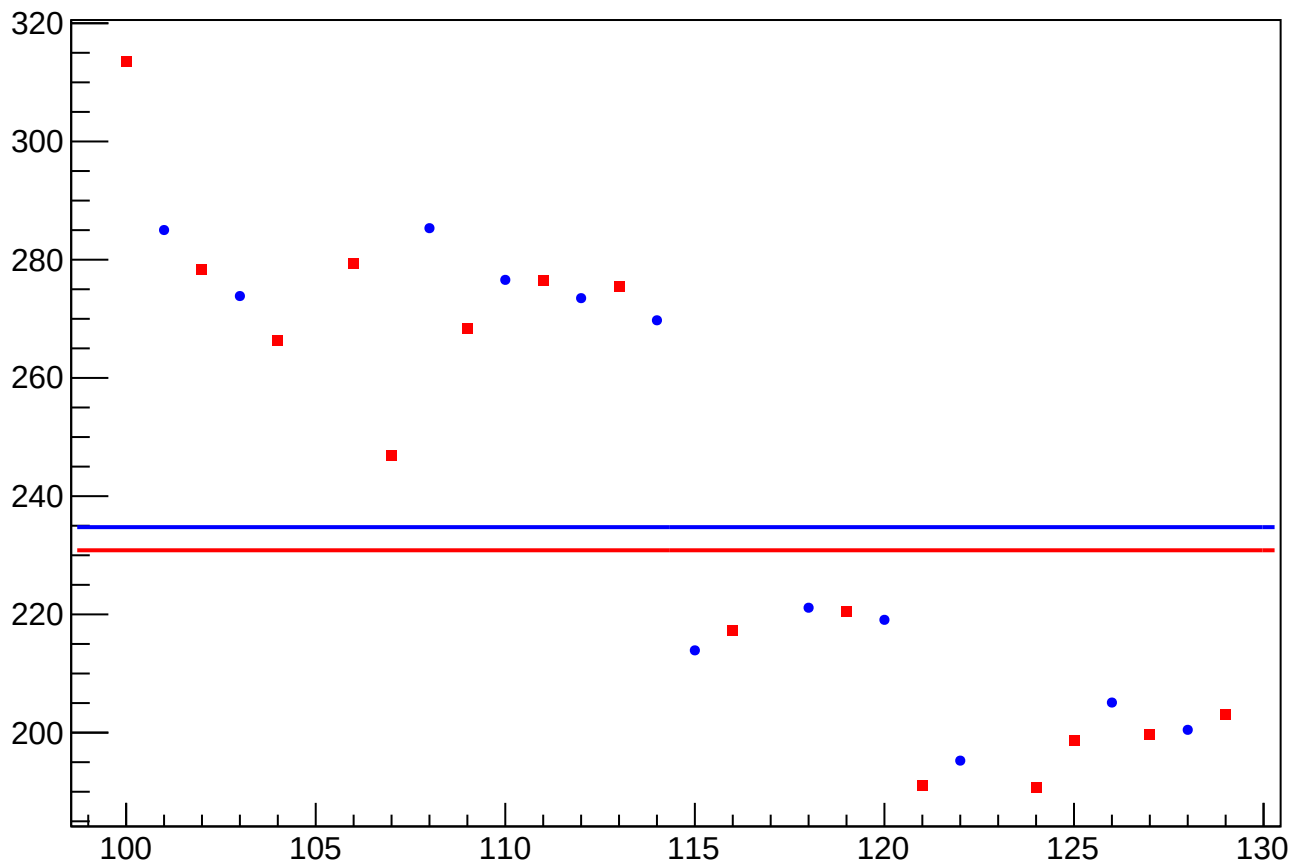
eigen_dit_asym_sam_26_dd_rms vs Slug, Sign Corrected
