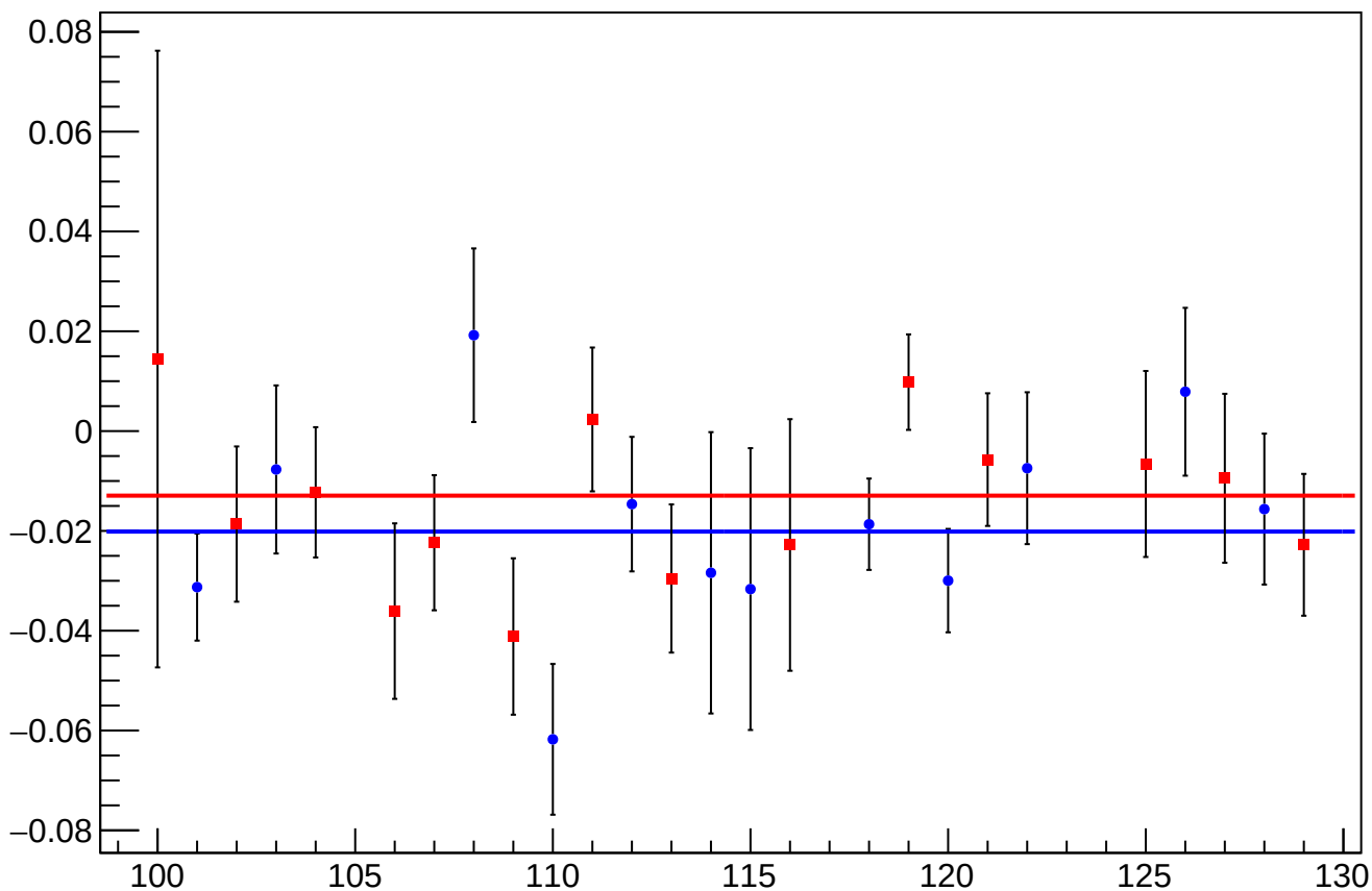
reg_asym_bcm_an_us_an_ds_dd_diff_bpm4aY_slope vs Slug, Sign Corrected
