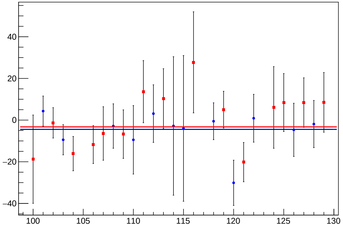
diff_targ_positionY_mean vs Slug, Sign Corrected
