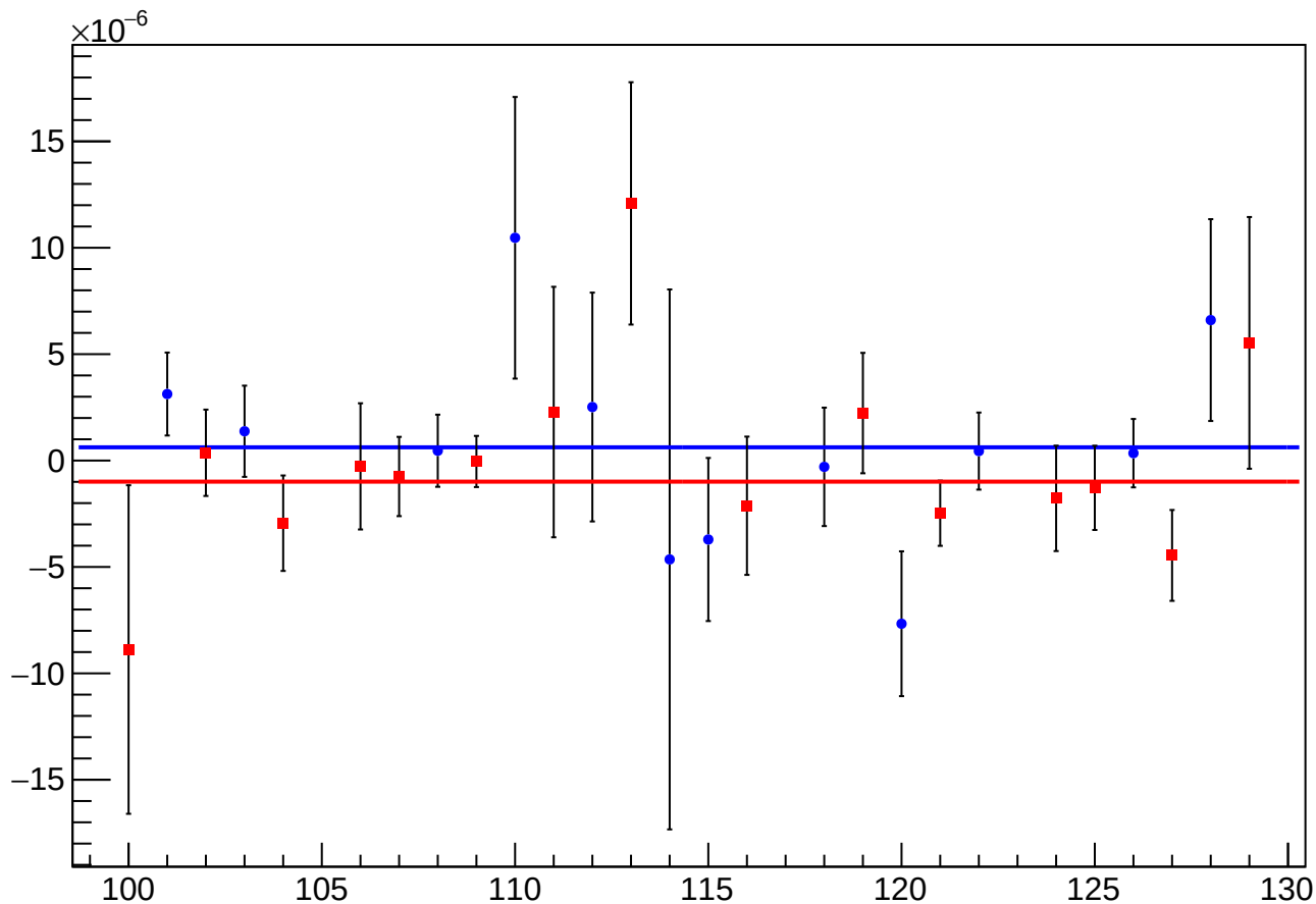
asym_sam_1357_2468_dd_eigen_dit_vs_dit_diff_mean vs Slug, Sign Corrected
