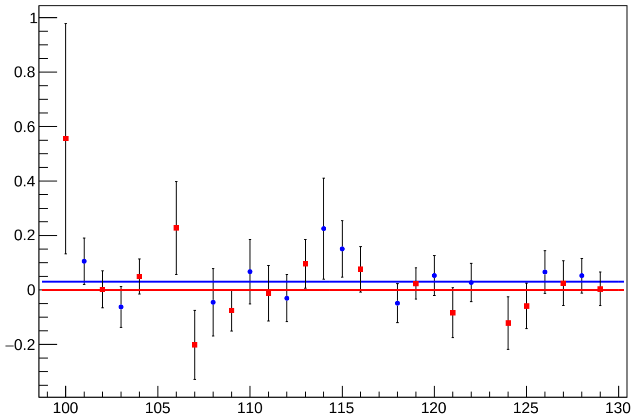
asym_sam_2468_avg_dit_vs_eigen_cor_diff_mean vs Slug, Sign Corrected
