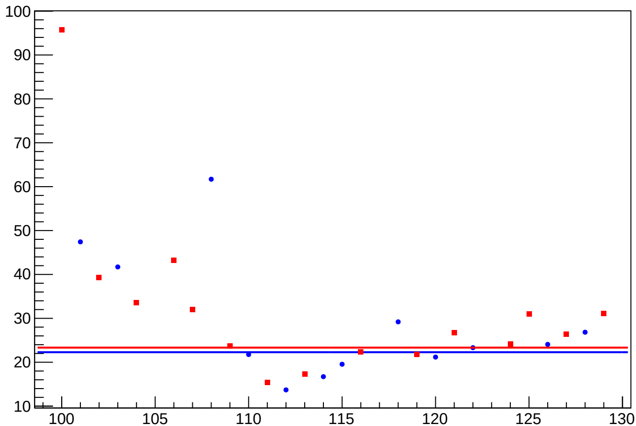
asym_sam_15_48_dd_dit_vs_eigen_cor_diff_rms vs Slug, Sign Corrected
