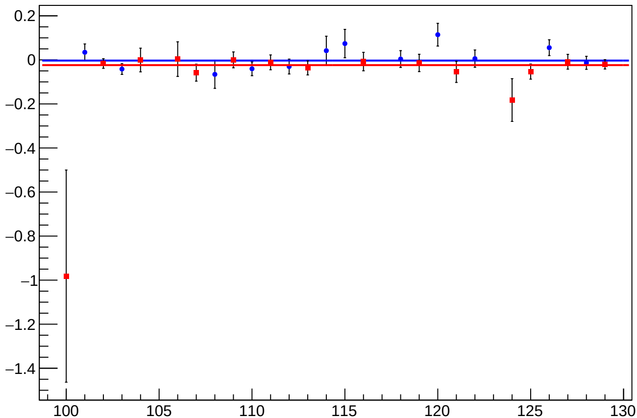
asym_sam_1357_avg_dit_vs_cor_diff_mean vs Slug, Sign Corrected
