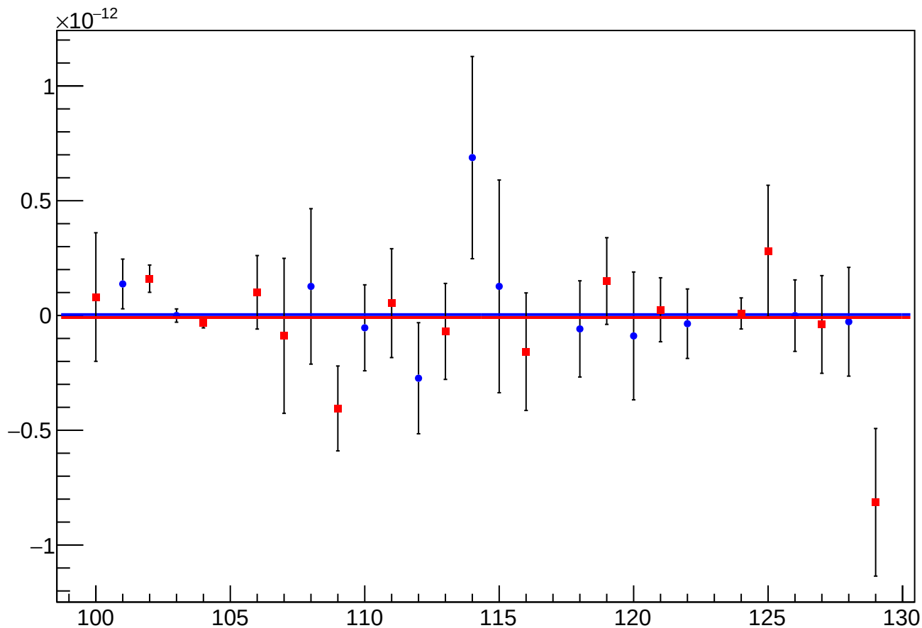
asym_atl_avg_eigen_cor_vs_cor_diff_mean vs Slug, Sign Corrected
