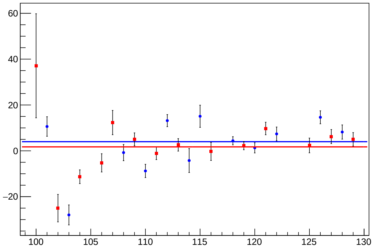
reg_asym_us_dd_atlr_dd_avg_diff_bpm4aY_slope vs Slug, Sign Corrected
