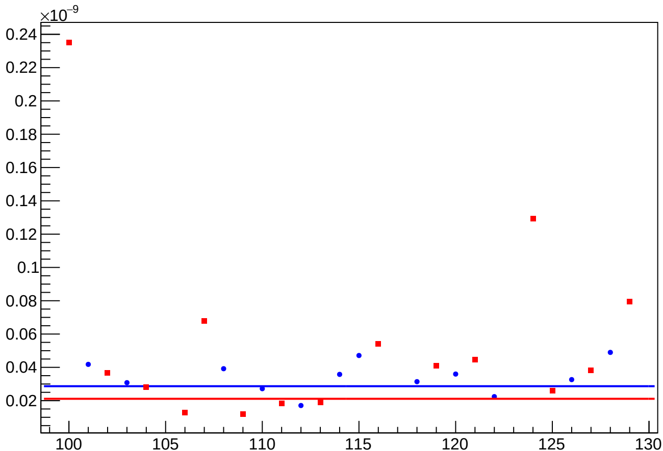
asym_atl1r2_dd_atl2r1_dd_avg_reg_vs_cor_diff_rms vs Slug, Sign Corrected
