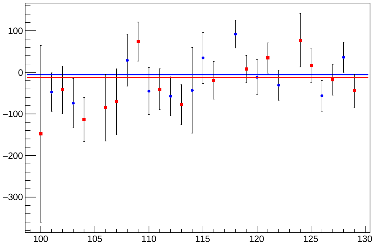
cor_asym_sam_1357_2468_dd_mean vs Slug, Sign Corrected
