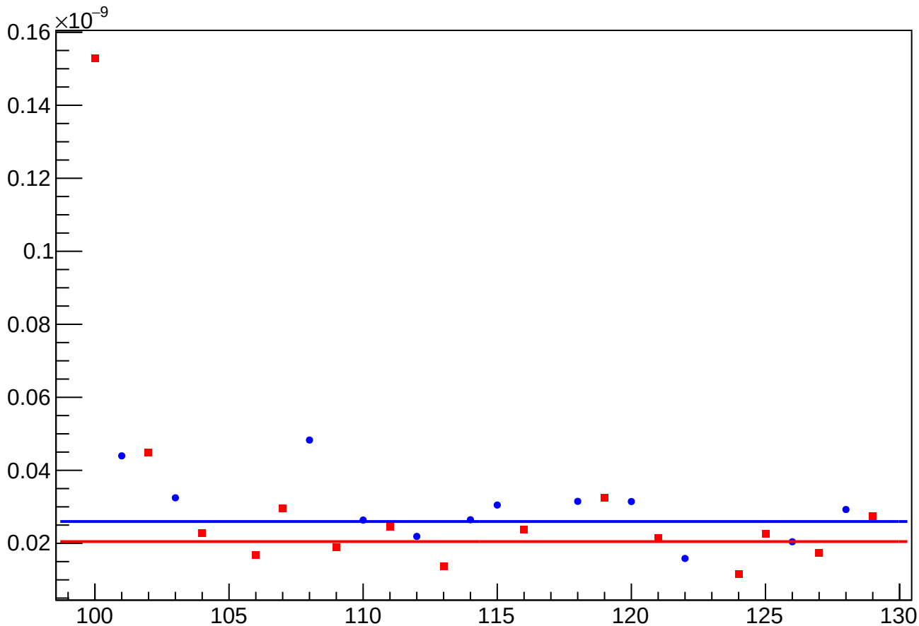
asym_atr1_eigen_cor_vs_cor_diff_rms vs Slug, Sign Corrected
