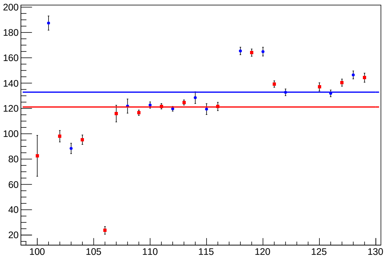
reg_asym_usl_atl2_dd_diff_bpm1X_slope vs Slug, Sign Corrected
