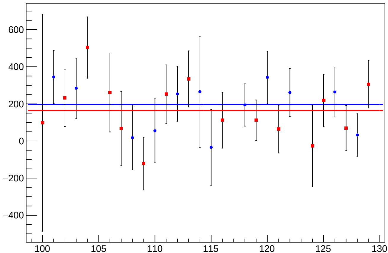
cor_asym_sam_24_68_dd_mean vs Slug, Sign Corrected
