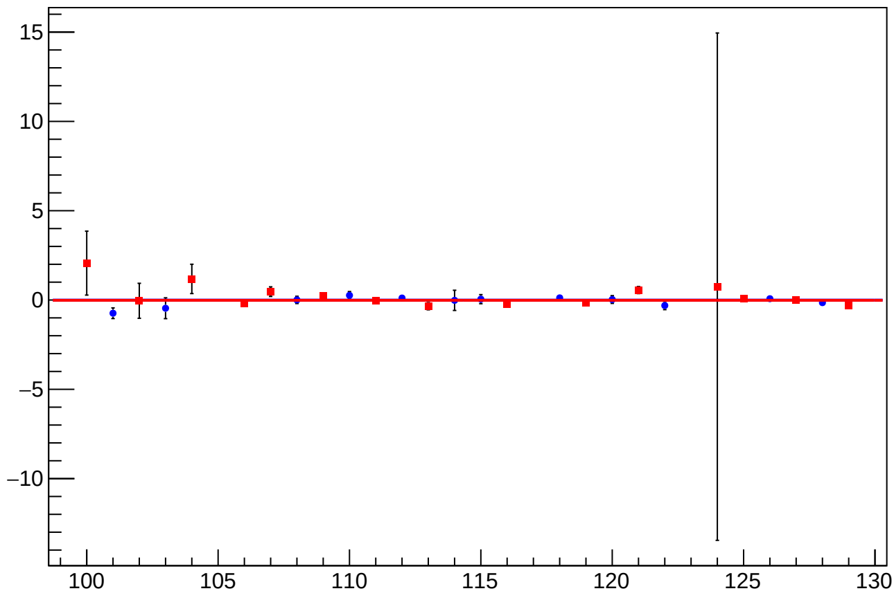
asym_atr1l2_avg_eigen_dit_vs_cor_diff_mean vs Slug, Sign Corrected
