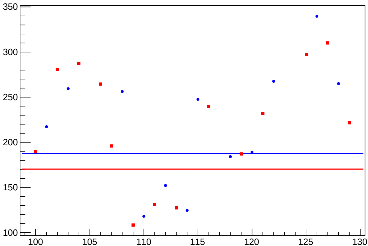
asym_bcm_dg_us_an_ds_avg_rms vs Slug, Sign Corrected
