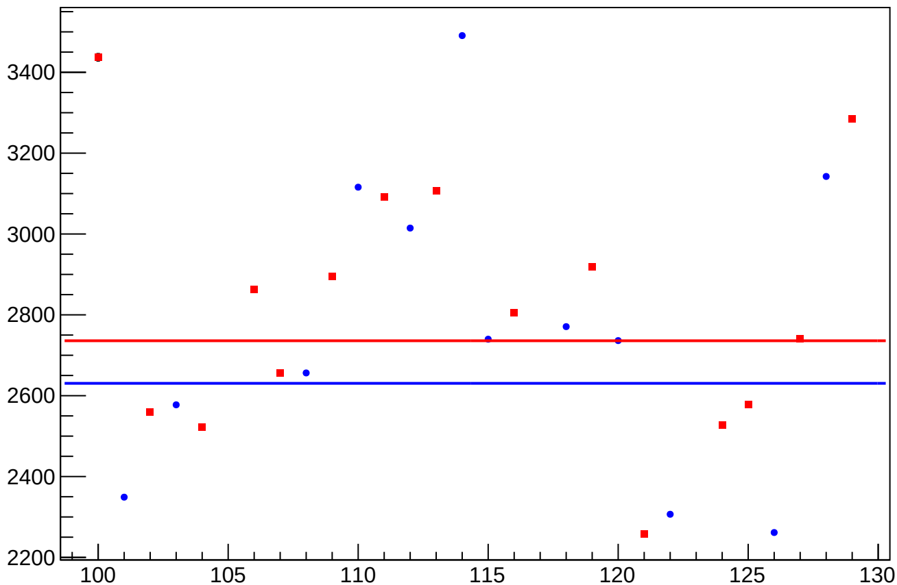
asym_sam_26_dd_eigen_dit_correction_rms vs Slug, Sign Corrected
