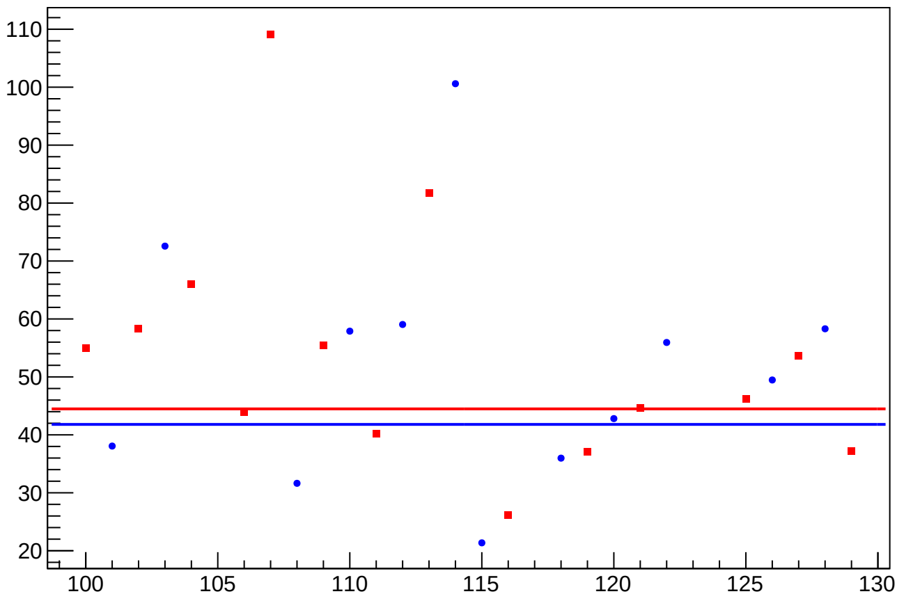
asym_usl_dit_vs_eigen_cor_diff_rms vs Slug, Sign Corrected
