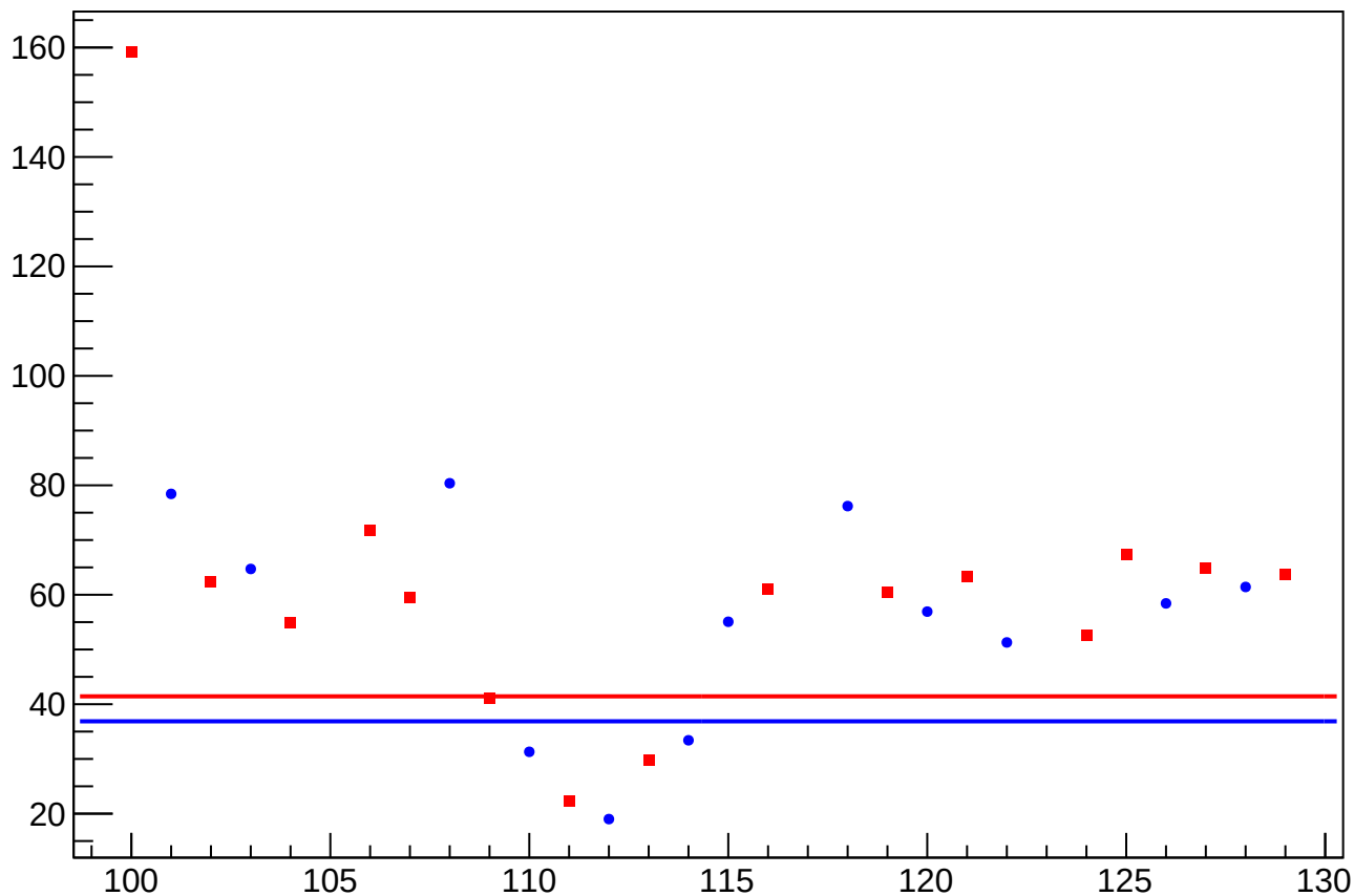
asym_sam_48_avg_eigen_dit_vs_eigen_cor_diff_rms vs Slug, Sign Corrected
