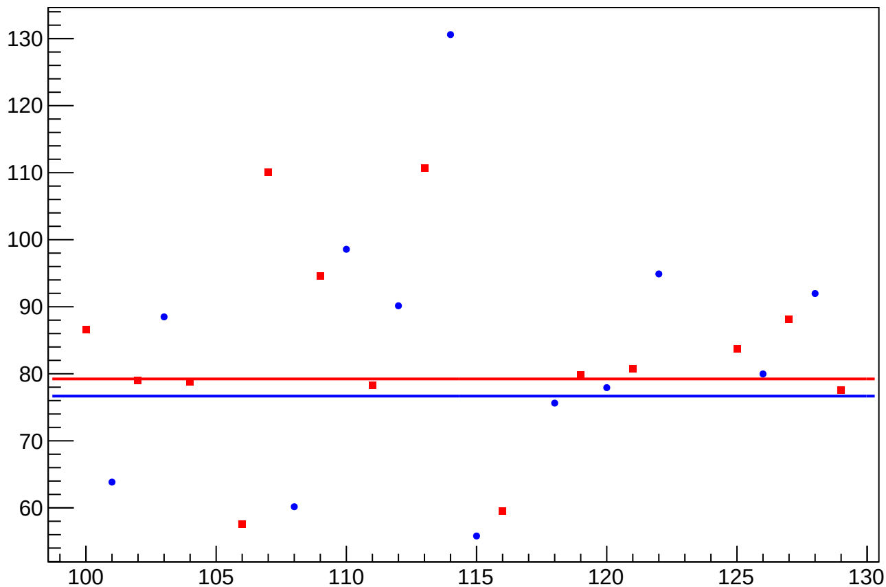
asym_us_avg_dit_vs_overload_cor_diff_rms vs Slug, Sign Corrected
