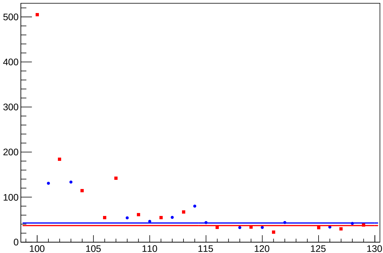
asym_us_dd_at1lr_dd_dd_dit_vs_cor_diff_rms vs Slug, Sign Corrected
