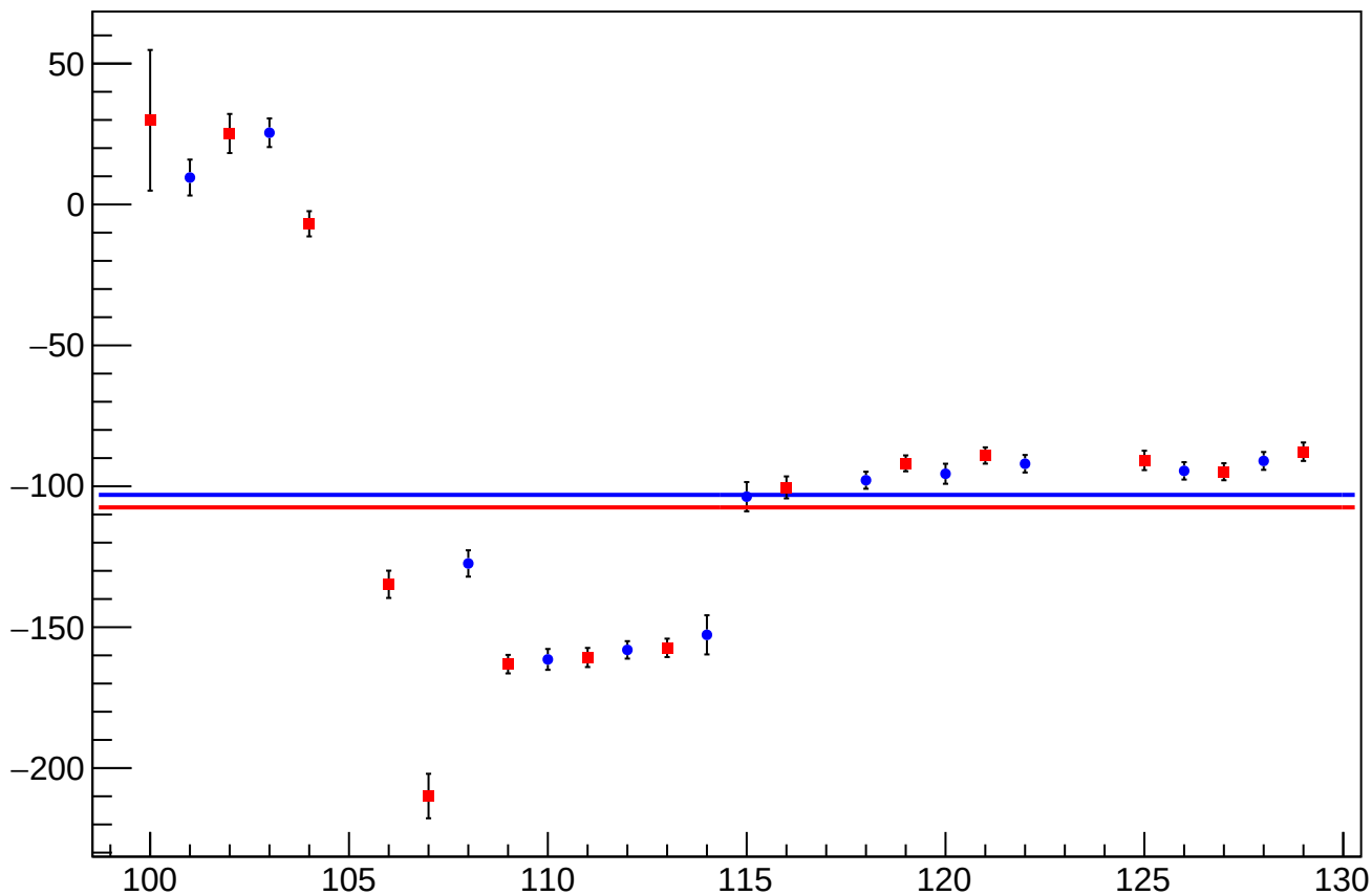
reg_asym_us_dd_at1lr_dd_dd_diff_bpm4eX_slope vs Slug, Sign Corrected
