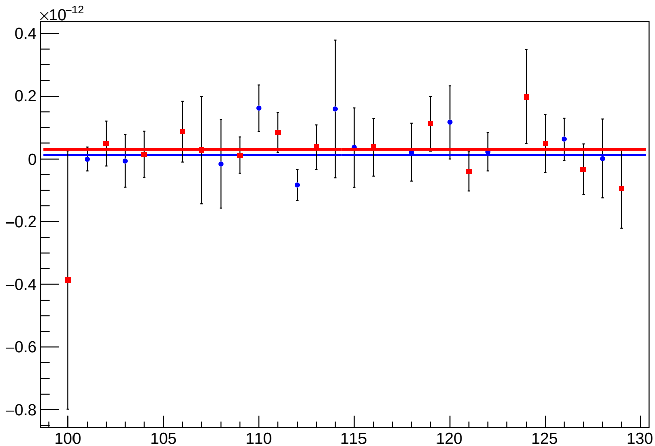
asym_sam_2468_avg_eigen_cor_vs_cor_diff_mean vs Slug, Sign Corrected
