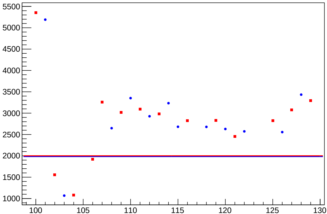
asym_us_avg_atlr_avg_dd_rms vs Slug, Sign Corrected
