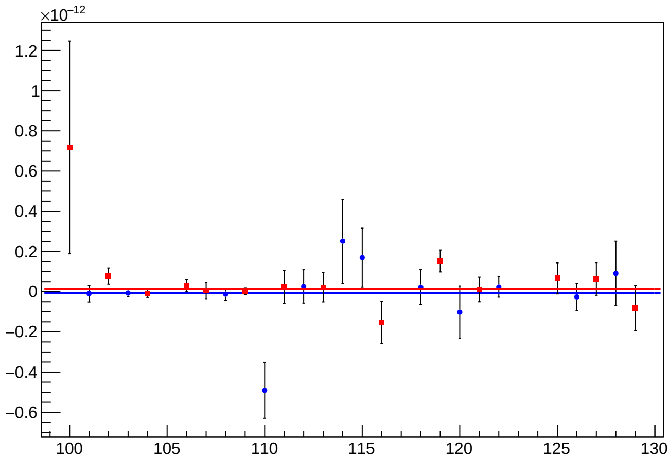
asym_us_dd_at2lr_dd_dd_eigen_cor_vs_cor_diff_mean vs Slug, Sign Corrected
