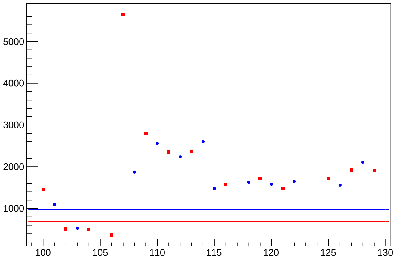
asym_us_avg_at1lr_avg_avg_eigen_dit_correction_rms vs Slug, Sign Corrected
