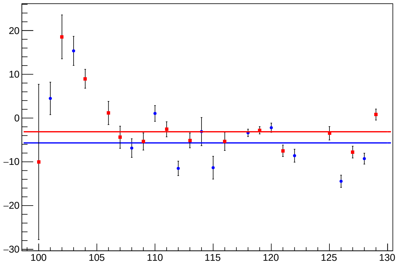
reg_asym_us_dd_atlr_dd_dd_diff_bpm4aY_slope vs Slug, Sign Corrected
