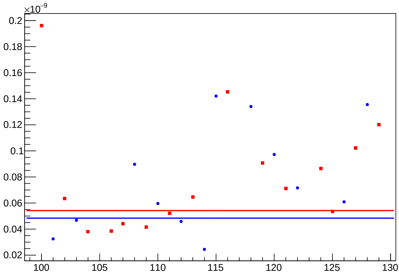
asym_sam_48_avg_reg_vs_cor_diff_rms vs Slug, Sign Corrected
