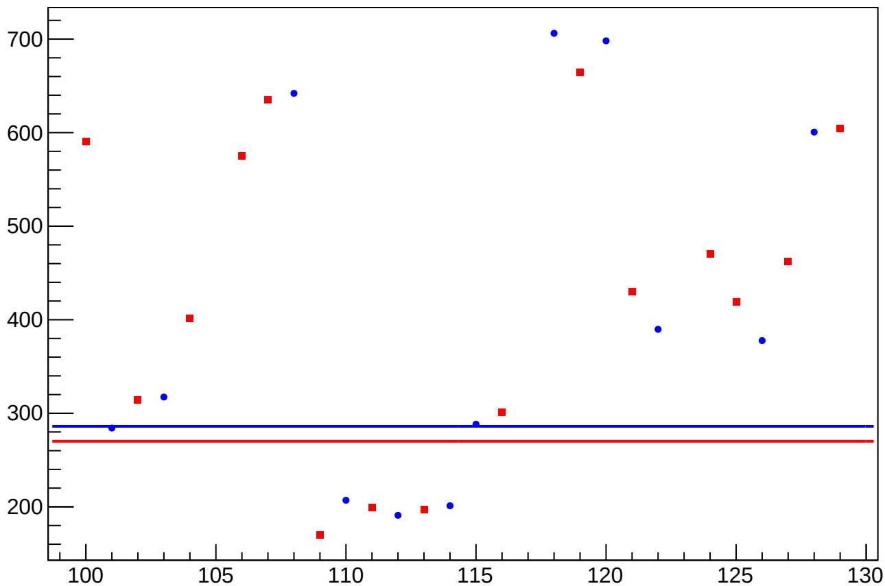
asym_sam7_reg_correction_rms vs Slug, Sign Corrected
