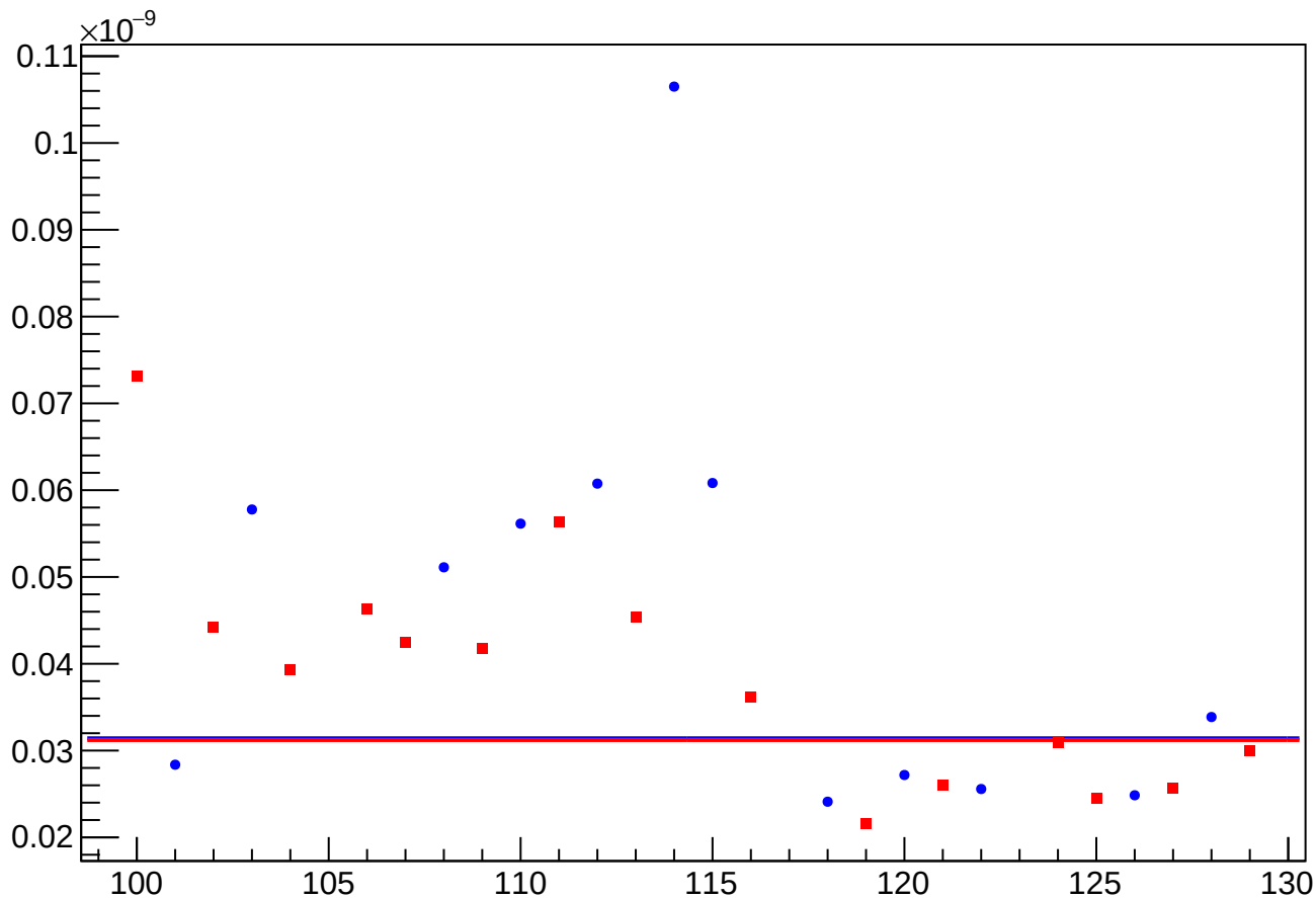
asym_sam_26_48_dd_reg_vs_cor_diff_rms vs Slug, Sign Corrected
