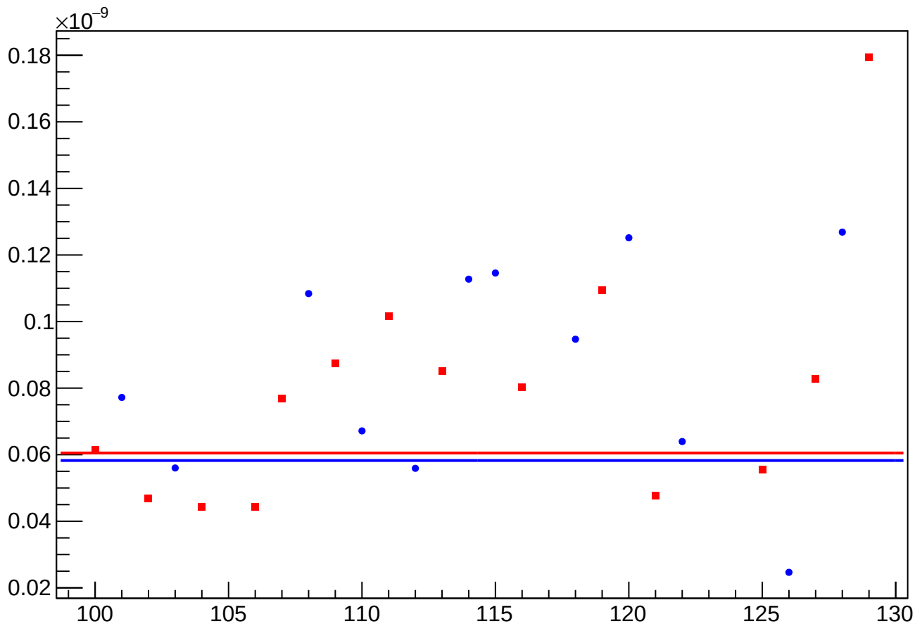
asym_usl_atl2_dd_eigen_cor_vs_cor_diff_rms vs Slug, Sign Corrected
