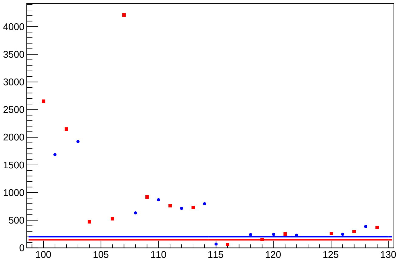
asym_us_dd_at1lr_dd_avg_eigen_cor_correction_rms vs Slug, Sign Corrected
