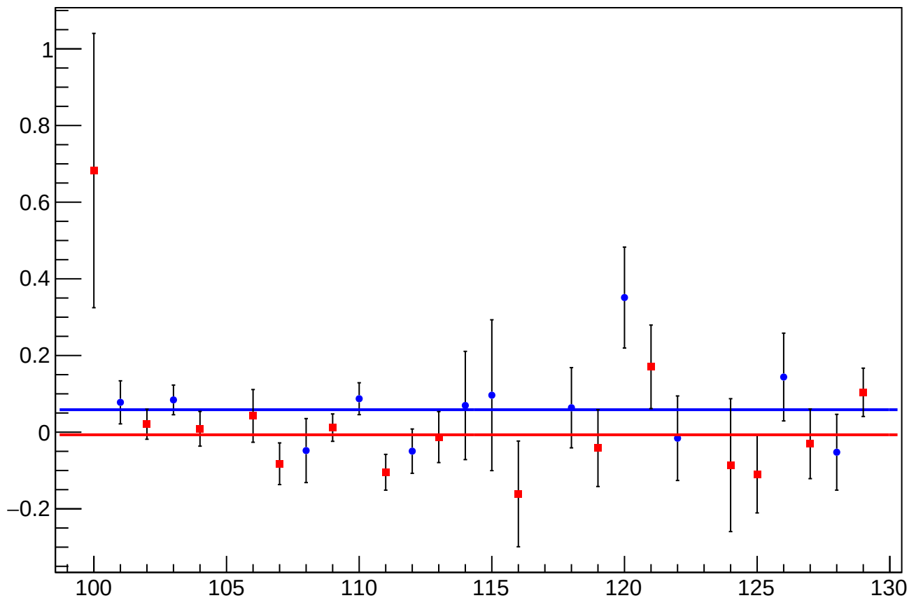
asym_sam6_eigen_dit_vs_cor_diff_mean vs Slug, Sign Corrected
