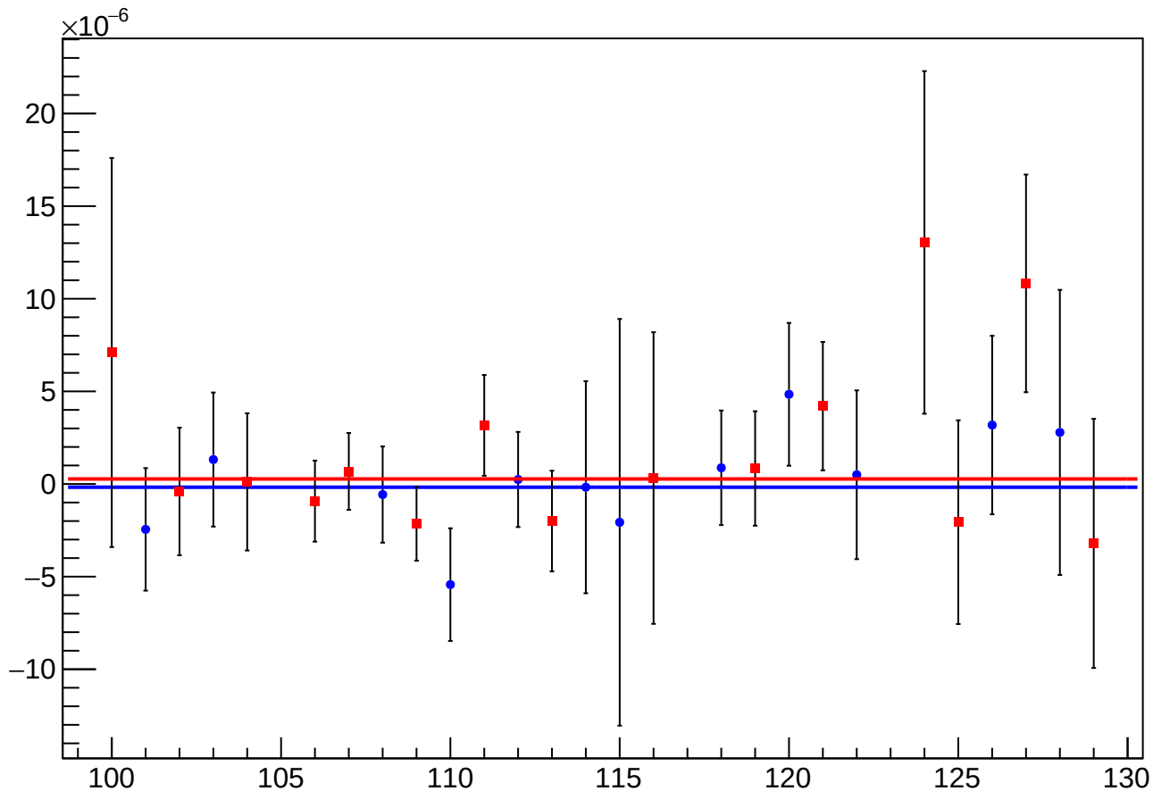
asym_sam_48_dd_eigen_dit_vs_dit_diff_mean vs Slug, Sign Corrected
