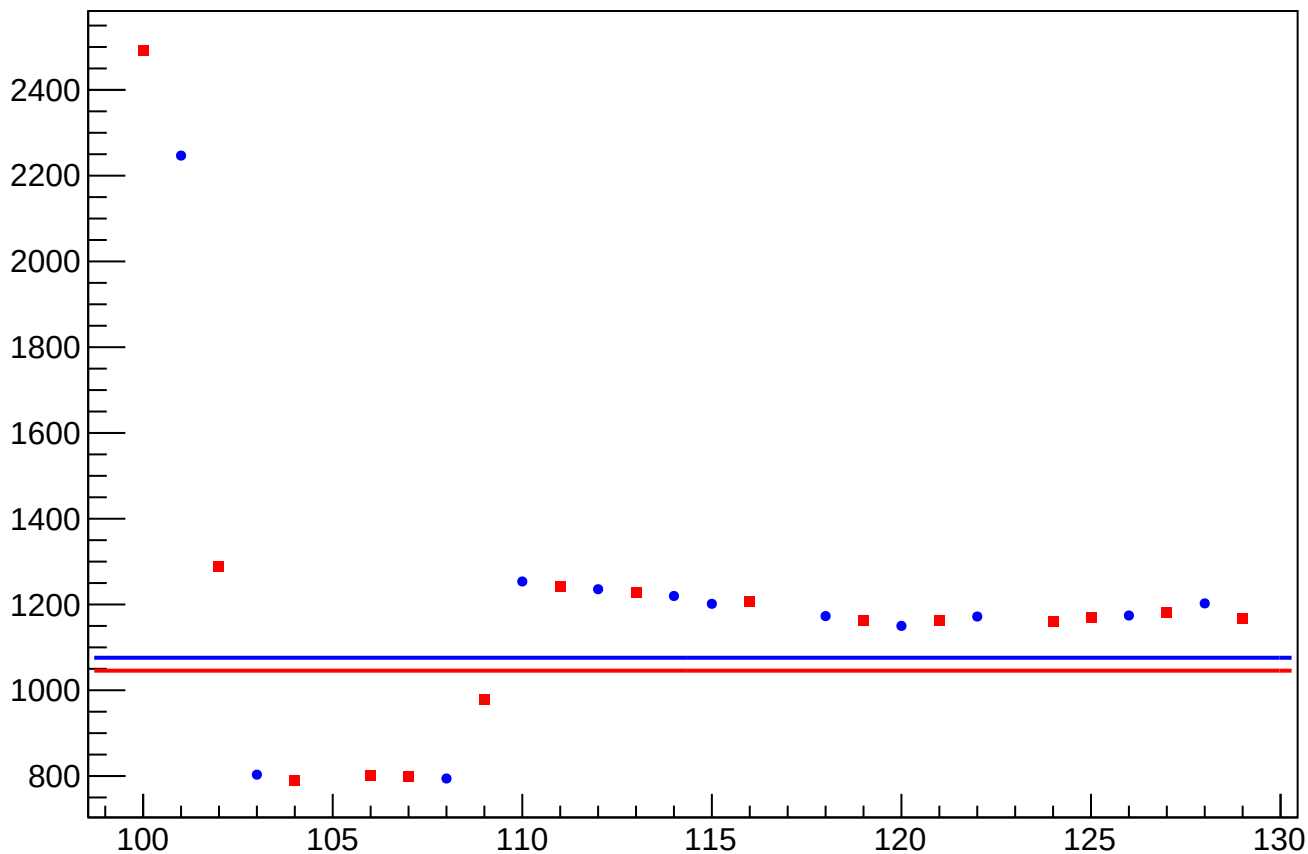
eigen_cor_asym_usr_atr2_dd_rms vs Slug, Sign Corrected
