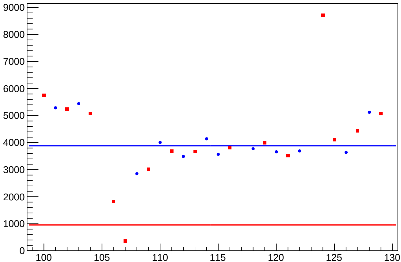
asym_atl1r2_dd_dit_correction_rms vs Slug, Sign Corrected
