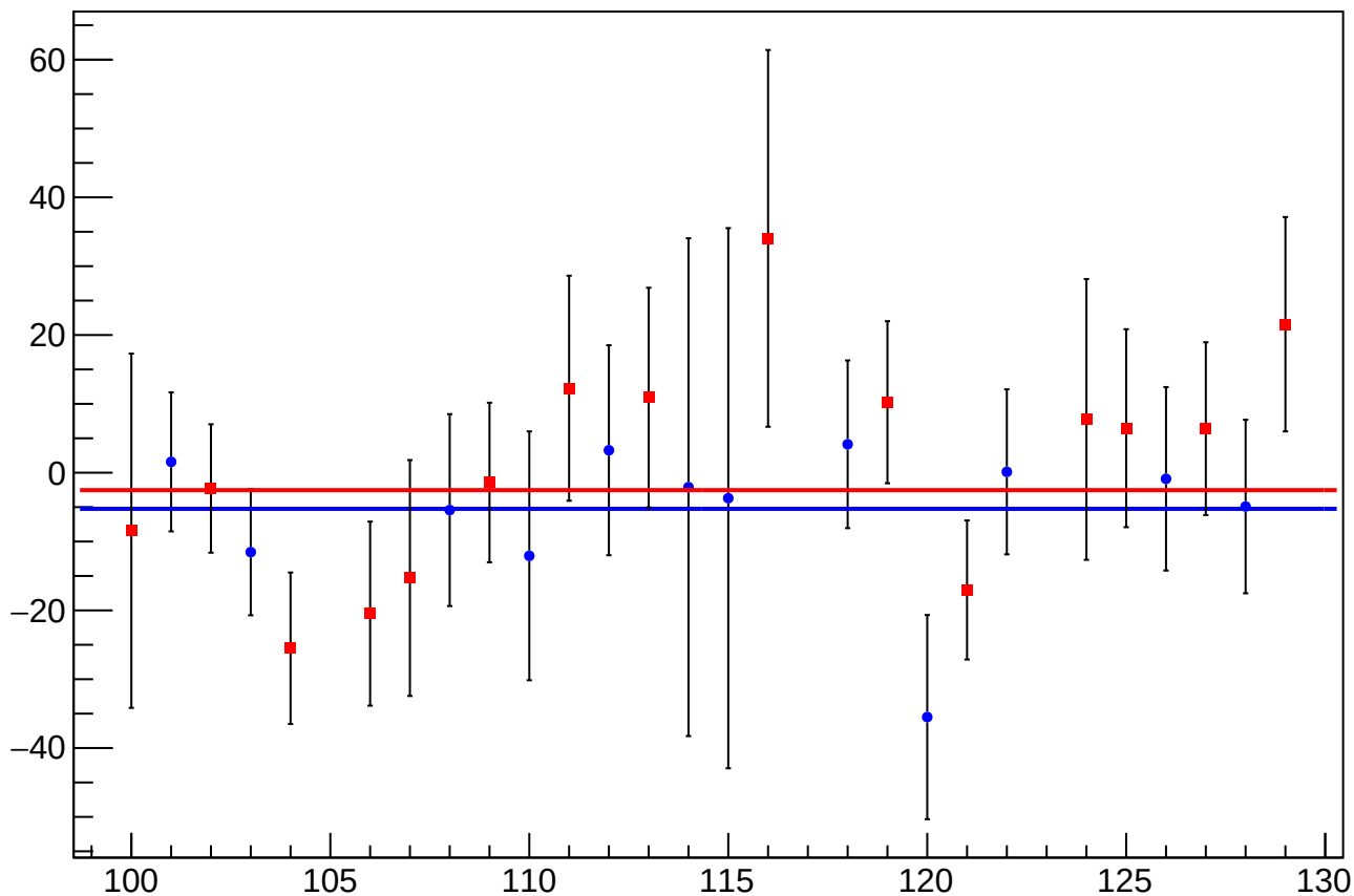
diff_bpm_4aY_4acY_avg_mean vs Slug, Sign Corrected
