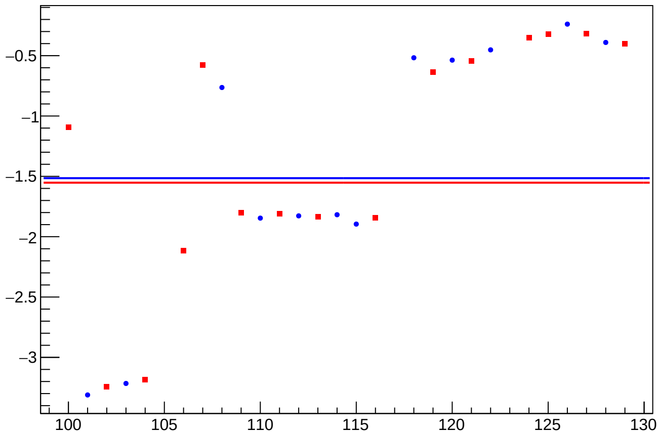
yield_bpm0r03X_mean vs Slug, Sign Corrected
