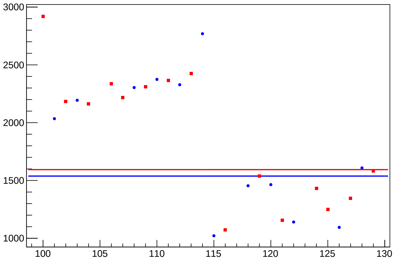
asym_sam_26_avg_cor_correction_rms vs Slug, Sign Corrected
