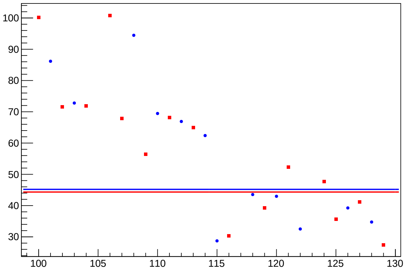
asym_sam_3726_avg_dit_vs_cor_diff_rms vs Slug, Sign Corrected
