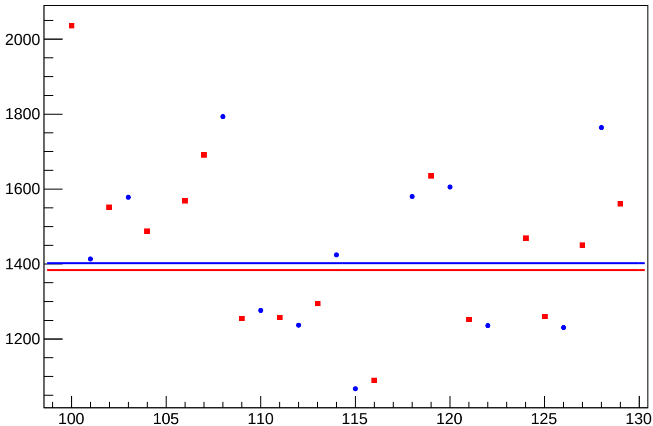
asym_sam_2468_avg_eigen_cor_correction_rms vs Slug, Sign Corrected
