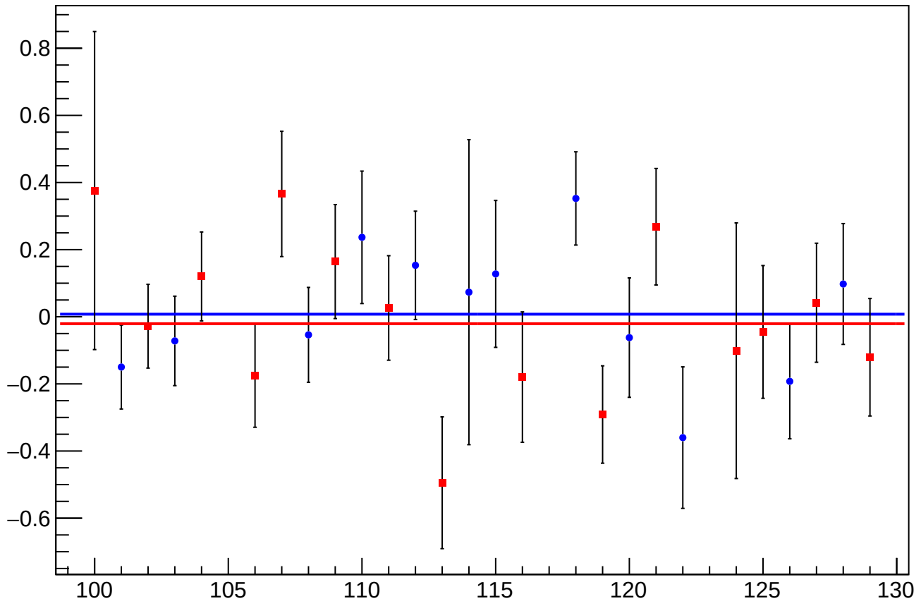
asym_usr_eigen_dit_vs_overload_cor_diff_mean vs Slug, Sign Corrected
