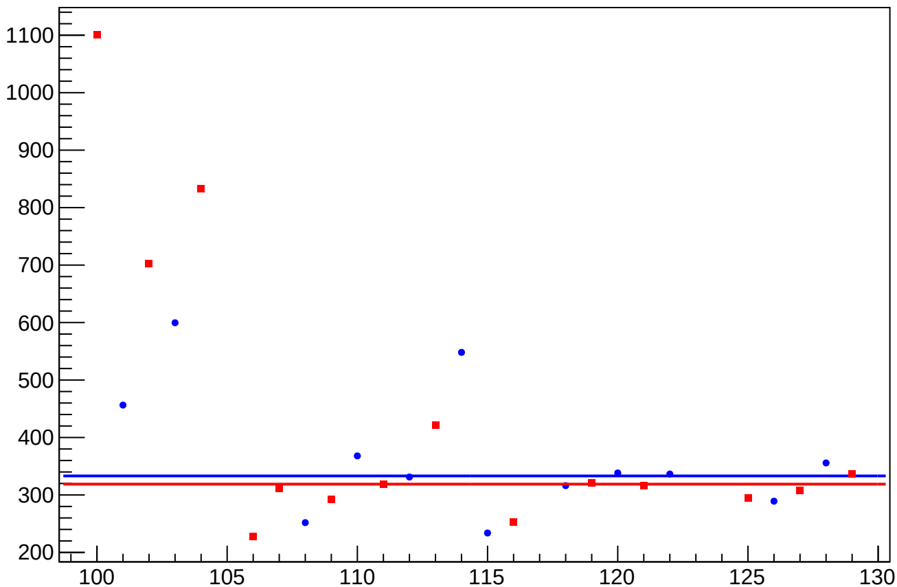
asym_us_avg_at2lr_avg_avg_eigen_dit_vs_cor_diff_rms vs Slug, Sign Corrected
