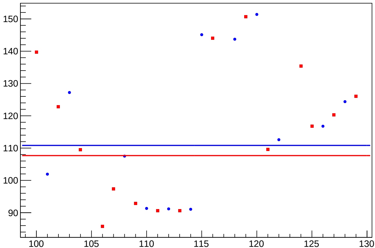
eigen_cor_asym_sam_48_dd_rms vs Slug, Sign Corrected
