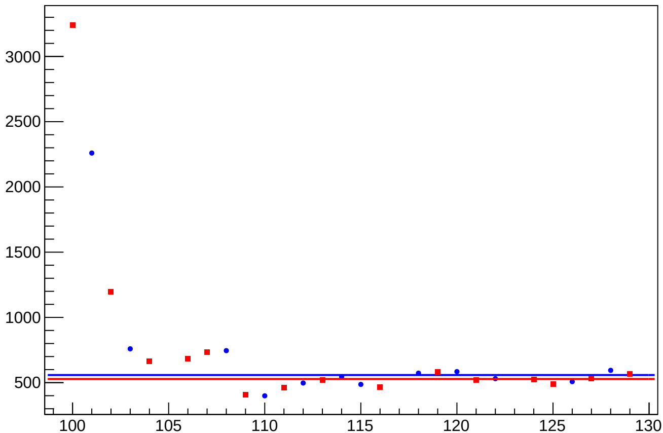
asym_atr1_cor_correction_rms vs Slug, Sign Corrected
