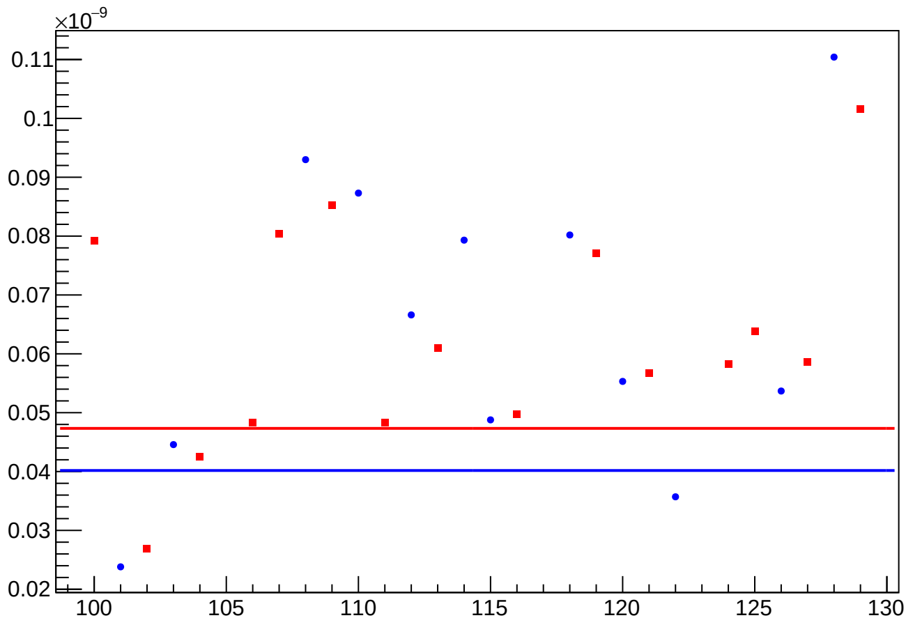
asym_usr_eigen_cor_vs_cor_diff_rms vs Slug, Sign Corrected
