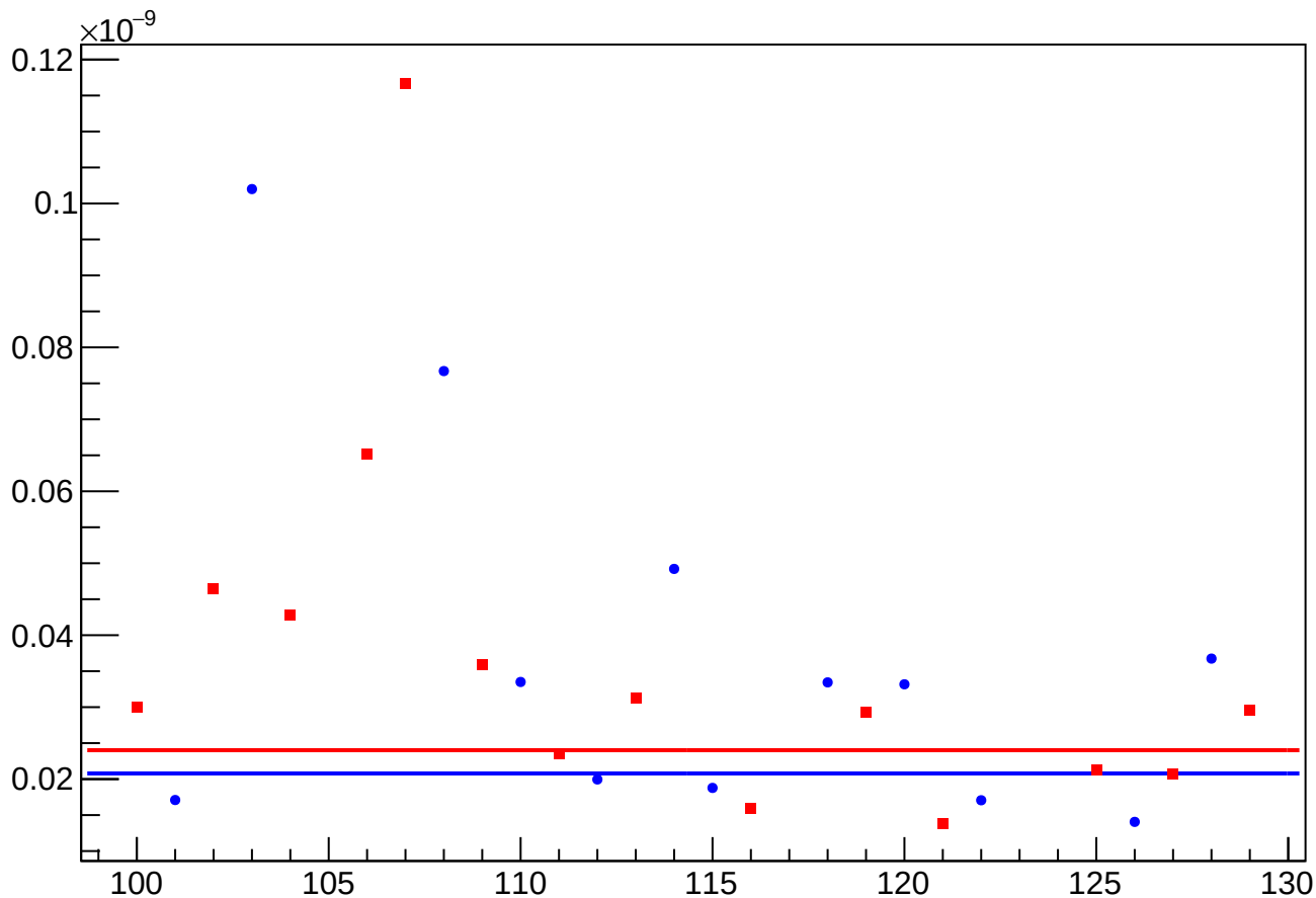
asym_usl_atl1_dd_reg_vs_cor_diff_rms vs Slug, Sign Corrected
