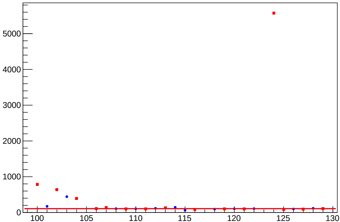
asym_atr1l2_dd_eigen_dit_vs_eigen_cor_diff_rms vs Slug, Sign Corrected
