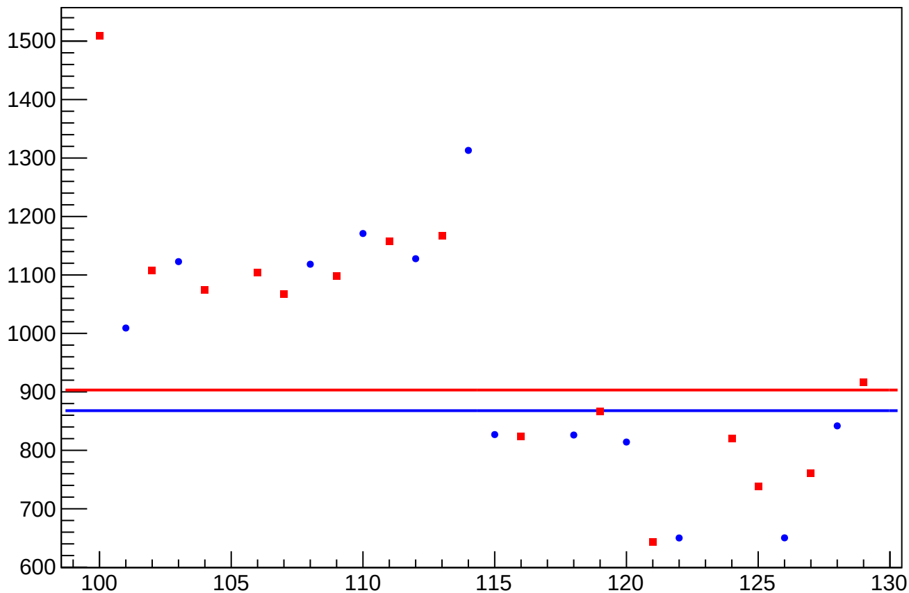
asym_sam_15_26_dd_dit_correction_rms vs Slug, Sign Corrected
