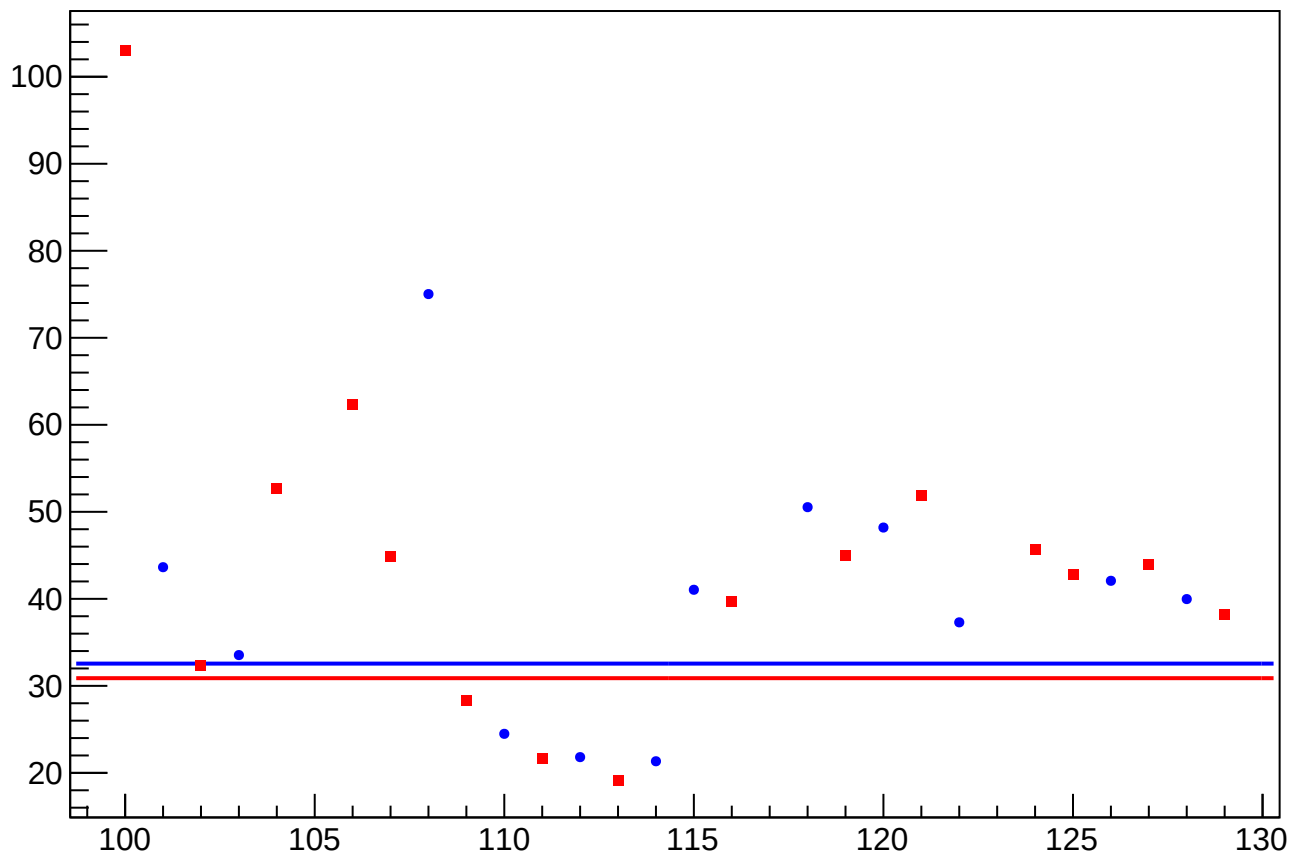
asym_sam_3748_avg_eigen_dit_vs_eigen_cor_diff_rms vs Slug, Sign Corrected
