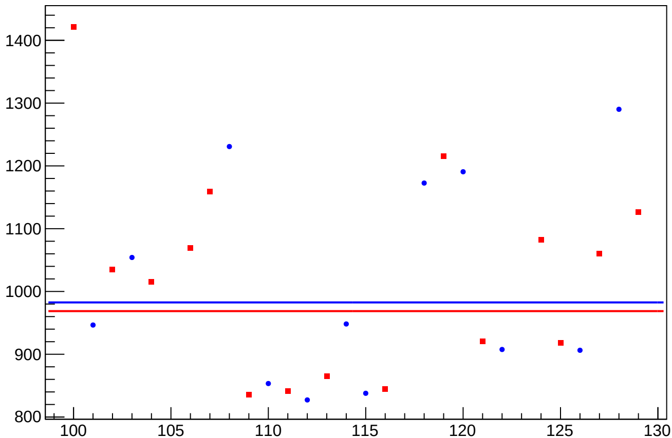
asym_sam_12345678_avg_eigen_cor_correction_rms vs Slug, Sign Corrected
