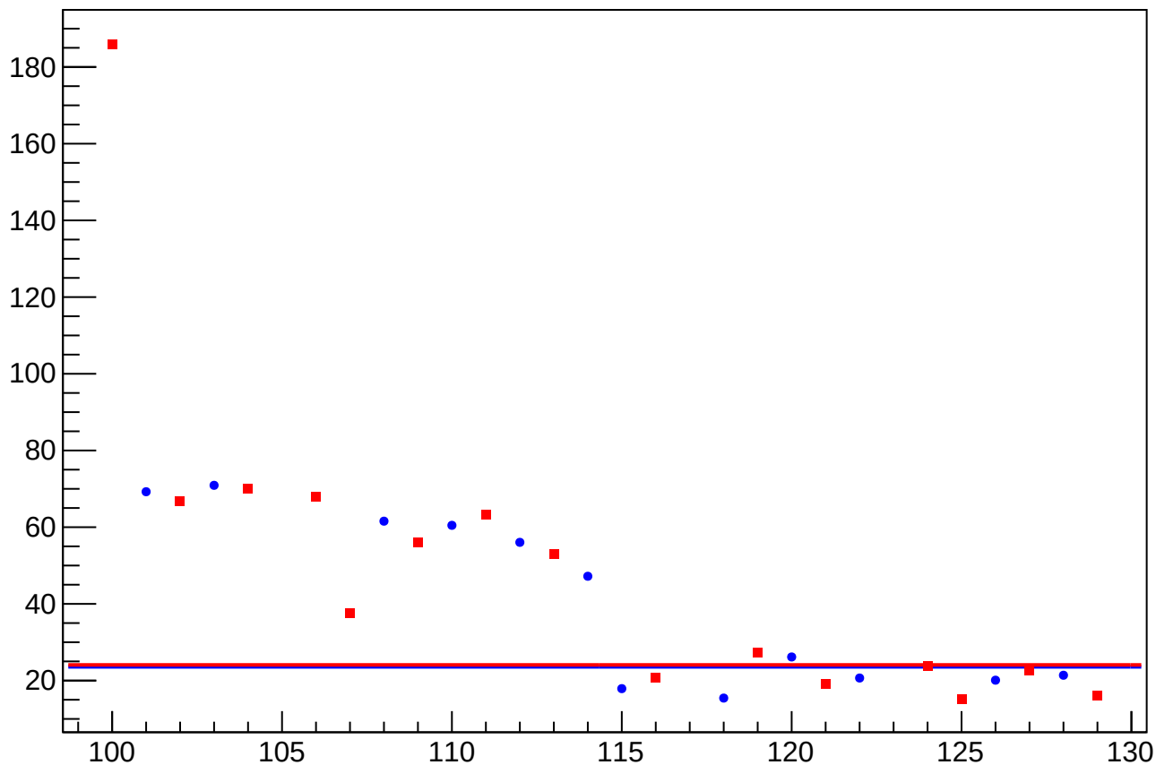
asym_sam_37_26_dd_dit_vs_cor_diff_rms vs Slug, Sign Corrected
