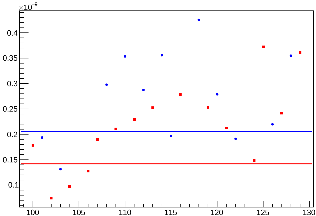
asym_at2_avg_eigen_cor_vs_cor_diff_rms vs Slug, Sign Corrected
