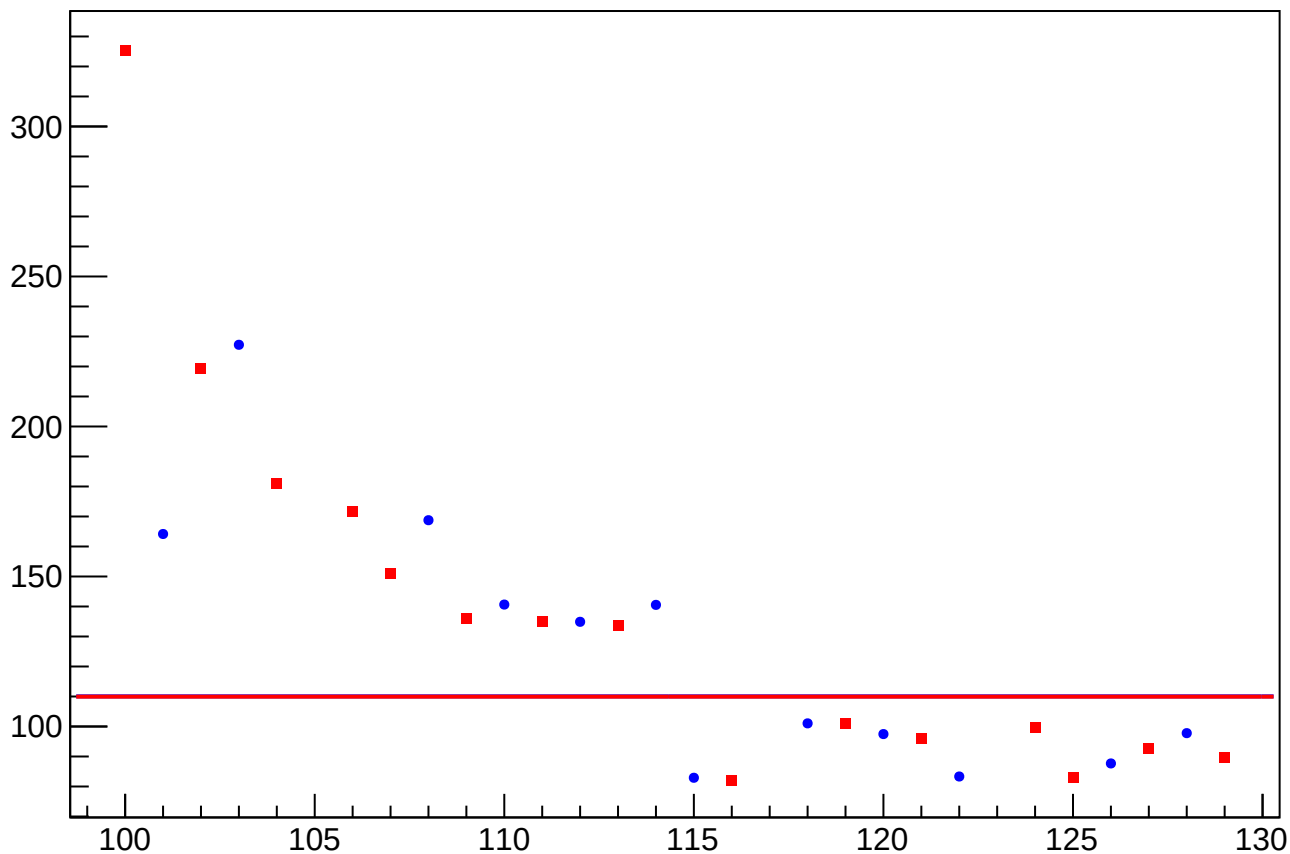
eigen_dit_asym_sam_3726_avg_rms vs Slug, Sign Corrected
