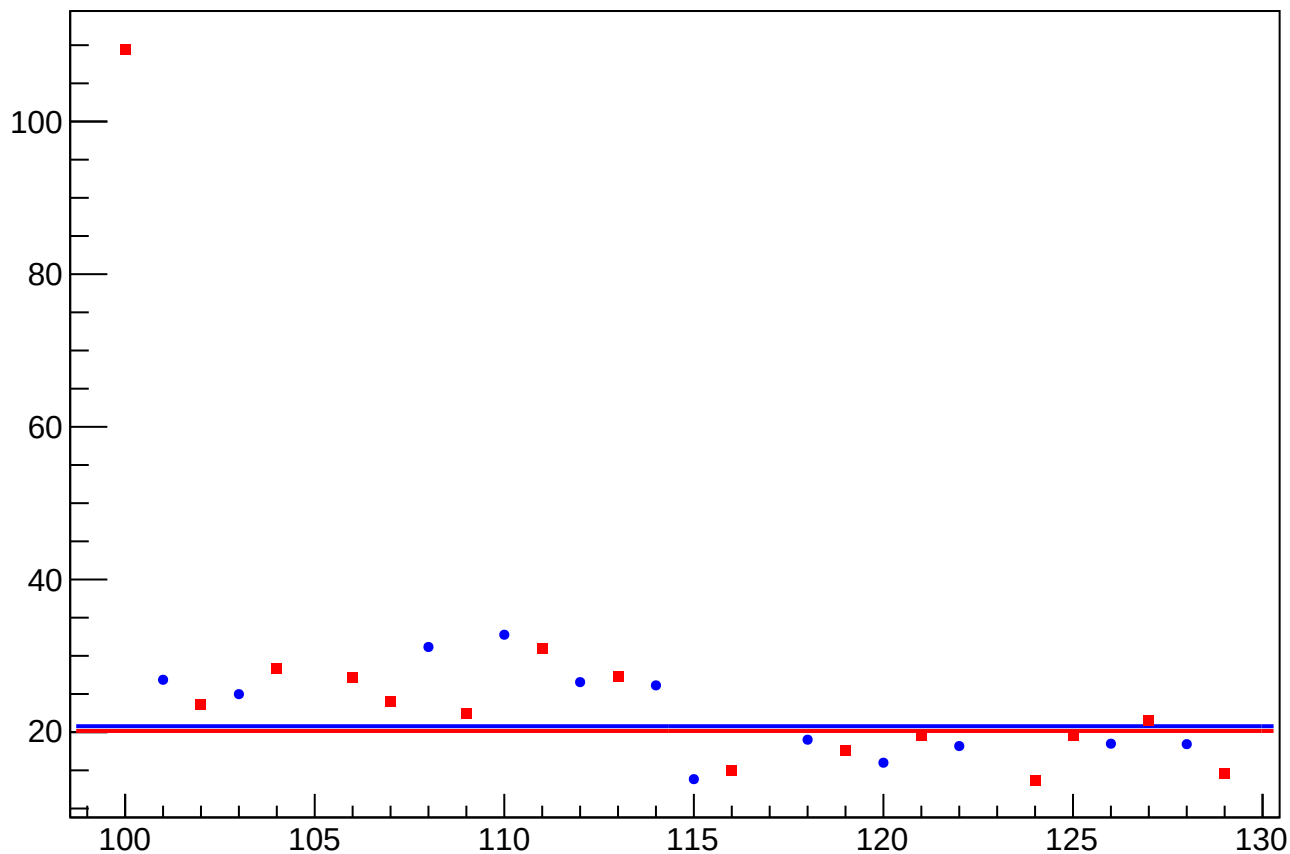
asym_sam_1357_2468_dd_eigen_dit_vs_eigen_cor_diff_rms vs Slug, Sign Corrected
