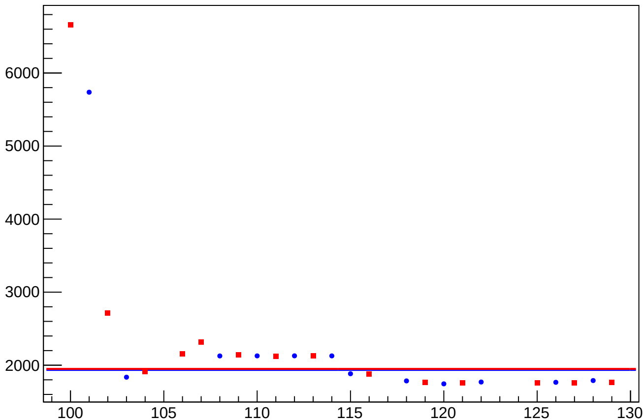
dit_asym_us_dd_at1lr_dd_dd_rms vs Slug, Sign Corrected
