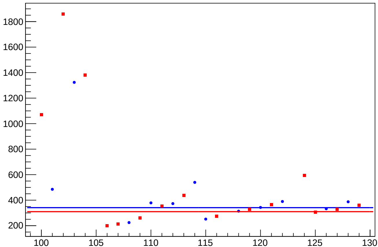
asym_atr2_eigen_dit_vs_cor_diff_rms vs Slug, Sign Corrected
