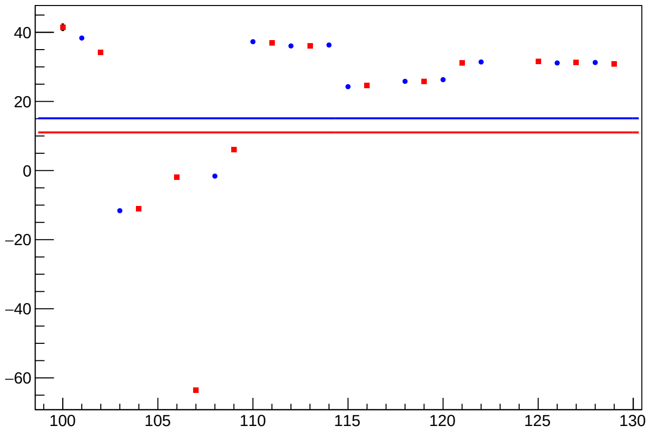
reg_asym_us_dd_at2lr_dd_avg_diff_bpm12X_slope vs Slug, Sign Corrected
