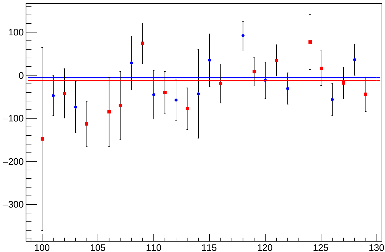
eigen_cor_asym_sam_1357_2468_dd_mean vs Slug, Sign Corrected
