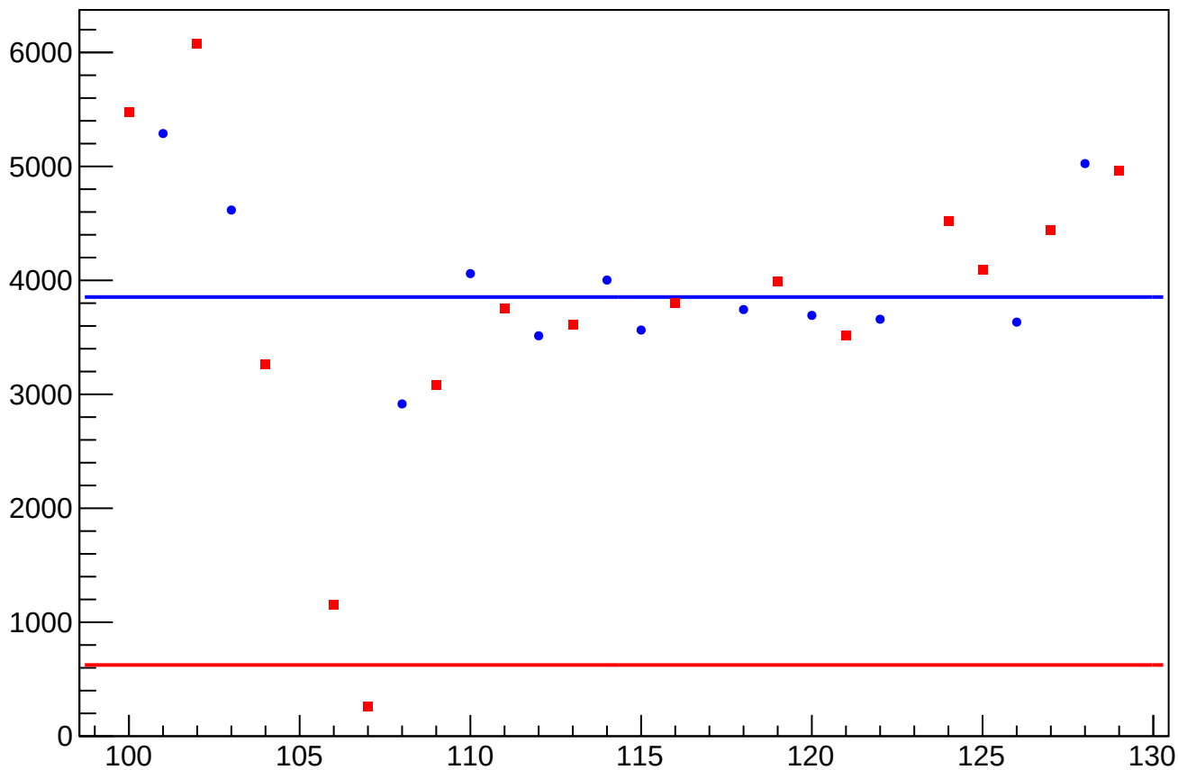
asym_atl1r2_dd_reg_correction_rms vs Slug, Sign Corrected
