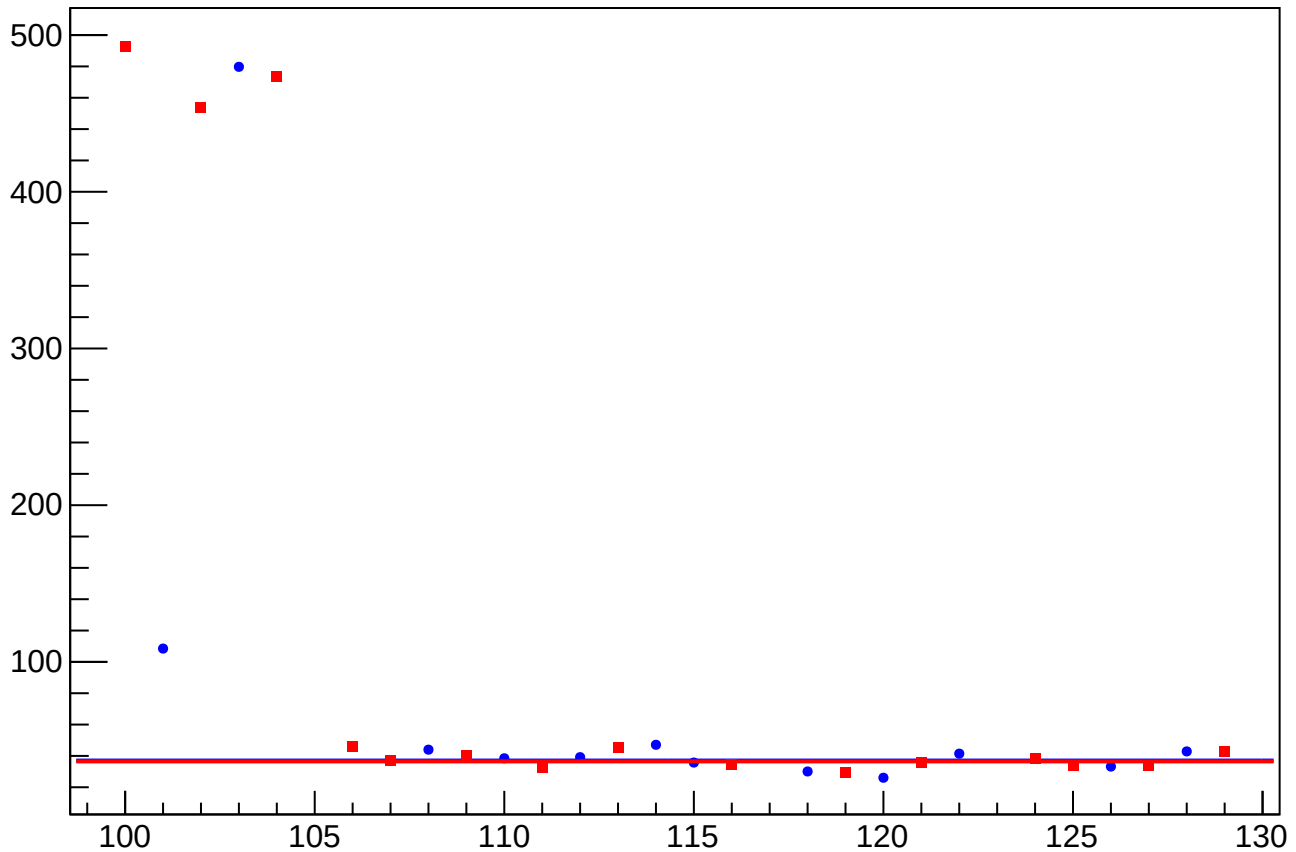
asym_usr_atr1_dd_eigen_dit_vs_eigen_cor_diff_rms vs Slug, Sign Corrected
