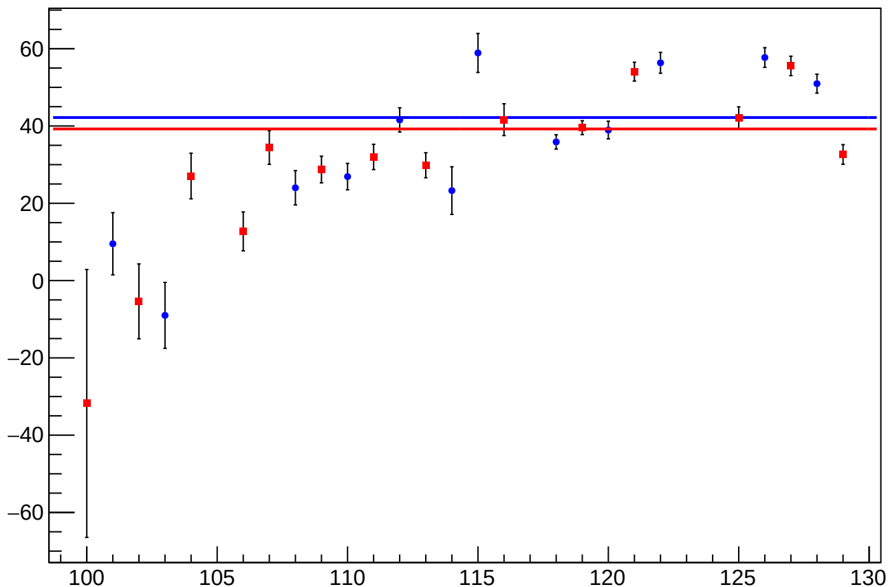
reg_asym_us_avg_at1lr_avg_dd_diff_bpm4eY_slope vs Slug, Sign Corrected
