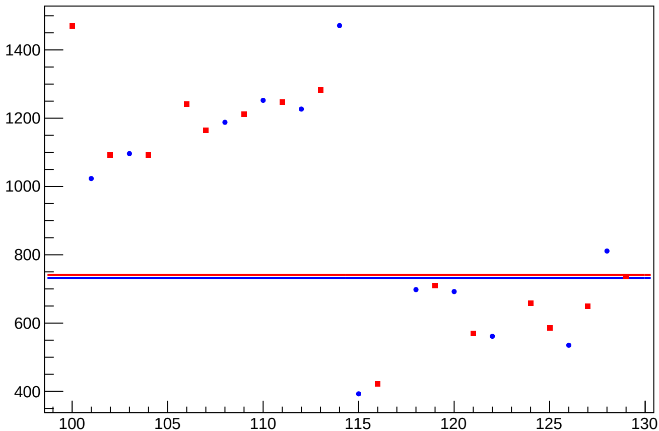
asym_sam_1526_avg_cor_correction_rms vs Slug, Sign Corrected
