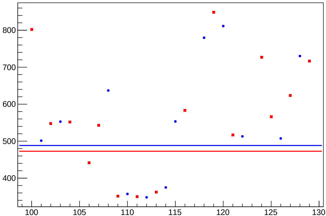
asym_sam_15_37_dd_cor_correction_rms vs Slug, Sign Corrected
