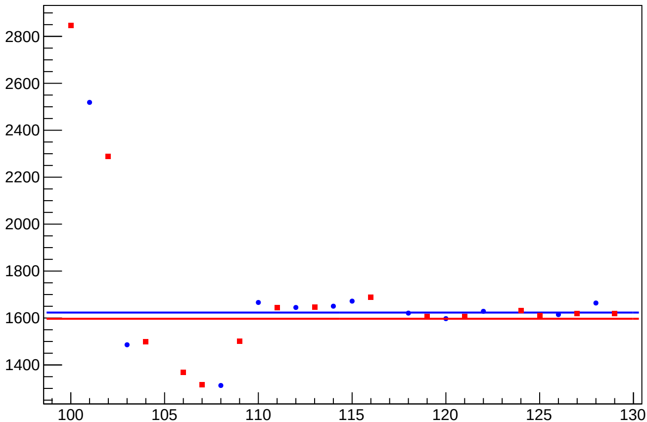
eigen_dit_asym_usr_atr2_avg_rms vs Slug, Sign Corrected
