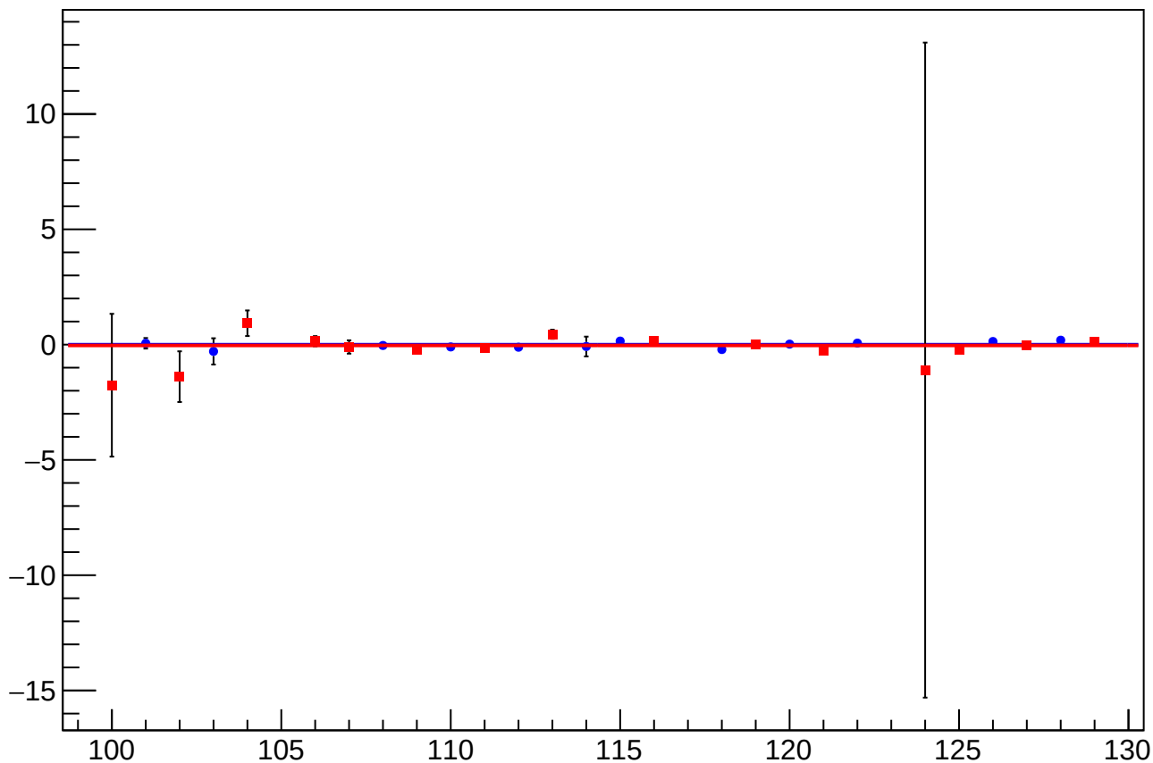
asym_atr1l2_dd_eigen_dit_vs_cor_diff_mean vs Slug, Sign Corrected
