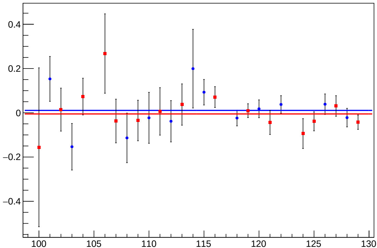
asym_sam_1526_avg_eigen_dit_vs_cor_diff_mean vs Slug, Sign Corrected
