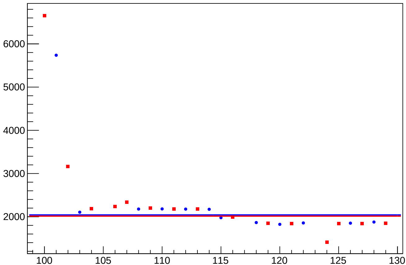
eigen_dit_asym_at1_avg_rms vs Slug, Sign Corrected
