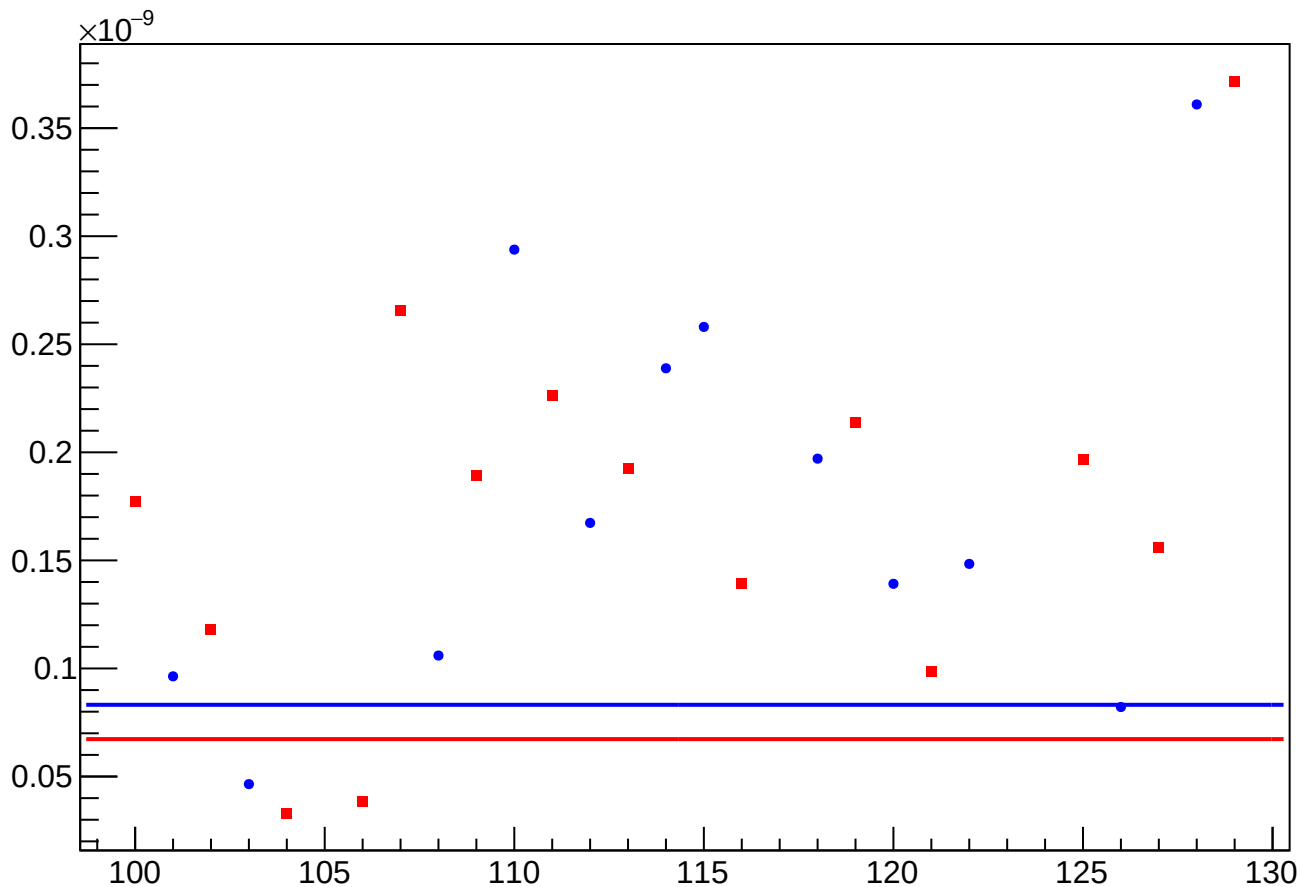
asym_us_avg_atlr_avg_avg_eigen_cor_vs_cor_diff_rms vs Slug, Sign Corrected
