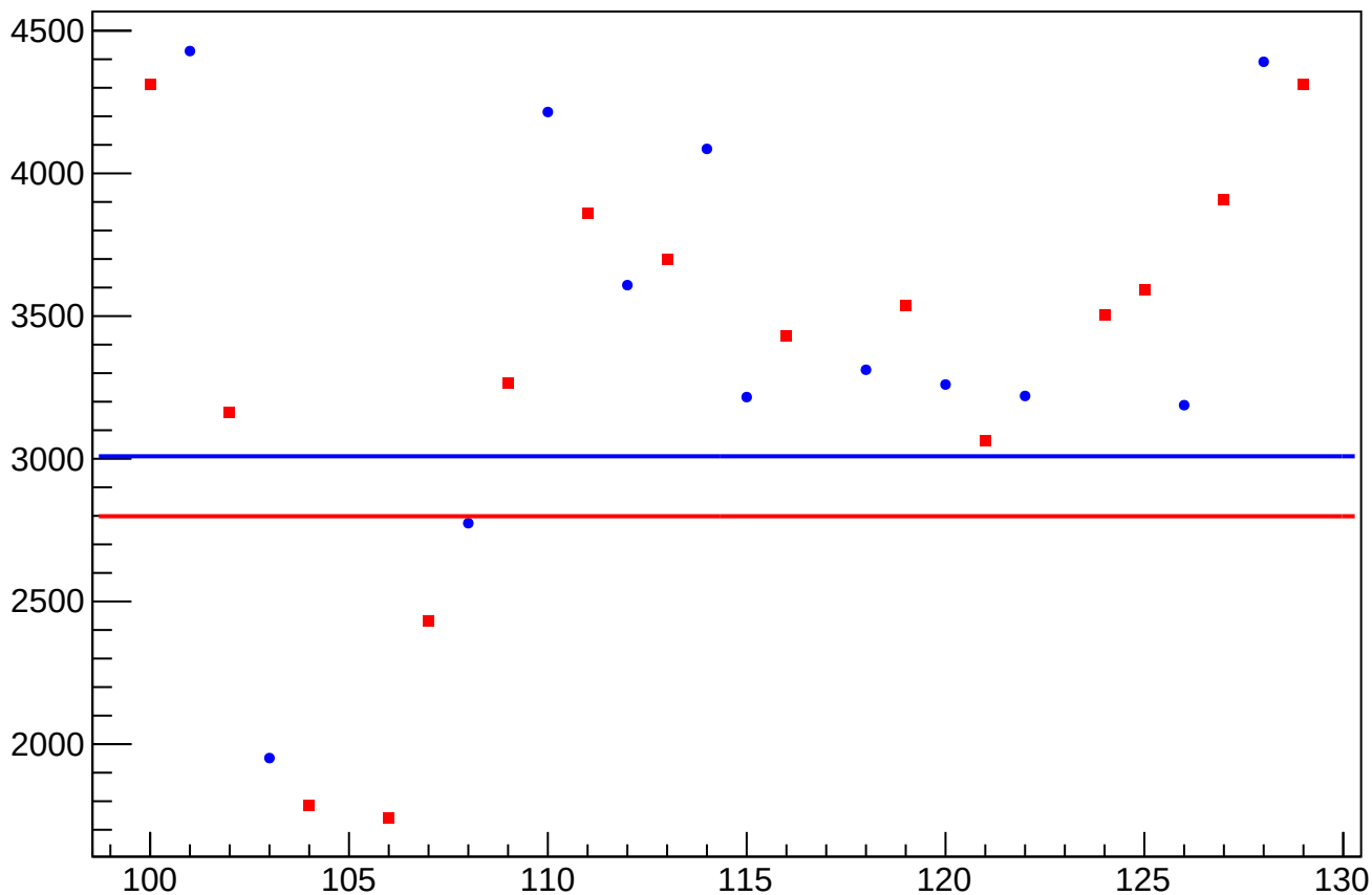
asym_usr_atr2_dd_cor_correction_rms vs Slug, Sign Corrected
