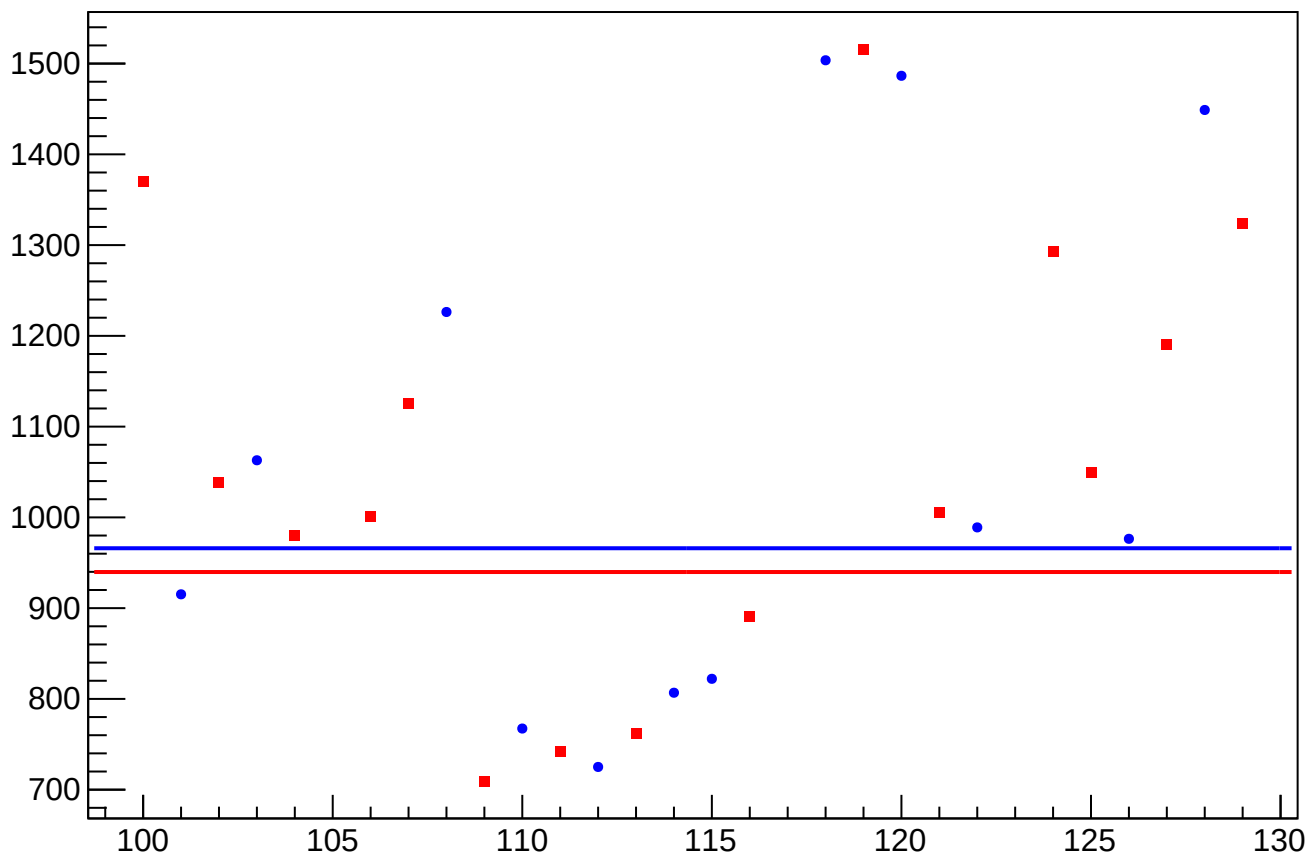
asym_sam_37_avg_dit_correction_rms vs Slug, Sign Corrected
