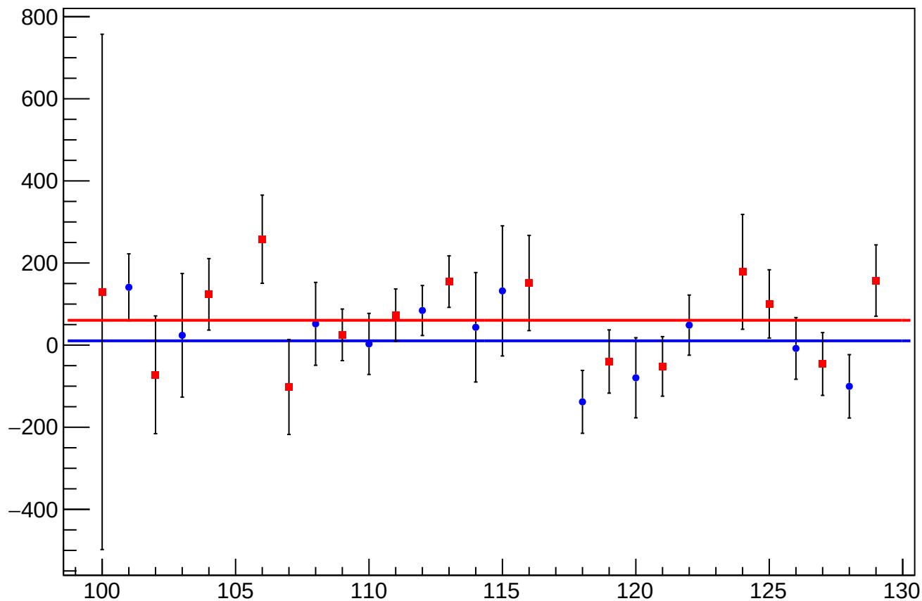
eigen_cor_asym_sam_1357_avg_mean vs Slug, Sign Corrected
