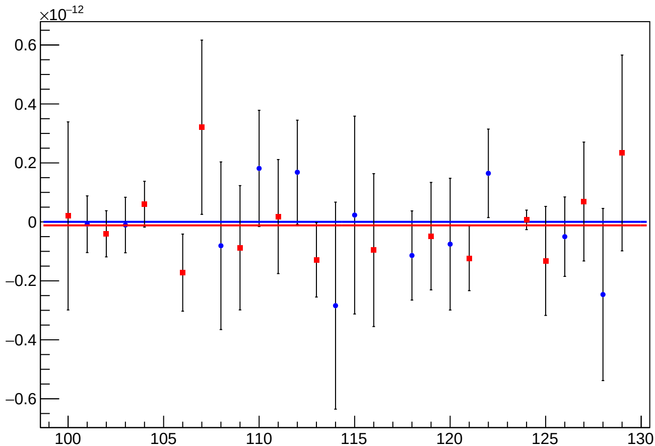
asym_atr1l2_dd_eigen_cor_vs_cor_diff_mean vs Slug, Sign Corrected
