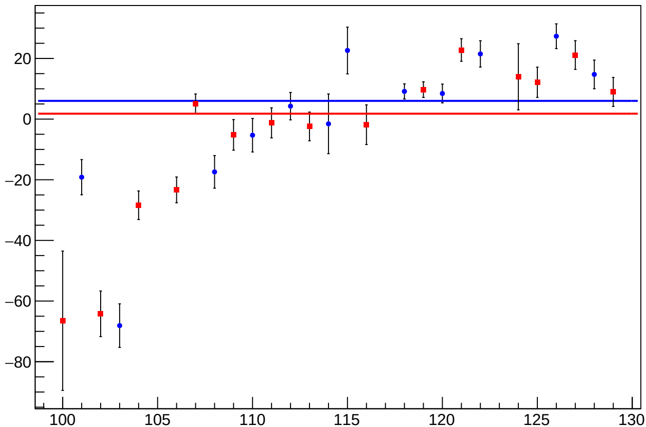
reg_asym_atl1r2_dd_atl2r1_dd_dd_diff_bpm4aY_slope vs Slug, Sign Corrected
