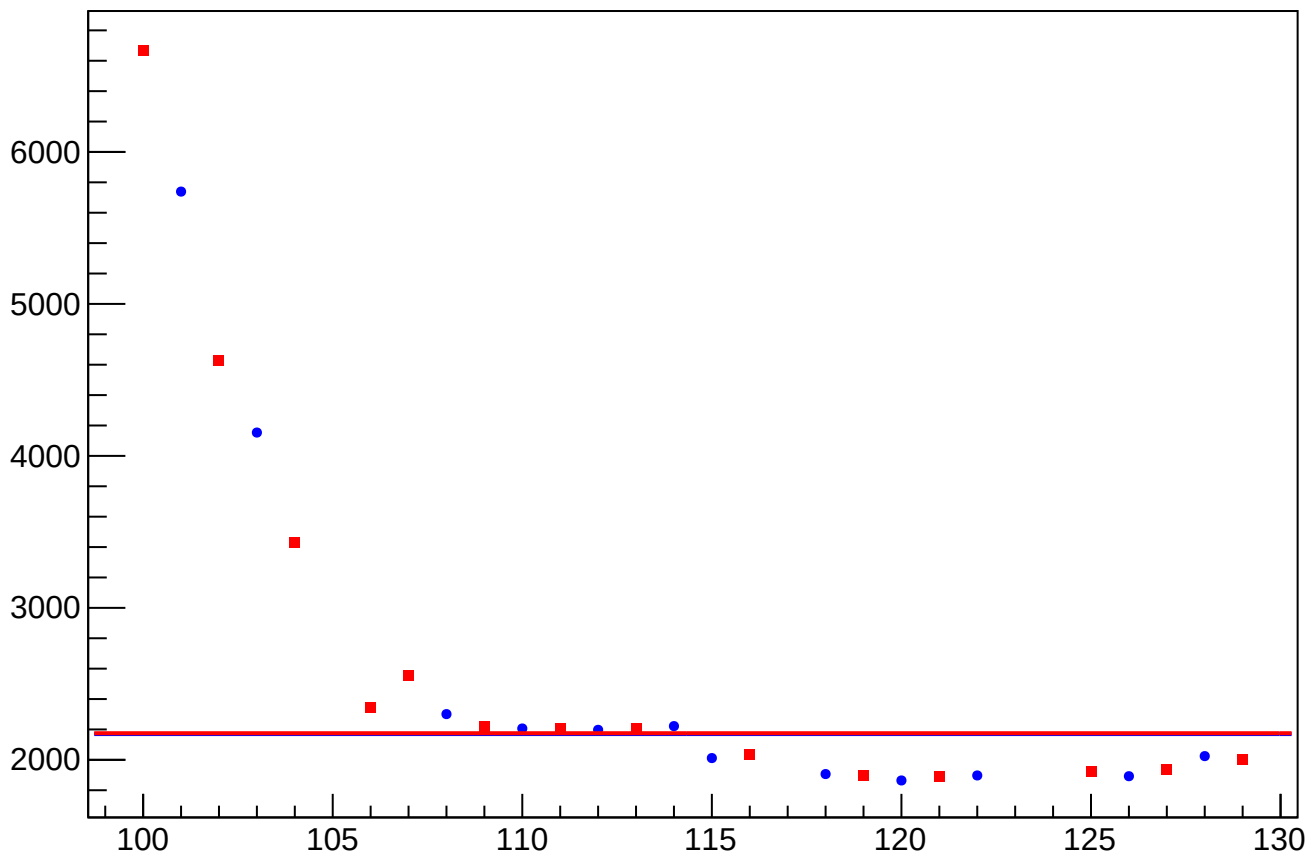
asym_us_avg_at1lr_avg_dd_rms vs Slug, Sign Corrected
