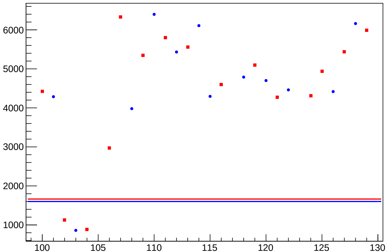
asym_atl1r2_avg_cor_correction_rms vs Slug, Sign Corrected
