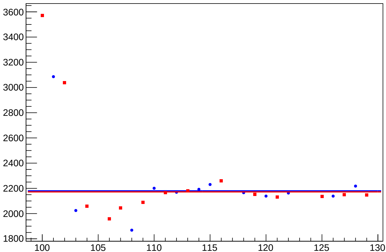
eigen_dit_asym_us_avg_at2lr_avg_avg_rms vs Slug, Sign Corrected
