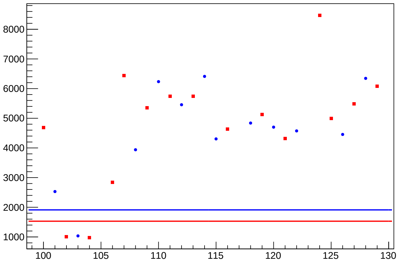
asym_atl1r2_avg_dit_correction_rms vs Slug, Sign Corrected
