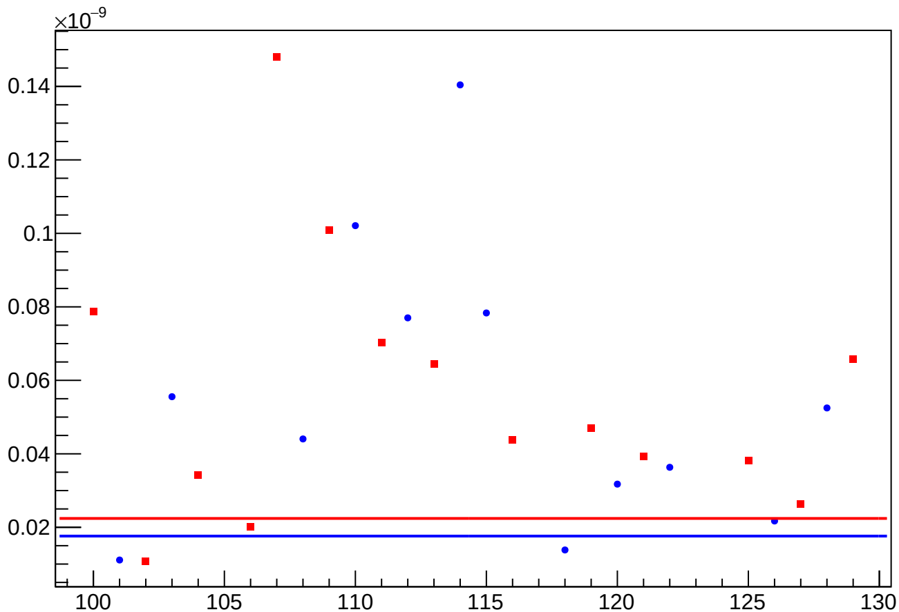
asym_usl_atl1_avg_reg_vs_cor_diff_rms vs Slug, Sign Corrected
