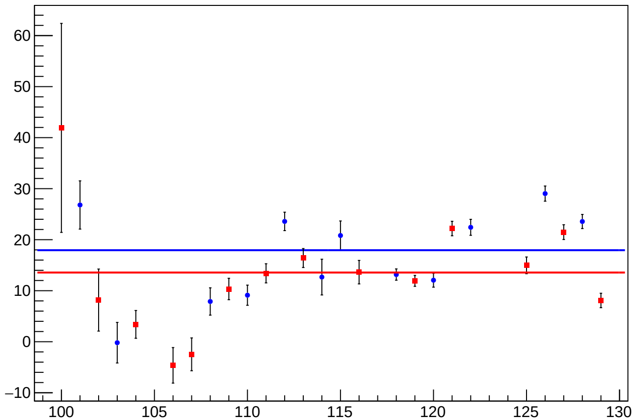
reg_asym_us_dd_atlr_dd_dd_diff_bpm4eY_slope vs Slug, Sign Corrected
