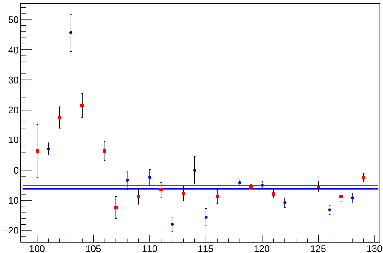
reg_asym_usl_atl1_dd_diff_bpm4aY_slope vs Slug, Sign Corrected
