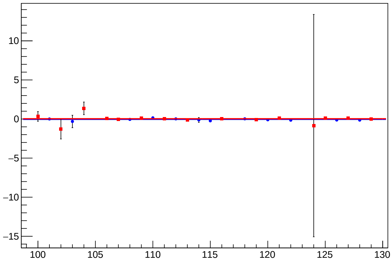
asym_at2_dd_eigen_dit_vs_cor_diff_mean vs Slug, Sign Corrected
