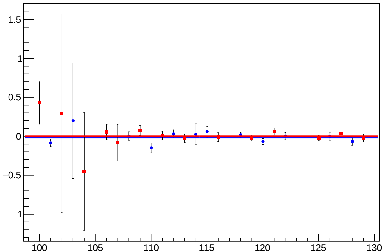
asym_usl_atl1_dd_dit_vs_cor_diff_mean vs Slug, Sign Corrected
