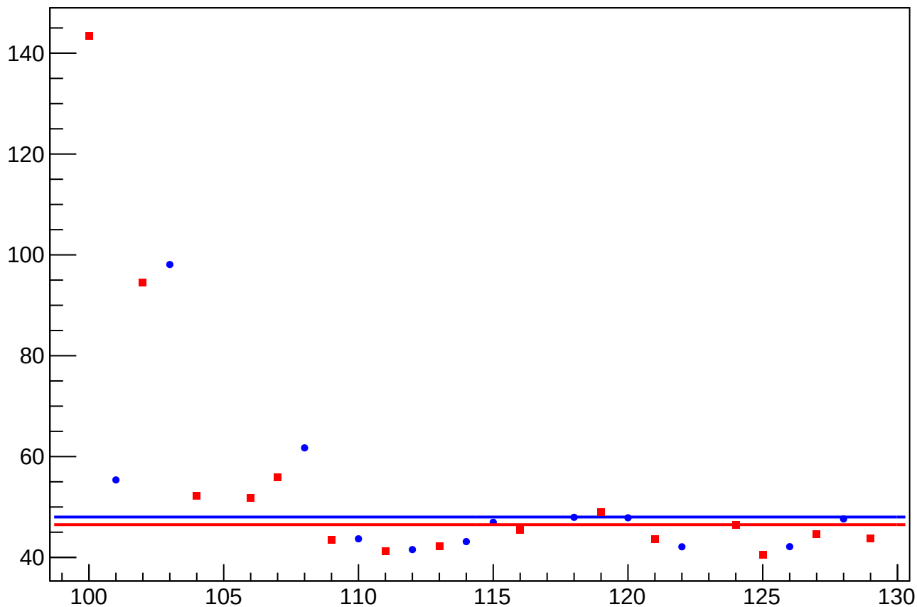
cor_asym_sam_15_37_dd_rms vs Slug, Sign Corrected
