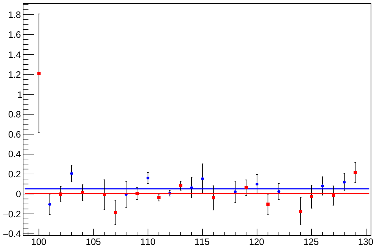
asym_sam_48_avg_eigen_dit_vs_eigen_cor_diff_mean vs Slug, Sign Corrected
