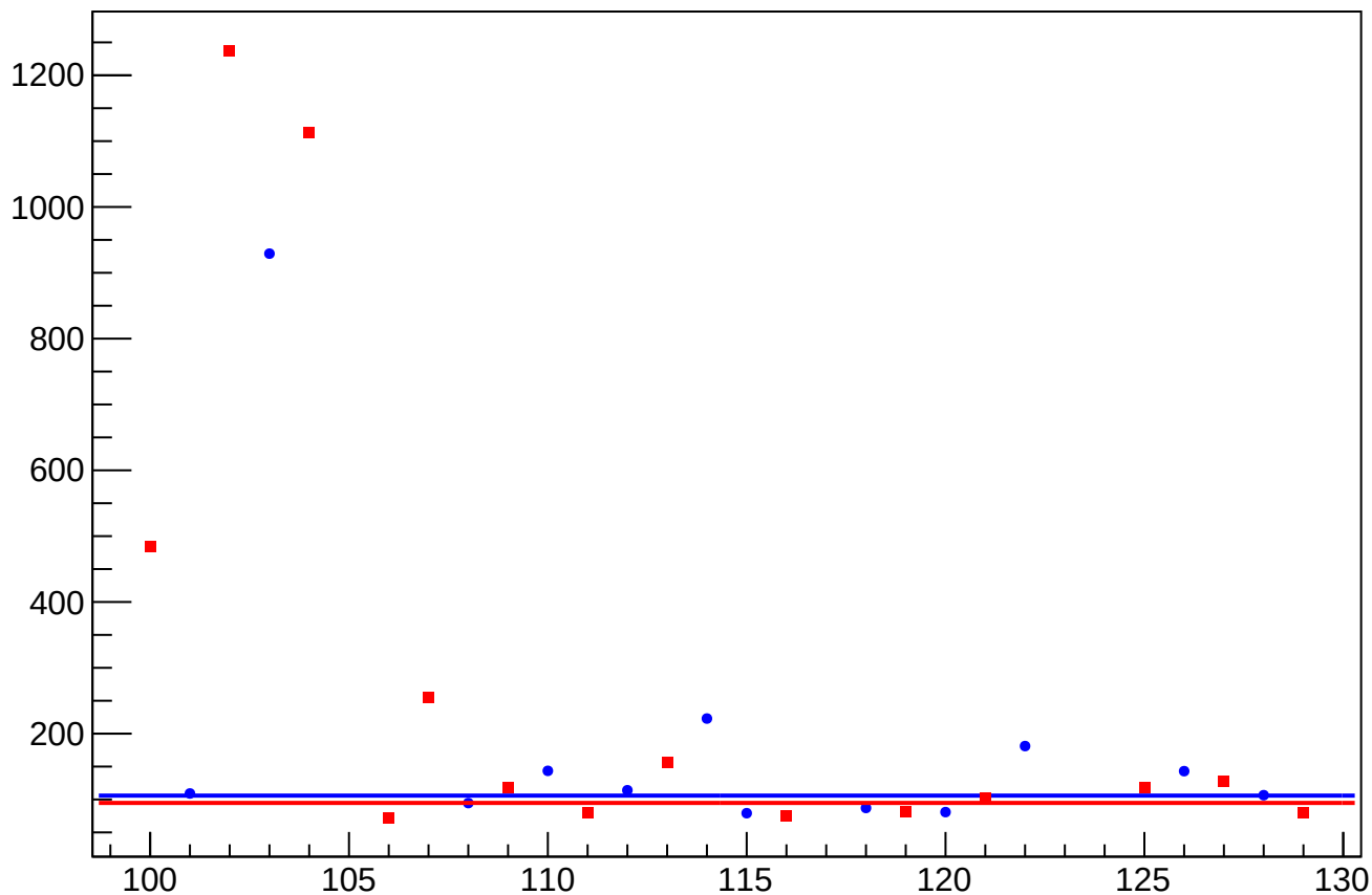
asym_us_avg_at1lr_avg_avg_dit_vs_eigen_cor_diff_rms vs Slug, Sign Corrected
