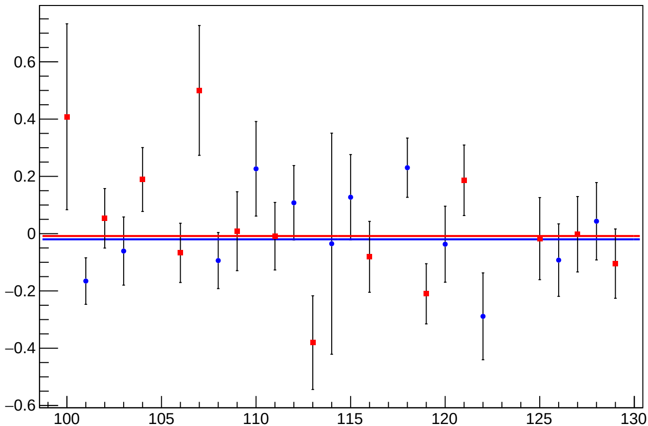
asym_us_avg_dit_vs_overload_cor_diff_mean vs Slug, Sign Corrected
