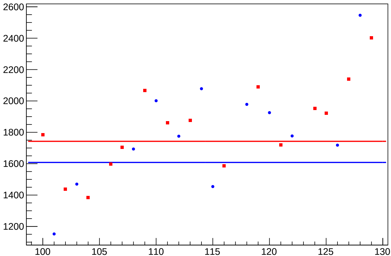
asym_usr_dit_correction_rms vs Slug, Sign Corrected
