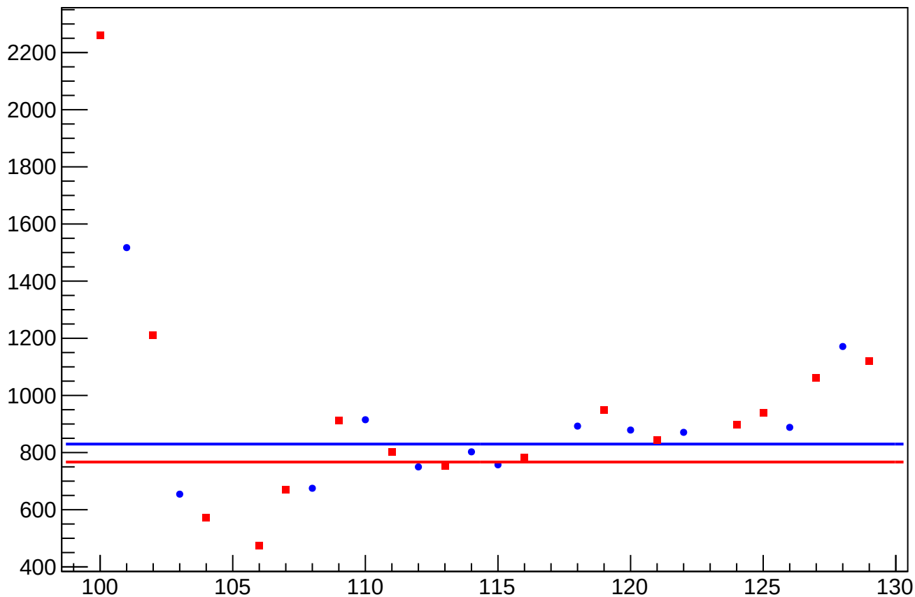
asym_usr_atr1_avg_reg_correction_rms vs Slug, Sign Corrected
