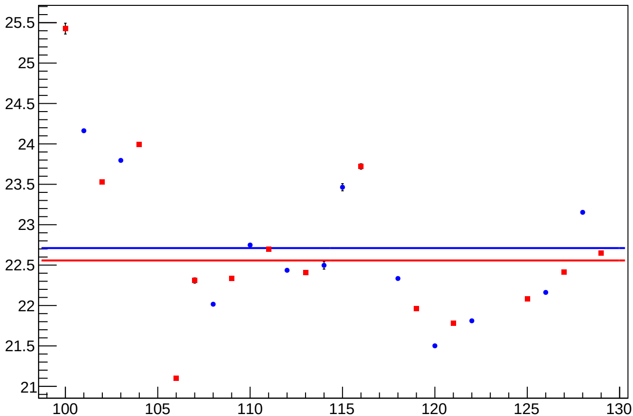
asym_bcm_dg_us_an_us_dd_rms vs Slug, Sign Corrected
