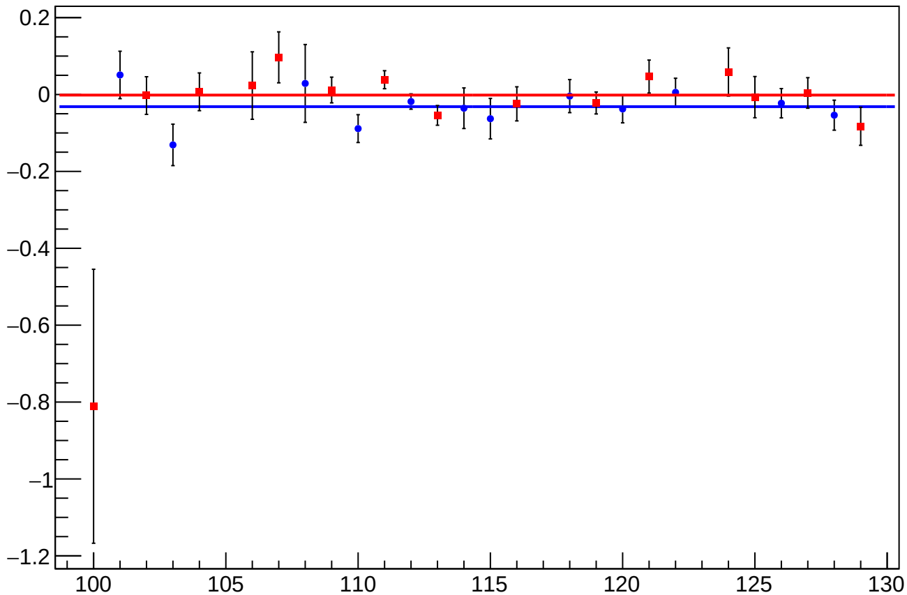
asym_sam_15_48_dd_eigen_dit_vs_cor_diff_mean vs Slug, Sign Corrected
