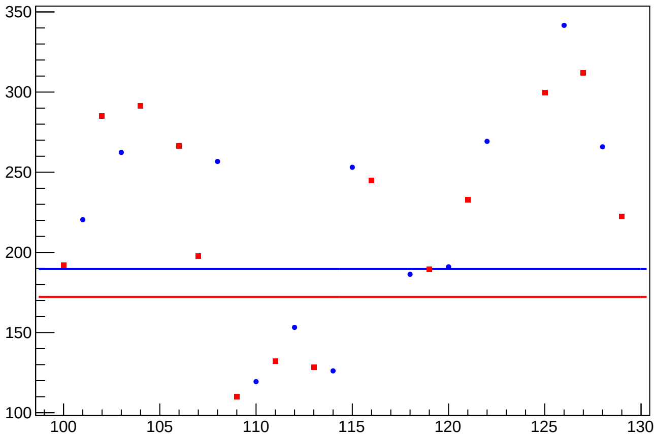
asym_bcm_dg_us_dg_ds_avg_rms vs Slug, Sign Corrected
