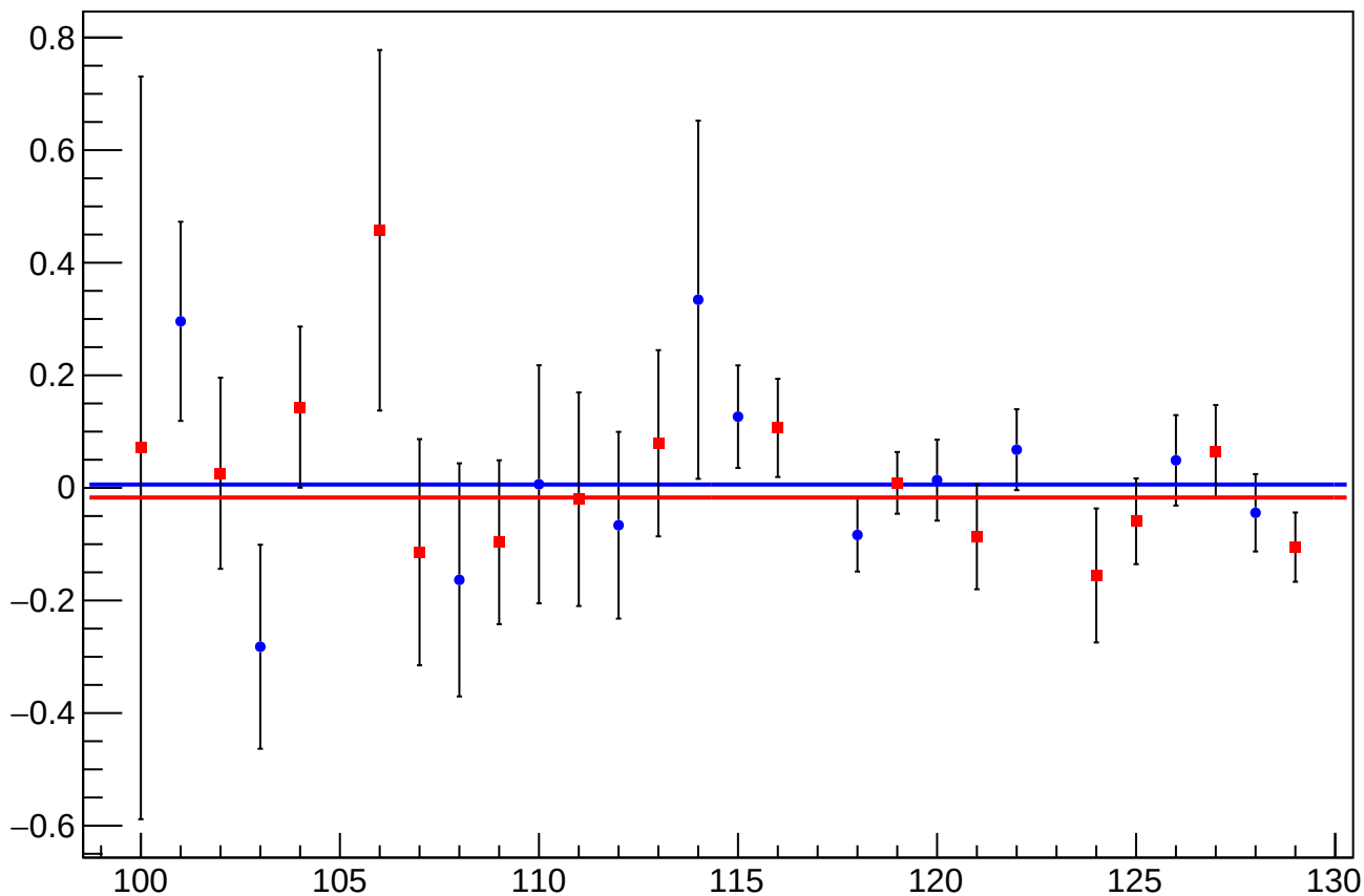
asym_sam_26_avg_dit_vs_cor_diff_mean vs Slug, Sign Corrected
