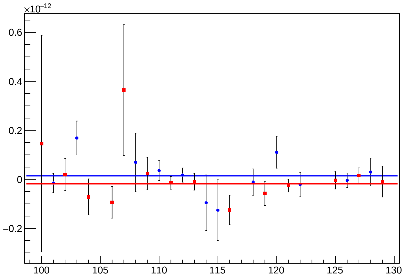
asym_us_dd_atlr_dd_dd_reg_vs_cor_diff_mean vs Slug, Sign Corrected
