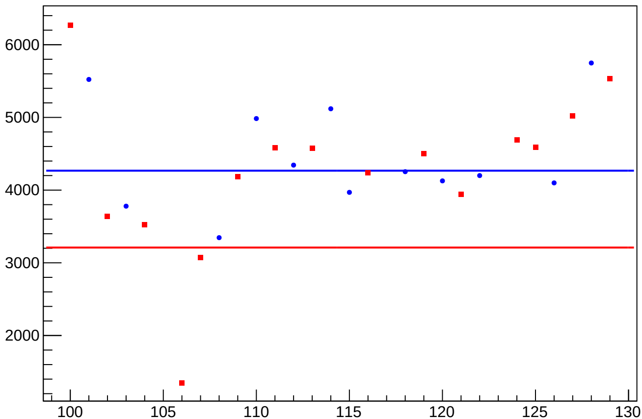
asym_atr_avg_eigen_dit_correction_rms vs Slug, Sign Corrected
