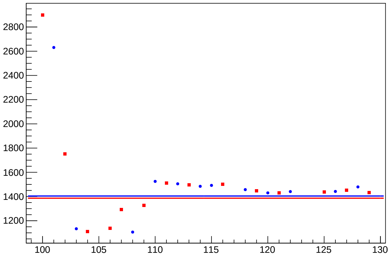
cor_asym_us_avg_at2lr_avg_dd_rms vs Slug, Sign Corrected
