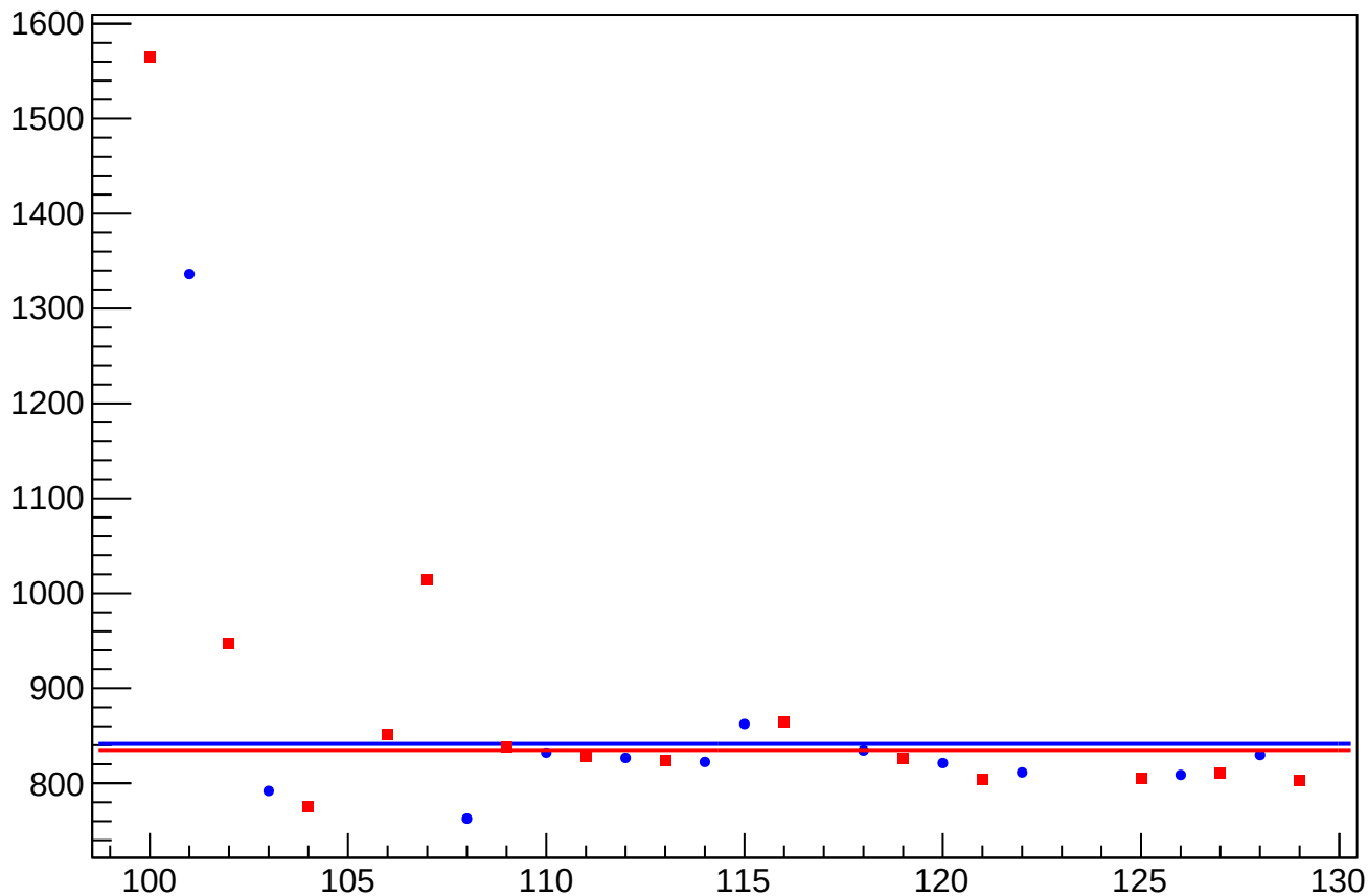
eigen_dit_asym_usl_atl2_dd_rms vs Slug, Sign Corrected
