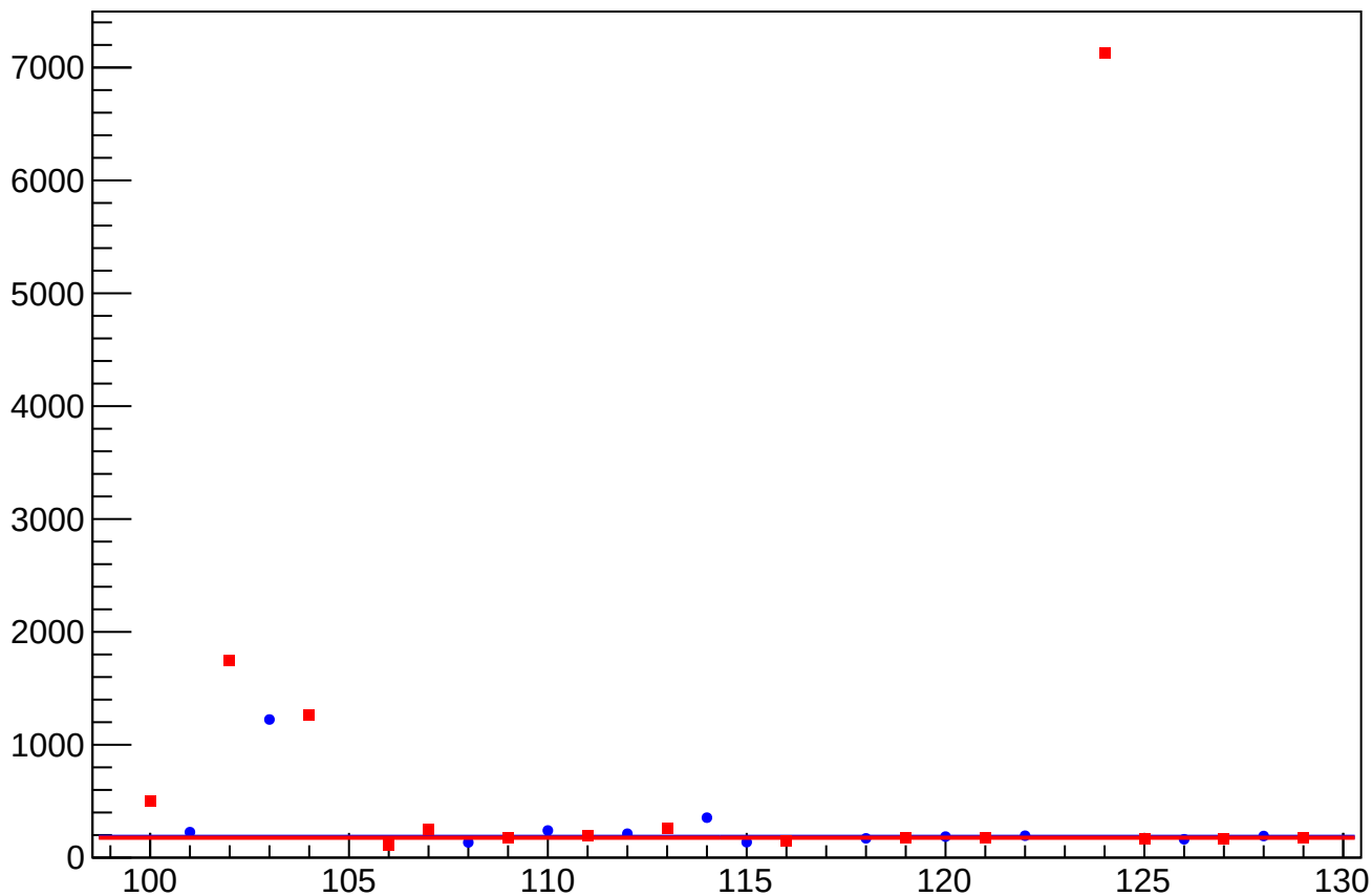
asym_atl1r2_avg_eigen_dit_vs_eigen_cor_diff_rms vs Slug, Sign Corrected
