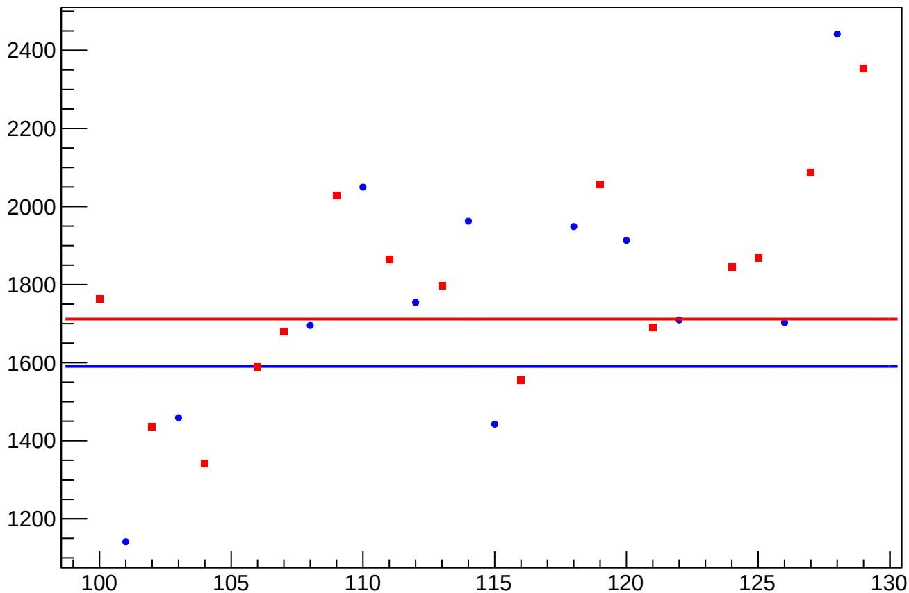
asym_usr_reg_correction_rms vs Slug, Sign Corrected
