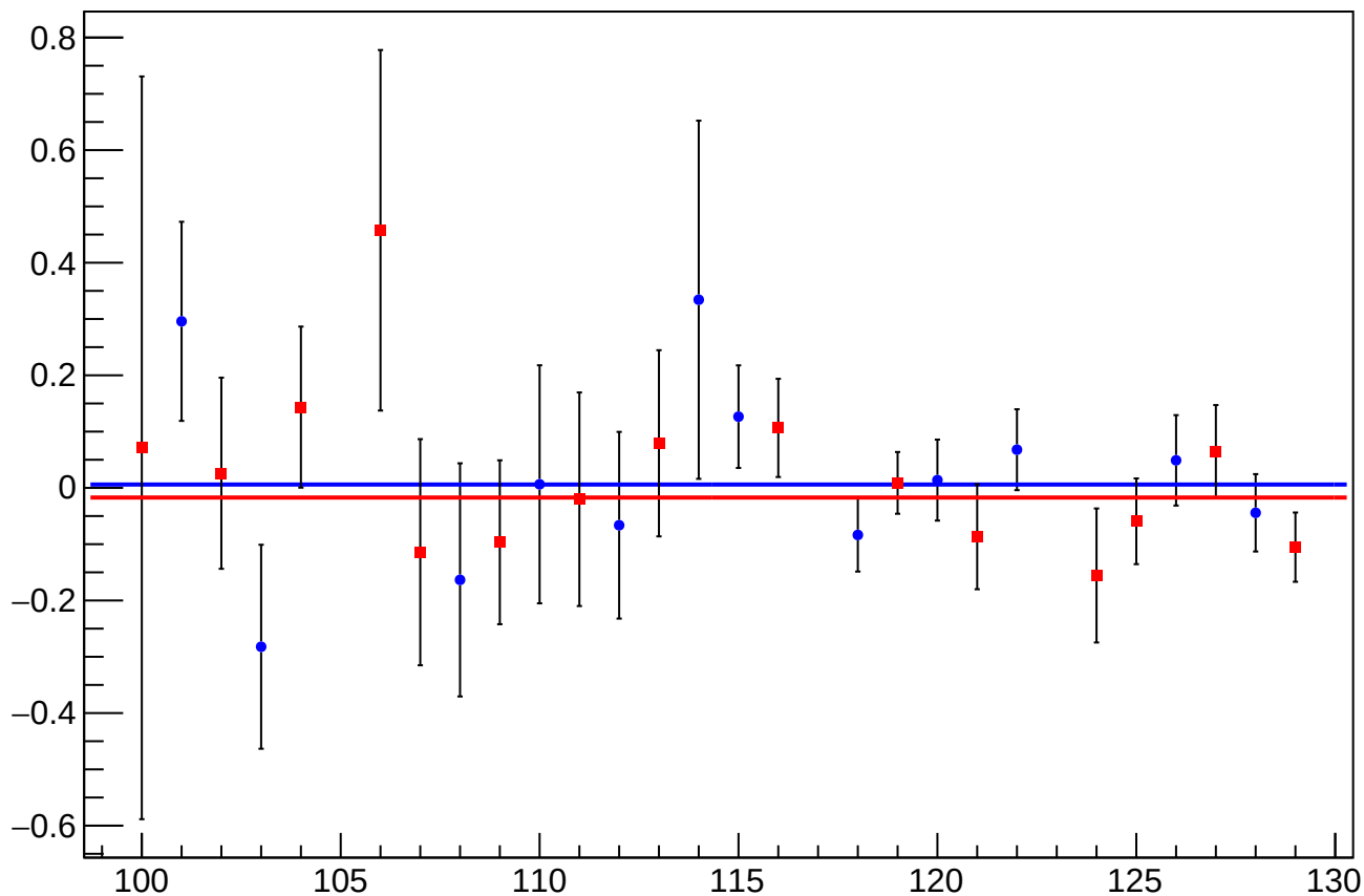
asym_sam_26_avg_eigen_dit_vs_eigen_cor_diff_mean vs Slug, Sign Corrected
