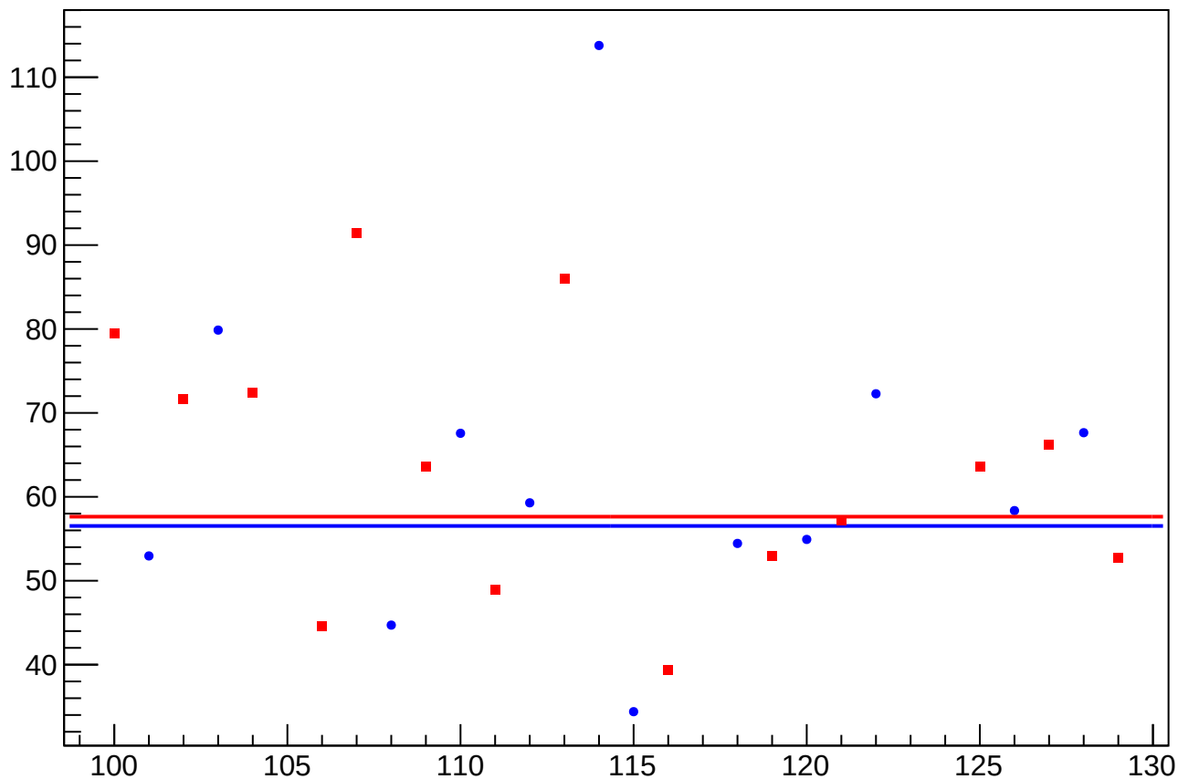
asym_us_avg_dit_vs_eigen_cor_diff_rms vs Slug, Sign Corrected
