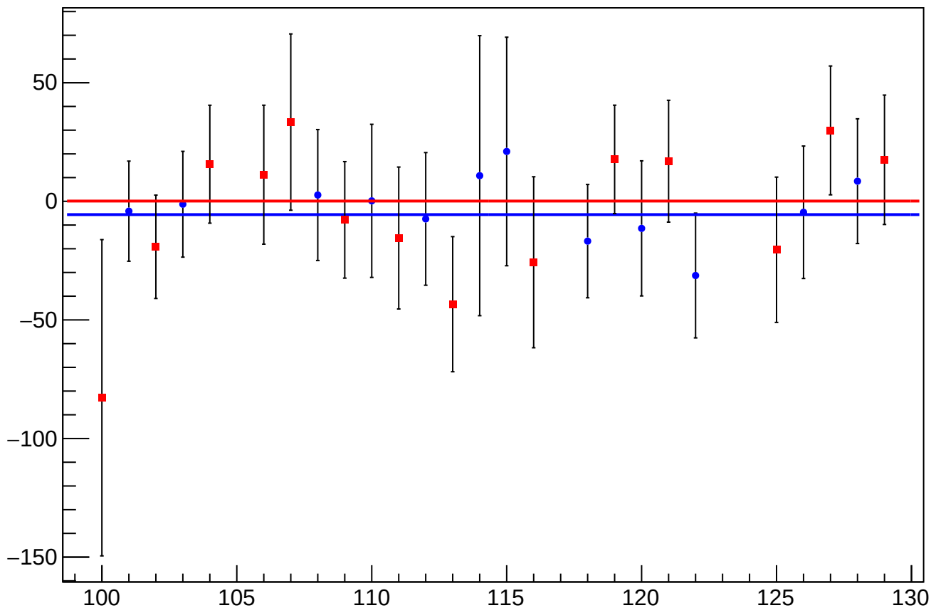
asym_bcm_dg_ds_an_ds_dd_mean vs Slug, Sign Corrected
