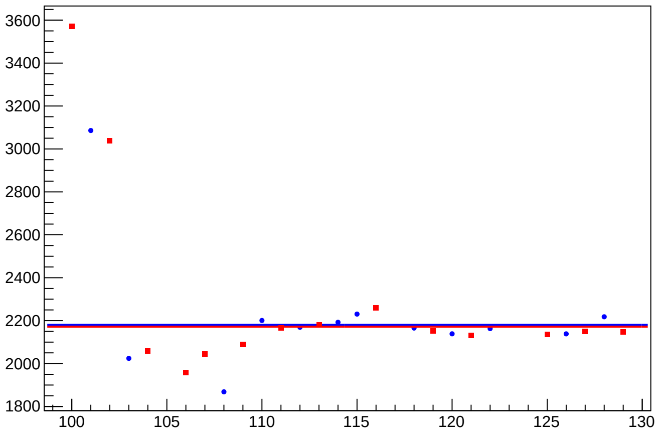
dit_asym_us_avg_at2lr_avg_avg_rms vs Slug, Sign Corrected
