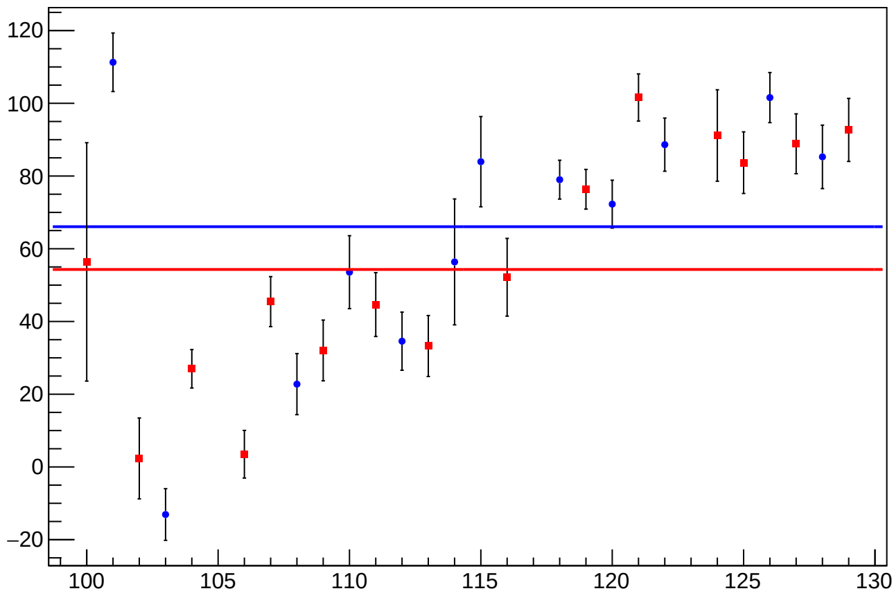
reg_asym_usr_atr2_avg_diff_bpm4eY_slope vs Slug, Sign Corrected
