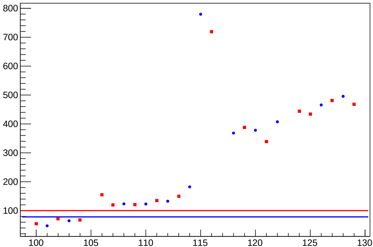
asym_sam_15_avg_reg_correction_rms vs Slug, Sign Corrected
