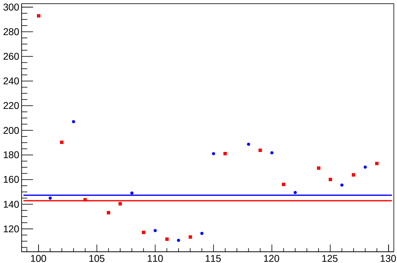
eigen_dit_asym_sam_48_avg_rms vs Slug, Sign Corrected
