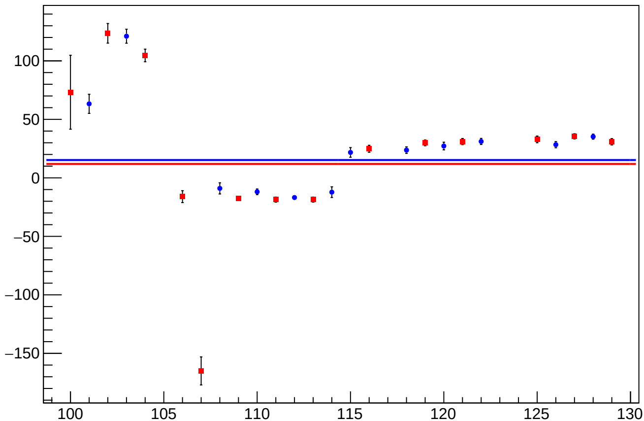
reg_asym_us_dd_at1lr_dd_avg_diff_bpm1X_slope vs Slug, Sign Corrected
