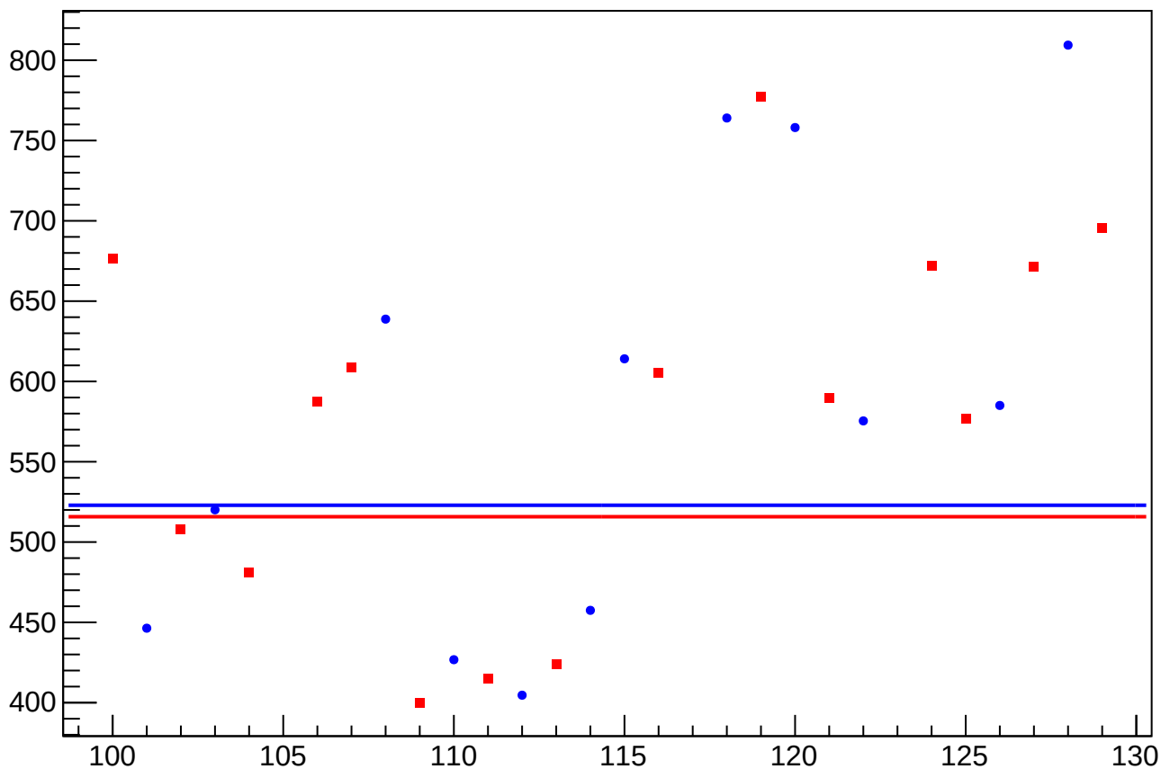
asym_sam_1357_avg_dit_correction_rms vs Slug, Sign Corrected
