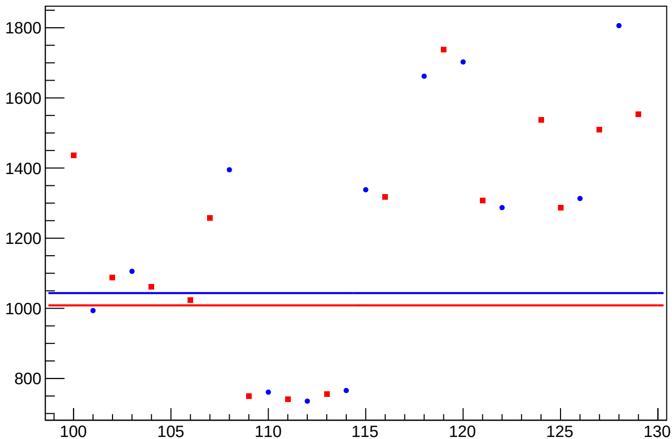
asym_sam_3748_avg_reg_correction_rms vs Slug, Sign Corrected
