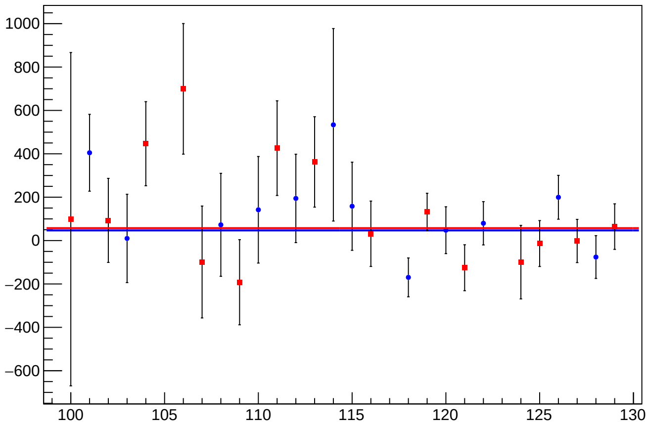
eigen_dit_asym_sam_1526_avg_mean vs Slug, Sign Corrected
