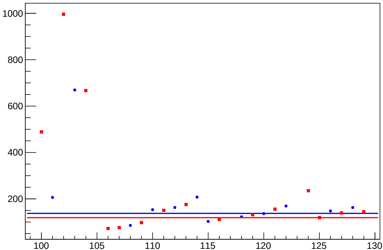
asym_usr_atr2_dd_eigen_dit_vs_cor_diff_rms vs Slug, Sign Corrected
