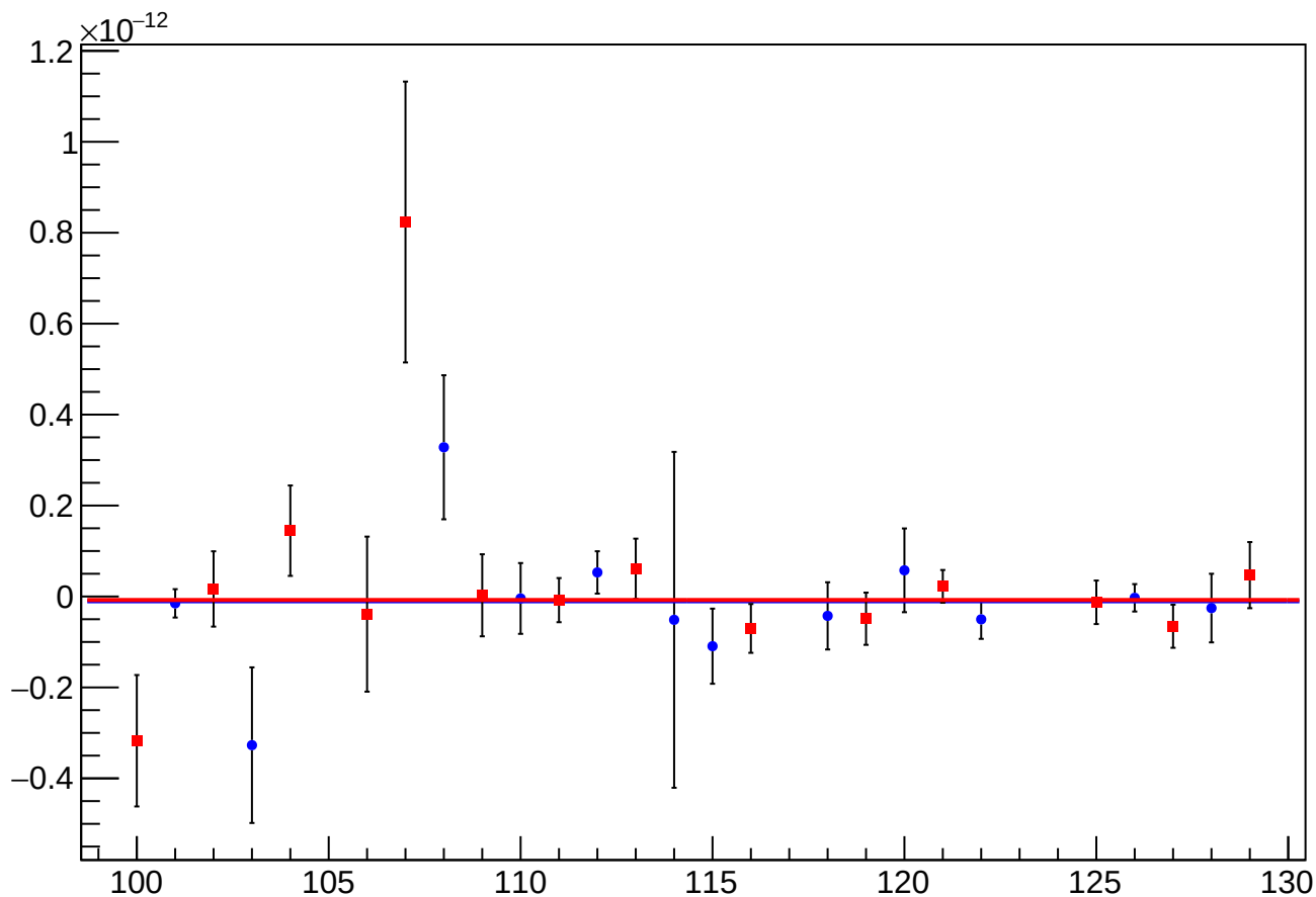
asym_usl_atl1_dd_reg_vs_cor_diff_mean vs Slug, Sign Corrected
