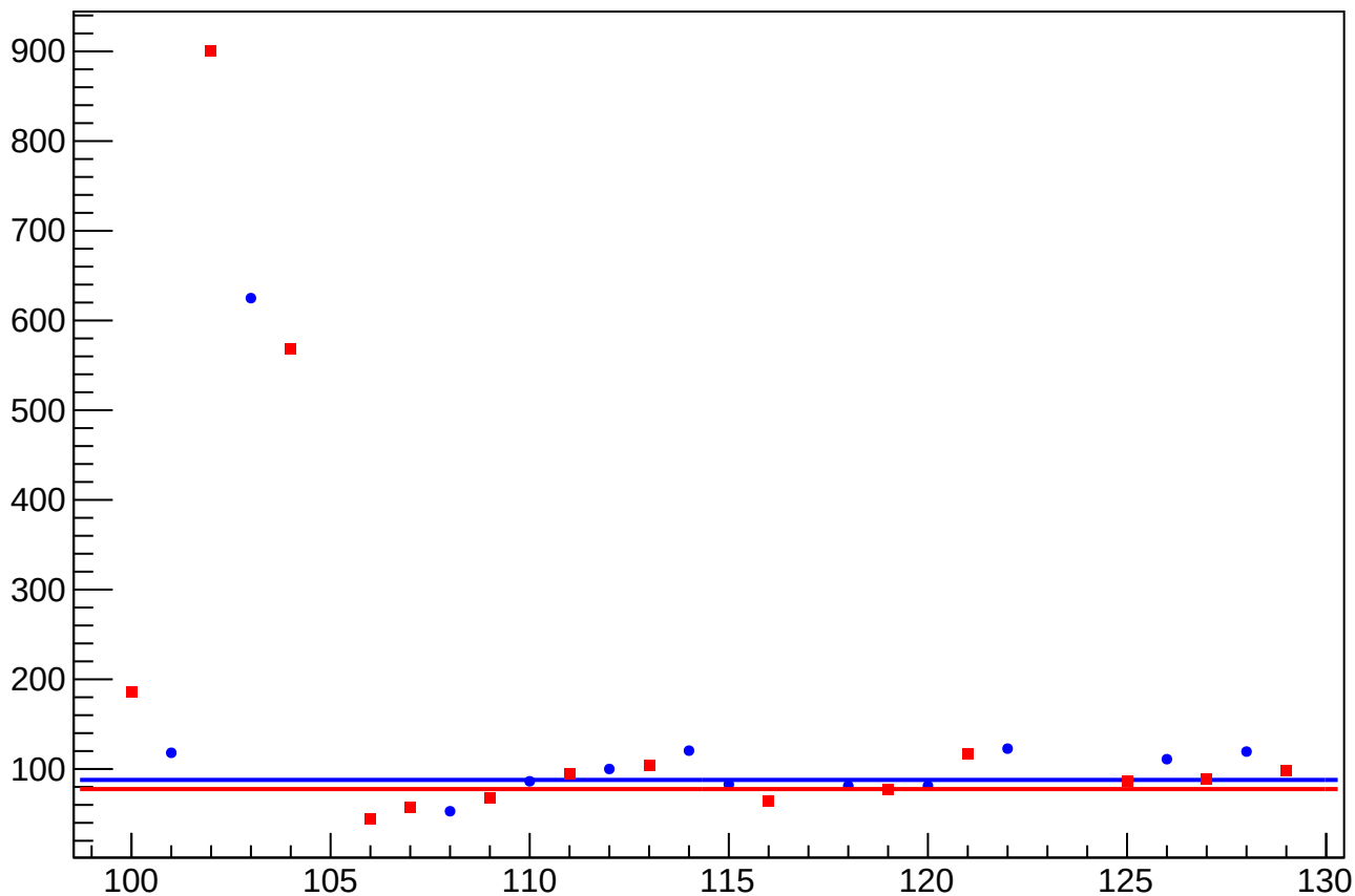
asym_us_dd_at2lr_dd_avg_eigen_dit_vs_eigen_cor_diff_rms vs Slug, Sign Corrected
