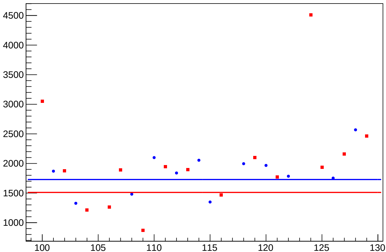
asym_at2_dd_eigen_cor_correction_rms vs Slug, Sign Corrected
