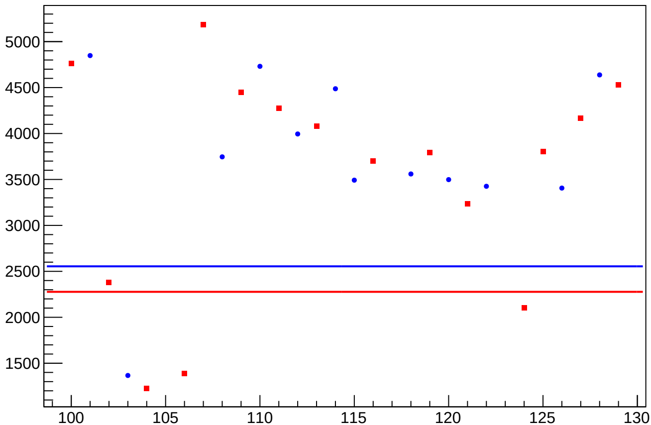
asym_atl_avg_atr_avg_avg_reg_correction_rms vs Slug, Sign Corrected
