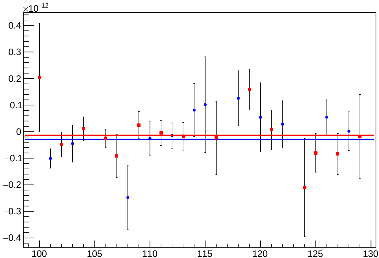
asym_sam_15_48_dd_reg_vs_cor_diff_mean vs Slug, Sign Corrected
