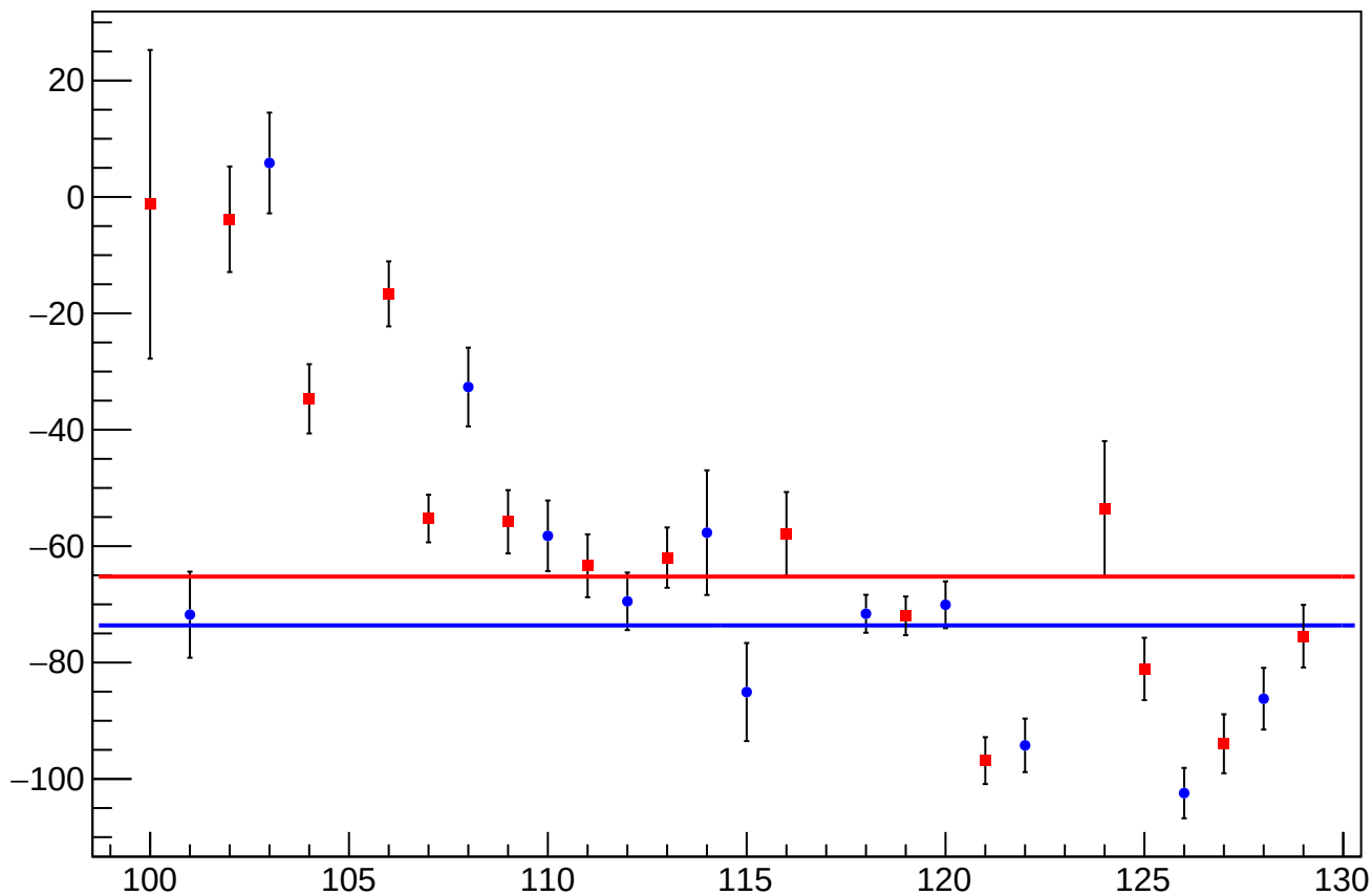
reg_asym_atl1r2_dd_atl2r1_dd_dd_diff_bpm4eY_slope vs Slug, Sign Corrected
