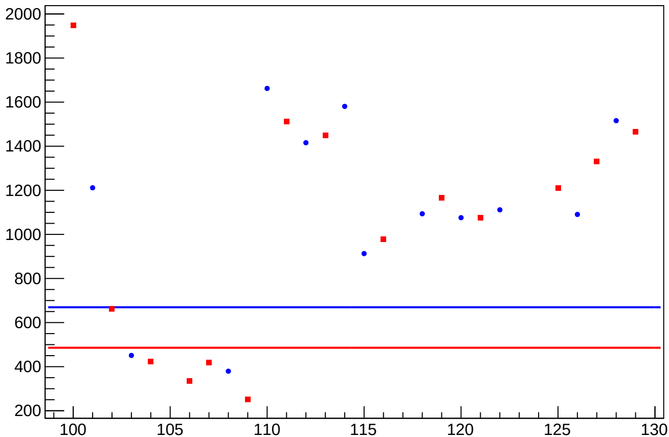
asym_us_dd_at2lr_dd_dd_reg_correction_rms vs Slug, Sign Corrected
