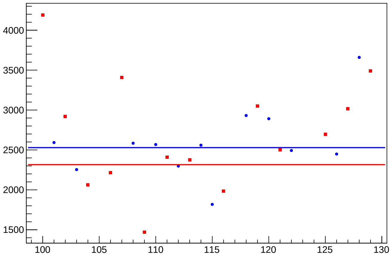
asym_us_dd_at2lr_dd_avg_cor_correction_rms vs Slug, Sign Corrected
