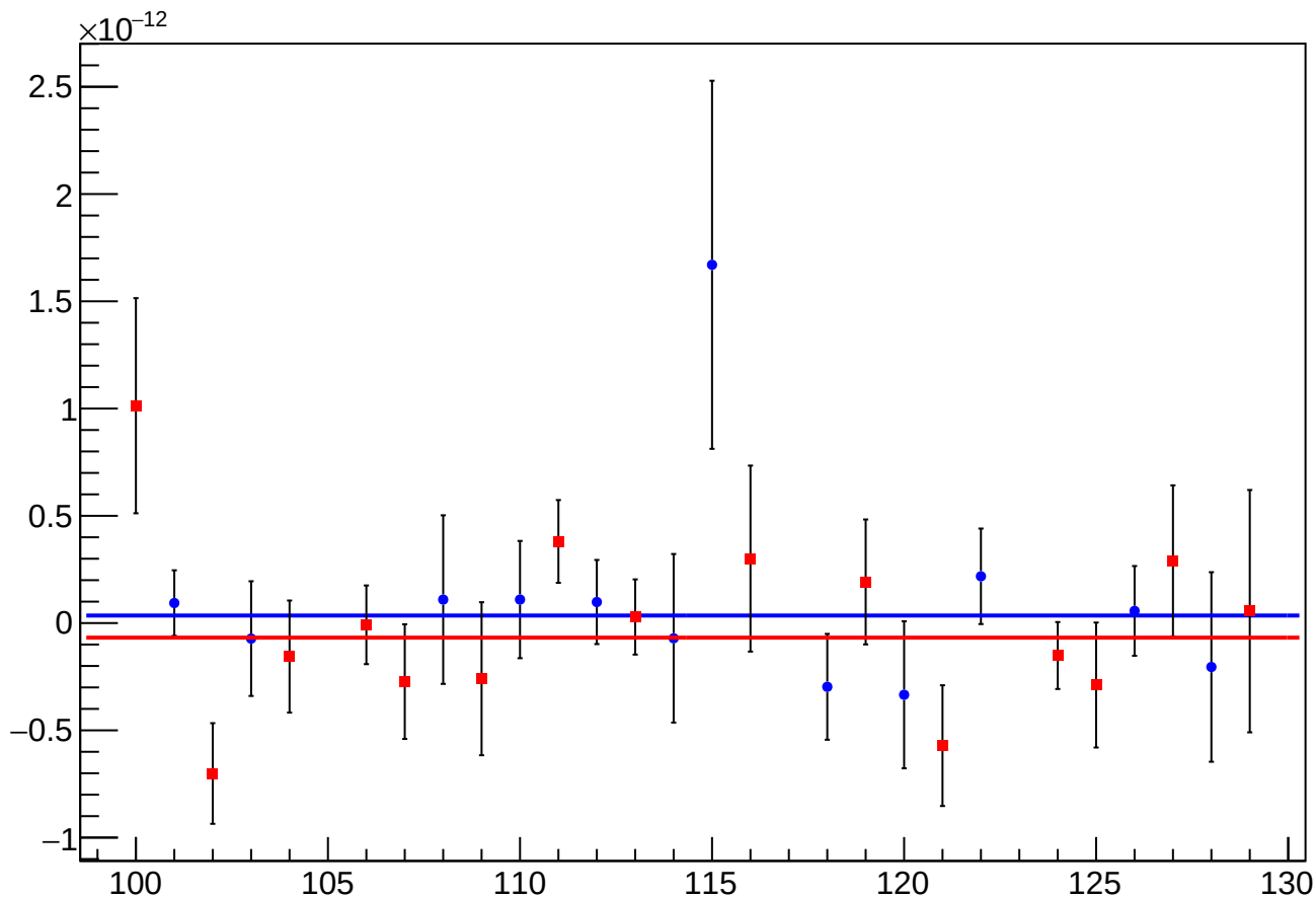
asym_atl_dd_reg_vs_cor_diff_mean vs Slug, Sign Corrected
