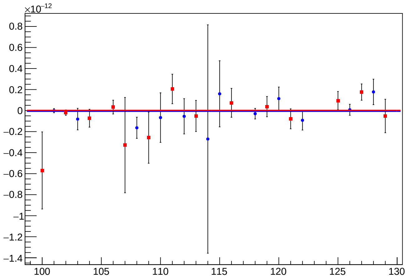
asym_usl_atl1_avg_reg_vs_cor_diff_mean vs Slug, Sign Corrected
