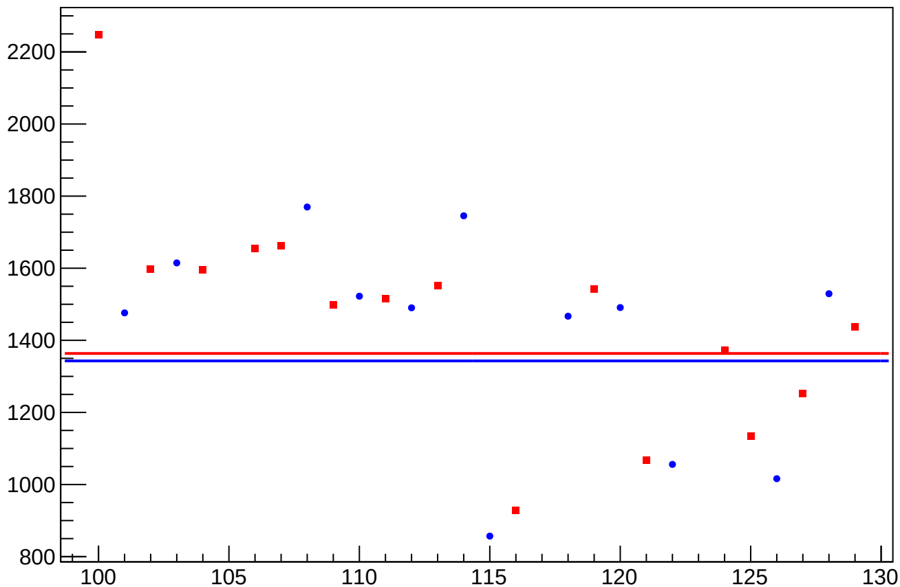
asym_sam_3726_avg_eigen_cor_correction_rms vs Slug, Sign Corrected
