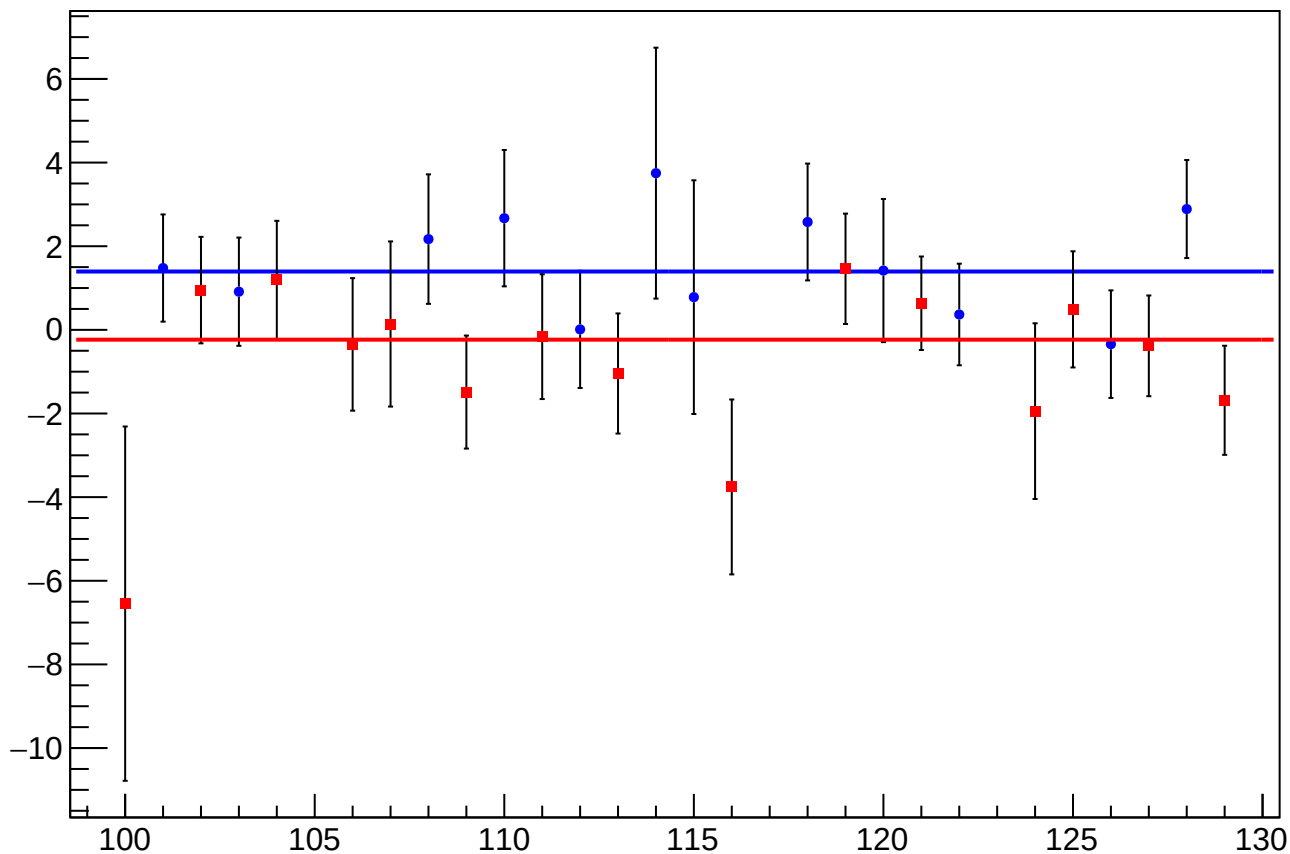
diff_bpm_4aY_4acY_dd_mean vs Slug, Sign Corrected
