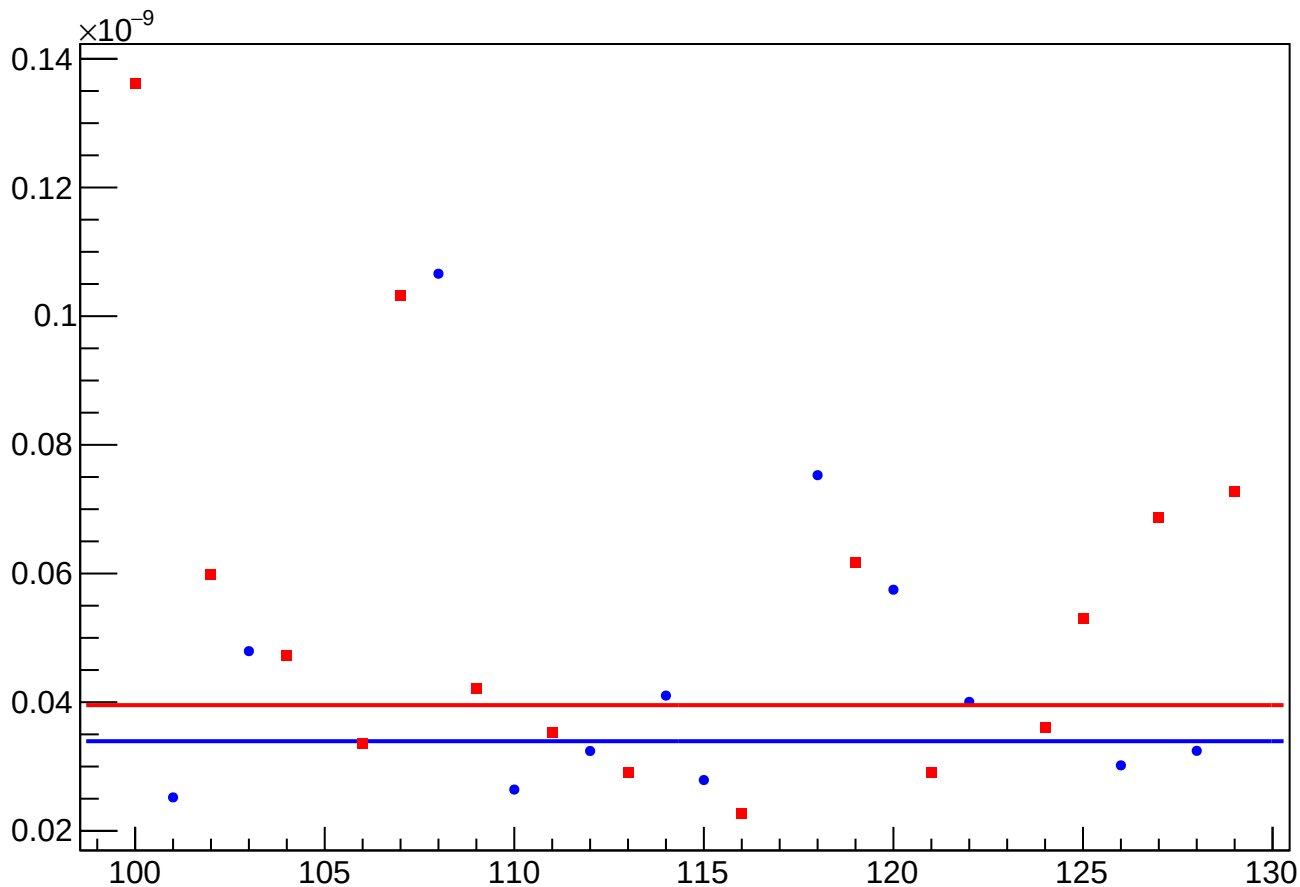
asym_sam3_eigen_cor_vs_cor_diff_rms vs Slug, Sign Corrected
