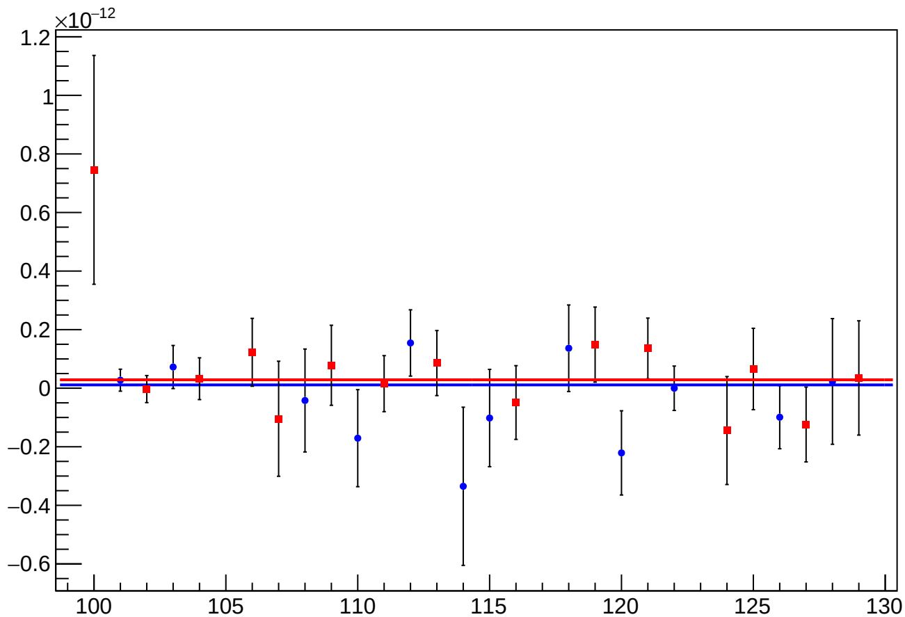
asym_usr_eigen_cor_vs_cor_diff_mean vs Slug, Sign Corrected
