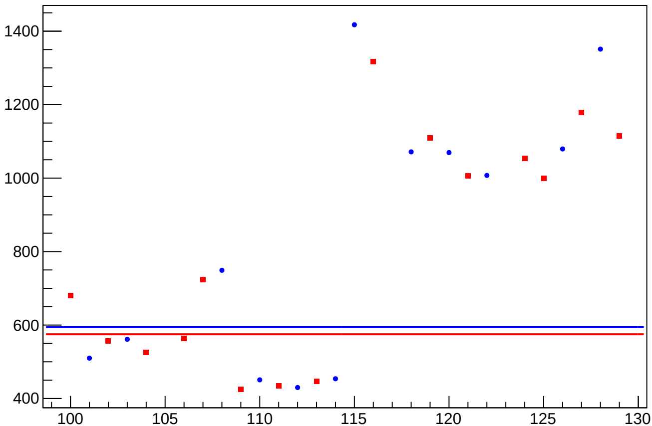
asym_sam_1548_avg_dit_correction_rms vs Slug, Sign Corrected
