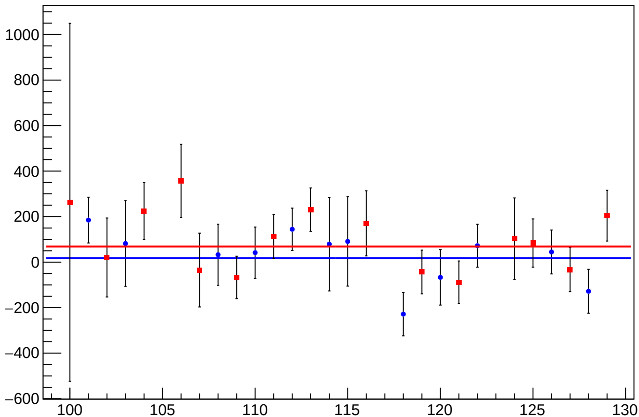
cor_asym_sam_12345678_avg_mean vs Slug, Sign Corrected
