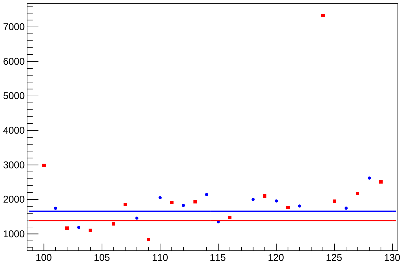
asym_at2_dd_eigen_dit_correction_rms vs Slug, Sign Corrected
