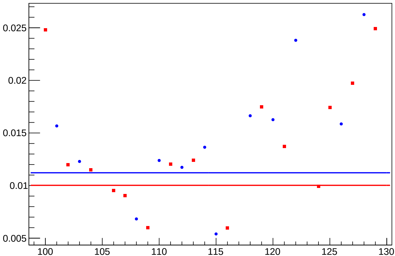
asym_atl1r2_dd_eigen_dit_vs_dit_diff_rms vs Slug, Sign Corrected
