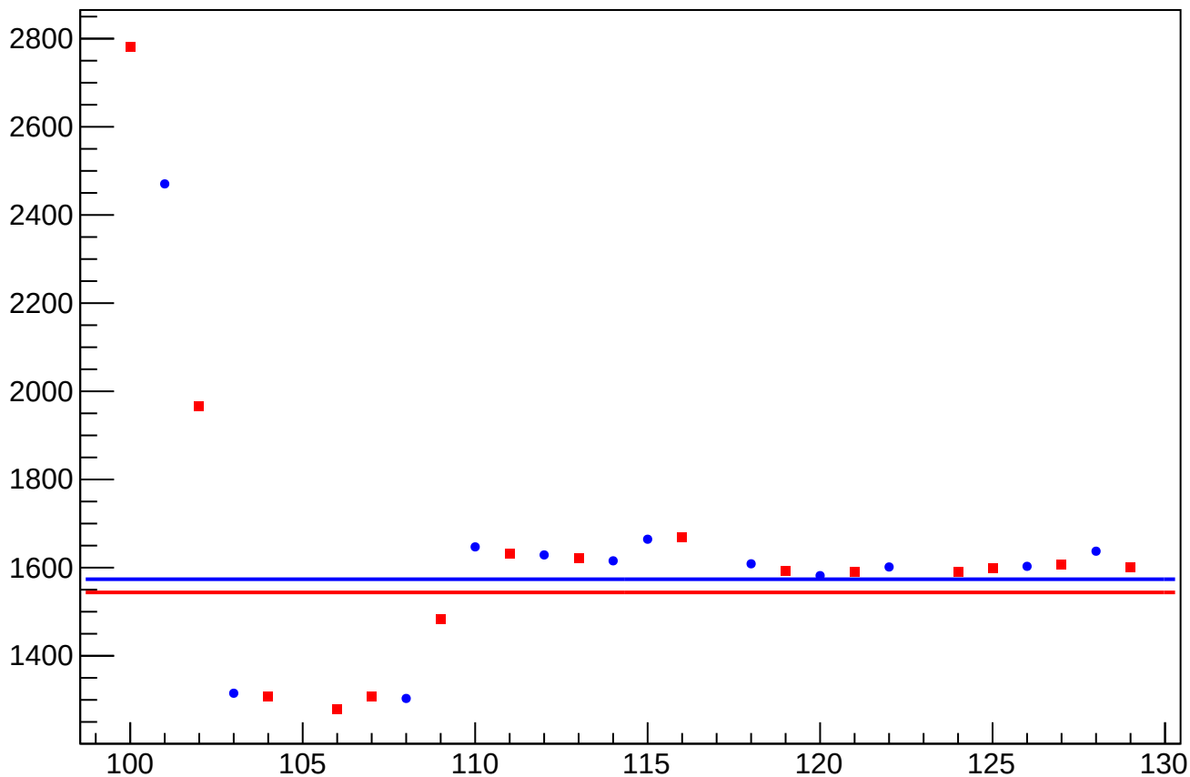
eigen_cor_asym_usr_atr2_avg_rms vs Slug, Sign Corrected
