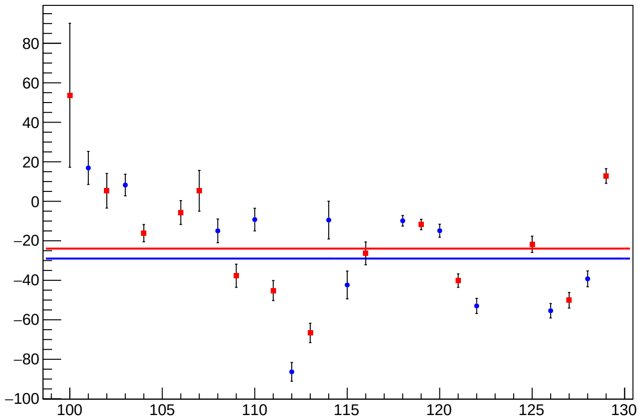
reg_asym_us_avg_at1lr_avg_avg_diff_bpm4eY_slope vs Slug, Sign Corrected
