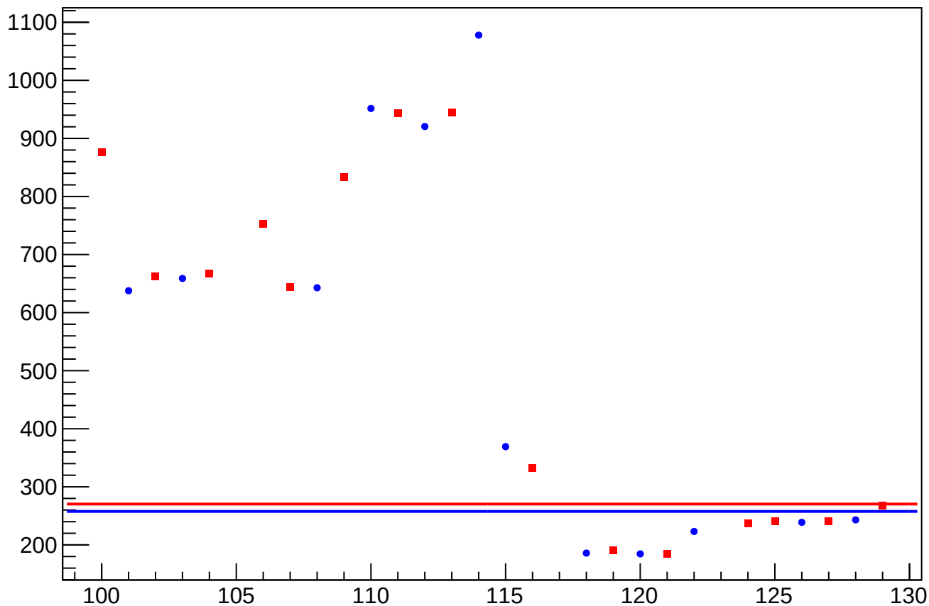
asym_sam_37_26_dd_dit_correction_rms vs Slug, Sign Corrected
