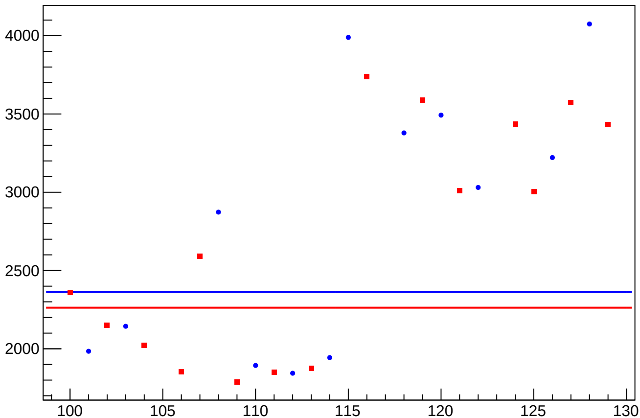
asym_sam4_reg_correction_rms vs Slug, Sign Corrected
