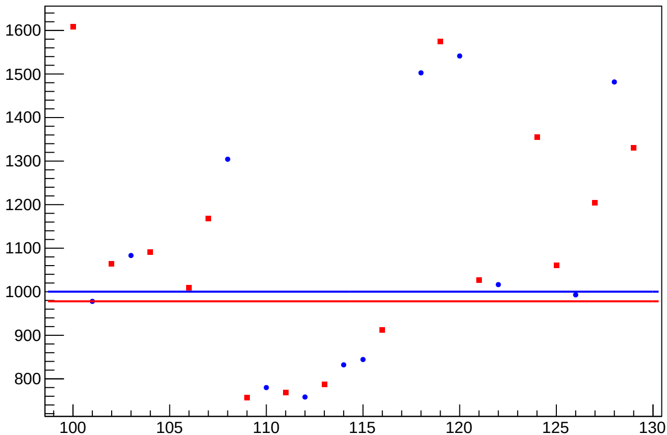
asym_sam_37_avg_cor_correction_rms vs Slug, Sign Corrected
