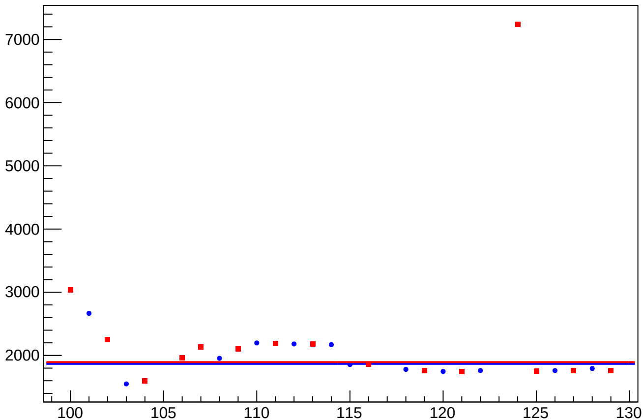
cor_asym_atl1r2_avg_rms vs Slug, Sign Corrected
