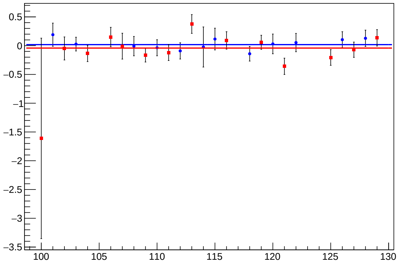
asym_usl_atl2_dd_eigen_dit_vs_eigen_cor_diff_mean vs Slug, Sign Corrected
