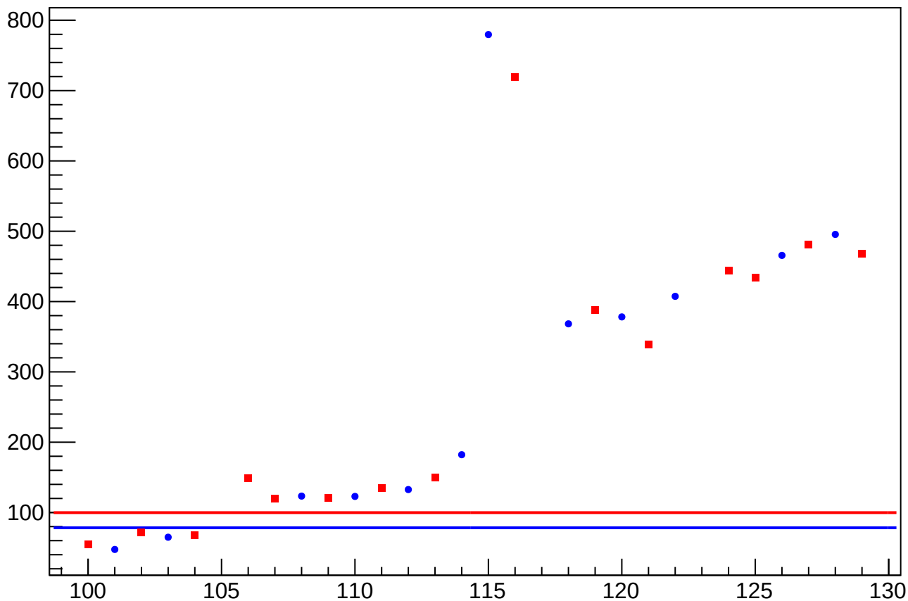
asym_sam_15_avg_eigen_cor_correction_rms vs Slug, Sign Corrected
