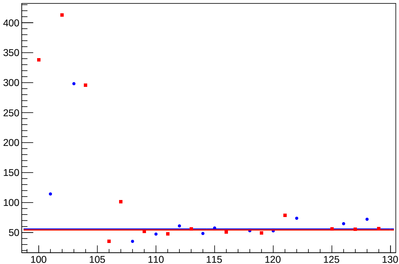
asym_us_dd_atlr_dd_avg_eigen_dit_vs_cor_diff_rms vs Slug, Sign Corrected
