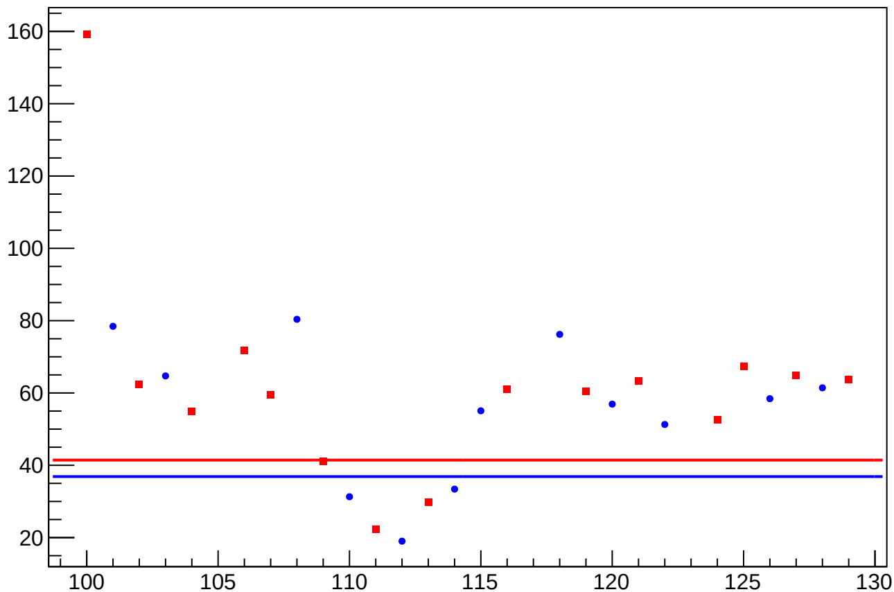
asym_sam_48_avg_dit_vs_eigen_cor_diff_rms vs Slug, Sign Corrected
