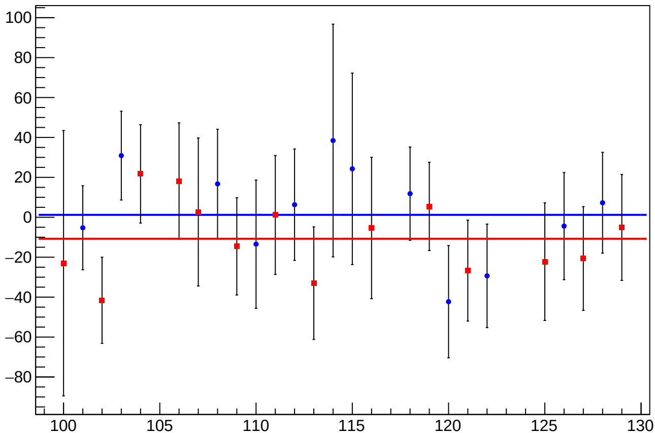
asym_bcm_dg_ds_an_us_dd_mean vs Slug, Sign Corrected
