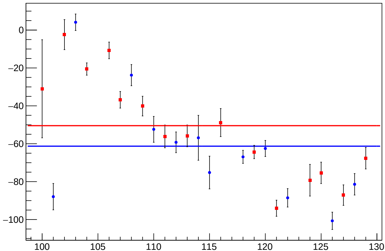
reg_asym_usr_atr2_dd_diff_bpm4eY_slope vs Slug, Sign Corrected
