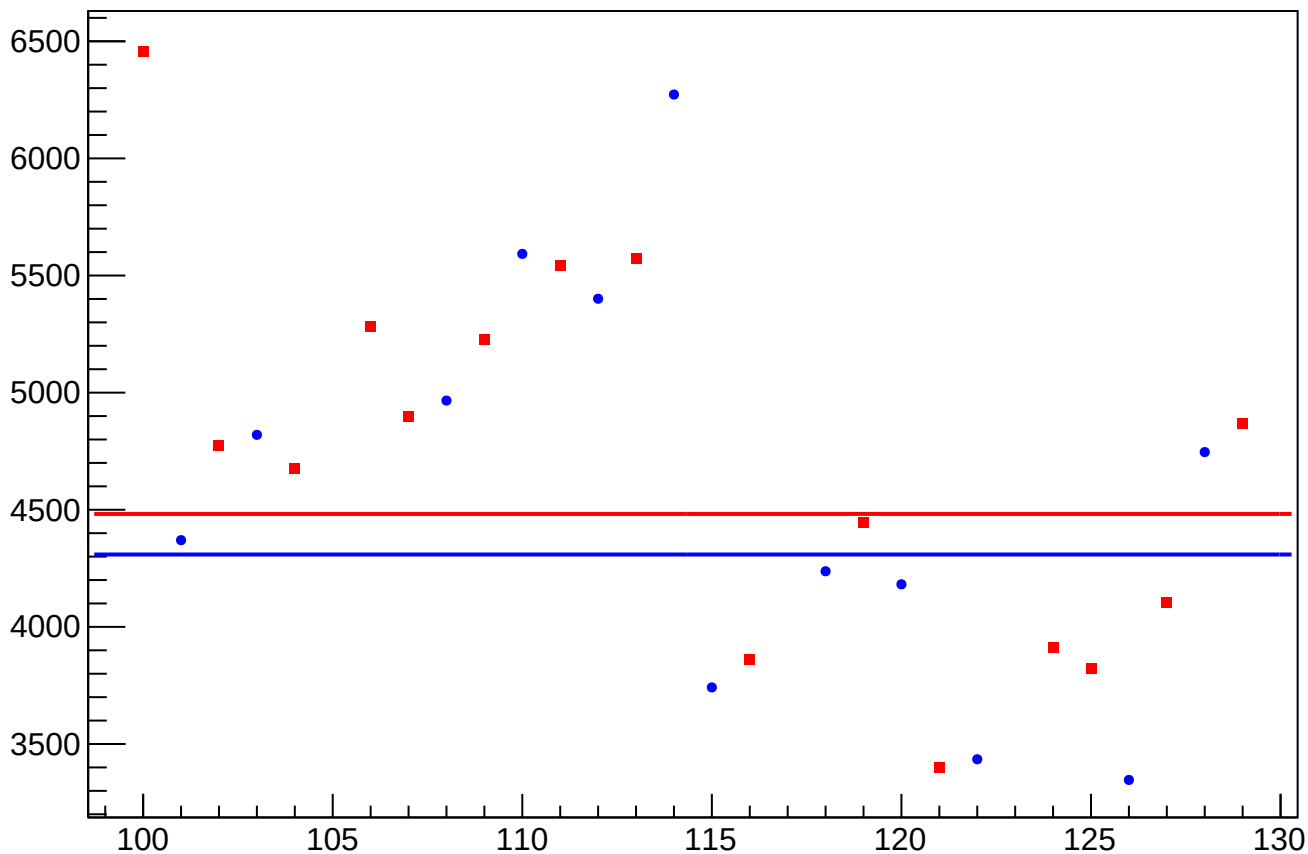
asym_sam2_eigen_dit_correction_rms vs Slug, Sign Corrected
