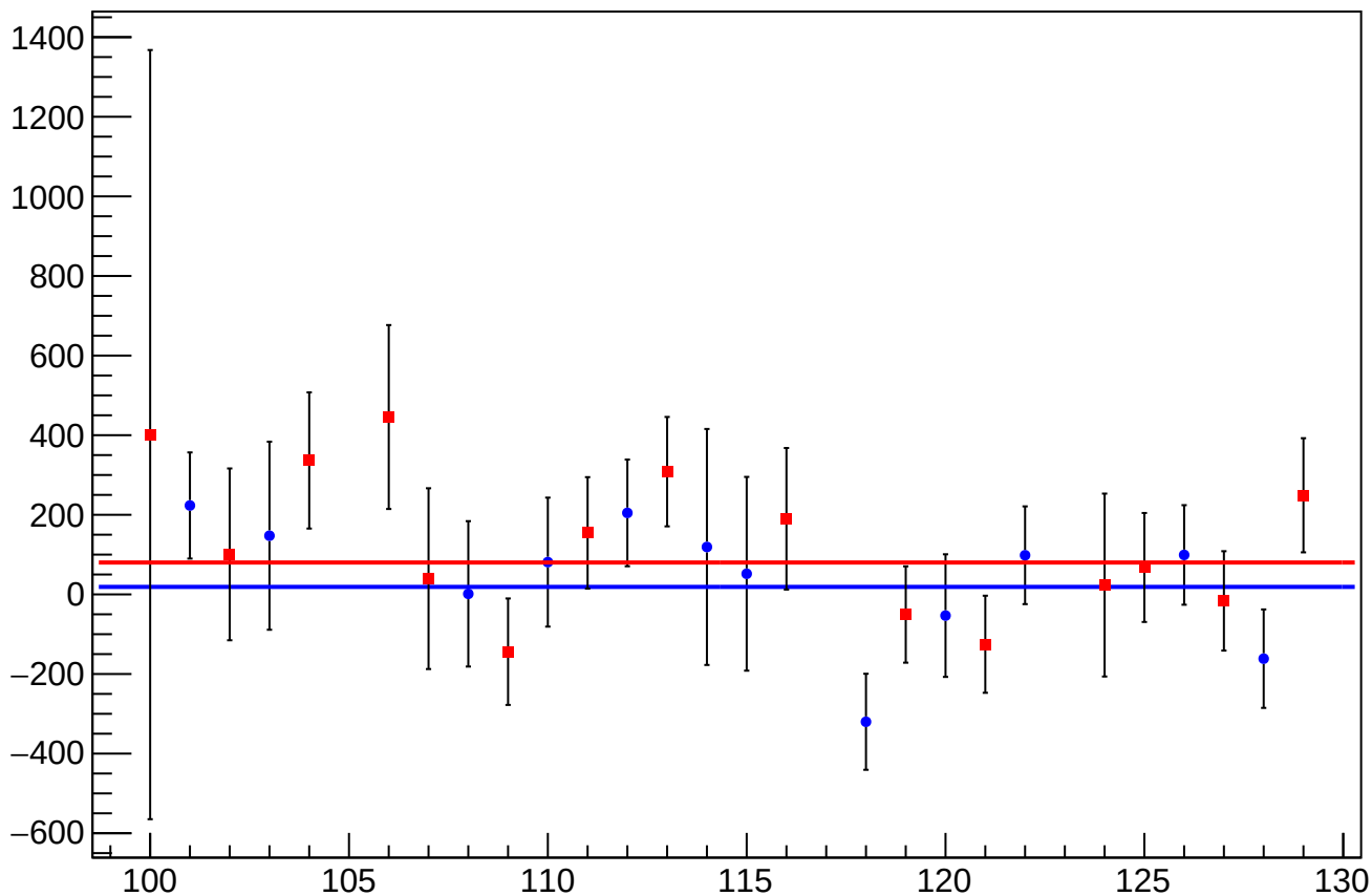
cor_asym_sam_2468_avg_mean vs Slug, Sign Corrected
