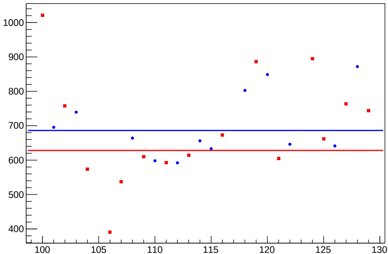
asym_sam_37_dd_cor_correction_rms vs Slug, Sign Corrected
