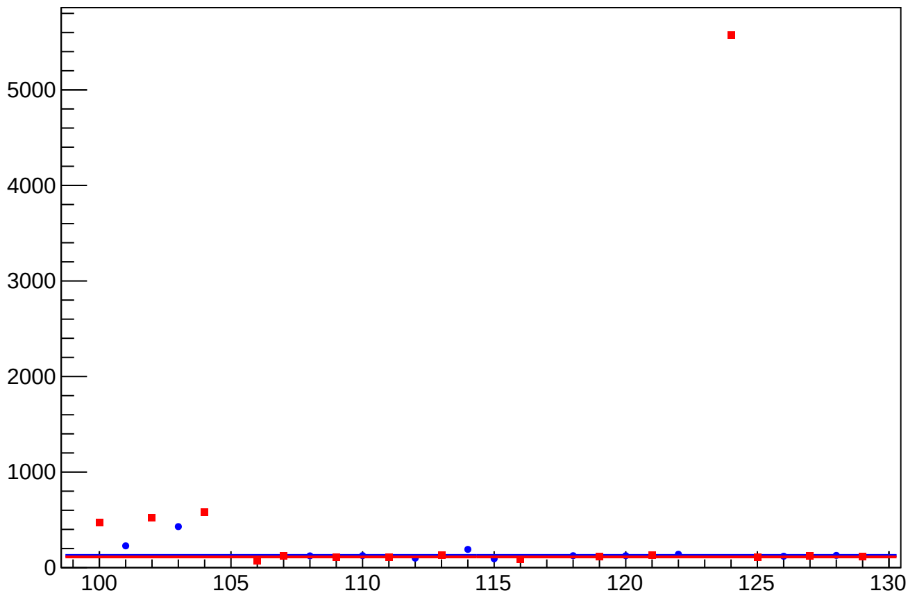
asym_atr1l2_avg_eigen_dit_vs_eigen_cor_diff_rms vs Slug, Sign Corrected
