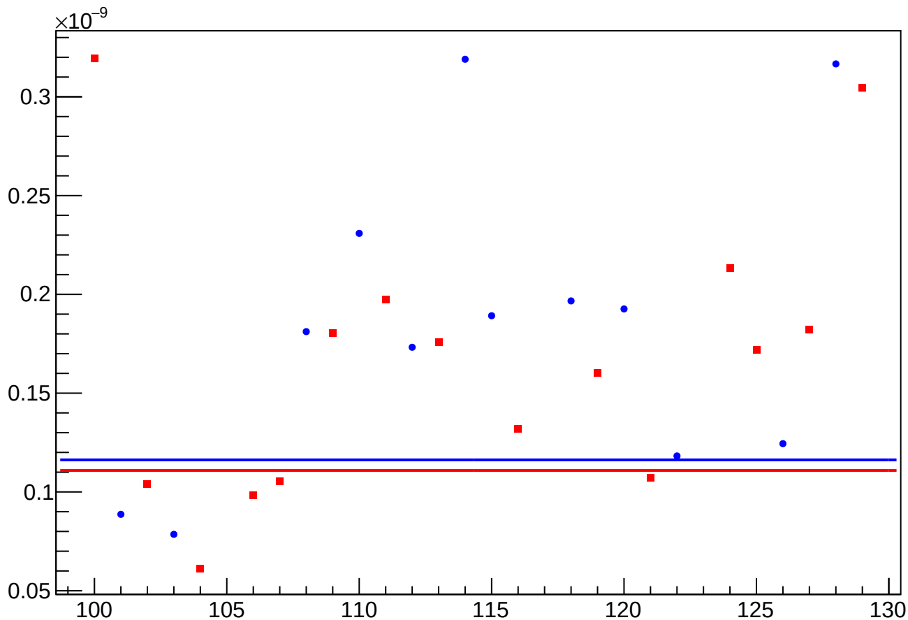
asym_usr_atr2_avg_eigen_cor_vs_cor_diff_rms vs Slug, Sign Corrected
