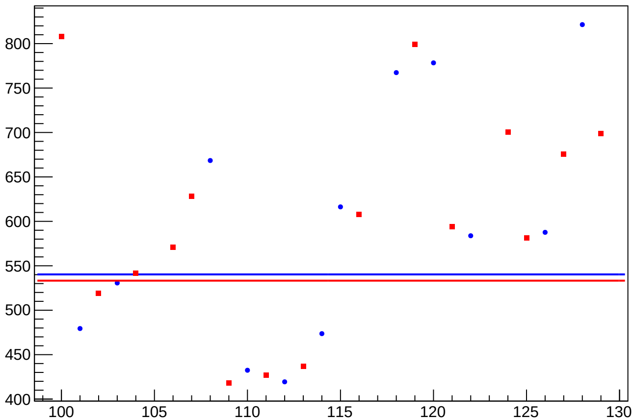
asym_sam_1357_avg_cor_correction_rms vs Slug, Sign Corrected
