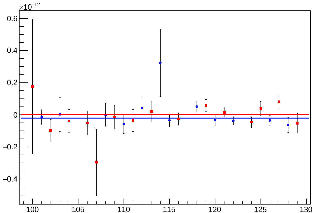
asym_at1_dd_eigen_cor_vs_cor_diff_mean vs Slug, Sign Corrected
