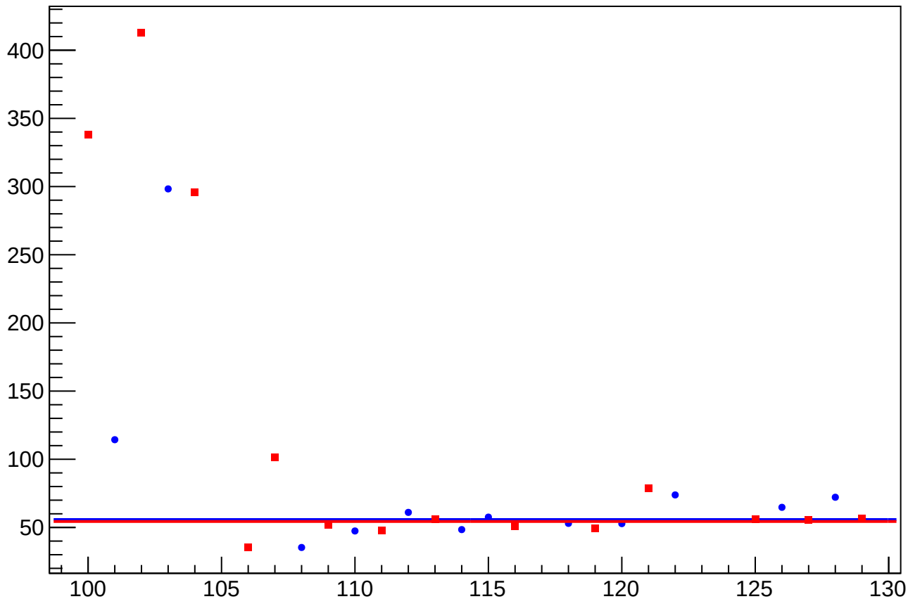
asym_us_dd_atlr_dd_avg_eigen_dit_vs_eigen_cor_diff_rms vs Slug, Sign Corrected
