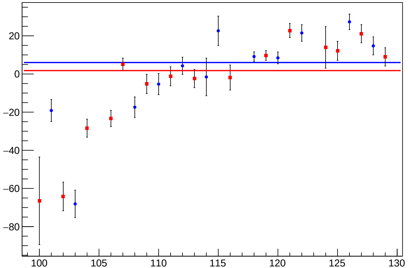
reg_asym_at1_avg_at2_avg_dd_diff_bpm4aY_slope vs Slug, Sign Corrected
