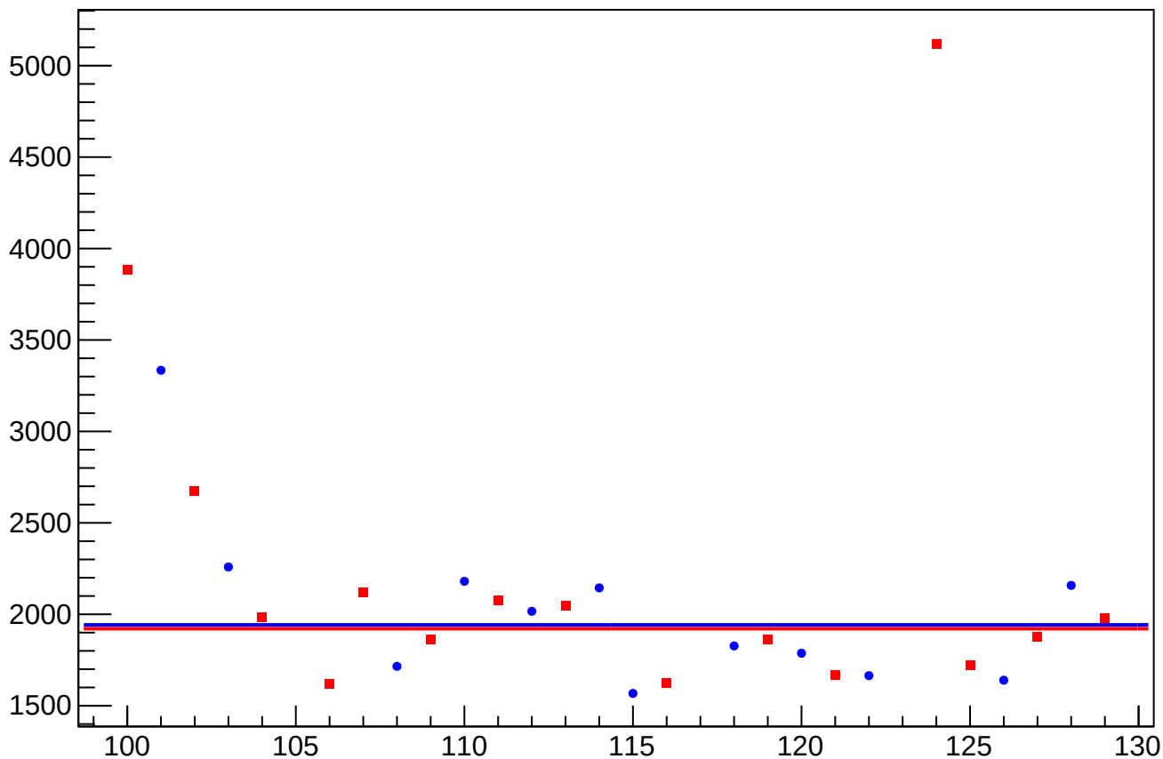
asym_at1_dd_at2_dd_avg_rms vs Slug, Sign Corrected
