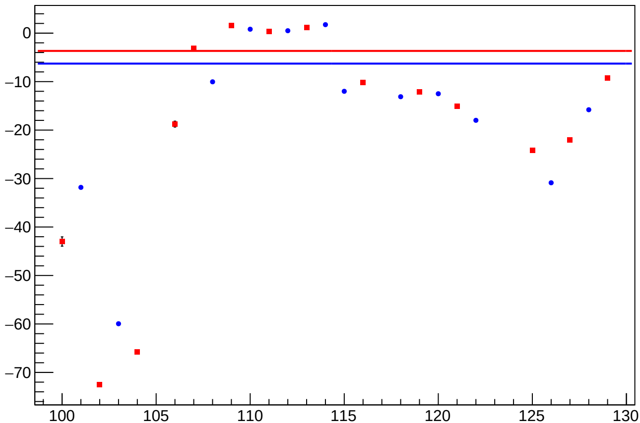
reg_asym_bcm_an_us_an_ds_avg_diff_bpm1X_slope vs Slug, Sign Corrected
