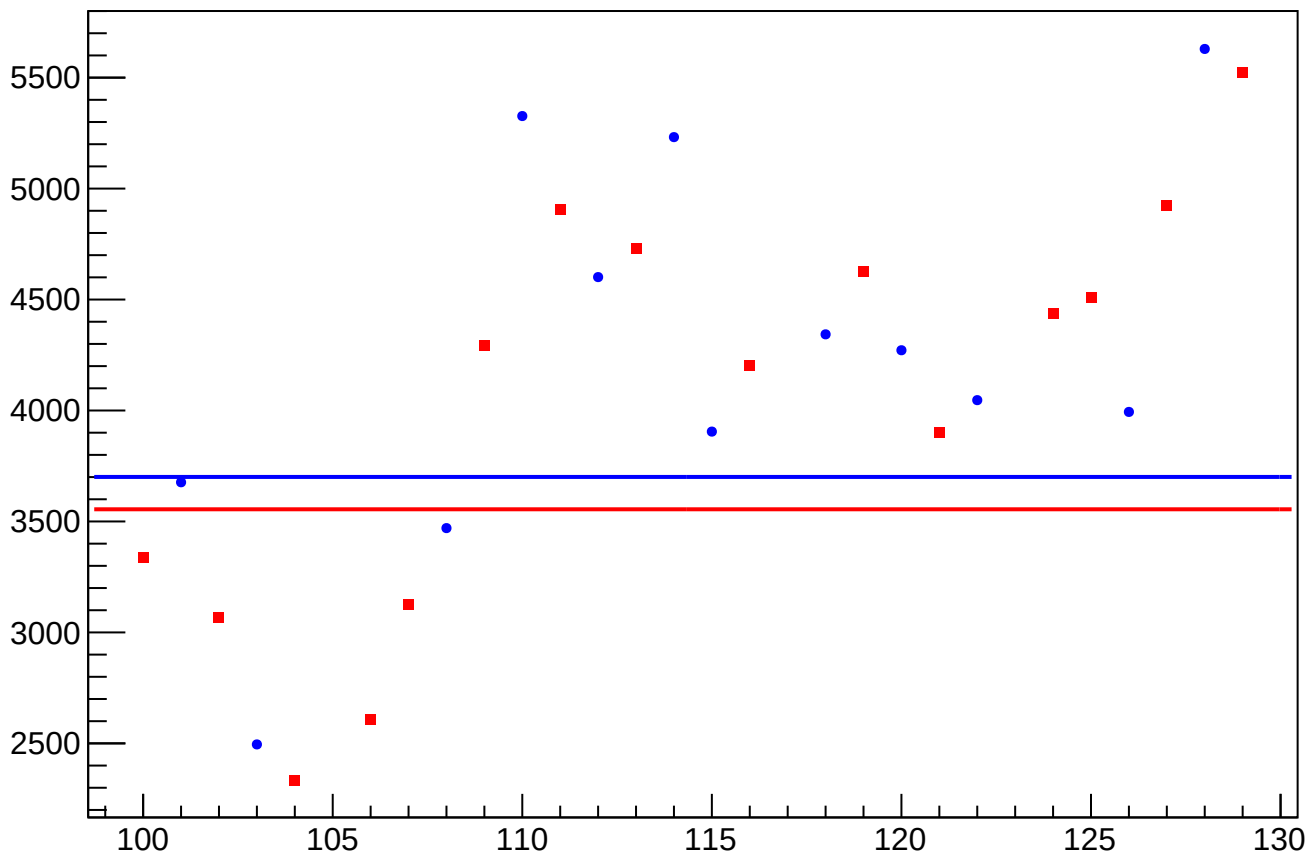
asym_atr_dd_eigen_cor_correction_rms vs Slug, Sign Corrected
