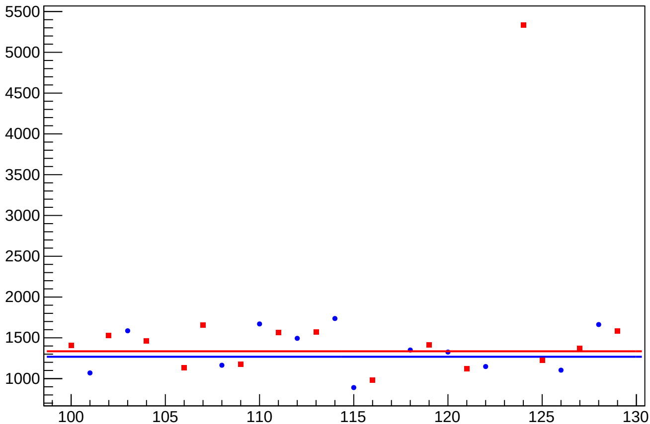
asym_atl_dd_atr_dd_dd_eigen_dit_correction_rms vs Slug, Sign Corrected
