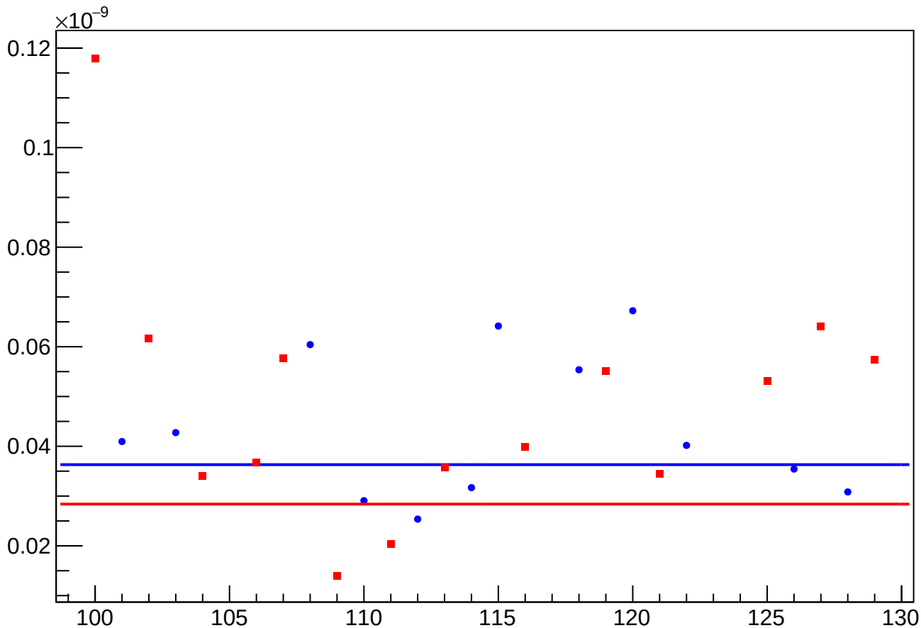
asym_us_dd_atlr_dd_avg_eigen_cor_vs_cor_diff_rms vs Slug, Sign Corrected
