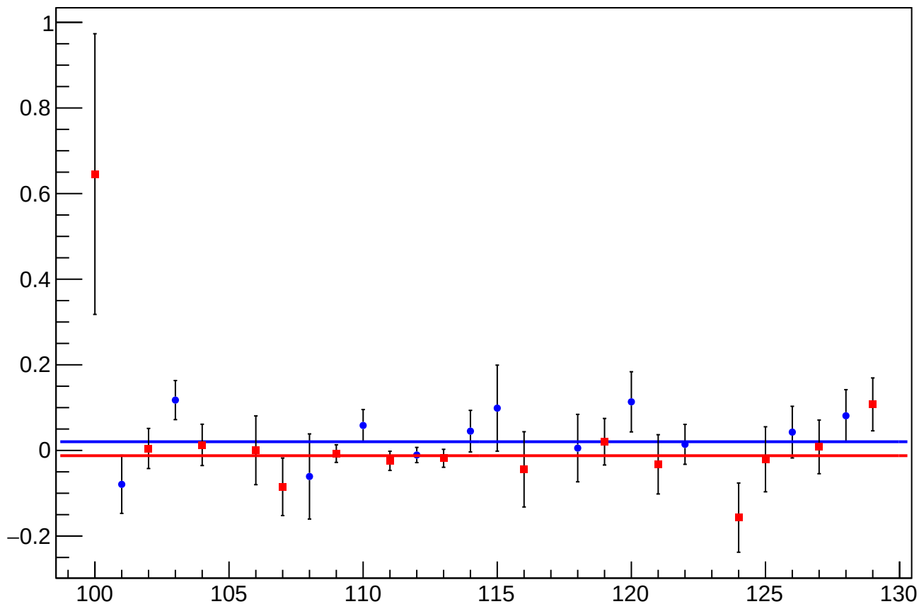
asym_sam_48_dd_dit_vs_cor_diff_mean vs Slug, Sign Corrected
