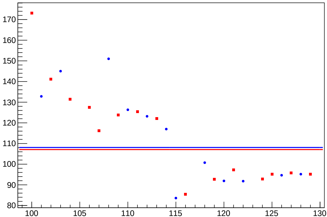
eigen_dit_asym_sam_24_68_dd_rms vs Slug, Sign Corrected
