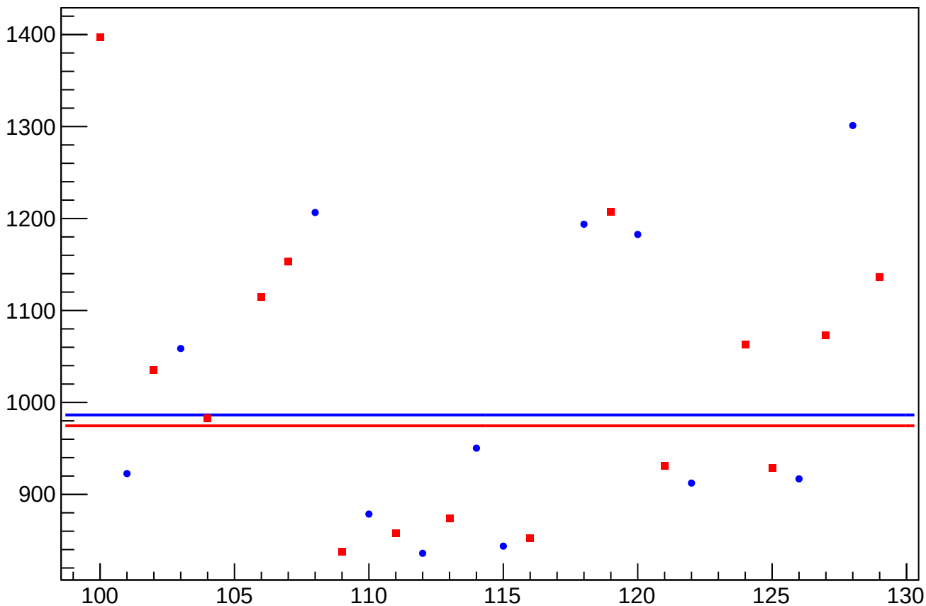
asym_sam_12345678_avg_dit_correction_rms vs Slug, Sign Corrected
