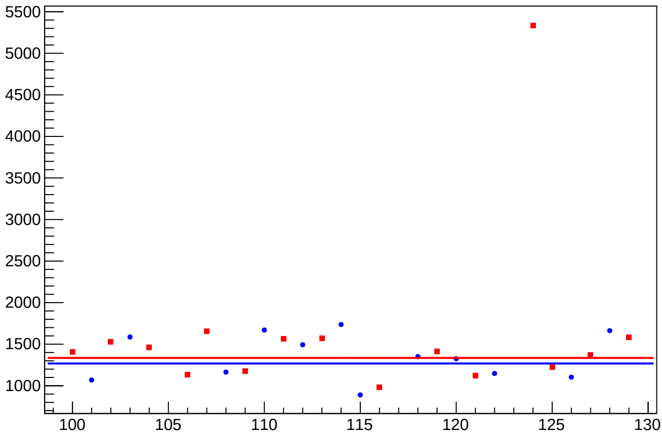
asym_atl_dd_atr_dd_dd_dit_correction_rms vs Slug, Sign Corrected
