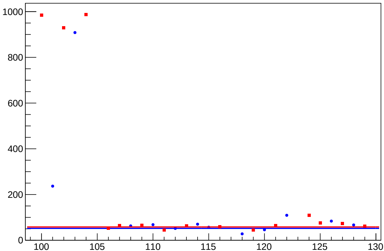
asym_atr1_eigen_dit_vs_cor_diff_rms vs Slug, Sign Corrected
