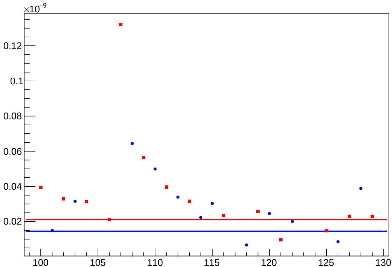
asym_usl_eigen_cor_vs_cor_diff_rms vs Slug, Sign Corrected
