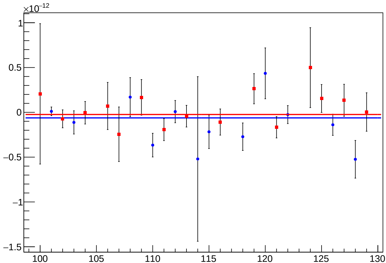
asym_sam_24_68_dd_reg_vs_cor_diff_mean vs Slug, Sign Corrected
