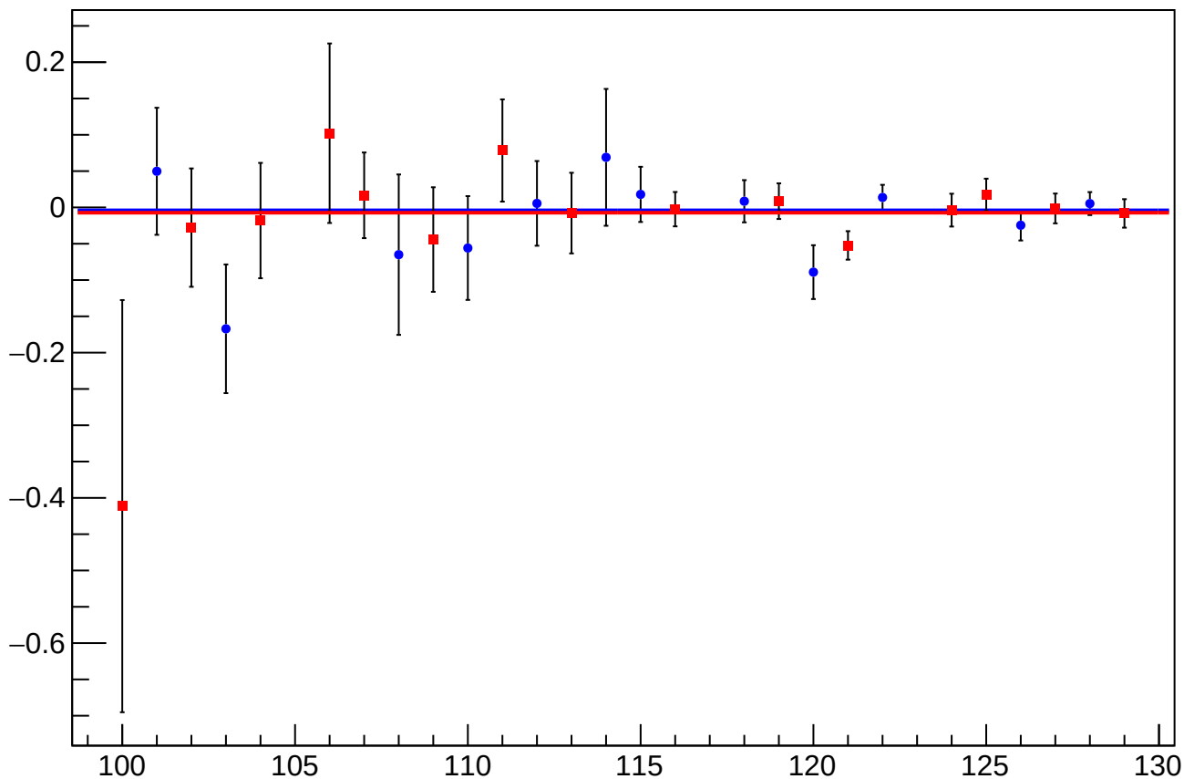
asym_sam1_eigen_dit_vs_cor_diff_mean vs Slug, Sign Corrected
