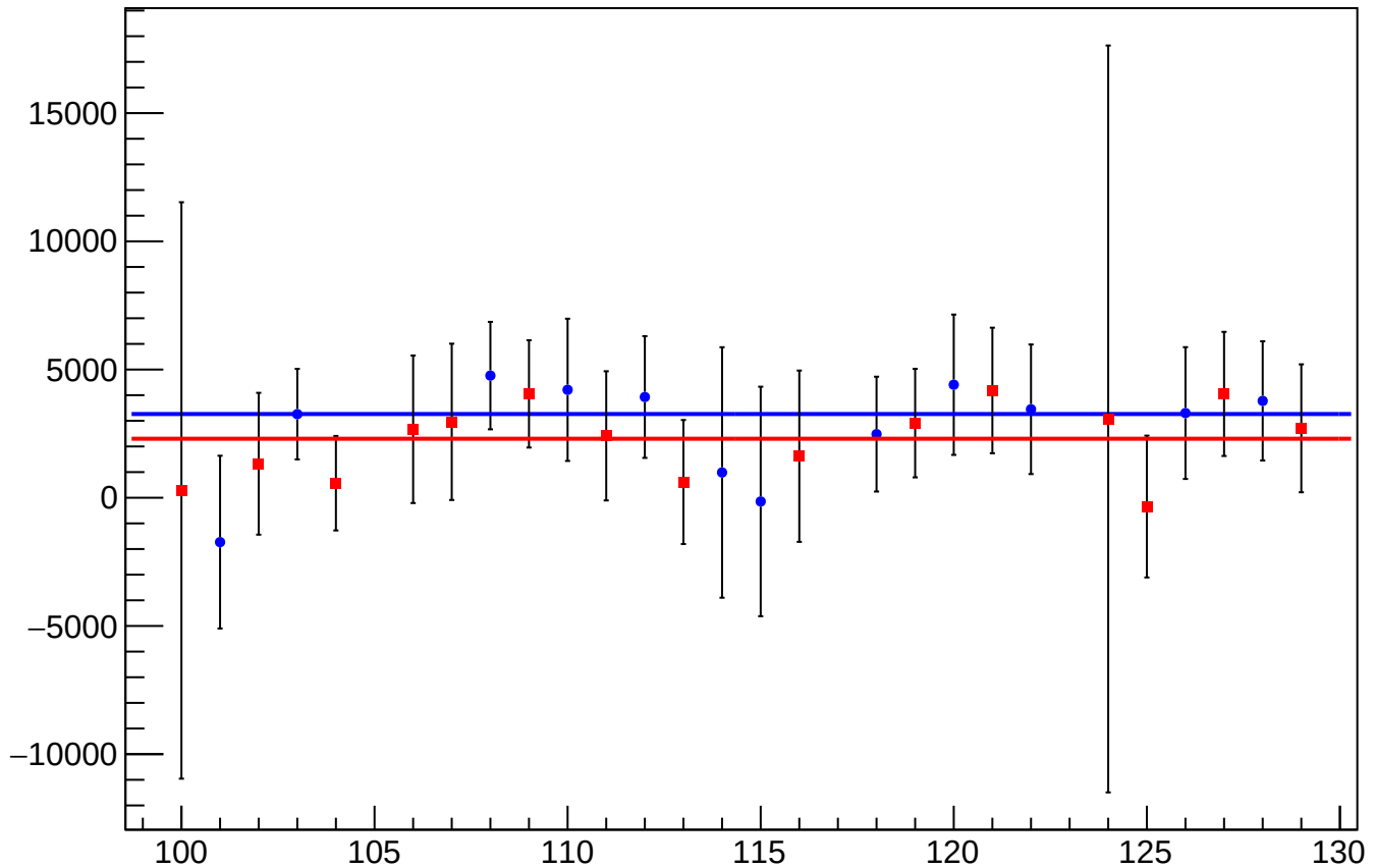
cor_asym_at2_avg_mean vs Slug, Sign Corrected
