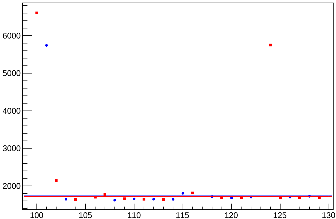
eigen_cor_asym_atr1l2_dd_rms vs Slug, Sign Corrected
