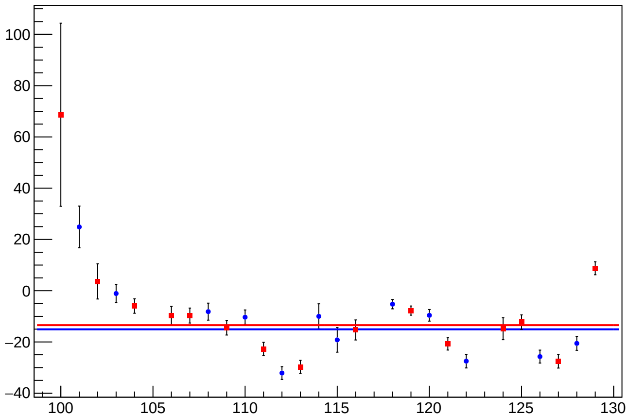
reg_asym_usr_atr1_avg_diff_bpm4eY_slope vs Slug, Sign Corrected
