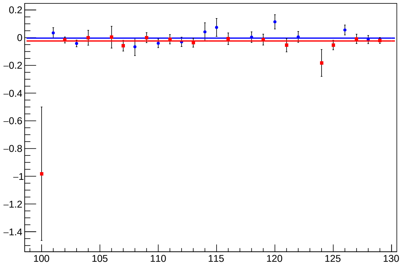
asym_sam_1357_avg_eigen_dit_vs_cor_diff_mean vs Slug, Sign Corrected
