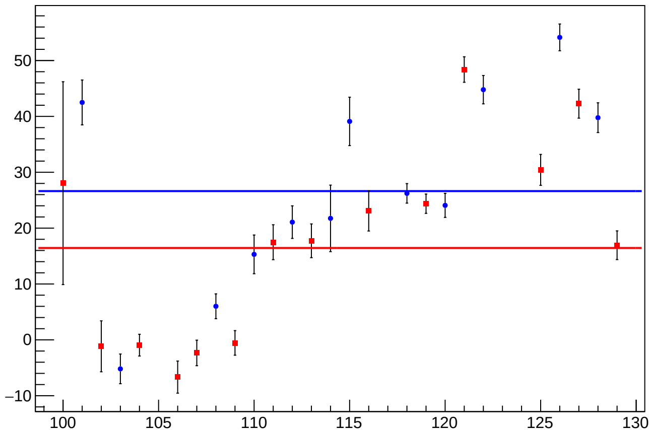
reg_asym_us_dd_at2lr_dd_dd_diff_bpm4eY_slope vs Slug, Sign Corrected
