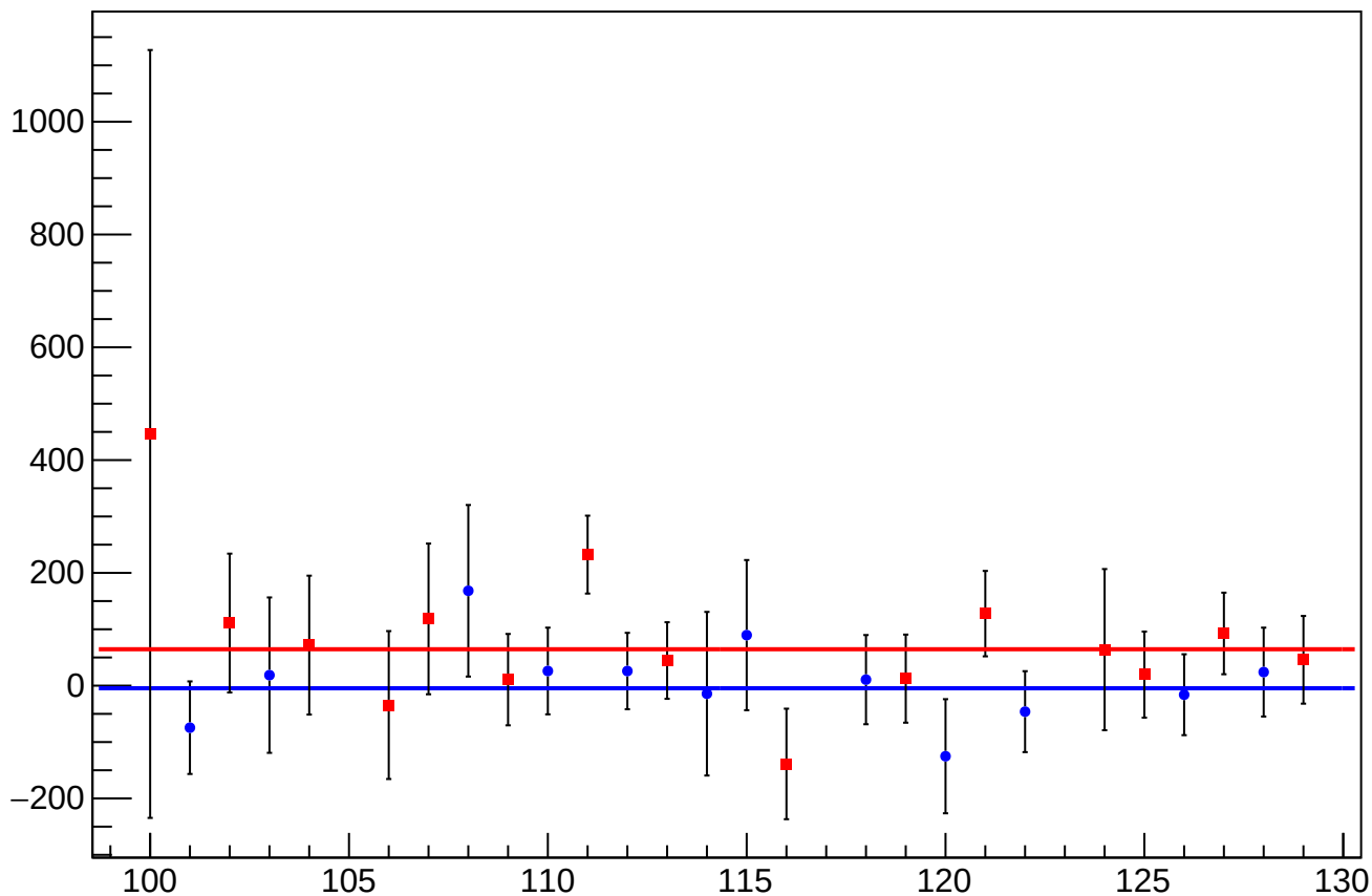
eigen_dit_asym_sam_15_37_dd_mean vs Slug, Sign Corrected
