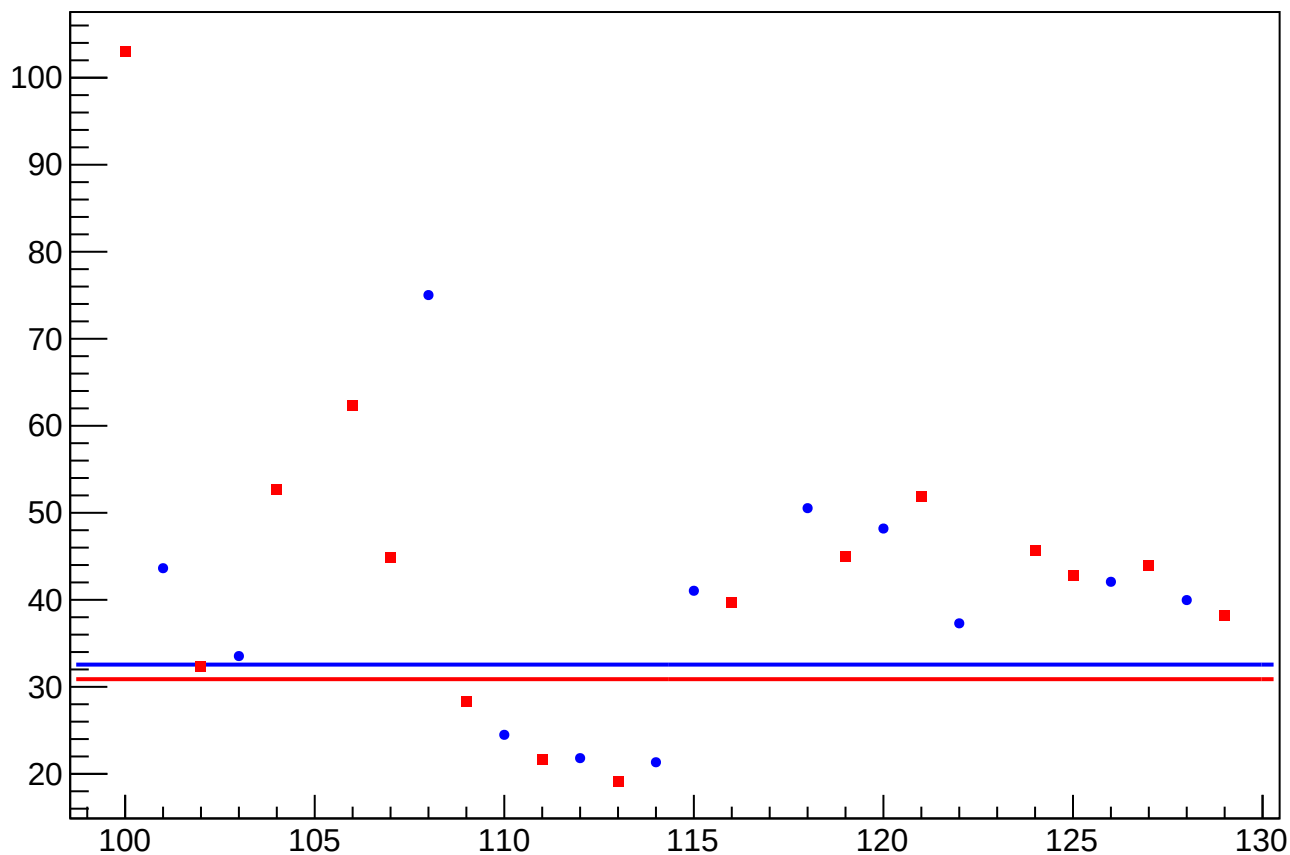
asym_sam_3748_avg_dit_vs_eigen_cor_diff_rms vs Slug, Sign Corrected
