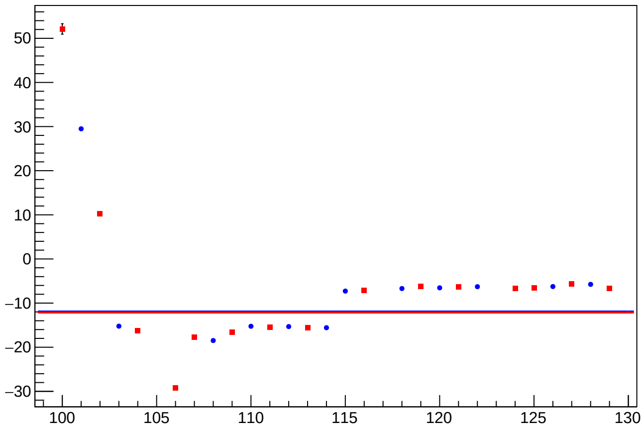
reg_asym_usr_atr1_dd_diff_bpm12X_slope vs Slug, Sign Corrected
