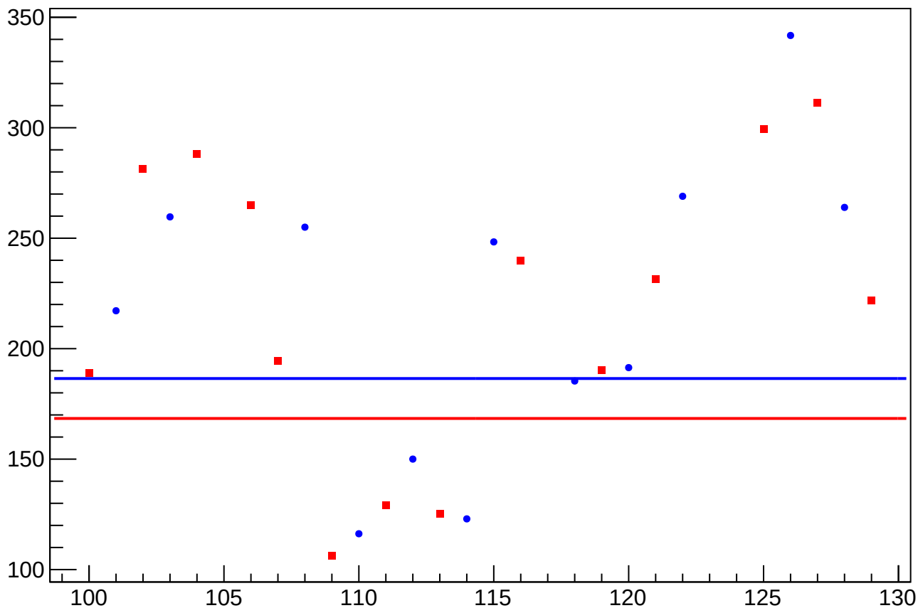
asym_bcm_dg_ds_an_ds_avg_rms vs Slug, Sign Corrected
