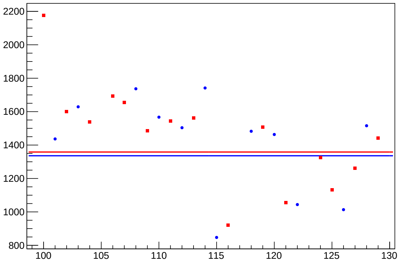
asym_sam_3726_avg_dit_correction_rms vs Slug, Sign Corrected
