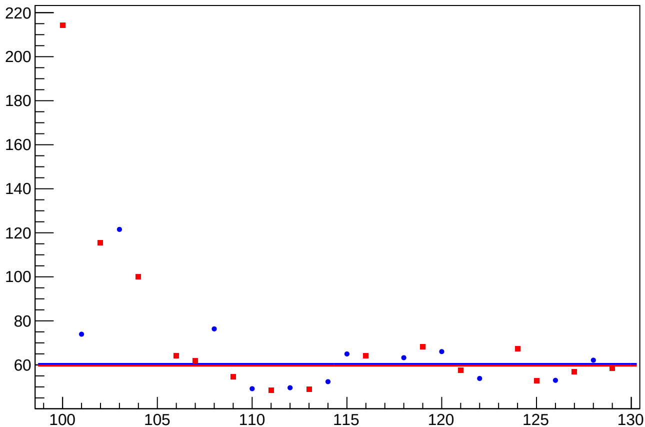
eigen_dit_asym_sam_1357_avg_rms vs Slug, Sign Corrected
