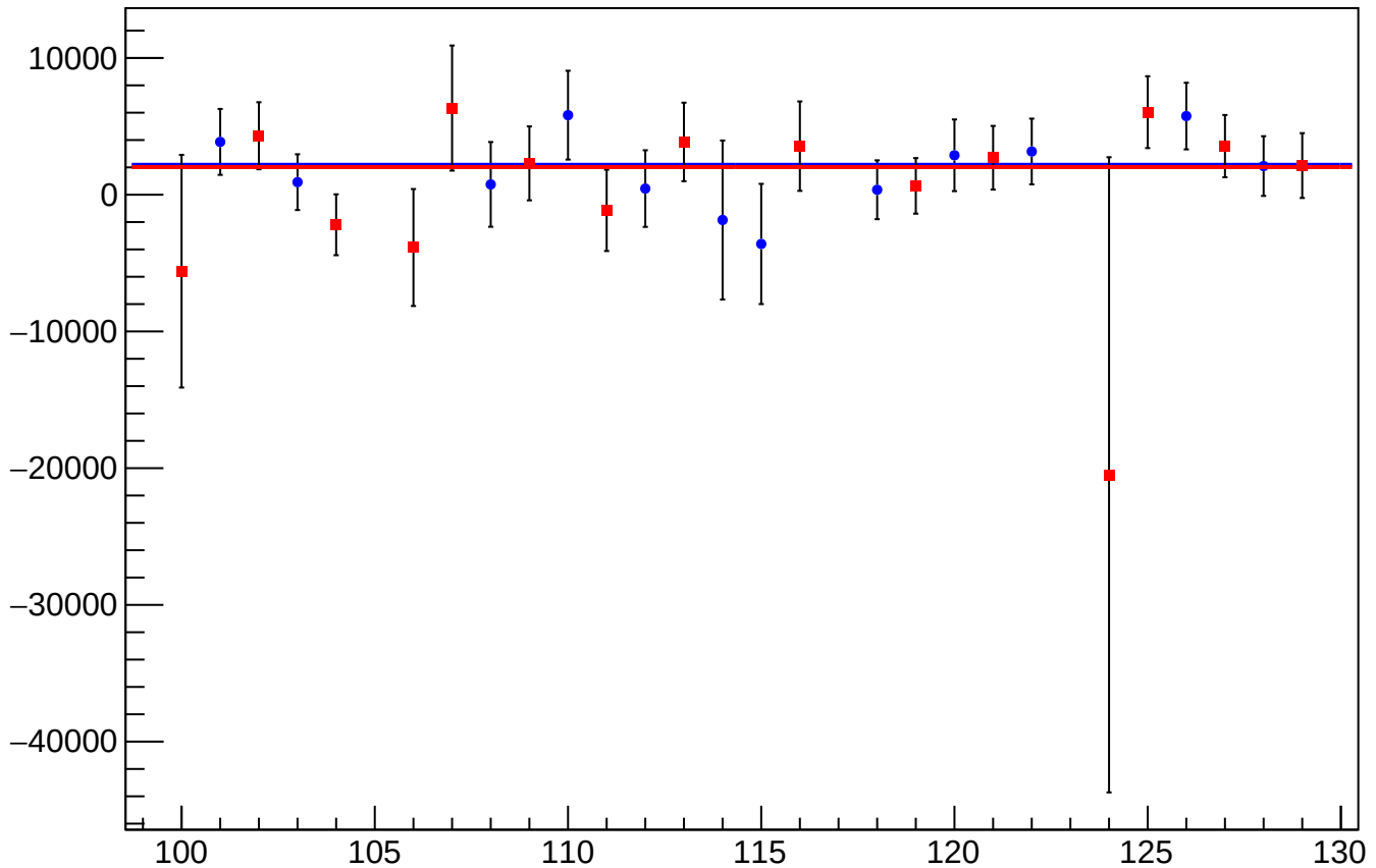
eigen_cor_asym_atl_avg_mean vs Slug, Sign Corrected
