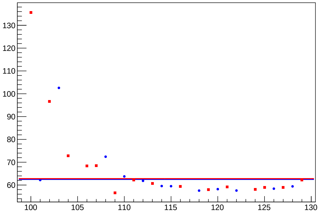
eigen_cor_asym_sam8_rms vs Slug, Sign Corrected
