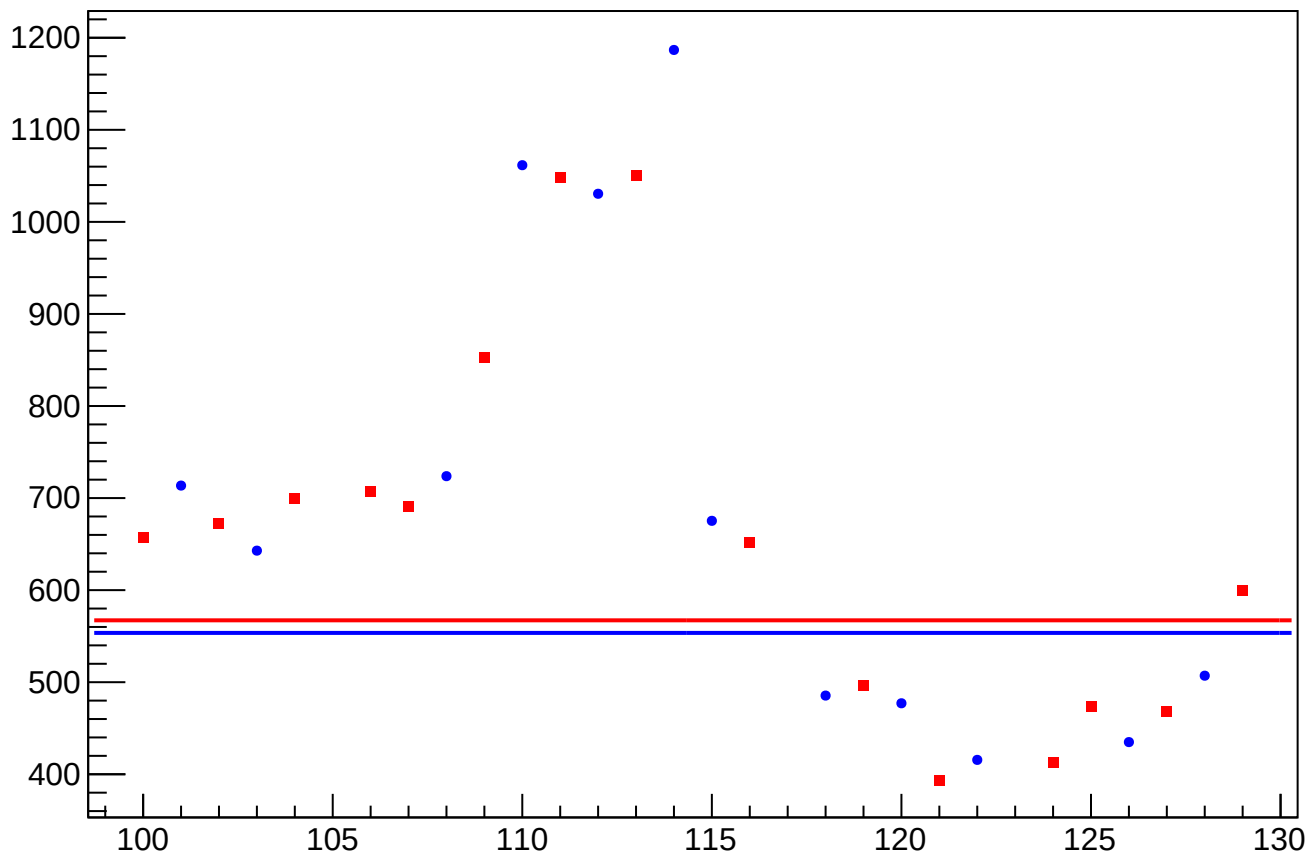
asym_sam1_eigen_dit_correction_rms vs Slug, Sign Corrected
