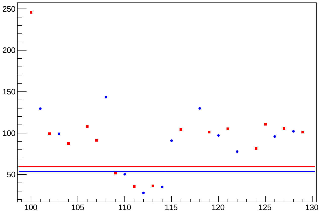
asym_sam4_dit_vs_cor_diff_rms vs Slug, Sign Corrected
