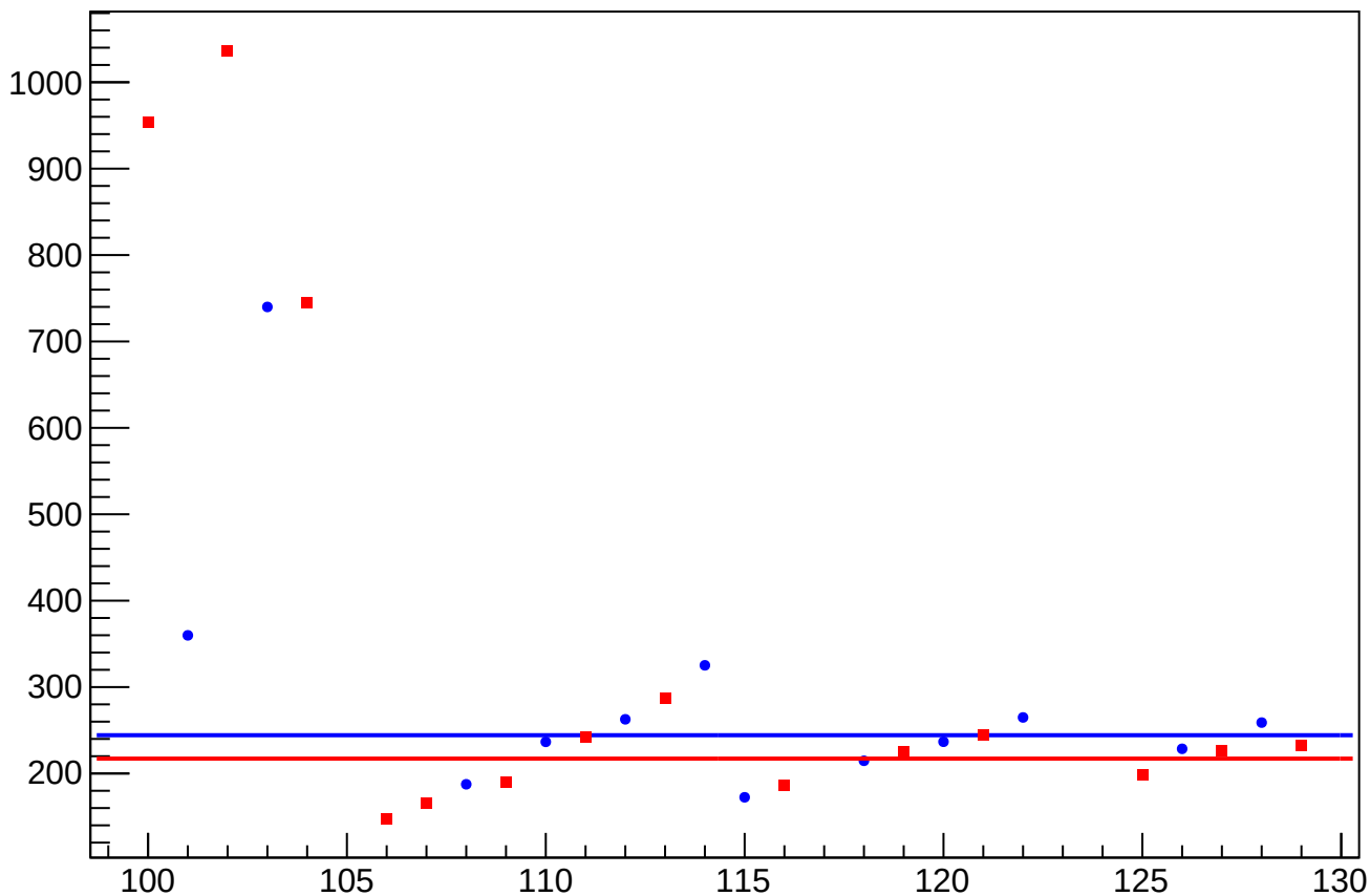
asym_us_avg_at2lr_avg_dd_eigen_dit_vs_cor_diff_rms vs Slug, Sign Corrected
