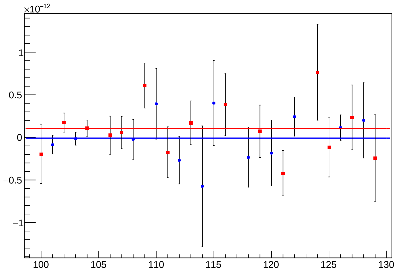
asym_atr_dd_eigen_cor_vs_cor_diff_mean vs Slug, Sign Corrected
