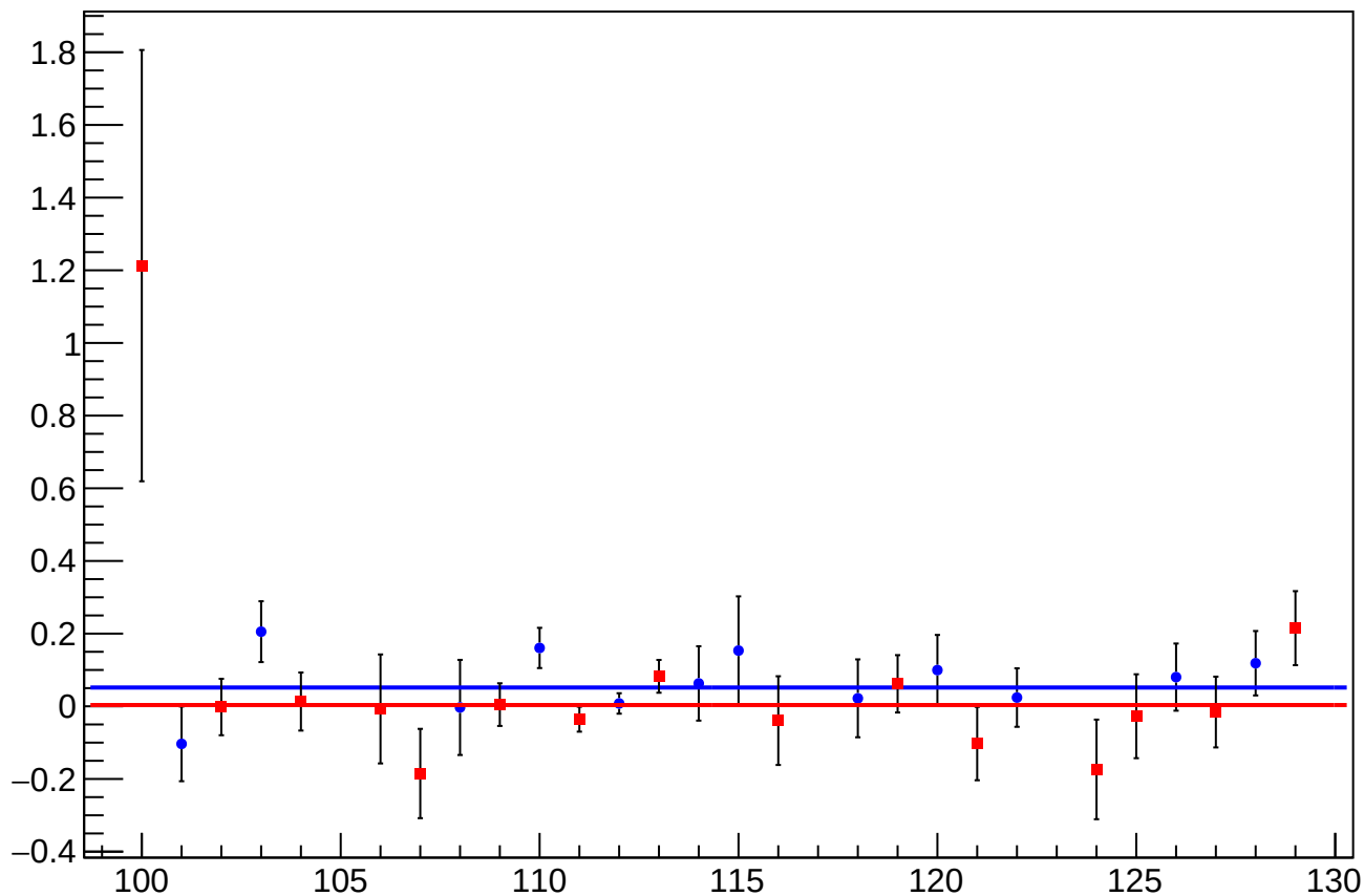
asym_sam_48_avg_dit_vs_cor_diff_mean vs Slug, Sign Corrected
