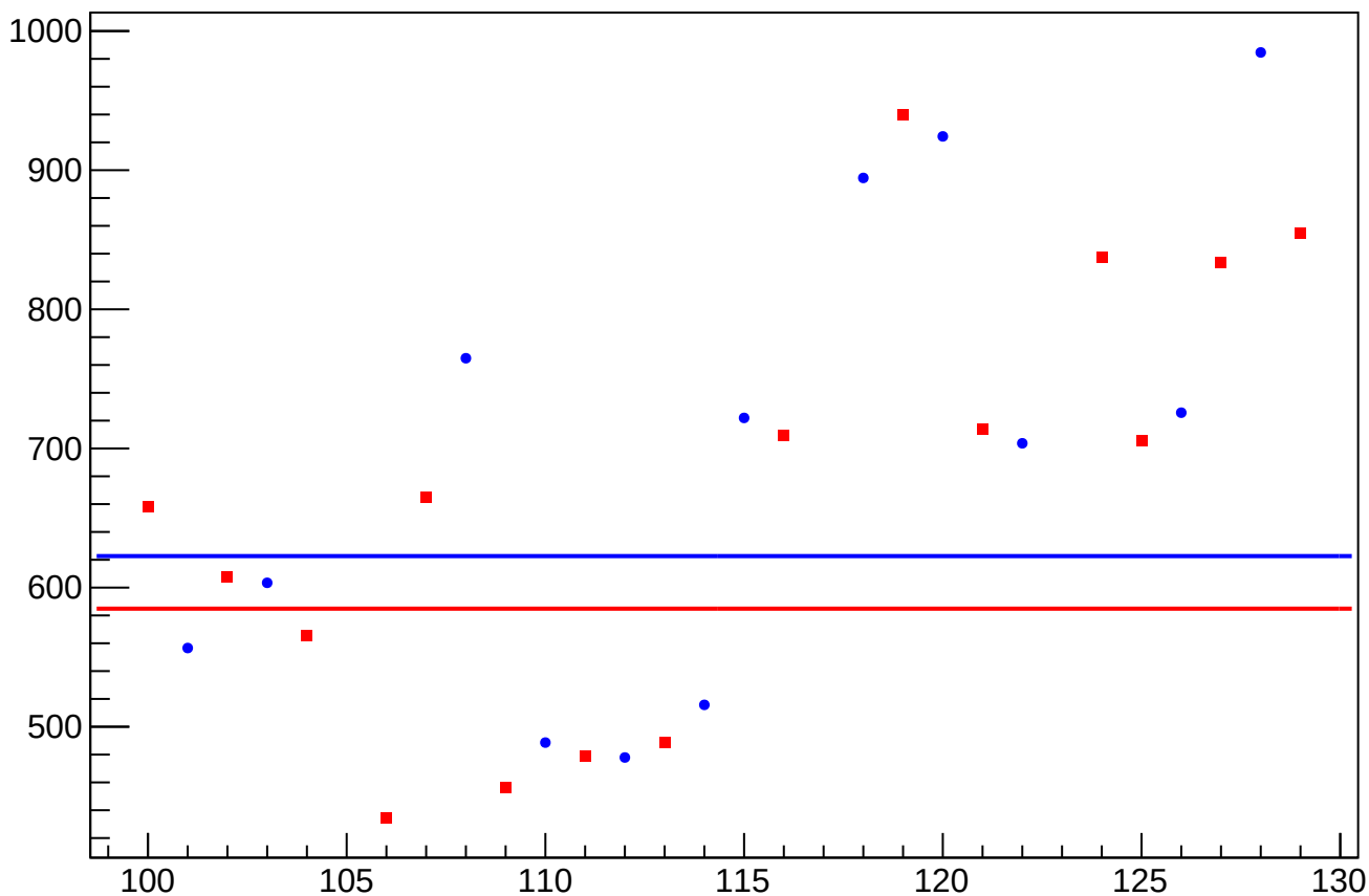
asym_sam_15_48_dd_cor_correction_rms vs Slug, Sign Corrected
