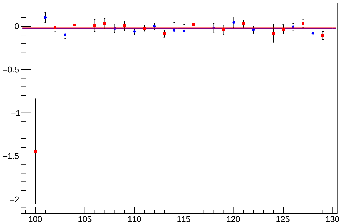
asym_sam_37_48_dd_dit_vs_cor_diff_mean vs Slug, Sign Corrected
