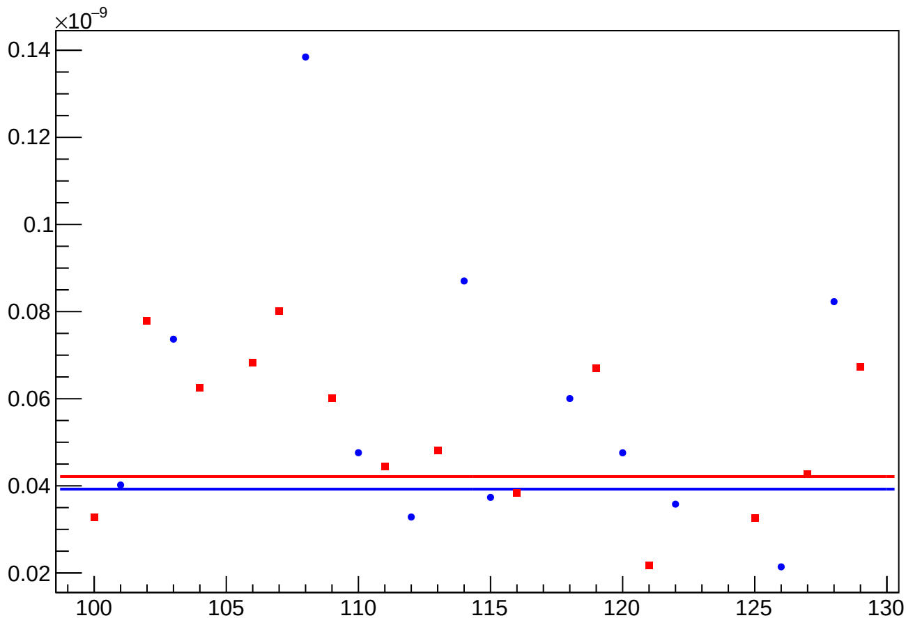
asym_us_dd_at1lr_dd_dd_eigen_cor_vs_cor_diff_rms vs Slug, Sign Corrected
