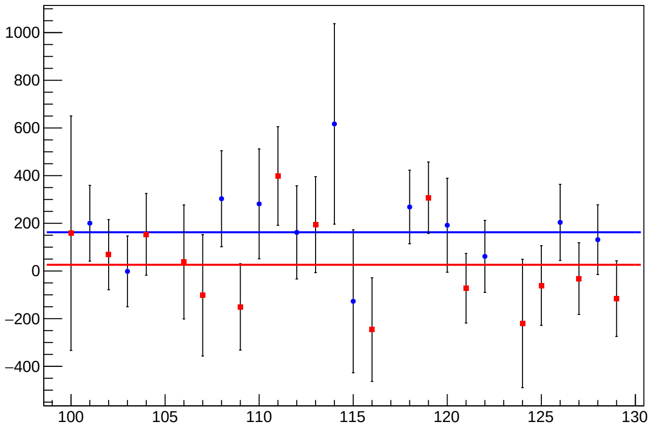
cor_asym_sam_26_48_dd_mean vs Slug, Sign Corrected
