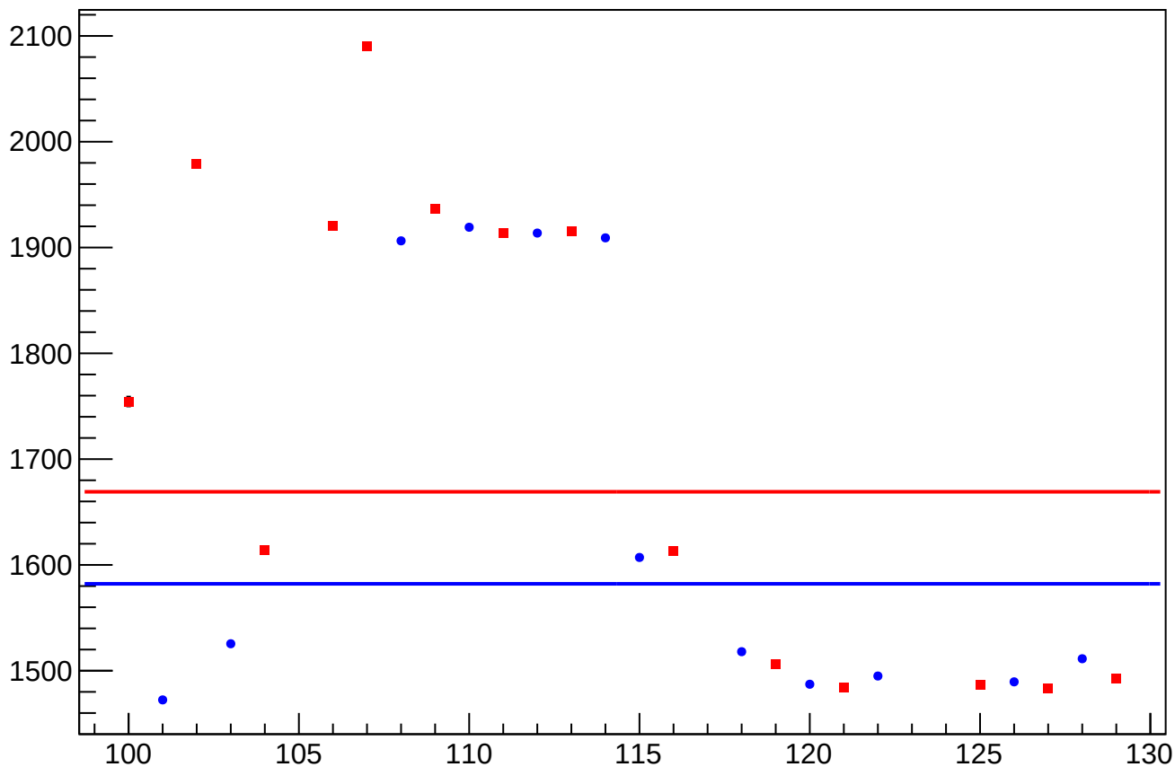
eigen_dit_asym_usl_atl1_avg_rms vs Slug, Sign Corrected
