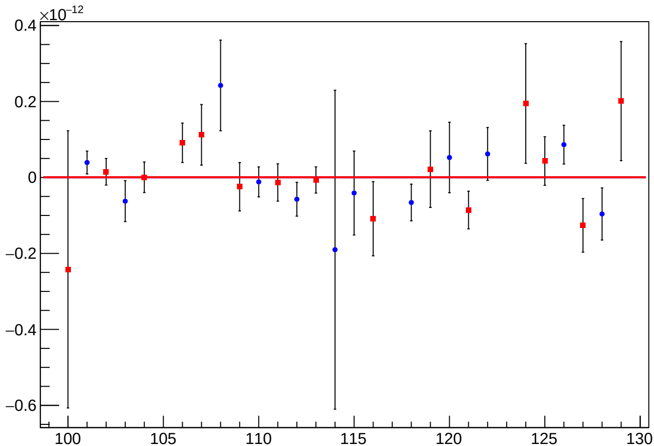
asym_sam_37_dd_reg_vs_cor_diff_mean vs Slug, Sign Corrected
