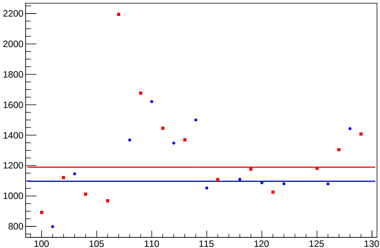
asym_us_avg_cor_correction_rms vs Slug, Sign Corrected
