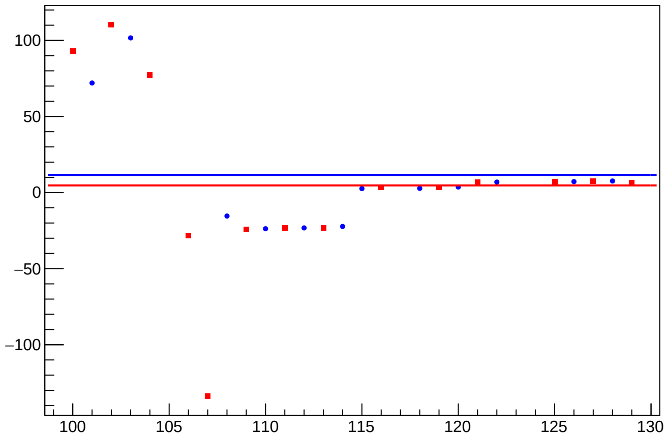
reg_asym_us_dd_at1lr_dd_avg_diff_bpm12X_slope vs Slug, Sign Corrected
