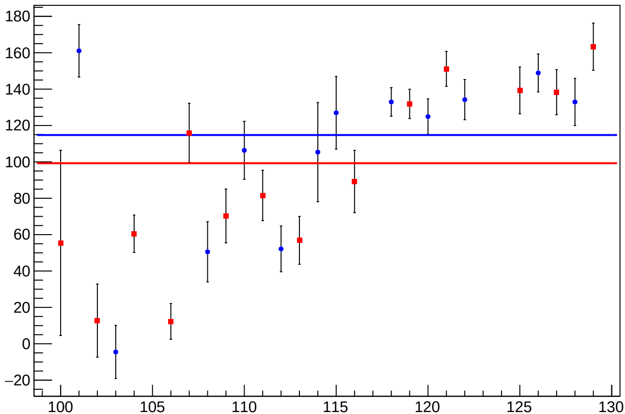
reg_asym_us_avg_at2lr_avg_avg_diff_bpm4eY_slope vs Slug, Sign Corrected
