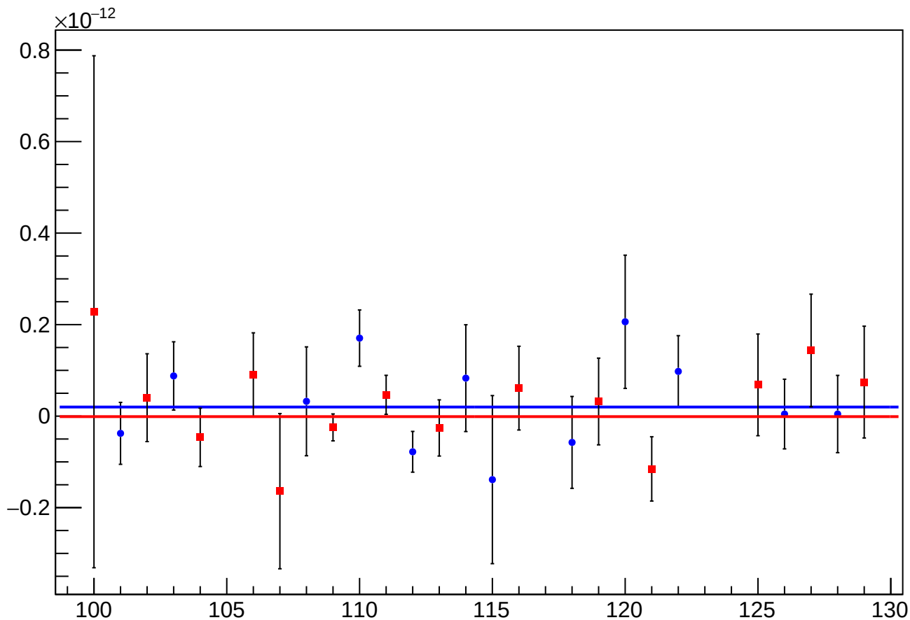
asym_us_dd_atlr_dd_avg_eigen_cor_vs_cor_diff_mean vs Slug, Sign Corrected
