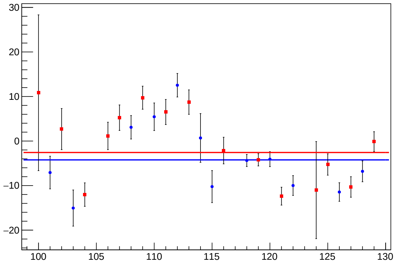
reg_asym_at1_dd_at2_dd_avg_diff_bpm4aY_slope vs Slug, Sign Corrected
