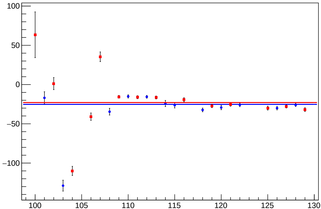
reg_asym_us_avg_at1lr_avg_dd_diff_bpm1X_slope vs Slug, Sign Corrected
