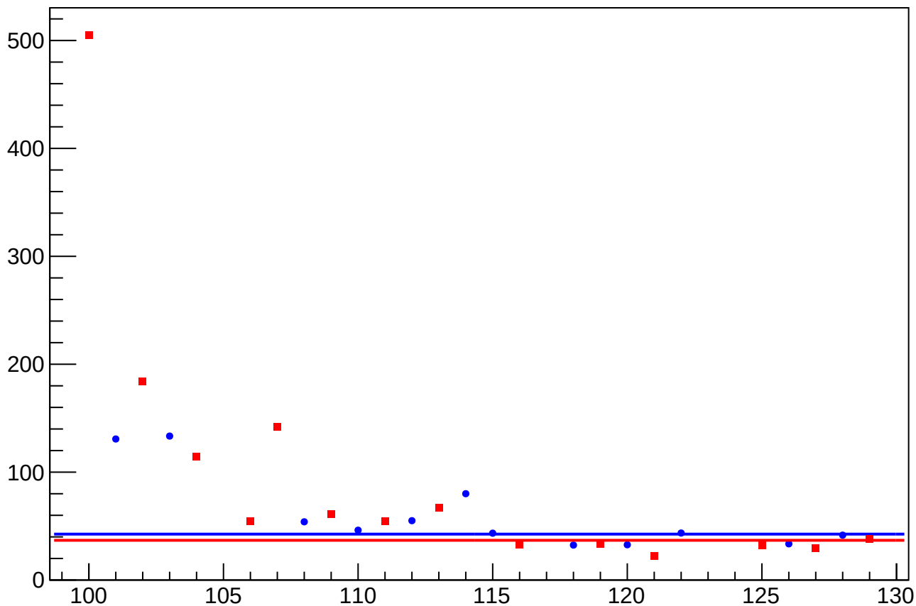
asym_us_dd_at1lr_dd_dd_eigen_dit_vs_eigen_cor_diff_rms vs Slug, Sign Corrected
