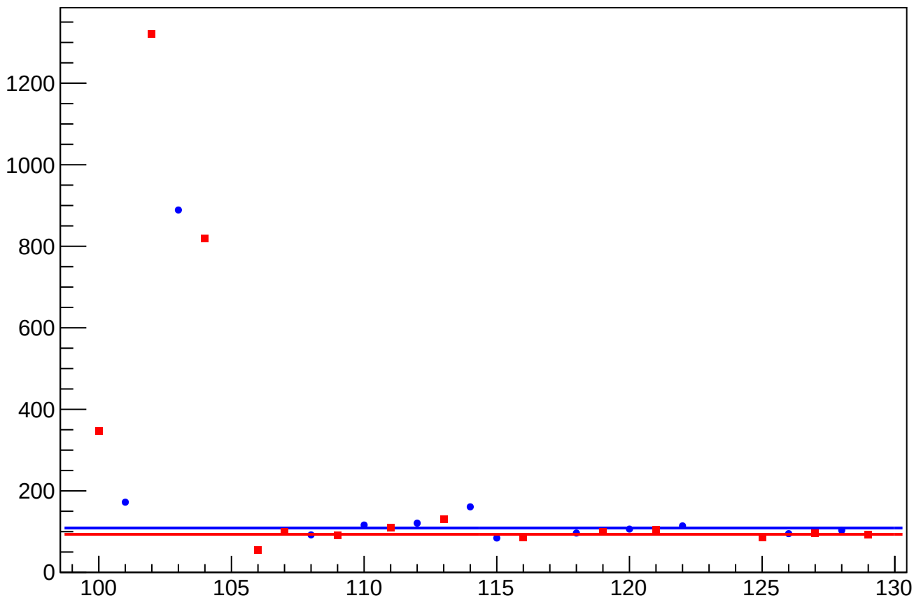
asym_us_avg_atlr_avg_dd_eigen_dit_vs_cor_diff_rms vs Slug, Sign Corrected
