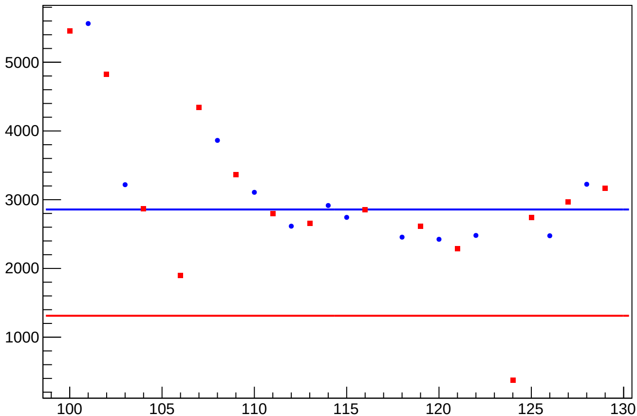
asym_atr1l2_avg_reg_correction_rms vs Slug, Sign Corrected
