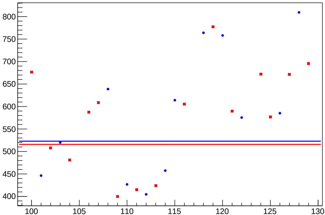
asym_sam_1357_avg_eigen_dit_correction_rms vs Slug, Sign Corrected
