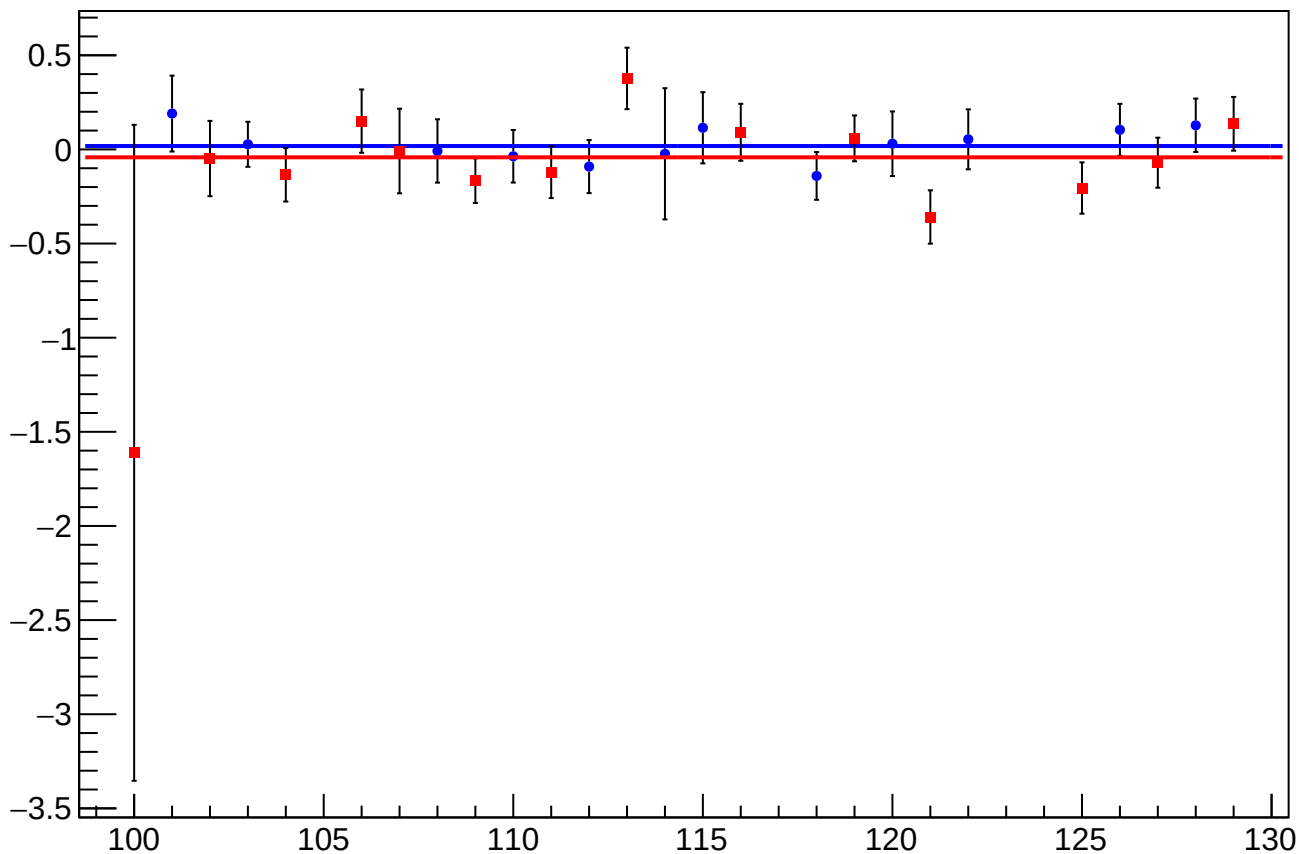
asym_usl_atl2_dd_dit_vs_cor_diff_mean vs Slug, Sign Corrected
