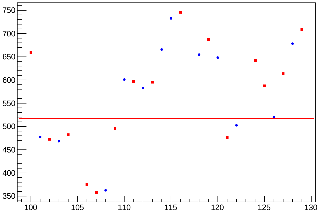
asym_sam_13_57_dd_dit_correction_rms vs Slug, Sign Corrected
