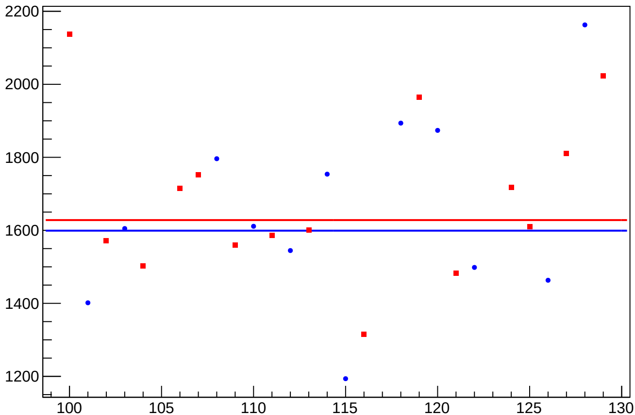
asym_sam_24_68_dd_eigen_dit_correction_rms vs Slug, Sign Corrected
