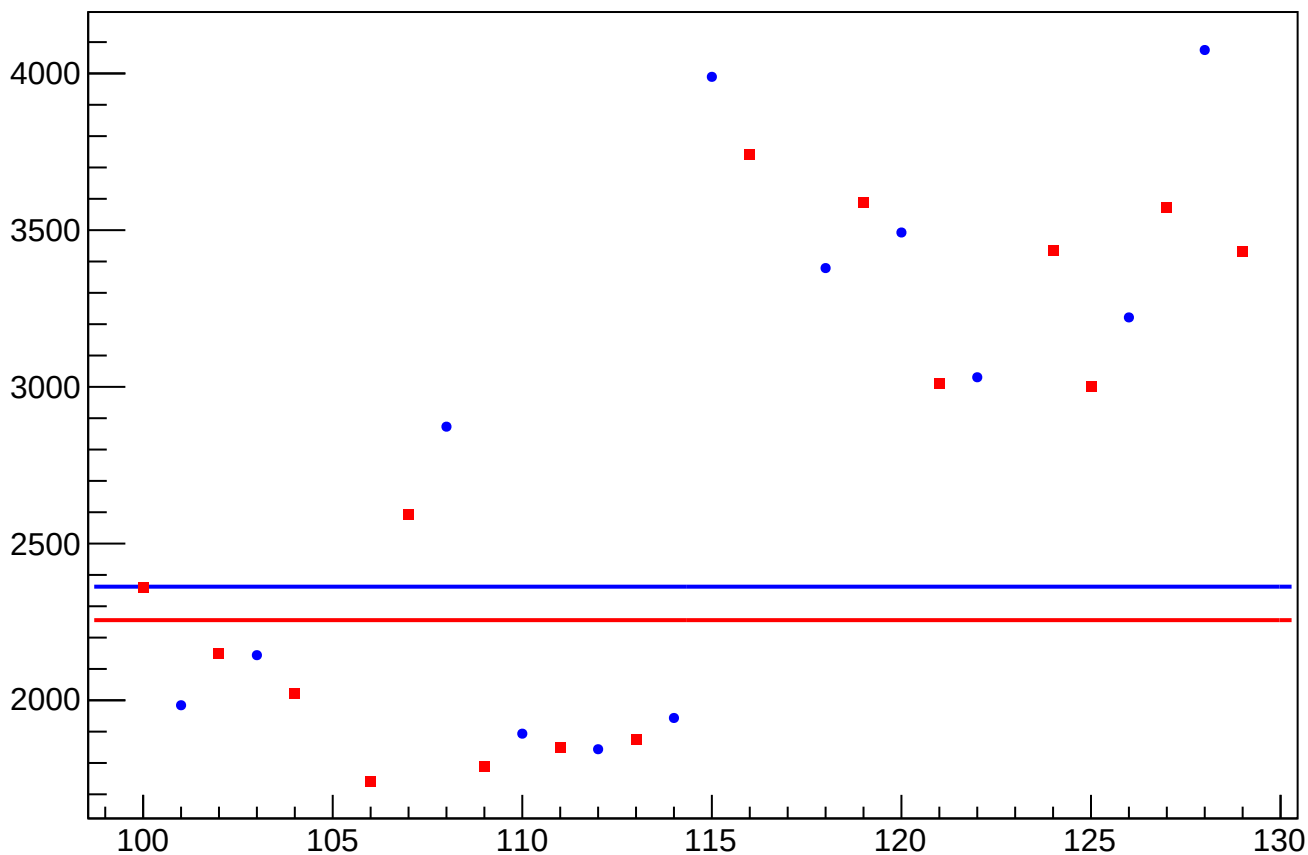
asym_sam4_eigen_cor_correction_rms vs Slug, Sign Corrected
