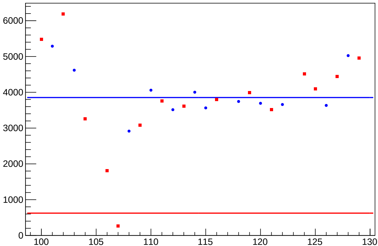
asym_atl1r2_dd_eigen_cor_correction_rms vs Slug, Sign Corrected
