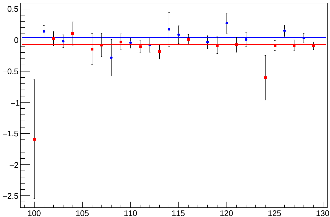
asym_sam3_dit_vs_eigen_cor_diff_mean vs Slug, Sign Corrected
