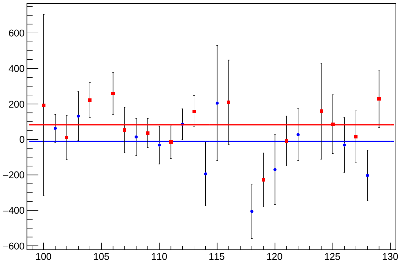
cor_asym_sam_1548_avg_mean vs Slug, Sign Corrected
