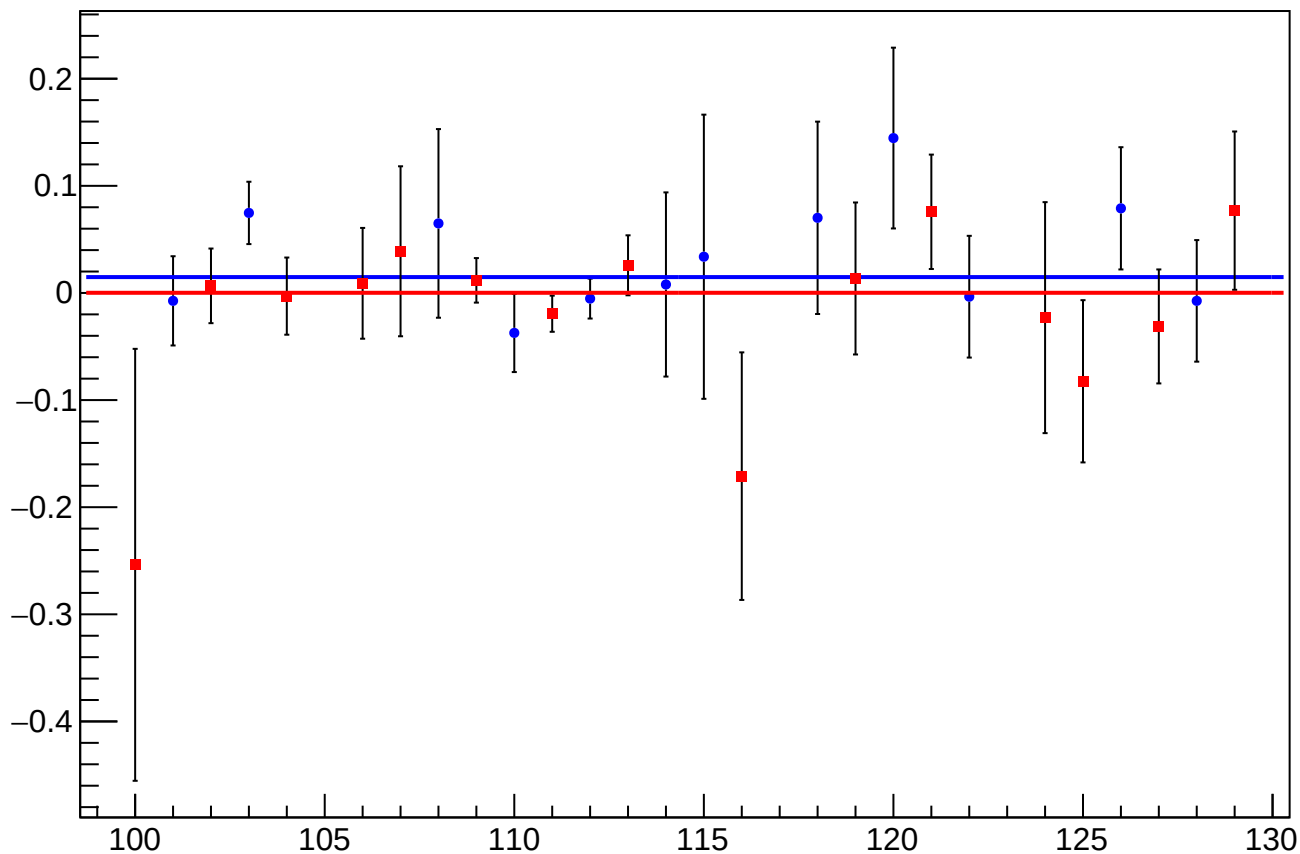
asym_sam5_eigen_dit_vs_eigen_cor_diff_mean vs Slug, Sign Corrected
