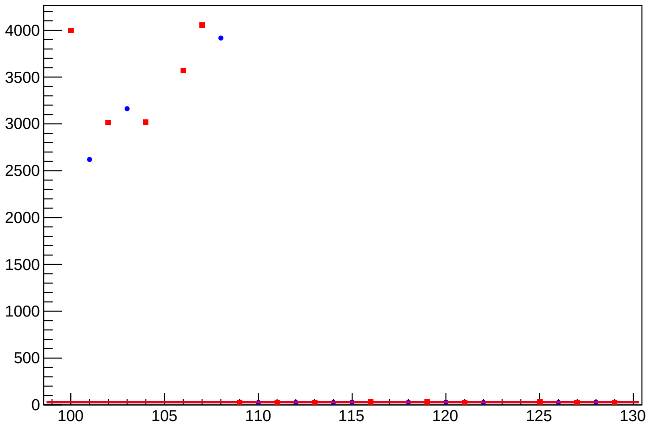
asym_bcm_cav4cQ_an_ds_dd_rms vs Slug, Sign Corrected
