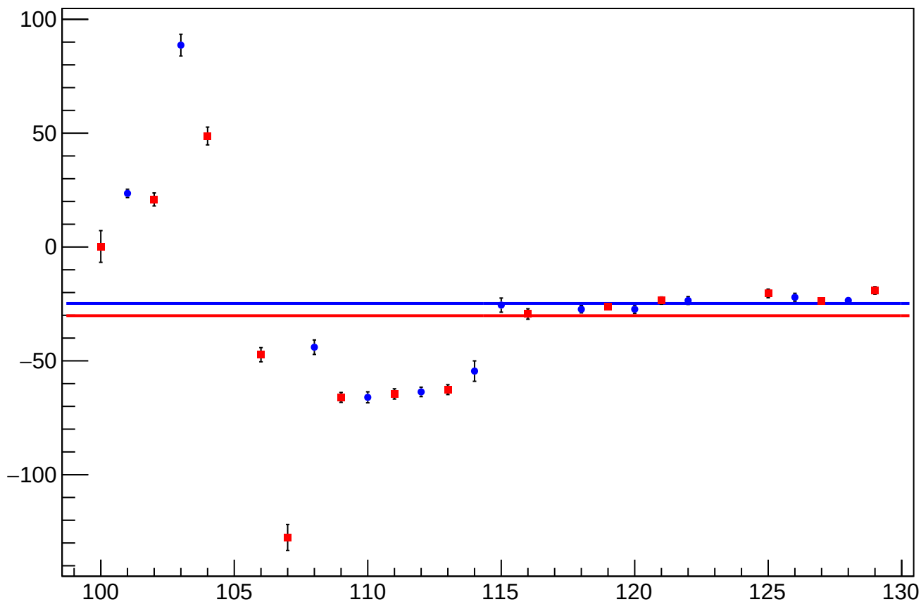
reg_asym_usl_atl1_dd_diff_bpm4eX_slope vs Slug, Sign Corrected
