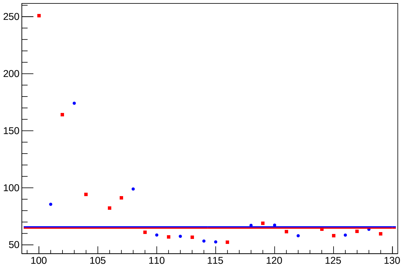
cor_asym_sam_37_dd_rms vs Slug, Sign Corrected
