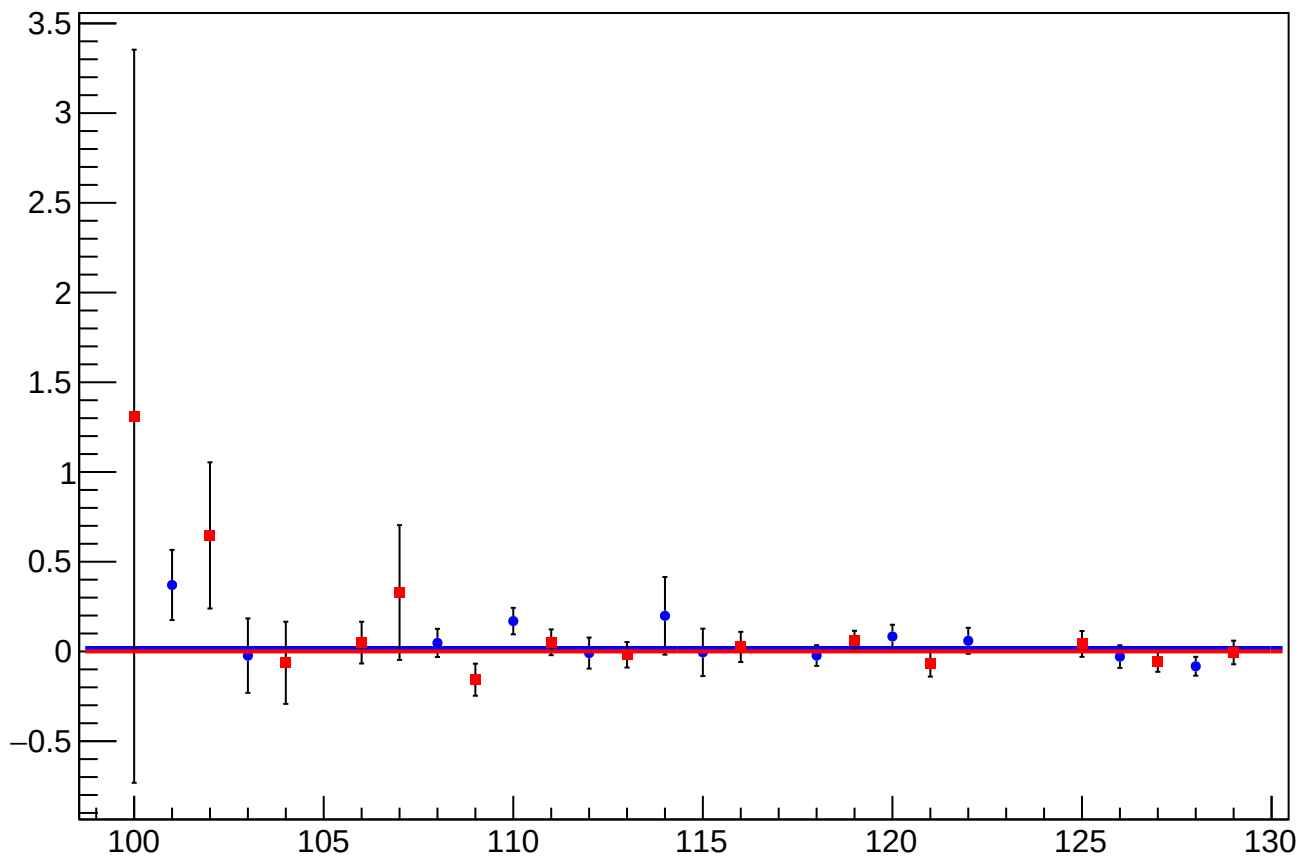
asym_us_dd_at1lr_dd_avg_eigen_dit_vs_eigen_cor_diff_mean vs Slug, Sign Corrected
