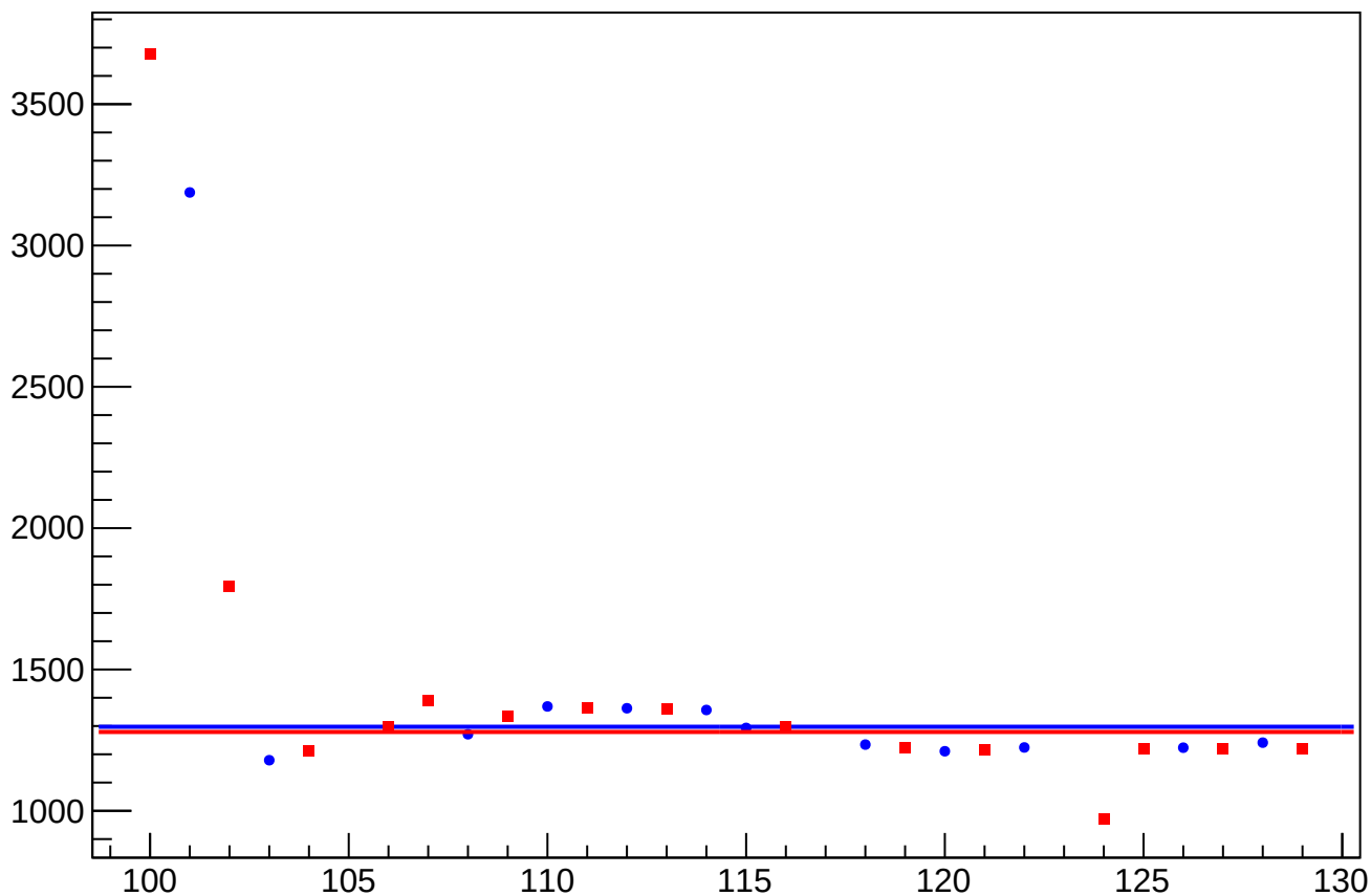
dit_asym_atl1r2_dd_atl2r1_dd_avg_rms vs Slug, Sign Corrected
