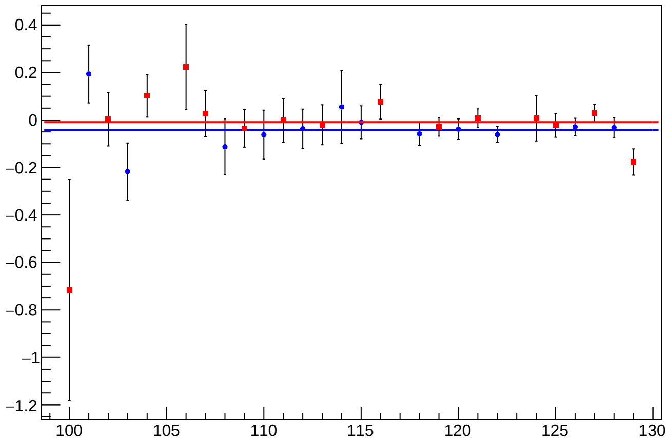
asym_sam_26_48_dd_eigen_dit_vs_eigen_cor_diff_mean vs Slug, Sign Corrected
