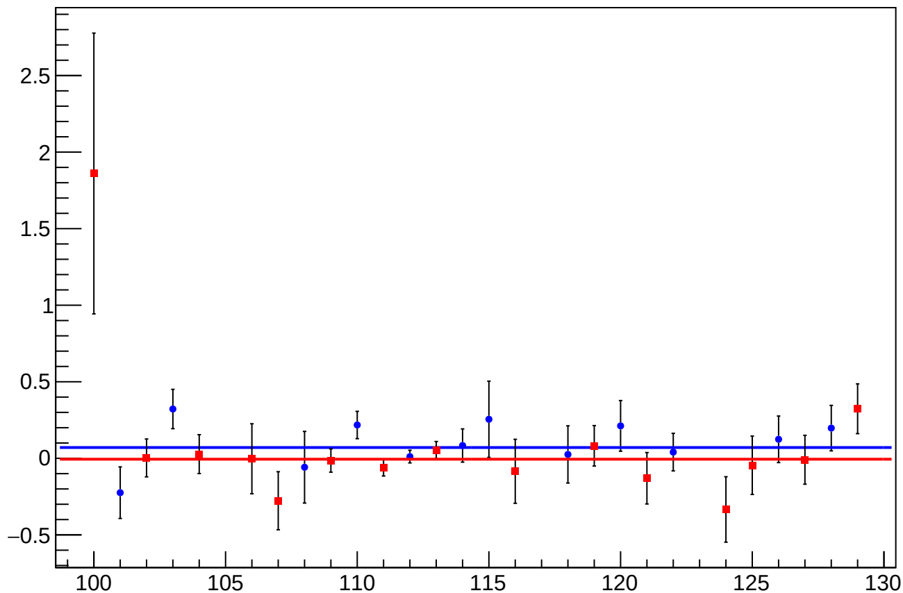
asym_sam4_eigen_dit_vs_eigen_cor_diff_mean vs Slug, Sign Corrected
