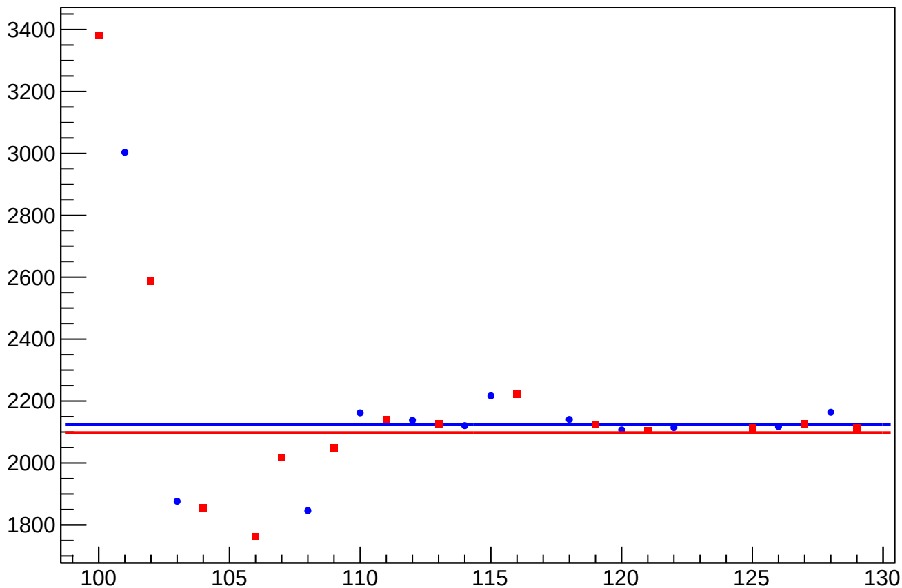
eigen_cor_asym_us_avg_at2lr_avg_avg_rms vs Slug, Sign Corrected
