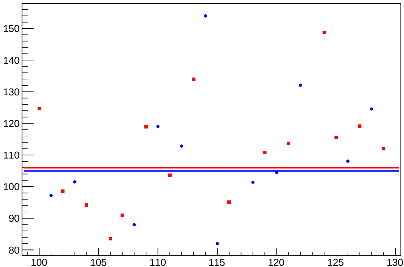
asym_usr_eigen_dit_vs_overload_cor_diff_rms vs Slug, Sign Corrected
