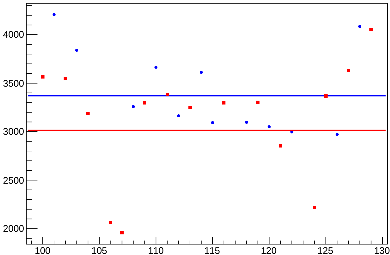
asym_at1_avg_at2_avg_dd_eigen_cor_correction_rms vs Slug, Sign Corrected
