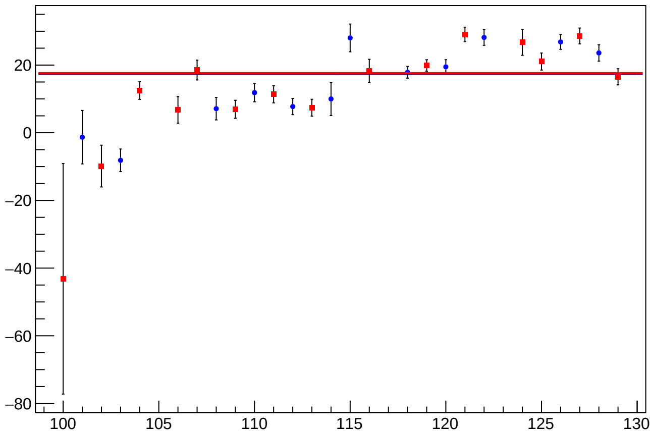
reg_asym_usr_atr1_dd_diff_bpm4eY_slope vs Slug, Sign Corrected
