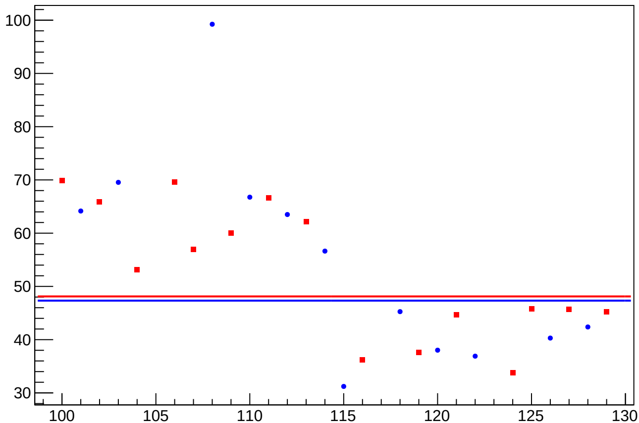
asym_sam_24_68_dd_eigen_dit_vs_eigen_cor_diff_rms vs Slug, Sign Corrected
