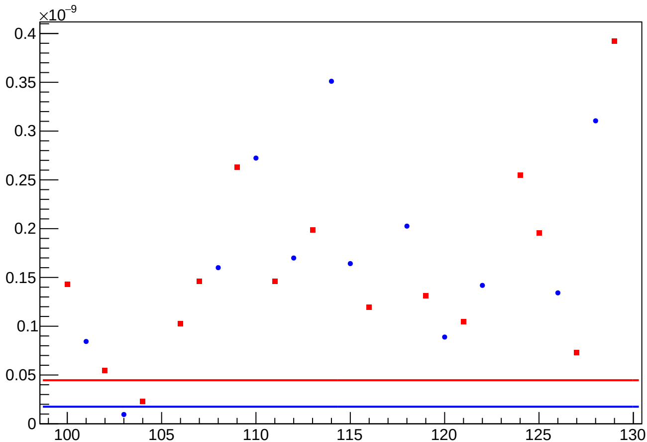
asym_atl1r2_avg_eigen_cor_vs_cor_diff_rms vs Slug, Sign Corrected
