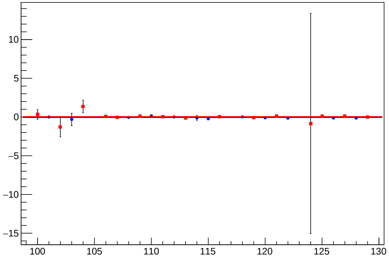
asym_at2_dd_eigen_dit_vs_eigen_cor_diff_mean vs Slug, Sign Corrected
