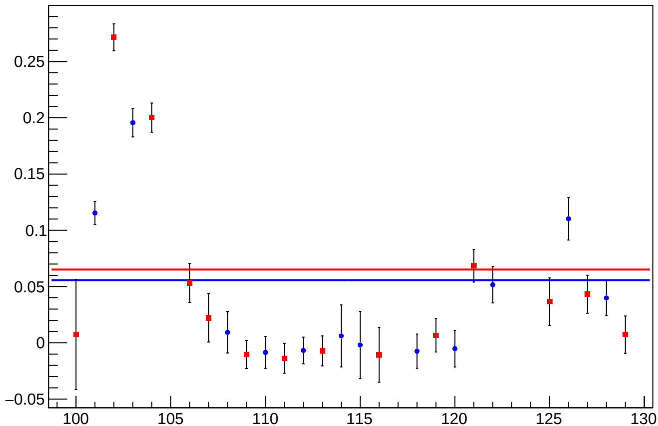
reg_asym_bcm_an_us_an_ds_dd_diff_bpm4eX_slope vs Slug, Sign Corrected
