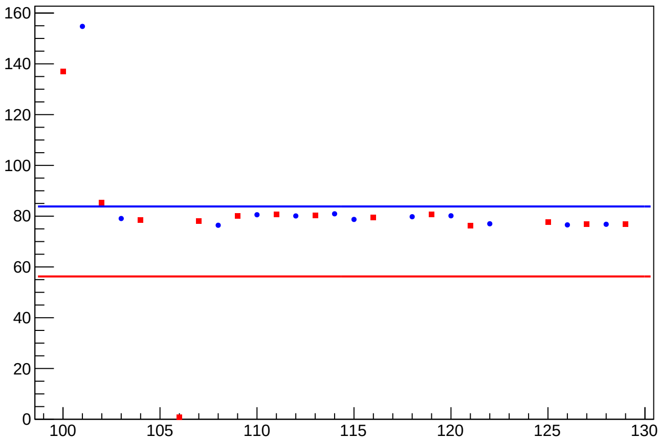
reg_asym_usl_atl2_dd_diff_bpm12X_slope vs Slug, Sign Corrected
