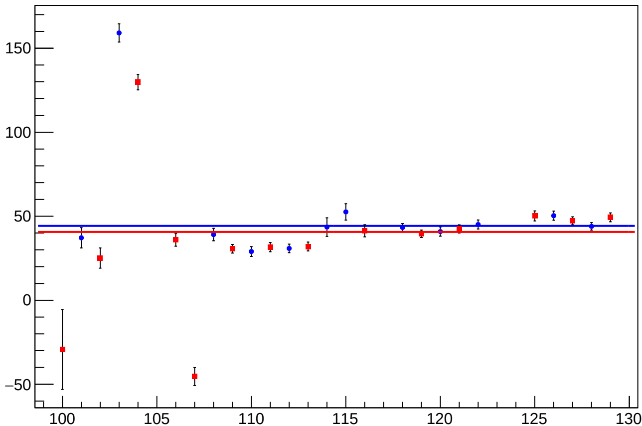
reg_asym_us_avg_at1lr_avg_dd_diff_bpm4eX_slope vs Slug, Sign Corrected
