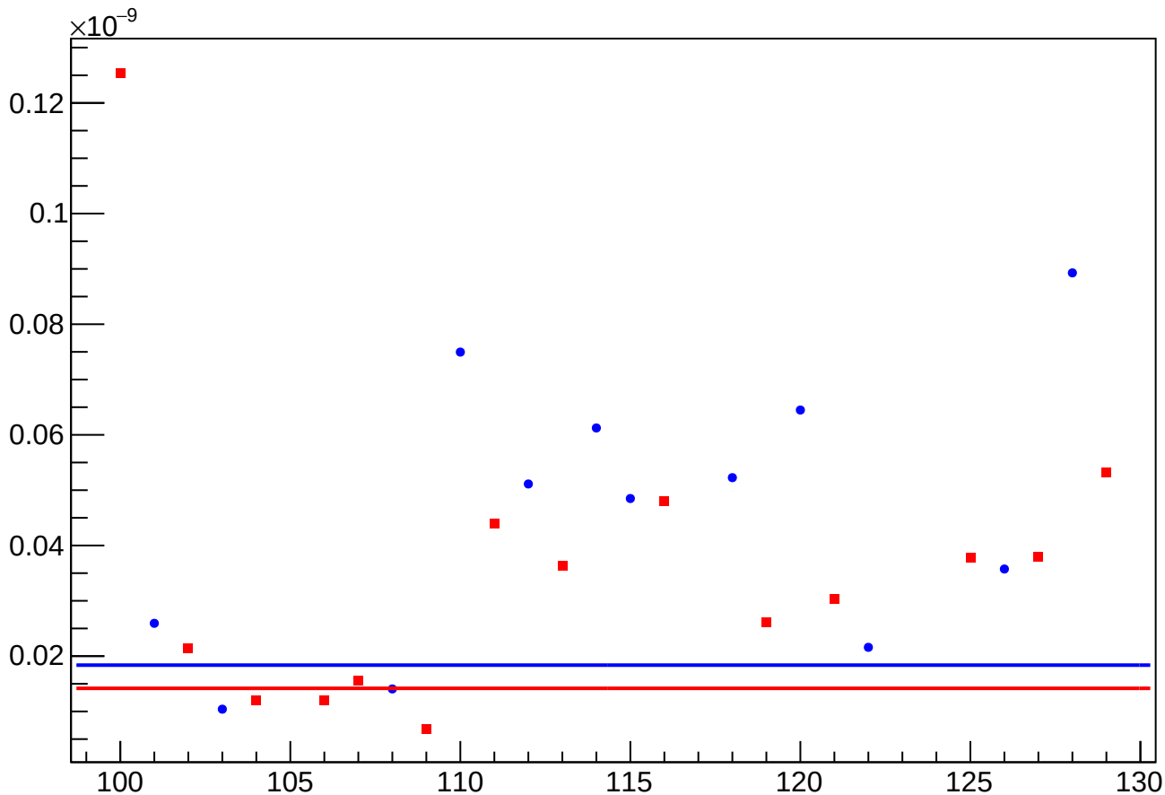
asym_us_dd_at2lr_dd_dd_eigen_cor_vs_cor_diff_rms vs Slug, Sign Corrected
