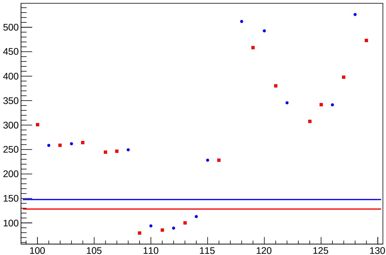
asym_sam8_cor_correction_rms vs Slug, Sign Corrected
