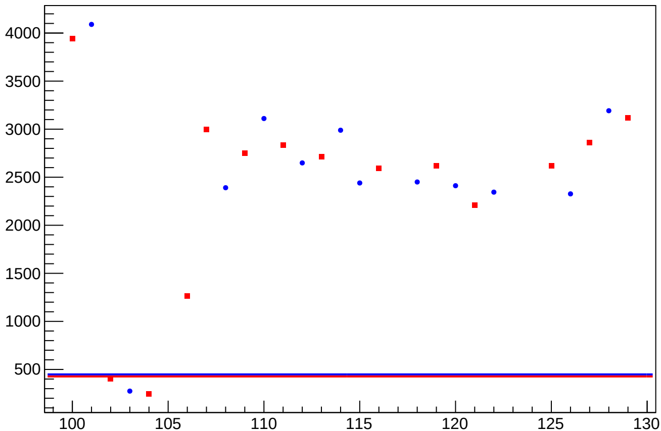
asym_us_avg_atlr_avg_dd_cor_correction_rms vs Slug, Sign Corrected
