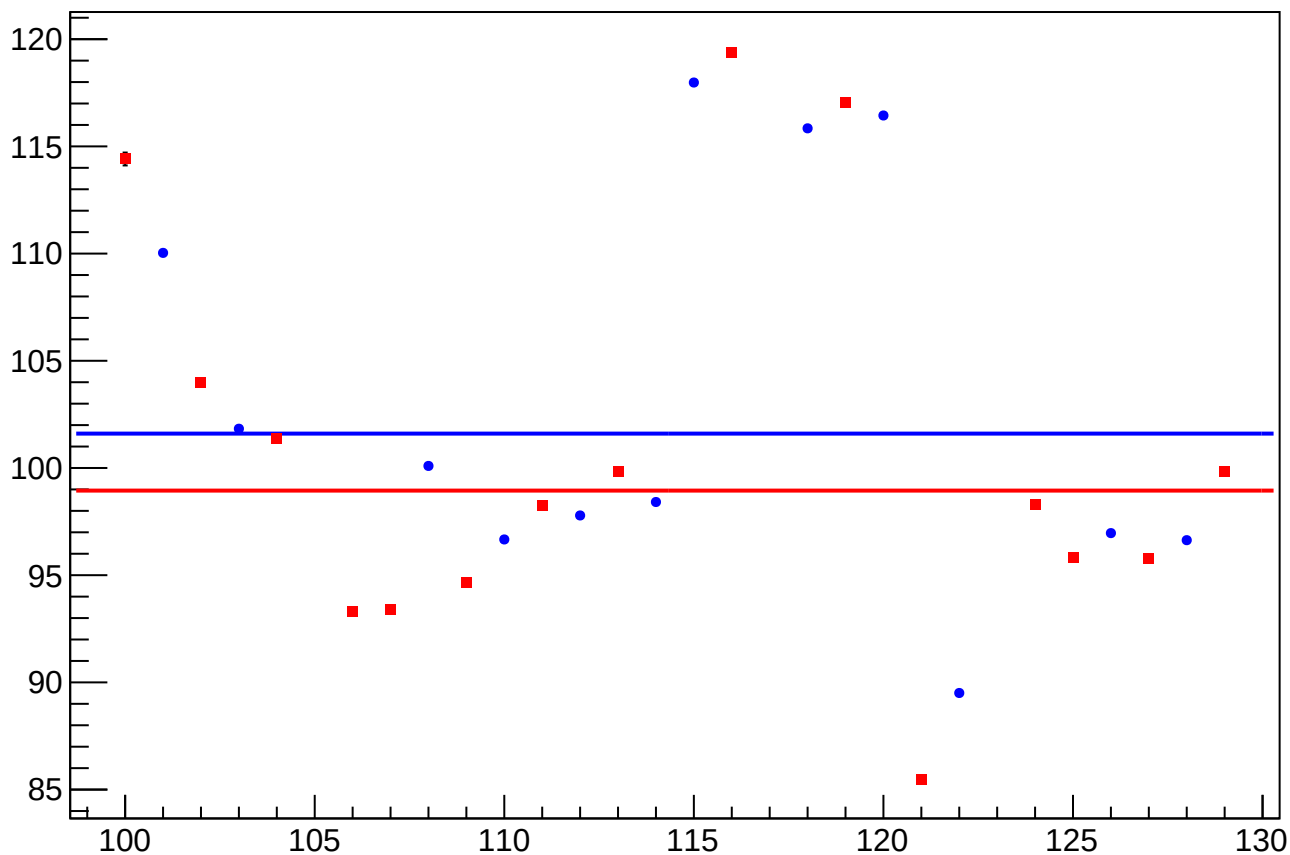
eigen_dit_asym_sam_15_dd_rms vs Slug, Sign Corrected
