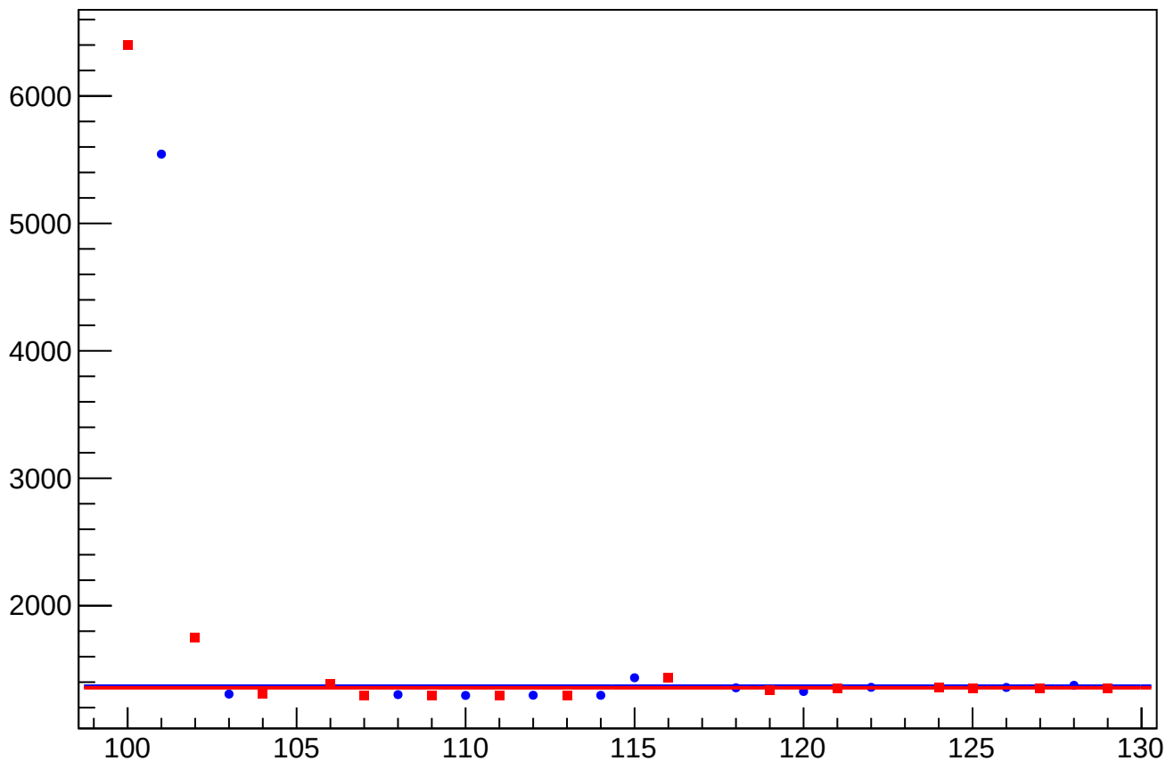
eigen_cor_asym_usr_atr1_dd_rms vs Slug, Sign Corrected
