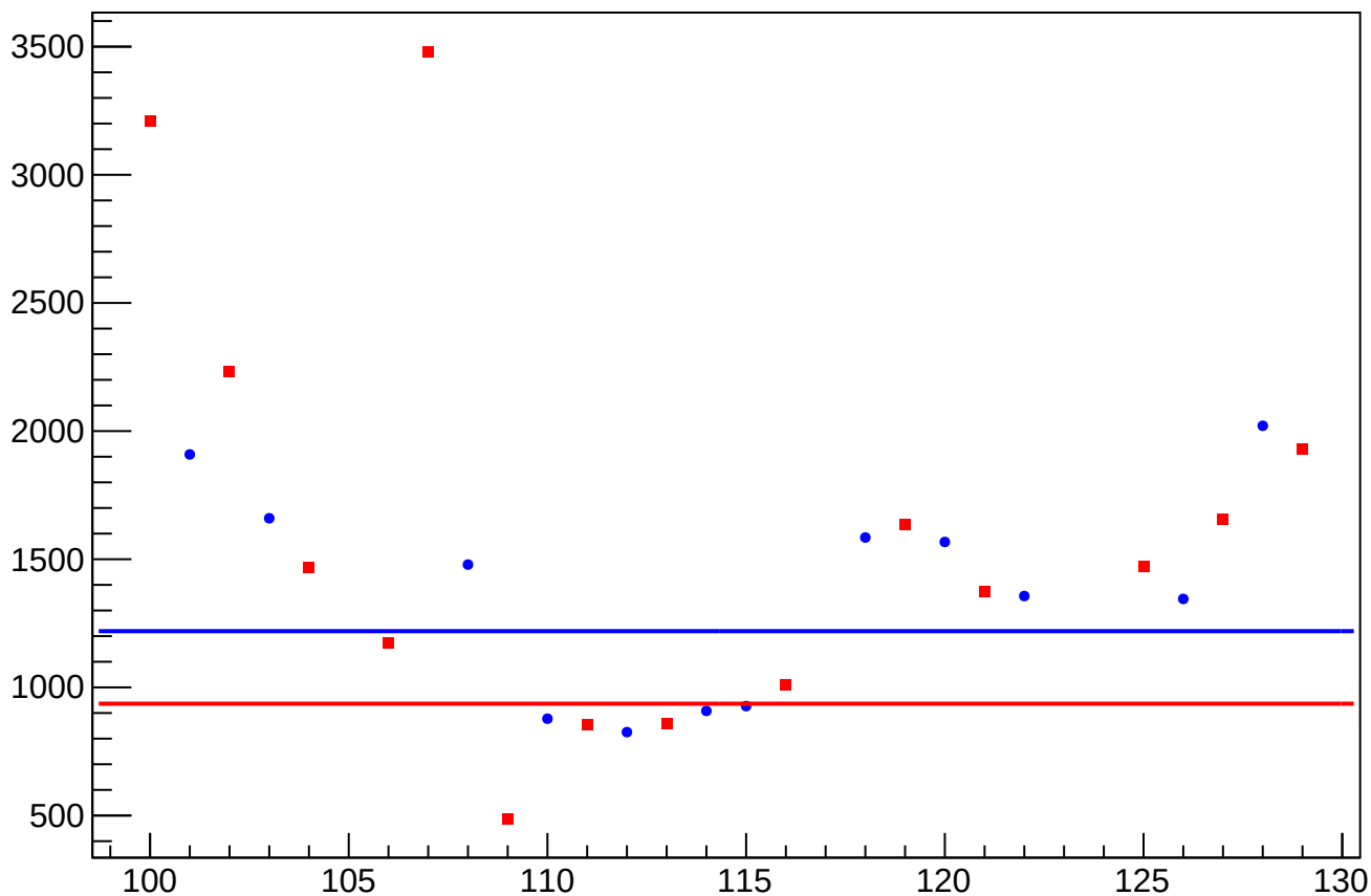
asym_us_dd_atlr_dd_avg_reg_correction_rms vs Slug, Sign Corrected
