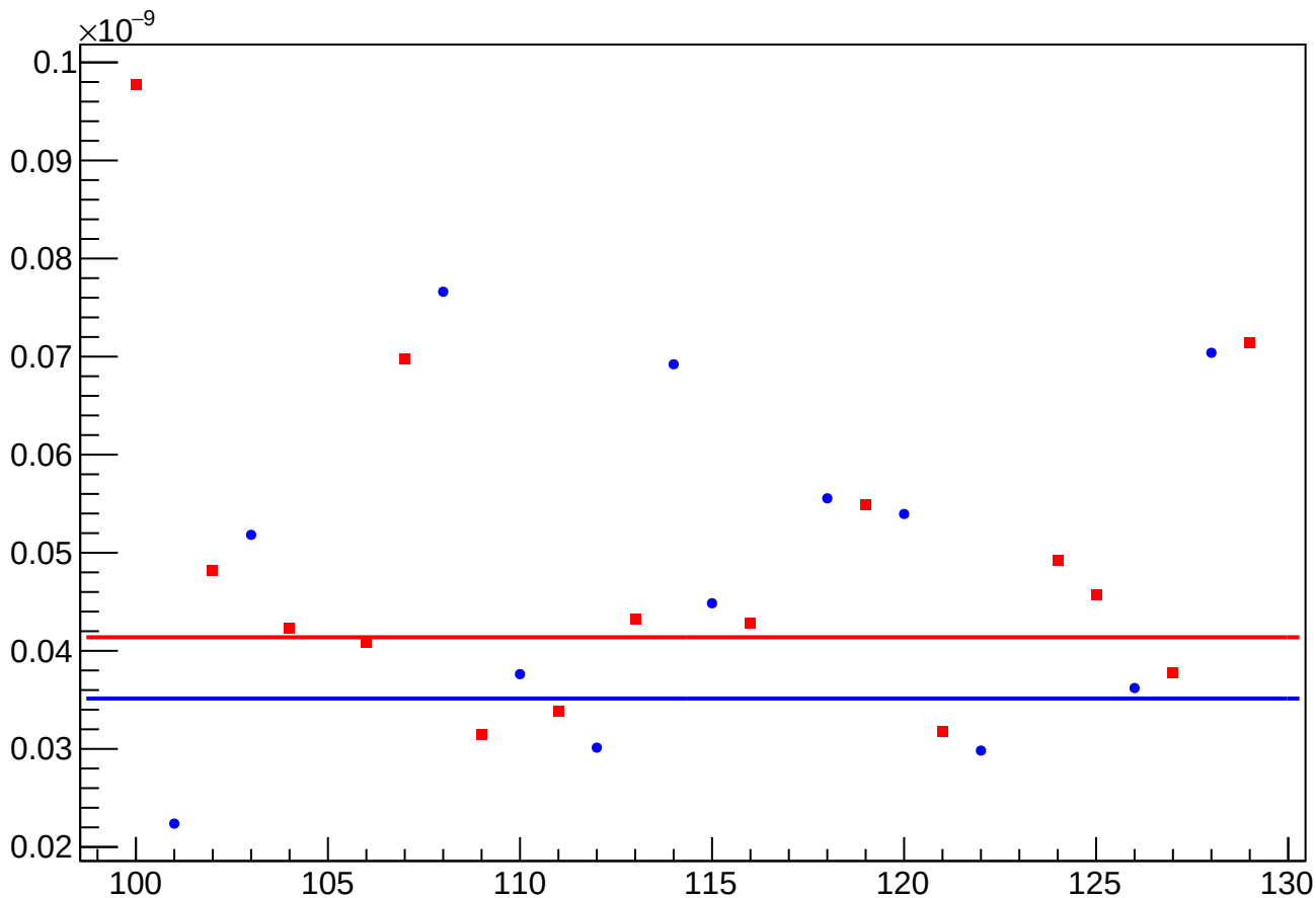
asym_sam_2468_avg_eigen_cor_vs_cor_diff_rms vs Slug, Sign Corrected
