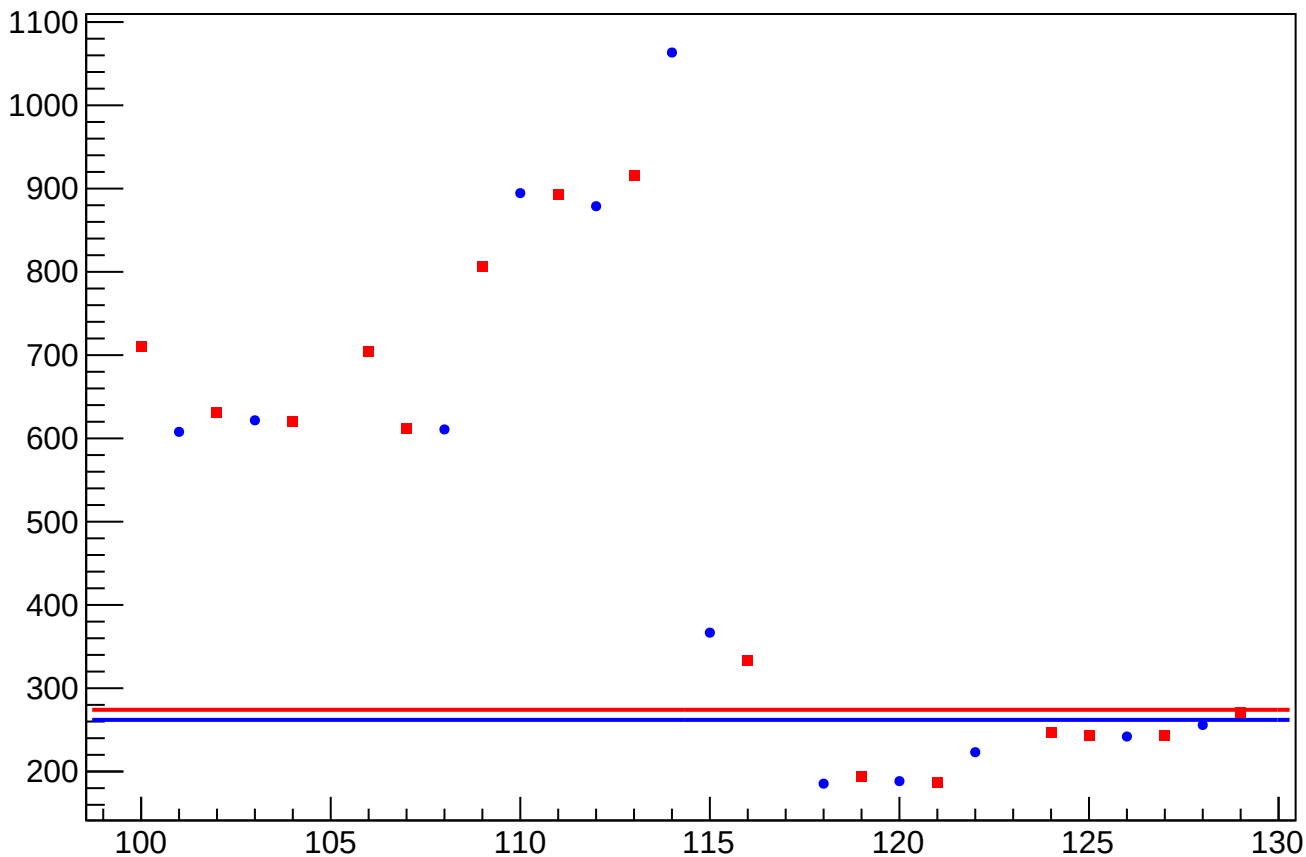
asym_sam_37_26_dd_cor_correction_rms vs Slug, Sign Corrected
