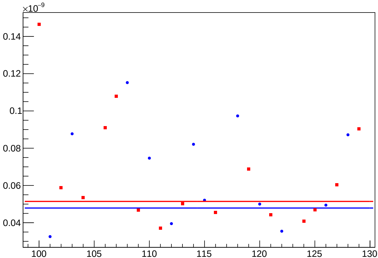
asym_sam_2468_avg_reg_vs_cor_diff_rms vs Slug, Sign Corrected
