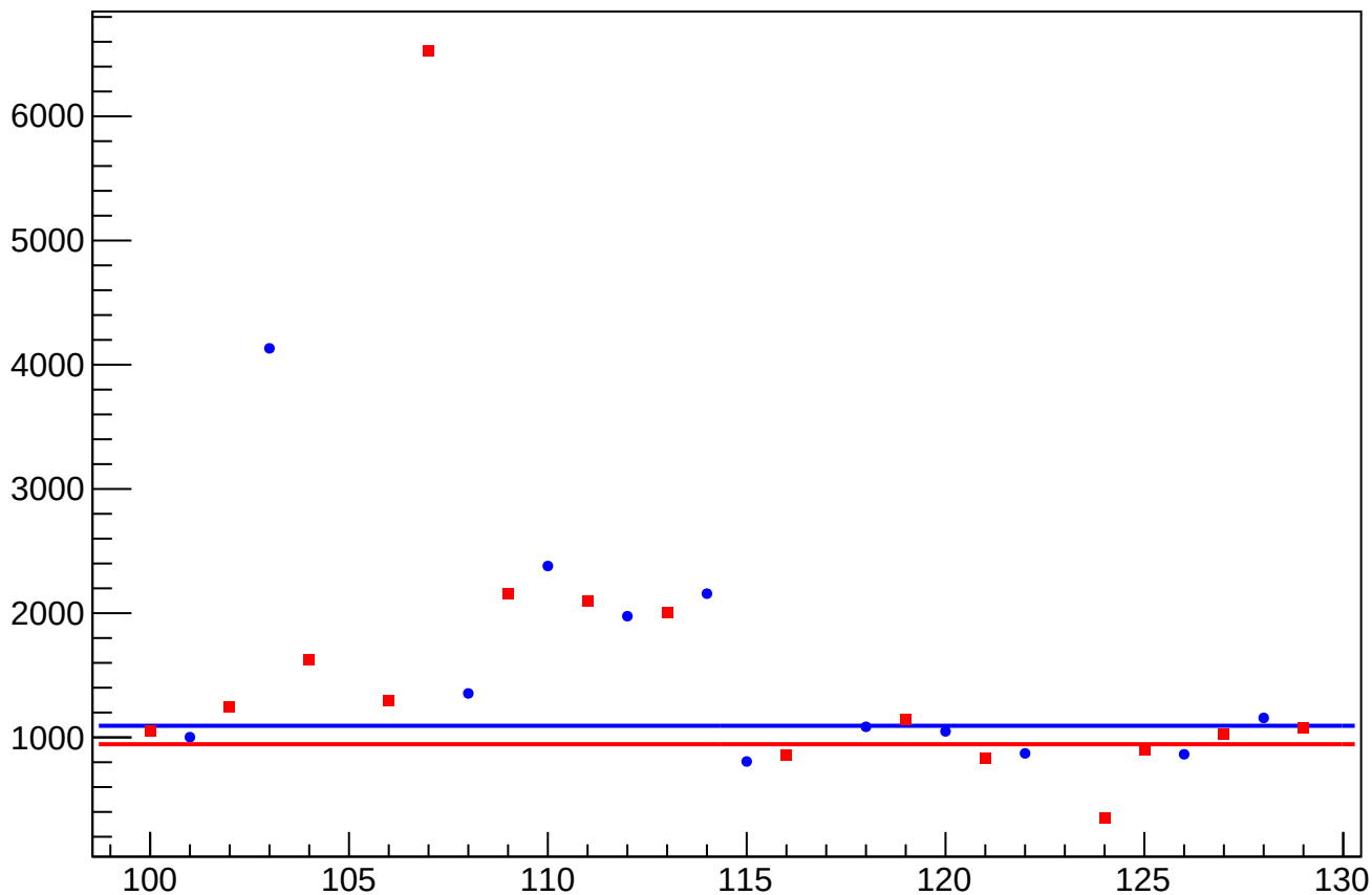
asym_atl1_eigen_cor_correction_rms vs Slug, Sign Corrected
