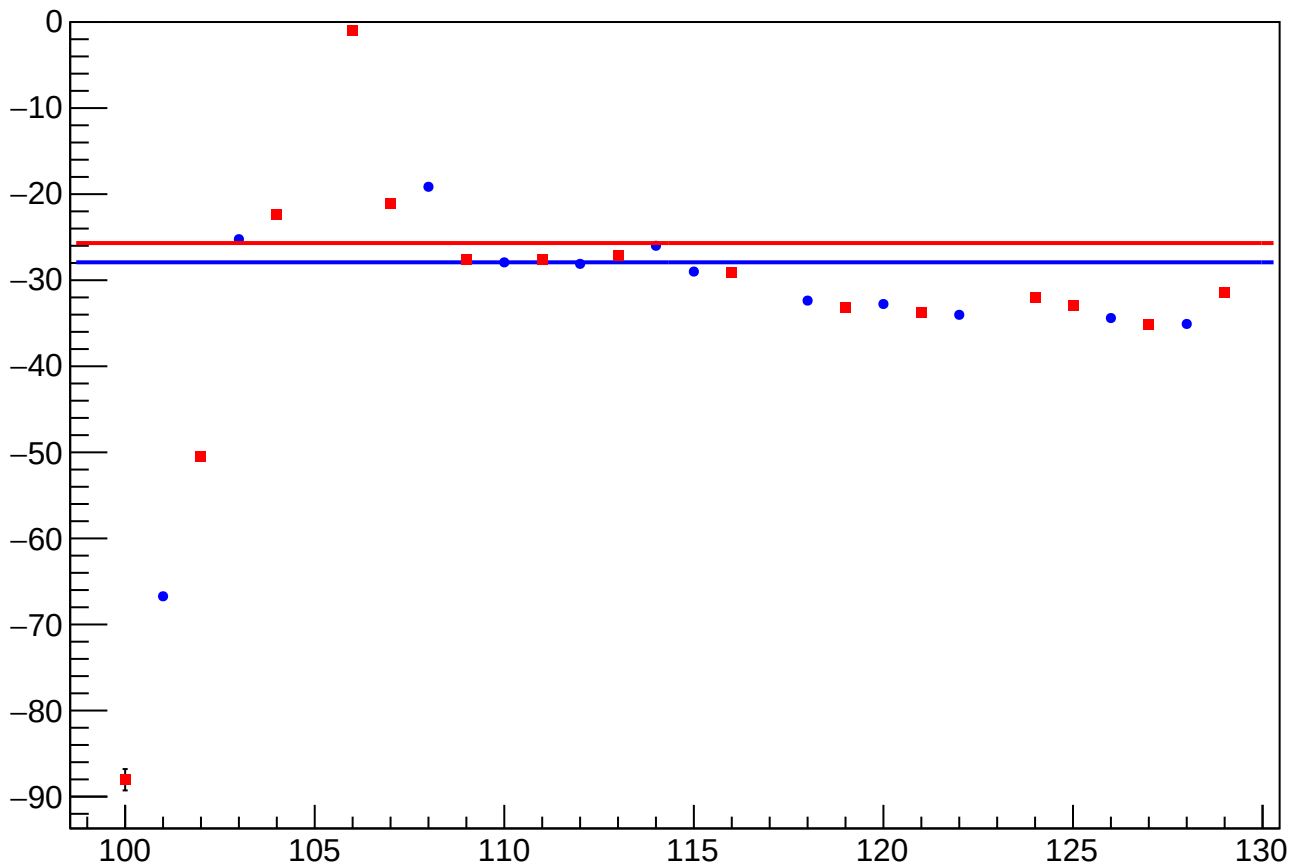
reg_asym_usr_atr1_avg_diff_bpm12X_slope vs Slug, Sign Corrected
