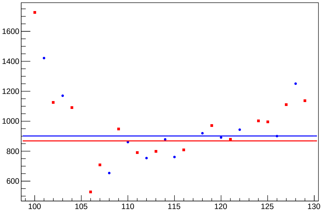
asym_usr_atr1_avg_dit_correction_rms vs Slug, Sign Corrected
