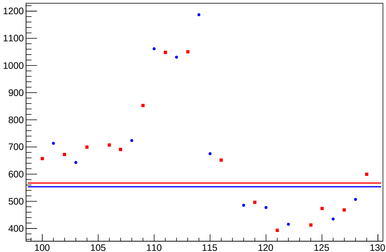
asym_sam1_dit_correction_rms vs Slug, Sign Corrected
