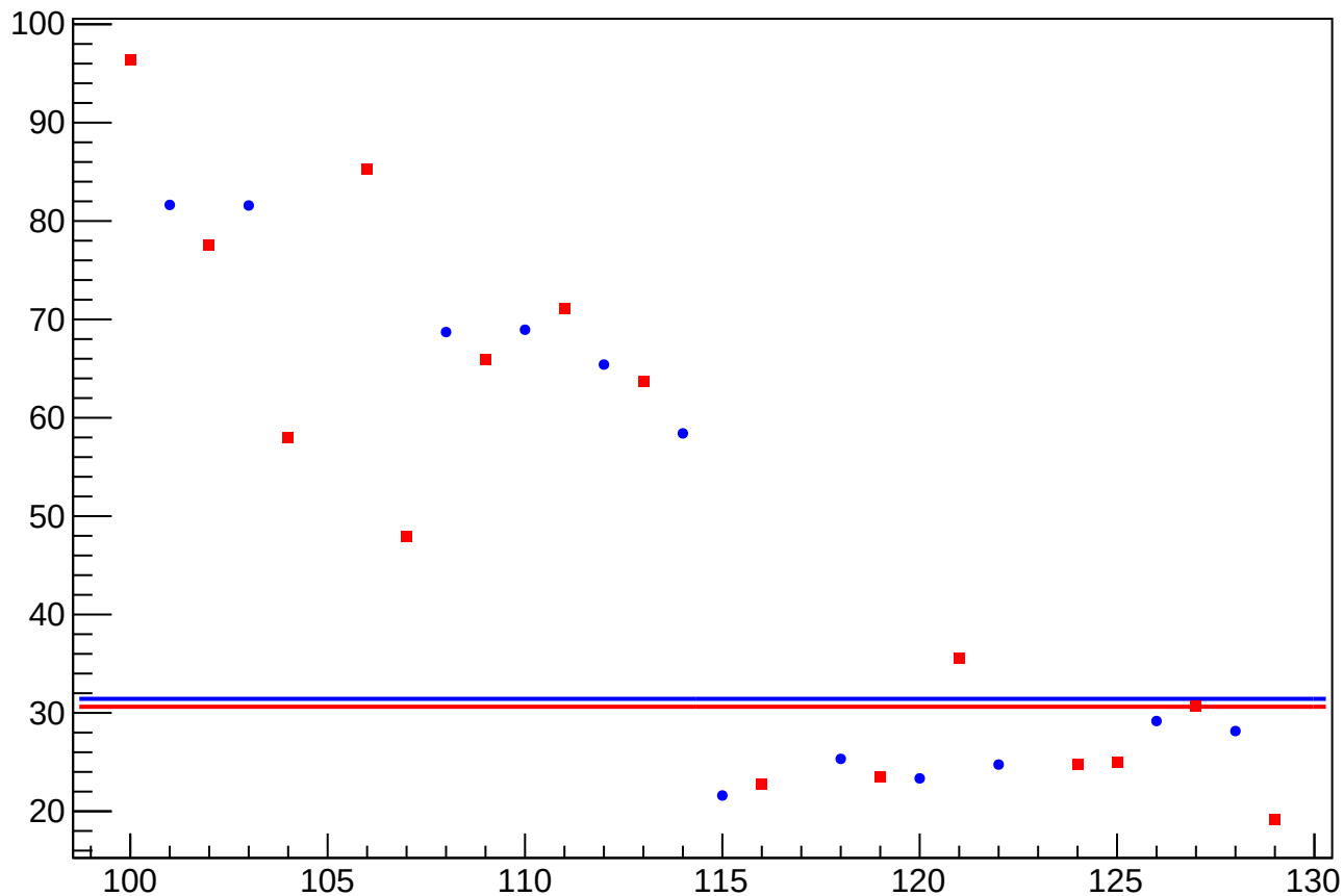
asym_sam_1526_avg_eigen_dit_vs_eigen_cor_diff_rms vs Slug, Sign Corrected
