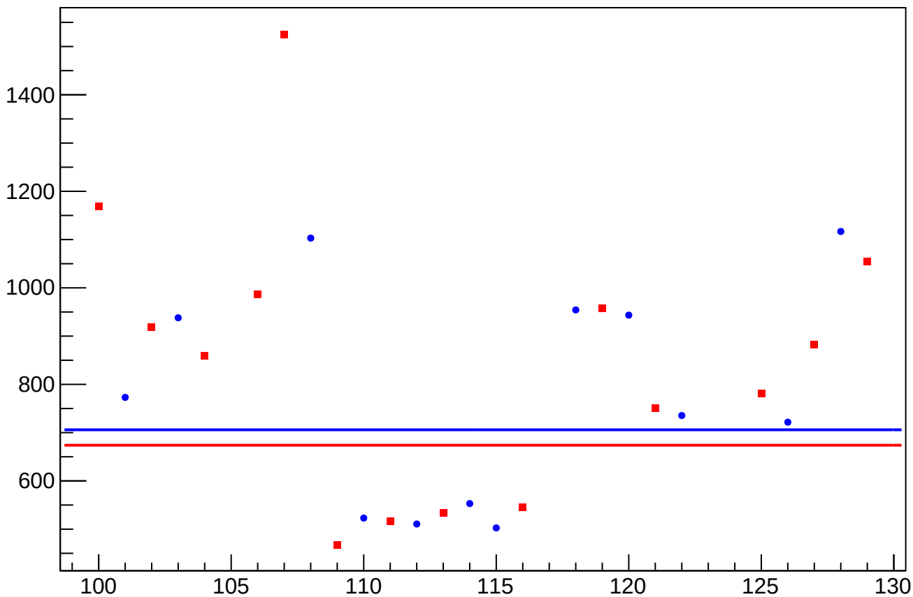
asym_us_dd_reg_correction_rms vs Slug, Sign Corrected
