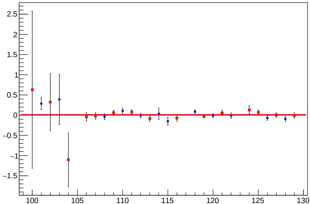
asym_usr_atr1_dd_dit_vs_cor_diff_mean vs Slug, Sign Corrected
