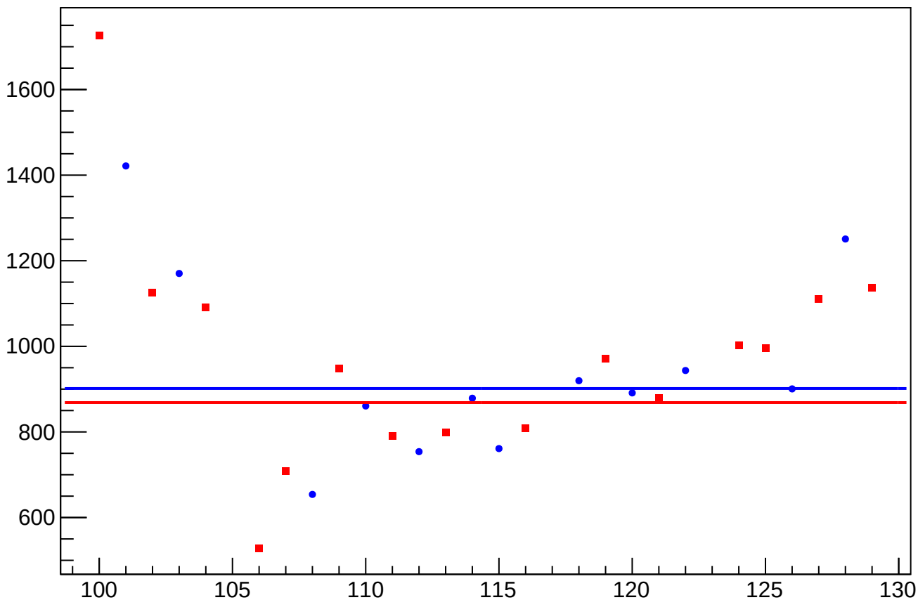
asym_usr_atr1_avg_eigen_dit_correction_rms vs Slug, Sign Corrected
