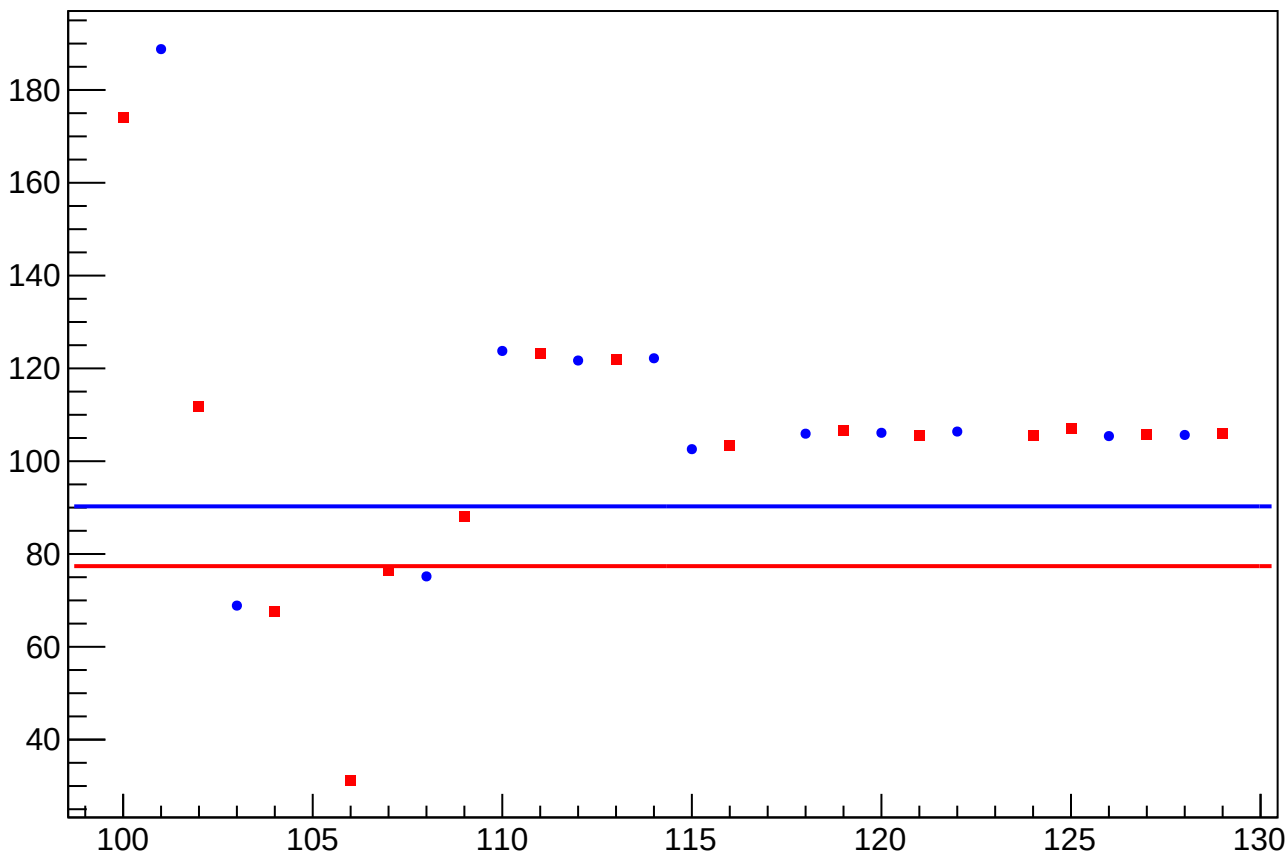
reg_asym_usr_atr2_dd_diff_bpm12X_slope vs Slug, Sign Corrected
