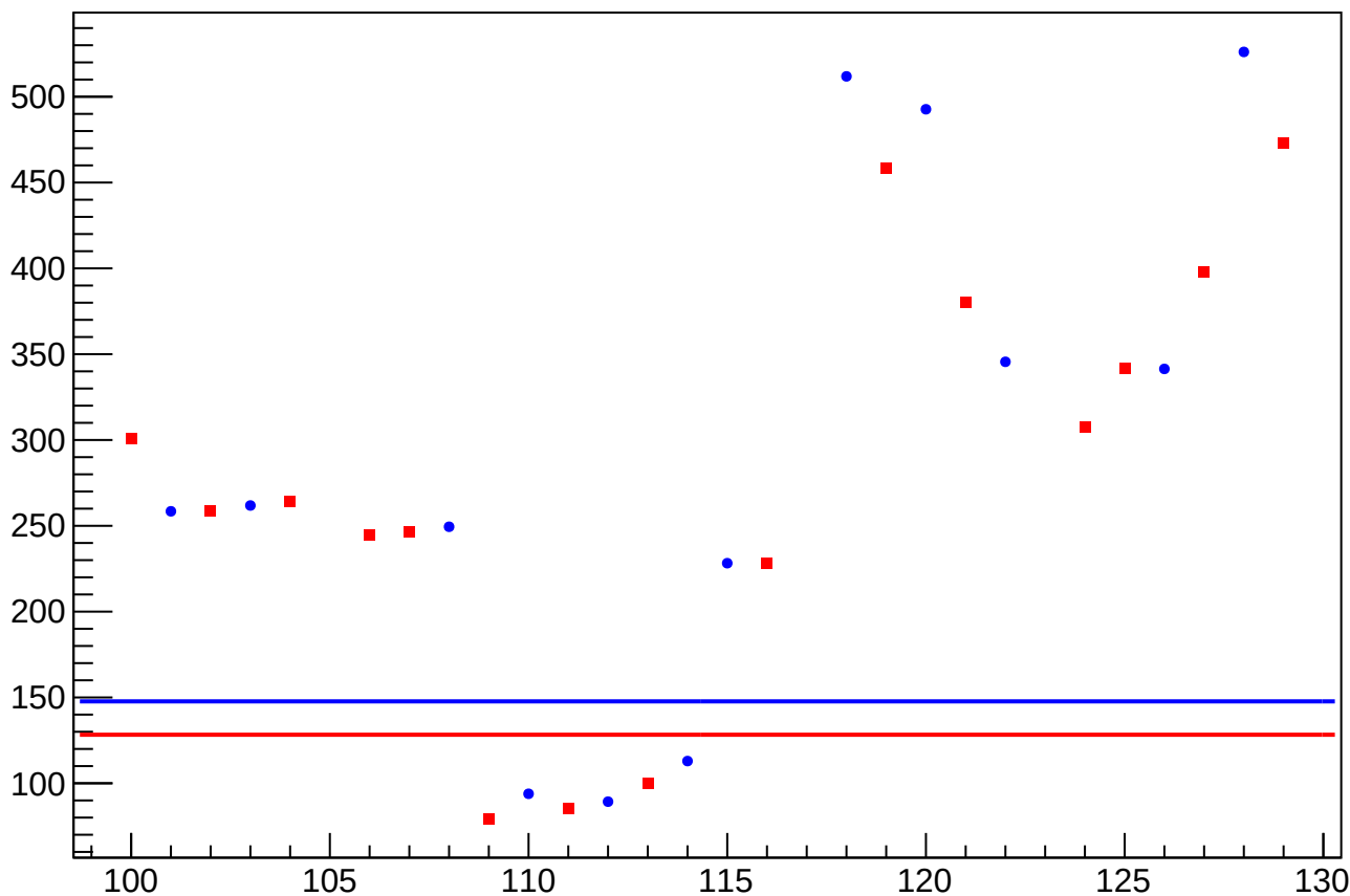
asym_sam8_eigen_cor_correction_rms vs Slug, Sign Corrected
