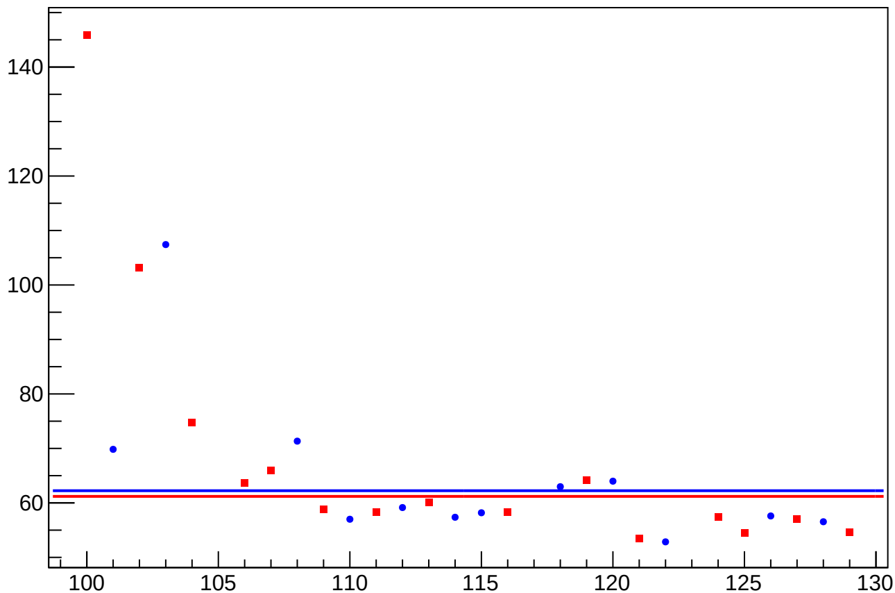
cor_asym_sam_13_57_dd_rms vs Slug, Sign Corrected
