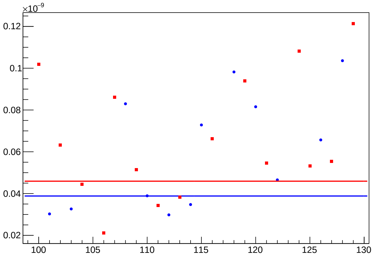
asym_sam_3748_avg_reg_vs_cor_diff_rms vs Slug, Sign Corrected
