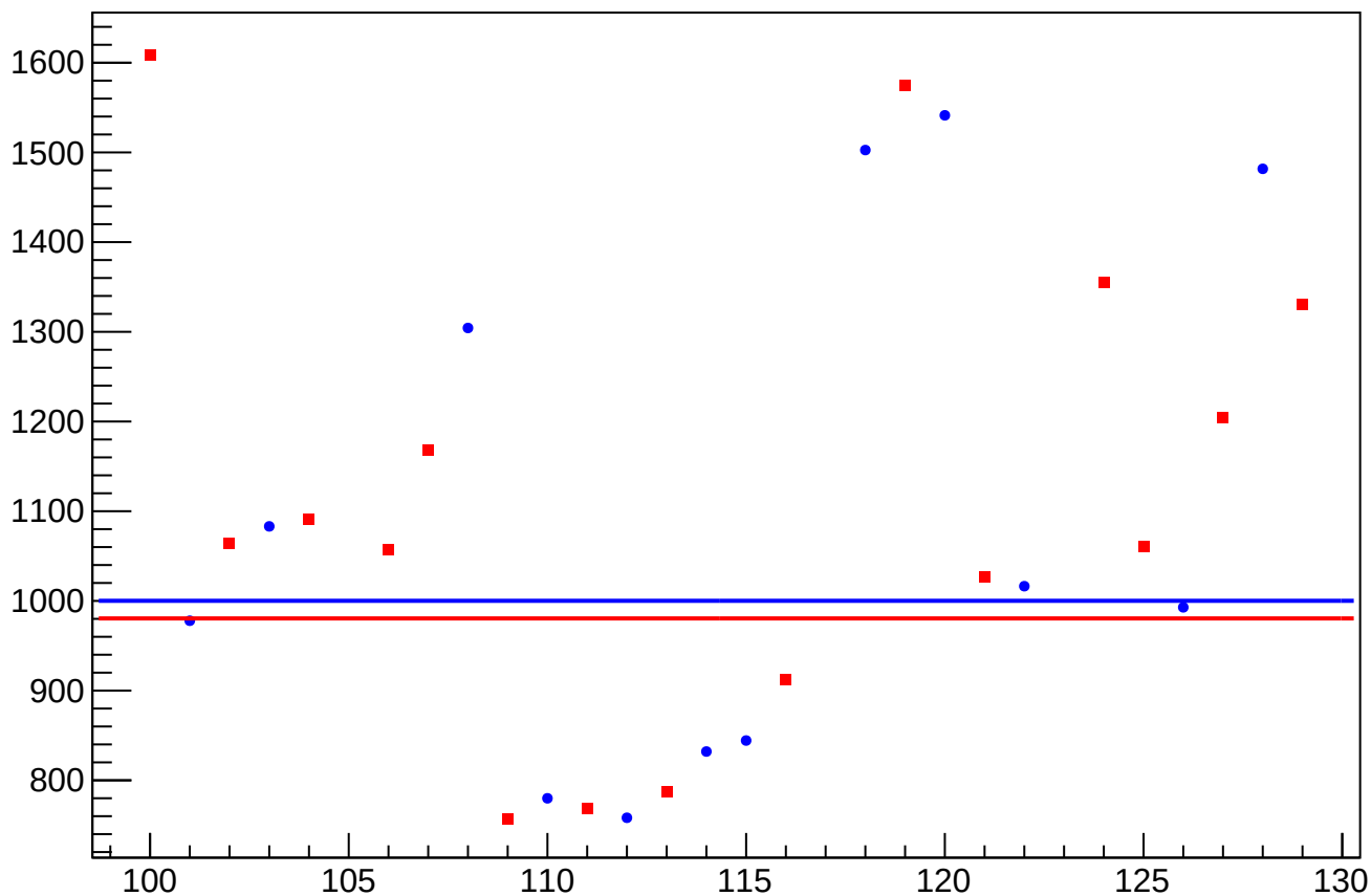
asym_sam_37_avg_reg_correction_rms vs Slug, Sign Corrected
