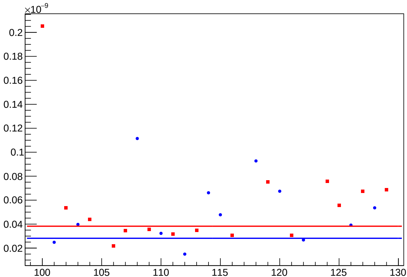
asym_sam_37_avg_reg_vs_cor_diff_rms vs Slug, Sign Corrected
