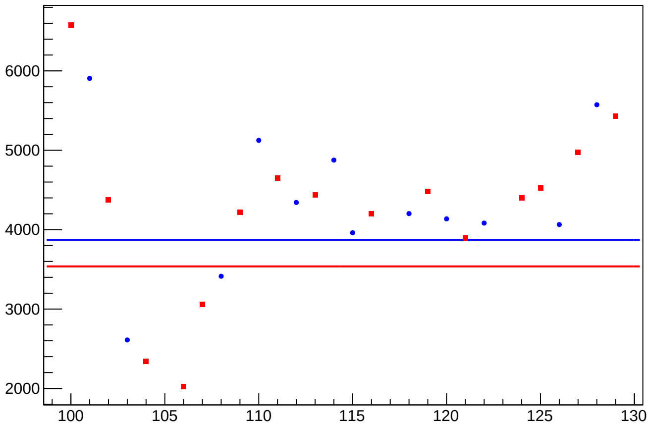
asym_atr_avg_eigen_cor_correction_rms vs Slug, Sign Corrected
