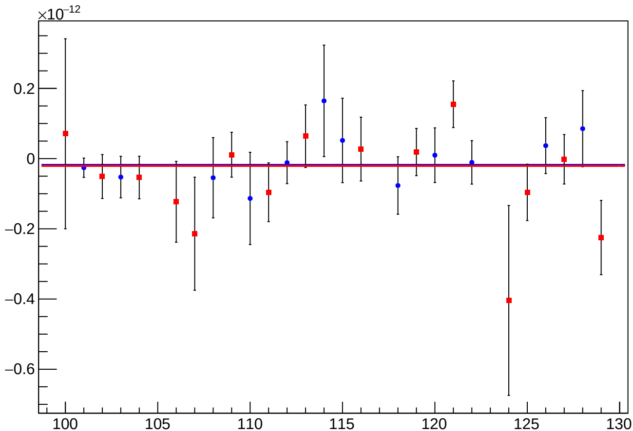
asym_atl_dd_atr_dd_dd_eigen_cor_vs_cor_diff_mean vs Slug, Sign Corrected
