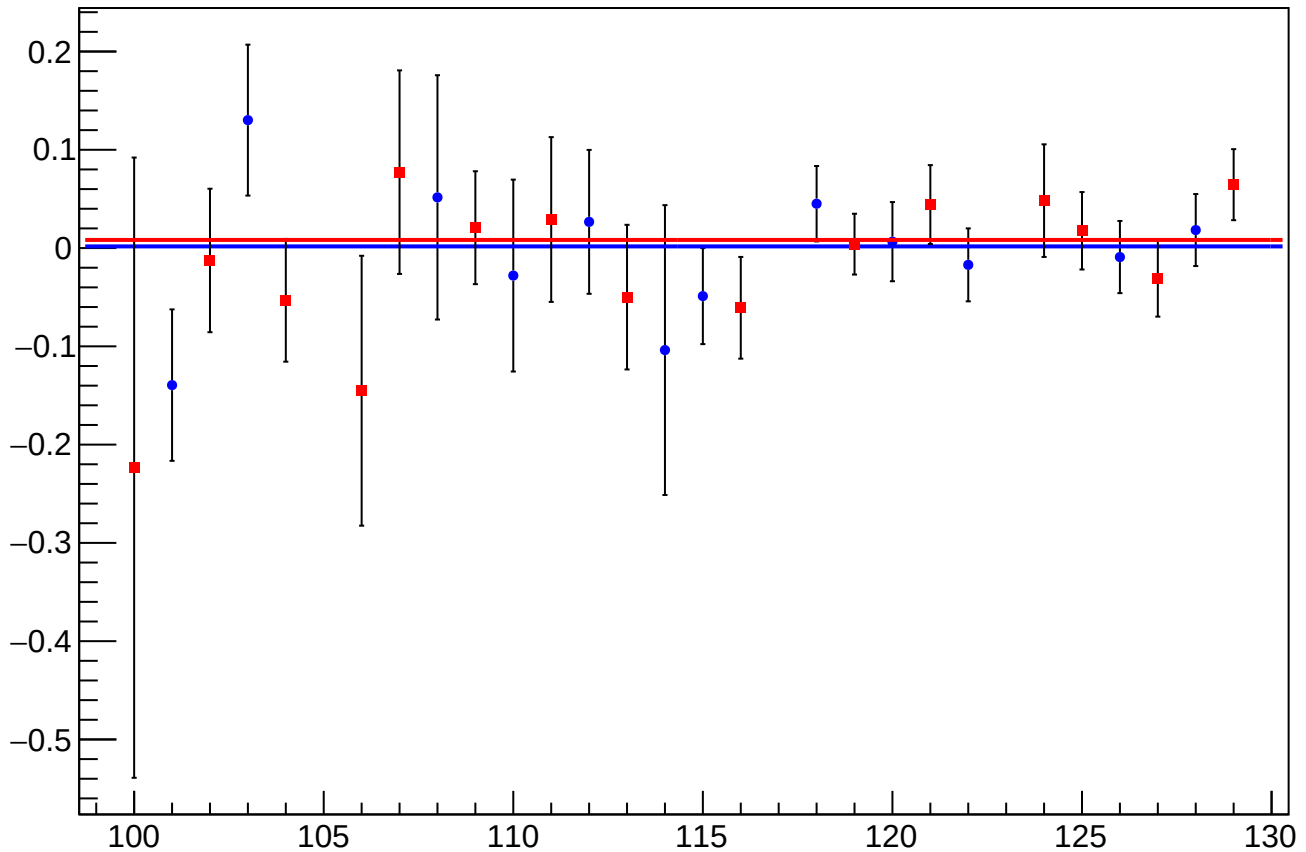
asym_sam_15_26_dd_dit_vs_eigen_cor_diff_mean vs Slug, Sign Corrected
