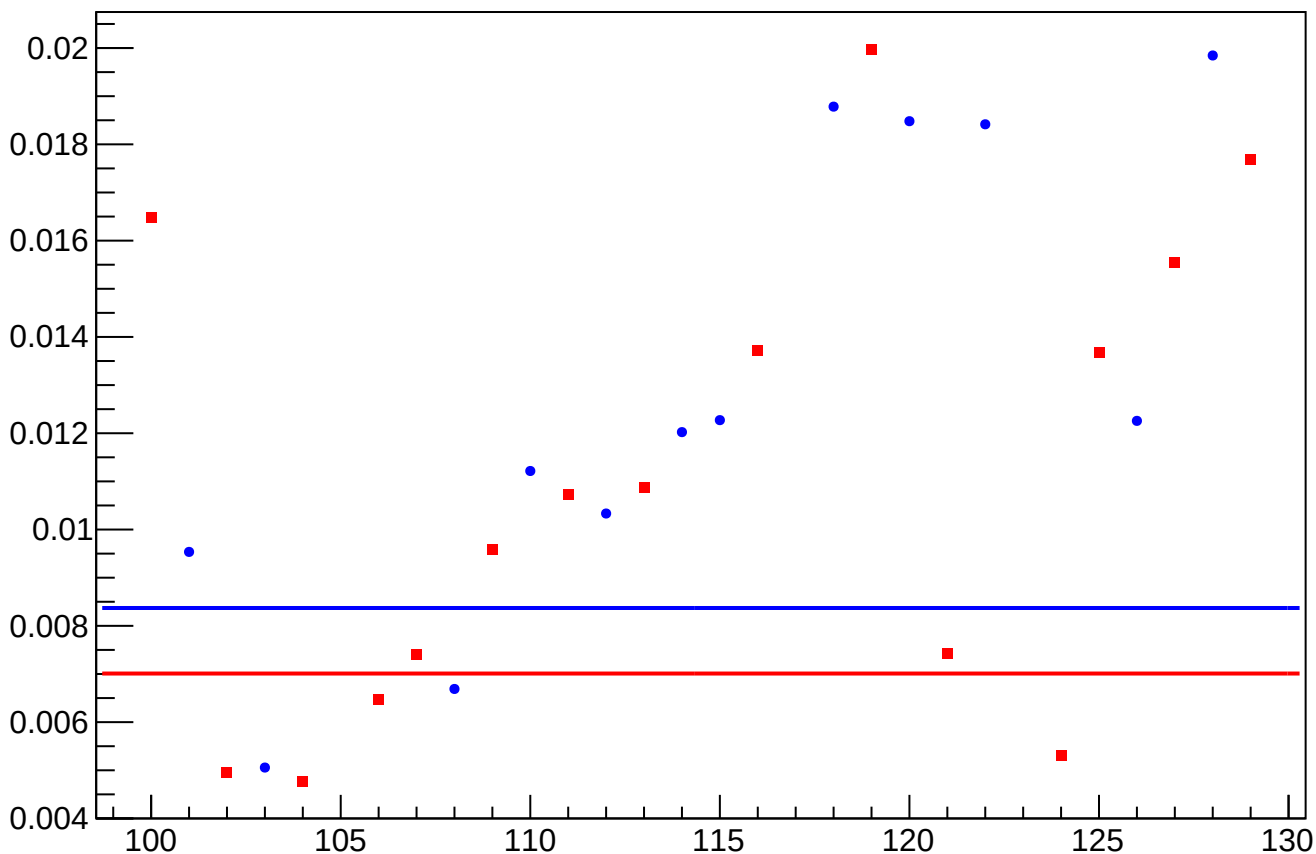
asym_atl_avg_atr_avg_avg_eigen_dit_vs_dit_diff_rms vs Slug, Sign Corrected
