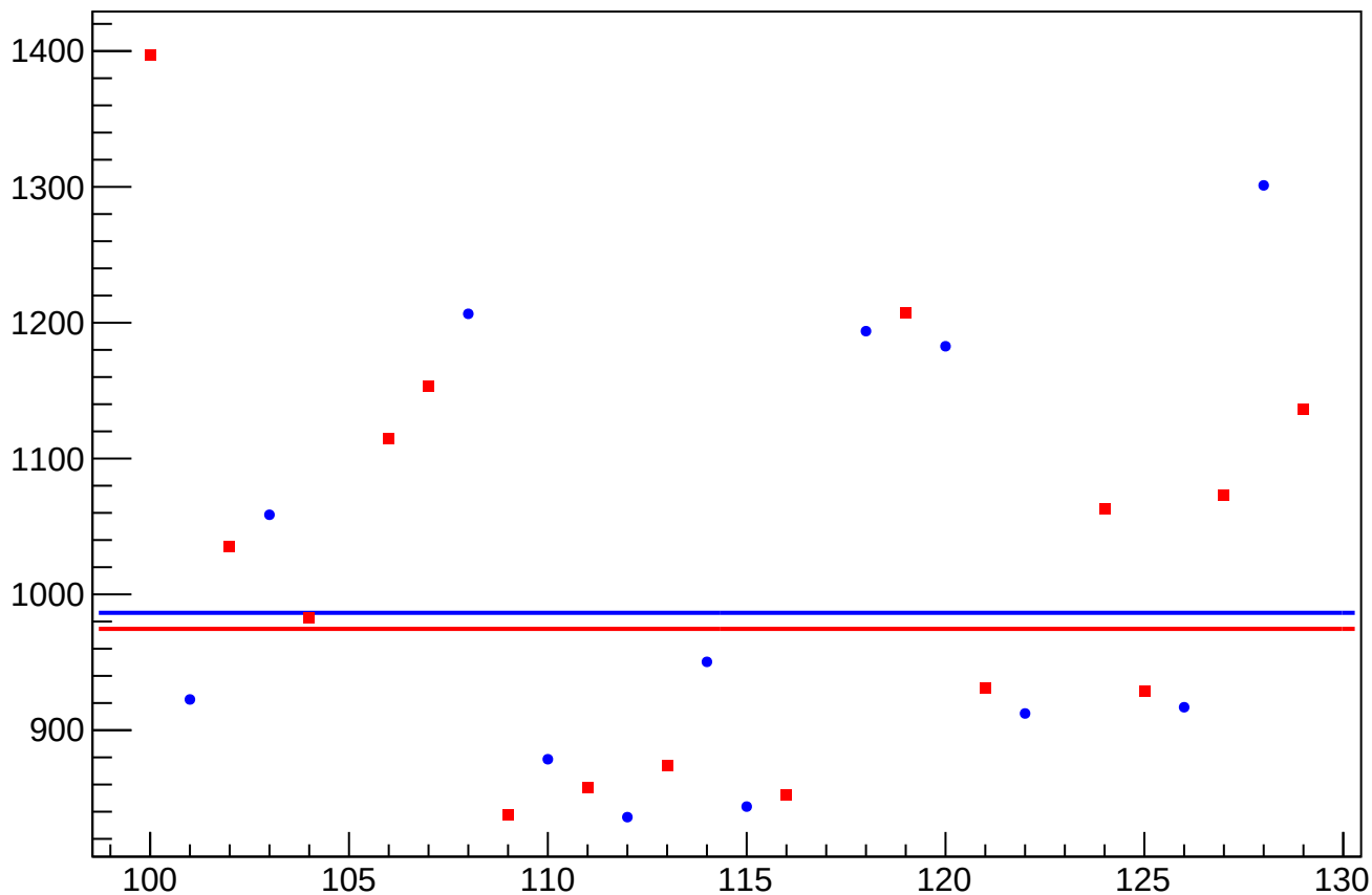
asym_sam_12345678_avg_eigen_dit_correction_rms vs Slug, Sign Corrected
