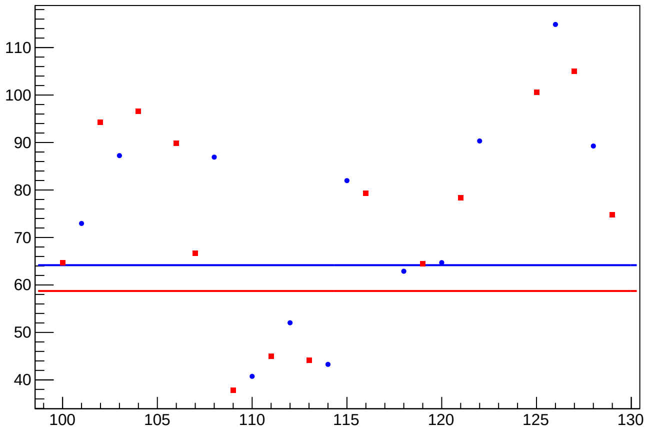
asym_bcm_2an_us_an_ds_dd_rms vs Slug, Sign Corrected
