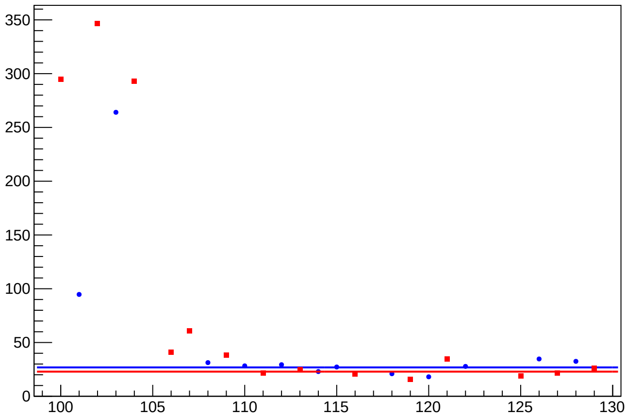
asym_us_dd_atlr_dd_dd_dit_vs_eigen_cor_diff_rms vs Slug, Sign Corrected
