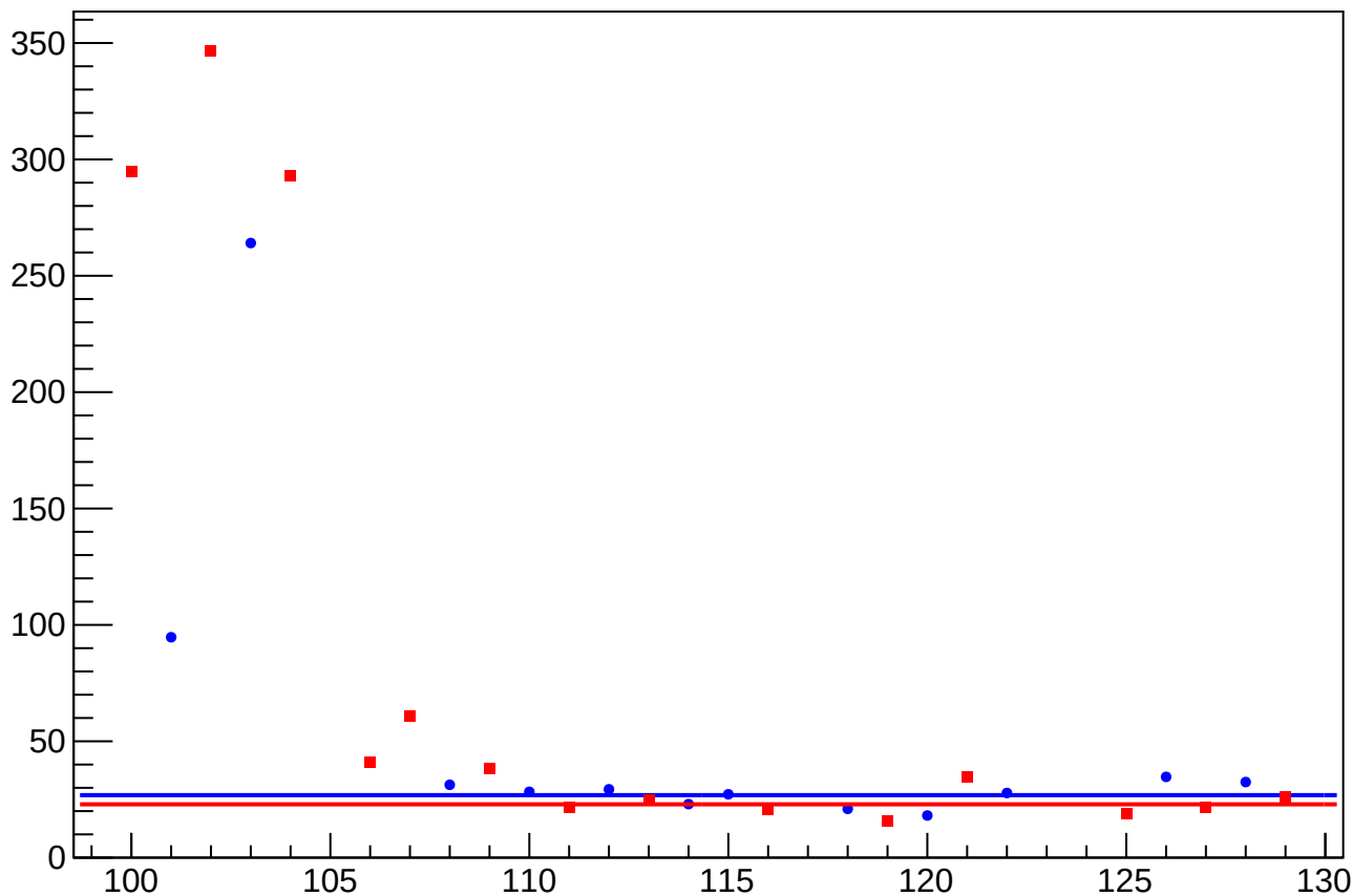
asym_us_dd_atlr_dd_dd_dit_vs_cor_diff_rms vs Slug, Sign Corrected
