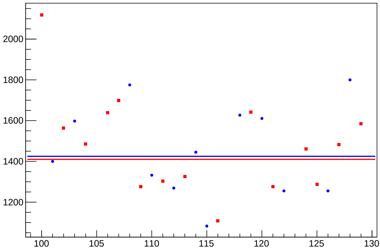
asym_sam_2468_avg_eigen_dit_correction_rms vs Slug, Sign Corrected
