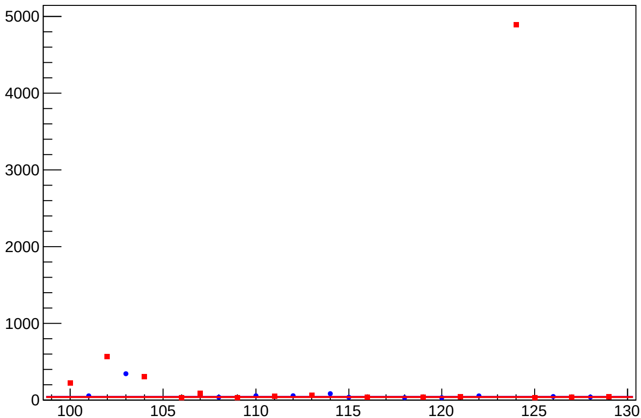
asym_atl_dd_atr_dd_dd_eigen_dit_vs_cor_diff_rms vs Slug, Sign Corrected
