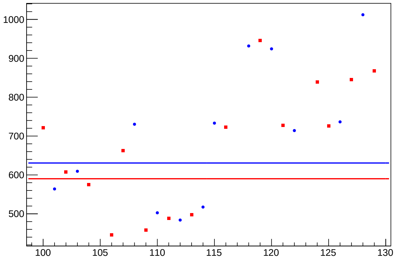
asym_sam_15_48_dd_eigen_dit_correction_rms vs Slug, Sign Corrected
