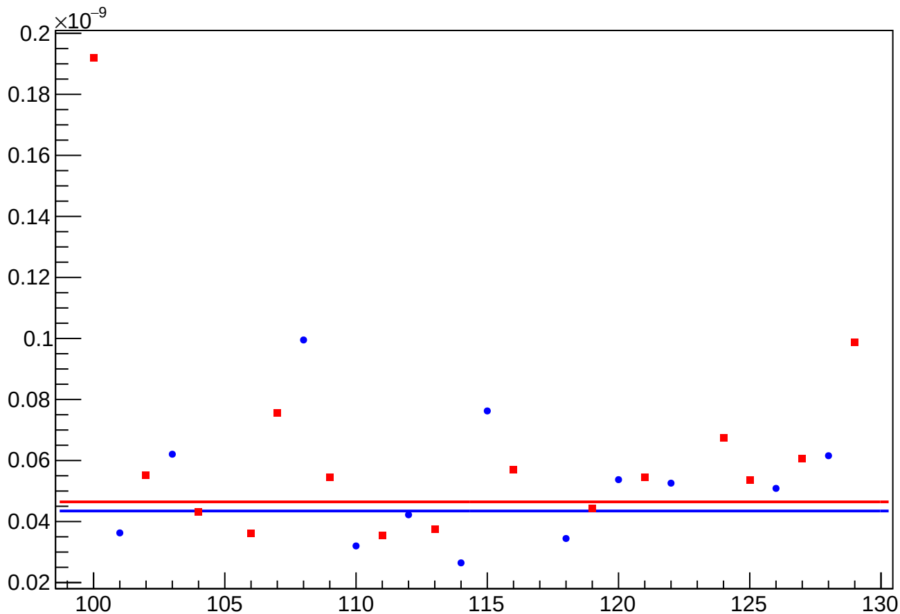
asym_sam_48_dd_reg_vs_cor_diff_rms vs Slug, Sign Corrected
