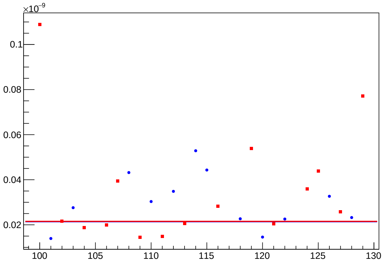
asym_sam7_reg_vs_cor_diff_rms vs Slug, Sign Corrected
