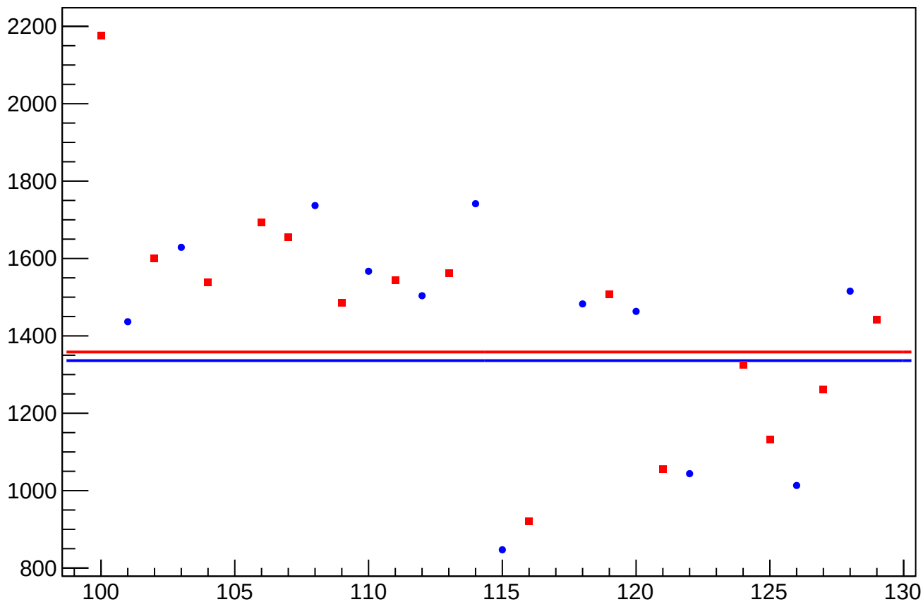
asym_sam_3726_avg_eigen_dit_correction_rms vs Slug, Sign Corrected
