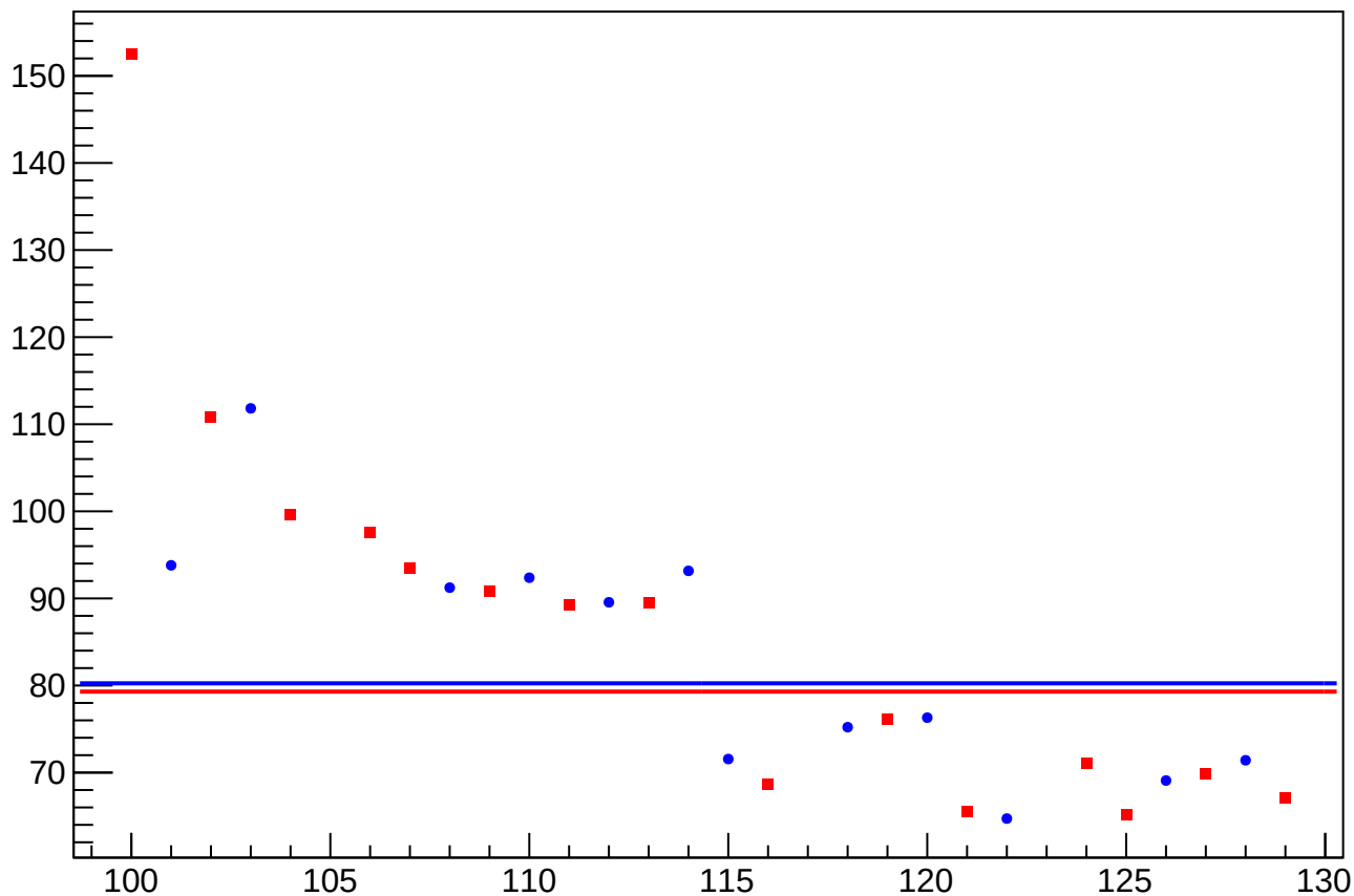
cor_asym_sam_15_26_dd_rms vs Slug, Sign Corrected
