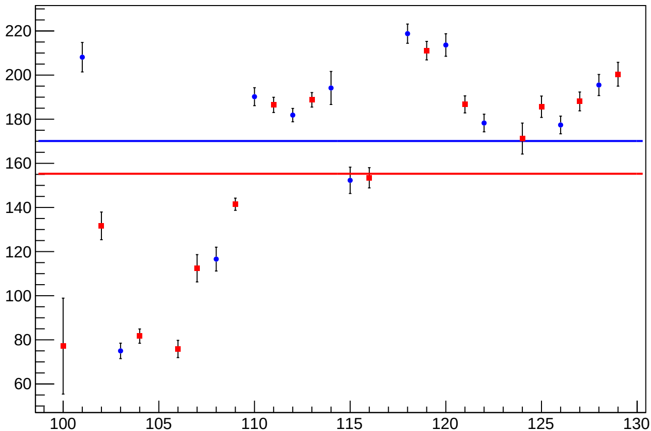
reg_asym_usr_atr2_dd_diff_bpm1X_slope vs Slug, Sign Corrected
