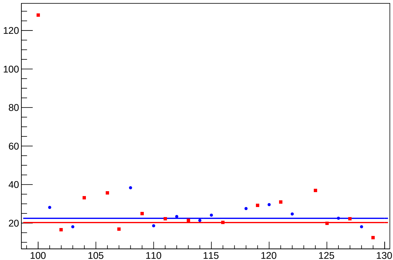
asym_sam_1357_avg_eigen_dit_vs_eigen_cor_diff_rms vs Slug, Sign Corrected
