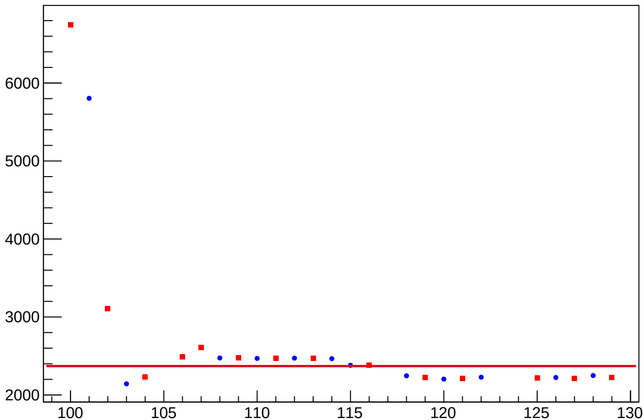
eigen_dit_asym_us_dd_at1lr_dd_avg_rms vs Slug, Sign Corrected
