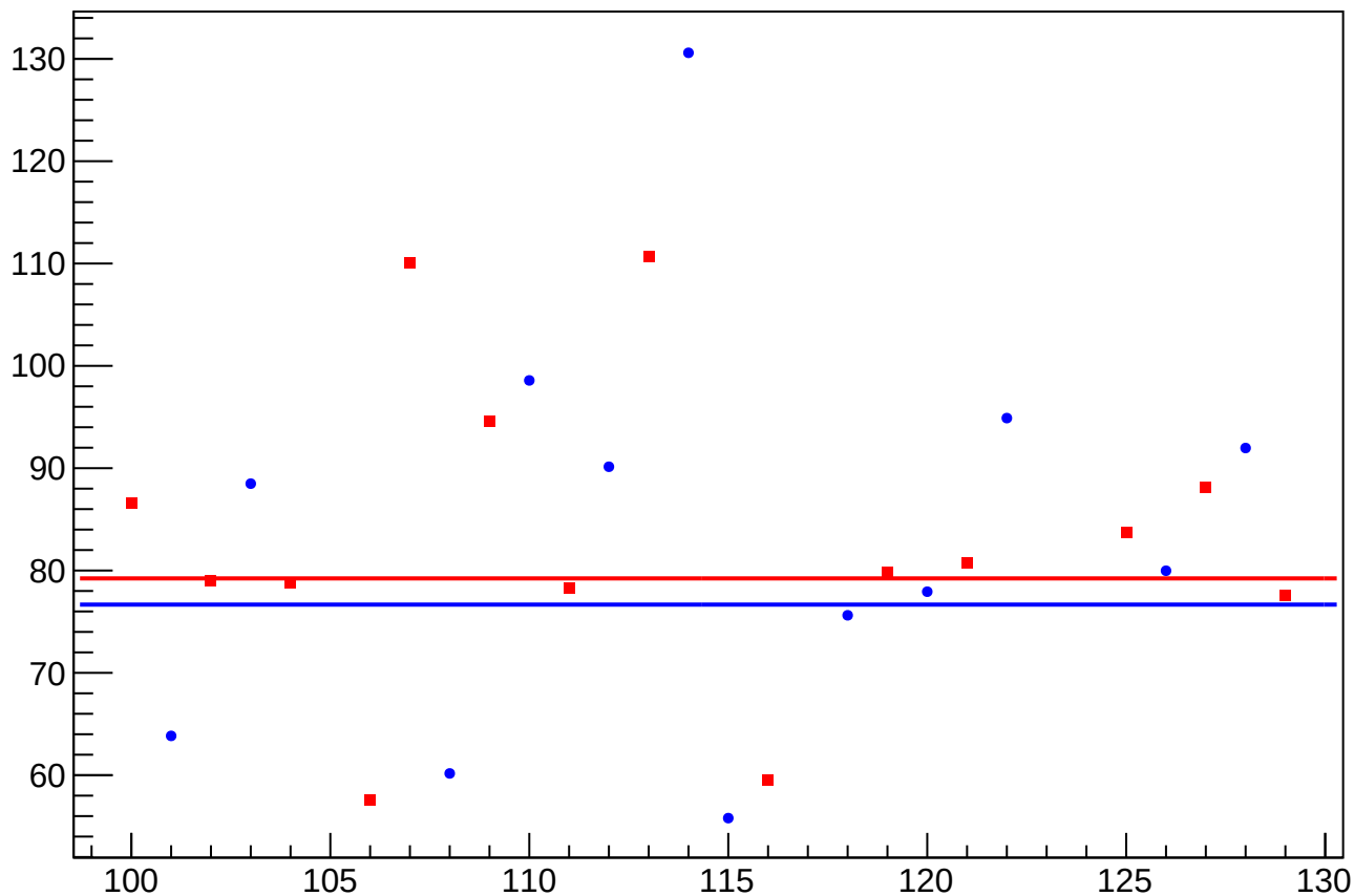
asym_us_avg_eigen_dit_vs_overload_cor_diff_rms vs Slug, Sign Corrected
