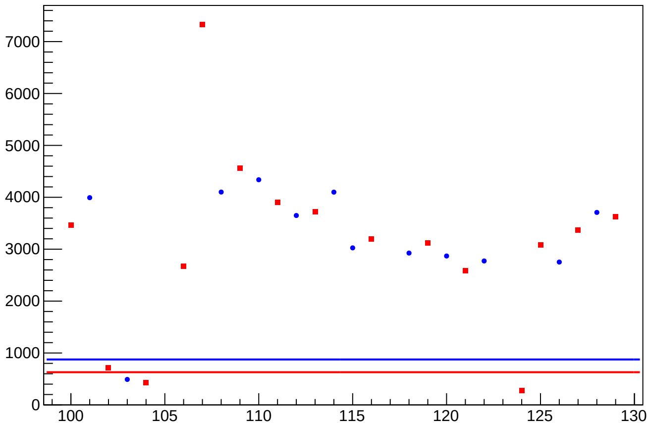
asym_atl_avg_eigen_cor_correction_rms vs Slug, Sign Corrected
