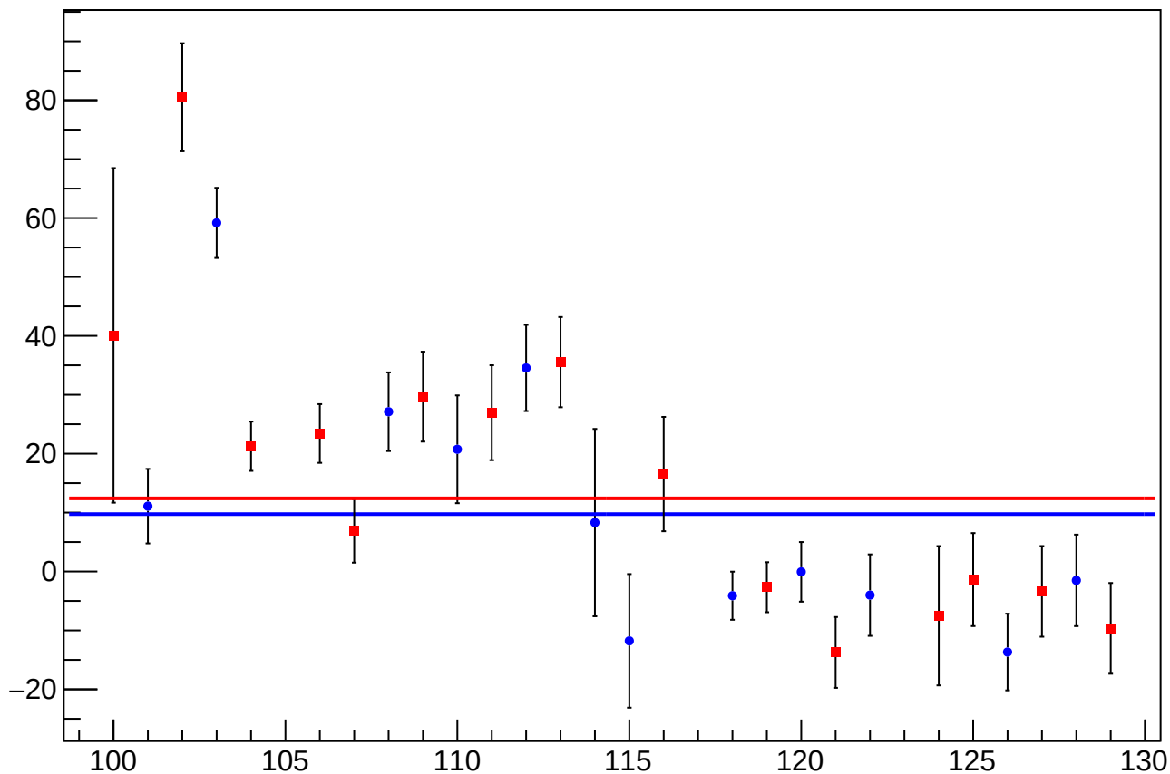
reg_asym_usr_atr2_avg_diff_bpm4aY_slope vs Slug, Sign Corrected
