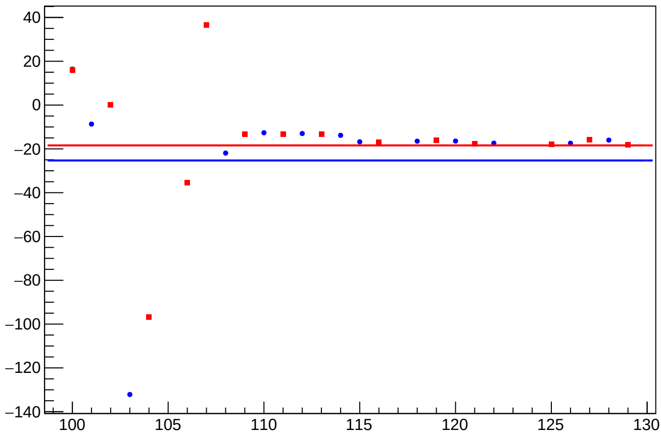
reg_asym_us_avg_at1lr_avg_dd_diff_bpm12X_slope vs Slug, Sign Corrected
