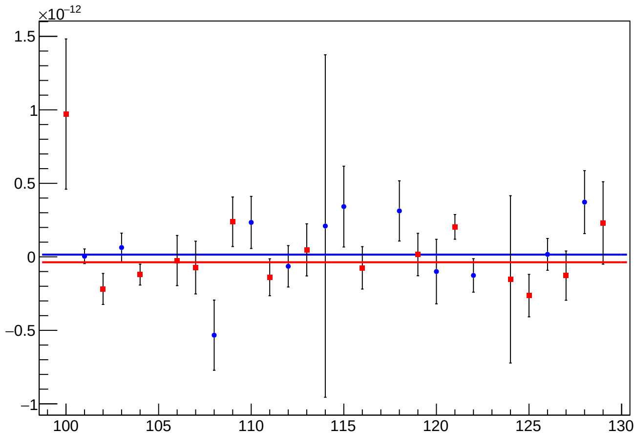
asym_at1_dd_at2_dd_avg_reg_vs_cor_diff_mean vs Slug, Sign Corrected
