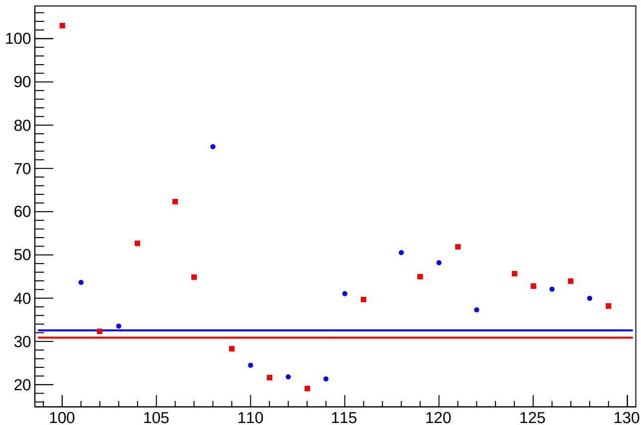
asym_sam_3748_avg_eigen_dit_vs_cor_diff_rms vs Slug, Sign Corrected
