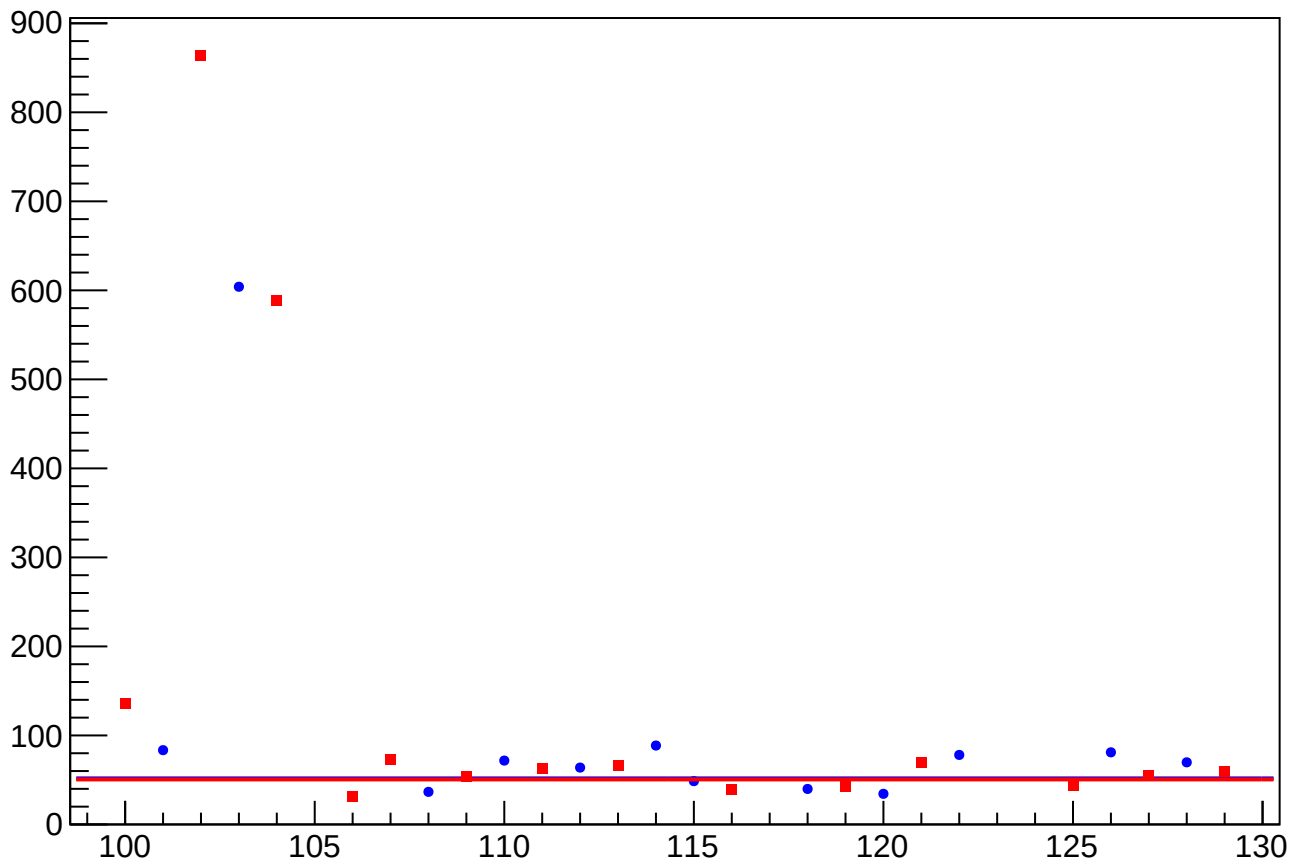
asym_us_dd_at2lr_dd_dd_eigen_dit_vs_eigen_cor_diff_rms vs Slug, Sign Corrected
