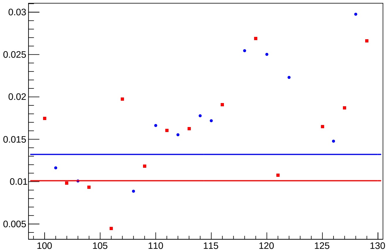
asym_us_avg_atlr_avg_avg_eigen_dit_vs_dit_diff_rms vs Slug, Sign Corrected
