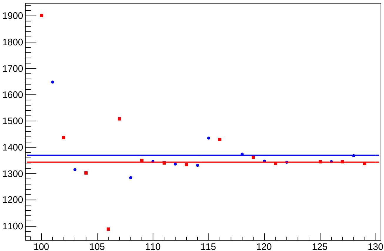
eigen_cor_asym_usl_atl2_avg_rms vs Slug, Sign Corrected
