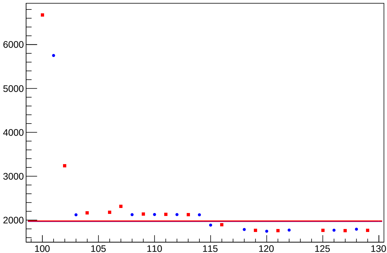
dit_asym_us_avg_at1lr_avg_dd_rms vs Slug, Sign Corrected
