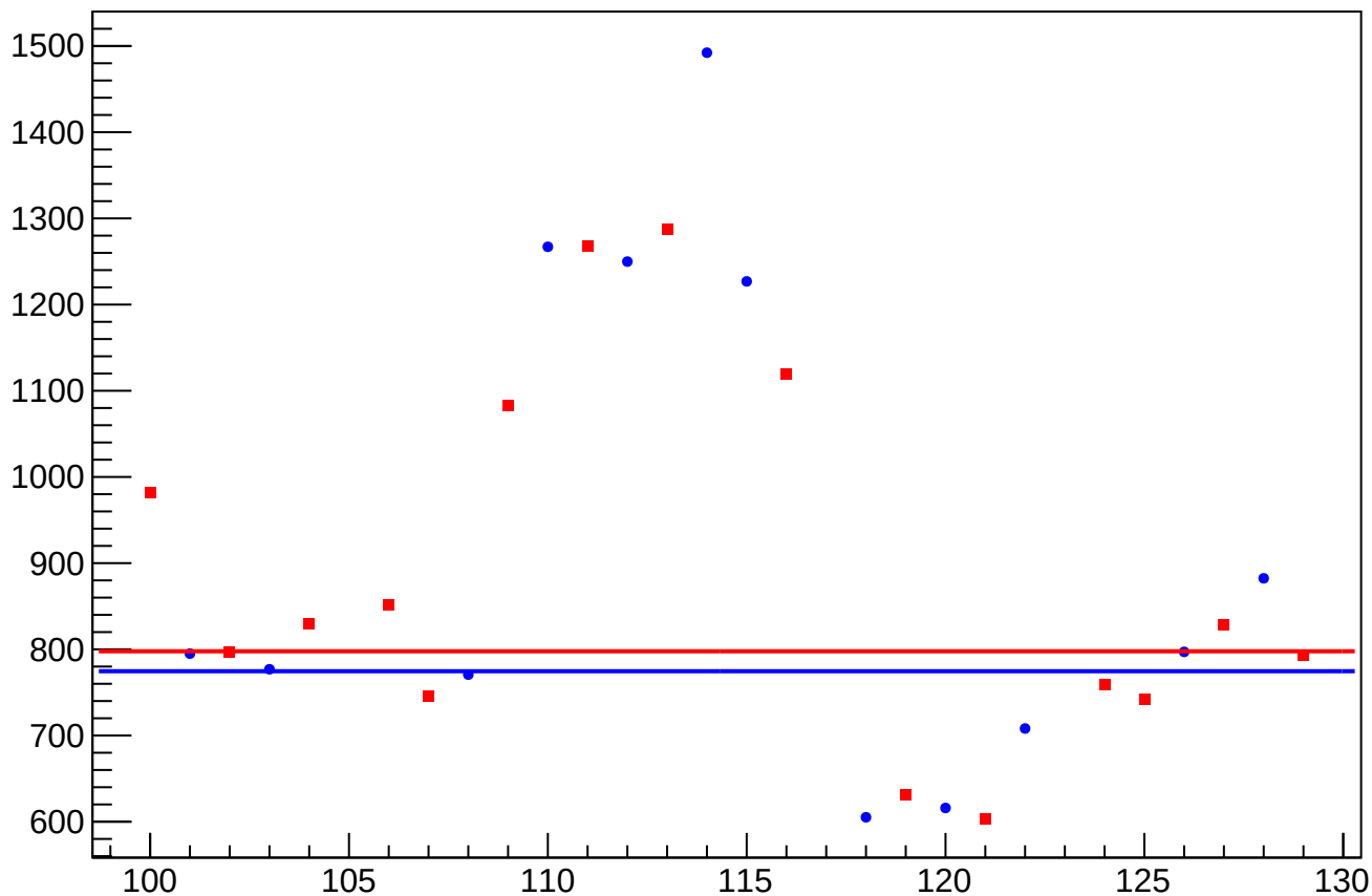
asym_sam_26_48_dd_eigen_cor_correction_rms vs Slug, Sign Corrected
