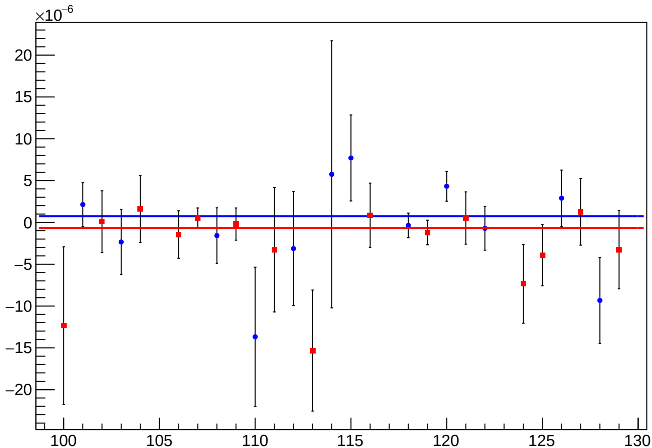
asym_sam_12345678_avg_eigen_dit_vs_dit_diff_mean vs Slug, Sign Corrected
