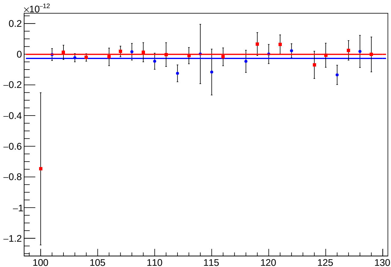
asym_usr_atr1_avg_eigen_cor_vs_cor_diff_mean vs Slug, Sign Corrected
