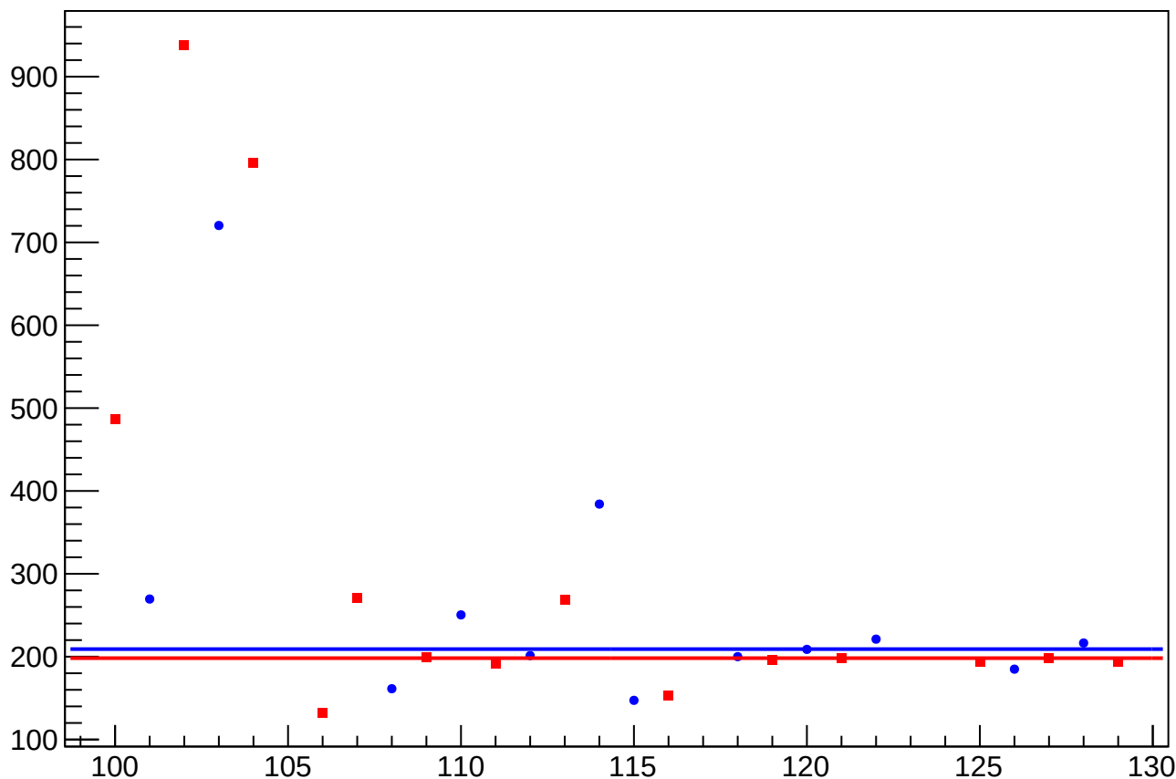
asym_us_avg_atlr_avg_avg_eigen_dit_vs_eigen_cor_diff_rms vs Slug, Sign Corrected
