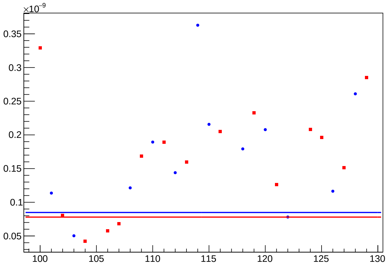
asym_usr_atr2_dd_reg_vs_cor_diff_rms vs Slug, Sign Corrected
