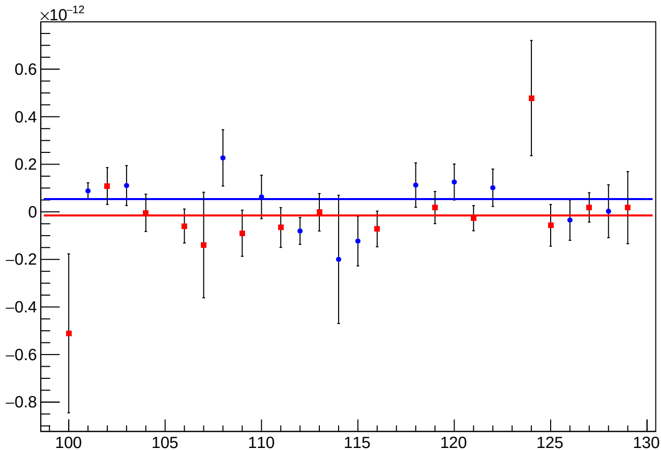
asym_sam_24_68_dd_eigen_cor_vs_cor_diff_mean vs Slug, Sign Corrected
