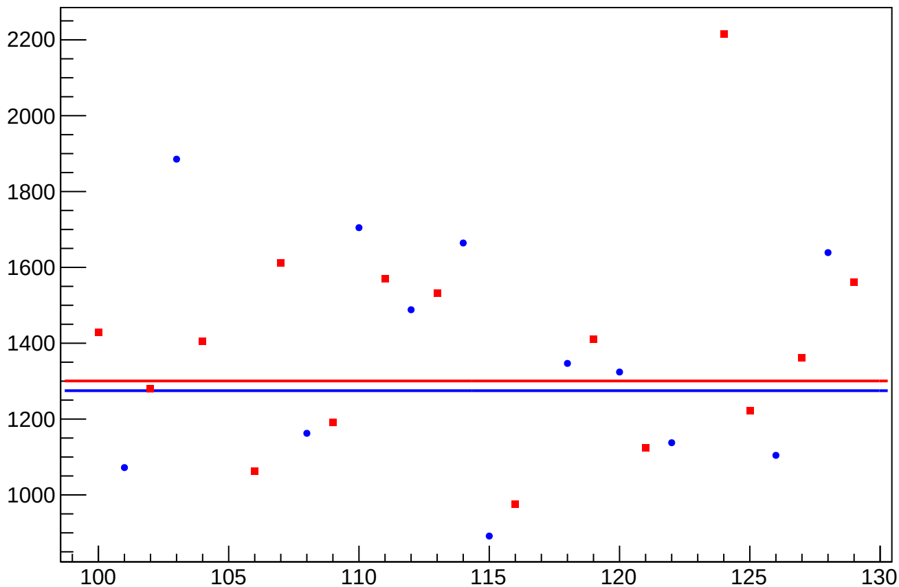
asym_atl_dd_atr_dd_dd_reg_correction_rms vs Slug, Sign Corrected
