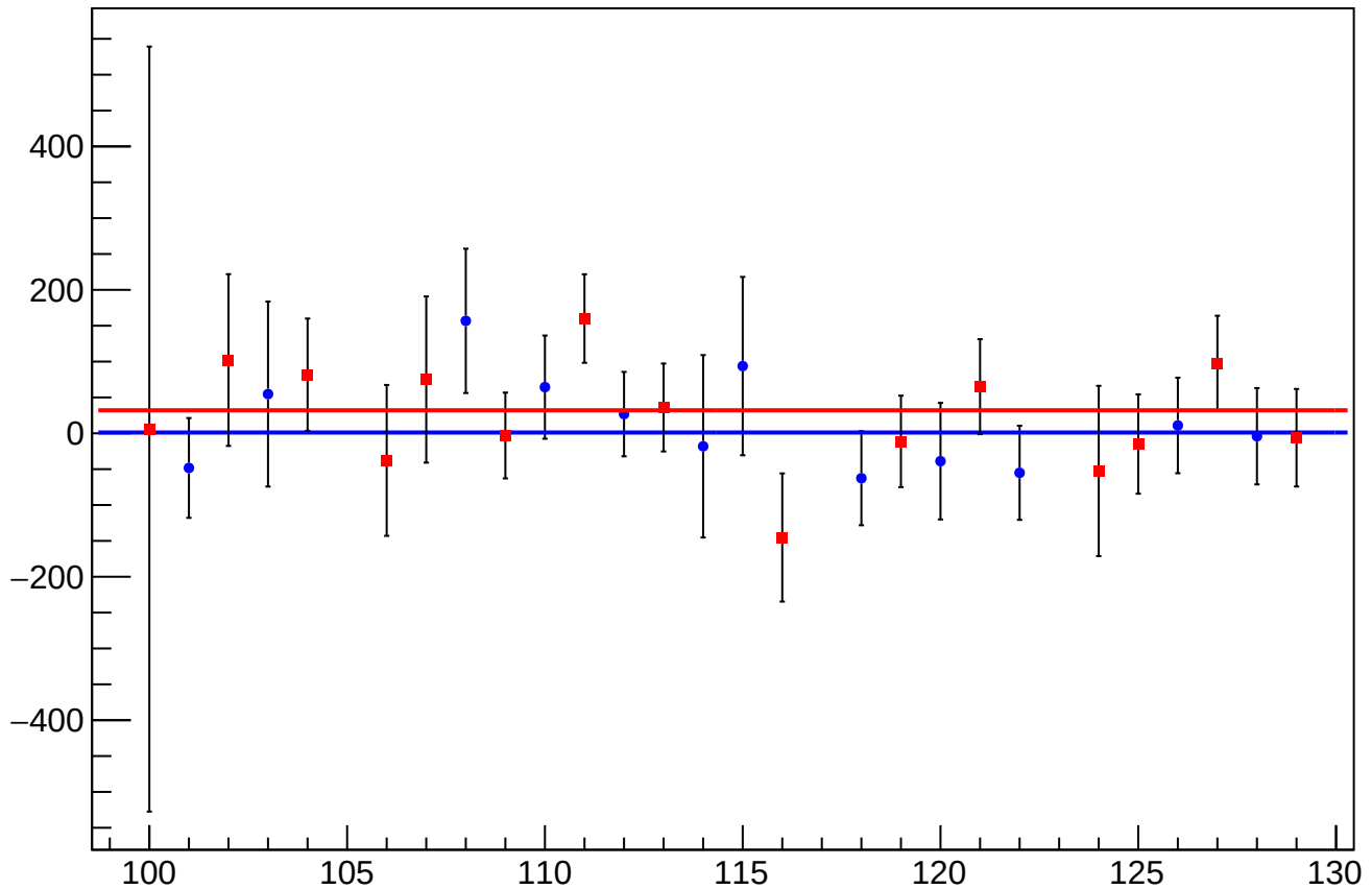
eigen_cor_asym_sam_15_37_dd_mean vs Slug, Sign Corrected
