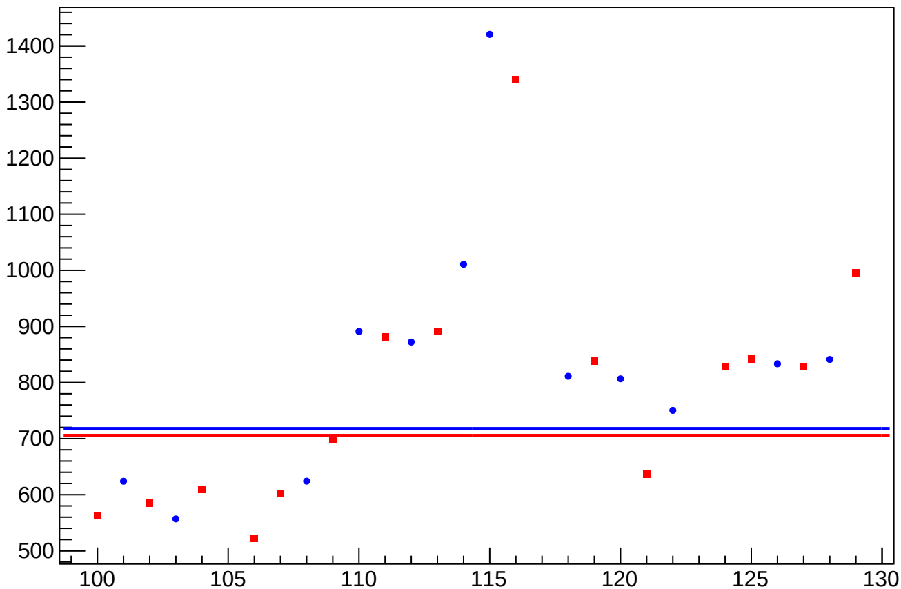
asym_sam_15_dd_eigen_cor_correction_rms vs Slug, Sign Corrected
