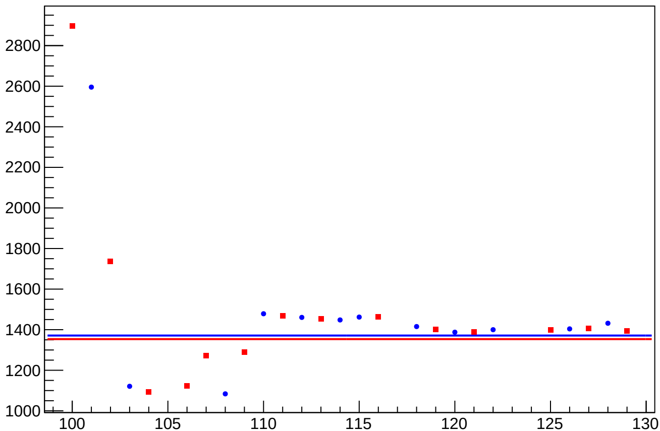
eigen_cor_asym_us_dd_at2lr_dd_dd_rms vs Slug, Sign Corrected
