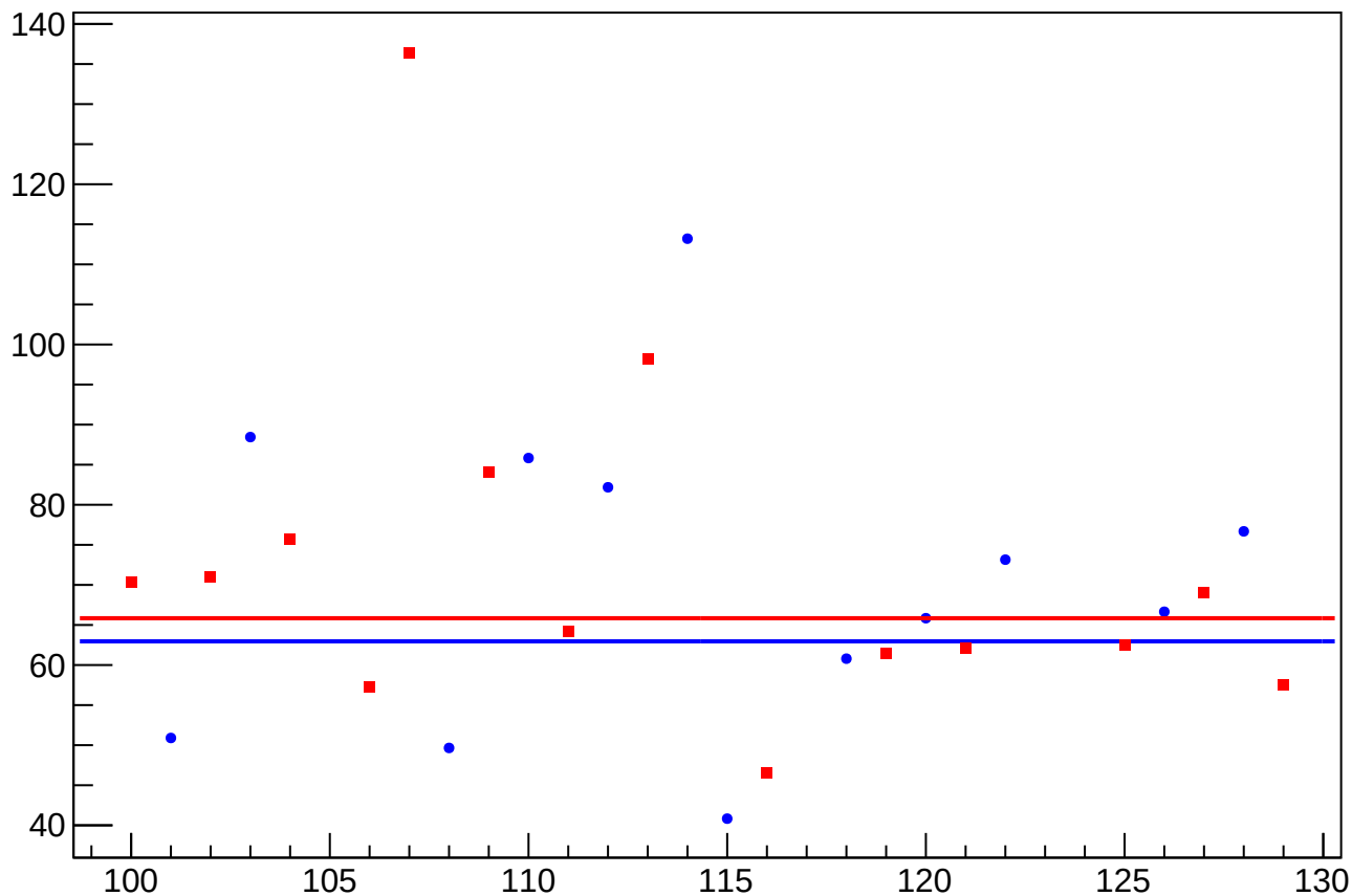
asym_usl_dit_vs_overload_cor_diff_rms vs Slug, Sign Corrected
