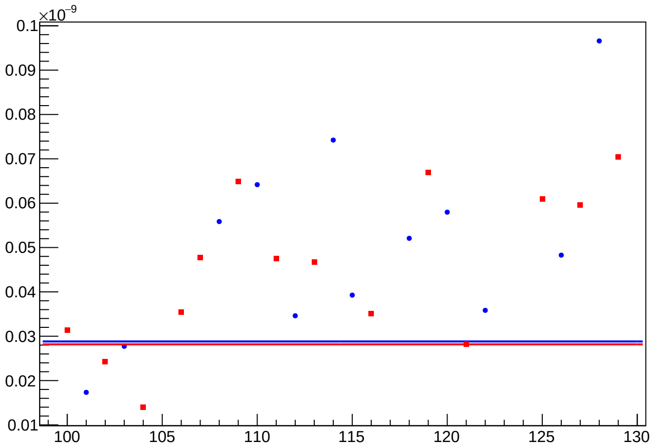
asym_us_avg_eigen_cor_vs_cor_diff_rms vs Slug, Sign Corrected
