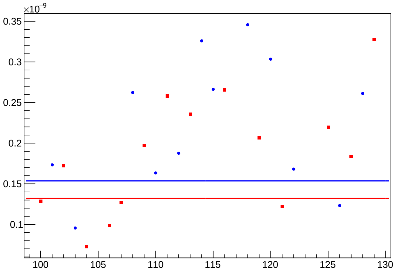
asym_us_avg_at2lr_avg_dd_eigen_cor_vs_cor_diff_rms vs Slug, Sign Corrected
