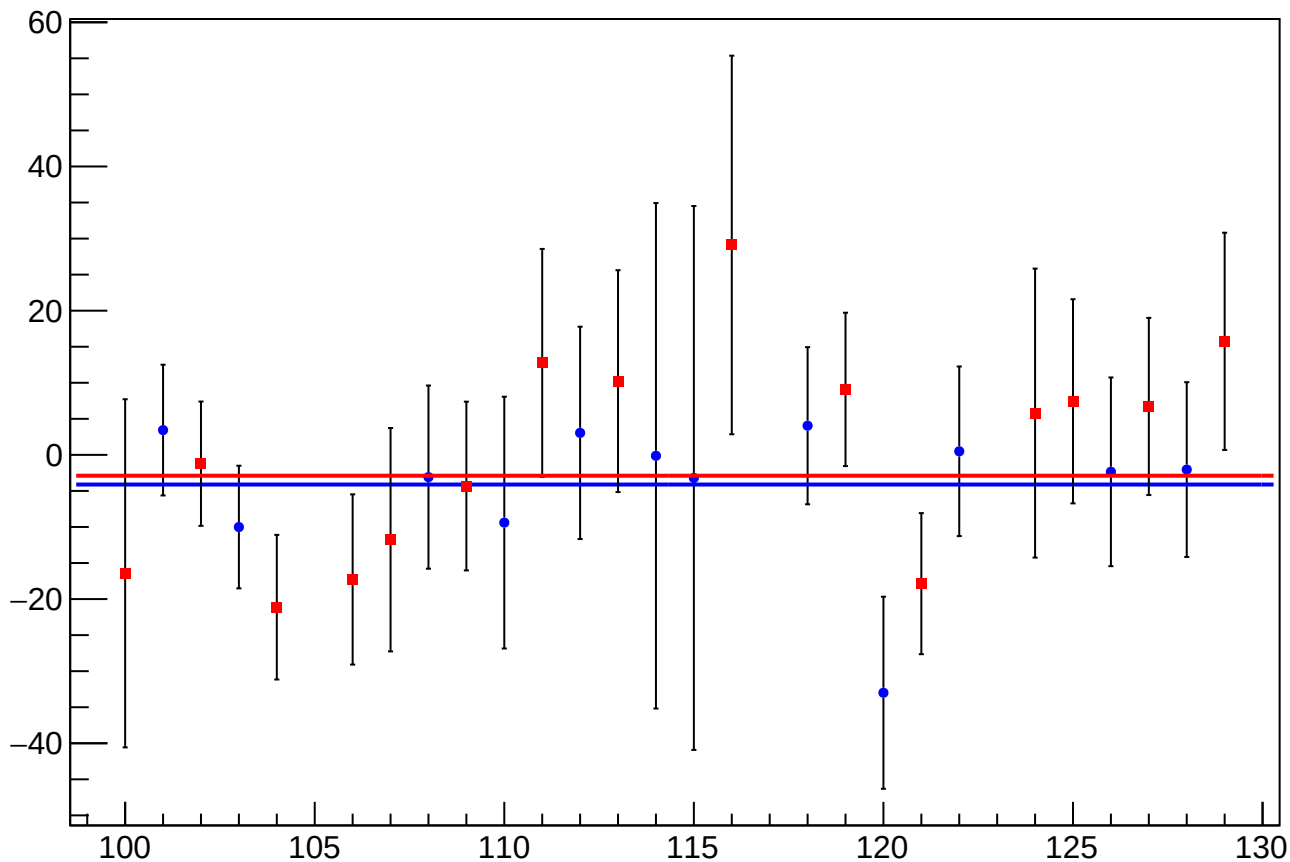
diff_bpm_4aY_4eY_avg_mean vs Slug, Sign Corrected
