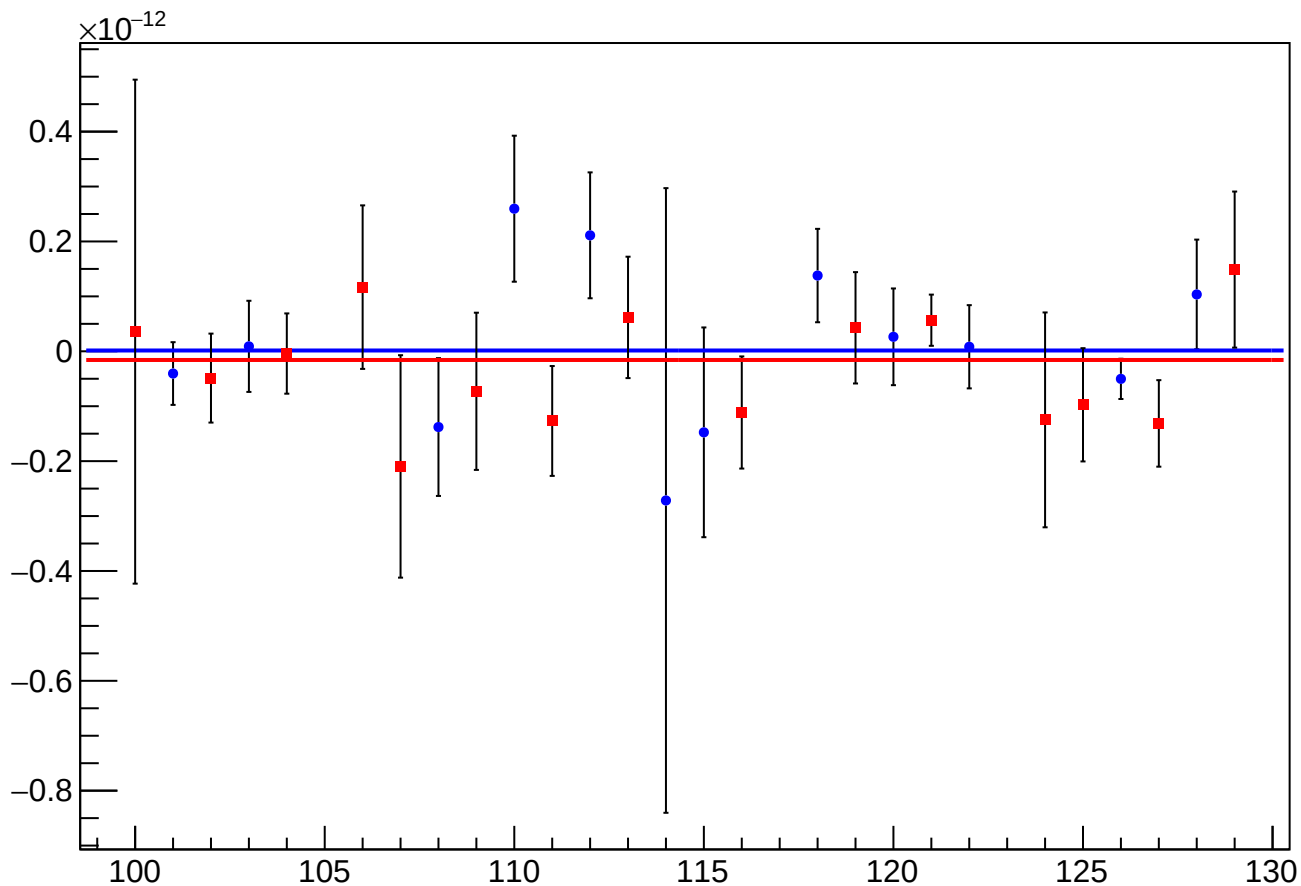
asym_sam_15_26_dd_reg_vs_cor_diff_mean vs Slug, Sign Corrected
