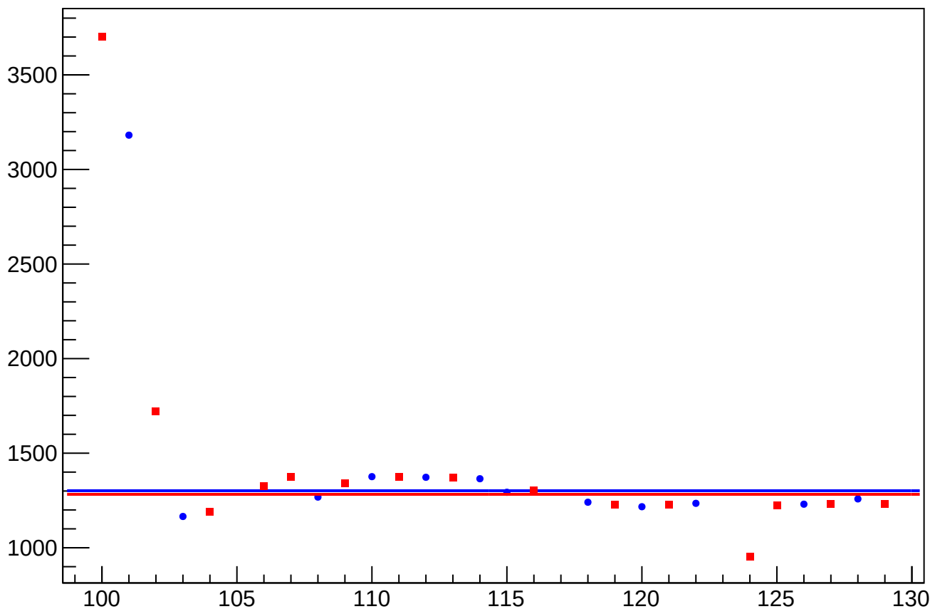
dit_asym_at1_avg_at2_avg_dd_rms vs Slug, Sign Corrected
