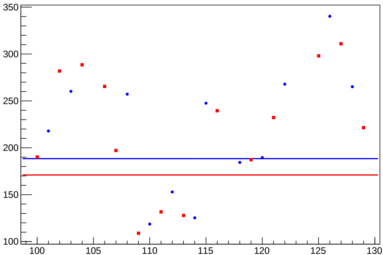
asym_bcm_dg_us_an_us_avg_rms vs Slug, Sign Corrected
