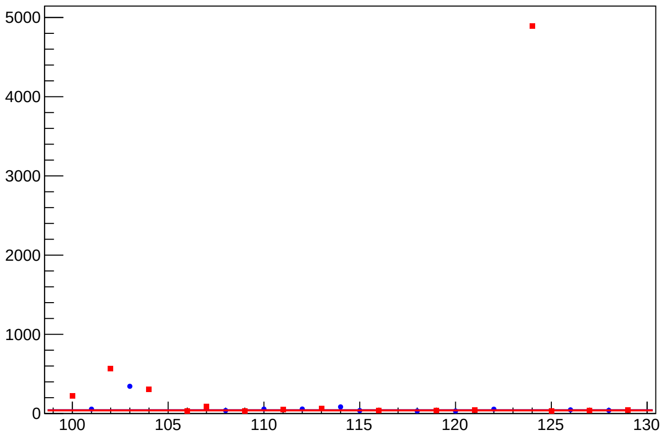
asym_at1_dd_at2_dd_avg_dit_vs_eigen_cor_diff_rms vs Slug, Sign Corrected
