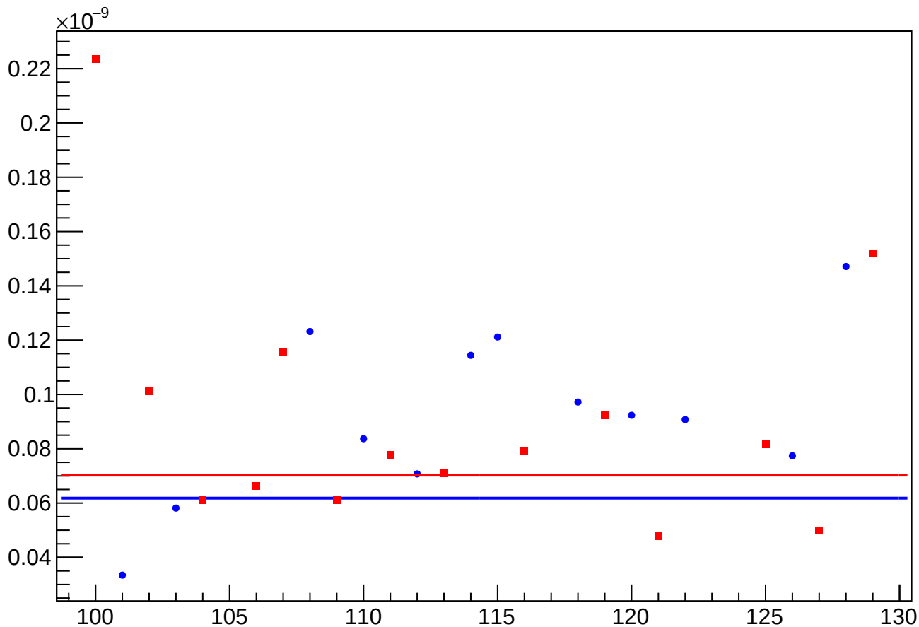
asym_us_dd_at2lr_dd_avg_eigen_cor_vs_cor_diff_rms vs Slug, Sign Corrected
