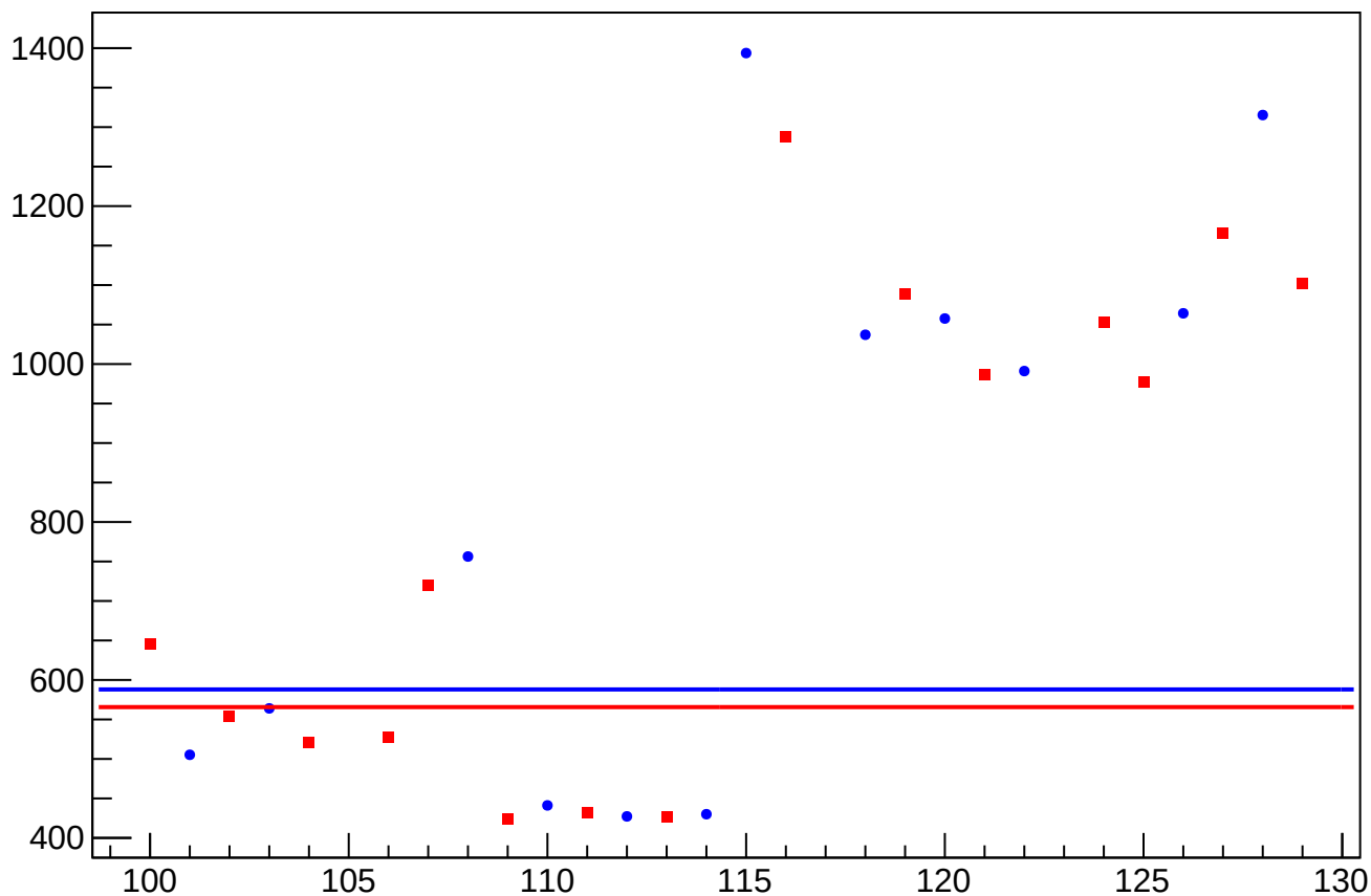
asym_sam_1548_avg_cor_correction_rms vs Slug, Sign Corrected
