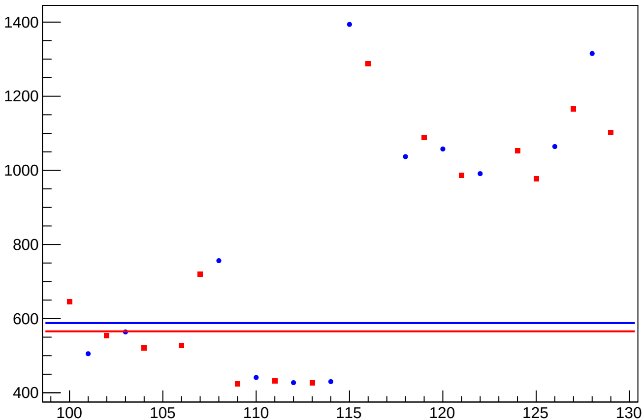
asym_sam_1548_avg_eigen_cor_correction_rms vs Slug, Sign Corrected
