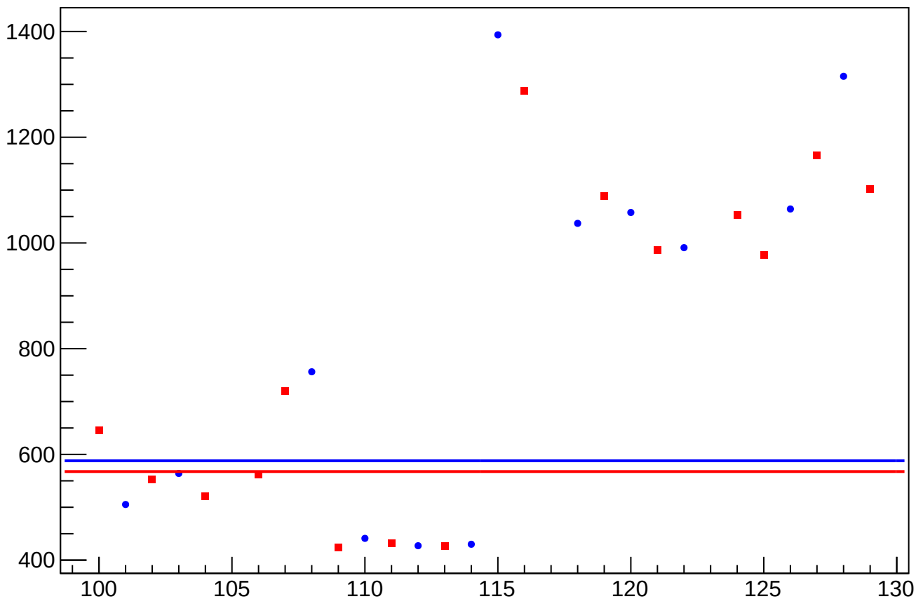
asym_sam_1548_avg_reg_correction_rms vs Slug, Sign Corrected
