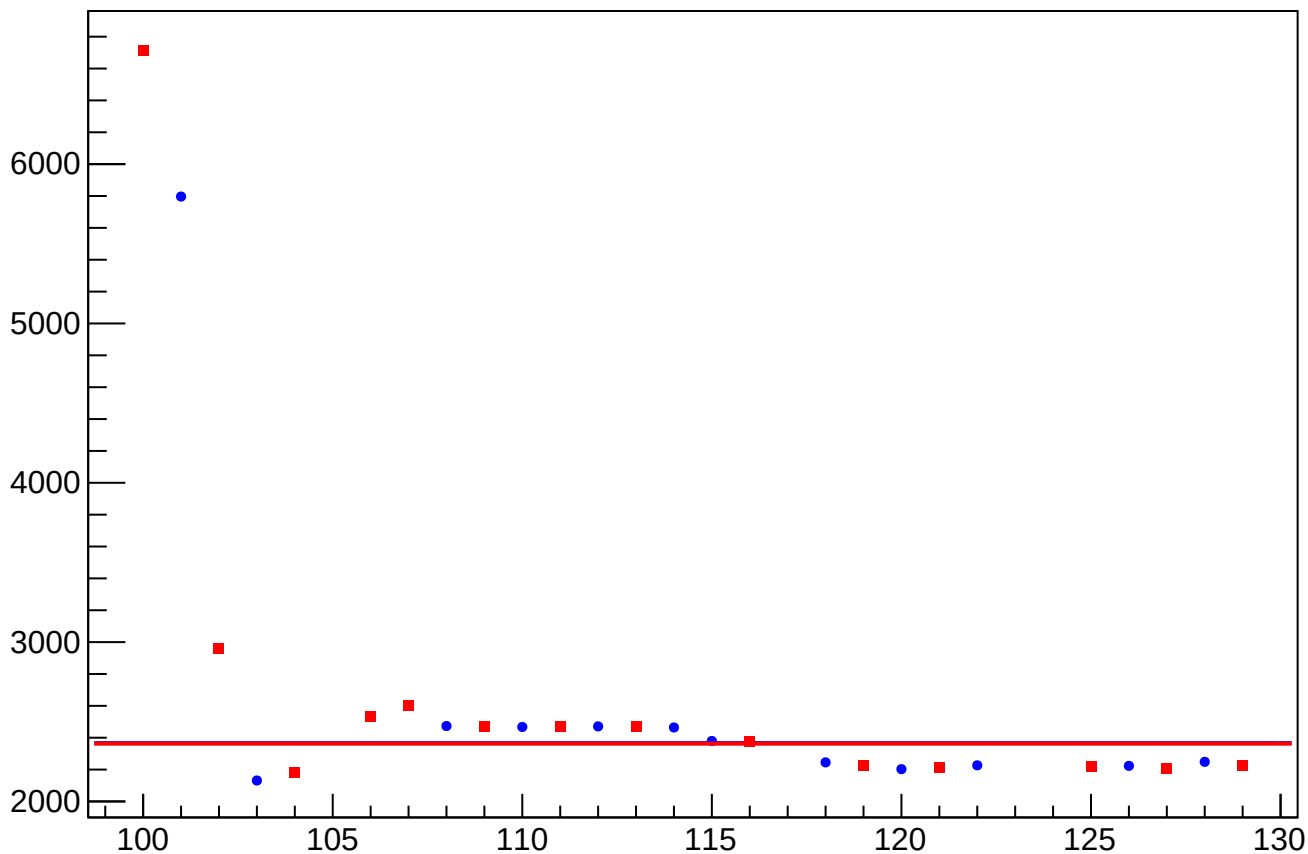
cor_asym_us_dd_at1lr_dd_avg_rms vs Slug, Sign Corrected
