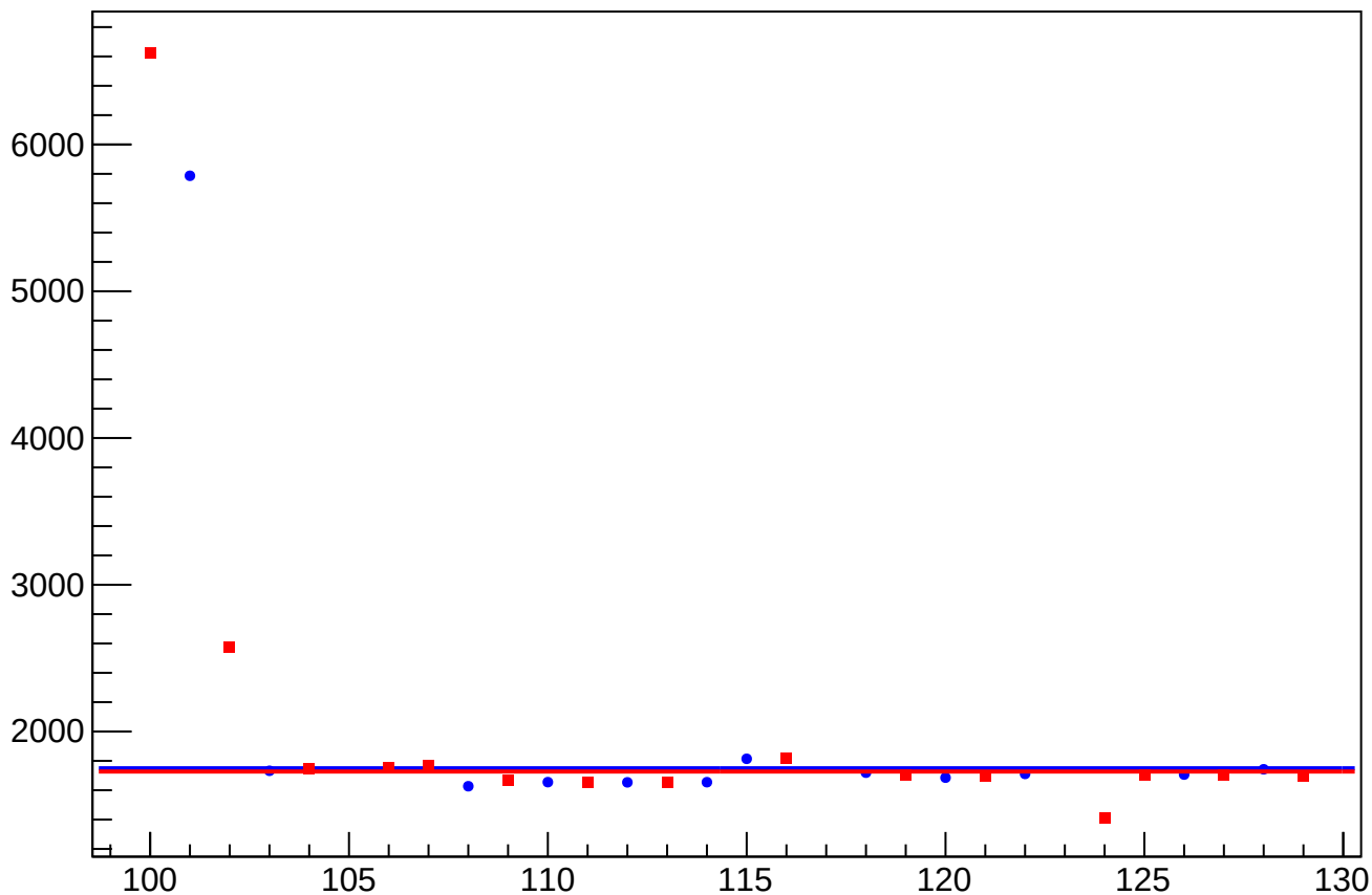
eigen_dit_asym_atr1l2_avg_rms vs Slug, Sign Corrected
