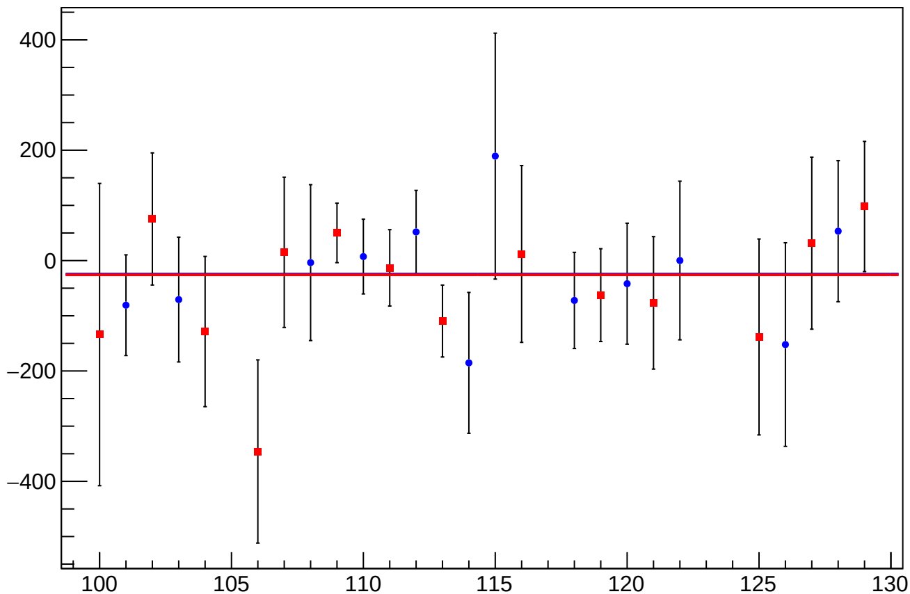
asym_bcm_2an_us_an_ds_dd_mean vs Slug, Sign Corrected
