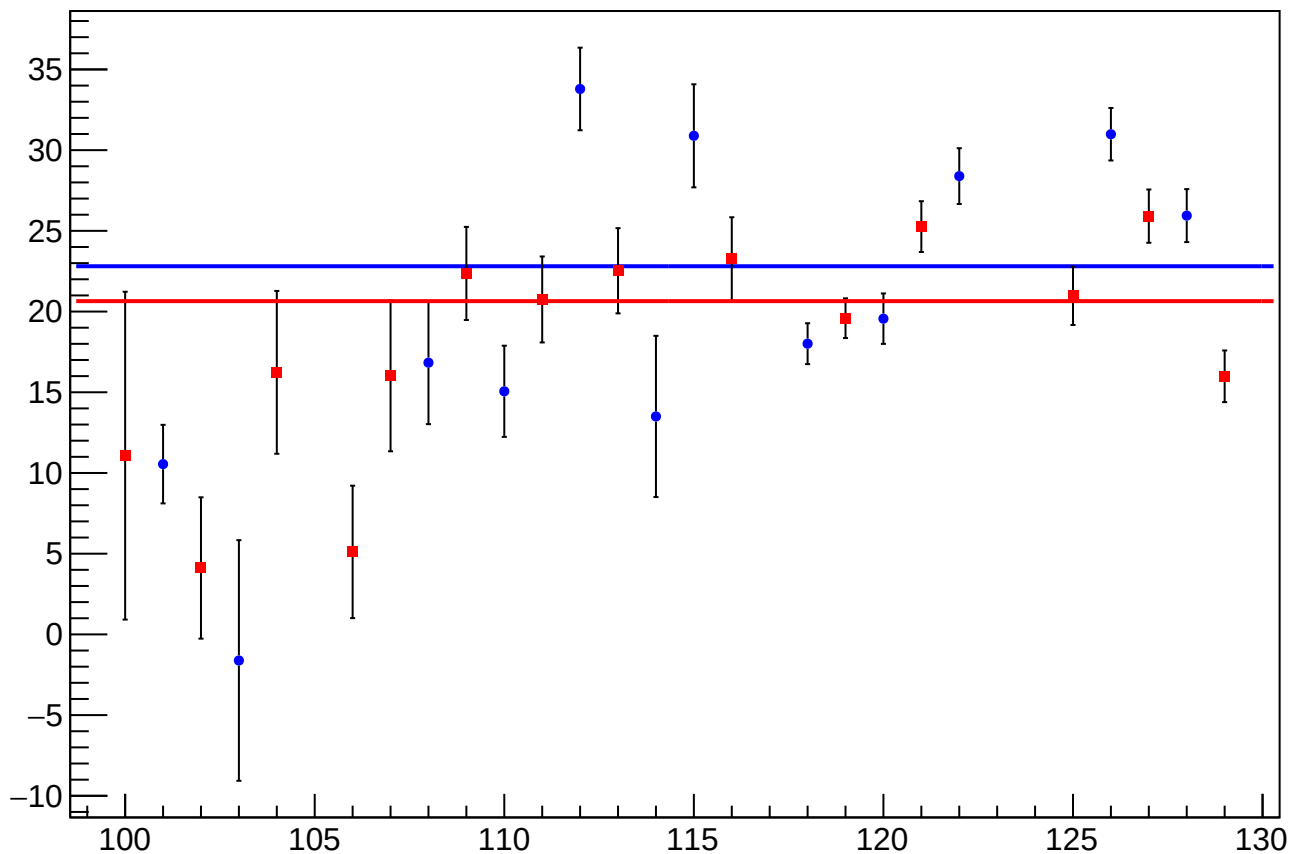
reg_asym_usl_atl1_dd_diff_bpm4eY_slope vs Slug, Sign Corrected
