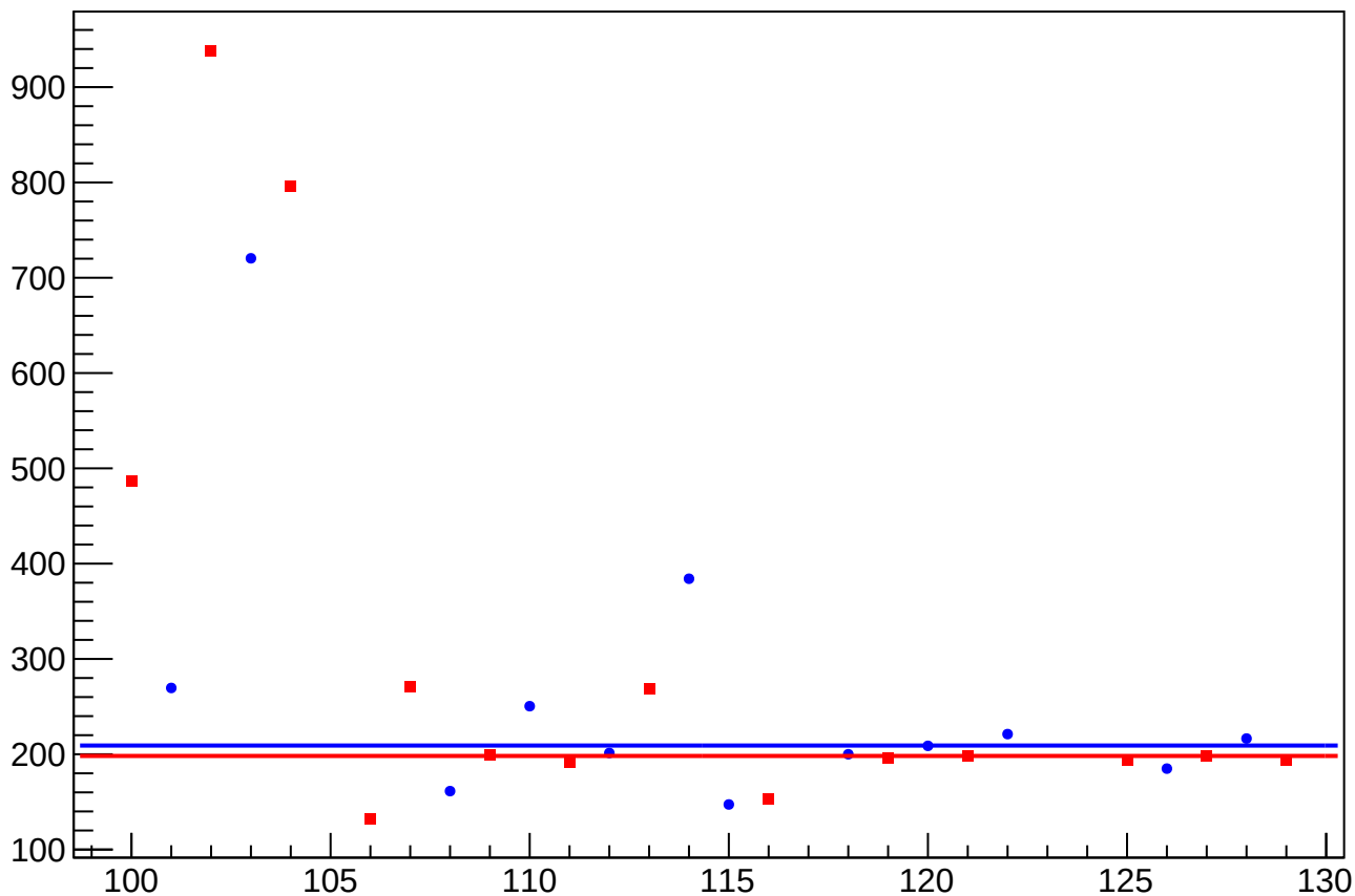
asym_us_avg_atlr_avg_avg_eigen_dit_vs_cor_diff_rms vs Slug, Sign Corrected
