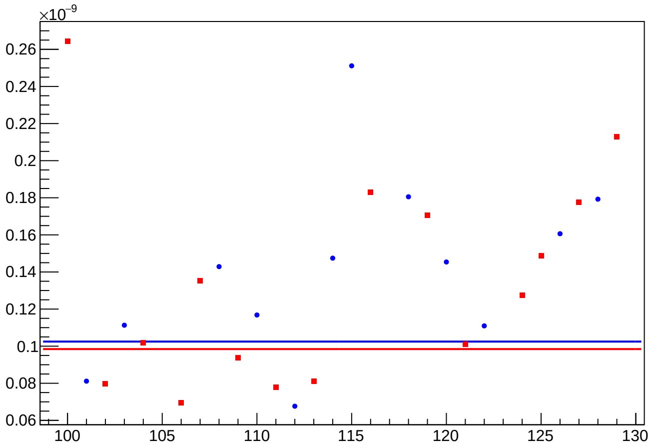
asym_sam4_reg_vs_cor_diff_rms vs Slug, Sign Corrected
