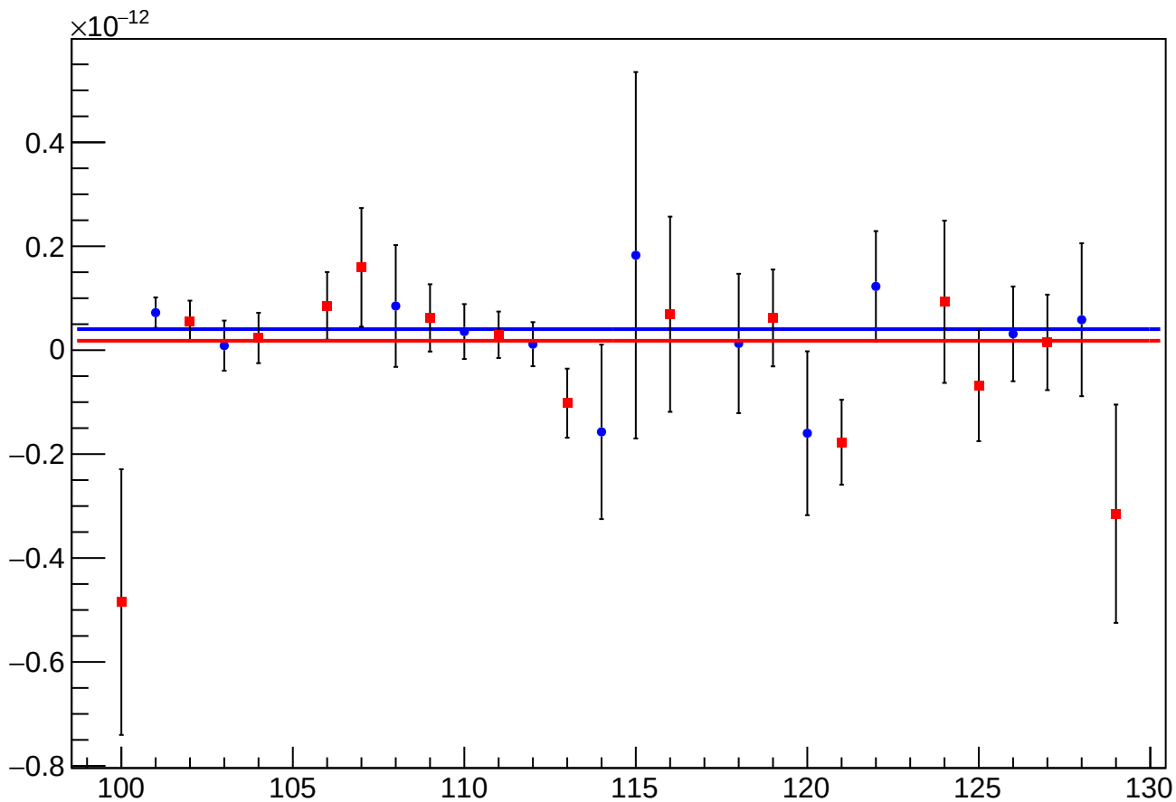
asym_sam_1548_avg_reg_vs_cor_diff_mean vs Slug, Sign Corrected
