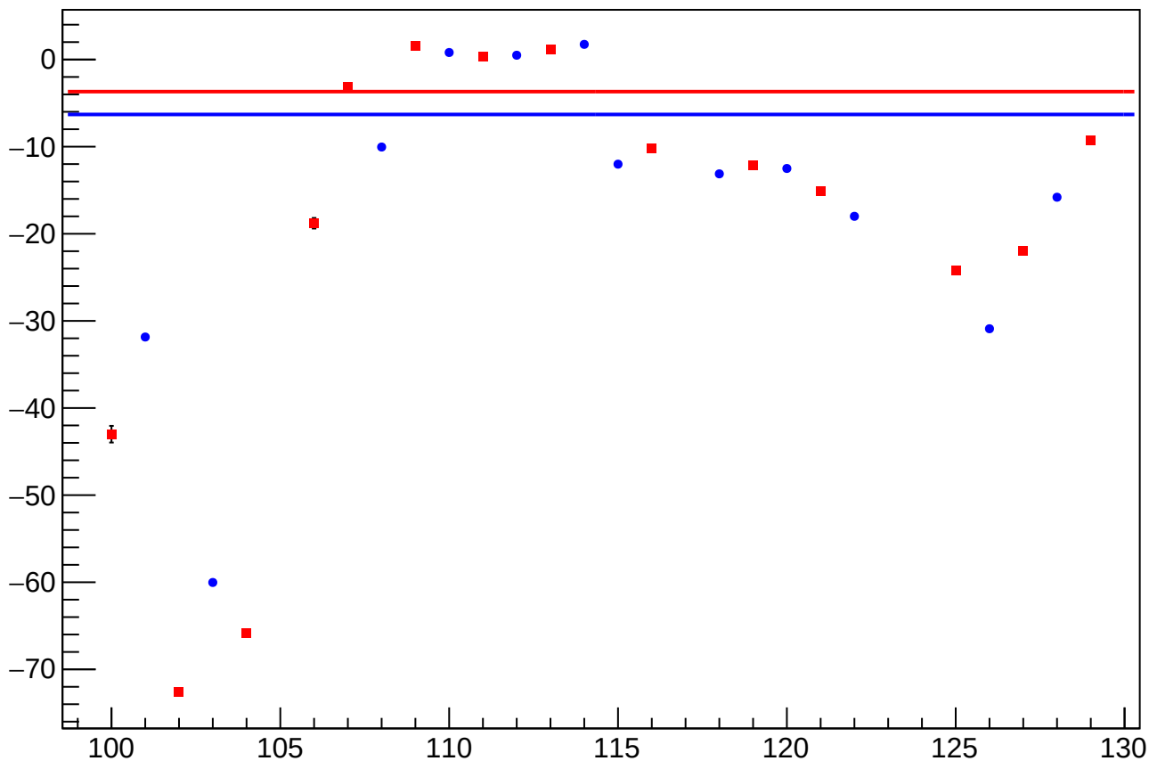
reg_asym_bcm_2an_us_an_ds_avg_diff_bpm1X_slope vs Slug, Sign Corrected
