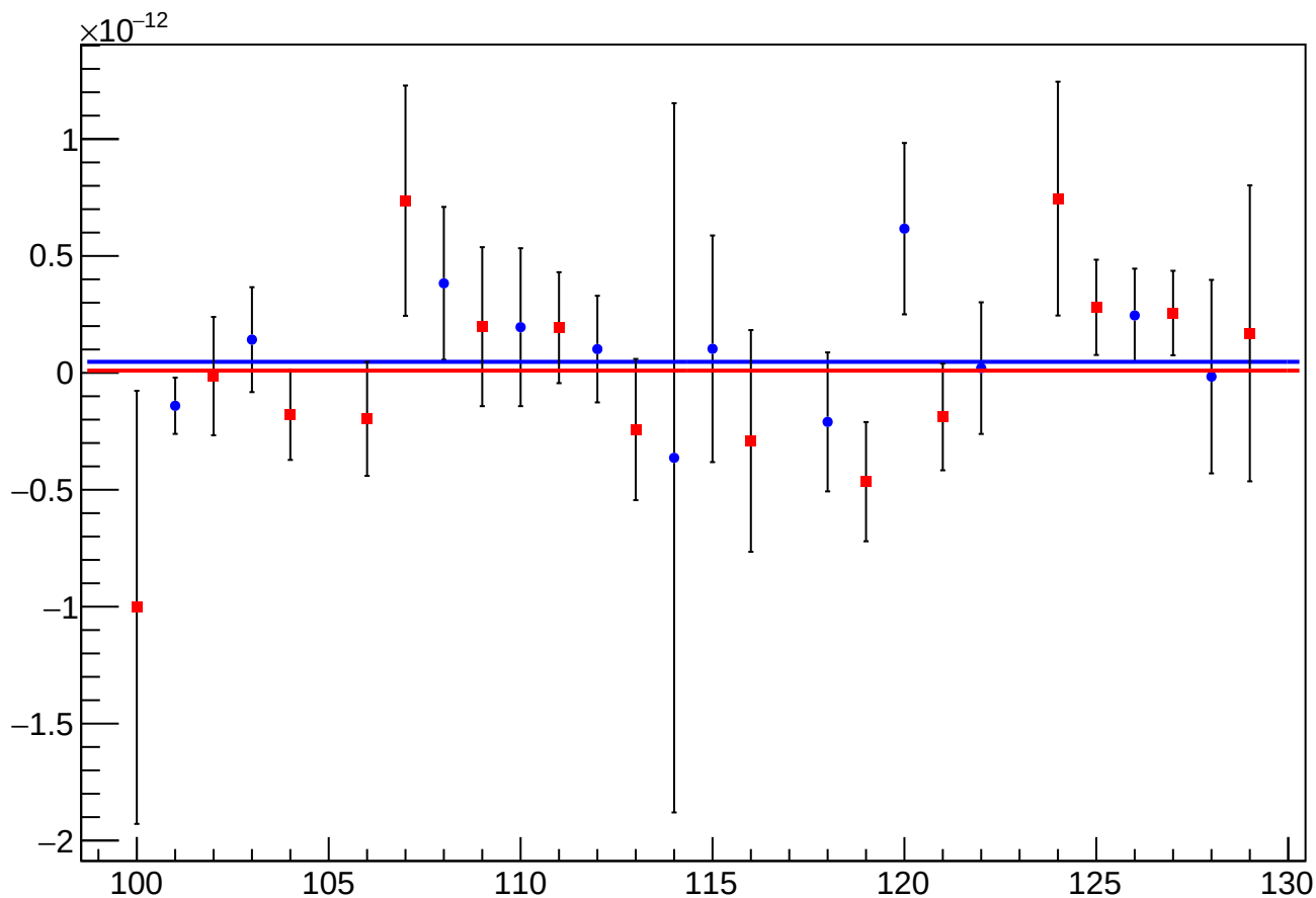
asym_sam_26_dd_reg_vs_cor_diff_mean vs Slug, Sign Corrected
