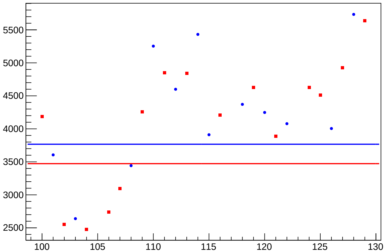
asym_atr_dd_dit_correction_rms vs Slug, Sign Corrected
