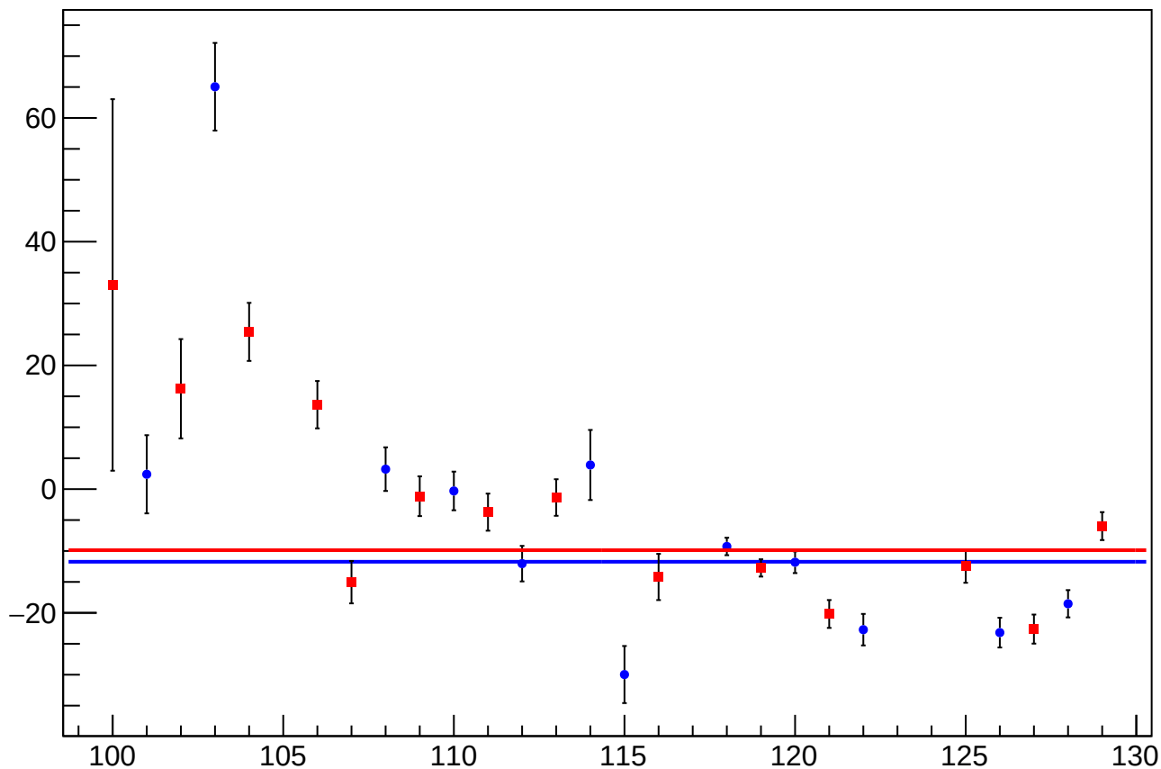
reg_asym_us_avg_at1lr_avg_dd_diff_bpm4aY_slope vs Slug, Sign Corrected
