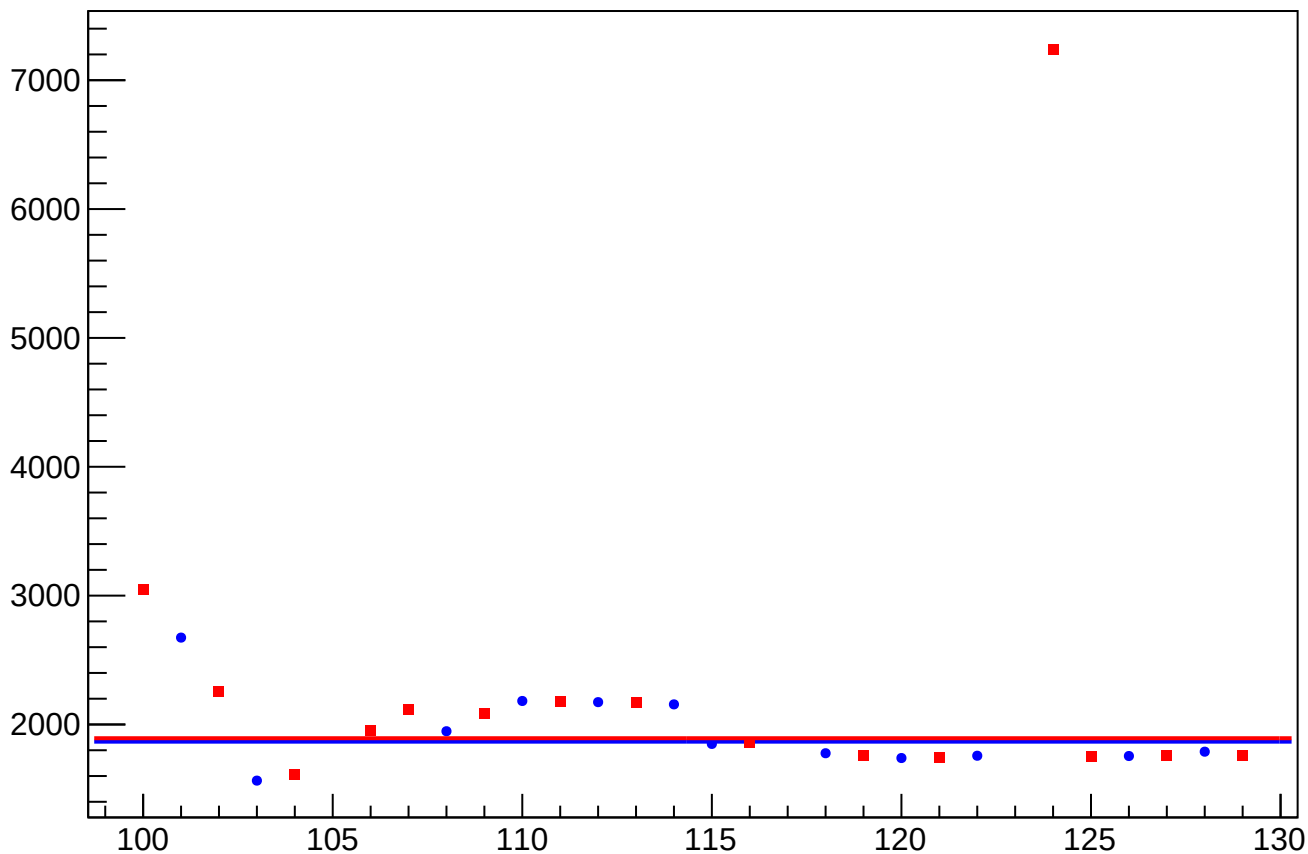
eigen_cor_asym_atl1r2_dd_rms vs Slug, Sign Corrected
