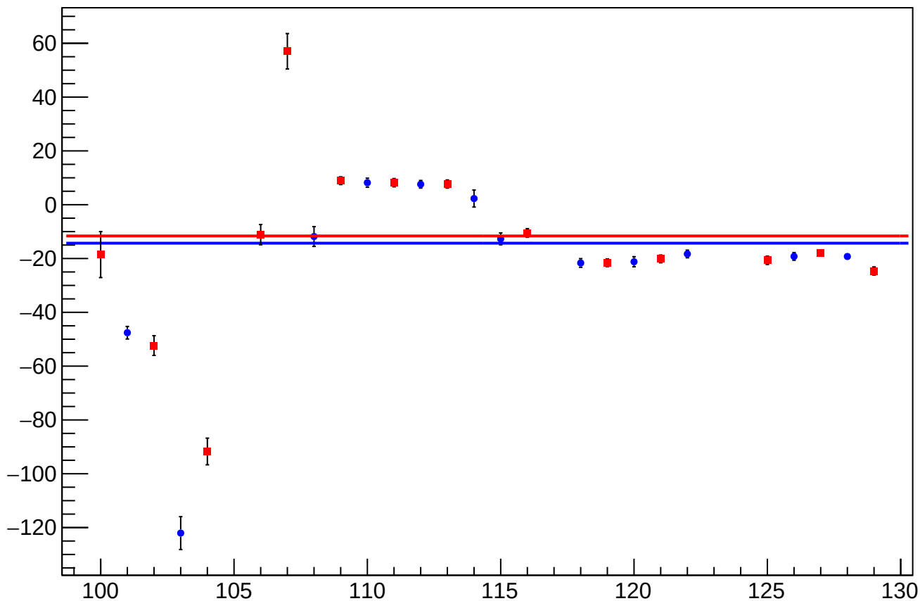
reg_asym_usl_atl1_dd_diff_bpm1X_slope vs Slug, Sign Corrected
