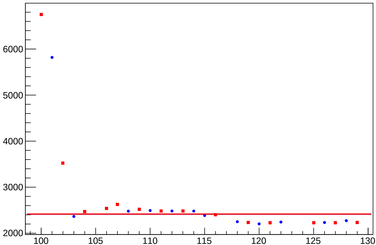
eigen_dit_asym_us_avg_at1lr_avg_avg_rms vs Slug, Sign Corrected
