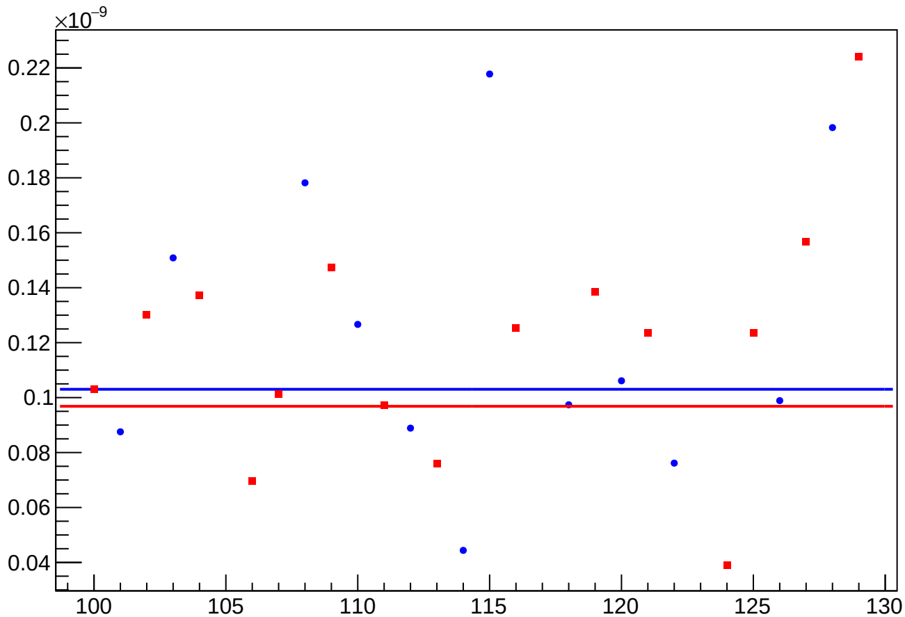
asym_atl_dd_reg_vs_cor_diff_rms vs Slug, Sign Corrected
