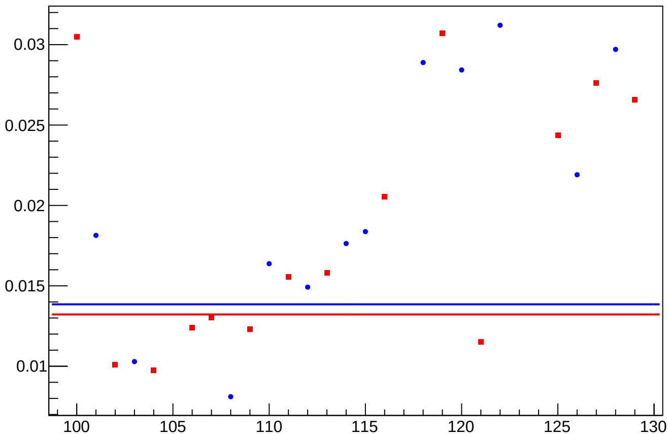
asym_us_avg_at2lr_avg_dd_eigen_dit_vs_dit_diff_rms vs Slug, Sign Corrected
