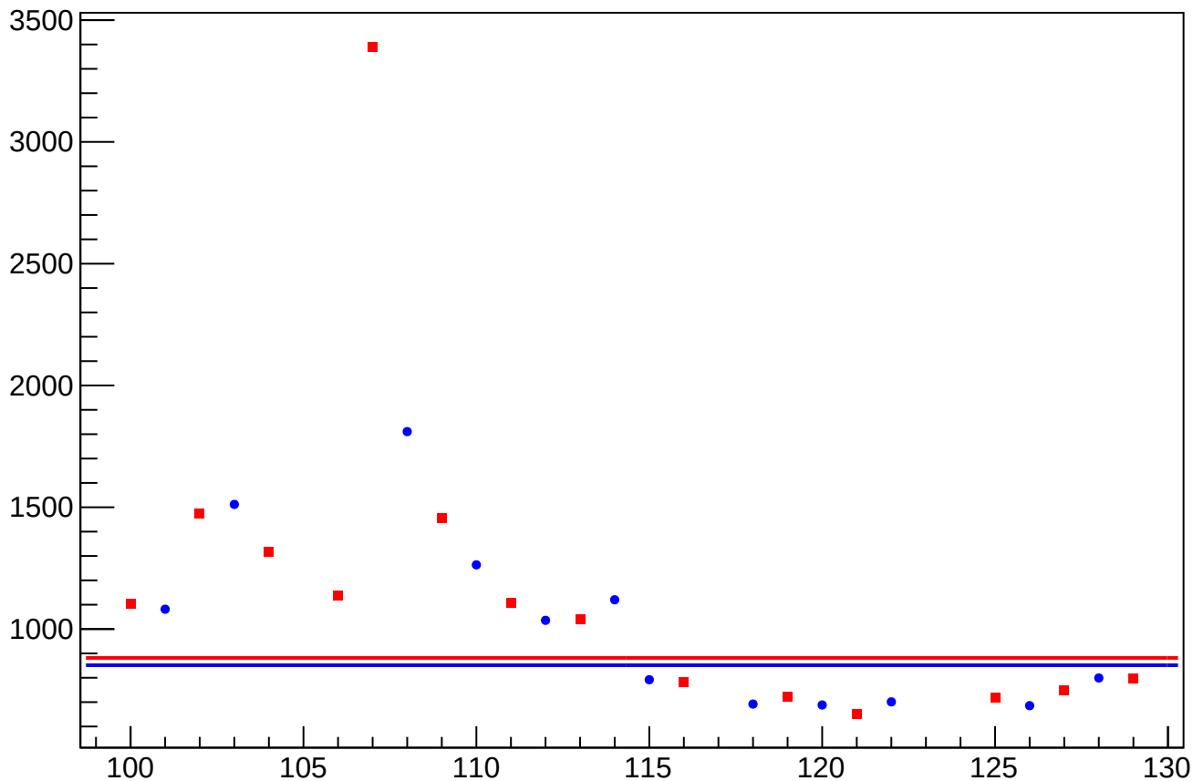
asym_usl_reg_correction_rms vs Slug, Sign Corrected
