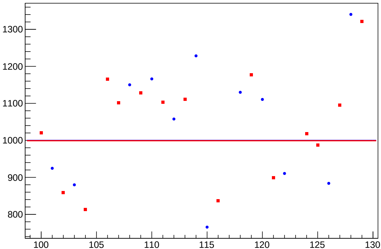
asym_usr_atr1_dd_dit_correction_rms vs Slug, Sign Corrected
