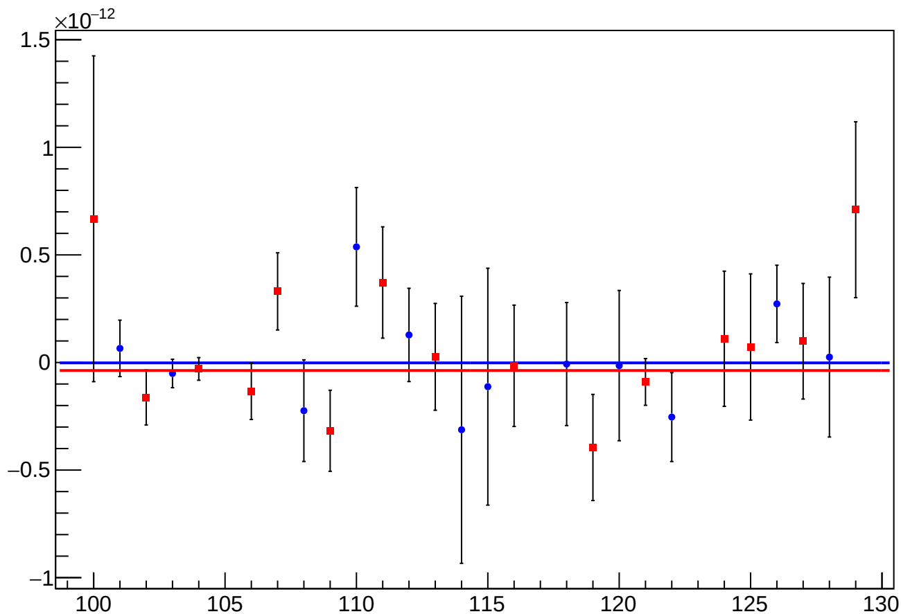
asym_usr_atr2_dd_eigen_cor_vs_cor_diff_mean vs Slug, Sign Corrected
