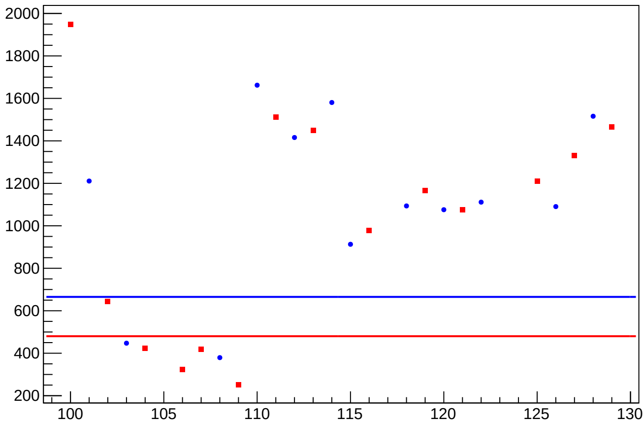
asym_us_dd_at2lr_dd_dd_eigen_cor_correction_rms vs Slug, Sign Corrected
