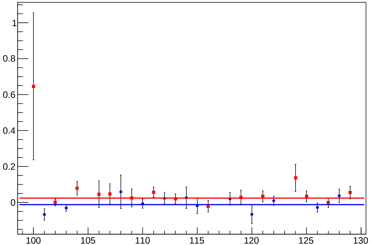
asym_sam_15_37_dd_dit_vs_cor_diff_mean vs Slug, Sign Corrected
