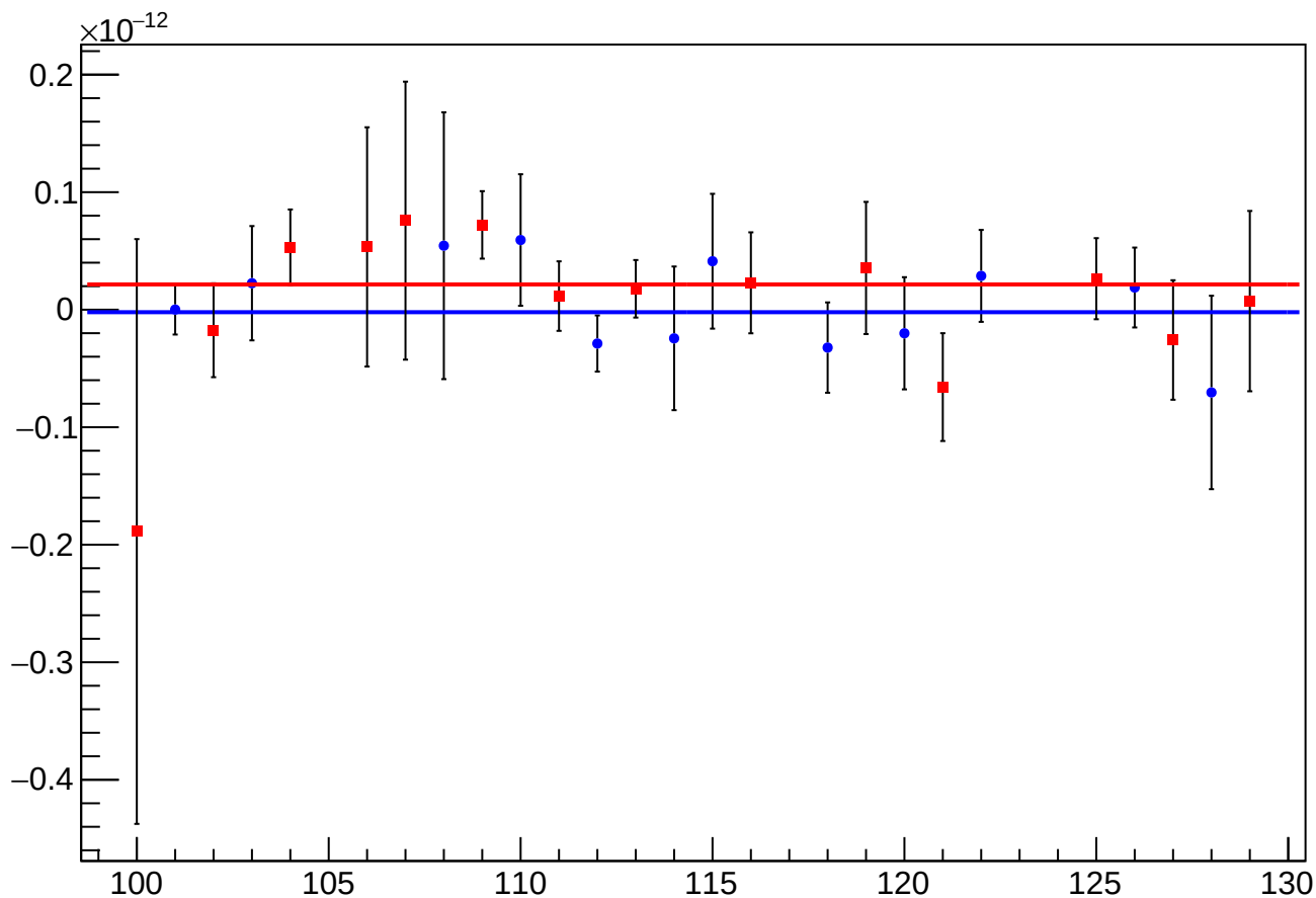
asym_us_dd_eigen_cor_vs_cor_diff_mean vs Slug, Sign Corrected
