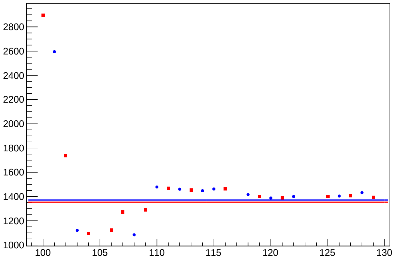
cor_asym_us_dd_at2lr_dd_dd_rms vs Slug, Sign Corrected
