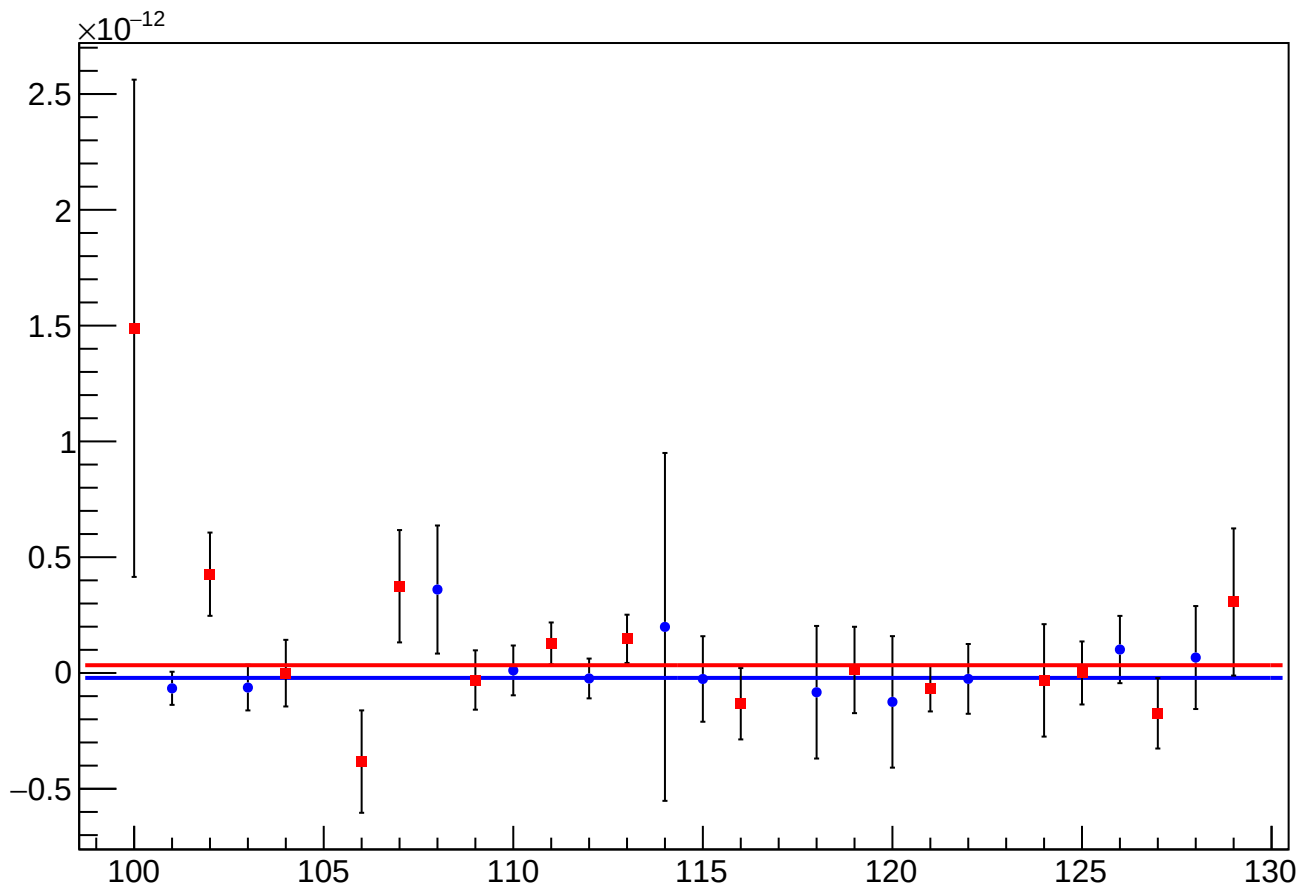
asym_sam3_reg_vs_cor_diff_mean vs Slug, Sign Corrected
