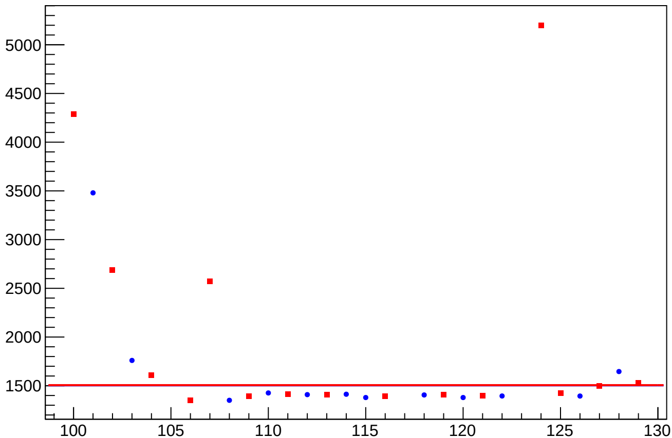
asym_atl1r2_dd_atl2r1_dd_avg_rms vs Slug, Sign Corrected
