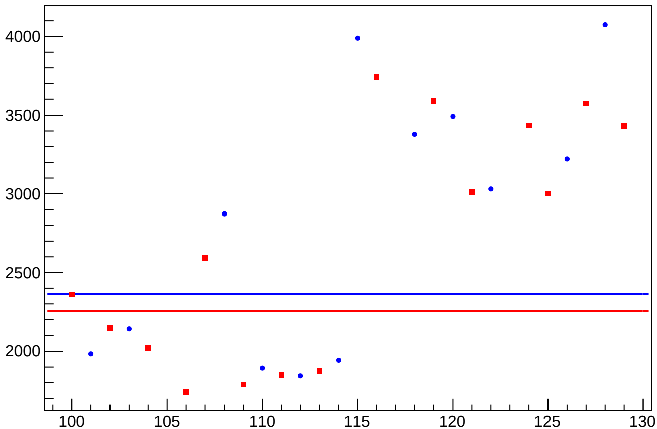
asym_sam4_cor_correction_rms vs Slug, Sign Corrected
