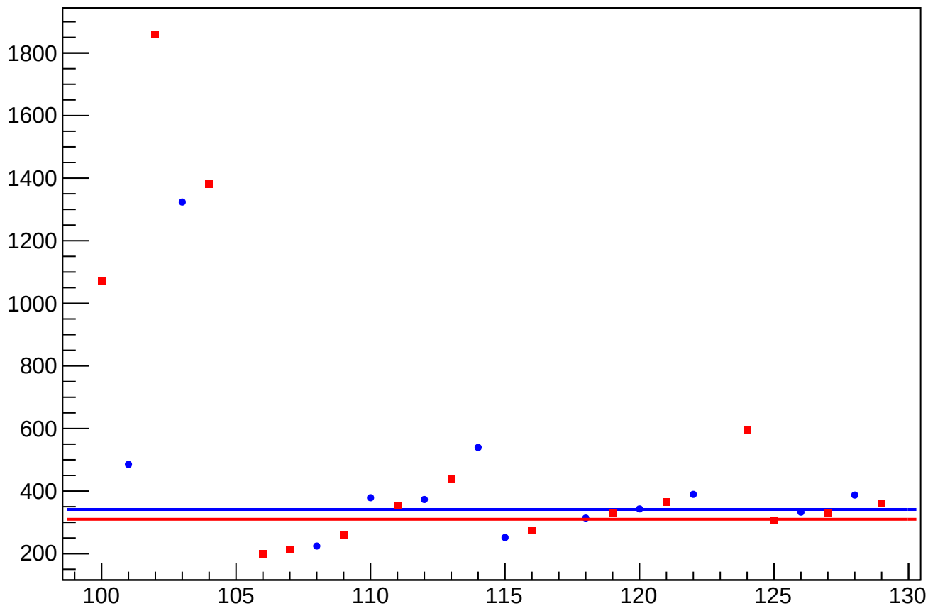
asym_atr2_dit_vs_eigen_cor_diff_rms vs Slug, Sign Corrected
