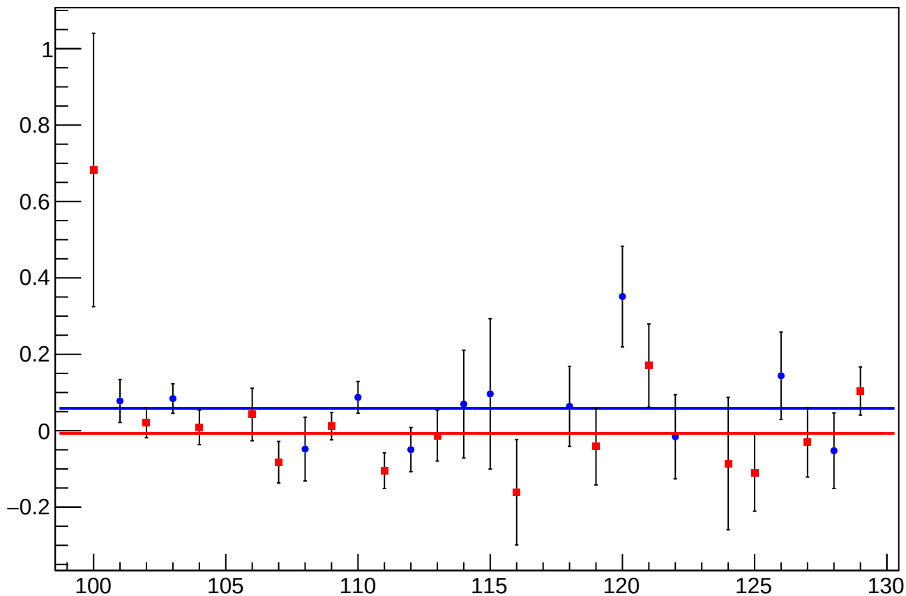
asym_sam6_dit_vs_eigen_cor_diff_mean vs Slug, Sign Corrected
