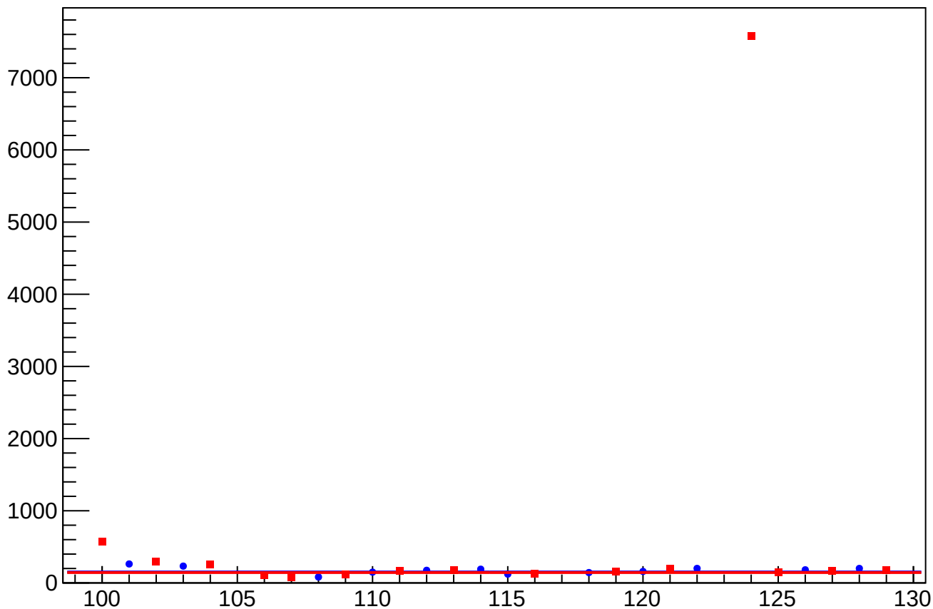
asym_atl1r2_dd_eigen_dit_vs_eigen_cor_diff_rms vs Slug, Sign Corrected
