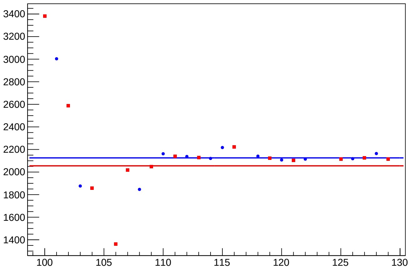
reg_asym_us_avg_at2lr_avg_avg_rms vs Slug, Sign Corrected
