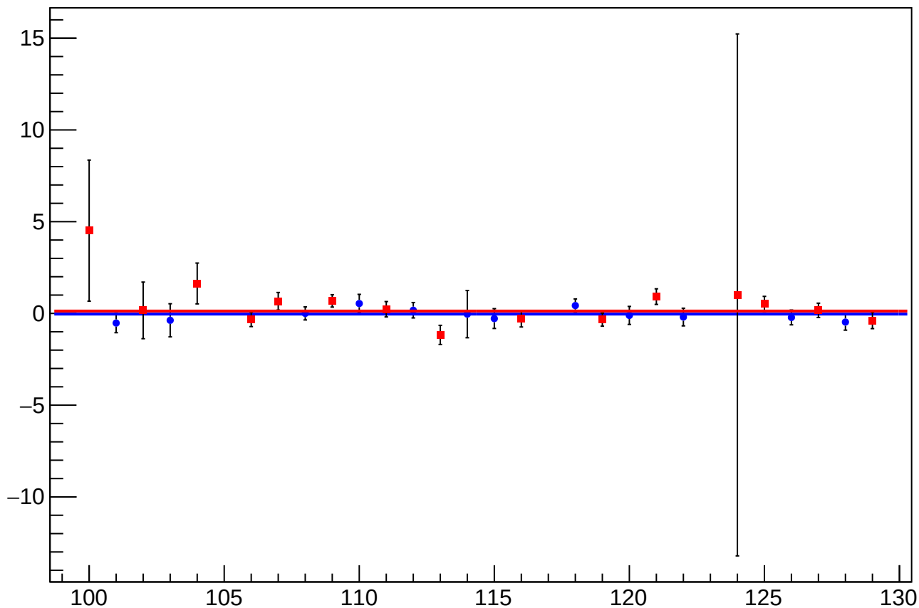
asym_at2_avg_eigen_dit_vs_eigen_cor_diff_mean vs Slug, Sign Corrected
