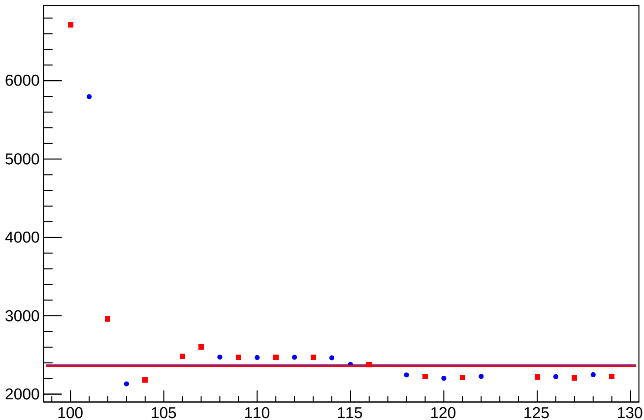
reg_asym_us_dd_at1lr_dd_avg_rms vs Slug, Sign Corrected
