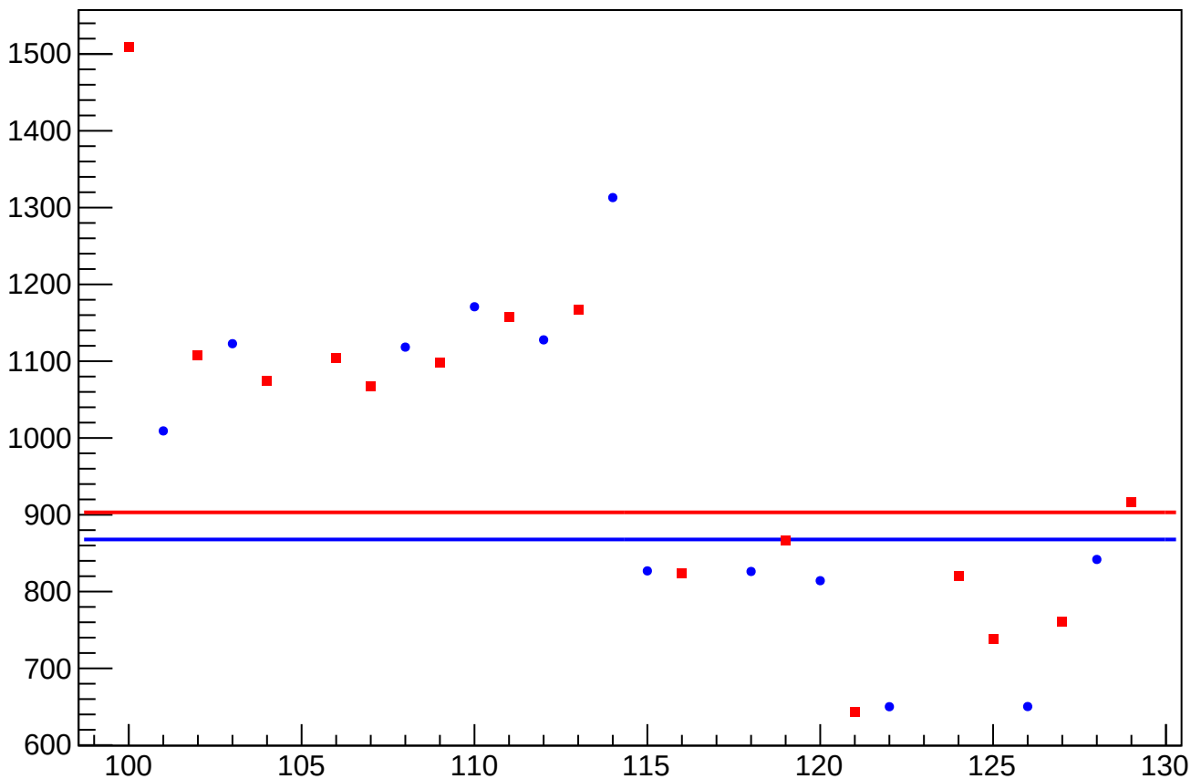
asym_sam_15_26_dd_eigen_dit_correction_rms vs Slug, Sign Corrected
