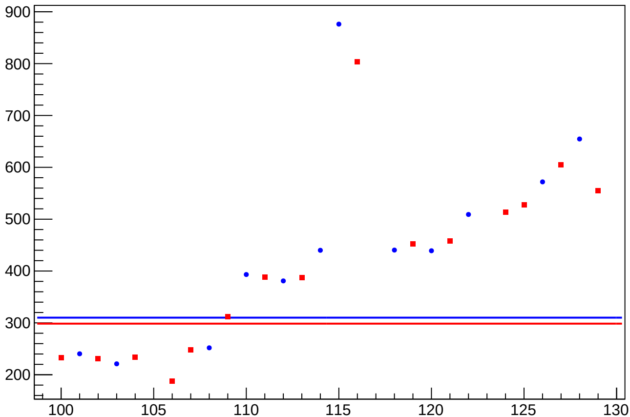
asym_sam_37_48_dd_eigen_dit_correction_rms vs Slug, Sign Corrected
