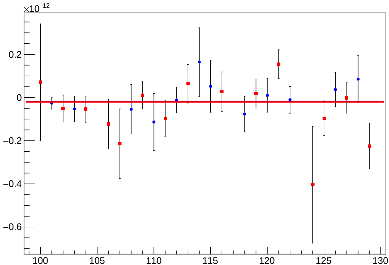
asym_at1_dd_at2_dd_avg_eigen_cor_vs_cor_diff_mean vs Slug, Sign Corrected
