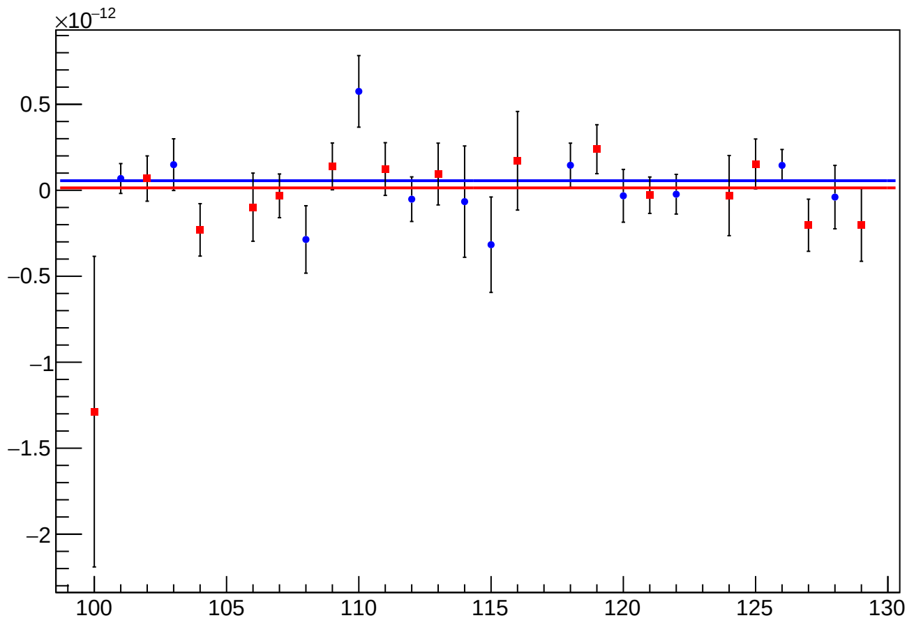
asym_sam_26_dd_eigen_cor_vs_cor_diff_mean vs Slug, Sign Corrected
