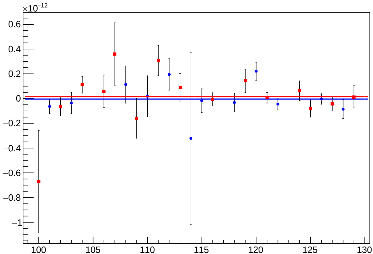
asym_sam_1526_avg_reg_vs_cor_diff_mean vs Slug, Sign Corrected
