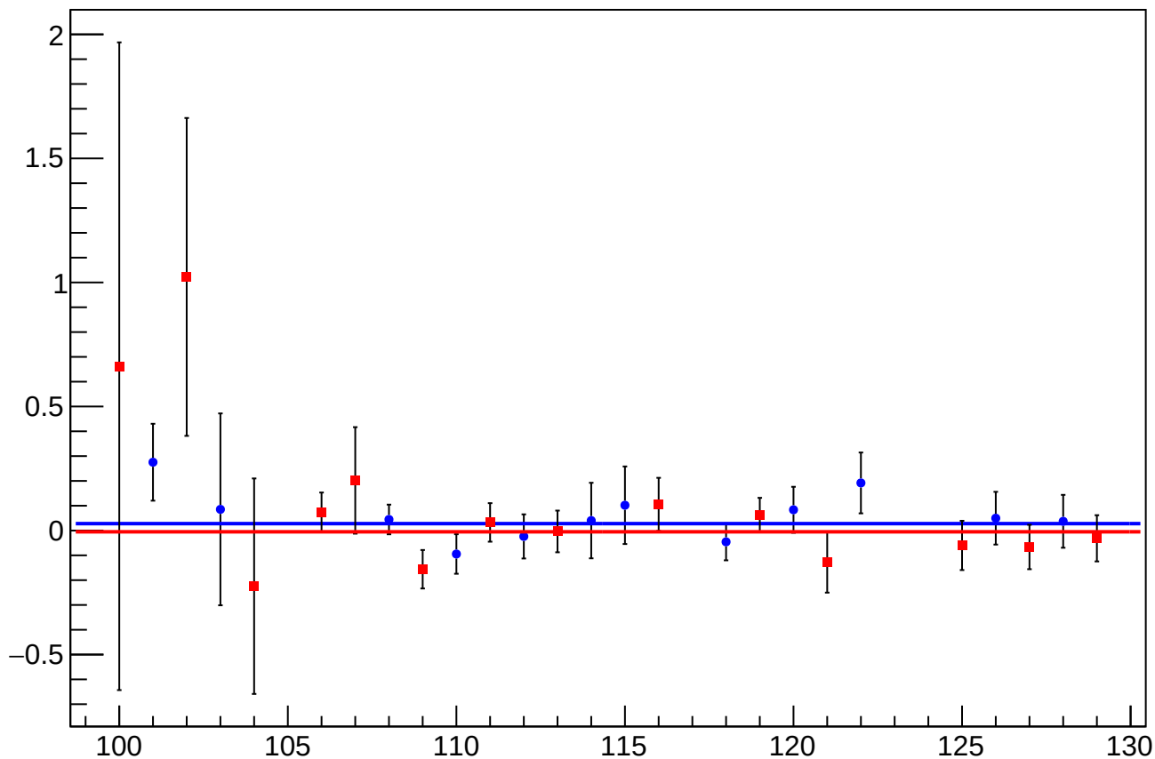
asym_us_dd_atlr_dd_avg_eigen_dit_vs_cor_diff_mean vs Slug, Sign Corrected
