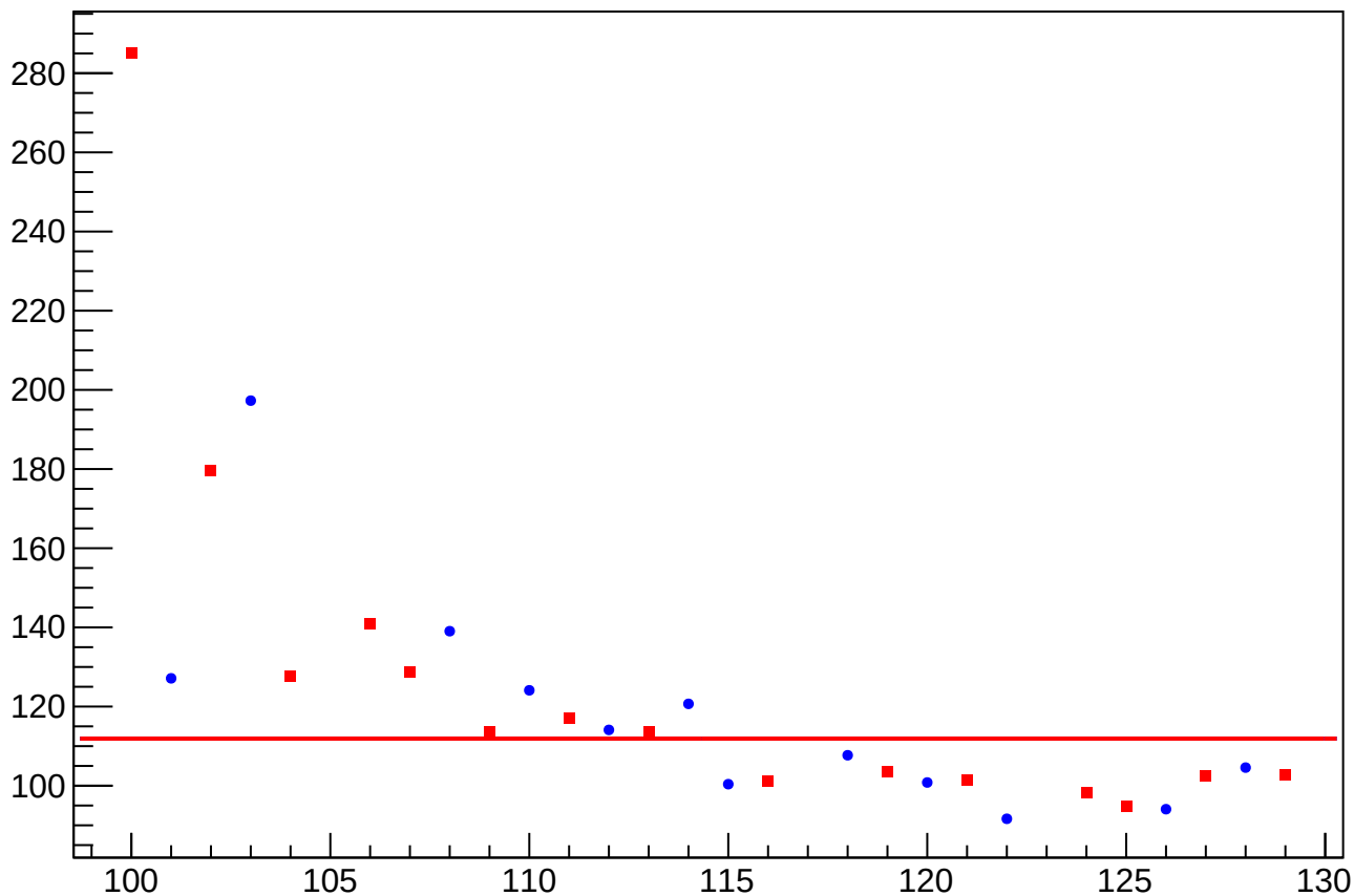
eigen_dit_asym_sam_2468_avg_rms vs Slug, Sign Corrected
