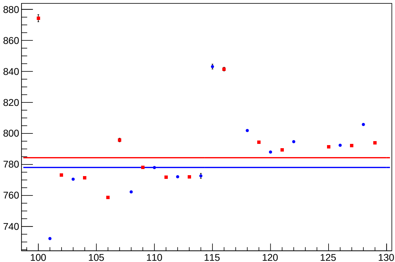
eigen_cor_asym_us_avg_rms vs Slug, Sign Corrected
