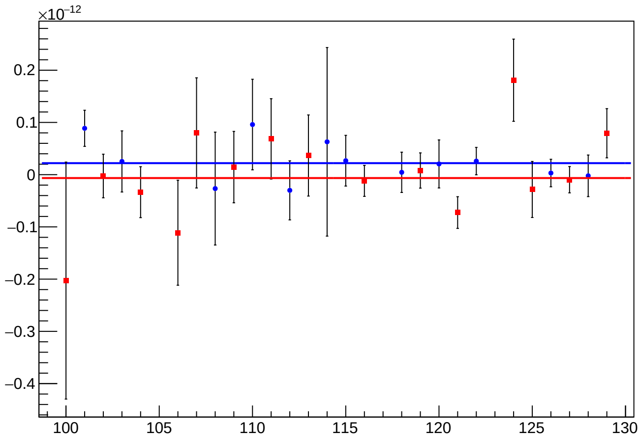
asym_sam_1526_avg_eigen_cor_vs_cor_diff_mean vs Slug, Sign Corrected
