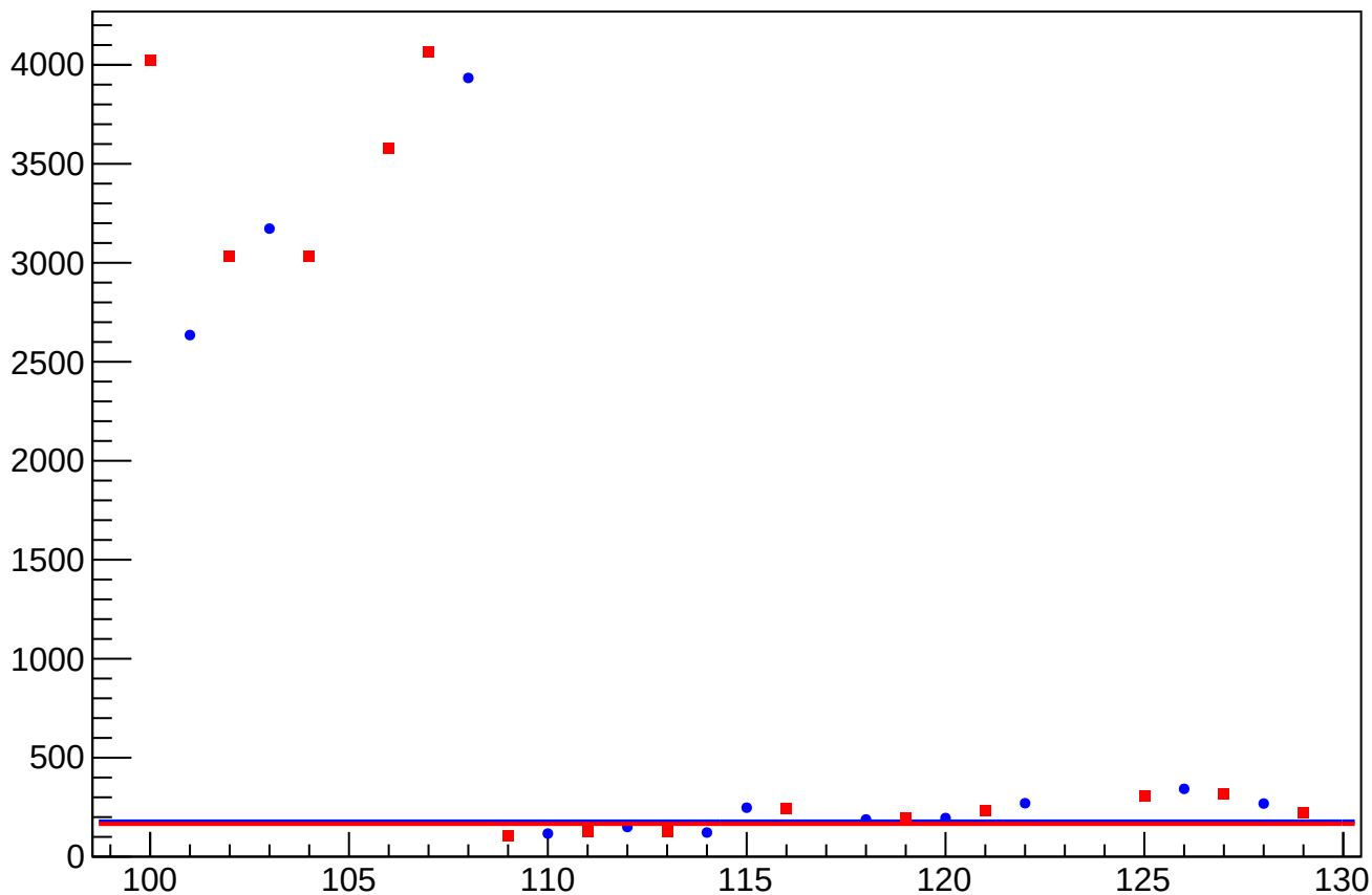
asym_bcm_cav4cQ_an_ds_avg_rms vs Slug, Sign Corrected
