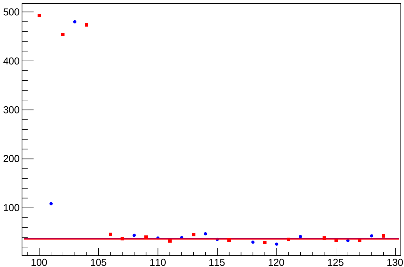
asym_usr_atr1_dd_eigen_dit_vs_cor_diff_rms vs Slug, Sign Corrected
