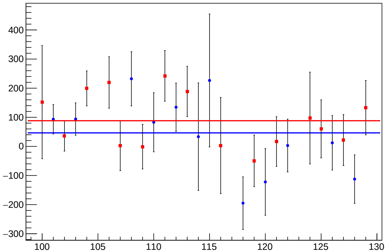
cor_asym_sam_15_avg_mean vs Slug, Sign Corrected
