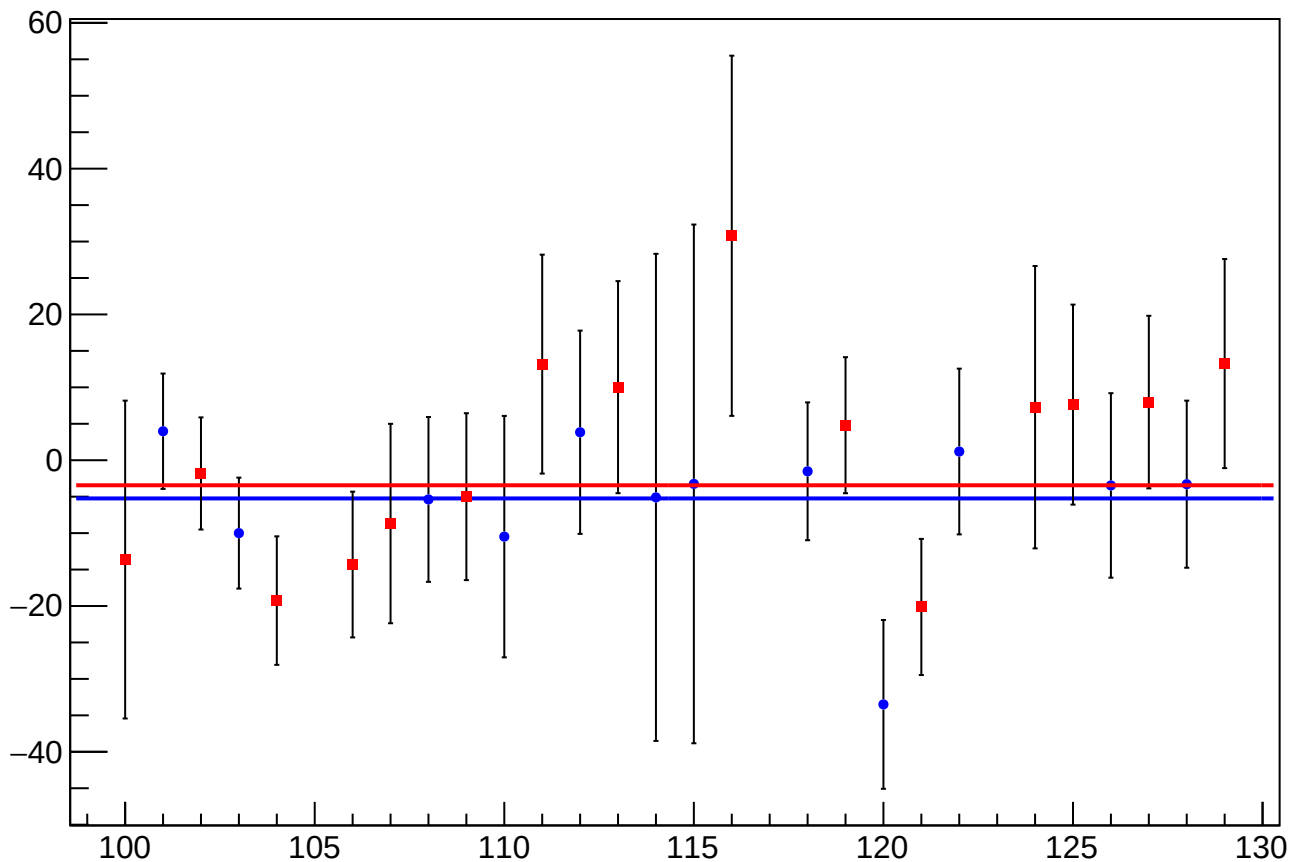
diff_bpm_4eY_4ecY_avg_mean vs Slug, Sign Corrected
