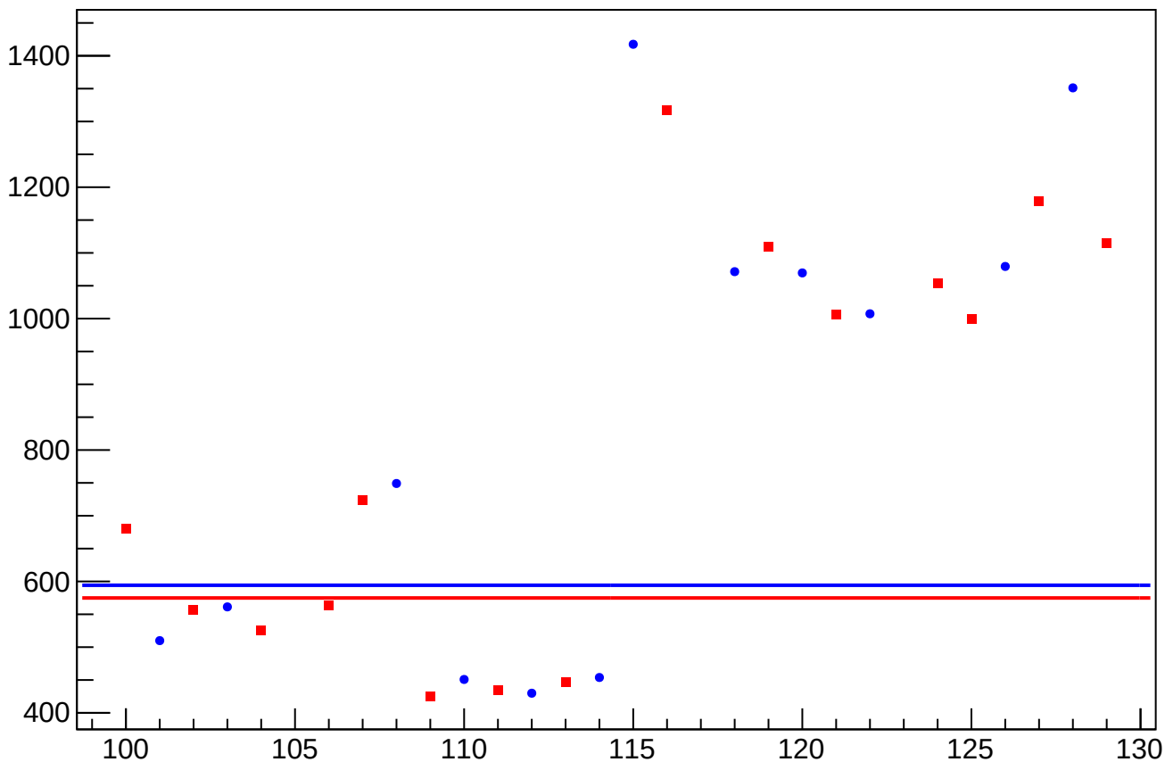
asym_sam_1548_avg_eigen_dit_correction_rms vs Slug, Sign Corrected
