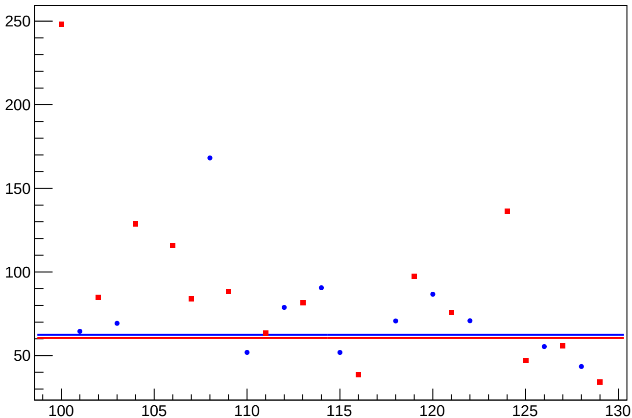
asym_sam3_eigen_dit_vs_cor_diff_rms vs Slug, Sign Corrected
