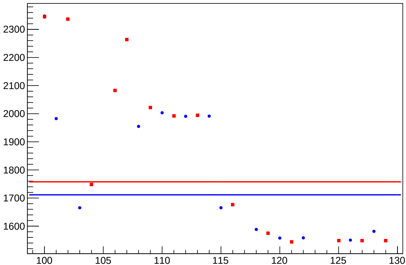
eigen_dit_asym_atl_avg_rms vs Slug, Sign Corrected
