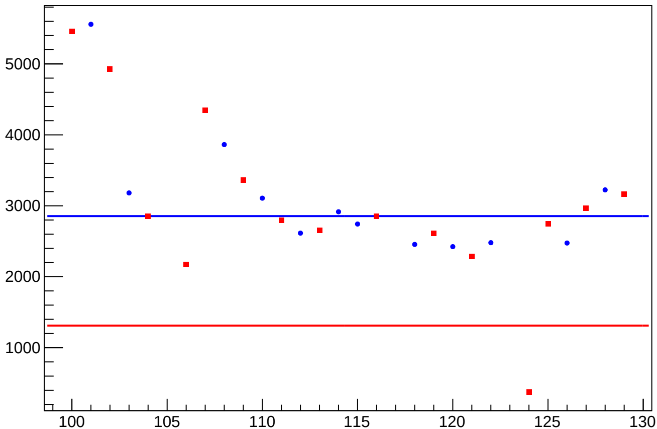
asym_atr1l2_avg_eigen_cor_correction_rms vs Slug, Sign Corrected
