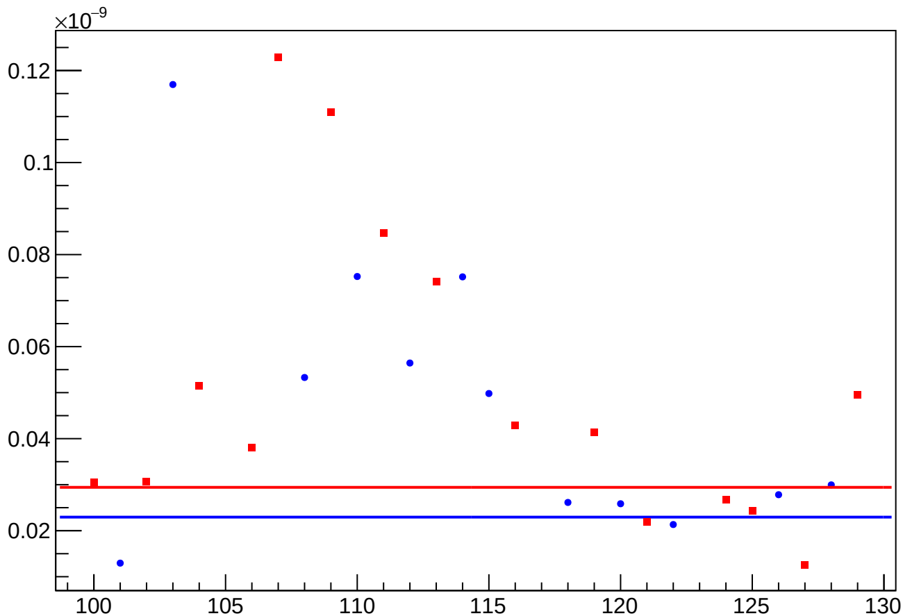
asym_atl1_eigen_cor_vs_cor_diff_rms vs Slug, Sign Corrected
