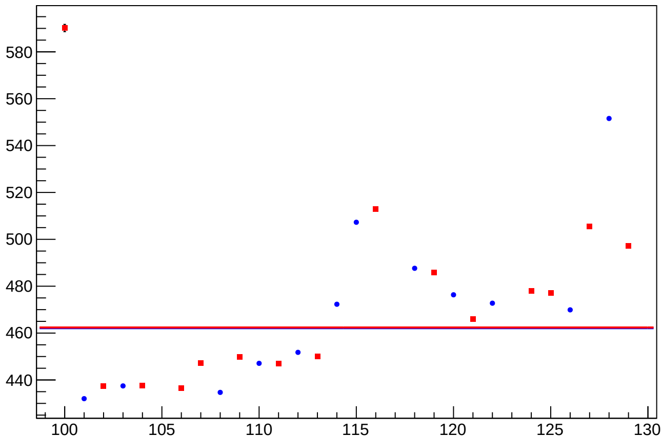
diff_bpm_4aX_4acX_dd_rms vs Slug, Sign Corrected
