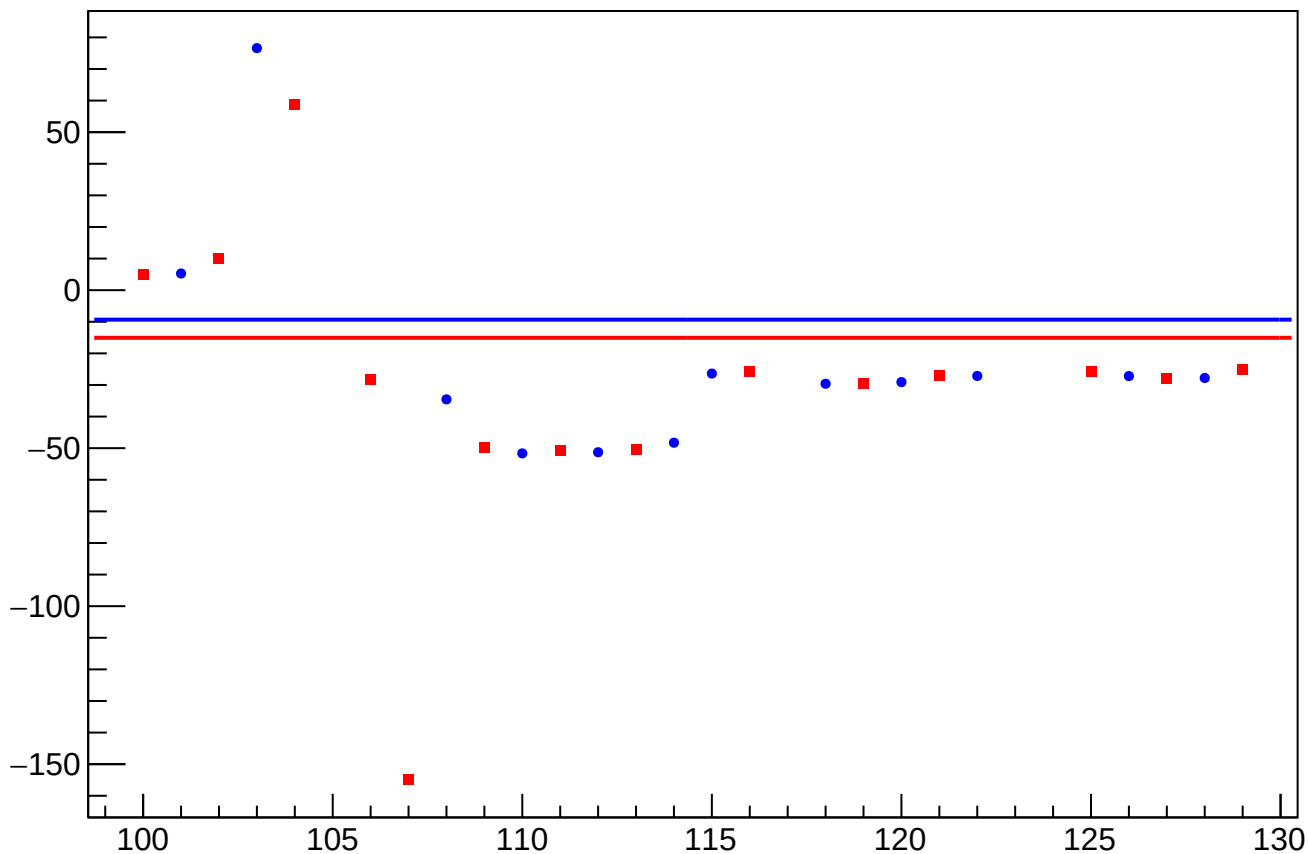
reg_asym_usl_atl1_avg_diff_bpm12X_slope vs Slug, Sign Corrected
