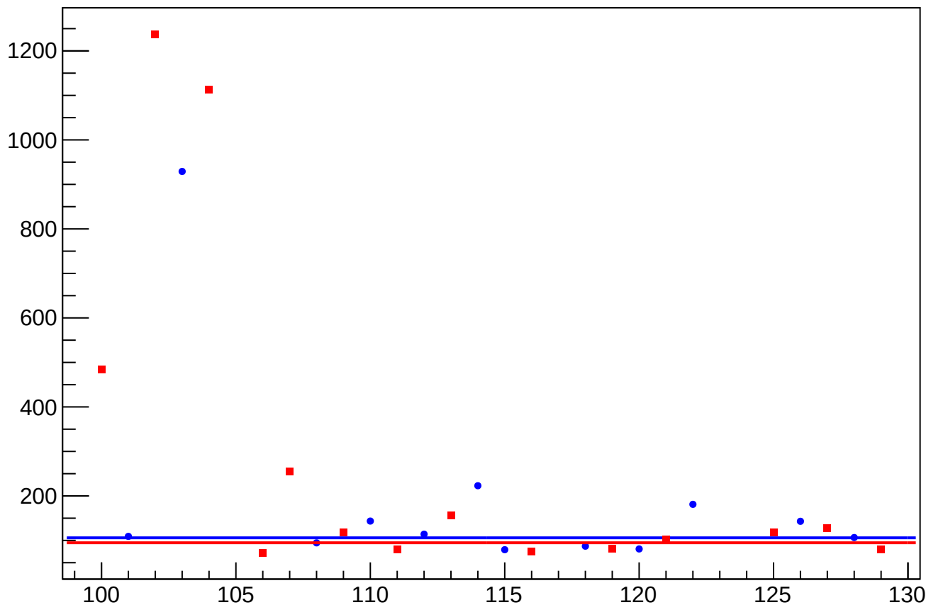
asym_us_avg_at1lr_avg_avg_eigen_dit_vs_eigen_cor_diff_rms vs Slug, Sign Corrected
