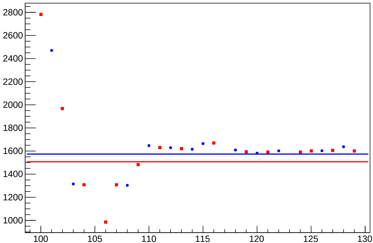
reg_asym_usr_atr2_avg_rms vs Slug, Sign Corrected
