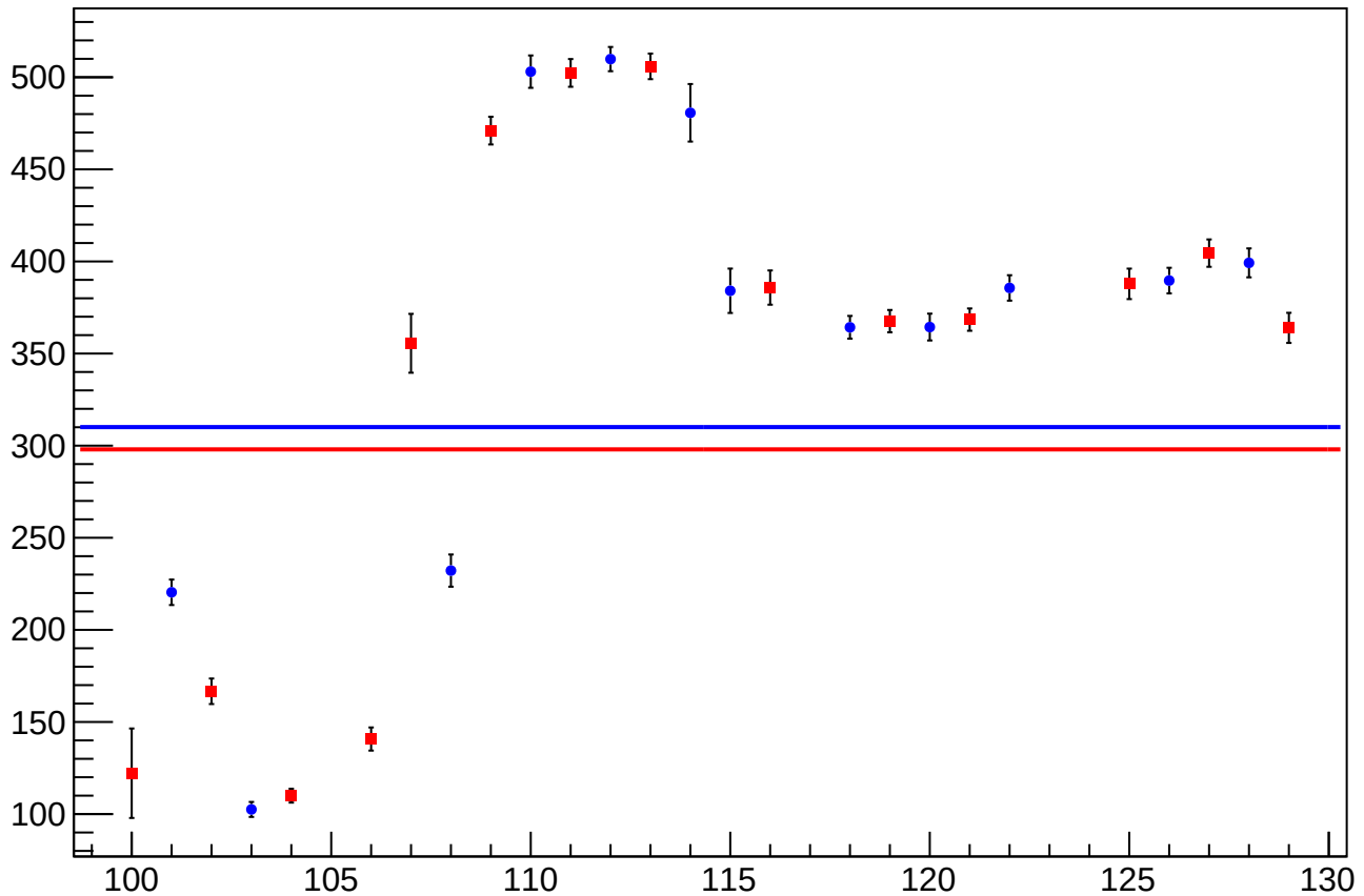
reg_asym_us_avg_atlr_avg_avg_diff_bpm4eX_slope vs Slug, Sign Corrected
