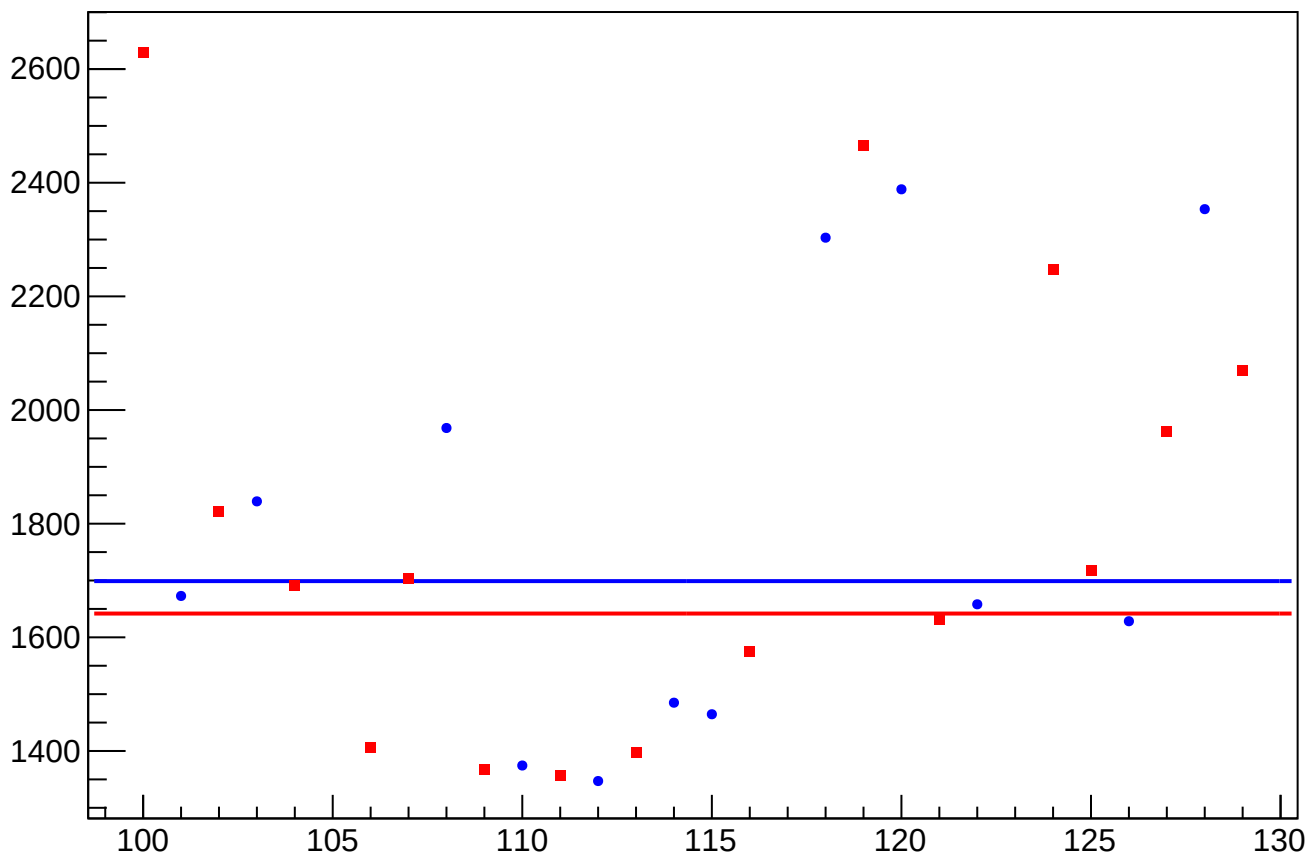
asym_sam3_eigen_cor_correction_rms vs Slug, Sign Corrected
