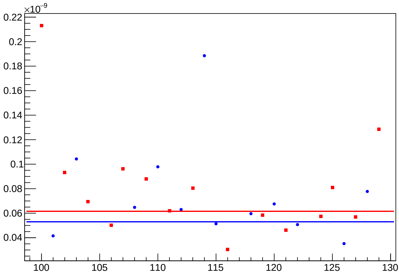
asym_sam_3726_avg_reg_vs_cor_diff_rms vs Slug, Sign Corrected
