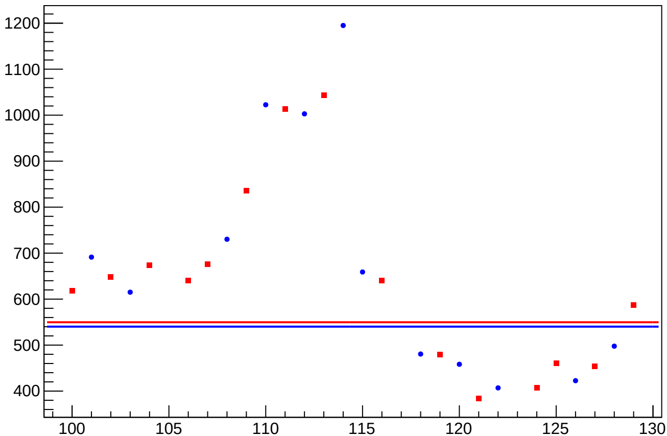
asym_sam1_eigen_cor_correction_rms vs Slug, Sign Corrected
