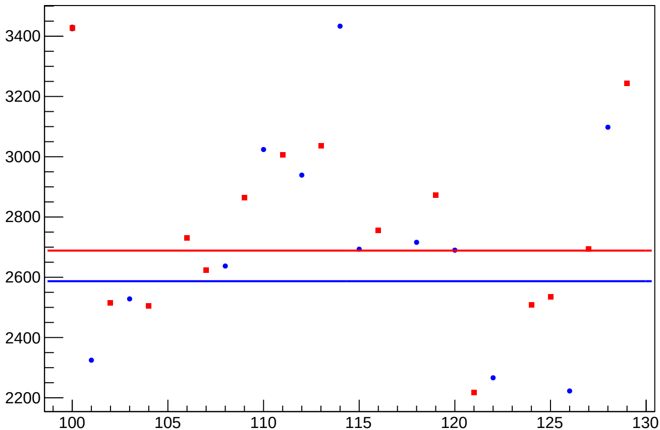
asym_sam_26_dd_cor_correction_rms vs Slug, Sign Corrected
