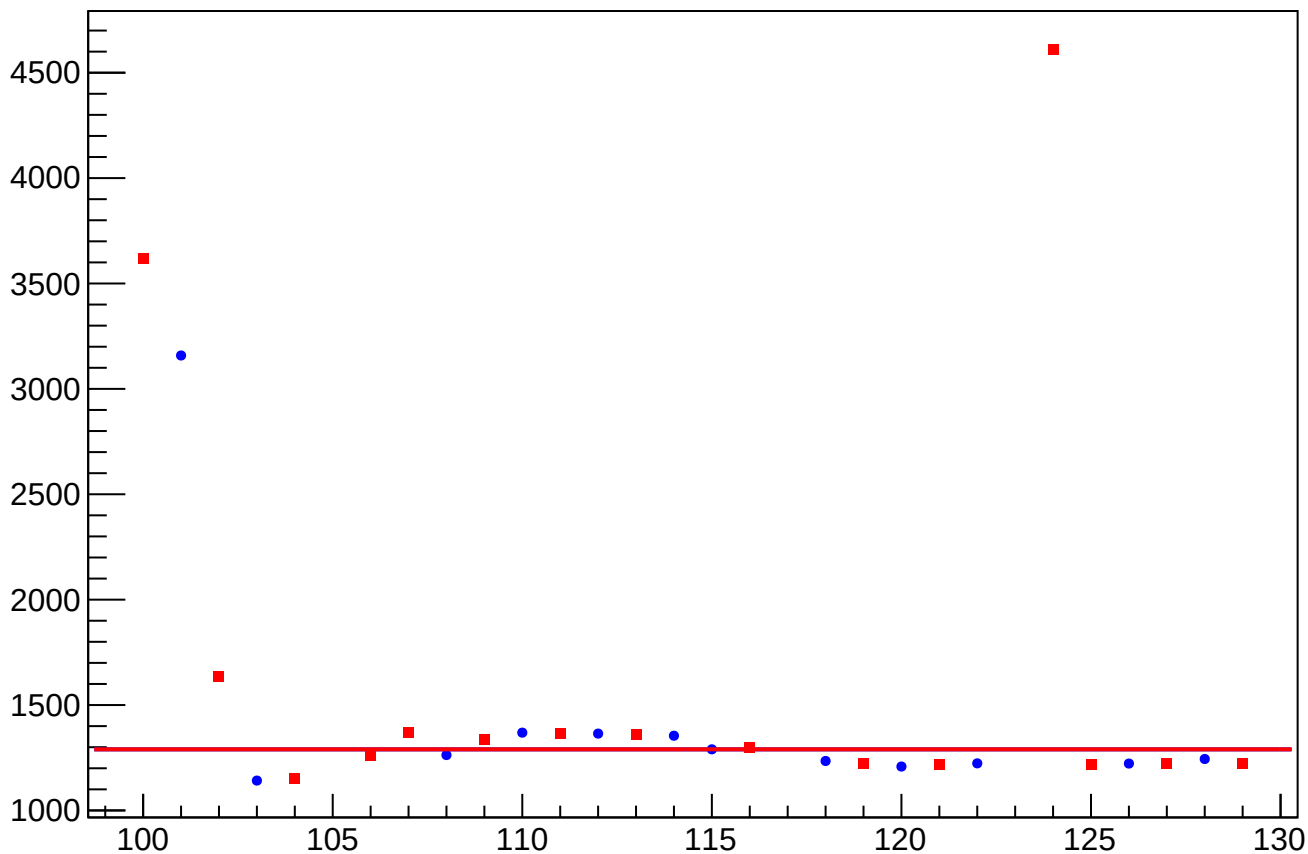
reg_asym_at1_avg_at2_avg_dd_rms vs Slug, Sign Corrected
