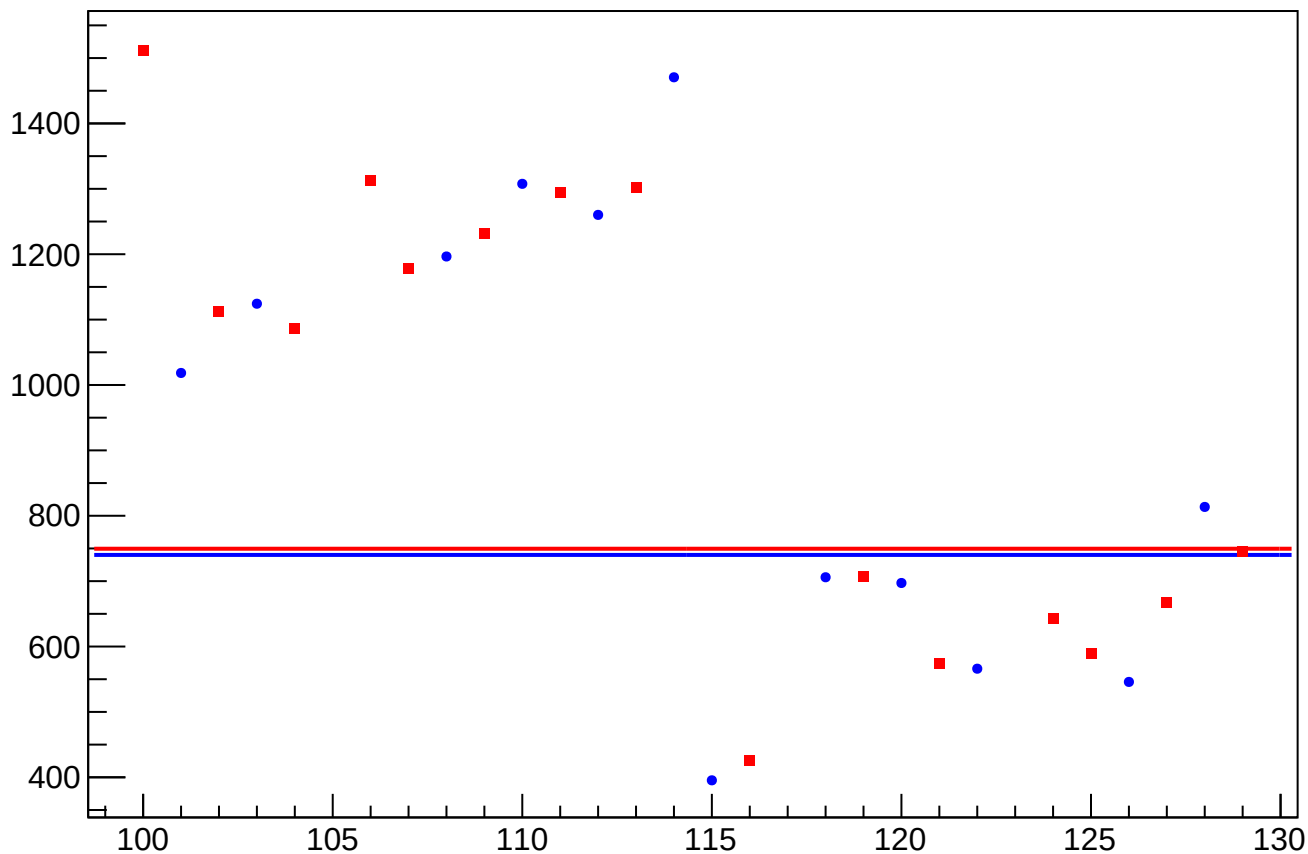
asym_sam_1526_avg_dit_correction_rms vs Slug, Sign Corrected
