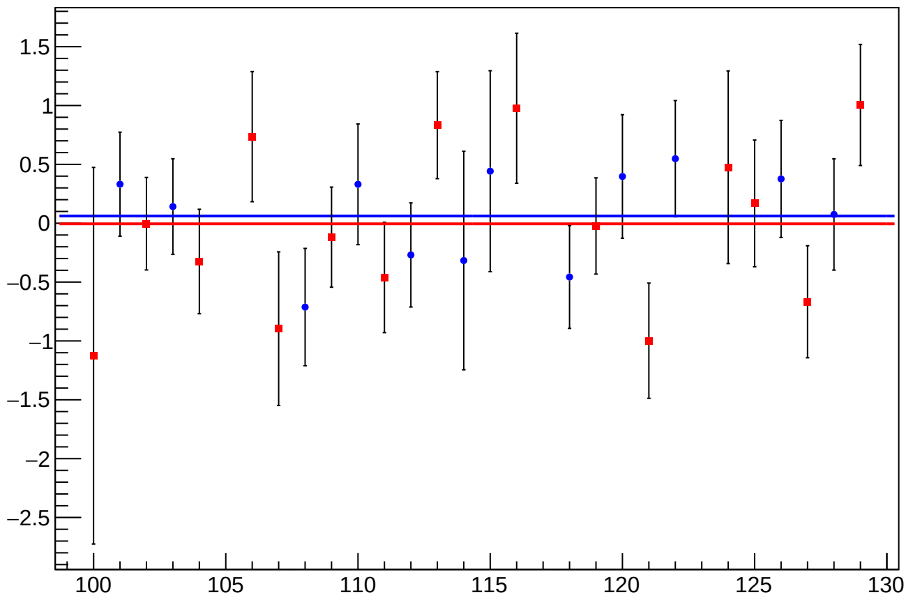
diff_bpm_4eX_4ecX_dd_mean vs Slug, Sign Corrected
