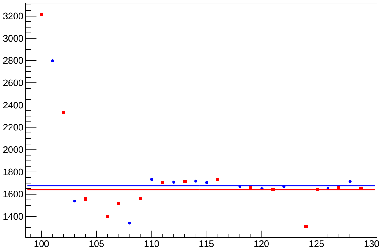
eigen_dit_asym_at2_avg_rms vs Slug, Sign Corrected
