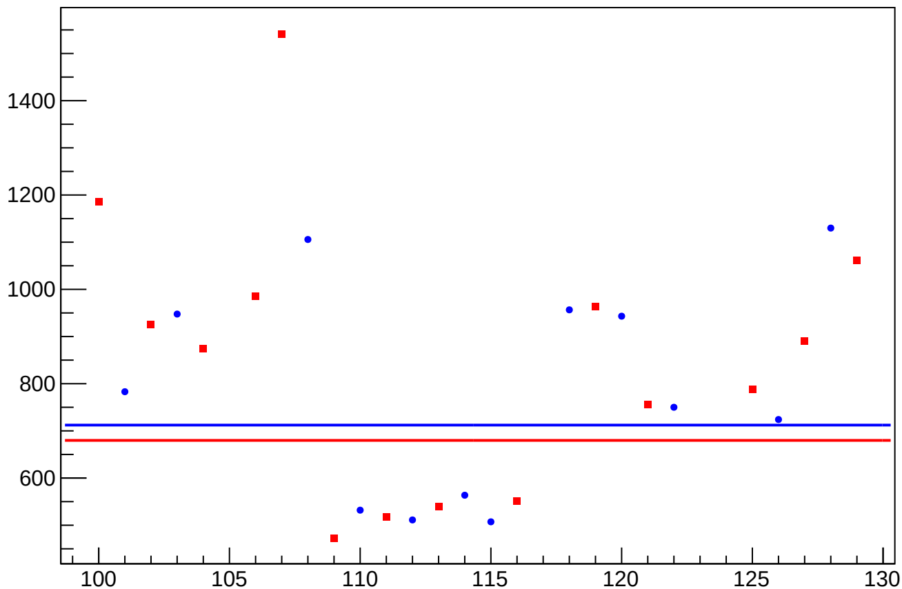
asym_us_dd_dit_correction_rms vs Slug, Sign Corrected
