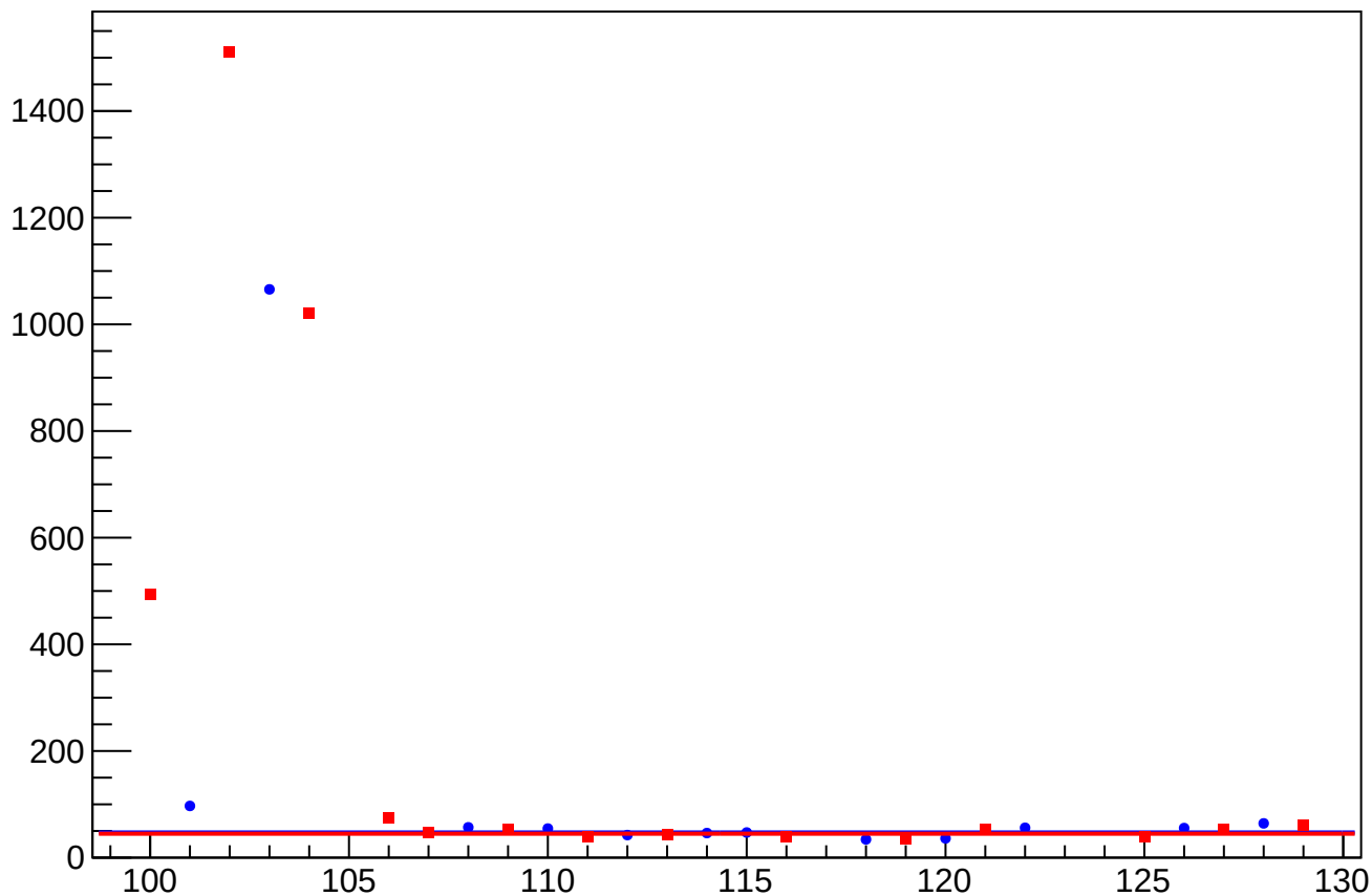
asym_us_avg_at1lr_avg_dd_dit_vs_eigen_cor_diff_rms vs Slug, Sign Corrected
