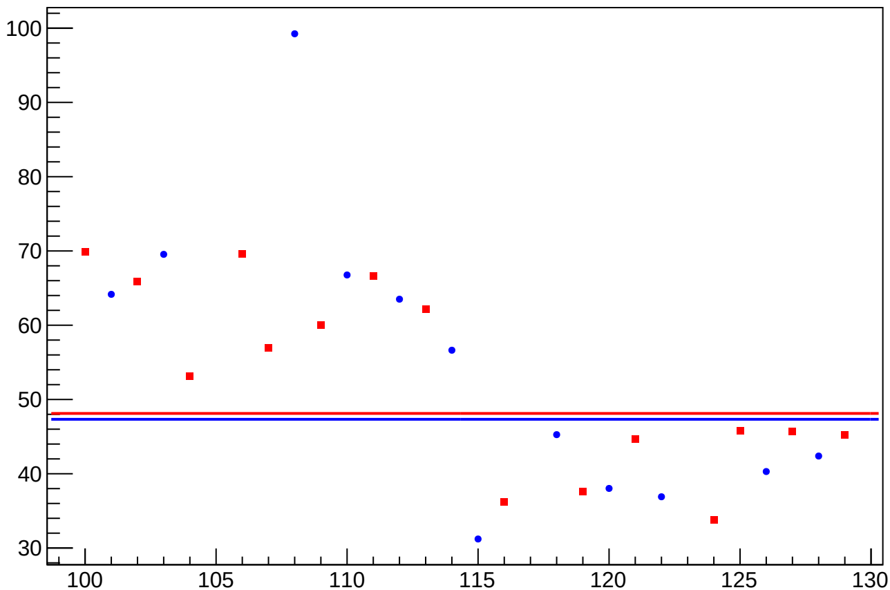
asym_sam_24_68_dd_dit_vs_cor_diff_rms vs Slug, Sign Corrected
