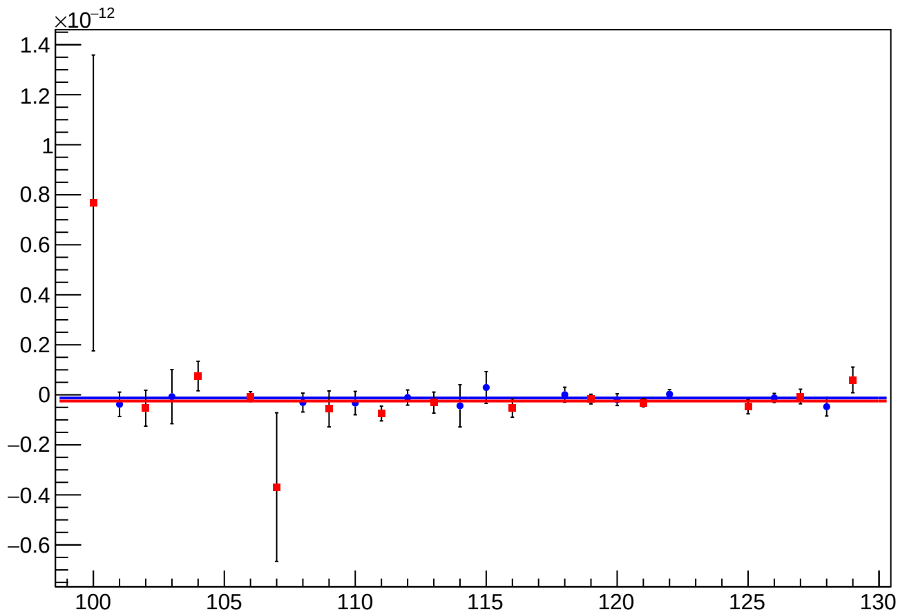
asym_us_dd_at1lr_dd_avg_eigen_cor_vs_cor_diff_mean vs Slug, Sign Corrected
