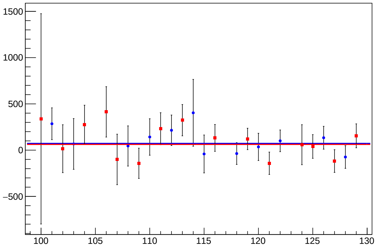
cor_asym_sam_3726_avg_mean vs Slug, Sign Corrected
