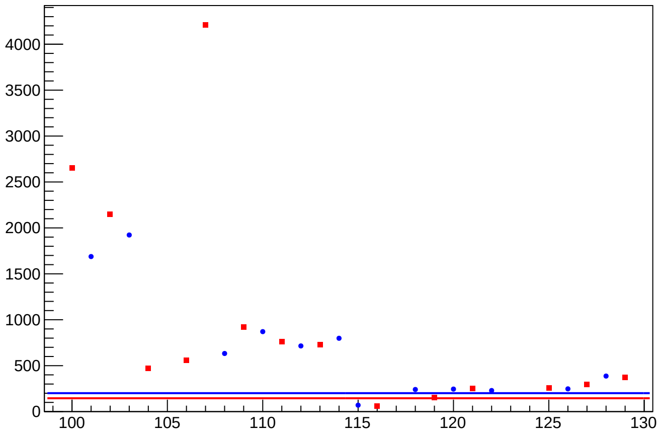
asym_us_dd_at1lr_dd_avg_reg_correction_rms vs Slug, Sign Corrected
