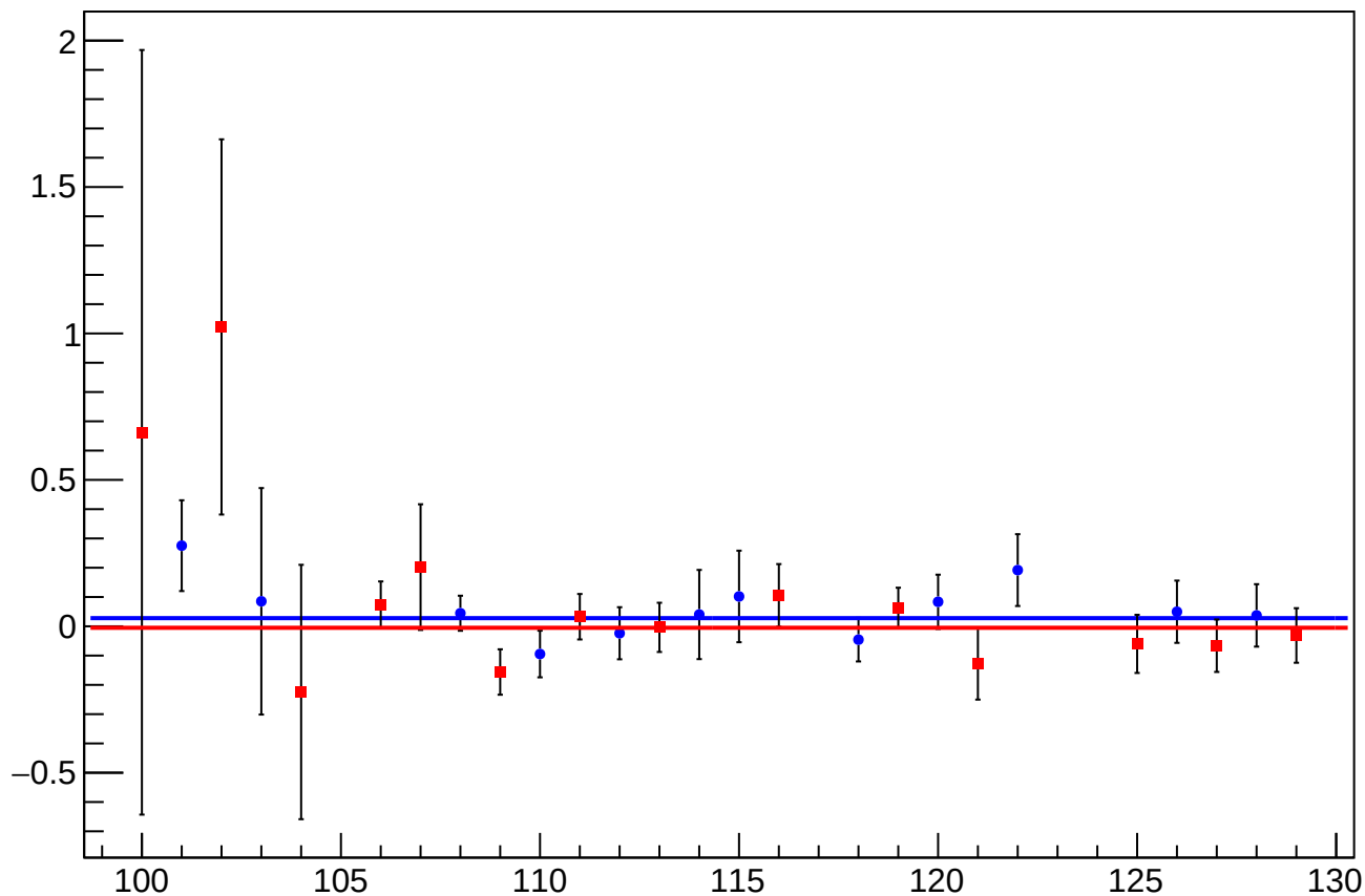
asym_us_dd_atlr_dd_avg_dit_vs_cor_diff_mean vs Slug, Sign Corrected
