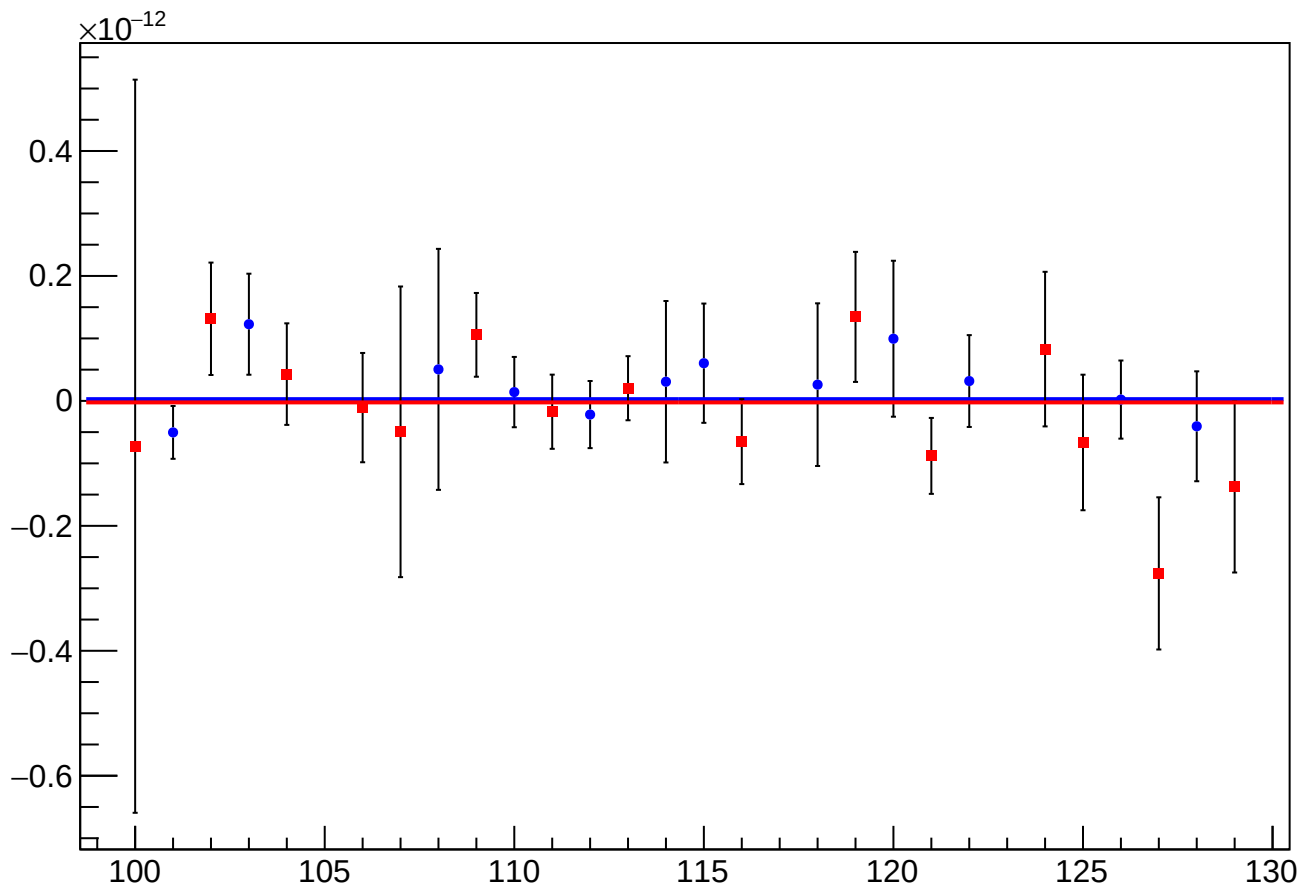
asym_sam3_eigen_cor_vs_cor_diff_mean vs Slug, Sign Corrected
