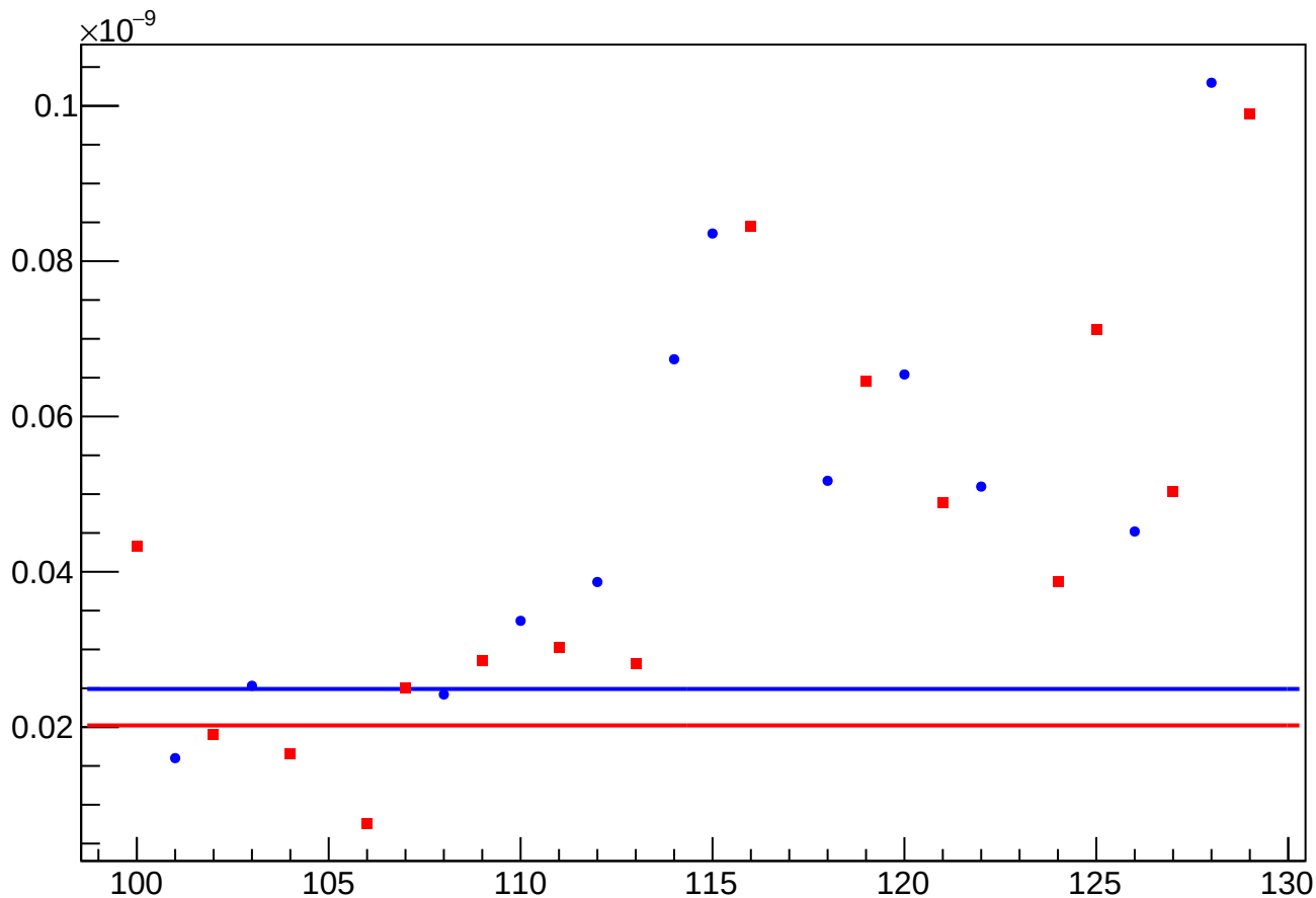
asym_sam6_reg_vs_cor_diff_rms vs Slug, Sign Corrected
