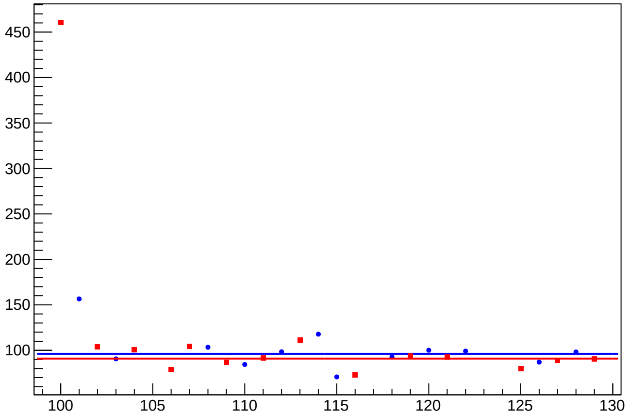
asym_usl_atl2_dd_dit_vs_eigen_cor_diff_rms vs Slug, Sign Corrected
