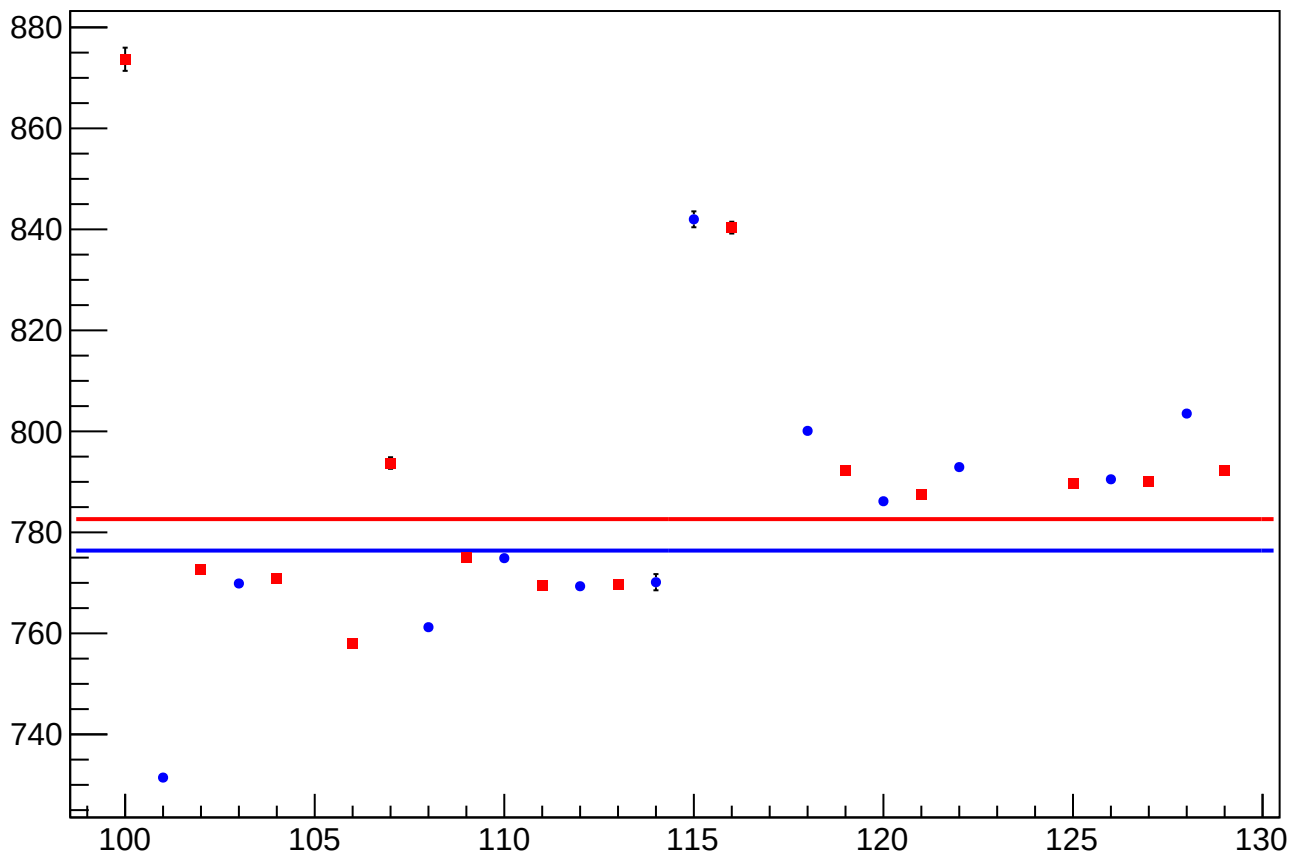
overload_cor_asym_us_avg_rms vs Slug, Sign Corrected
