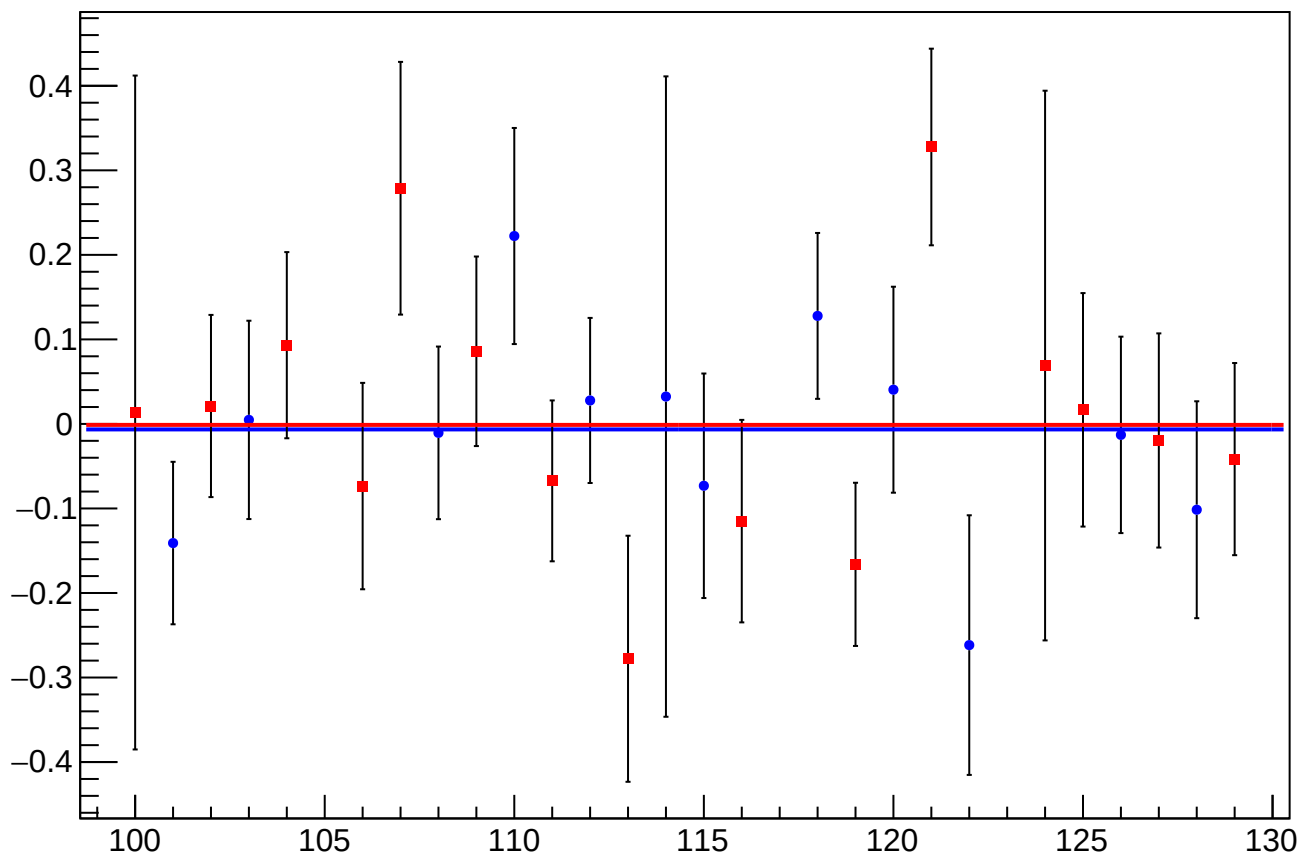
asym_usr_dit_vs_eigen_cor_diff_mean vs Slug, Sign Corrected
