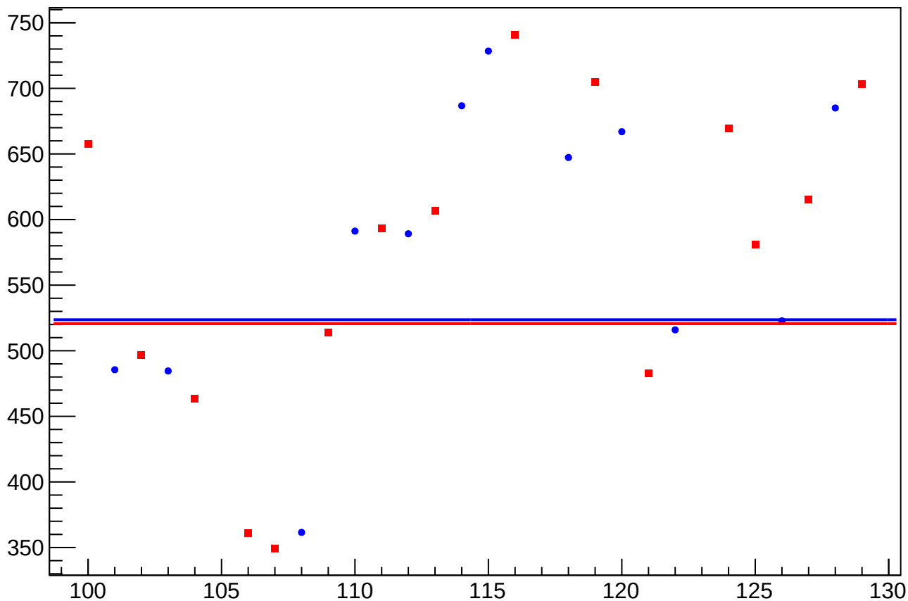
asym_sam_13_57_dd_eigen_cor_correction_rms vs Slug, Sign Corrected
