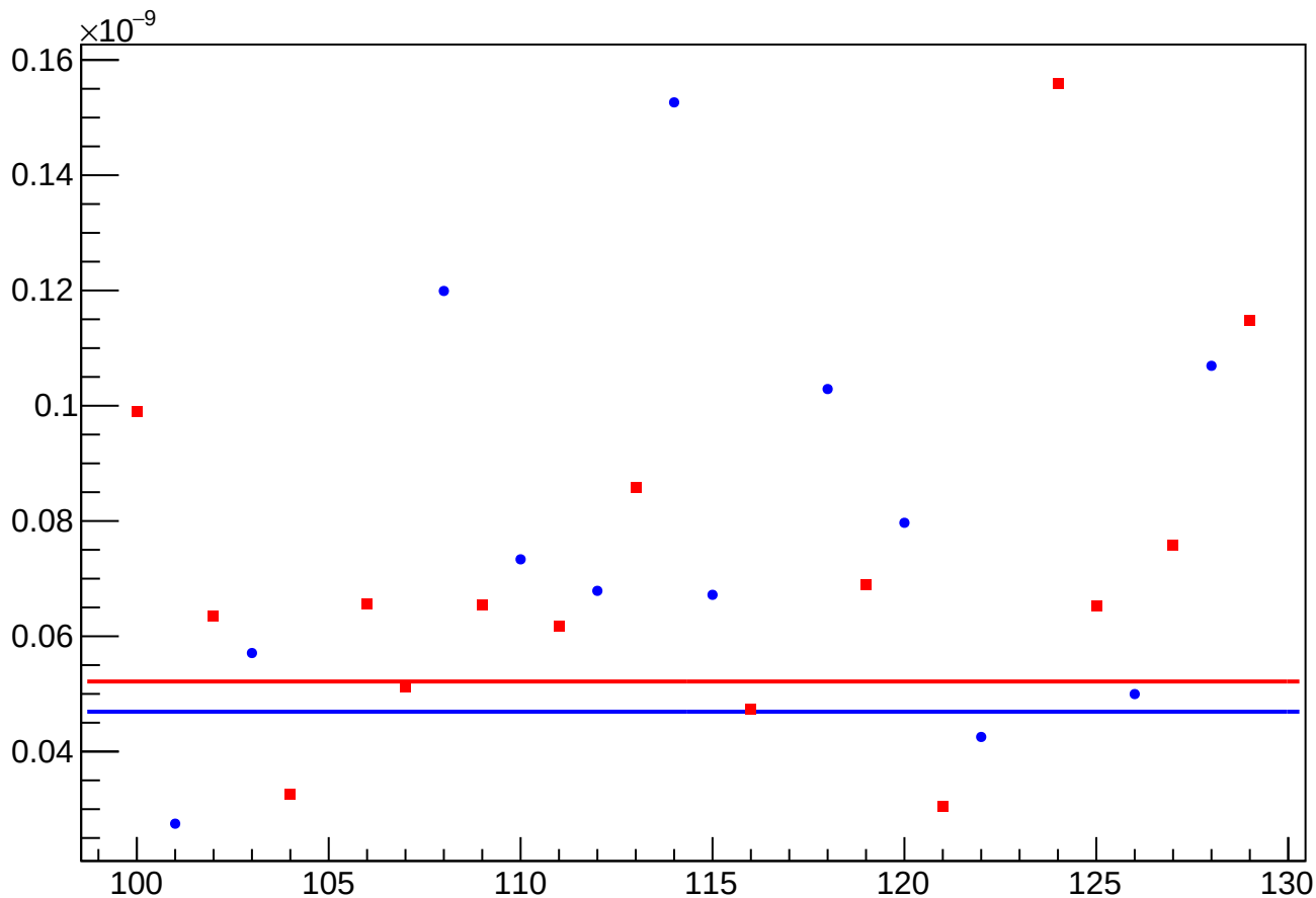
asym_at1_dd_at2_dd_avg_reg_vs_cor_diff_rms vs Slug, Sign Corrected
