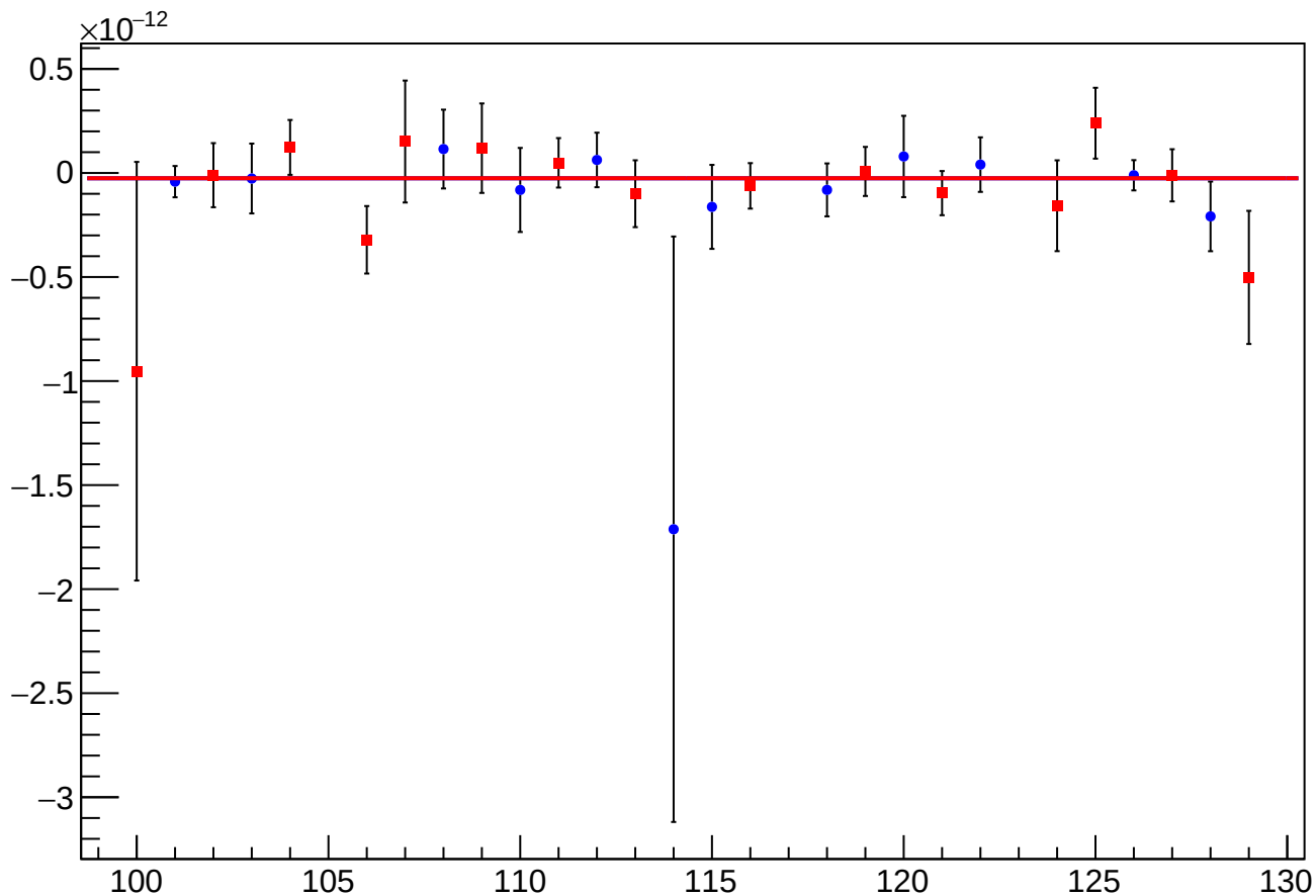
asym_sam_3726_avg_reg_vs_cor_diff_mean vs Slug, Sign Corrected
