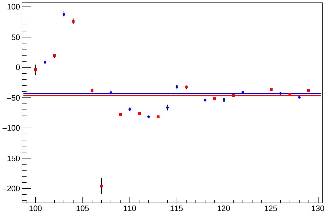
reg_asym_usl_atl1_avg_diff_bpm1X_slope vs Slug, Sign Corrected
