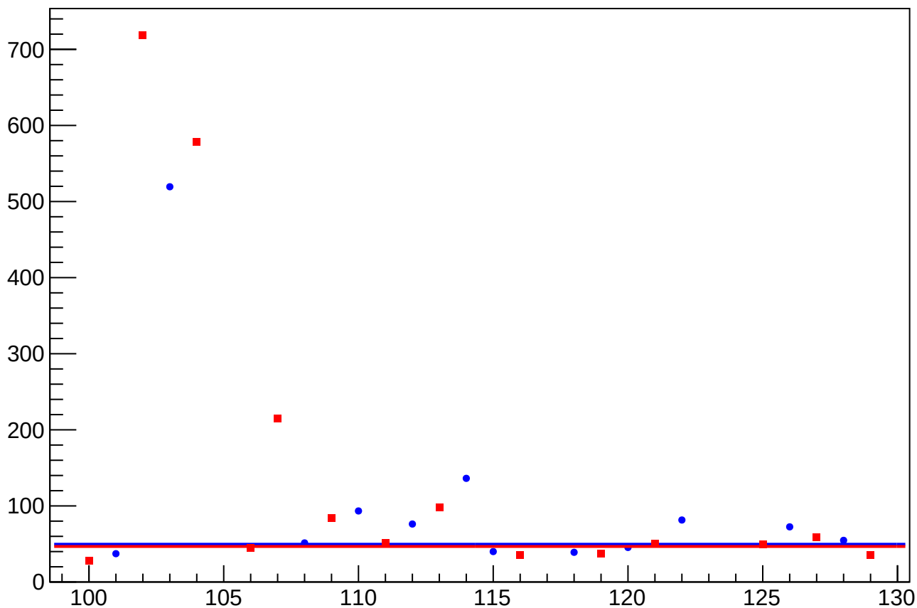
asym_usl_atl1_avg_dit_vs_cor_diff_rms vs Slug, Sign Corrected
