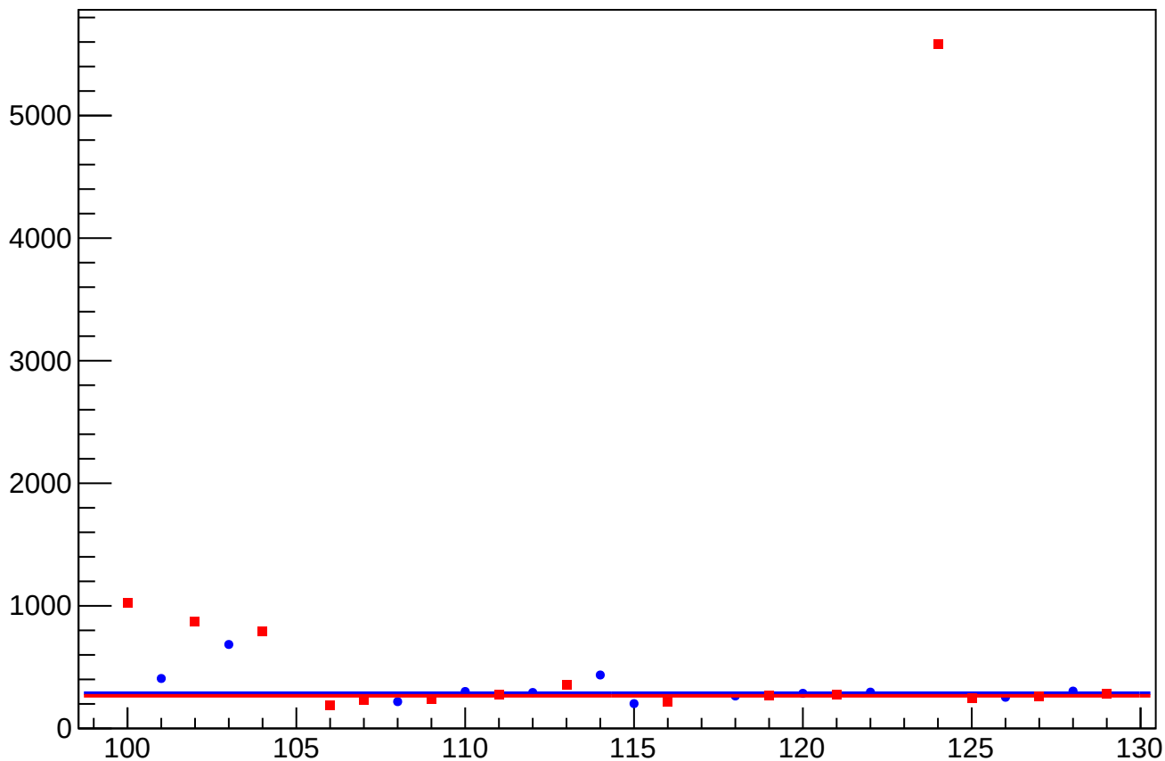
asym_at2_avg_dit_vs_eigen_cor_diff_rms vs Slug, Sign Corrected
