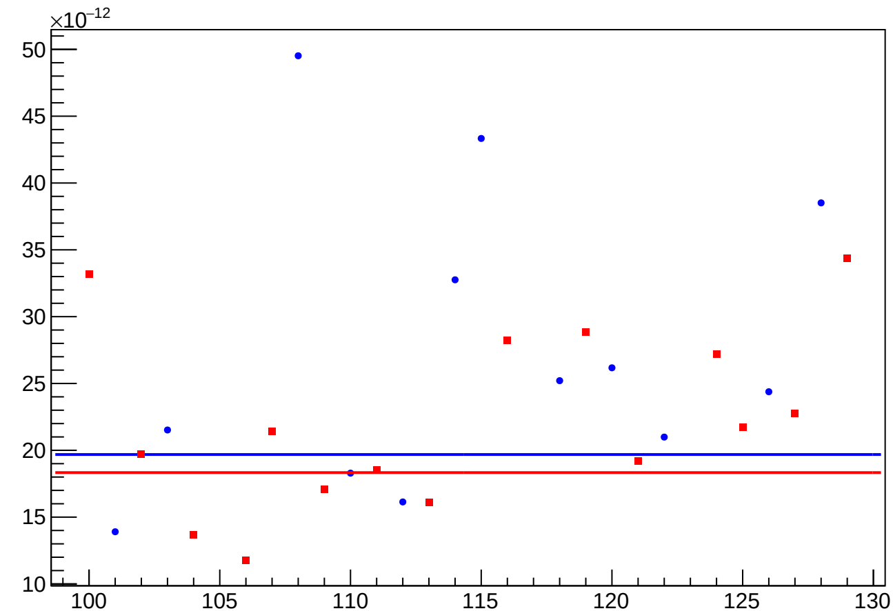
asym_sam_15_48_dd_eigen_cor_vs_cor_diff_rms vs Slug, Sign Corrected
