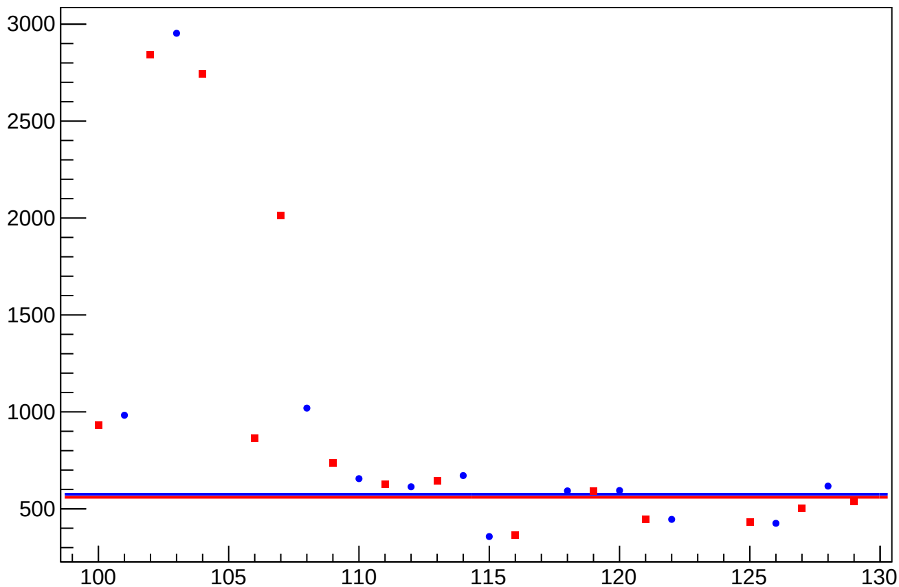
asym_usl_atl1_dd_dit_correction_rms vs Slug, Sign Corrected
