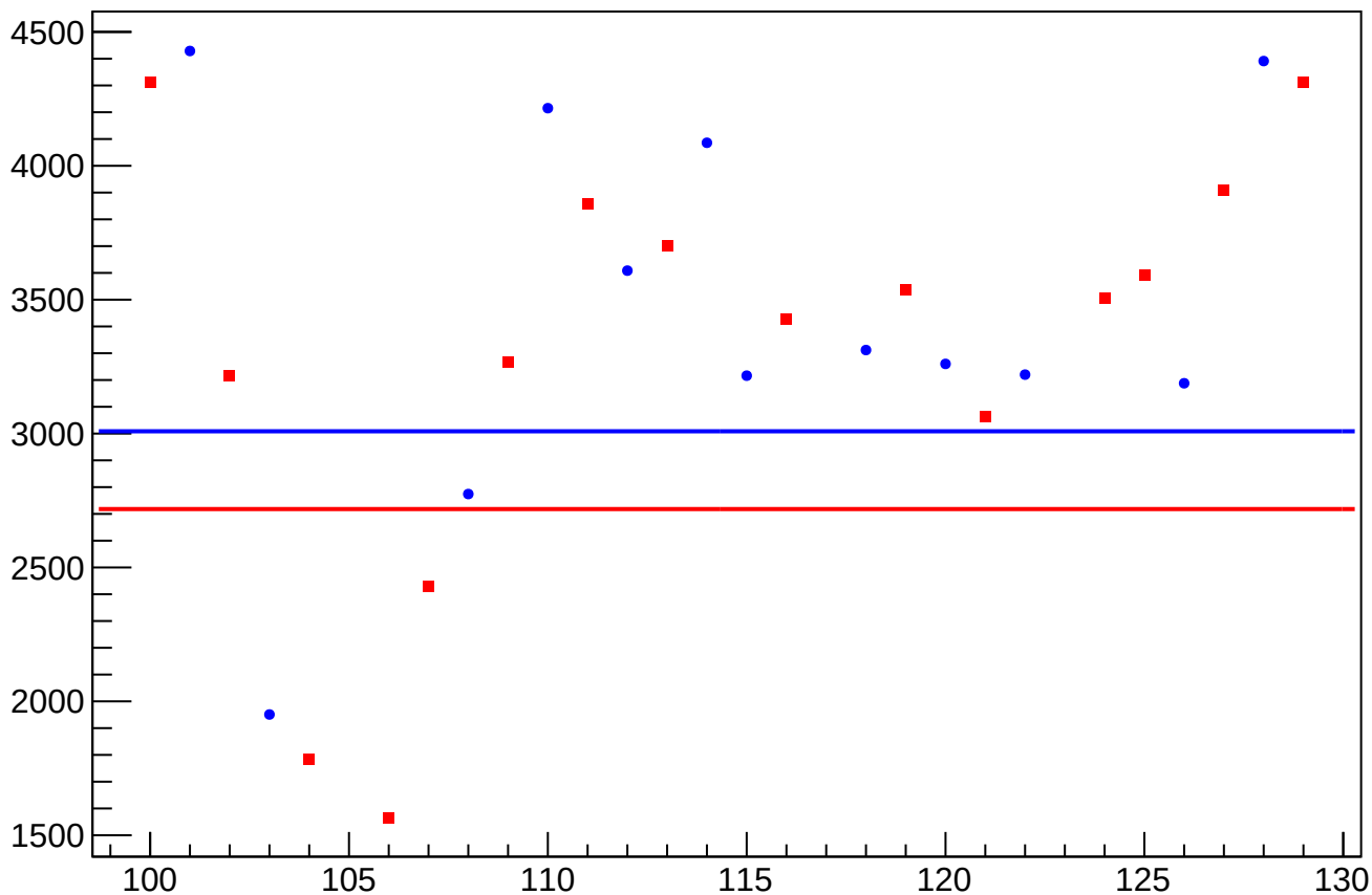
asym_usr_atr2_dd_reg_correction_rms vs Slug, Sign Corrected
