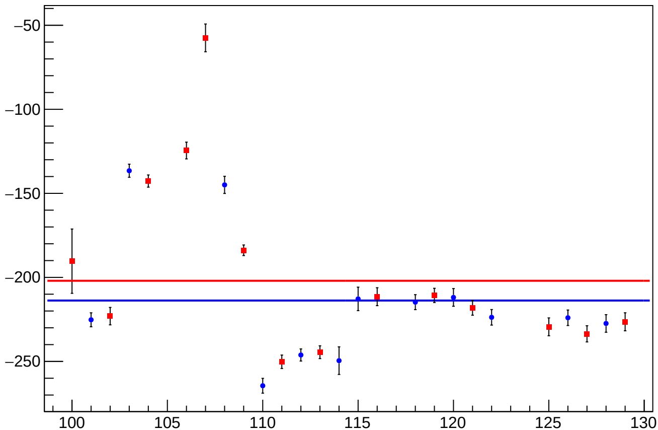
reg_asym_us_dd_at2lr_dd_avg_diff_bpm4eX_slope vs Slug, Sign Corrected
