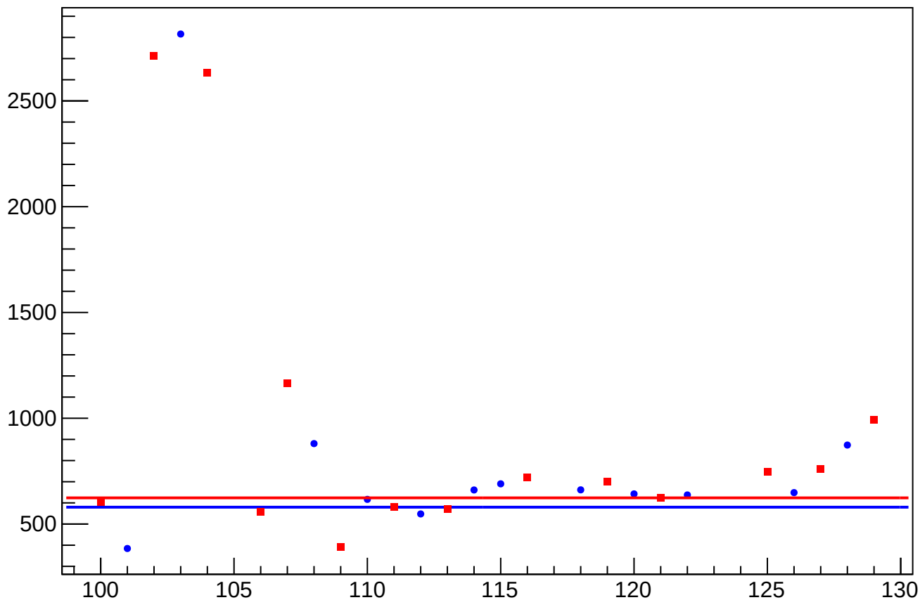
asym_us_avg_at1lr_avg_dd_eigen_dit_correction_rms vs Slug, Sign Corrected
