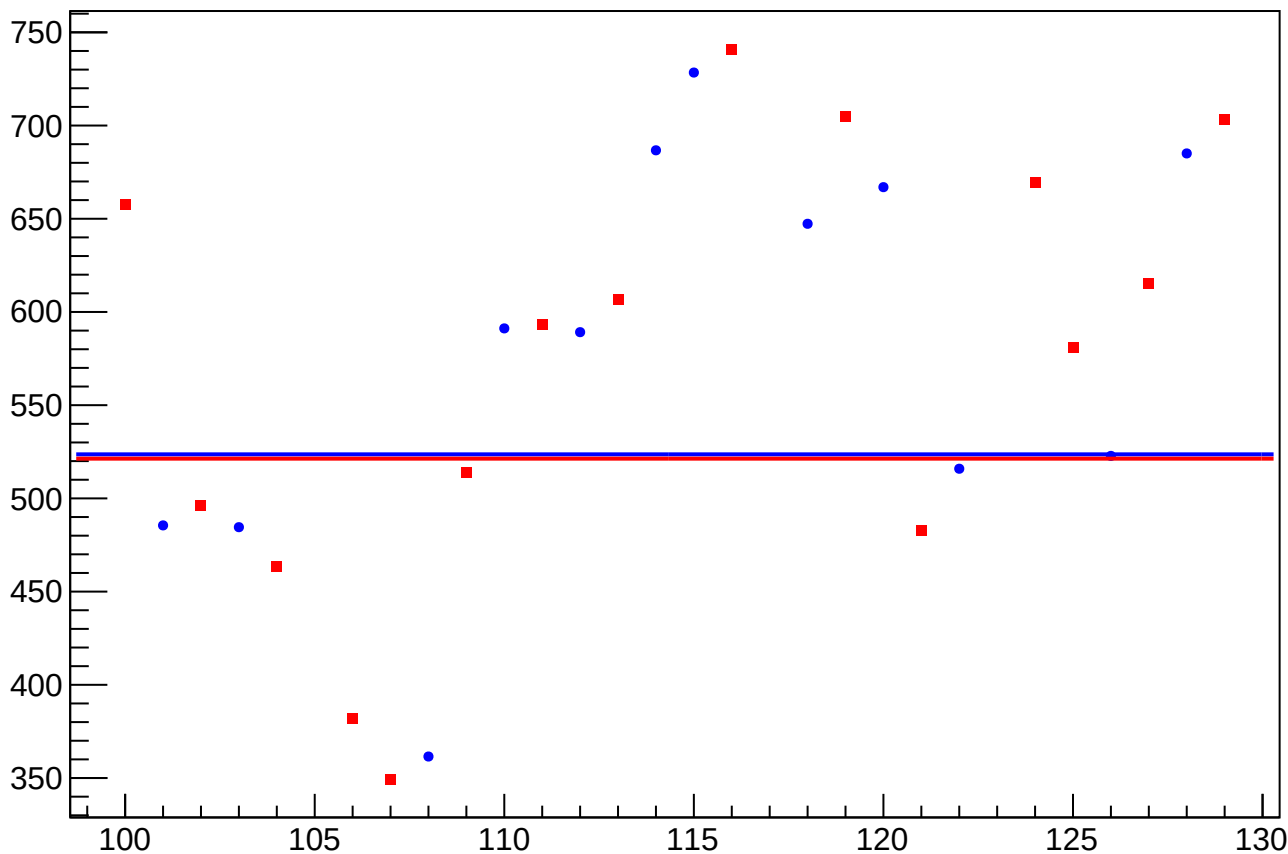
asym_sam_13_57_dd_reg_correction_rms vs Slug, Sign Corrected
