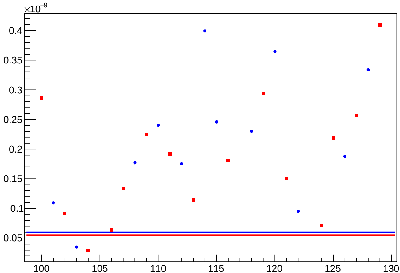
asym_atl_avg_atr_avg_avg_reg_vs_cor_diff_rms vs Slug, Sign Corrected
