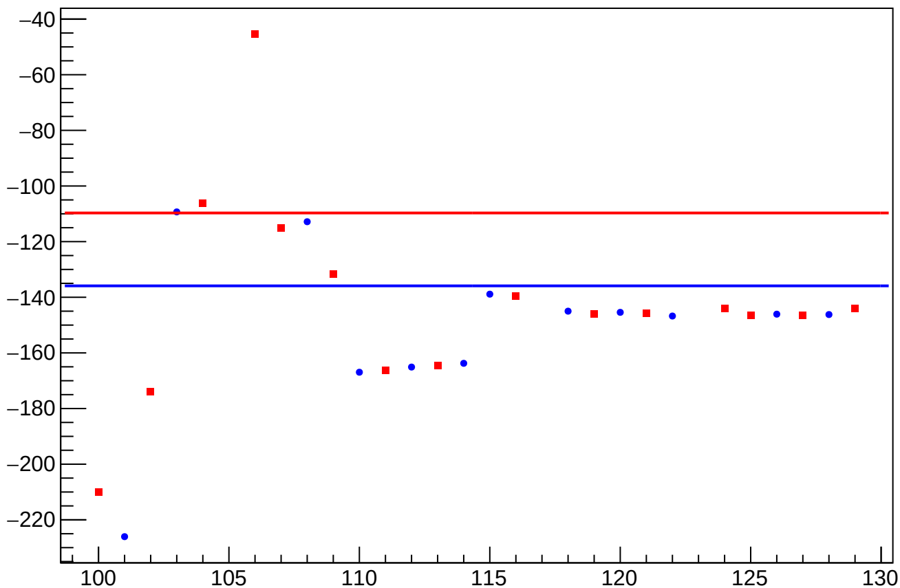
reg_asym_usr_atr2_avg_diff_bpm12X_slope vs Slug, Sign Corrected
