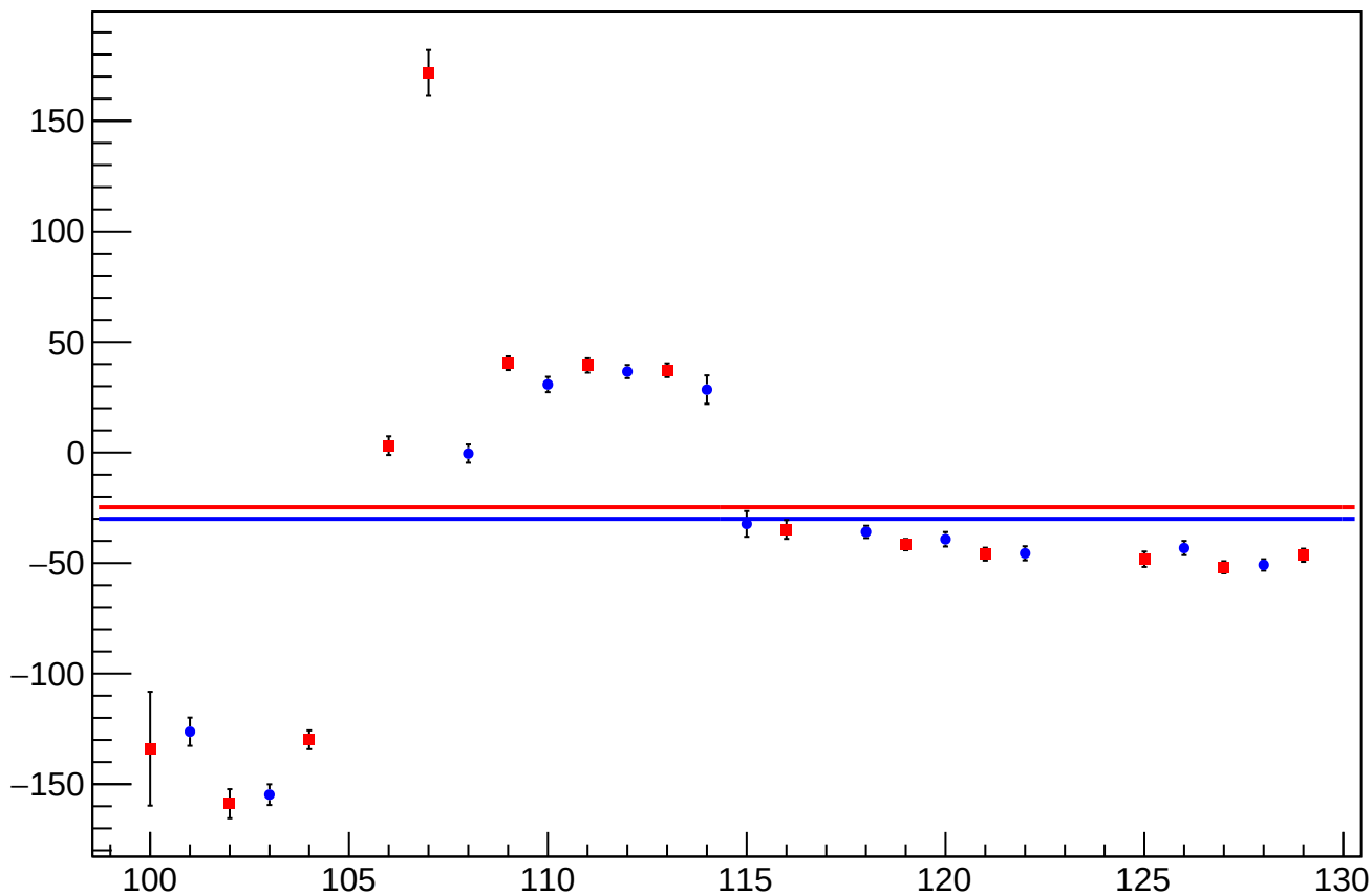
reg_asym_us_dd_at1lr_dd_avg_diff_bpm4eX_slope vs Slug, Sign Corrected
