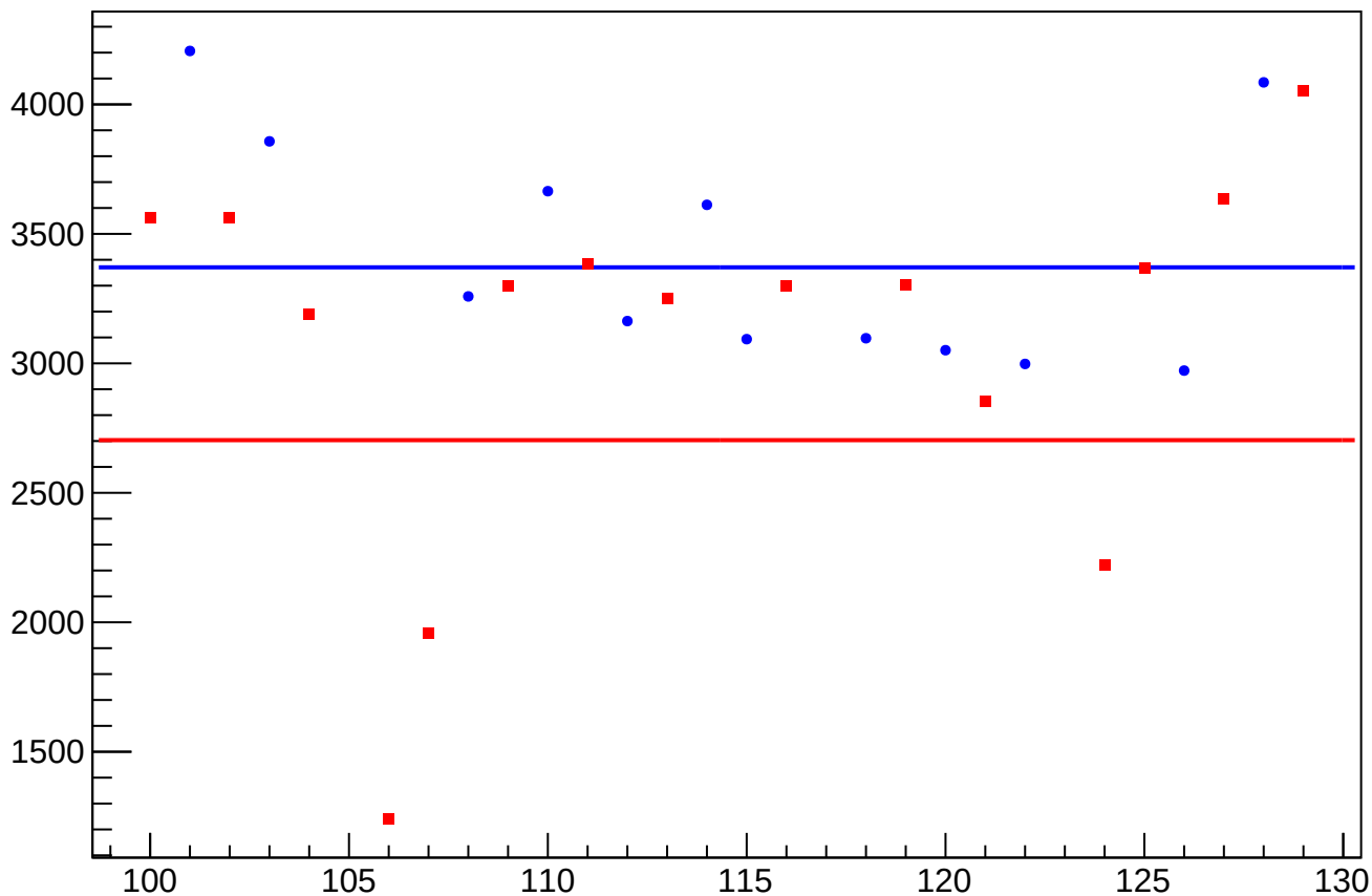
asym_atl1r2_dd_atl2r1_dd_dd_reg_correction_rms vs Slug, Sign Corrected
