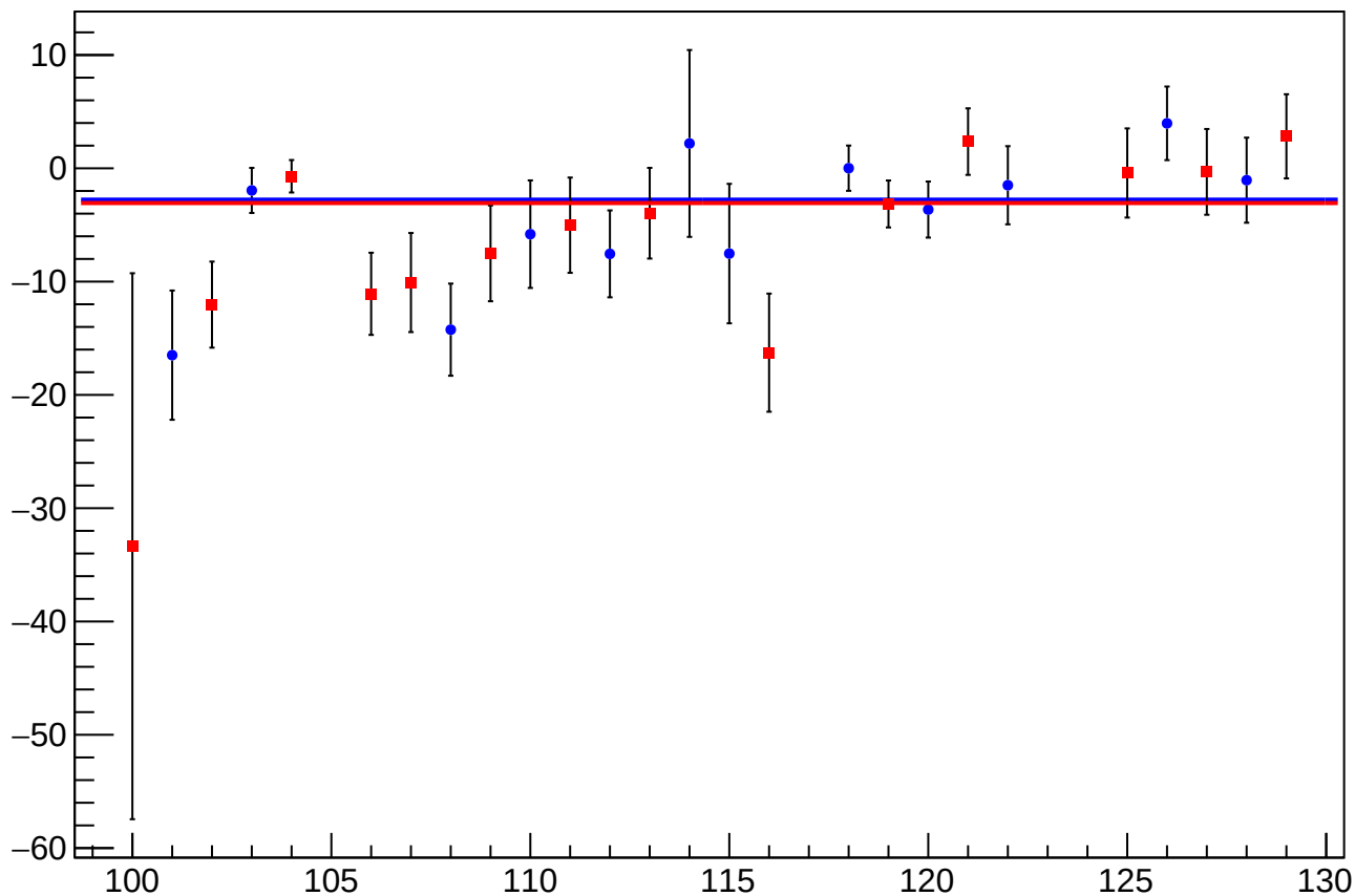
reg_asym_us_avg_atlr_avg_dd_diff_bpm4aY_slope vs Slug, Sign Corrected
