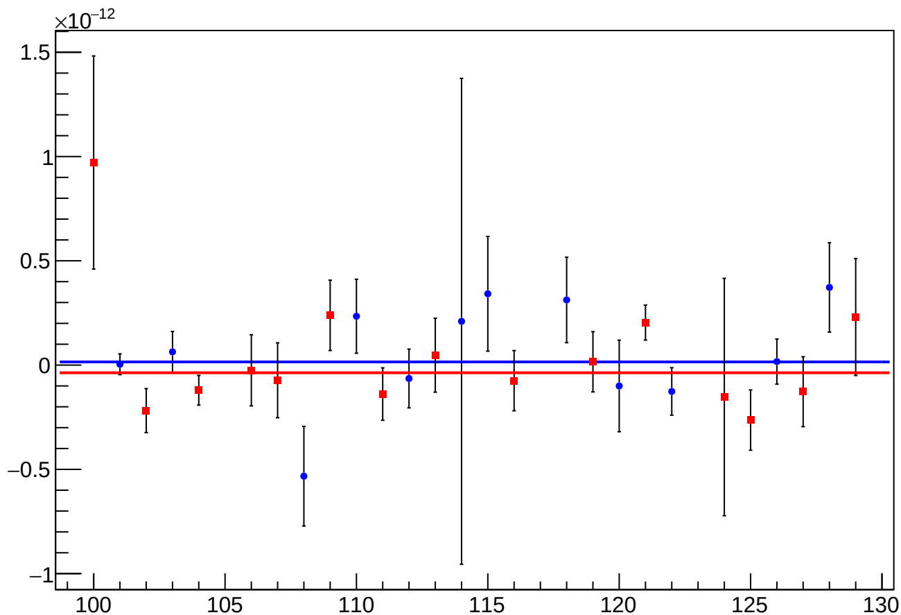
asym_atl_dd_atr_dd_dd_reg_vs_cor_diff_mean vs Slug, Sign Corrected
