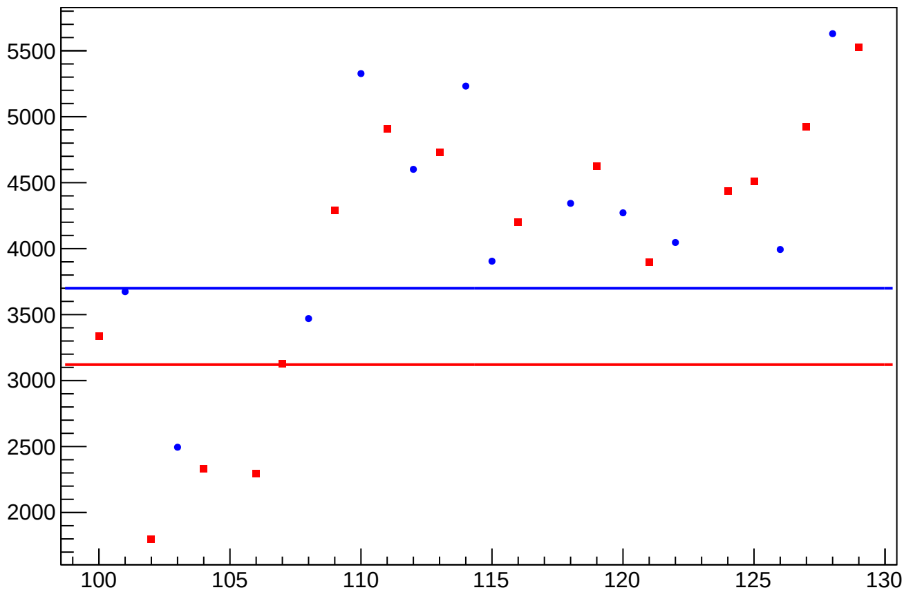
asym_atr_dd_reg_correction_rms vs Slug, Sign Corrected
