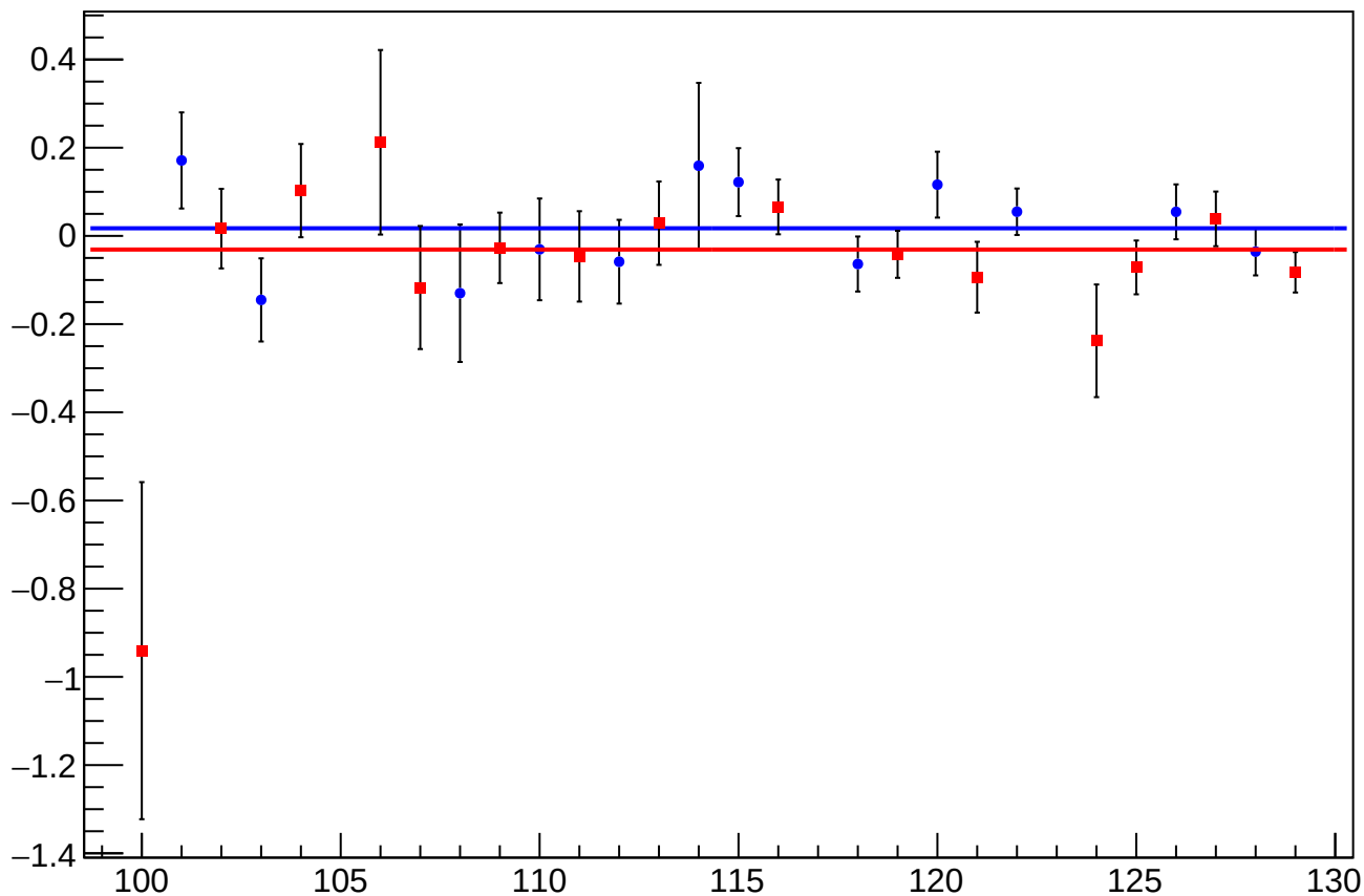
asym_sam_3726_avg_eigen_dit_vs_cor_diff_mean vs Slug, Sign Corrected
