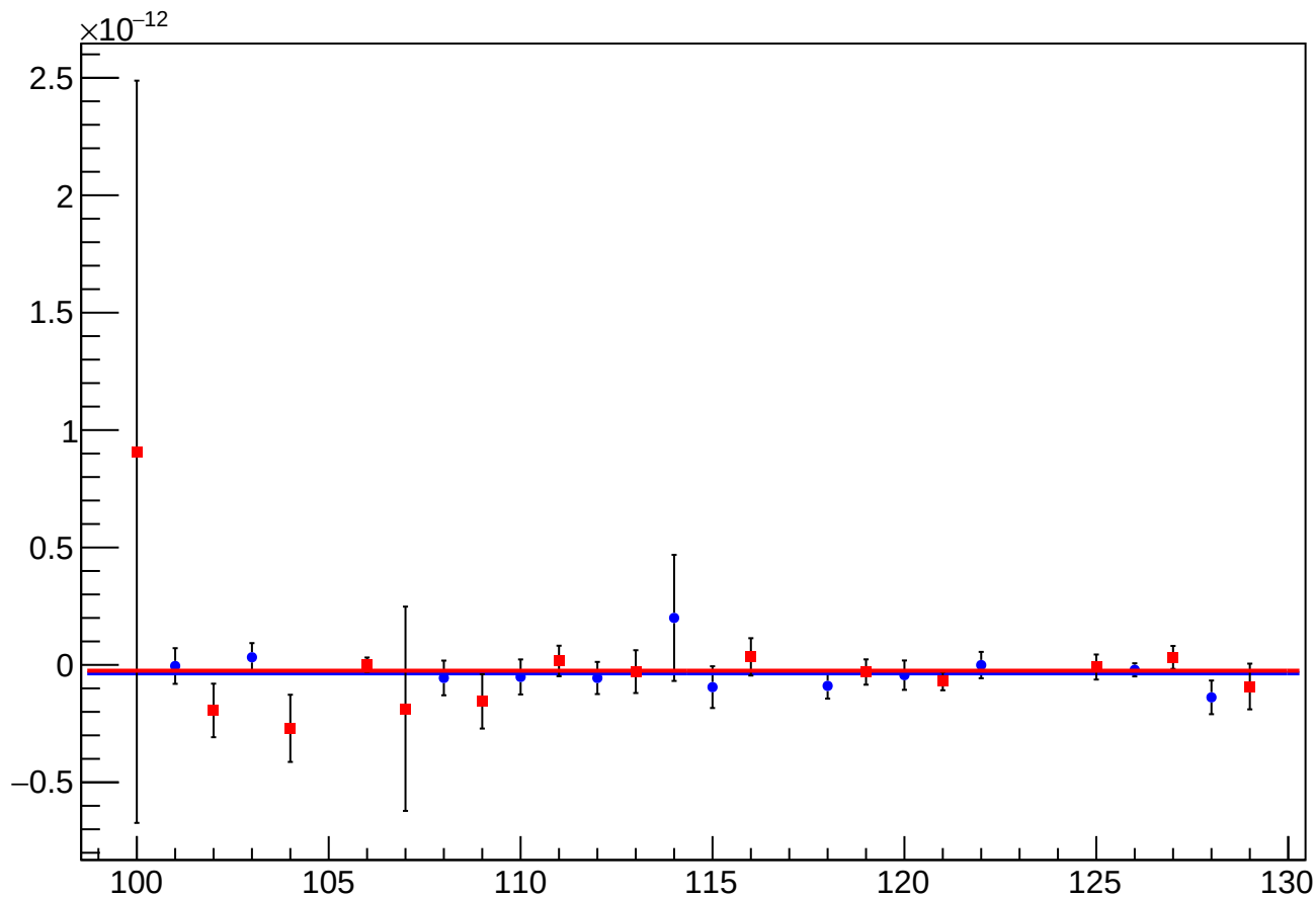
asym_us_dd_at1lr_dd_avg_reg_vs_cor_diff_mean vs Slug, Sign Corrected
