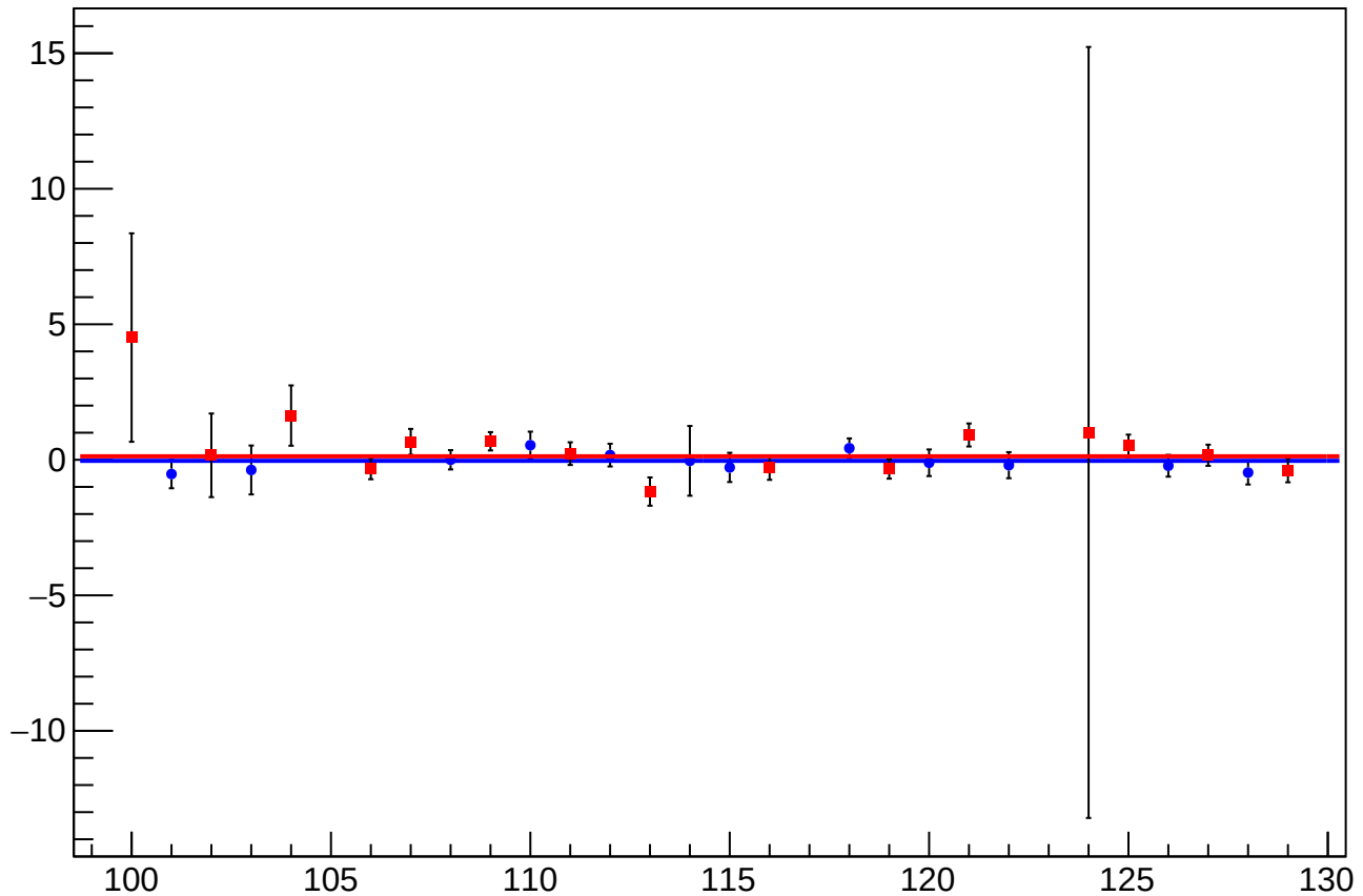
asym_at2_avg_eigen_dit_vs_cor_diff_mean vs Slug, Sign Corrected
