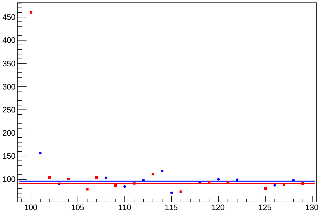
asym_usl_atl2_dd_dit_vs_cor_diff_rms vs Slug, Sign Corrected
