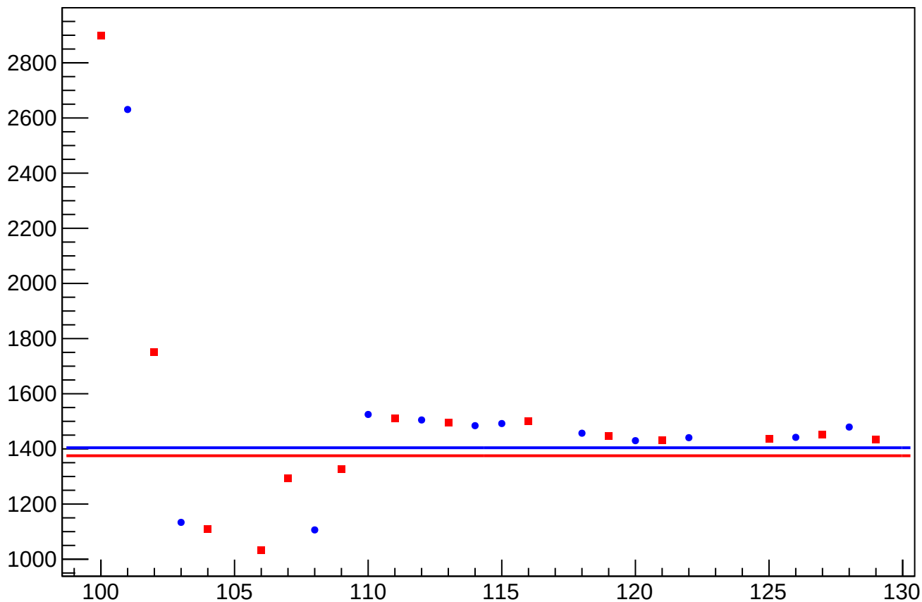
reg_asym_us_avg_at2lr_avg_dd_rms vs Slug, Sign Corrected
