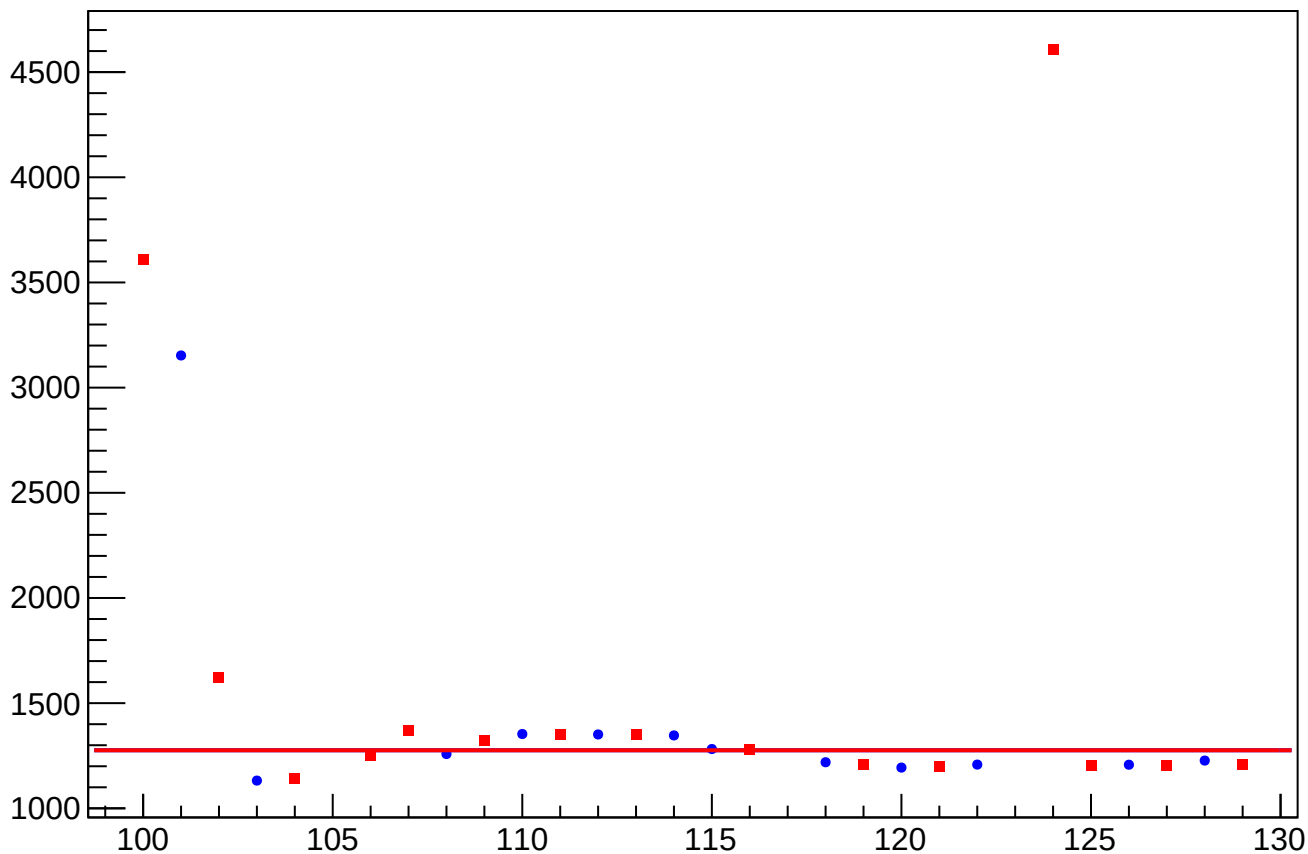
reg_asym_at1_dd_at2_dd_avg_rms vs Slug, Sign Corrected
