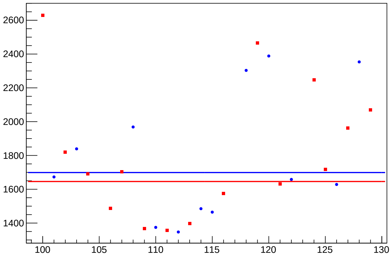
asym_sam3_reg_correction_rms vs Slug, Sign Corrected
