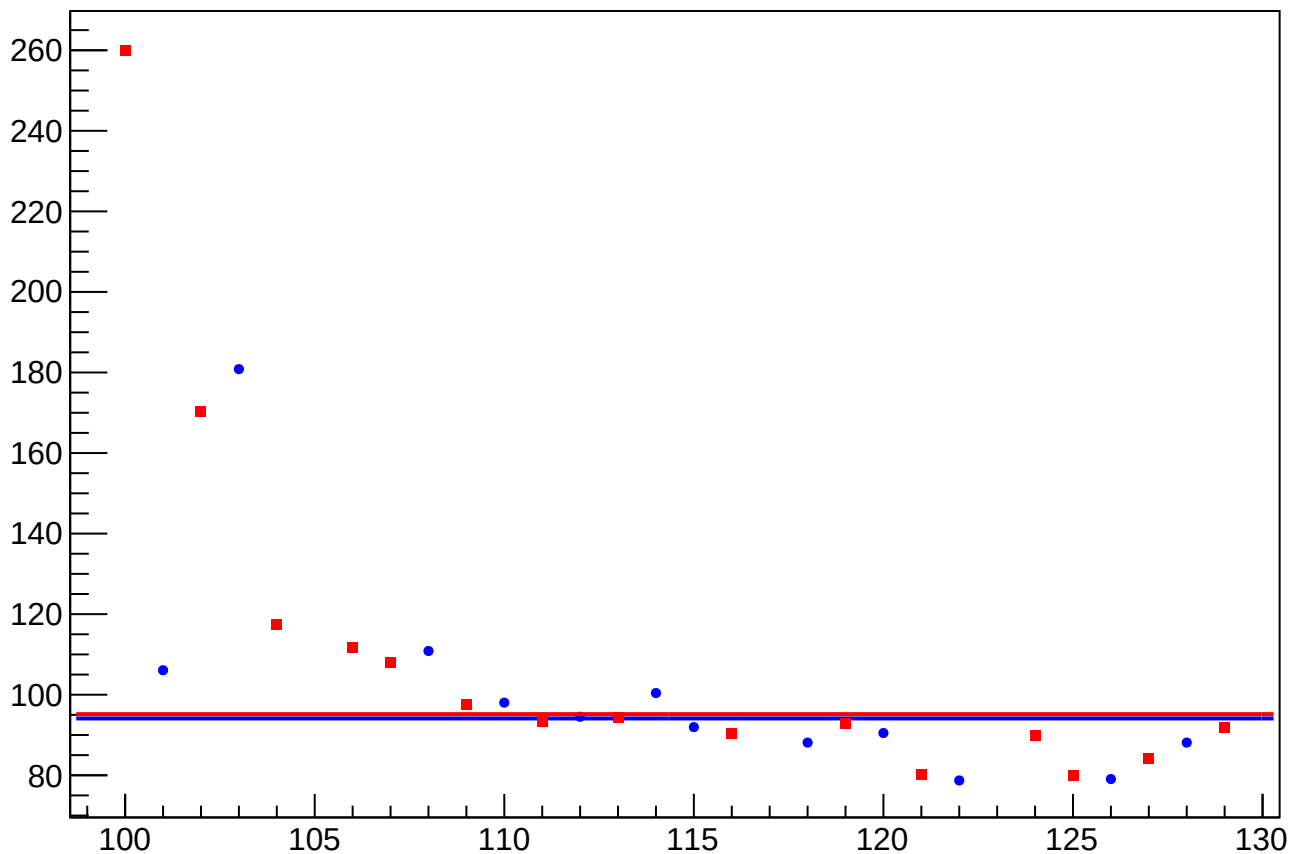
eigen_cor_asym_sam_2468_avg_rms vs Slug, Sign Corrected
