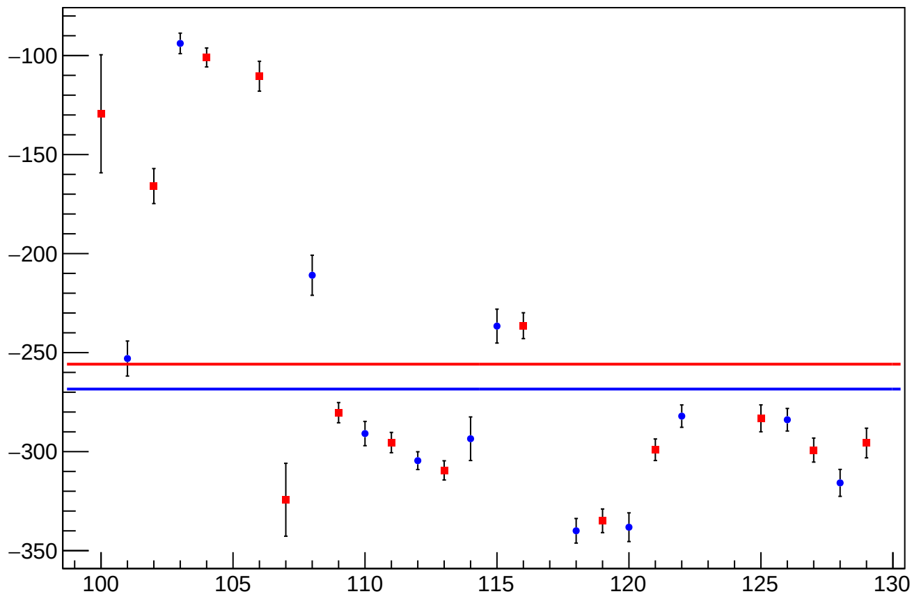
reg_asym_us_avg_atlr_avg_avg_diff_bpm1X_slope vs Slug, Sign Corrected
