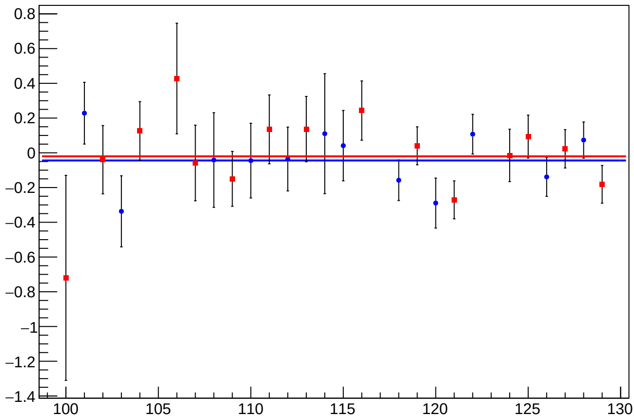
asym_sam_26_dd_eigen_dit_vs_cor_diff_mean vs Slug, Sign Corrected
