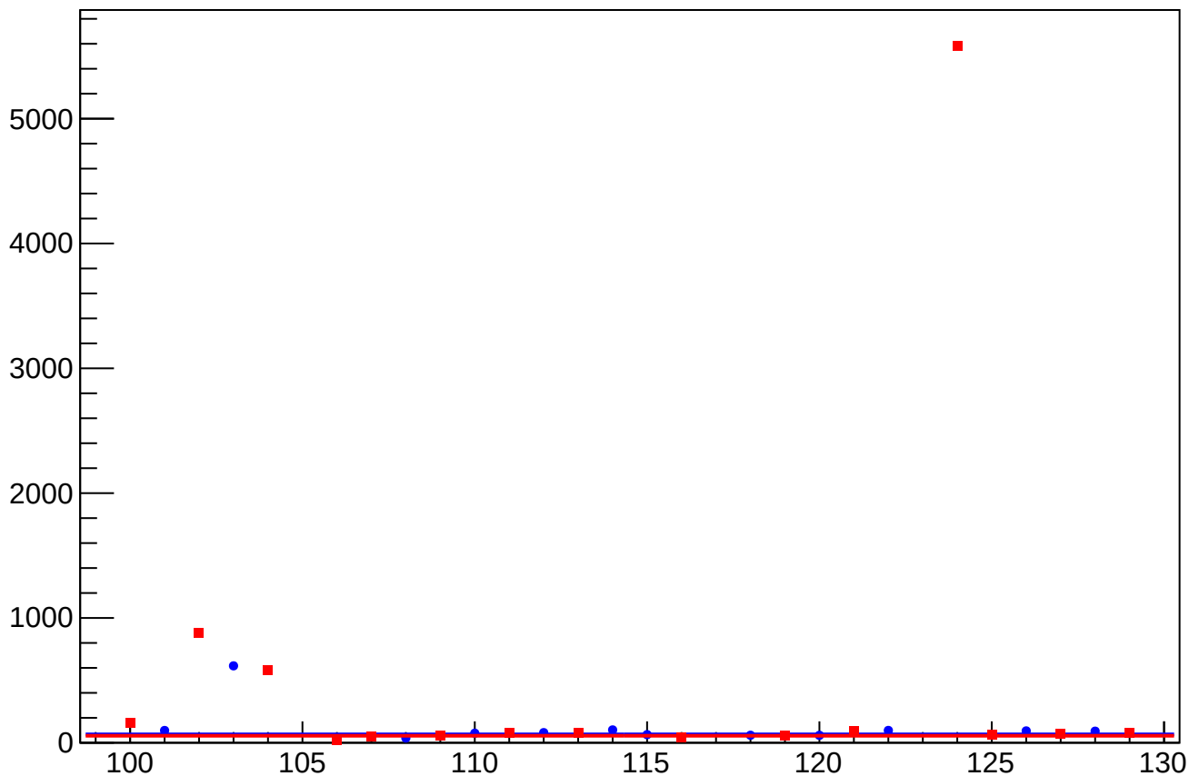
asym_at2_dd_dit_vs_eigen_cor_diff_rms vs Slug, Sign Corrected
