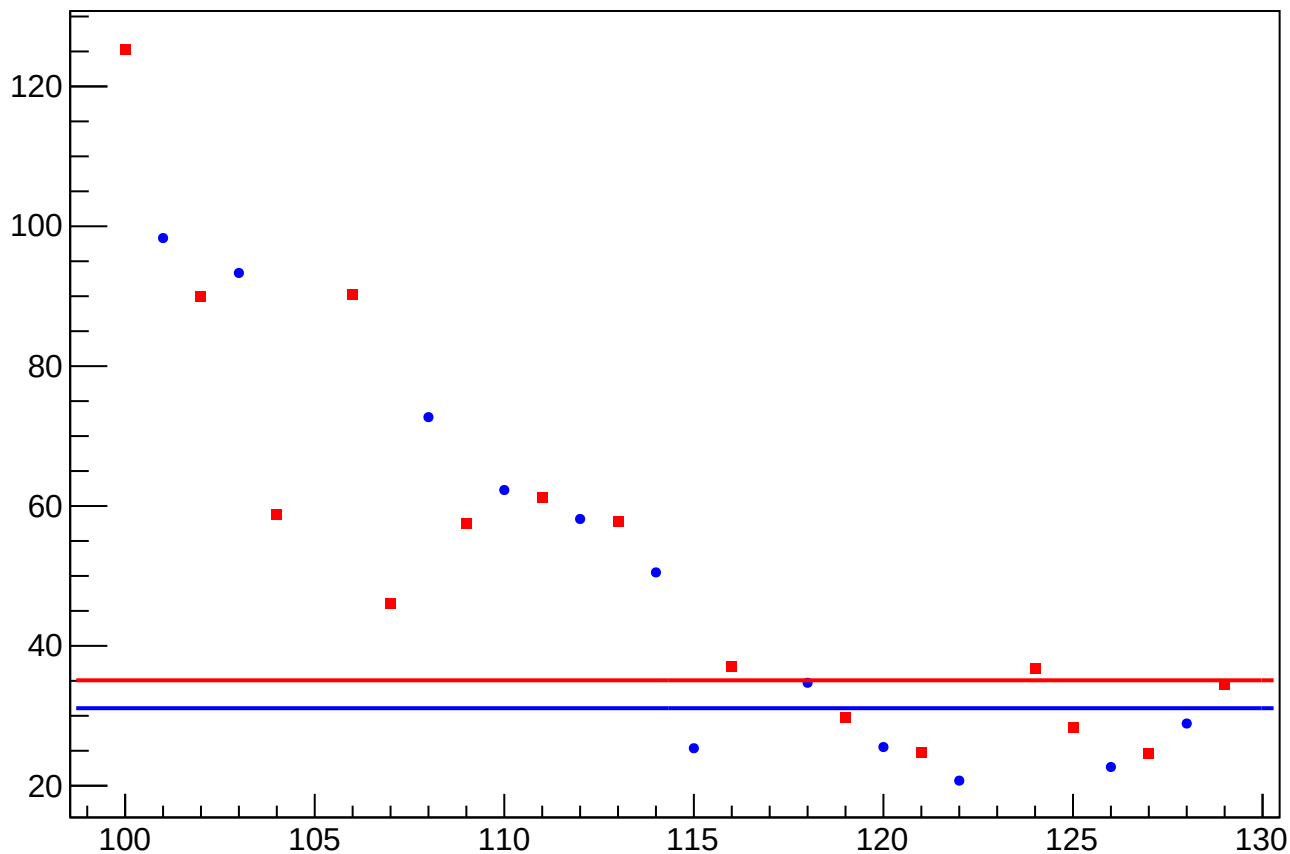
asym_sam_26_48_dd_dit_vs_cor_diff_rms vs Slug, Sign Corrected
