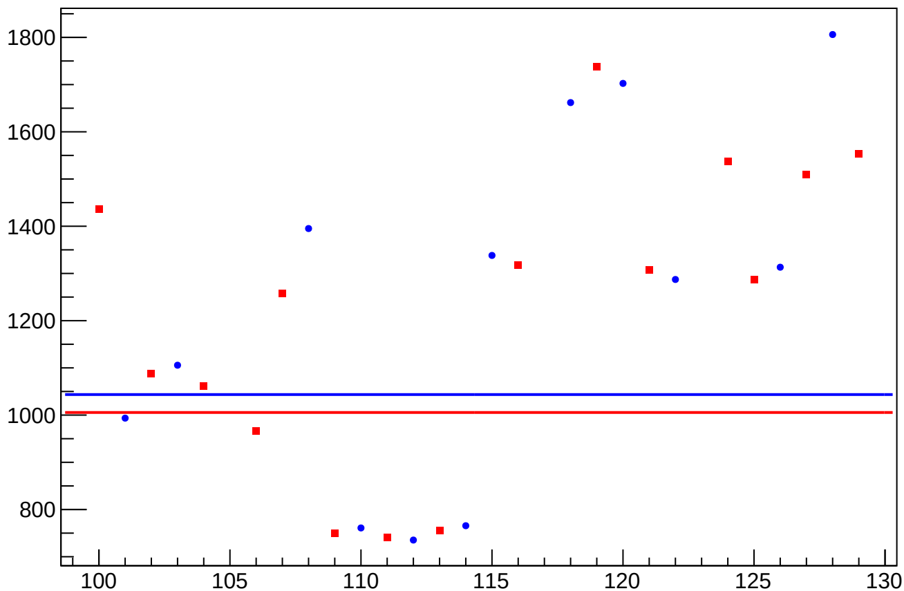
asym_sam_3748_avg_cor_correction_rms vs Slug, Sign Corrected
