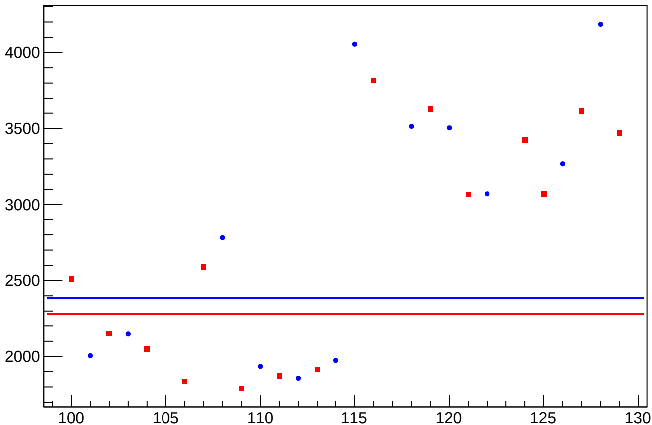
asym_sam4_eigen_dit_correction_rms vs Slug, Sign Corrected
