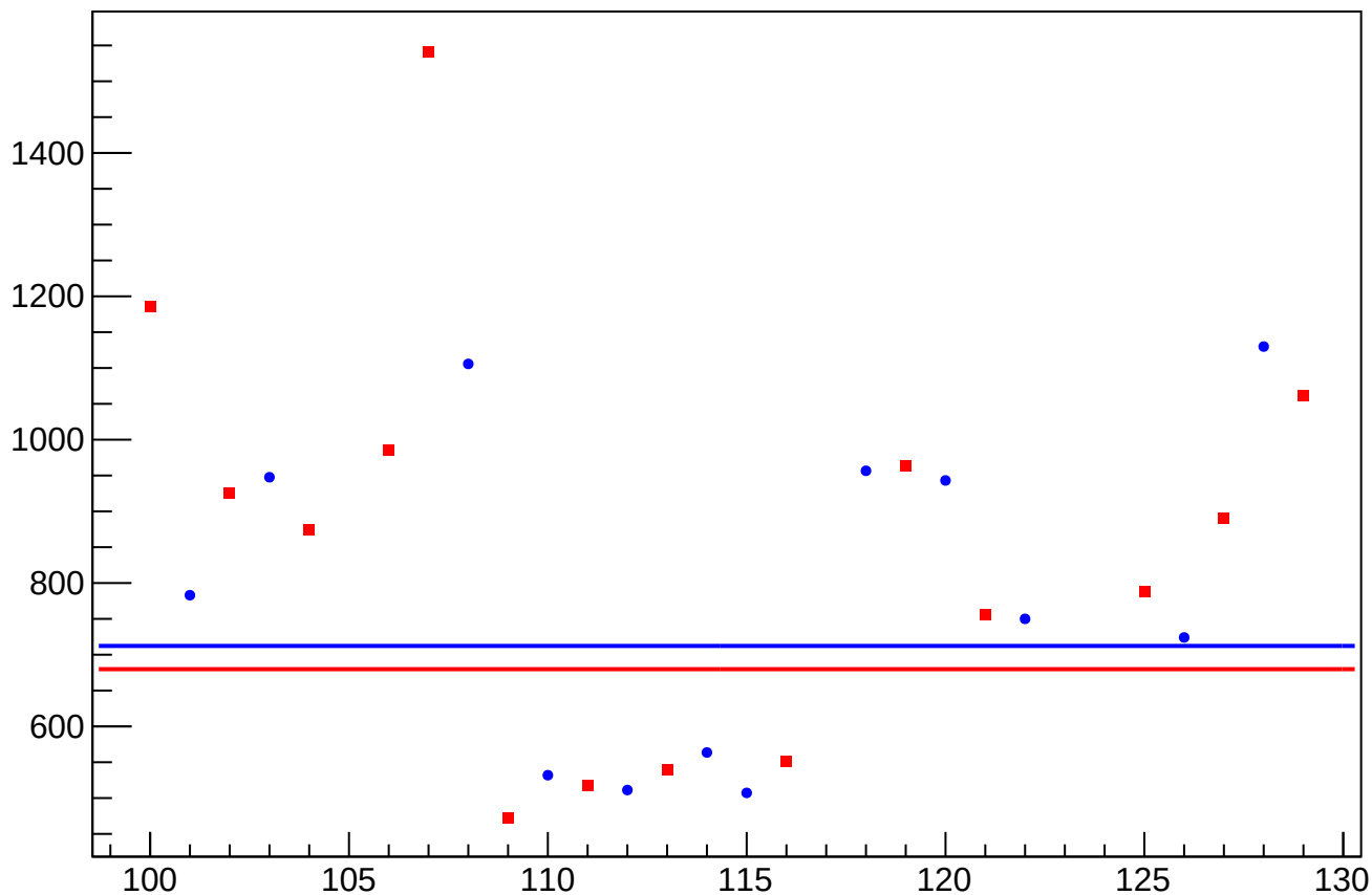
asym_us_dd_eigen_dit_correction_rms vs Slug, Sign Corrected
