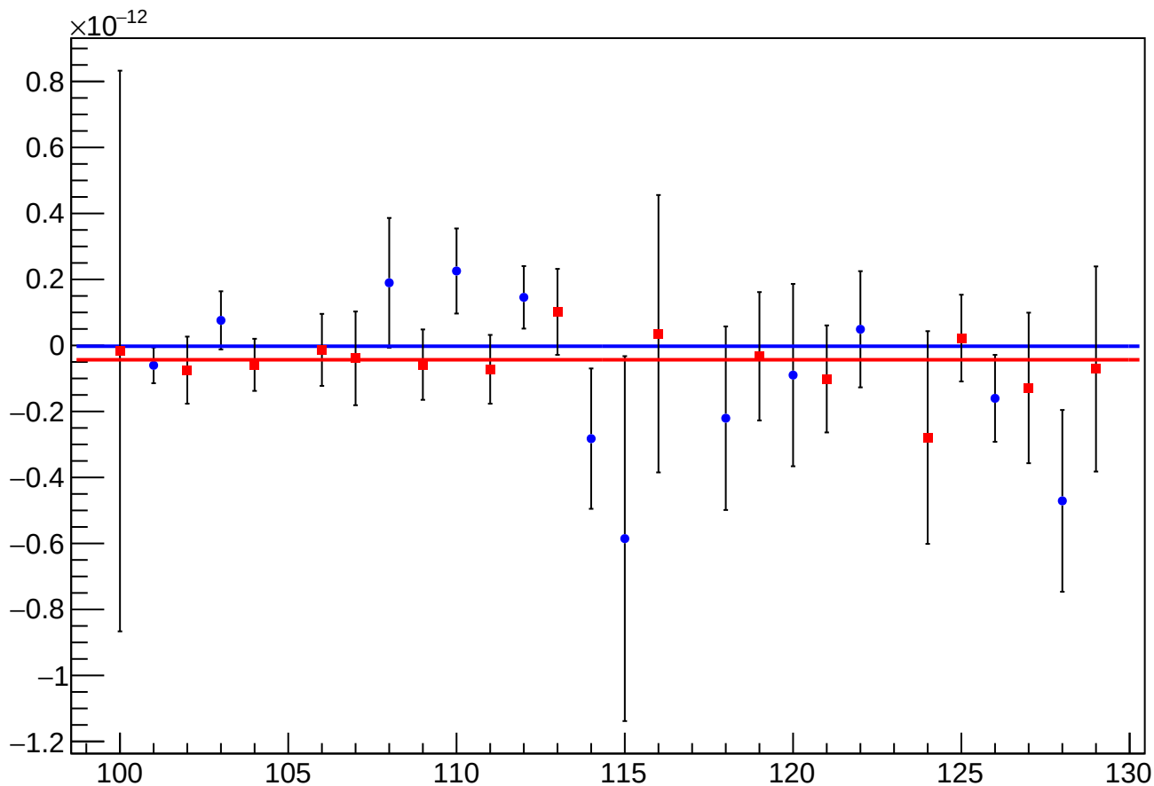
asym_sam_48_avg_reg_vs_cor_diff_mean vs Slug, Sign Corrected
