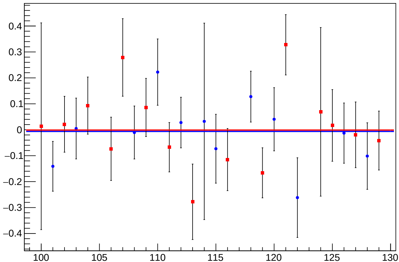
asym_usr_eigen_dit_vs_cor_diff_mean vs Slug, Sign Corrected
