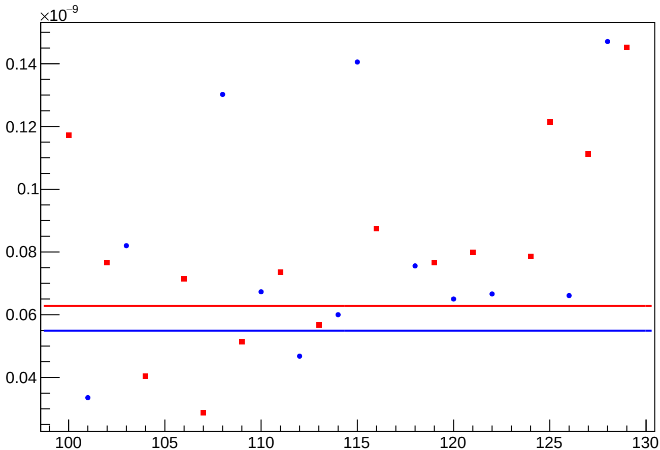
asym_sam4_eigen_cor_vs_cor_diff_rms vs Slug, Sign Corrected
