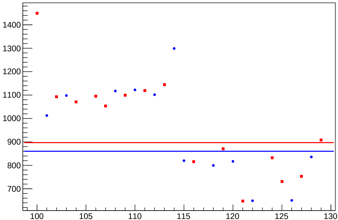
asym_sam_15_26_dd_cor_correction_rms vs Slug, Sign Corrected
