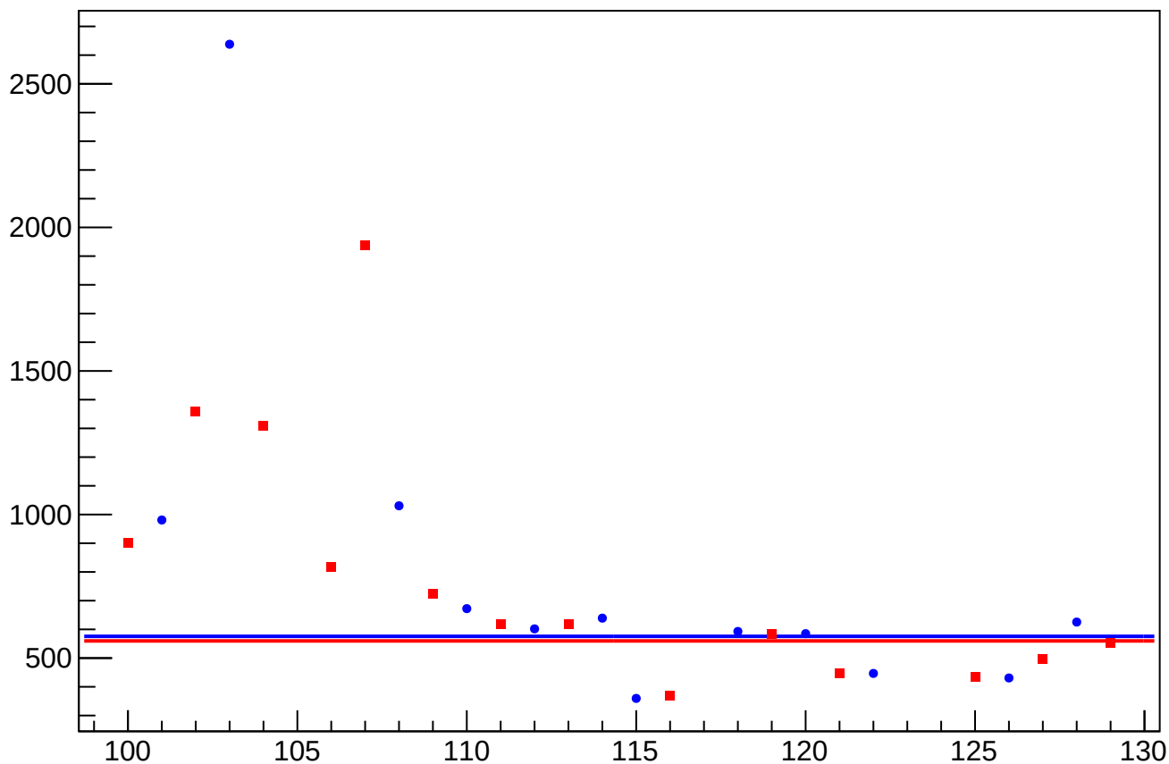
asym_usl_atl1_dd_cor_correction_rms vs Slug, Sign Corrected
