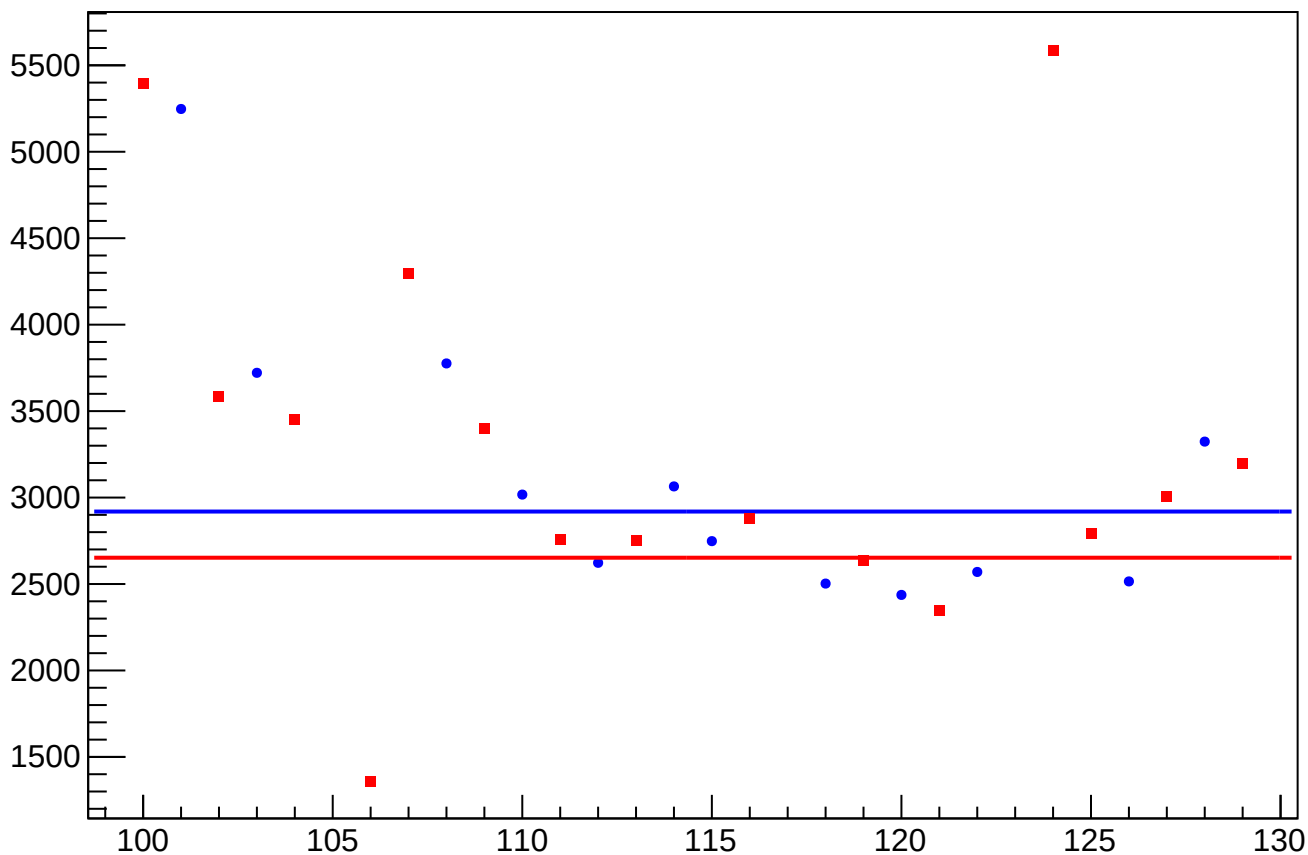
asym_atr1l2_avg_dit_correction_rms vs Slug, Sign Corrected
