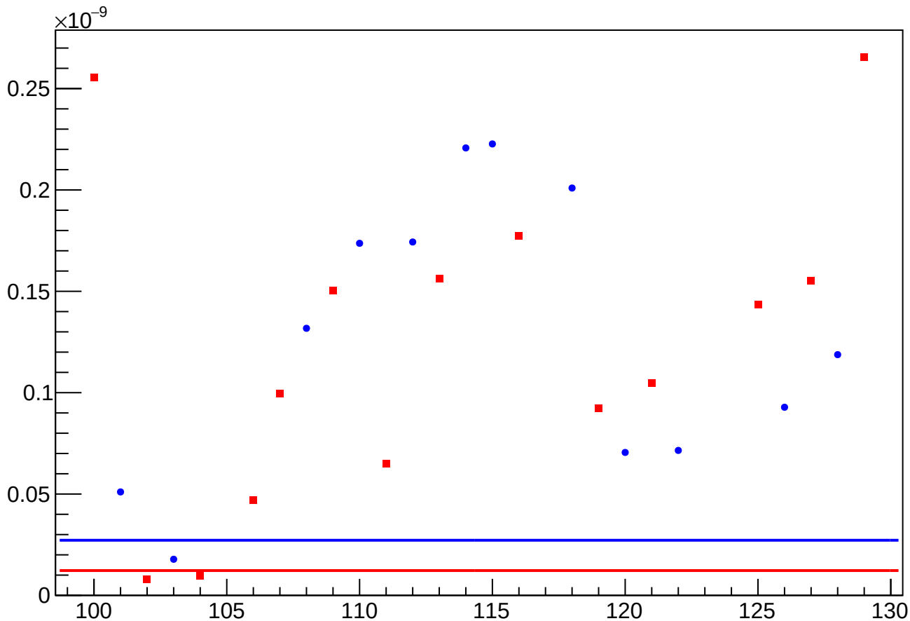
asym_us_avg_atlr_avg_dd_reg_vs_cor_diff_rms vs Slug, Sign Corrected
