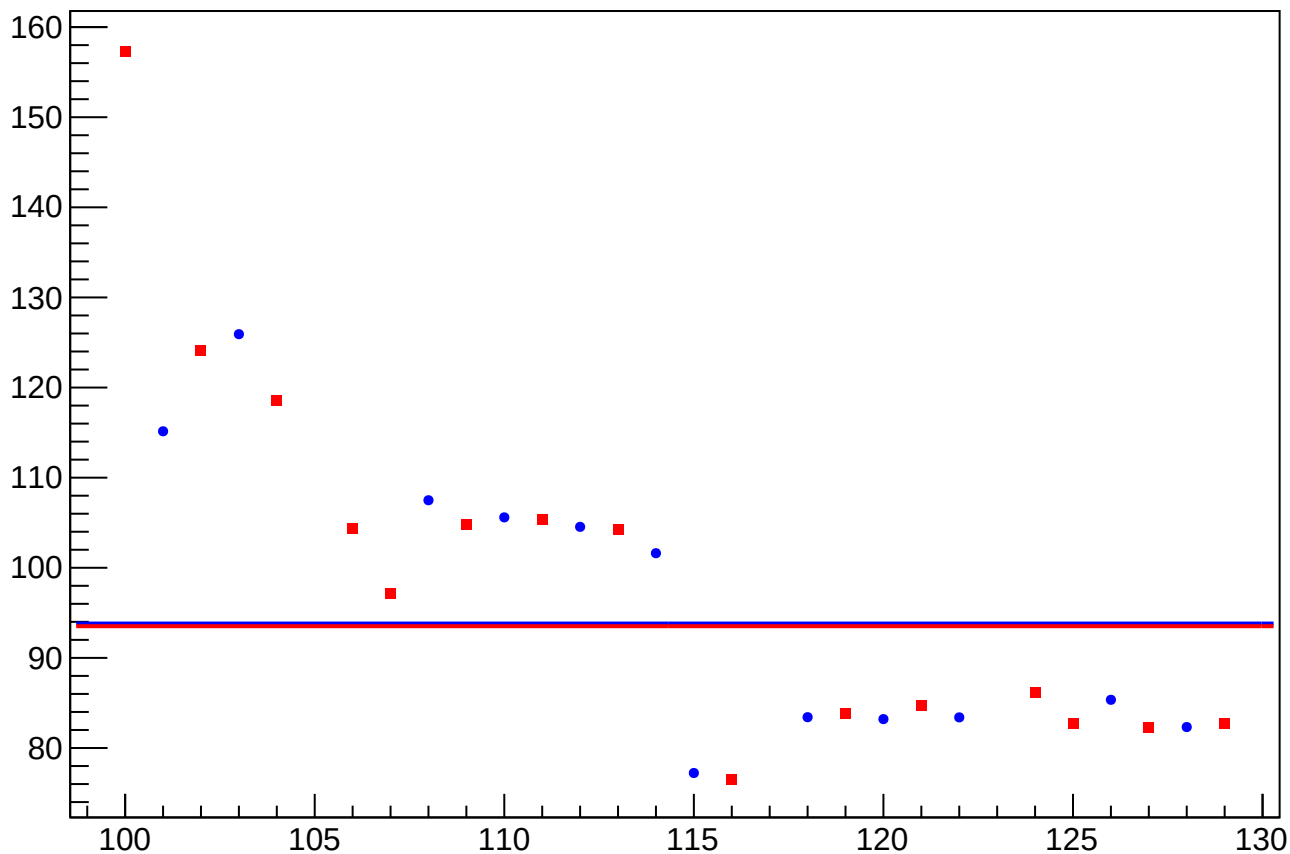
eigen_cor_asym_sam_24_68_dd_rms vs Slug, Sign Corrected
