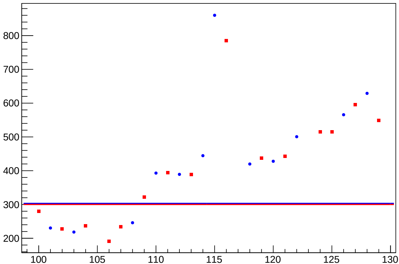
asym_sam_37_48_dd_reg_correction_rms vs Slug, Sign Corrected
