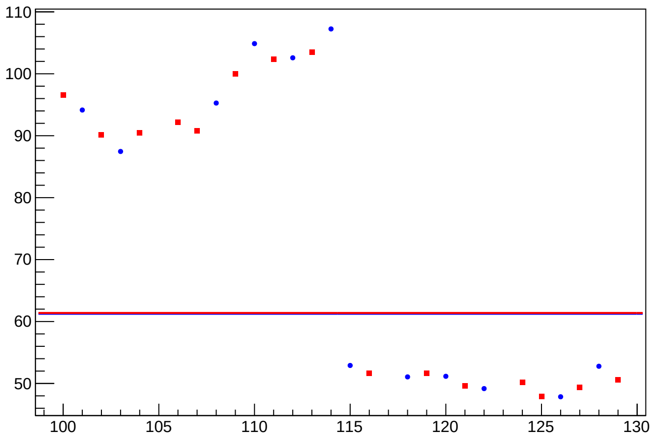
cor_asym_sam_37_26_dd_rms vs Slug, Sign Corrected
