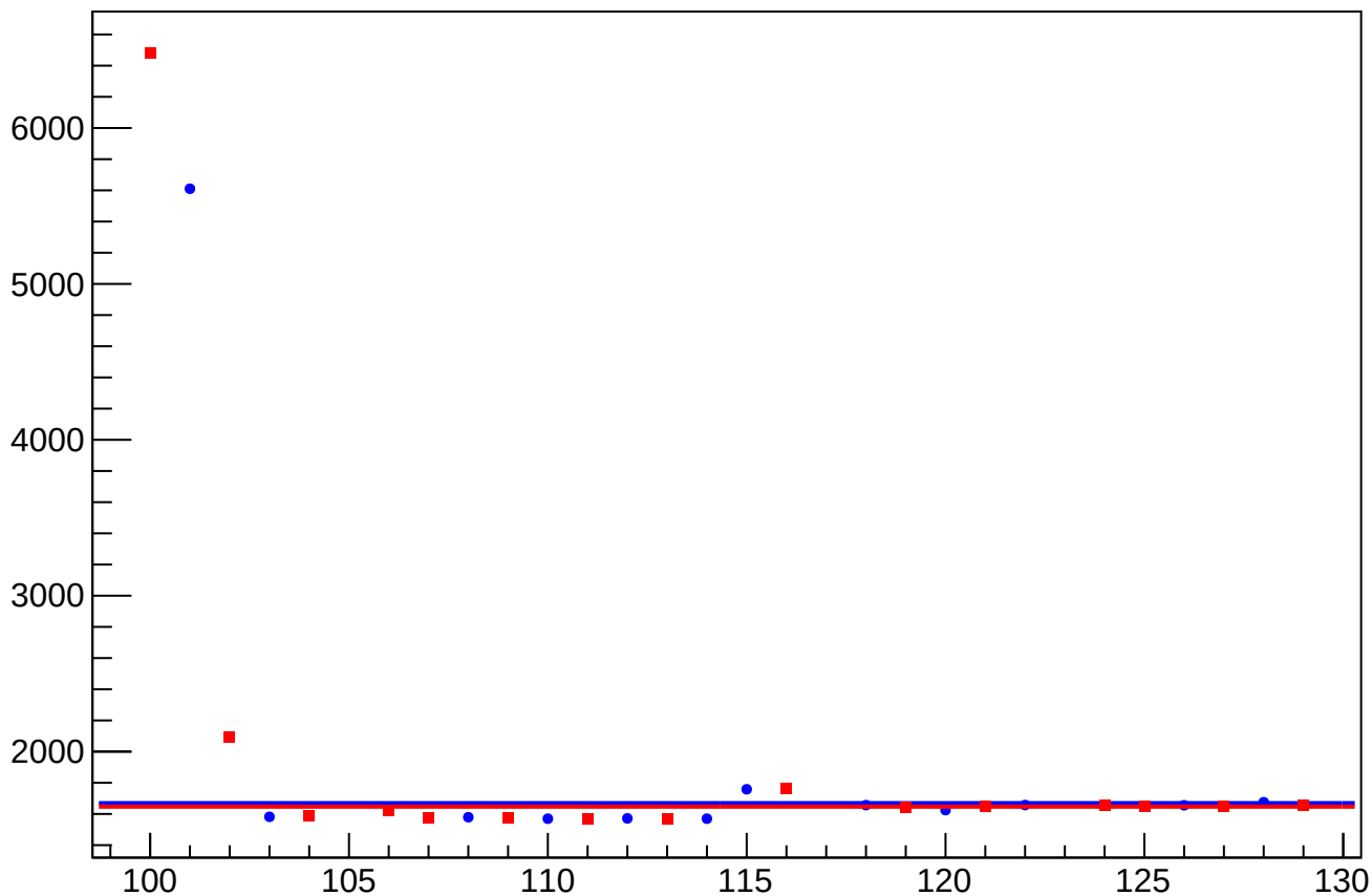
eigen_cor_asym_usr_atr1_avg_rms vs Slug, Sign Corrected
