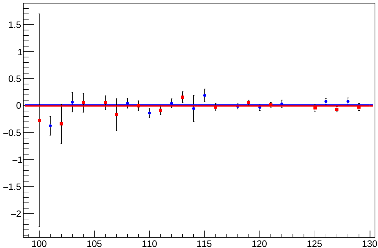
asym_us_dd_at1lr_dd_dd_dit_vs_eigen_cor_diff_mean vs Slug, Sign Corrected
