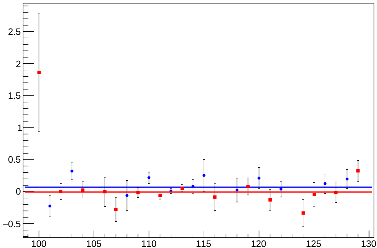
asym_sam4_dit_vs_eigen_cor_diff_mean vs Slug, Sign Corrected
