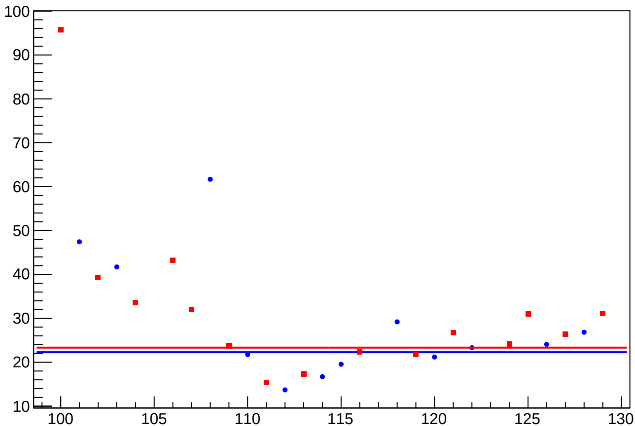
asym_sam_15_48_dd_dit_vs_cor_diff_rms vs Slug, Sign Corrected
