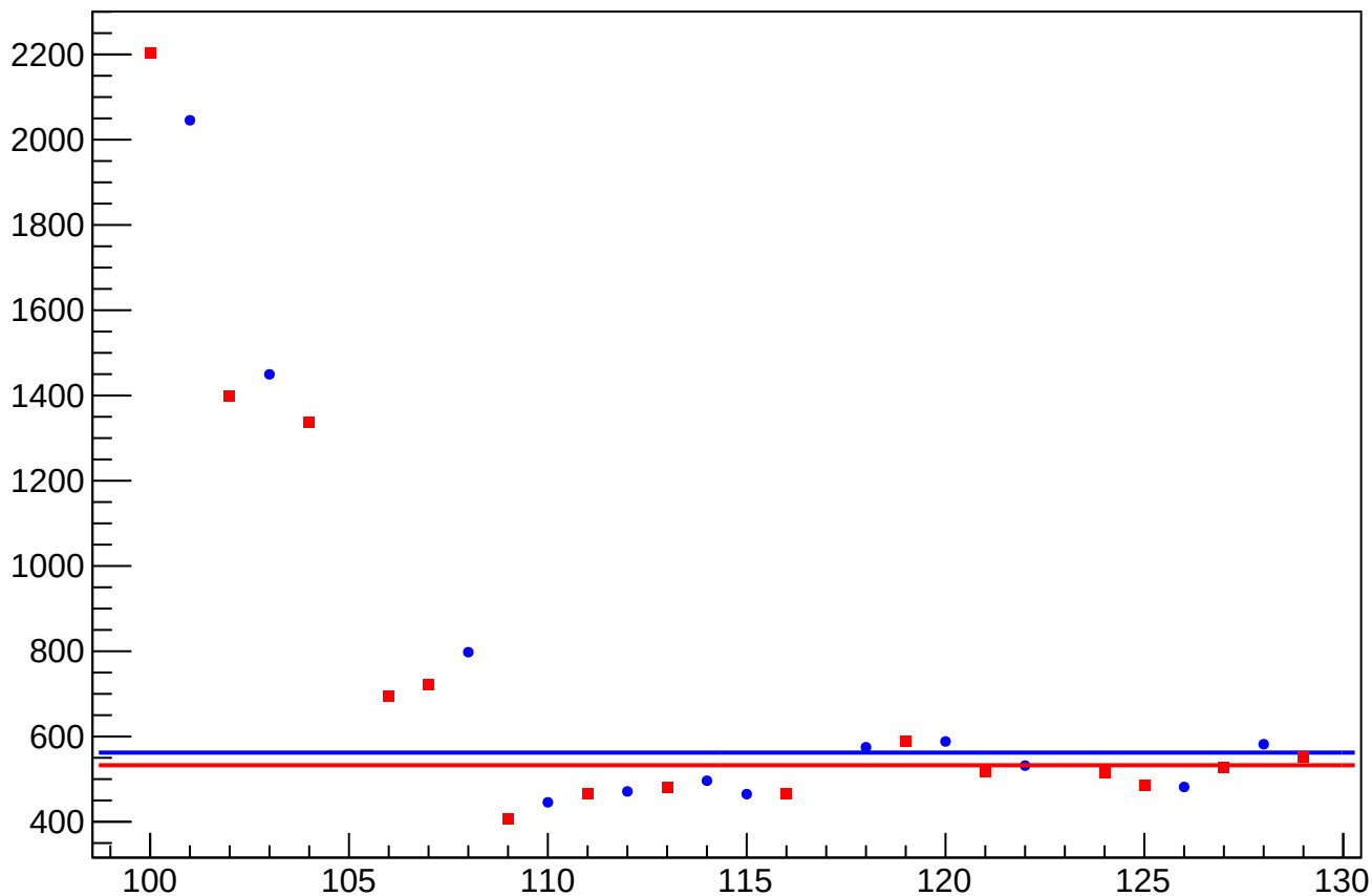
asym_atr1_eigen_dit_correction_rms vs Slug, Sign Corrected
