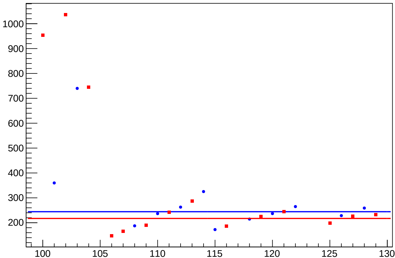
asym_us_avg_at2lr_avg_dd_dit_vs_cor_diff_rms vs Slug, Sign Corrected
