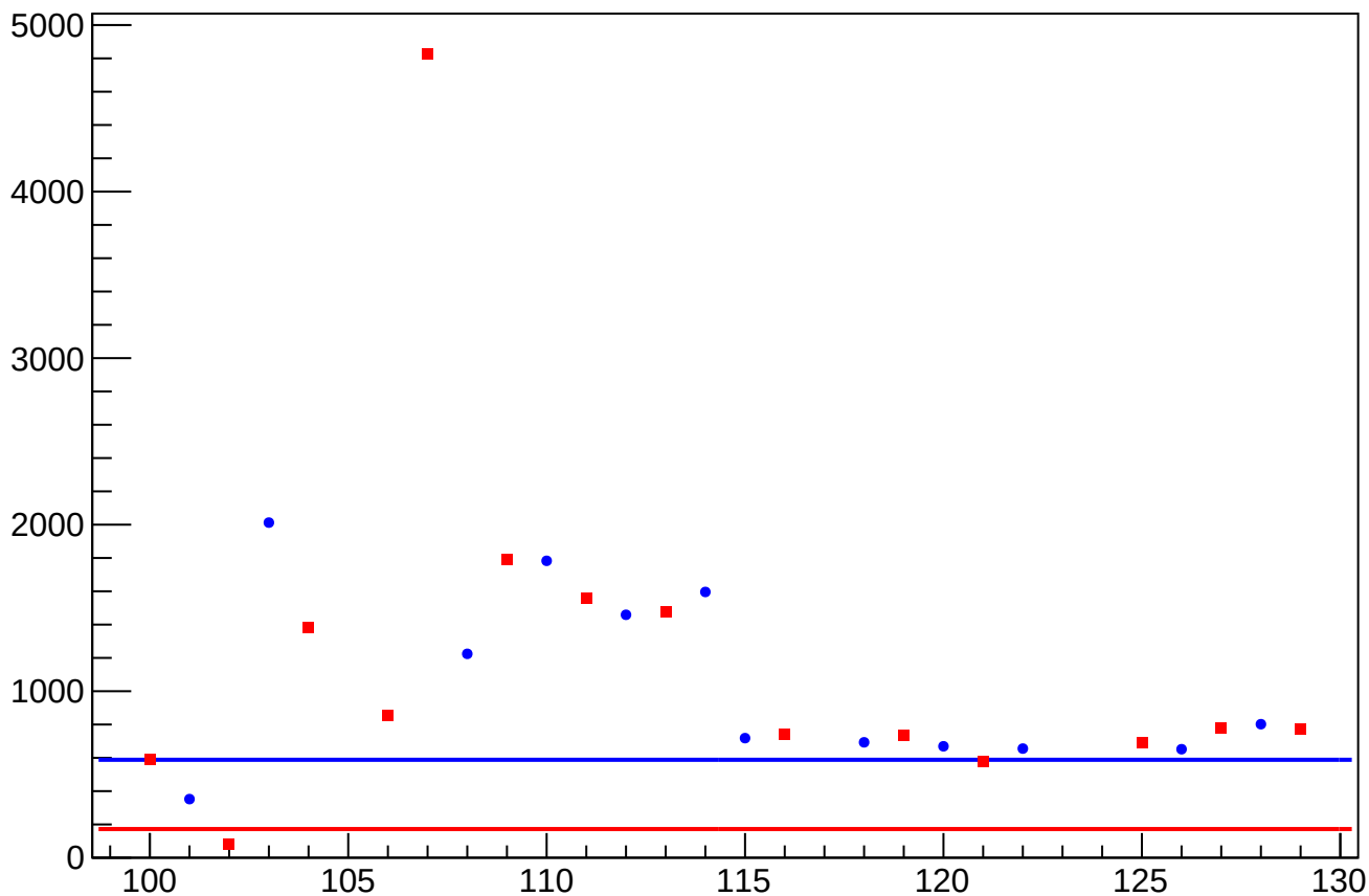
asym_usl_atl1_avg_eigen_cor_correction_rms vs Slug, Sign Corrected
