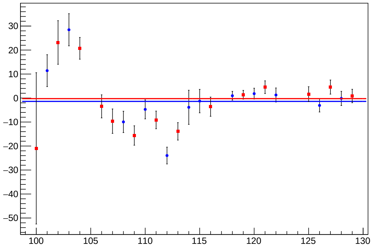
reg_asym_us_dd_at1lr_dd_dd_diff_bpm4aY_slope vs Slug, Sign Corrected
