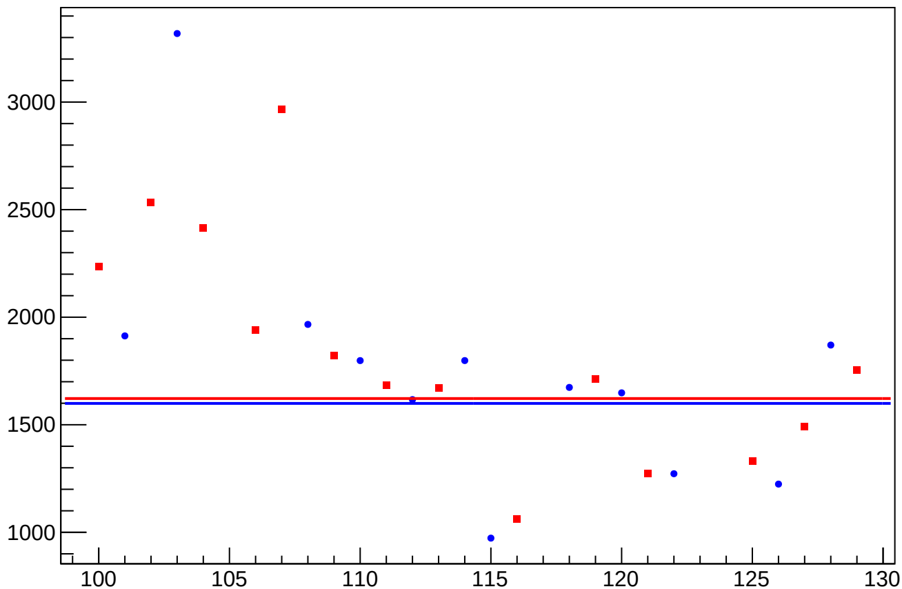
asym_us_dd_at1lr_dd_dd_reg_correction_rms vs Slug, Sign Corrected
