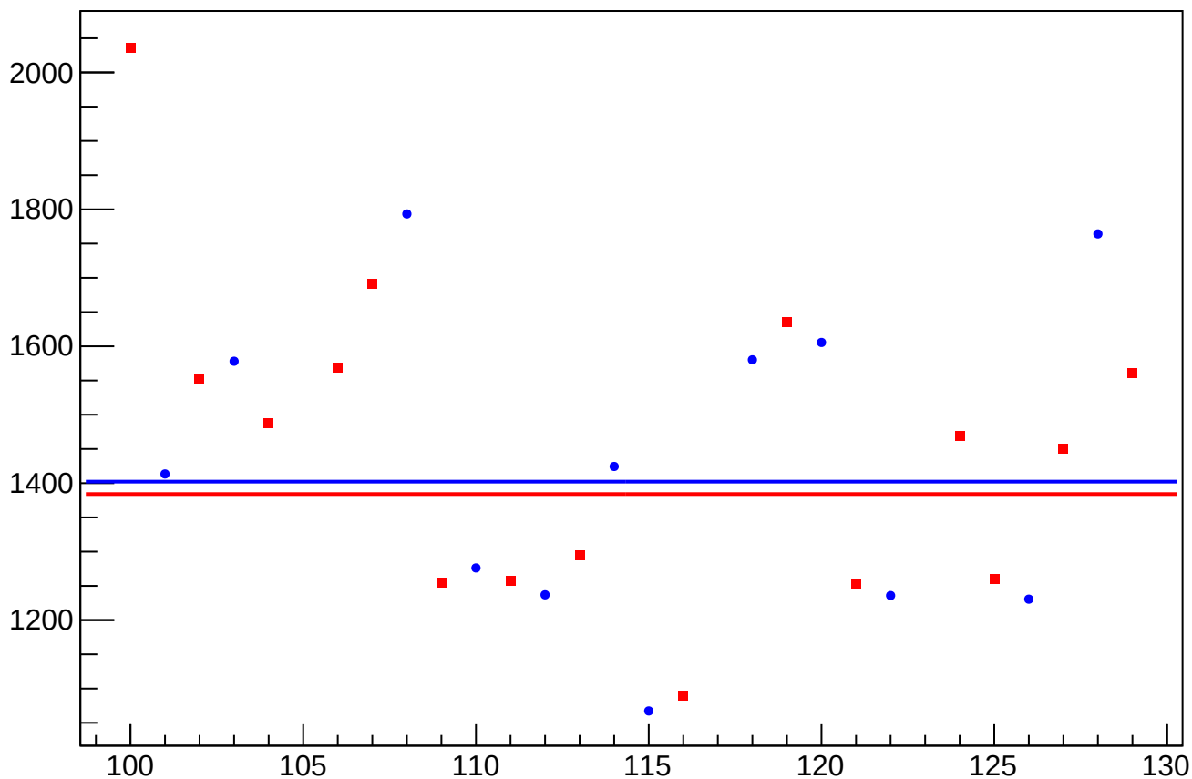
asym_sam_2468_avg_cor_correction_rms vs Slug, Sign Corrected
