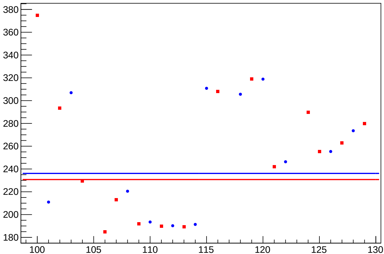
eigen_cor_asym_sam4_rms vs Slug, Sign Corrected
