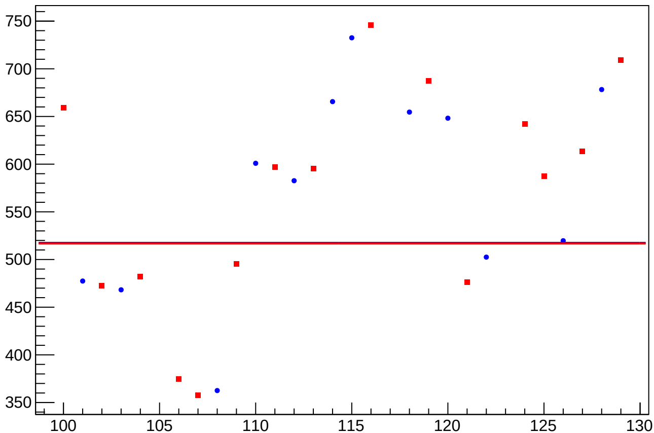
asym_sam_13_57_dd_eigen_dit_correction_rms vs Slug, Sign Corrected
