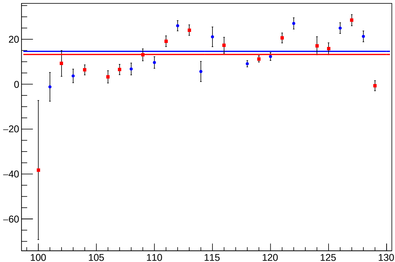
reg_asym_usr_atr1_avg_diff_bpm4aY_slope vs Slug, Sign Corrected
