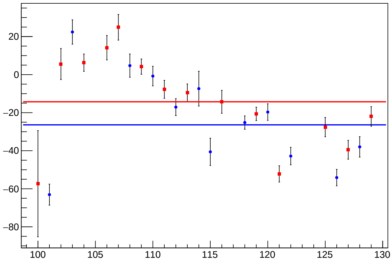
reg_asym_us_dd_at2lr_dd_avg_diff_bpm4eY_slope vs Slug, Sign Corrected
