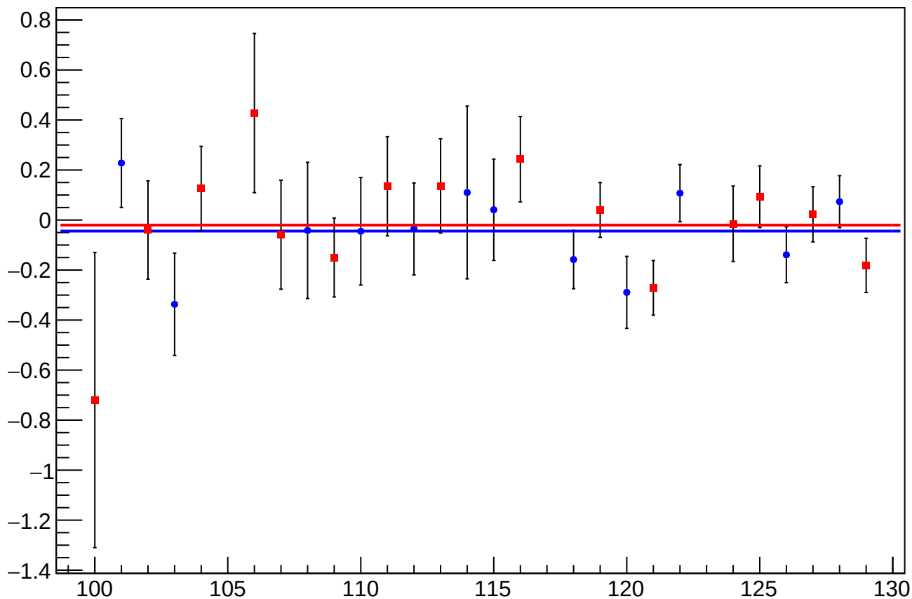
asym_sam_26_dd_dit_vs_eigen_cor_diff_mean vs Slug, Sign Corrected
