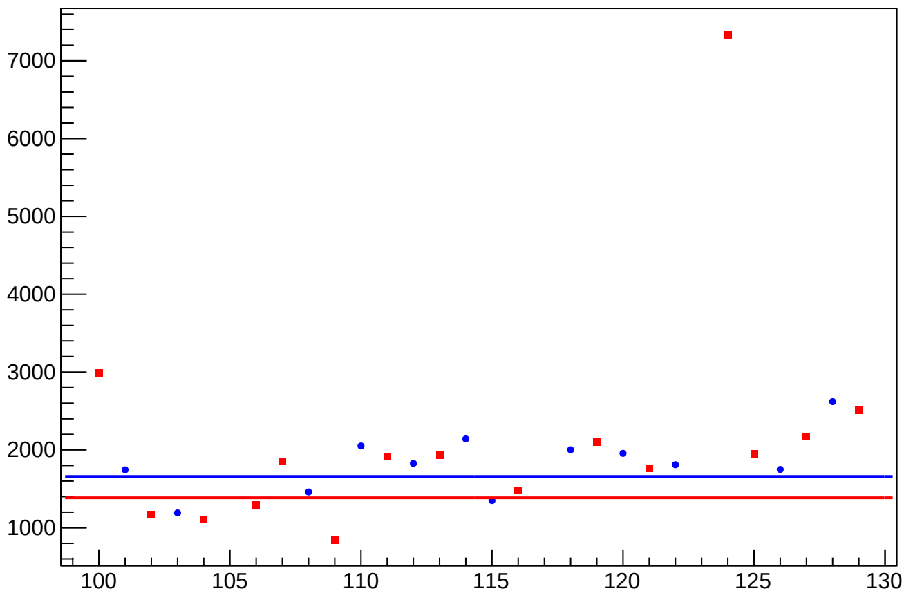
asym_at2_dd_dit_correction_rms vs Slug, Sign Corrected
