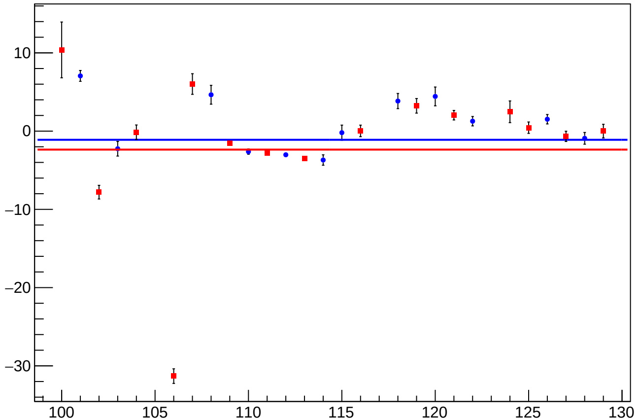
reg_asym_sam_15_37_dd_diff_bpm1X_slope vs Slug, Sign Corrected
