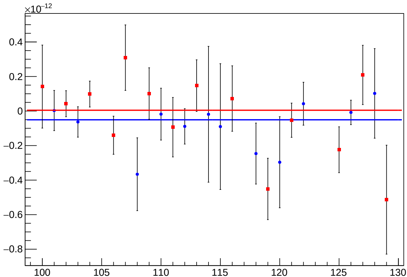
asym_usl_atl2_dd_eigen_cor_vs_cor_diff_mean vs Slug, Sign Corrected
