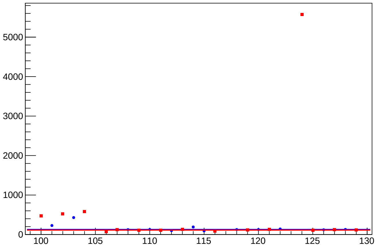
asym_atr1l2_avg_dit_vs_cor_diff_rms vs Slug, Sign Corrected
