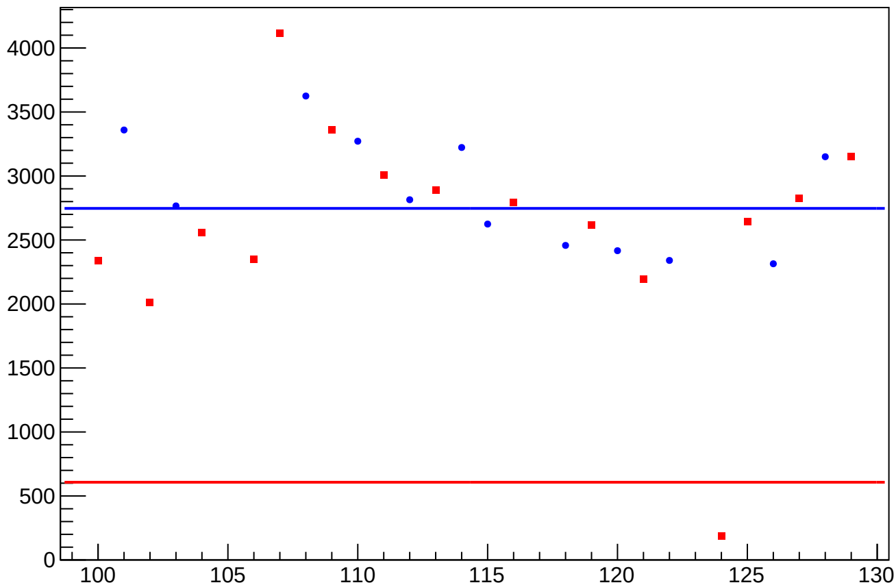
asym_atr1l2_dd_cor_correction_rms vs Slug, Sign Corrected
