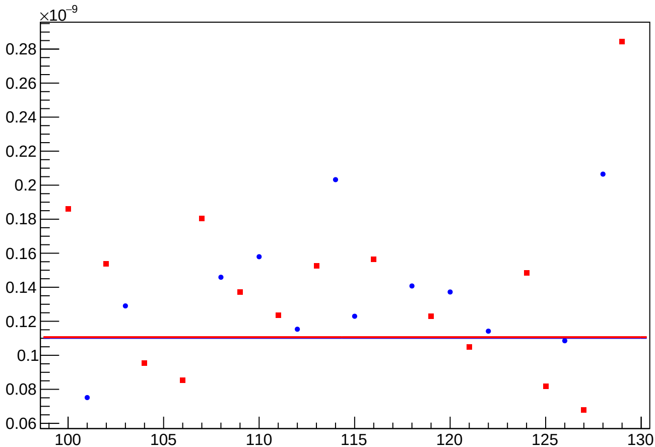
asym_sam_26_dd_reg_vs_cor_diff_rms vs Slug, Sign Corrected
