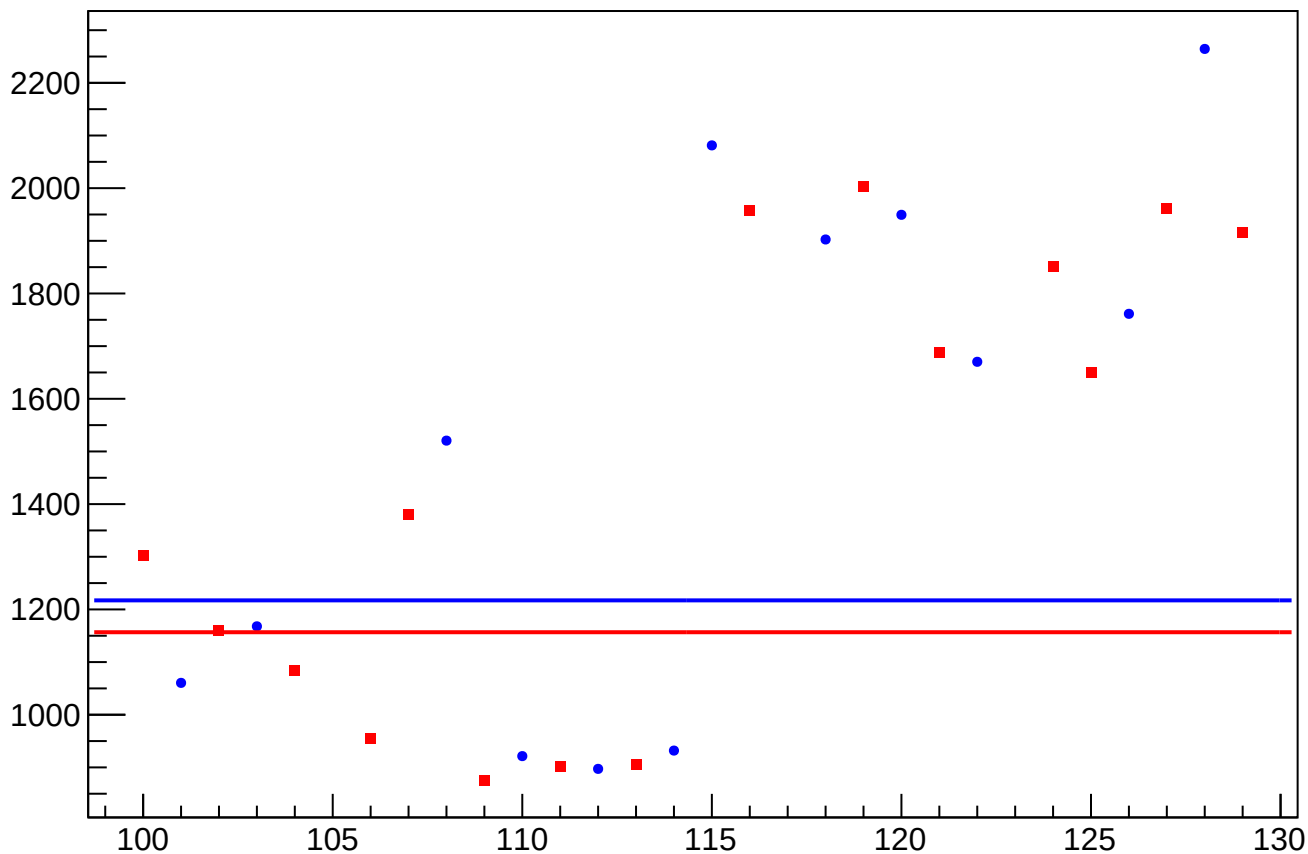
asym_sam_48_avg_eigen_cor_correction_rms vs Slug, Sign Corrected
