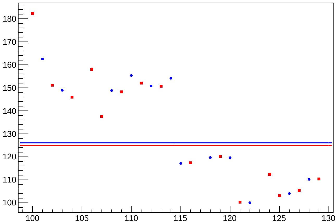
eigen_dit_asym_sam_26_48_dd_rms vs Slug, Sign Corrected
