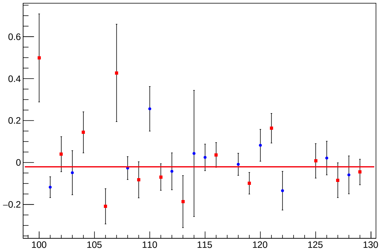
asym_usl_dit_vs_eigen_cor_diff_mean vs Slug, Sign Corrected
