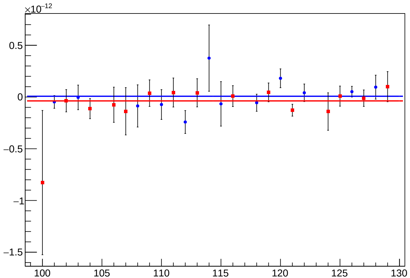
asym_sam_26_avg_eigen_cor_vs_cor_diff_mean vs Slug, Sign Corrected
