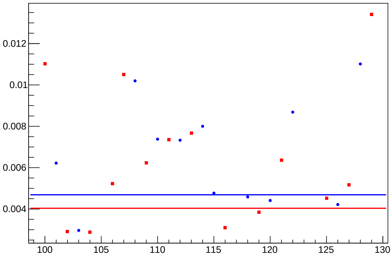
asym_us_dd_atlr_dd_avg_eigen_dit_vs_dit_diff_rms vs Slug, Sign Corrected
