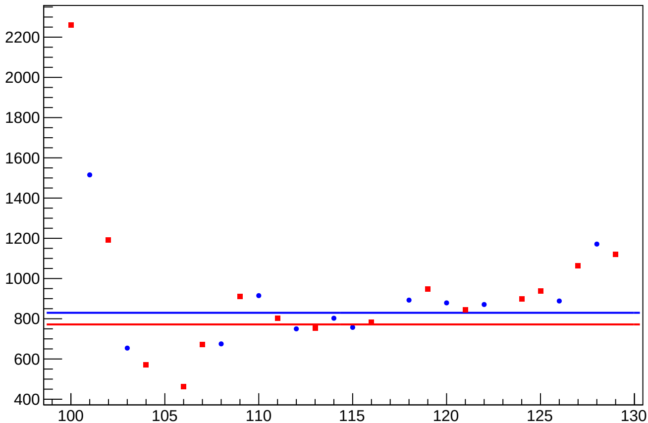
asym_usr_atr1_avg_eigen_cor_correction_rms vs Slug, Sign Corrected
