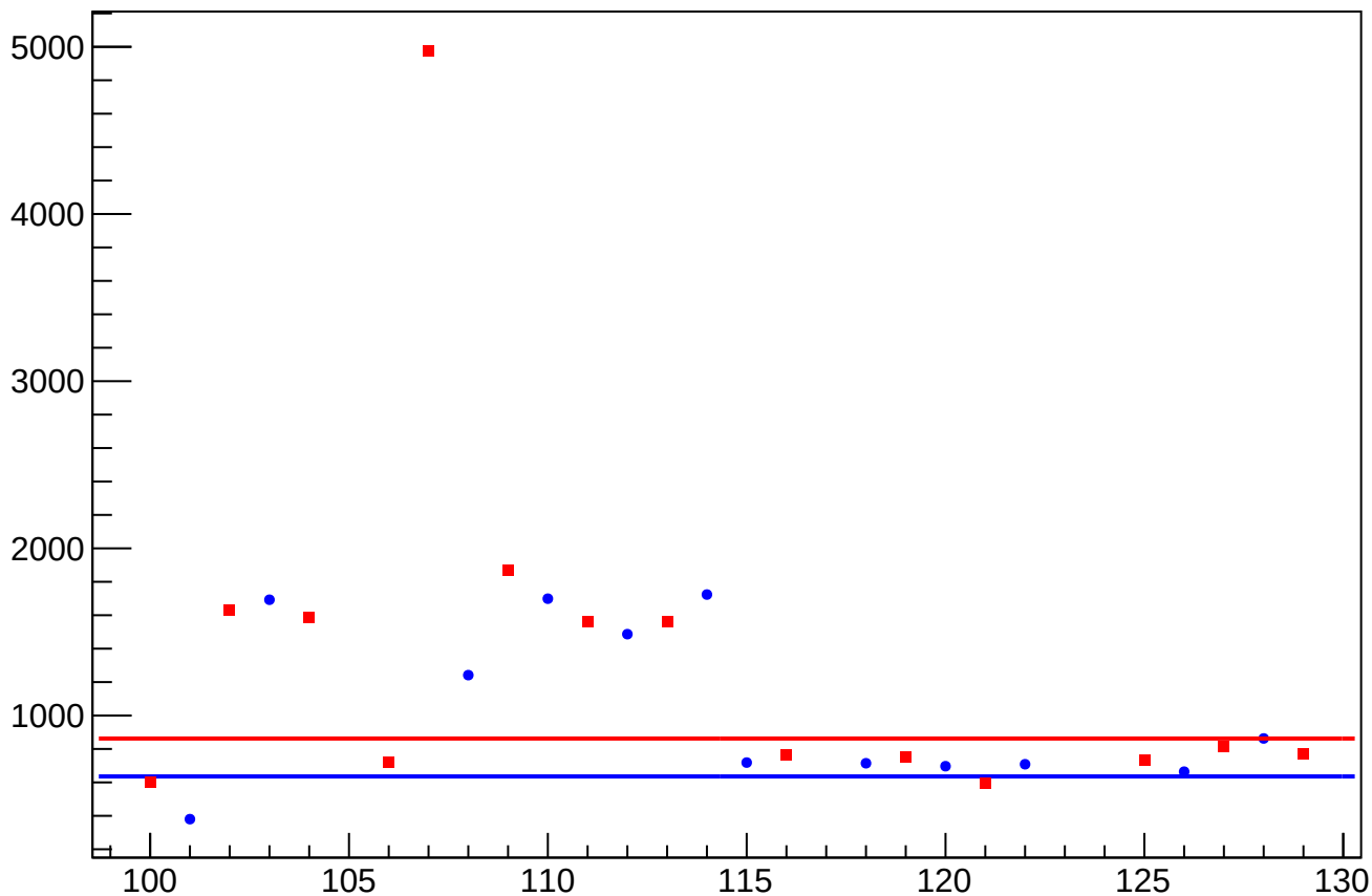
asym_usl_atl1_avg_dit_correction_rms vs Slug, Sign Corrected
