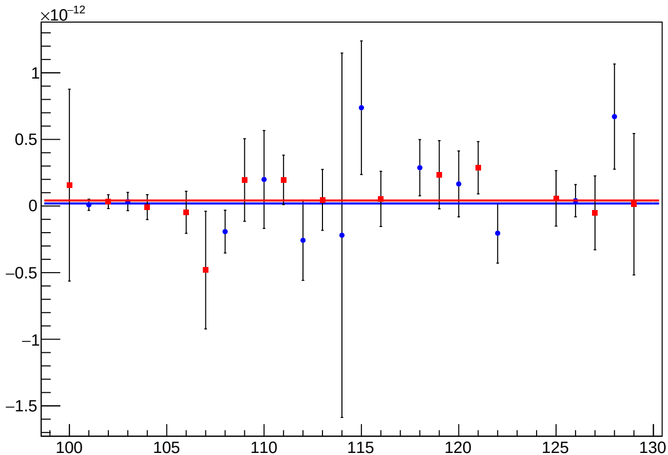
asym_us_avg_at1lr_avg_avg_reg_vs_cor_diff_mean vs Slug, Sign Corrected
