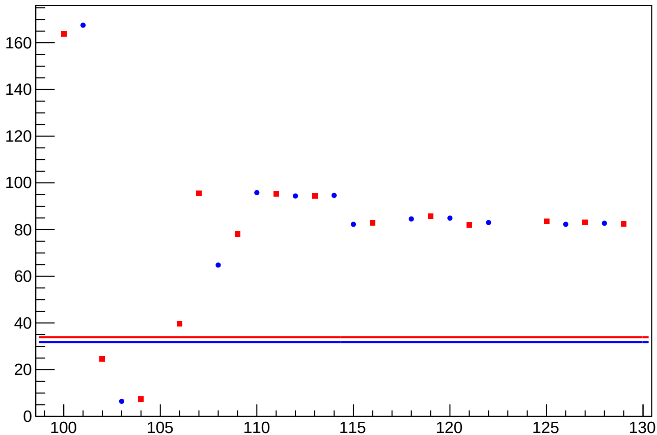
reg_asym_us_avg_atlr_avg_dd_diff_bpm12X_slope vs Slug, Sign Corrected
