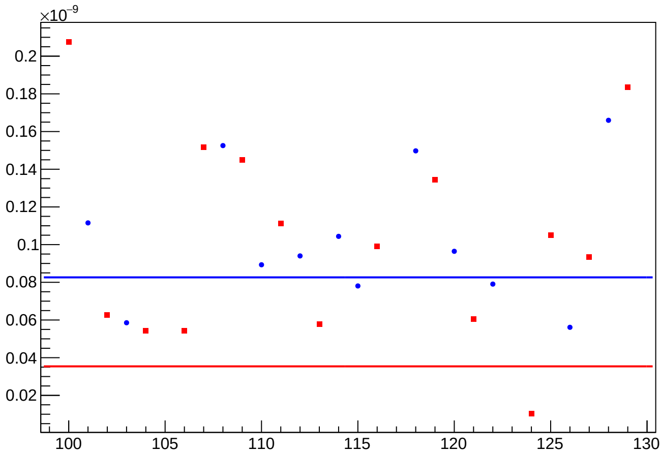
asym_atr1l2_avg_eigen_cor_vs_cor_diff_rms vs Slug, Sign Corrected
