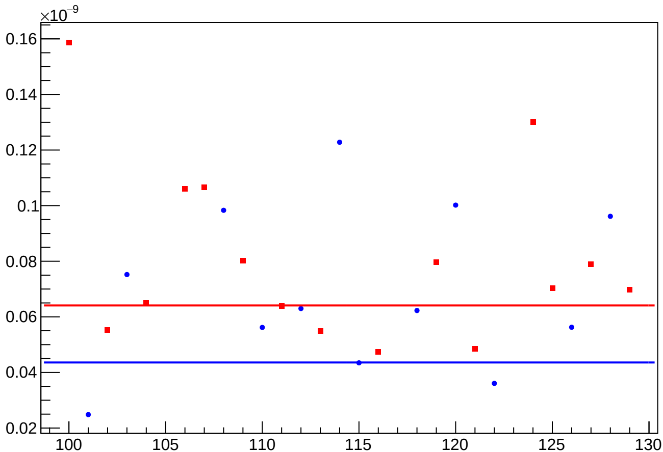
asym_sam_24_68_dd_reg_vs_cor_diff_rms vs Slug, Sign Corrected
