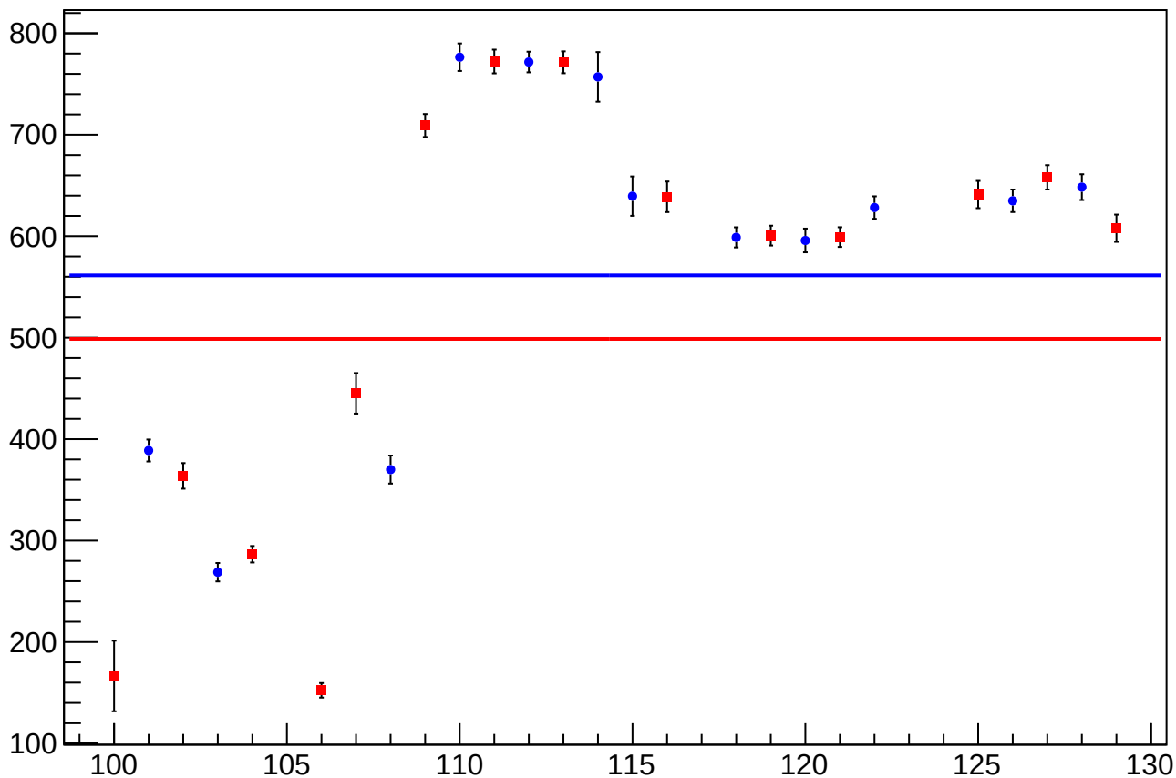
reg_asym_us_avg_at2lr_avg_avg_diff_bpm4eX_slope vs Slug, Sign Corrected
