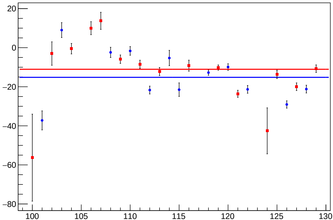
reg_asym_atl1r2_dd_atl2r1_dd_avg_diff_bpm4eY_slope vs Slug, Sign Corrected
