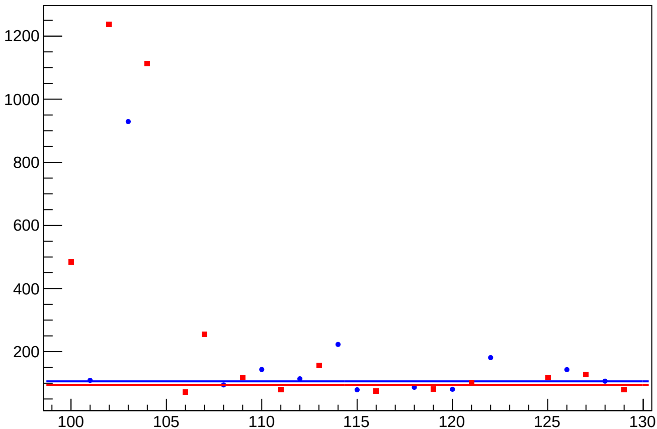
asym_us_avg_at1lr_avg_avg_dit_vs_cor_diff_rms vs Slug, Sign Corrected
