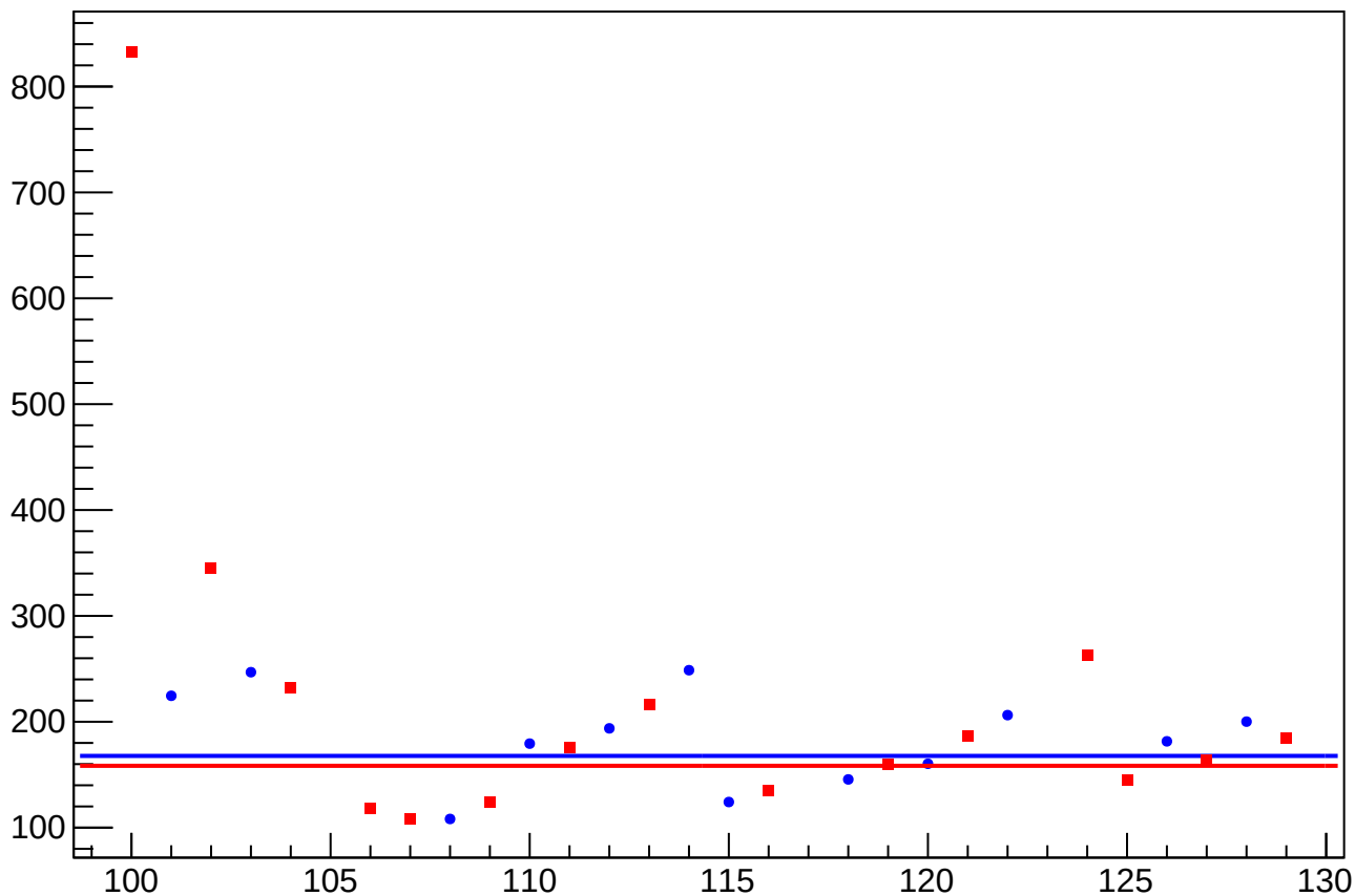
asym_atr_dd_eigen_dit_vs_cor_diff_rms vs Slug, Sign Corrected
