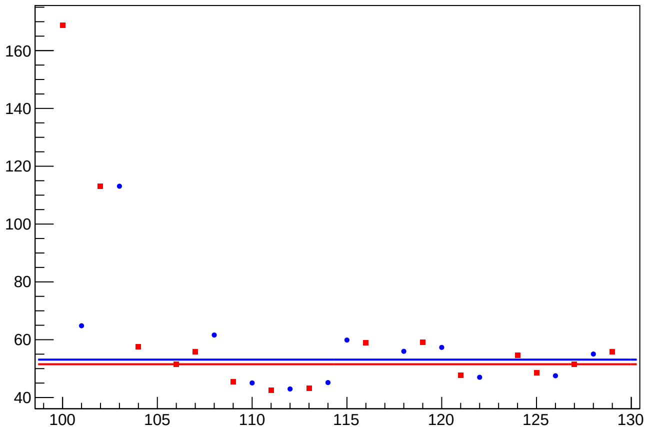
cor_asym_sam_1357_avg_rms vs Slug, Sign Corrected
