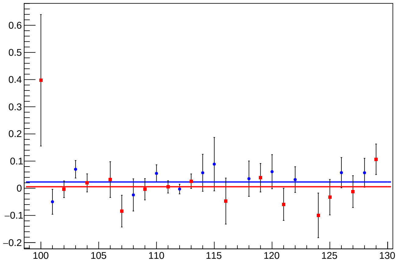
asym_sam_1548_avg_eigen_dit_vs_cor_diff_mean vs Slug, Sign Corrected
