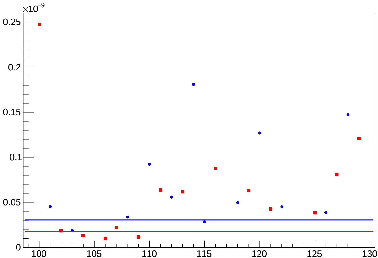
asym_us_dd_at2lr_dd_dd_reg_vs_cor_diff_rms vs Slug, Sign Corrected
