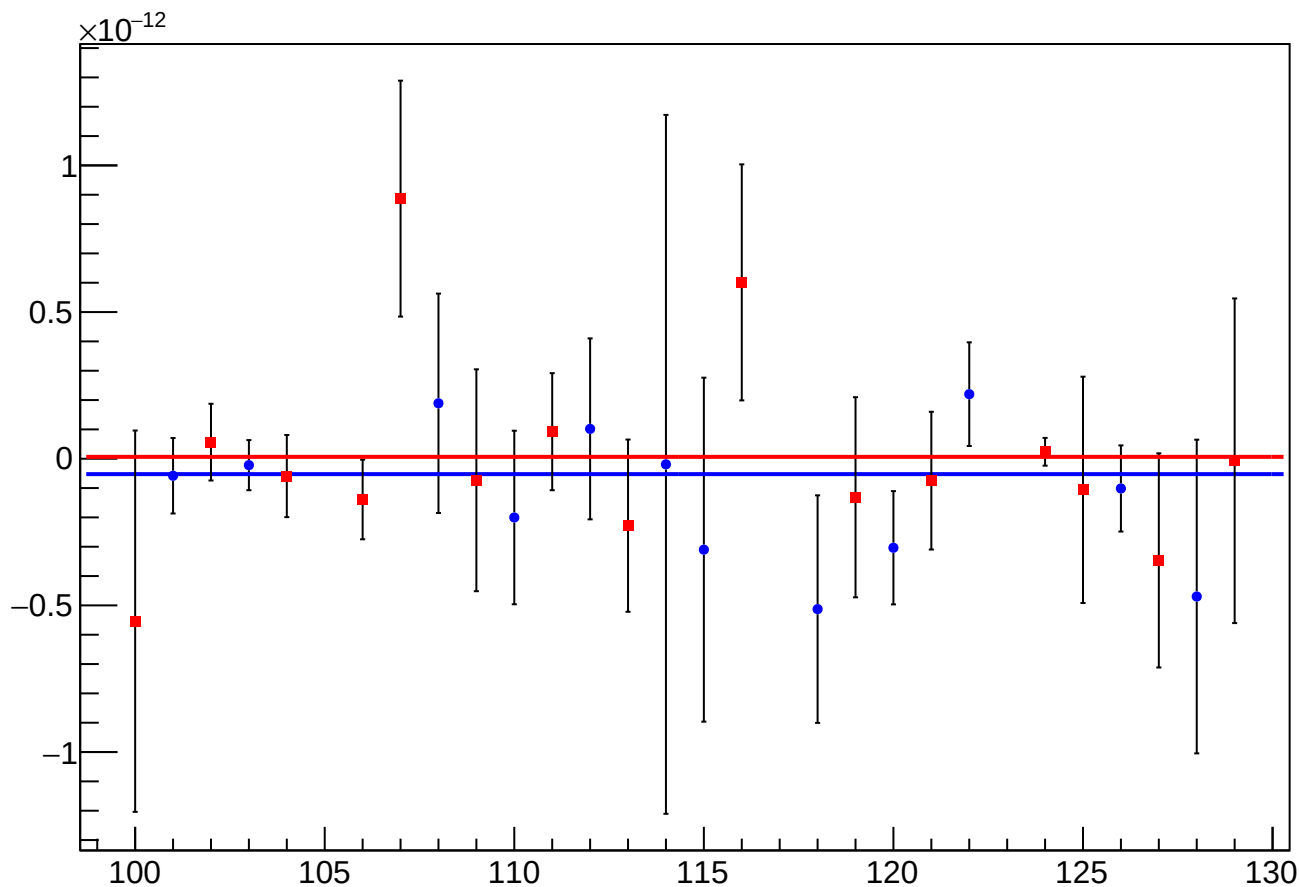
asym_atr1l2_dd_reg_vs_cor_diff_mean vs Slug, Sign Corrected
