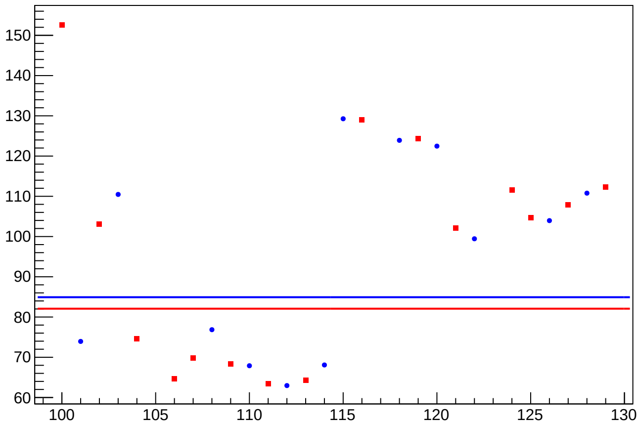
eigen_dit_asym_sam_1548_avg_rms vs Slug, Sign Corrected
