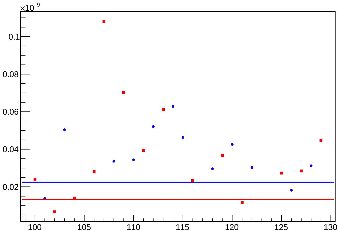
asym_usl_atl1_avg_eigen_cor_vs_cor_diff_rms vs Slug, Sign Corrected
