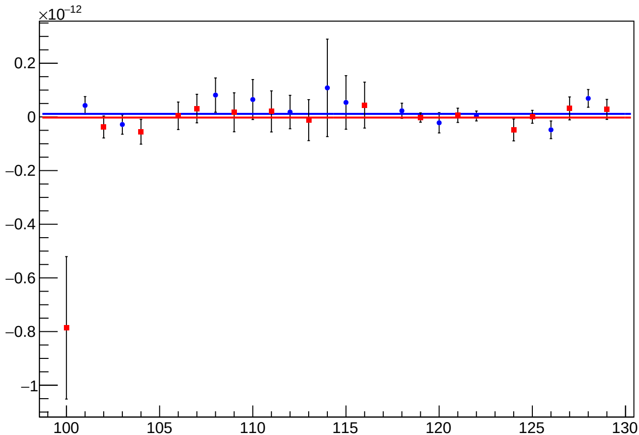
asym_sam_26_48_dd_eigen_cor_vs_cor_diff_mean vs Slug, Sign Corrected
