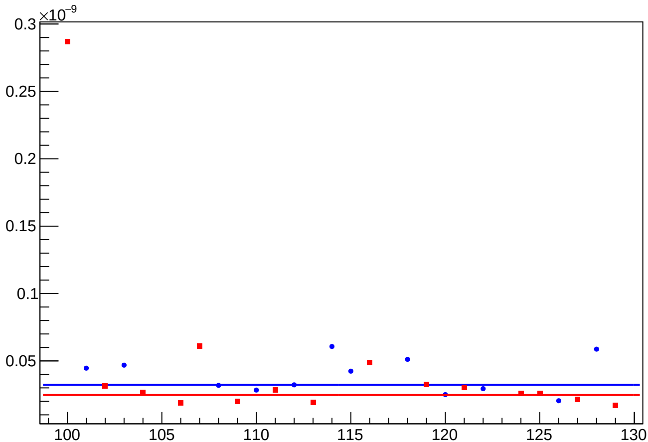
asym_atr1_reg_vs_cor_diff_rms vs Slug, Sign Corrected
