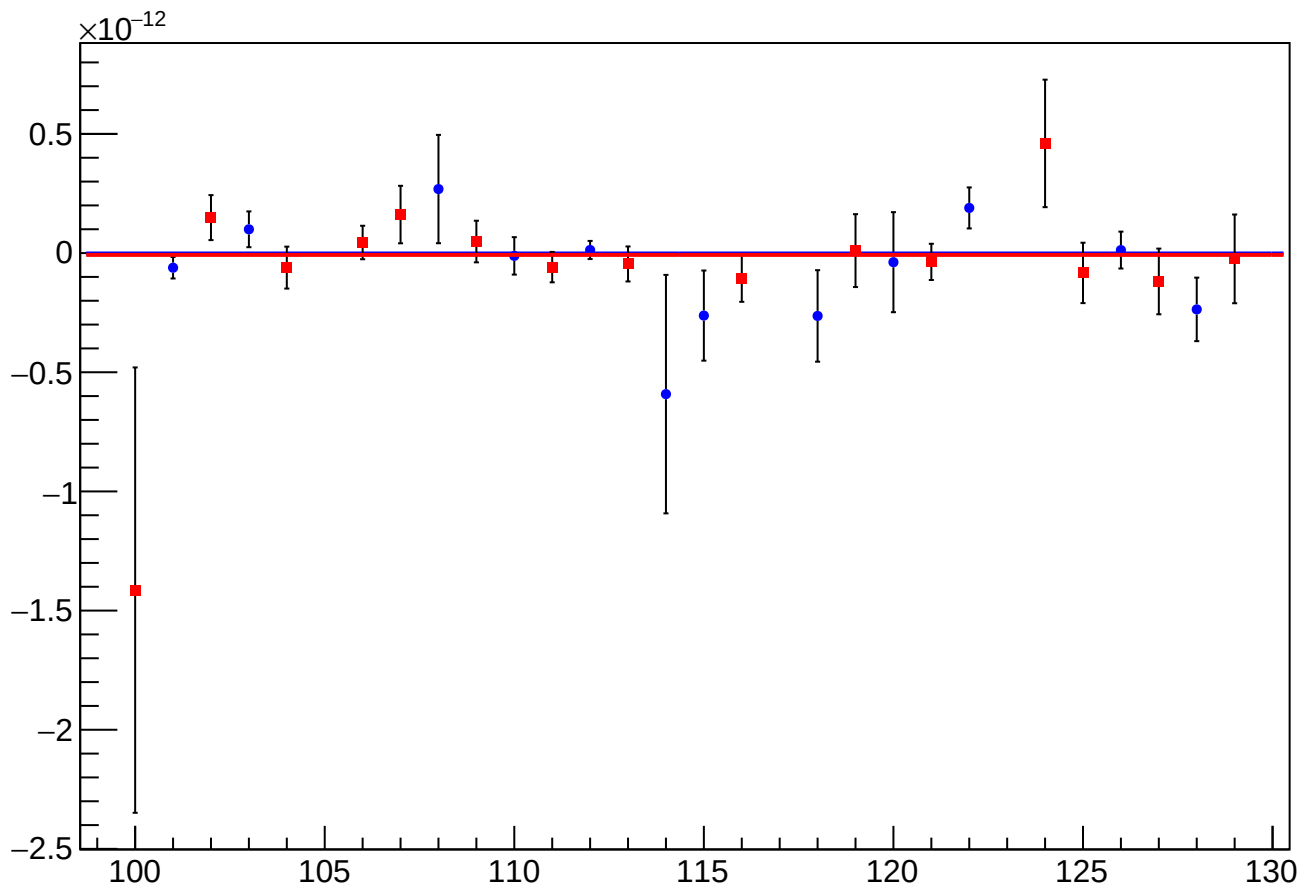
asym_sam_37_avg_reg_vs_cor_diff_mean vs Slug, Sign Corrected
