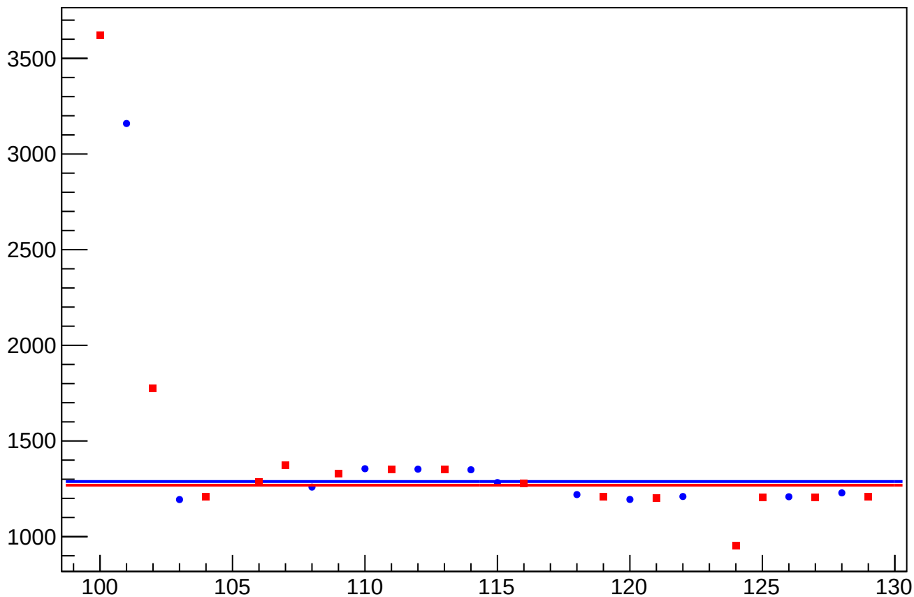
dit_asym_at1_dd_at2_dd_avg_rms vs Slug, Sign Corrected
