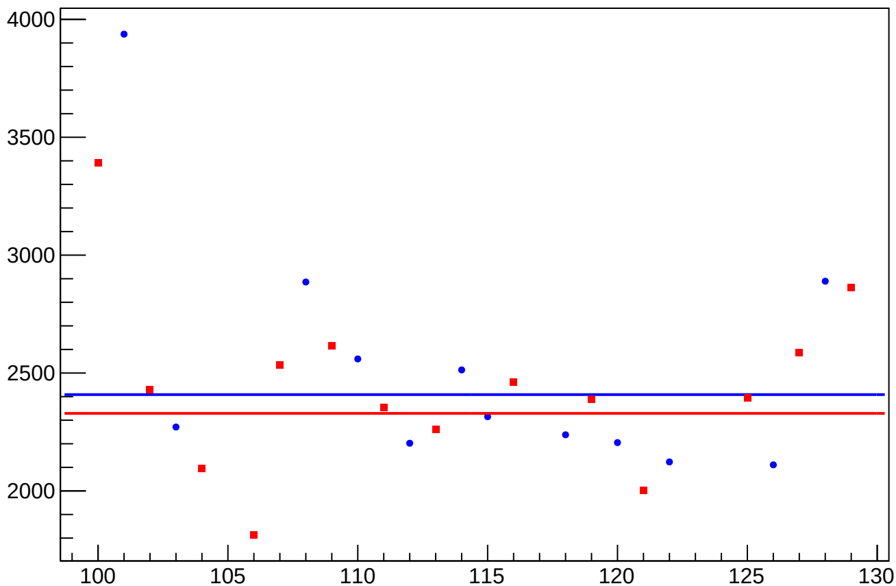
asym_usl_atl2_dd_eigen_cor_correction_rms vs Slug, Sign Corrected
