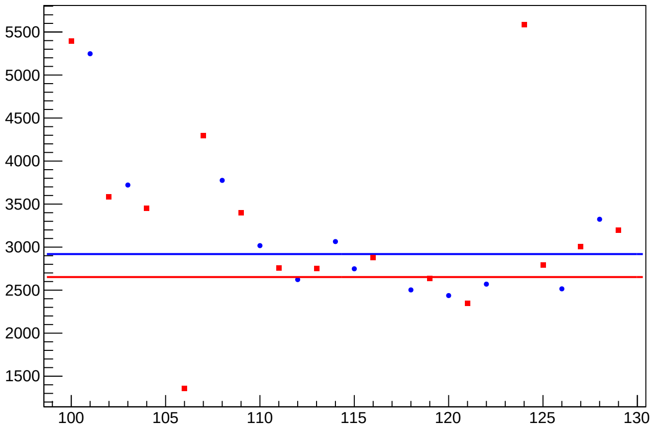
asym_atr1l2_avg_eigen_dit_correction_rms vs Slug, Sign Corrected
