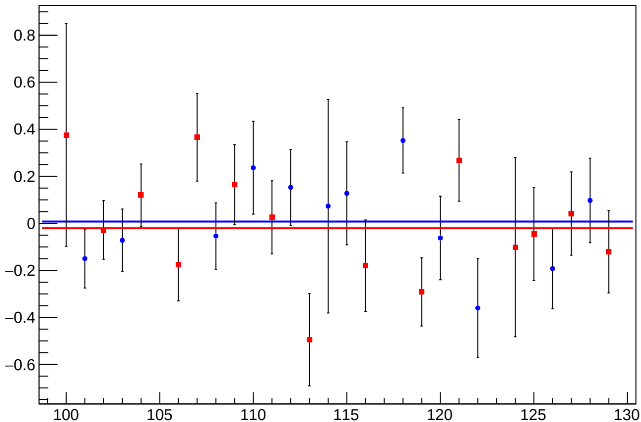
asym_usr_dit_vs_overload_cor_diff_mean vs Slug, Sign Corrected
