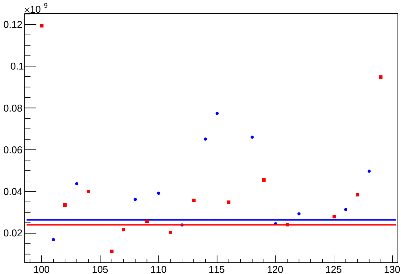
asym_us_avg_at1lr_avg_dd_reg_vs_cor_diff_rms vs Slug, Sign Corrected
