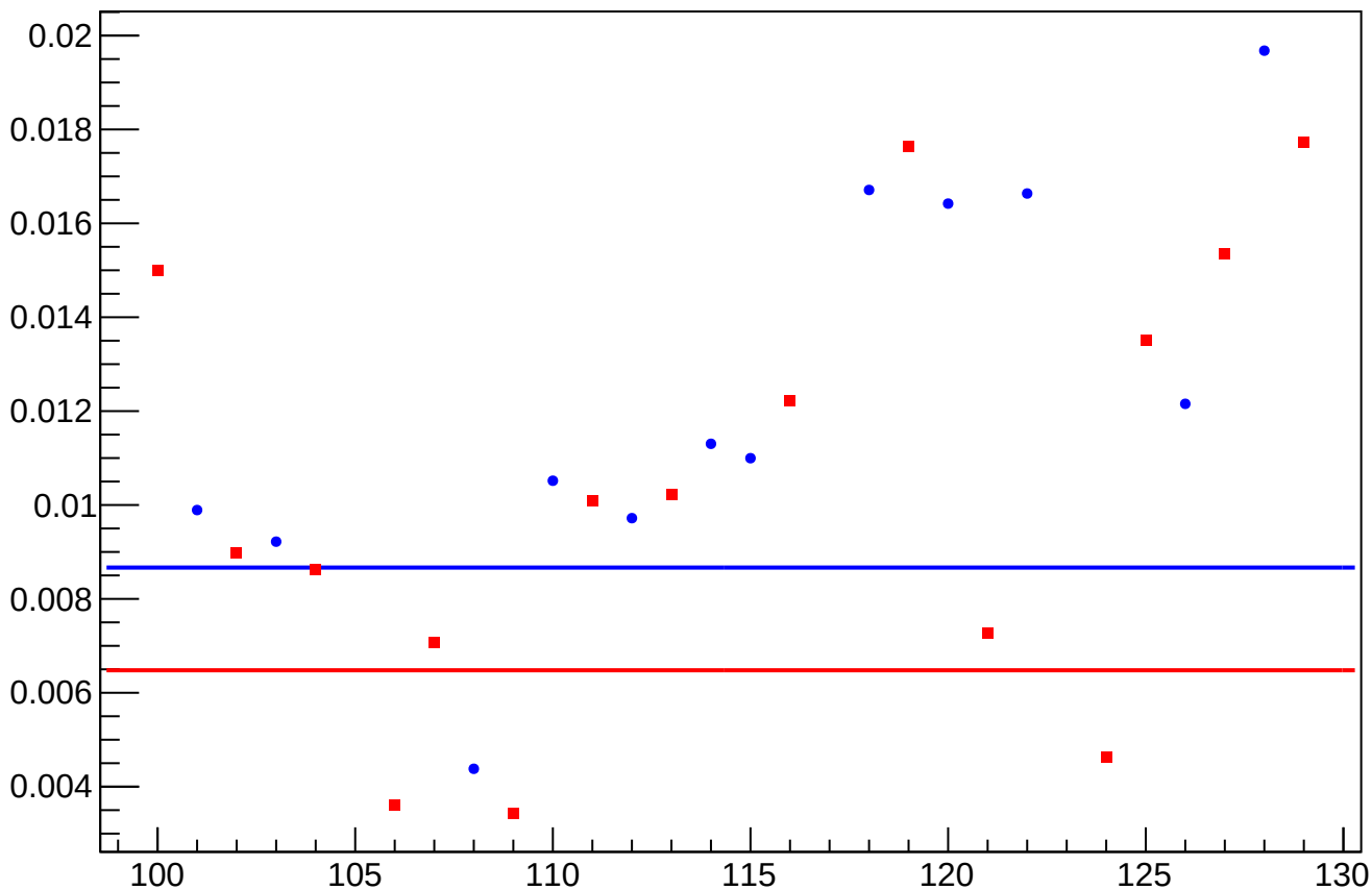
asym_atl_dd_atr_dd_avg_eigen_dit_vs_dit_diff_rms vs Slug, Sign Corrected
