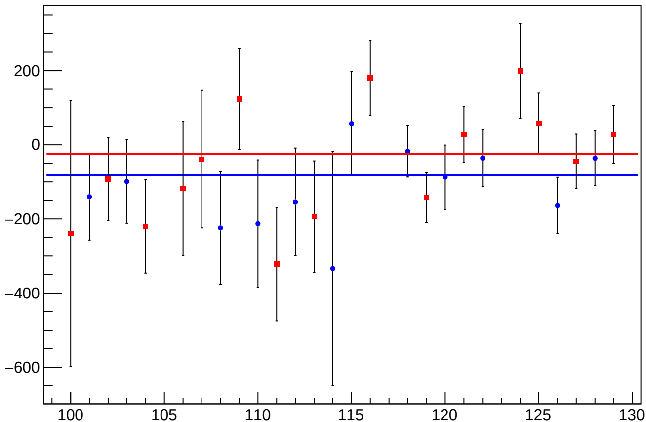
eigen_cor_asym_sam_37_26_dd_mean vs Slug, Sign Corrected
