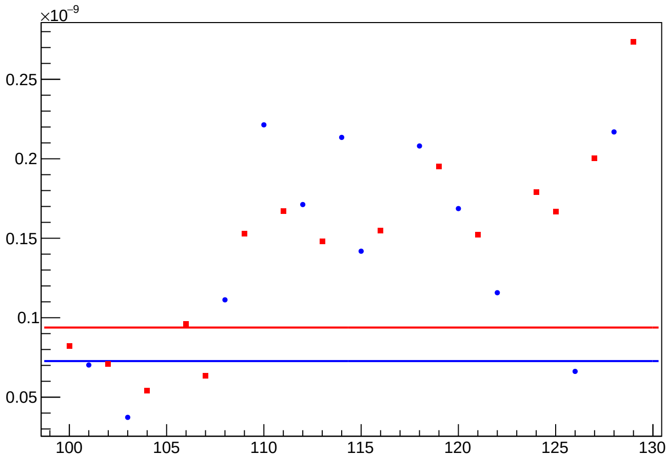
asym_atr_dd_eigen_cor_vs_cor_diff_rms vs Slug, Sign Corrected
