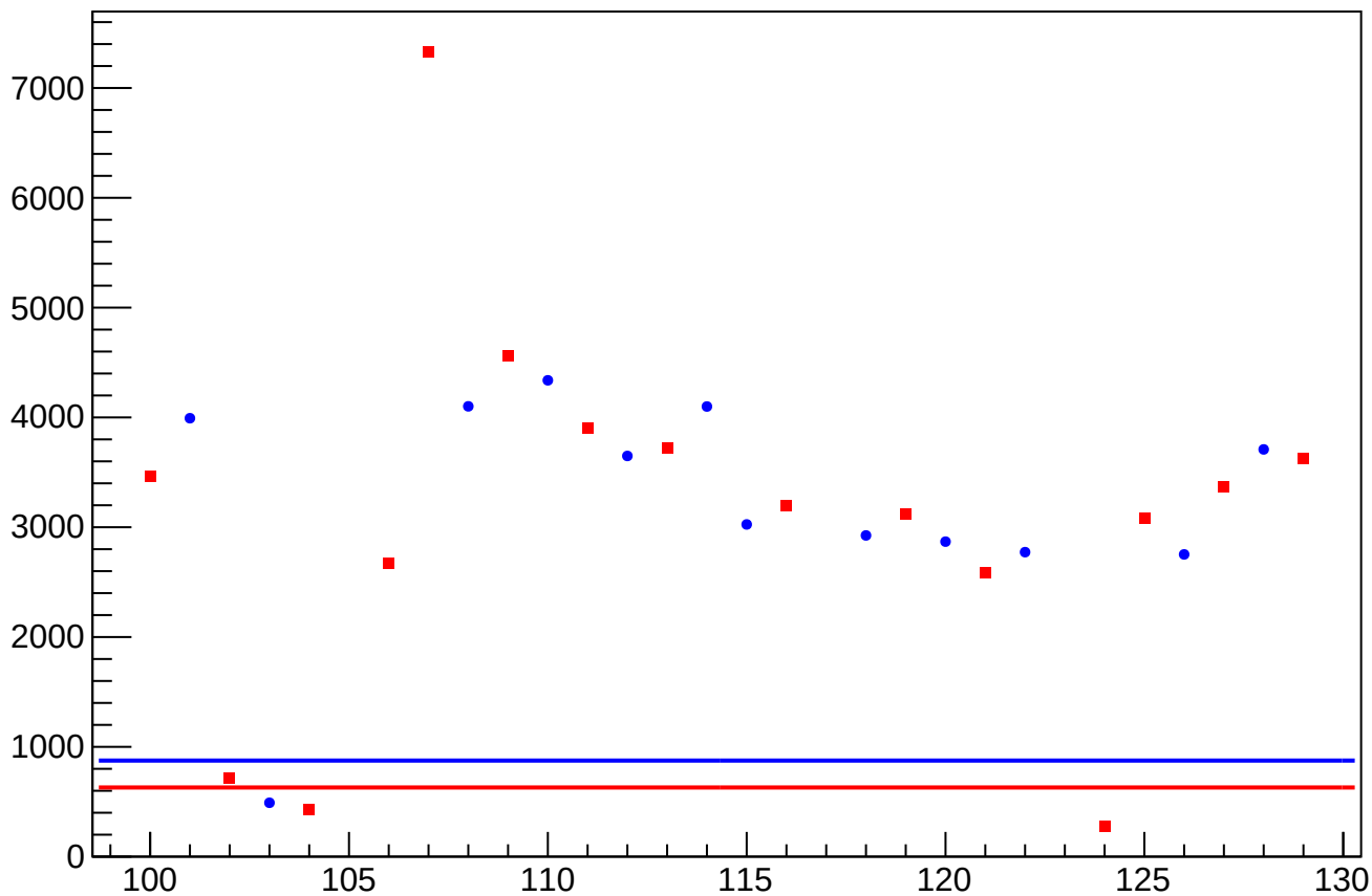
asym_atl_avg_cor_correction_rms vs Slug, Sign Corrected
