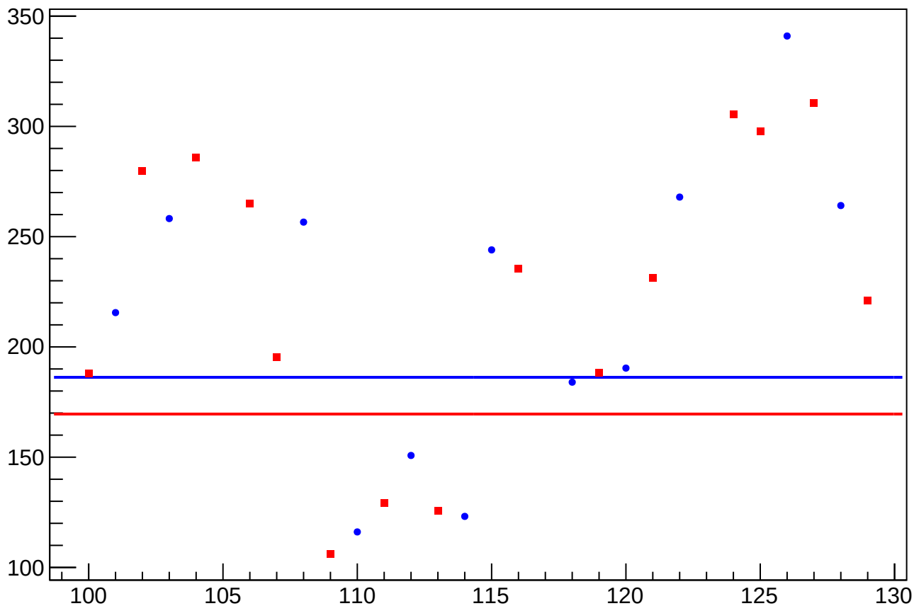
asym_bcm_an_us_an_ds3_avg_rms vs Slug, Sign Corrected
