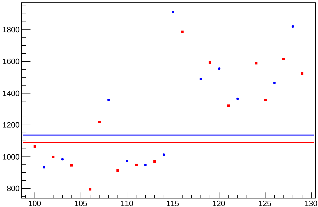
asym_sam_48_dd_cor_correction_rms vs Slug, Sign Corrected
