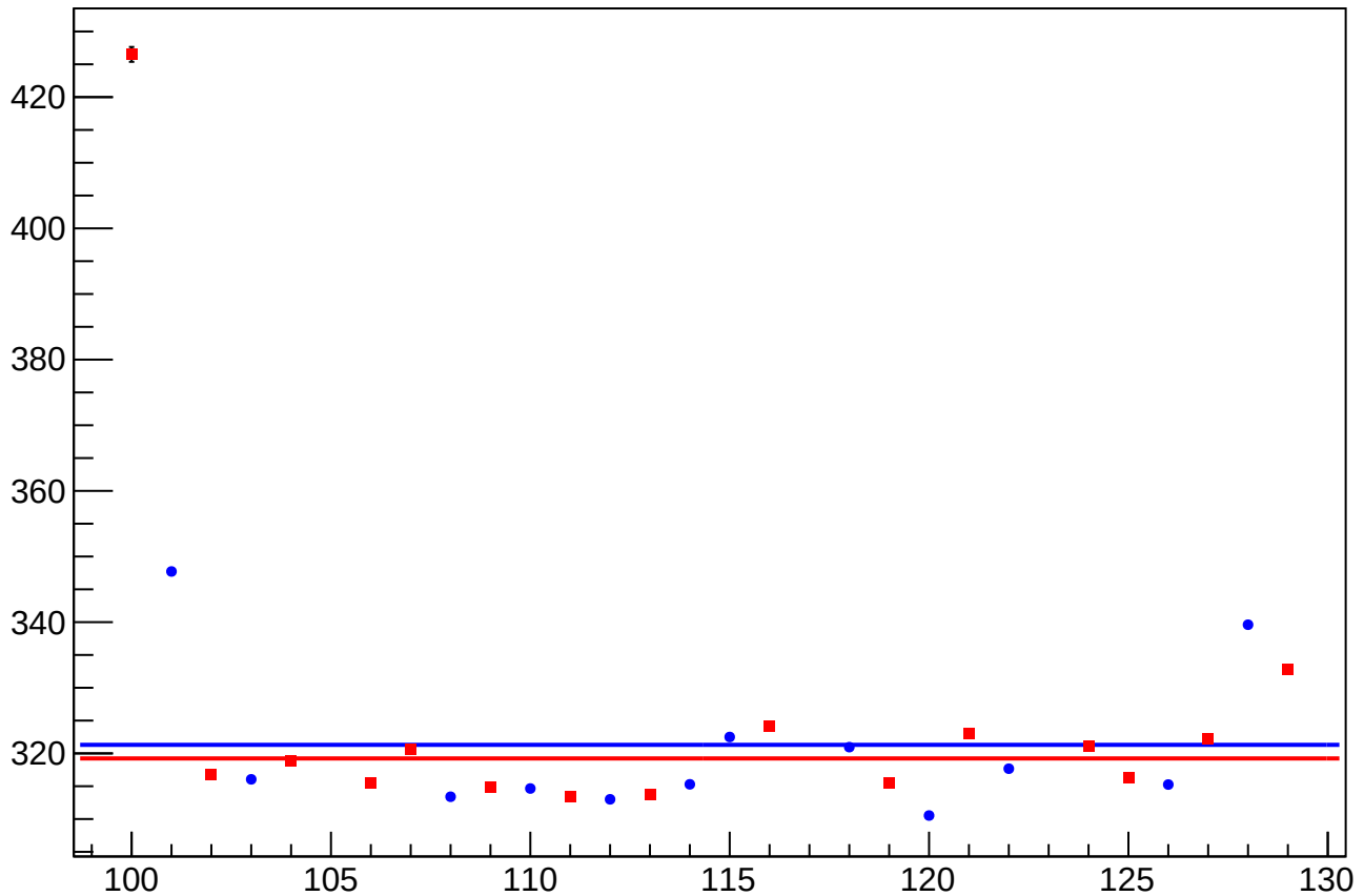
diff_bpm_4eX_4ecX_dd_rms vs Slug, Sign Corrected
