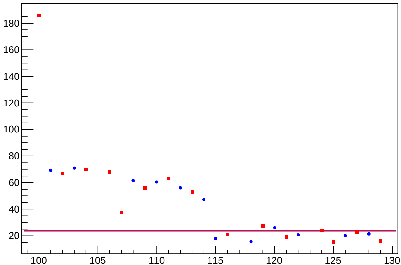
asym_sam_37_26_dd_eigen_dit_vs_eigen_cor_diff_rms vs Slug, Sign Corrected
