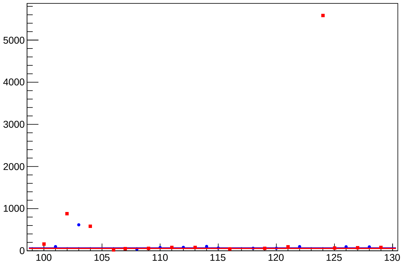
asym_at2_dd_eigen_dit_vs_cor_diff_rms vs Slug, Sign Corrected
