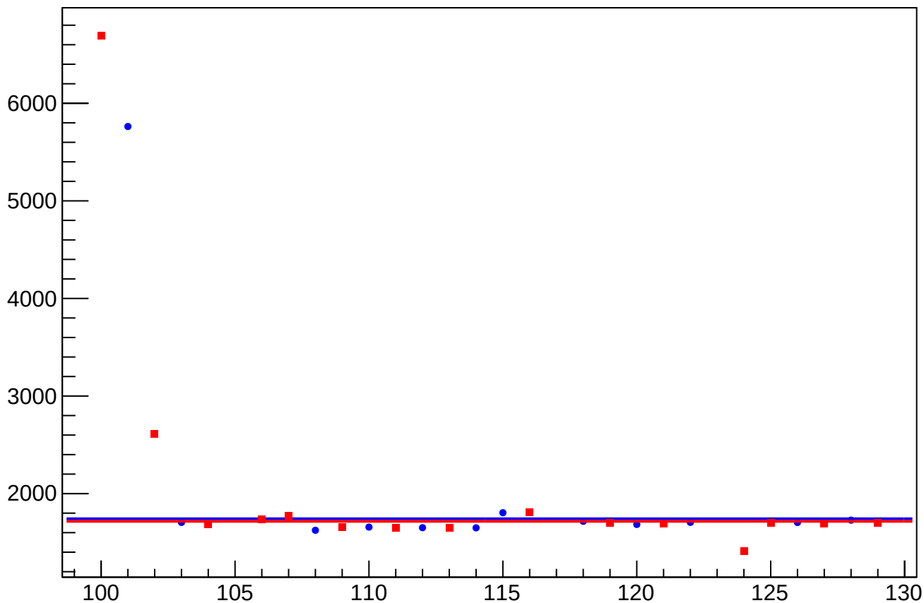
eigen_dit_asym_atr1l2_dd_rms vs Slug, Sign Corrected
