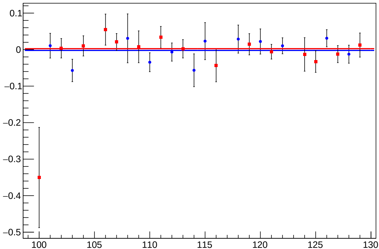
asym_sam_15_avg_eigen_dit_vs_eigen_cor_diff_mean vs Slug, Sign Corrected
