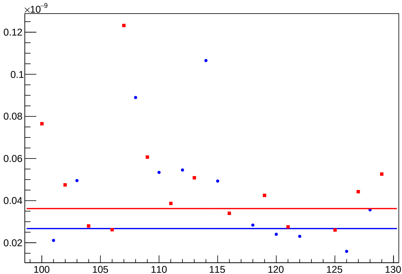
asym_usl_reg_vs_cor_diff_rms vs Slug, Sign Corrected
