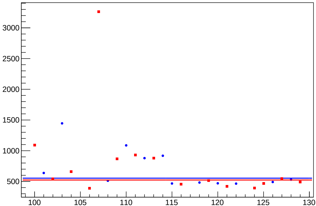
asym_at1_avg_cor_correction_rms vs Slug, Sign Corrected
