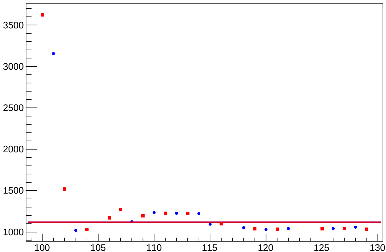
eigen_cor_asym_us_dd_atlr_dd_dd_rms vs Slug, Sign Corrected
