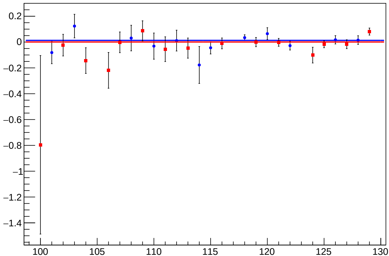
asym_sam_37_26_dd_eigen_dit_vs_cor_diff_mean vs Slug, Sign Corrected
