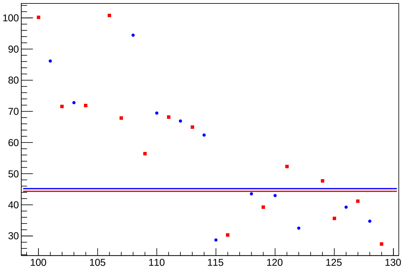
asym_sam_3726_avg_eigen_dit_vs_cor_diff_rms vs Slug, Sign Corrected
