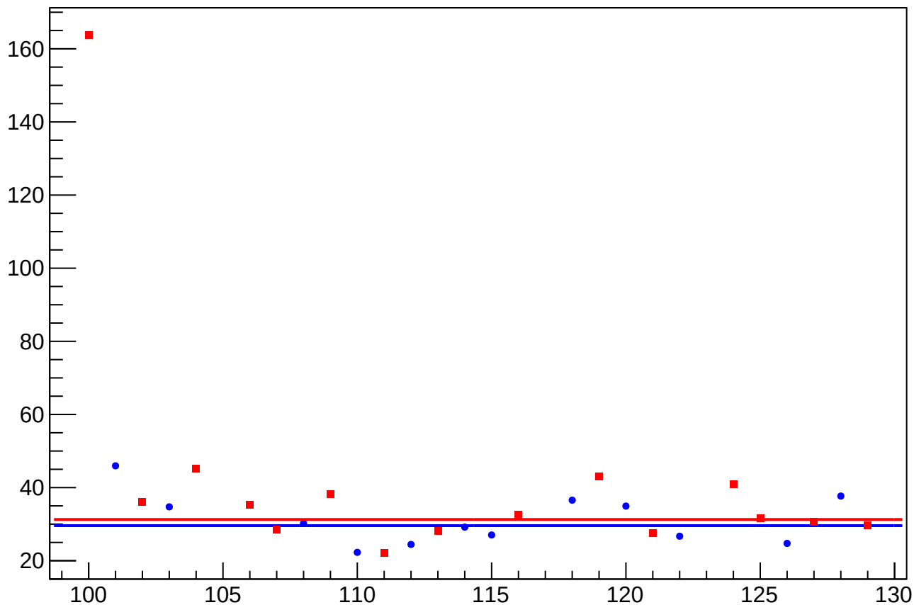
asym_sam_37_48_dd_dit_vs_cor_diff_rms vs Slug, Sign Corrected
