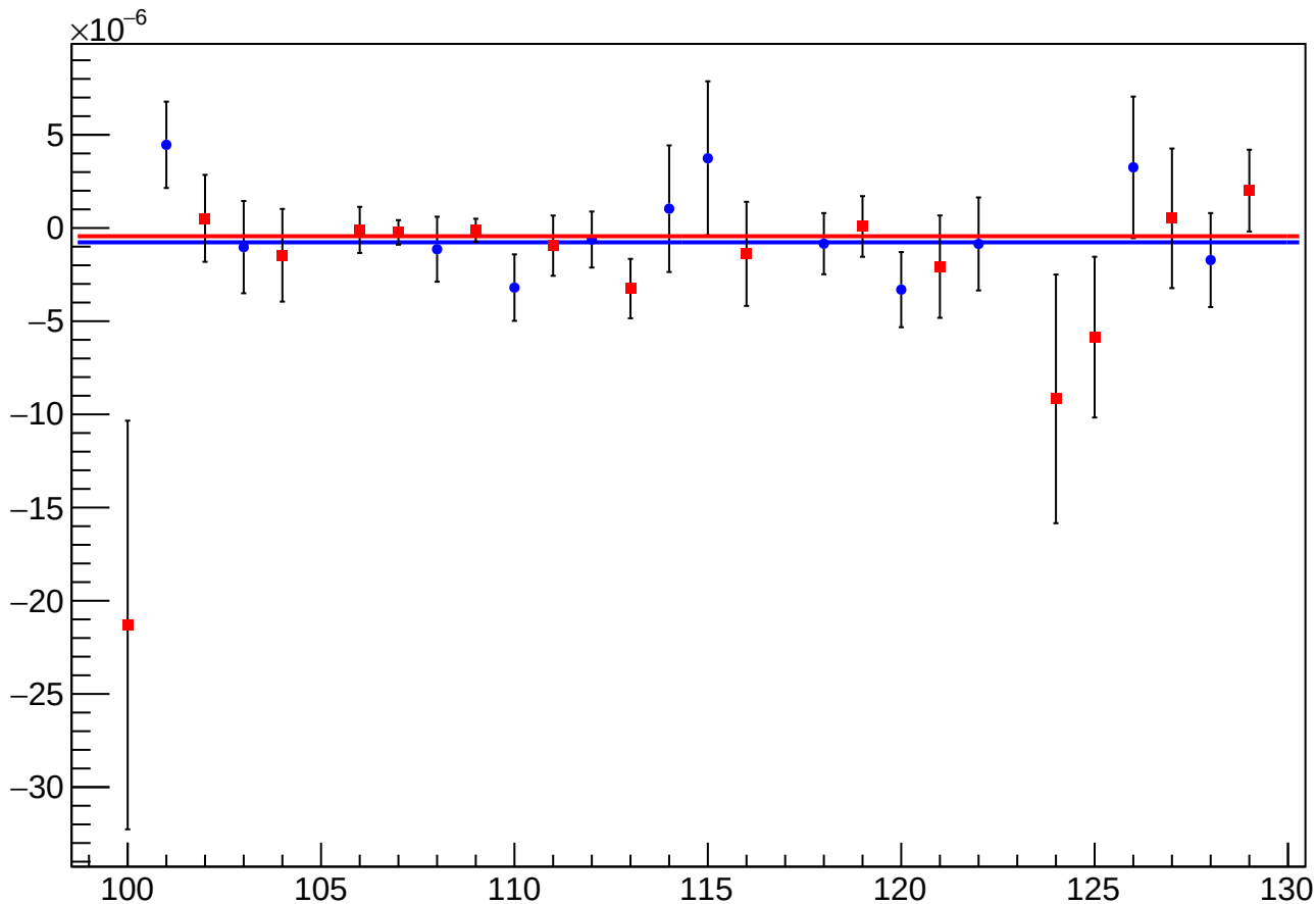
asym_sam_1357_avg_eigen_dit_vs_dit_diff_mean vs Slug, Sign Corrected
