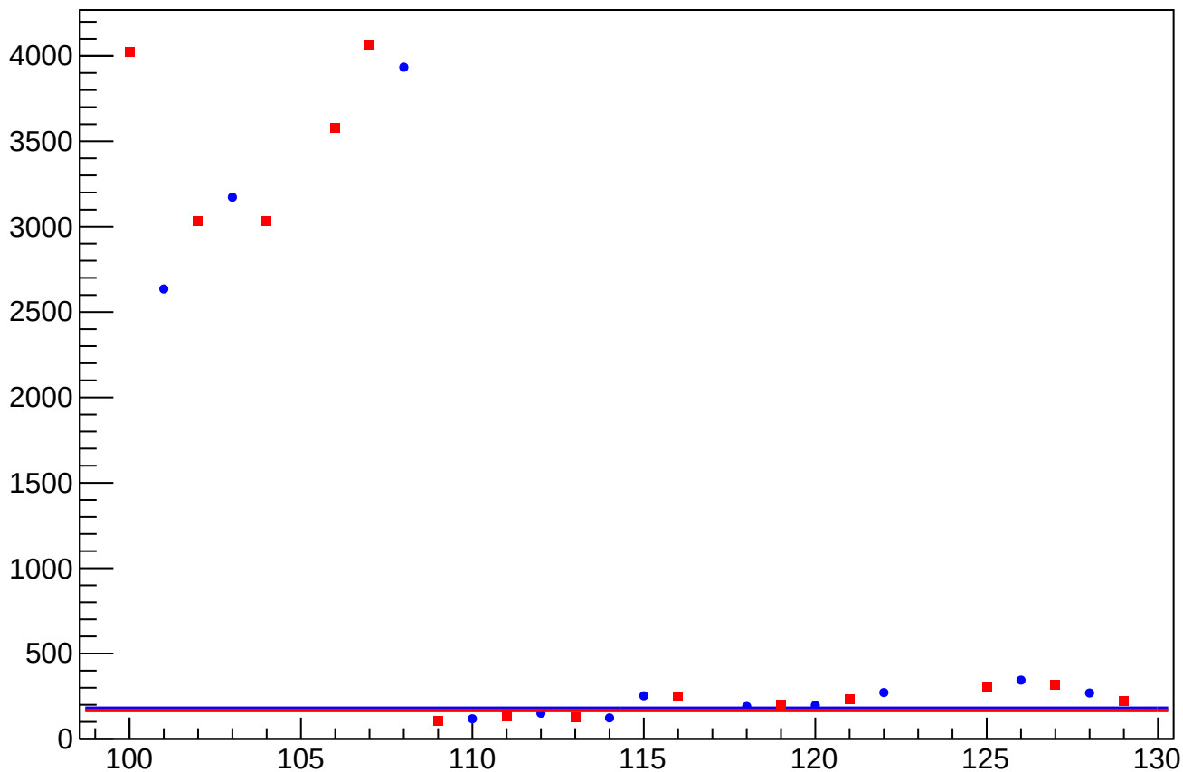
asym_bcm_cav4cQ_dg_ds_avg_rms vs Slug, Sign Corrected
