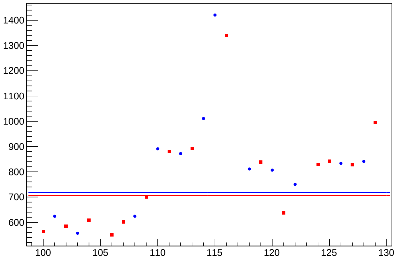
asym_sam_15_dd_reg_correction_rms vs Slug, Sign Corrected
