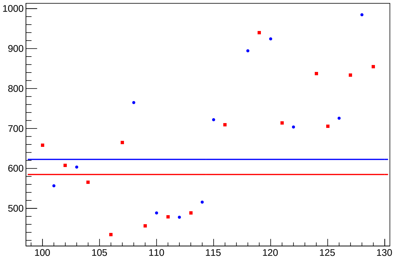
asym_sam_15_48_dd_eigen_cor_correction_rms vs Slug, Sign Corrected
