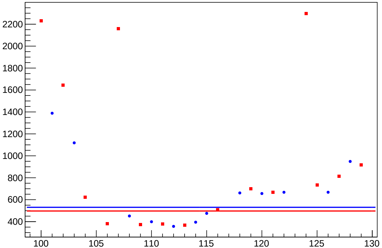
asym_atl1r2_dd_atl2r1_dd_avg_eigen_cor_correction_rms vs Slug, Sign Corrected
