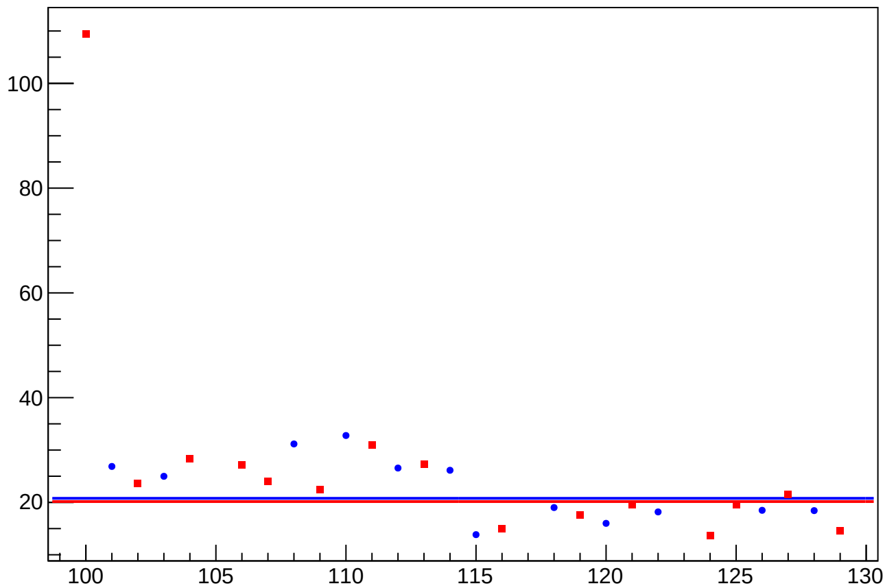
asym_sam_1357_2468_dd_dit_vs_eigen_cor_diff_rms vs Slug, Sign Corrected
