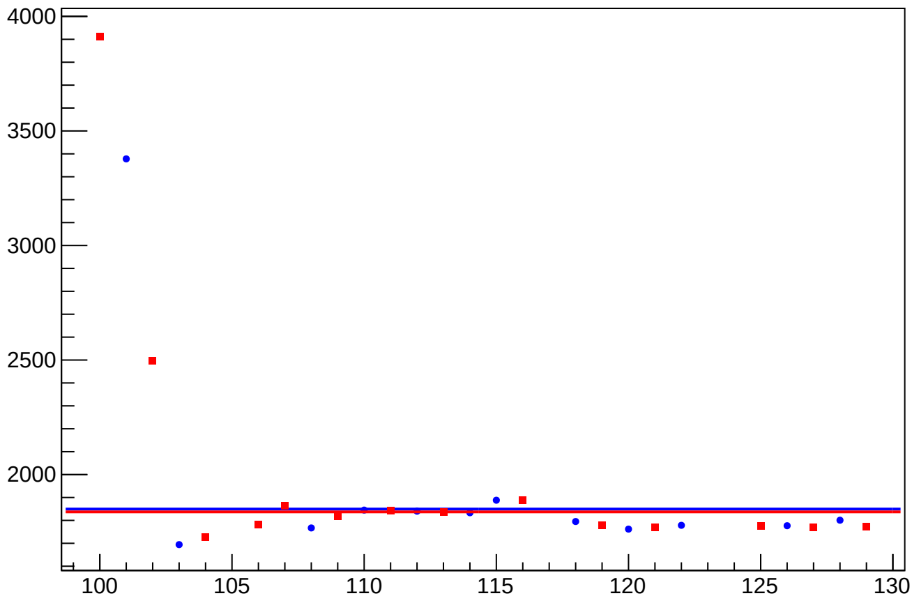
dit_asym_us_dd_atlr_dd_avg_rms vs Slug, Sign Corrected
