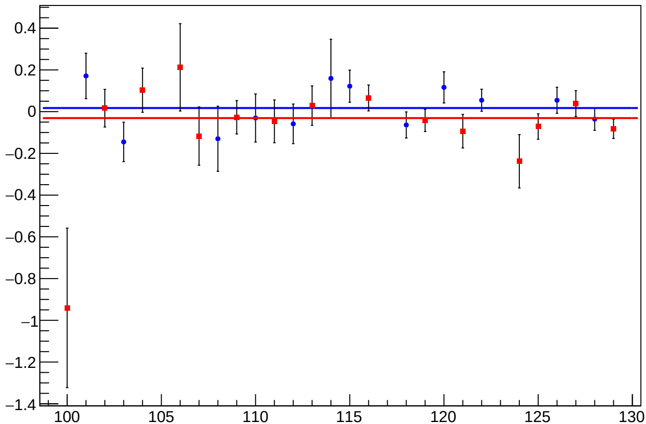
asym_sam_3726_avg_dit_vs_cor_diff_mean vs Slug, Sign Corrected
