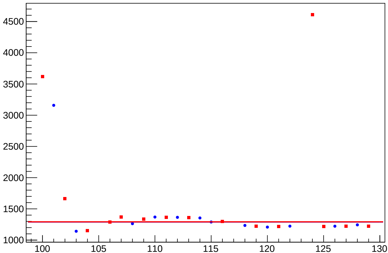
cor_asym_at1_avg_at2_avg_dd_rms vs Slug, Sign Corrected
