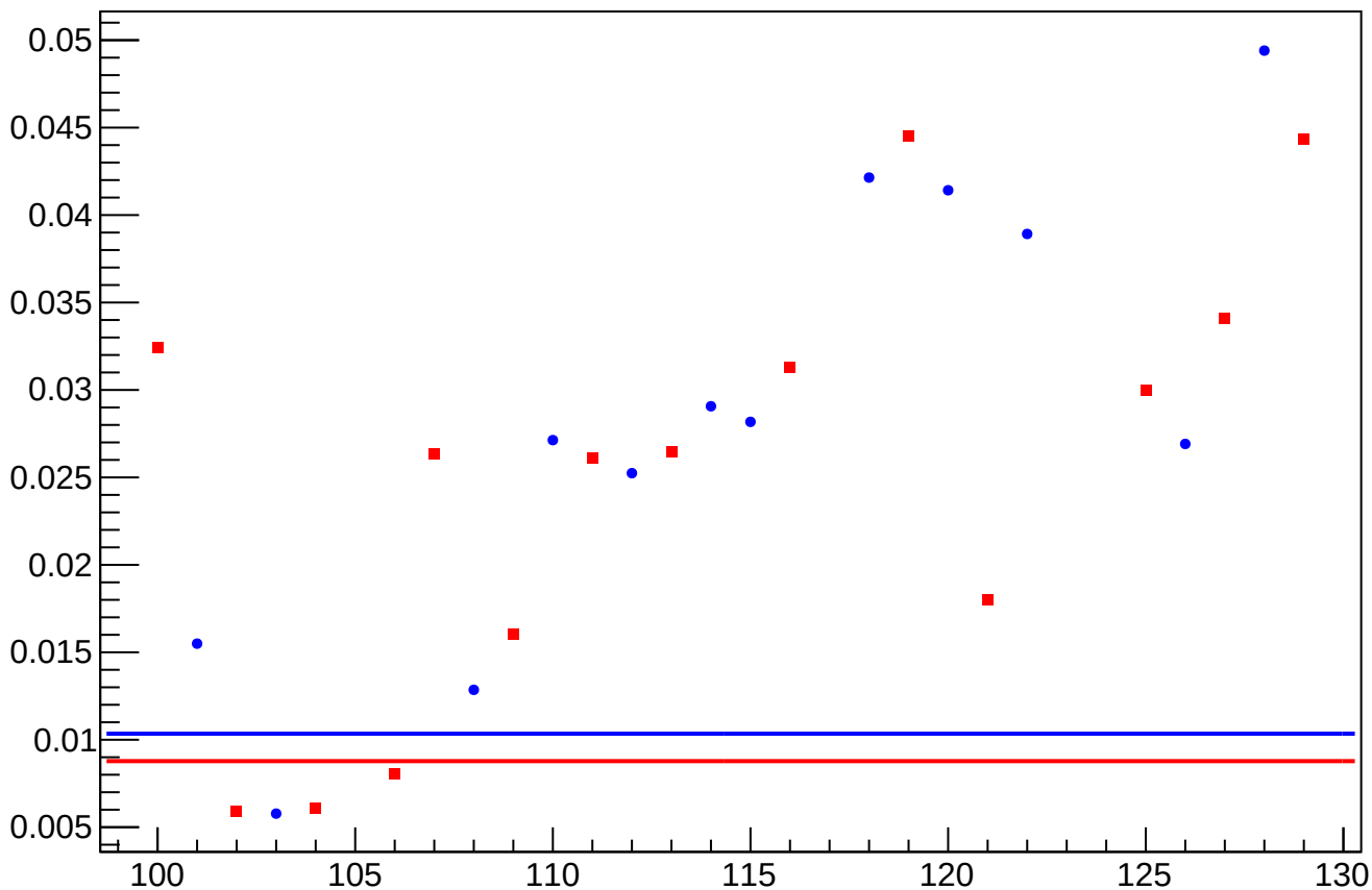
asym_us_avg_at2lr_avg_avg_eigen_dit_vs_dit_diff_rms vs Slug, Sign Corrected
