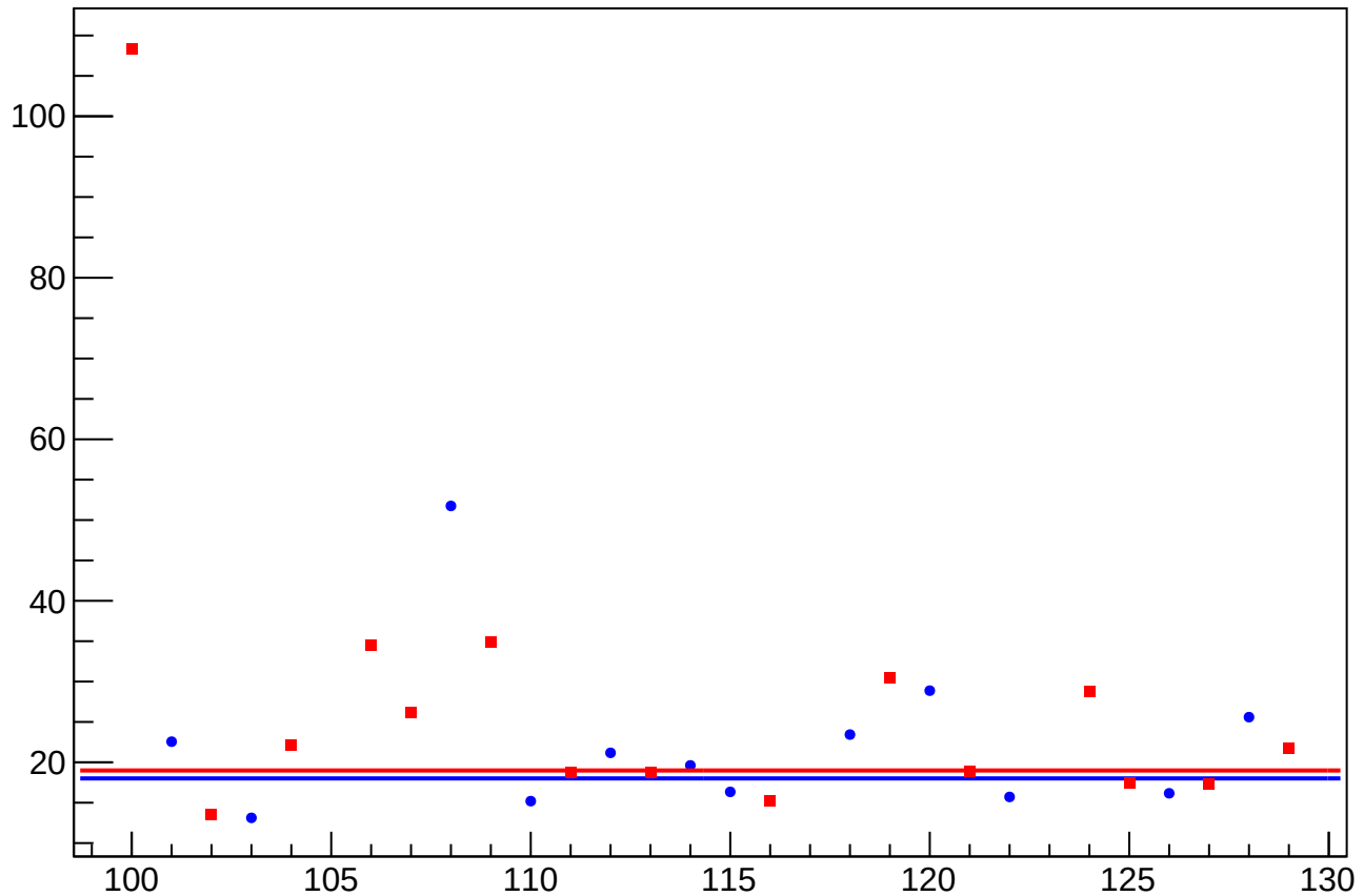
asym_sam_15_37_dd_eigen_dit_vs_cor_diff_rms vs Slug, Sign Corrected
