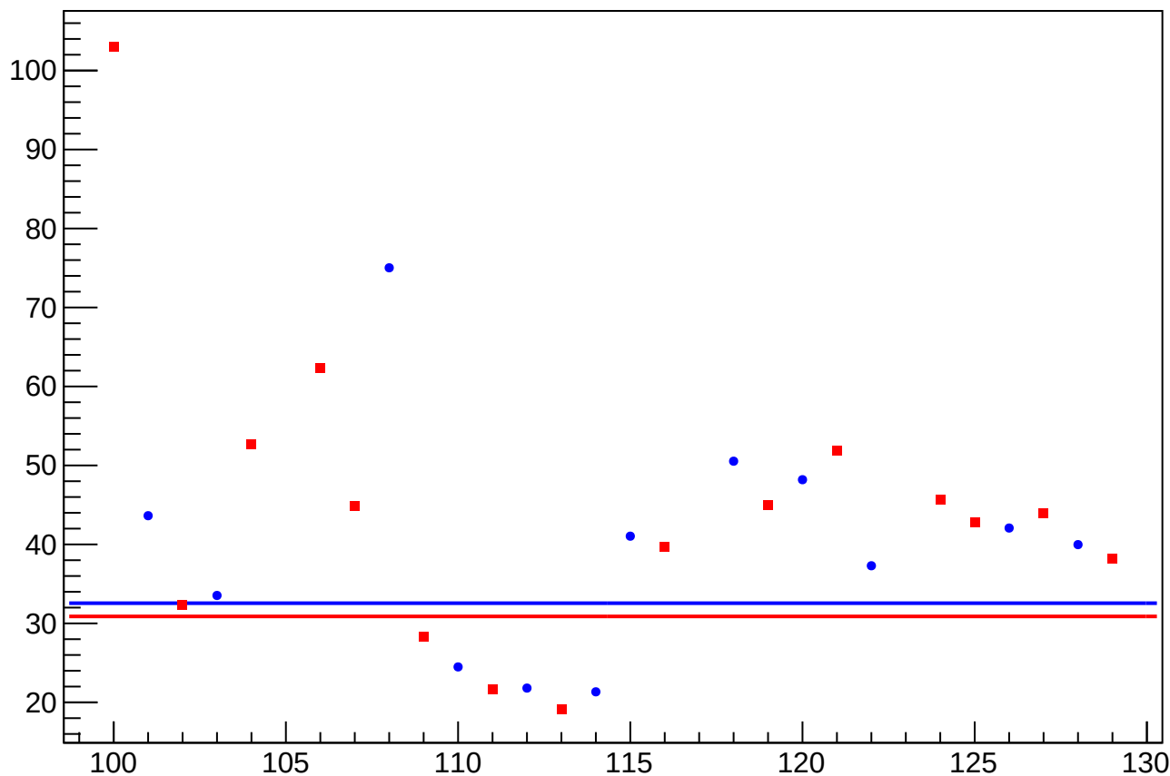
asym_sam_3748_avg_dit_vs_cor_diff_rms vs Slug, Sign Corrected
