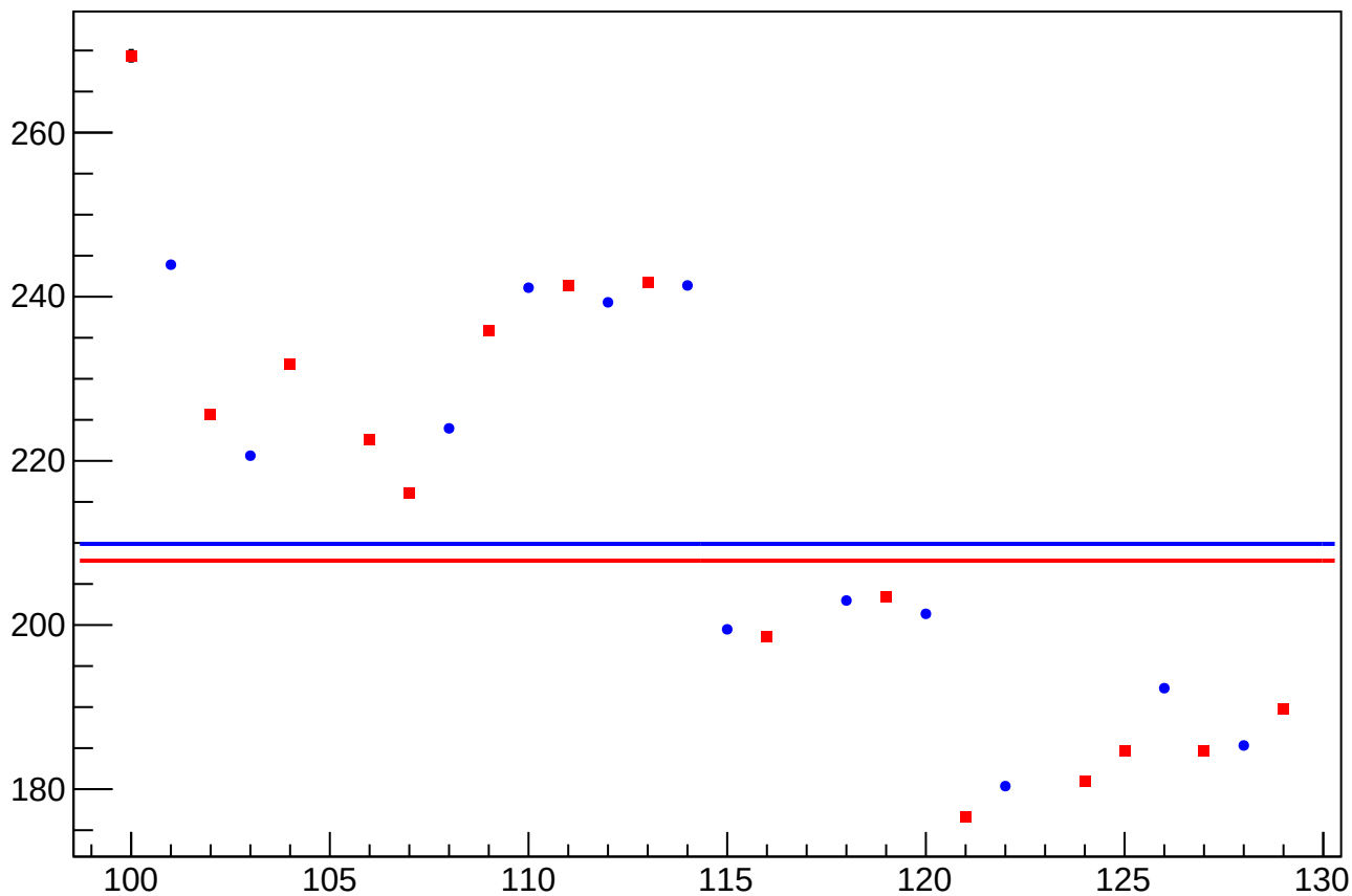
eigen_cor_asym_sam_26_dd_rms vs Slug, Sign Corrected
