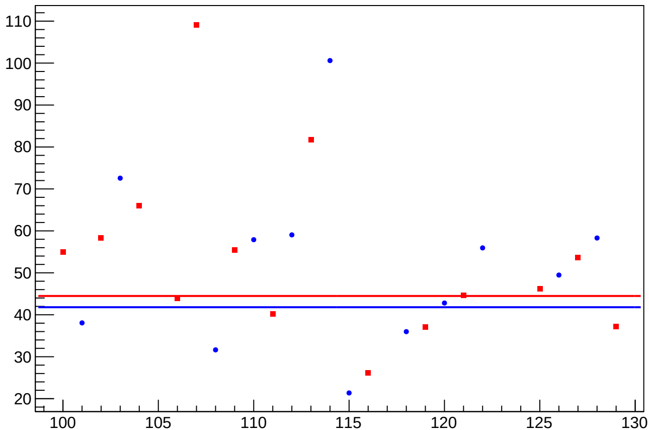
asym_usl_eigen_dit_vs_eigen_cor_diff_rms vs Slug, Sign Corrected
