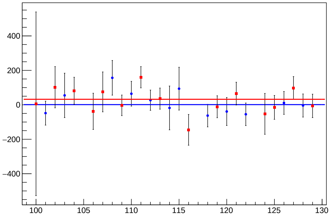
cor_asym_sam_15_37_dd_mean vs Slug, Sign Corrected
