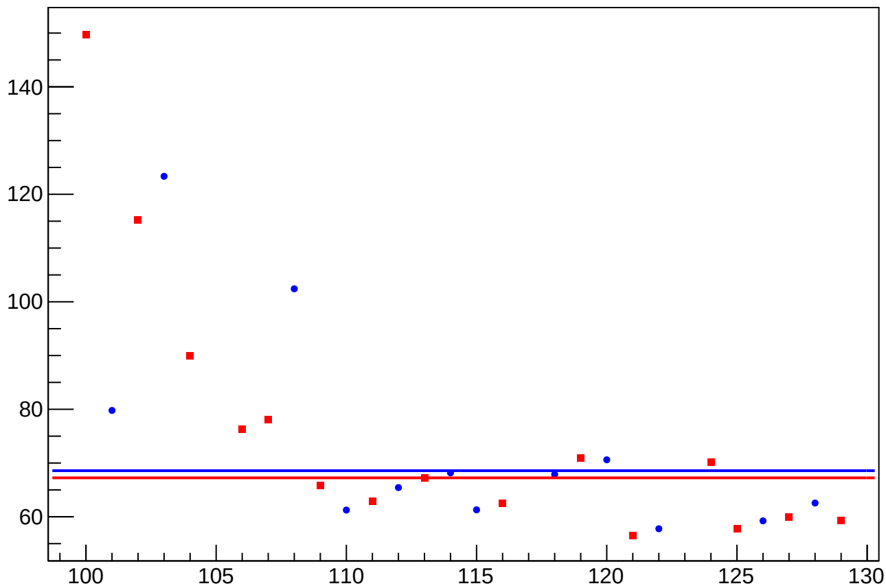
eigen_dit_asym_sam_13_57_dd_rms vs Slug, Sign Corrected
