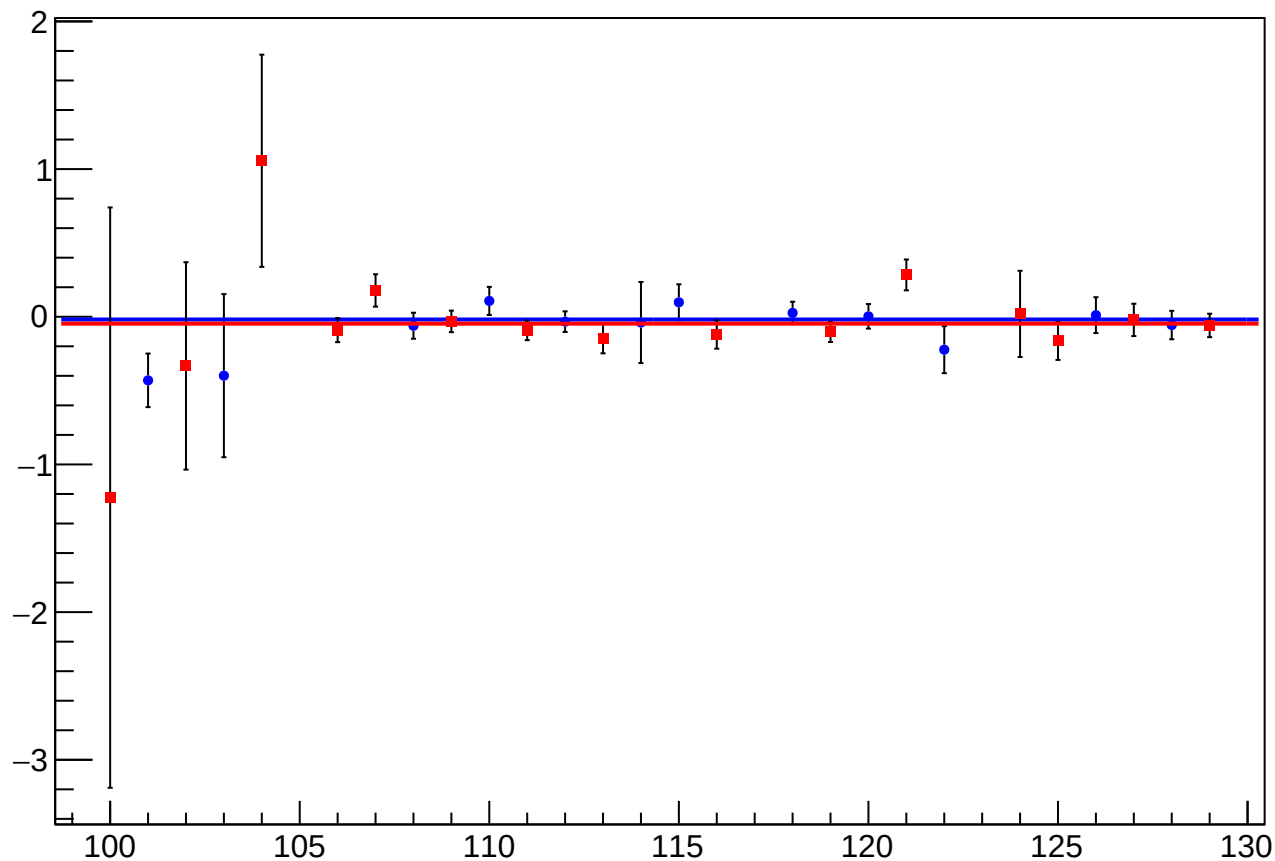
asym_usr_atr1_avg_dit_vs_Slug, Sign Corrected
