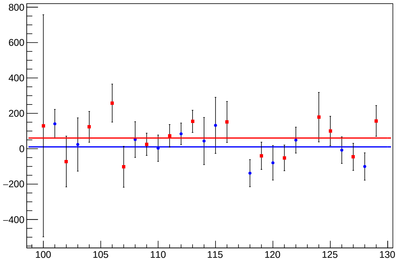
cor_asym_sam_1357_avg_mean vs Slug, Sign Corrected
