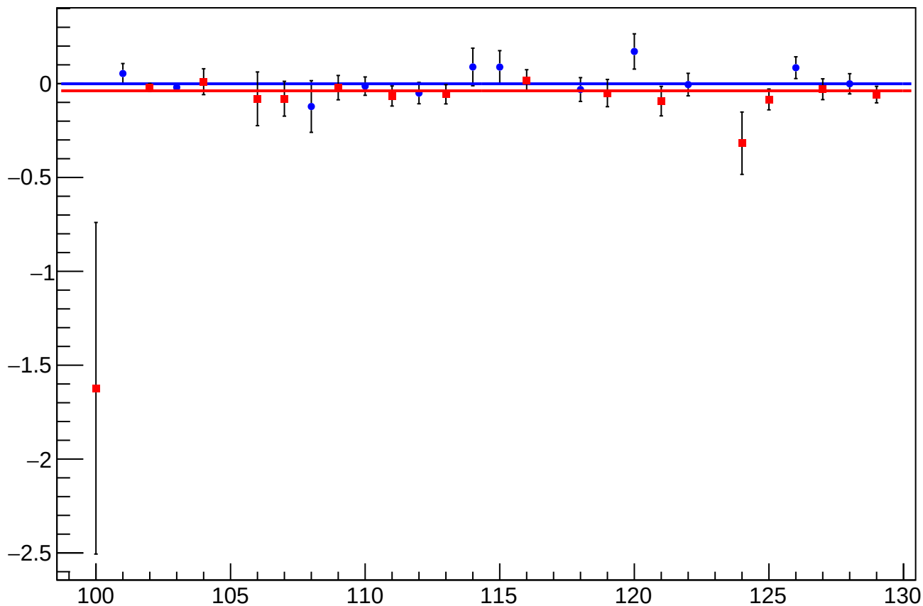
asym_sam_37_avg_eigen_dit_vs_eigen_cor_diff_mean vs Slug, Sign Corrected
