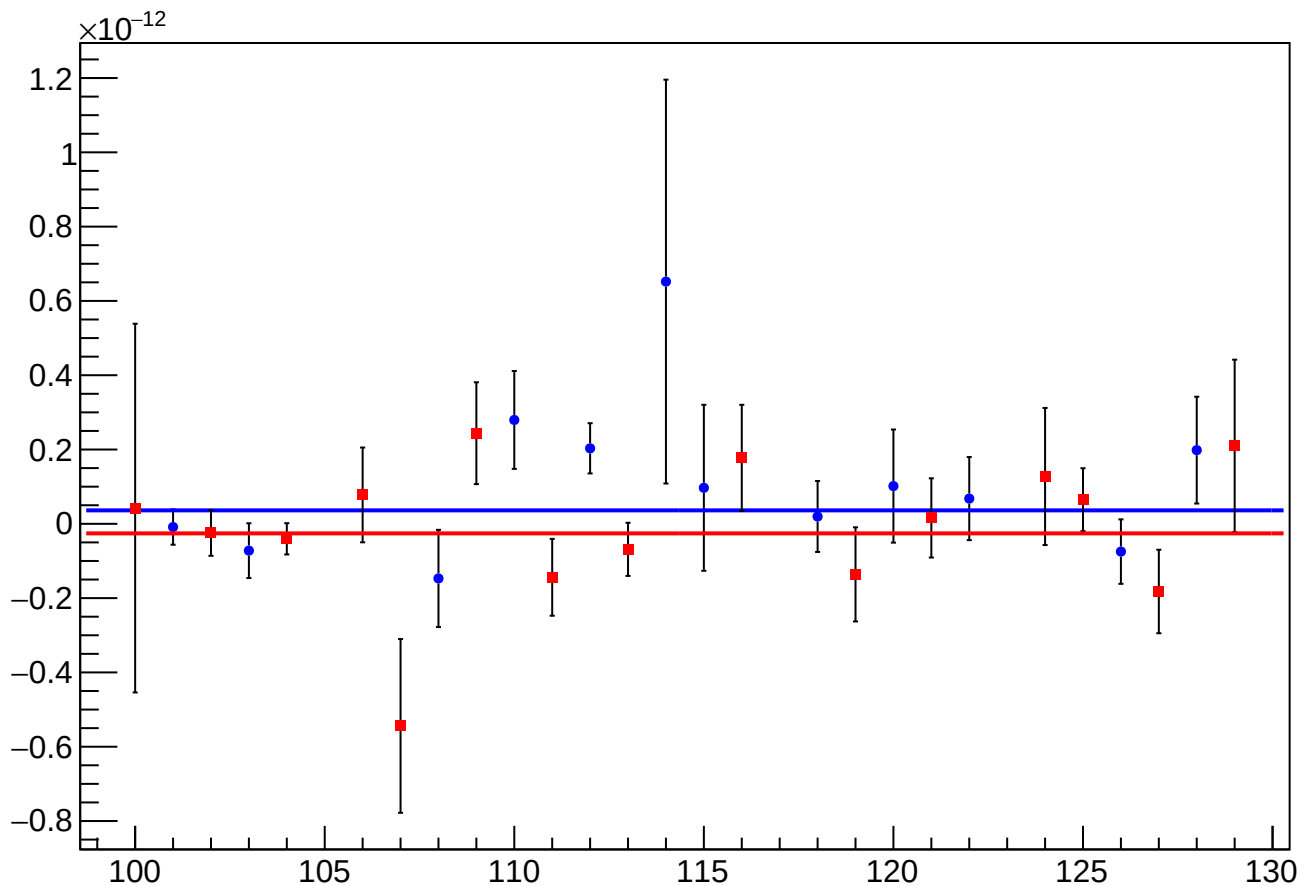
asym_usr_atr1_dd_reg_vs_cor_diff_mean vs Slug, Sign Corrected
