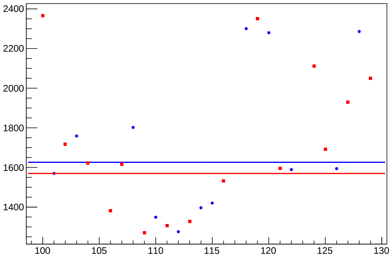
asym_sam3_eigen_dit_correction_rms vs Slug, Sign Corrected
