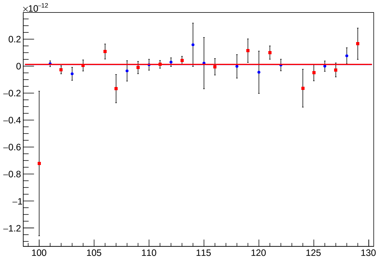
asym_sam_15_37_dd_reg_vs_cor_diff_mean vs Slug, Sign Corrected
