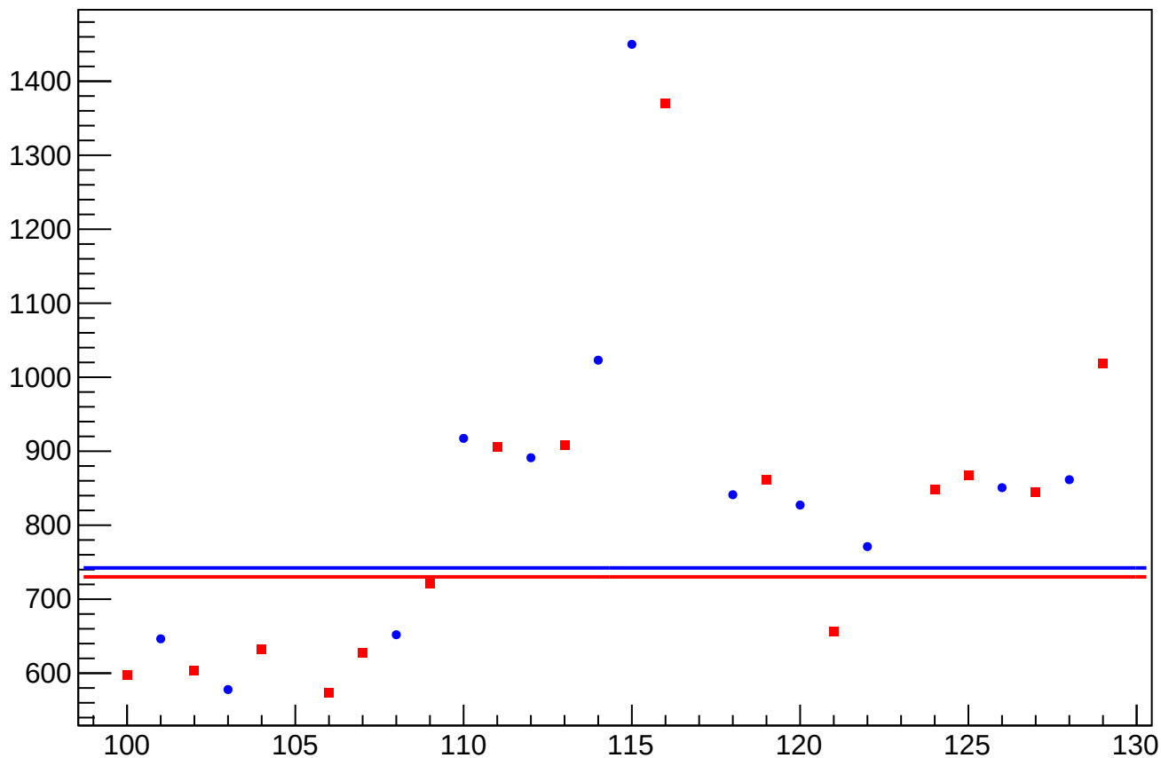
asym_sam_15_dd_eigen_dit_correction_rms vs Slug, Sign Corrected
