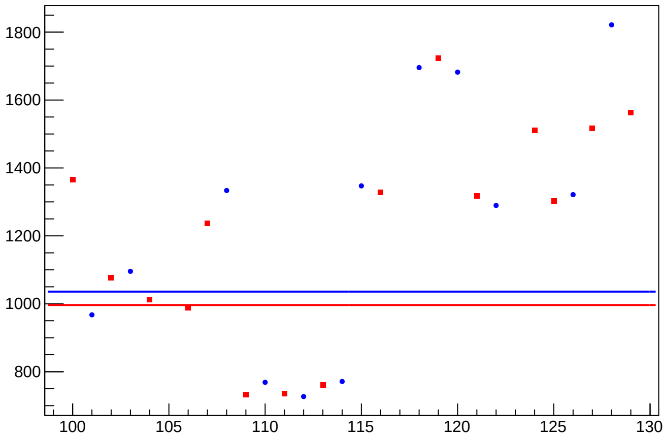
asym_sam_3748_avg_dit_correction_rms vs Slug, Sign Corrected
