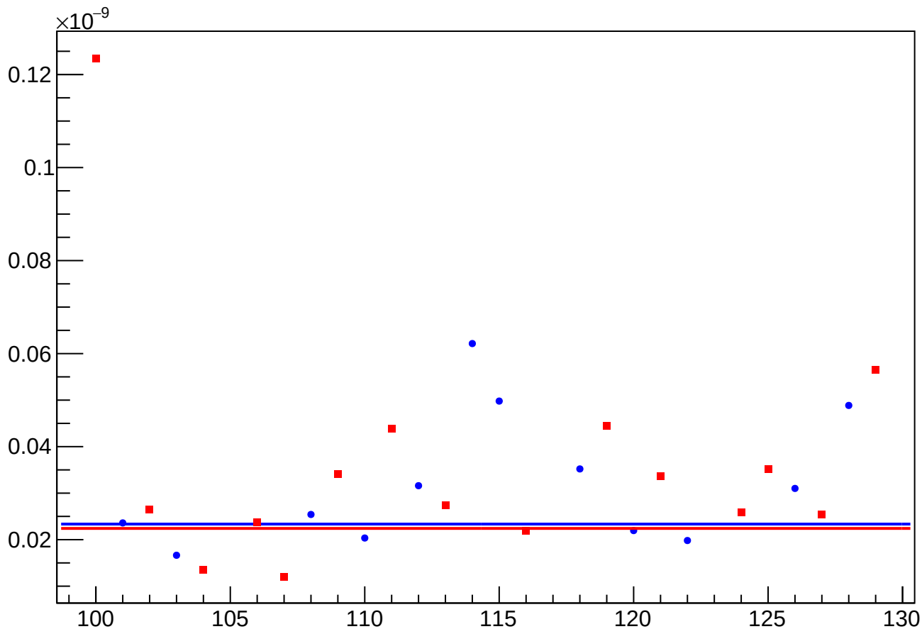
asym_usr_atr1_avg_eigen_cor_vs_cor_diff_rms vs Slug, Sign Corrected
