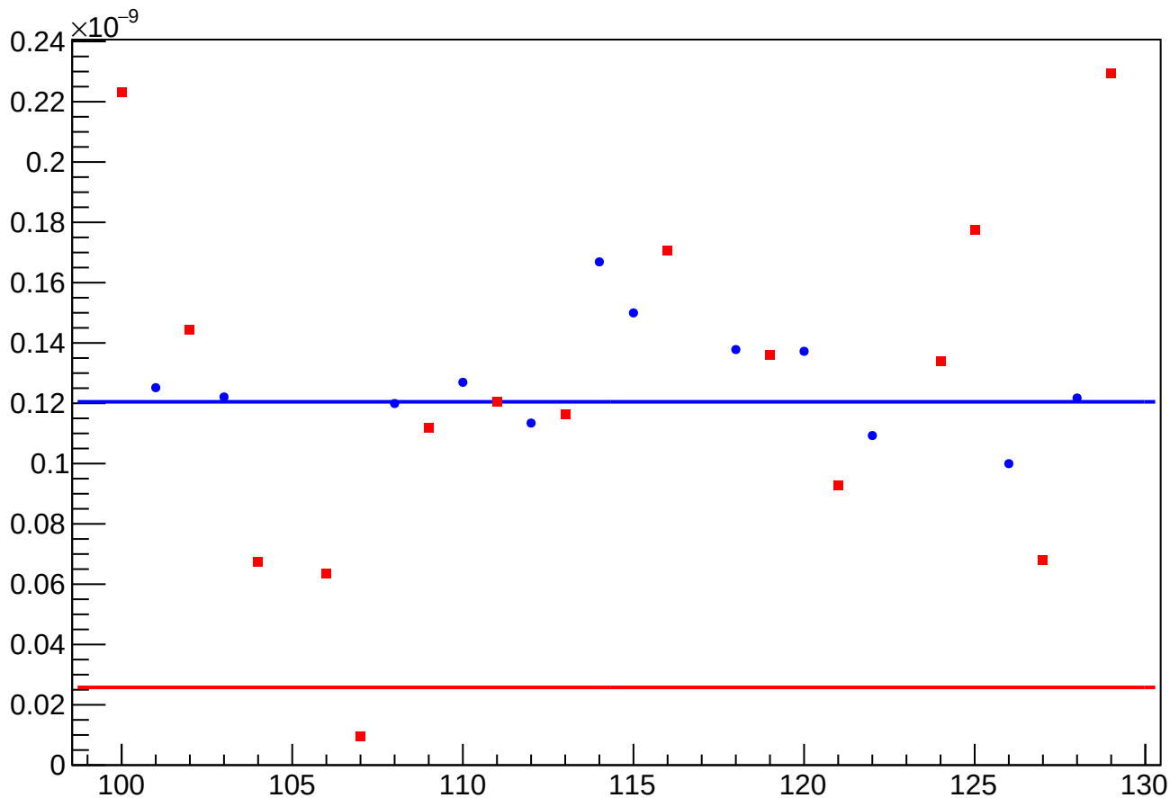
asym_atl1r2_dd_eigen_cor_vs_cor_diff_rms vs Slug, Sign Corrected
