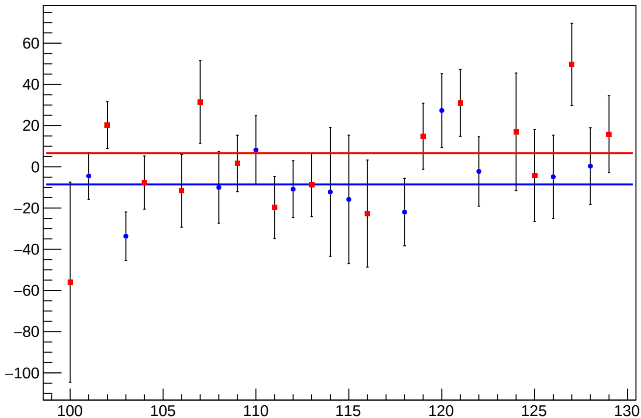
asym_bcm_an_us_an_ds3_dd_mean vs Slug, Sign Corrected
