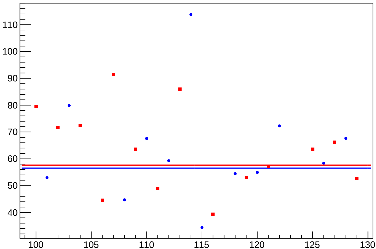
asym_us_avg_dit_vs_cor_diff_rms vs Slug, Sign Corrected
