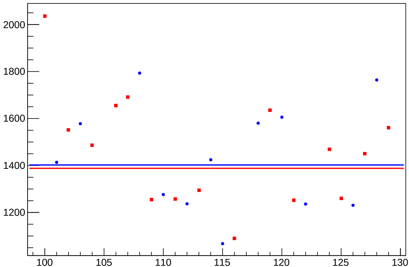
asym_sam_2468_avg_reg_correction_rms vs Slug, Sign Corrected
