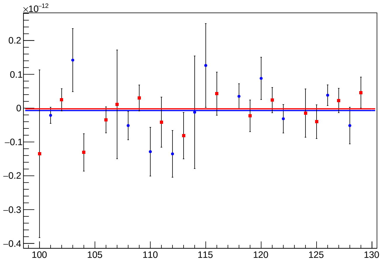
asym_at1_avg_eigen_cor_vs_cor_diff_mean vs Slug, Sign Corrected
