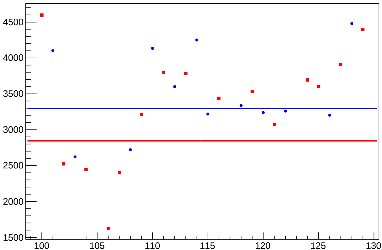
asym_usr_atr2_dd_dit_correction_rms vs Slug, Sign Corrected
