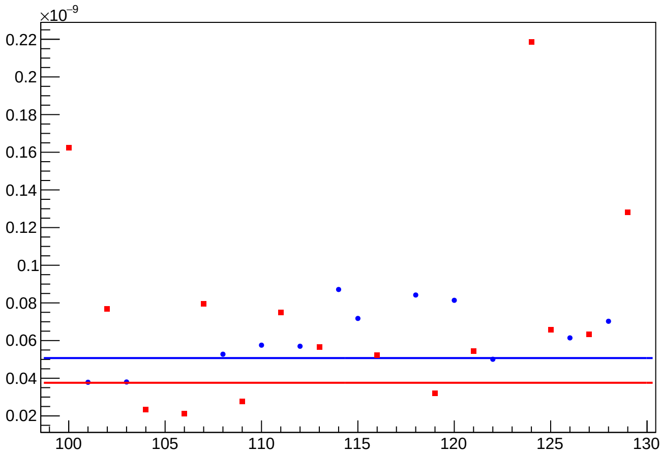
asym_at2_dd_eigen_cor_vs_cor_diff_rms vs Slug, Sign Corrected
