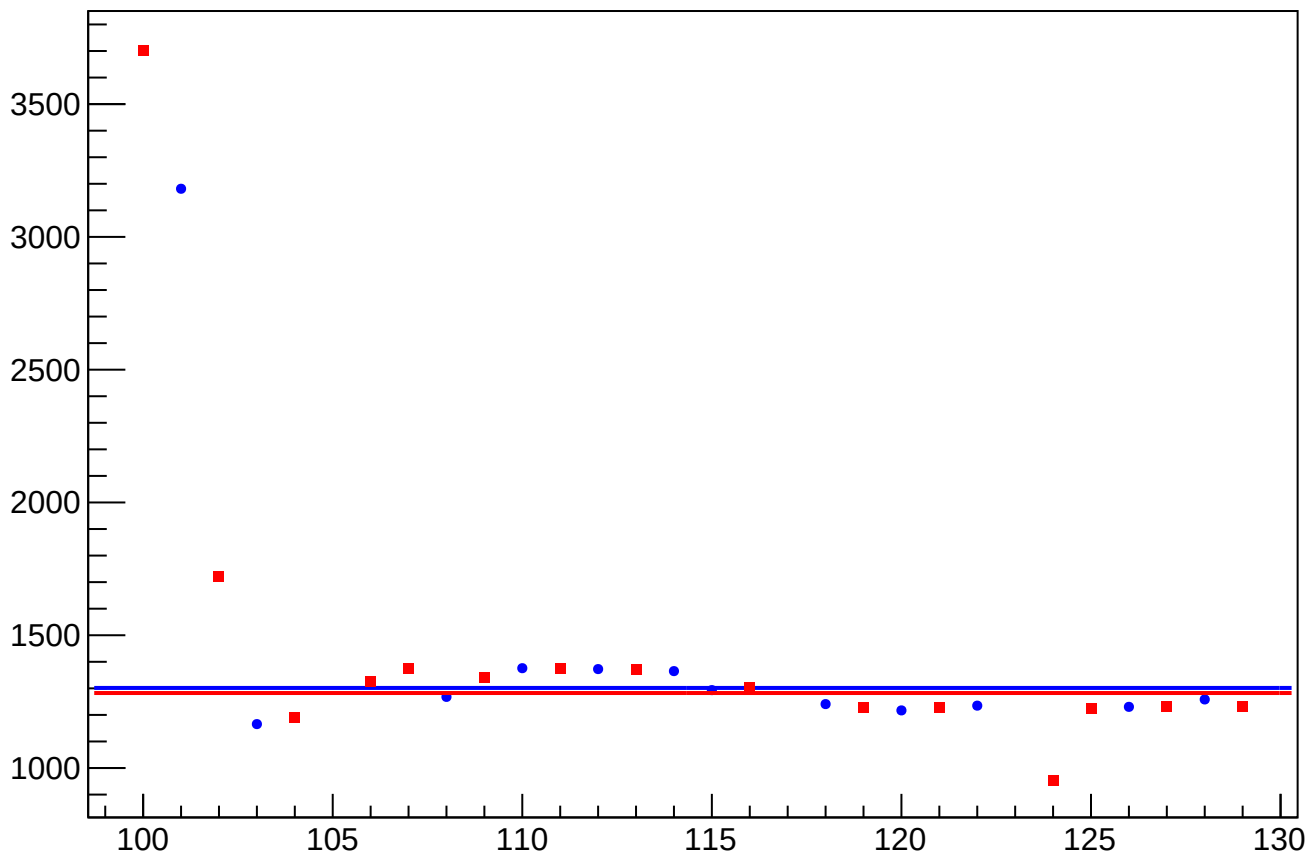
eigen_dit_asym_atl1r2_dd_atl2r1_dd_dd_rms vs Slug, Sign Corrected
