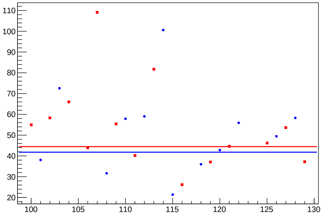
asym_usl_dit_vs_cor_diff_rms vs Slug, Sign Corrected
