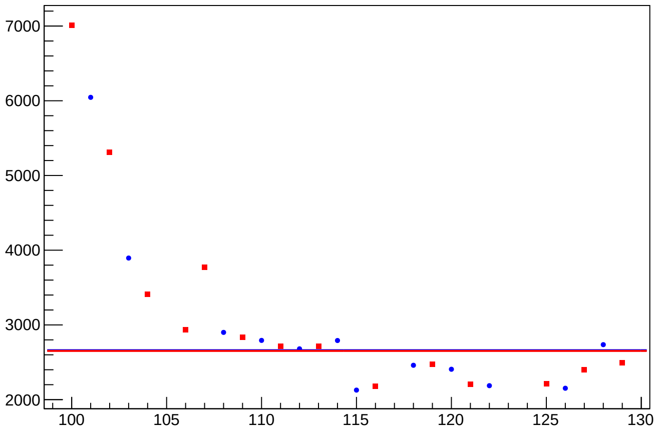
asym_us_dd_at1lr_dd_dd_rms vs Slug, Sign Corrected
