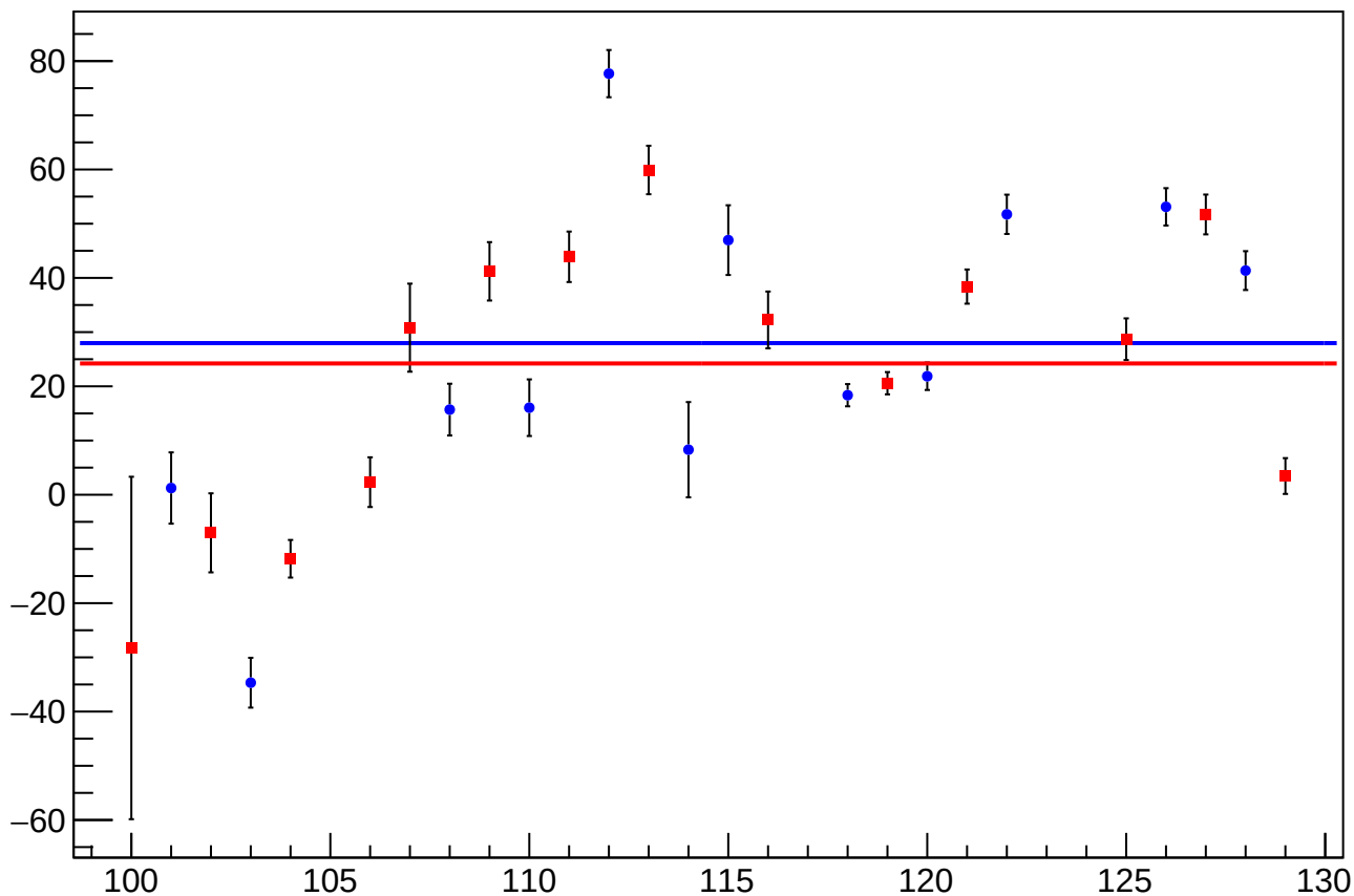
reg_asym_us_avg_at1lr_avg_avg_diff_bpm4aY_slope vs Slug, Sign Corrected
