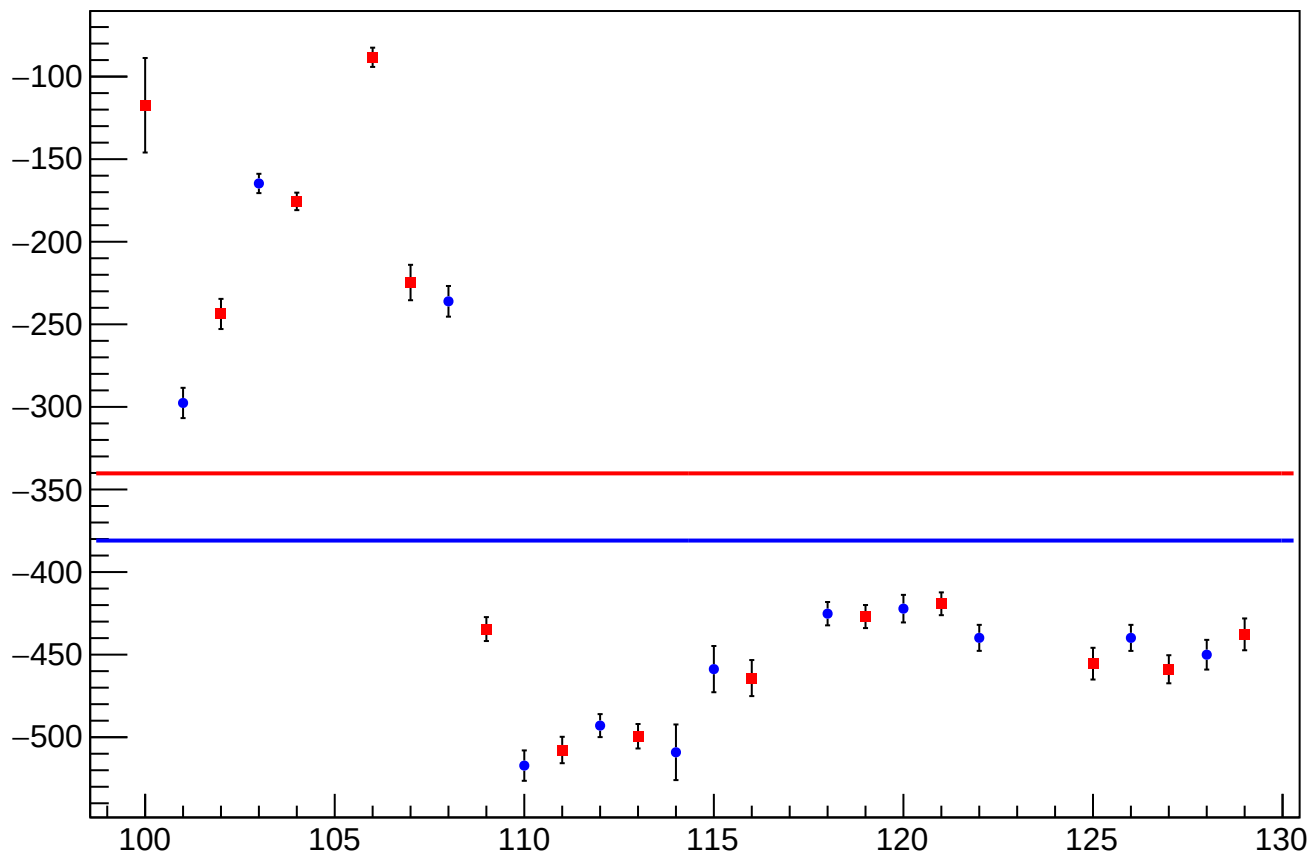
reg_asym_us_avg_at2lr_avg_dd_diff_bpm4eX_slope vs Slug, Sign Corrected
