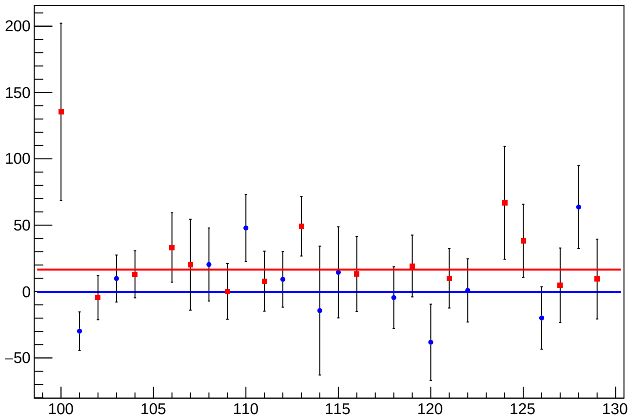
diff_bpm_4aX_4acX_avg_mean vs Slug, Sign Corrected
