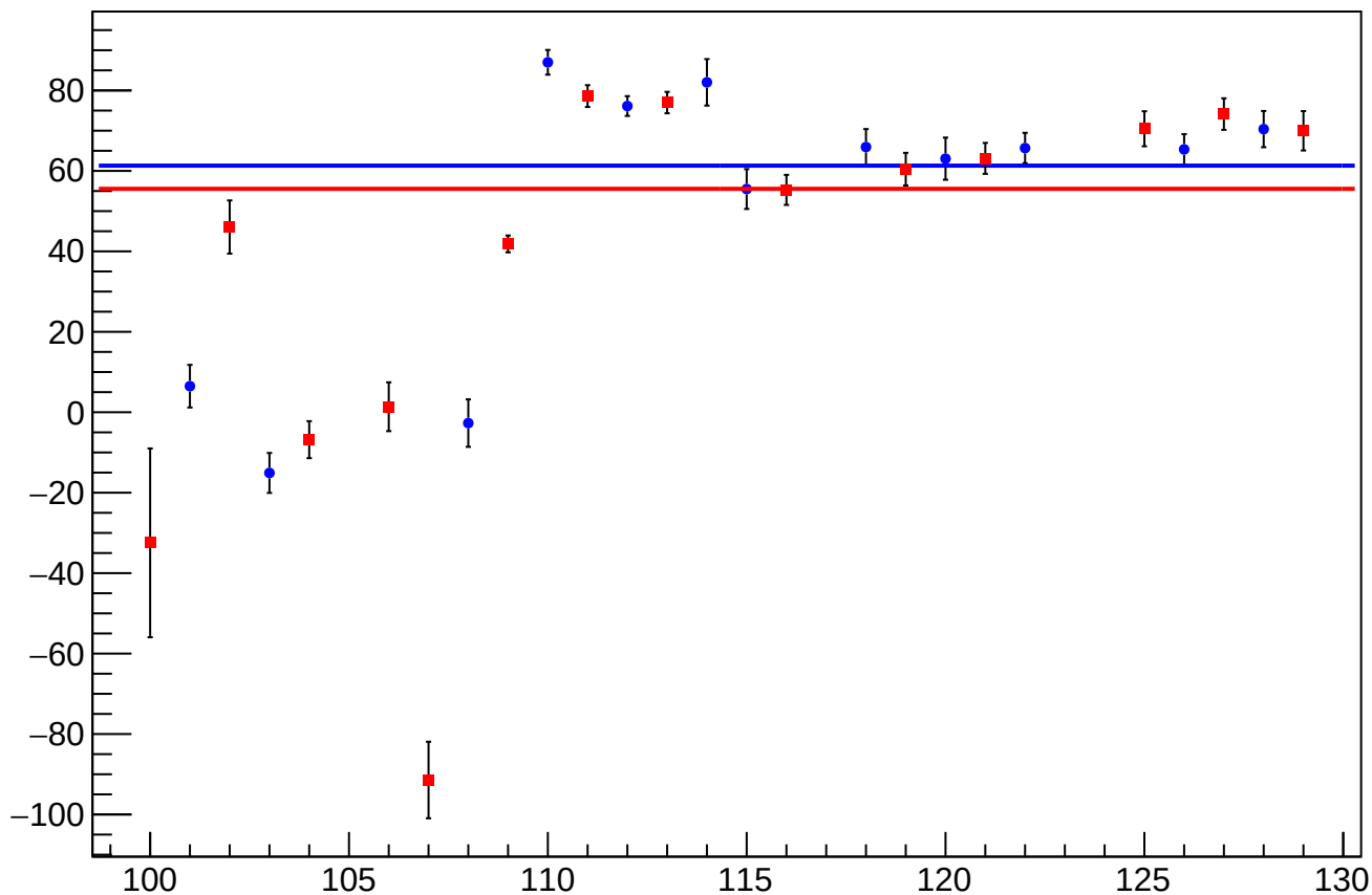
reg_asym_us_dd_at2lr_dd_avg_diff_bpm1X_slope vs Slug, Sign Corrected
