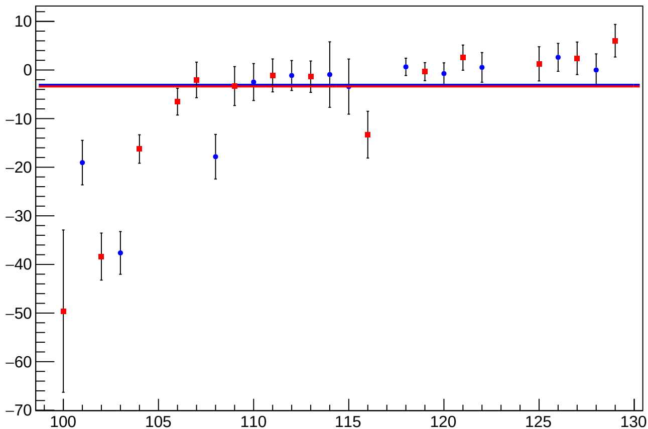
reg_asym_usl_atl2_dd_diff_bpm4aY_slope vs Slug, Sign Corrected
