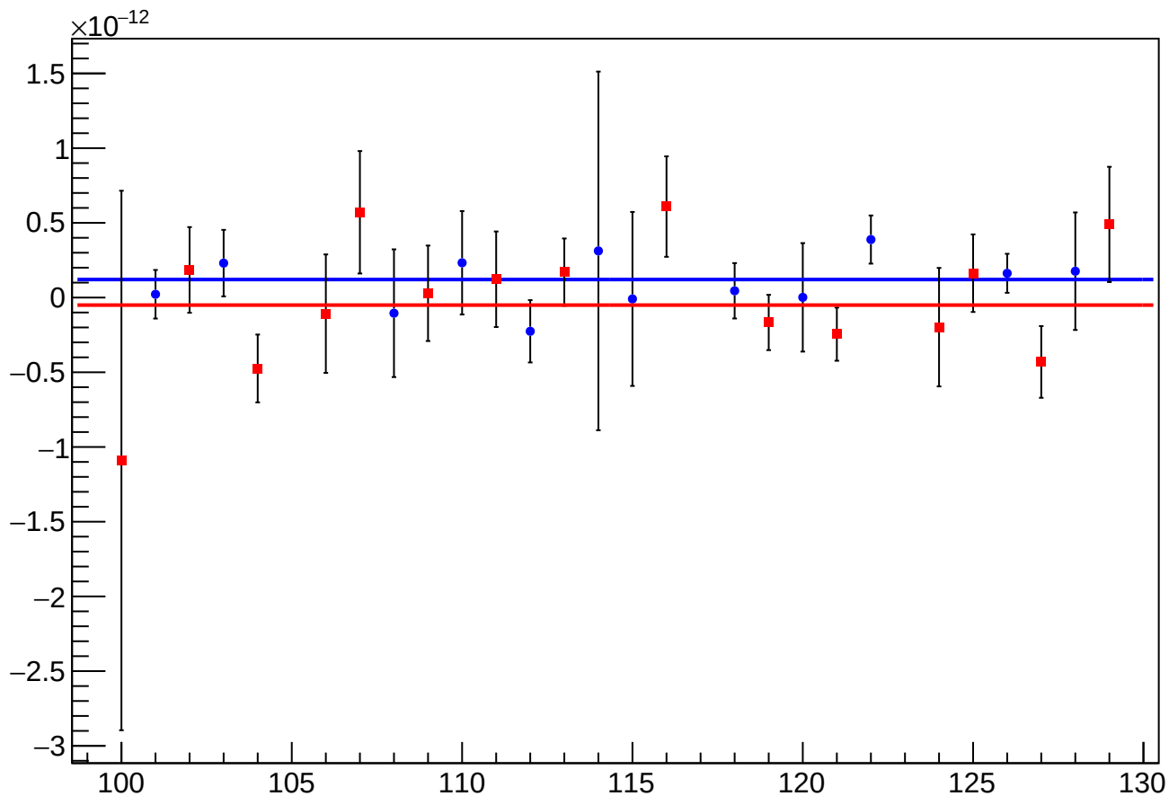
asym_sam2_eigen_cor_vs_cor_diff_mean vs Slug, Sign Corrected
