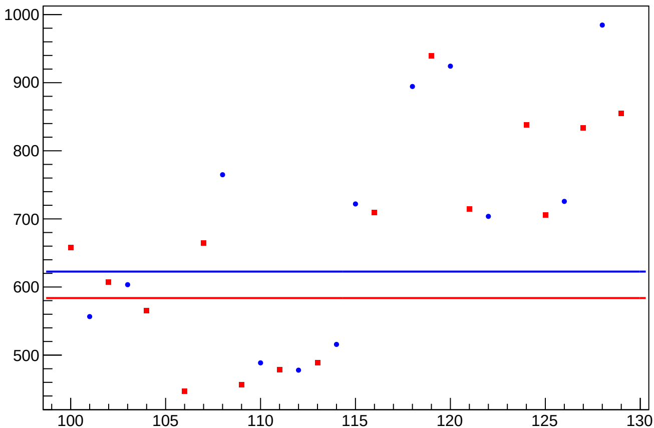
asym_sam_15_48_dd_reg_correction_rms vs Slug, Sign Corrected
