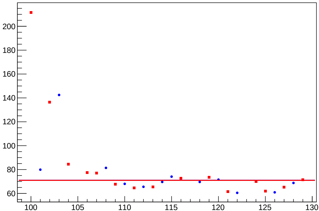
eigen_cor_asym_sam_12345678_avg_rms vs Slug, Sign Corrected
