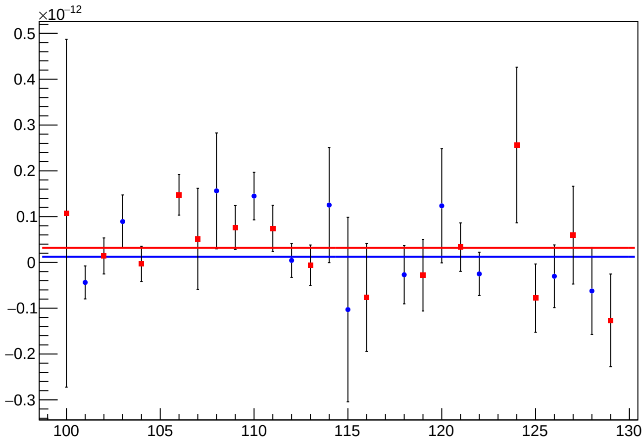
asym_sam_3748_avg_eigen_cor_vs_cor_diff_mean vs Slug, Sign Corrected
