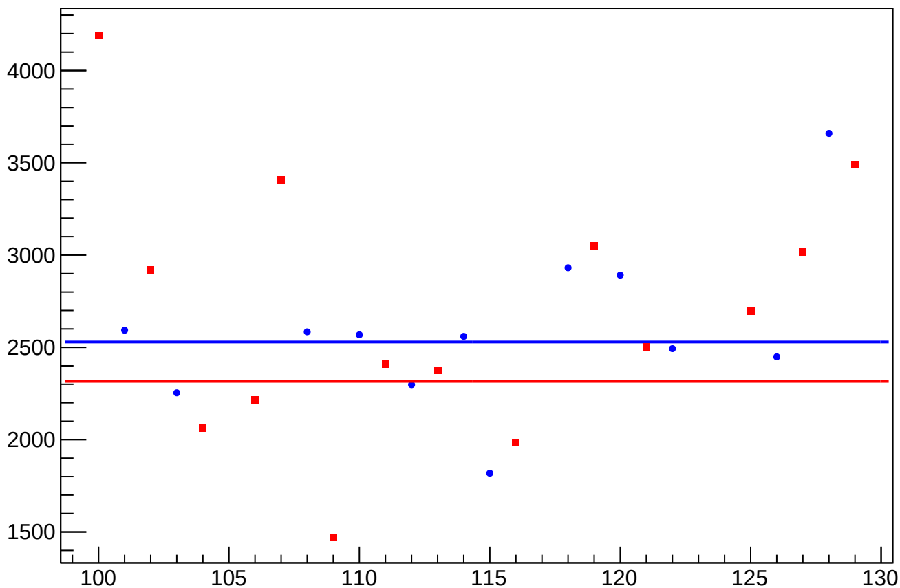
asym_us_dd_at2lr_dd_avg_eigen_cor_correction_rms vs Slug, Sign Corrected
