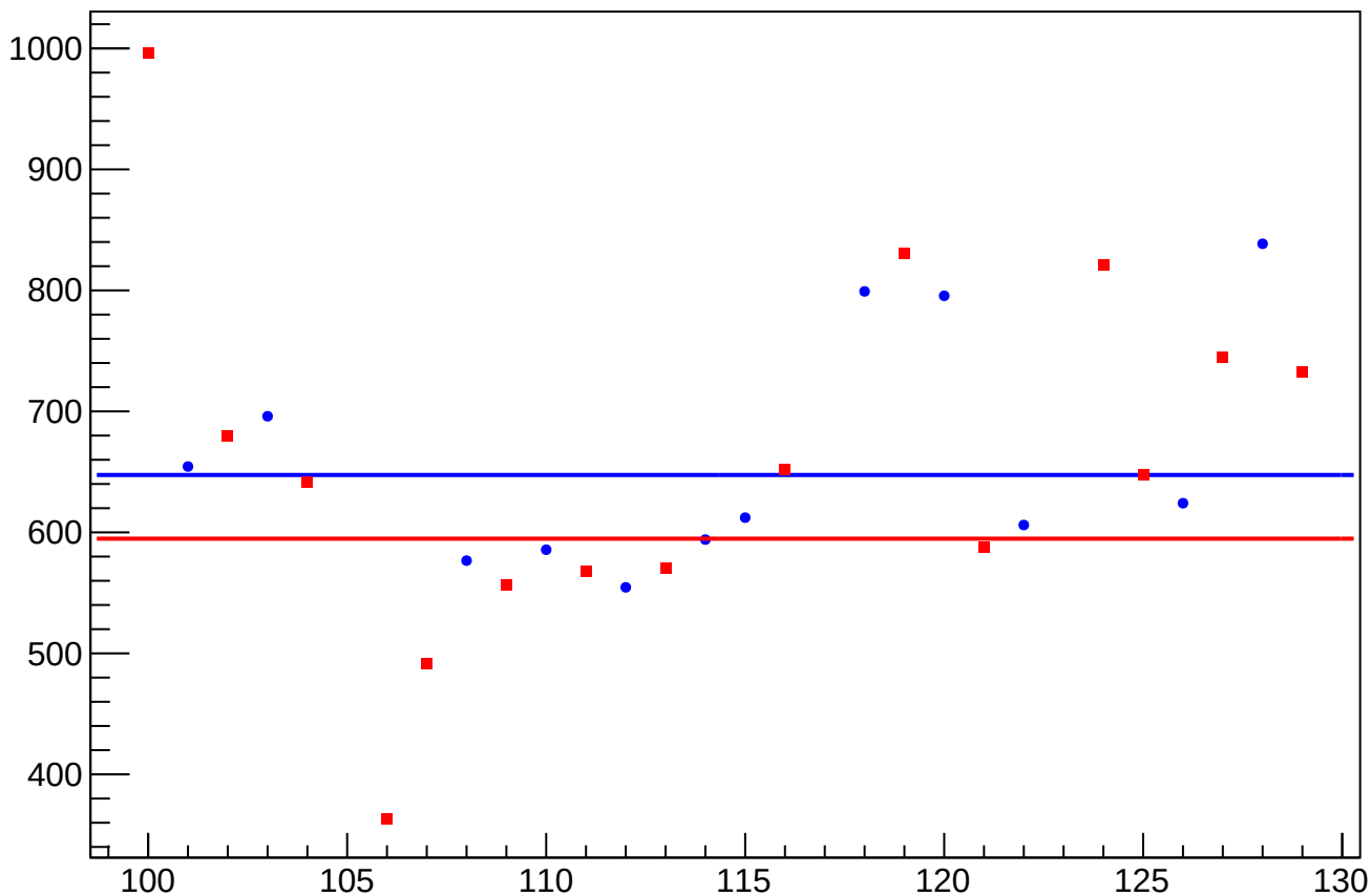
asym_sam_37_dd_dit_correction_rms vs Slug, Sign Corrected
