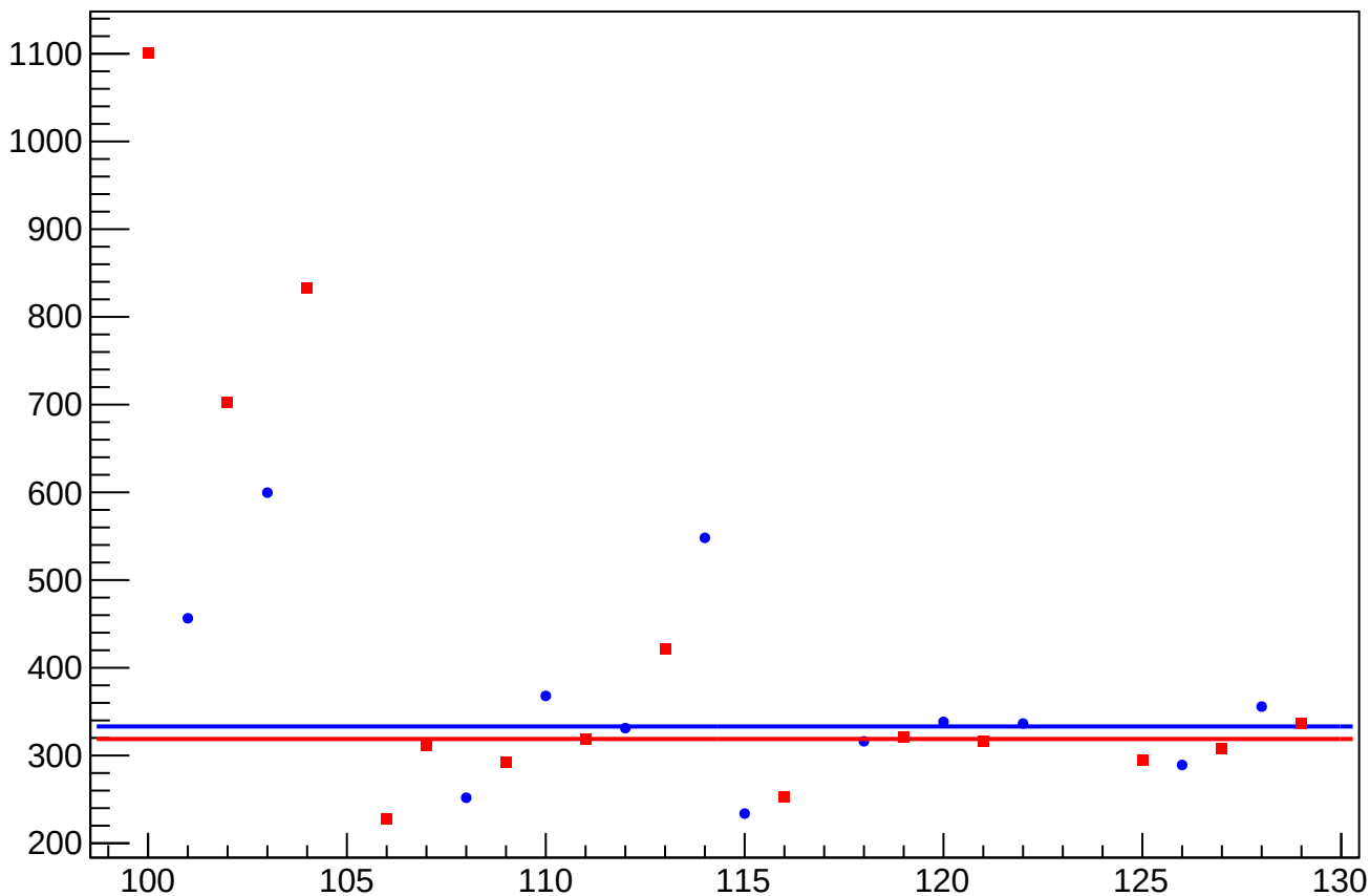
asym_us_avg_at2lr_avg_avg_dit_vs_cor_diff_rms vs Slug, Sign Corrected
