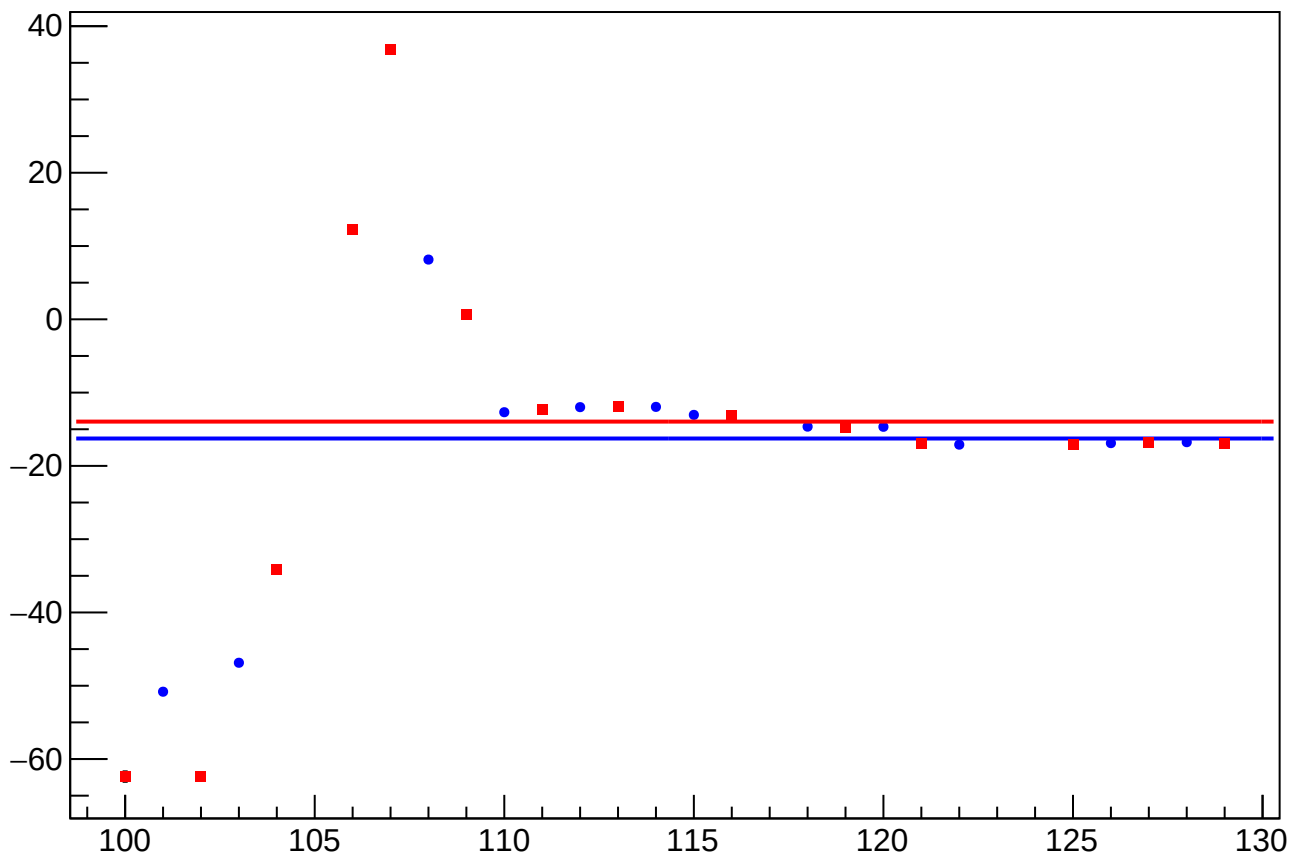
reg_asym_us_dd_atlr_dd_dd_diff_bpm12X_slope vs Slug, Sign Corrected
