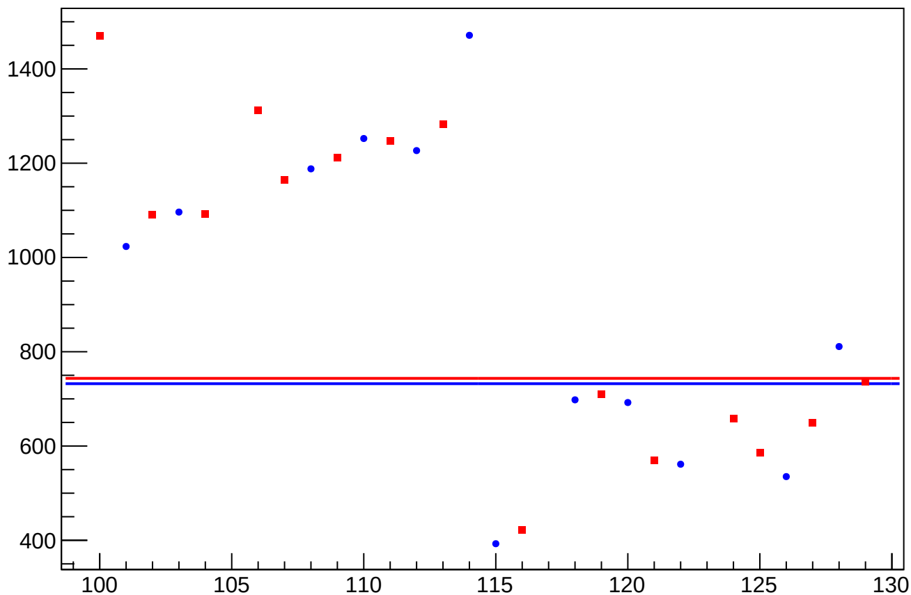
asym_sam_1526_avg_reg_correction_rms vs Slug, Sign Corrected
