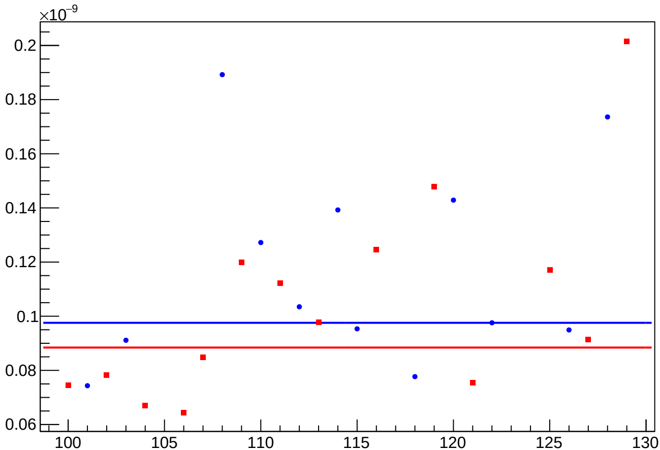
asym_usl_atl2_avg_eigen_cor_vs_cor_diff_rms vs Slug, Sign Corrected
