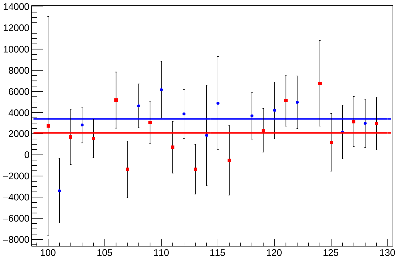
eigen_cor_asym_usr_atr2_avg_mean vs Slug, Sign Corrected
