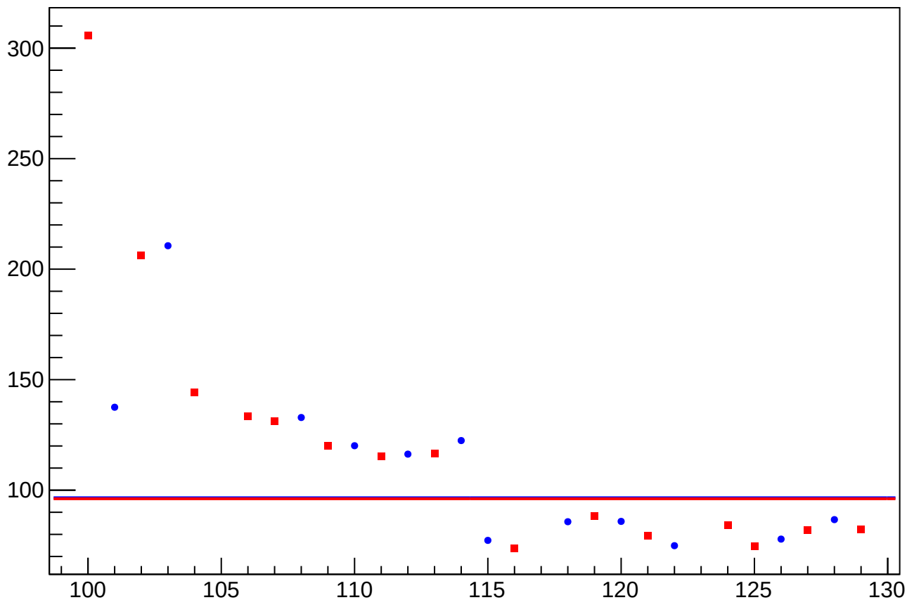
cor_asym_sam_3726_avg_rms vs Slug, Sign Corrected
