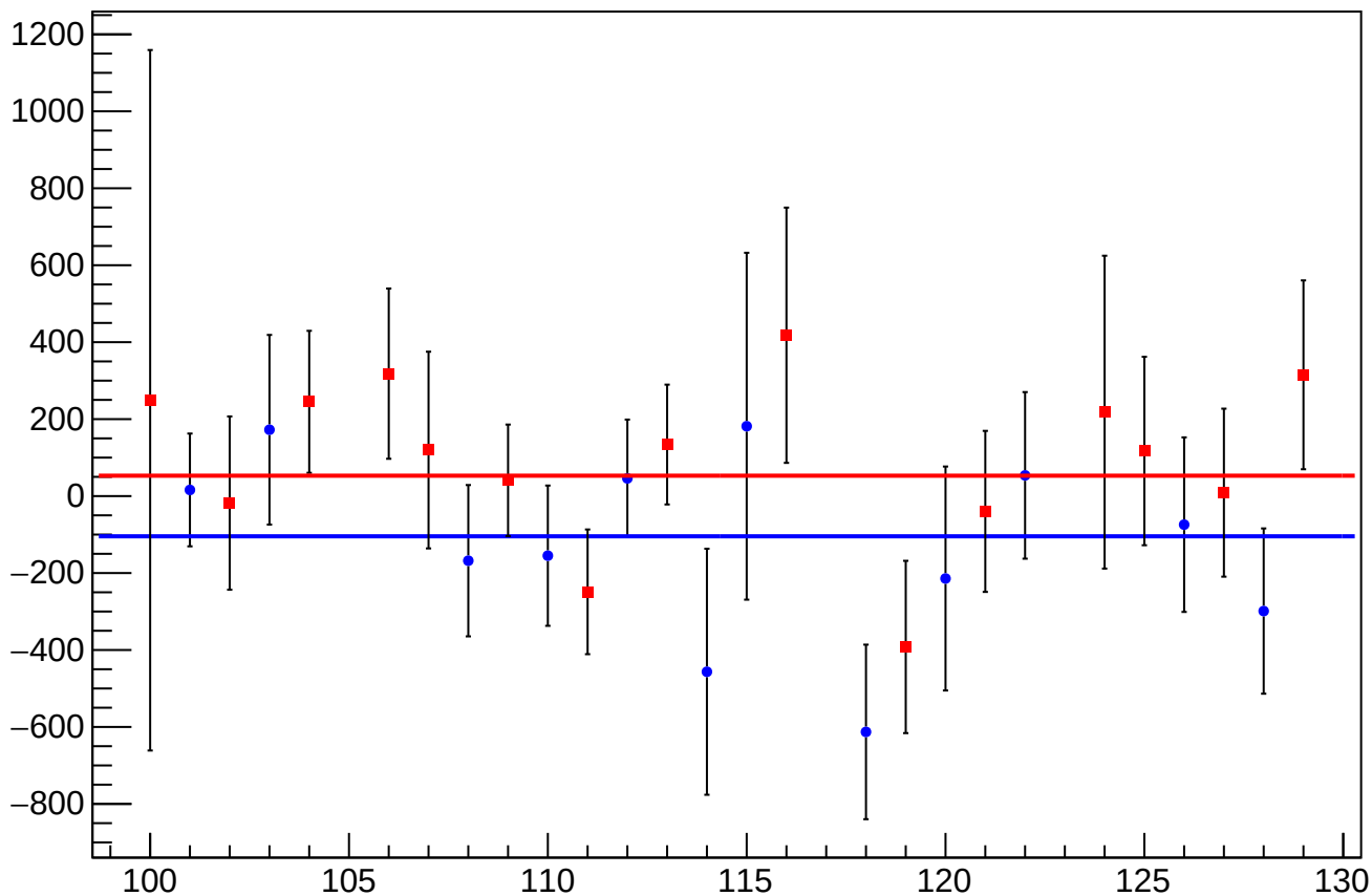
cor_asym_sam_48_avg_mean vs Slug, Sign Corrected
