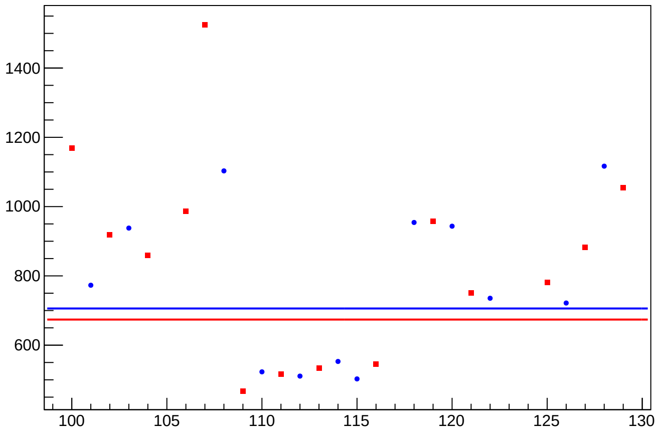
asym_us_dd_eigen_cor_correction_rms vs Slug, Sign Corrected
