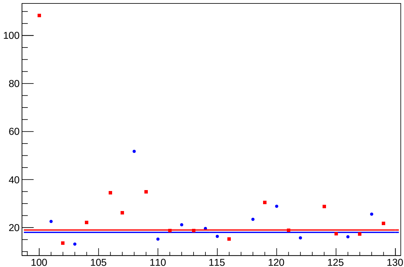
asym_sam_15_37_dd_dit_vs_cor_diff_rms vs Slug, Sign Corrected
