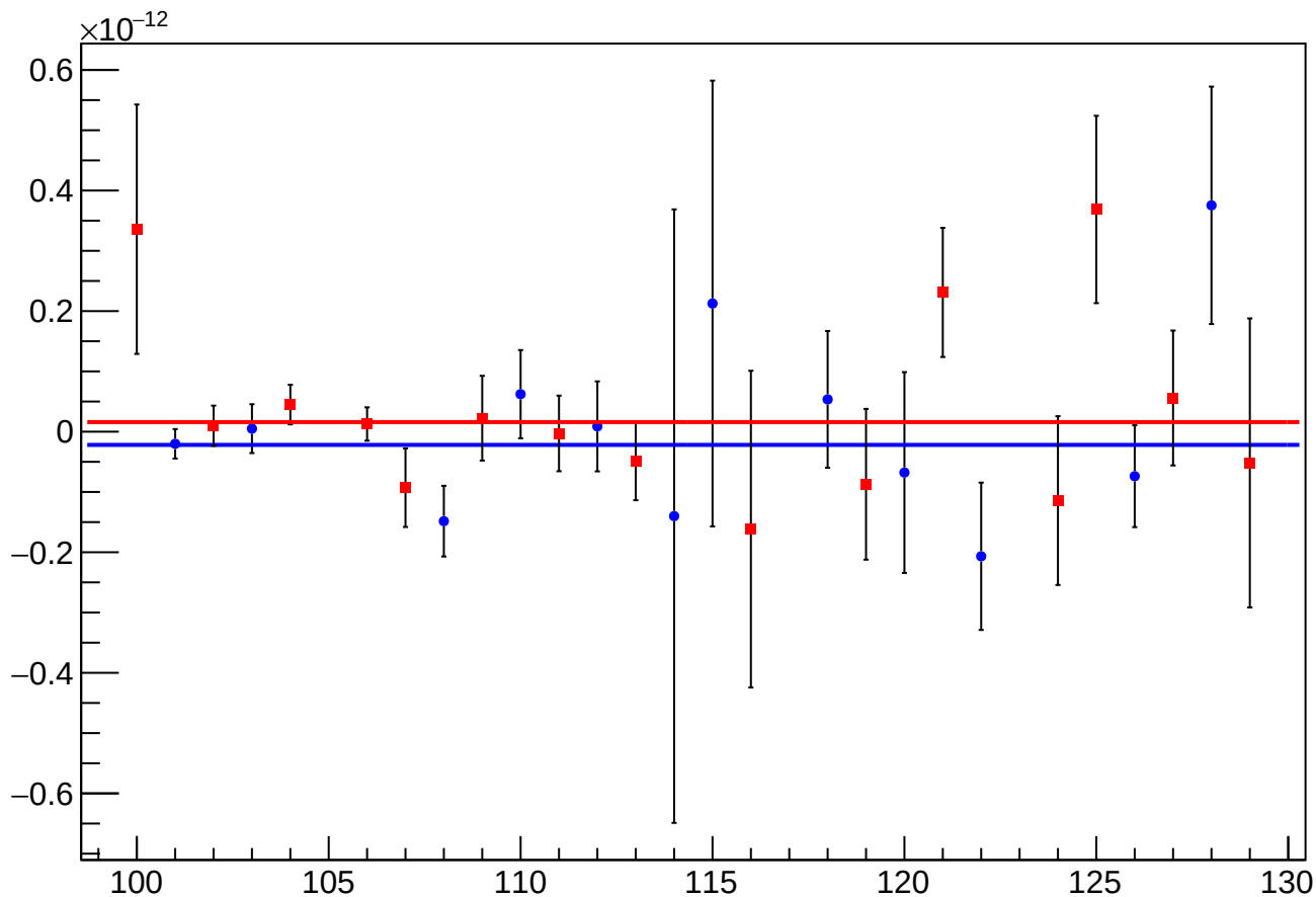
asym_sam6_reg_vs_cor_diff_mean vs Slug, Sign Corrected
