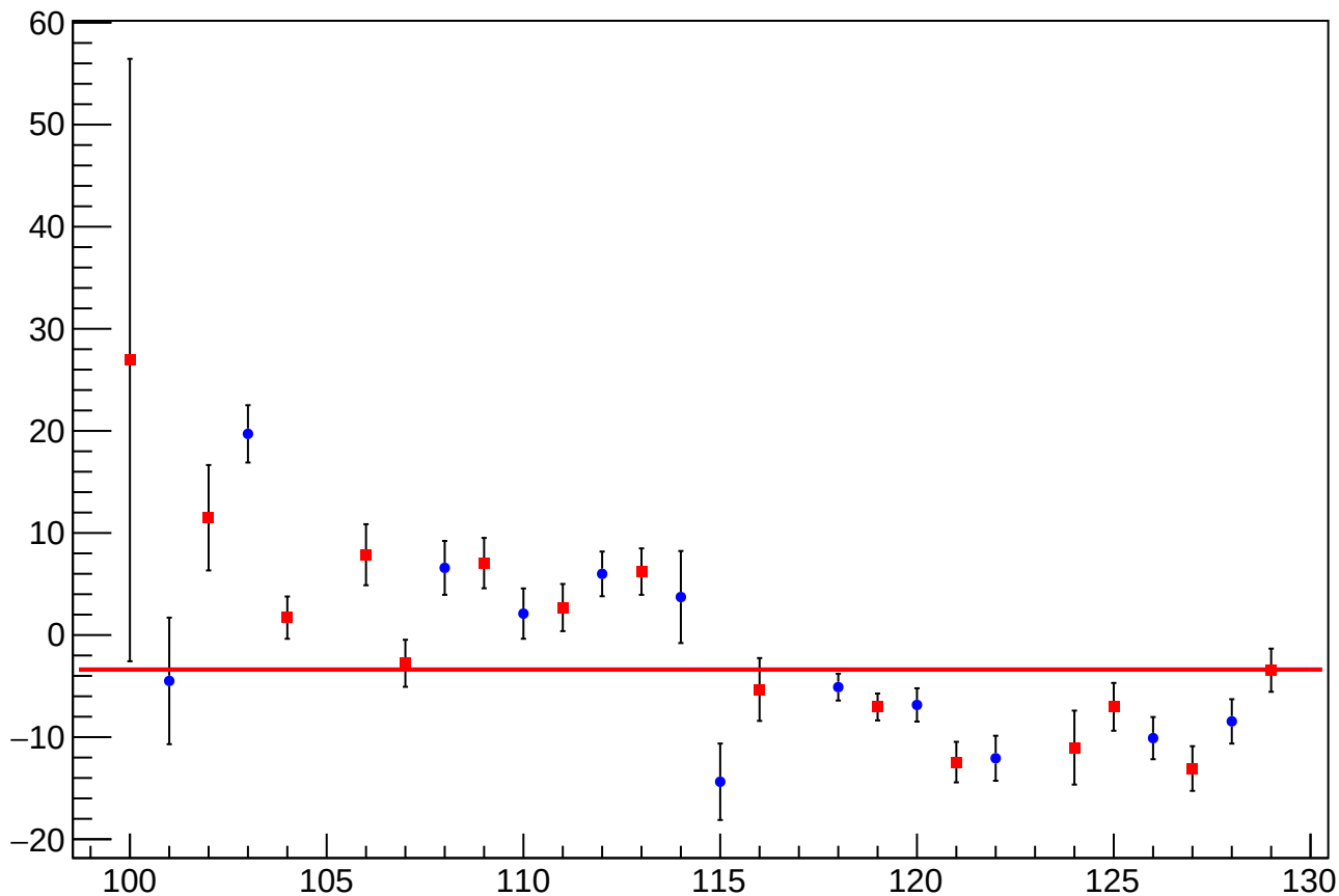
reg_asym_usr_atr1_dd_diff_bpm4aY_slope vs Slug, Sign Corrected
