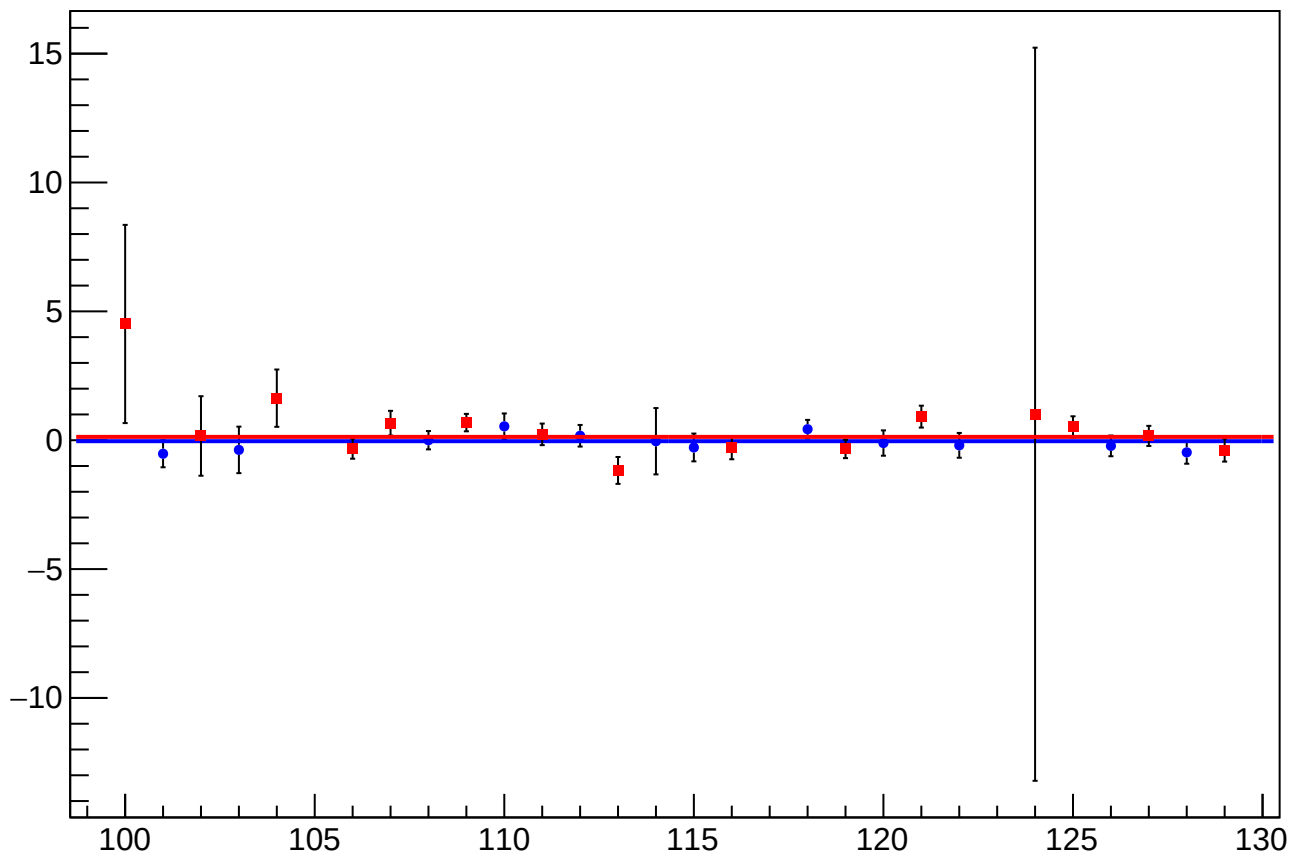
asym_at2_avg_dit_vs_cor_diff_mean vs Slug, Sign Corrected
