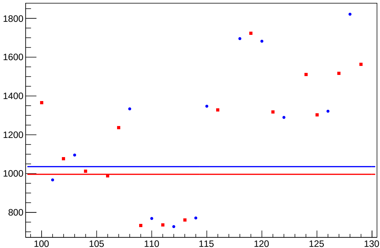
asym_sam_3748_avg_eigen_dit_correction_rms vs Slug, Sign Corrected
