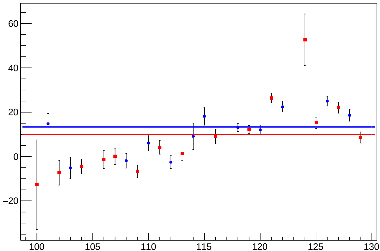
reg_asym_at1_dd_at2_dd_avg_diff_bpm4eY_slope vs Slug, Sign Corrected
