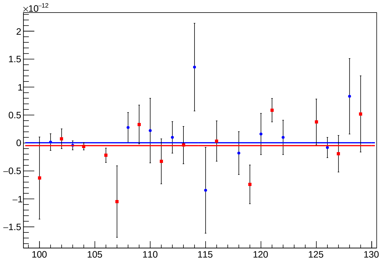
asym_us_avg_atlr_avg_avg_eigen_cor_vs_cor_diff_mean vs Slug, Sign Corrected
