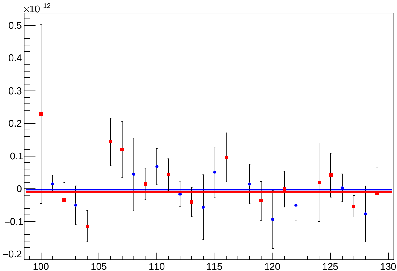
asym_sam_12345678_avg_eigen_cor_vs_cor_diff_mean vs Slug, Sign Corrected
