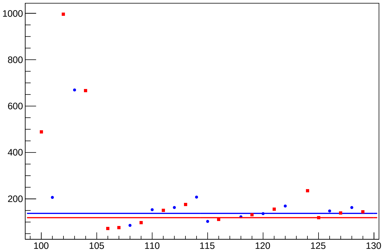
asym_usr_atr2_dd_dit_vs_cor_diff_rms vs Slug, Sign Corrected
