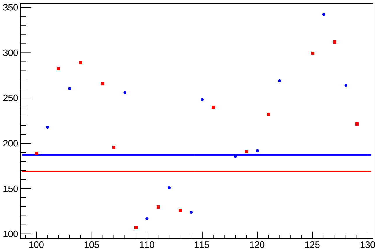
asym_bcm_dg_ds_an_us_avg_rms vs Slug, Sign Corrected
