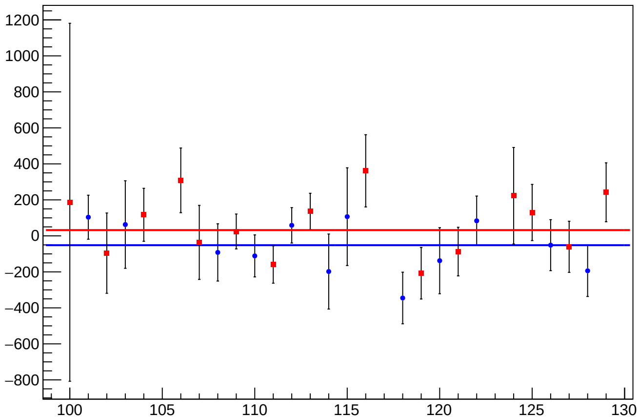
cor_asym_sam_3748_avg_mean vs Slug, Sign Corrected
