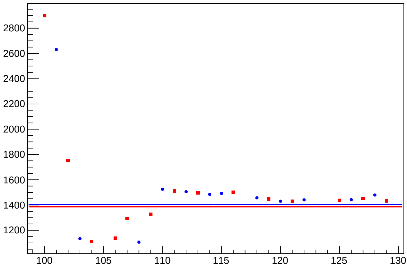
eigen_cor_asym_us_avg_at2lr_avg_dd_rms vs Slug, Sign Corrected
