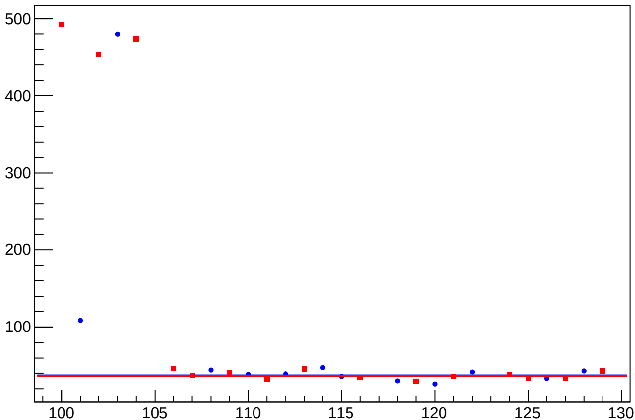
asym_usr_atr1_dd_dit_vs_eigen_cor_diff_rms vs Slug, Sign Corrected
