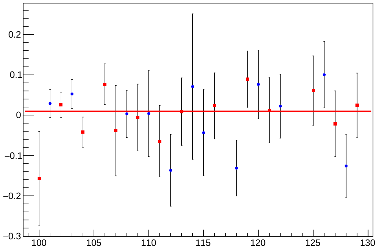
asym_us_avg_overload_cor_vs_eigen_cor_diff_mean vs Slug, Sign Corrected
