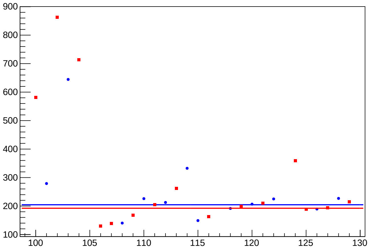
asym_usr_atr2_avg_eigen_dit_vs_cor_diff_rms vs Slug, Sign Corrected
