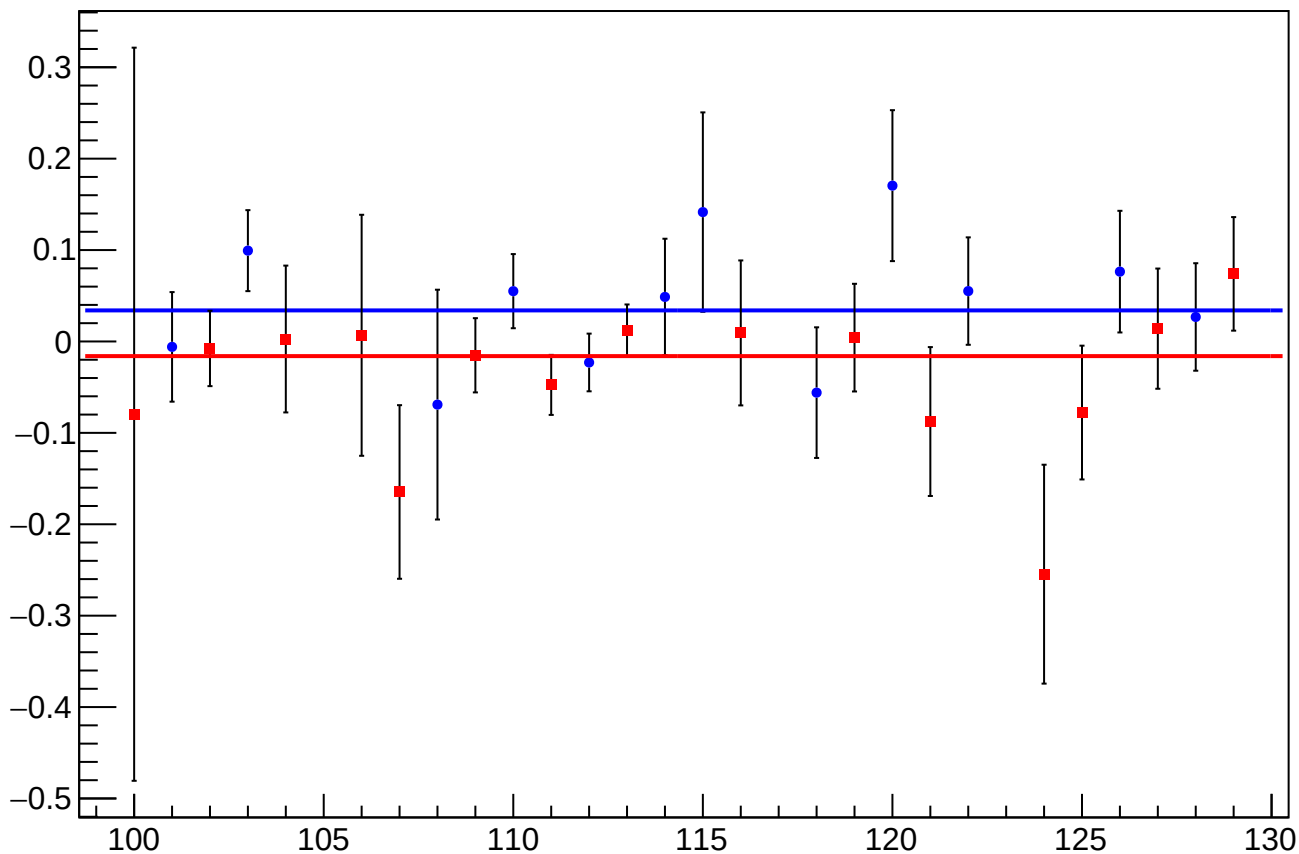
asym_sam_3748_avg_eigen_dit_vs_cor_diff_mean vs Slug, Sign Corrected
