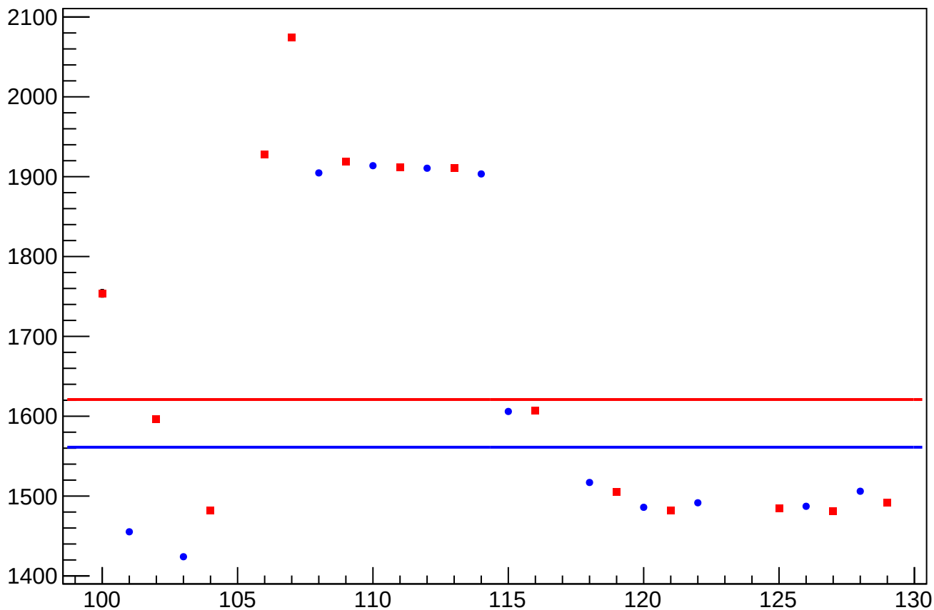
cor_asym_usl_atl1_avg_rms vs Slug, Sign Corrected
