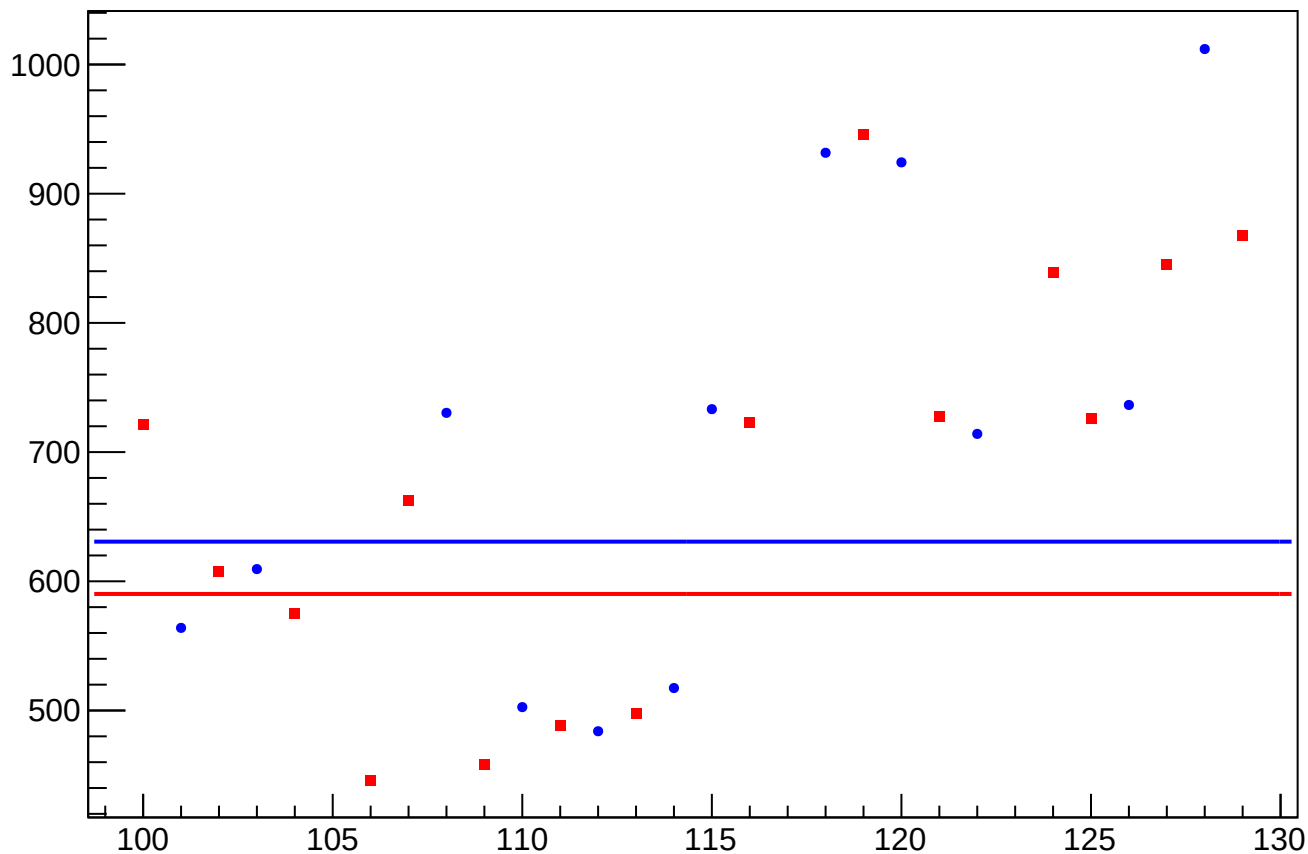
asym_sam_15_48_dd_dit_correction_rms vs Slug, Sign Corrected
