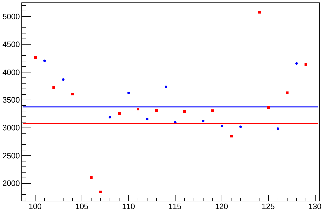
asym_atl_dd_atr_dd_avg_dit_correction_rms vs Slug, Sign Corrected
