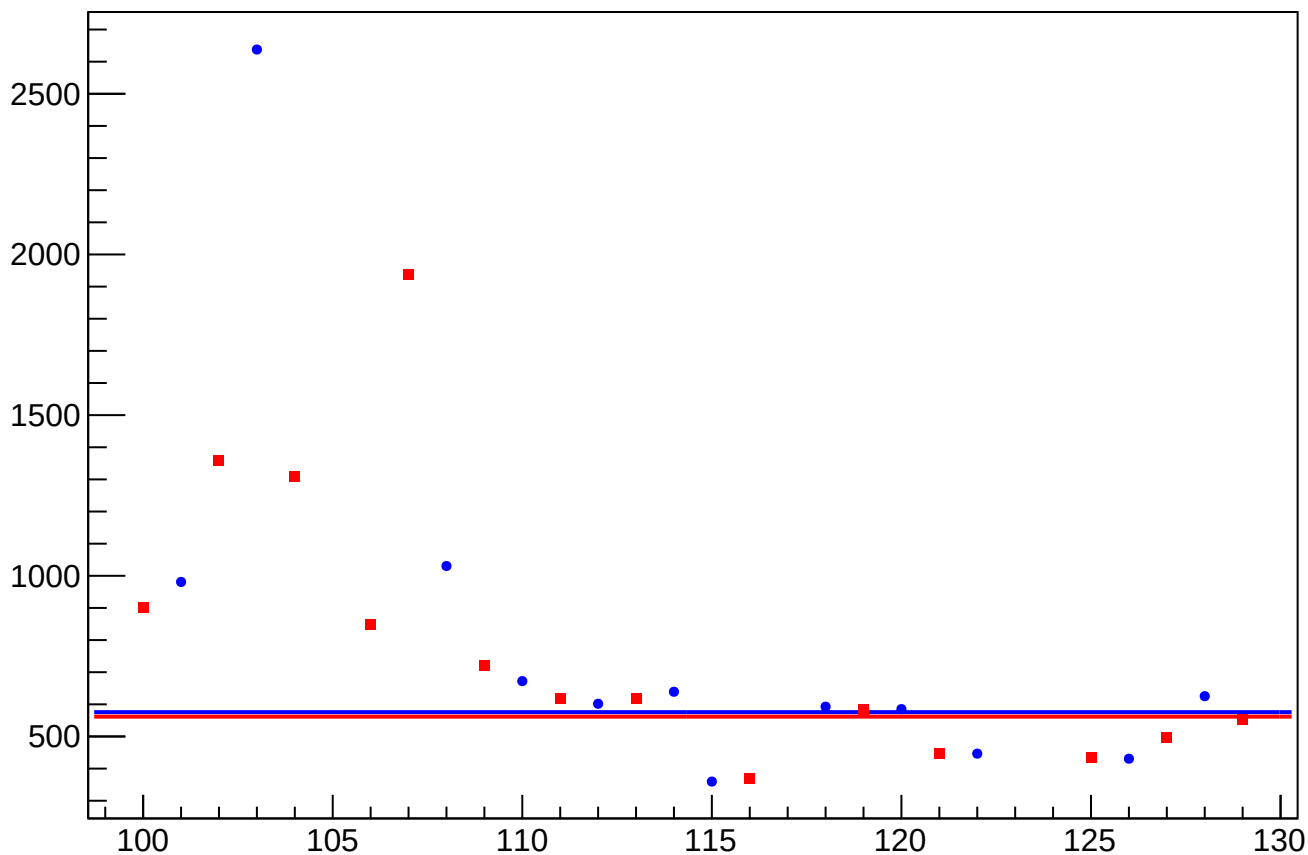
asym_usl_atl1_dd_reg_correction_rms vs Slug, Sign Corrected
