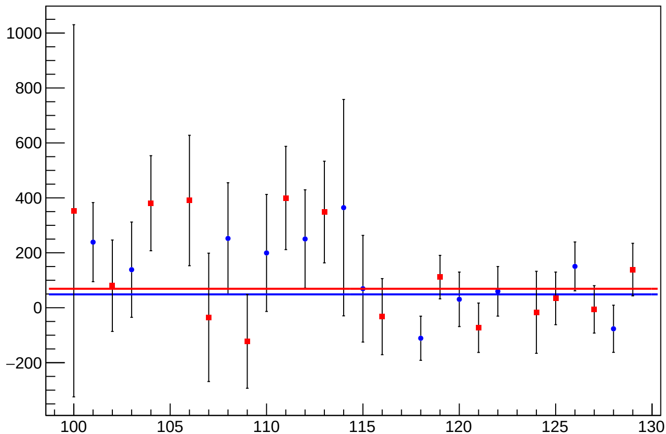
eigen_cor_asym_sam_1526_avg_mean vs Slug, Sign Corrected
