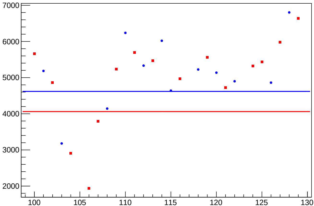
asym_usr_atr2_avg_reg_correction_rms vs Slug, Sign Corrected
