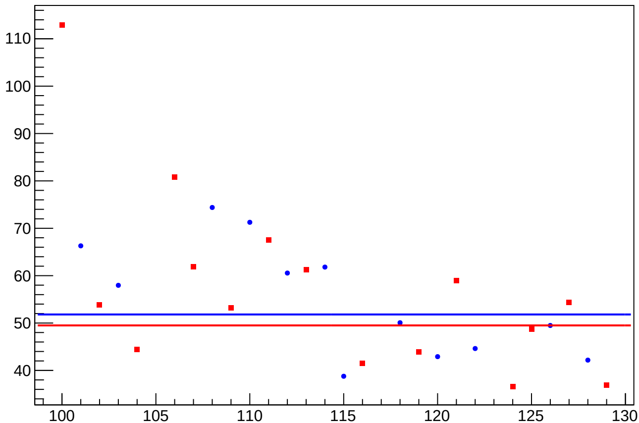
asym_sam_2468_avg_eigen_dit_vs_cor_diff_rms vs Slug, Sign Corrected
