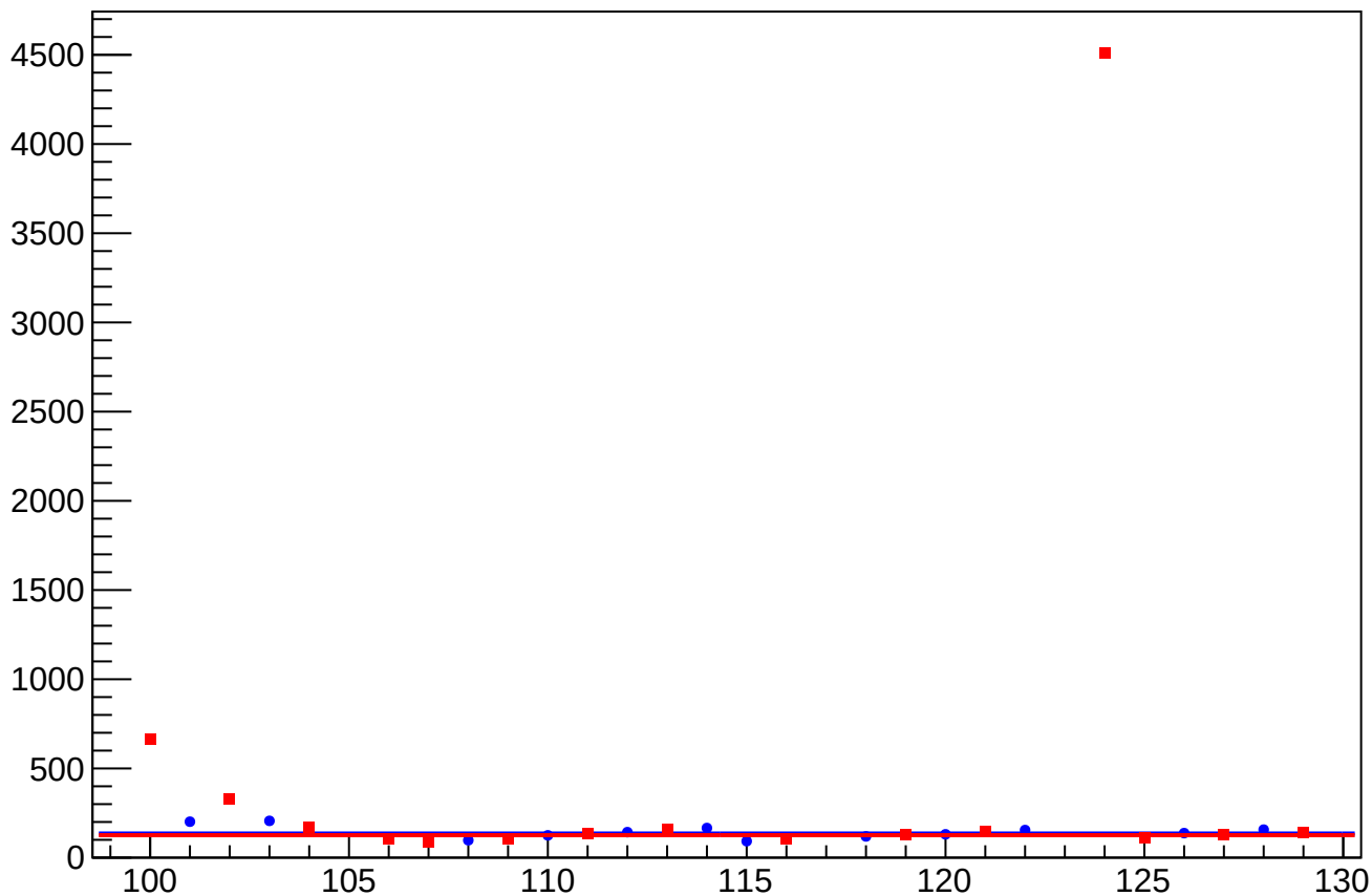
asym_atl1r2_dd_atl2r1_dd_dd_dit_vs_cor_diff_rms vs Slug, Sign Corrected
