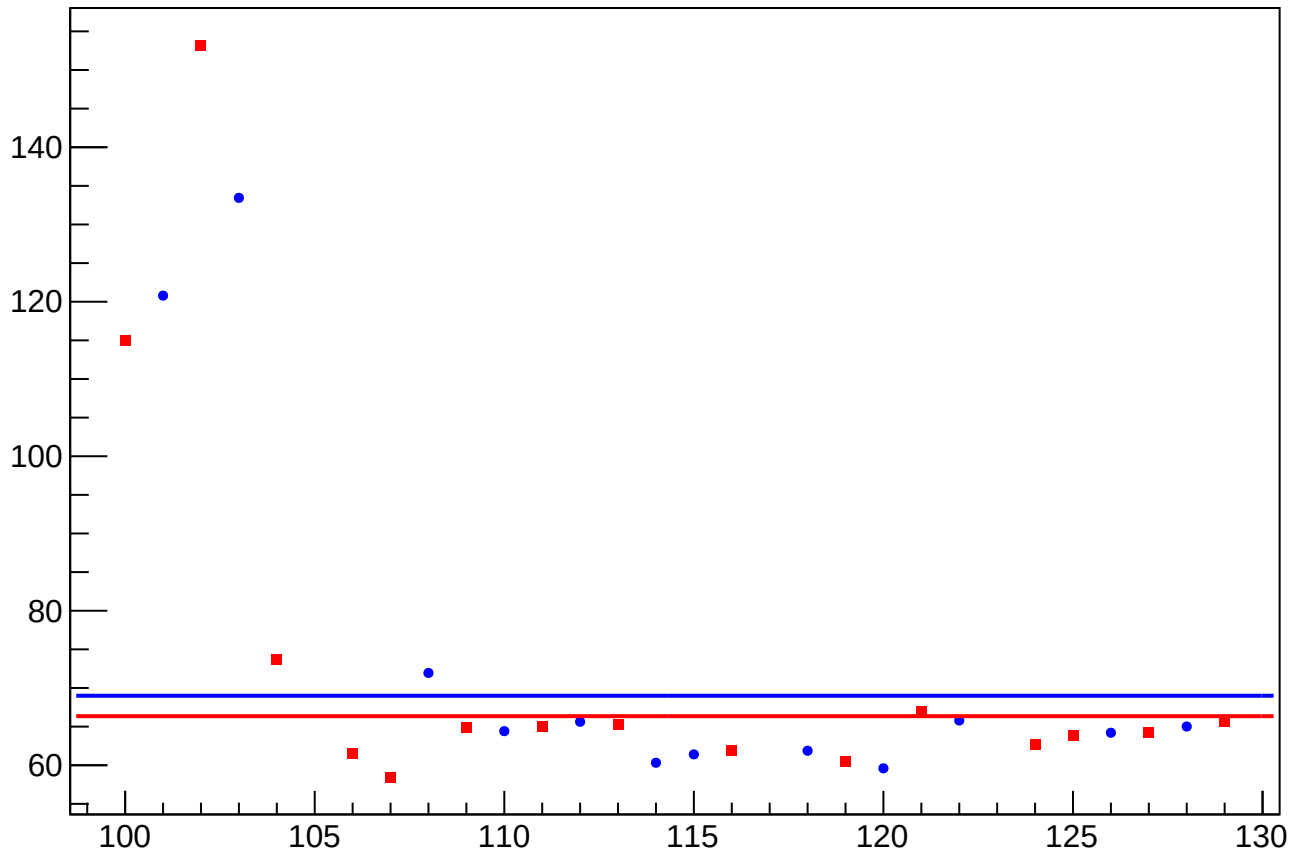
eigen_cor_asym_sam7_rms vs Slug, Sign Corrected
