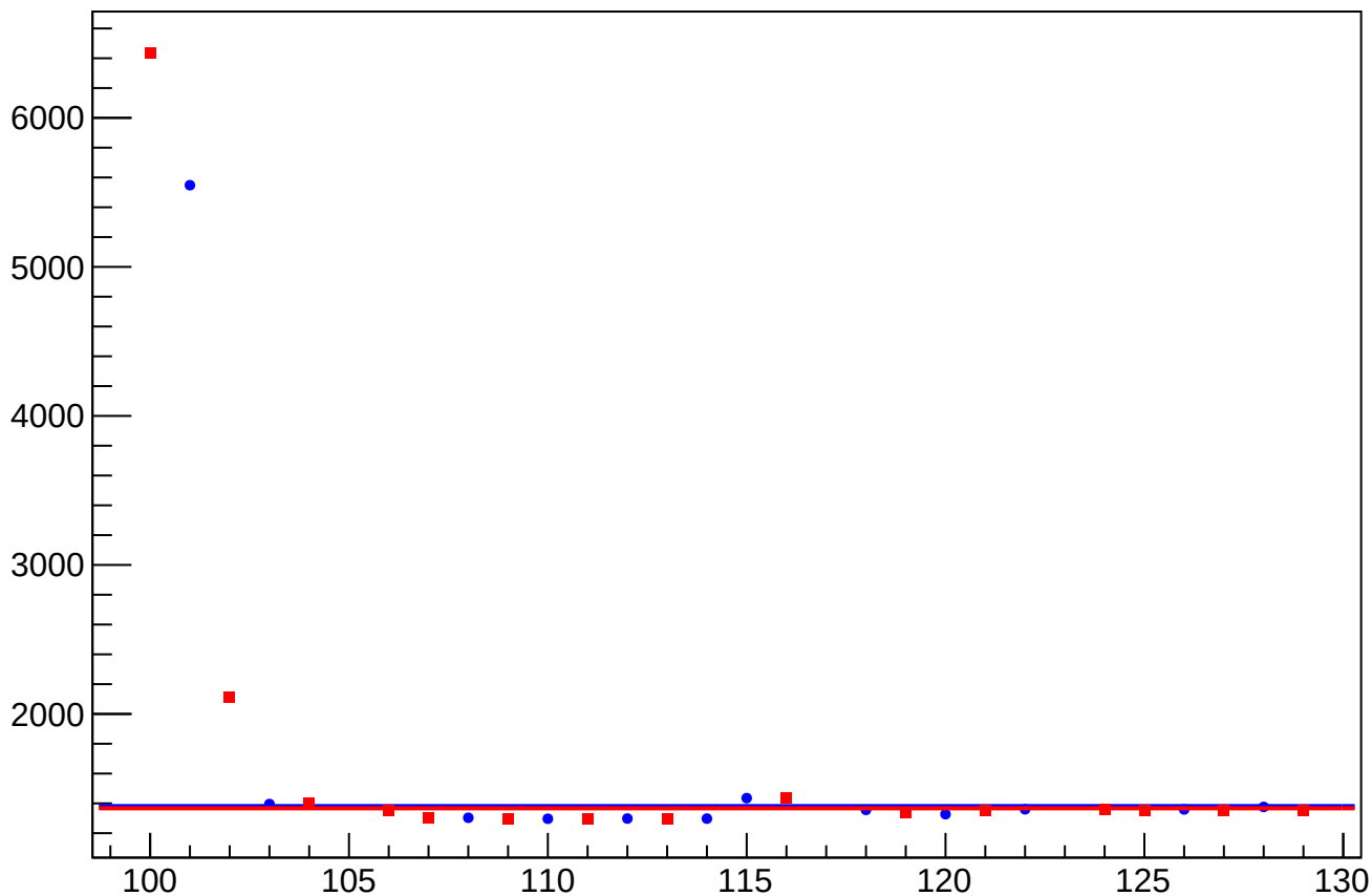
eigen_dit_asym_usr_atr1_dd_rms vs Slug, Sign Corrected
