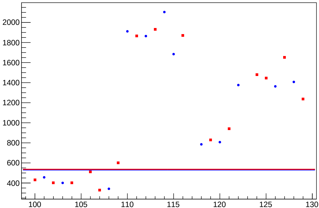
diff_bpm_4aX_4eX_dd_rms vs Slug, Sign Corrected
