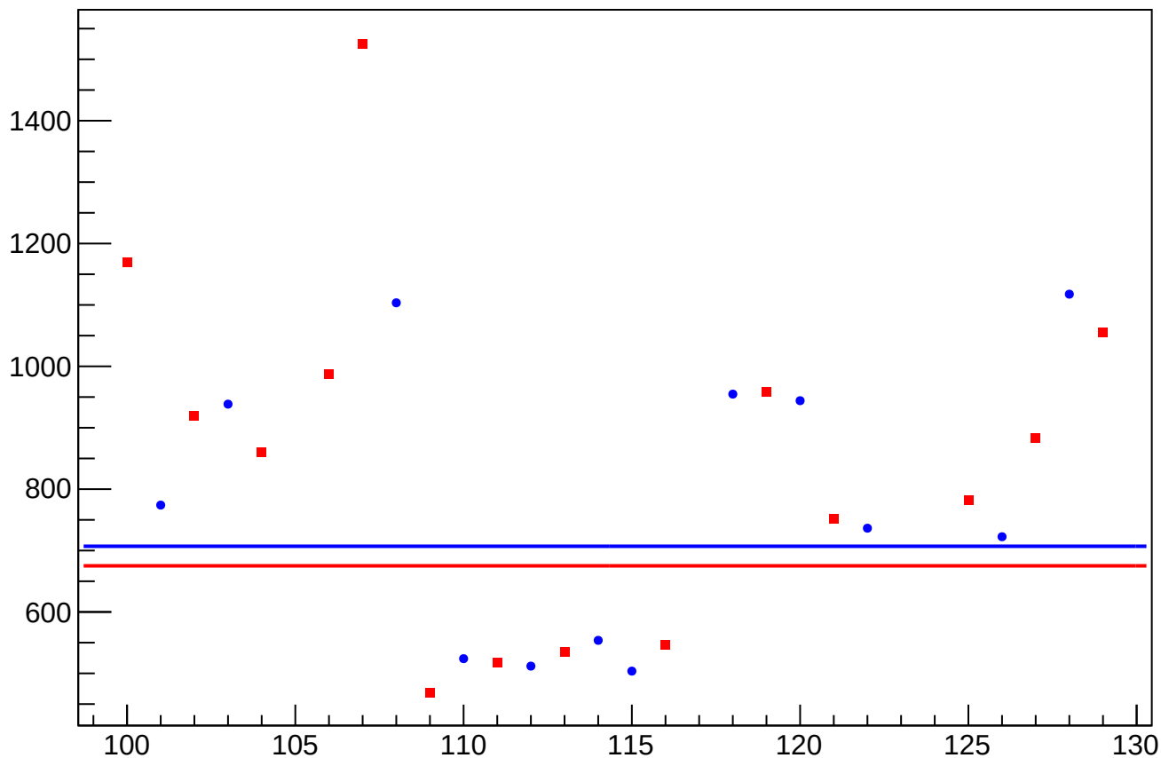
asym_us_dd_overload_cor_correction_rms vs Slug, Sign Corrected
