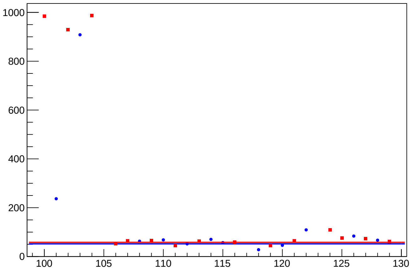
asym_atr1_dit_vs_cor_diff_rms vs Slug, Sign Corrected
