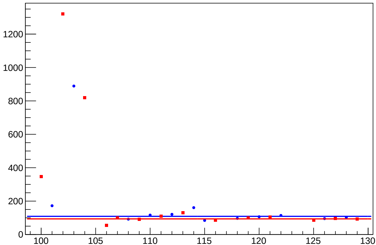
asym_us_avg_atlr_avg_dd_dit_vs_eigen_cor_diff_rms vs Slug, Sign Corrected
