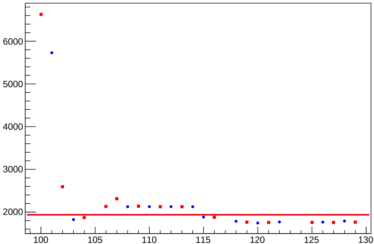
reg_asym_us_dd_at1lr_dd_dd_rms vs Slug, Sign Corrected
