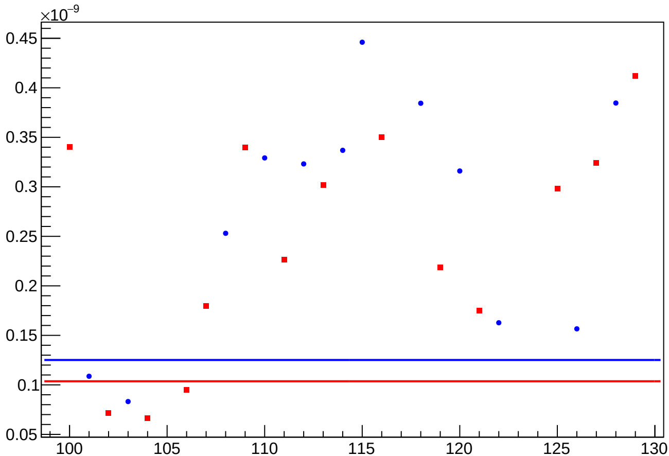
asym_us_avg_atlr_avg_avg_reg_vs_cor_diff_rms vs Slug, Sign Corrected
