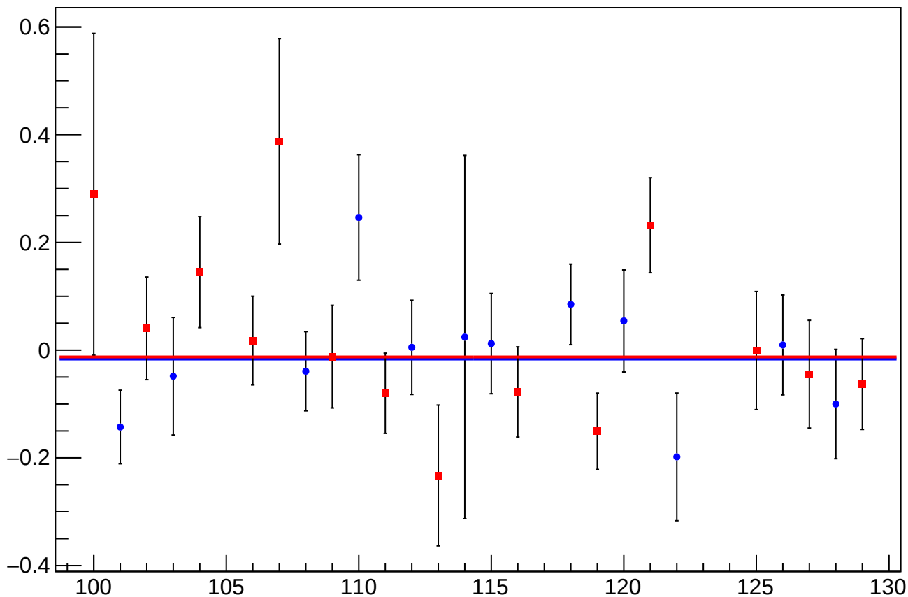
asym_us_avg_eigen_dit_vs_cor_diff_mean vs Slug, Sign Corrected
