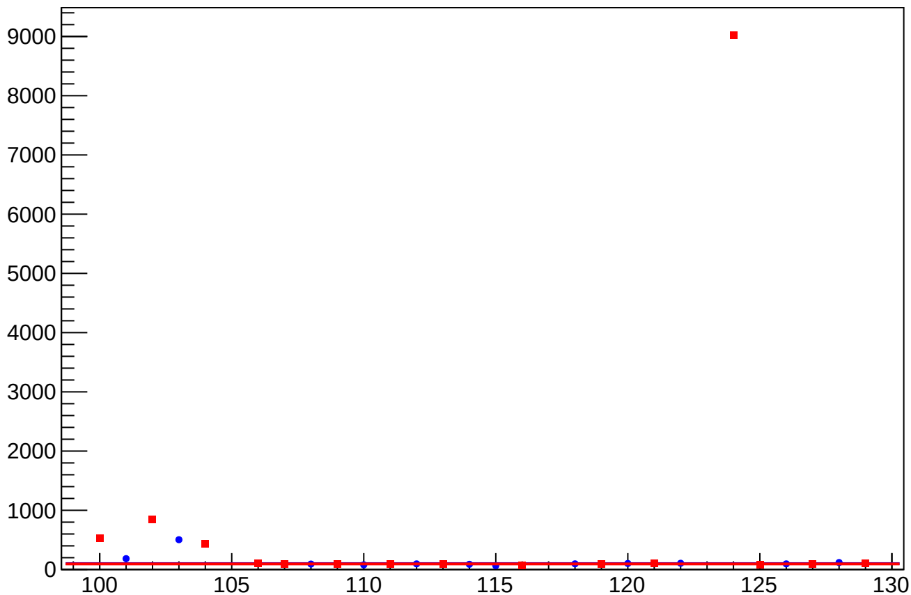
asym_atl_dd_eigen_dit_vs_eigen_cor_diff_rms vs Slug, Sign Corrected
