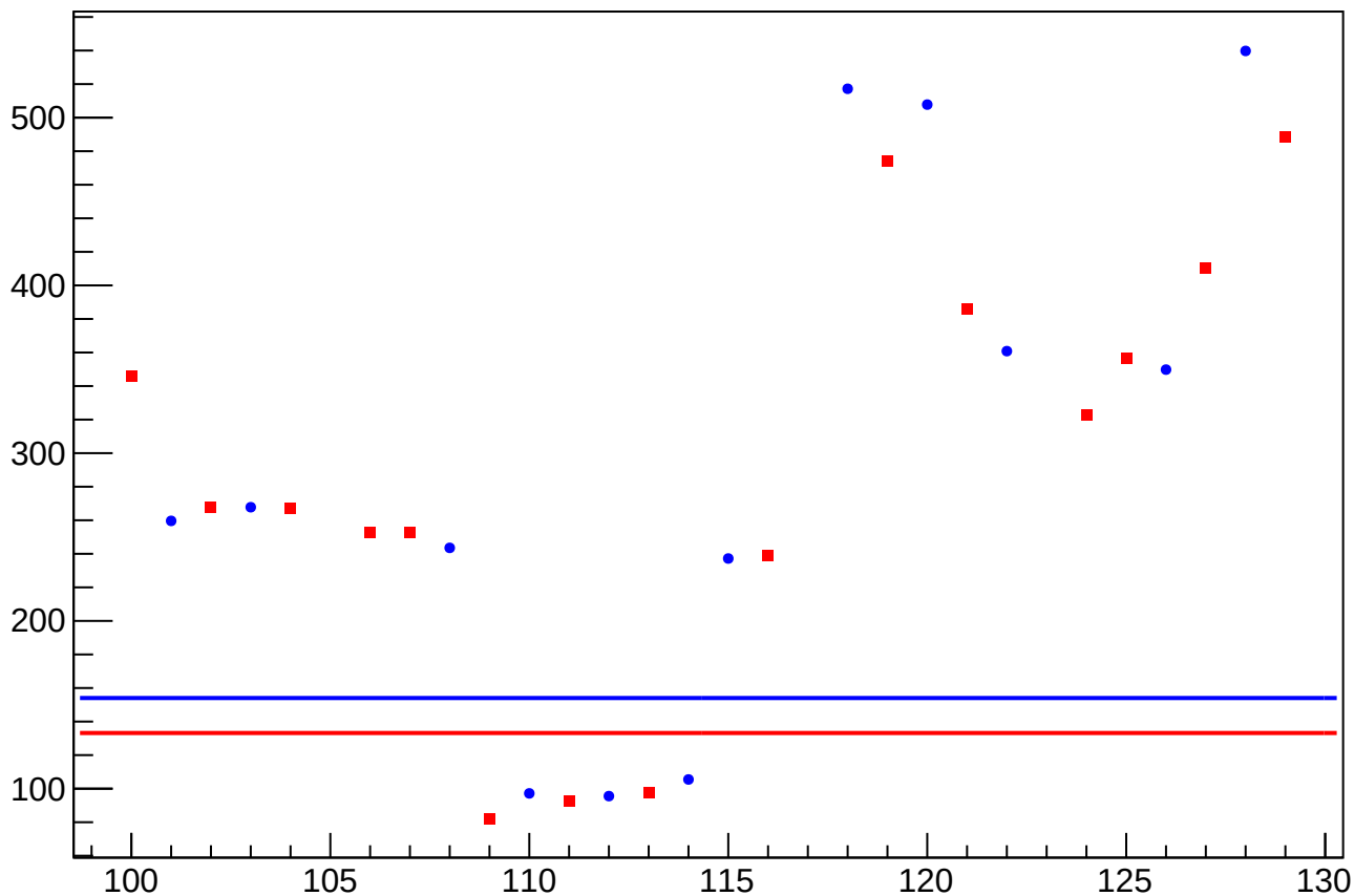
asym_sam8_dit_correction_rms vs Slug, Sign Corrected
