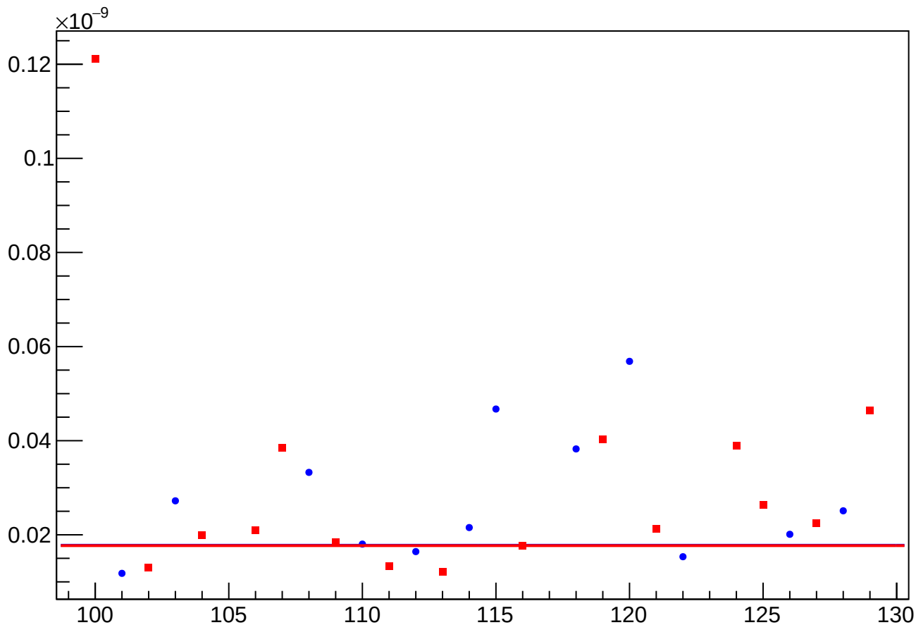
asym_sam_15_37_dd_reg_vs_cor_diff_rms vs Slug, Sign Corrected
