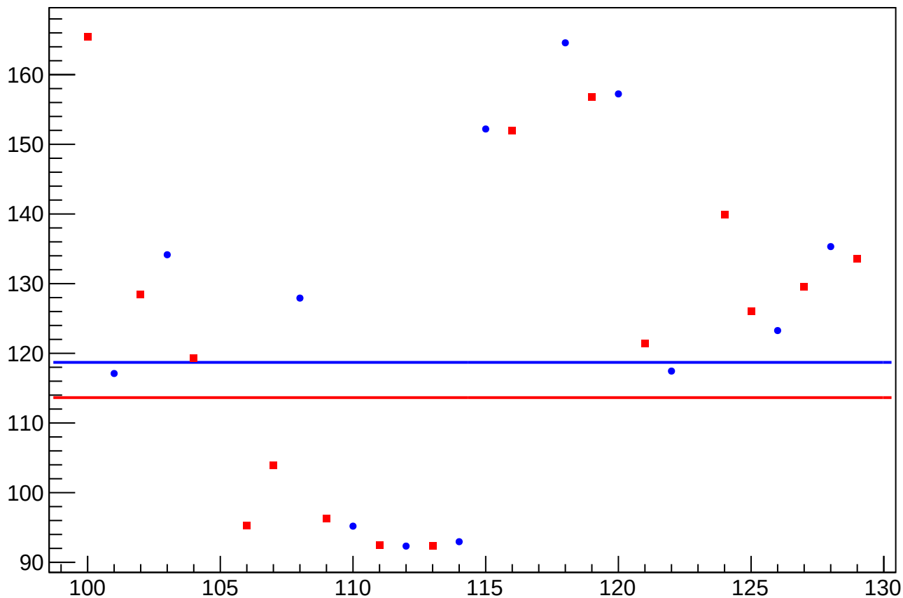
eigen_dit_asym_sam_48_dd_rms vs Slug, Sign Corrected
