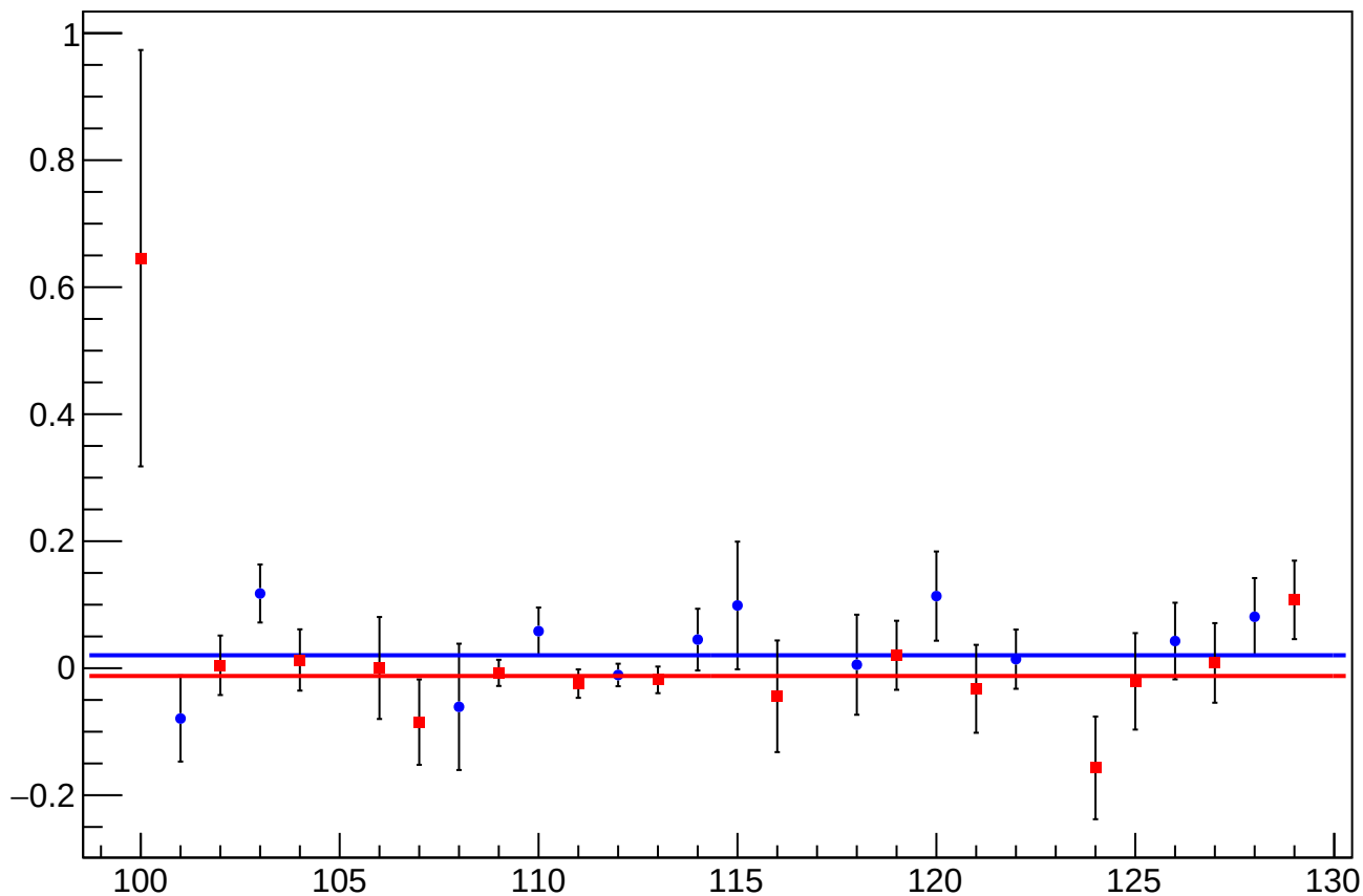
asym_sam_48_dd_eigen_dit_vs_eigen_cor_diff_mean vs Slug, Sign Corrected
