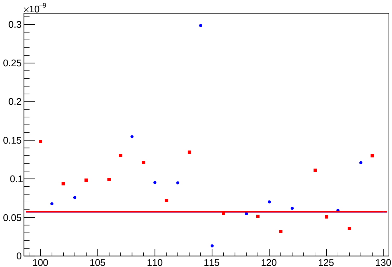
asym_sam_26_avg_reg_vs_cor_diff_rms vs Slug, Sign Corrected
