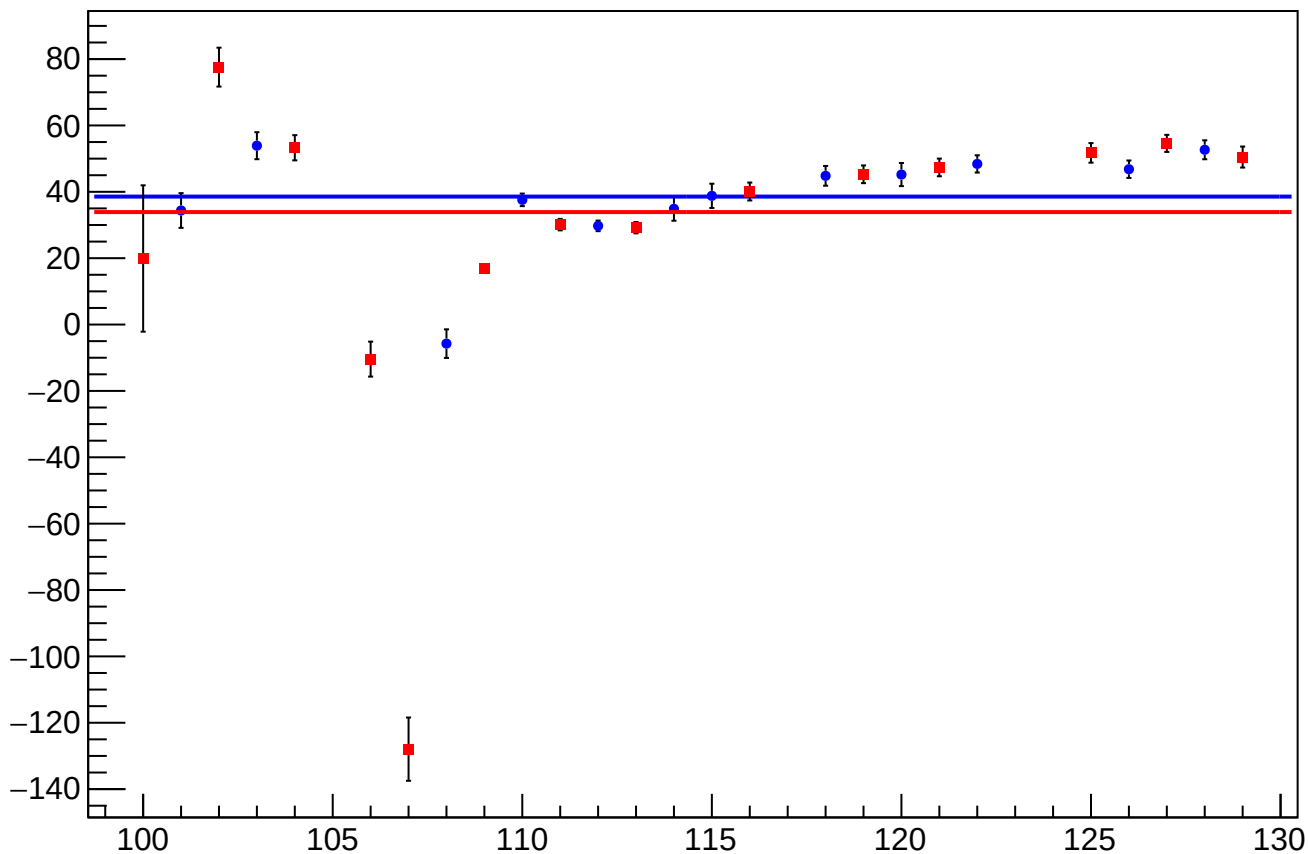
reg_asym_us_dd_atlr_dd_avg_diff_bpm1X_slope vs Slug, Sign Corrected
