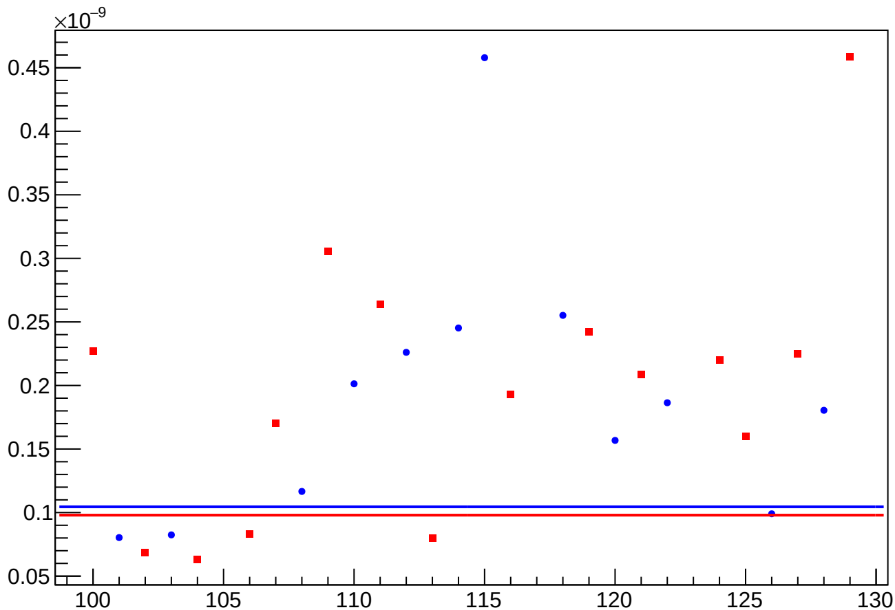
asym_atr_dd_reg_vs_cor_diff_rms vs Slug, Sign Corrected
