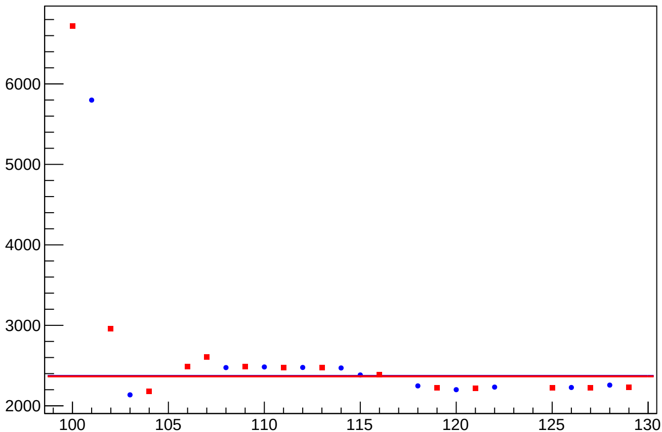
reg_asym_us_avg_at1lr_avg_avg_rms vs Slug, Sign Corrected
