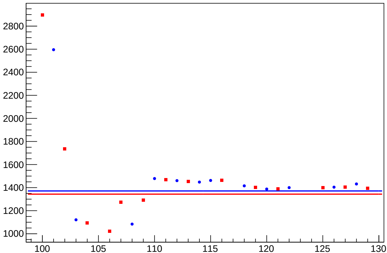
reg_asym_us_dd_at2lr_dd_dd_rms vs Slug, Sign Corrected
