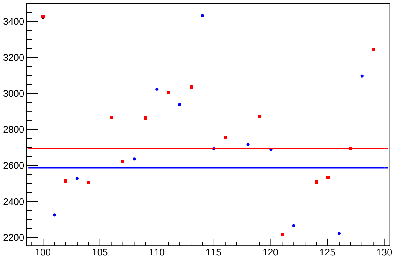
asym_sam_26_dd_reg_correction_rms vs Slug, Sign Corrected
