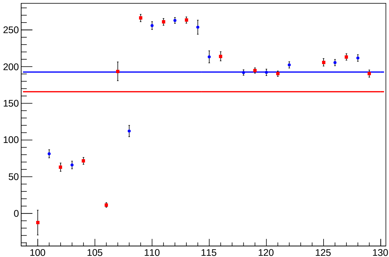
reg_asym_usl_atl2_avg_diff_bpm4eX_slope vs Slug, Sign Corrected
