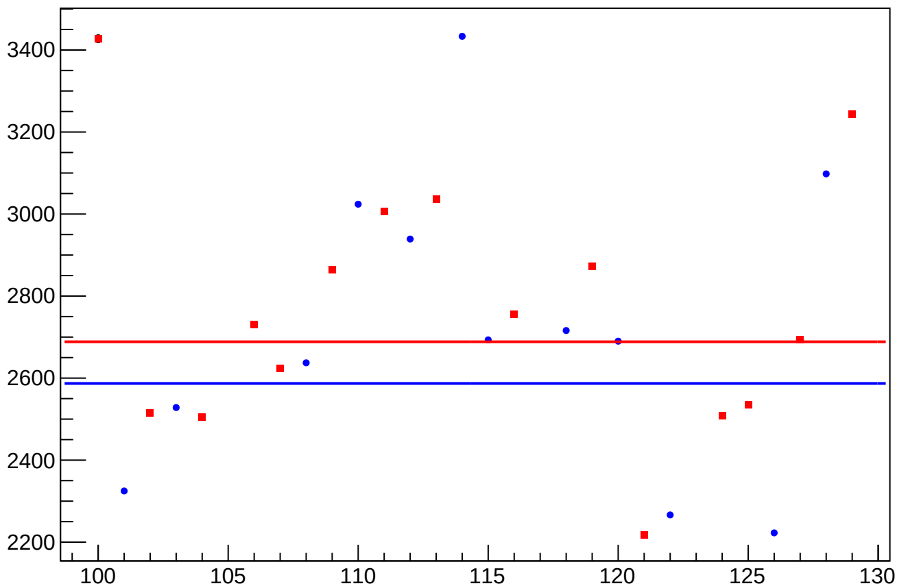
asym_sam_26_dd_eigen_cor_correction_rms vs Slug, Sign Corrected
