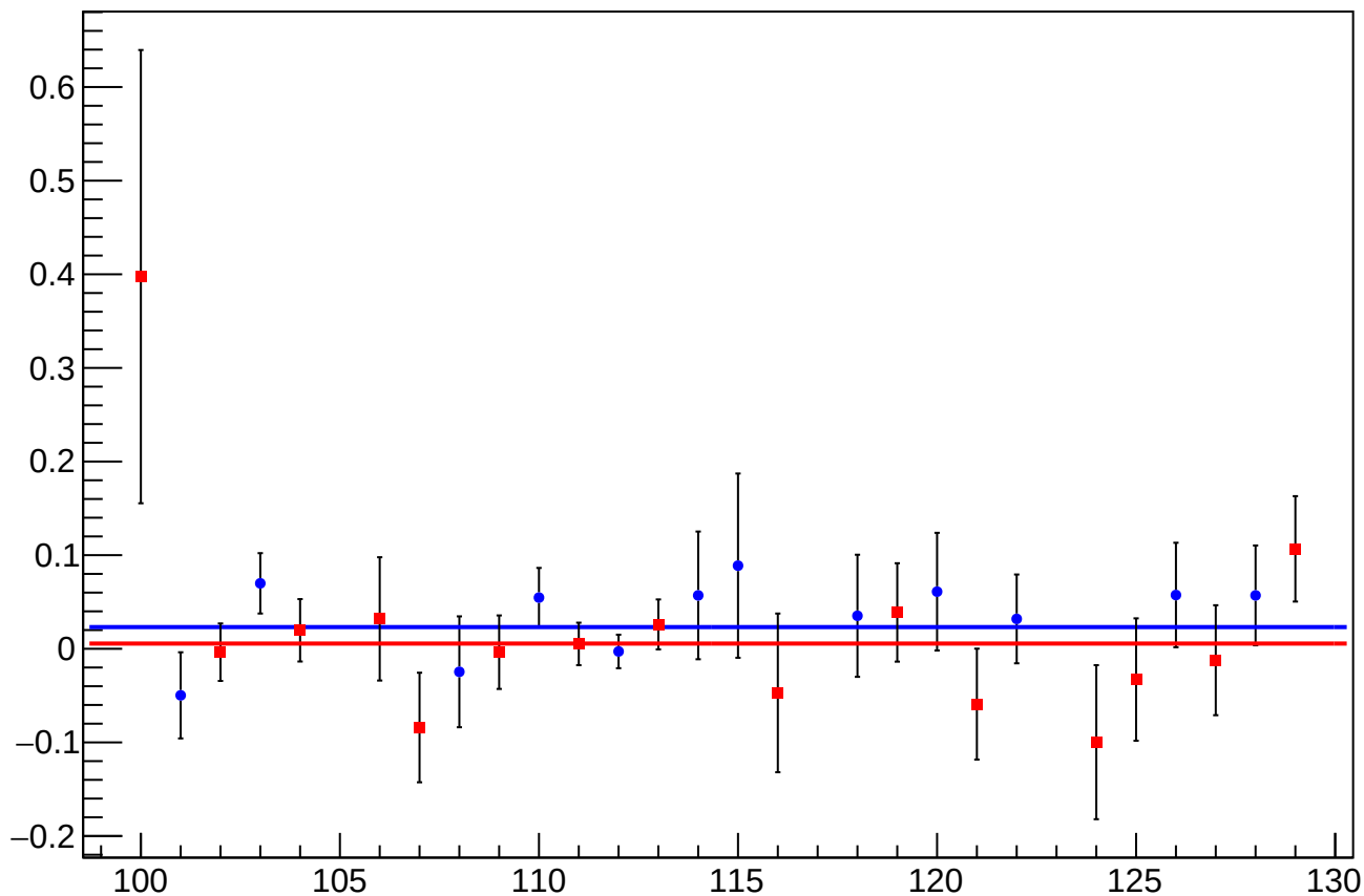
asym_sam_1548_avg_dit_vs_eigen_cor_diff_mean vs Slug, Sign Corrected
