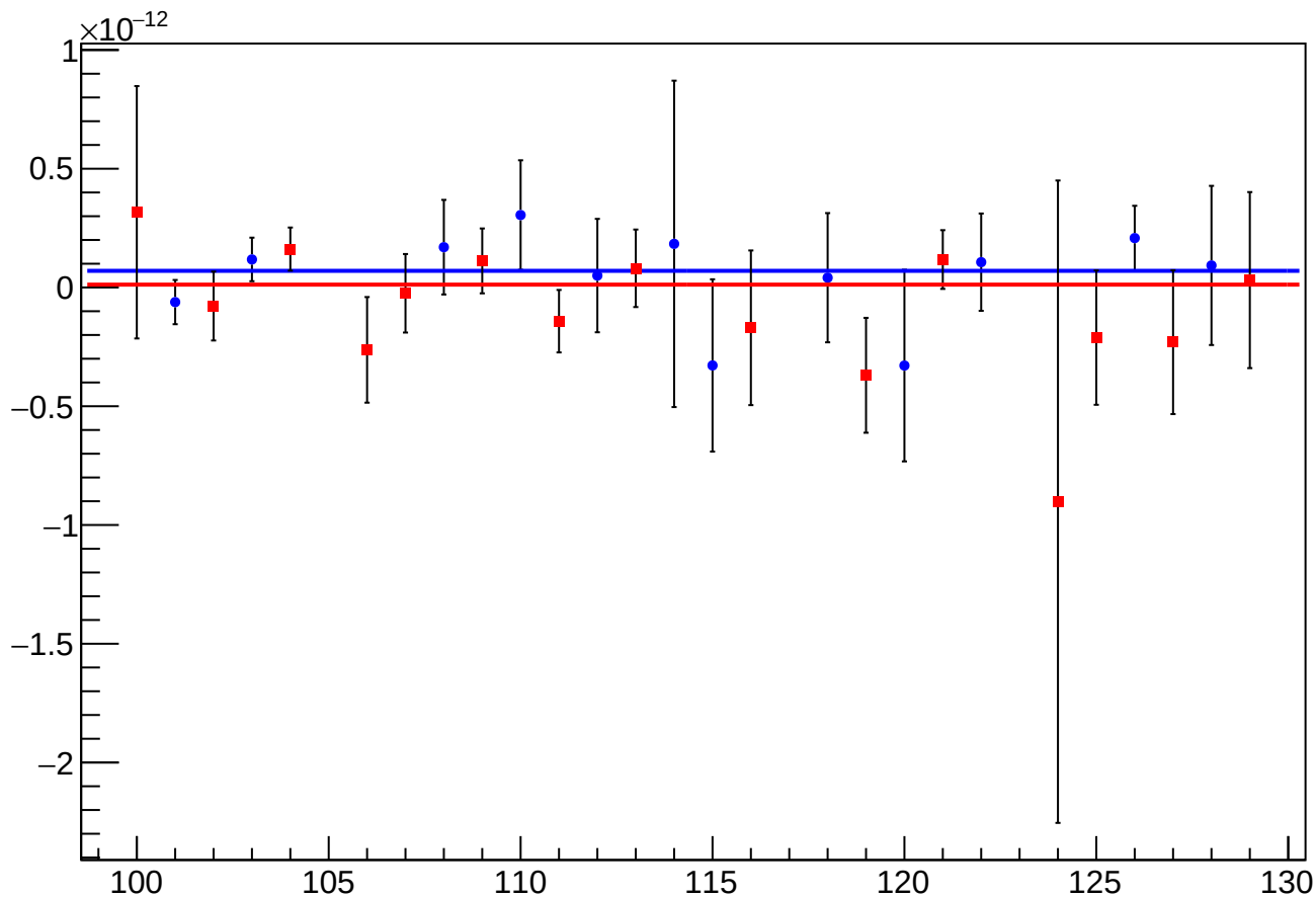
asym_at2_dd_reg_vs_cor_diff_mean vs Slug, Sign Corrected
