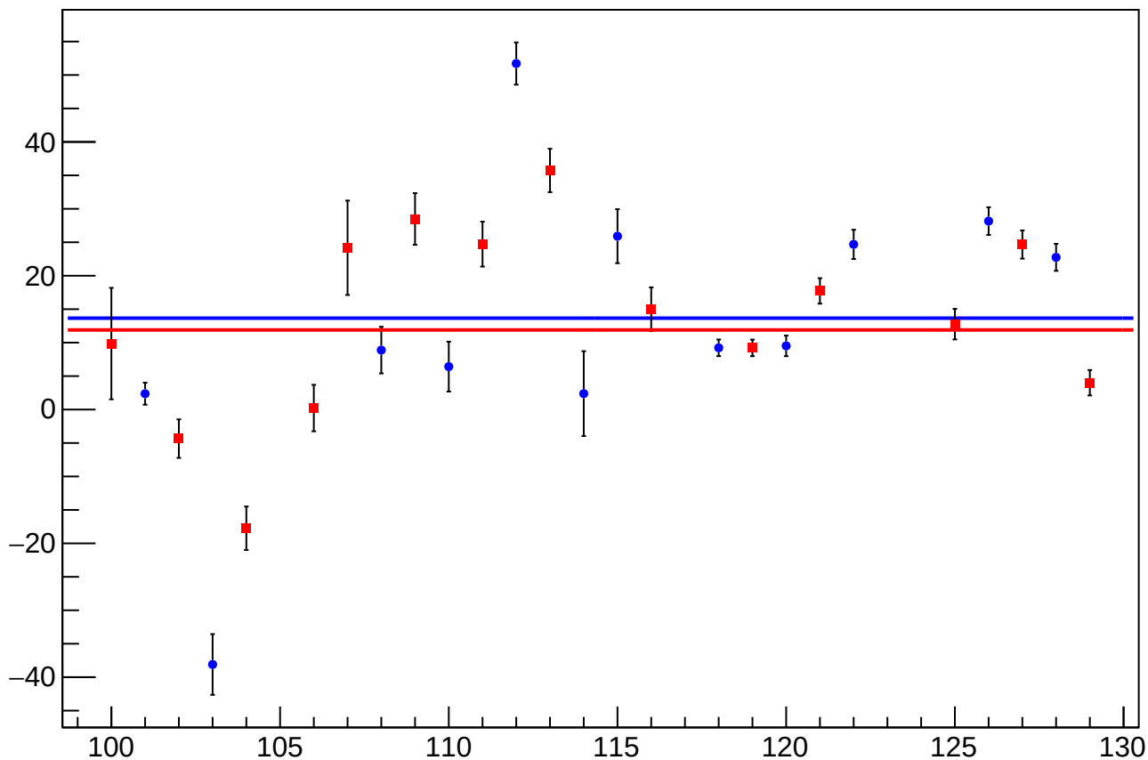
reg_asym_usl_atl1_avg_diff_bpm4aY_slope vs Slug, Sign Corrected
