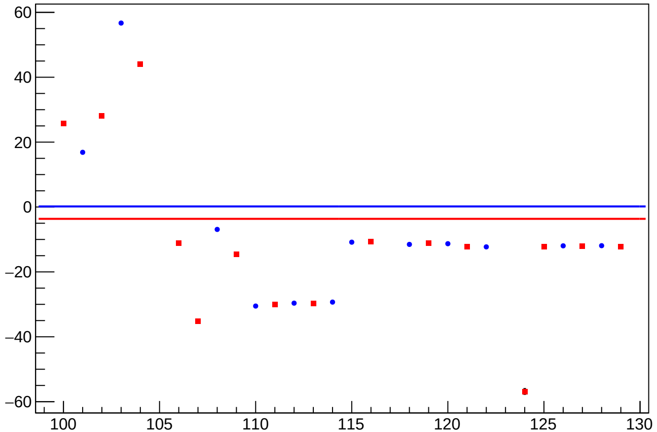
reg_asym_at1_dd_at2_dd_avg_diff_bpm12X_slope vs Slug, Sign Corrected
