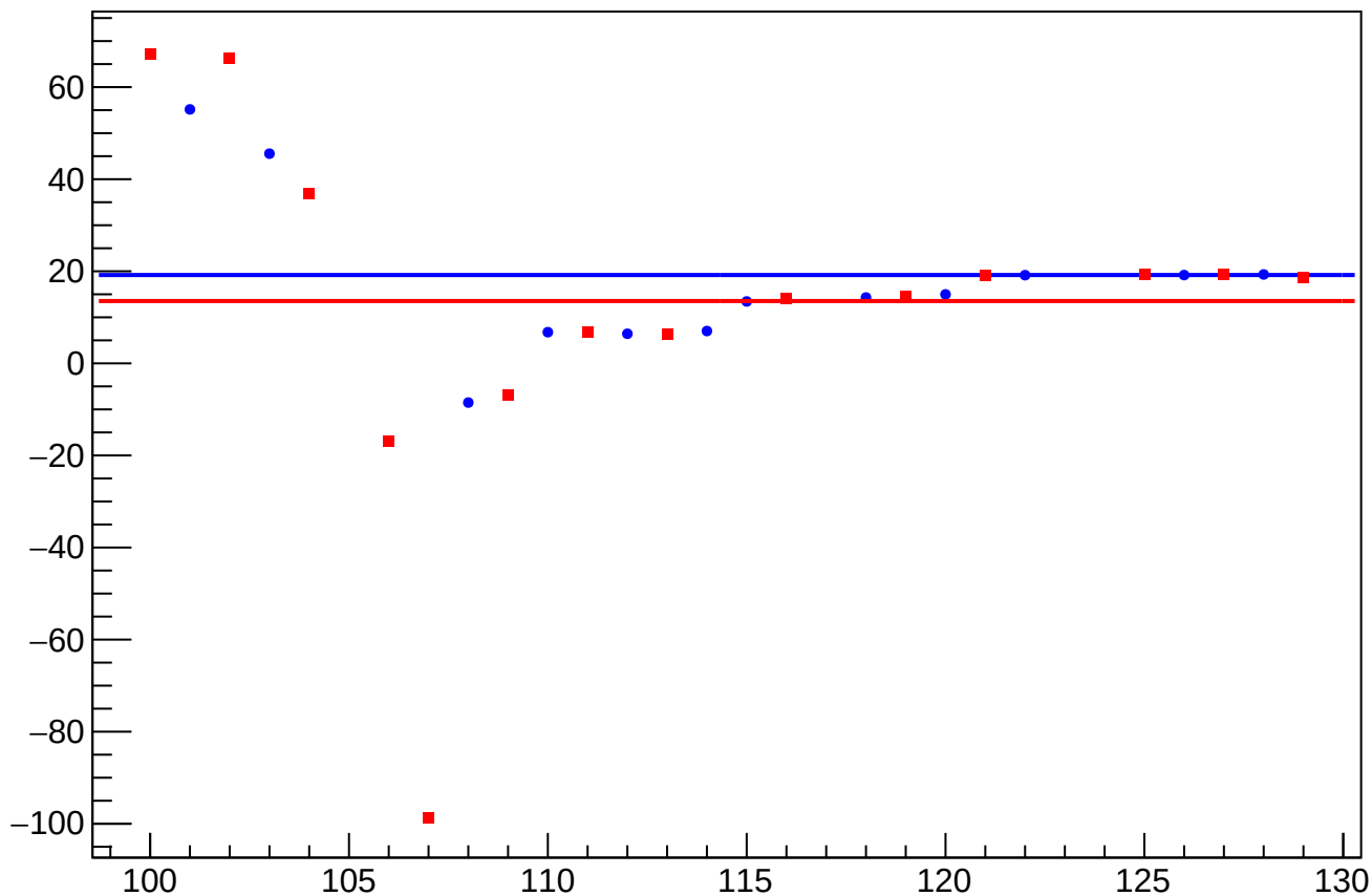
reg_asym_us_dd_atlr_dd_avg_diff_bpm12X_slope vs Slug, Sign Corrected
