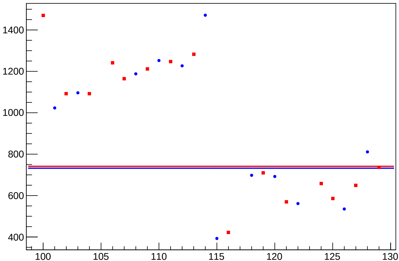
asym_sam_1526_avg_eigen_cor_correction_rms vs Slug, Sign Corrected
