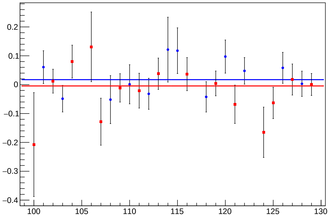
asym_sam_12345678_avg_eigen_dit_vs_eigen_cor_diff_mean vs Slug, Sign Corrected
