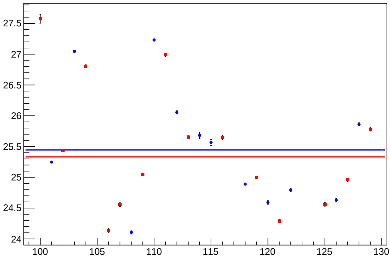
asym_bcm_dg_us_dg_ds_dd_rms vs Slug, Sign Corrected
