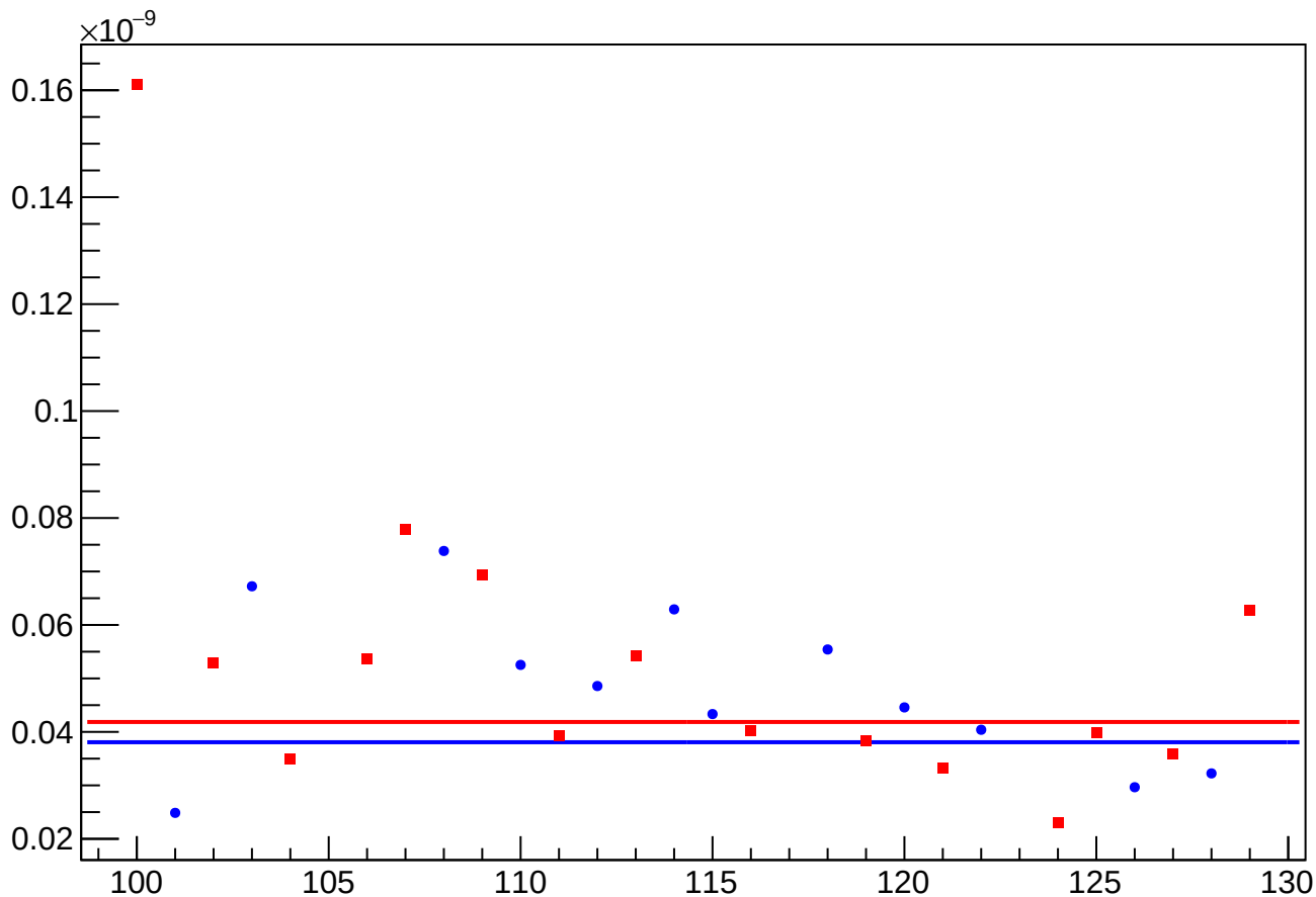
asym_sam_3726_avg_eigen_cor_vs_cor_diff_rms vs Slug, Sign Corrected
