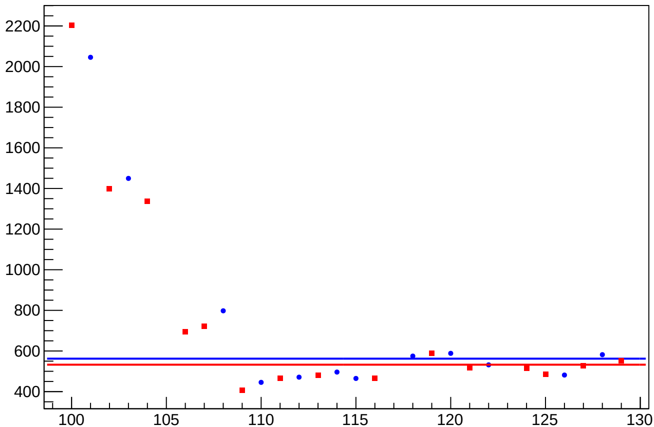
asym_atr1_dit_correction_rms vs Slug, Sign Corrected
