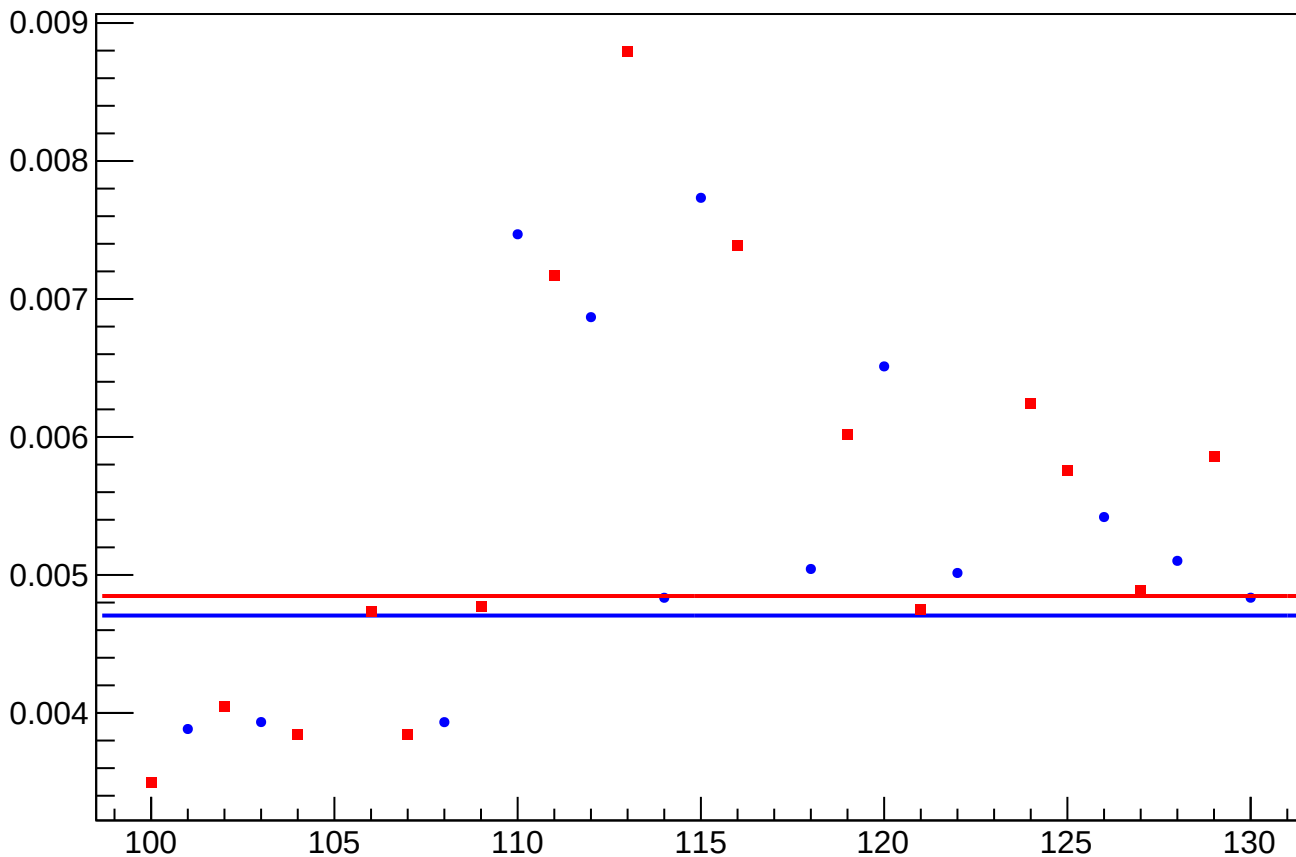
yield_bpm0l09Y_rms vs Slug, Sign Corrected
