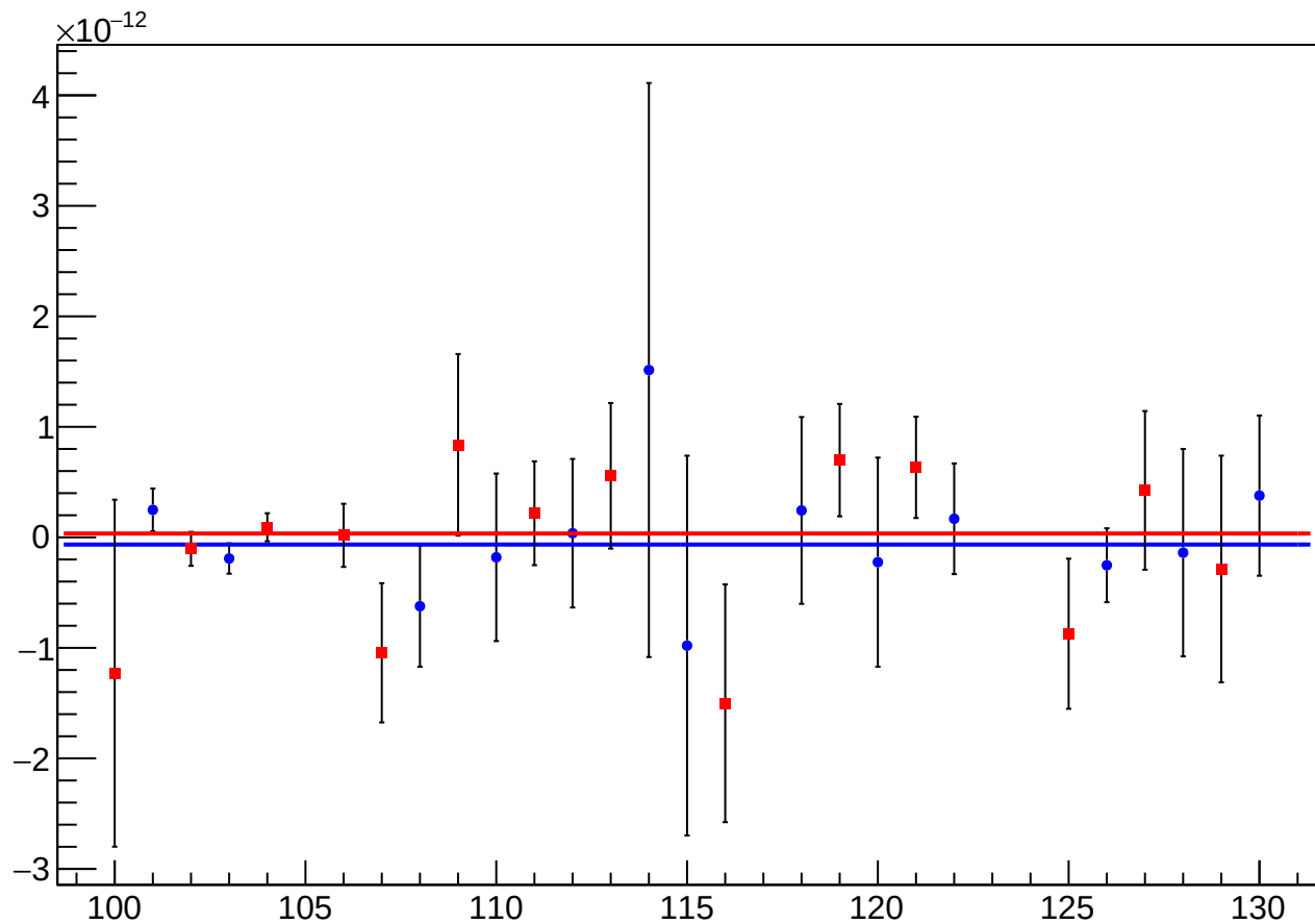
asym_us_atlr_avg_avg_reg_vs_cor_diff_mean vs Slug, Sign Corrected
