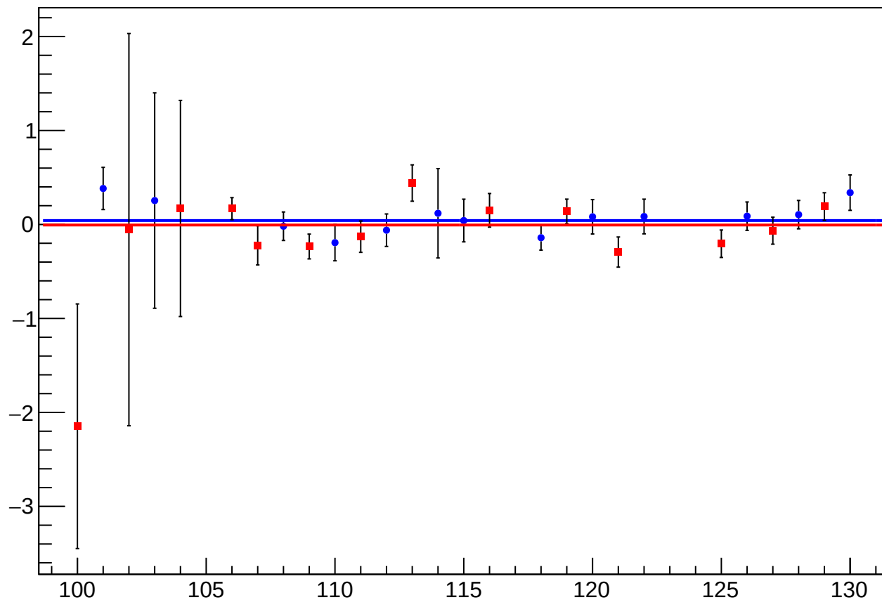
asym_us_avg_atlr_avg_dd_eigen_dit_vs_Slug, Sign Corrected
