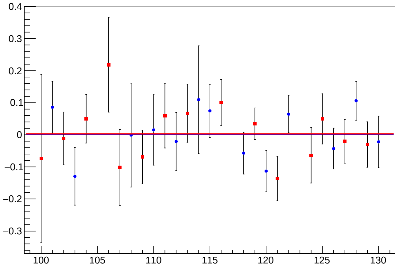
asym_sam_24_68_dd_eigen_dit_vs_eigen_cor_diff_mean vs Slug, Sign Corrected
