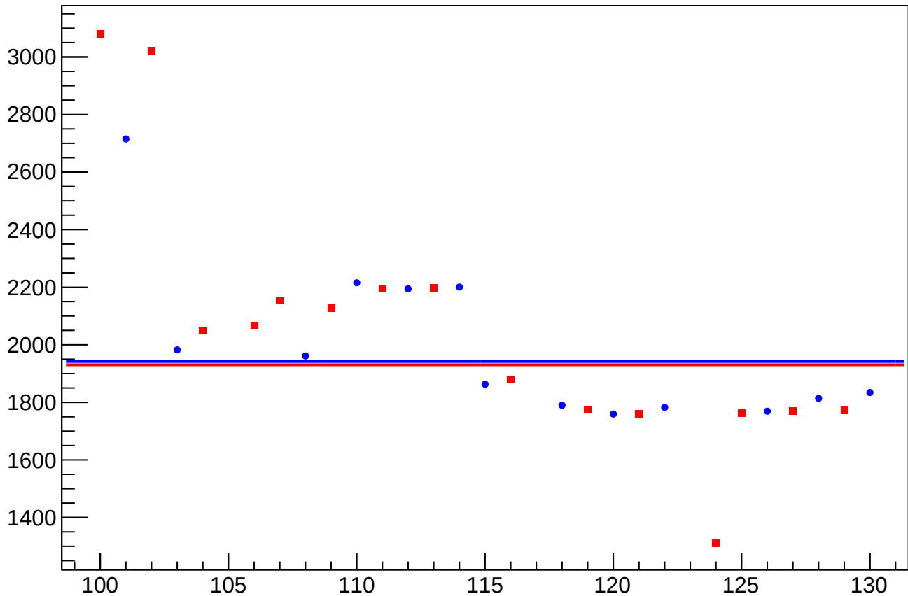
dit_asym_atl1r2_avg_rms vs Slug, Sign Corrected
