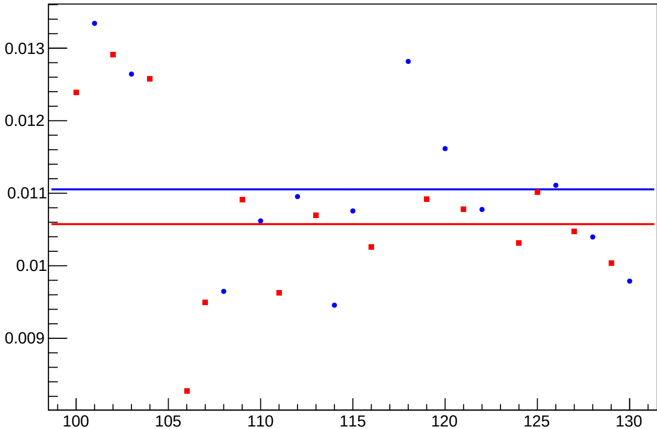
yield_bpm0l09X_rms vs Slug, Sign Corrected
