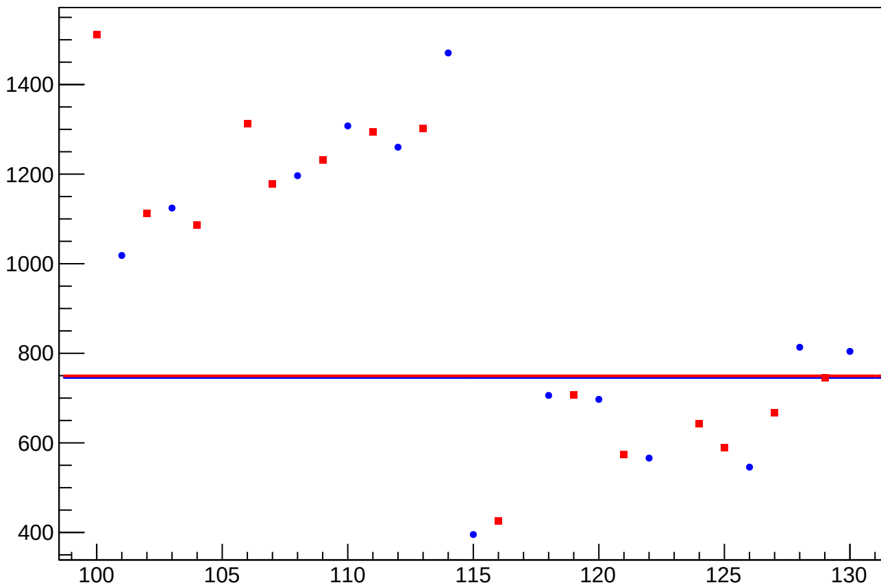
asym_sam_1526_avg_eigen_dit_correction_rms vs Slug, Sign Corrected
