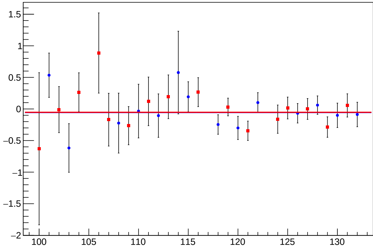
asym_sam2_eigen_dit_vs_eigen_cor_diff_mean vs Slug, Sign Corrected
