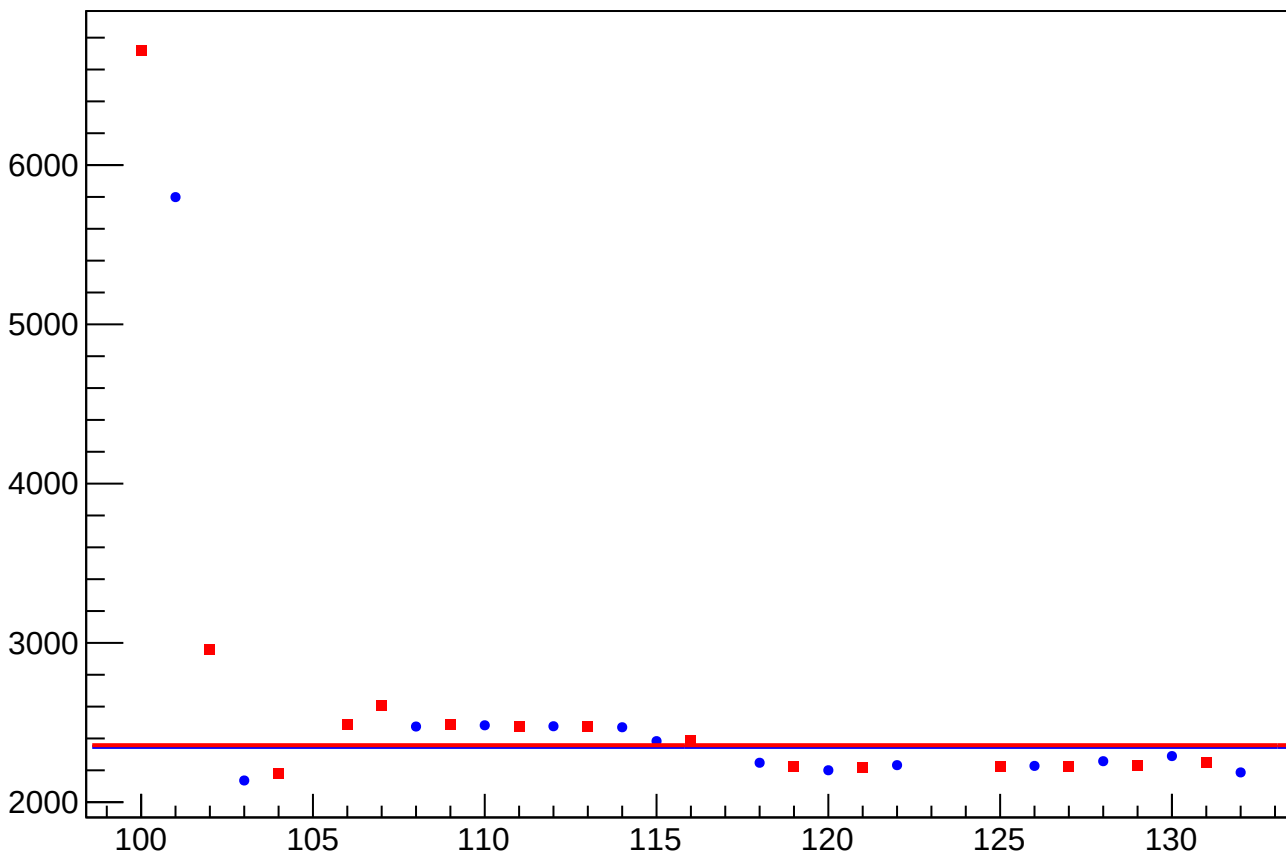
reg_asym_us_avg_at1lr_avg_avg_rms vs Slug, Sign Corrected
