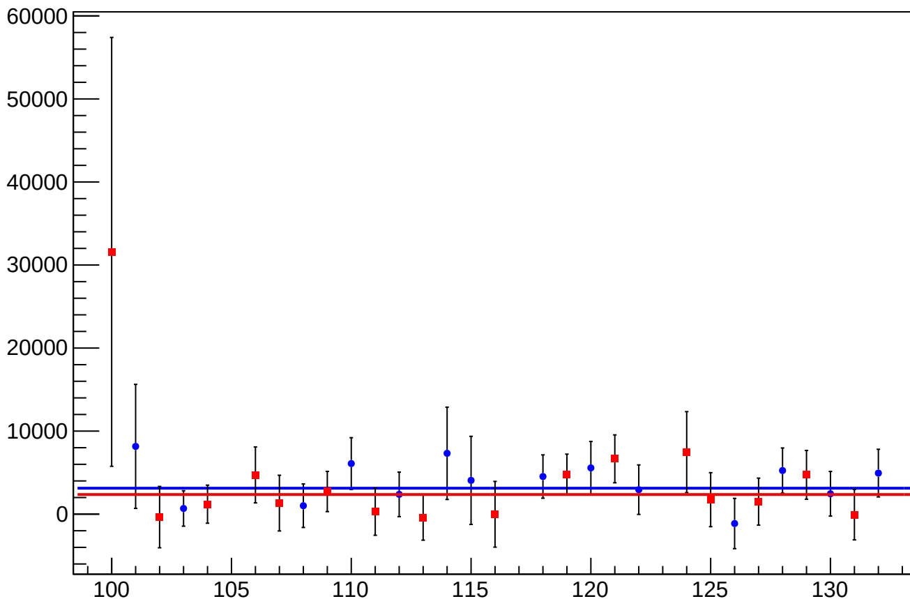
reg_asym_atr_avg_mean vs Slug, Sign Corrected
