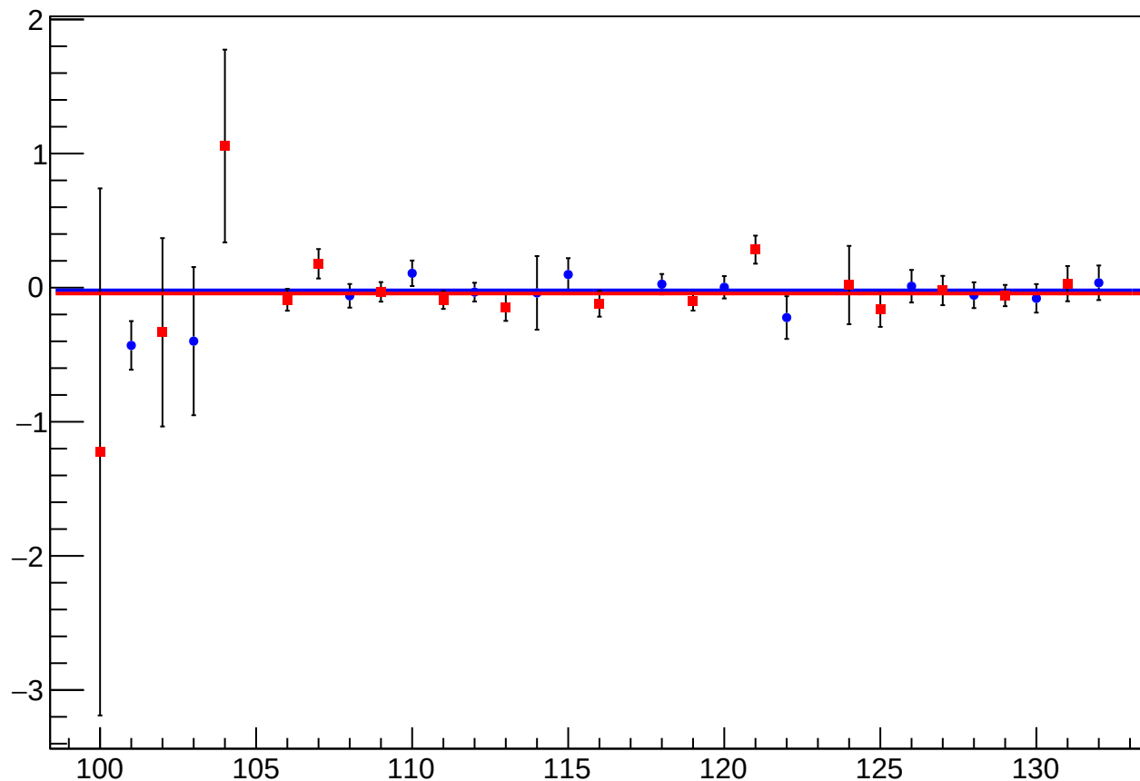
asym_usr_atr1_avg_dit_vs_cor_diff_mean vs Slug, Sign Corrected
