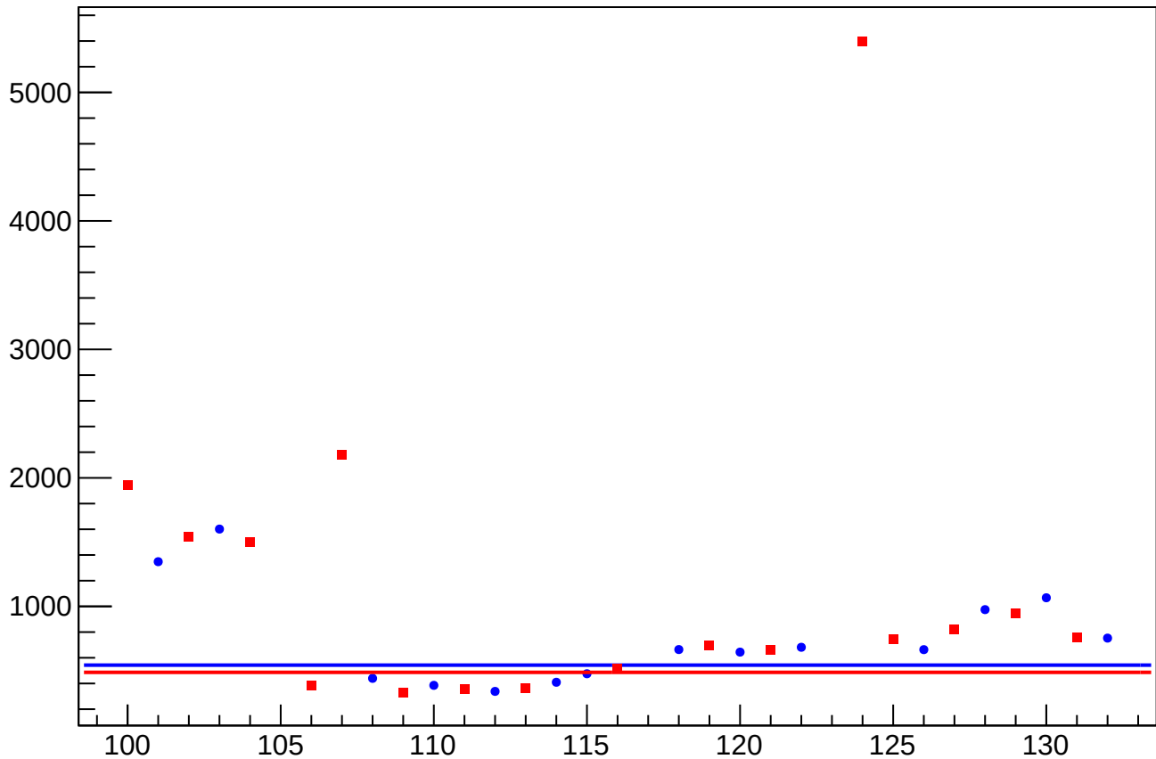
asym_atl_avg_atr_avg_dd_dit_correction_rms vs Slug, Sign Corrected
