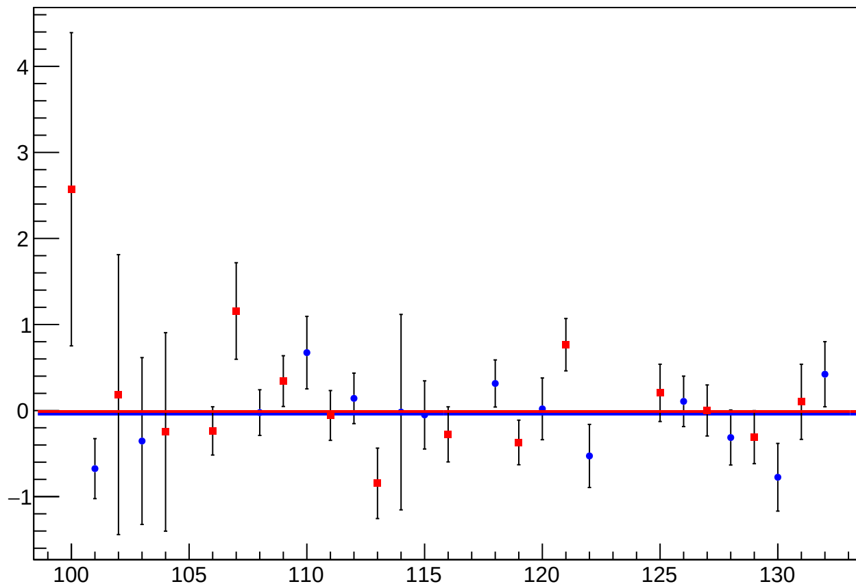
asym_us_atlr_avg_avg_eigen_dit_vs_cor_diff_mean vs Slug, Sign Corrected
