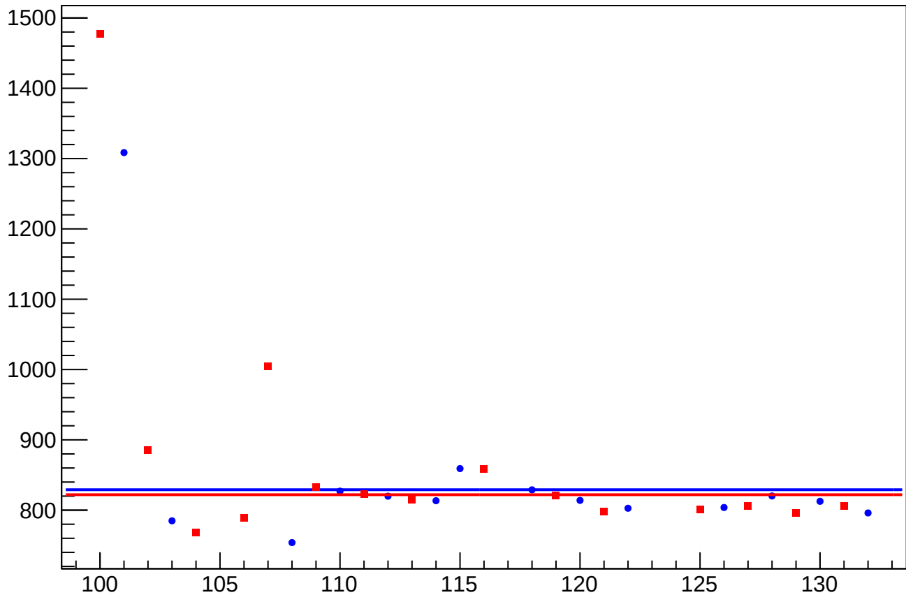
eigen_cor_asym_usl_atl2_dd_rms vs Slug, Sign Corrected
