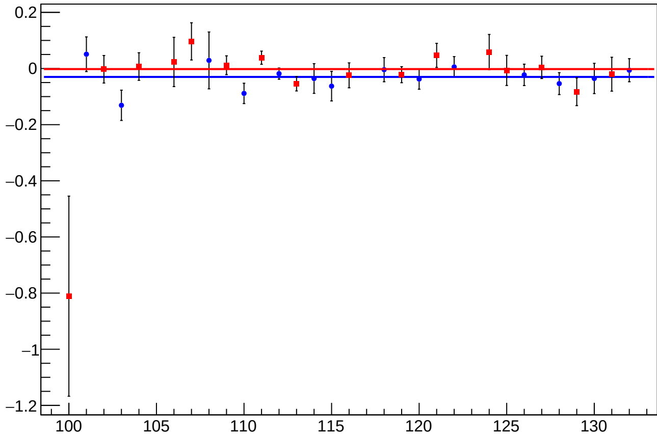
asym_sam_15_48_dd_eigen_dit_vs_cor_diff_mean vs Slug, Sign Corrected
