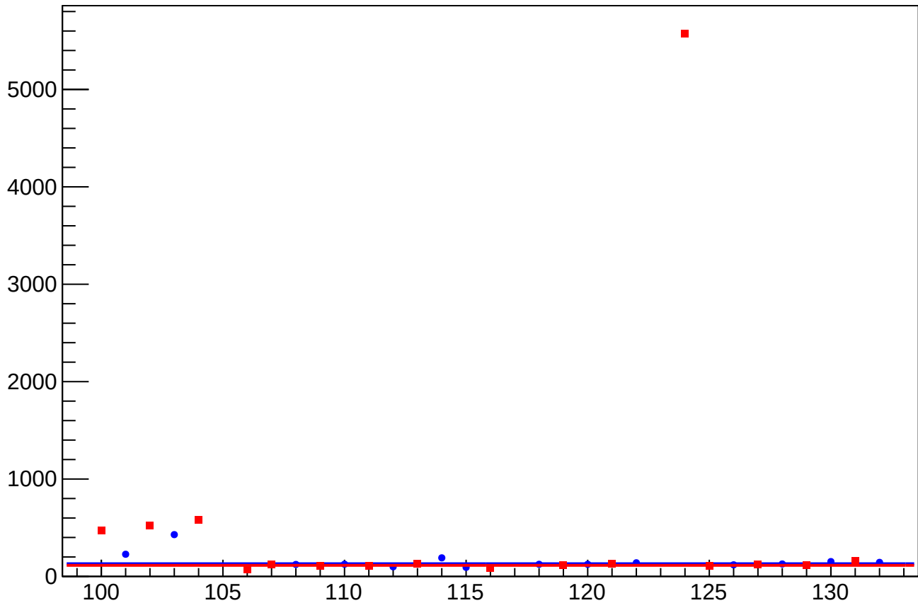
asym_atr1l2_avg_eigen_dit_vs_cor_diff_rms vs Slug, Sign Corrected
