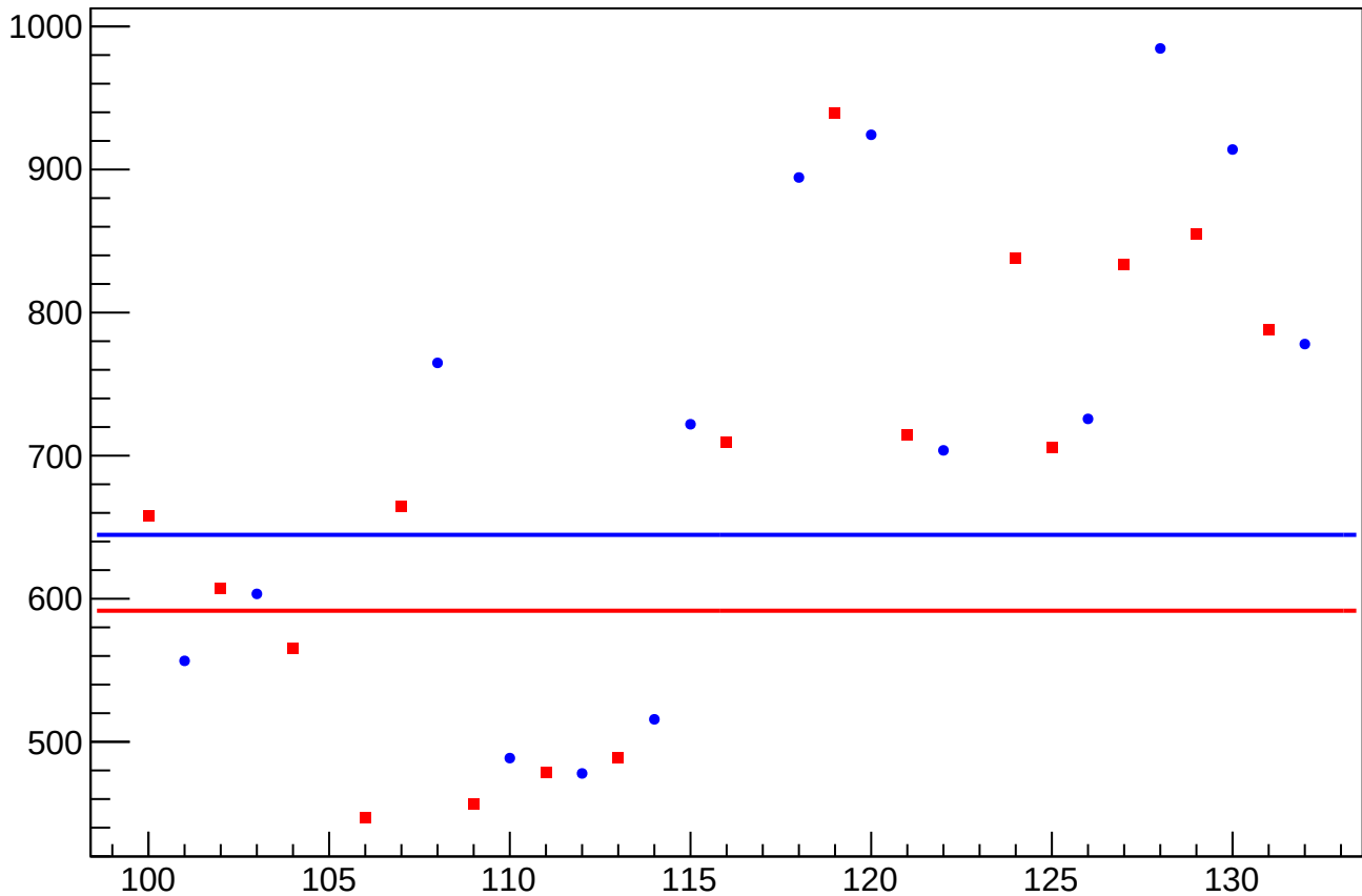
asym_sam_15_48_dd_reg_correction_rms vs Slug, Sign Corrected
