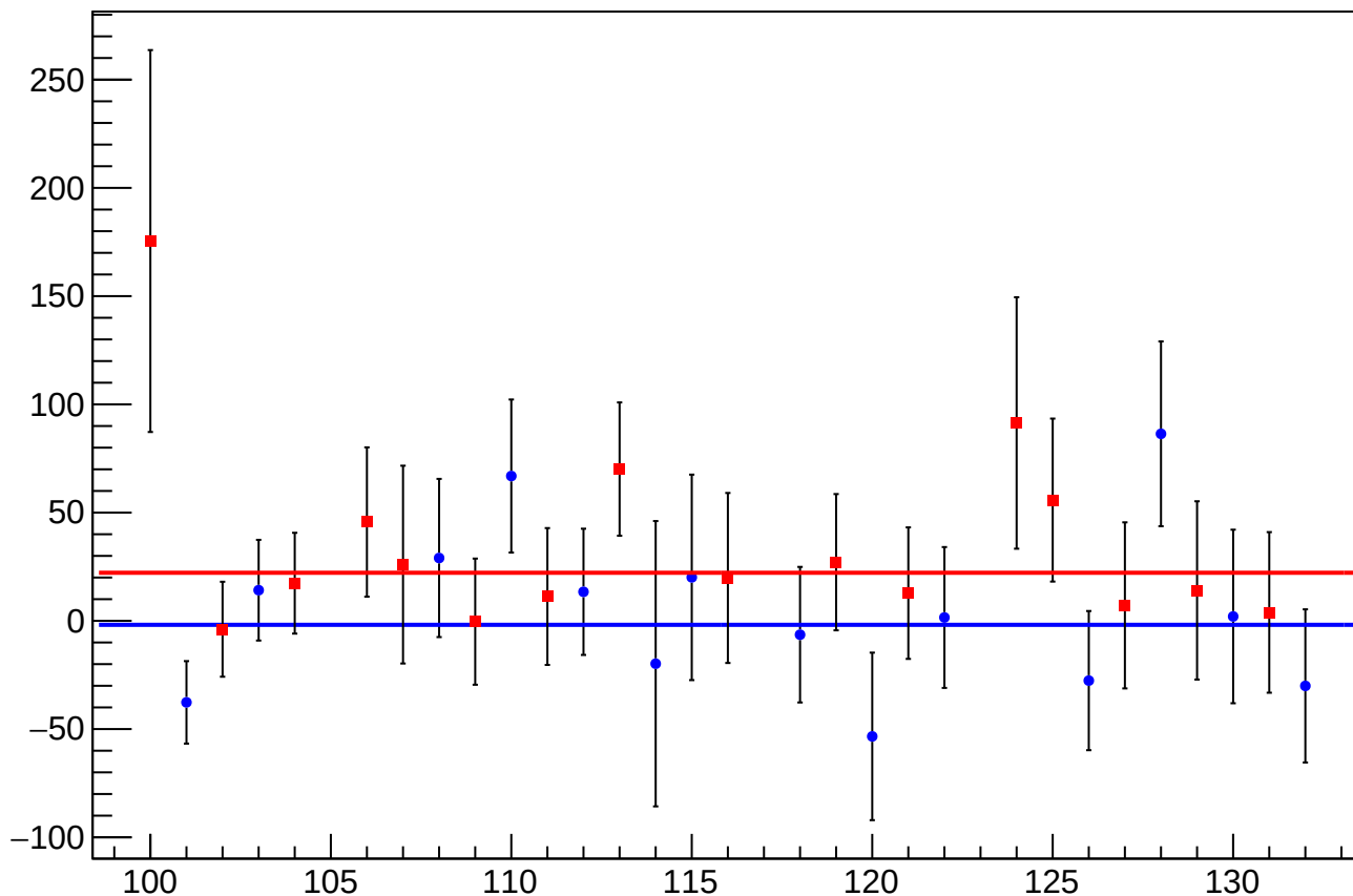
diff_bpmtargetsumX_mean vs Slug, Sign Corrected
