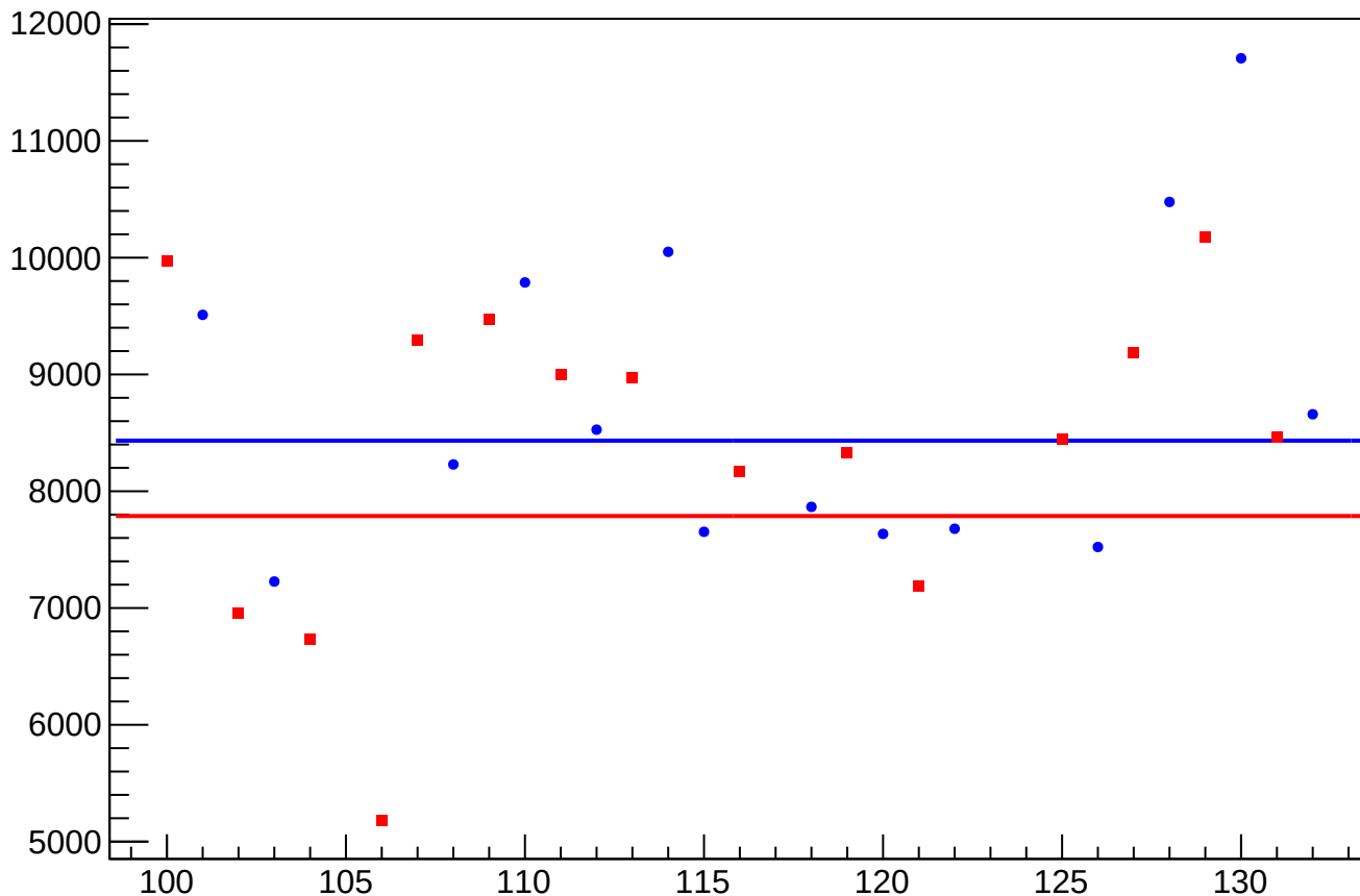
asym_us_avg_at2lr_avg_avg_eigen_dit_correction_rms vs Slug, Sign Corrected
