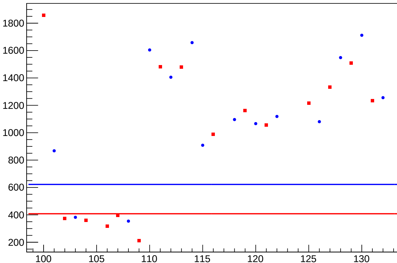
asym_us_dd_at2lr_dd_dd_dit_correction_rms vs Slug, Sign Corrected
