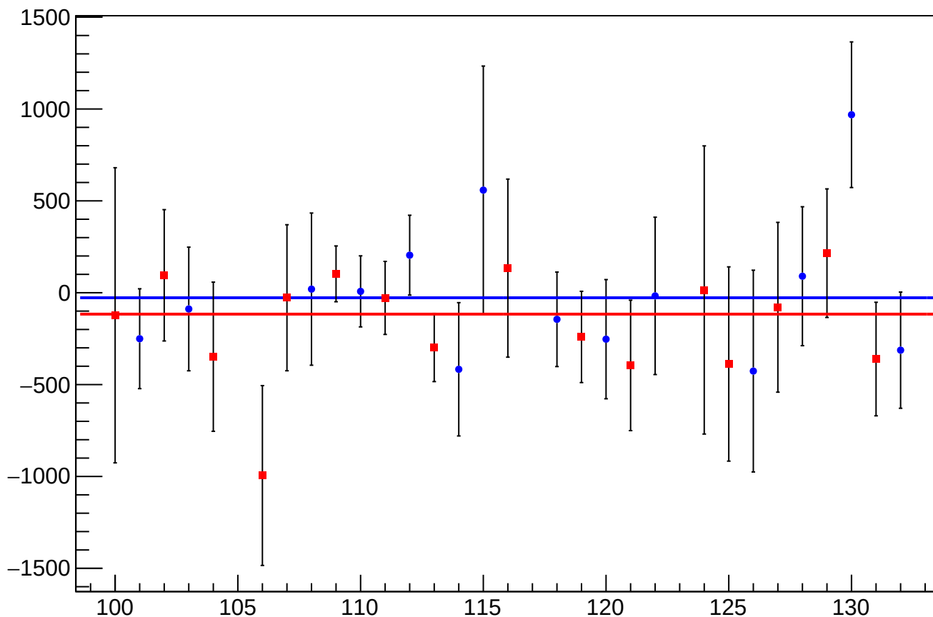
asym_bcm_dg_ds_bcm_an_ds_agg_avg_mean vs Slug, Sign Corrected
