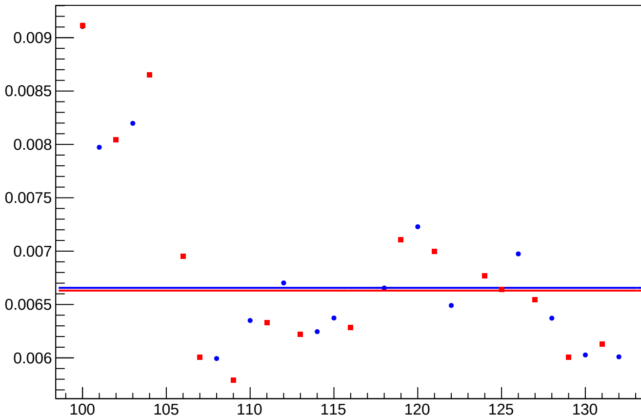
yield_bpm1i04X_rms vs Slug, Sign Corrected
