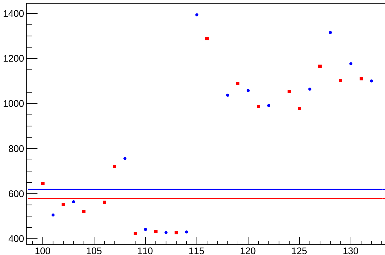
asym_sam_1548_avg_reg_correction_rms vs Slug, Sign Corrected
