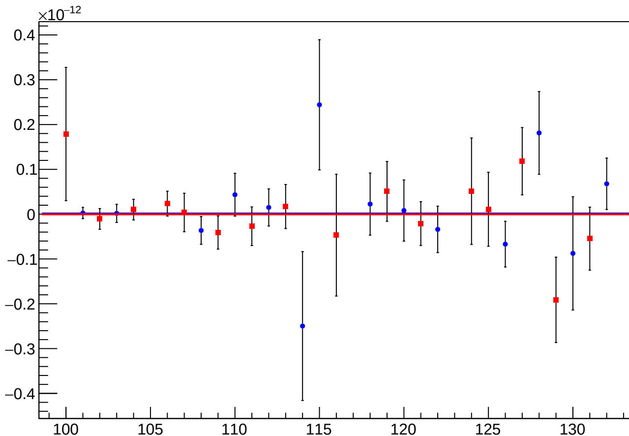
asym_sam6_eigen_cor_vs_cor_diff_mean vs Slug, Sign Corrected
