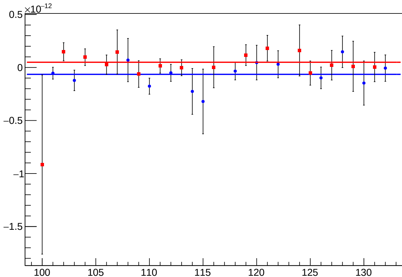
asym_sam_48_dd_reg_vs_cor_diff_mean vs Slug, Sign Corrected
