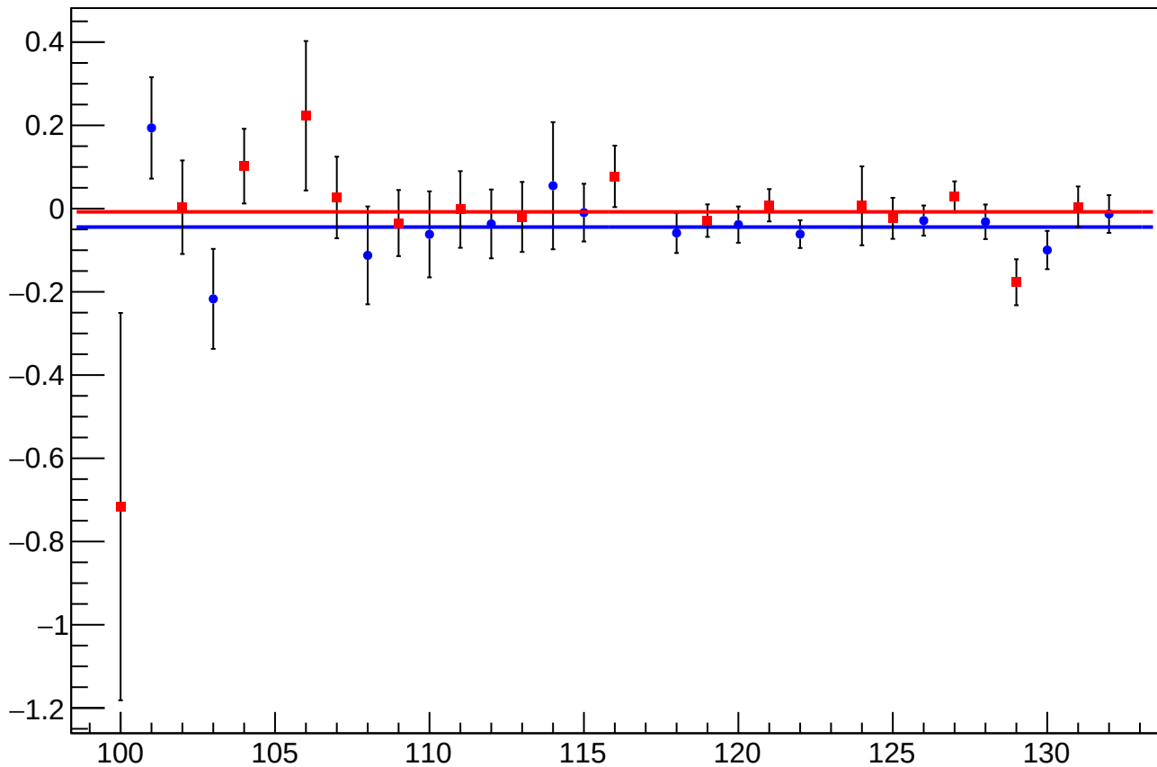
asym_sam_26_48_dd_eigen_dit_vs_cor_diff_mean vs Slug, Sign Corrected
