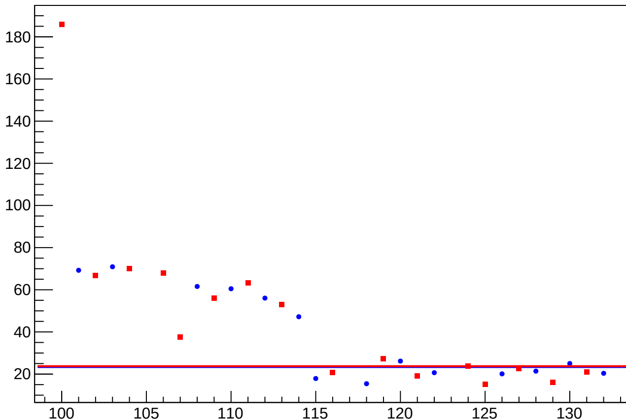
asym_sam_37_26_dd_dit_vs_slug, Sign Corrected
