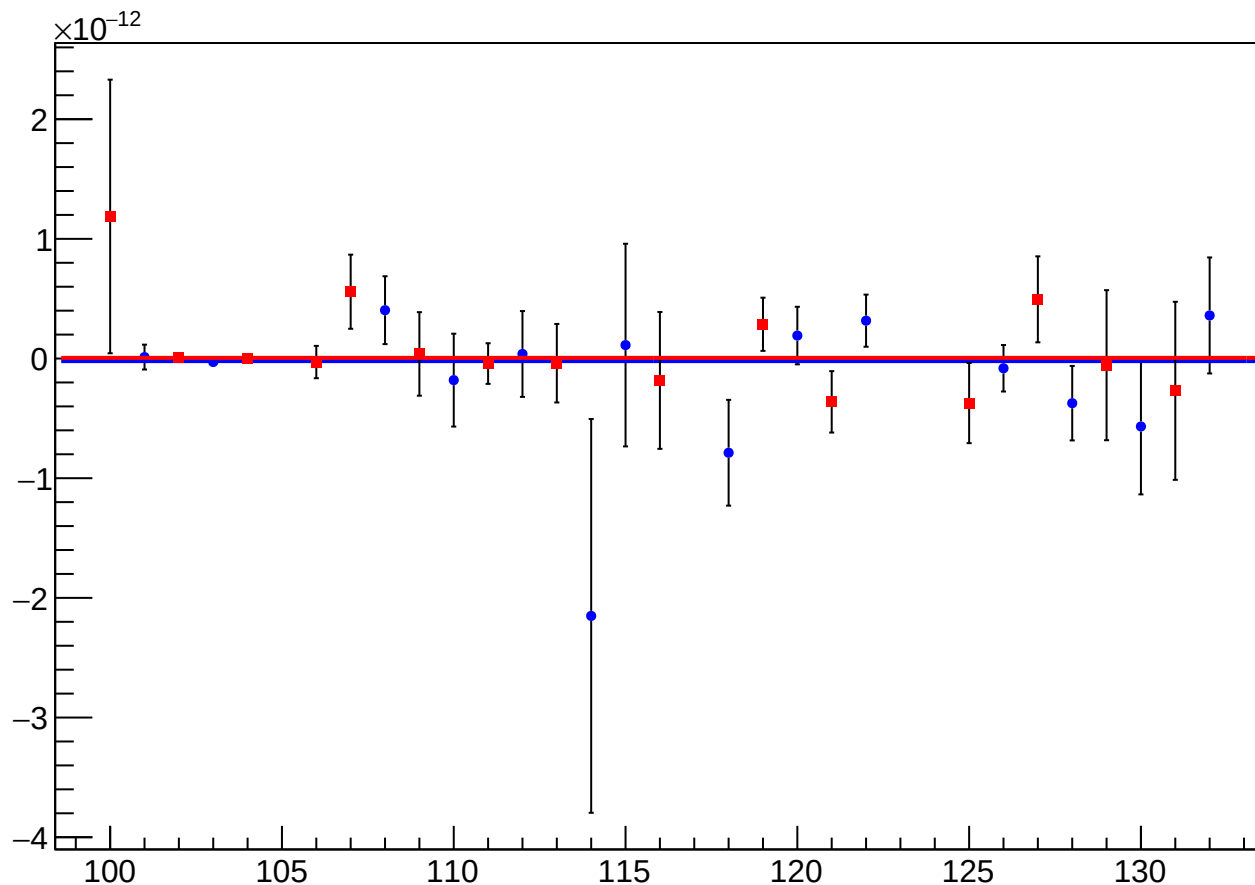
asym_us_avg_atlr_avg_dd_reg_vs_Slug, Sign Corrected
