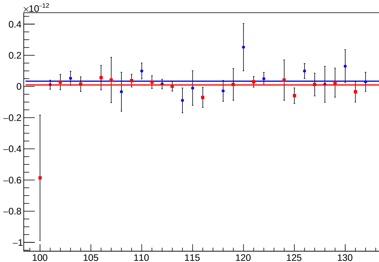
asym_sam_37_avg_eigen_cor_vs_cor_diff_mean vs Slug, Sign Corrected
