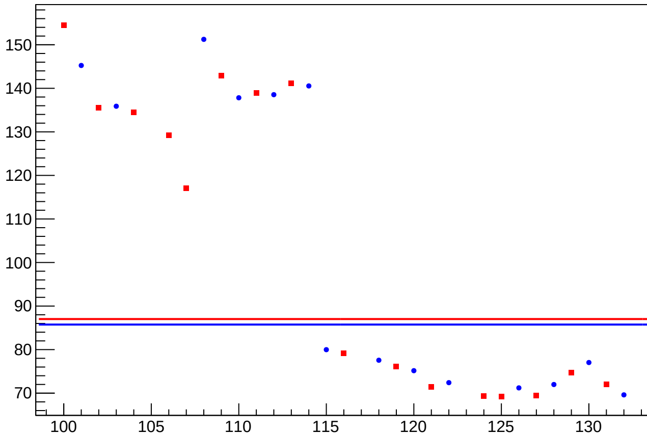
eigen_dit_asym_sam1_rms vs Slug, Sign Corrected
