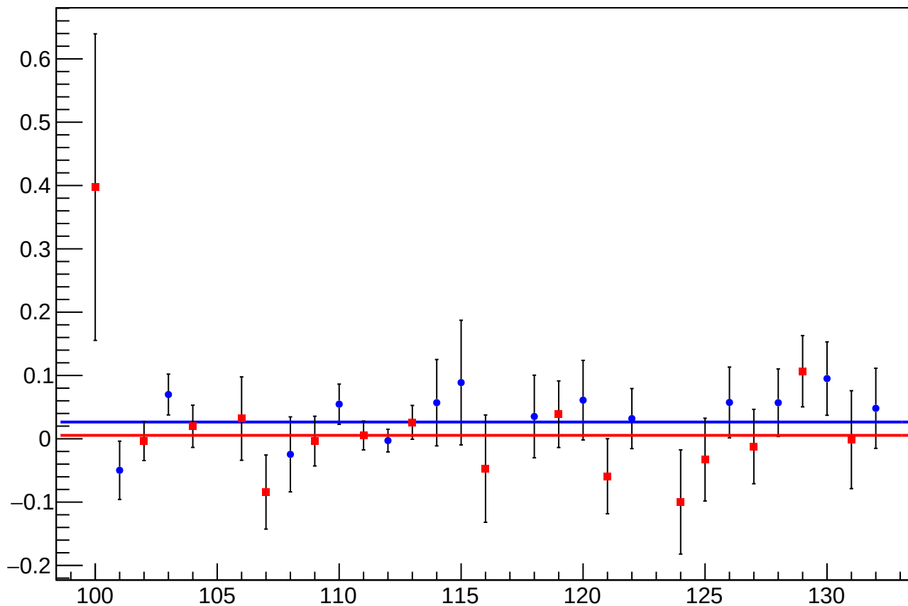
asym_sam_1548_avg_eigen_dit_vs_slug, Sign Corrected
