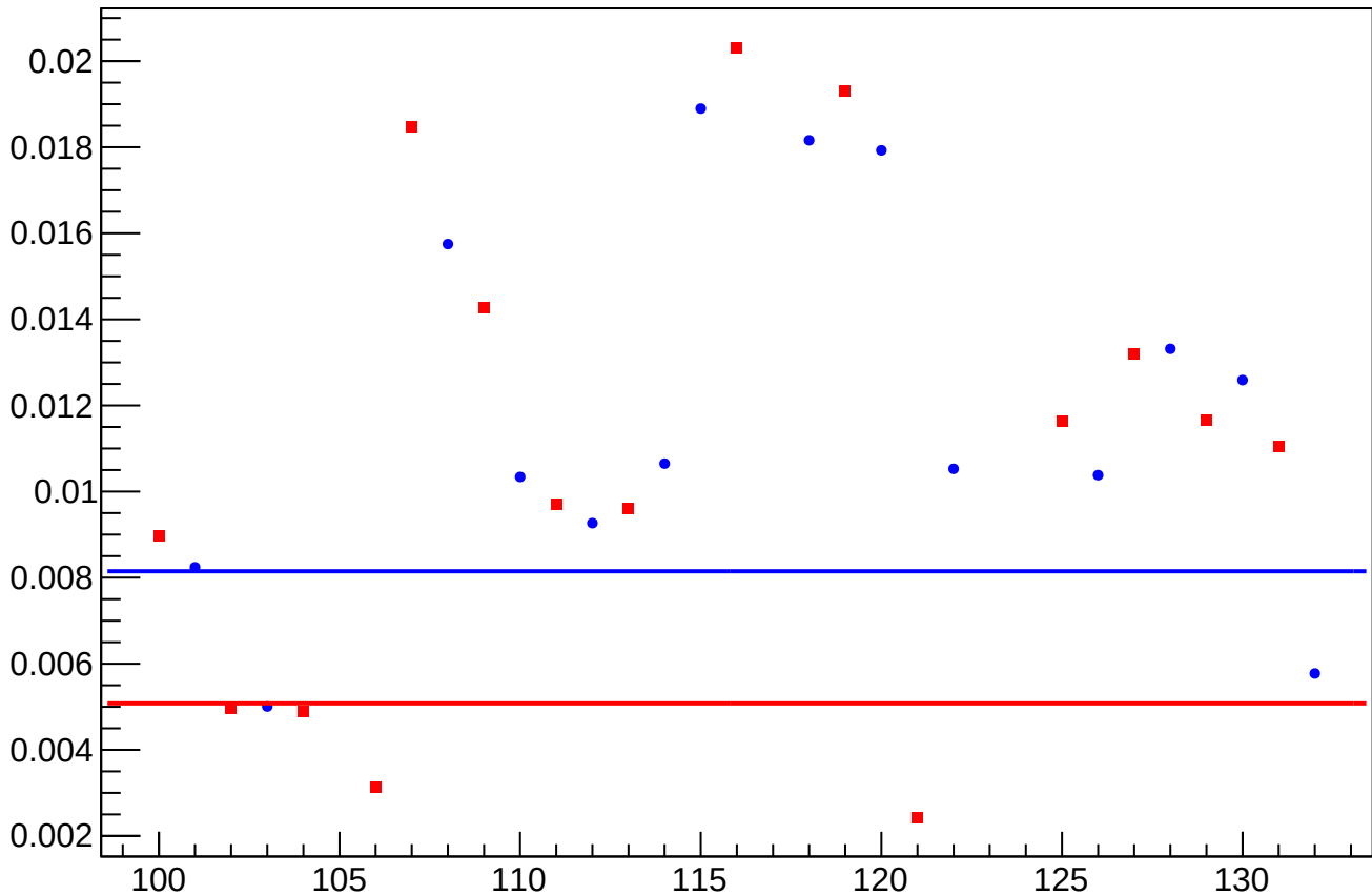
asym_usl_atl2_avg_eigen_dit_vs_dit_diff_rms vs Slug, Sign Corrected
