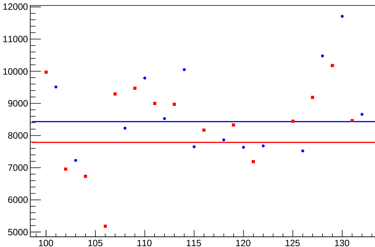
asym_us_avg_at2lr_avg_avg_dit_correction_rms vs Slug, Sign Corrected
