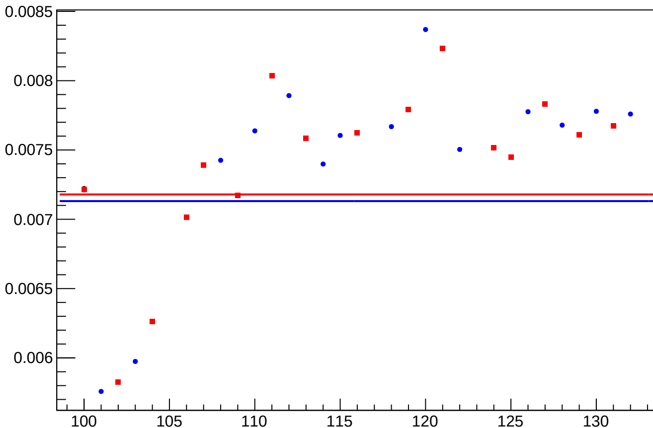
yield_bpm1i02Y_rms vs Slug, Sign Corrected
