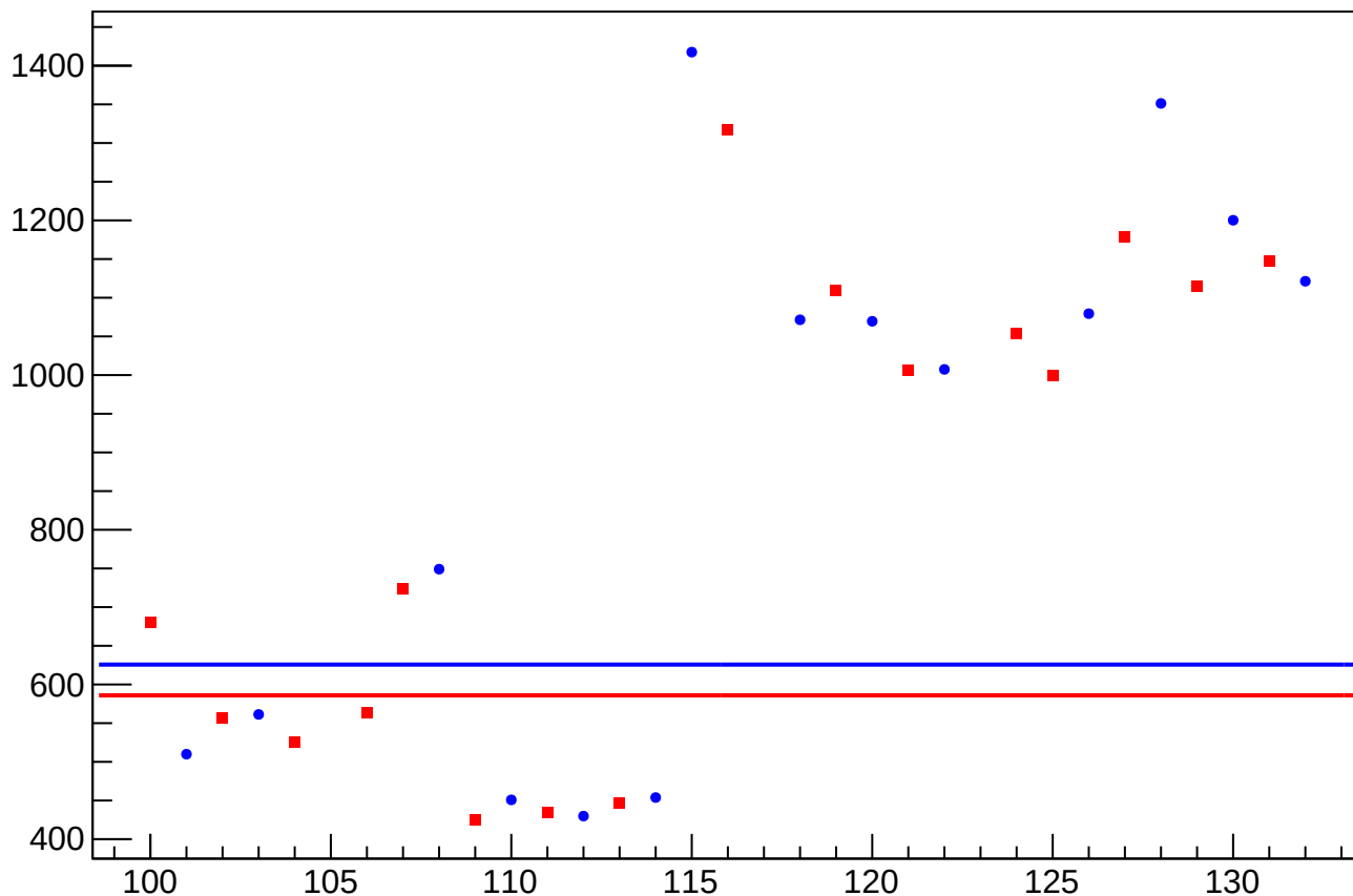
asym_sam_1548_avg_dit_correction_rms vs Slug, Sign Corrected
