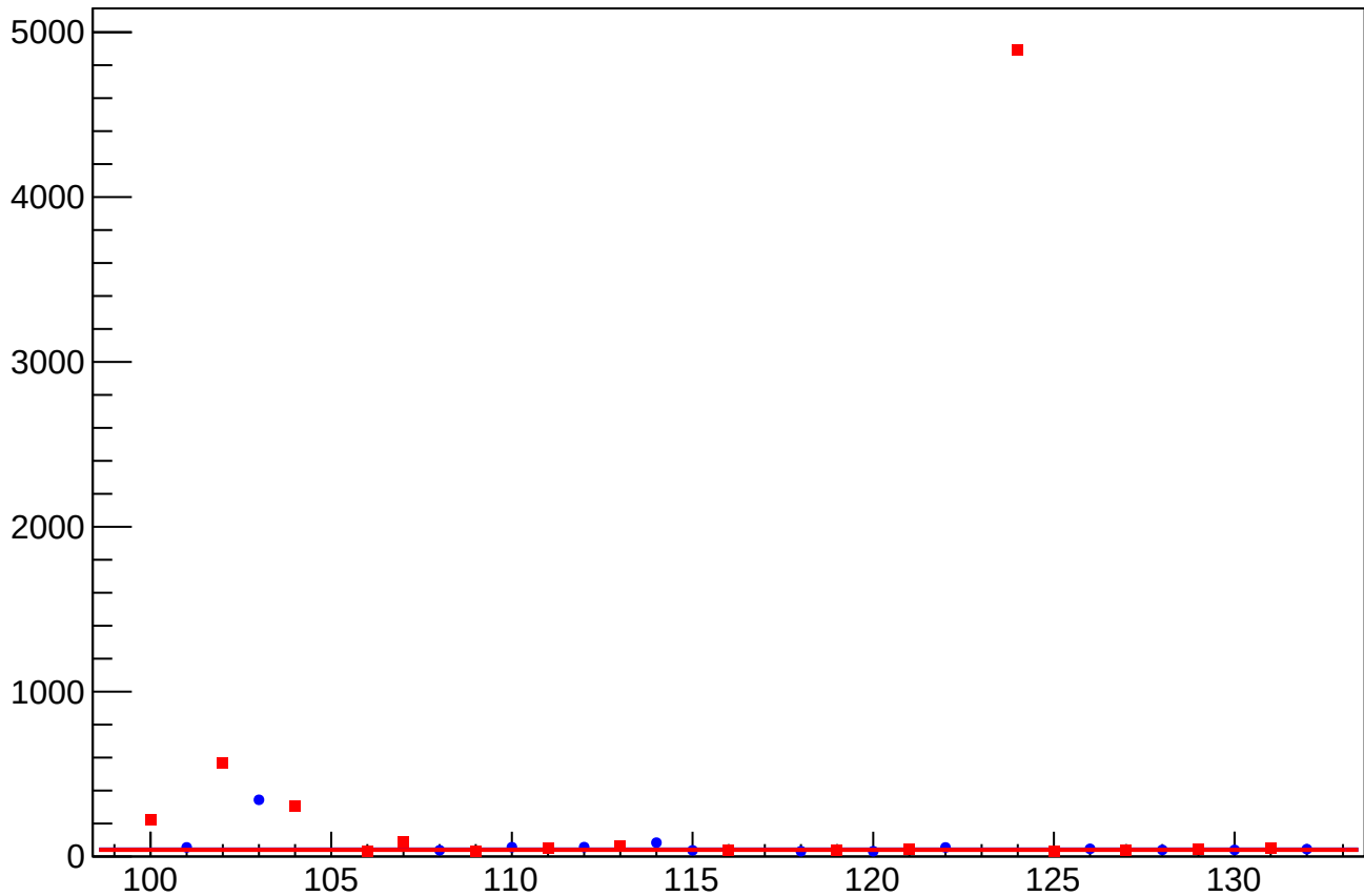
asym_atl_dd_atr_dd_dd_eigen_dit_vs_eigen_cor_diff_rms vs Slug, Sign Corrected
