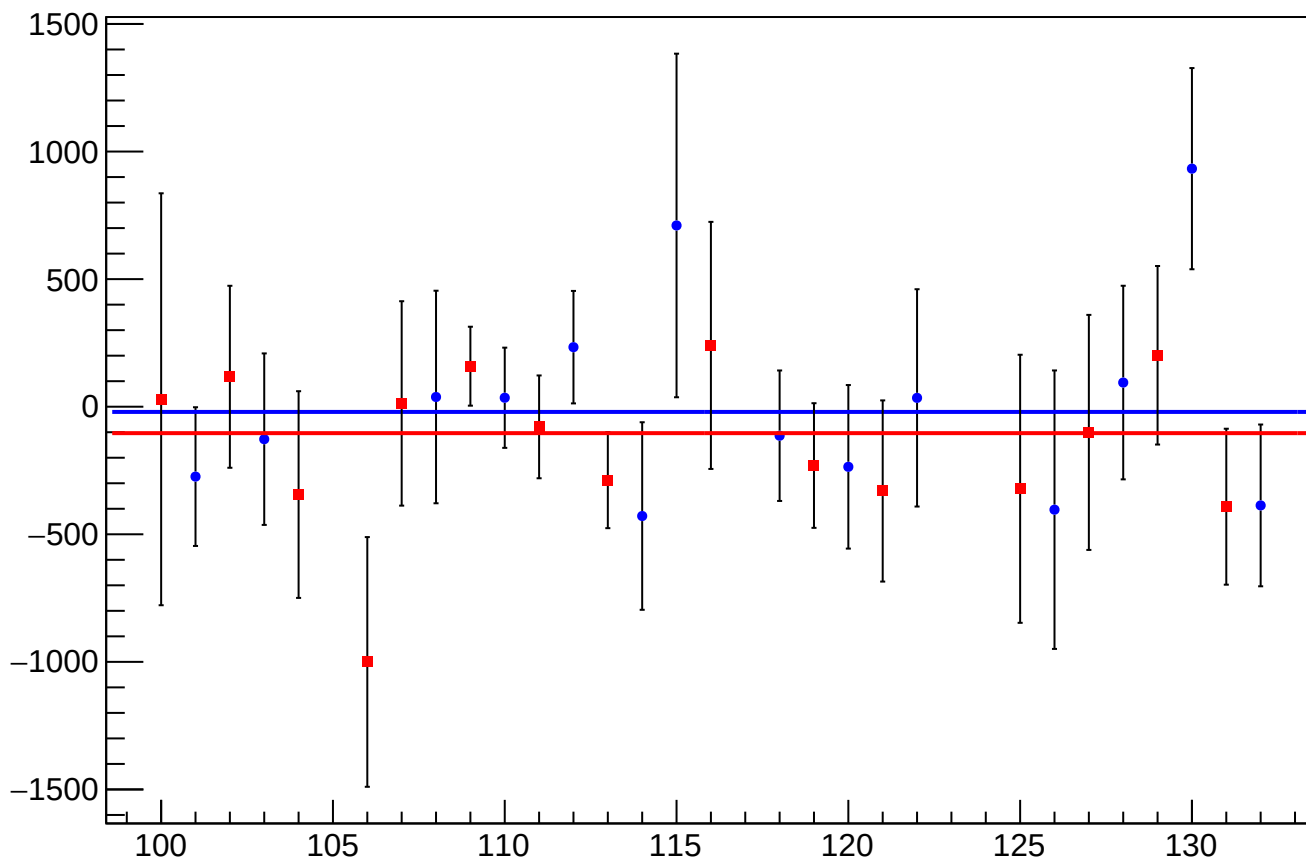
asym_bcm_dg_us_an_ds_avg_mean vs Slug, Sign Corrected
