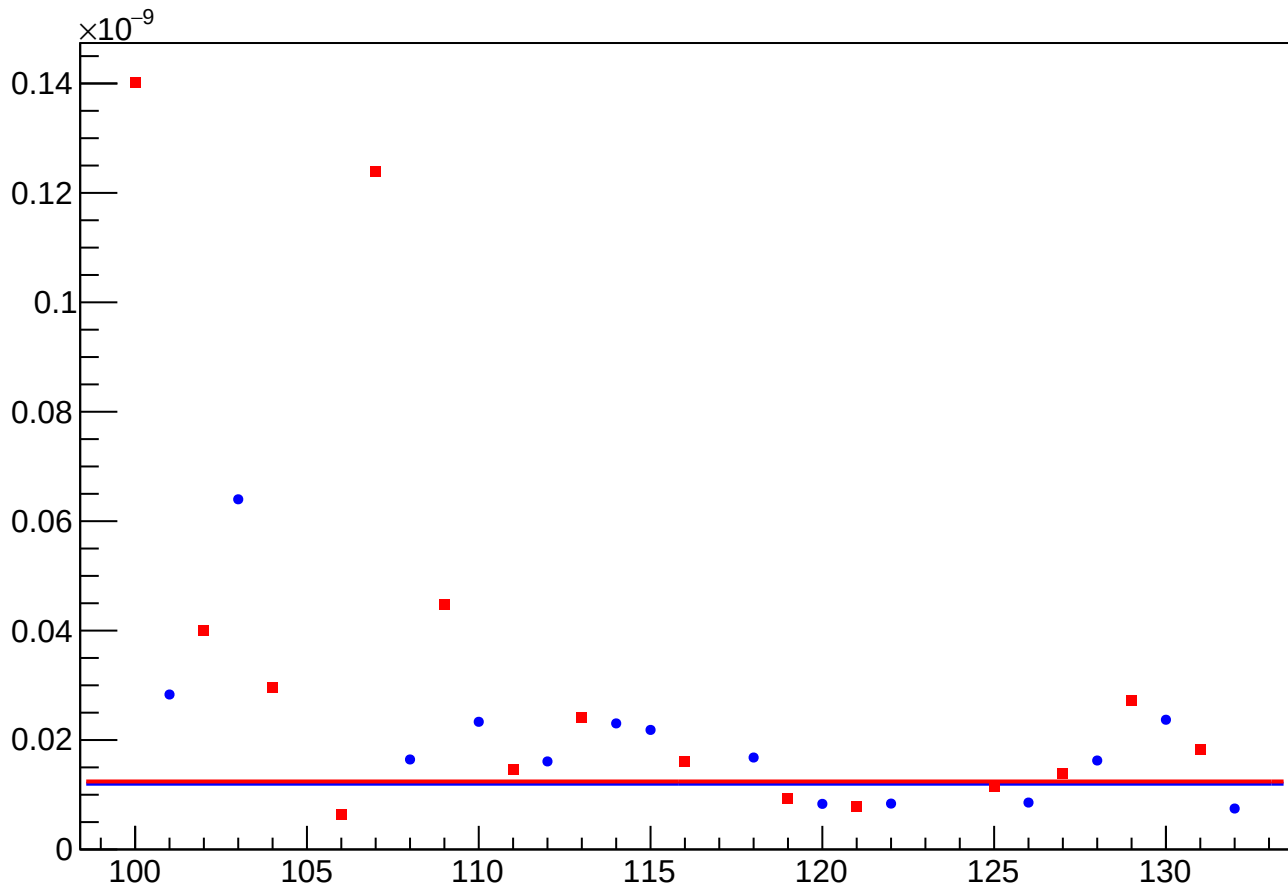
asym_us_dd_at1lr_dd_avg_eigen_cor_vs_cor_diff_rms vs Slug, Sign Corrected
