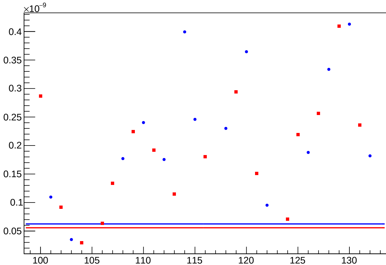
asym_atl_avg_atr_avg_avg_reg_vs_cor_diff_rms vs Slug, Sign Corrected
