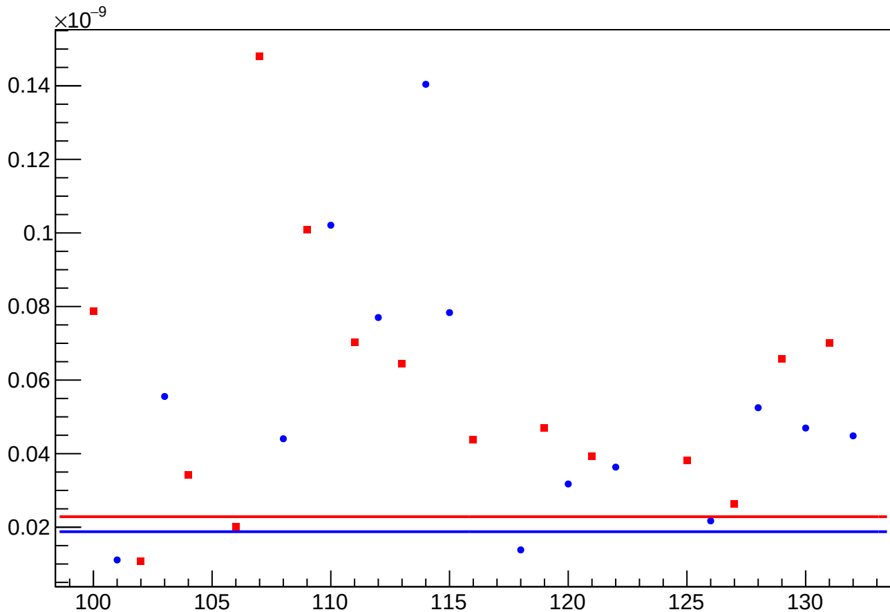
asym_usl_atl1_avg_reg_vs_cor_diff_rms vs Slug, Sign Corrected
