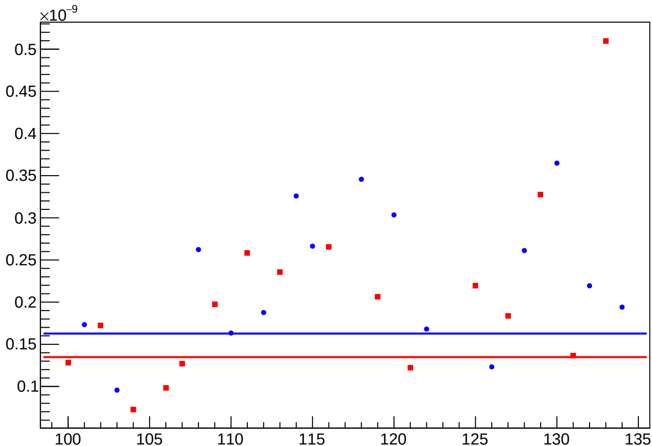
asym_us_avg_at2lr_avg_dd_eigen_cor_vs_cor_diff_rms vs Slug, Sign Corrected
