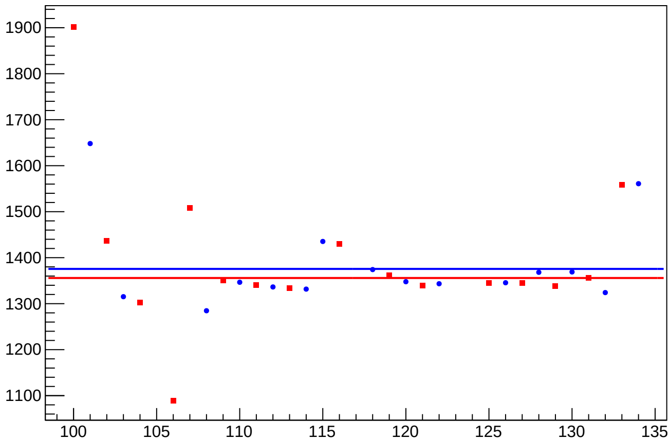
cor_asym_usl_atl2_avg_rms vs Slug, Sign Corrected
