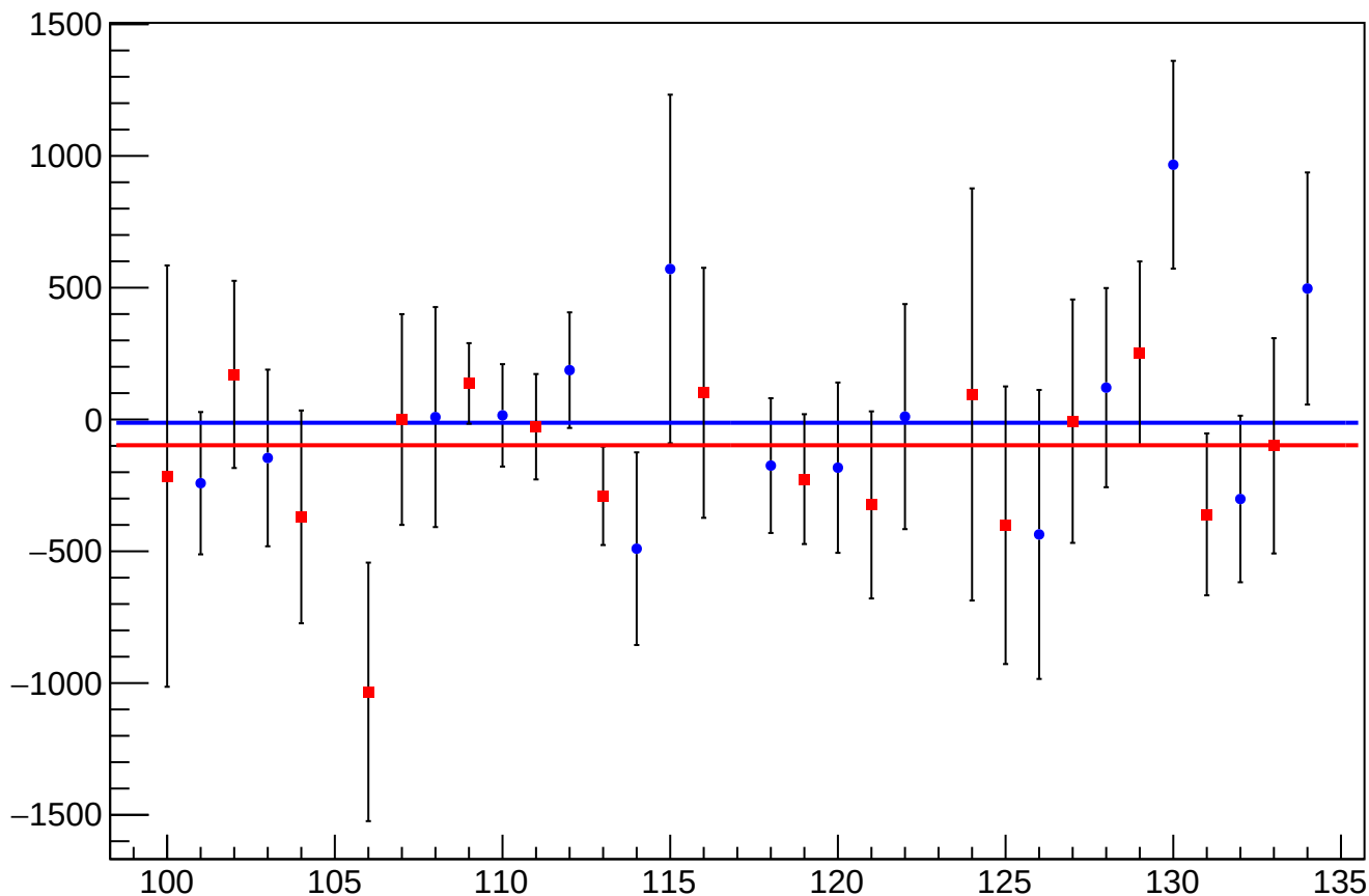
asym_bcm_target_mean vs Slug, Sign Corrected
