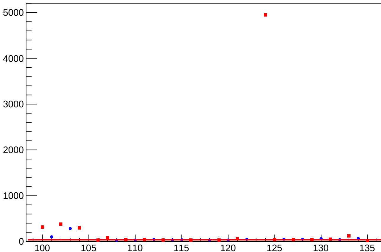
asym atl avg atr avg dd dit vs cor diff rms vs Slug
