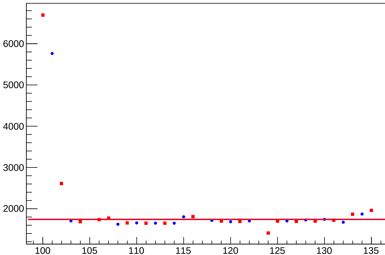
dit_asym_atr1l2_dd_rms vs Slug
