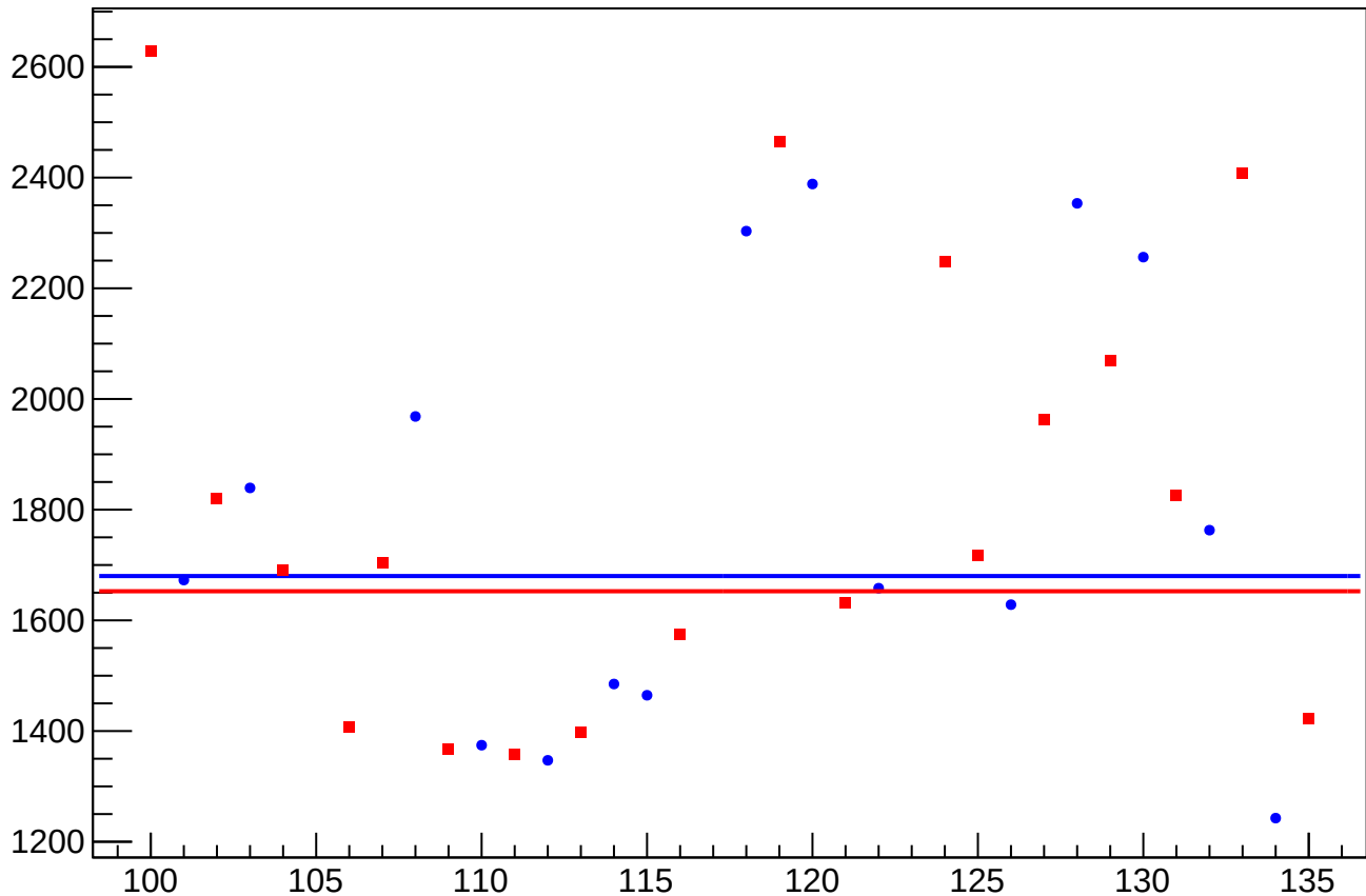
asym_sam3_eigen_cor_correction_rms vs Slug
