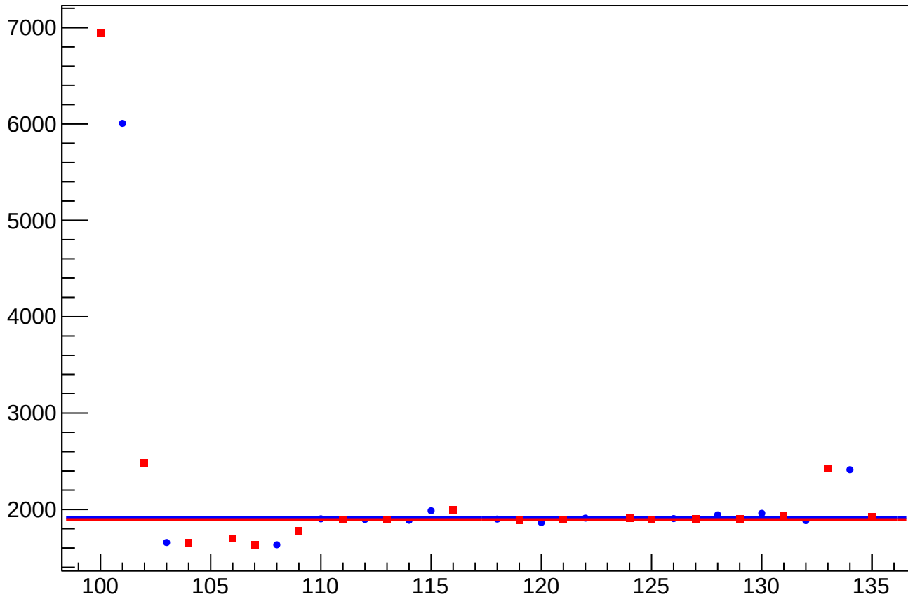
eigen_dit_asym_atr_dd_rms vs Slug
