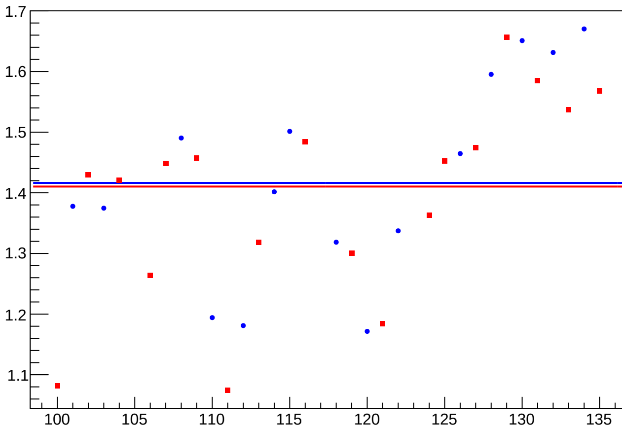
yield_bpm1i02Y_mean vs Slug
