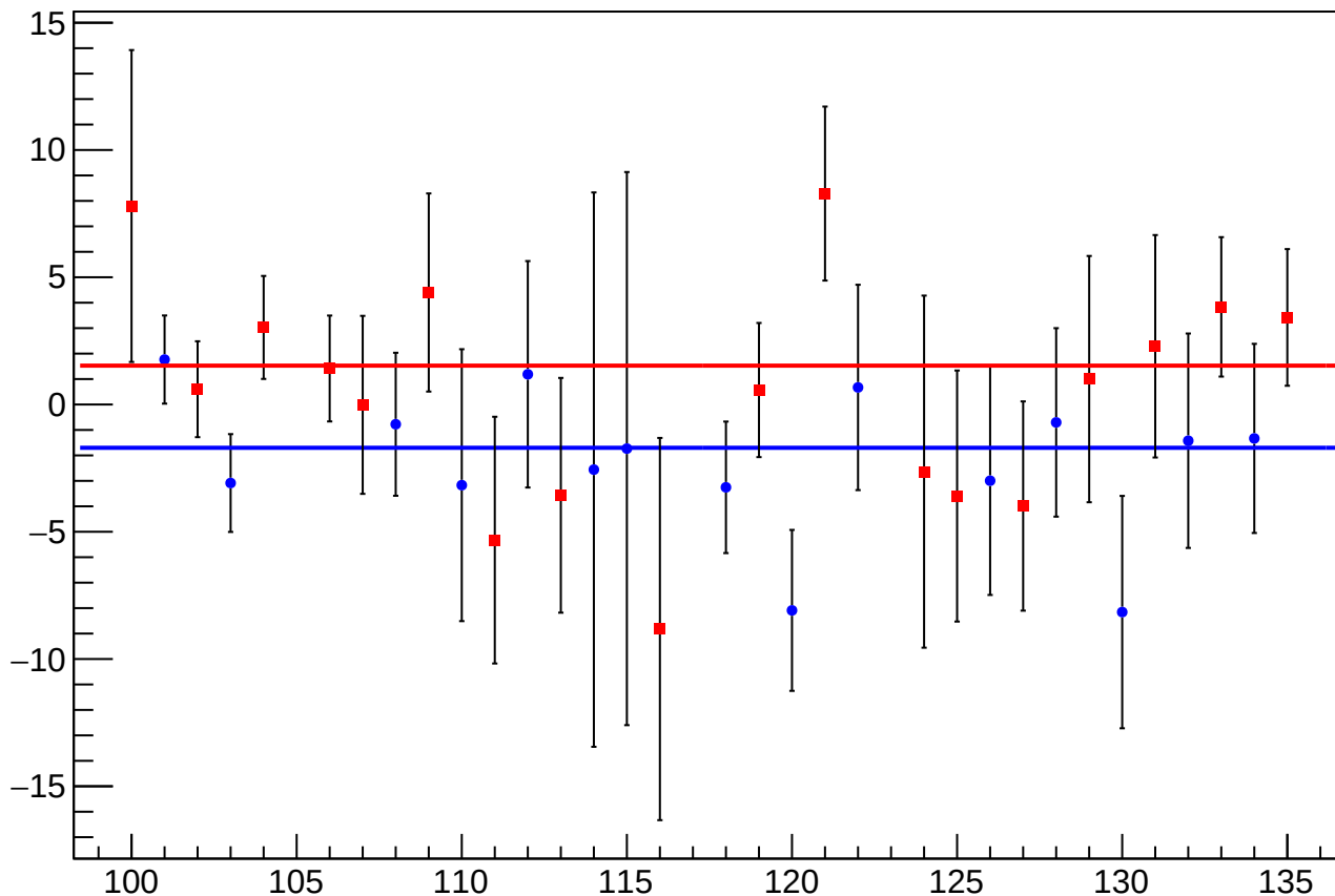
diff_bpm4aeddifffY_mean vs Slug
